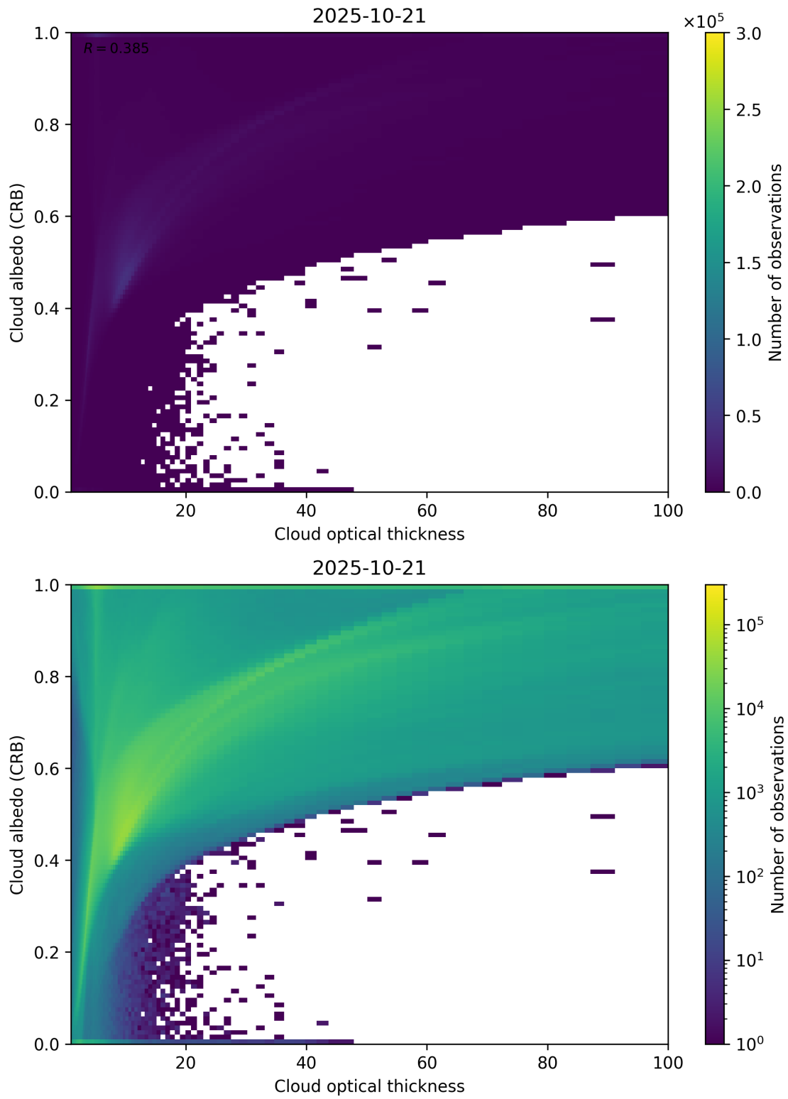
Figure 82: Scatter density plot of “Cloud optical thickness” against “Cloud albedo (CRB)” for 2025-10-20 to 2025-10-22.
