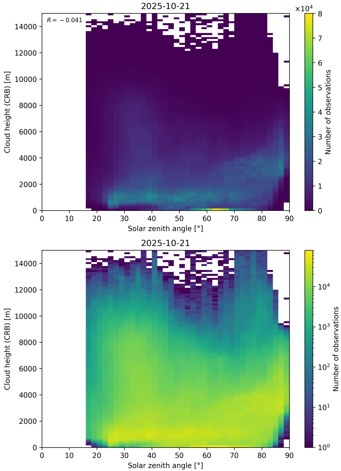
Figure 102: Scatter density plot of “Solar zenith angle” against “Cloud height (CRB)” for 2025-10-20 to 2025-10-22.
