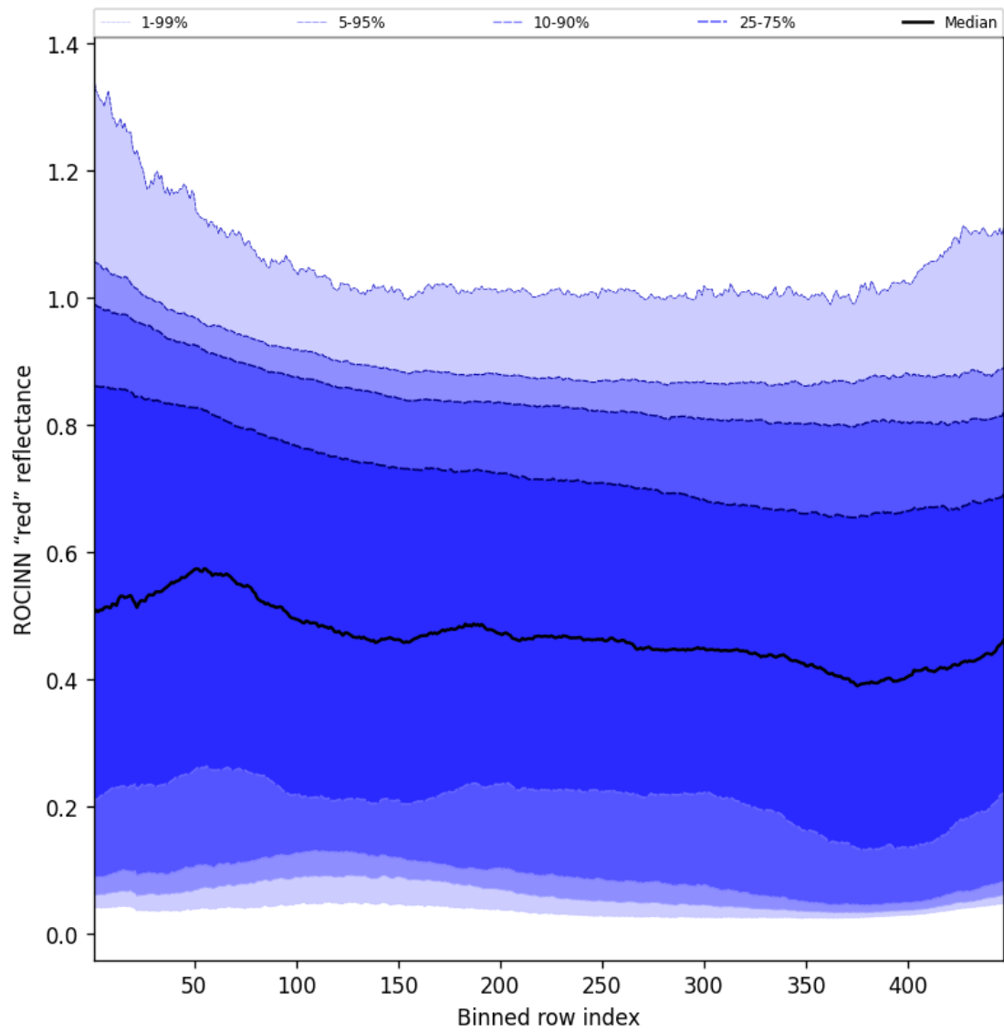
Figure 69: Along track statistics of "ROCINN "red" reflectance" for 2025-10-20 to 2025-10-22
