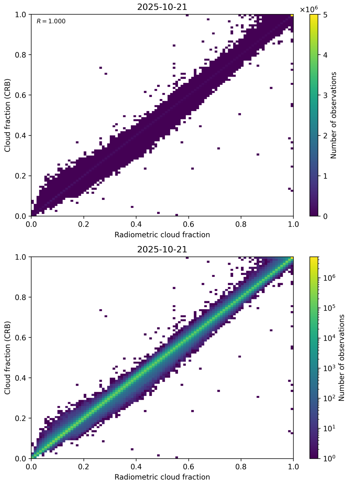
Figure 73: Scatter density plot of “Radiometric cloud fraction” against “Cloud fraction (CRB)” for 2025-10-20 to 2025-10-22.
