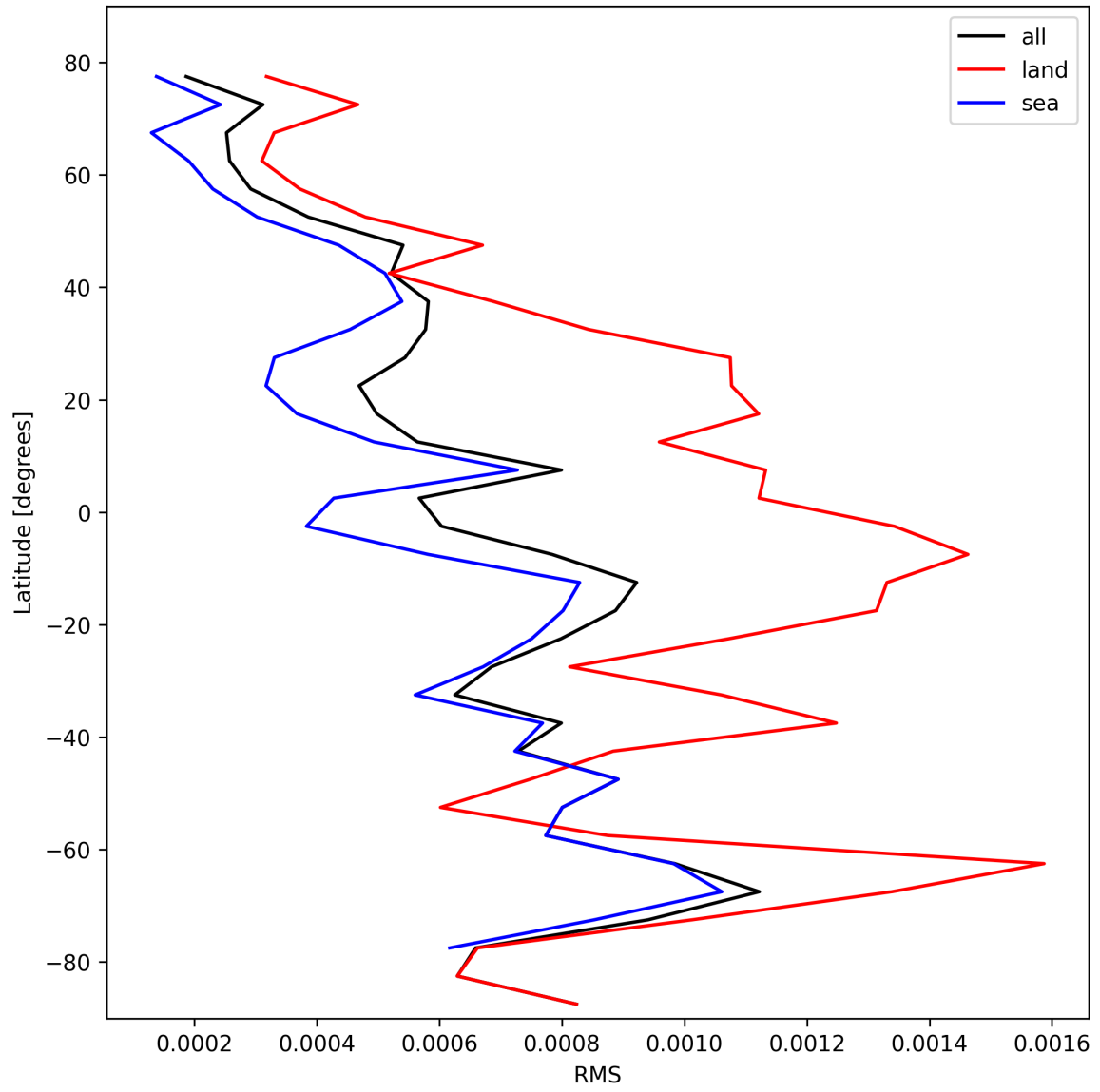
Figure 31: Zonal average of “RMS” for 2025-10-20 to 2025-10-22.
