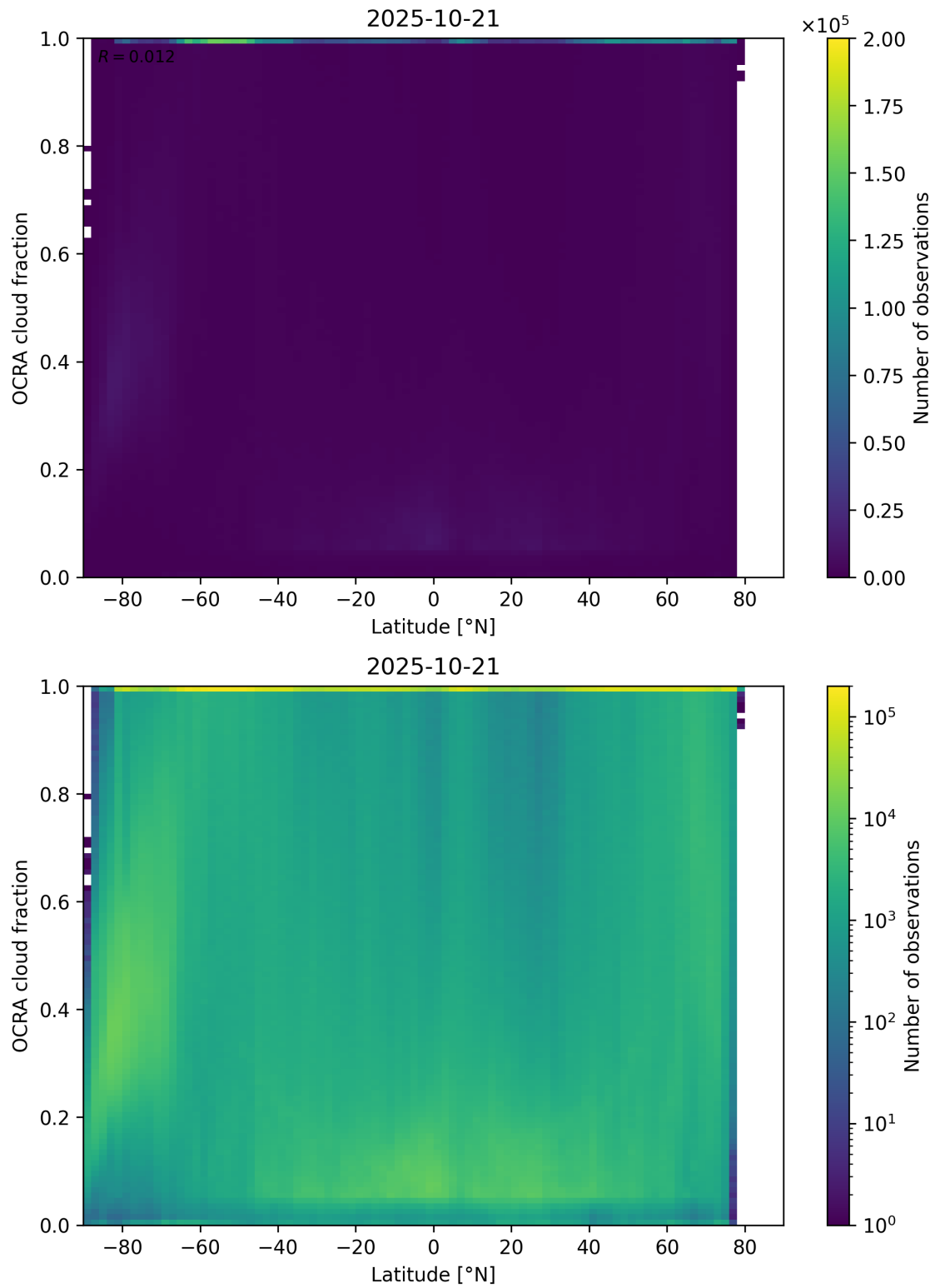
Figure 93: Scatter density plot of “Latitude” against “OCRA cloud fraction” for 2025-10-20 to 2025-10-22.
