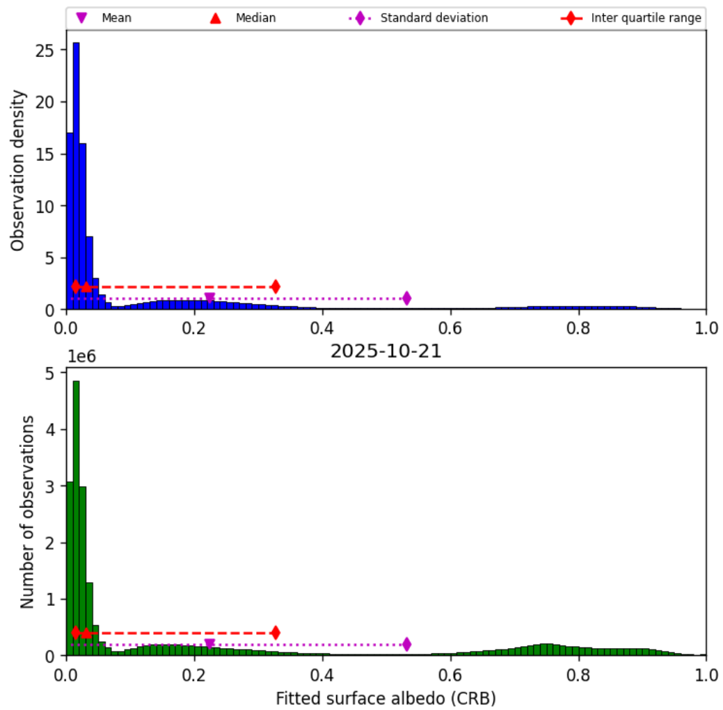
Figure 46: Histogram of “Fitted surface albedo (CRB)” for 2025-10-20 to 2025-10-22
