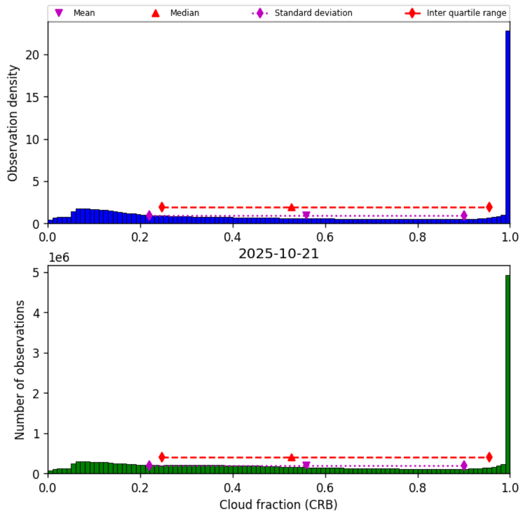
Figure 42: Histogram of “Cloud fraction (CRB)” for 2025-10-20 to 2025-10-22
