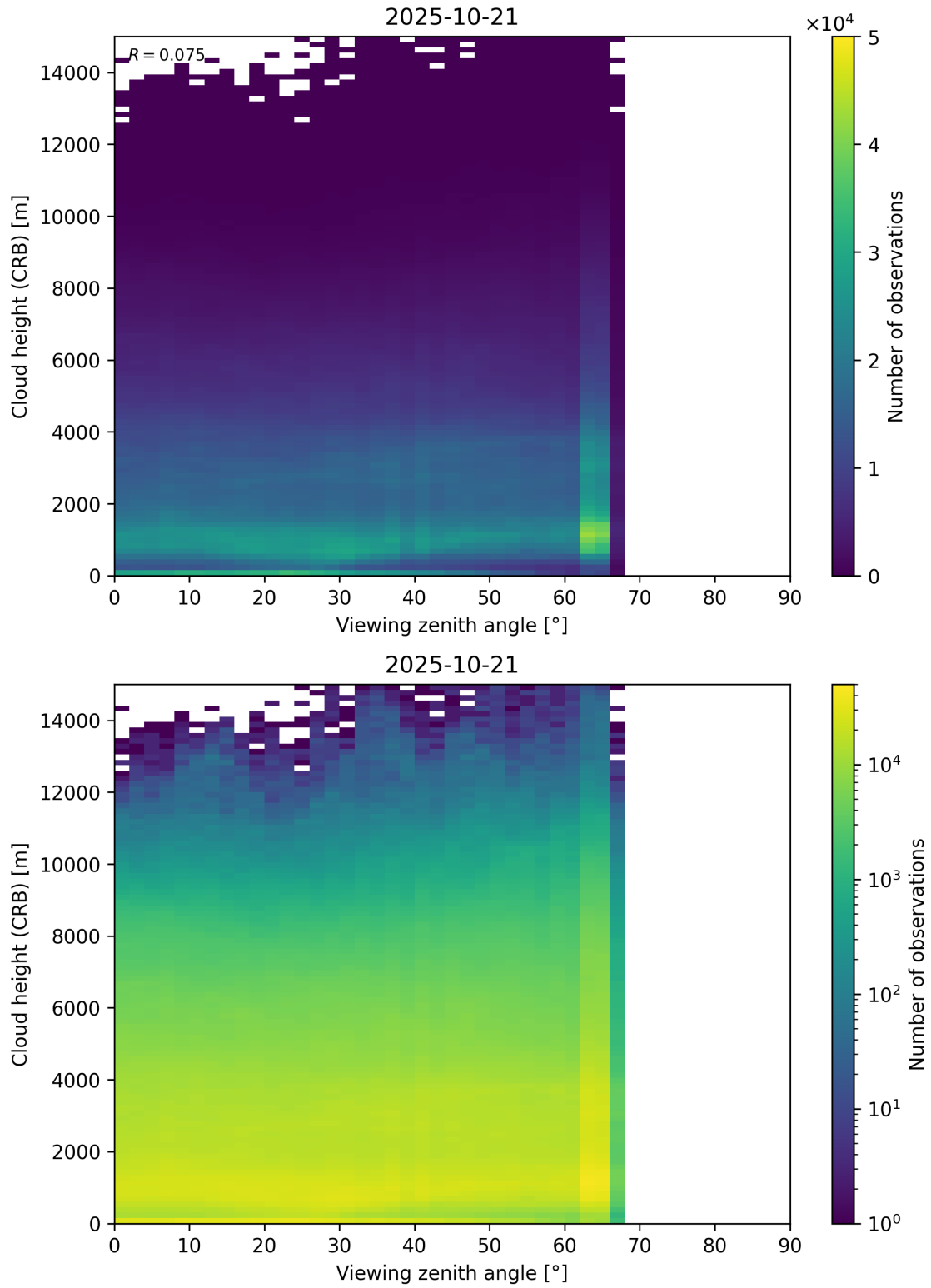
Figure 110: Scatter density plot of “Viewing zenith angle” against “Cloud height (CRB)” for 2025-10-20 to 2025-10-22.
