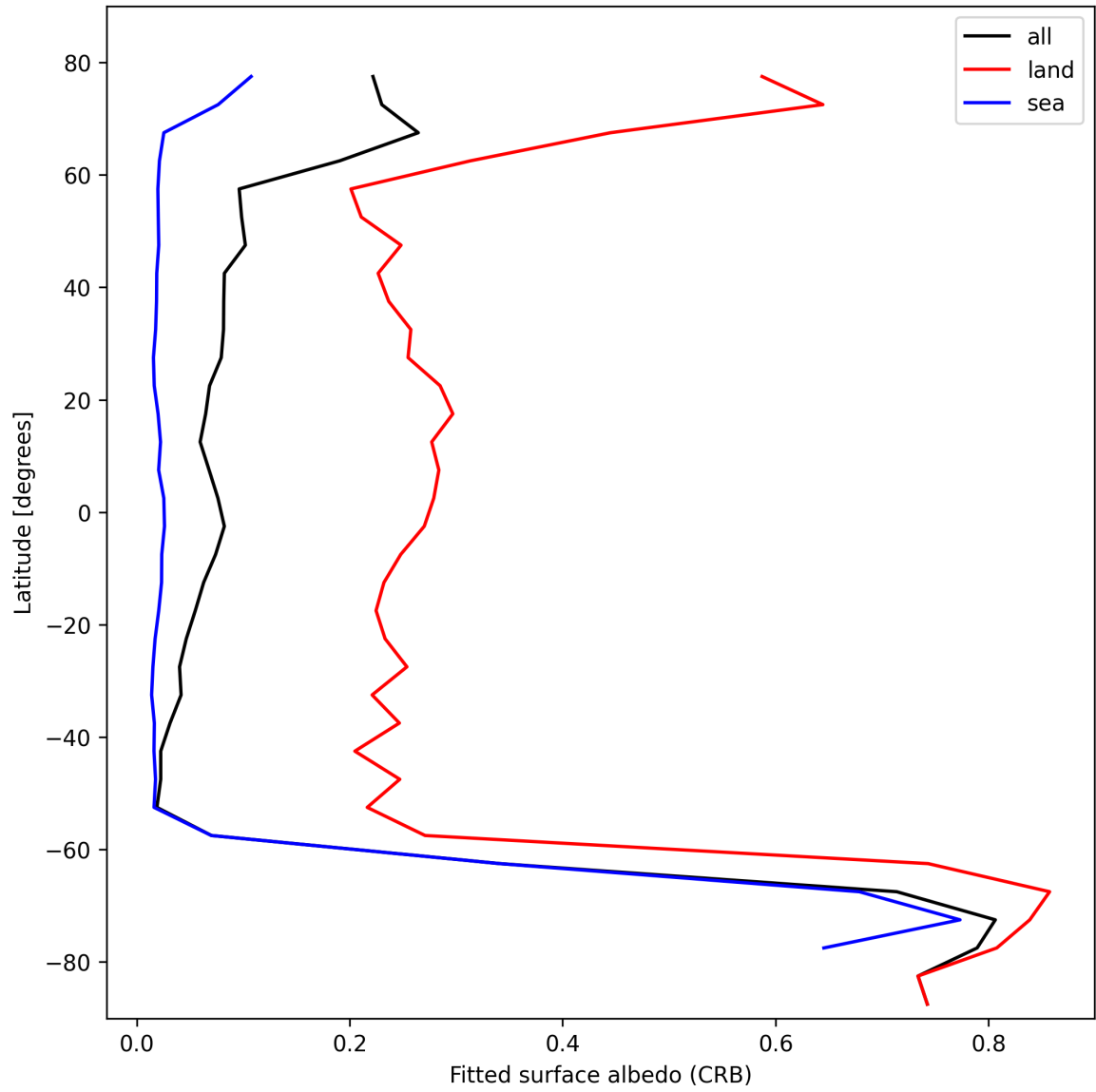
Figure 30: Zonal average of “Fitted surface albedo (CRB)” for 2025-10-20 to 2025-10-22.
