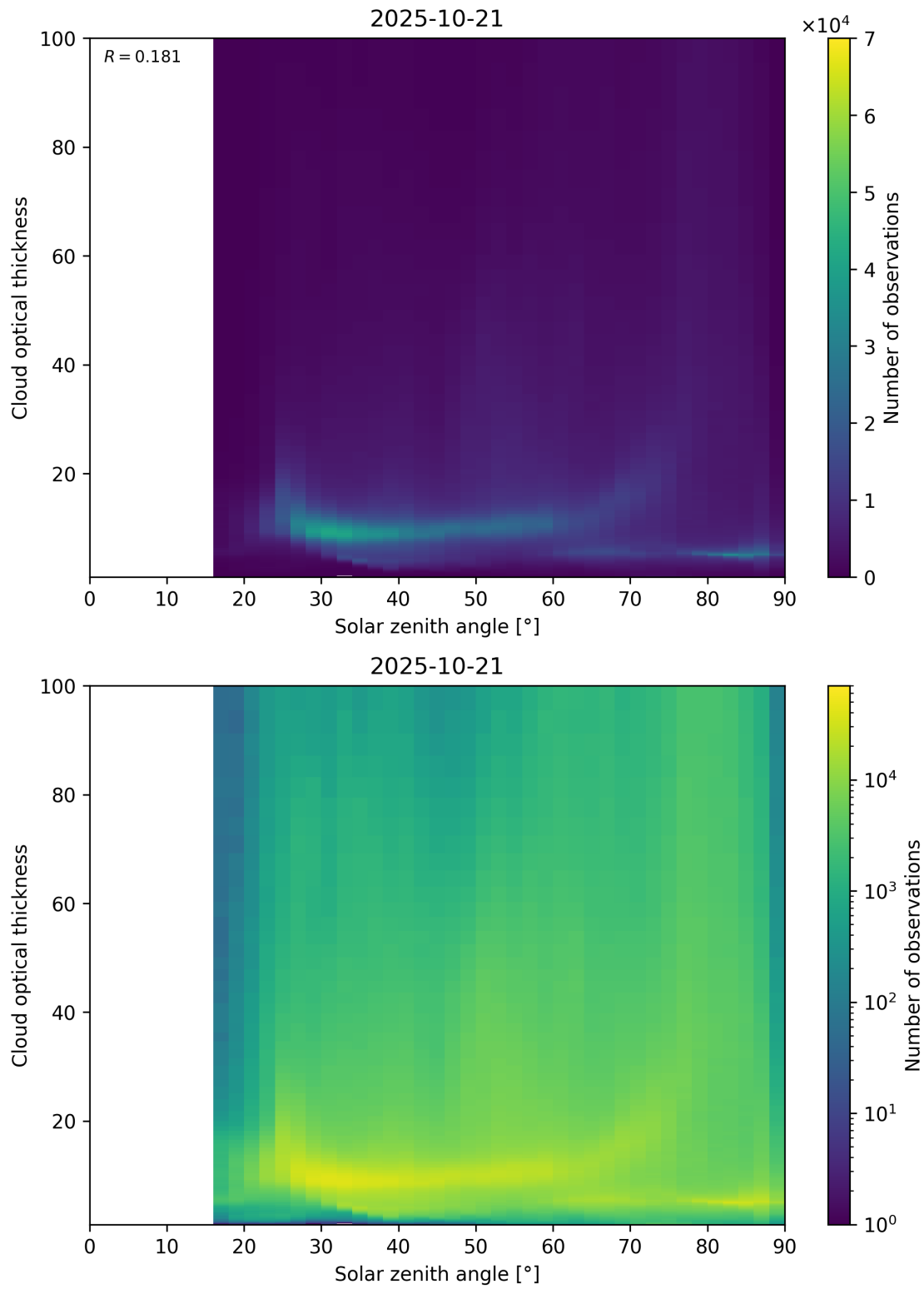
Figure 103: Scatter density plot of “Solar zenith angle” against “Cloud optical thickness” for 2025-10-20 to 2025-10-22.
