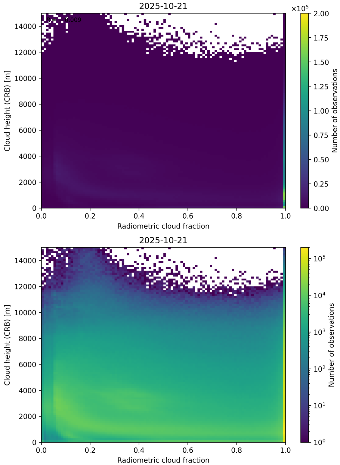
Figure 74: Scatter density plot of “Radiometric cloud fraction” against “Cloud height (CRB)” for 2025-10-20 to 2025-10-22.
