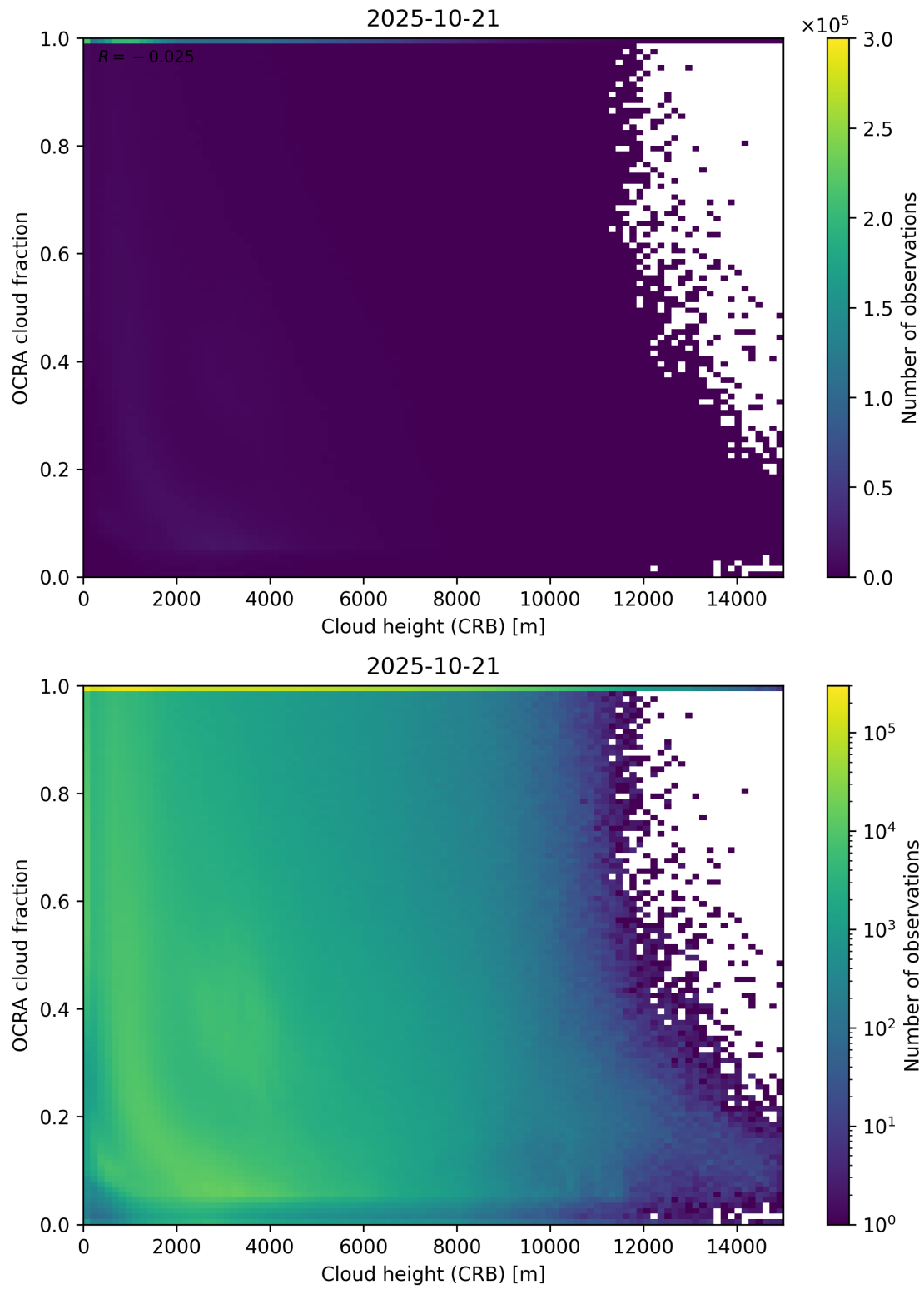
Figure 81: Scatter density plot of “Cloud height (CRB)” against “OCRA cloud fraction” for 2025-10-20 to 2025-10-22.
