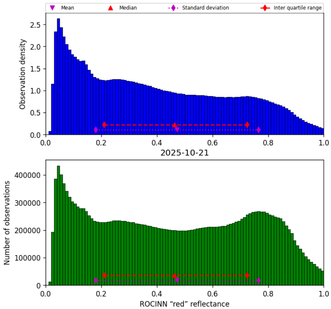
Figure 53: Histogram of “ROCINN “red” reflectance” for 2025-10-20 to 2025-10-22
