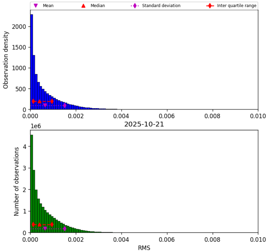
Figure 47: Histogram of “RMS” for 2025-10-20 to 2025-10-22
