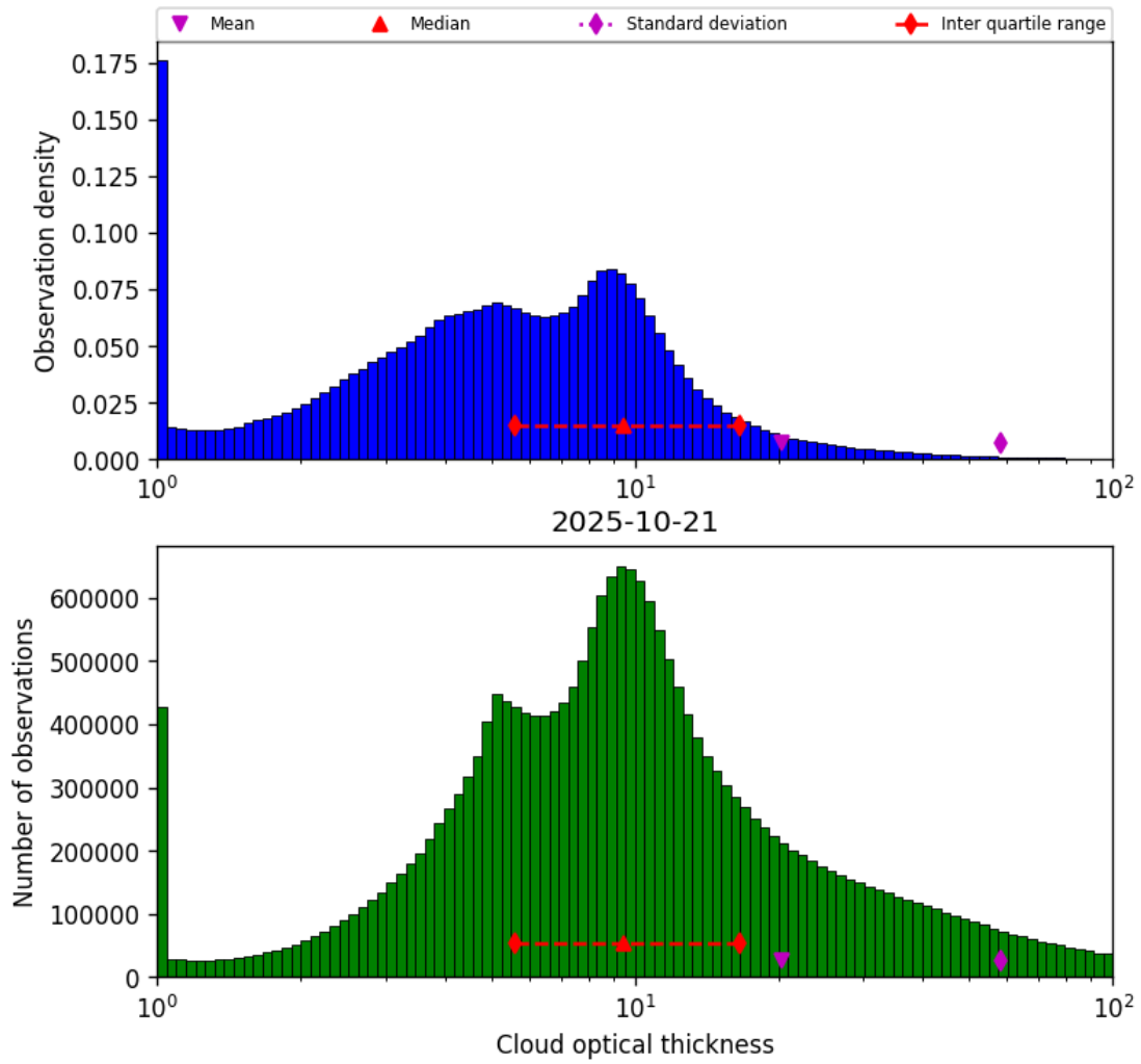
Figure 41: Histogram of “Cloud optical thickness” for 2025-10-20 to 2025-10-22
