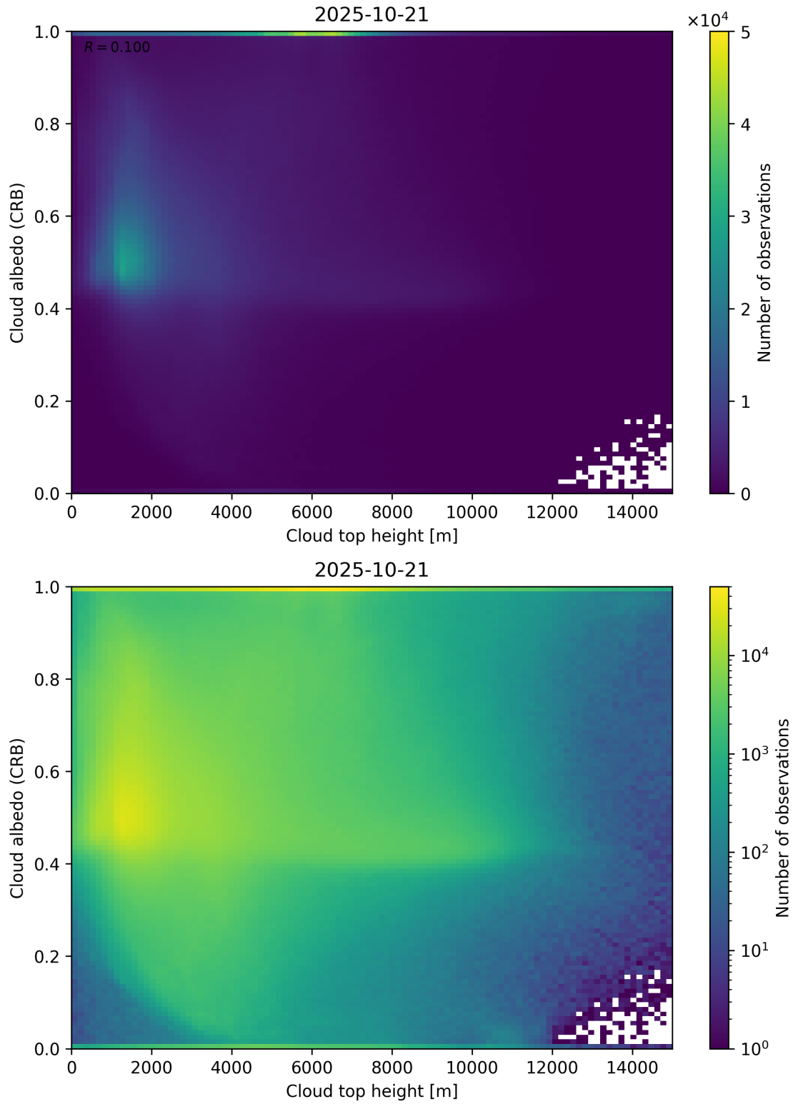
Figure 86: Scatter density plot of “Cloud top height” against “Cloud albedo (CRB)” for 2025-10-20 to 2025-10-22.
