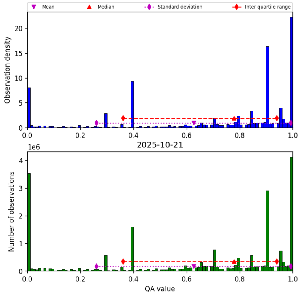
Figure 38: Histogram of “QA value” for 2025-10-20 to 2025-10-22
