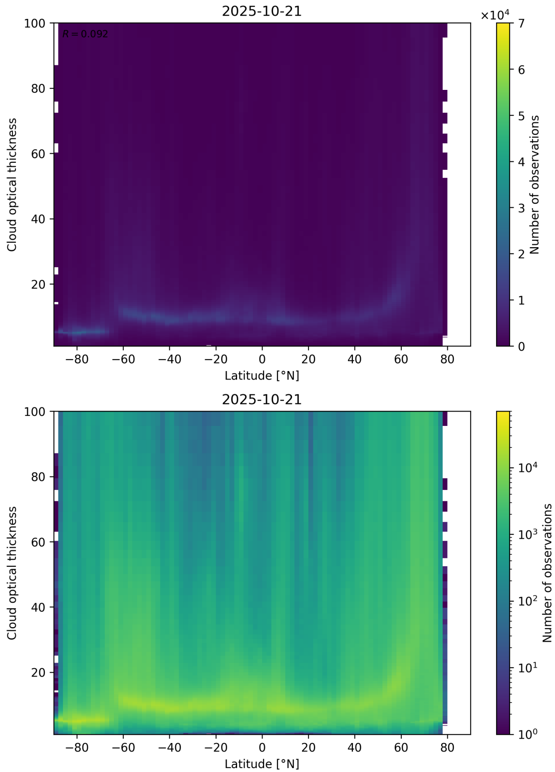
Figure 96: Scatter density plot of “Latitude” against “Cloud optical thickness” for 2025-10-20 to 2025-10-22.
