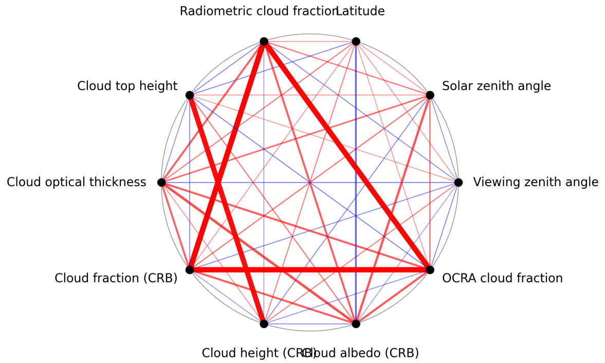
Figure 1: Map of correlation graph for 2025-10-20 to 2025-10-22.
