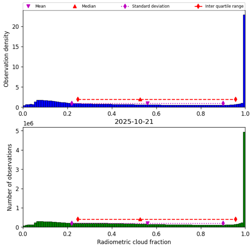
Figure 39: Histogram of "Radiometric cloud fraction" for 2025-10-20 to 2025-10-22
