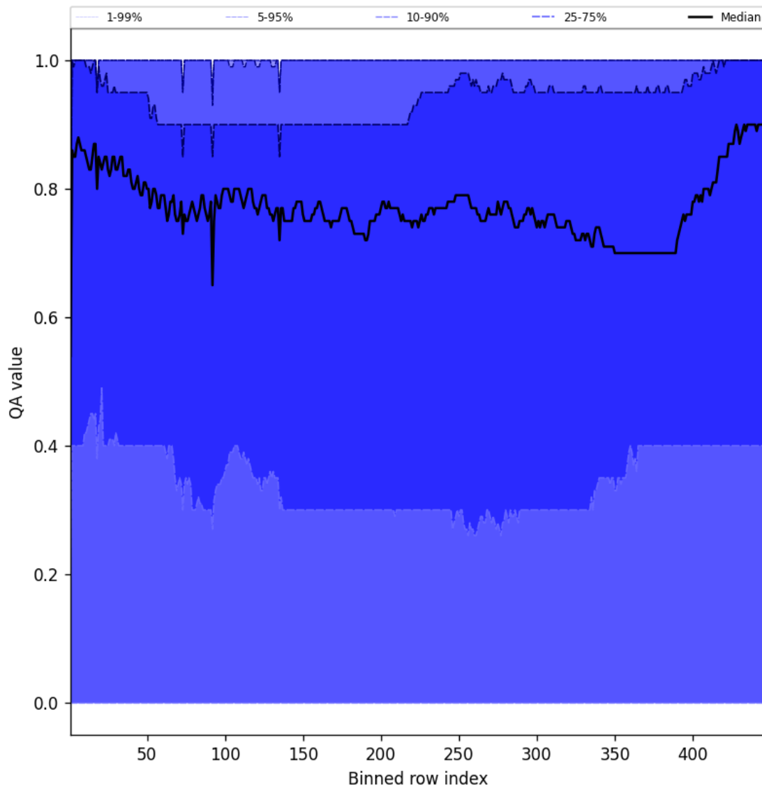
Figure 54: Along track statistics of “QA value” for 2025-10-20 to 2025-10-22
