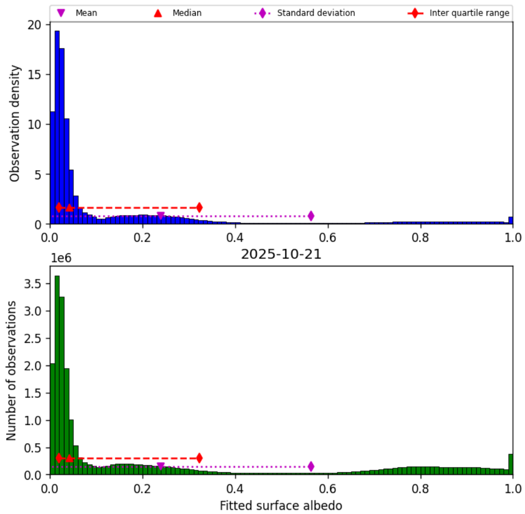
Figure 45: Histogram of “Fitted surface albedo” for 2025-10-20 to 2025-10-22
