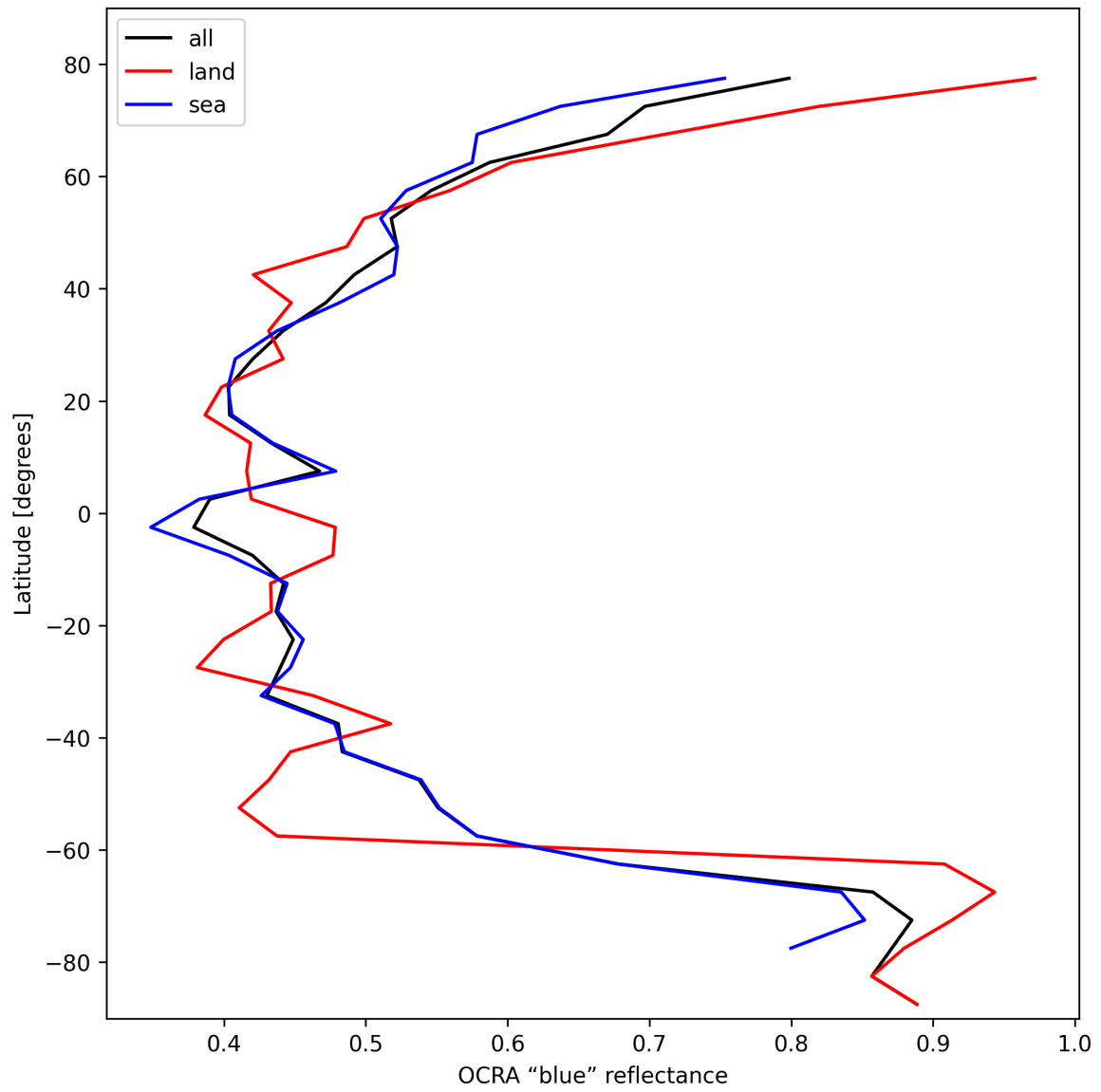
Figure 35: Zonal average of “OCRA “blue” reflectance” for 2025-10-20 to 2025-10-22.
