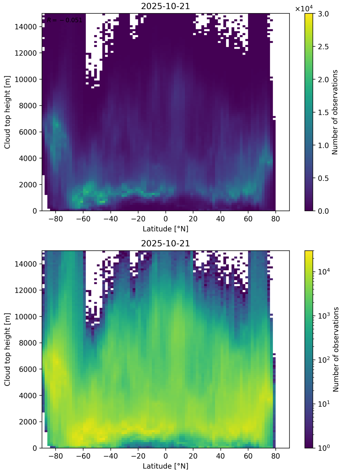
Figure 97: Scatter density plot of “Latitude” against “Cloud top height” for 2025-10-20 to 2025-10-22.
