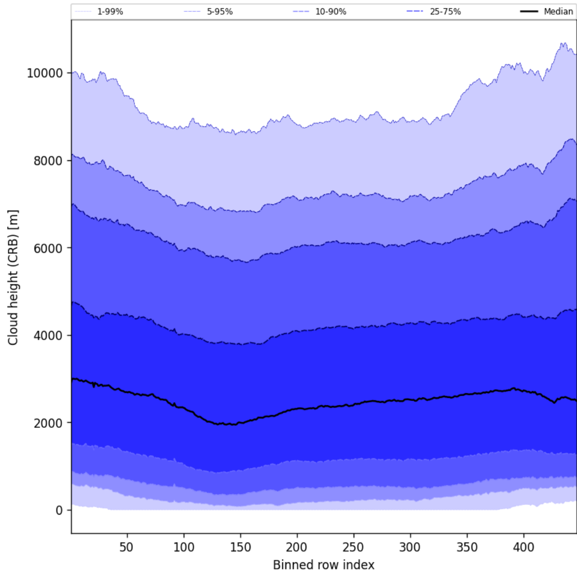
Figure 59: Along track statistics of “Cloud height (CRB)” for 2025-10-20 to 2025-10-22
