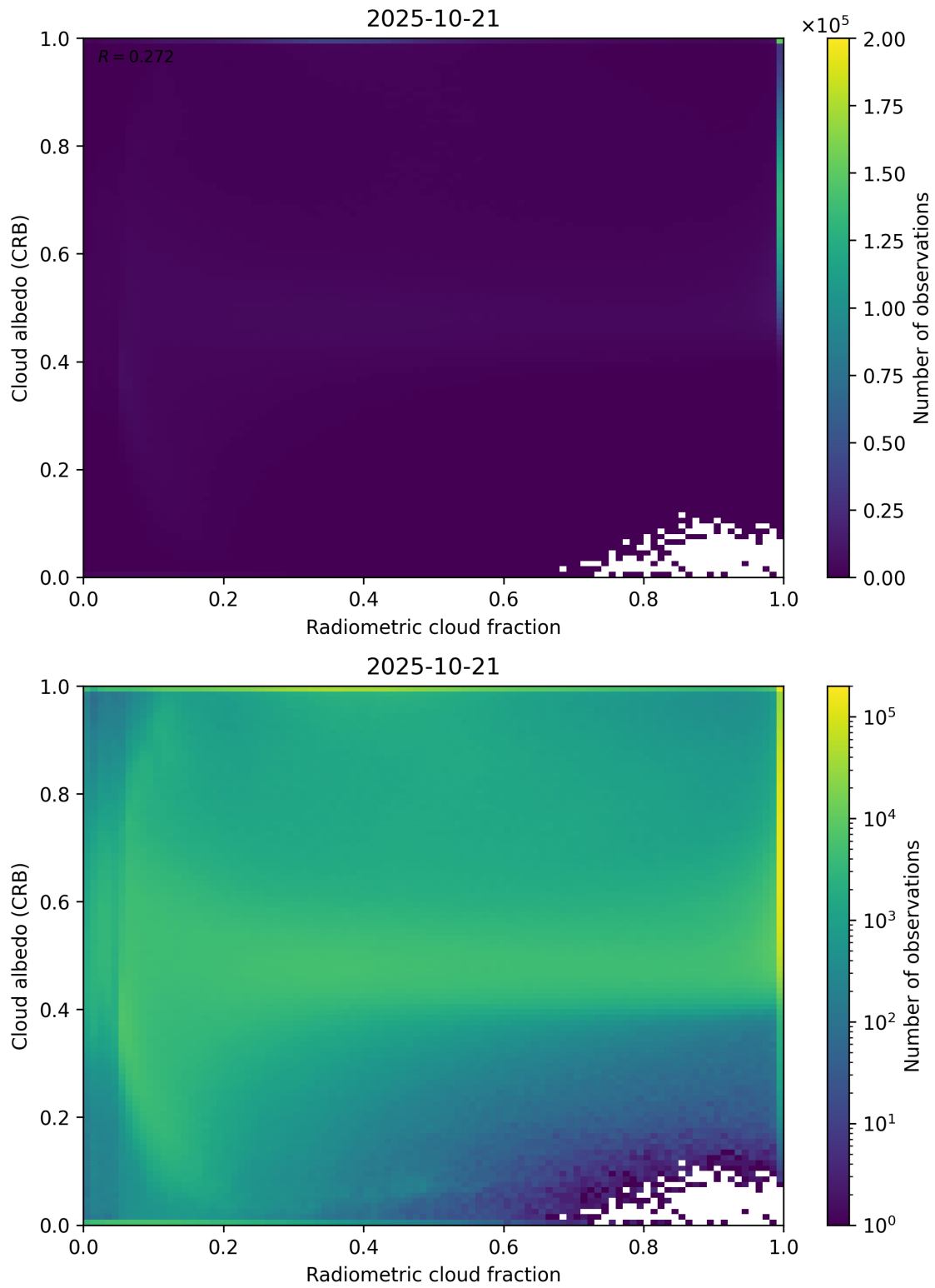
Figure 71: Scatter density plot of “Radiometric cloud fraction” against “Cloud albedo (CRB)” for 2025-10-20 to 2025-10-22.
