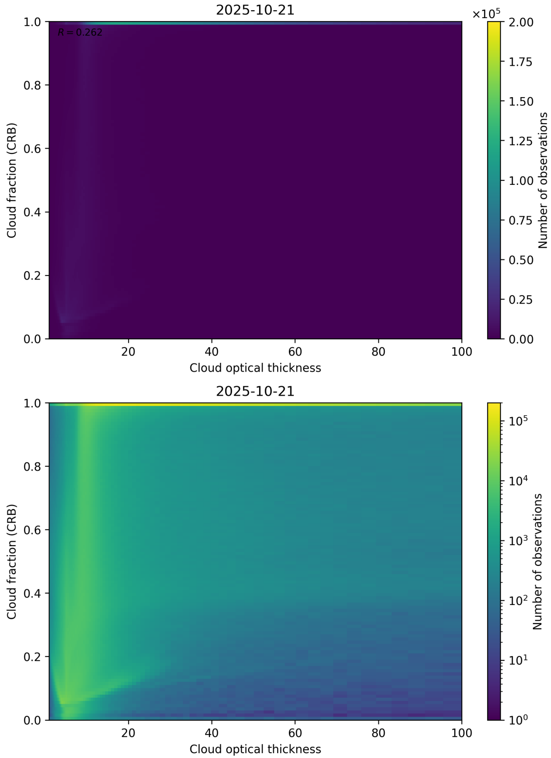
Figure 84: Scatter density plot of “Cloud optical thickness” against “Cloud fraction (CRB)” for 2025-10-20 to 2025-10-22.
