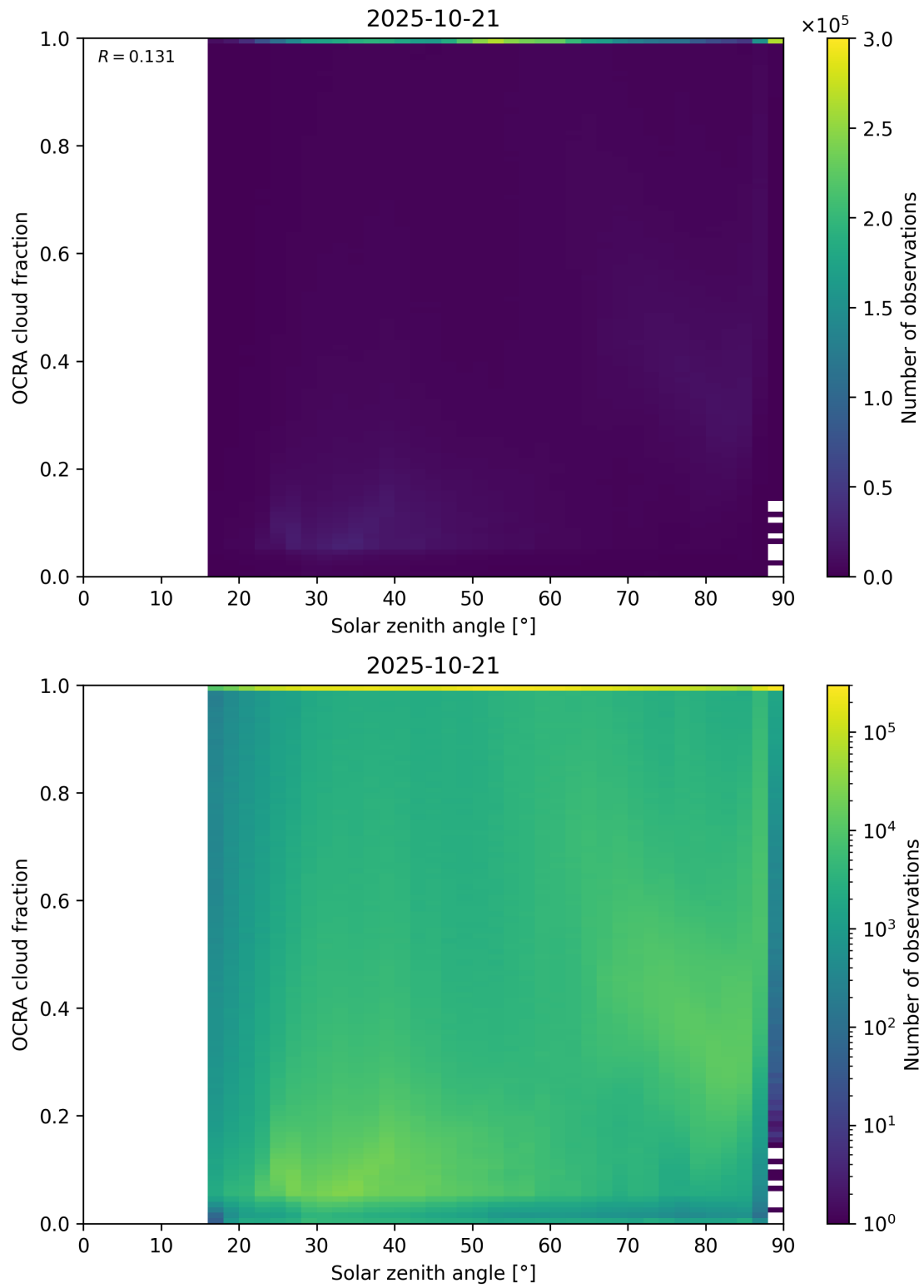
Figure 100: Scatter density plot of “Solar zenith angle” against “OCRA cloud fraction” for 2025-10-20 to 2025-10-22.
