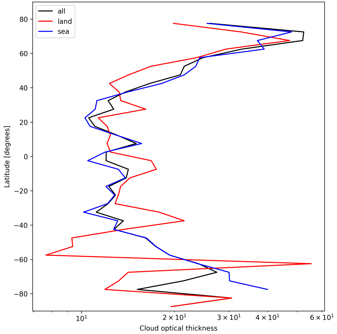
Figure 25: Zonal average of “Cloud optical thickness” for 2025-10-20 to 2025-10-22.
