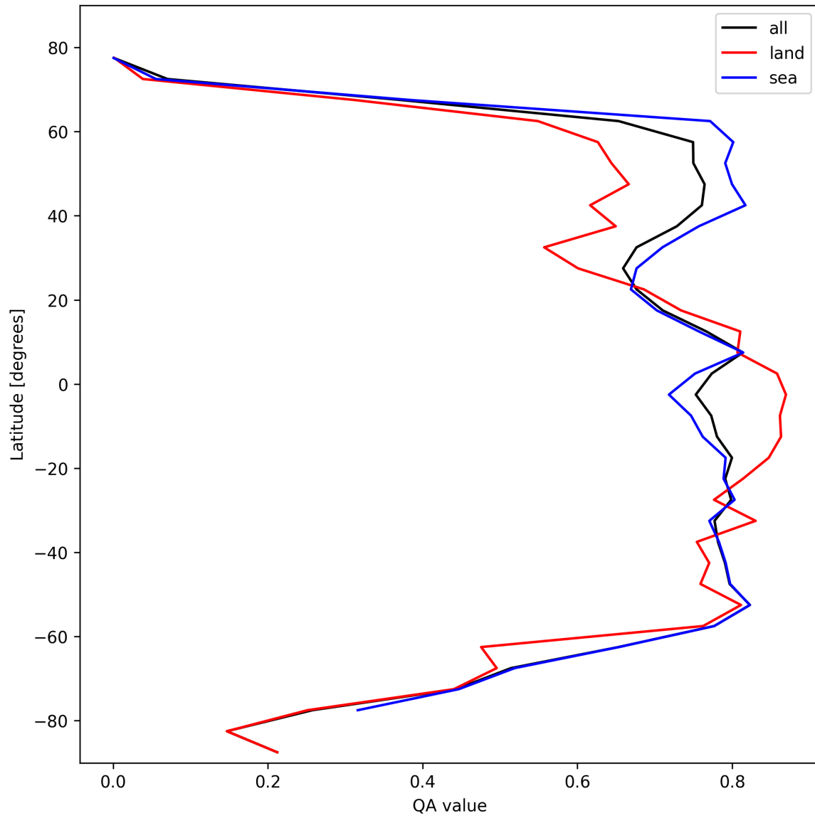
Figure 22: Zonal average of “QA value” for 2025-10-20 to 2025-10-22.
