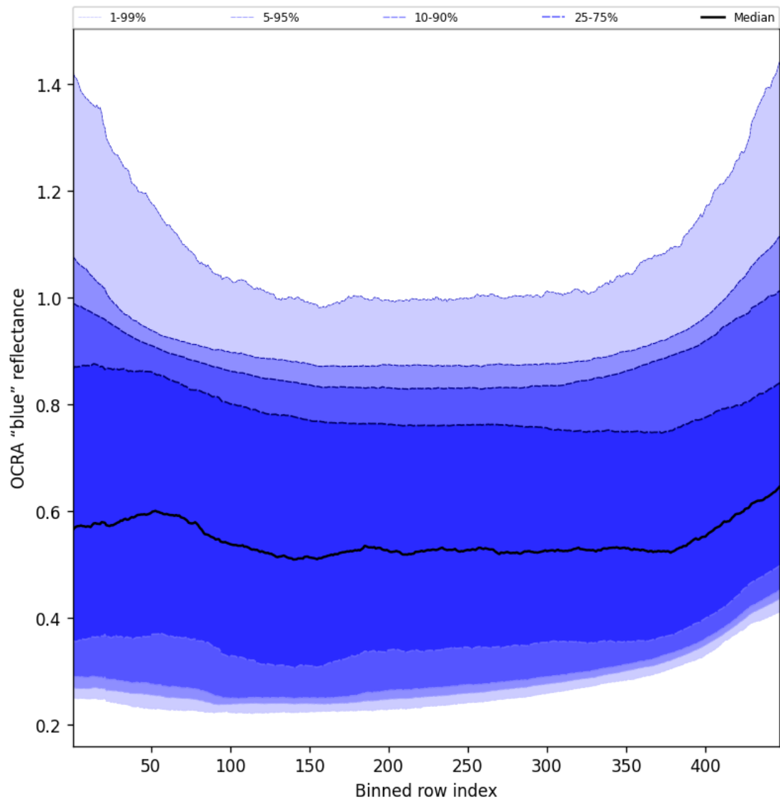
Figure 67: Along track statistics of "OCRA "blue" reflectance" for 2025-10-20 to 2025-10-22
