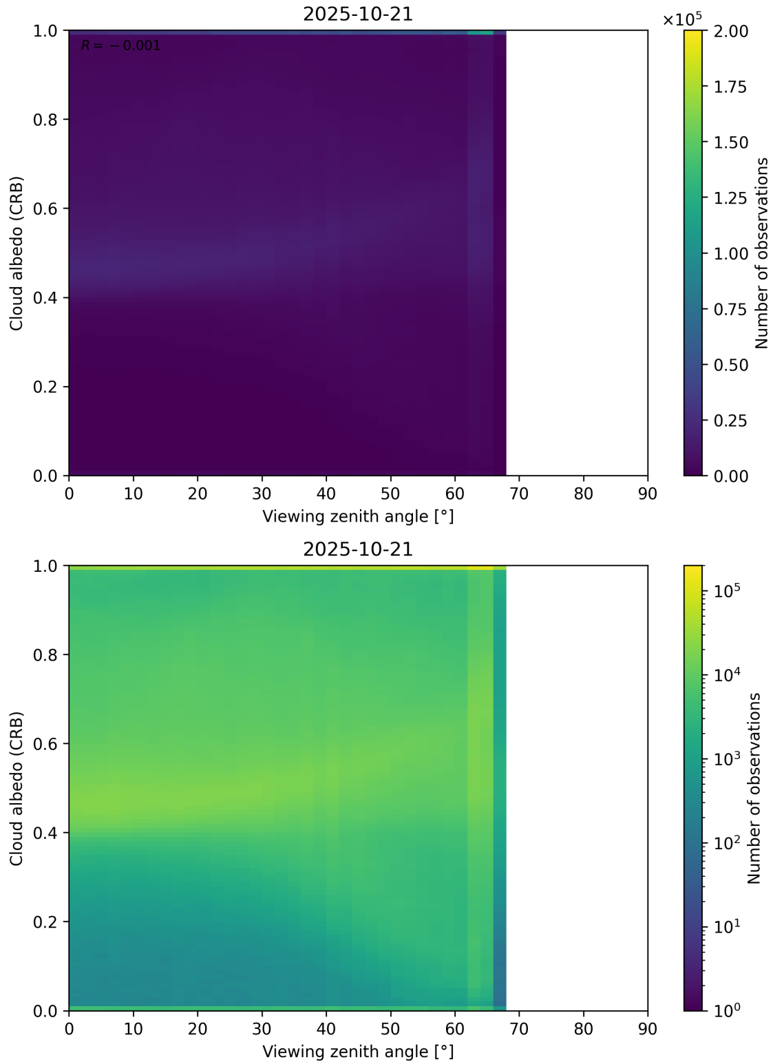
Figure 106: Scatter density plot of “Viewing zenith angle” against “Cloud albedo (CRB)” for 2025-10-20 to 2025-10-22.
