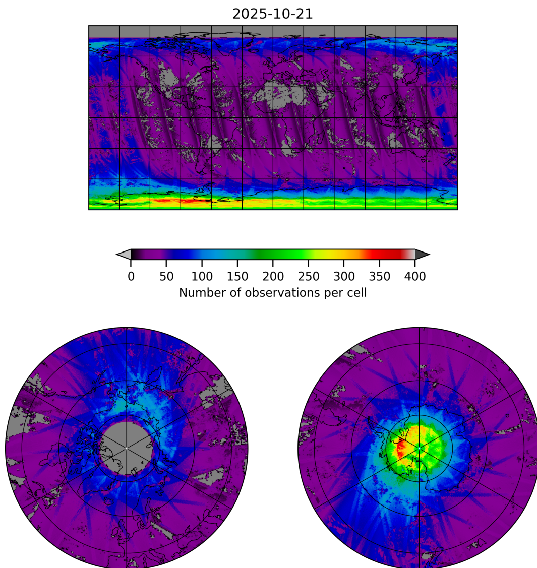
Figure 21: Map of the number of observations for 2025-10-20 to 2025-10-22
