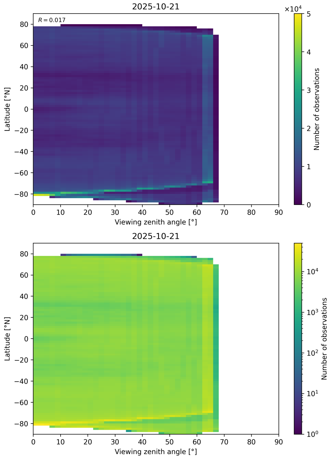
Figure 113: Scatter density plot of “Viewing zenith angle” against “Latitude” for 2025-10-20 to 2025-10-22.
