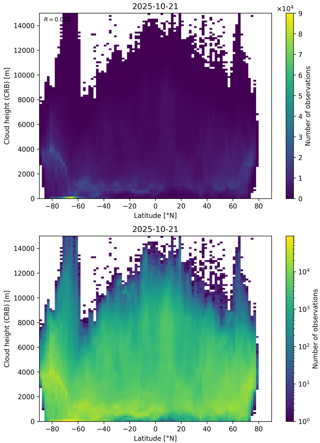
Figure 95: Scatter density plot of “Latitude” against “Cloud height (CRB)” for 2025-10-20 to 2025-10-22.
