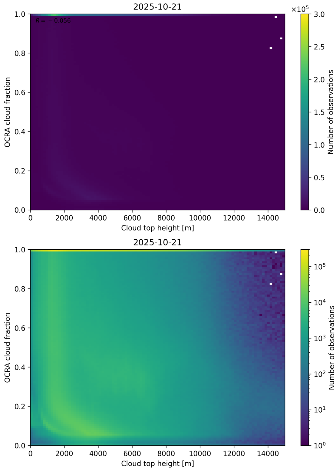
Figure 87: Scatter density plot of “Cloud top height” against “OCRA cloud fraction” for 2025-10-20 to 2025-10-22.
