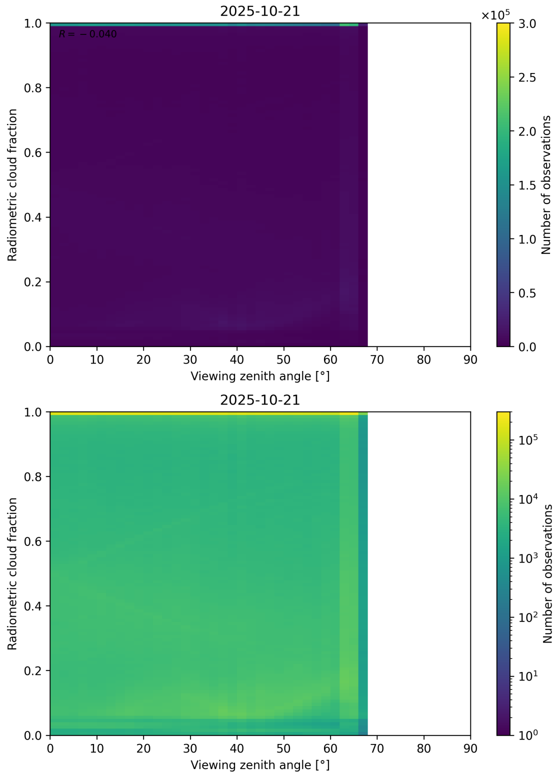
Figure 107: Scatter density plot of “Viewing zenith angle” against “Radiometric cloud fraction” for 2025-10-20 to 2025-10-22.
