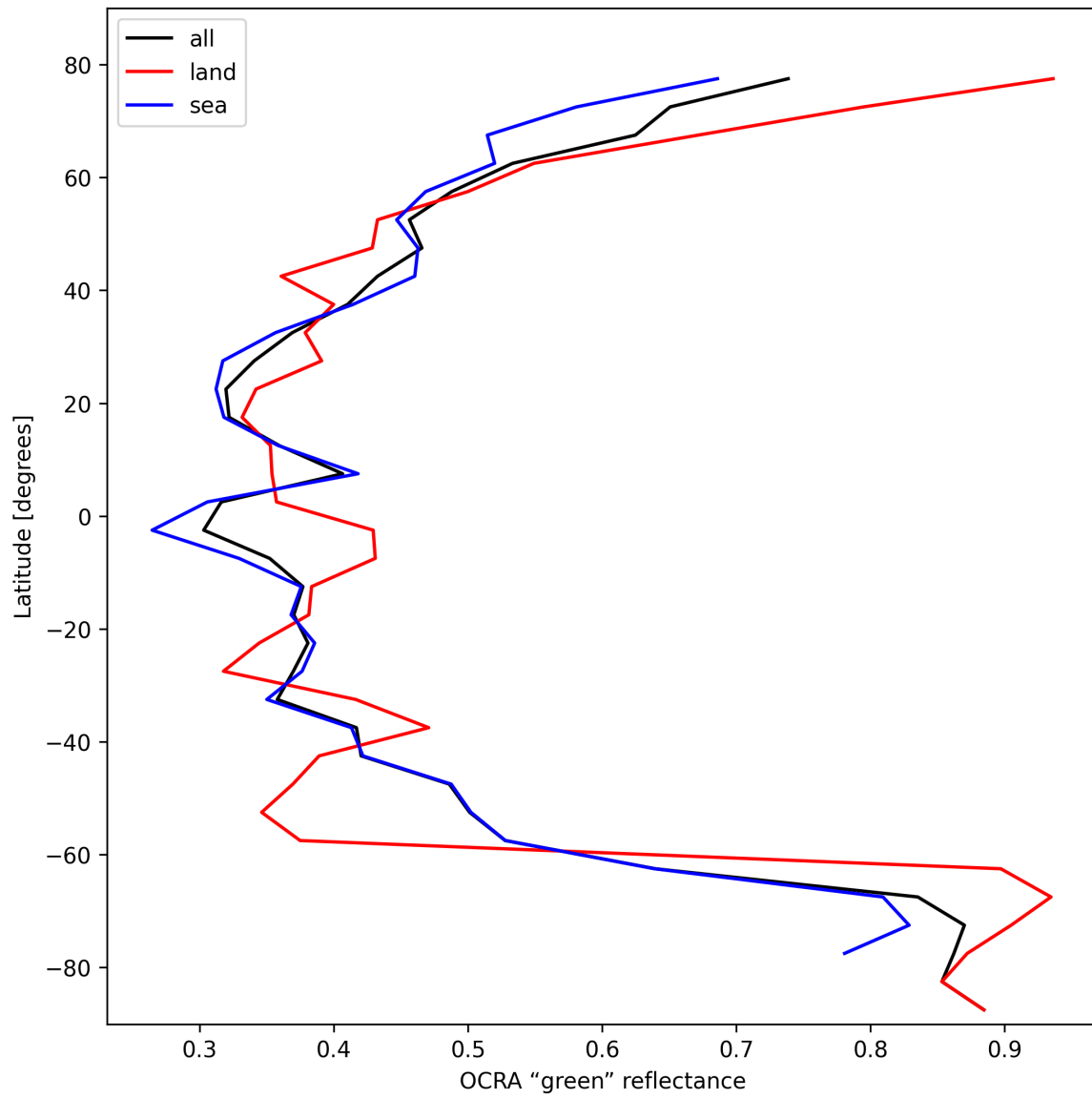
Figure 36: Zonal average of “OCRA “green” reflectance” for 2025-10-20 to 2025-10-22.
