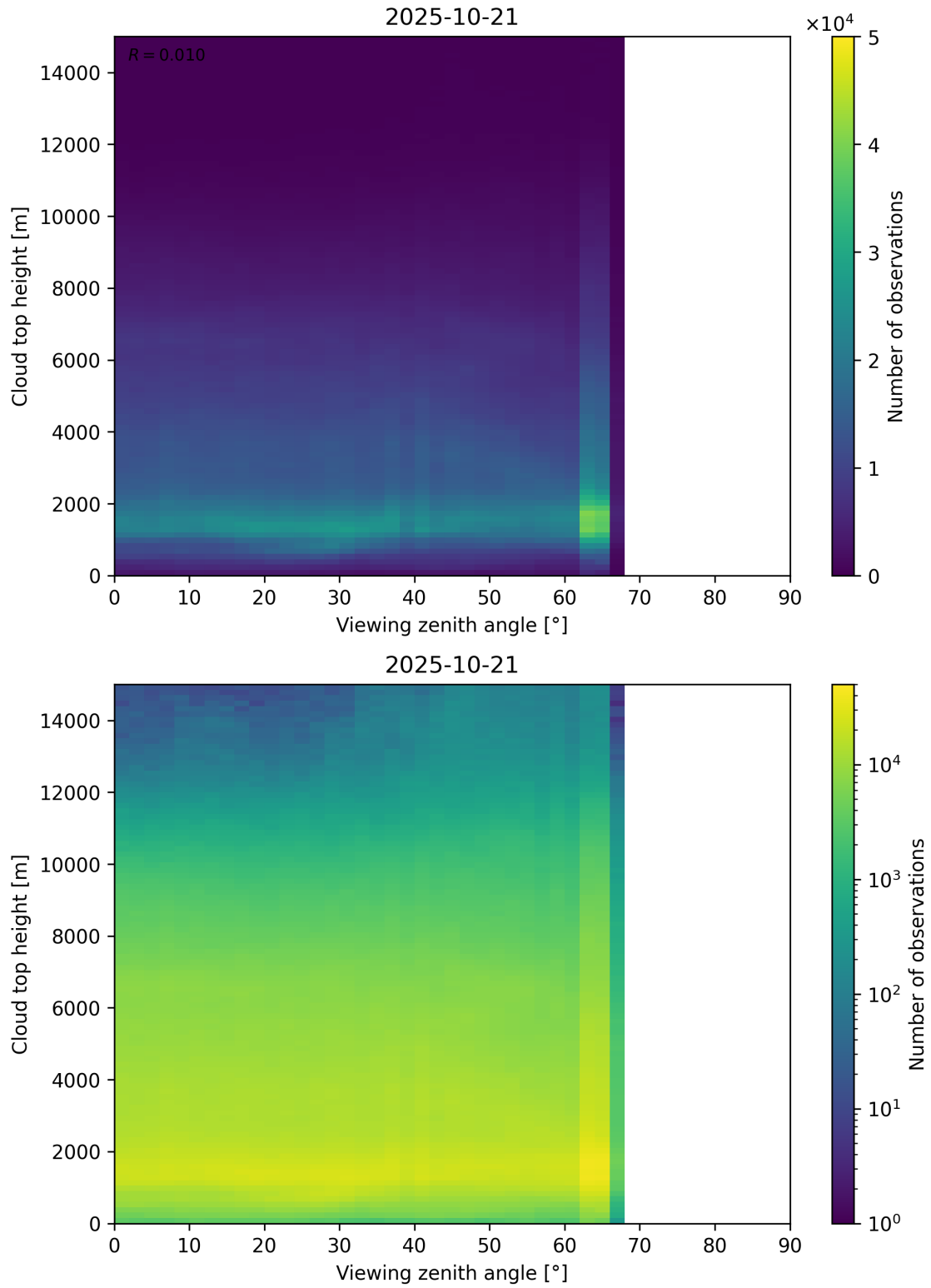
Figure 112: Scatter density plot of “Viewing zenith angle” against “Cloud top height” for 2025-10-20 to 2025-10-22.
