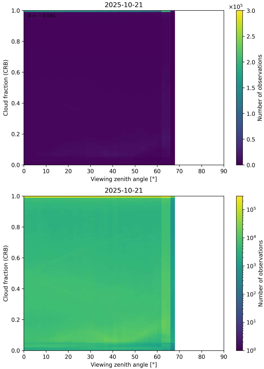
Figure 109: Scatter density plot of “Viewing zenith angle” against “Cloud fraction (CRB)” for 2025-10-20 to 2025-10-22.
