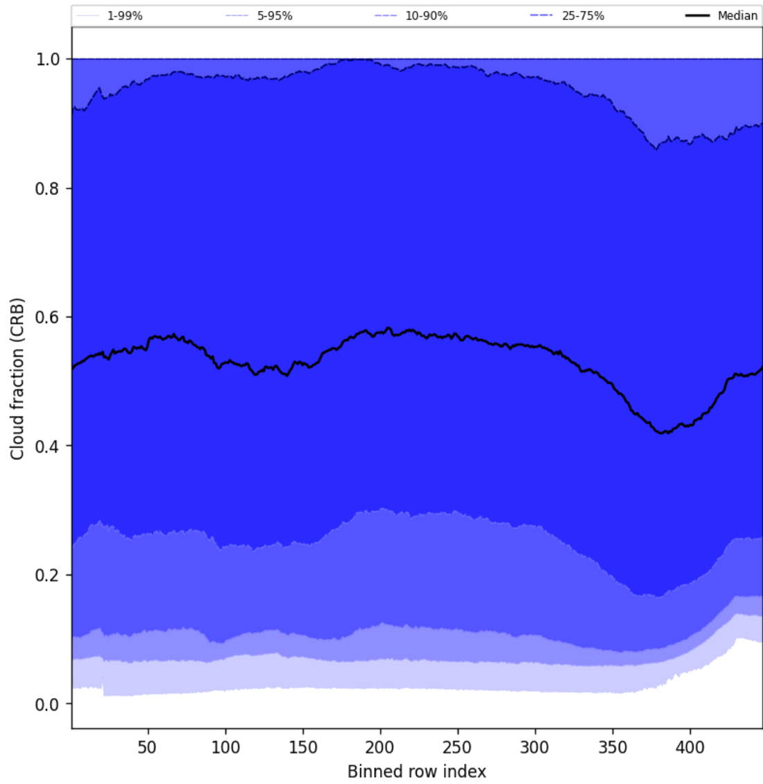
Figure 58: Along track statistics of “Cloud fraction (CRB)” for 2025-10-20 to 2025-10-22
