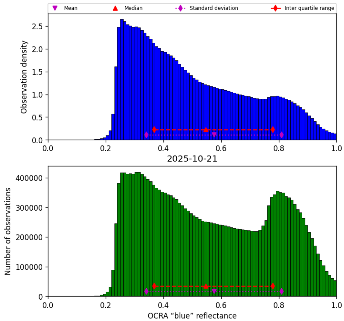
Figure 51: Histogram of “OCRA “blue” reflectance” for 2025-10-20 to 2025-10-22
