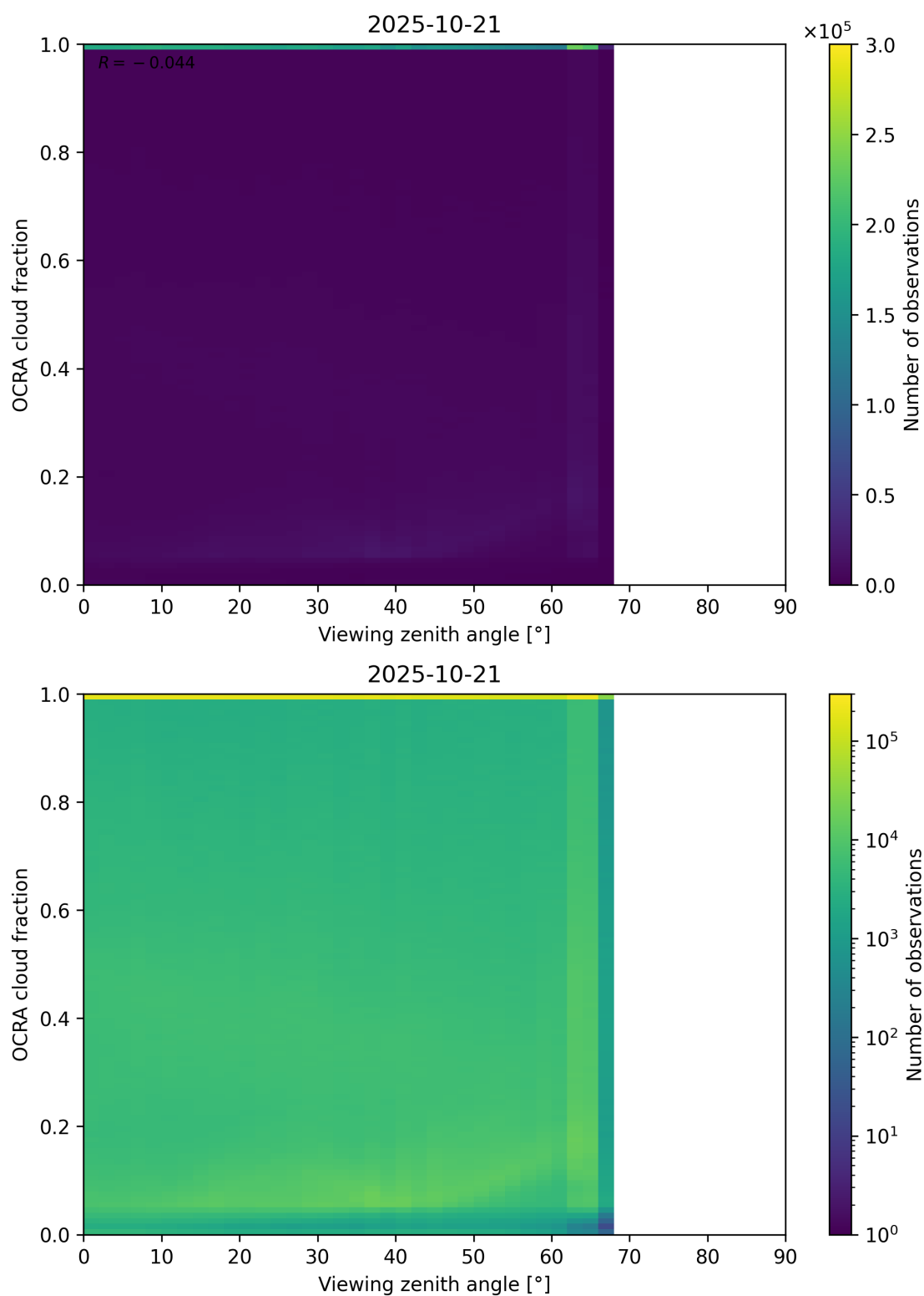
Figure 108: Scatter density plot of “Viewing zenith angle” against “OCRA cloud fraction” for 2025-10-20 to 2025-10-22.
