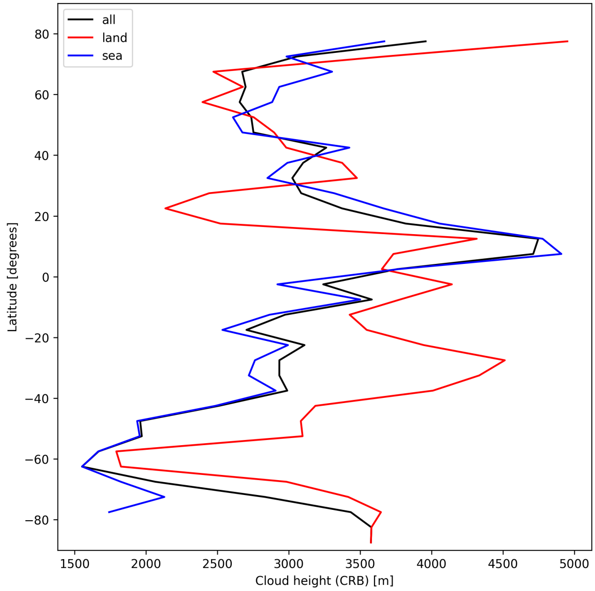
Figure 27: Zonal average of “Cloud height (CRB)” for 2025-10-20 to 2025-10-22.
