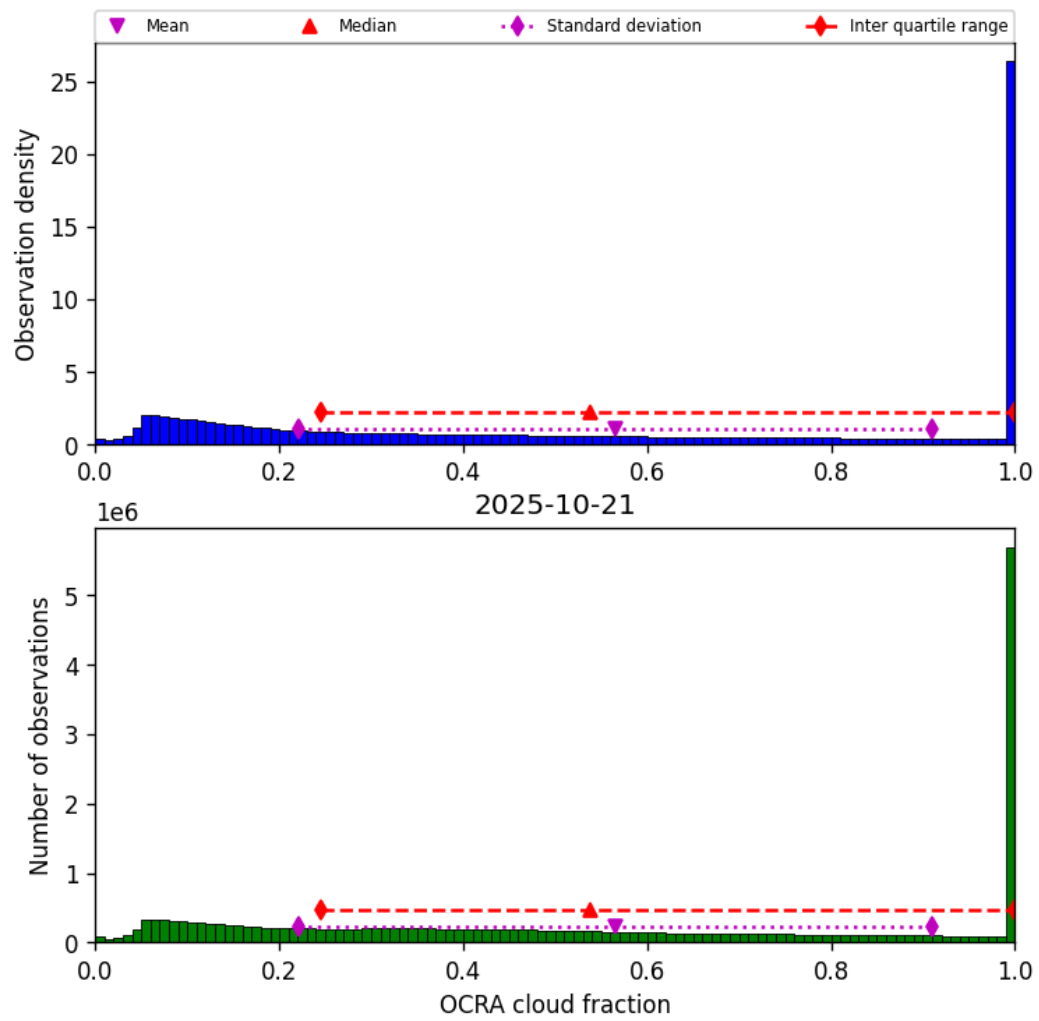
Figure 50: Histogram of “OCRA cloud fraction” for 2025-10-20 to 2025-10-22
