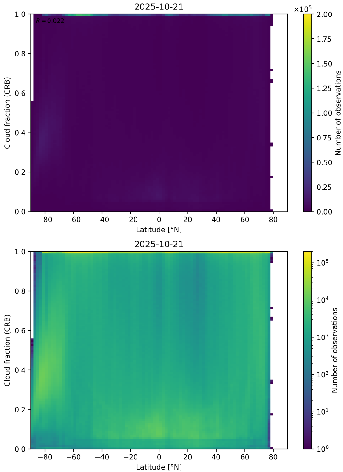
Figure 94: Scatter density plot of “Latitude” against “Cloud fraction (CRB)” for 2025-10-20 to 2025-10-22.
