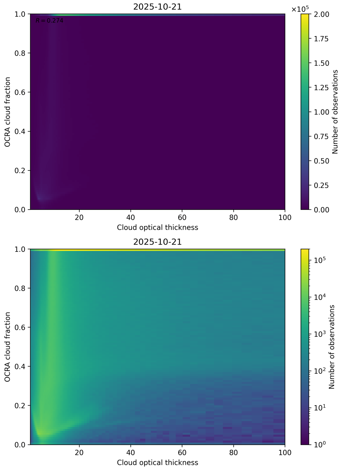
Figure 83: Scatter density plot of “Cloud optical thickness” against “OCRA cloud fraction” for 2025-10-20 to 2025-10-22.
