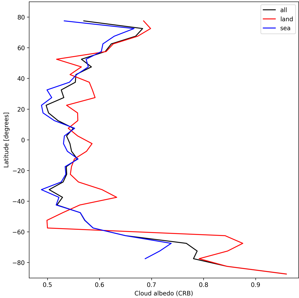
Figure 28: Zonal average of “Cloud albedo (CRB)” for 2025-10-20 to 2025-10-22.
