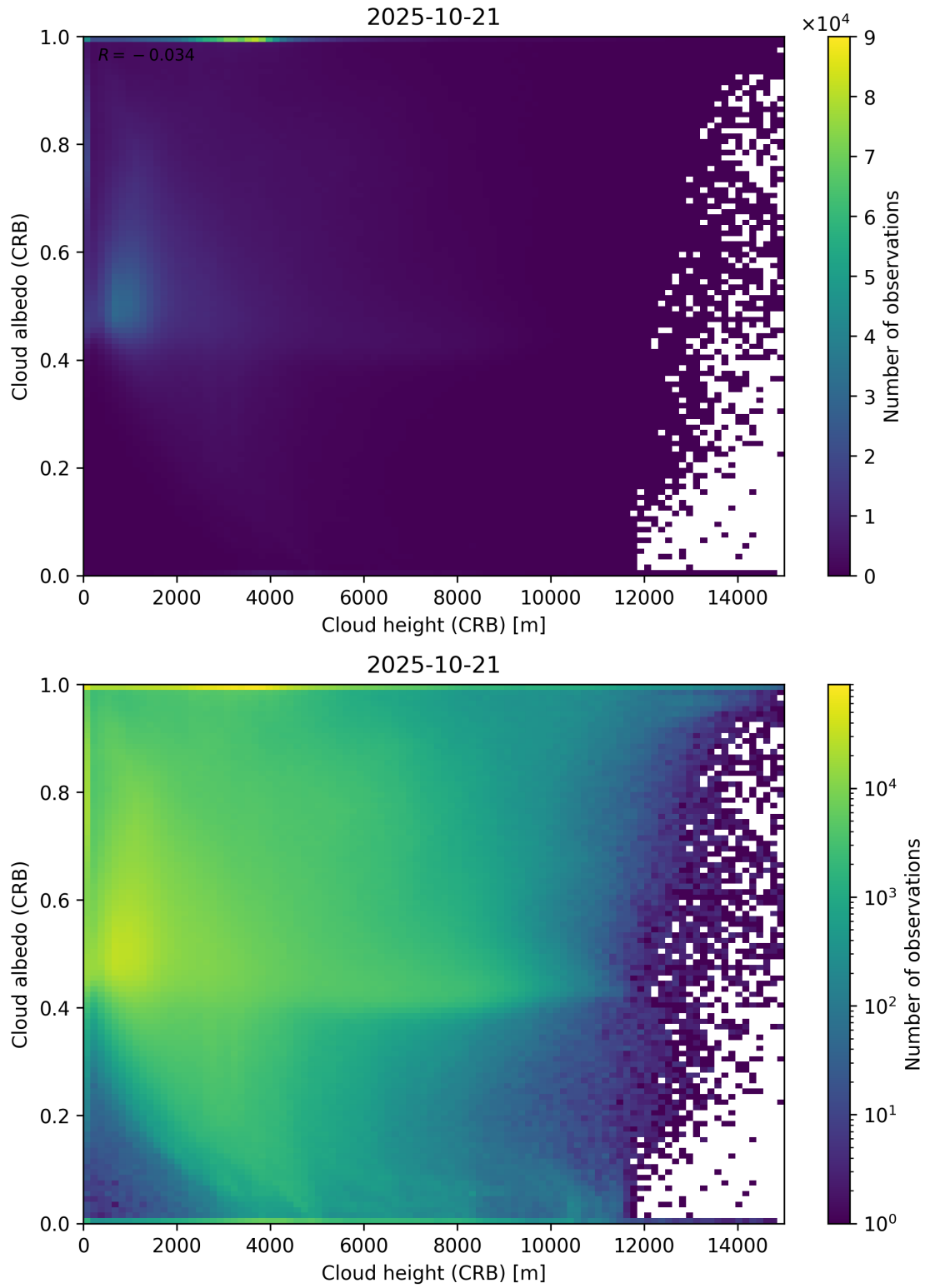
Figure 80: Scatter density plot of “Cloud height (CRB)” against “Cloud albedo (CRB)” for 2025-10-20 to 2025-10-22.
