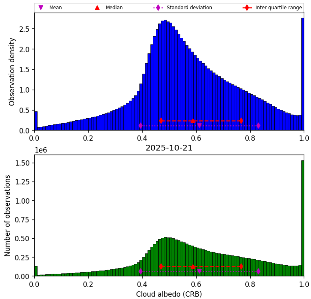
Figure 44: Histogram of “Cloud albedo (CRB)” for 2025-10-20 to 2025-10-22
