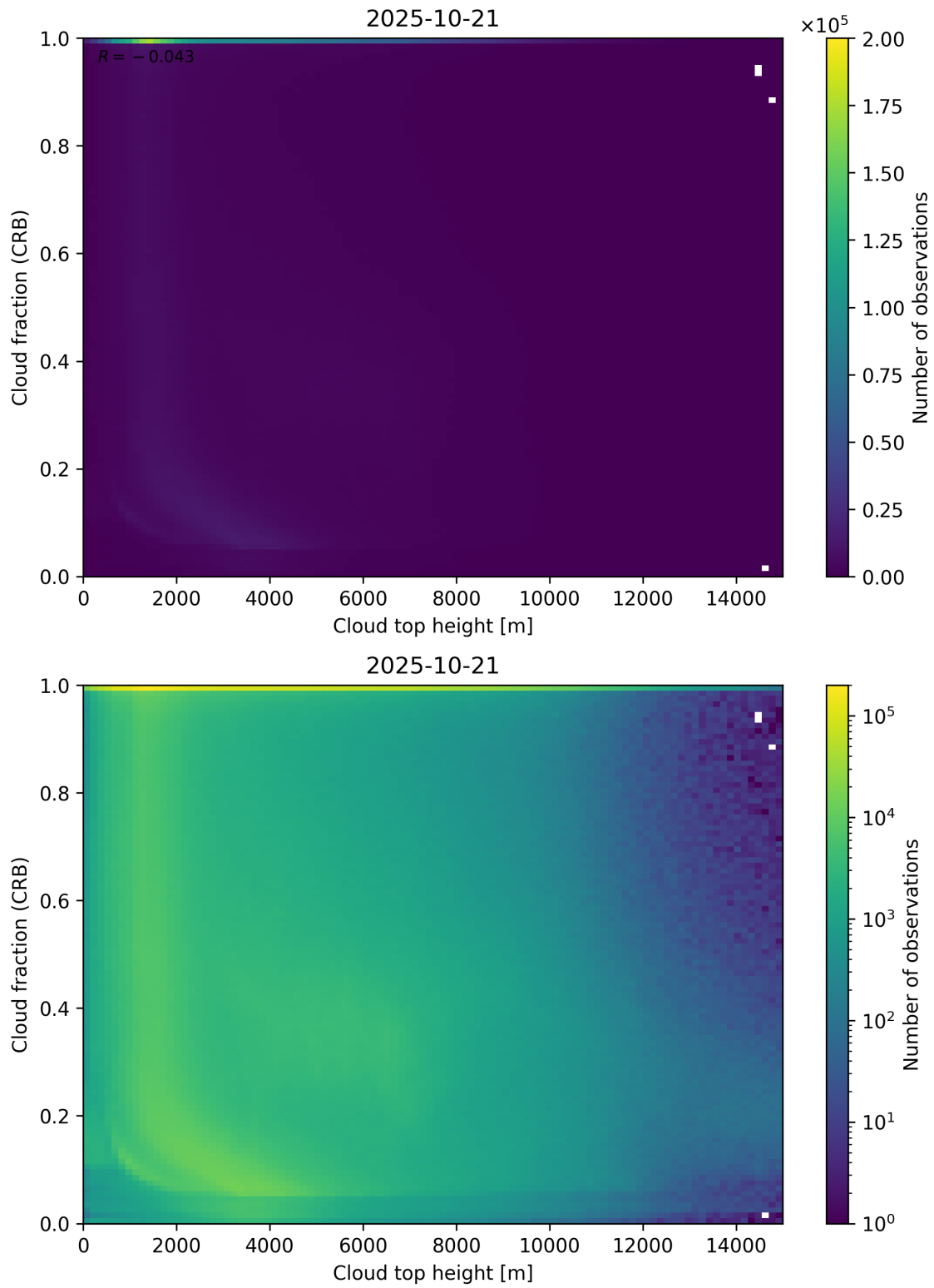
Figure 88: Scatter density plot of “Cloud top height” against “Cloud fraction (CRB)” for 2025-10-20 to 2025-10-22.
