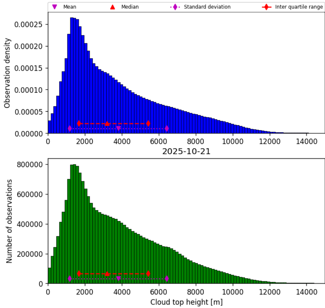
Figure 40: Histogram of “Cloud top height” for 2025-10-20 to 2025-10-22
