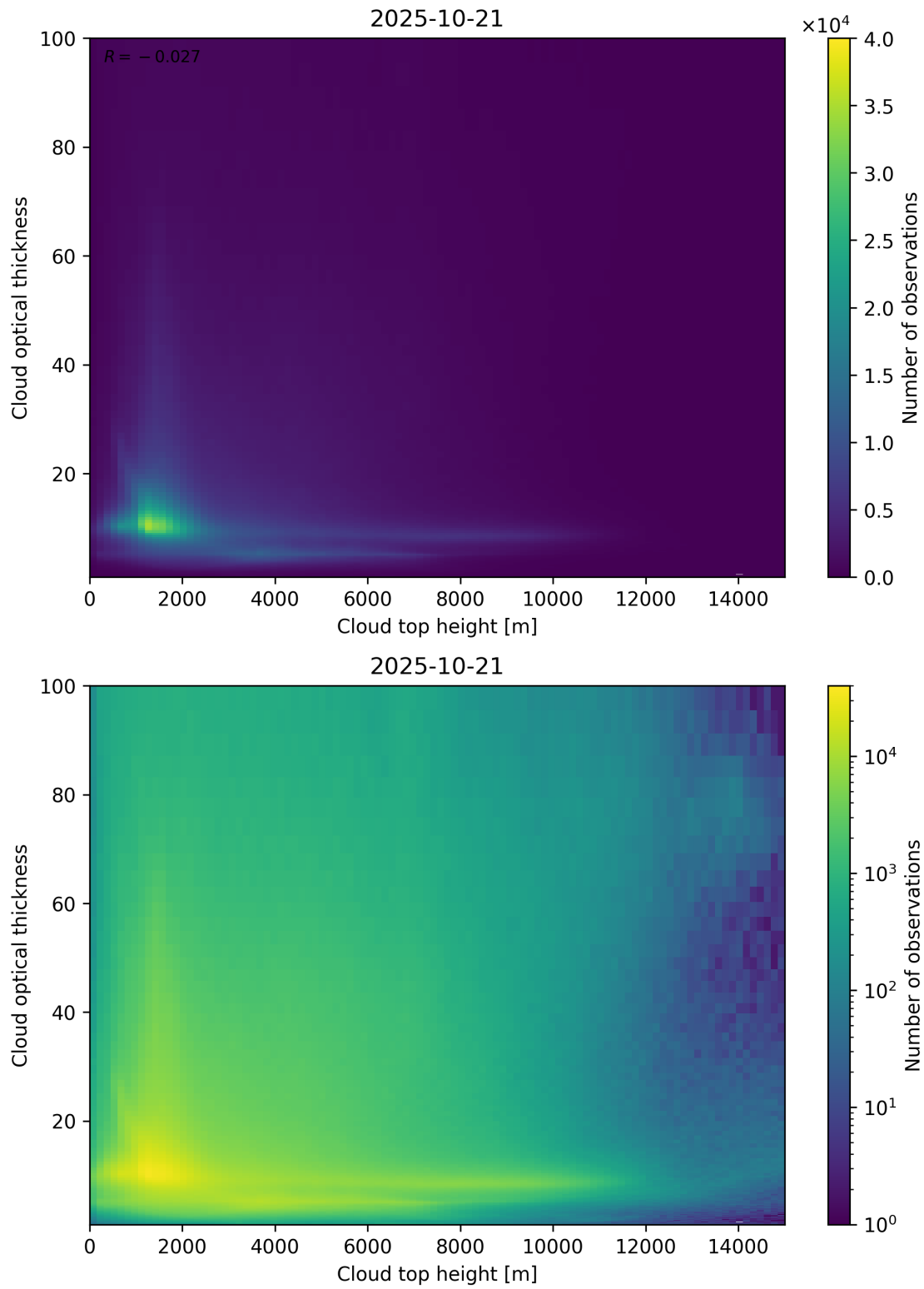
Figure 90: Scatter density plot of “Cloud top height” against “Cloud optical thickness” for 2025-10-20 to 2025-10-22.
