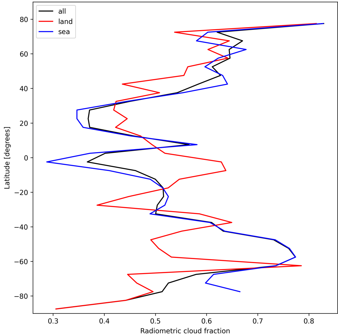
Figure 23: Zonal average of “Radiometric cloud fraction” for 2025-10-20 to 2025-10-22.
