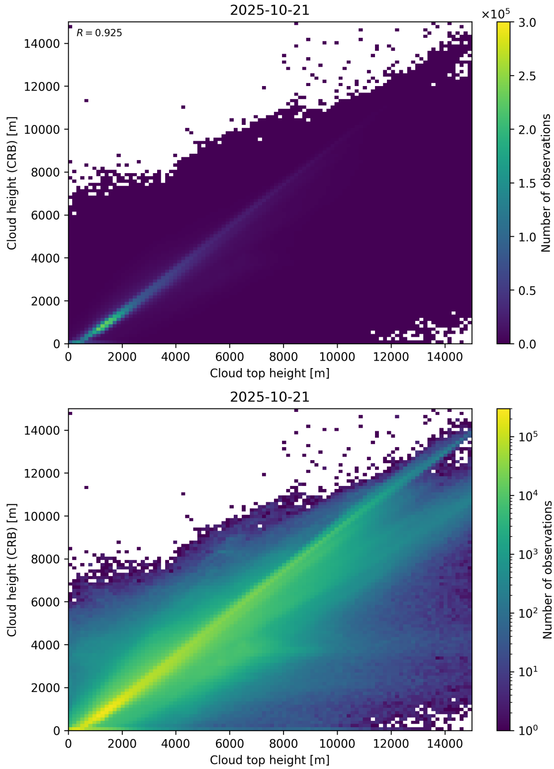
Figure 89: Scatter density plot of “Cloud top height” against “Cloud height (CRB)” for 2025-10-20 to 2025-10-22.
