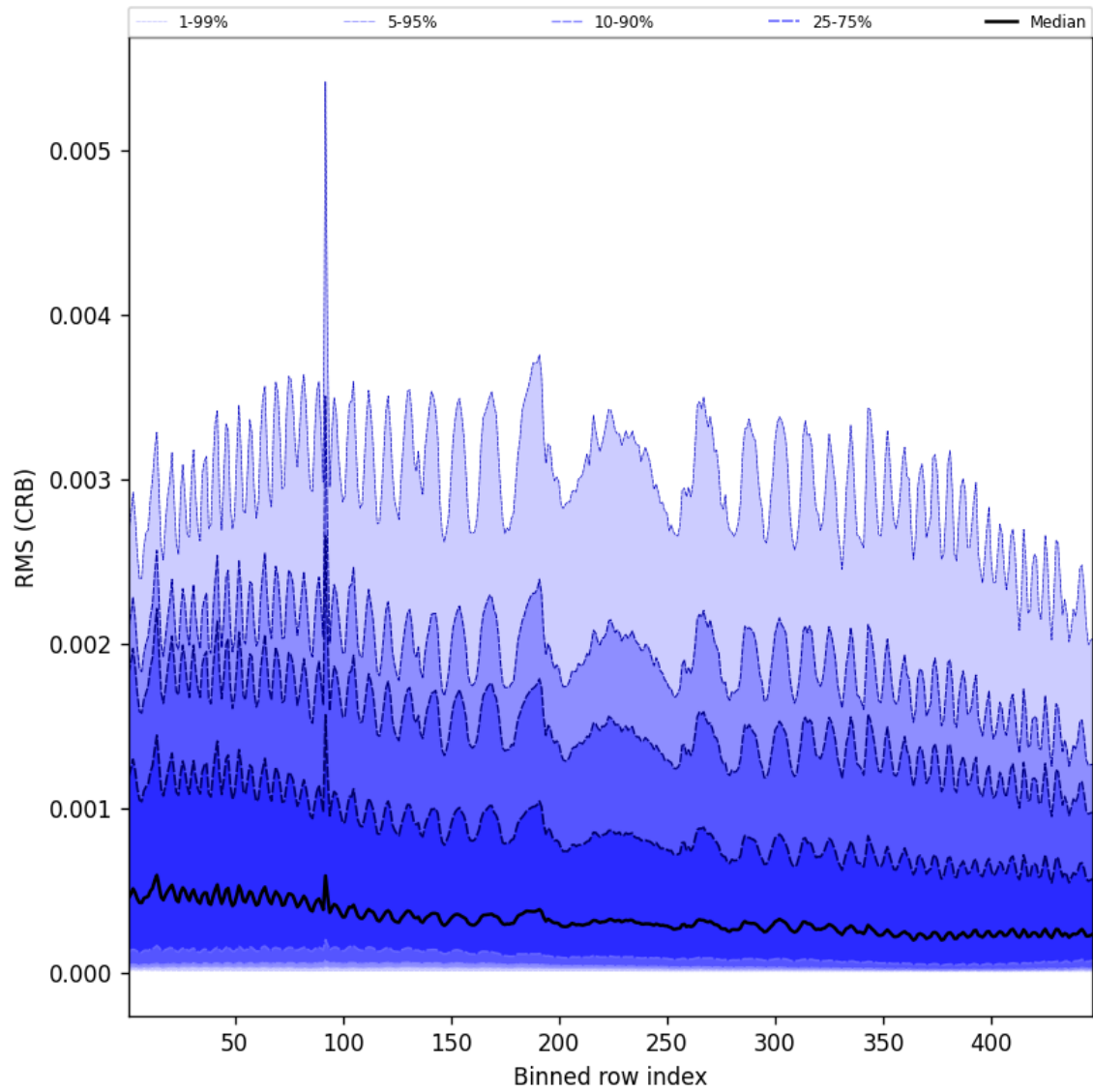
Figure 64: Along track statistics of “RMS (CRB)” for 2025-10-20 to 2025-10-22
