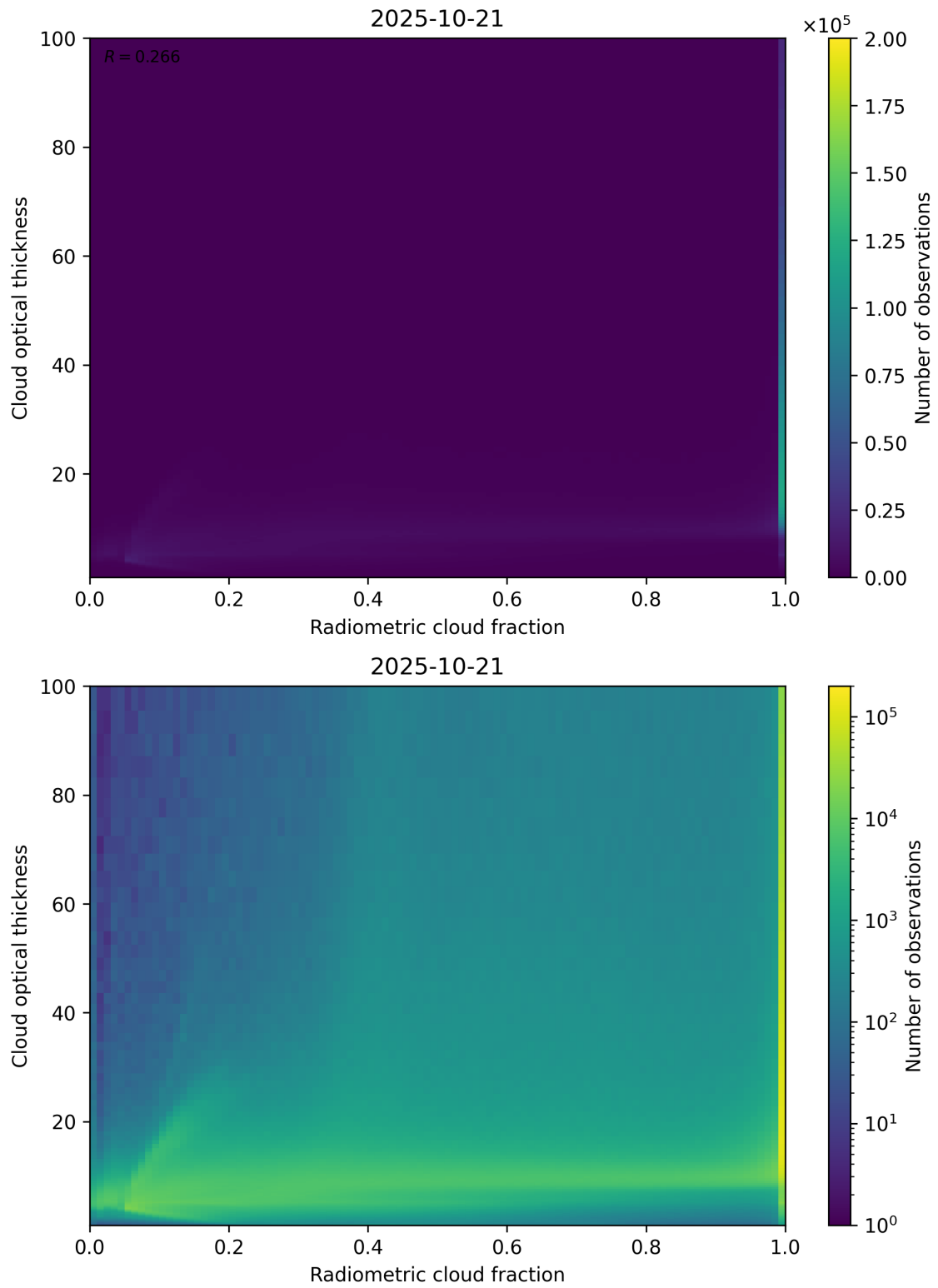
Figure 75: Scatter density plot of “Radiometric cloud fraction” against “Cloud optical thickness” for 2025-10-20 to 2025-10-22.
