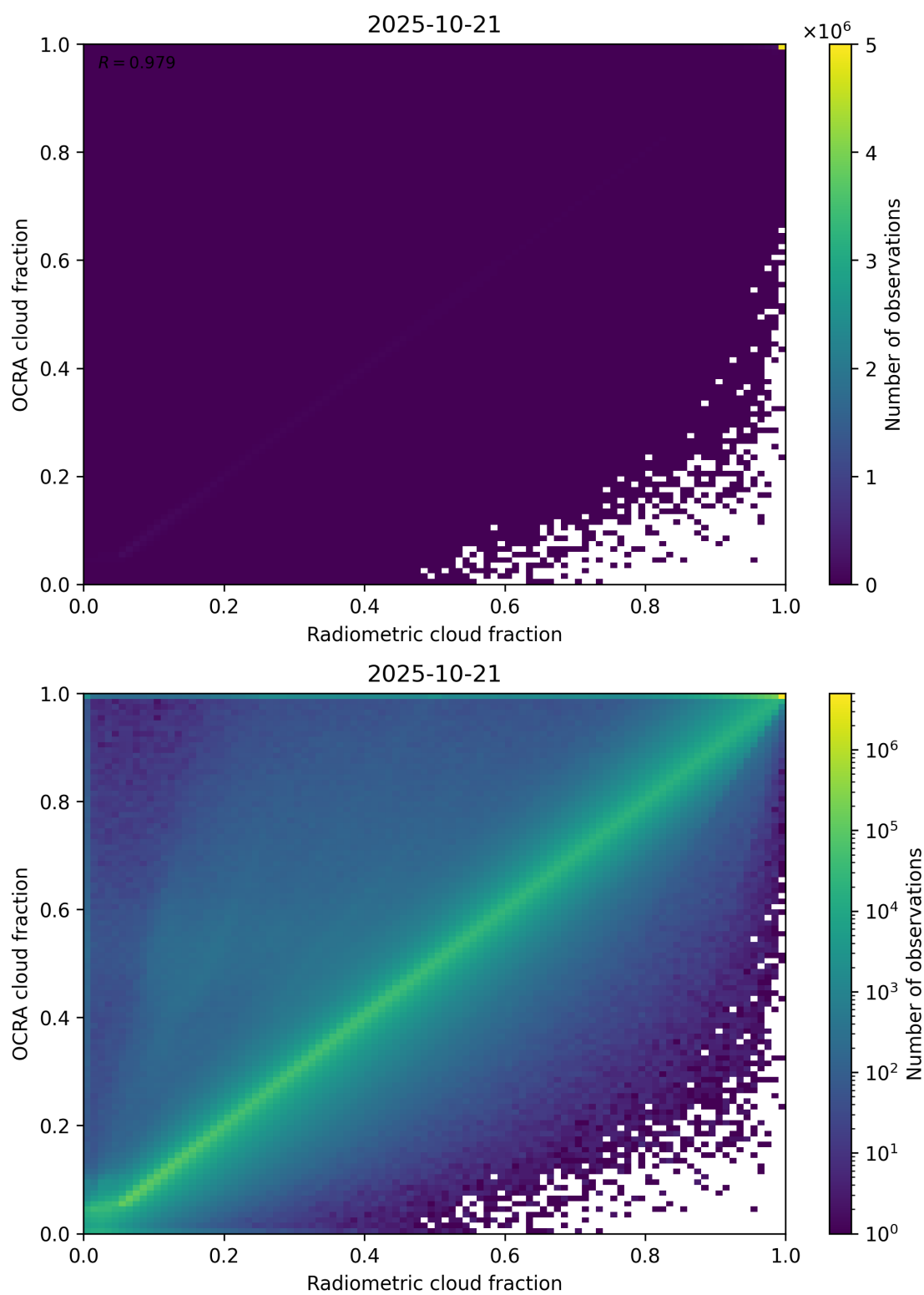
Figure 72: Scatter density plot of “Radiometric cloud fraction” against “OCRA cloud fraction” for 2025-10-20 to 2025-10-22.
