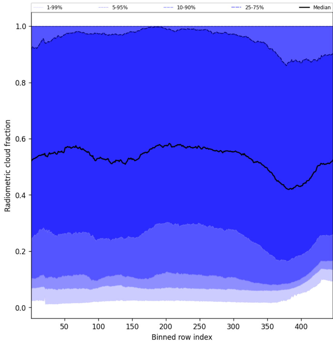
Figure 55: Along track statistics of “Radiometric cloud fraction” for 2025-10-20 to 2025-10-22
