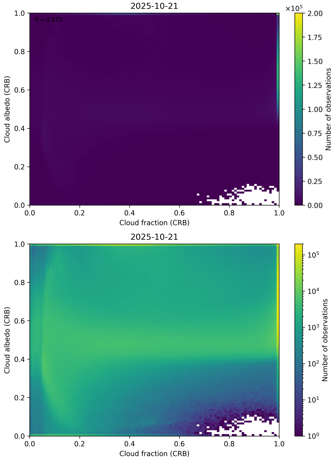
Figure 77: Scatter density plot of “Cloud fraction (CRB)” against “Cloud albedo (CRB)” for 2025-10-20 to 2025-10-22.
