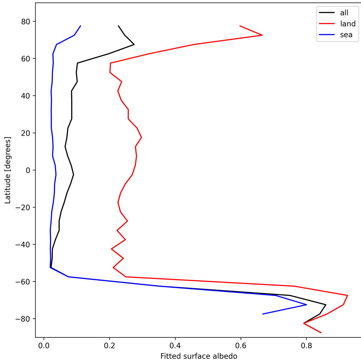
Figure 29: Zonal average of “Fitted surface albedo” for 2025-10-20 to 2025-10-22.
