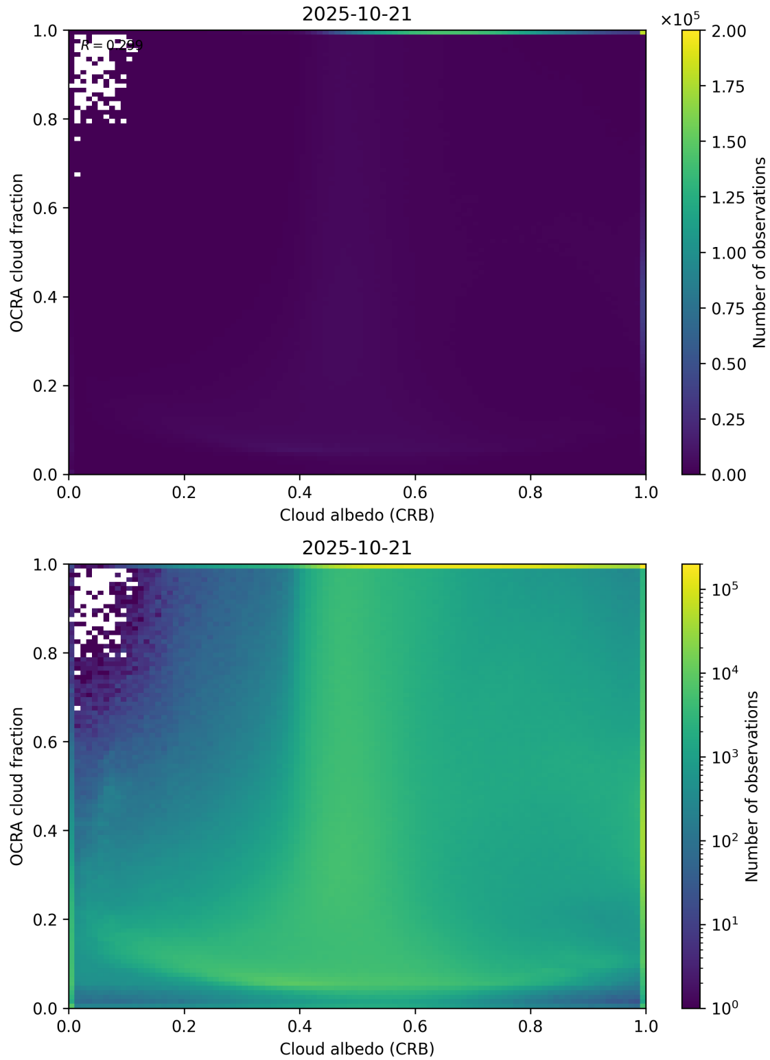
Figure 70: Scatter density plot of “Cloud albedo (CRB)” against “OCRA cloud fraction” for 2025-10-20 to 2025-10-22.
