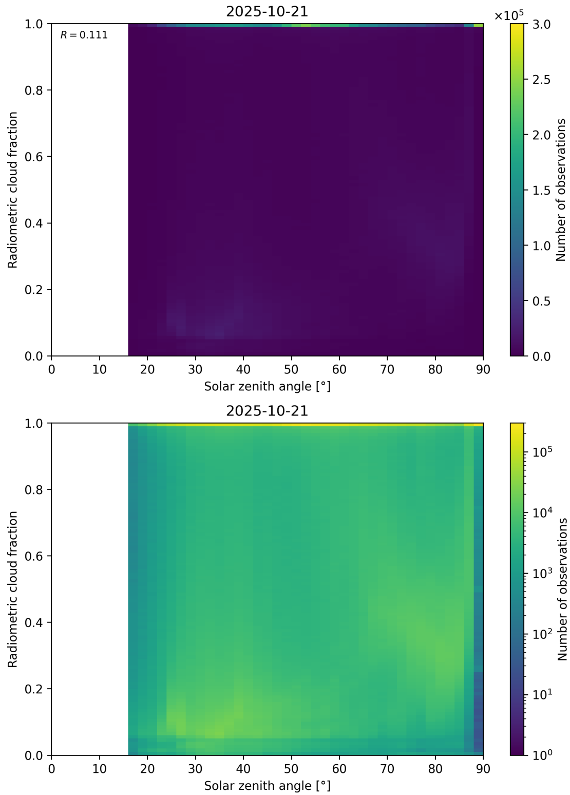
Figure 99: Scatter density plot of “Solar zenith angle” against “Radiometric cloud fraction” for 2025-10-20 to 2025-10-22.
