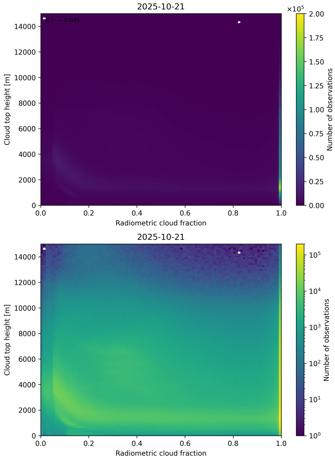
Figure 76: Scatter density plot of “Radiometric cloud fraction” against “Cloud top height” for 2025-10-20 to 2025-10-22.
