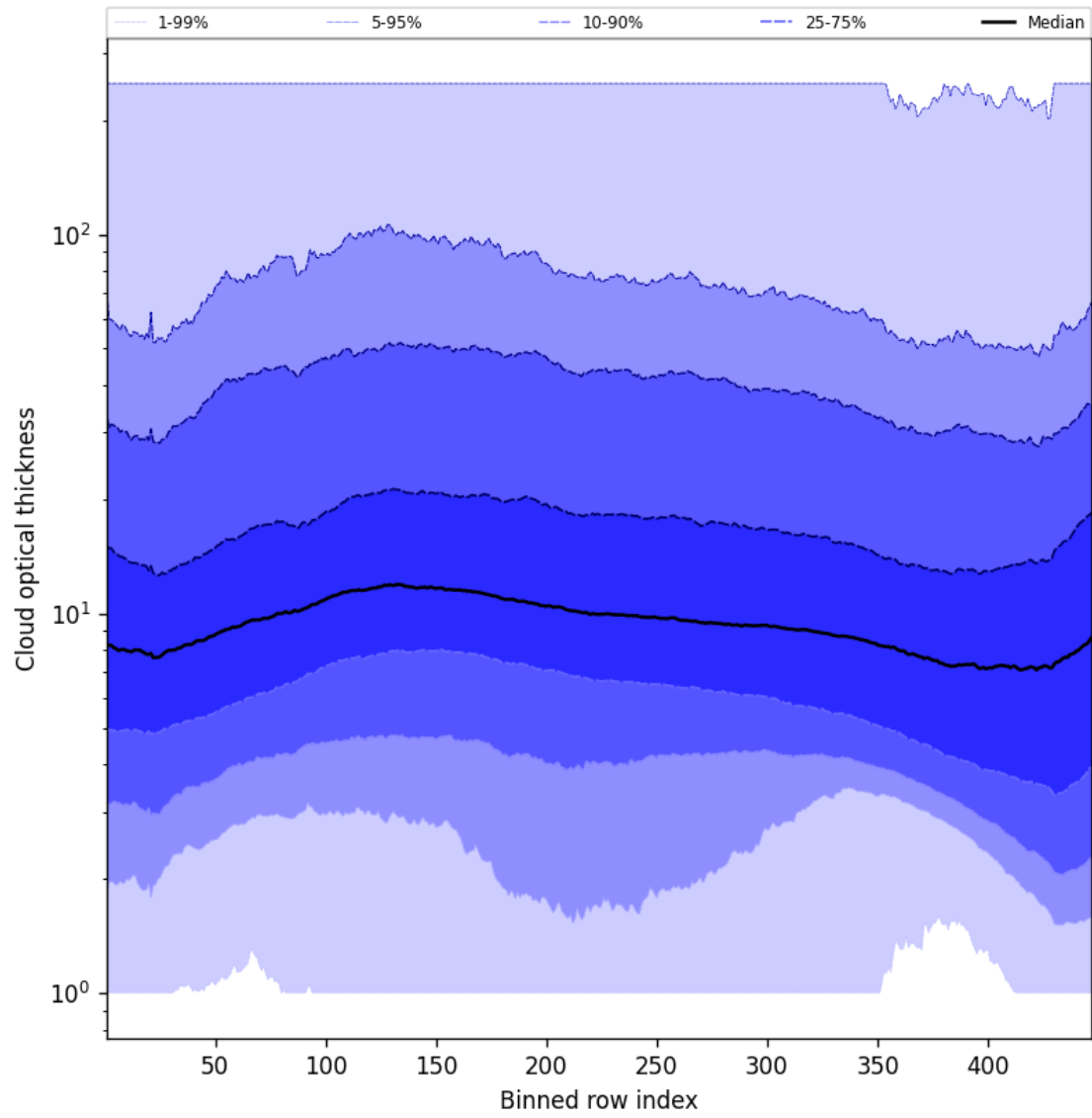
Figure 57: Along track statistics of “Cloud optical thickness” for 2025-10-20 to 2025-10-22
