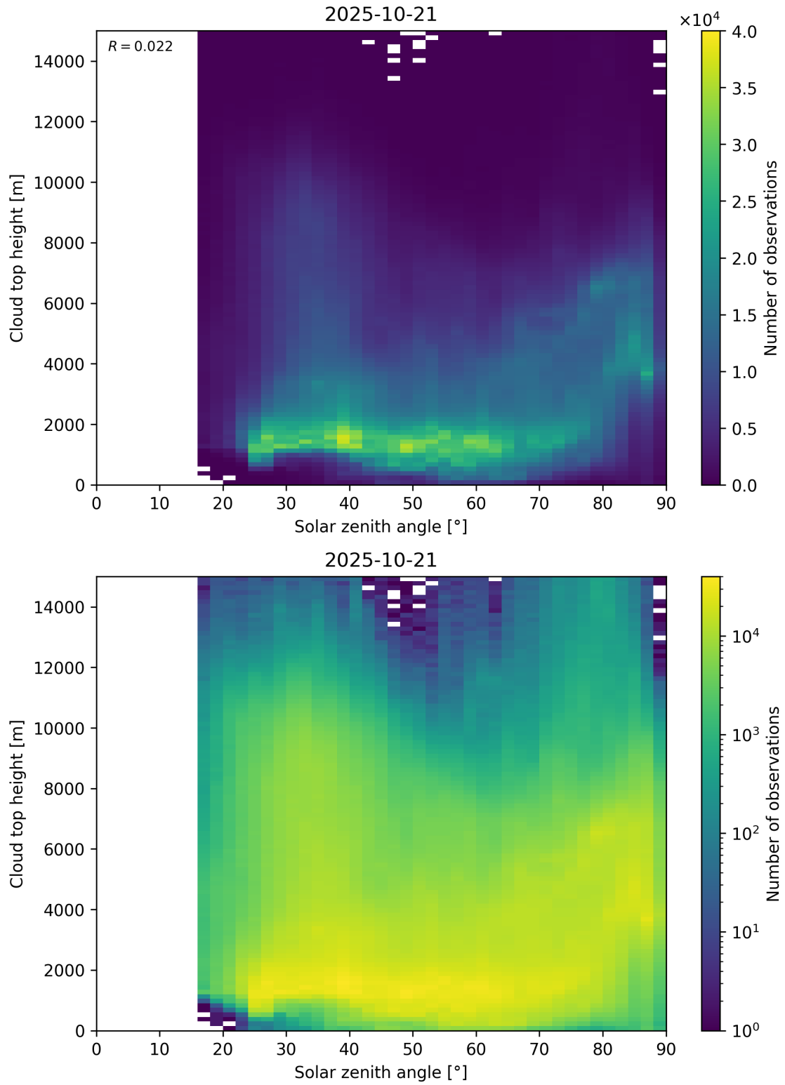
Figure 104: Scatter density plot of “Solar zenith angle” against “Cloud top height” for 2025-10-20 to 2025-10-22.
