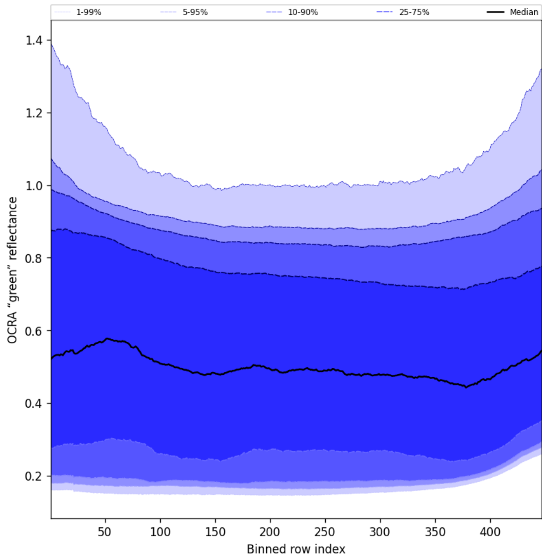
Figure 68: Along track statistics of “OCRA “green” reflectance” for 2025-10-20 to 2025-10-22
