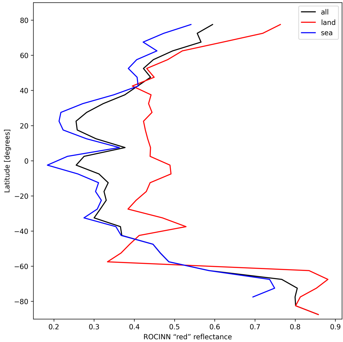
Figure 37: Zonal average of “ROCINN “red” reflectance” for 2025-10-20 to 2025-10-22.
