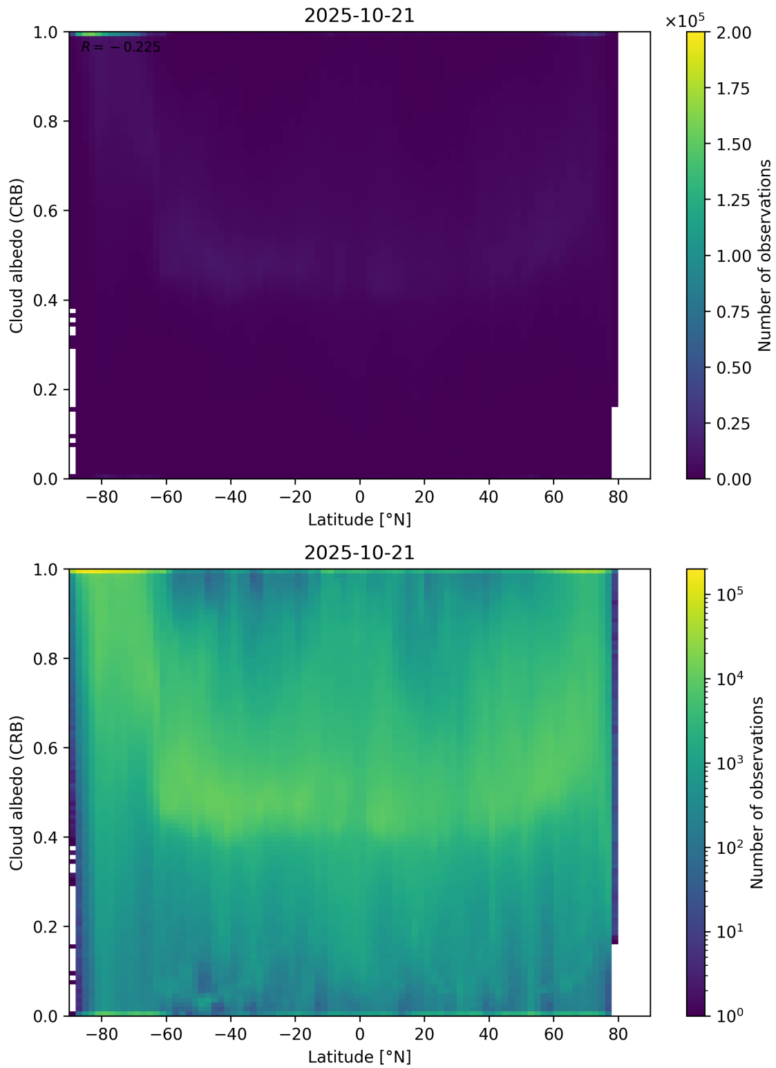
Figure 91: Scatter density plot of “Latitude” against “Cloud albedo (CRB)” for 2025-10-20 to 2025-10-22.
