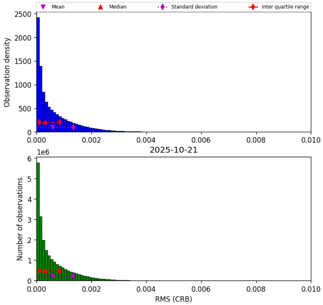
Figure 48: Histogram of “RMS (CRB)” for 2025-10-20 to 2025-10-22
