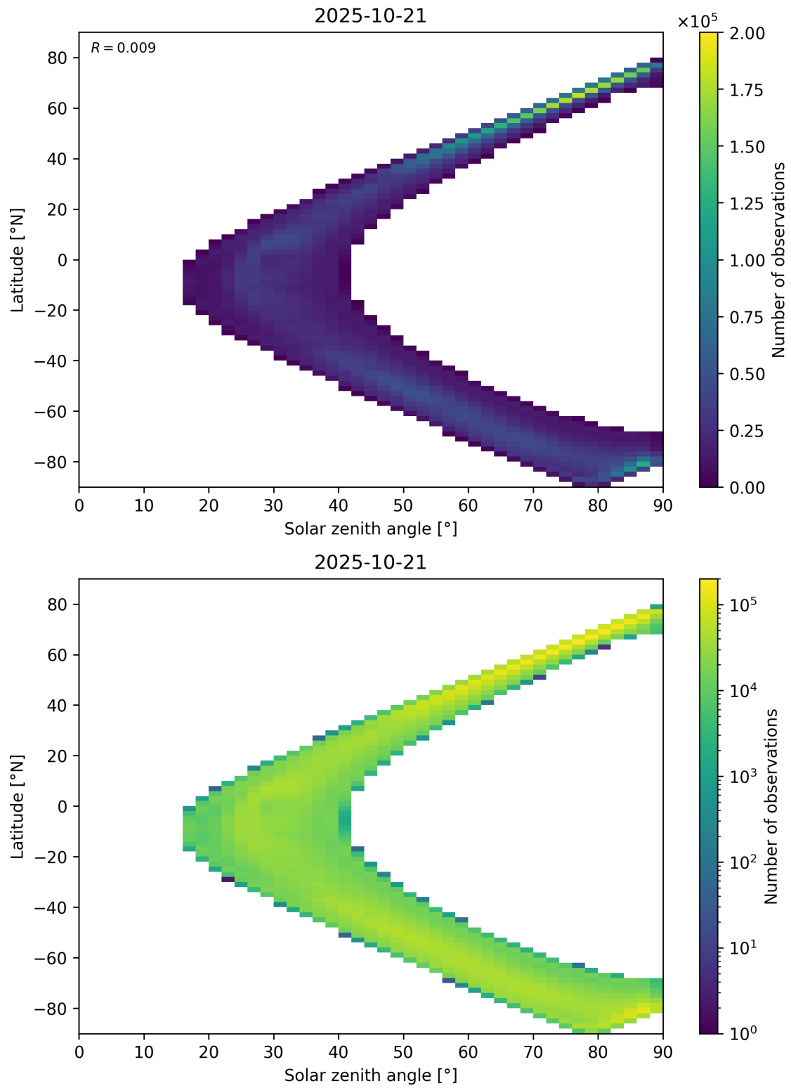
Figure 105: Scatter density plot of “Solar zenith angle” against “Latitude” for 2025-10-20 to 2025-10-22.
