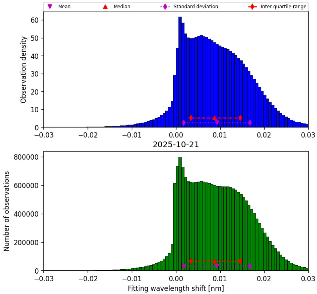
Figure 49: Histogram of “Fitting wavelength shift” for 2025-10-20 to 2025-10-22
