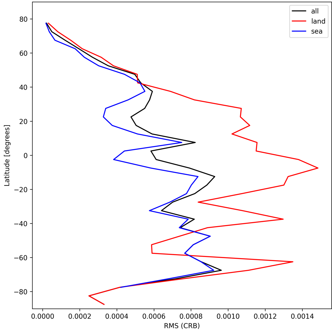
Figure 32: Zonal average of “RMS (CRB)” for 2025-10-20 to 2025-10-22.
