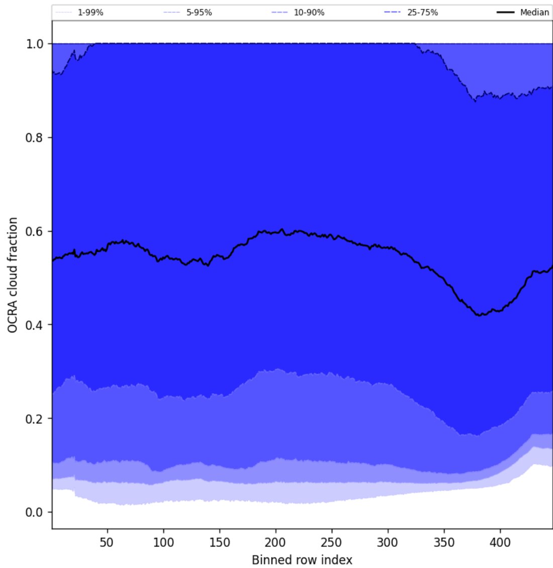
Figure 66: Along track statistics of “OCRA cloud fraction” for 2025-10-20 to 2025-10-22
