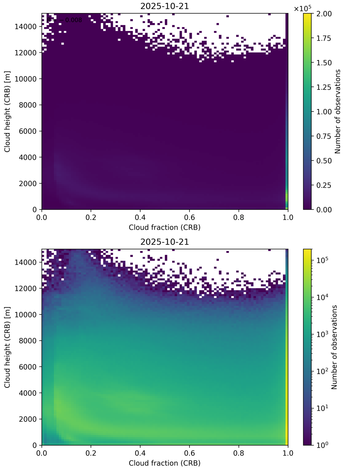
Figure 79: Scatter density plot of “Cloud fraction (CRB)” against “Cloud height (CRB)” for 2025-10-20 to 2025-10-22.
