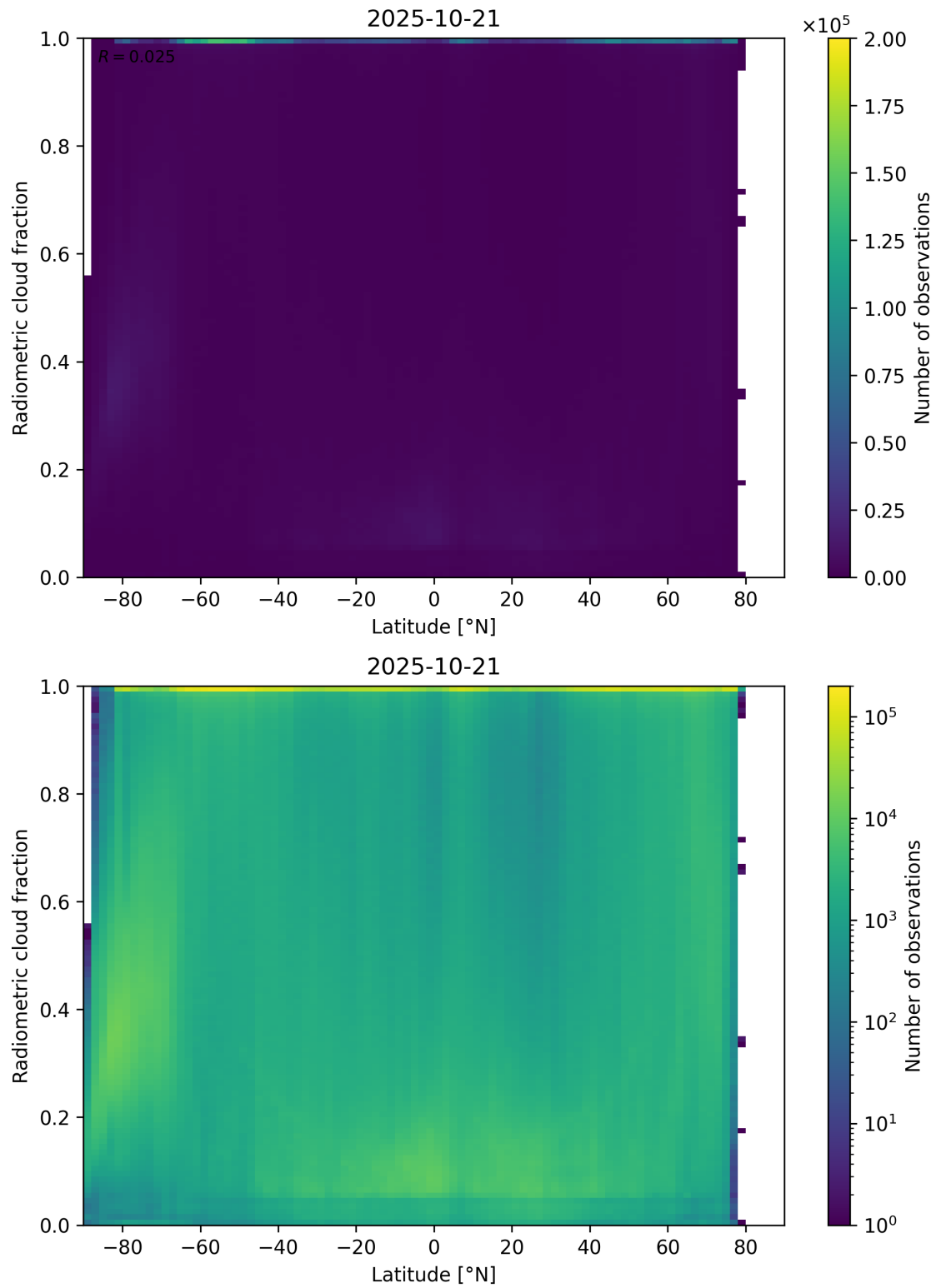
Figure 92: Scatter density plot of “Latitude” against “Radiometric cloud fraction” for 2025-10-20 to 2025-10-22.
