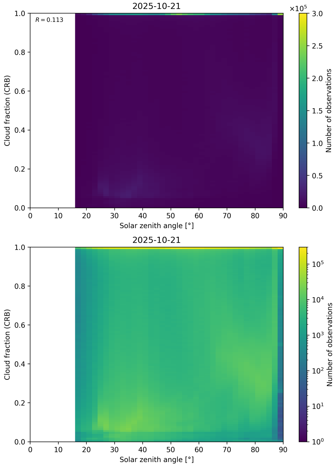
Figure 101: Scatter density plot of “Solar zenith angle” against “Cloud fraction (CRB)” for 2025-10-20 to 2025-10-22.
