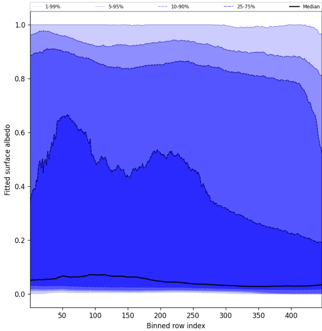
Figure 61: Along track statistics of “Fitted surface albedo” for 2025-10-20 to 2025-10-22
