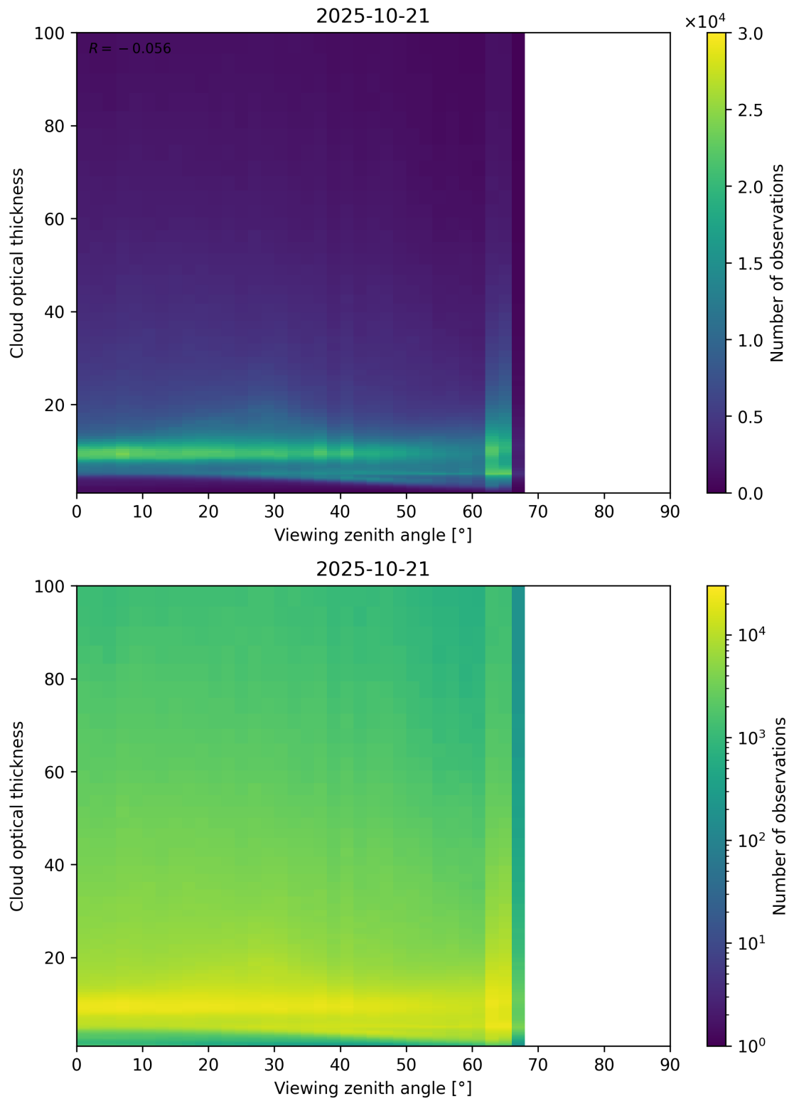
Figure 111: Scatter density plot of “Viewing zenith angle” against “Cloud optical thickness” for 2025-10-20 to 2025-10-22.
