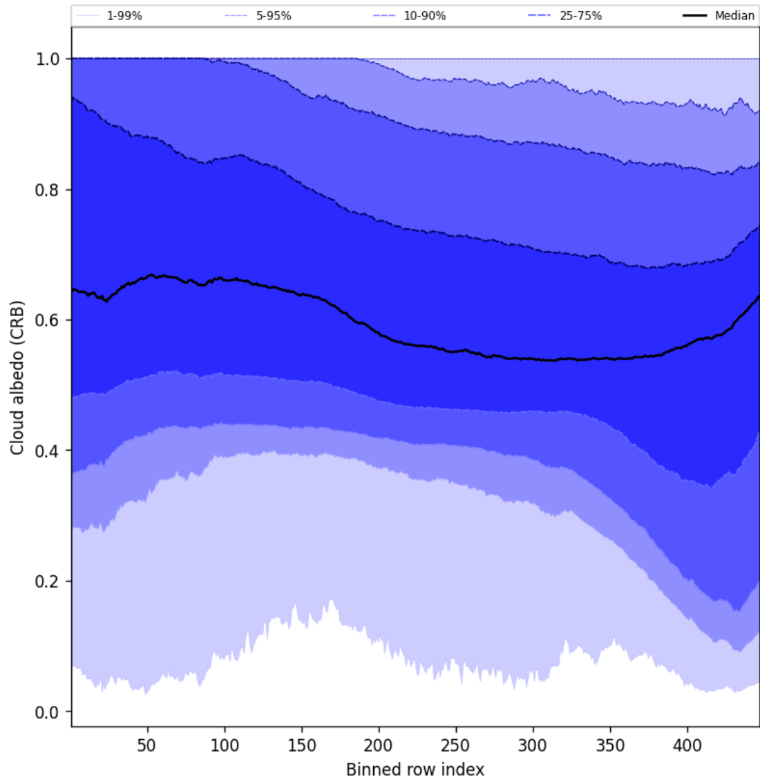
Figure 60: Along track statistics of “Cloud albedo (CRB)” for 2025-10-20 to 2025-10-22
