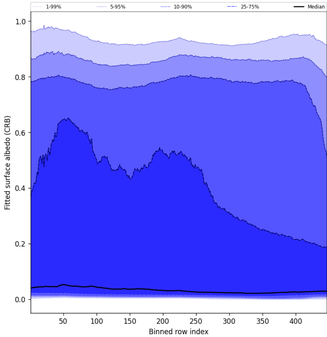
Figure 62: Along track statistics of “Fitted surface albedo (CRB)” for 2025-10-20 to 2025-10-22
