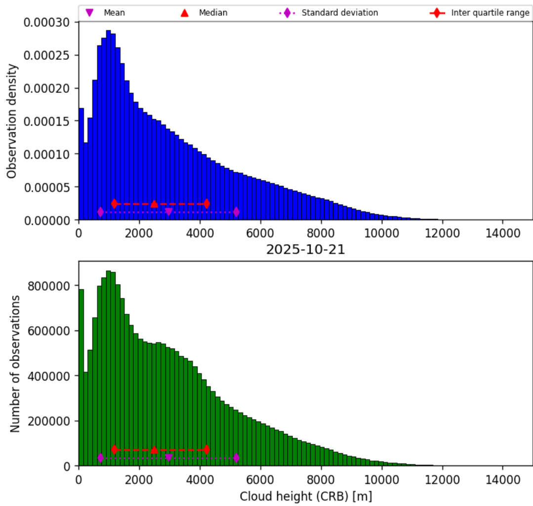
Figure 43: Histogram of “Cloud height (CRB)” for 2025-10-20 to 2025-10-22
