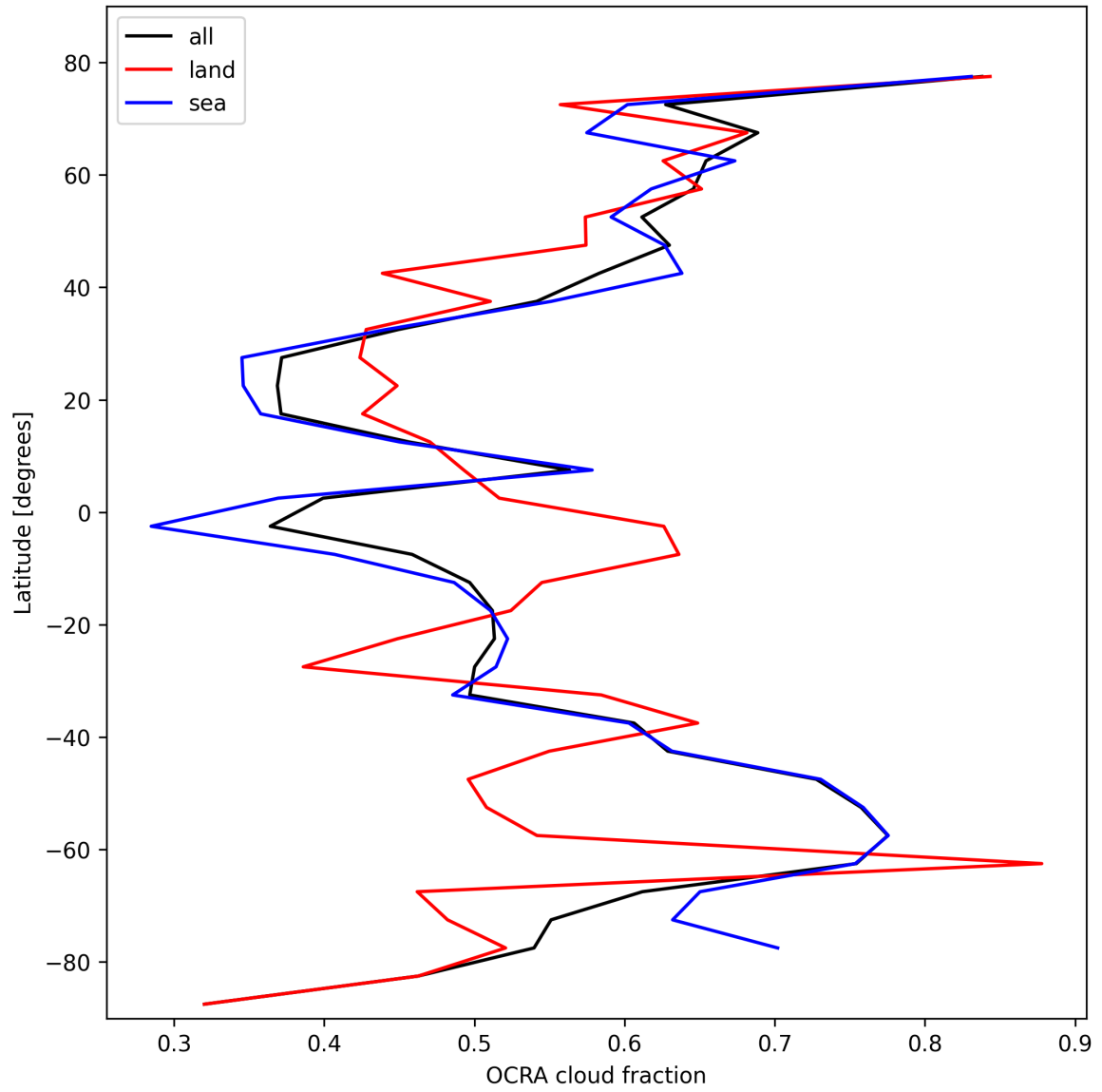
Figure 34: Zonal average of “OCRA cloud fraction” for 2025-10-20 to 2025-10-22.
