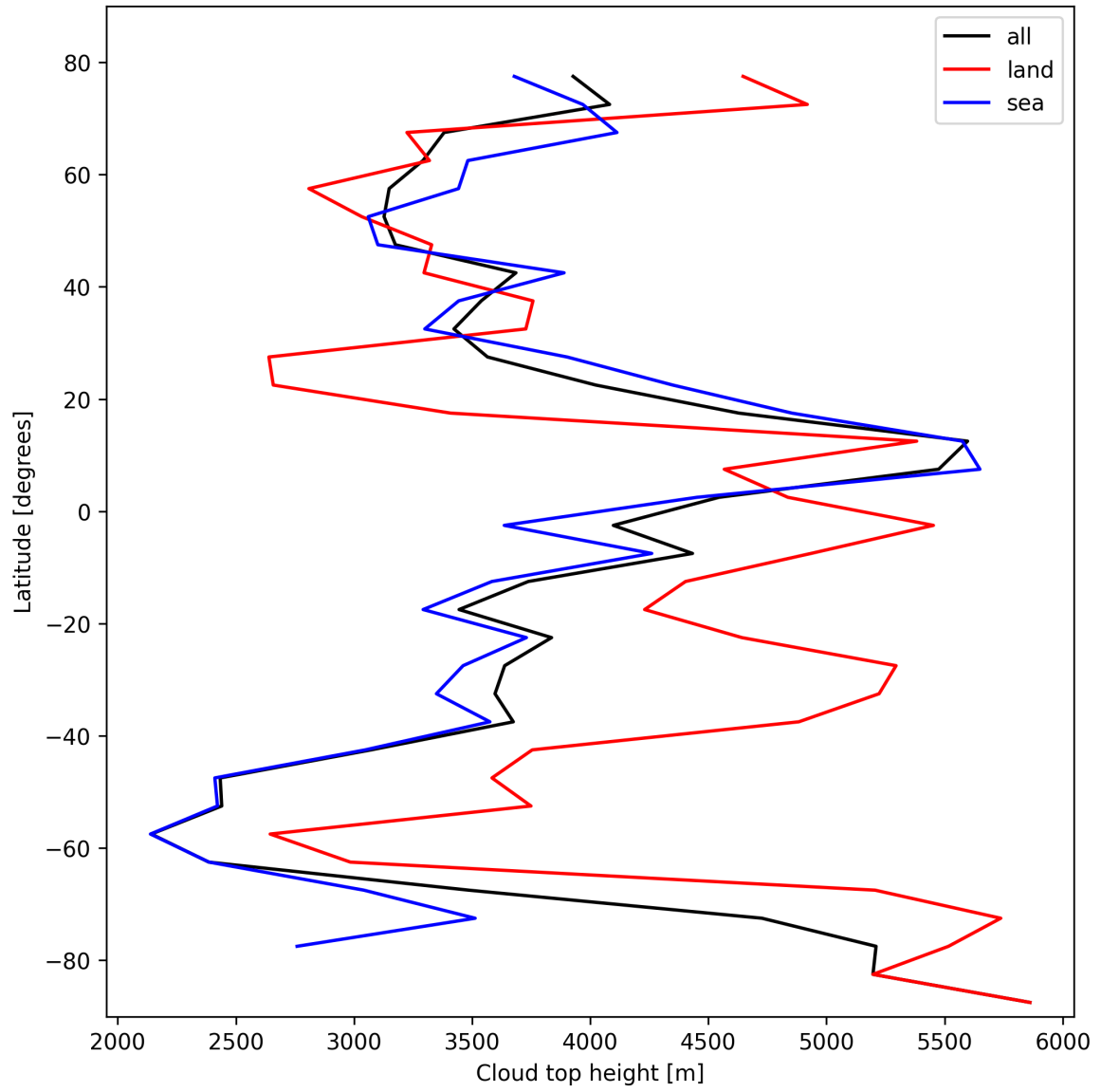
Figure 24: Zonal average of “Cloud top height” for 2025-10-20 to 2025-10-22.
