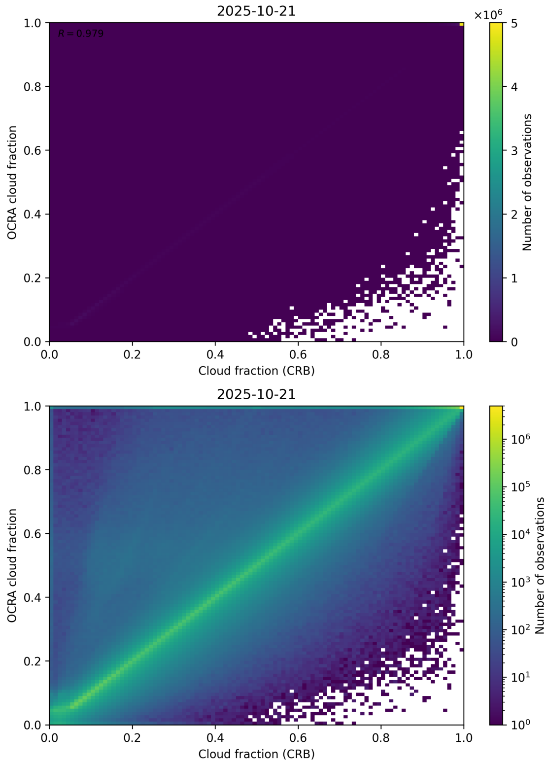
Figure 78: Scatter density plot of “Cloud fraction (CRB)” against “OCRA cloud fraction” for 2025-10-20 to 2025-10-22.
