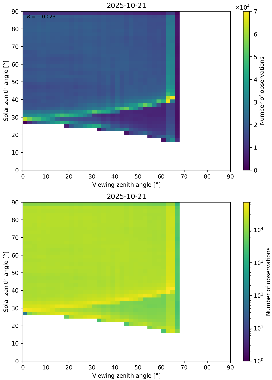
Figure 114: Scatter density plot of “Viewing zenith angle” against “Solar zenith angle” for 2025-10-20 to 2025-10-22.
