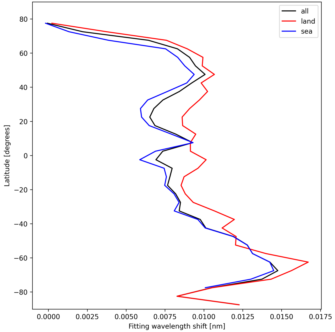
Figure 33: Zonal average of “Fitting wavelength shift” for 2025-10-20 to 2025-10-22.
