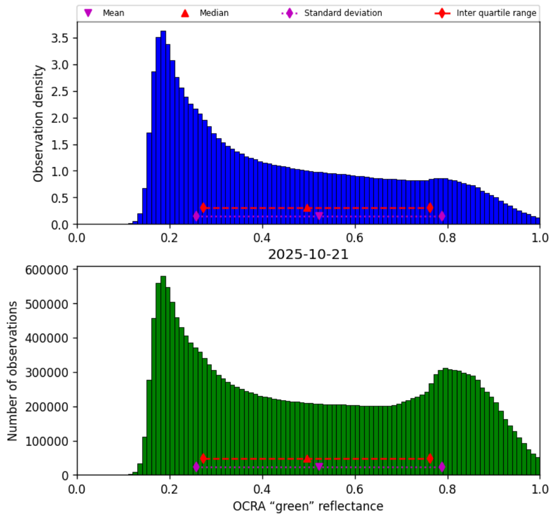
Figure 52: Histogram of “OCRA “green” reflectance” for 2025-10-20 to 2025-10-22
