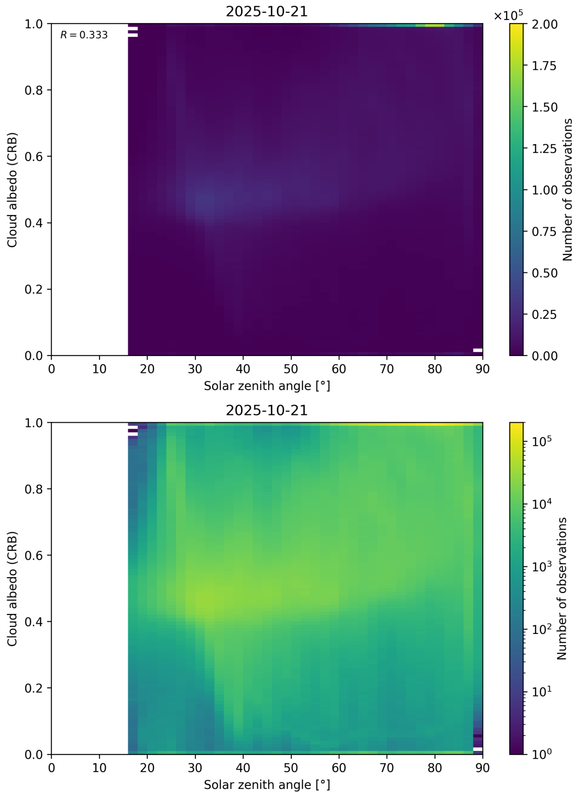
Figure 98: Scatter density plot of “Solar zenith angle” against “Cloud albedo (CRB)” for 2025-10-20 to 2025-10-22.
