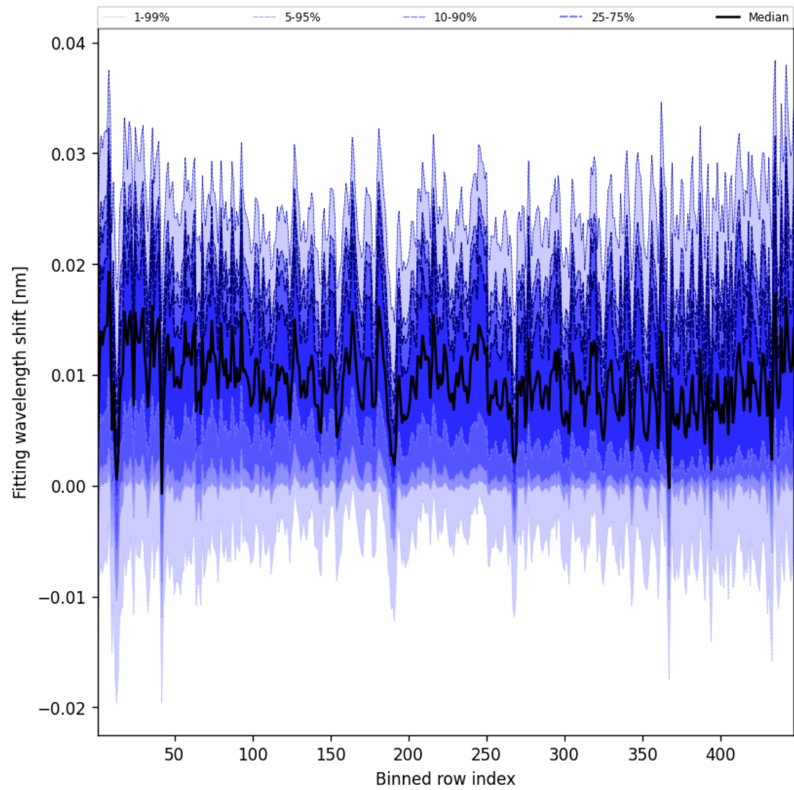
Figure 65: Along track statistics of “Fitting wavelength shift” for 2025-10-20 to 2025-10-22
