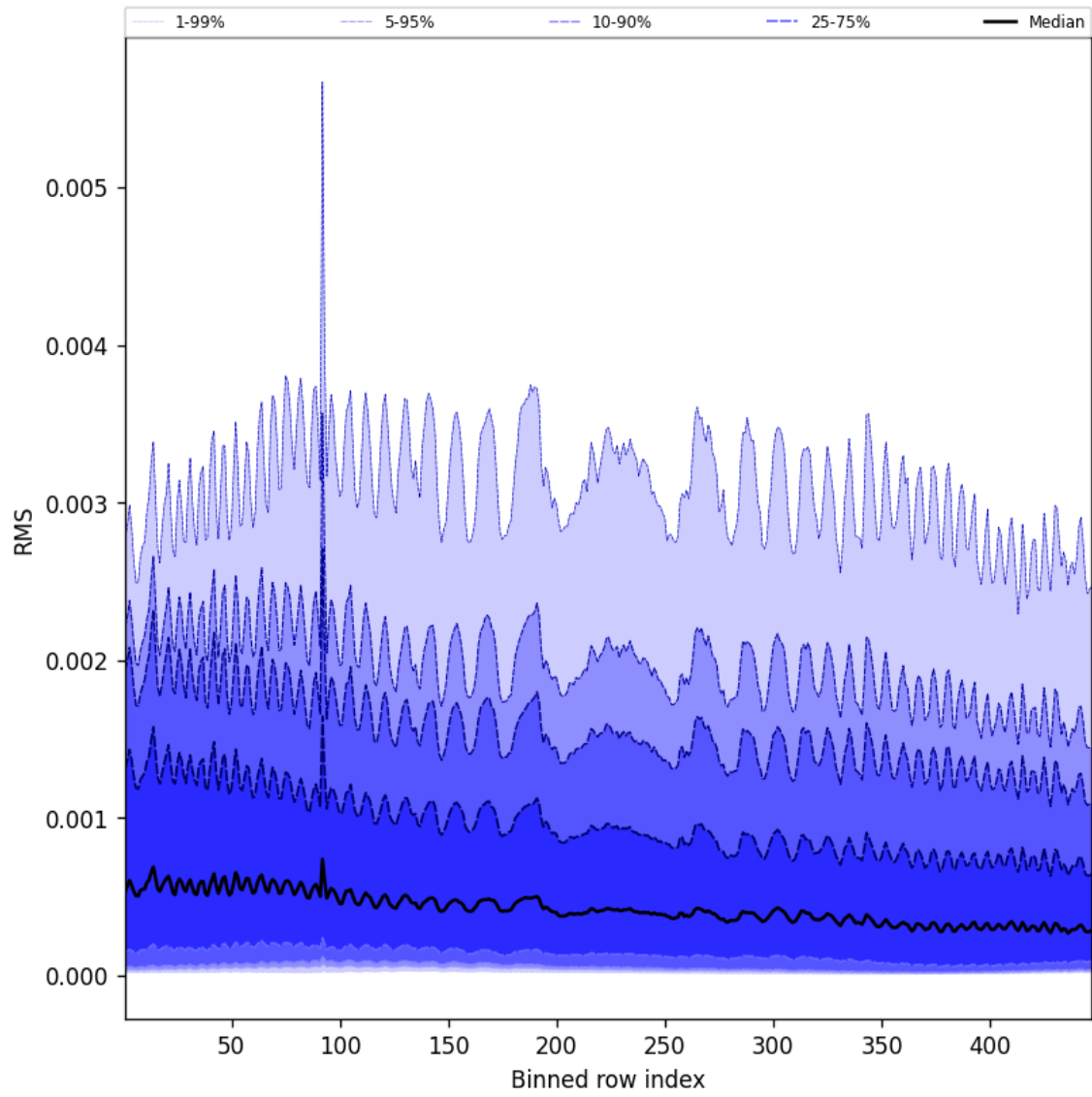
Figure 63: Along track statistics of “RMS” for 2025-10-20 to 2025-10-22
