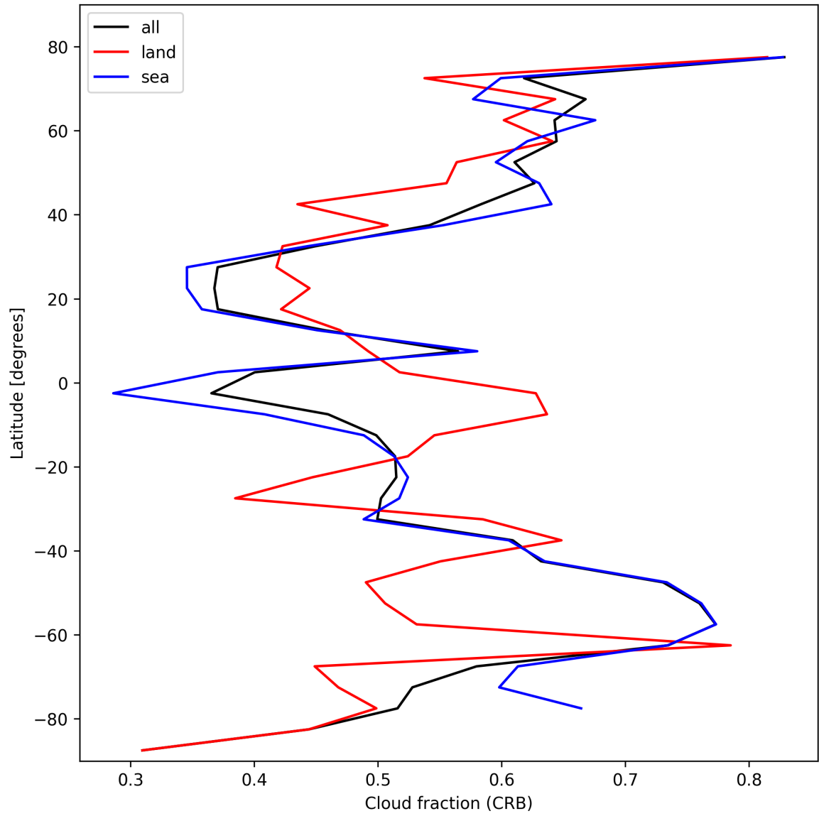
Figure 26: Zonal average of “Cloud fraction (CRB)” for 2025-10-20 to 2025-10-22.
