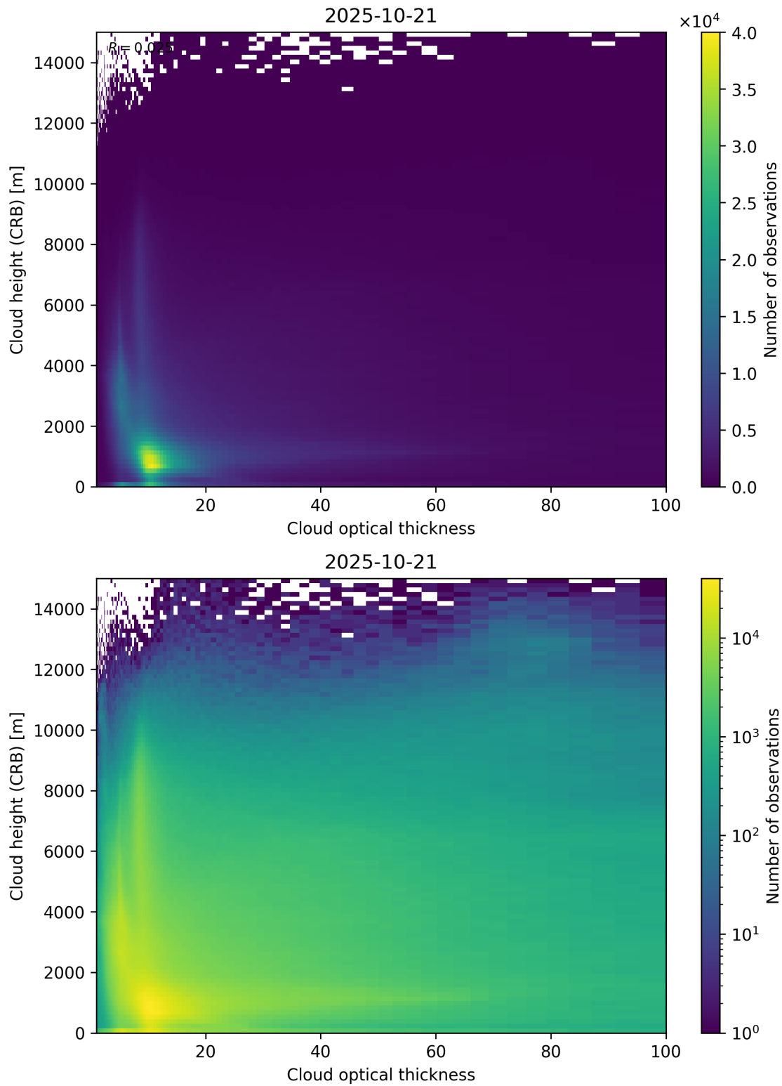
Figure 85: Scatter density plot of “Cloud optical thickness” against “Cloud height (CRB)” for 2025-10-20 to 2025-10-22.
