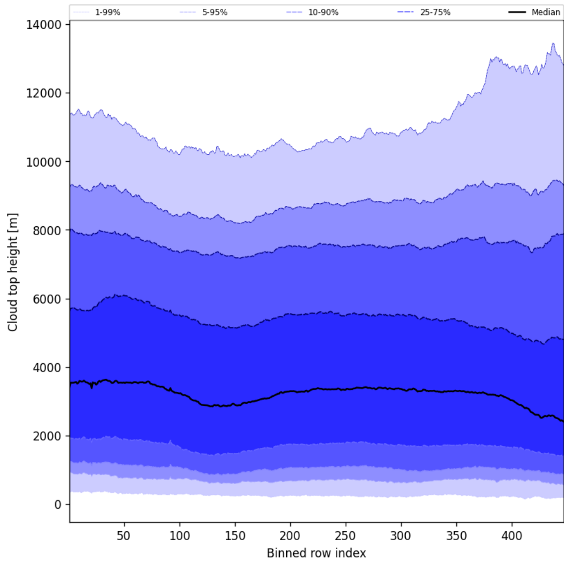
Figure 56: Along track statistics of “Cloud top height” for 2025-10-20 to 2025-10-22
