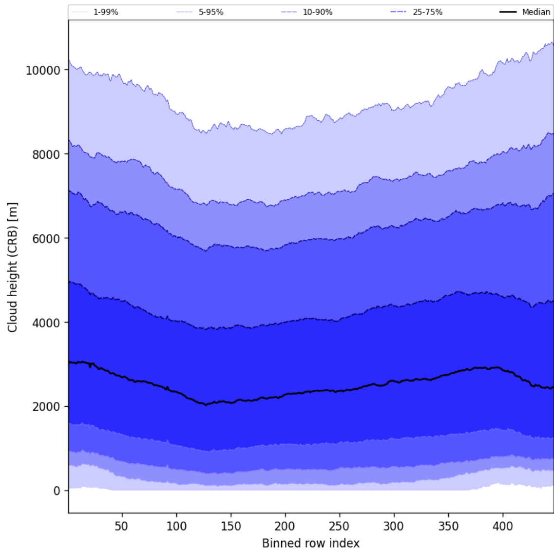
Figure 59: Along track statistics of “Cloud height (CRB)” for 2025-10-22 to 2025-10-23
