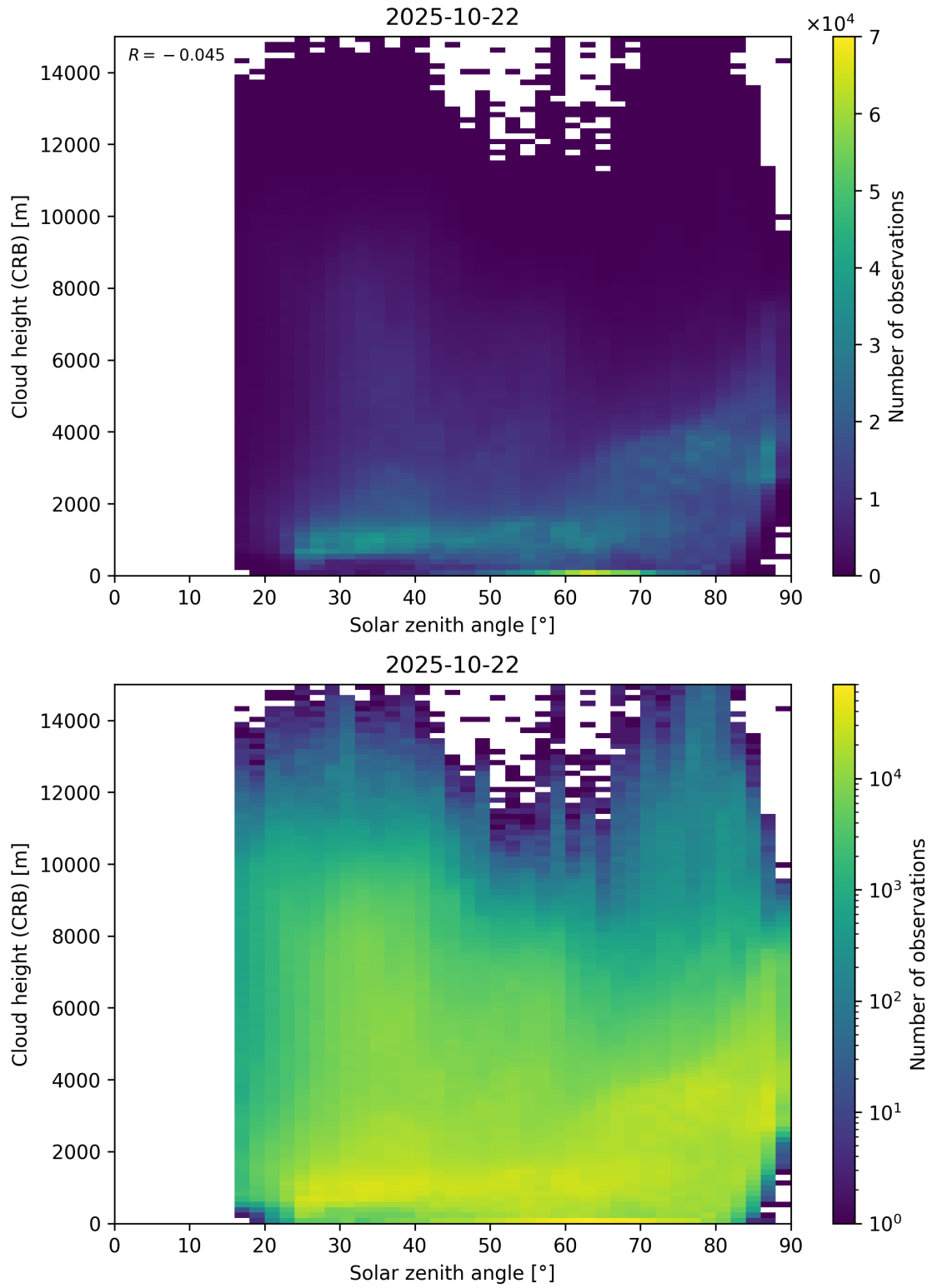
Figure 102: Scatter density plot of “Solar zenith angle” against “Cloud height (CRB)” for 2025-10-22 to 2025-10-23.
