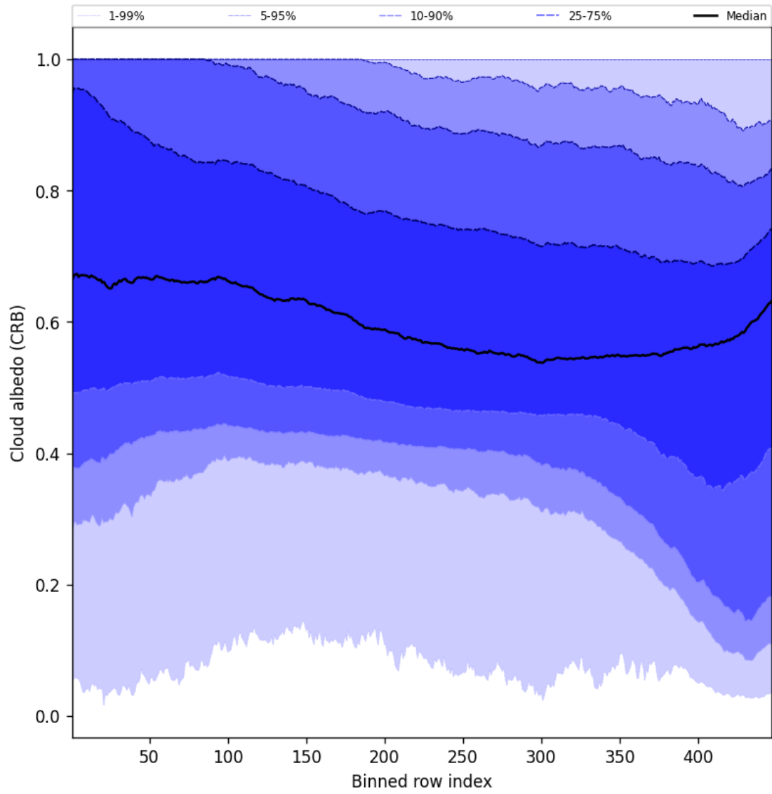
Figure 60: Along track statistics of “Cloud albedo (CRB)” for 2025-10-22 to 2025-10-23
