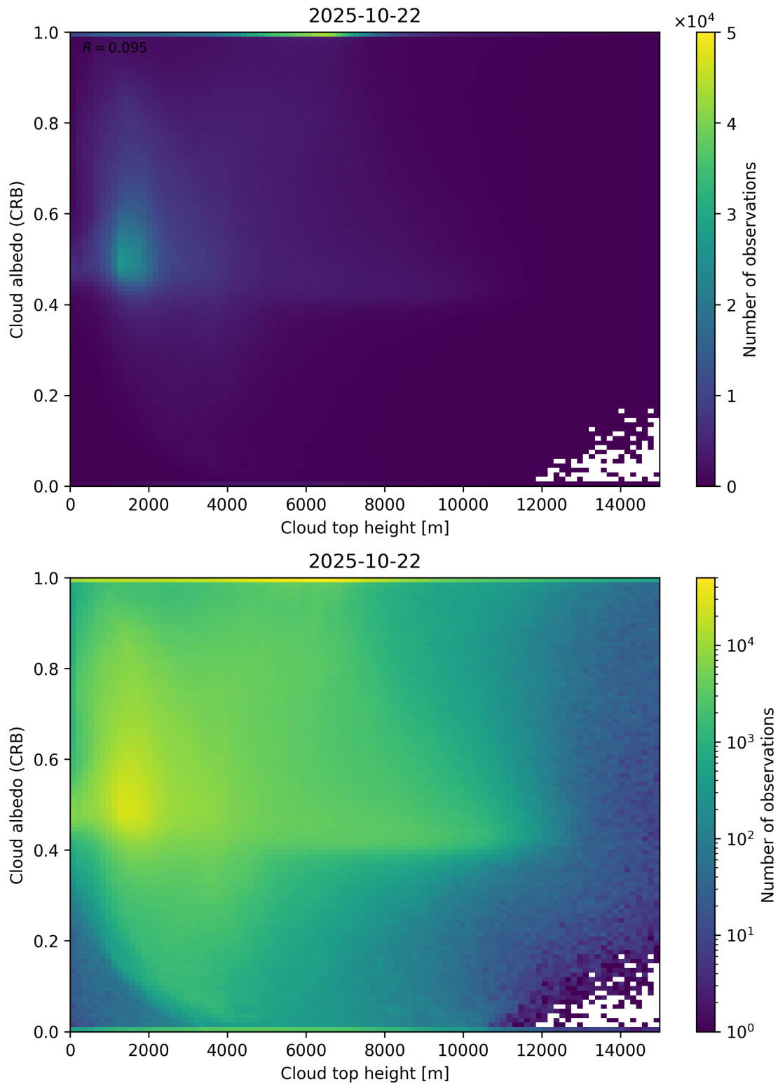
Figure 86: Scatter density plot of “Cloud top height” against “Cloud albedo (CRB)” for 2025-10-22 to 2025-10-23.
