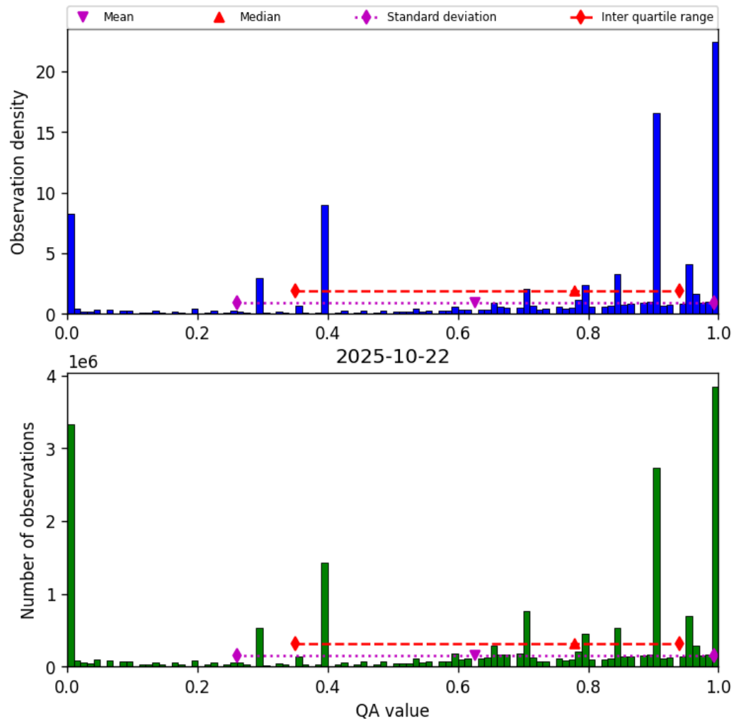
Figure 38: Histogram of “QA value” for 2025-10-22 to 2025-10-23
