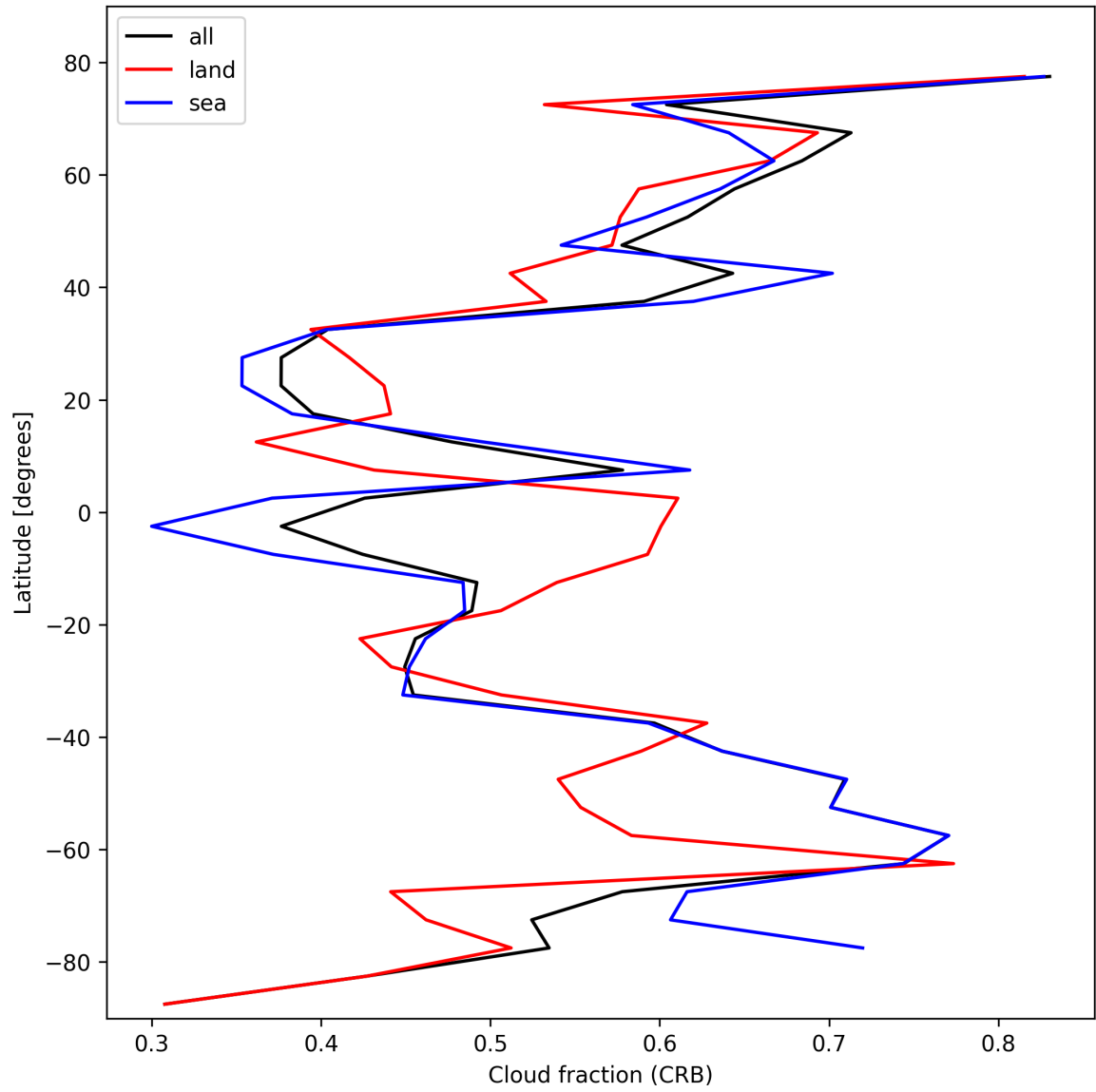
Figure 26: Zonal average of “Cloud fraction (CRB)” for 2025-10-22 to 2025-10-23.
