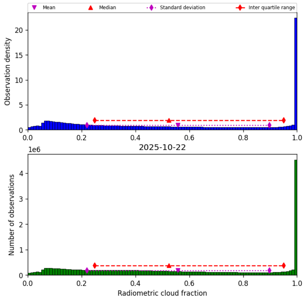
Figure 39: Histogram of “Radiometric cloud fraction” for 2025-10-22 to 2025-10-23
