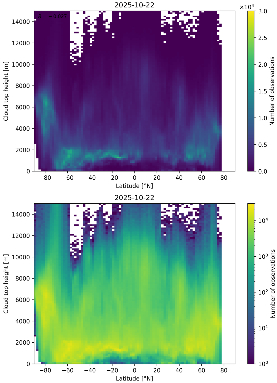
Figure 97: Scatter density plot of “Latitude” against “Cloud top height” for 2025-10-22 to 2025-10-23.
