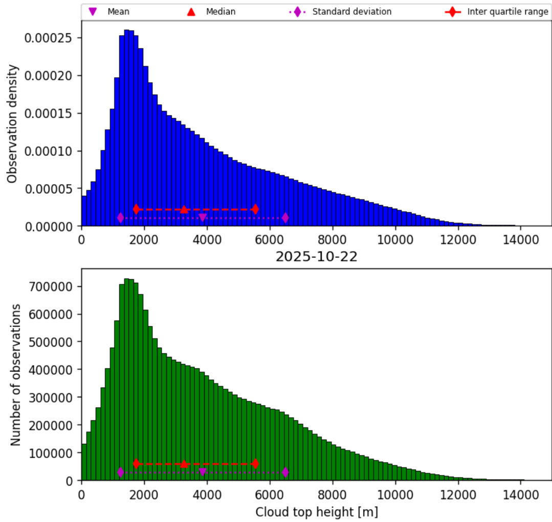
Figure 40: Histogram of “Cloud top height” for 2025-10-22 to 2025-10-23
