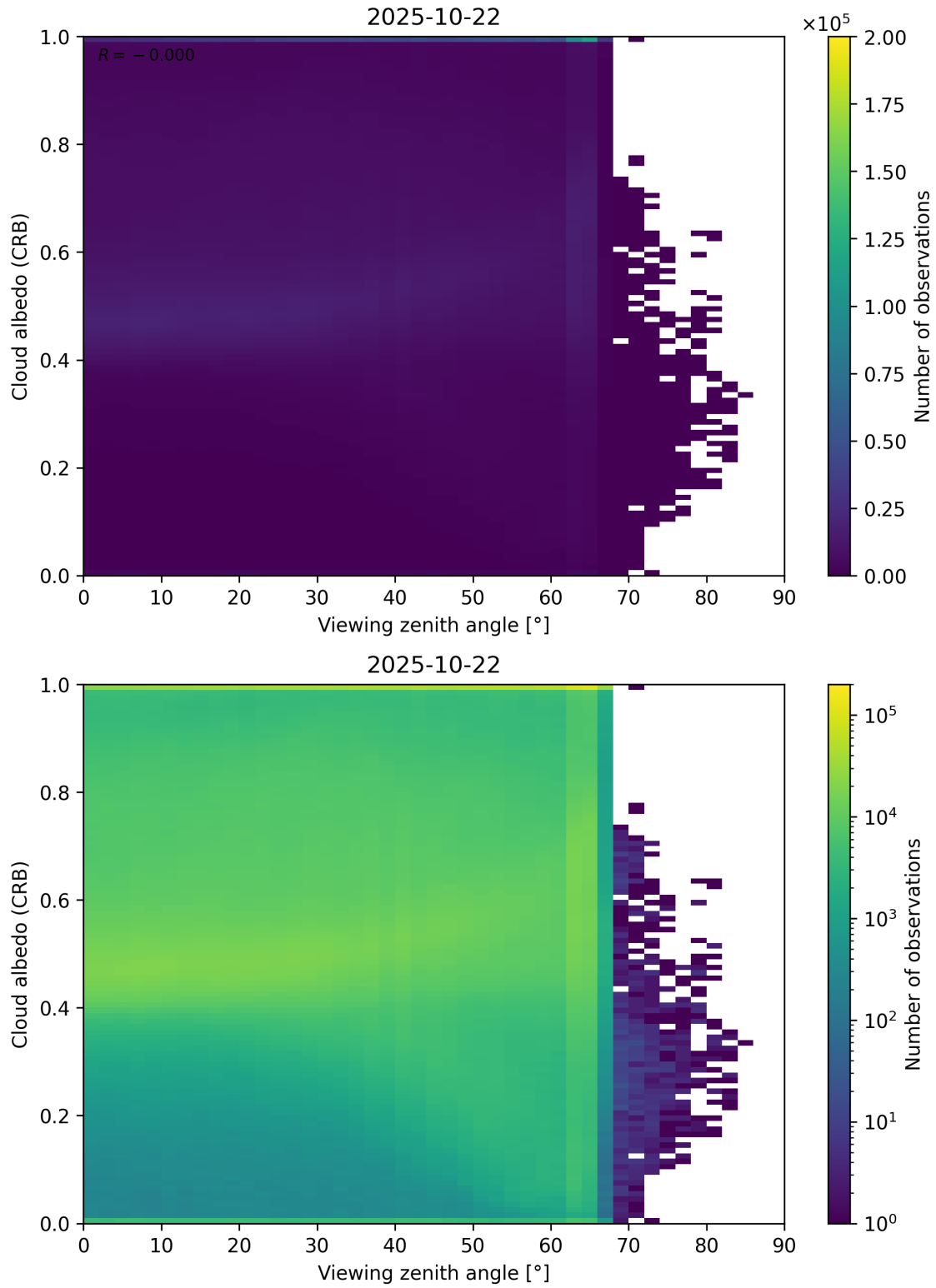
Figure 106: Scatter density plot of “Viewing zenith angle” against “Cloud albedo (CRB)” for 2025-10-22 to 2025-10-23.
