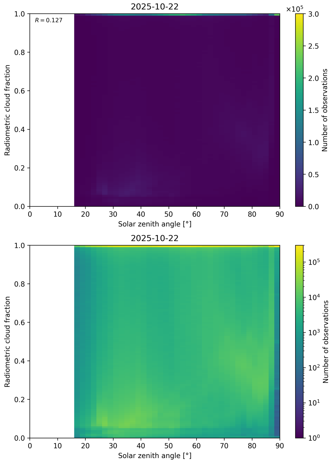
Figure 99: Scatter density plot of “Solar zenith angle” against “Radiometric cloud fraction” for 2025-10-22 to 2025-10-23.
