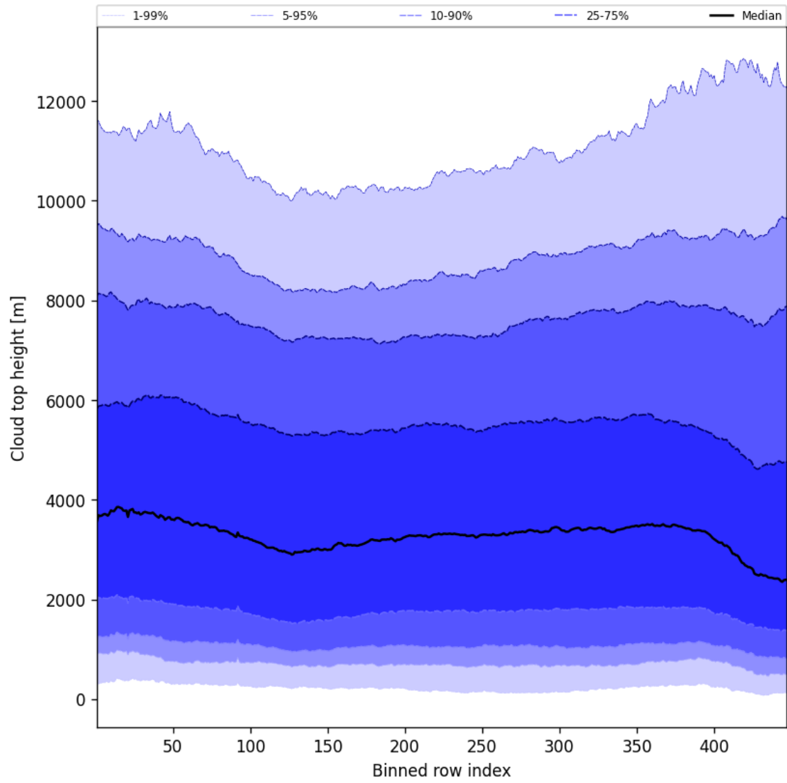
Figure 56: Along track statistics of “Cloud top height” for 2025-10-22 to 2025-10-23
