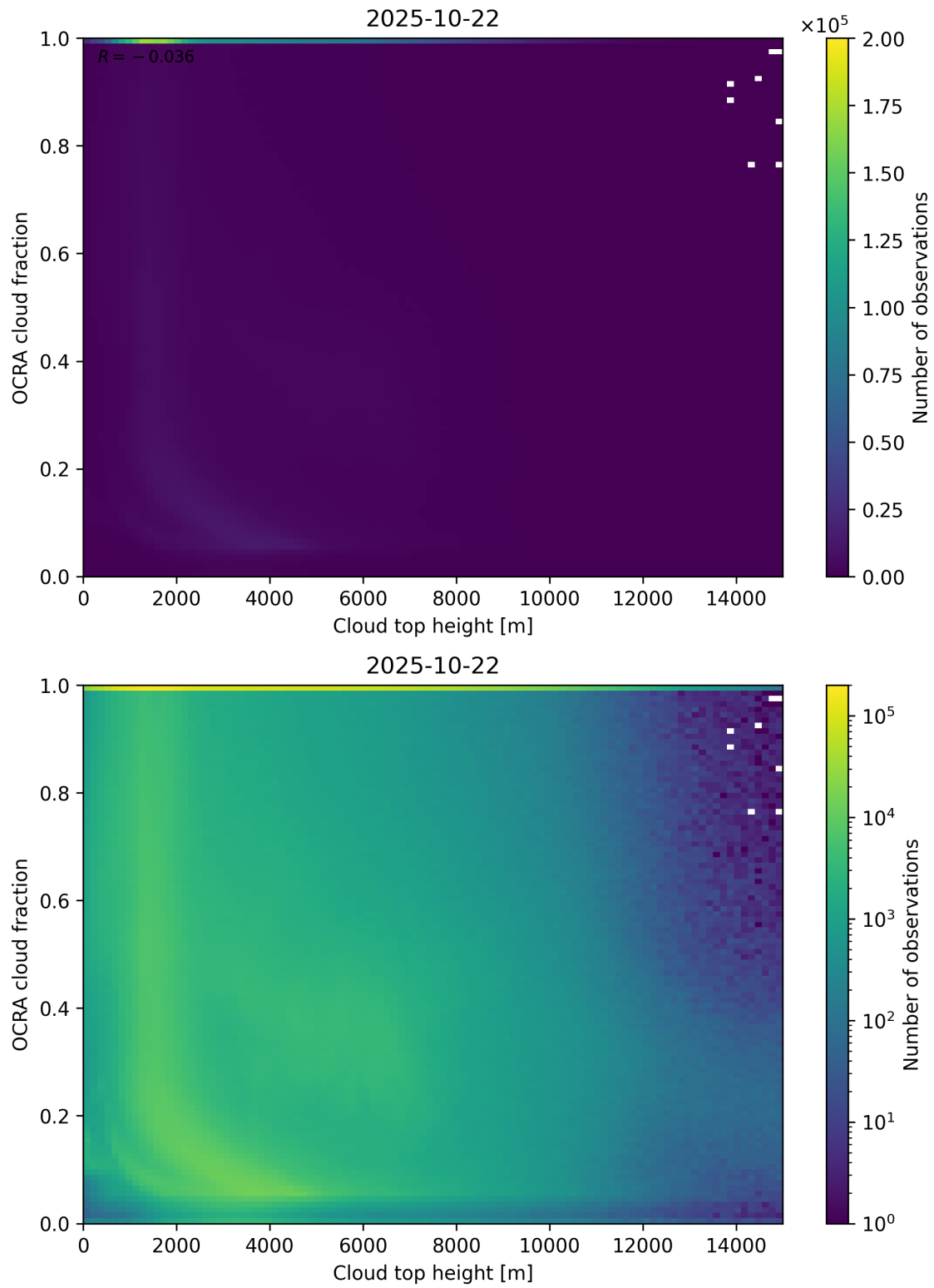
Figure 87: Scatter density plot of “Cloud top height” against “OCRA cloud fraction” for 2025-10-22 to 2025-10-23.
