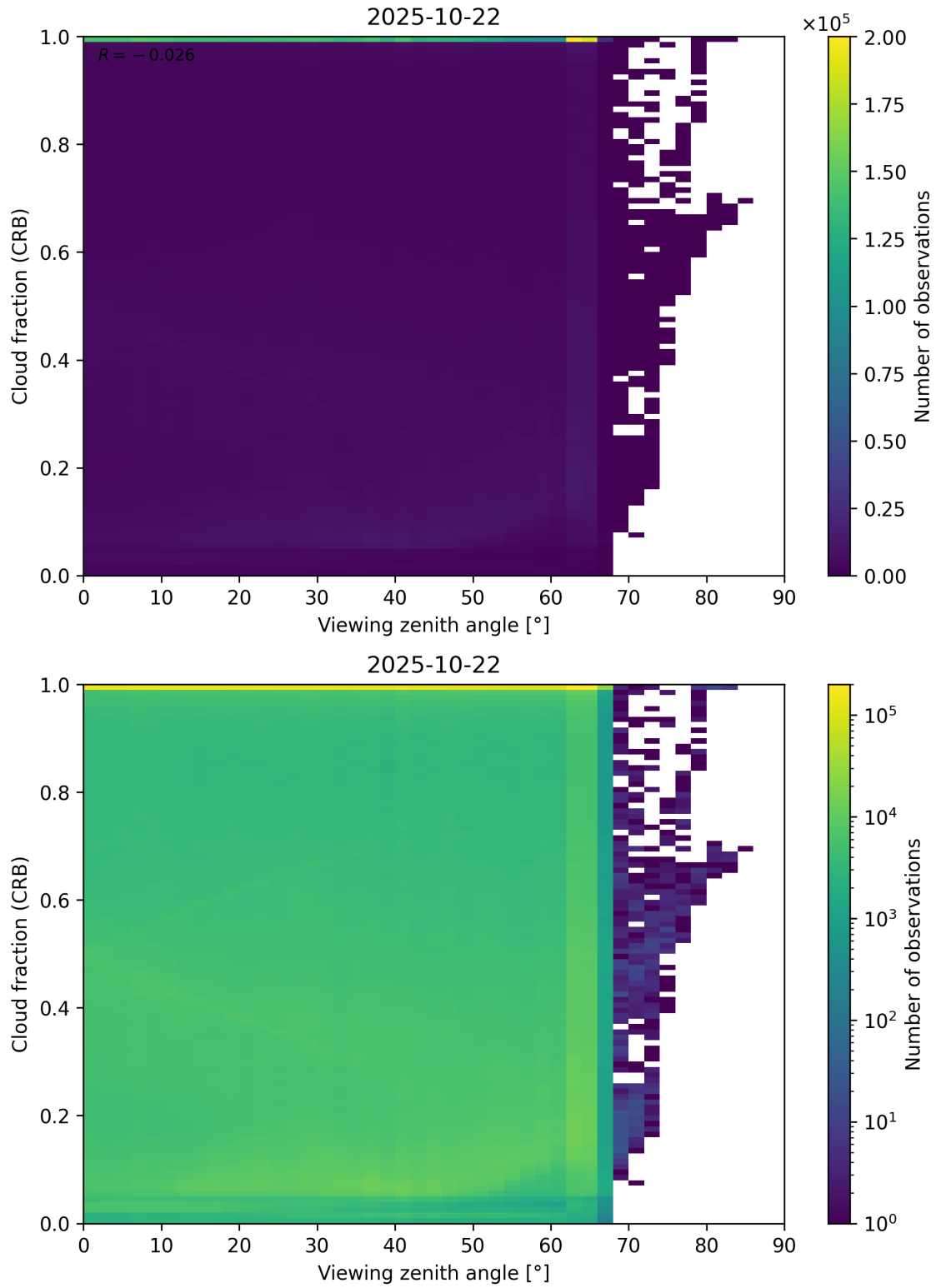
Figure 109: Scatter density plot of “Viewing zenith angle” against “Cloud fraction (CRB)” for 2025-10-22 to 2025-10-23.
