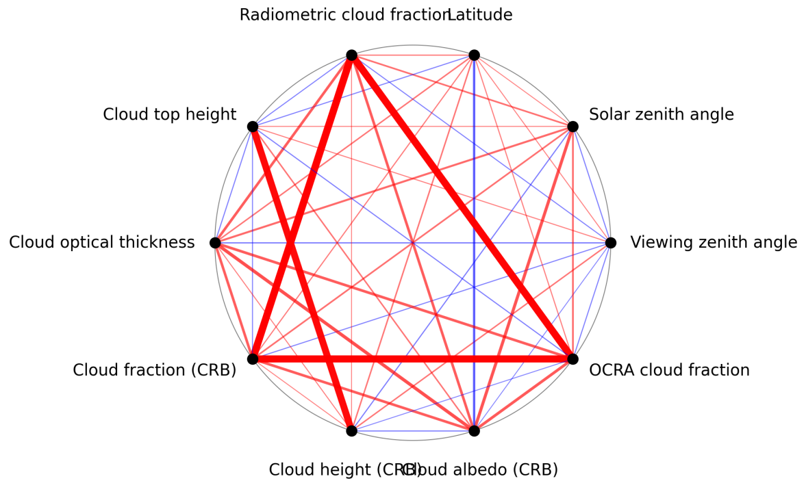
Figure 1: Map of correlation graph for 2025-10-22 to 2025-10-23.
