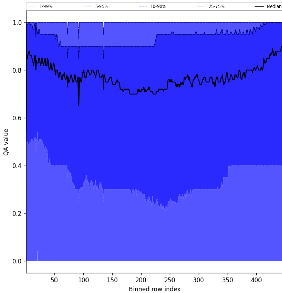
Figure 54: Along track statistics of “QA value” for 2025-10-22 to 2025-10-23
