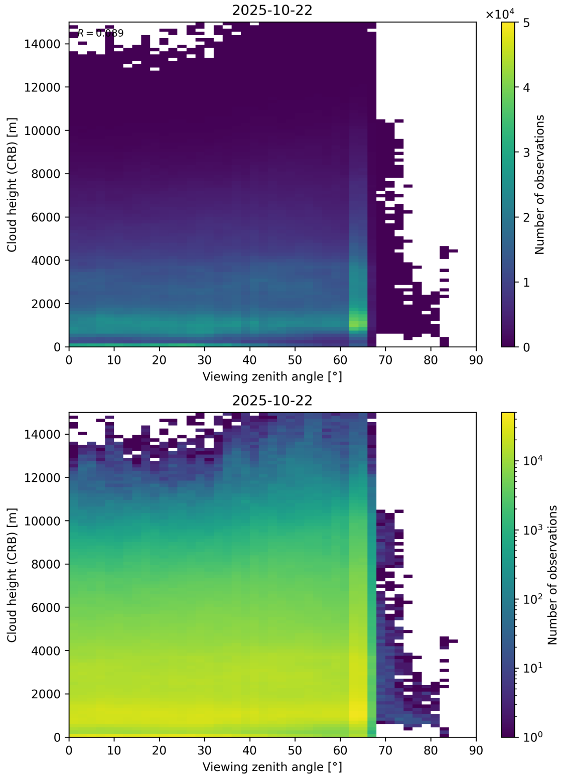
Figure 110: Scatter density plot of “Viewing zenith angle” against “Cloud height (CRB)” for 2025-10-22 to 2025-10-23.
