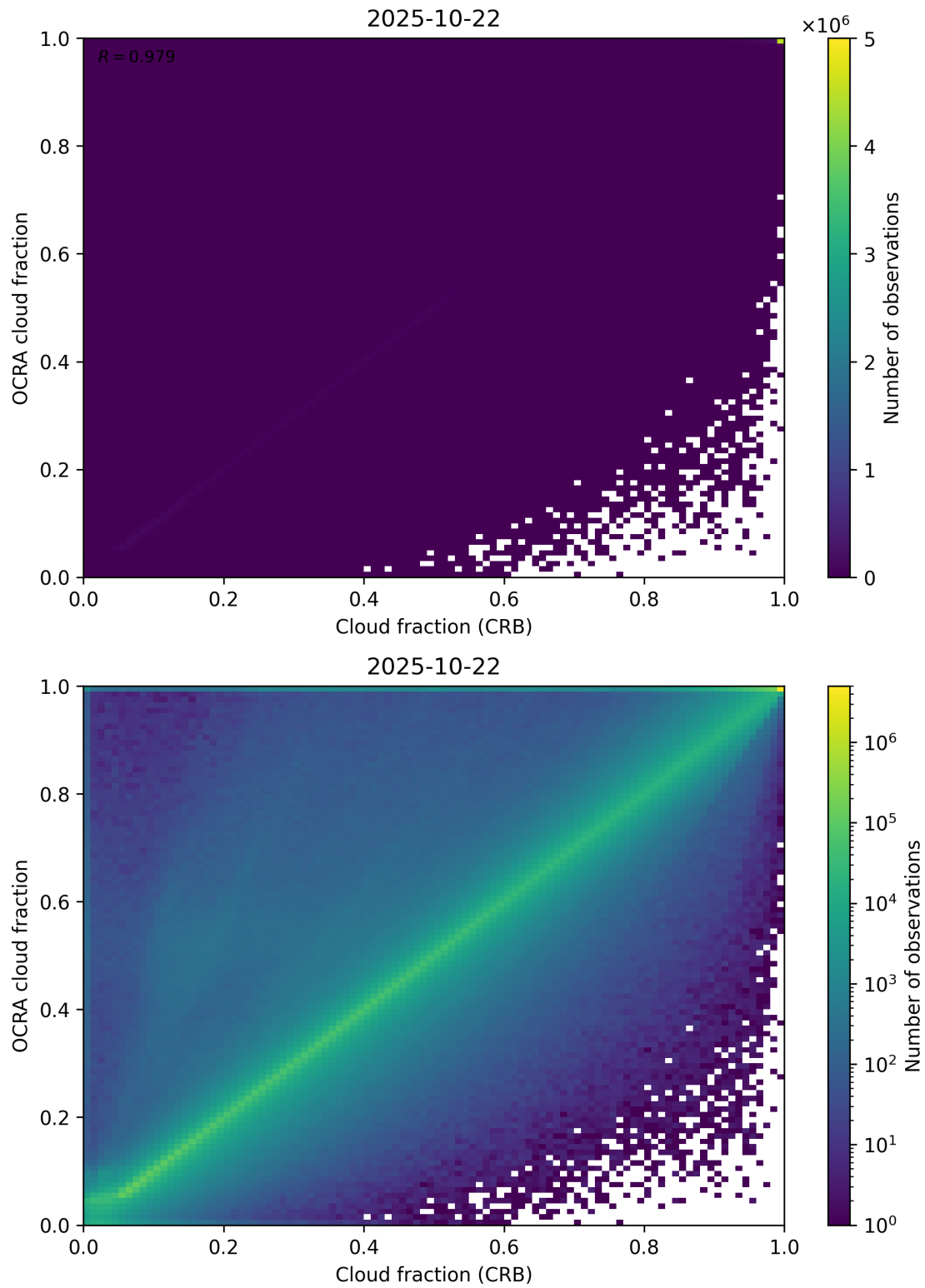
Figure 78: Scatter density plot of “Cloud fraction (CRB)” against “OCRA cloud fraction” for 2025-10-22 to 2025-10-23.
