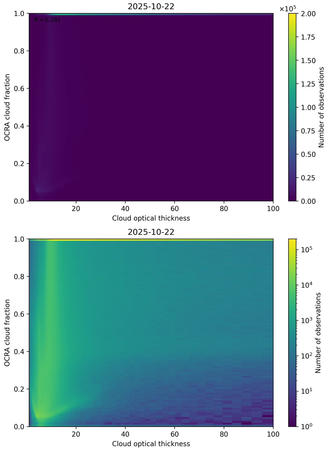
Figure 83: Scatter density plot of “Cloud optical thickness” against “OCRA cloud fraction” for 2025-10-22 to 2025-10-23.
