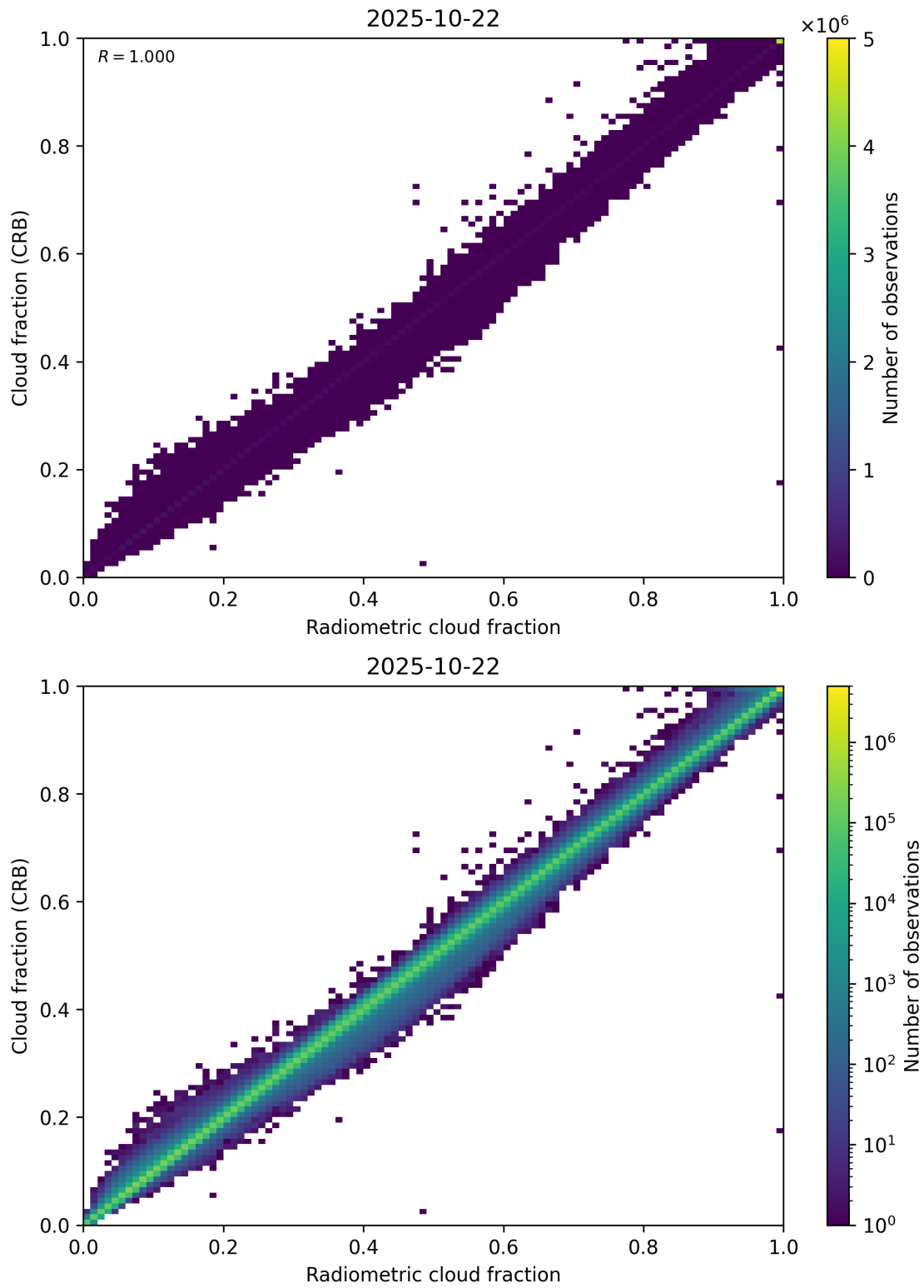
Figure 73: Scatter density plot of “Radiometric cloud fraction” against “Cloud fraction (CRB)” for 2025-10-22 to 2025-10-23.
