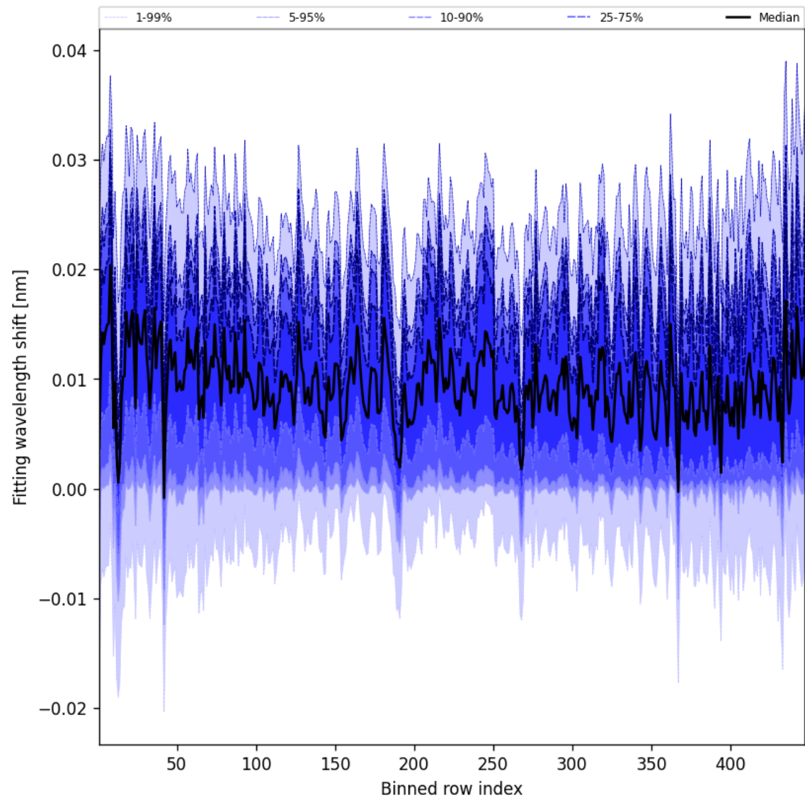
Figure 65: Along track statistics of “Fitting wavelength shift” for 2025-10-22 to 2025-10-23
