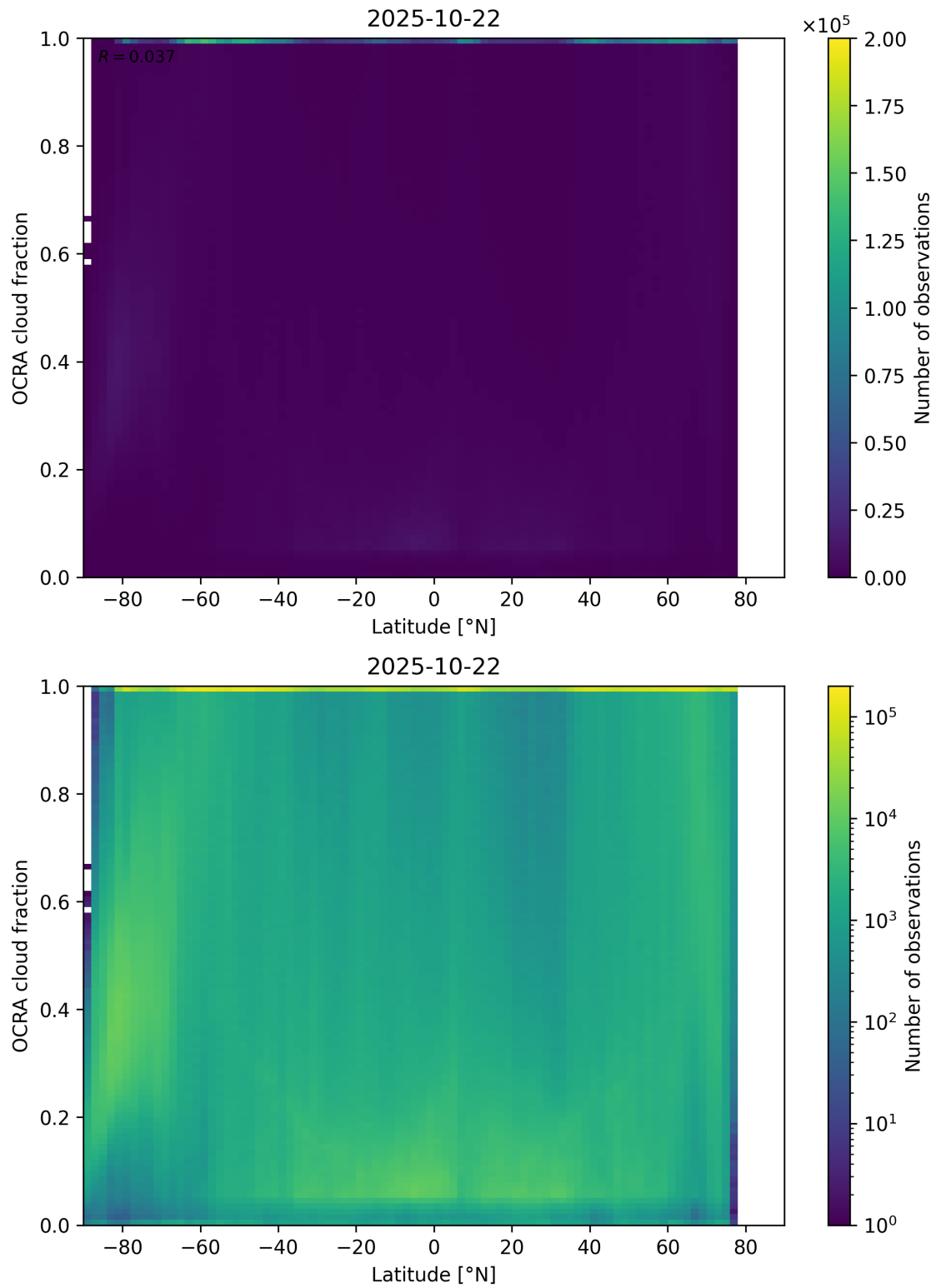
Figure 93: Scatter density plot of “Latitude” against “OCRA cloud fraction” for 2025-10-22 to 2025-10-23.
