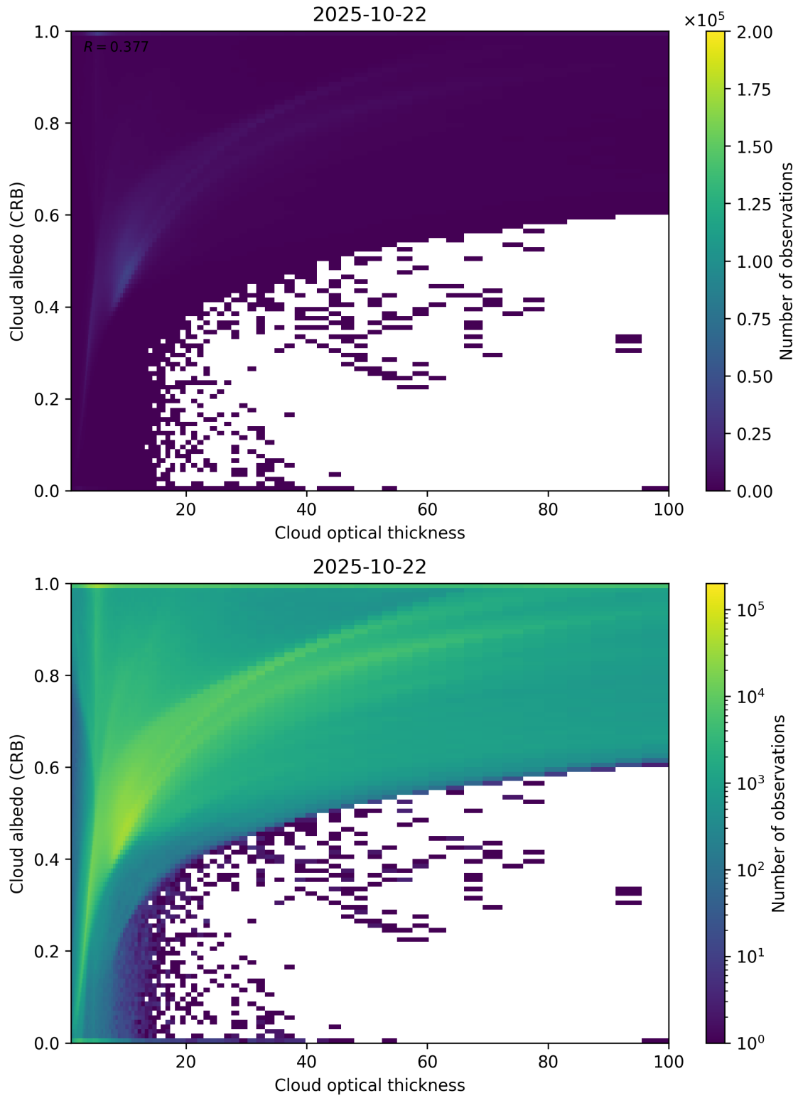
Figure 82: Scatter density plot of “Cloud optical thickness” against “Cloud albedo (CRB)” for 2025-10-22 to 2025-10-23.
