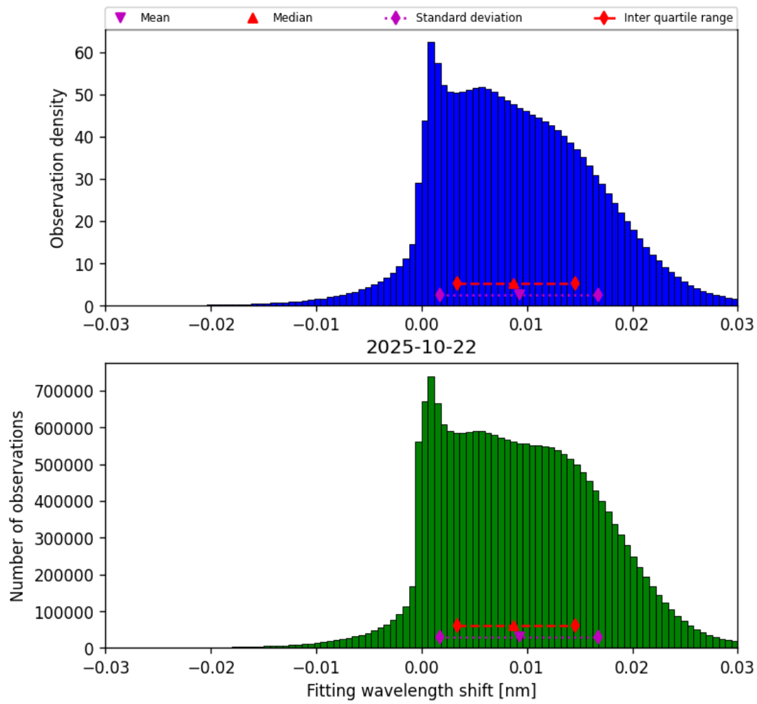
Figure 49: Histogram of “Fitting wavelength shift” for 2025-10-22 to 2025-10-23
