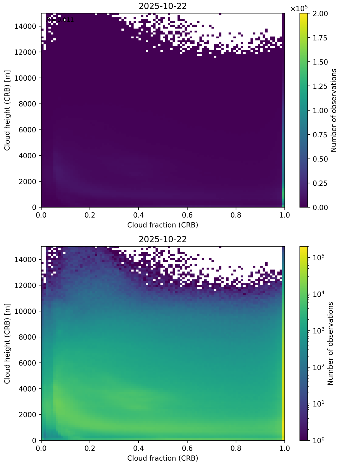
Figure 79: Scatter density plot of “Cloud fraction (CRB)” against “Cloud height (CRB)” for 2025-10-22 to 2025-10-23.
