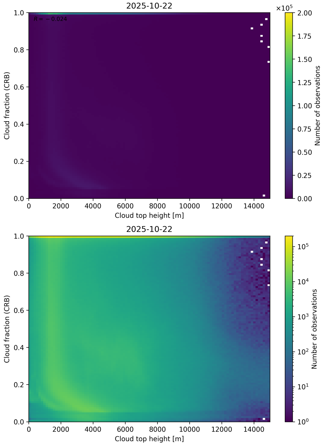
Figure 88: Scatter density plot of “Cloud top height” against “Cloud fraction (CRB)” for 2025-10-22 to 2025-10-23.
