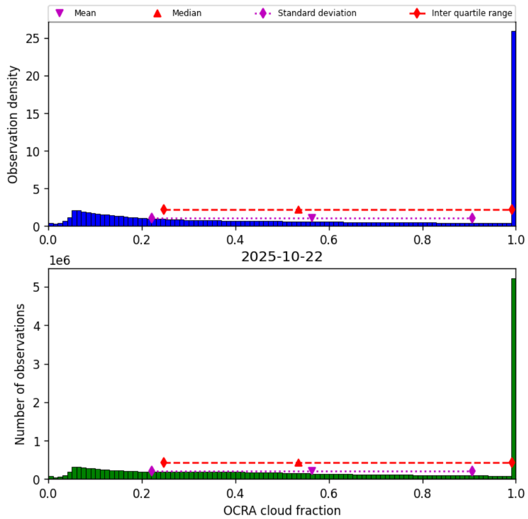
Figure 50: Histogram of “OCRA cloud fraction” for 2025-10-22 to 2025-10-23
