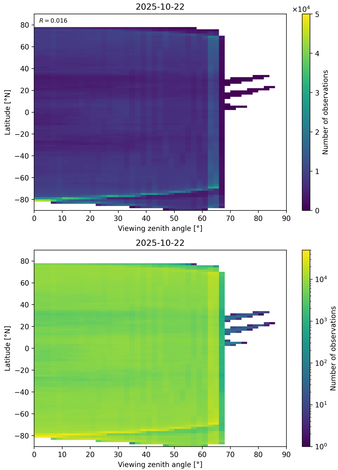
Figure 113: Scatter density plot of “Viewing zenith angle” against “Latitude” for 2025-10-22 to 2025-10-23.
