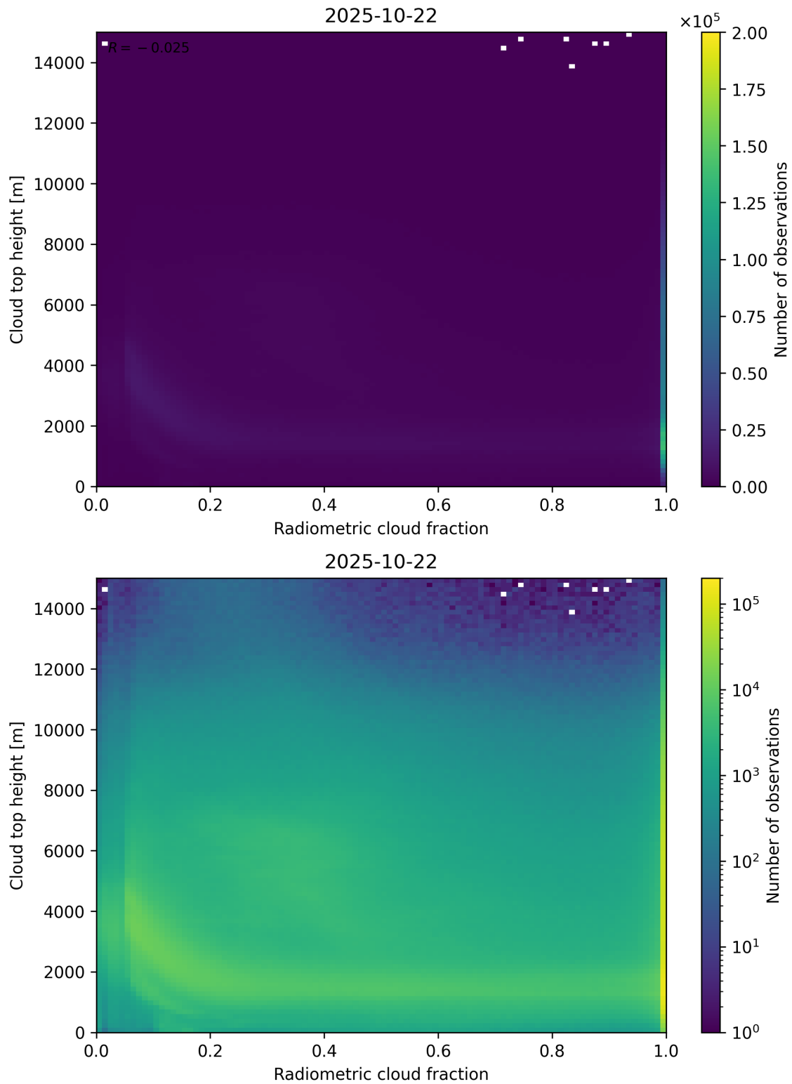
Figure 76: Scatter density plot of “Radiometric cloud fraction” against “Cloud top height” for 2025-10-22 to 2025-10-23.
