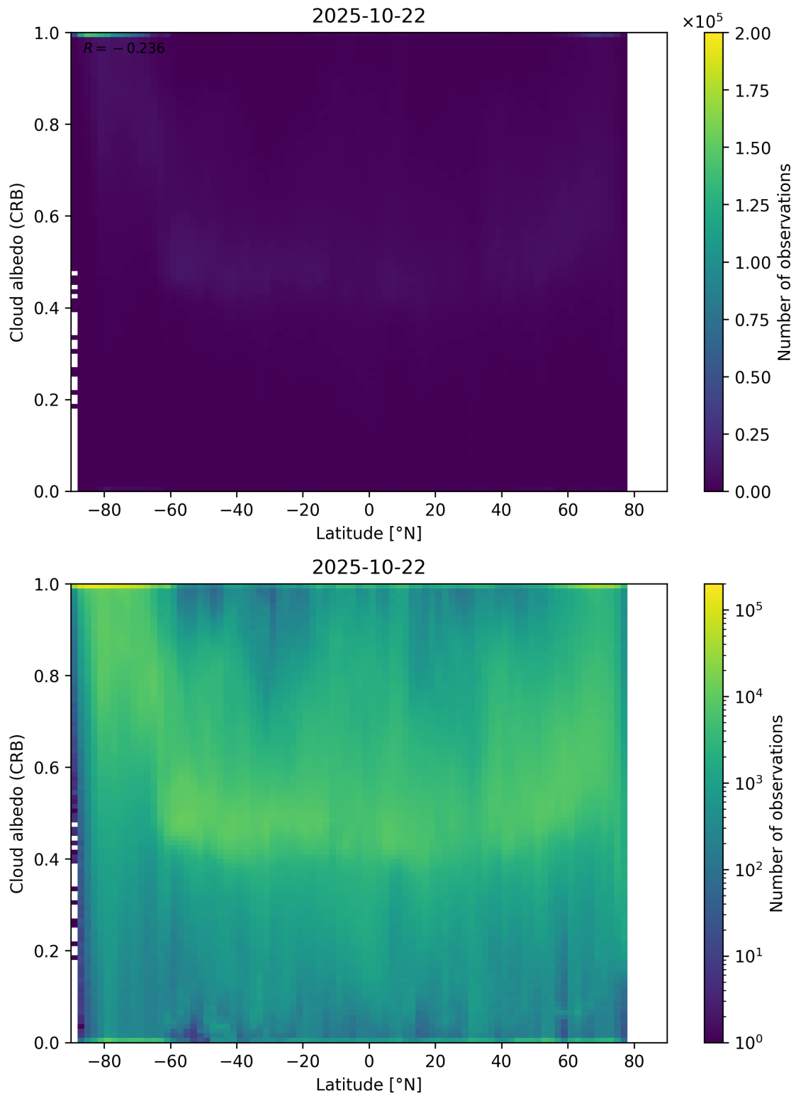
Figure 91: Scatter density plot of “Latitude” against “Cloud albedo (CRB)” for 2025-10-22 to 2025-10-23.
