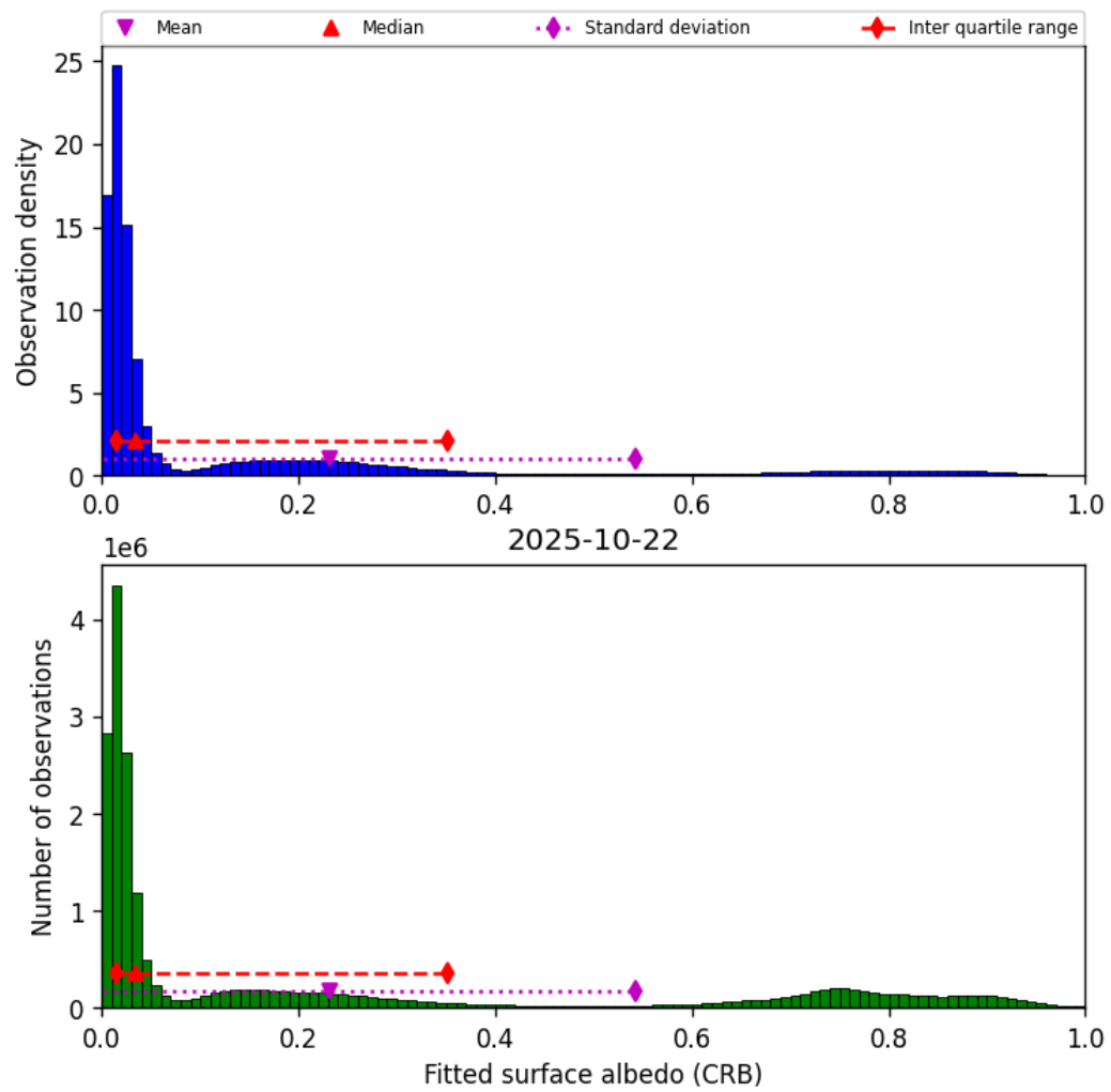
Figure 46: Histogram of “Fitted surface albedo (CRB)” for 2025-10-22 to 2025-10-23
