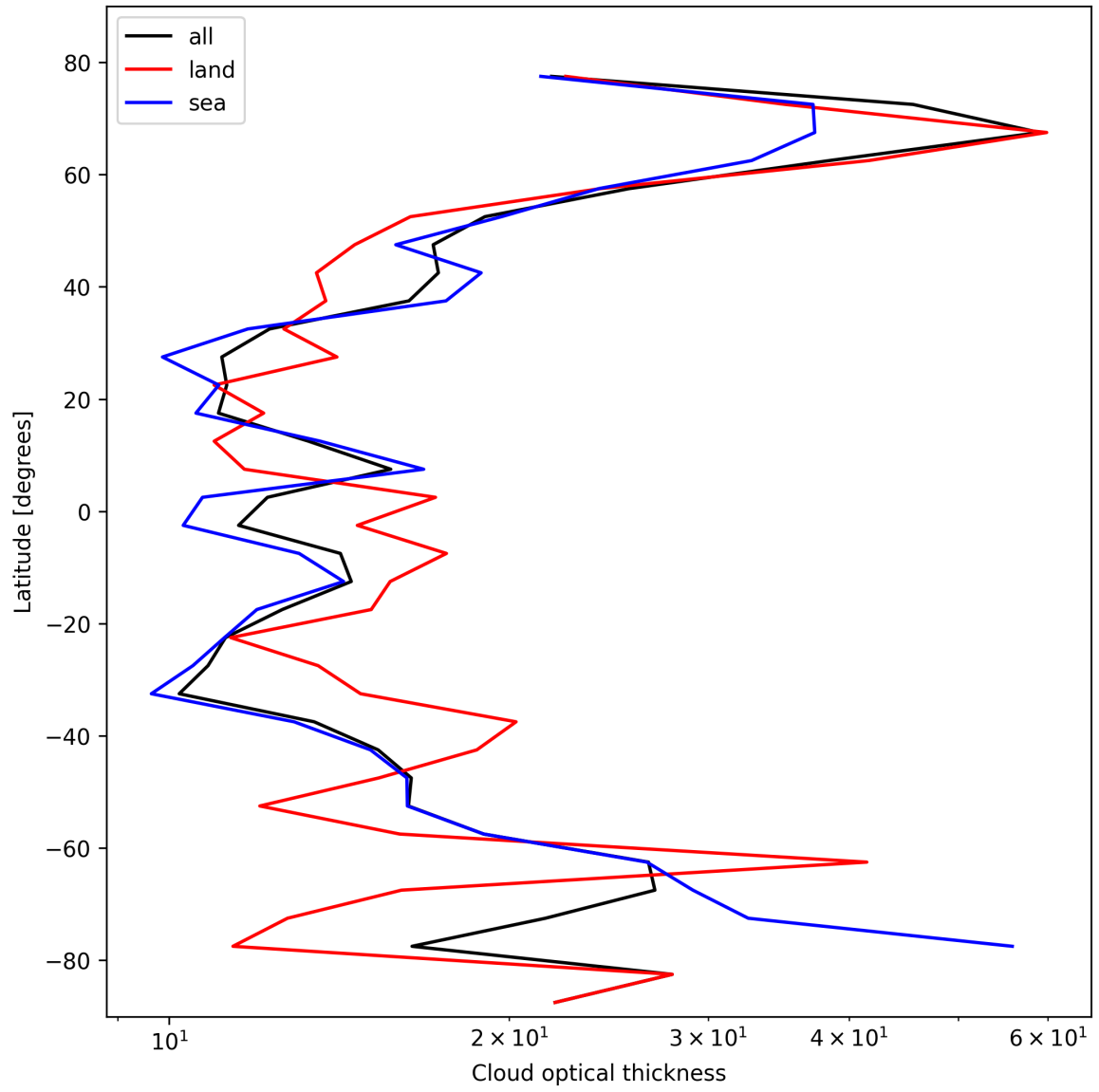
Figure 25: Zonal average of “Cloud optical thickness” for 2025-10-22 to 2025-10-23.
