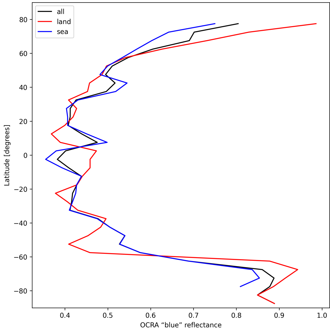
Figure 35: Zonal average of "OCRA "blue" reflectance" for 2025-10-22 to 2025-10-23.
