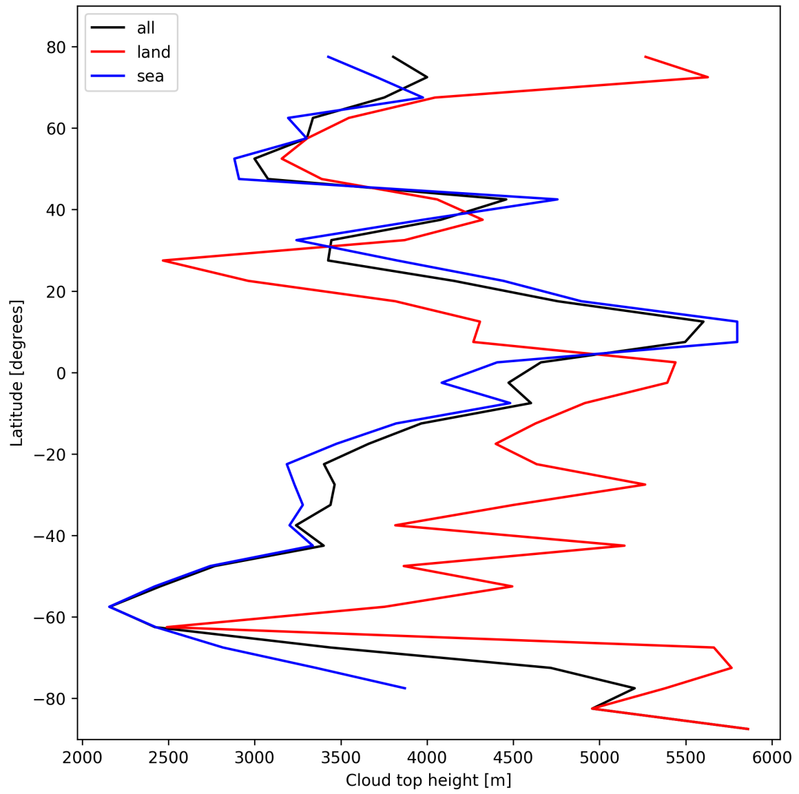
Figure 24: Zonal average of “Cloud top height” for 2025-10-22 to 2025-10-23.
