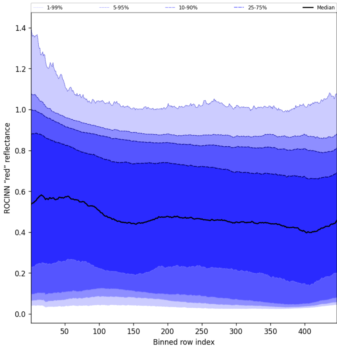
Figure 69: Along track statistics of "ROCINN "red" reflectance" for 2025-10-22 to 2025-10-23
