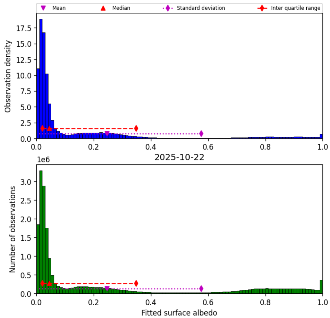
Figure 45: Histogram of “Fitted surface albedo” for 2025-10-22 to 2025-10-23
