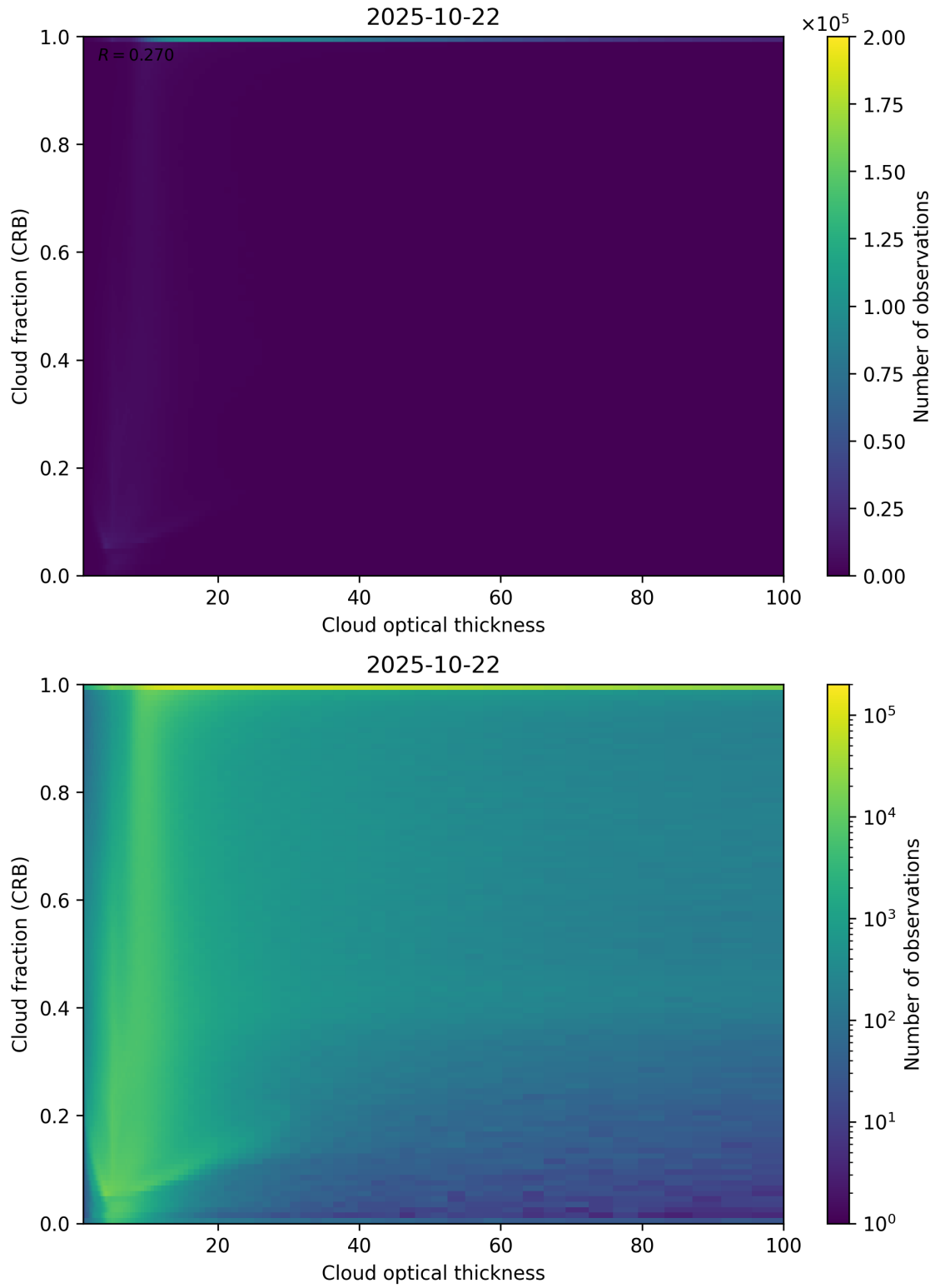
Figure 84: Scatter density plot of “Cloud optical thickness” against “Cloud fraction (CRB)” for 2025-10-22 to 2025-10-23.
