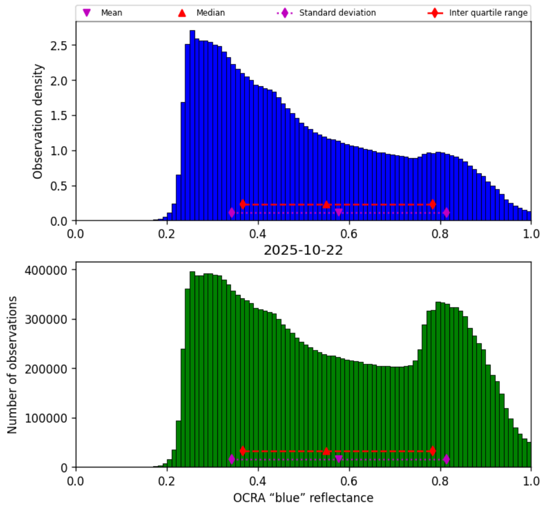
Figure 51: Histogram of “OCRA “blue” reflectance” for 2025-10-22 to 2025-10-23
