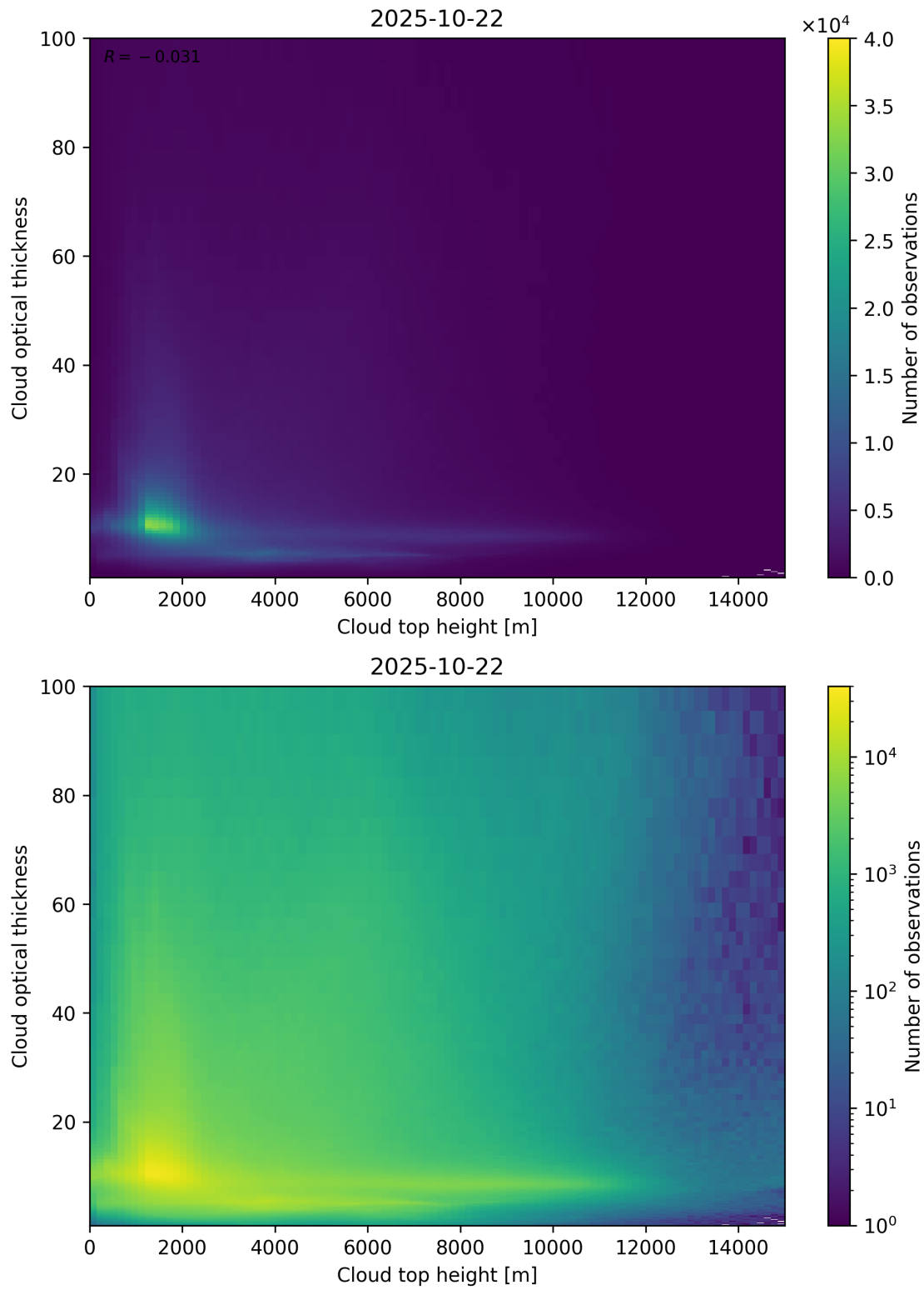
Figure 90: Scatter density plot of “Cloud top height” against “Cloud optical thickness” for 2025-10-22 to 2025-10-23.
