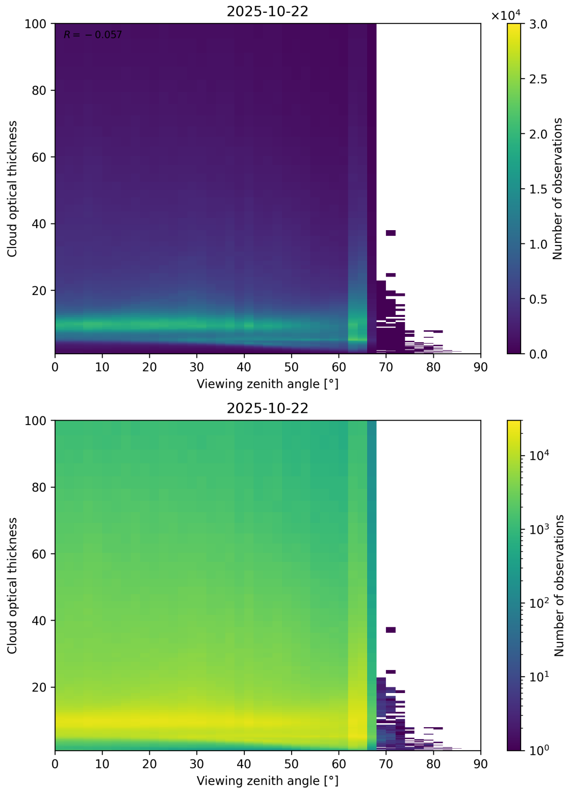
Figure 111: Scatter density plot of “Viewing zenith angle” against “Cloud optical thickness” for 2025-10-22 to 2025-10-23.
