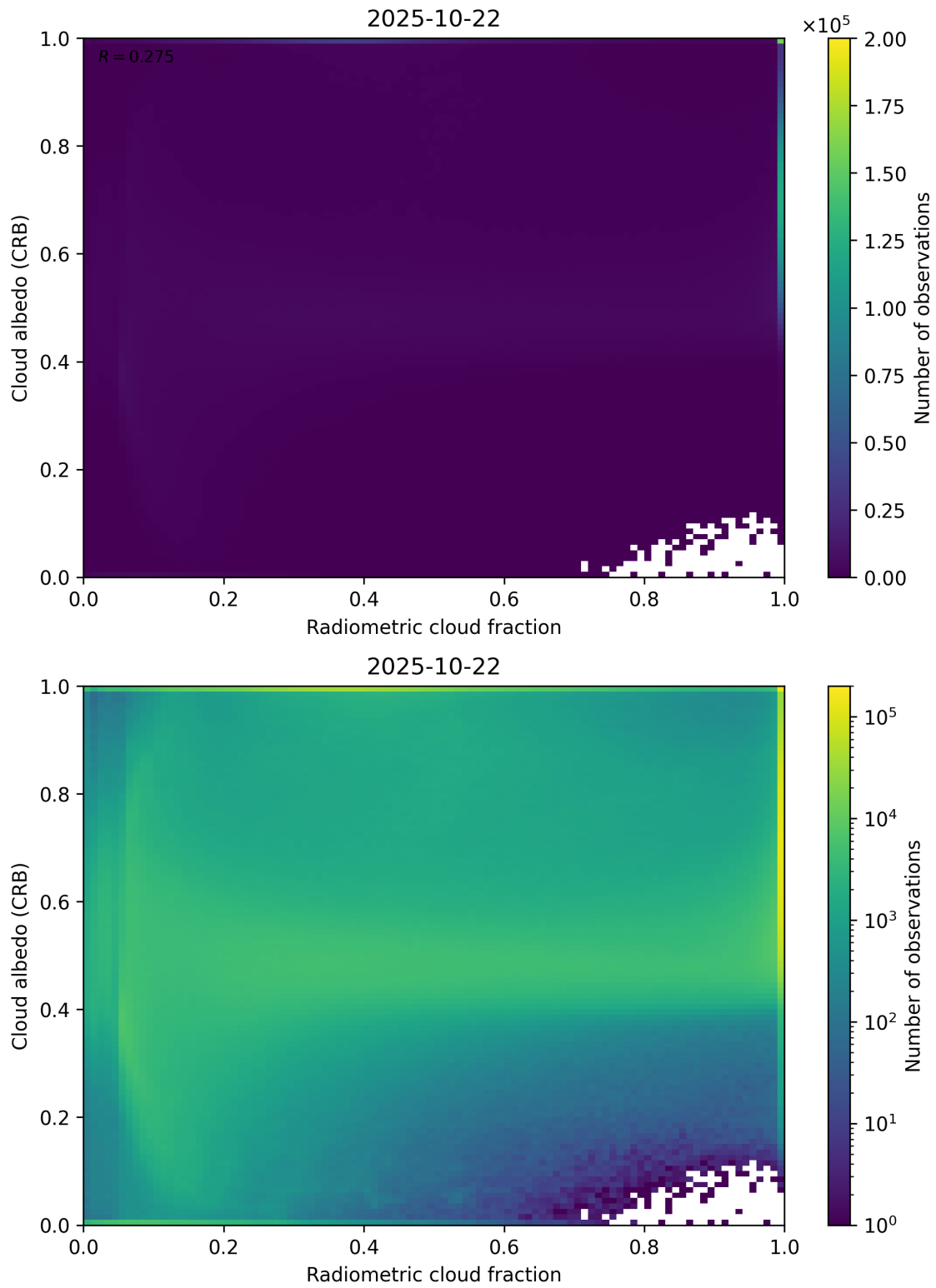
Figure 71: Scatter density plot of “Radiometric cloud fraction” against “Cloud albedo (CRB)” for 2025-10-22 to 2025-10-23.
