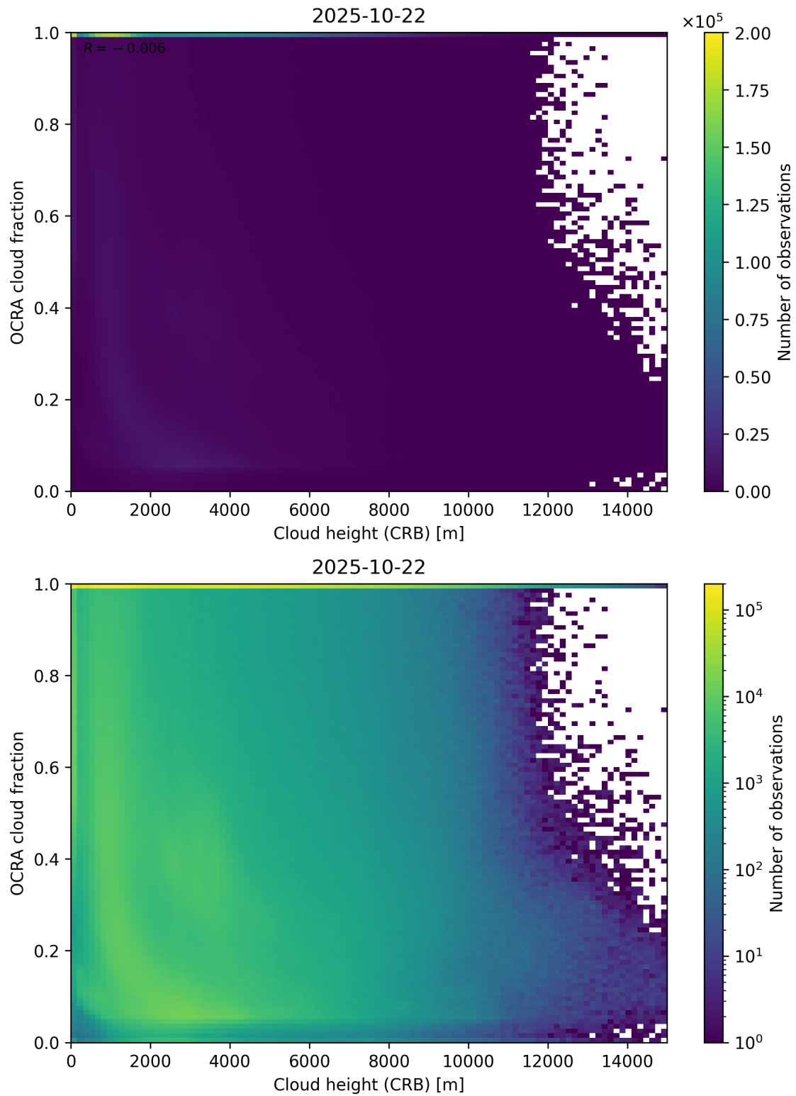
Figure 81: Scatter density plot of “Cloud height (CRB)” against “OCRA cloud fraction” for 2025-10-22 to 2025-10-23.
