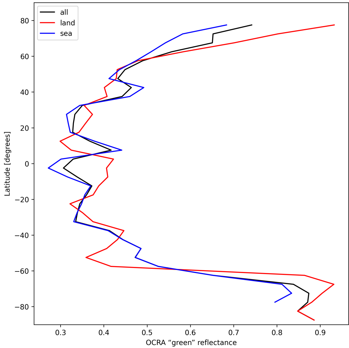
Figure 36: Zonal average of “OCRA “green” reflectance” for 2025-10-22 to 2025-10-23.
