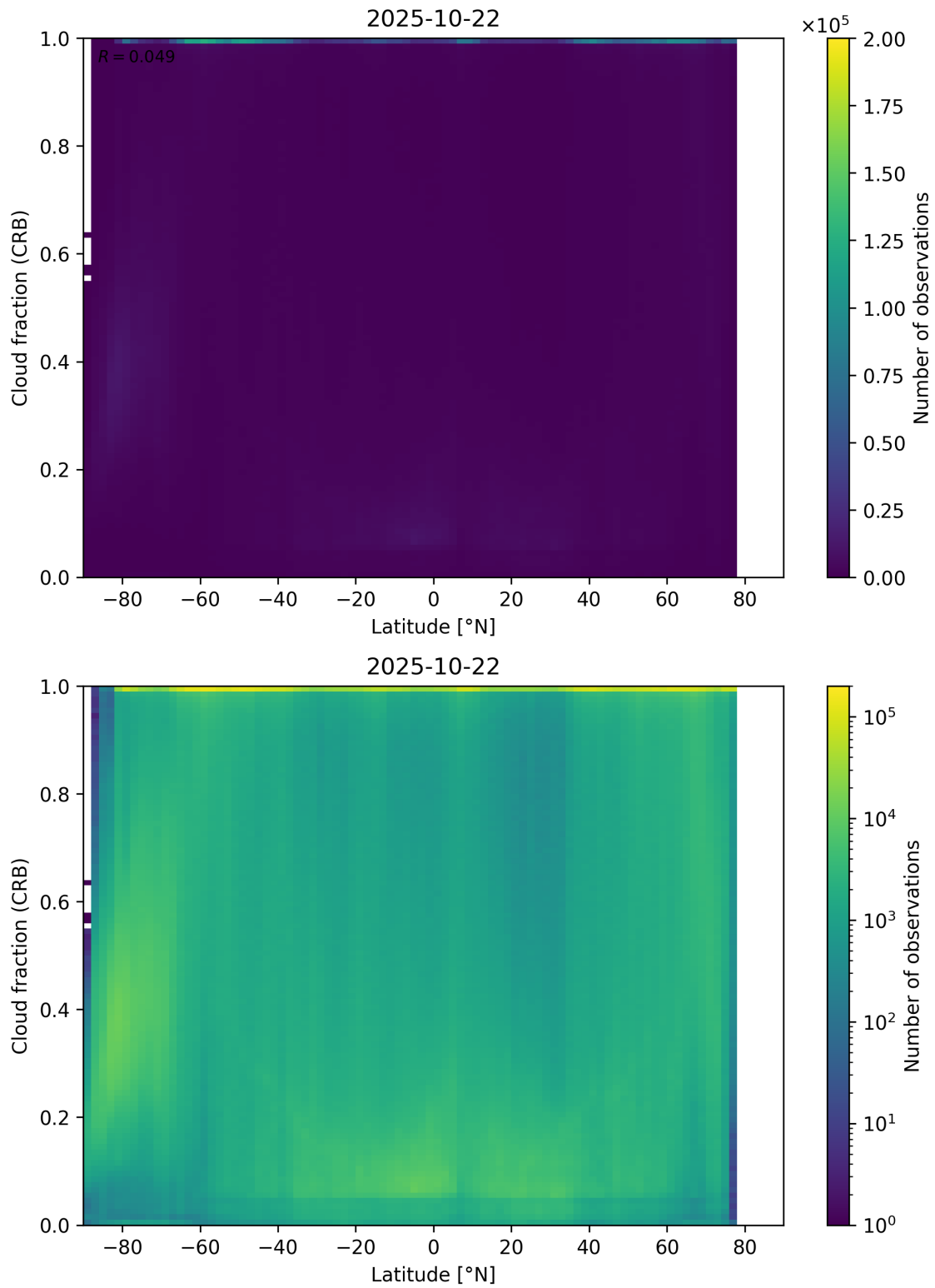
Figure 94: Scatter density plot of “Latitude” against “Cloud fraction (CRB)” for 2025-10-22 to 2025-10-23.
