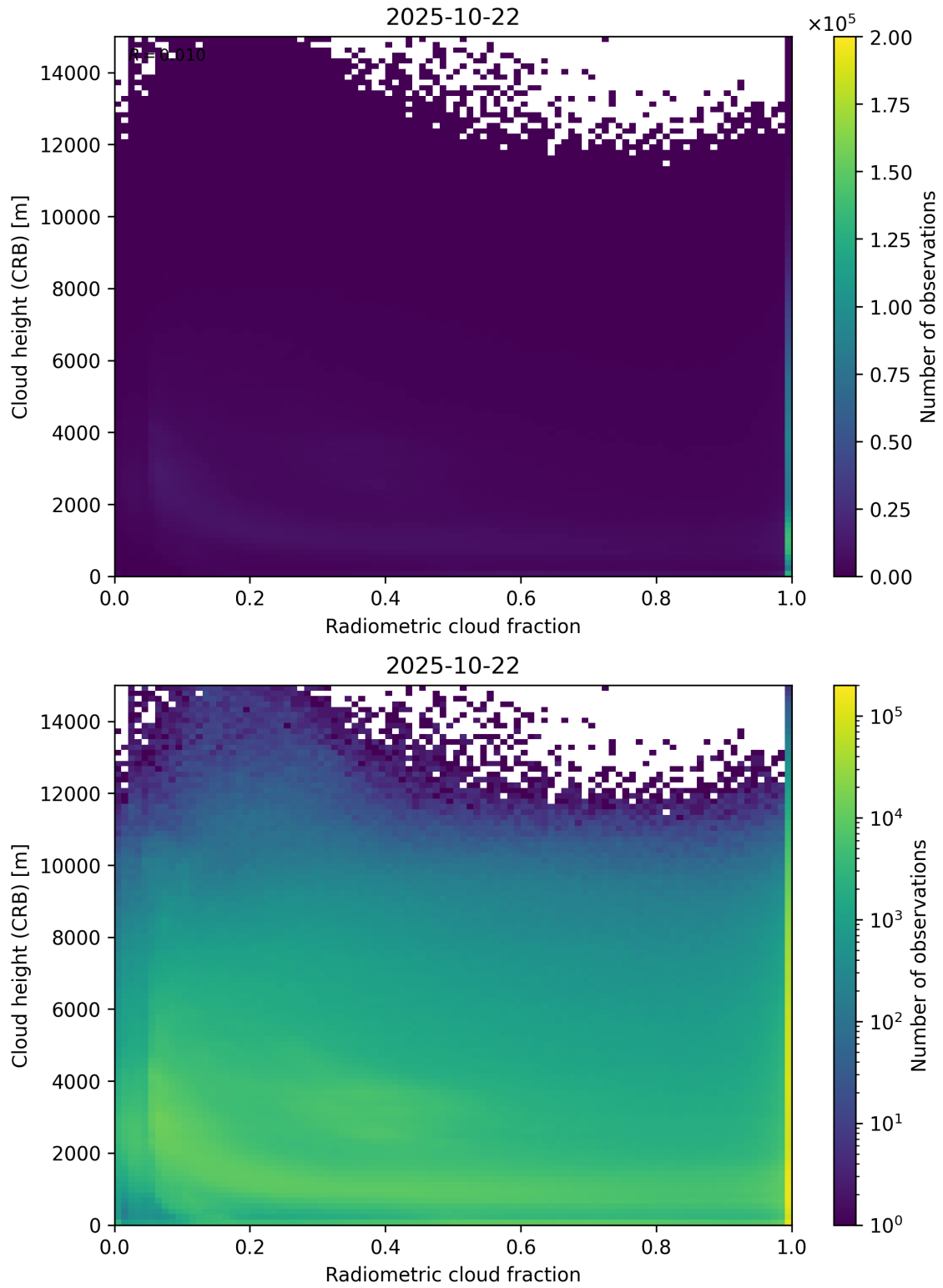
Figure 74: Scatter density plot of “Radiometric cloud fraction” against “Cloud height (CRB)” for 2025-10-22 to 2025-10-23.
