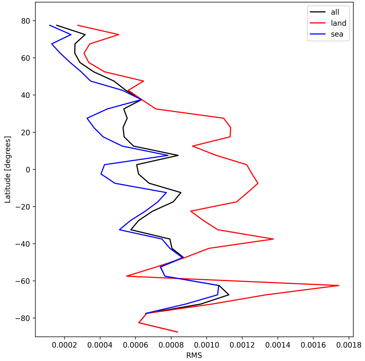
Figure 31: Zonal average of “RMS” for 2025-10-22 to 2025-10-23.
