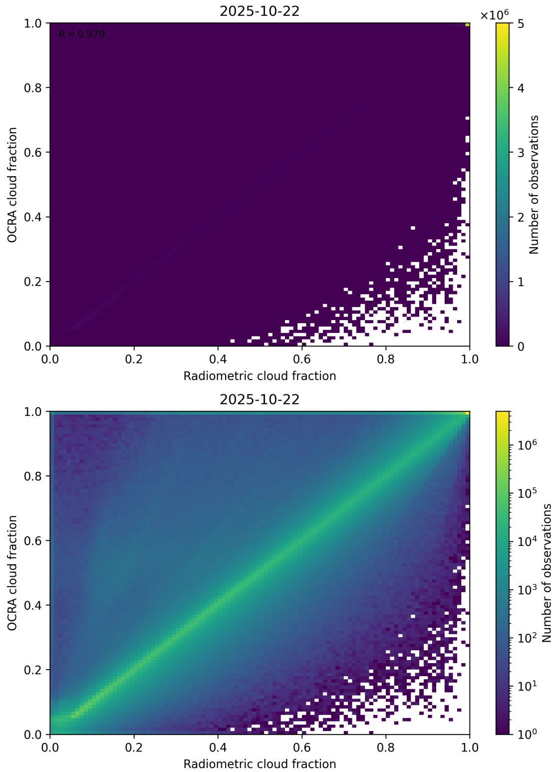
Figure 72: Scatter density plot of “Radiometric cloud fraction” against “OCRA cloud fraction” for 2025-10-22 to 2025-10-23.
