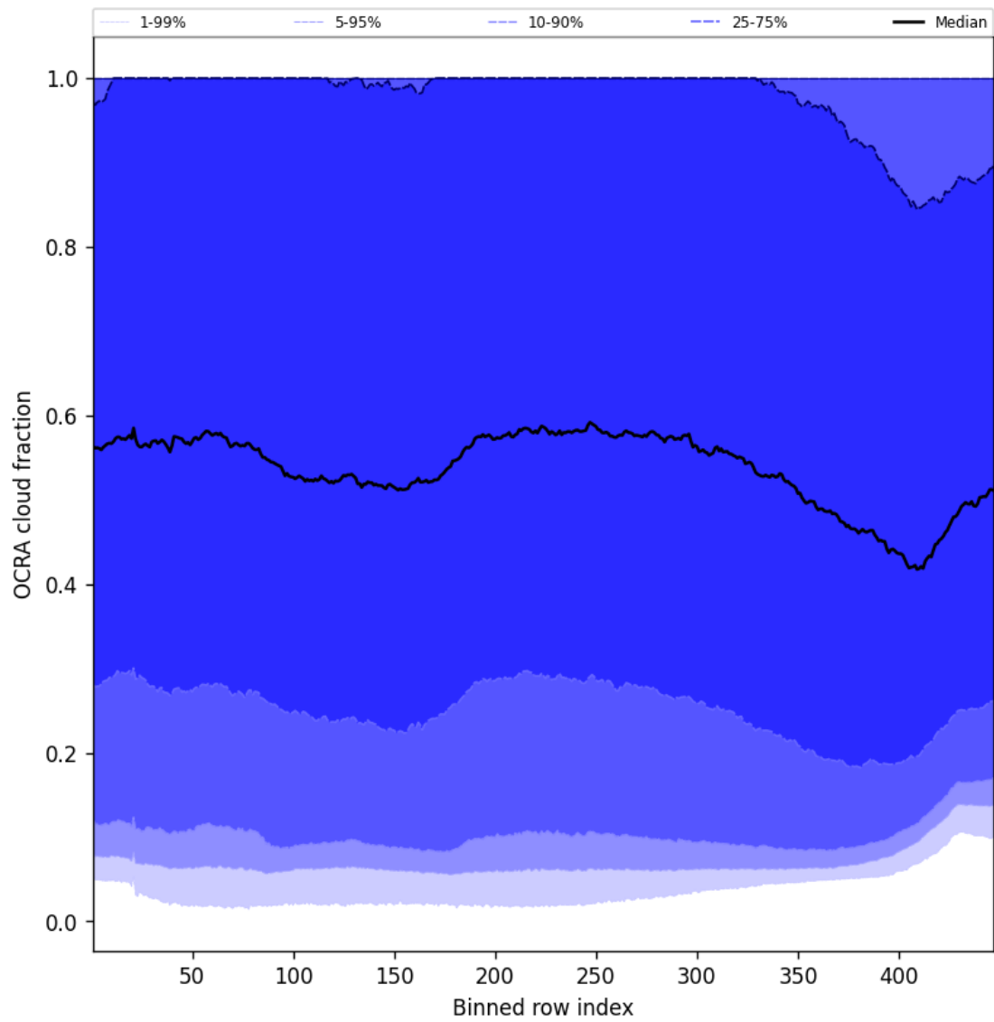
Figure 66: Along track statistics of “OCRA cloud fraction” for 2025-10-22 to 2025-10-23
