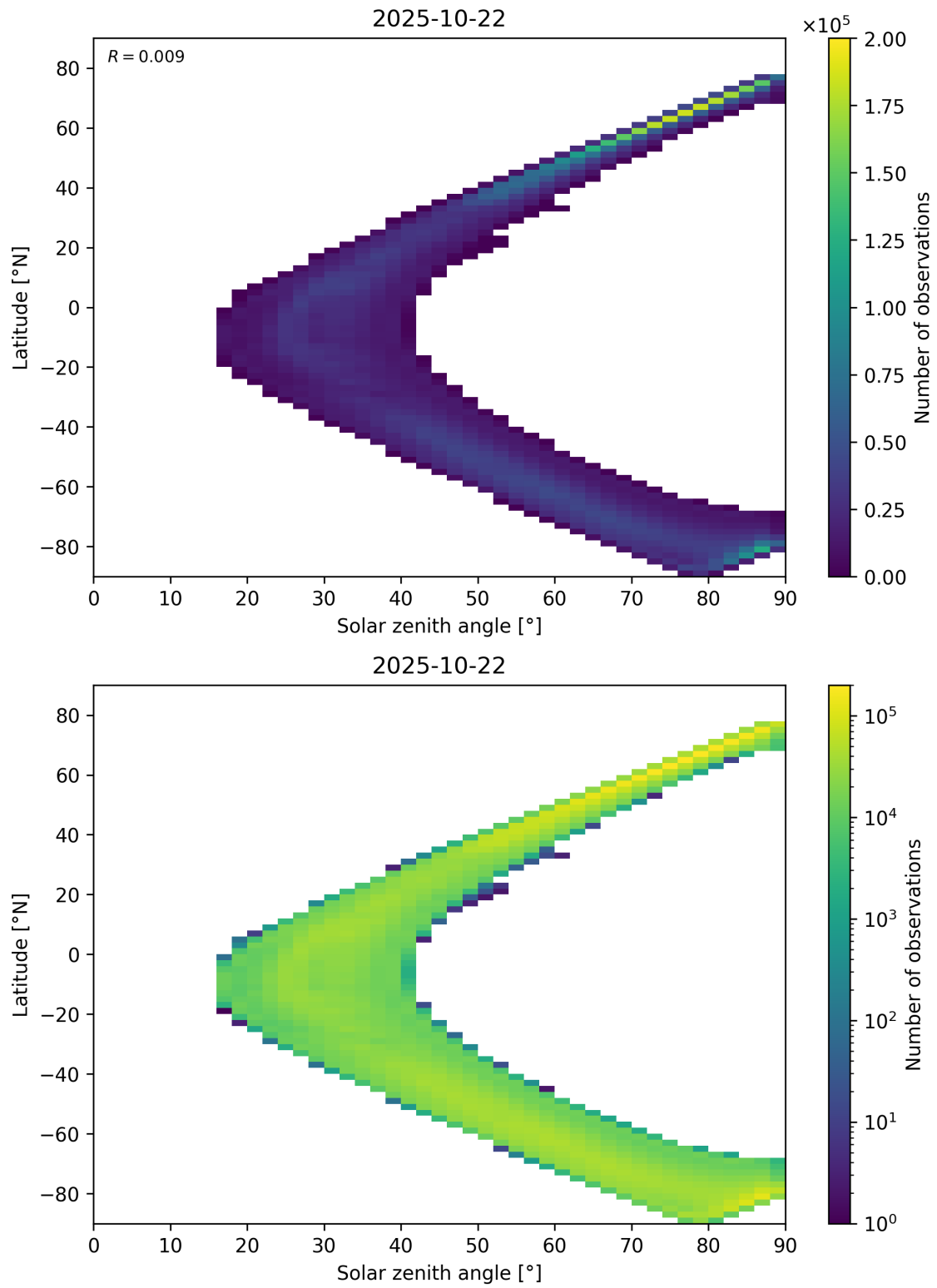
Figure 105: Scatter density plot of “Solar zenith angle” against “Latitude” for 2025-10-22 to 2025-10-23.
