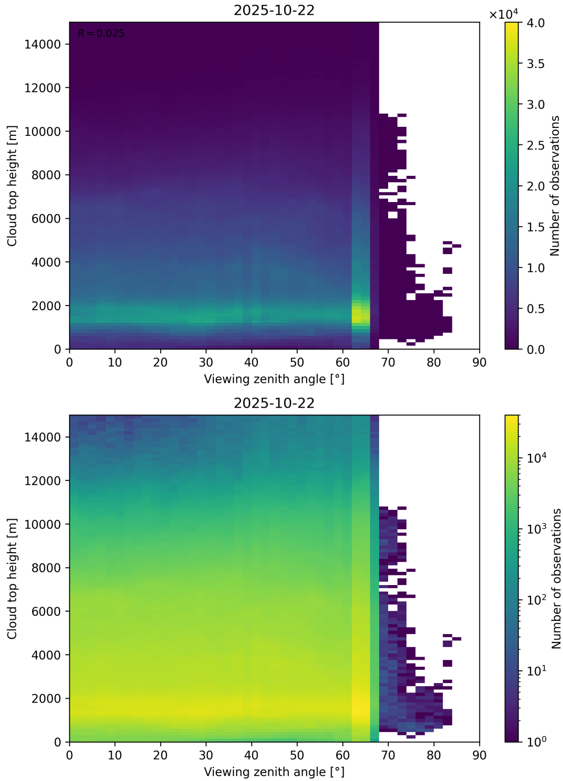
Figure 112: Scatter density plot of “Viewing zenith angle” against “Cloud top height” for 2025-10-22 to 2025-10-23.
