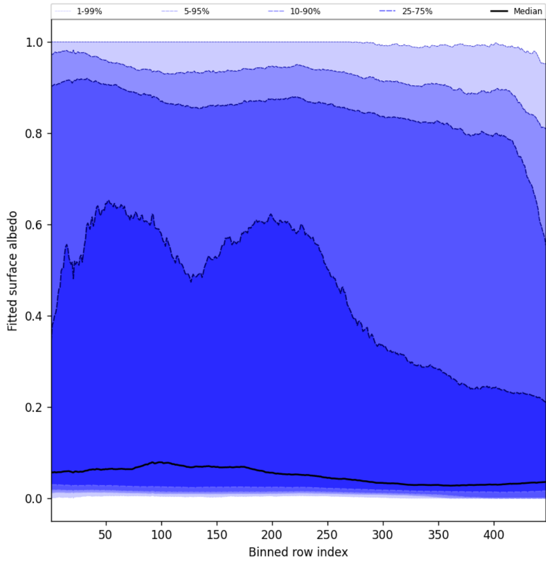
Figure 61: Along track statistics of “Fitted surface albedo” for 2025-10-22 to 2025-10-23
