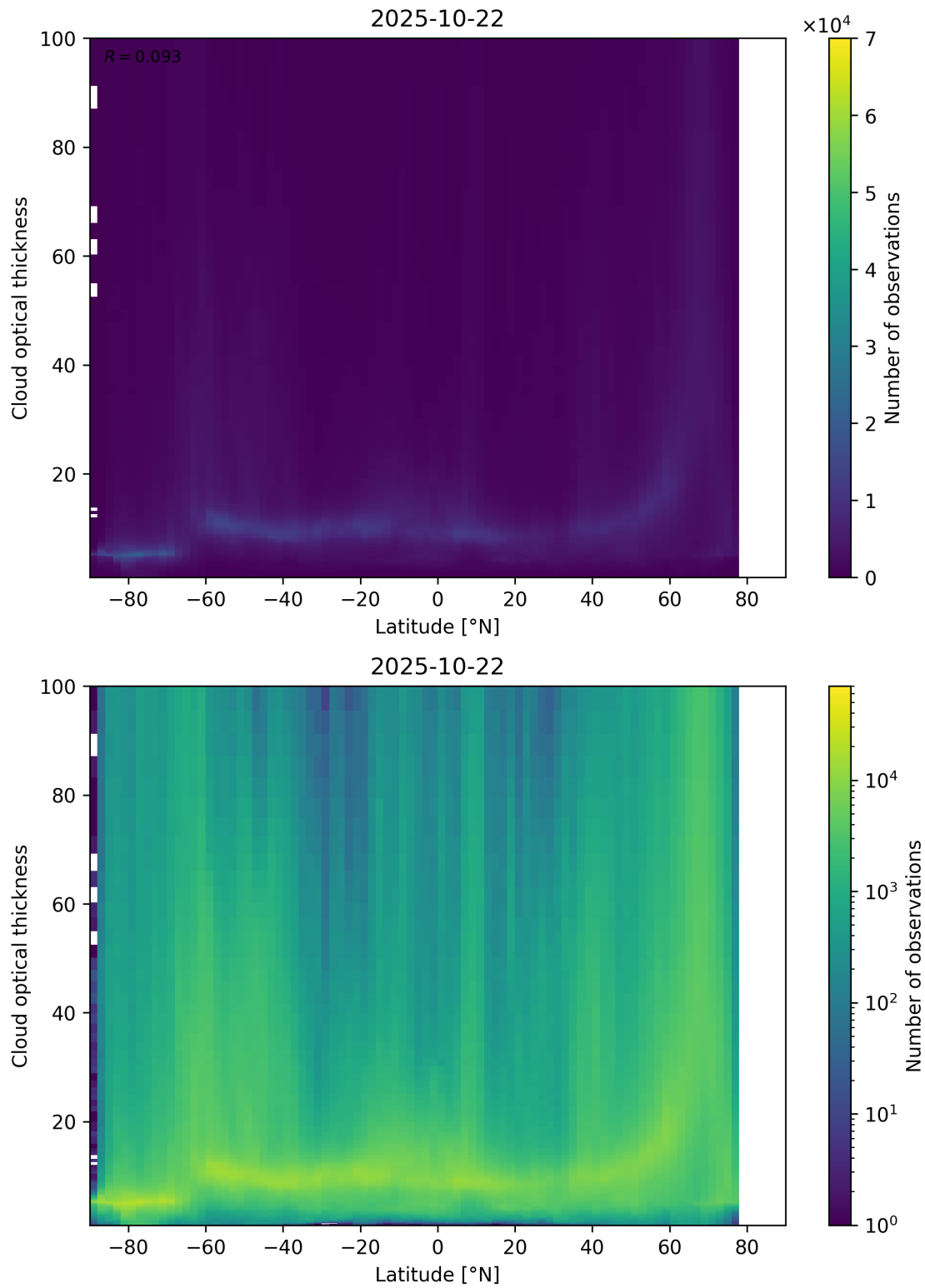
Figure 96: Scatter density plot of “Latitude” against “Cloud optical thickness” for 2025-10-22 to 2025-10-23.
