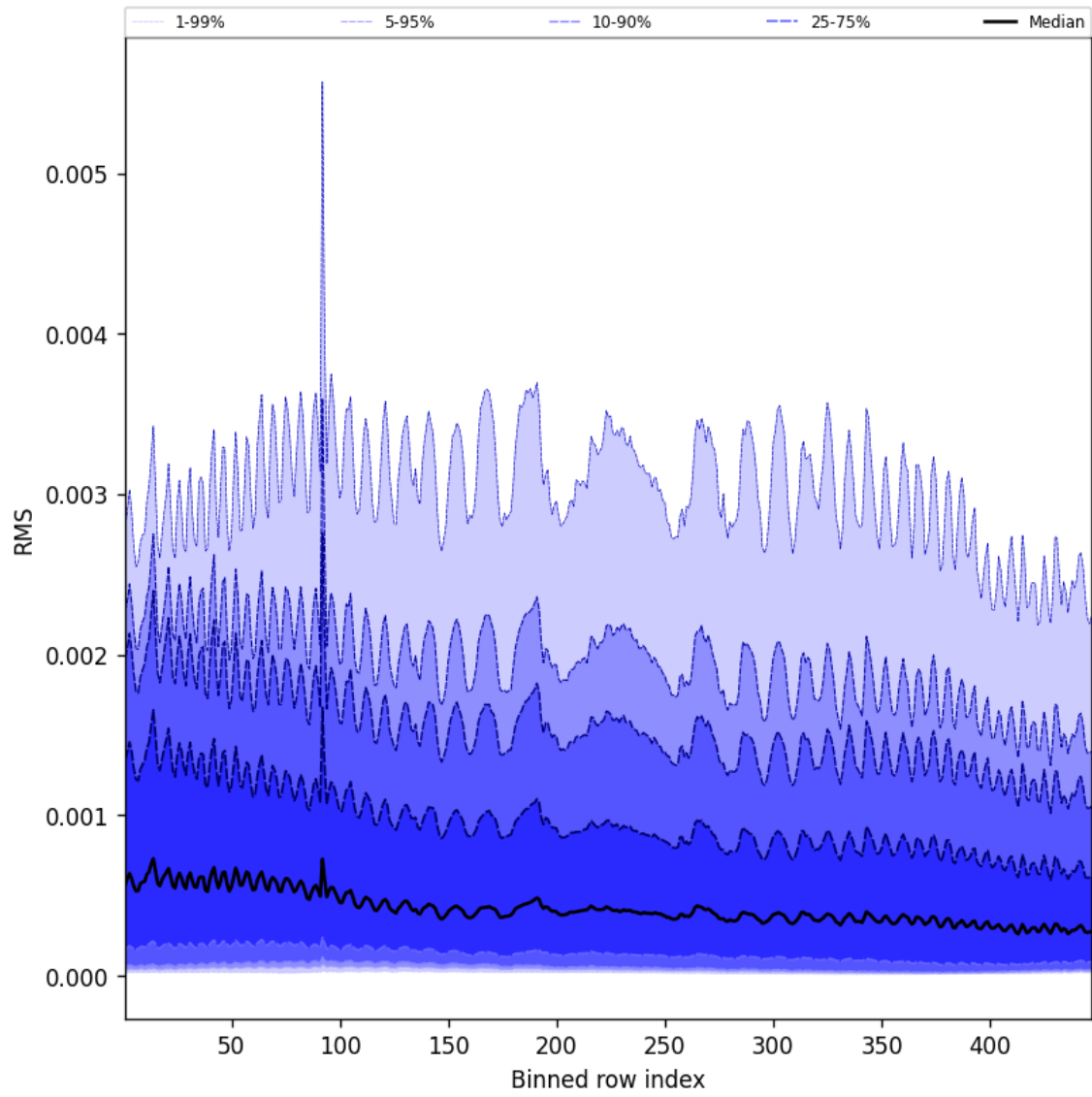
Figure 63: Along track statistics of “RMS” for 2025-10-22 to 2025-10-23
