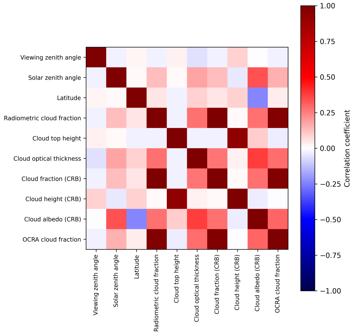
Figure 2: Map of correlation matrix for 2025-10-22 to 2025-10-23.
