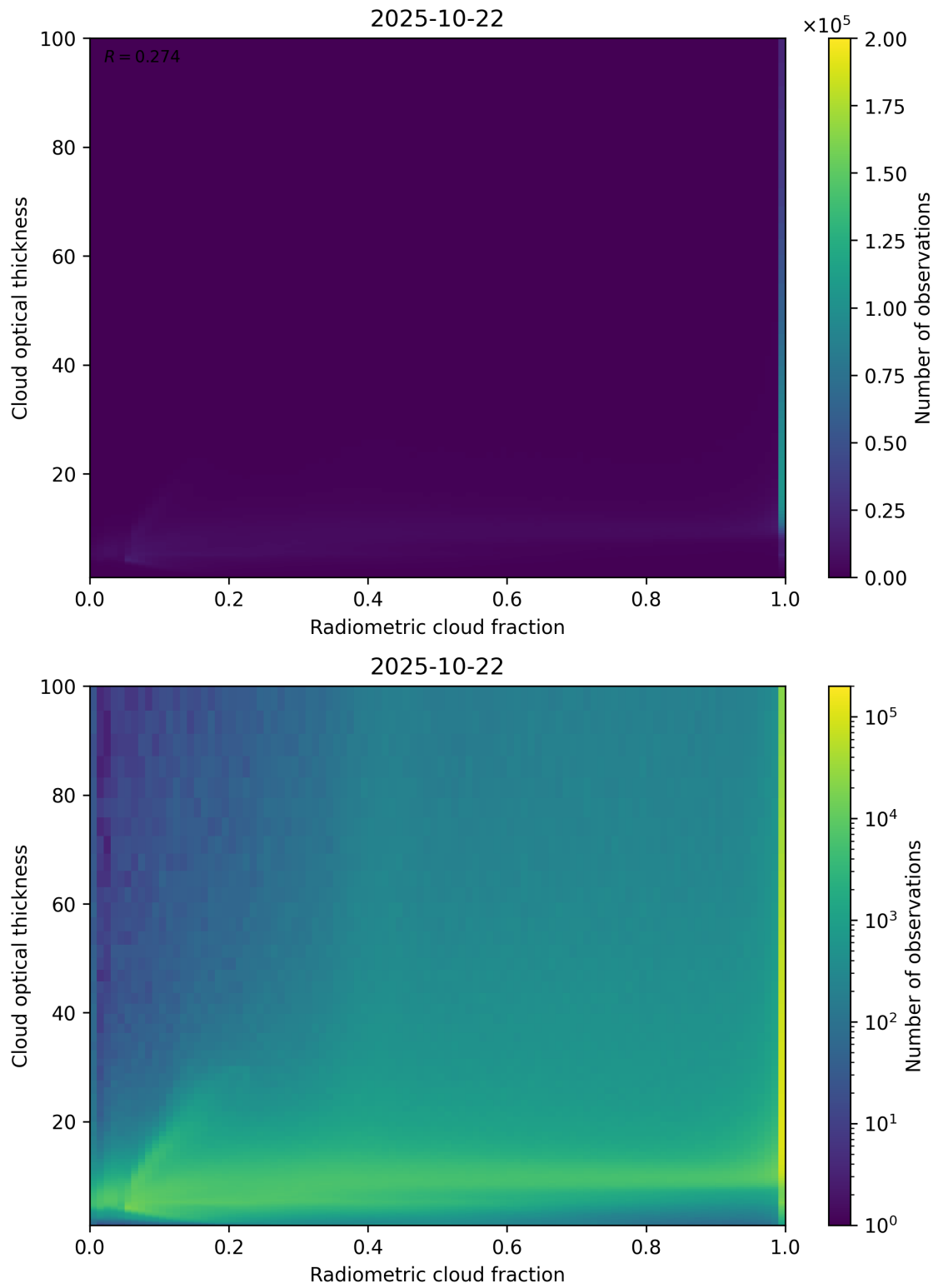
Figure 75: Scatter density plot of “Radiometric cloud fraction” against “Cloud optical thickness” for 2025-10-22 to 2025-10-23.
