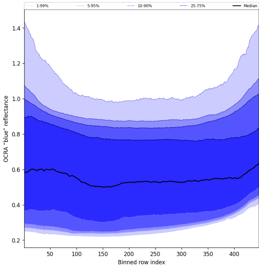
Figure 67: Along track statistics of “OCRA “blue” reflectance” for 2025-10-22 to 2025-10-23
