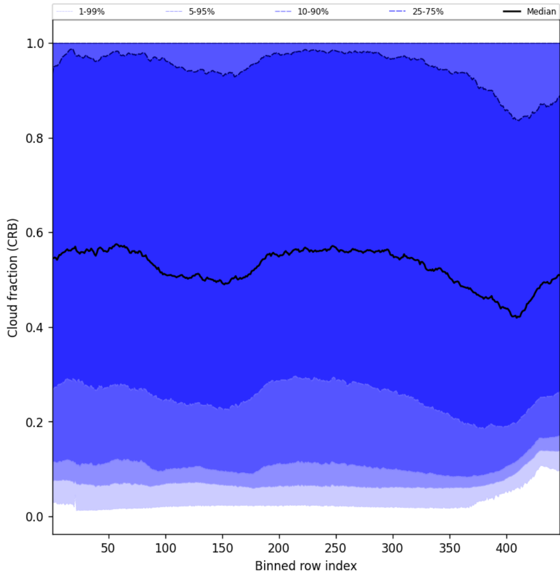
Figure 58: Along track statistics of “Cloud fraction (CRB)” for 2025-10-22 to 2025-10-23
