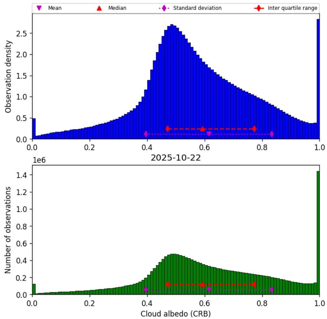
Figure 44: Histogram of “Cloud albedo (CRB)” for 2025-10-22 to 2025-10-23
