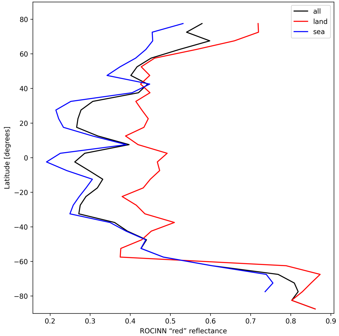
Figure 37: Zonal average of “ROCINN “red” reflectance” for 2025-10-22 to 2025-10-23.
