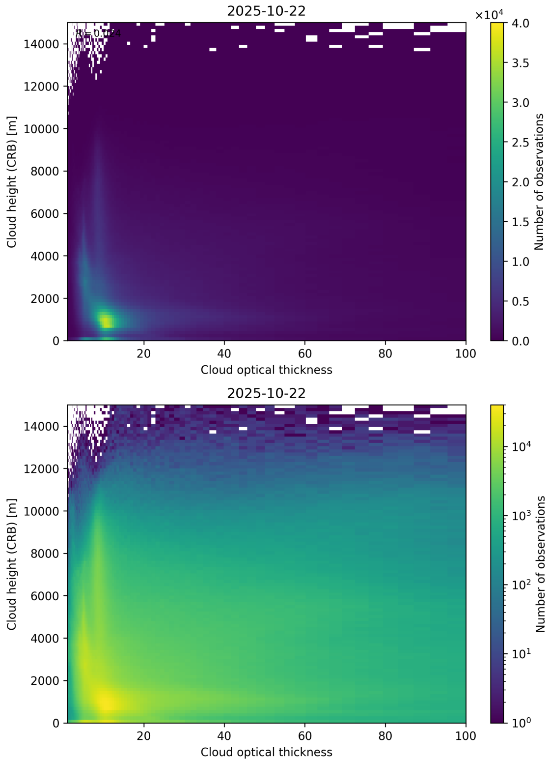
Figure 85: Scatter density plot of “Cloud optical thickness” against “Cloud height (CRB)” for 2025-10-22 to 2025-10-23.
