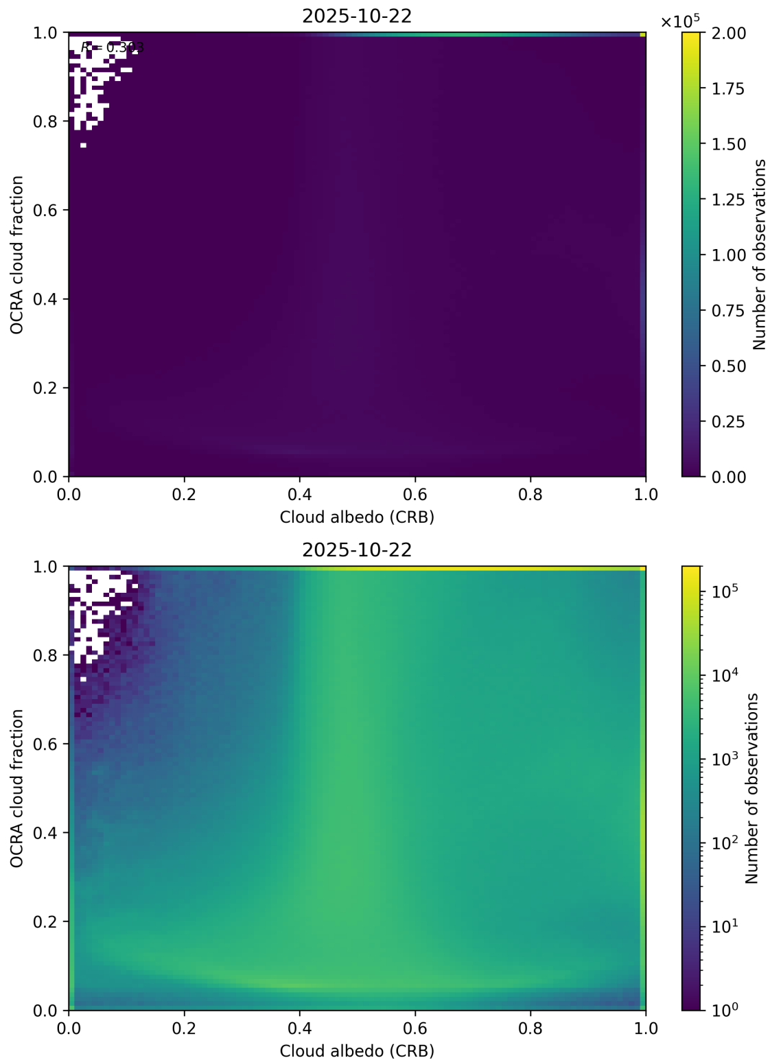
Figure 70: Scatter density plot of “Cloud albedo (CRB)” against “OCRA cloud fraction” for 2025-10-22 to 2025-10-23.
