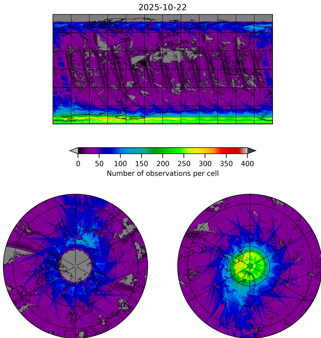
Figure 21: Map of the number of observations for 2025-10-22 to 2025-10-23
