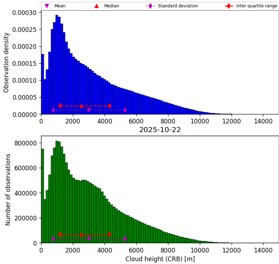
Figure 43: Histogram of “Cloud height (CRB)” for 2025-10-22 to 2025-10-23
