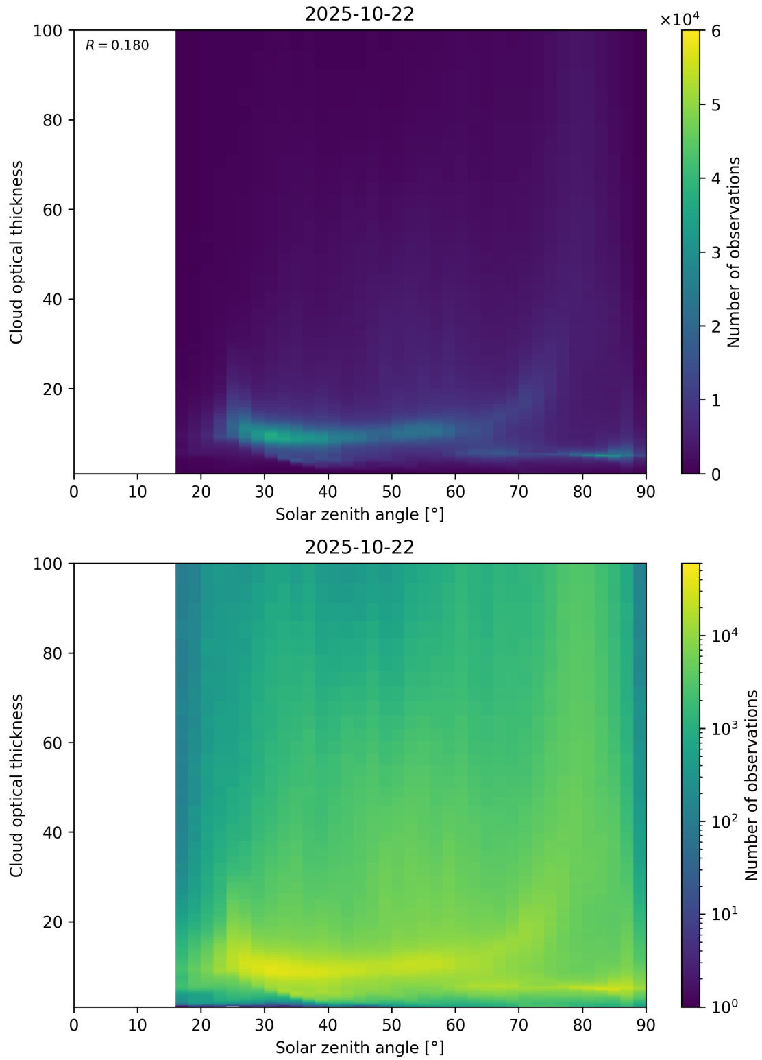
Figure 103: Scatter density plot of “Solar zenith angle” against “Cloud optical thickness” for 2025-10-22 to 2025-10-23.
