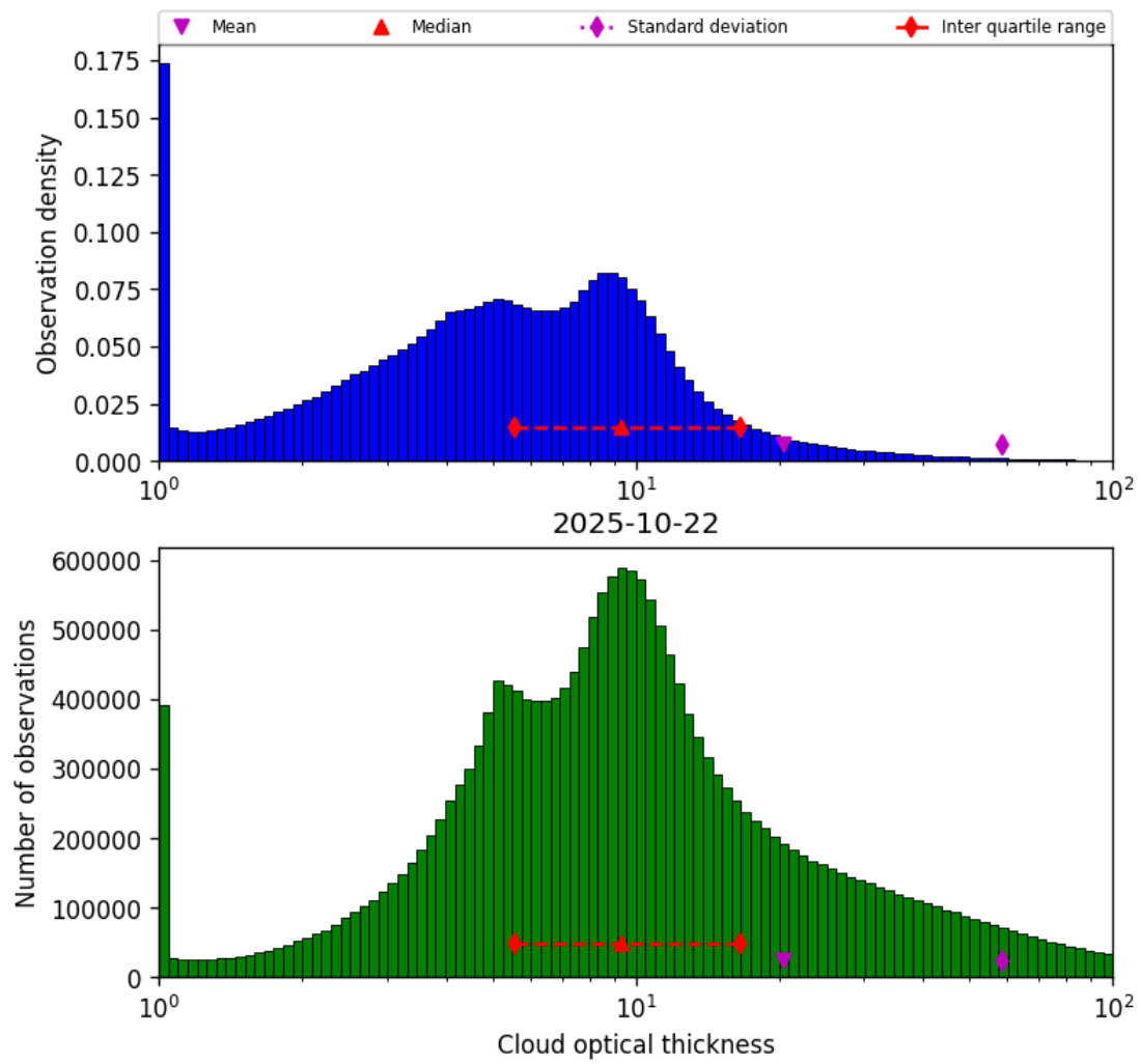
Figure 41: Histogram of “Cloud optical thickness” for 2025-10-22 to 2025-10-23
