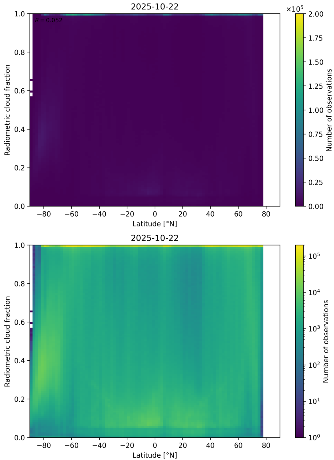
Figure 92: Scatter density plot of “Latitude” against “Radiometric cloud fraction” for 2025-10-22 to 2025-10-23.
