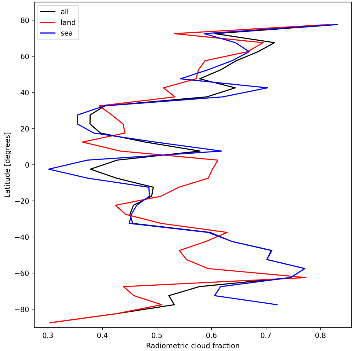
Figure 23: Zonal average of “Radiometric cloud fraction” for 2025-10-22 to 2025-10-23.
