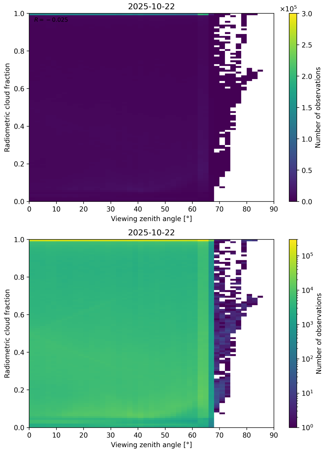
Figure 107: Scatter density plot of “Viewing zenith angle” against “Radiometric cloud fraction” for 2025-10-22 to 2025-10-23.
