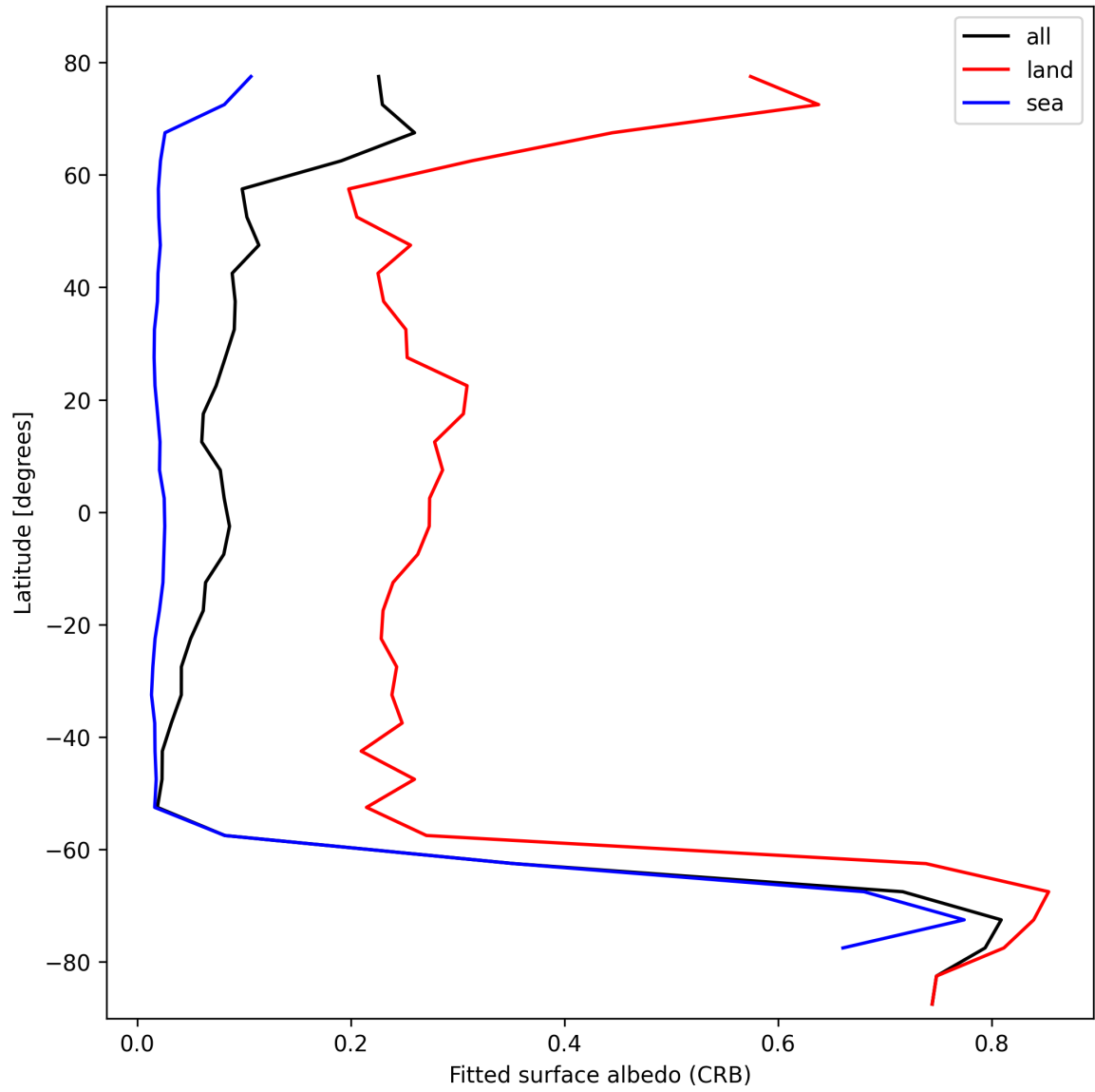
Figure 30: Zonal average of “Fitted surface albedo (CRB)” for 2025-10-22 to 2025-10-23.
