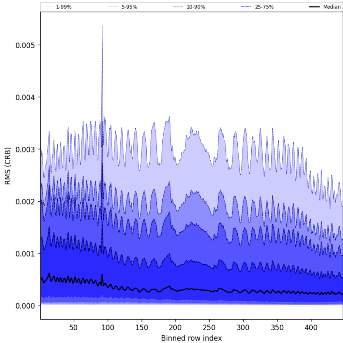
Figure 64: Along track statistics of “RMS (CRB)” for 2025-10-22 to 2025-10-23
