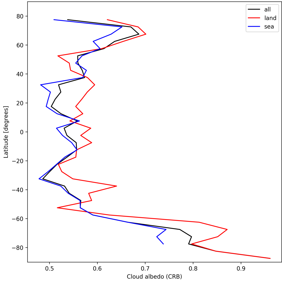
Figure 28: Zonal average of “Cloud albedo (CRB)” for 2025-10-22 to 2025-10-23.
