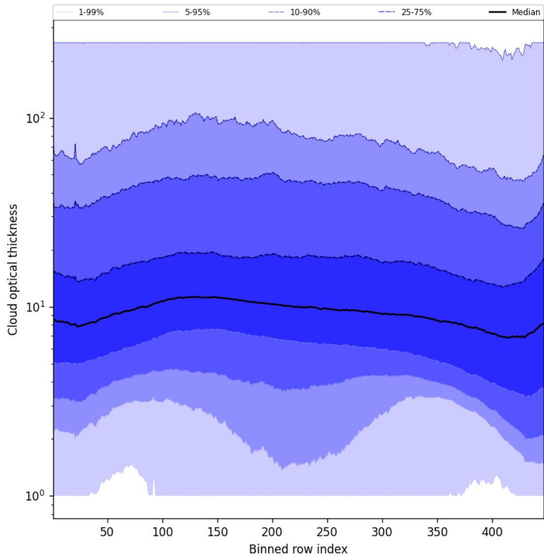
Figure 57: Along track statistics of “Cloud optical thickness” for 2025-10-22 to 2025-10-23
