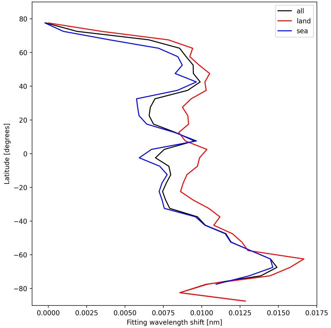
Figure 33: Zonal average of “Fitting wavelength shift” for 2025-10-22 to 2025-10-23.
