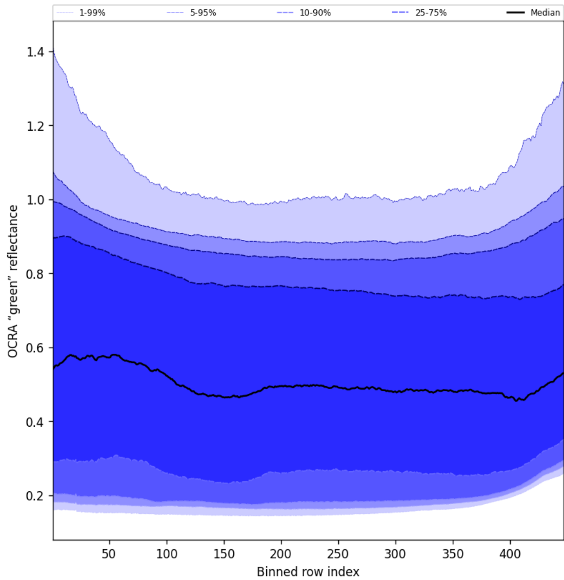
Figure 68: Along track statistics of “OCRA “green” reflectance” for 2025-10-22 to 2025-10-23
