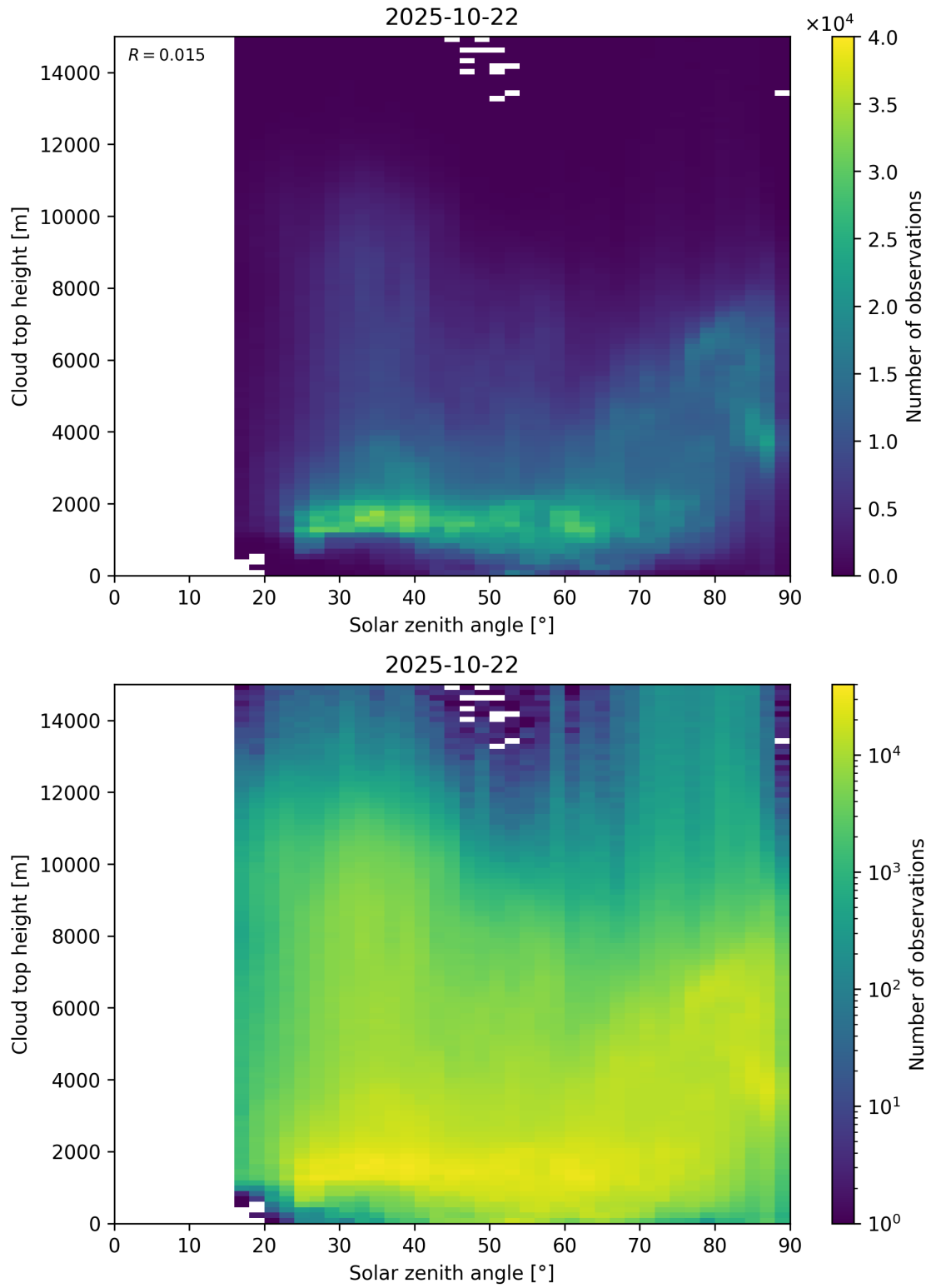
Figure 104: Scatter density plot of “Solar zenith angle” against “Cloud top height” for 2025-10-22 to 2025-10-23.
