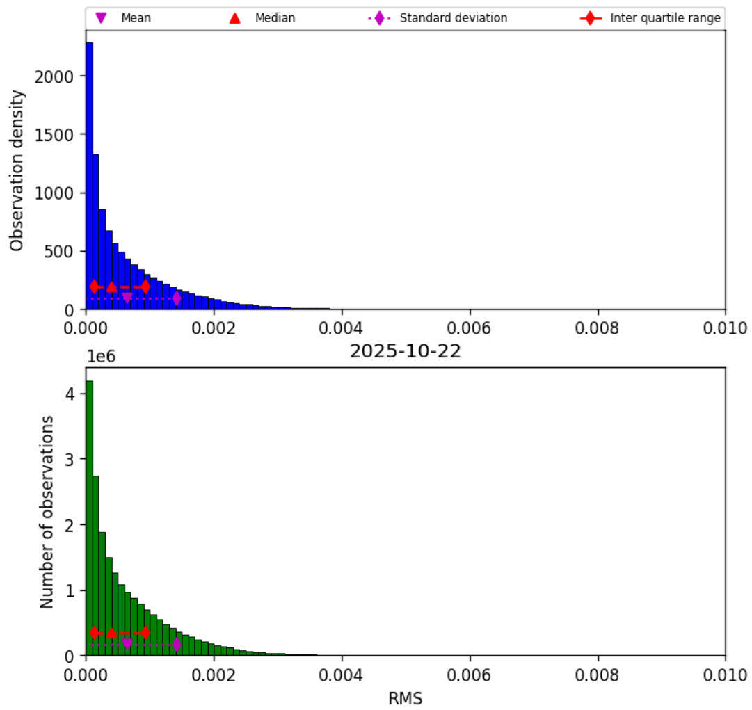
Figure 47: Histogram of “RMS” for 2025-10-22 to 2025-10-23
