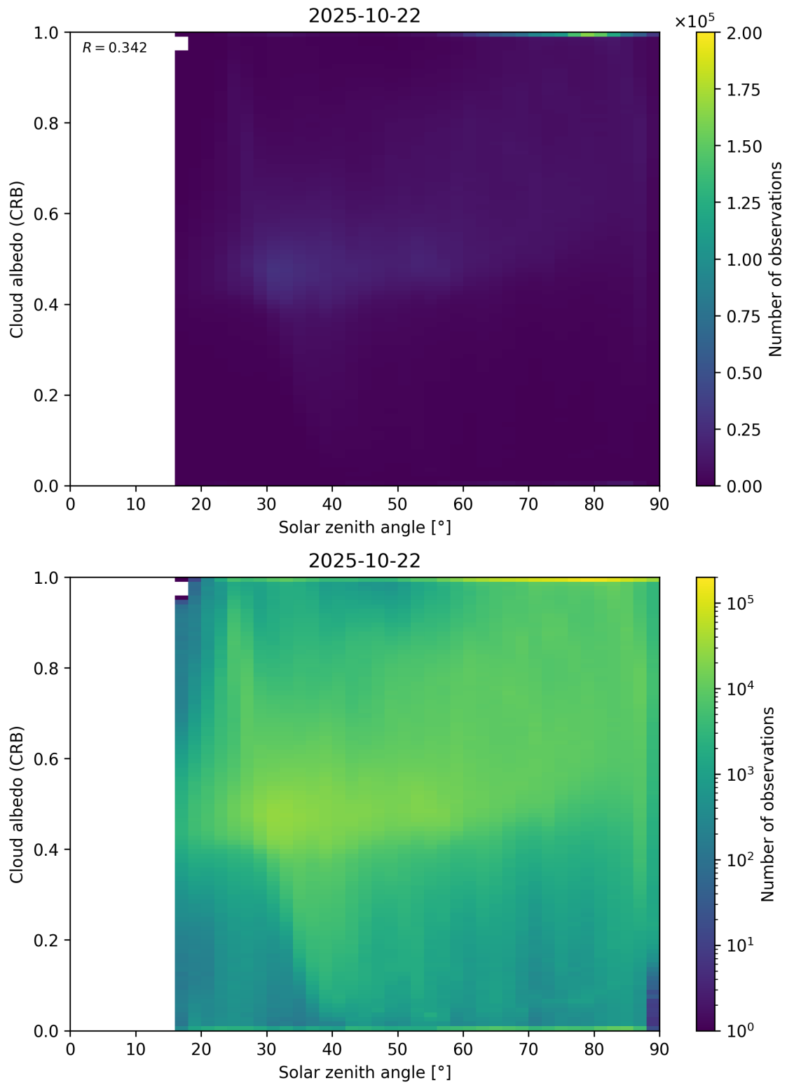
Figure 98: Scatter density plot of “Solar zenith angle” against “Cloud albedo (CRB)” for 2025-10-22 to 2025-10-23.
