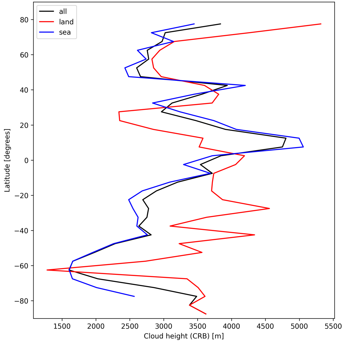
Figure 27: Zonal average of “Cloud height (CRB)” for 2025-10-22 to 2025-10-23.
