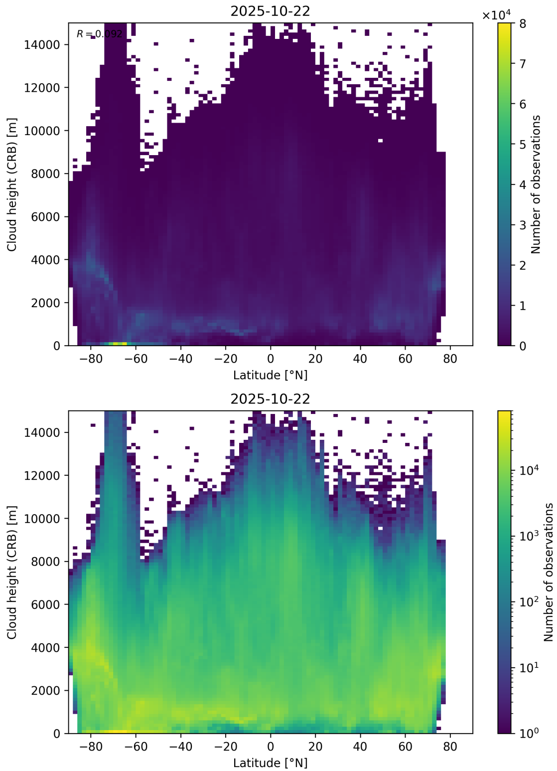
Figure 95: Scatter density plot of “Latitude” against “Cloud height (CRB)” for 2025-10-22 to 2025-10-23.
