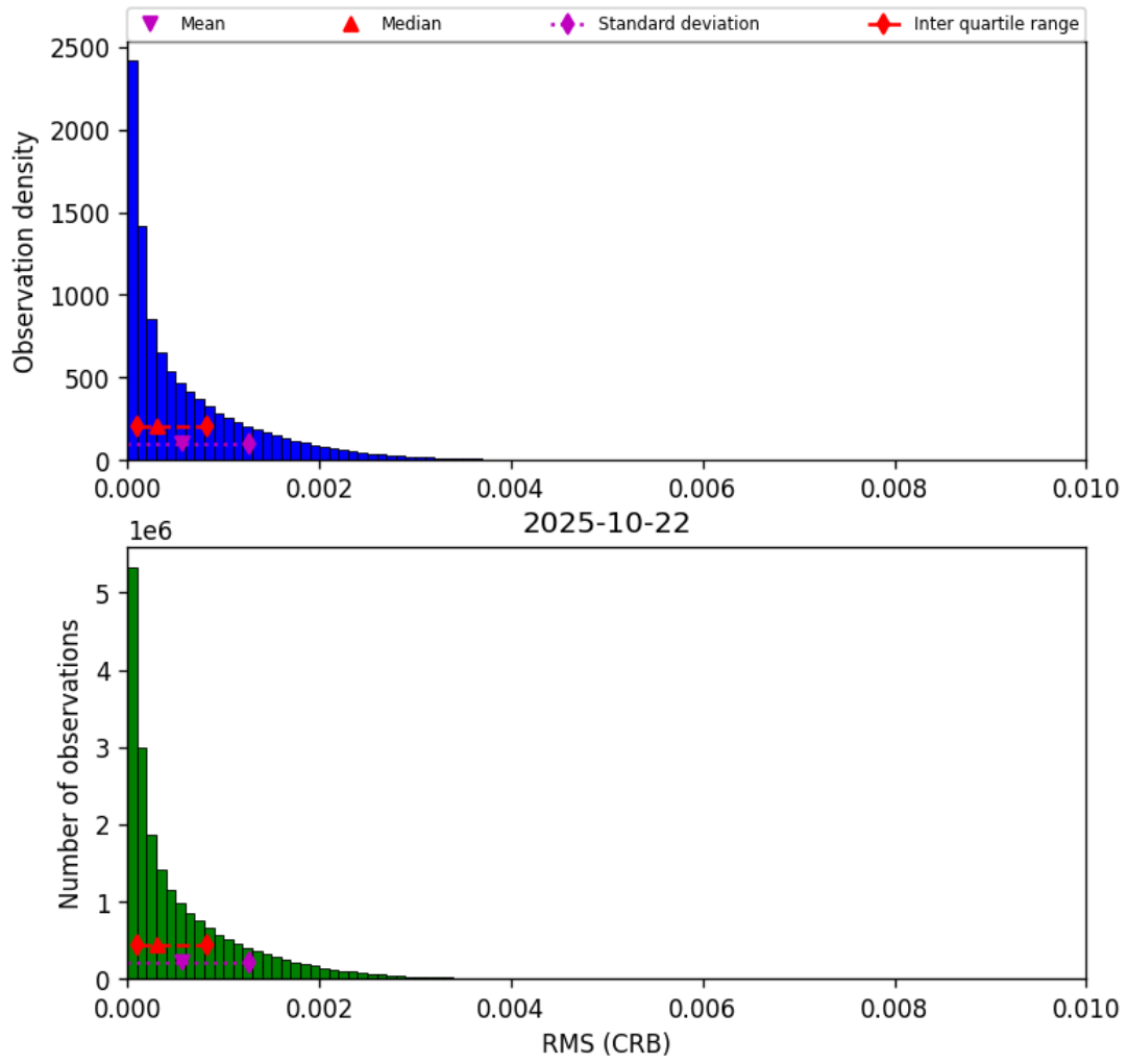
Figure 48: Histogram of “RMS (CRB)” for 2025-10-22 to 2025-10-23
