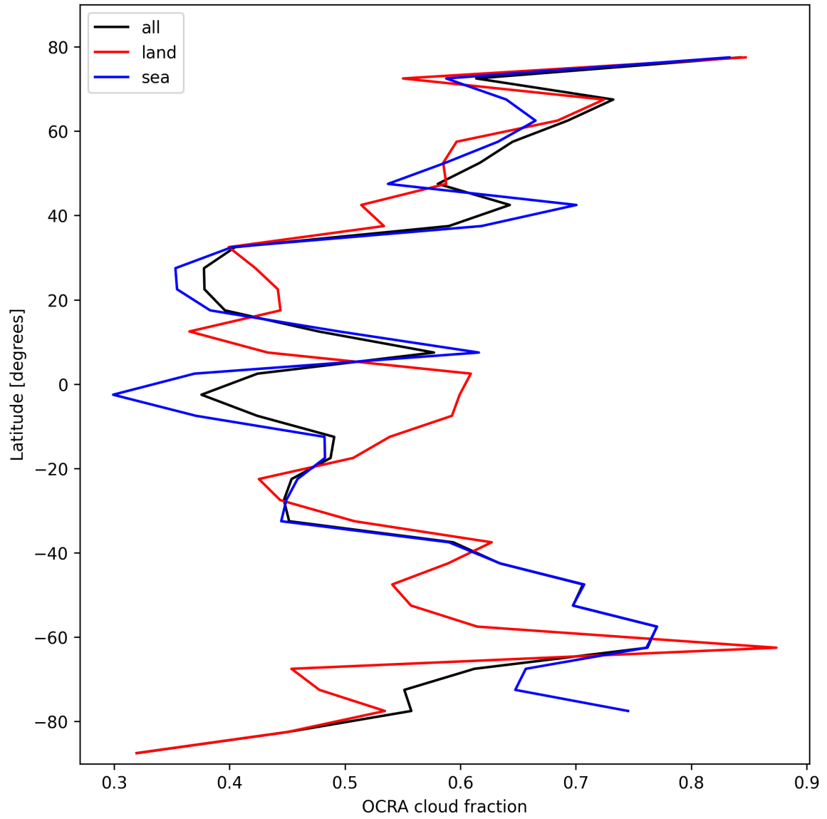
Figure 34: Zonal average of “OCRA cloud fraction” for 2025-10-22 to 2025-10-23.
