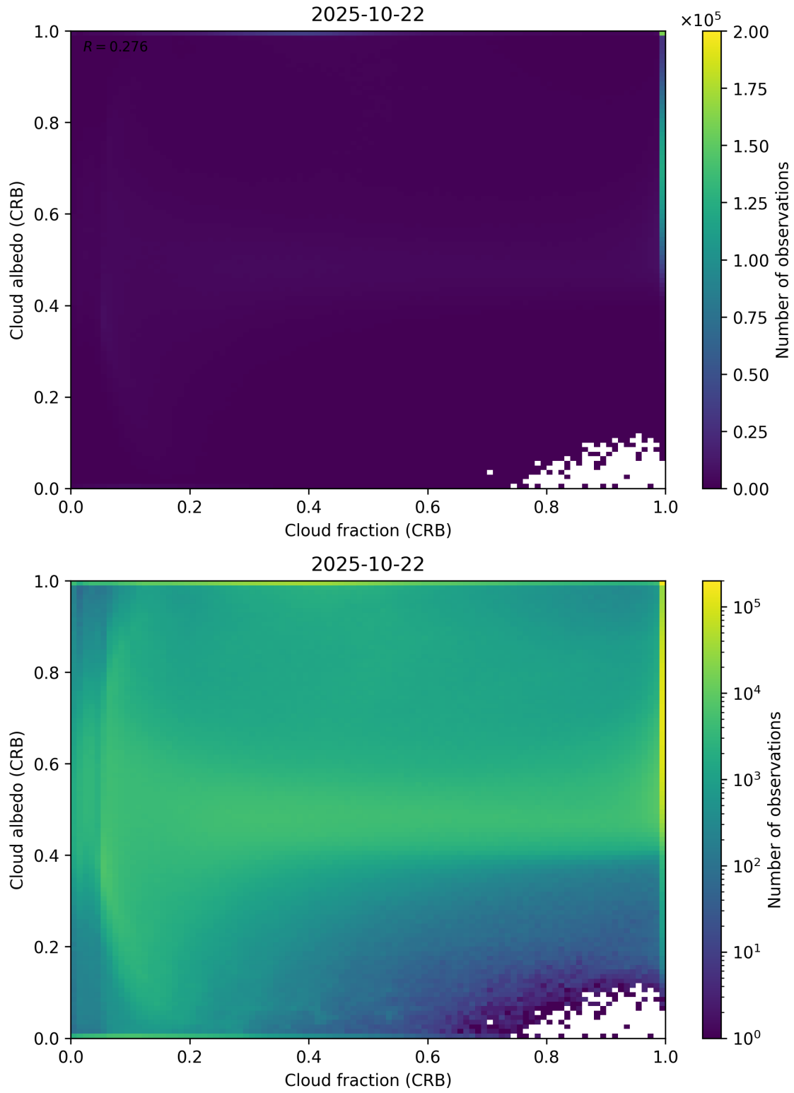
Figure 77: Scatter density plot of “Cloud fraction (CRB)” against “Cloud albedo (CRB)” for 2025-10-22 to 2025-10-23.
