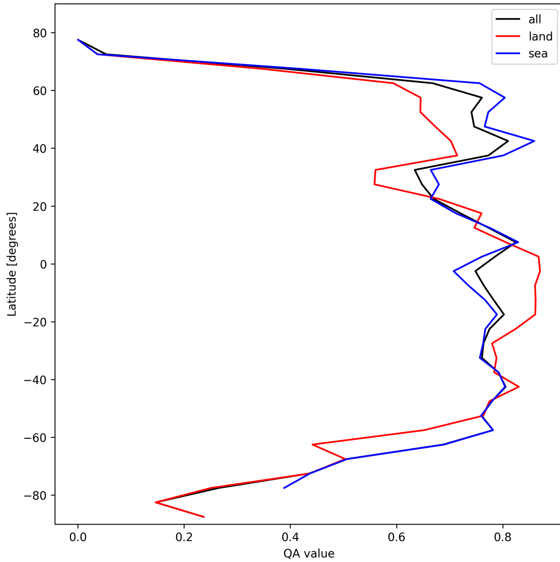
Figure 22: Zonal average of “QA value” for 2025-10-22 to 2025-10-23.
