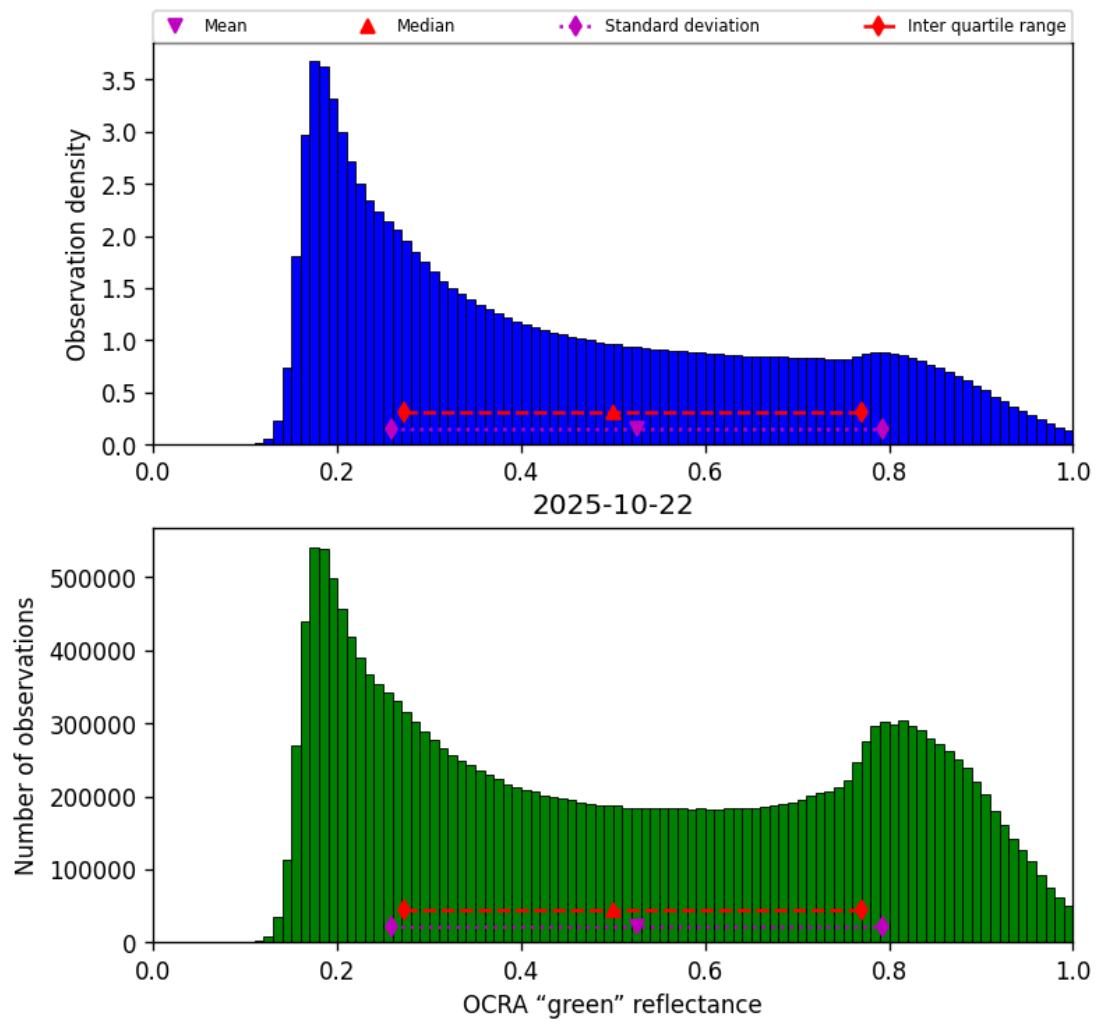
Figure 52: Histogram of “OCRA “green” reflectance” for 2025-10-22 to 2025-10-23
