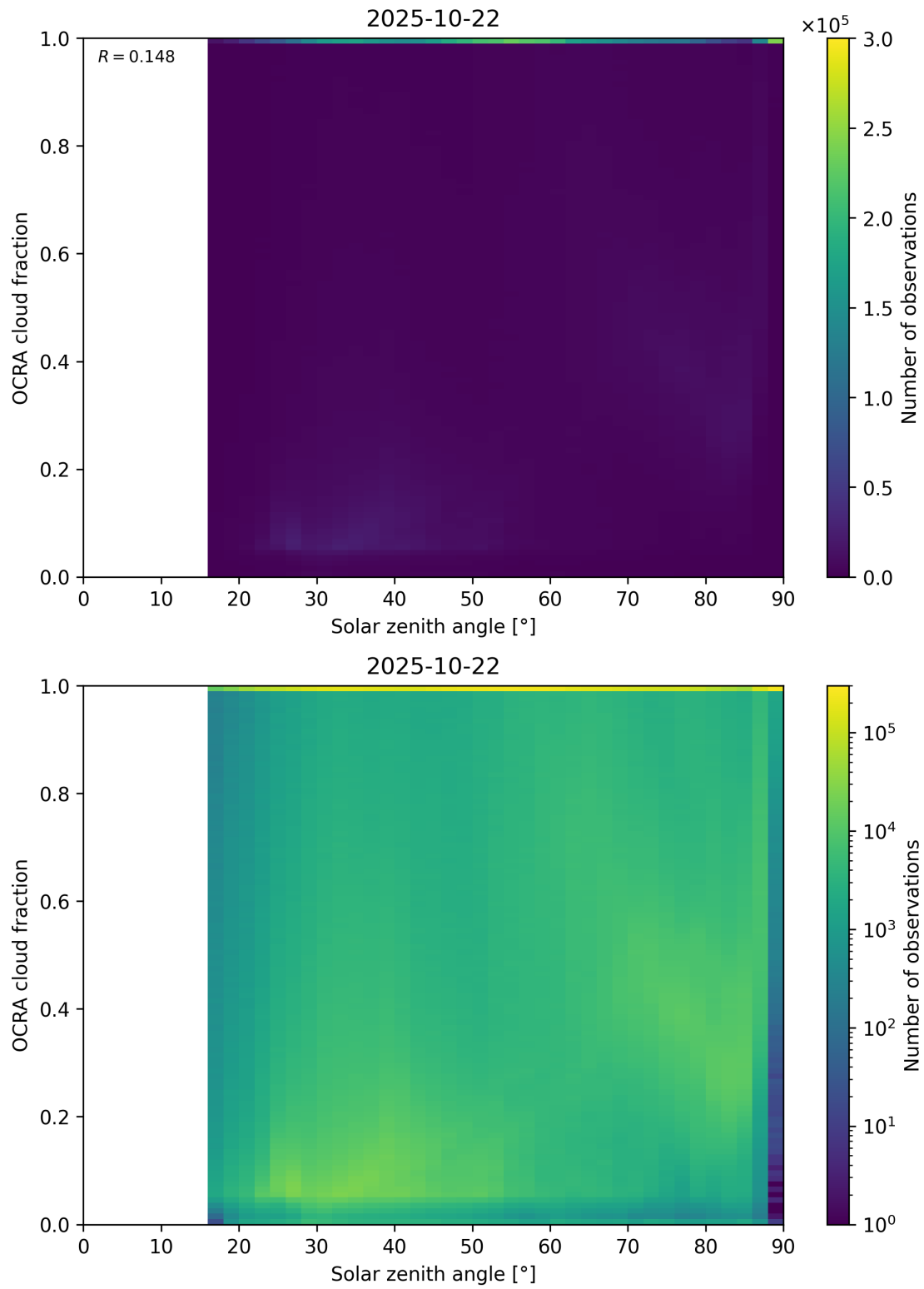
Figure 100: Scatter density plot of “Solar zenith angle” against “OCRA cloud fraction” for 2025-10-22 to 2025-10-23.
