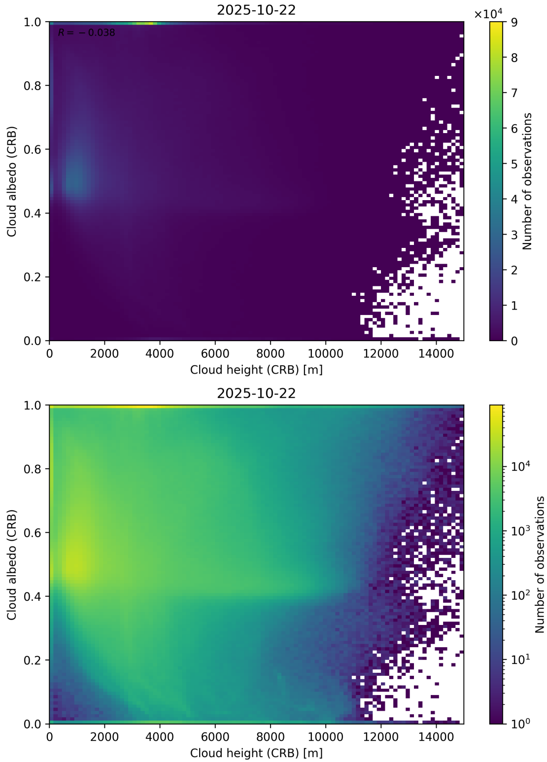
Figure 80: Scatter density plot of “Cloud height (CRB)” against “Cloud albedo (CRB)” for 2025-10-22 to 2025-10-23.
