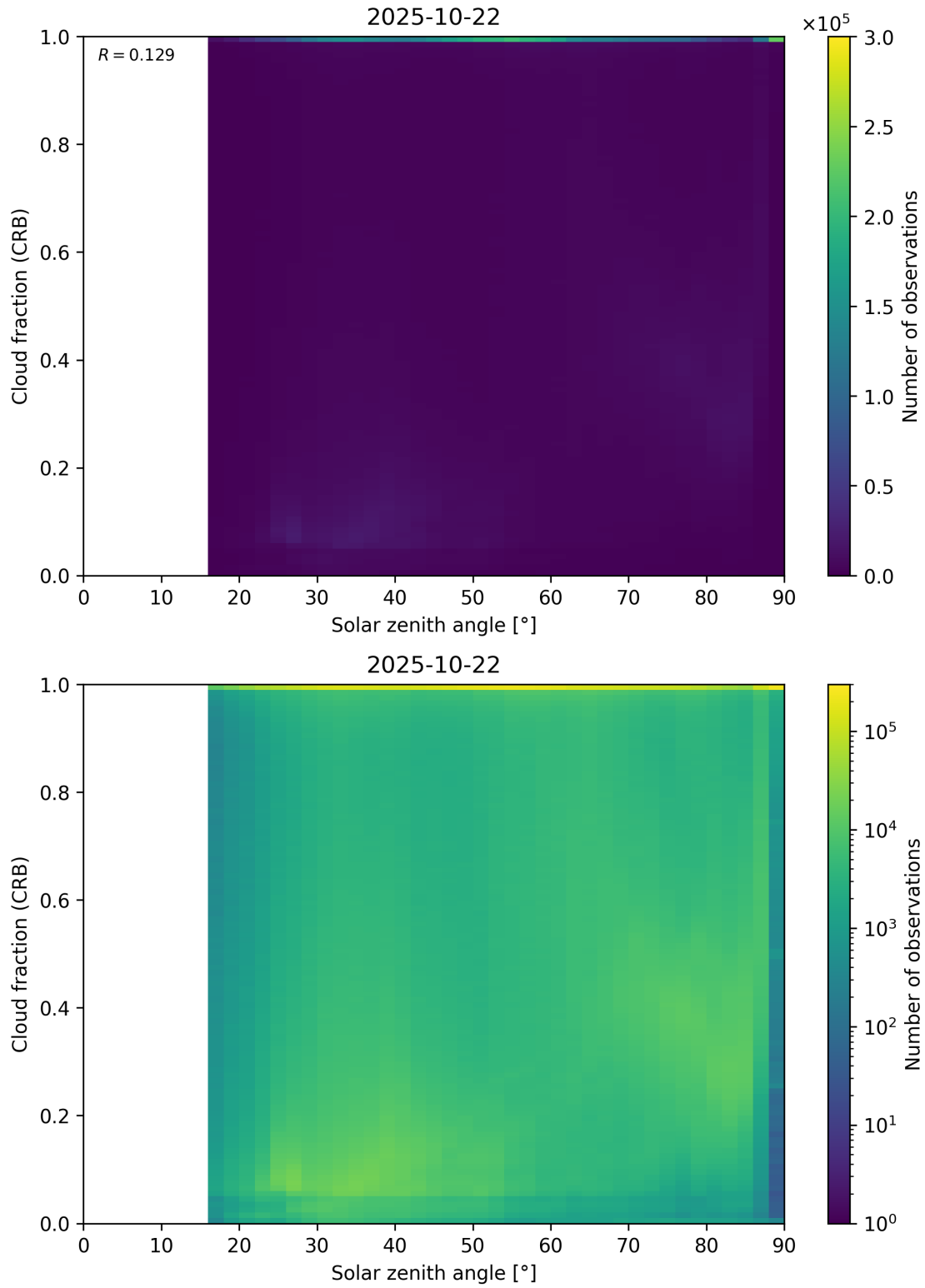
Figure 101: Scatter density plot of “Solar zenith angle” against “Cloud fraction (CRB)” for 2025-10-22 to 2025-10-23.
