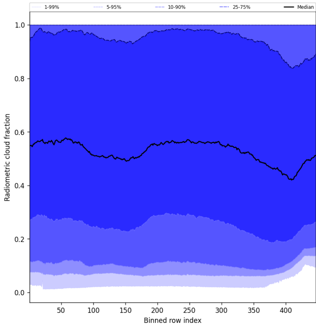
Figure 55: Along track statistics of “Radiometric cloud fraction” for 2025-10-22 to 2025-10-23
