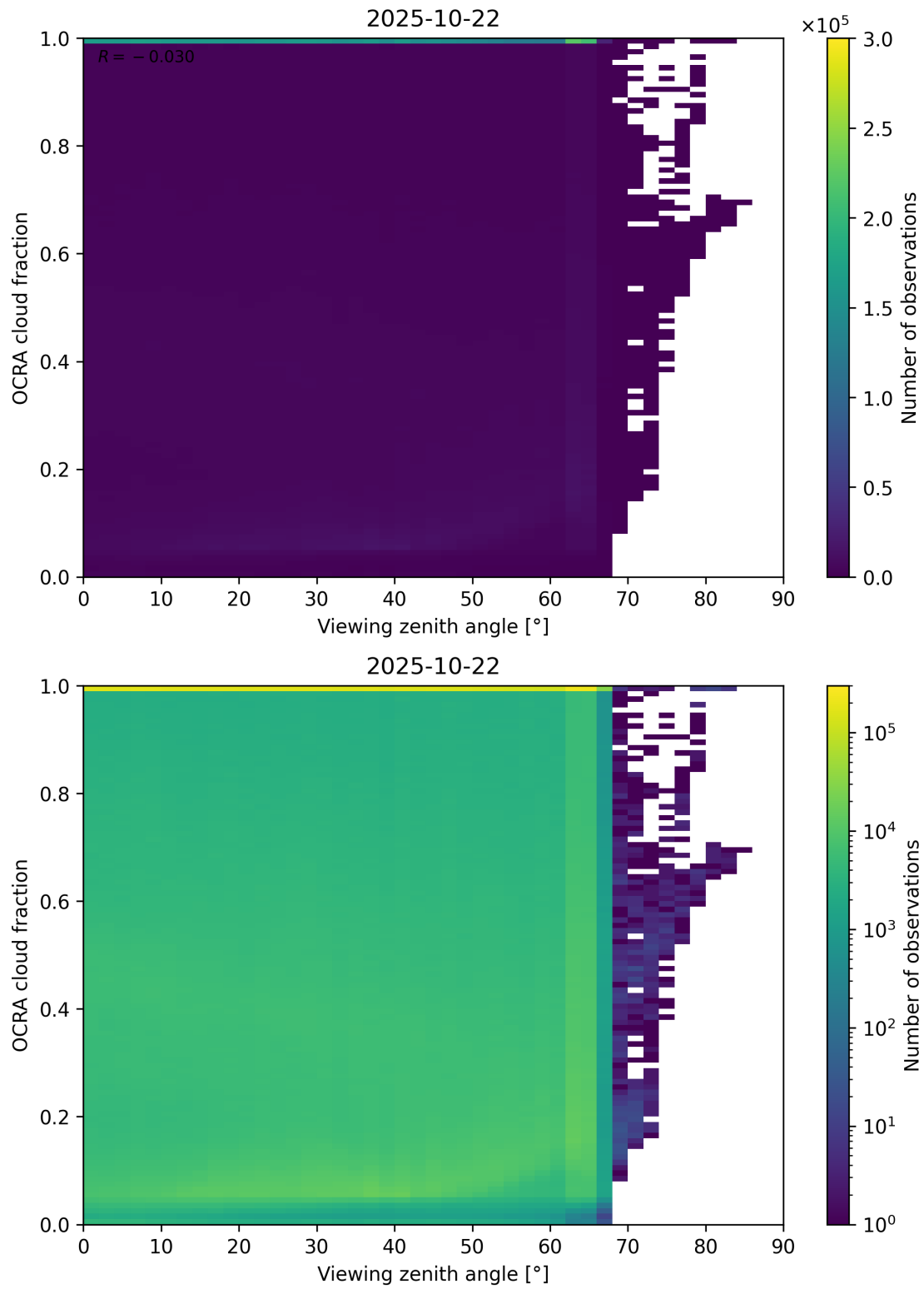
Figure 108: Scatter density plot of “Viewing zenith angle” against “OCRA cloud fraction” for 2025-10-22 to 2025-10-23.
