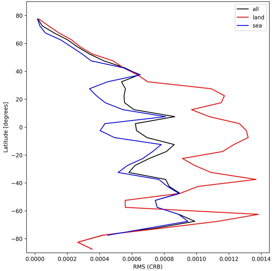
Figure 32: Zonal average of “RMS (CRB)” for 2025-10-22 to 2025-10-23.
