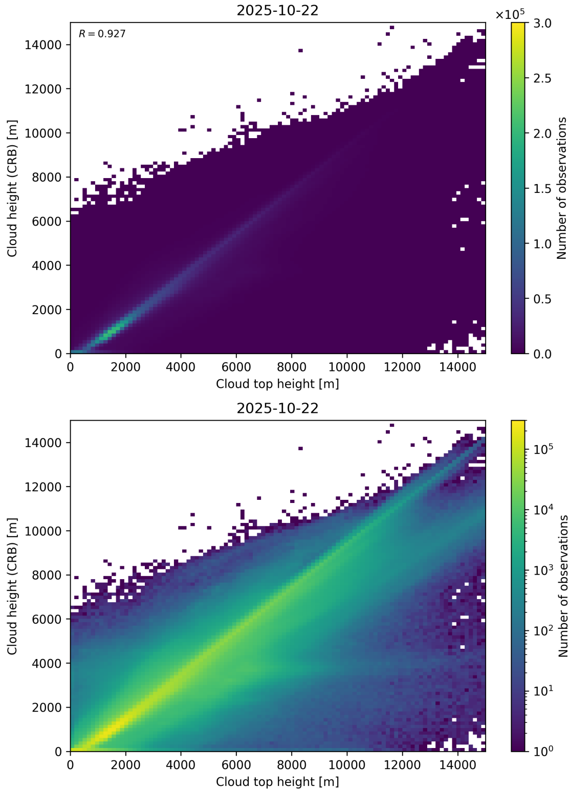
Figure 89: Scatter density plot of “Cloud top height” against “Cloud height (CRB)” for 2025-10-22 to 2025-10-23.
