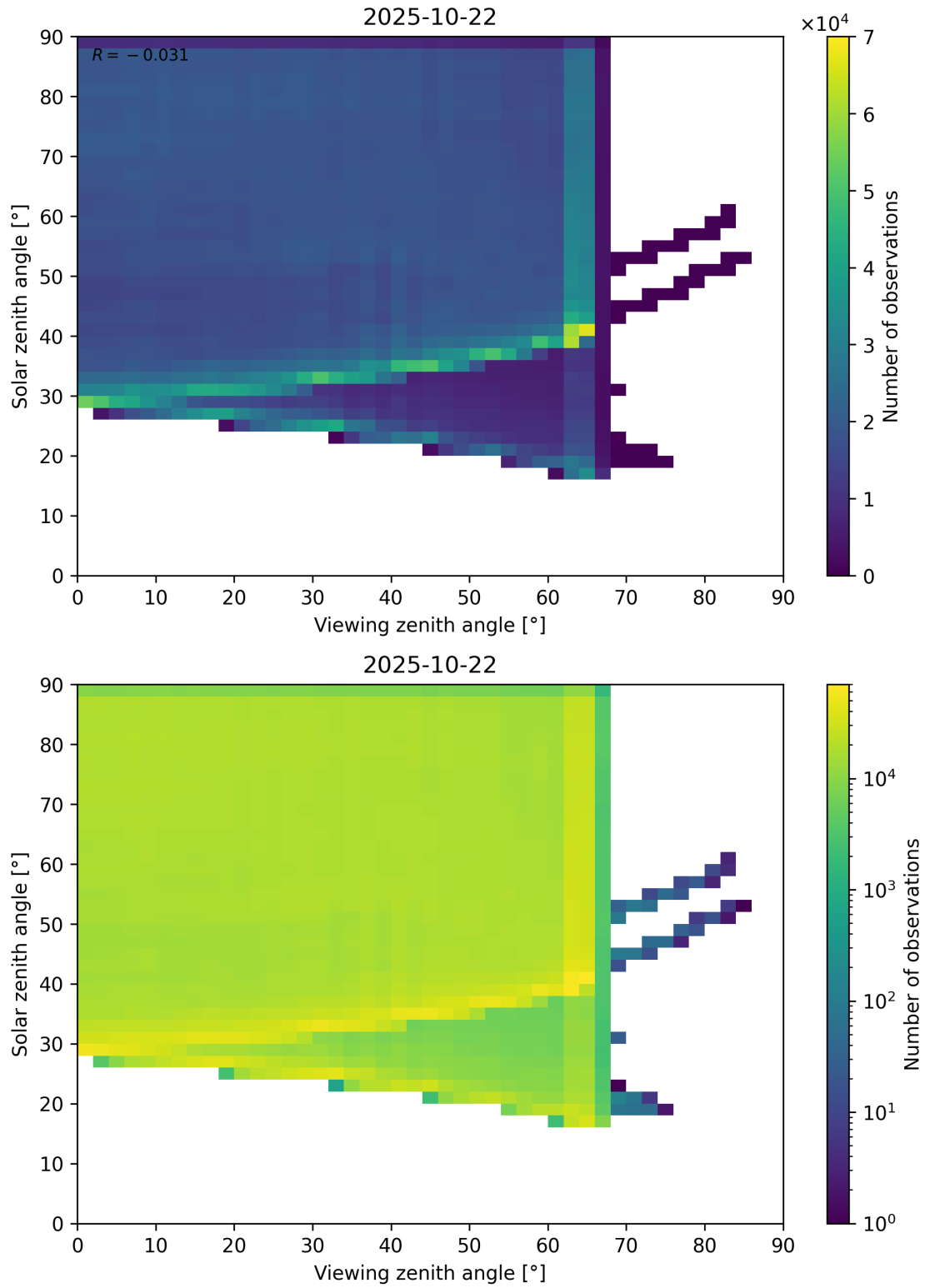
Figure 114: Scatter density plot of “Viewing zenith angle” against “Solar zenith angle” for 2025-10-22 to 2025-10-23.
