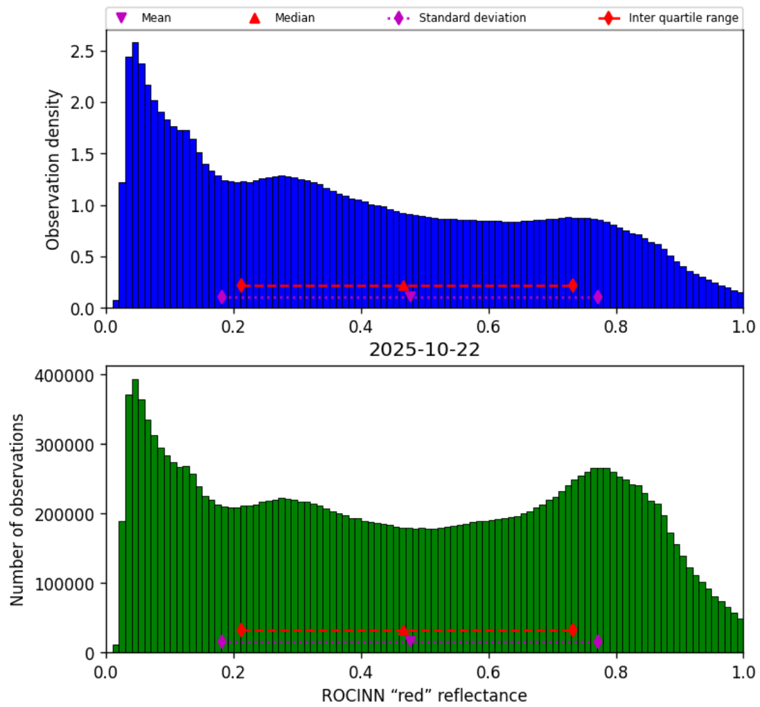
Figure 53: Histogram of “ROCINN “red” reflectance” for 2025-10-22 to 2025-10-23
