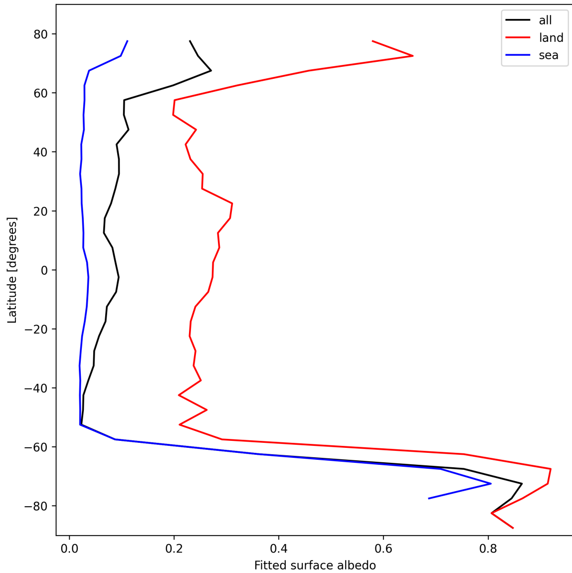
Figure 29: Zonal average of “Fitted surface albedo” for 2025-10-22 to 2025-10-23.
