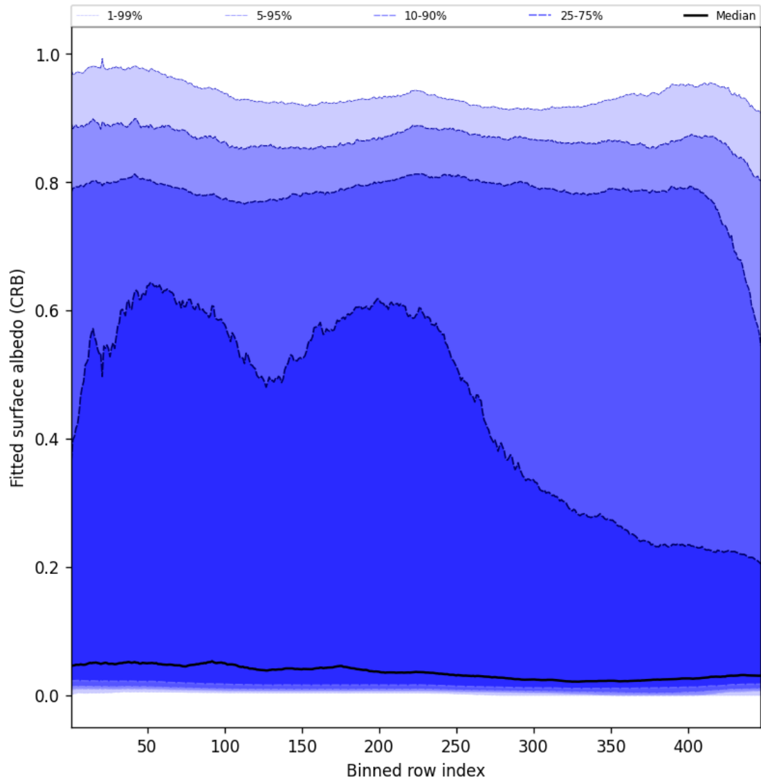
Figure 62: Along track statistics of “Fitted surface albedo (CRB)” for 2025-10-22 to 2025-10-23
