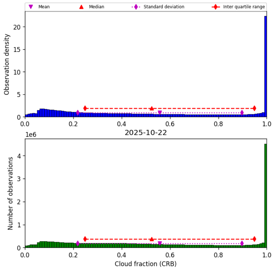
Figure 42: Histogram of “Cloud fraction (CRB)” for 2025-10-22 to 2025-10-23
