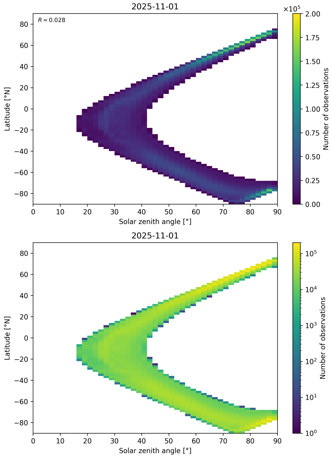
Figure 105: Scatter density plot of “Solar zenith angle” against “Latitude” for 2025-10-31 to 2025-11-02.
