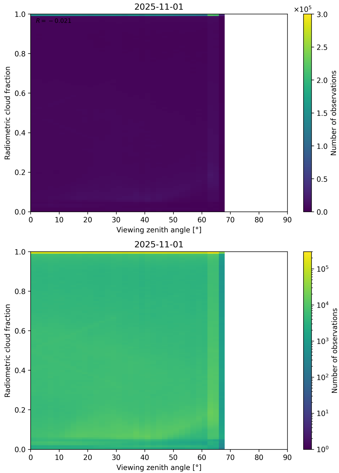
Figure 107: Scatter density plot of “Viewing zenith angle” against “Radiometric cloud fraction” for 2025-10-31 to 2025-11-02.
