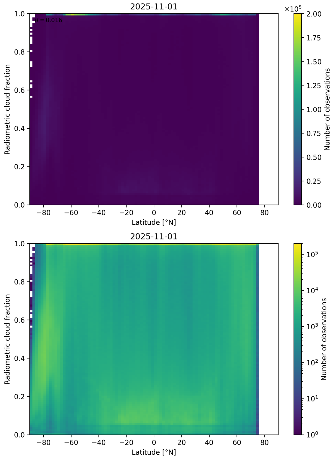
Figure 92: Scatter density plot of “Latitude” against “Radiometric cloud fraction” for 2025-10-31 to 2025-11-02.
