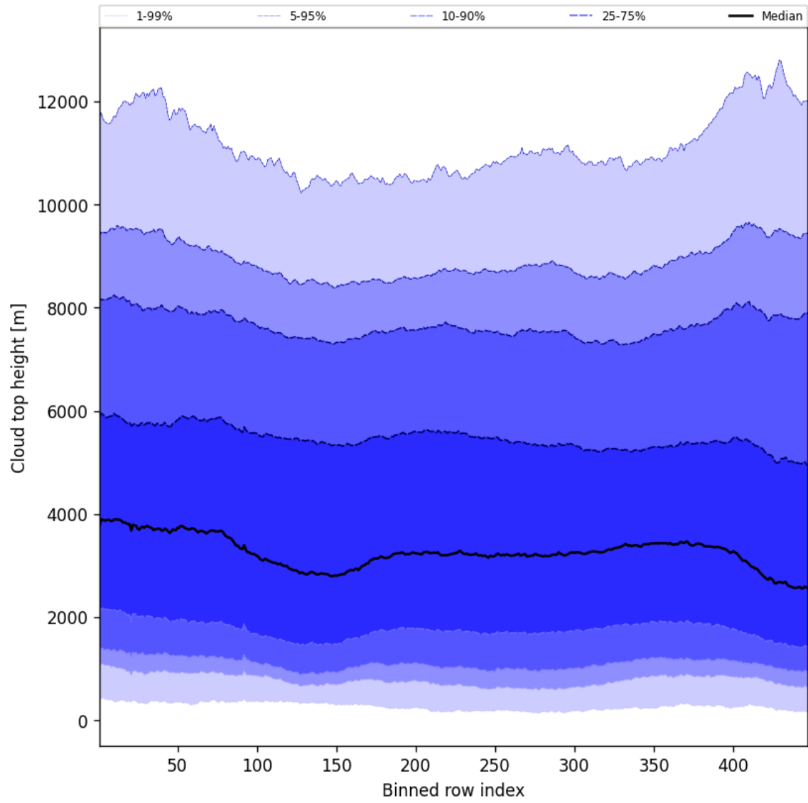
Figure 56: Along track statistics of “Cloud top height” for 2025-10-31 to 2025-11-02
