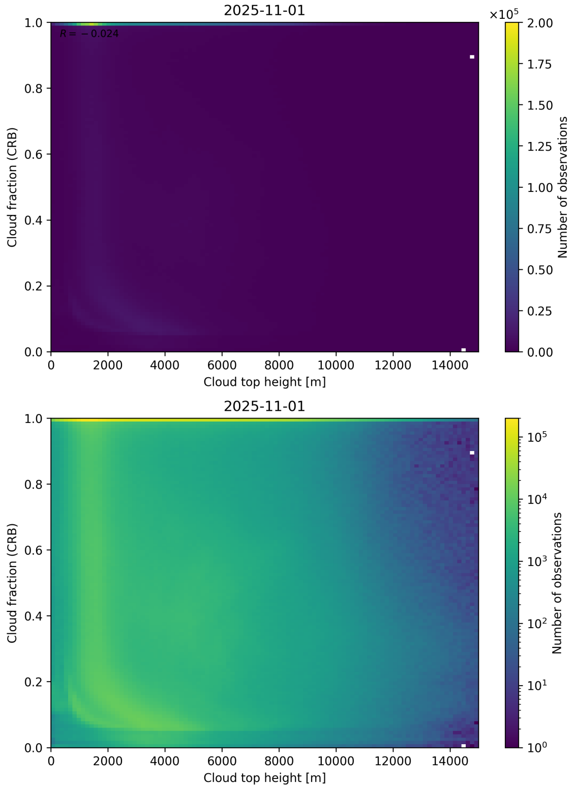
Figure 88: Scatter density plot of “Cloud top height” against “Cloud fraction (CRB)” for 2025-10-31 to 2025-11-02.
