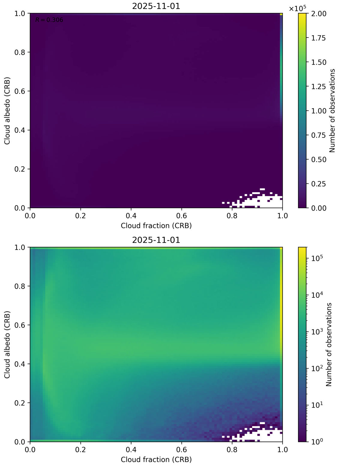
Figure 77: Scatter density plot of “Cloud fraction (CRB)” against “Cloud albedo (CRB)” for 2025-10-31 to 2025-11-02.
