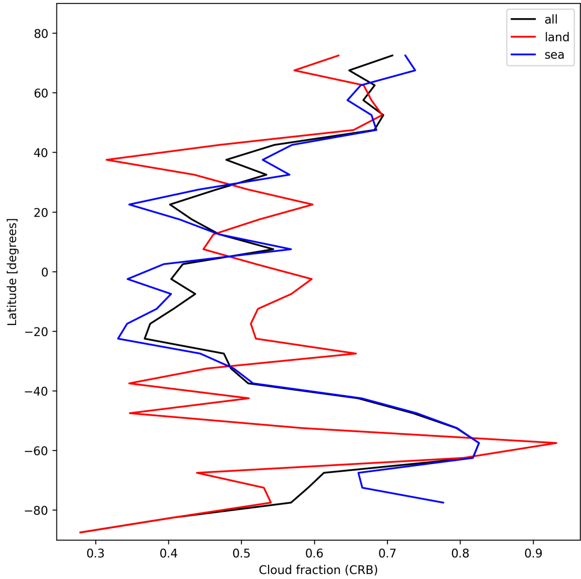
Figure 26: Zonal average of “Cloud fraction (CRB)” for 2025-10-31 to 2025-11-02.
