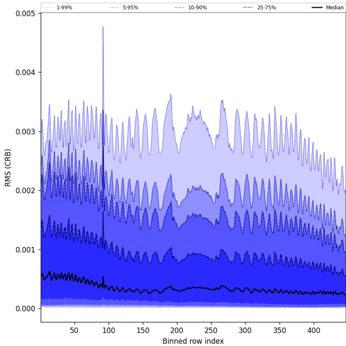
Figure 64: Along track statistics of “RMS (CRB)” for 2025-10-31 to 2025-11-02
