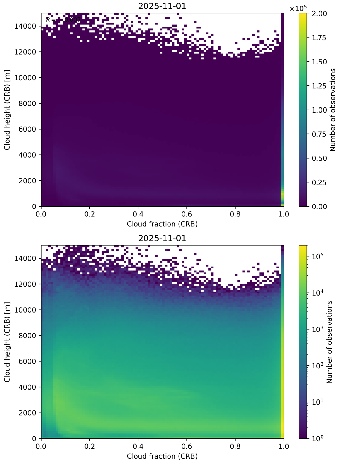
Figure 79: Scatter density plot of “Cloud fraction (CRB)” against “Cloud height (CRB)” for 2025-10-31 to 2025-11-02.
