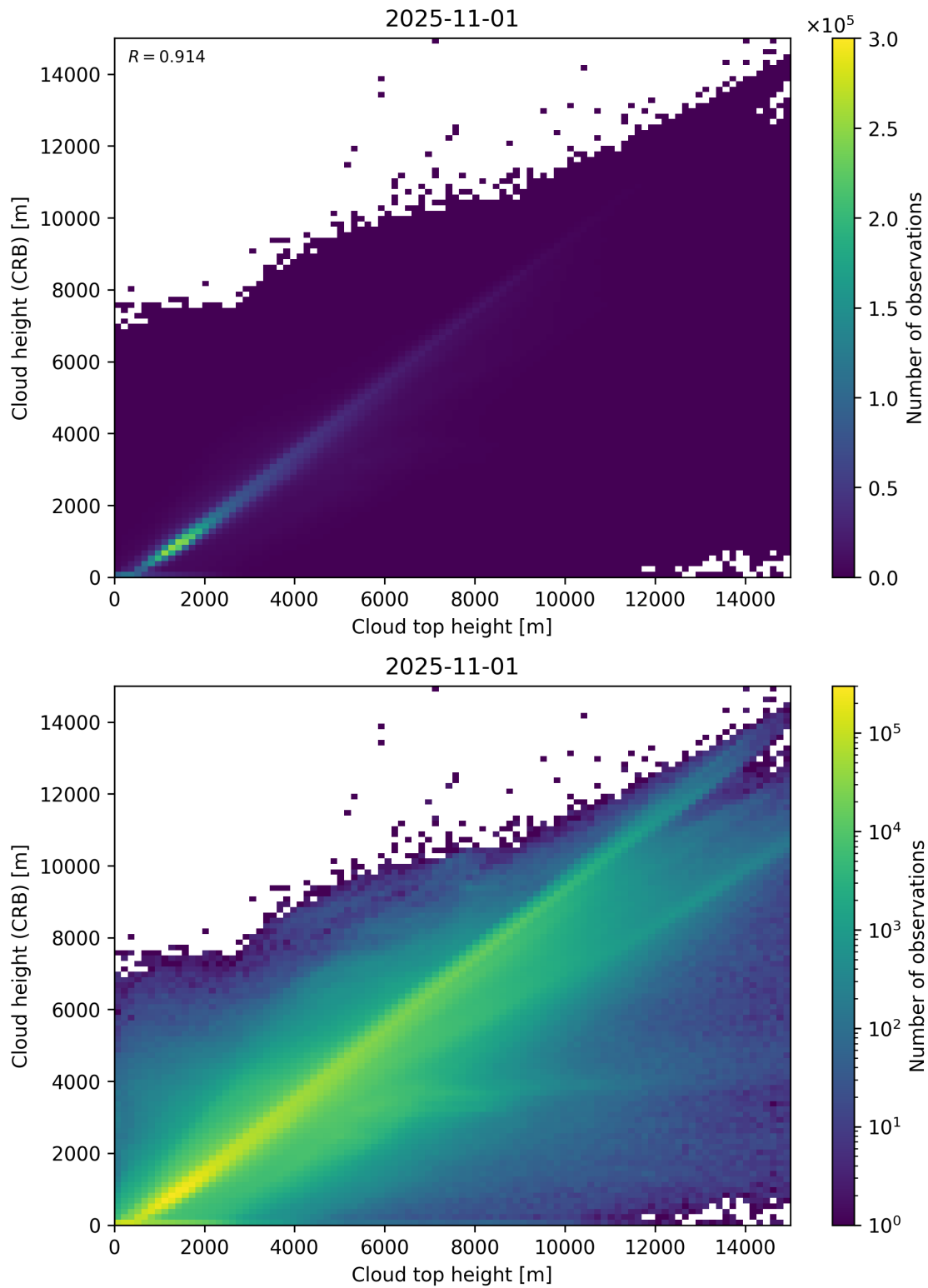
Figure 89: Scatter density plot of “Cloud top height” against “Cloud height (CRB)” for 2025-10-31 to 2025-11-02.
