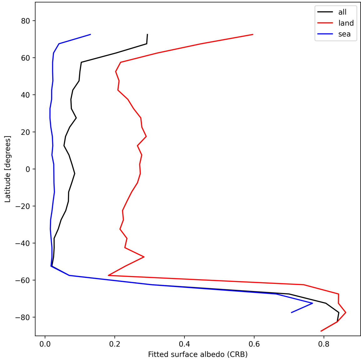
Figure 30: Zonal average of “Fitted surface albedo (CRB)” for 2025-10-31 to 2025-11-02.
