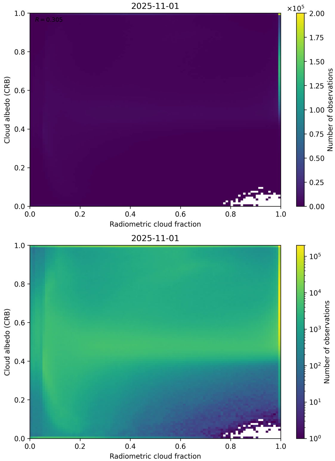
Figure 71: Scatter density plot of “Radiometric cloud fraction” against “Cloud albedo (CRB)” for 2025-10-31 to 2025-11-02.
