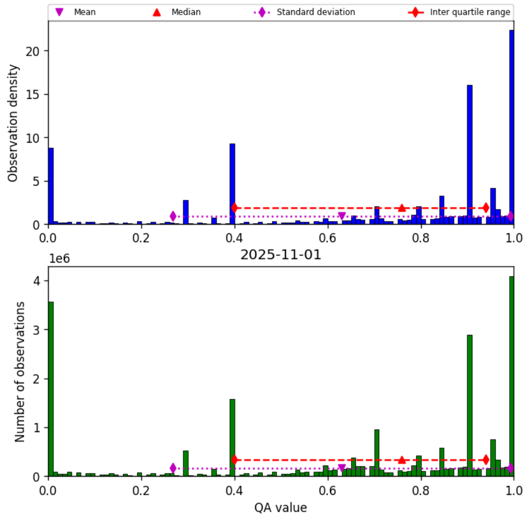
Figure 38: Histogram of “QA value” for 2025-10-31 to 2025-11-02
