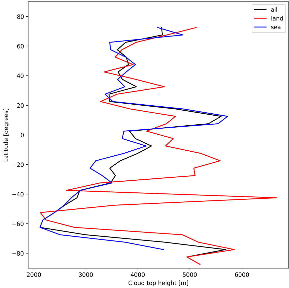
Figure 24: Zonal average of “Cloud top height” for 2025-10-31 to 2025-11-02.
