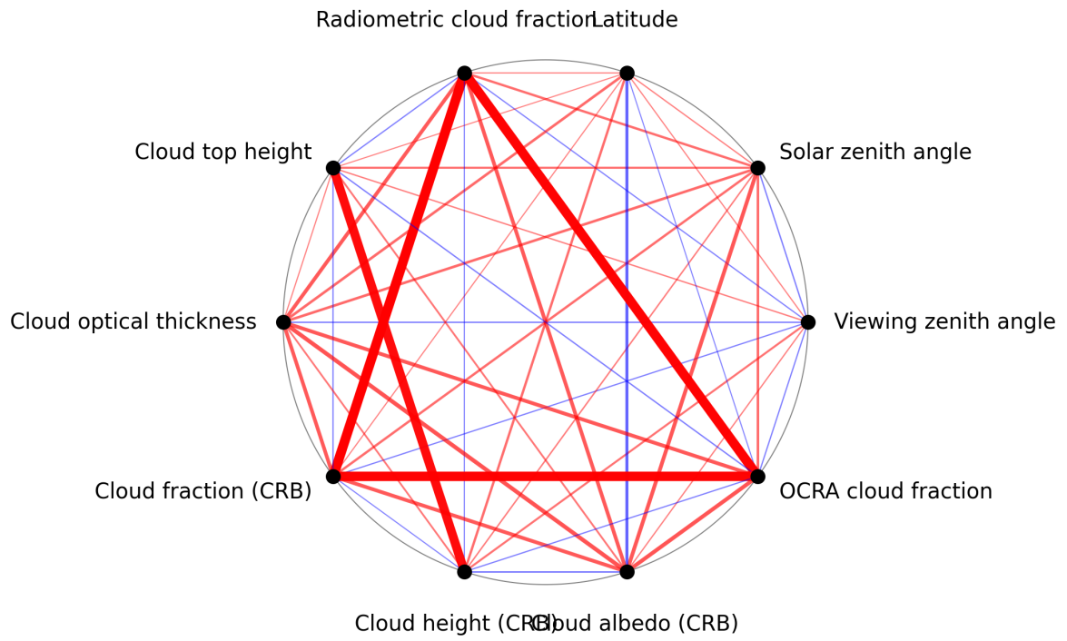
Figure 1: Map of correlation graph for 2025-10-31 to 2025-11-02.
