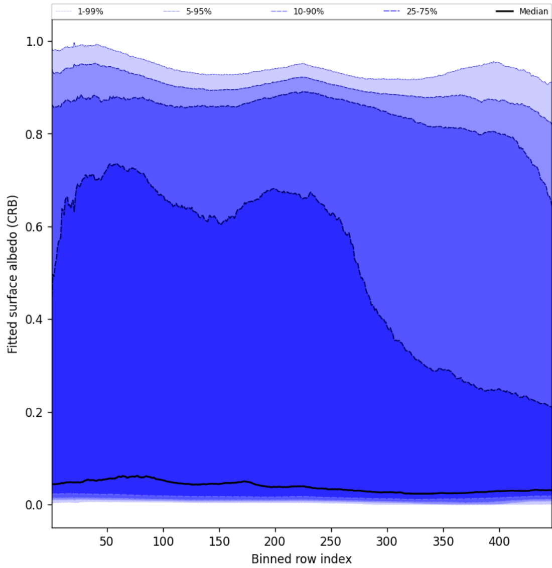
Figure 62: Along track statistics of “Fitted surface albedo (CRB)” for 2025-10-31 to 2025-11-02
