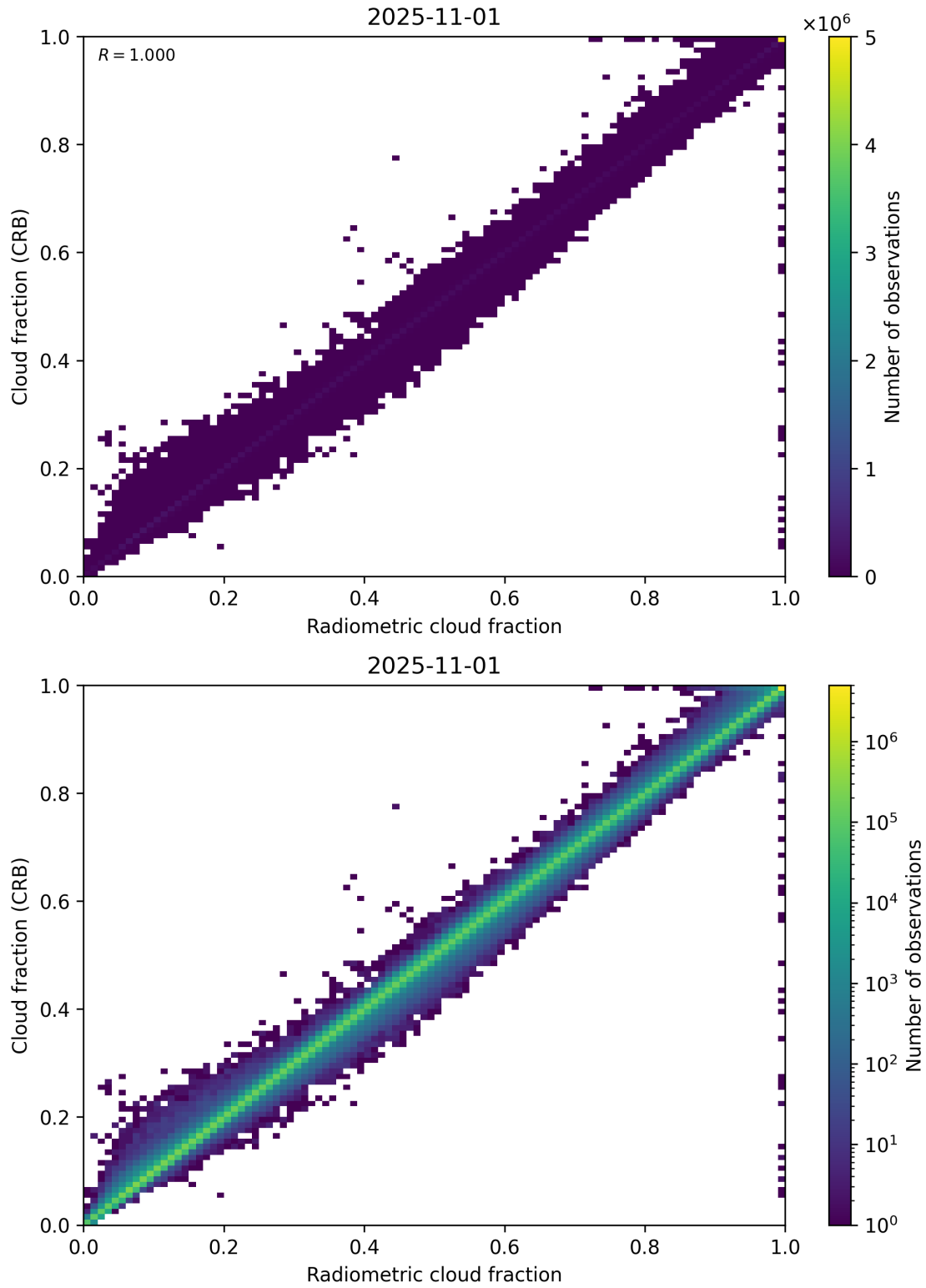
Figure 73: Scatter density plot of “Radiometric cloud fraction” against “Cloud fraction (CRB)” for 2025-10-31 to 2025-11-02.
