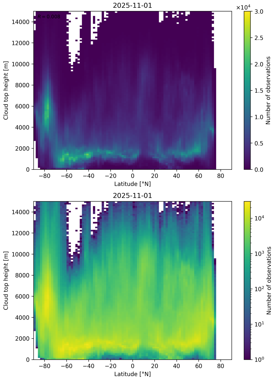
Figure 97: Scatter density plot of “Latitude” against “Cloud top height” for 2025-10-31 to 2025-11-02.
