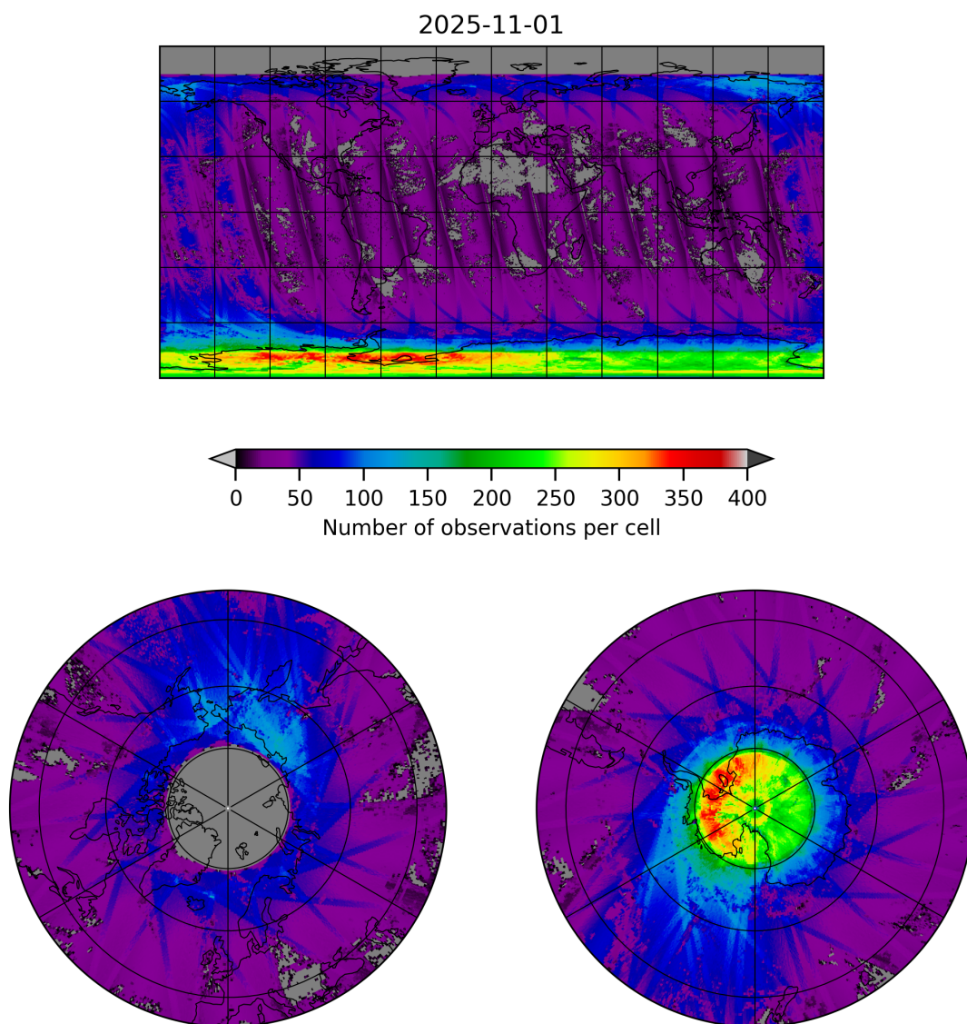
Figure 21: Map of the number of observations for 2025-10-31 to 2025-11-02
