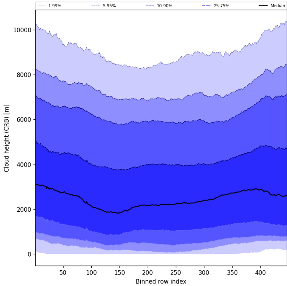
Figure 59: Along track statistics of “Cloud height (CRB)” for 2025-10-31 to 2025-11-02
