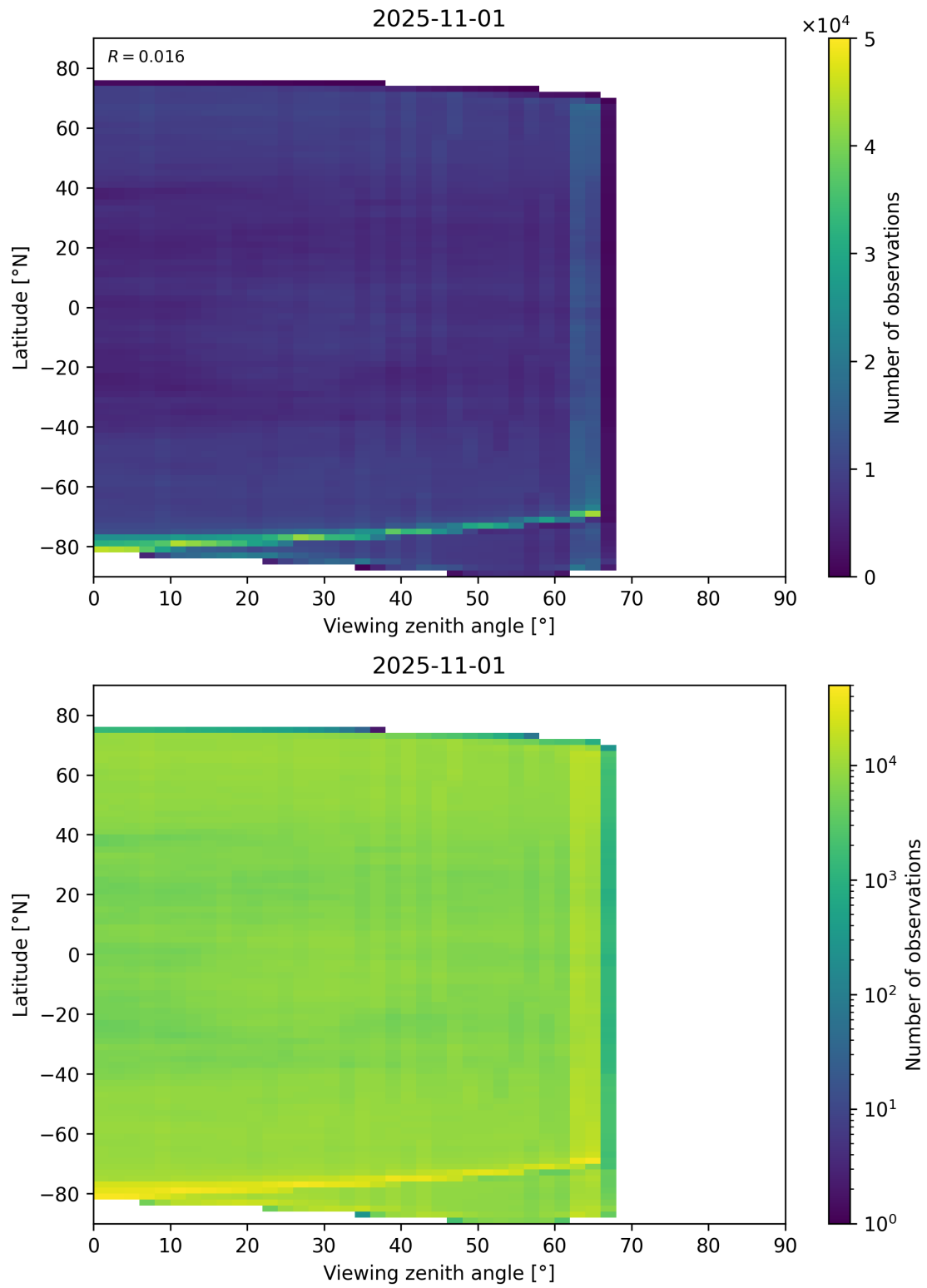
Figure 113: Scatter density plot of “Viewing zenith angle” against “Latitude” for 2025-10-31 to 2025-11-02.
