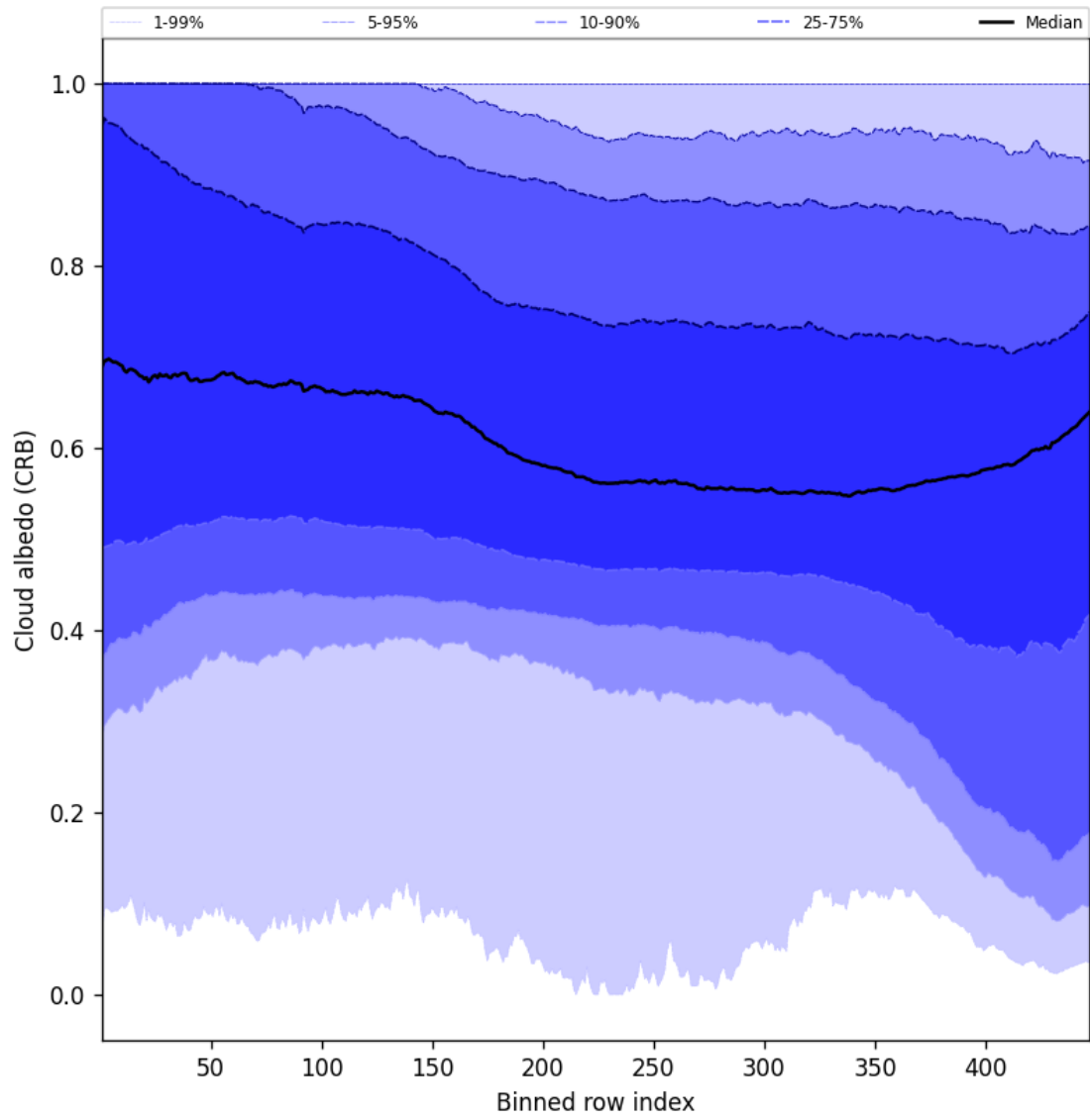
Figure 60: Along track statistics of “Cloud albedo (CRB)” for 2025-10-31 to 2025-11-02
