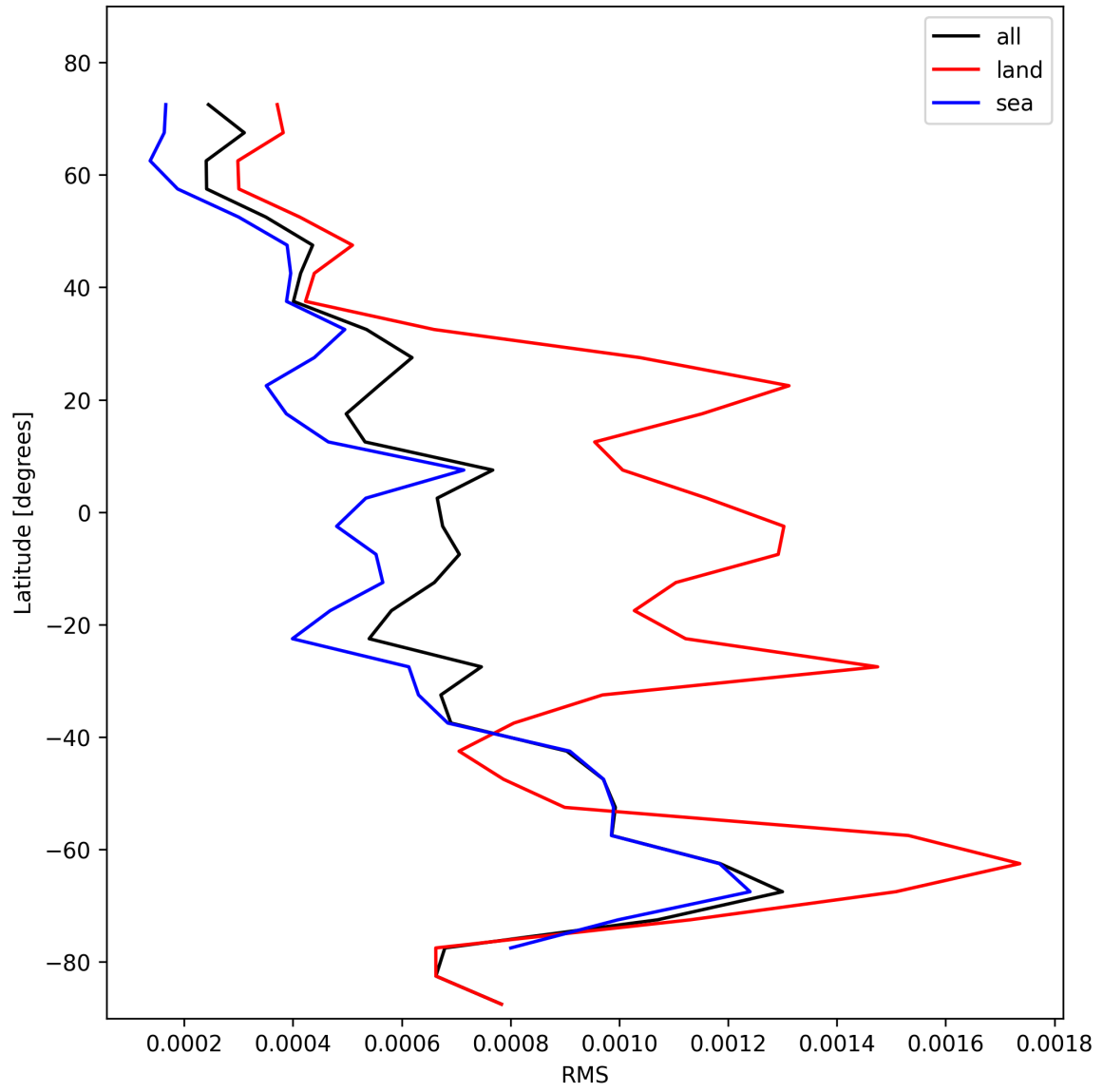
Figure 31: Zonal average of “RMS” for 2025-10-31 to 2025-11-02.
