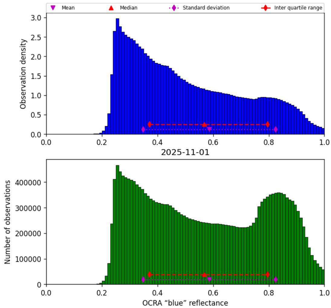
Figure 51: Histogram of "OCRA "blue" reflectance" for 2025-10-31 to 2025-11-02
