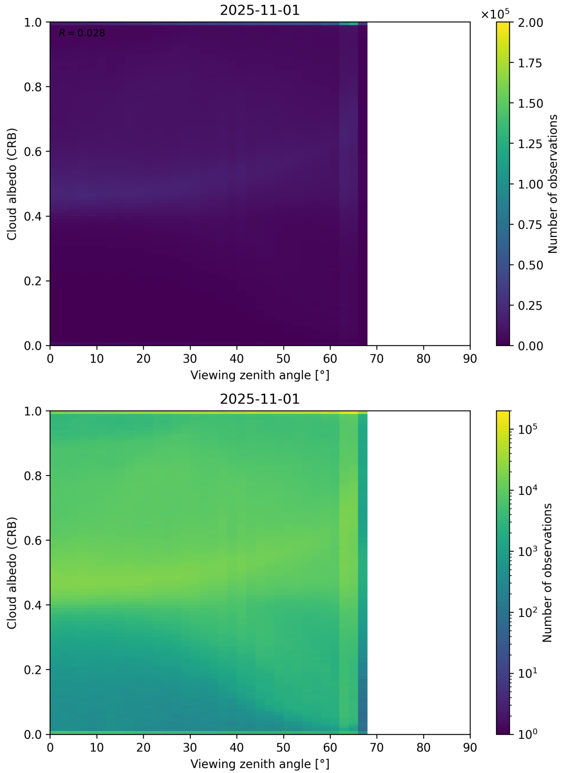
Figure 106: Scatter density plot of “Viewing zenith angle” against “Cloud albedo (CRB)” for 2025-10-31 to 2025-11-02.
