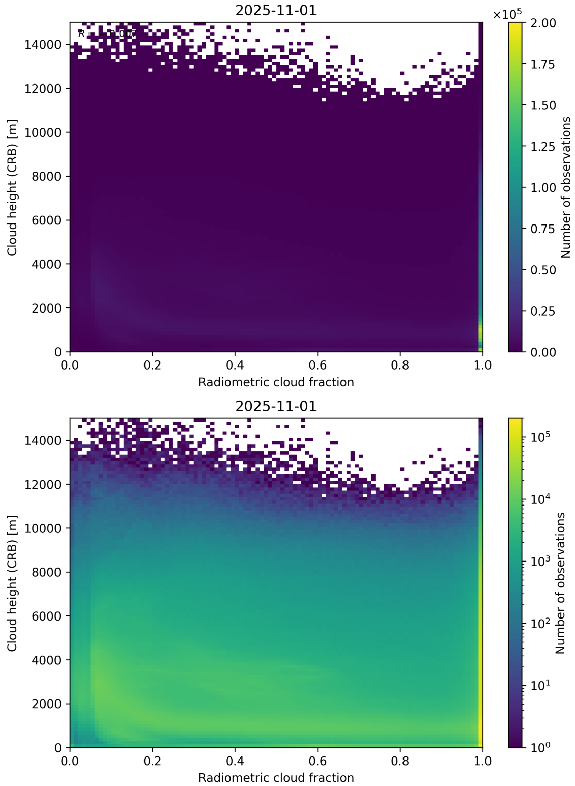
Figure 74: Scatter density plot of “Radiometric cloud fraction” against “Cloud height (CRB)” for 2025-10-31 to 2025-11-02.
