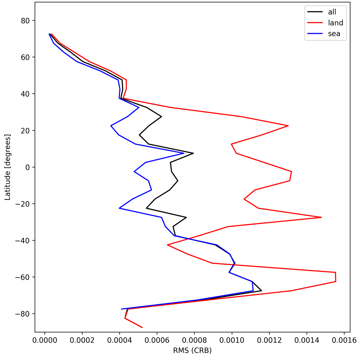
Figure 32: Zonal average of “RMS (CRB)” for 2025-10-31 to 2025-11-02.
