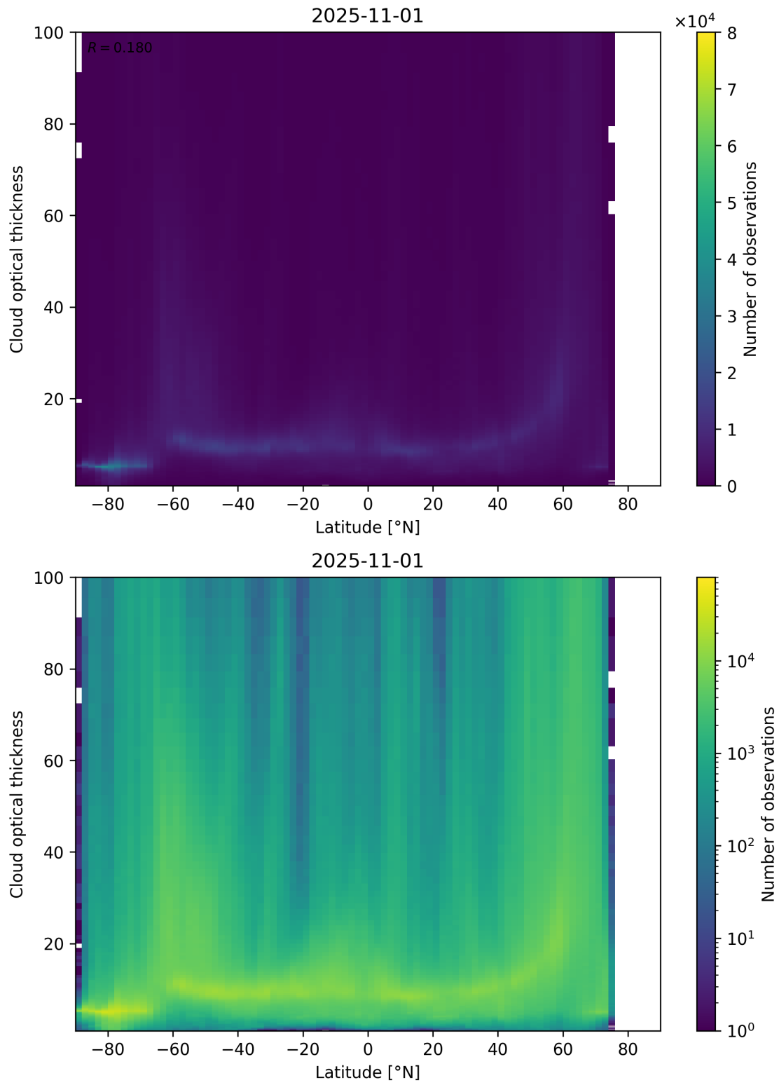
Figure 96: Scatter density plot of “Latitude” against “Cloud optical thickness” for 2025-10-31 to 2025-11-02.
