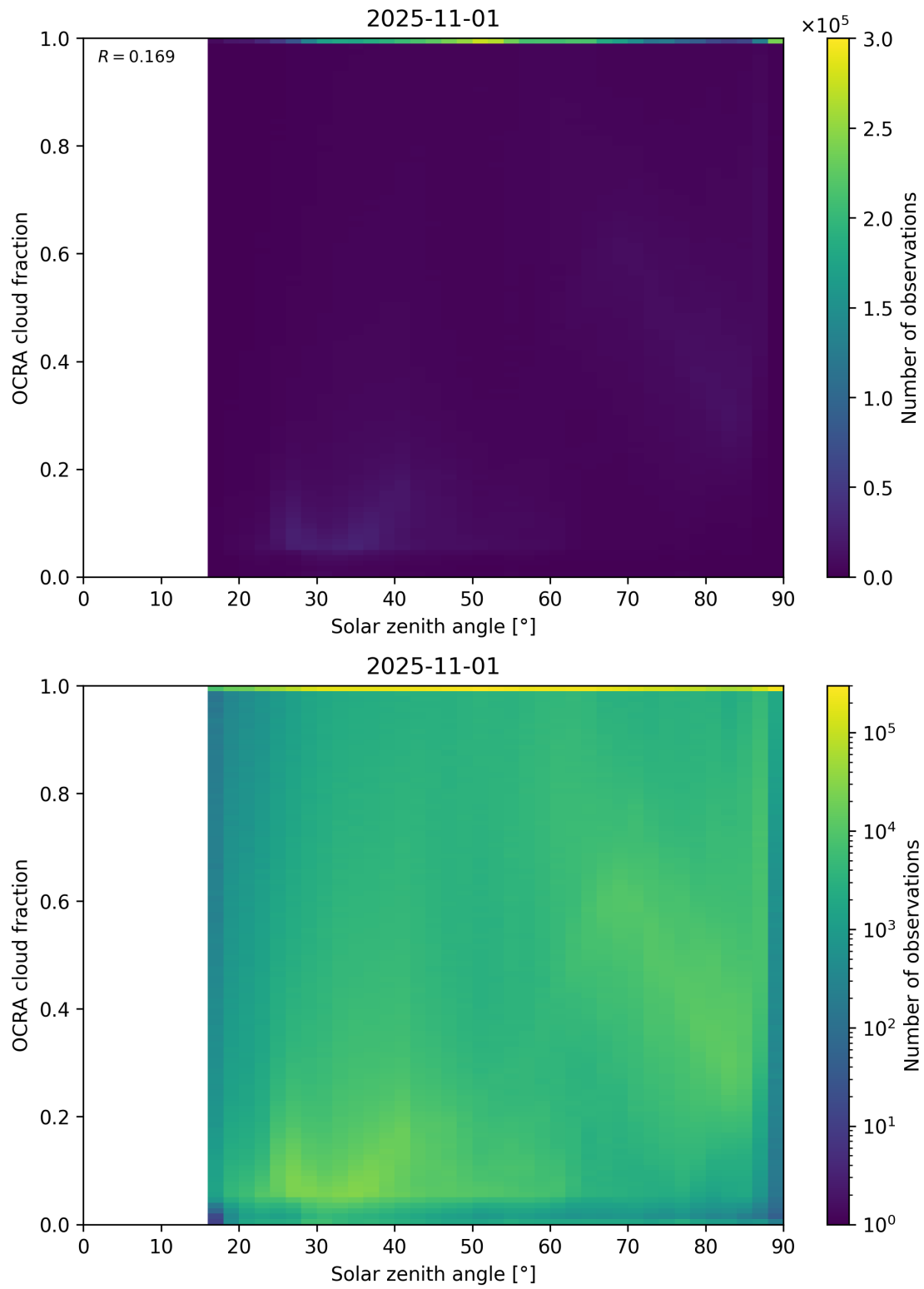
Figure 100: Scatter density plot of “Solar zenith angle” against “OCRA cloud fraction” for 2025-10-31 to 2025-11-02.
