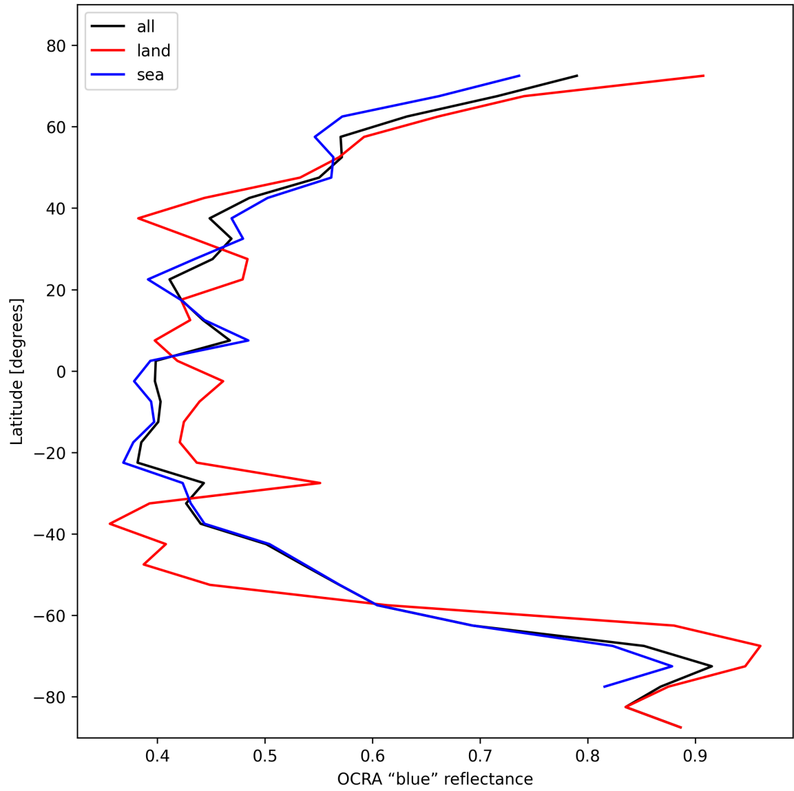
Figure 35: Zonal average of "OCRA "blue" reflectance" for 2025-10-31 to 2025-11-02.
