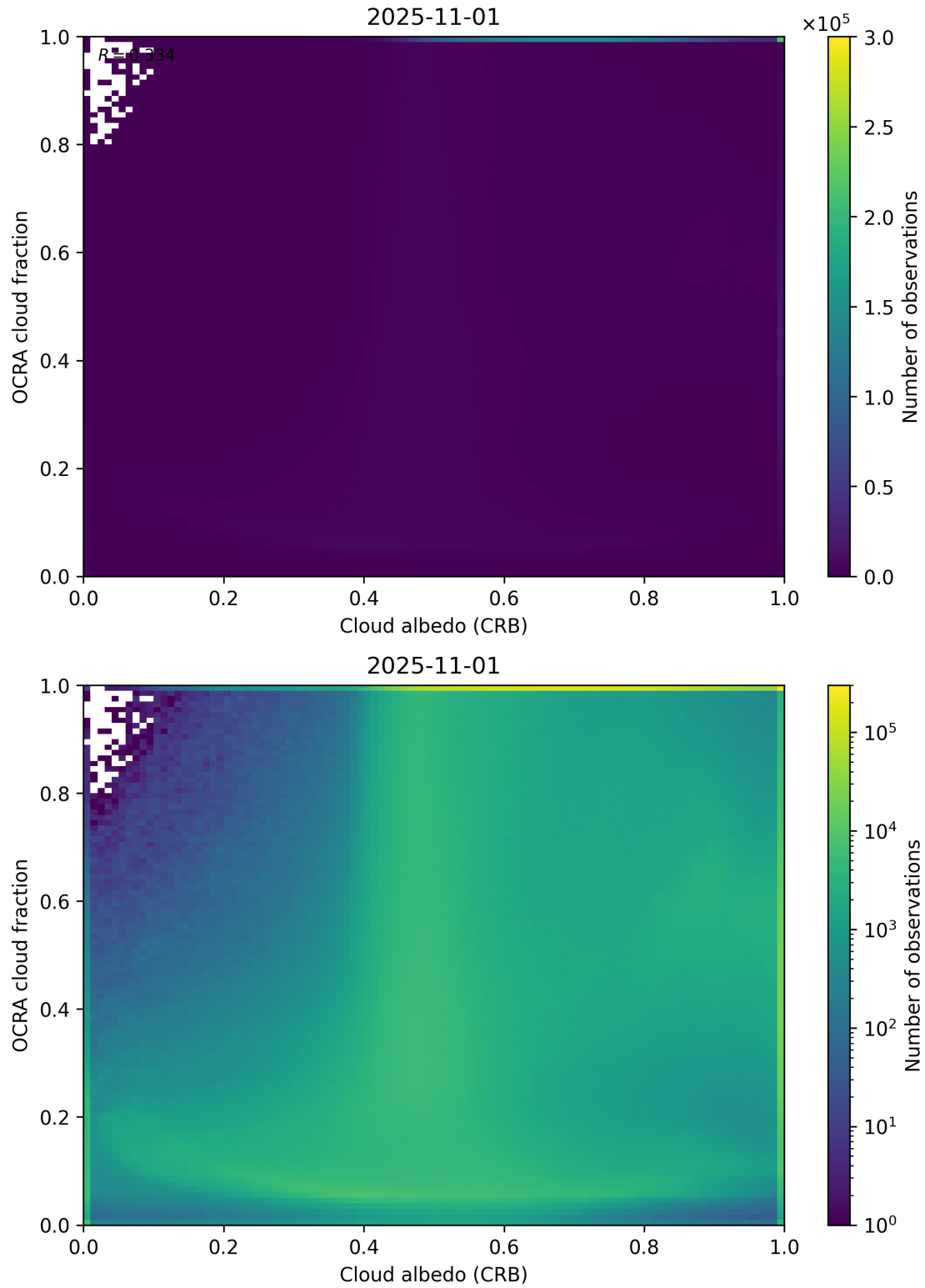
Figure 70: Scatter density plot of “Cloud albedo (CRB)” against “OCRA cloud fraction” for 2025-10-31 to 2025-11-02.
