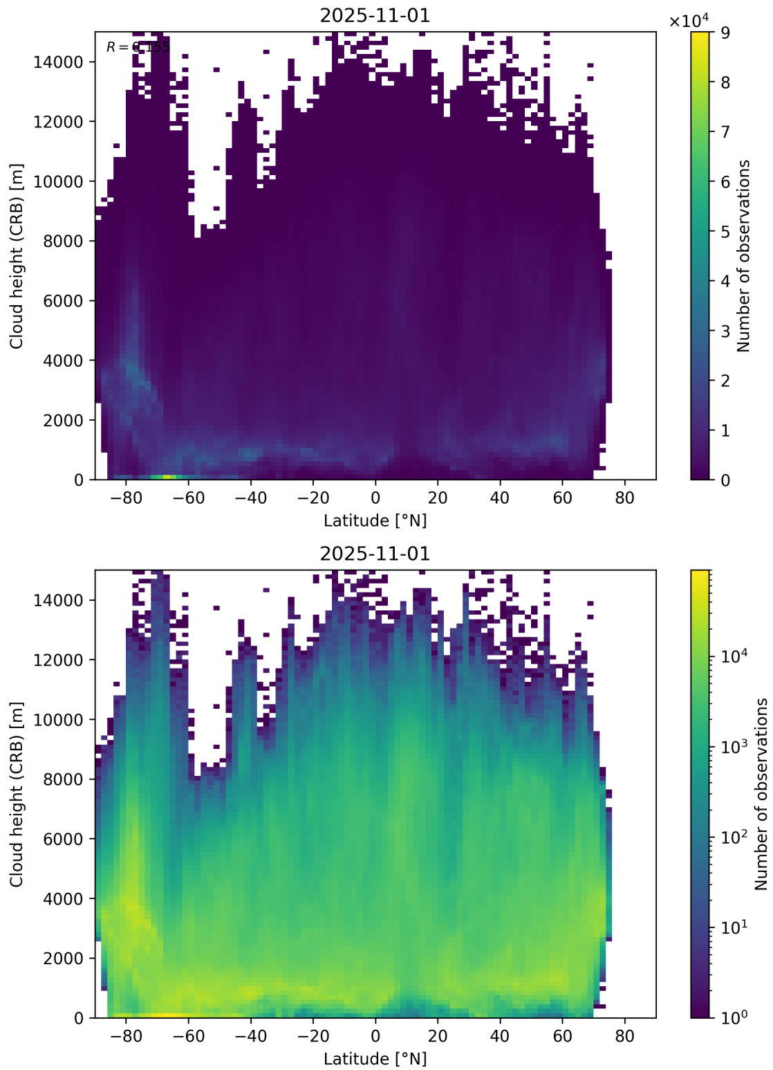
Figure 95: Scatter density plot of “Latitude” against “Cloud height (CRB)” for 2025-10-31 to 2025-11-02.
