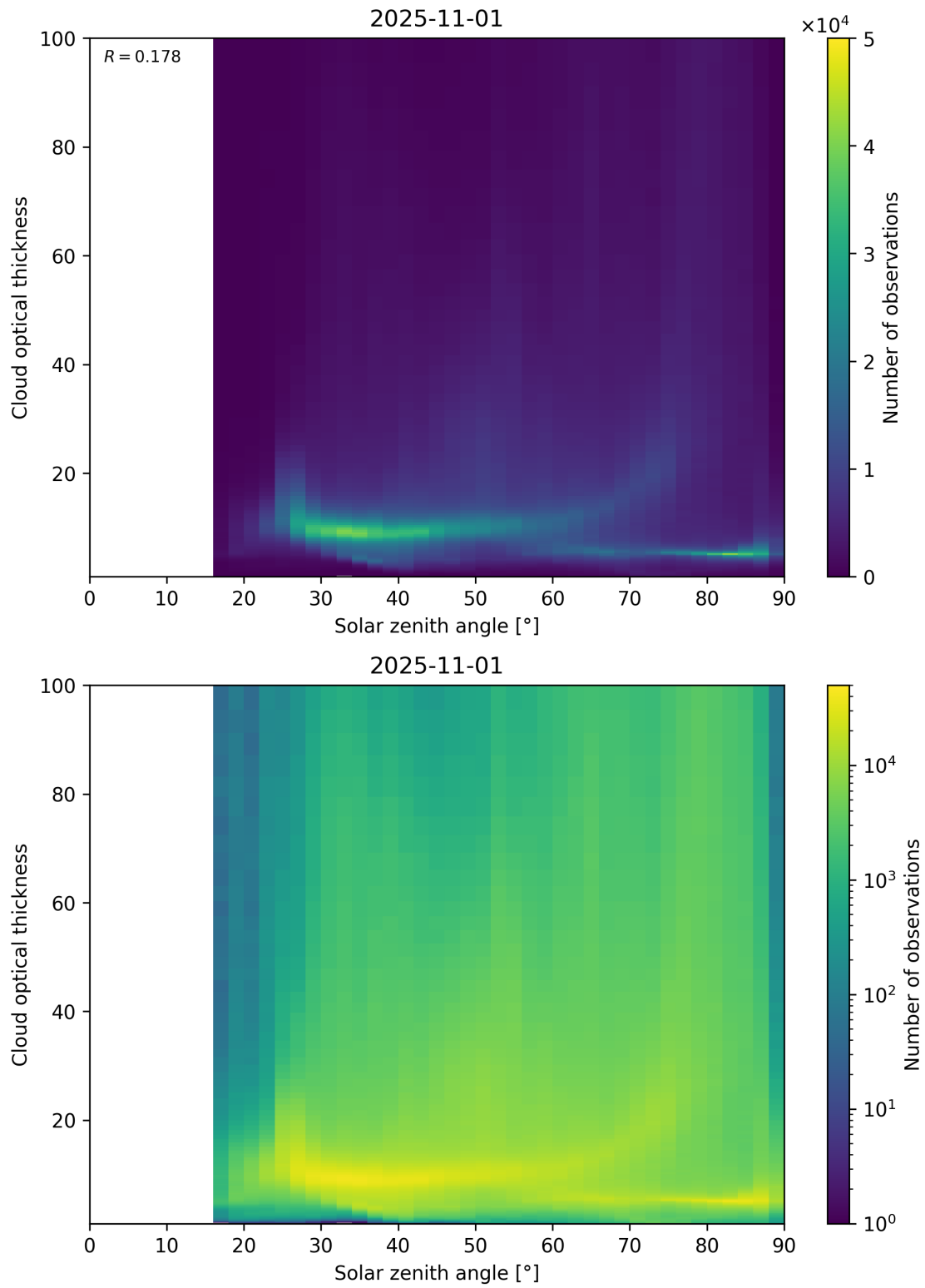
Figure 103: Scatter density plot of “Solar zenith angle” against “Cloud optical thickness” for 2025-10-31 to 2025-11-02.
