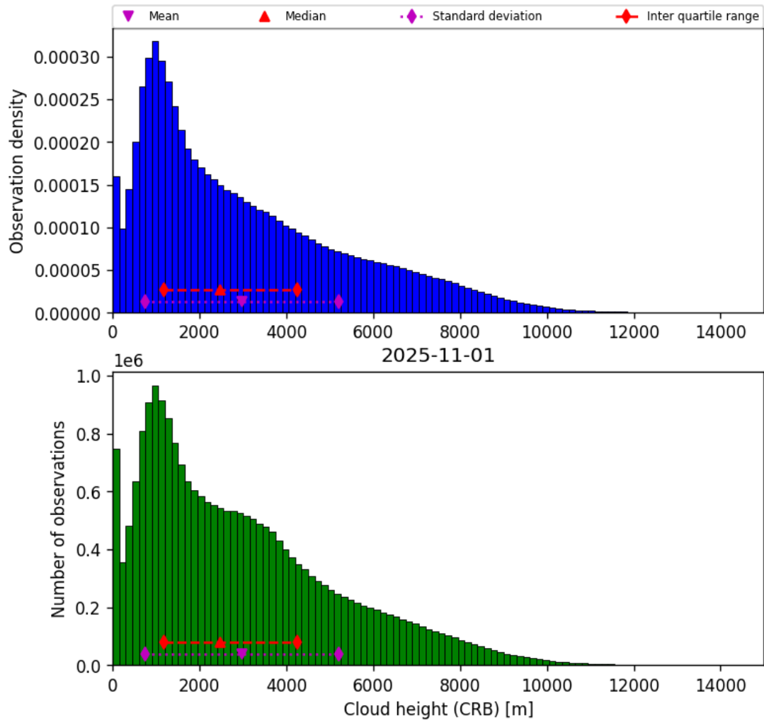
Figure 43: Histogram of “Cloud height (CRB)” for 2025-10-31 to 2025-11-02
