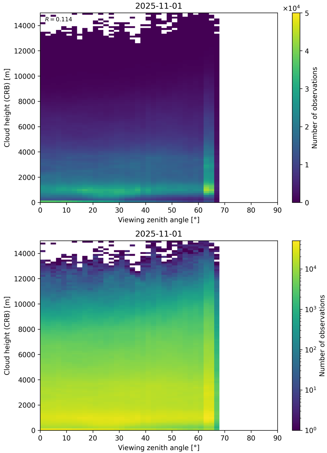
Figure 110: Scatter density plot of “Viewing zenith angle” against “Cloud height (CRB)” for 2025-10-31 to 2025-11-02.
