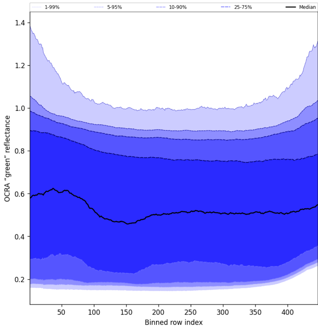
Figure 68: Along track statistics of "OCRA "green" reflectance" for 2025-10-31 to 2025-11-02
