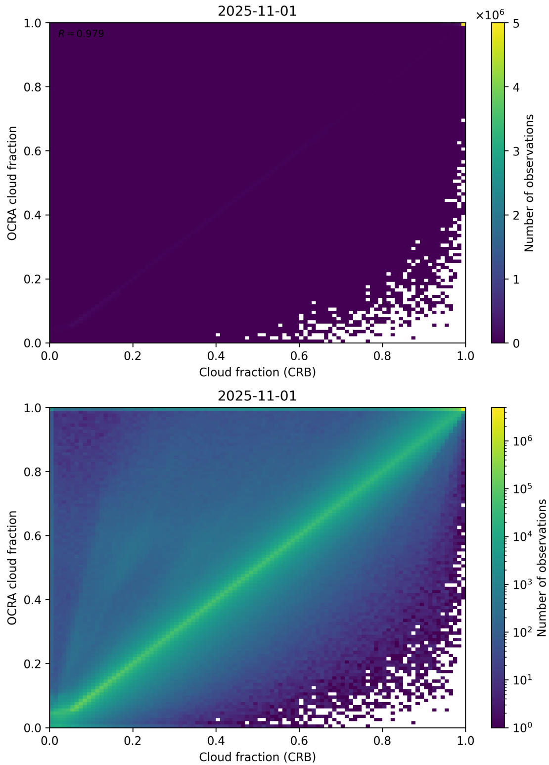
Figure 78: Scatter density plot of “Cloud fraction (CRB)” against “OCRA cloud fraction” for 2025-10-31 to 2025-11-02.
