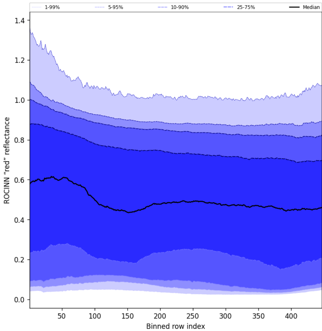
Figure 69: Along track statistics of "ROCINN "red" reflectance" for 2025-10-31 to 2025-11-02
