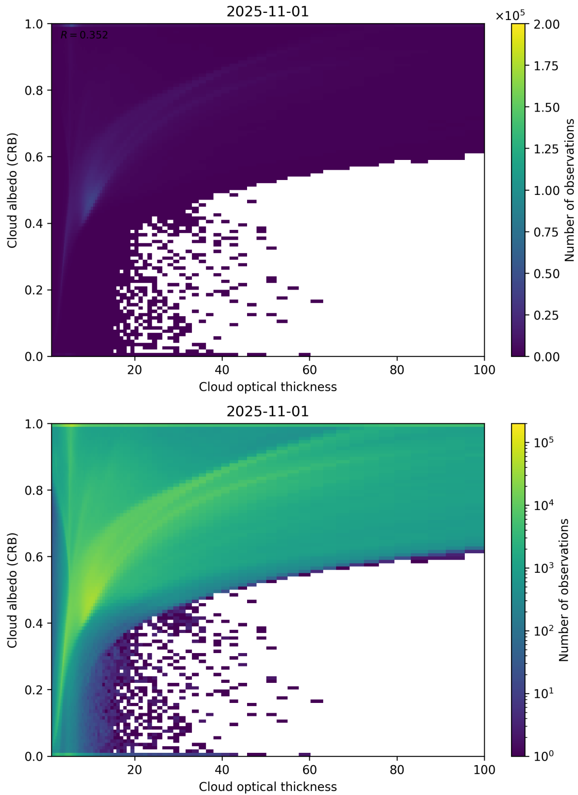
Figure 82: Scatter density plot of “Cloud optical thickness” against “Cloud albedo (CRB)” for 2025-10-31 to 2025-11-02.
