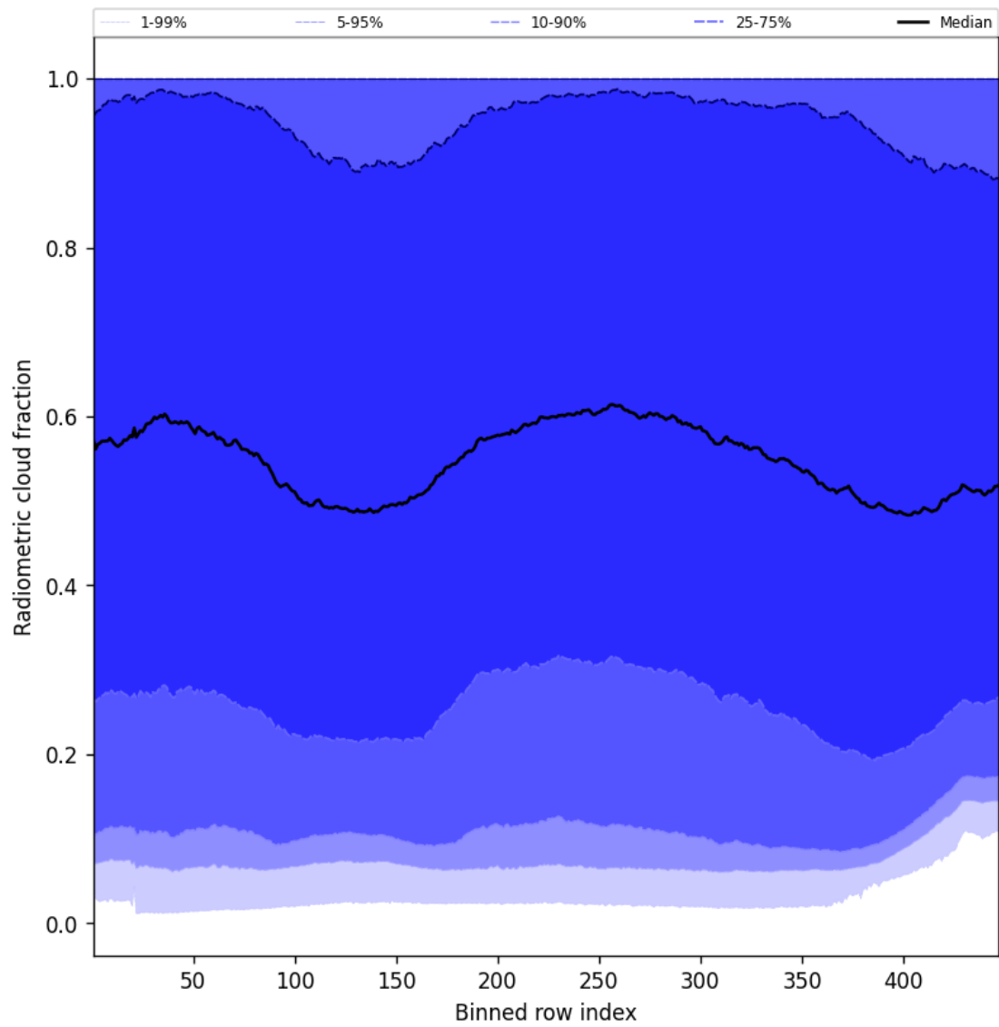
Figure 55: Along track statistics of “Radiometric cloud fraction” for 2025-10-31 to 2025-11-02
