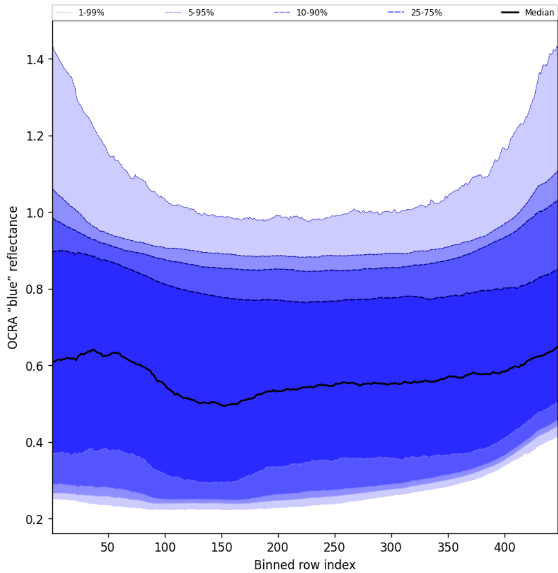
Figure 67: Along track statistics of “OCRA “blue” reflectance” for 2025-10-31 to 2025-11-02
