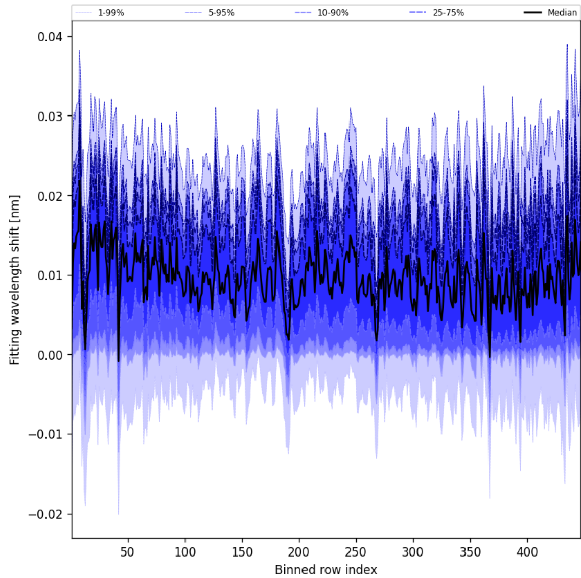
Figure 65: Along track statistics of “Fitting wavelength shift” for 2025-10-31 to 2025-11-02
