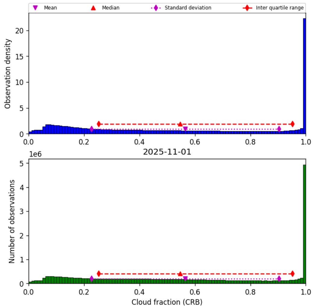
Figure 42: Histogram of “Cloud fraction (CRB)” for 2025-10-31 to 2025-11-02
