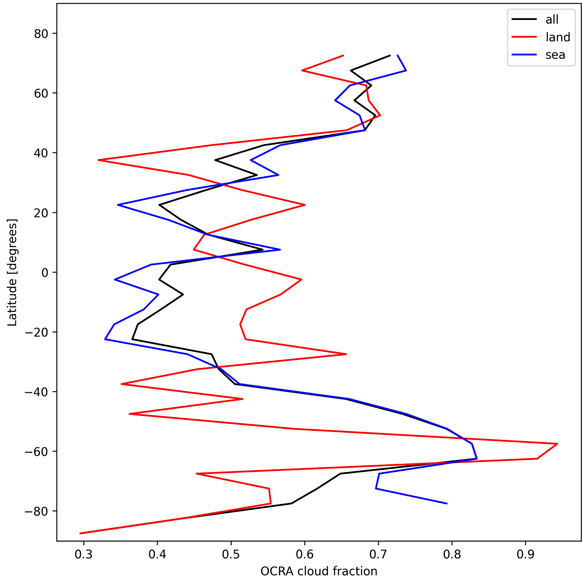
Figure 34: Zonal average of “OCRA cloud fraction” for 2025-10-31 to 2025-11-02.
