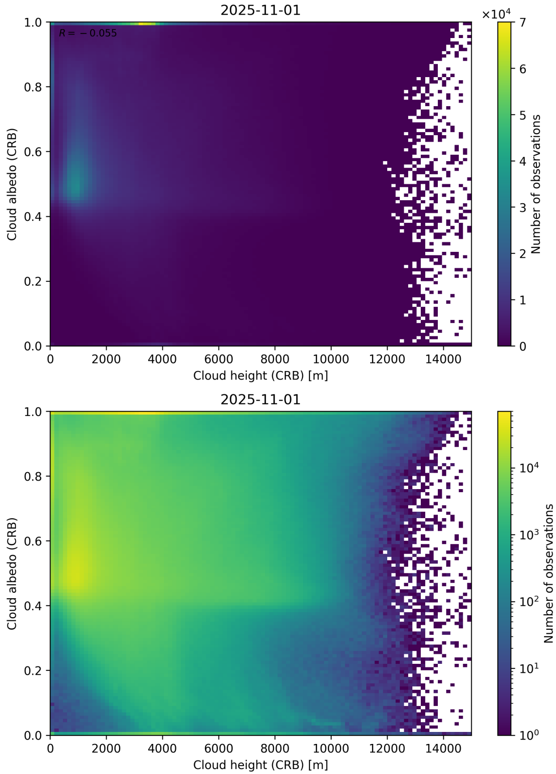
Figure 80: Scatter density plot of “Cloud height (CRB)” against “Cloud albedo (CRB)” for 2025-10-31 to 2025-11-02.
