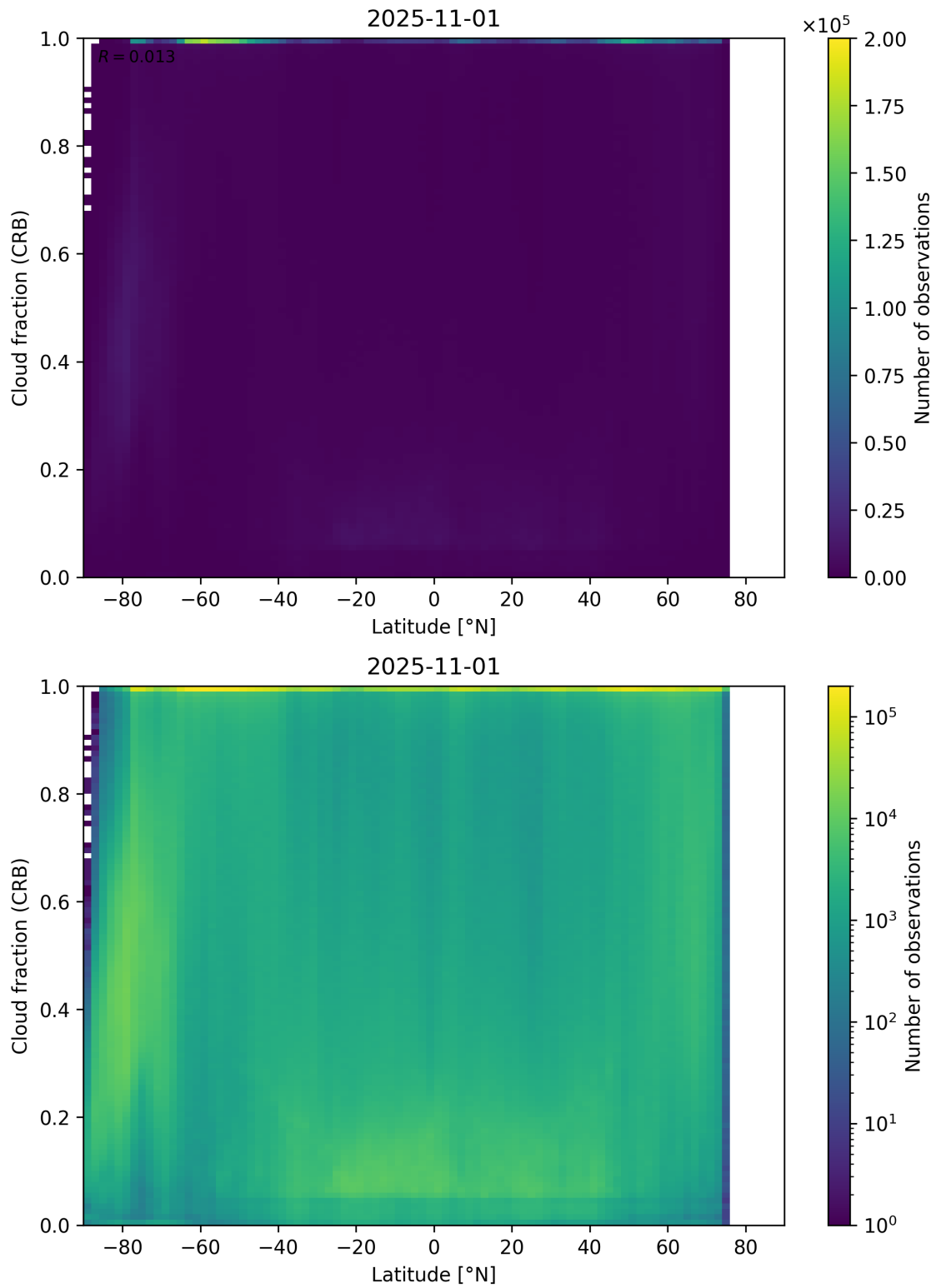
Figure 94: Scatter density plot of “Latitude” against “Cloud fraction (CRB)” for 2025-10-31 to 2025-11-02.
