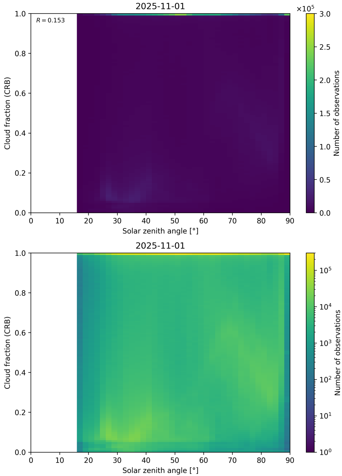
Figure 101: Scatter density plot of “Solar zenith angle” against “Cloud fraction (CRB)” for 2025-10-31 to 2025-11-02.
