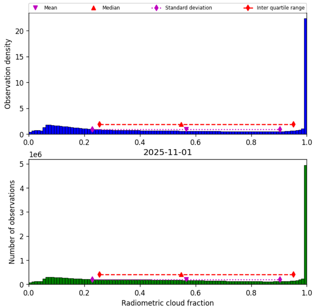
Figure 39: Histogram of “Radiometric cloud fraction” for 2025-10-31 to 2025-11-02
