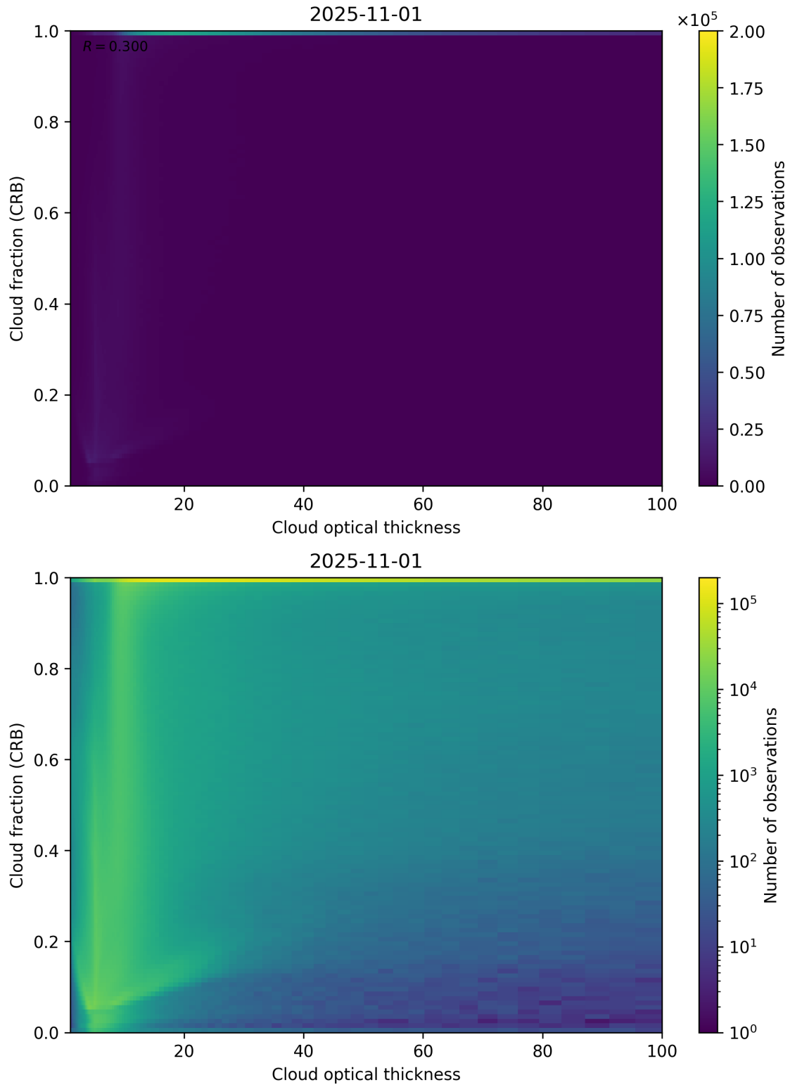
Figure 84: Scatter density plot of “Cloud optical thickness” against “Cloud fraction (CRB)” for 2025-10-31 to 2025-11-02.
