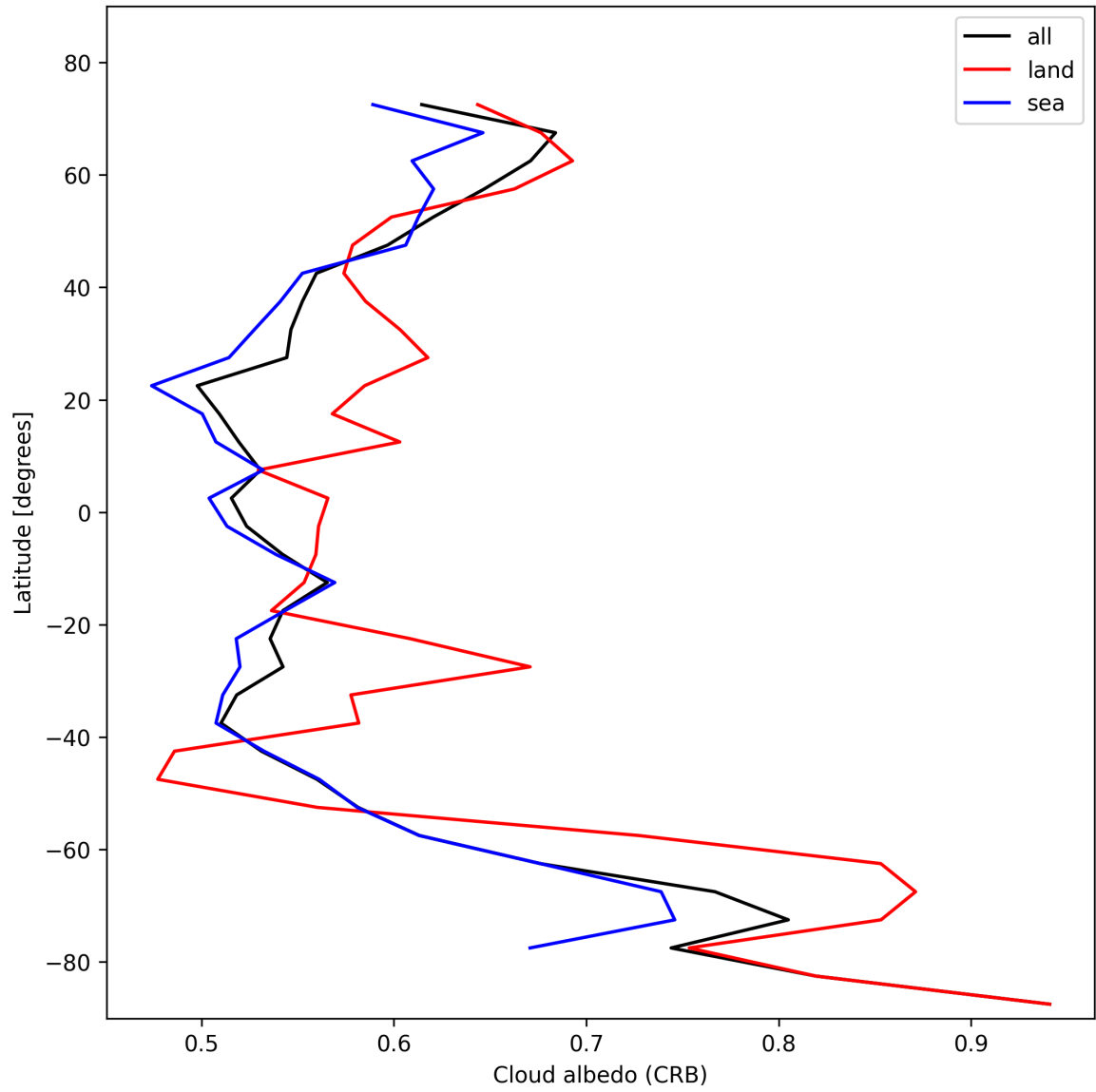
Figure 28: Zonal average of “Cloud albedo (CRB)” for 2025-10-31 to 2025-11-02.
