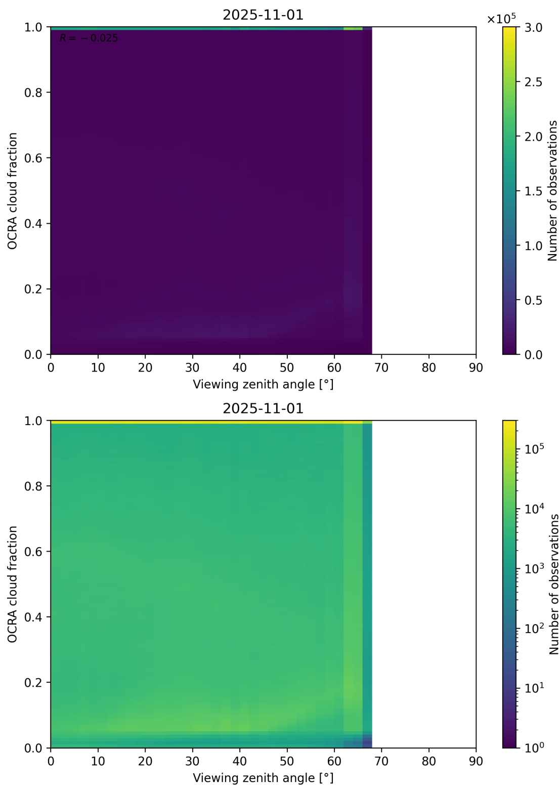
Figure 108: Scatter density plot of “Viewing zenith angle” against “OCRA cloud fraction” for 2025-10-31 to 2025-11-02.
