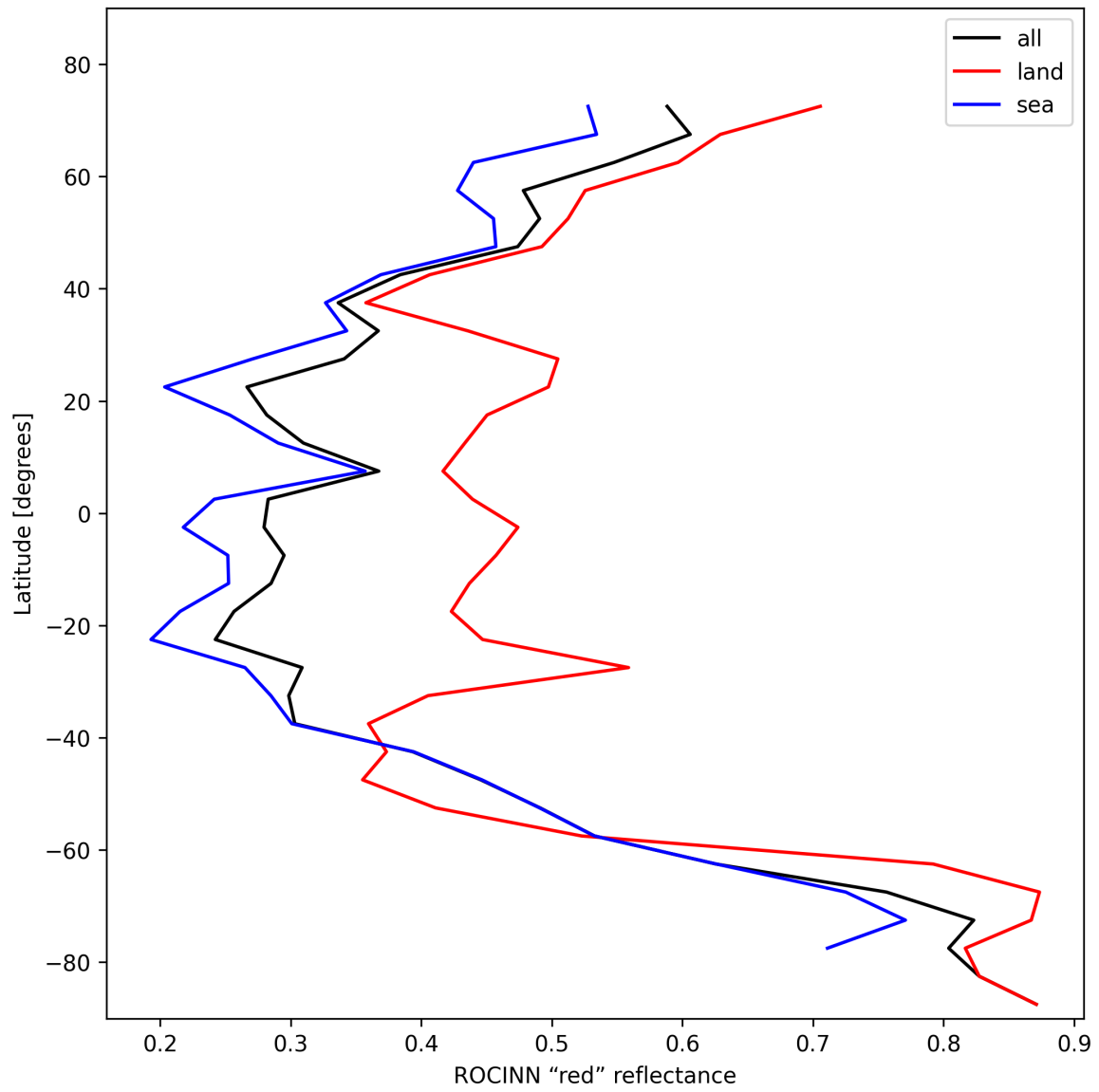
Figure 37: Zonal average of “ROCINN “red” reflectance” for 2025-10-31 to 2025-11-02.
