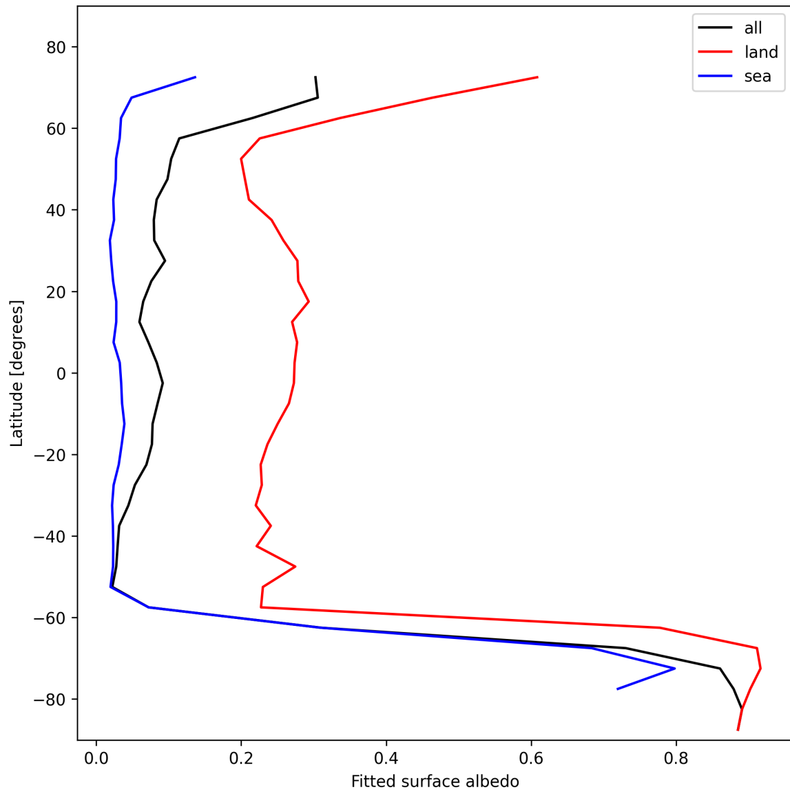
Figure 29: Zonal average of “Fitted surface albedo” for 2025-10-31 to 2025-11-02.
