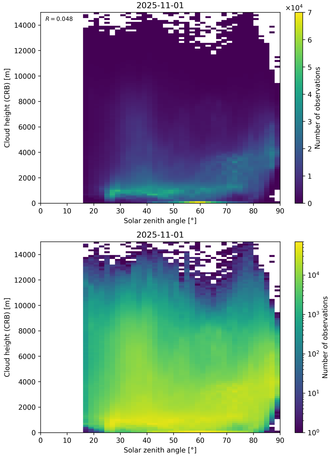
Figure 102: Scatter density plot of “Solar zenith angle” against “Cloud height (CRB)” for 2025-10-31 to 2025-11-02.
