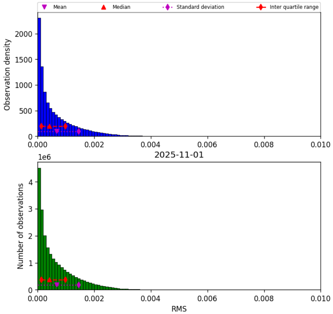
Figure 47: Histogram of “RMS” for 2025-10-31 to 2025-11-02
