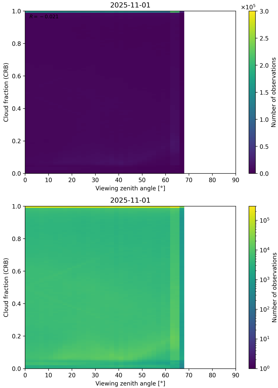
Figure 109: Scatter density plot of “Viewing zenith angle” against “Cloud fraction (CRB)” for 2025-10-31 to 2025-11-02.
