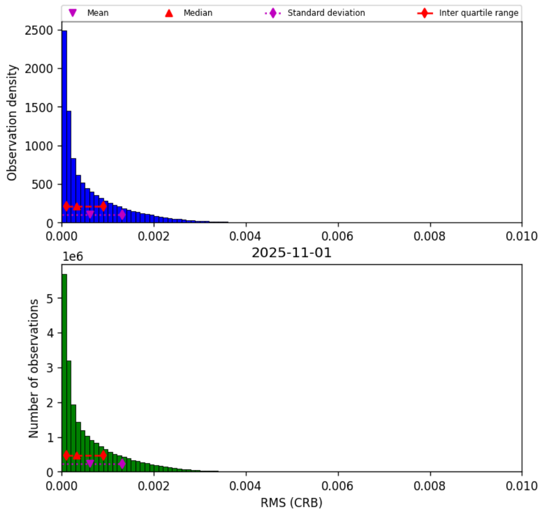
Figure 48: Histogram of “RMS (CRB)” for 2025-10-31 to 2025-11-02
