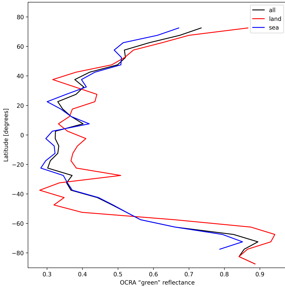
Figure 36: Zonal average of “OCRA “green” reflectance” for 2025-10-31 to 2025-11-02.
