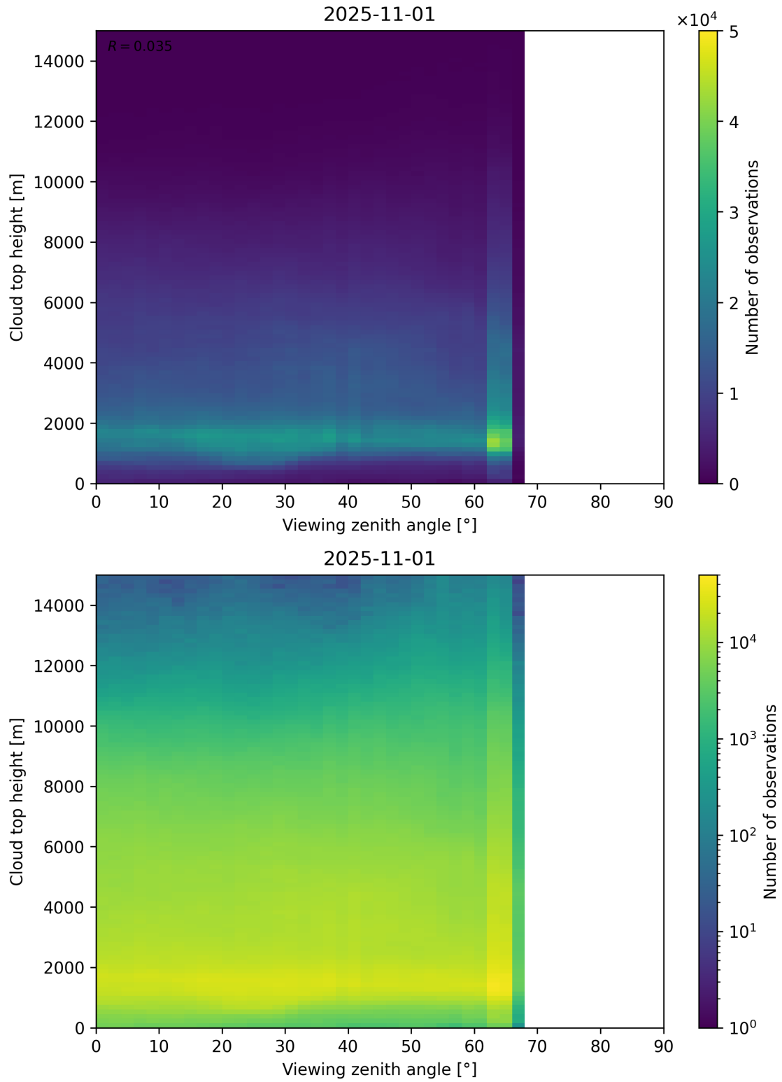
Figure 112: Scatter density plot of “Viewing zenith angle” against “Cloud top height” for 2025-10-31 to 2025-11-02.
