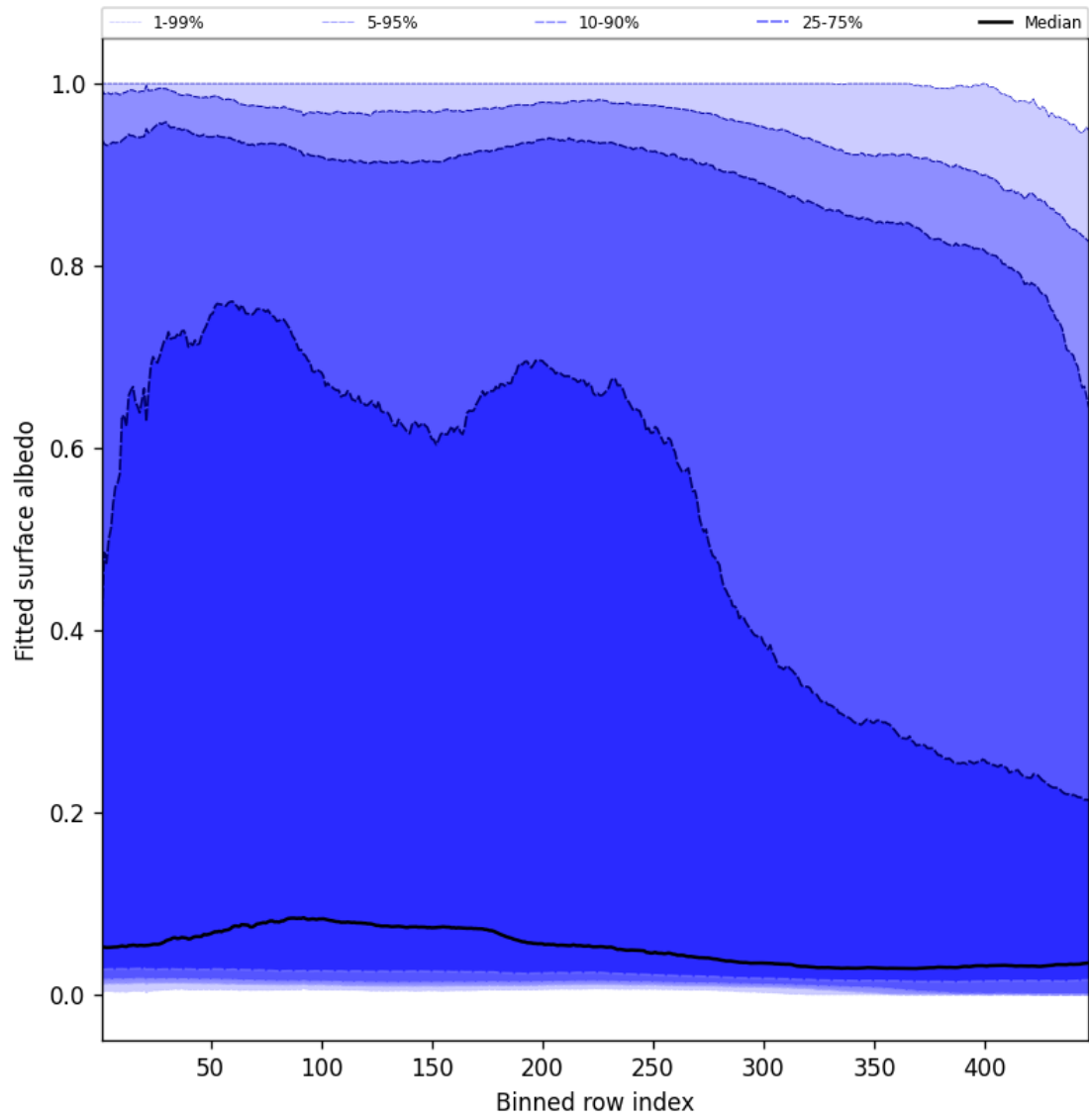
Figure 61: Along track statistics of “Fitted surface albedo” for 2025-10-31 to 2025-11-02
