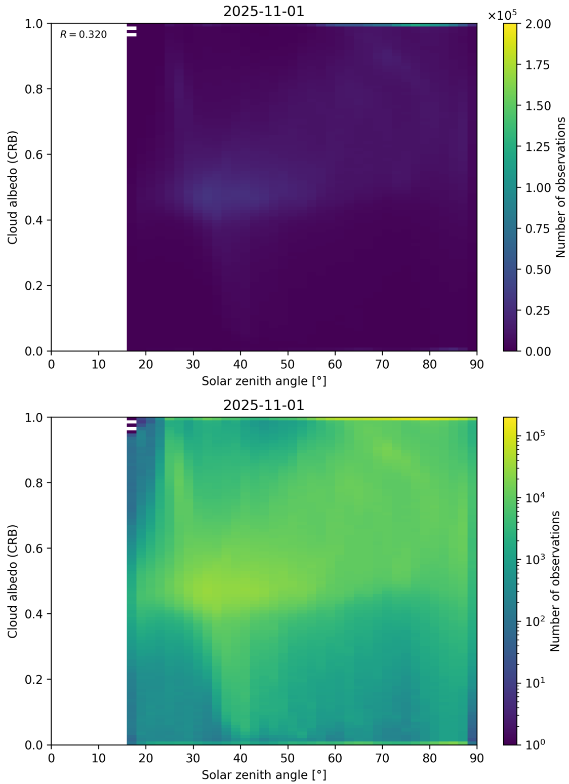
Figure 98: Scatter density plot of “Solar zenith angle” against “Cloud albedo (CRB)” for 2025-10-31 to 2025-11-02.
