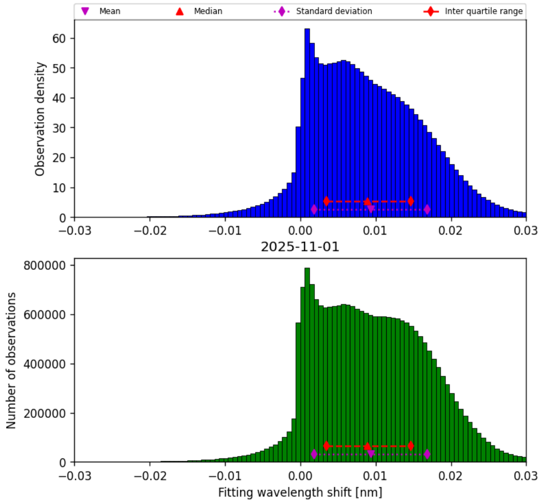
Figure 49: Histogram of “Fitting wavelength shift” for 2025-10-31 to 2025-11-02
