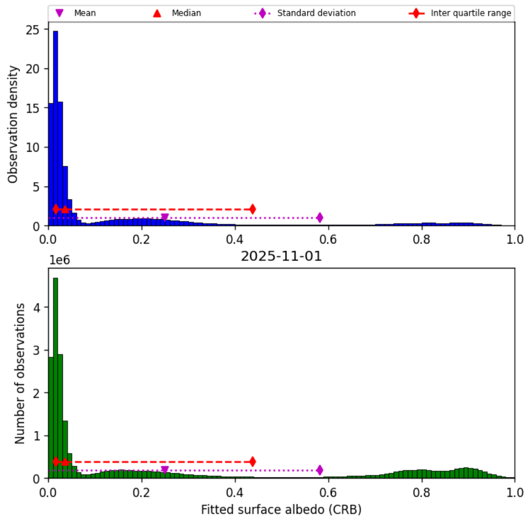
Figure 46: Histogram of “Fitted surface albedo (CRB)” for 2025-10-31 to 2025-11-02
