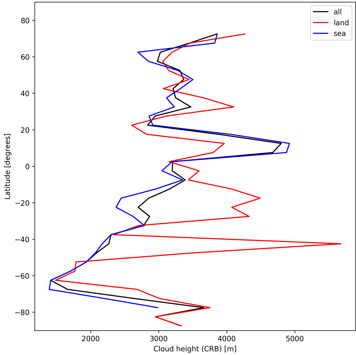
Figure 27: Zonal average of “Cloud height (CRB)” for 2025-10-31 to 2025-11-02.
