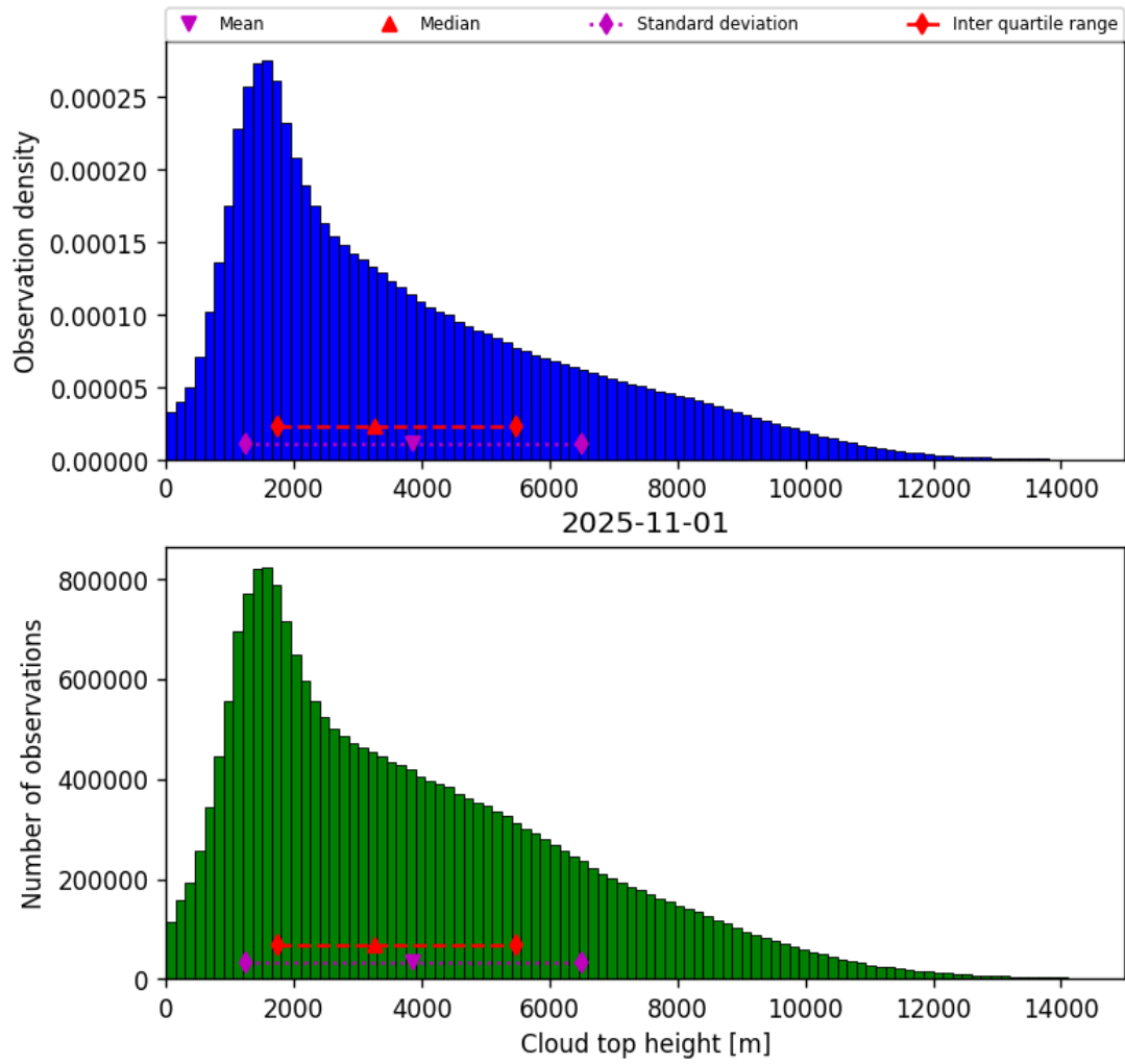
Figure 40: Histogram of “Cloud top height” for 2025-10-31 to 2025-11-02
