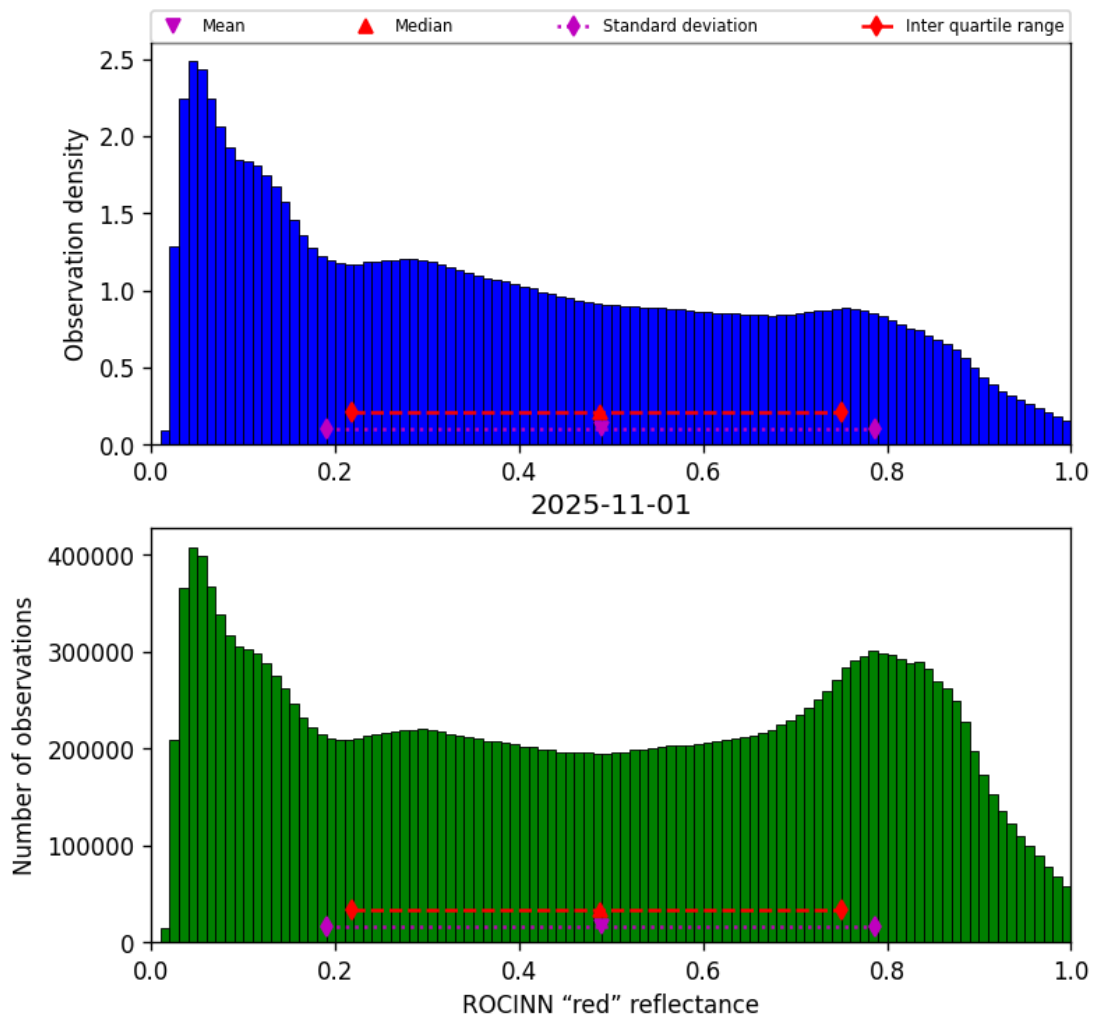
Figure 53: Histogram of “ROCINN “red” reflectance” for 2025-10-31 to 2025-11-02
