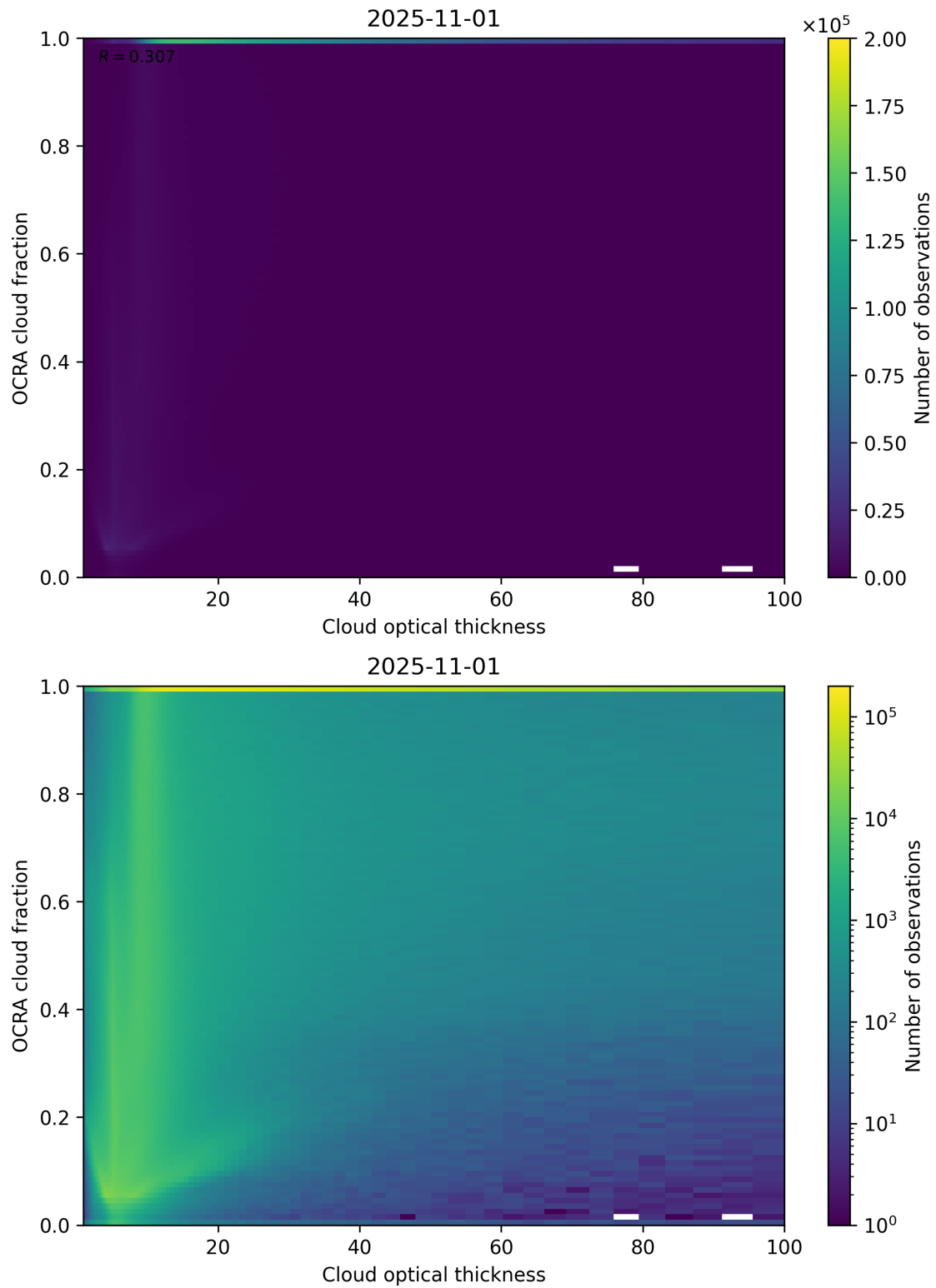
Figure 83: Scatter density plot of “Cloud optical thickness” against “OCRA cloud fraction” for 2025-10-31 to 2025-11-02.
