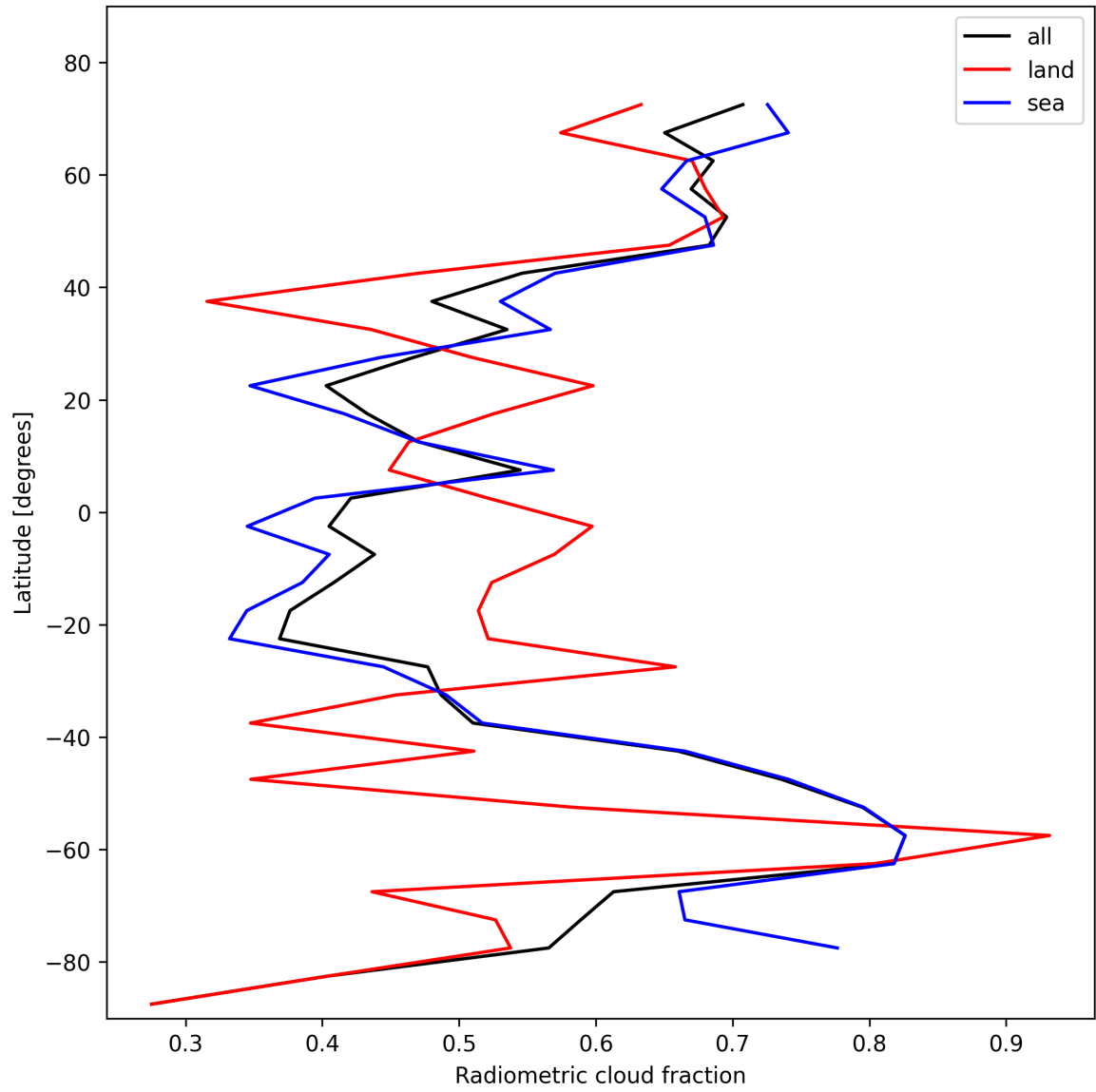
Figure 23: Zonal average of “Radiometric cloud fraction” for 2025-10-31 to 2025-11-02.
