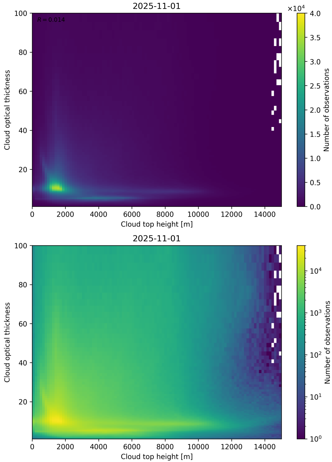
Figure 90: Scatter density plot of “Cloud top height” against “Cloud optical thickness” for 2025-10-31 to 2025-11-02.
