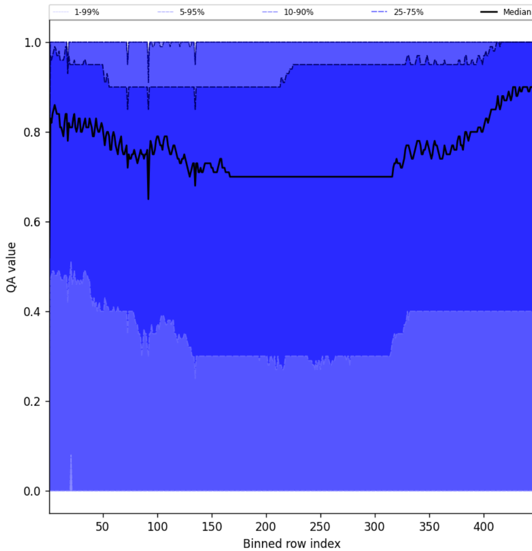
Figure 54: Along track statistics of “QA value” for 2025-10-31 to 2025-11-02
