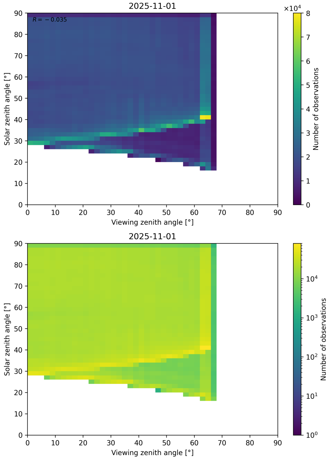
Figure 114: Scatter density plot of “Viewing zenith angle” against “Solar zenith angle” for 2025-10-31 to 2025-11-02.
