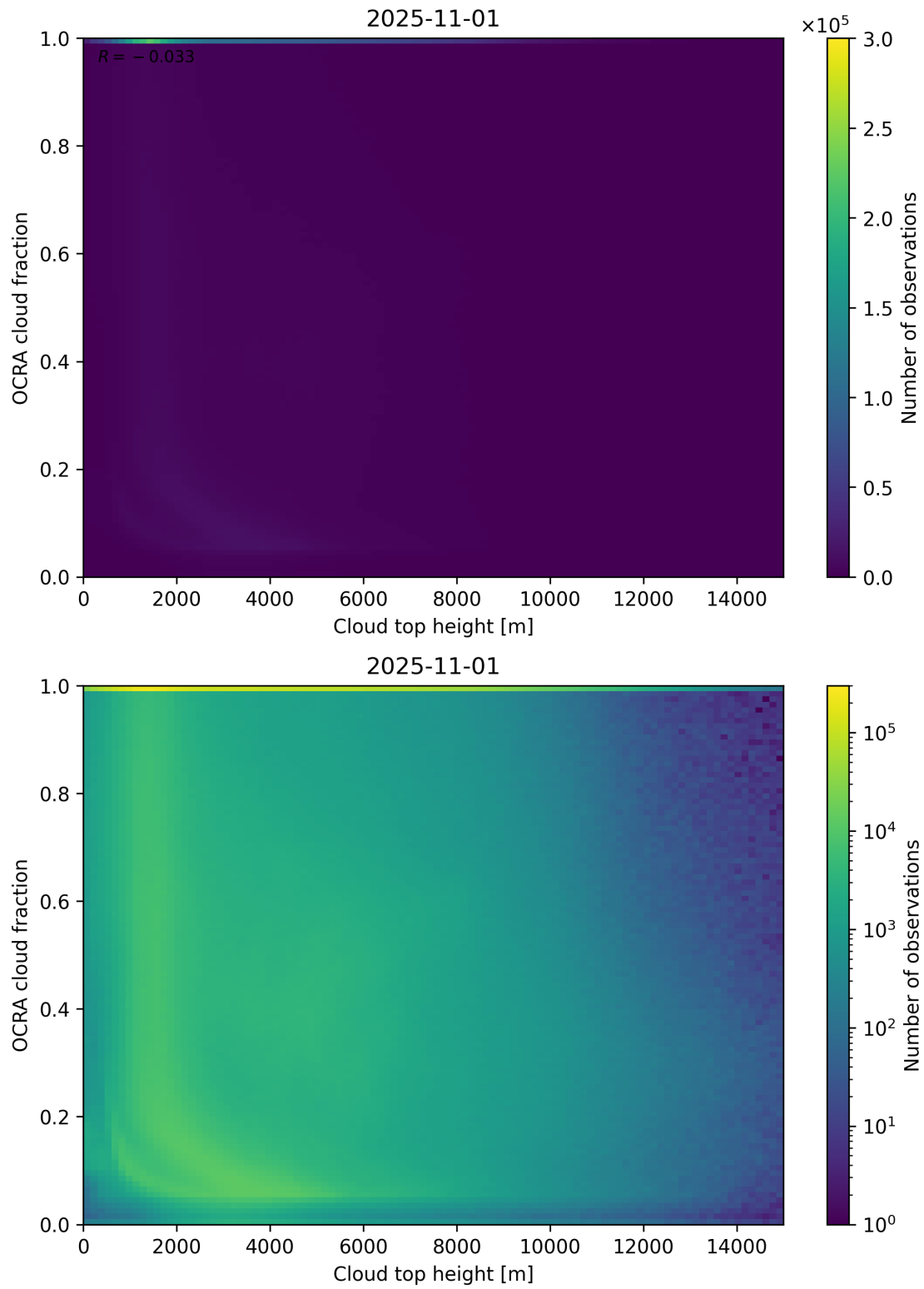
Figure 87: Scatter density plot of “Cloud top height” against “OCRA cloud fraction” for 2025-10-31 to 2025-11-02.
