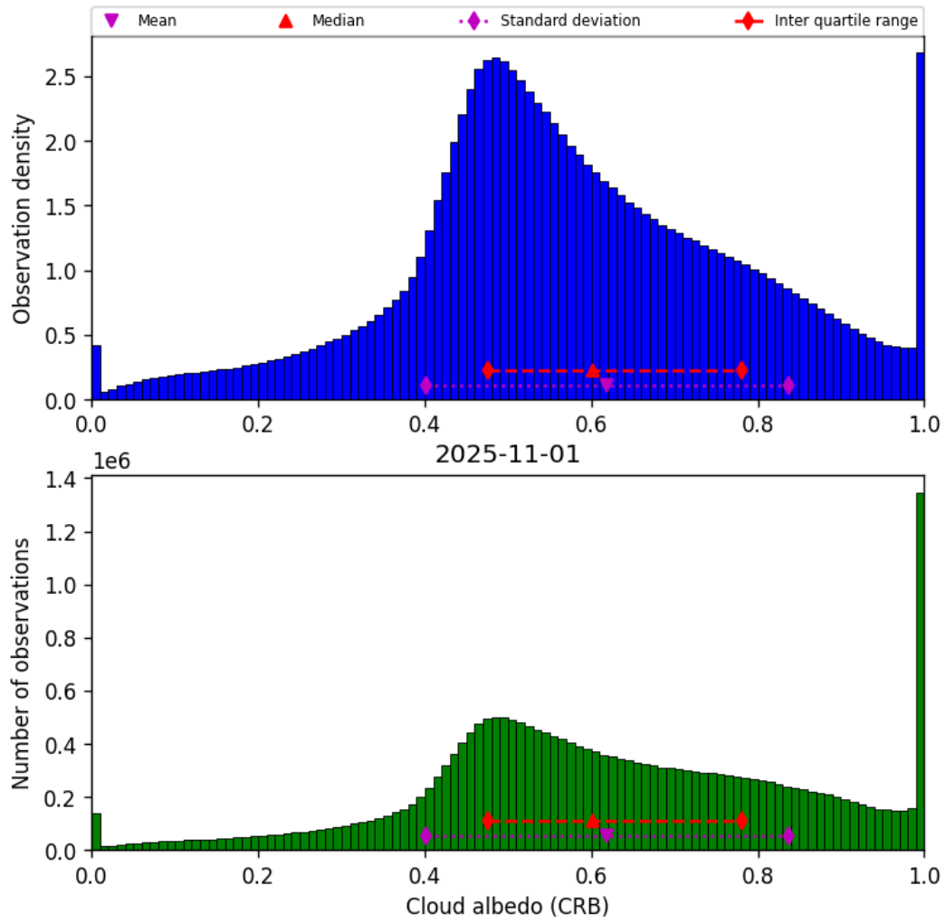
Figure 44: Histogram of “Cloud albedo (CRB)” for 2025-10-31 to 2025-11-02
