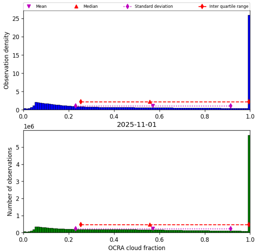
Figure 50: Histogram of “OCRA cloud fraction” for 2025-10-31 to 2025-11-02
