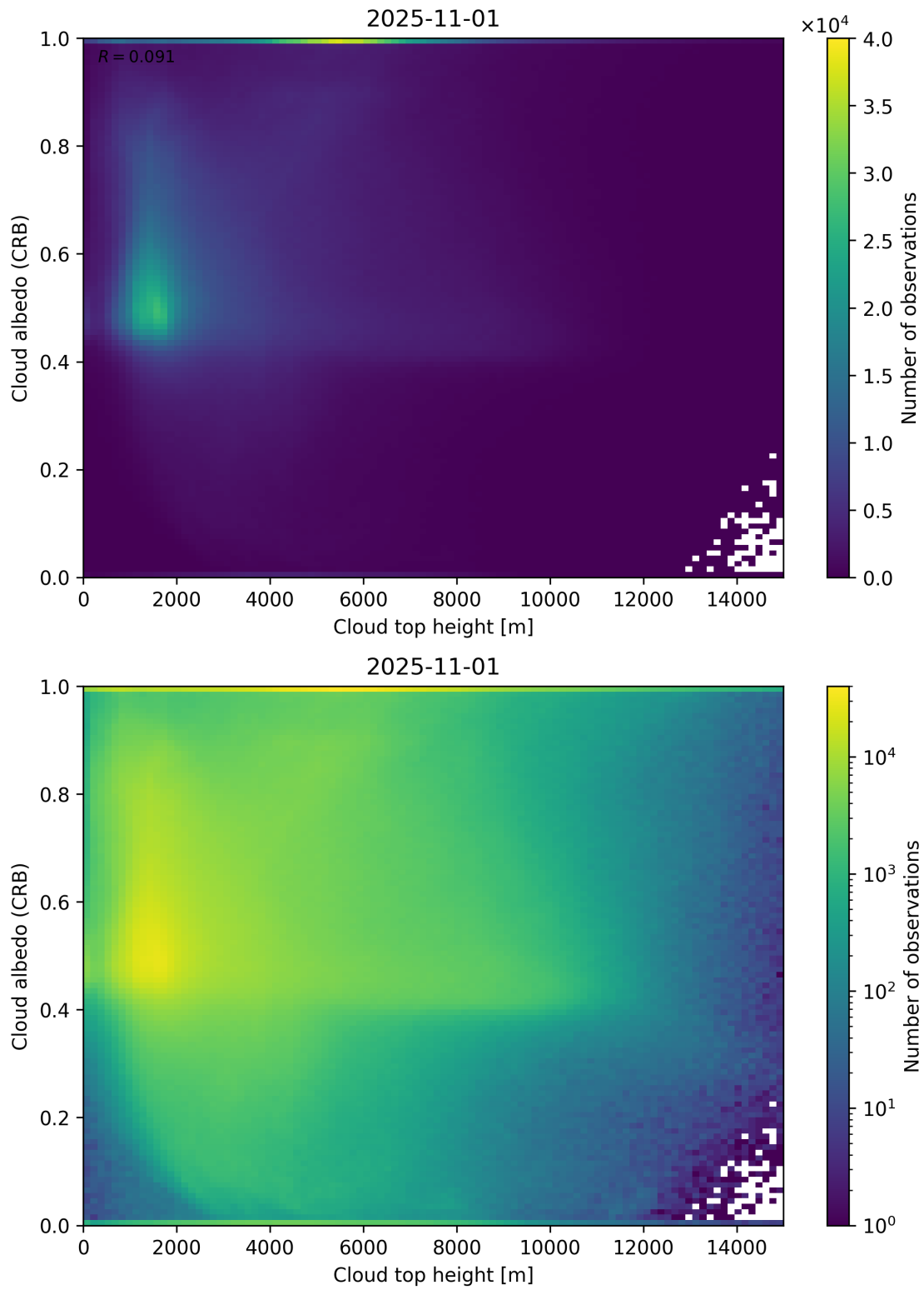
Figure 86: Scatter density plot of “Cloud top height” against “Cloud albedo (CRB)” for 2025-10-31 to 2025-11-02.
