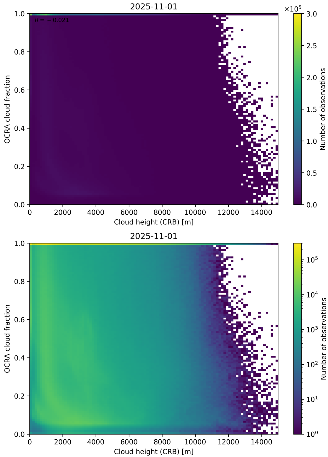
Figure 81: Scatter density plot of “Cloud height (CRB)” against “OCRA cloud fraction” for 2025-10-31 to 2025-11-02.
