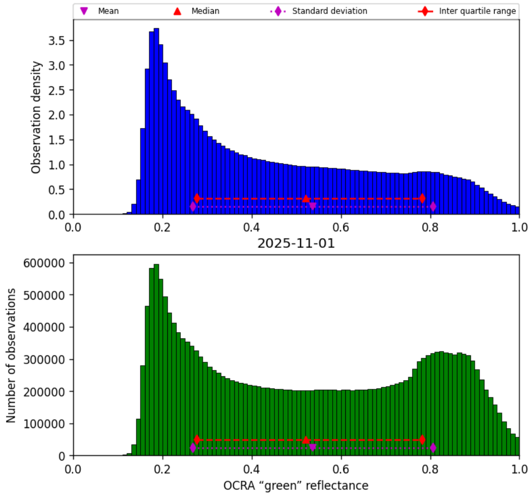
Figure 52: Histogram of “OCRA “green” reflectance” for 2025-10-31 to 2025-11-02
