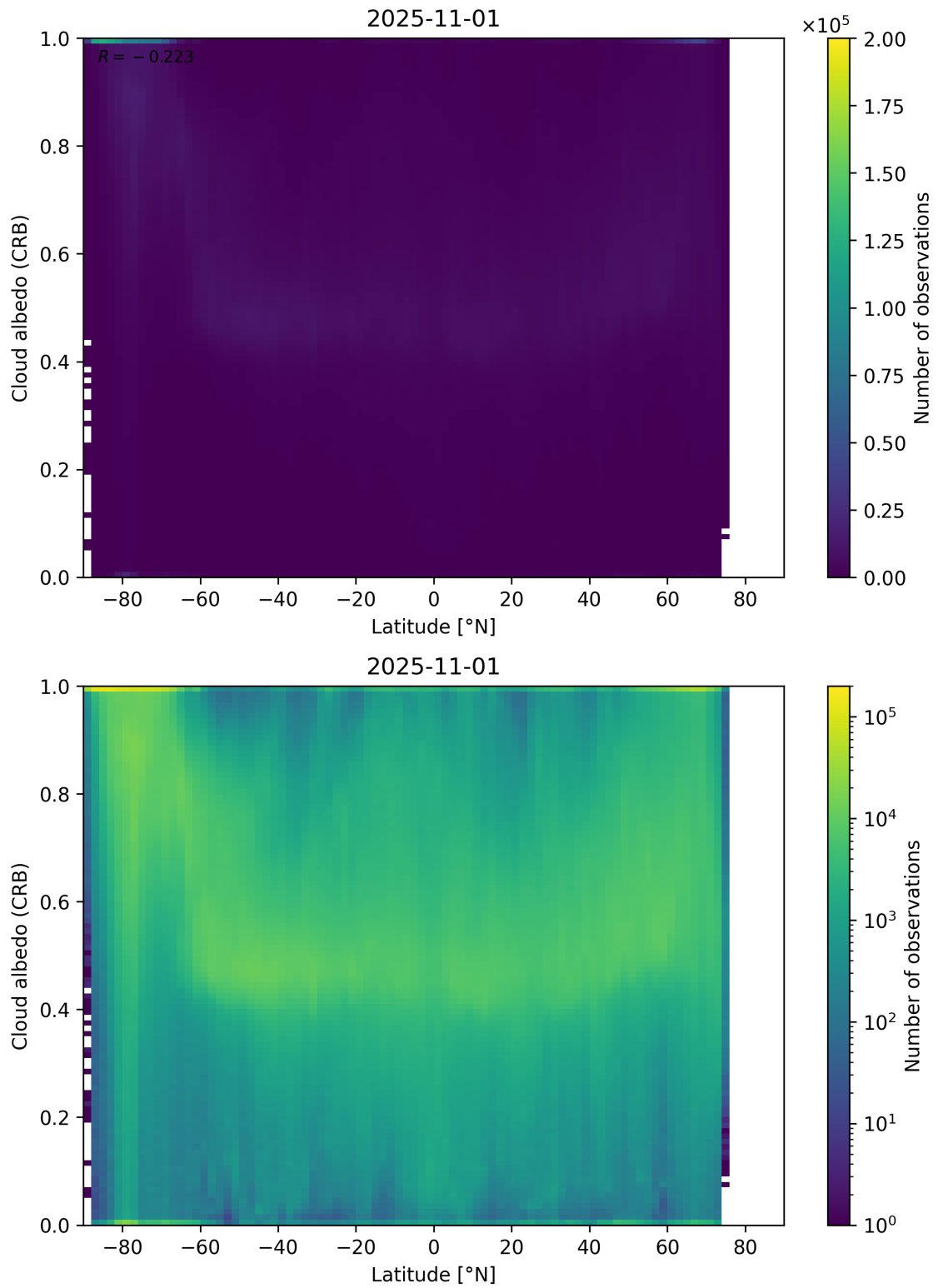
Figure 91: Scatter density plot of “Latitude” against “Cloud albedo (CRB)” for 2025-10-31 to 2025-11-02.
