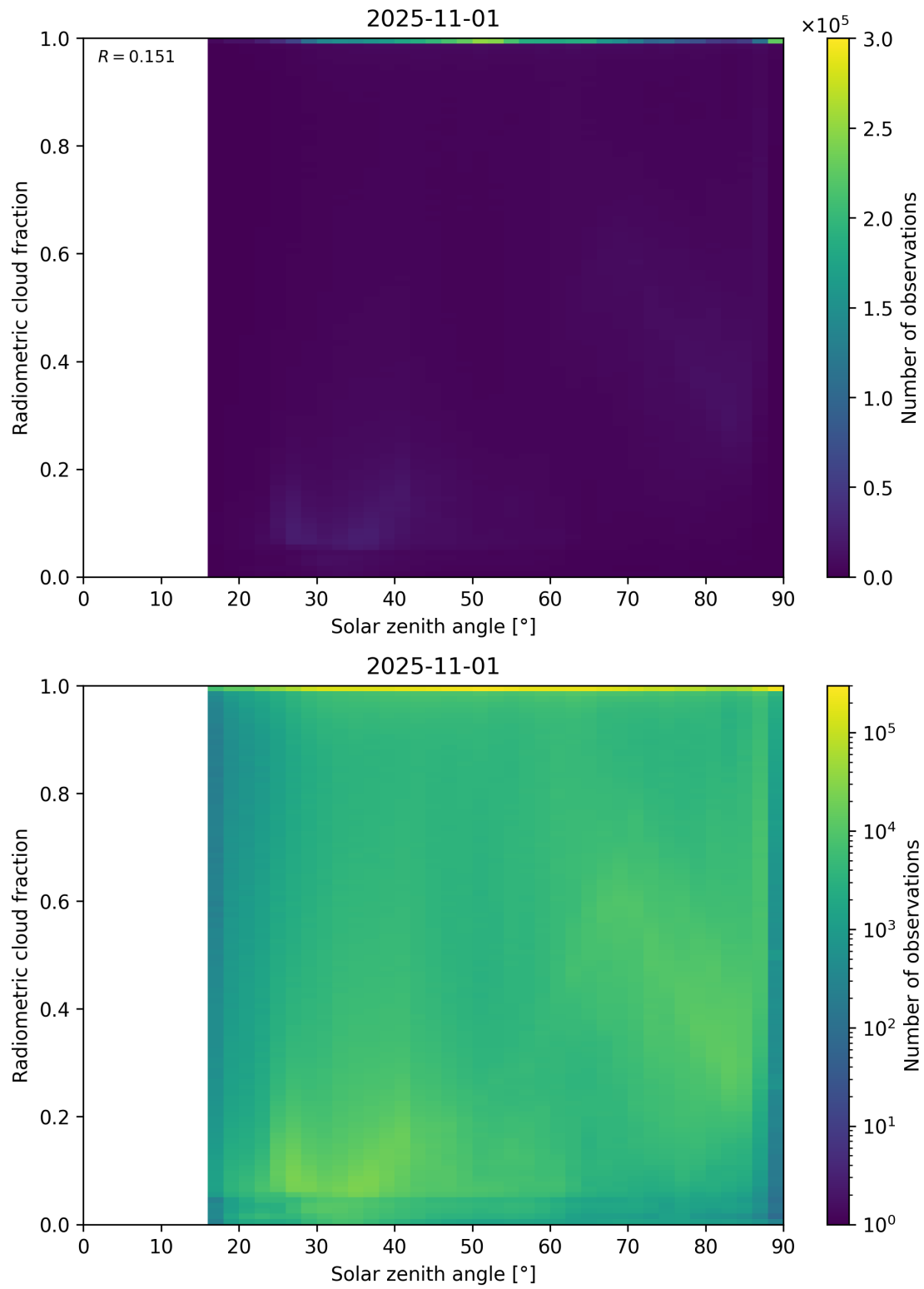
Figure 99: Scatter density plot of “Solar zenith angle” against “Radiometric cloud fraction” for 2025-10-31 to 2025-11-02.
