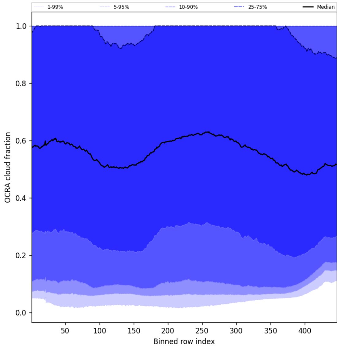
Figure 66: Along track statistics of “OCRA cloud fraction” for 2025-10-31 to 2025-11-02
