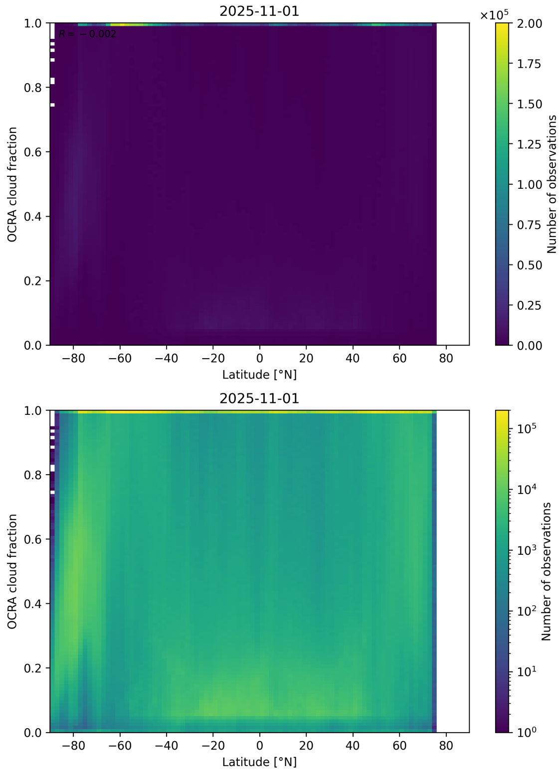
Figure 93: Scatter density plot of “Latitude” against “OCRA cloud fraction” for 2025-10-31 to 2025-11-02.
