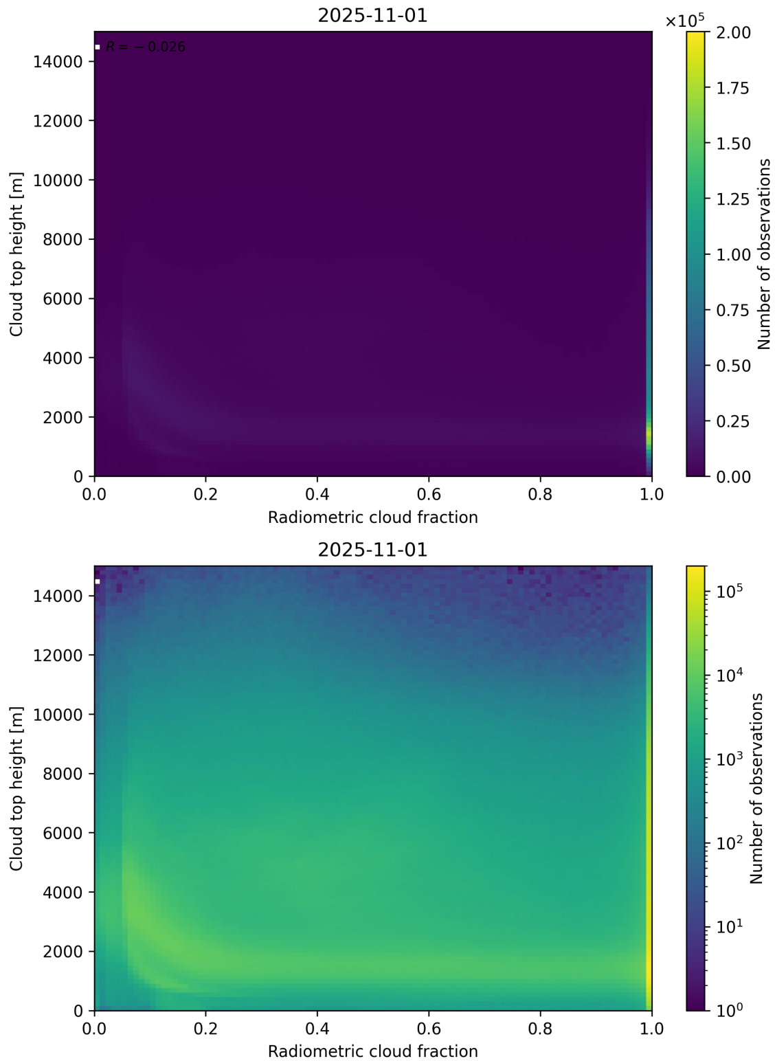
Figure 76: Scatter density plot of “Radiometric cloud fraction” against “Cloud top height” for 2025-10-31 to 2025-11-02.
