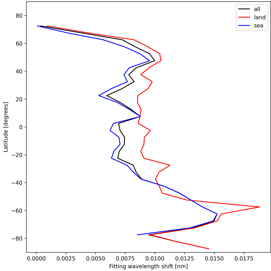
Figure 33: Zonal average of “Fitting wavelength shift” for 2025-10-31 to 2025-11-02.
