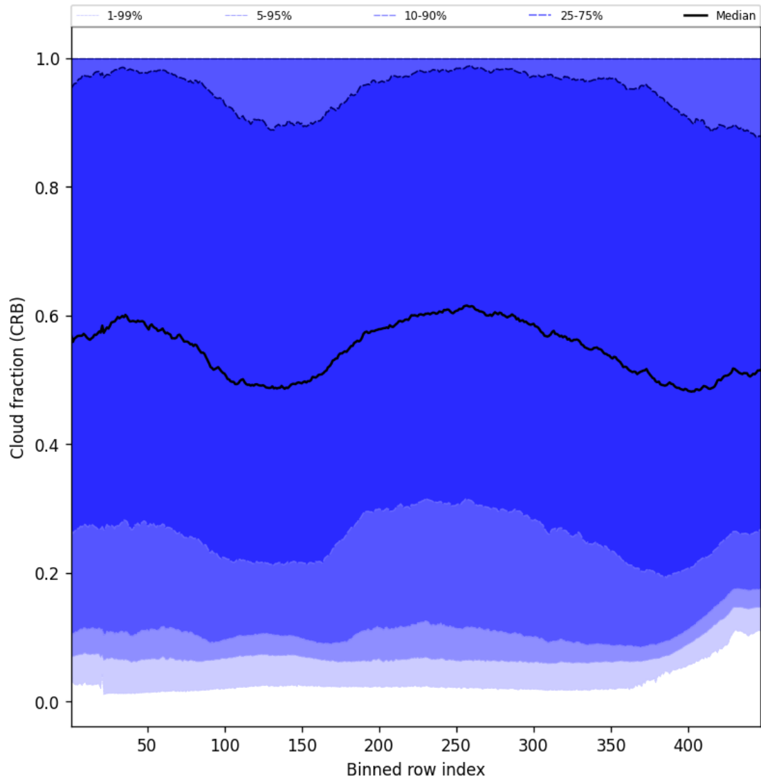
Figure 58: Along track statistics of “Cloud fraction (CRB)” for 2025-10-31 to 2025-11-02
