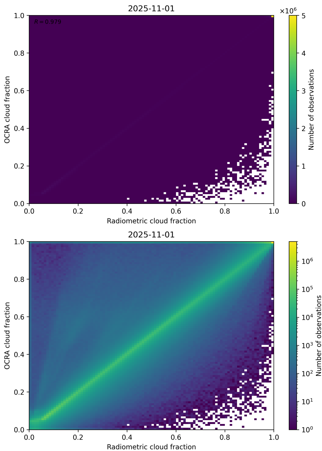
Figure 72: Scatter density plot of “Radiometric cloud fraction” against “OCRA cloud fraction” for 2025-10-31 to 2025-11-02.
