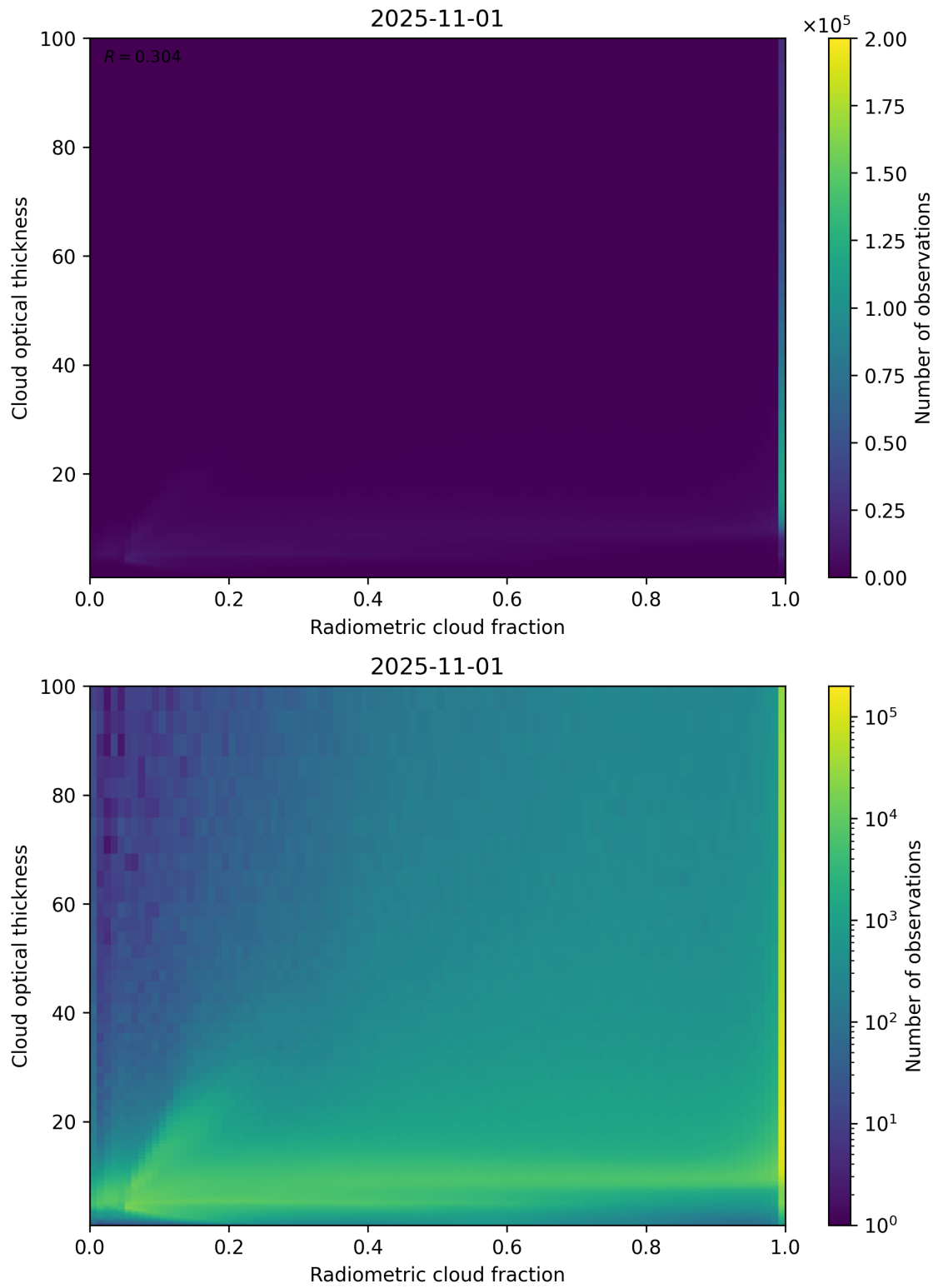
Figure 75: Scatter density plot of “Radiometric cloud fraction” against “Cloud optical thickness” for 2025-10-31 to 2025-11-02.
