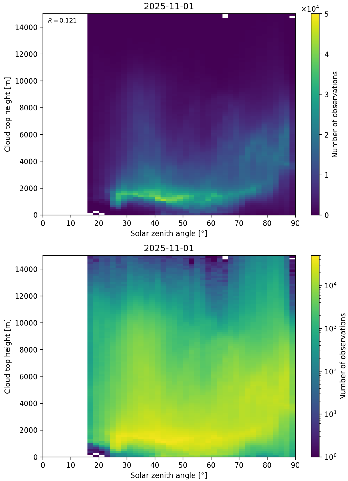
Figure 104: Scatter density plot of “Solar zenith angle” against “Cloud top height” for 2025-10-31 to 2025-11-02.
