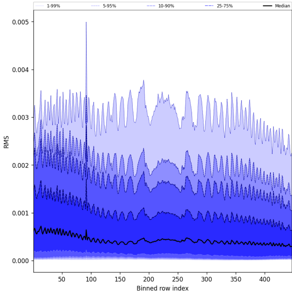
Figure 63: Along track statistics of “RMS” for 2025-10-31 to 2025-11-02
