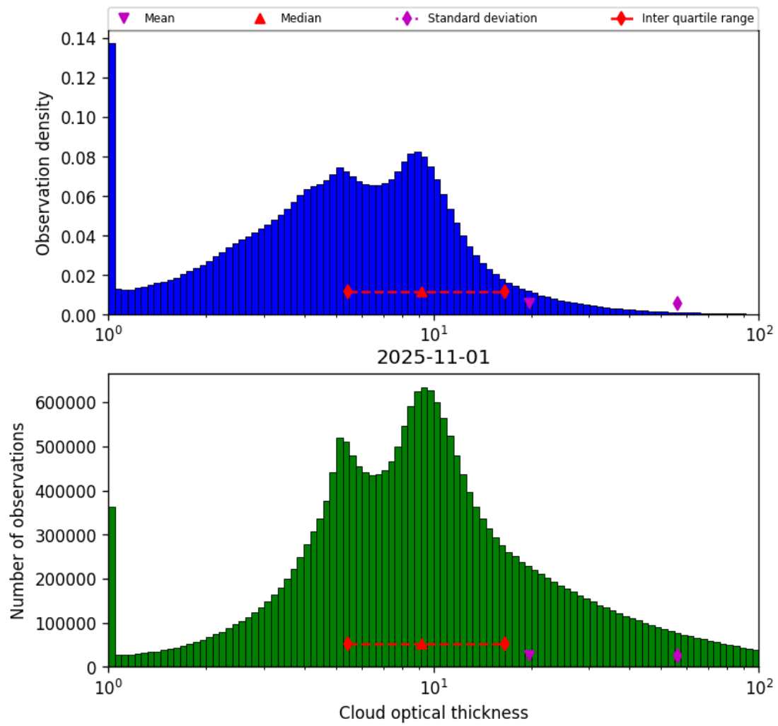
Figure 41: Histogram of “Cloud optical thickness” for 2025-10-31 to 2025-11-02
