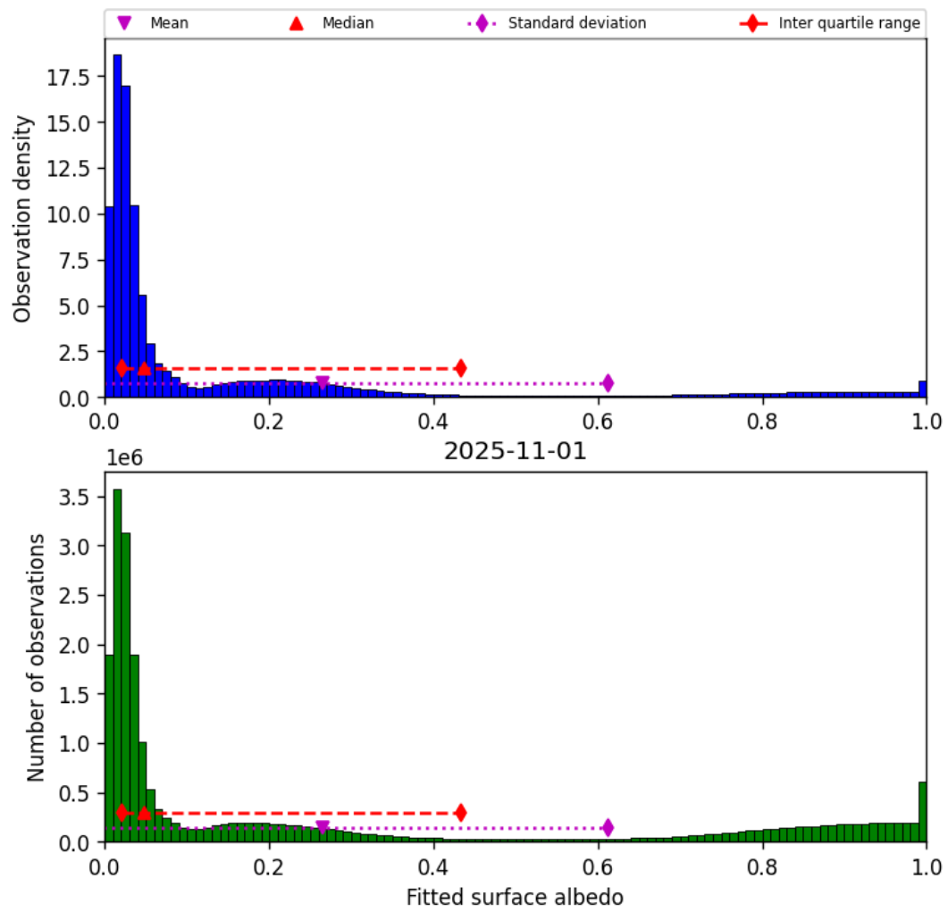
Figure 45: Histogram of “Fitted surface albedo” for 2025-10-31 to 2025-11-02
