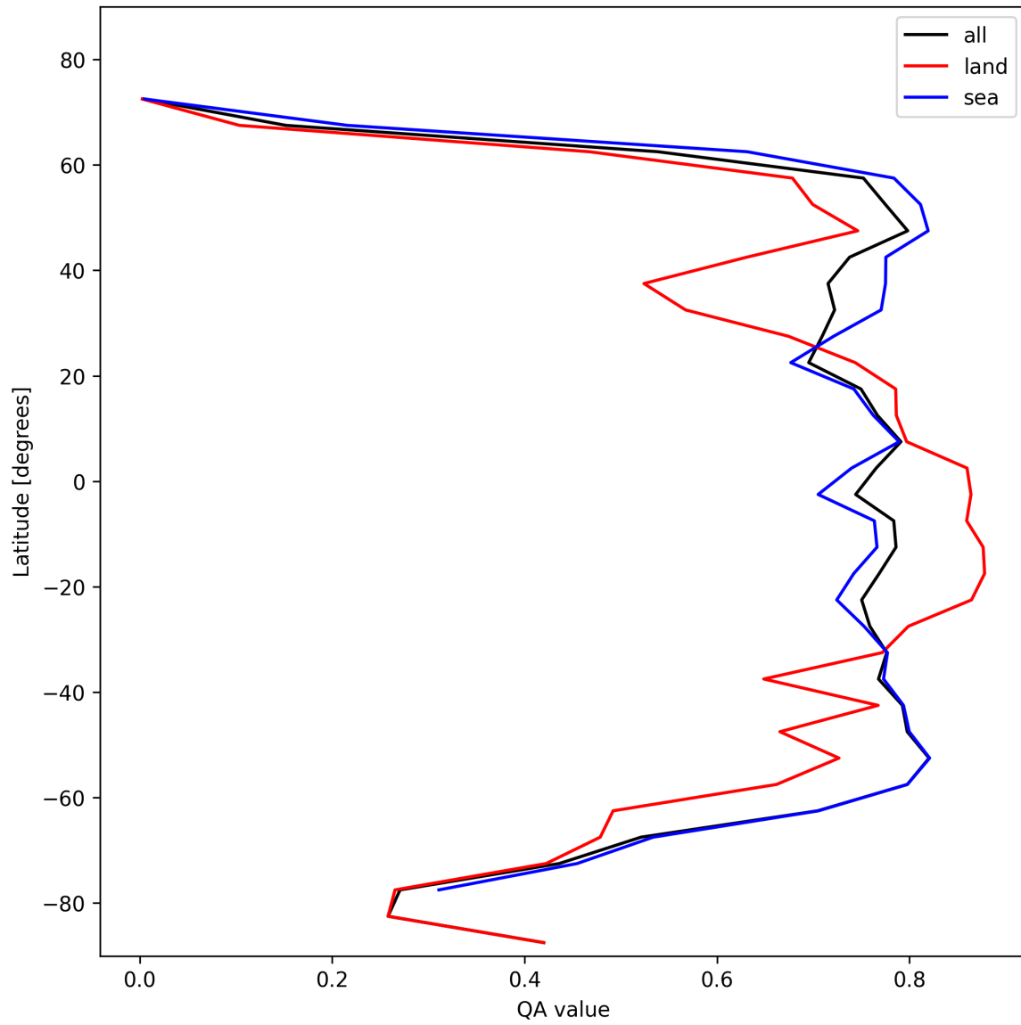
Figure 22: Zonal average of “QA value” for 2025-10-31 to 2025-11-02.
