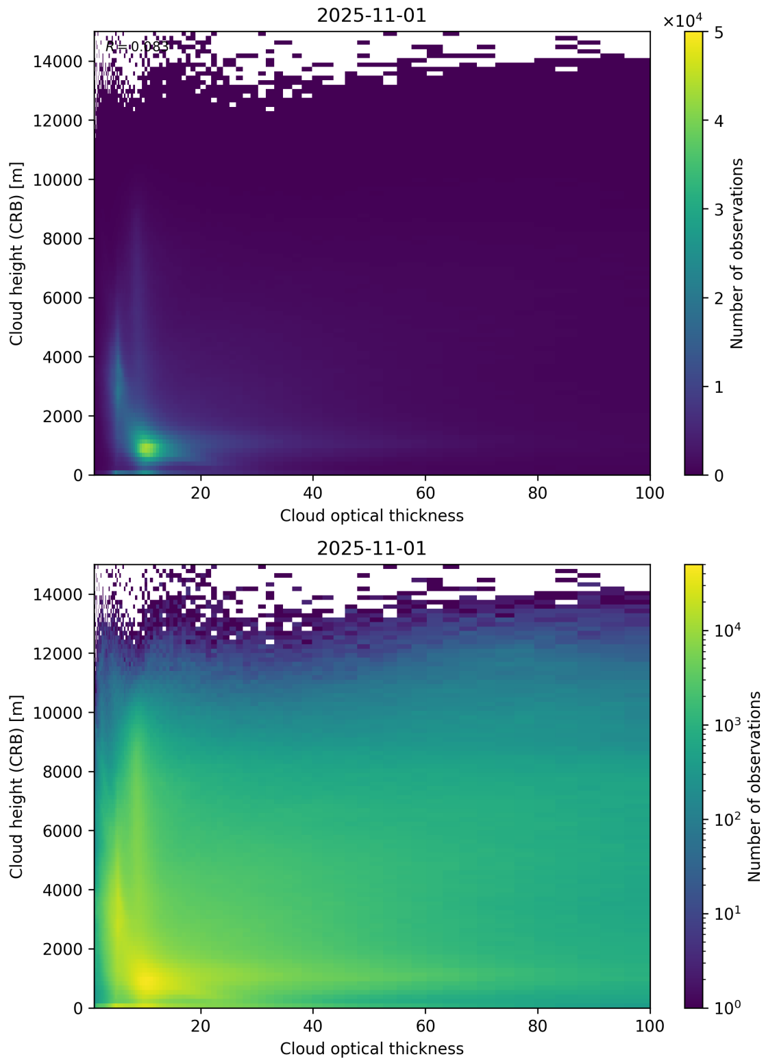
Figure 85: Scatter density plot of “Cloud optical thickness” against “Cloud height (CRB)” for 2025-10-31 to 2025-11-02.
