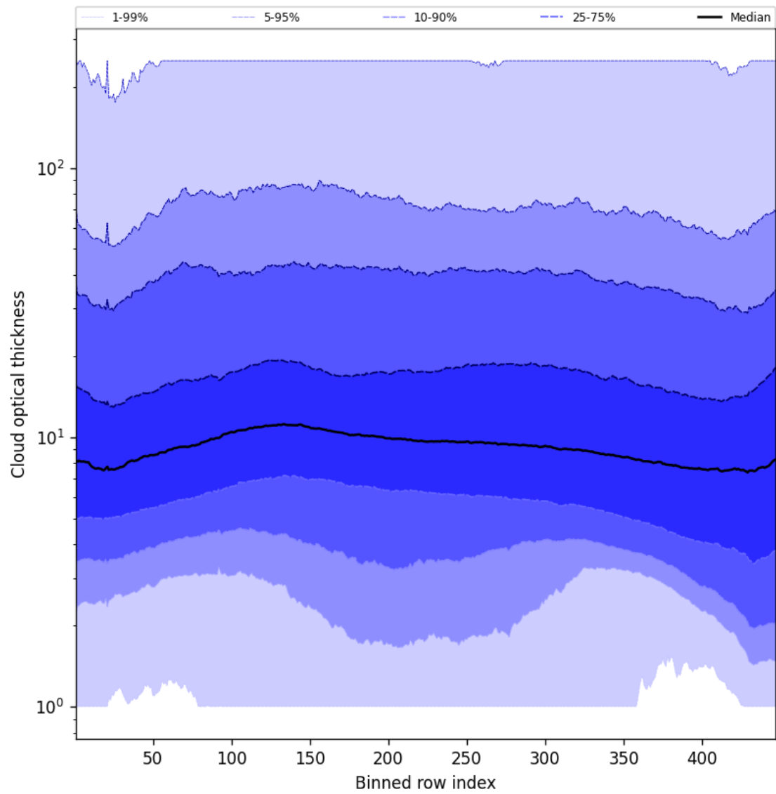
Figure 57: Along track statistics of “Cloud optical thickness” for 2025-10-31 to 2025-11-02
