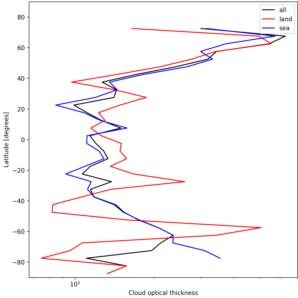
Figure 25: Zonal average of “Cloud optical thickness” for 2025-10-31 to 2025-11-02.
