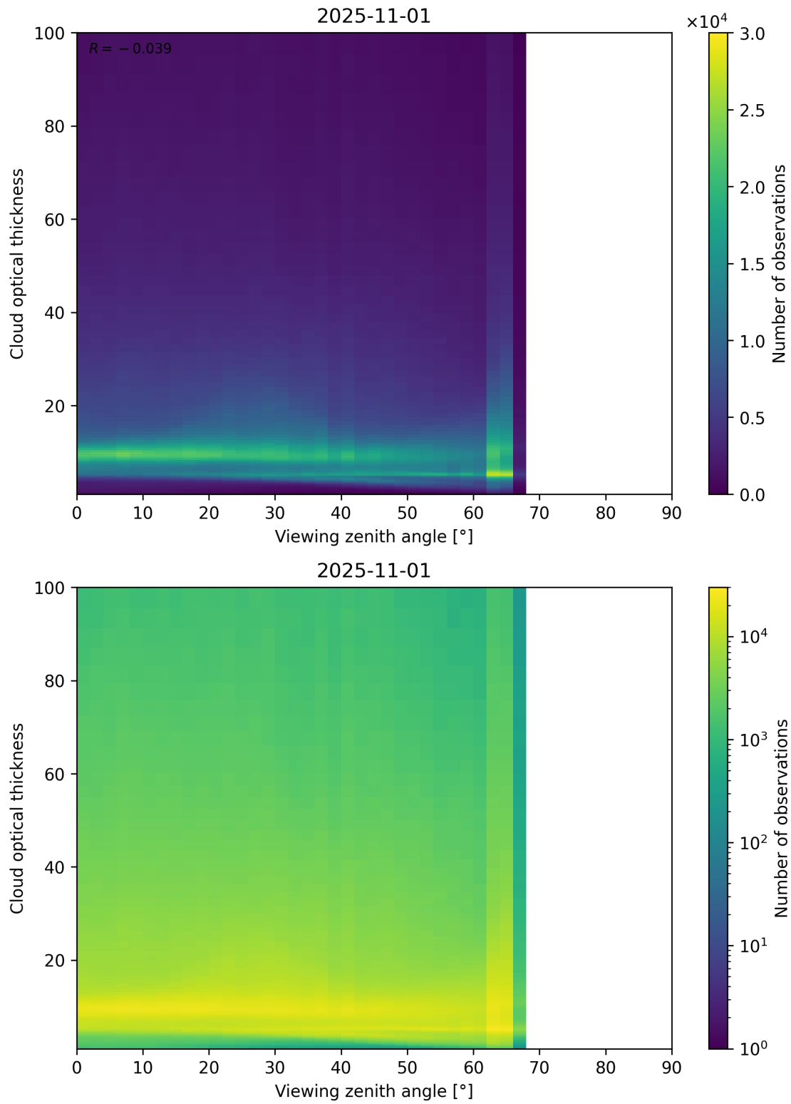
Figure 111: Scatter density plot of “Viewing zenith angle” against “Cloud optical thickness” for 2025-10-31 to 2025-11-02.
