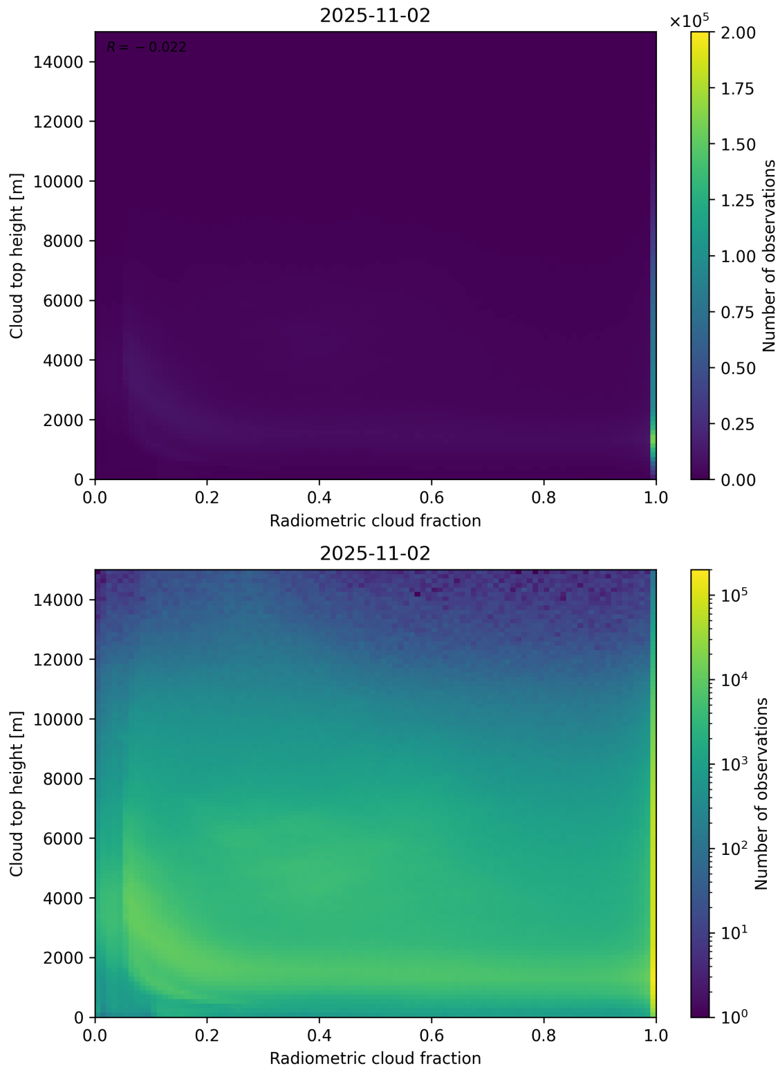
Figure 76: Scatter density plot of “Radiometric cloud fraction” against “Cloud top height” for 2025-11-02 to 2025-11-03.
