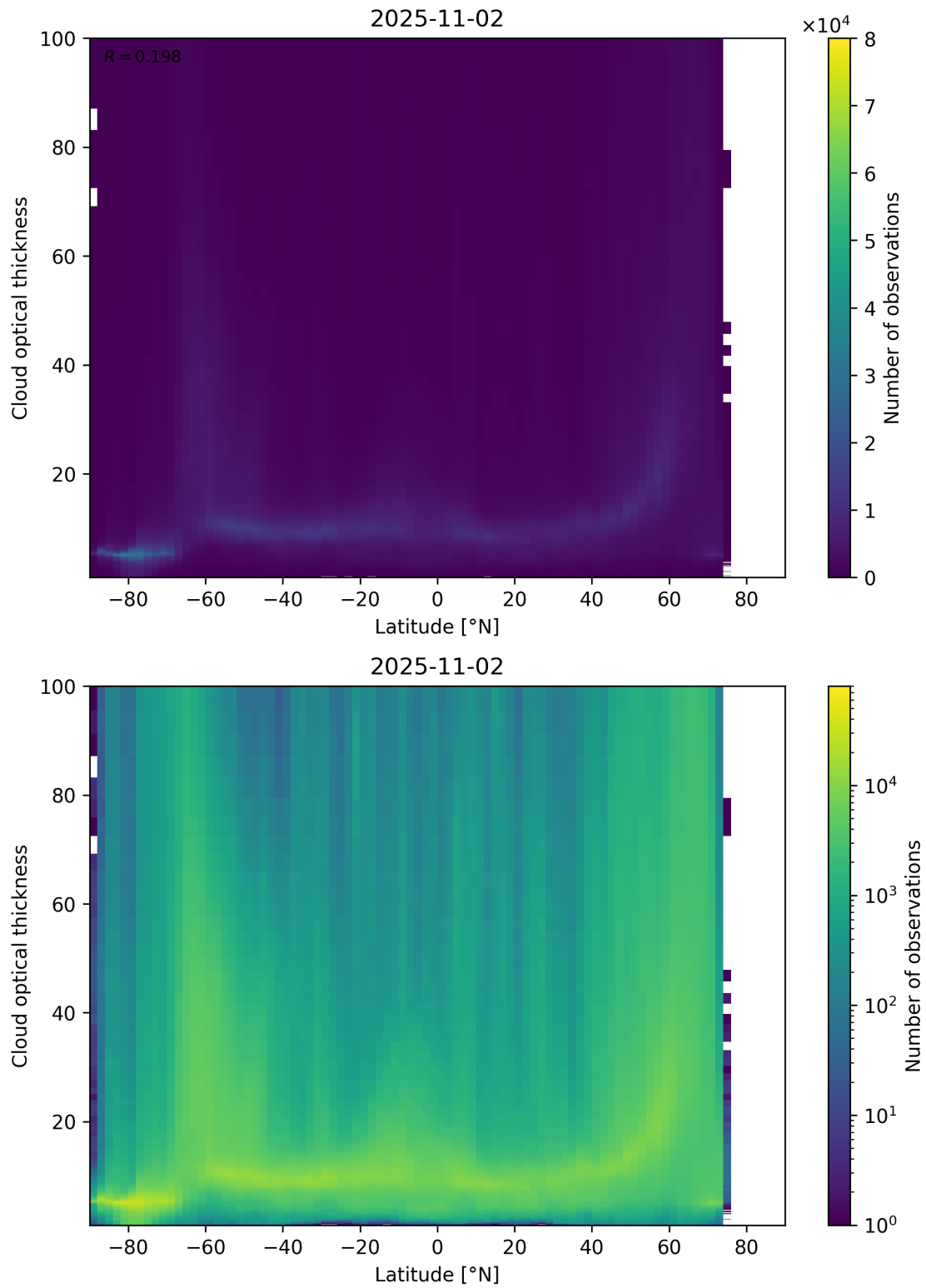
Figure 96: Scatter density plot of “Latitude” against “Cloud optical thickness” for 2025-11-02 to 2025-11-03.
