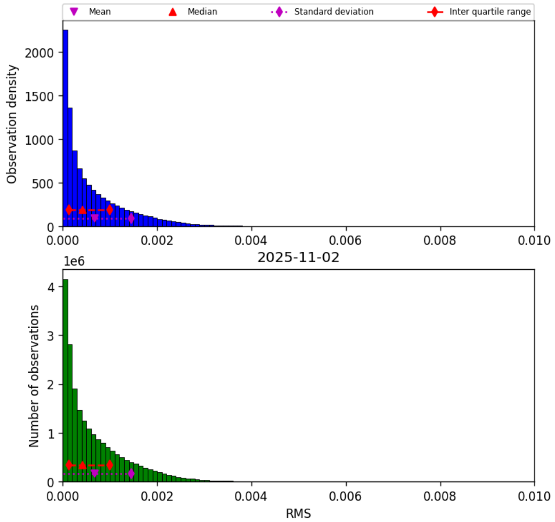
Figure 47: Histogram of “RMS” for 2025-11-02 to 2025-11-03
