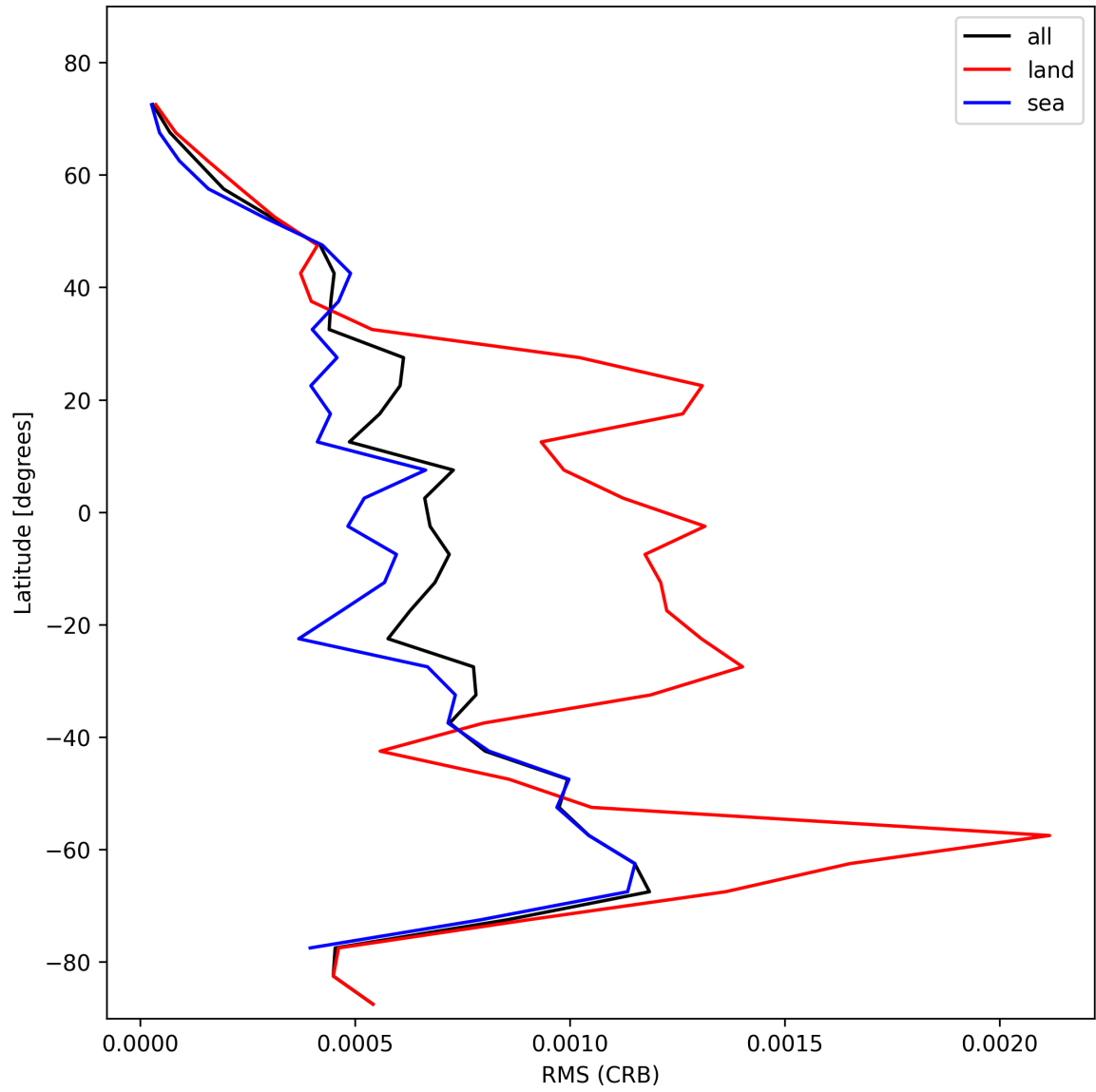
Figure 32: Zonal average of “RMS (CRB)” for 2025-11-02 to 2025-11-03.
