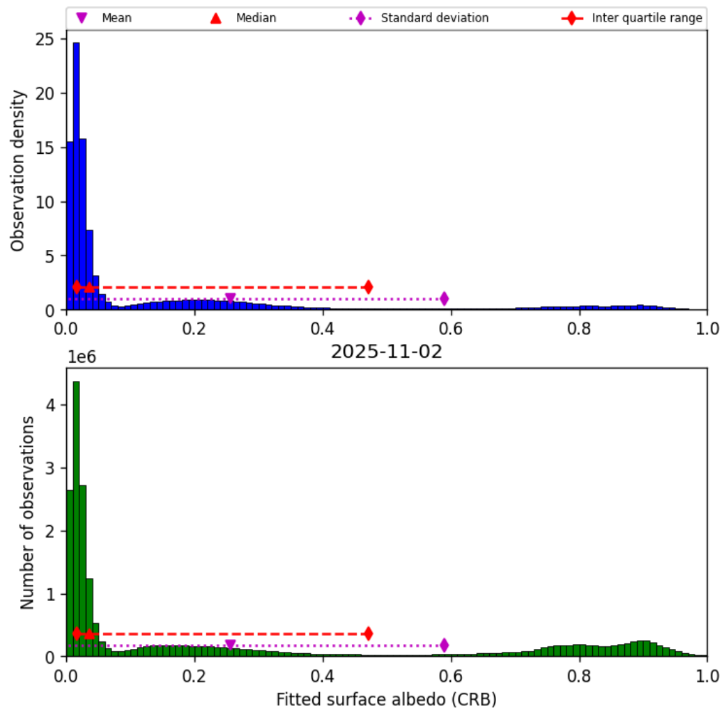
Figure 46: Histogram of “Fitted surface albedo (CRB)” for 2025-11-02 to 2025-11-03
