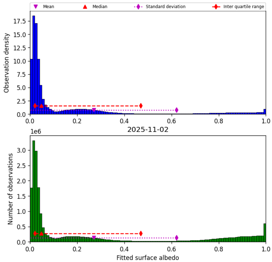
Figure 45: Histogram of “Fitted surface albedo” for 2025-11-02 to 2025-11-03
