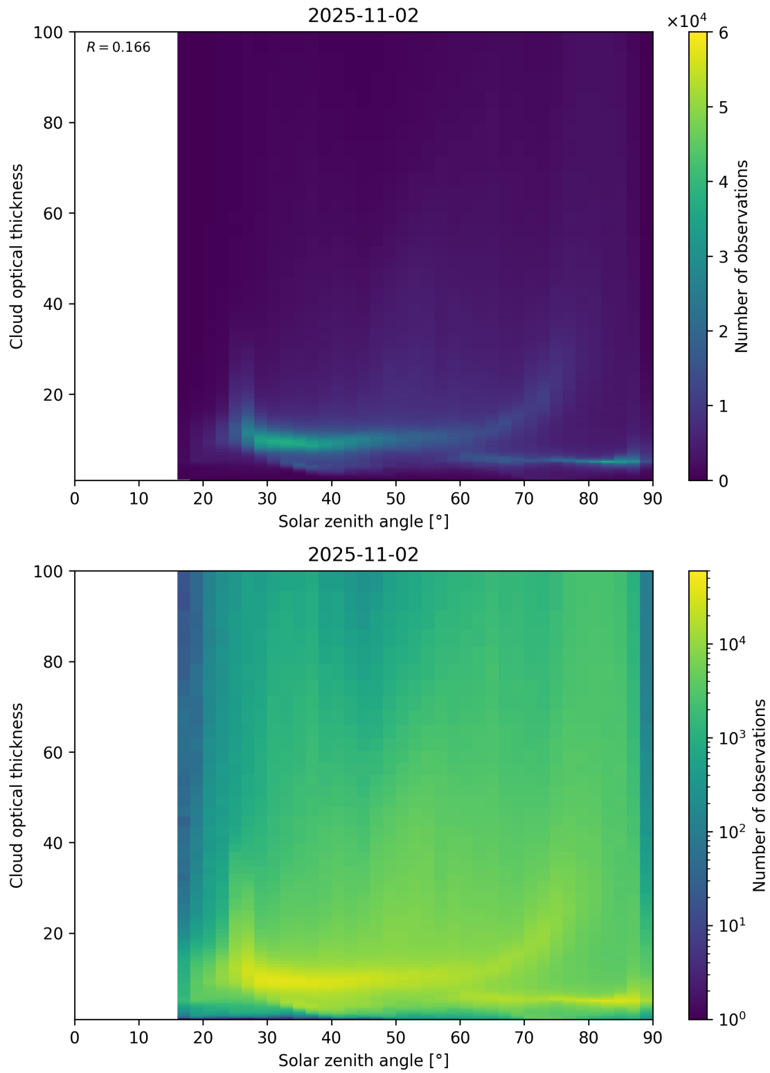
Figure 103: Scatter density plot of “Solar zenith angle” against “Cloud optical thickness” for 2025-11-02 to 2025-11-03.
