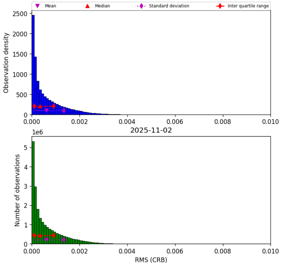
Figure 48: Histogram of “RMS (CRB)” for 2025-11-02 to 2025-11-03
