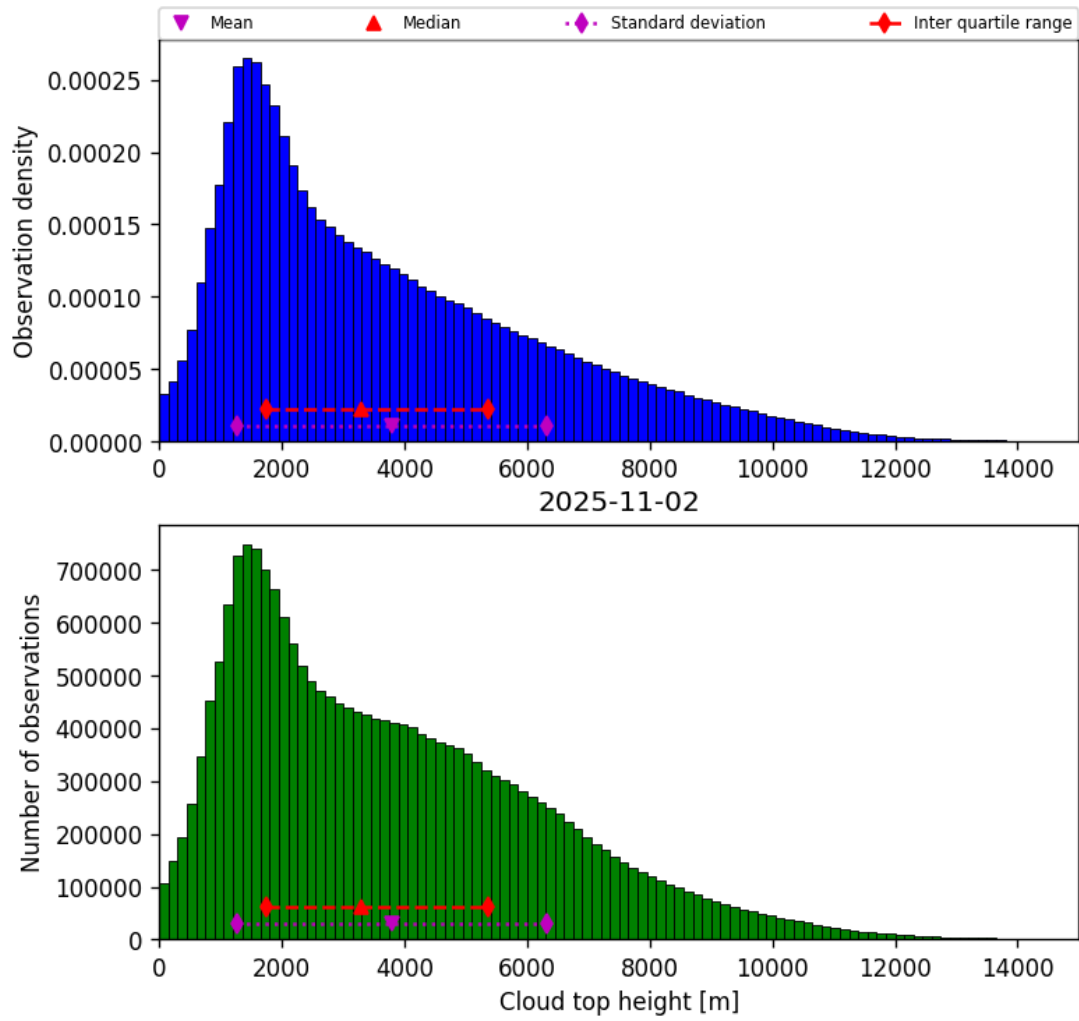
Figure 40: Histogram of “Cloud top height” for 2025-11-02 to 2025-11-03
