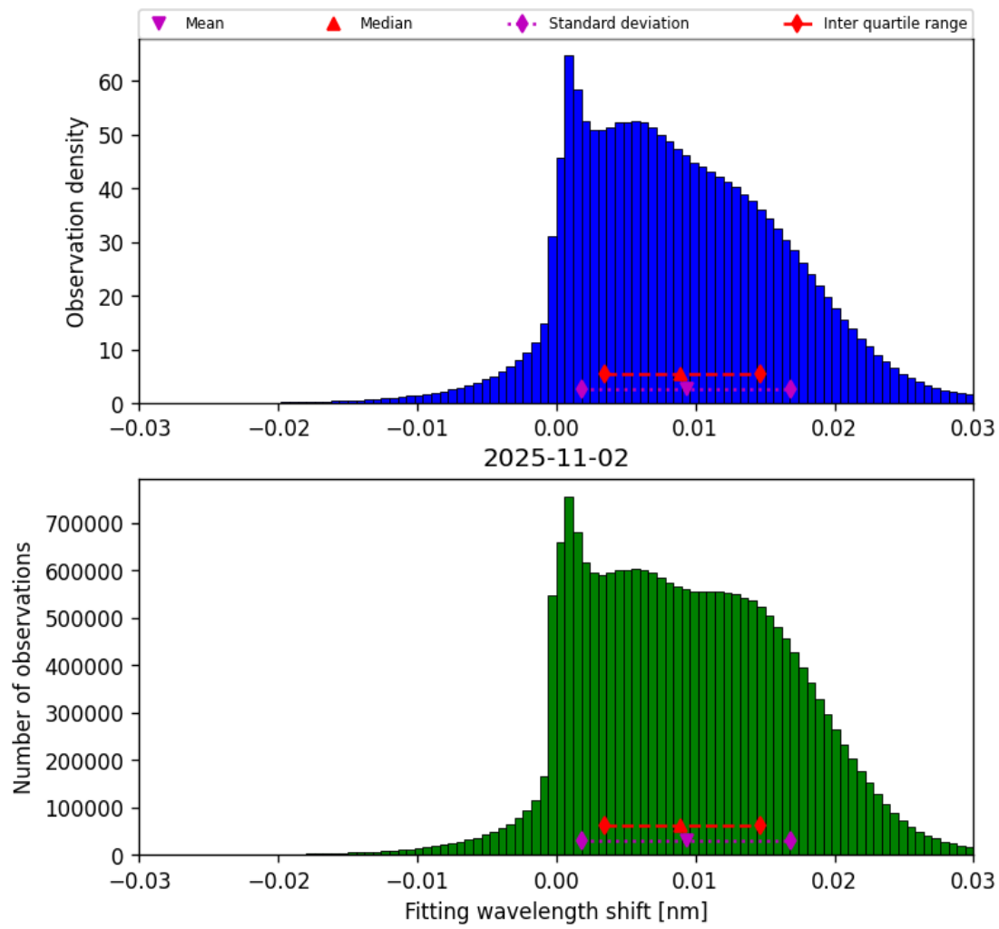
Figure 49: Histogram of “Fitting wavelength shift” for 2025-11-02 to 2025-11-03
