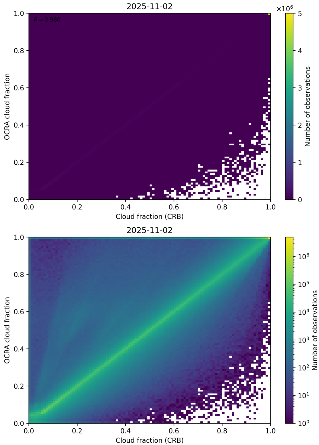
Figure 78: Scatter density plot of “Cloud fraction (CRB)” against “OCRA cloud fraction” for 2025-11-02 to 2025-11-03.
