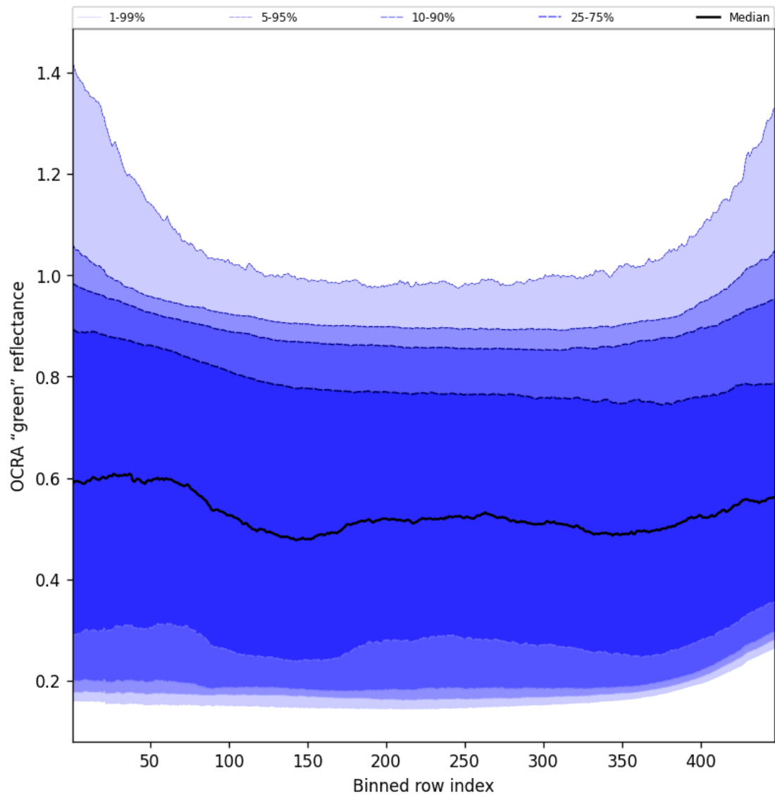
Figure 68: Along track statistics of "OCRA "green" reflectance" for 2025-11-02 to 2025-11-03
