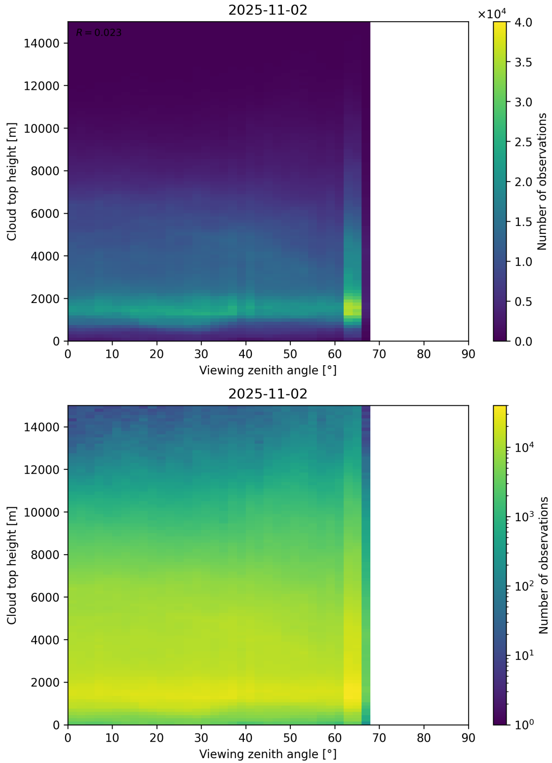
Figure 112: Scatter density plot of “Viewing zenith angle” against “Cloud top height” for 2025-11-02 to 2025-11-03.
