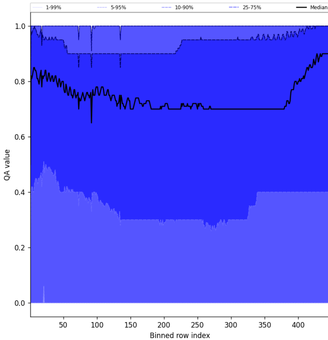
Figure 54: Along track statistics of “QA value” for 2025-11-02 to 2025-11-03
