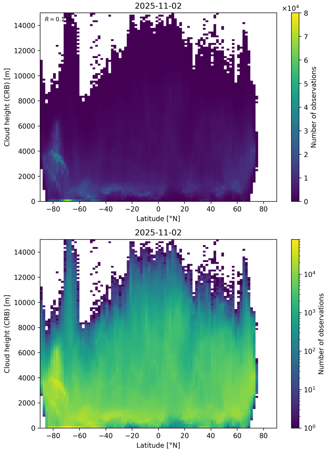
Figure 95: Scatter density plot of “Latitude” against “Cloud height (CRB)” for 2025-11-02 to 2025-11-03.
