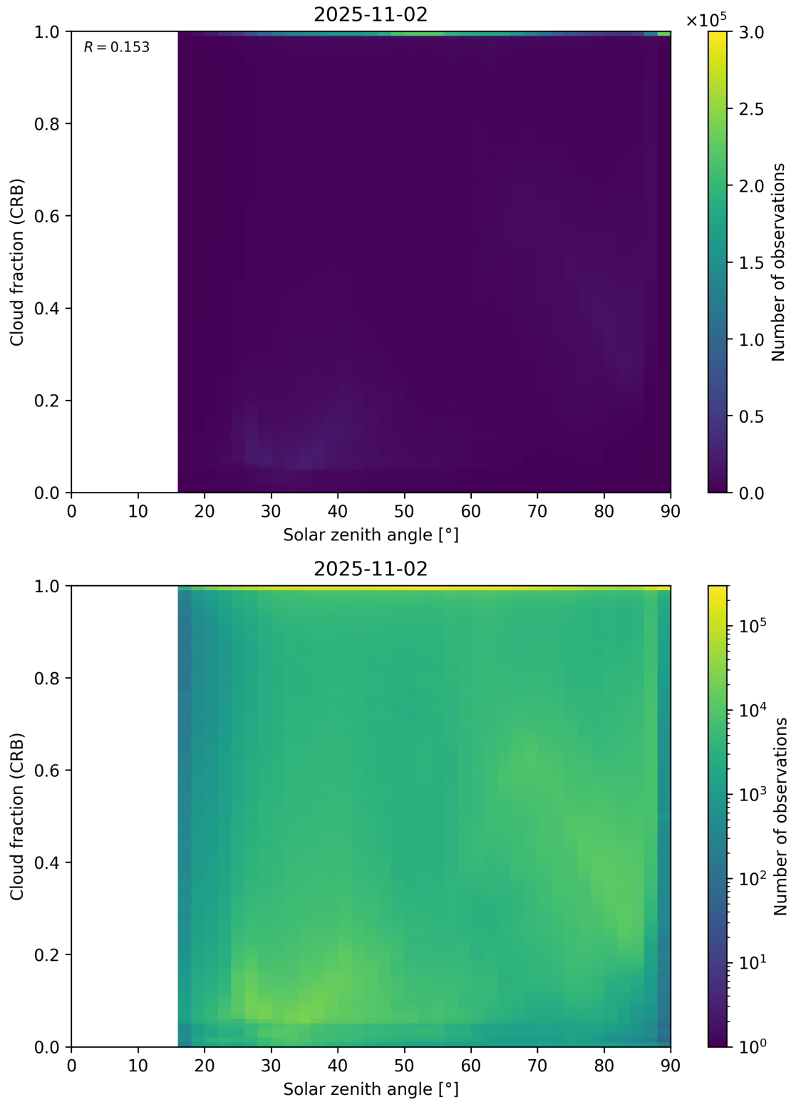
Figure 101: Scatter density plot of “Solar zenith angle” against “Cloud fraction (CRB)” for 2025-11-02 to 2025-11-03.
