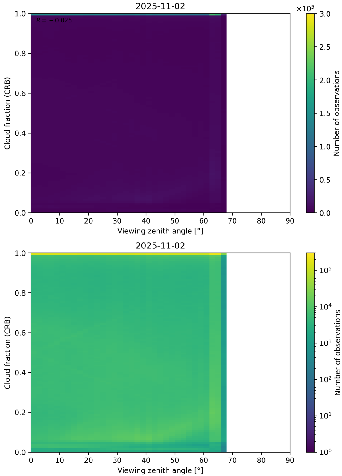
Figure 109: Scatter density plot of “Viewing zenith angle” against “Cloud fraction (CRB)” for 2025-11-02 to 2025-11-03.
