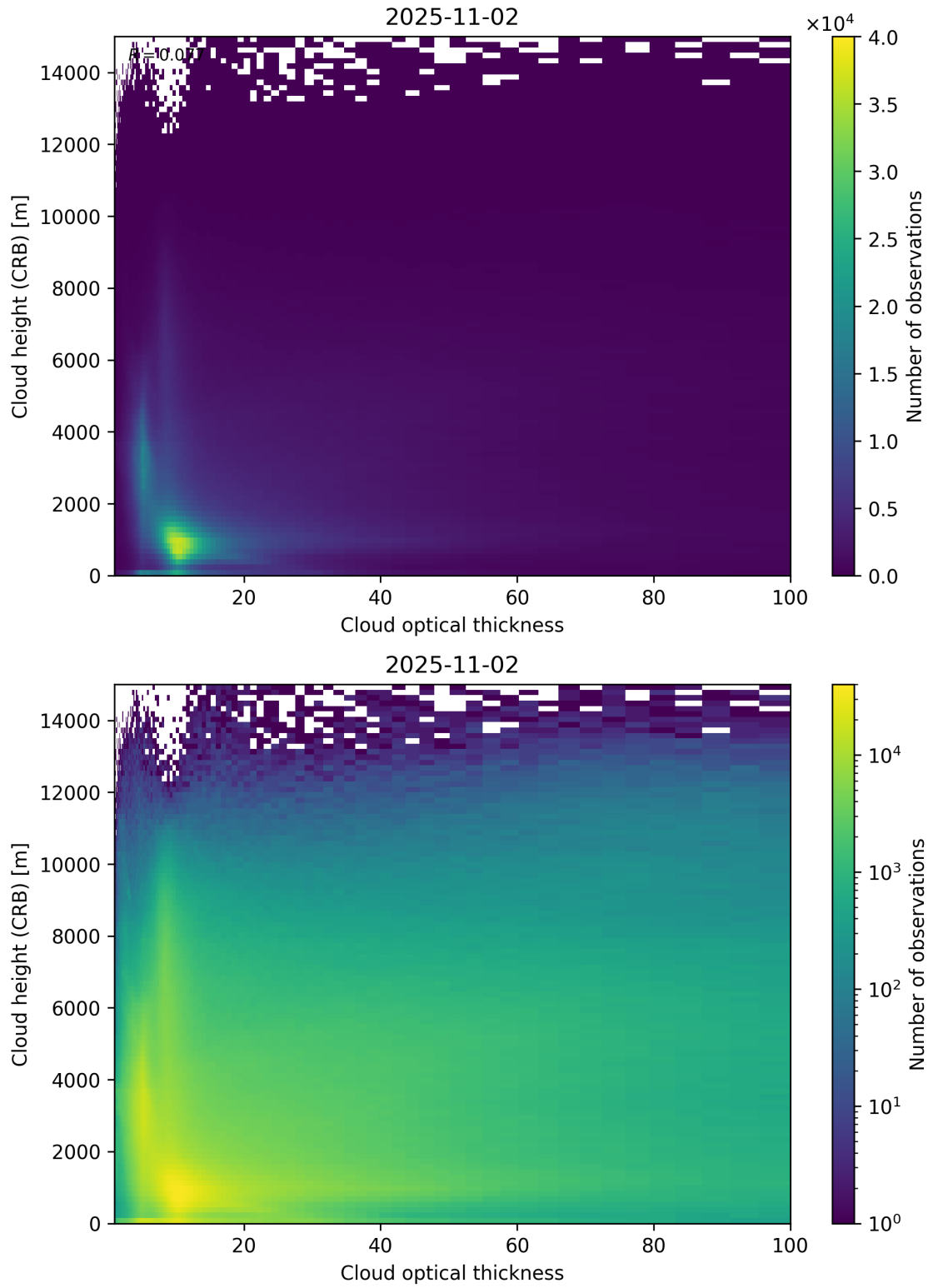
Figure 85: Scatter density plot of “Cloud optical thickness” against “Cloud height (CRB)” for 2025-11-02 to 2025-11-03.
