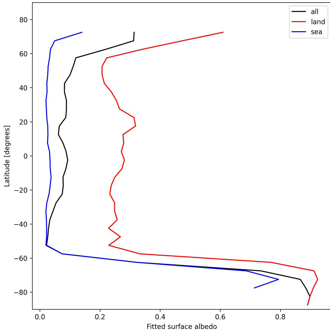
Figure 29: Zonal average of “Fitted surface albedo” for 2025-11-02 to 2025-11-03.
