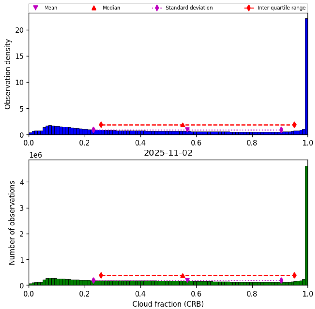
Figure 42: Histogram of “Cloud fraction (CRB)” for 2025-11-02 to 2025-11-03
