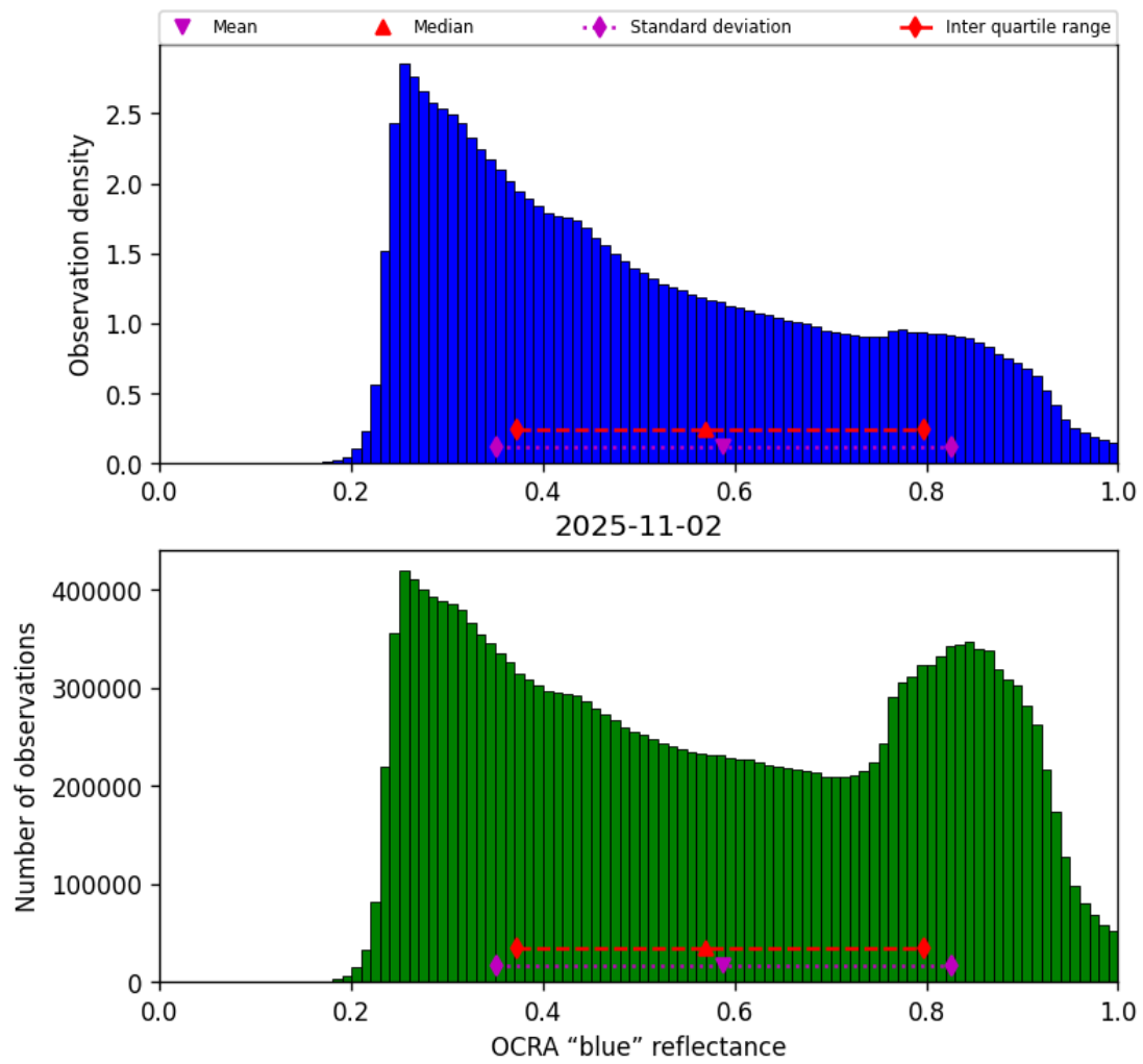
Figure 51: Histogram of “OCRA “blue” reflectance” for 2025-11-02 to 2025-11-03
