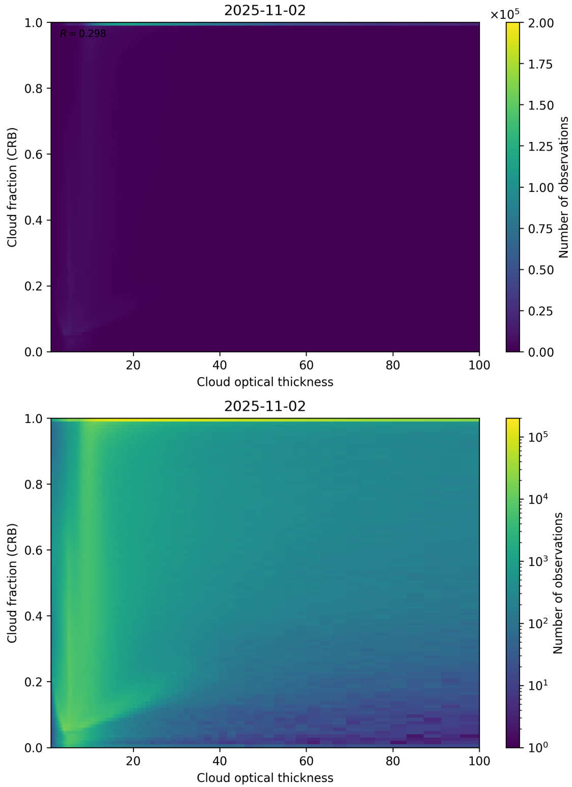
Figure 84: Scatter density plot of “Cloud optical thickness” against “Cloud fraction (CRB)” for 2025-11-02 to 2025-11-03.
