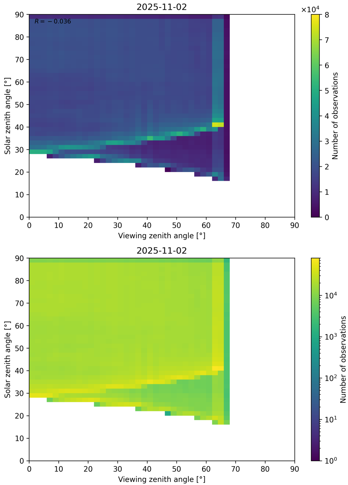
Figure 114: Scatter density plot of “Viewing zenith angle” against “Solar zenith angle” for 2025-11-02 to 2025-11-03.
