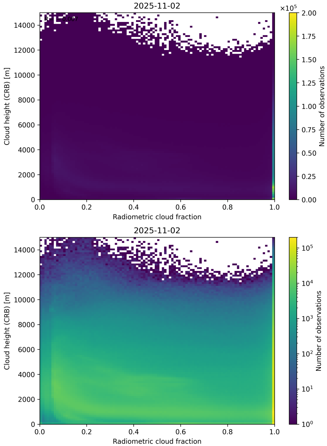
Figure 74: Scatter density plot of “Radiometric cloud fraction” against “Cloud height (CRB)” for 2025-11-02 to 2025-11-03.
