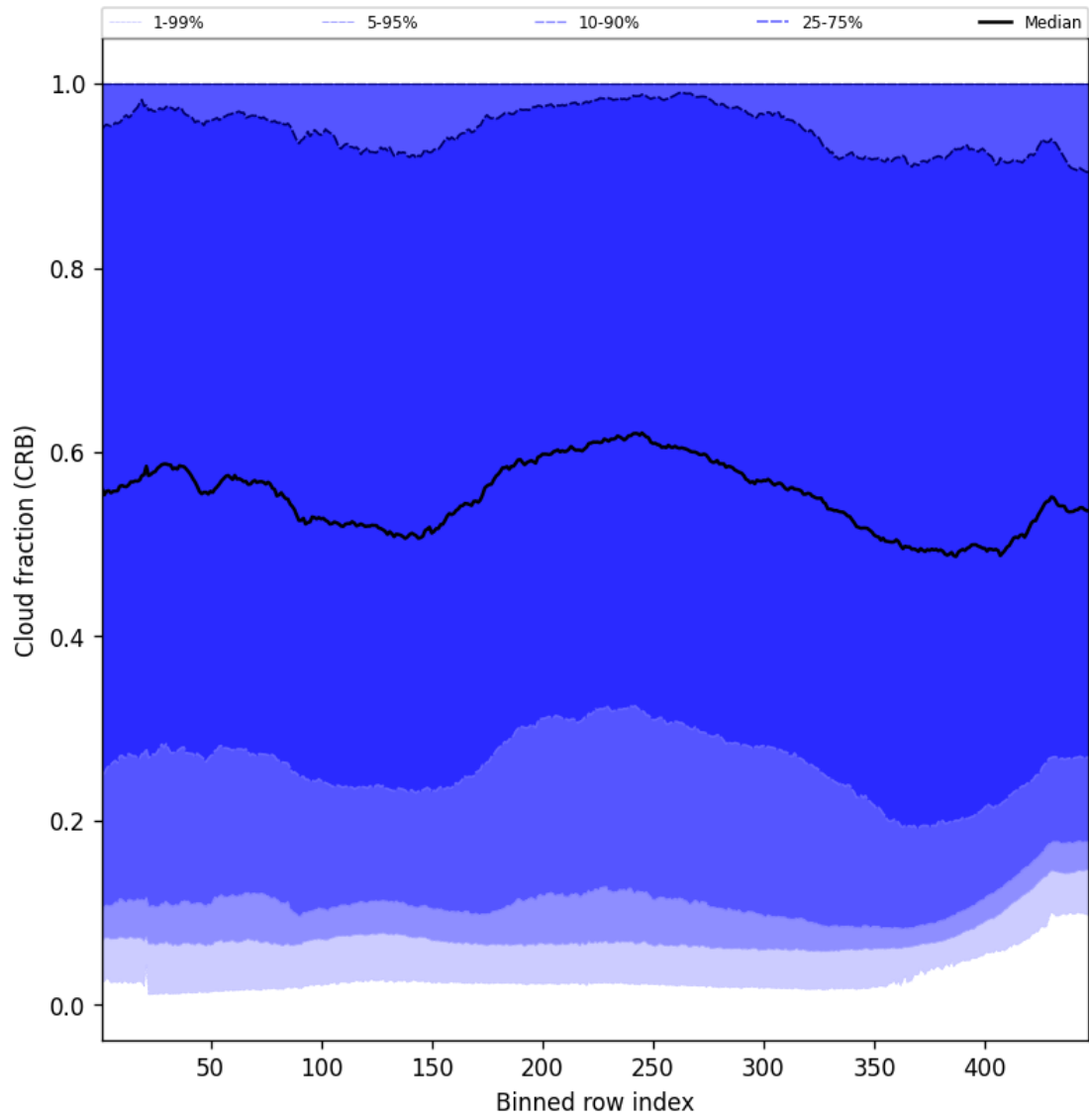
Figure 58: Along track statistics of “Cloud fraction (CRB)” for 2025-11-02 to 2025-11-03
