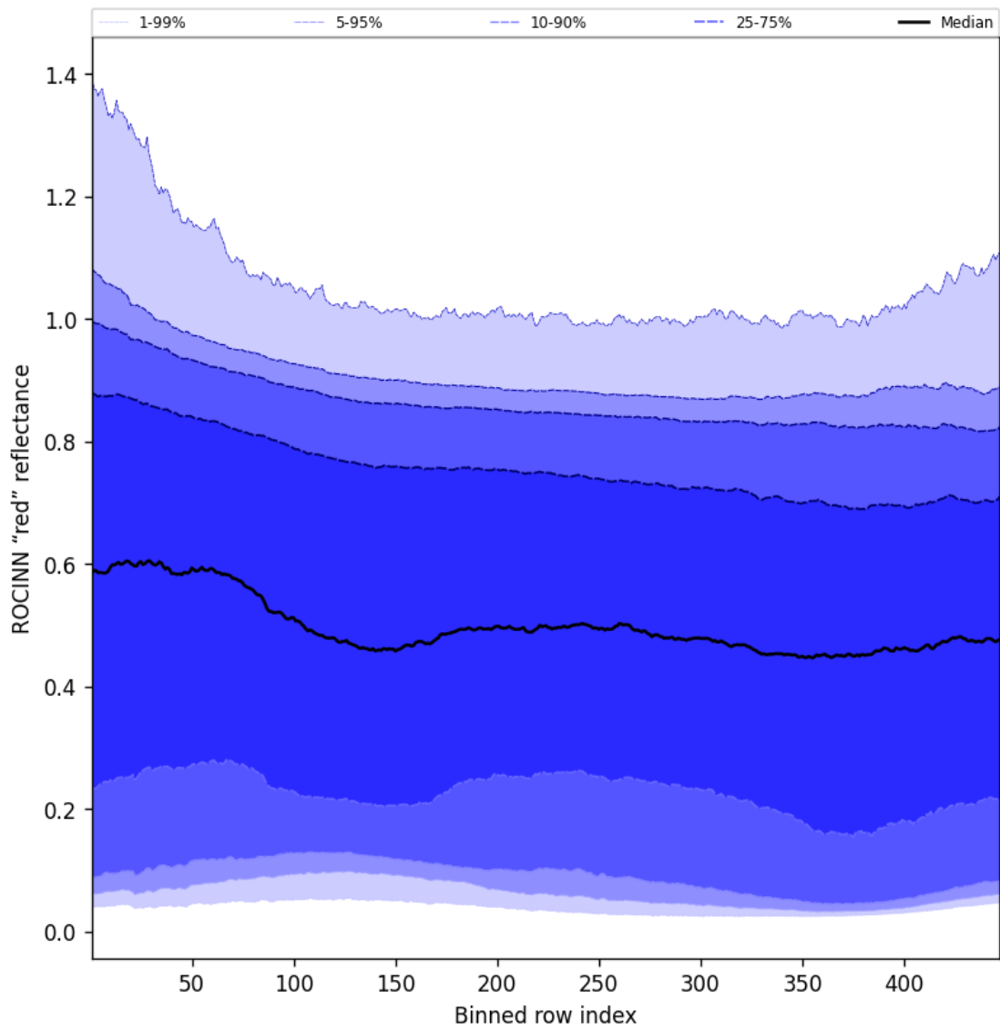
Figure 69: Along track statistics of "ROCINN "red" reflectance" for 2025-11-02 to 2025-11-03
