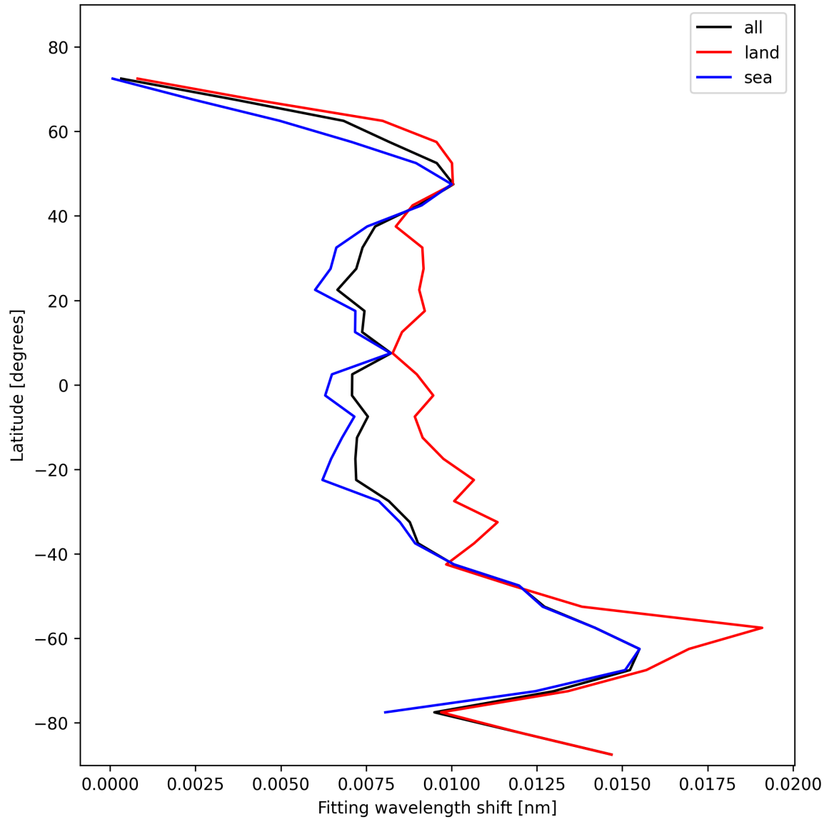
Figure 33: Zonal average of “Fitting wavelength shift” for 2025-11-02 to 2025-11-03.
