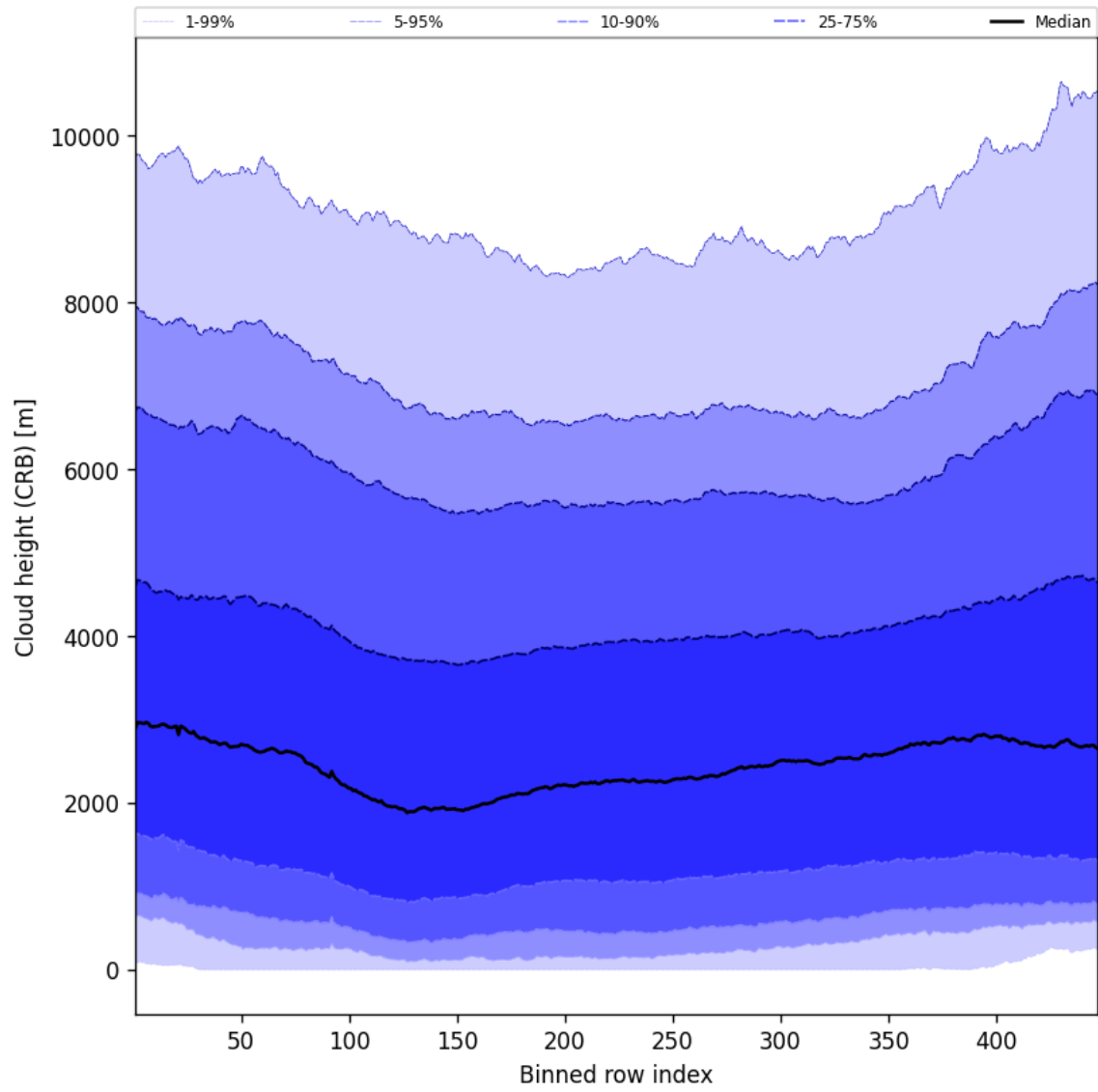
Figure 59: Along track statistics of “Cloud height (CRB)” for 2025-11-02 to 2025-11-03
