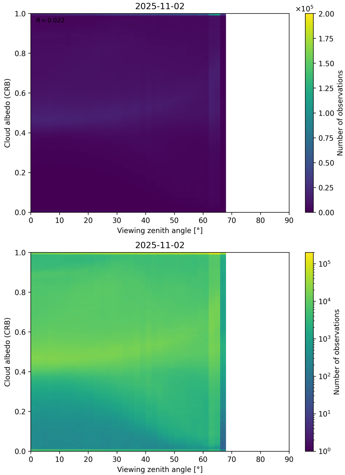
Figure 106: Scatter density plot of “Viewing zenith angle” against “Cloud albedo (CRB)” for 2025-11-02 to 2025-11-03.
