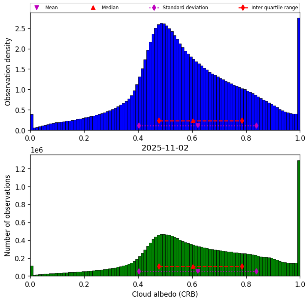
Figure 44: Histogram of “Cloud albedo (CRB)” for 2025-11-02 to 2025-11-03
