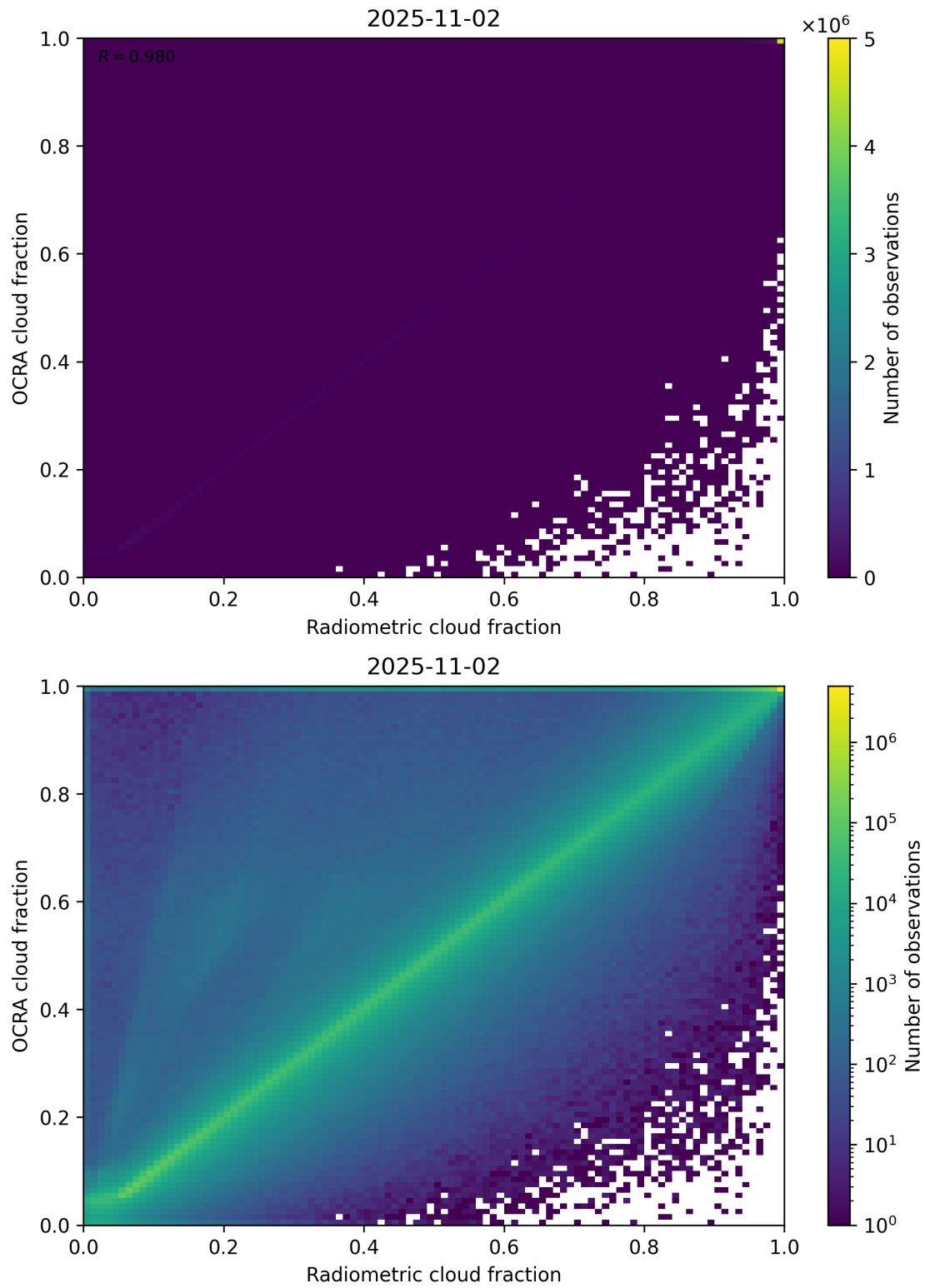
Figure 72: Scatter density plot of “Radiometric cloud fraction” against “OCRA cloud fraction” for 2025-11-02 to 2025-11-03.
