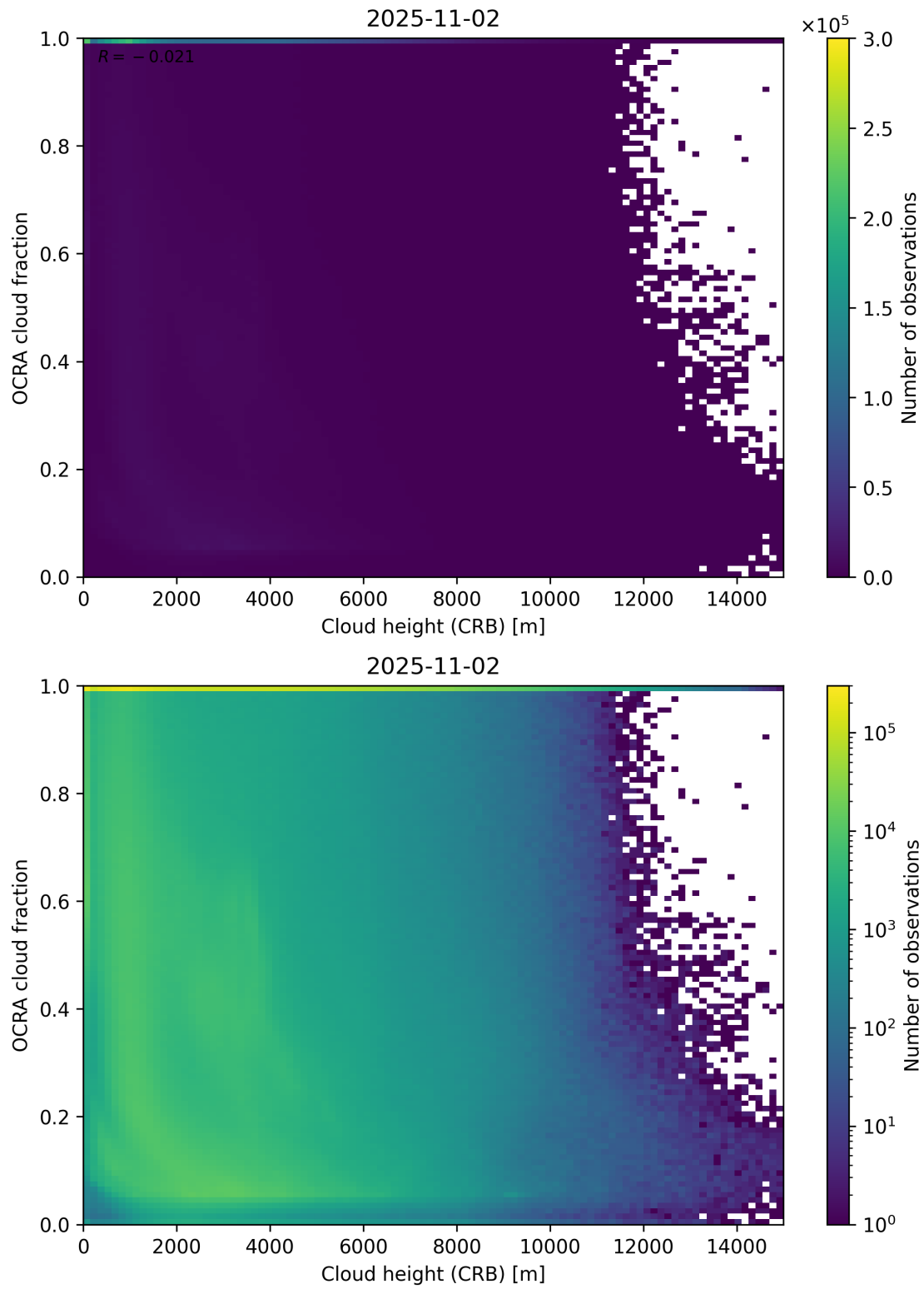
Figure 81: Scatter density plot of “Cloud height (CRB)” against “OCRA cloud fraction” for 2025-11-02 to 2025-11-03.
