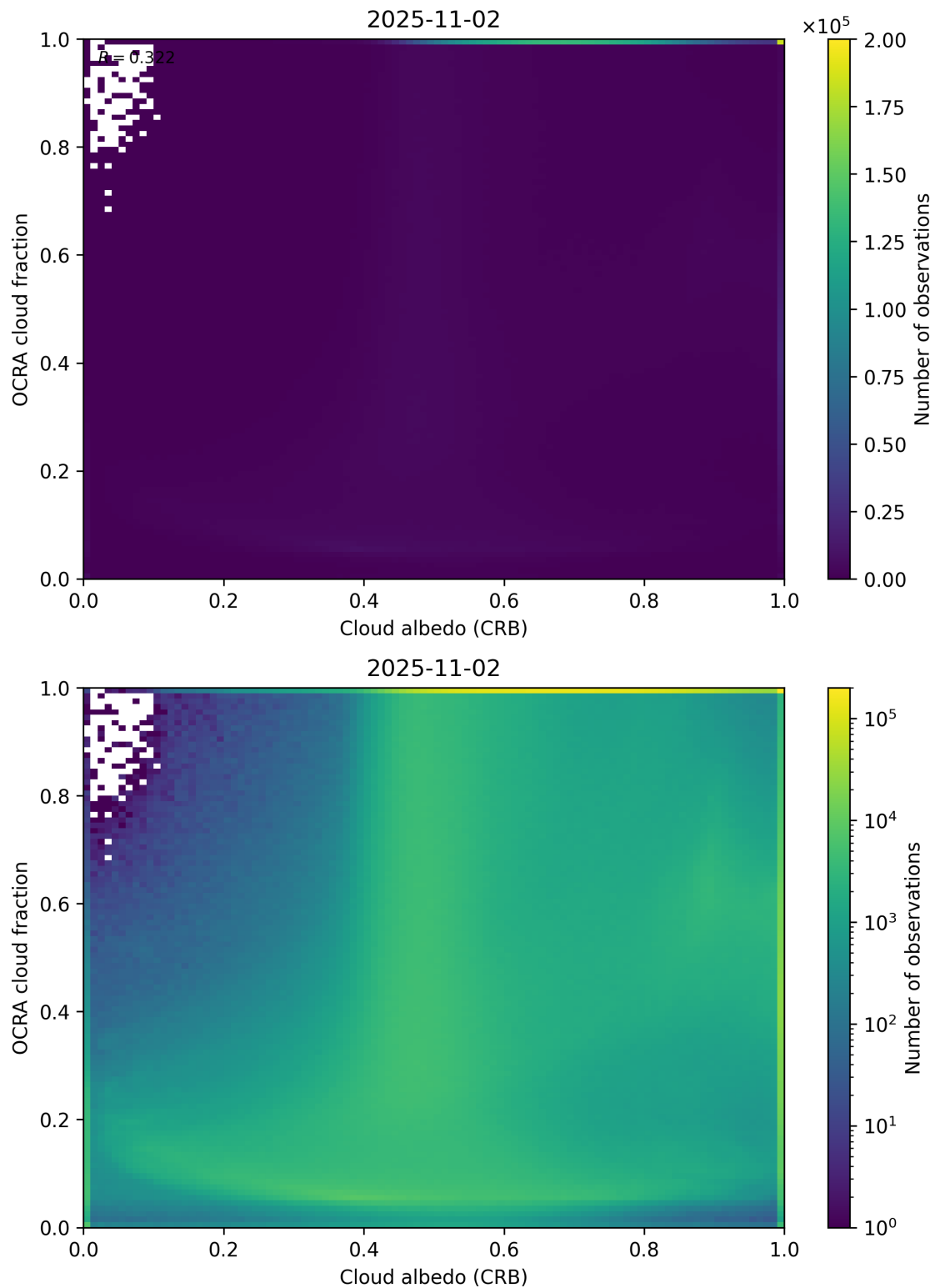
Figure 70: Scatter density plot of “Cloud albedo (CRB)” against “OCRA cloud fraction” for 2025-11-02 to 2025-11-03.
