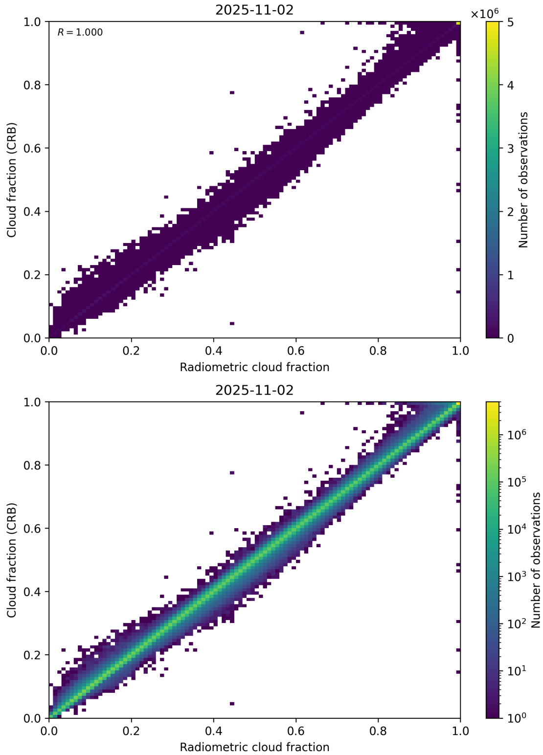
Figure 73: Scatter density plot of “Radiometric cloud fraction” against “Cloud fraction (CRB)” for 2025-11-02 to 2025-11-03.
