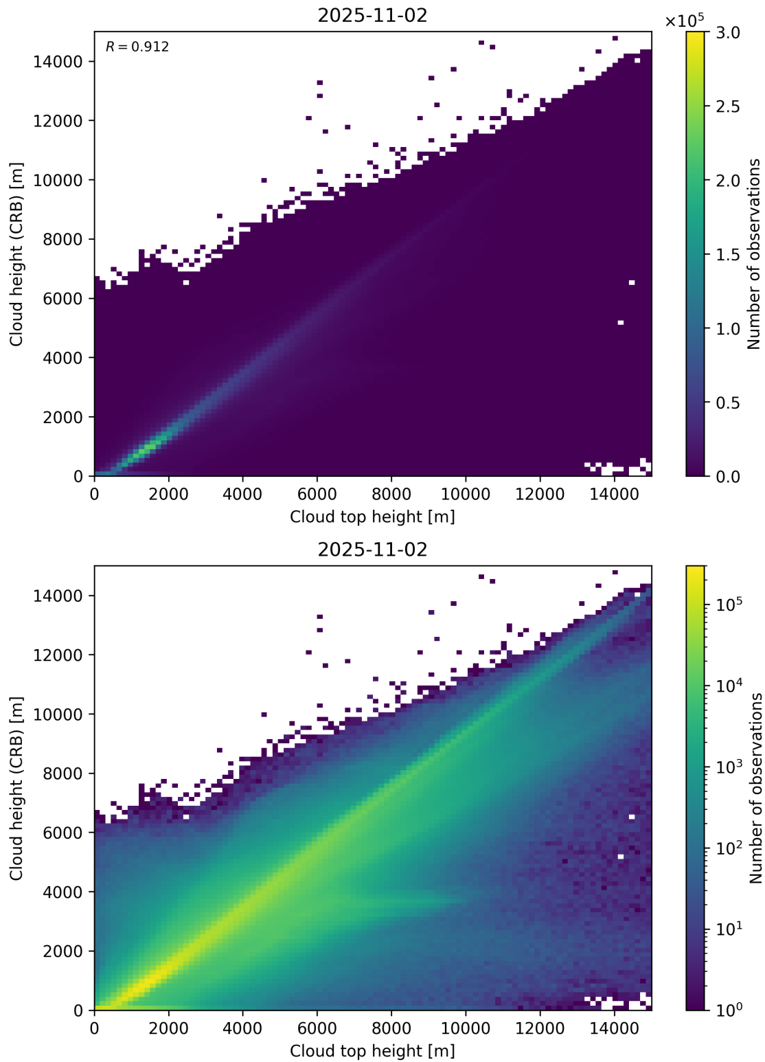
Figure 89: Scatter density plot of “Cloud top height” against “Cloud height (CRB)” for 2025-11-02 to 2025-11-03.
