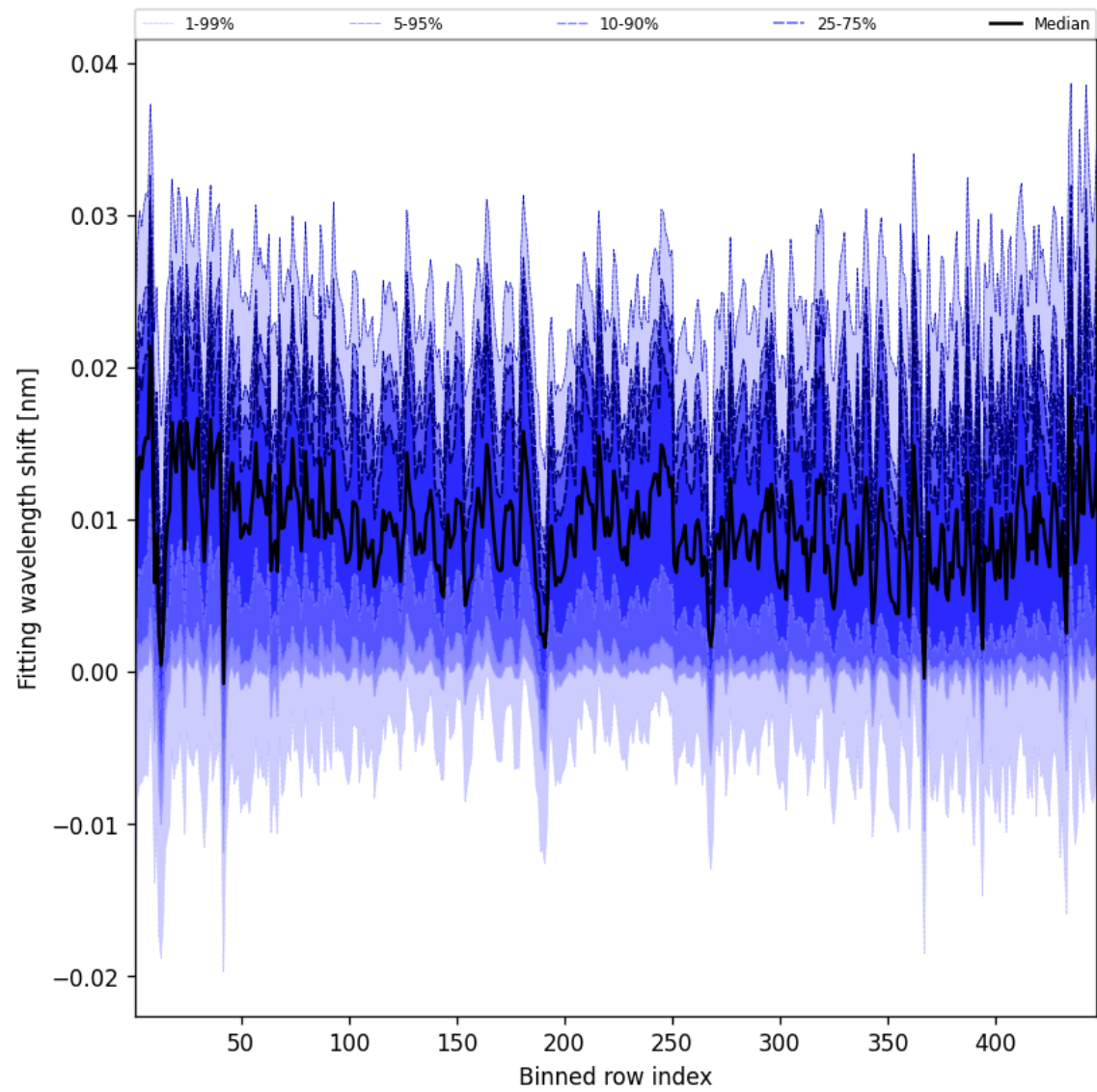
Figure 65: Along track statistics of “Fitting wavelength shift” for 2025-11-02 to 2025-11-03
