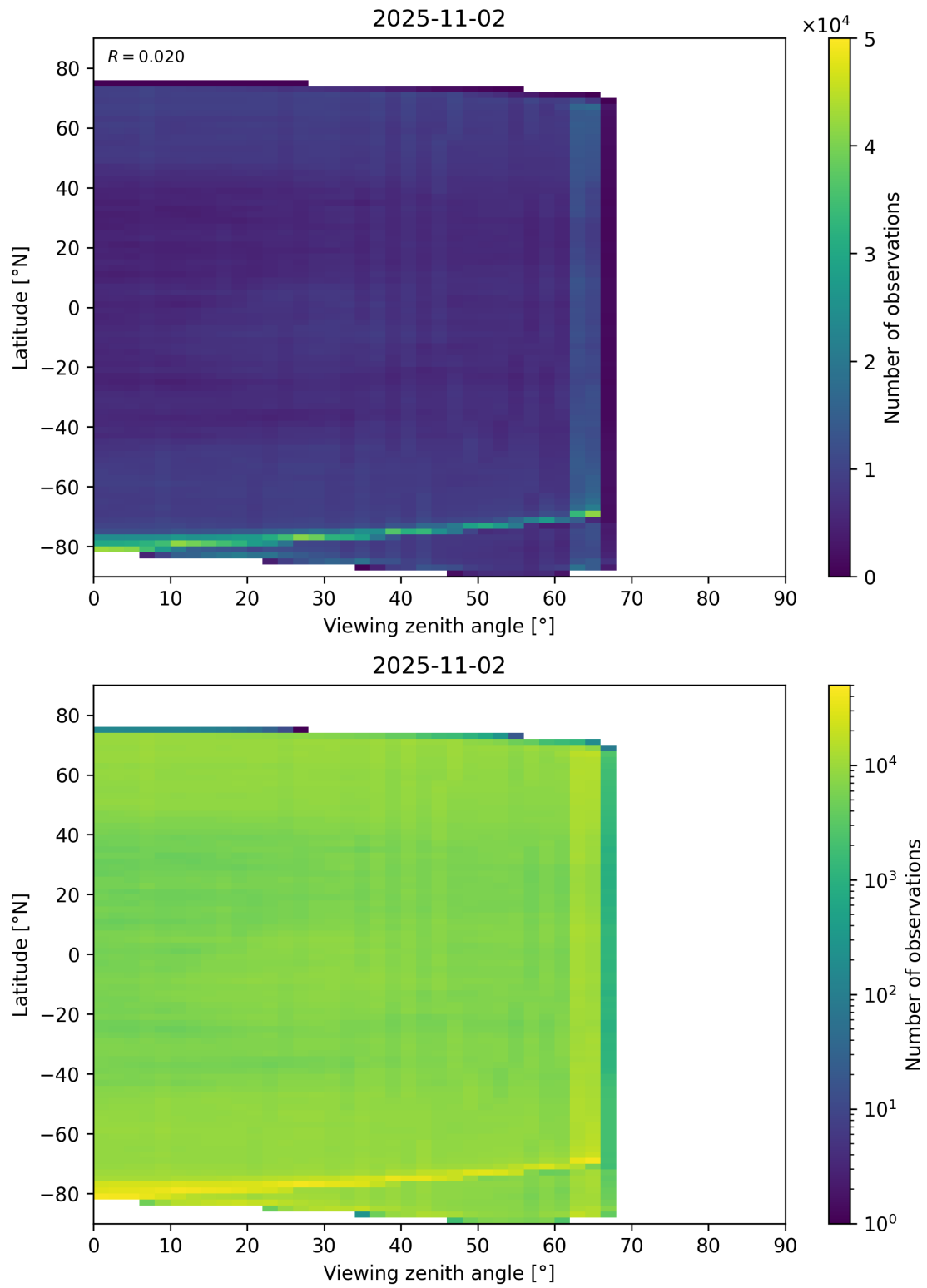
Figure 113: Scatter density plot of “Viewing zenith angle” against “Latitude” for 2025-11-02 to 2025-11-03.
