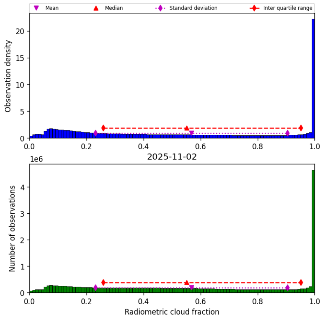
Figure 39: Histogram of “Radiometric cloud fraction” for 2025-11-02 to 2025-11-03
