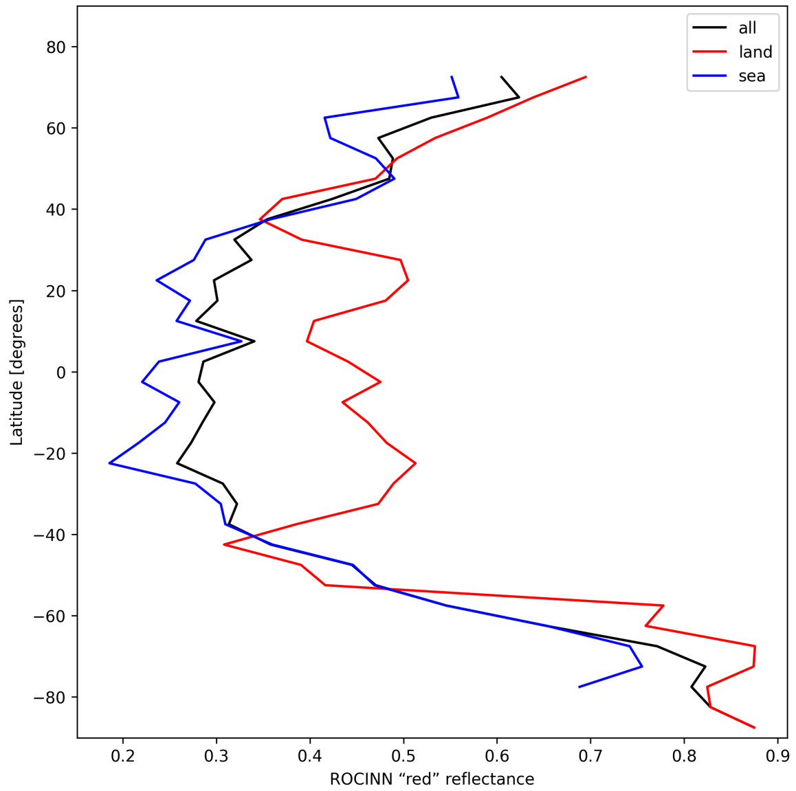
Figure 37: Zonal average of “ROCINN “red” reflectance” for 2025-11-02 to 2025-11-03.
