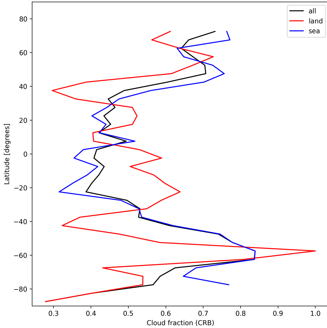
Figure 26: Zonal average of “Cloud fraction (CRB)” for 2025-11-02 to 2025-11-03.
