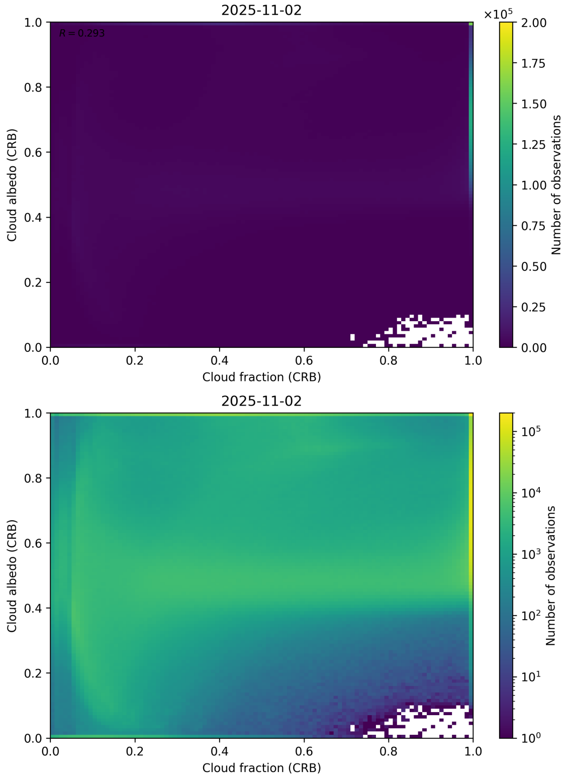
Figure 77: Scatter density plot of “Cloud fraction (CRB)” against “Cloud albedo (CRB)” for 2025-11-02 to 2025-11-03.
