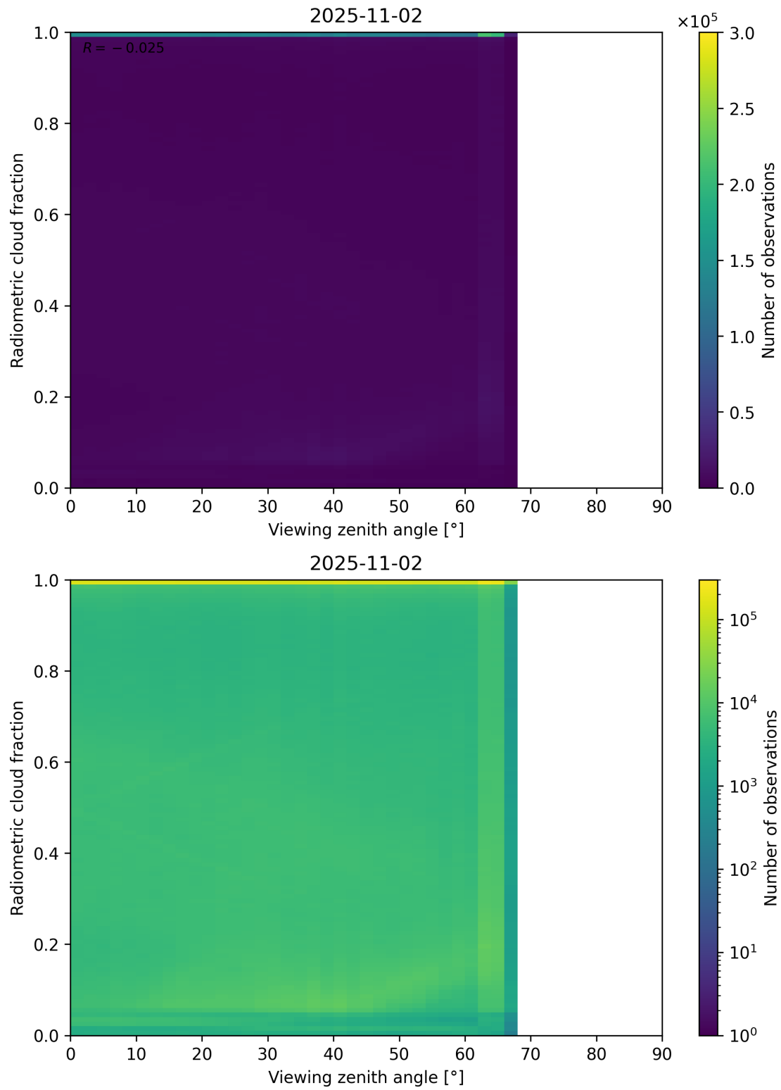
Figure 107: Scatter density plot of “Viewing zenith angle” against “Radiometric cloud fraction” for 2025-11-02 to 2025-11-03.
