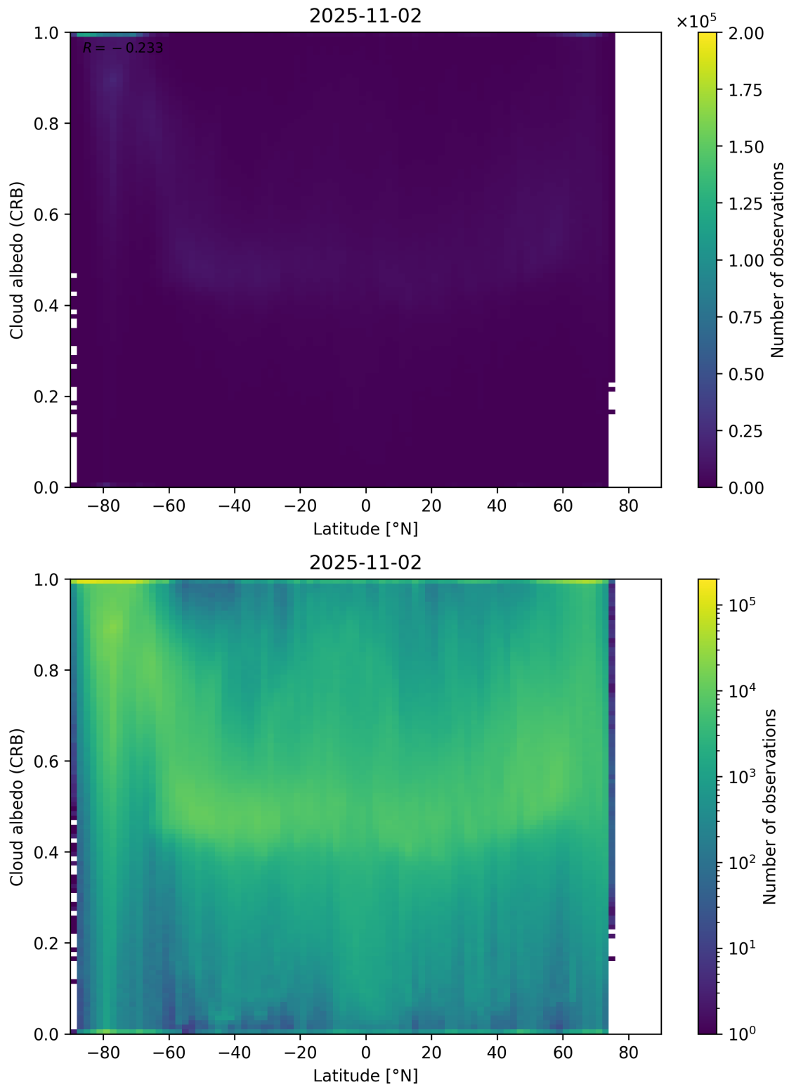
Figure 91: Scatter density plot of “Latitude” against “Cloud albedo (CRB)” for 2025-11-02 to 2025-11-03.
