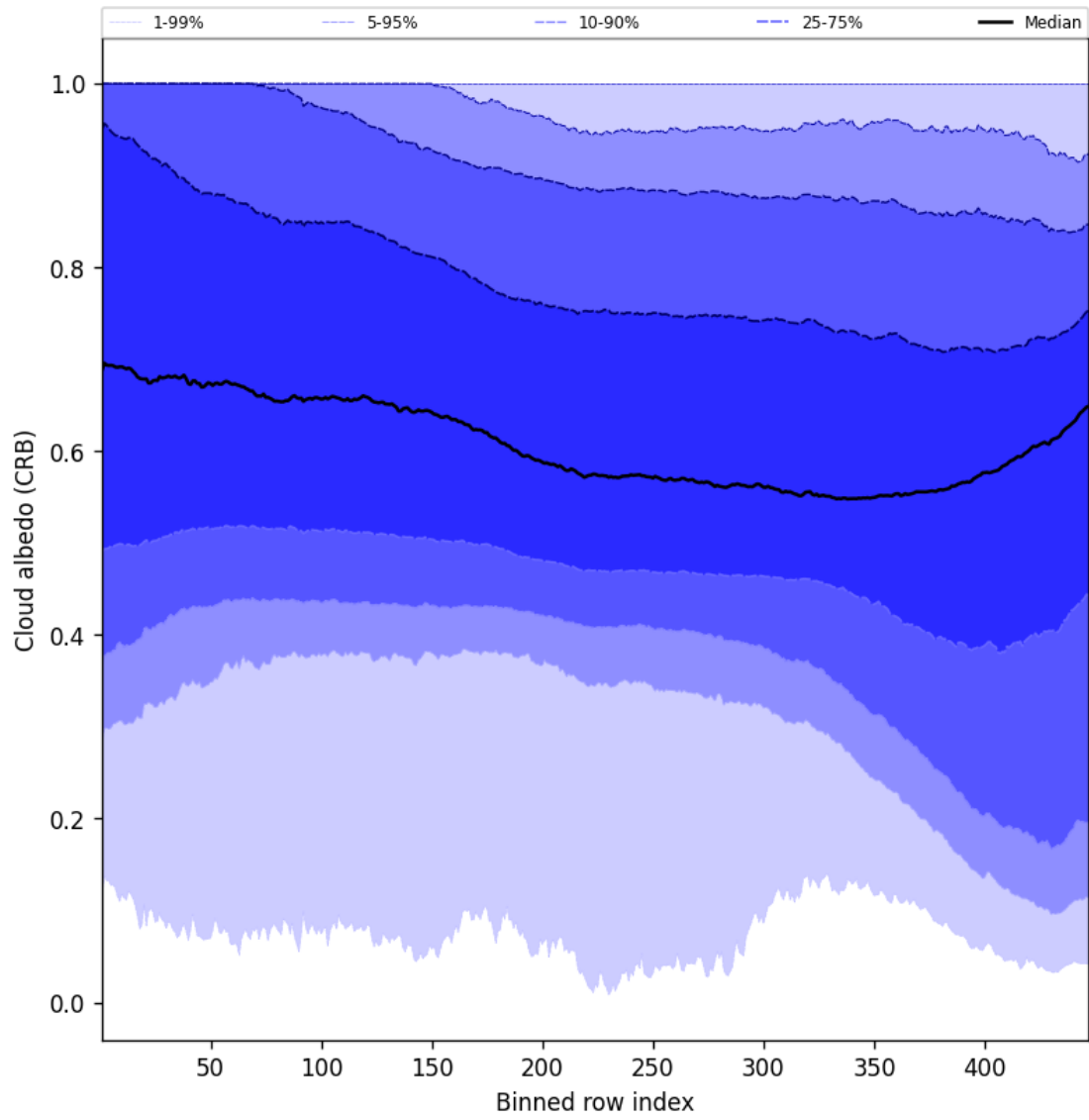
Figure 60: Along track statistics of “Cloud albedo (CRB)” for 2025-11-02 to 2025-11-03
