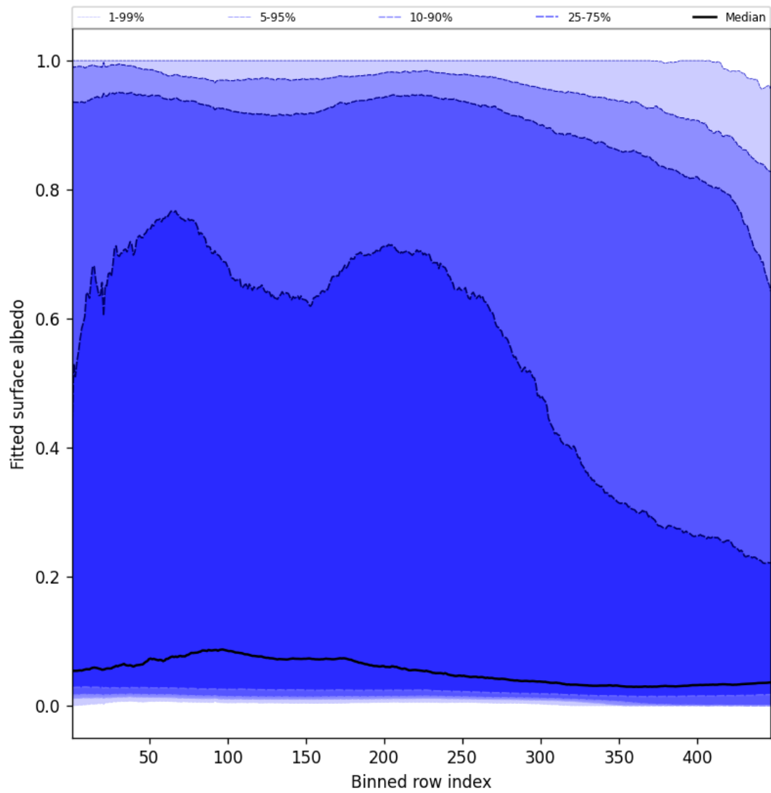
Figure 61: Along track statistics of “Fitted surface albedo” for 2025-11-02 to 2025-11-03
