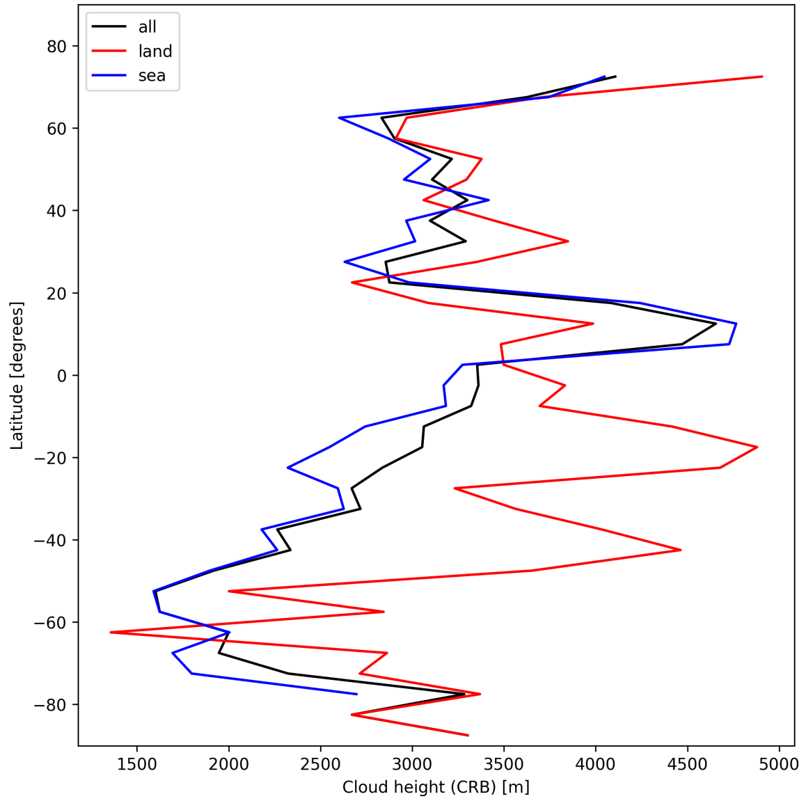
Figure 27: Zonal average of “Cloud height (CRB)” for 2025-11-02 to 2025-11-03.
