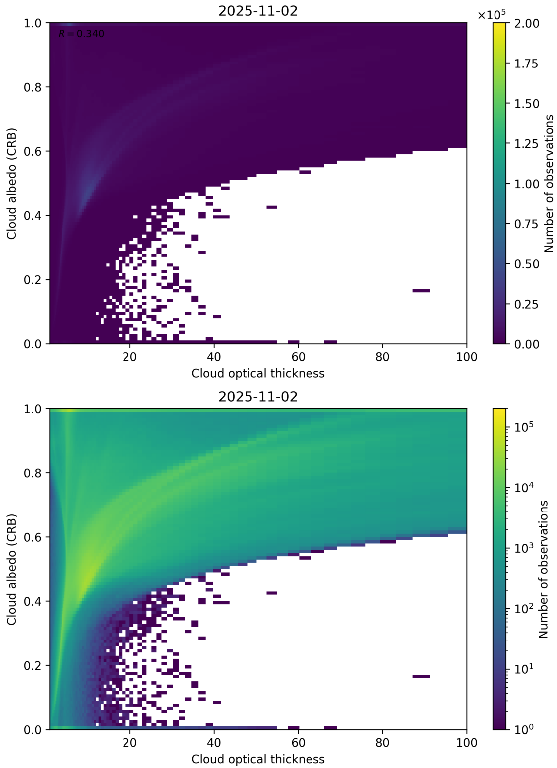
Figure 82: Scatter density plot of “Cloud optical thickness” against “Cloud albedo (CRB)” for 2025-11-02 to 2025-11-03.
