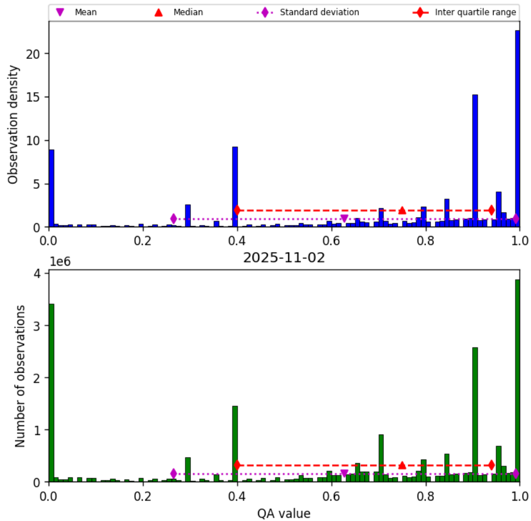
Figure 38: Histogram of “QA value” for 2025-11-02 to 2025-11-03
