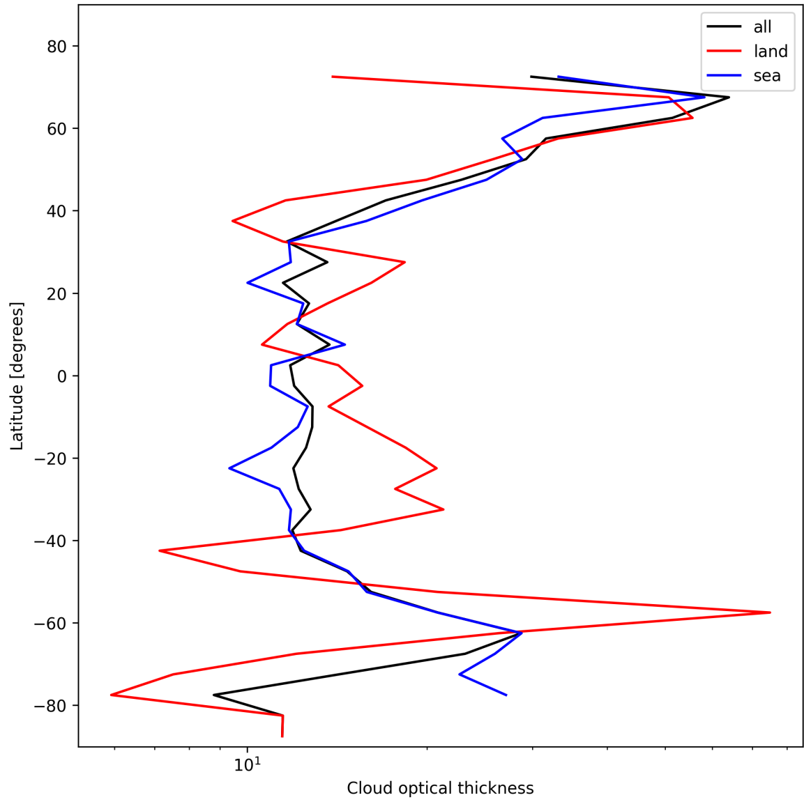
Figure 25: Zonal average of “Cloud optical thickness” for 2025-11-02 to 2025-11-03.
