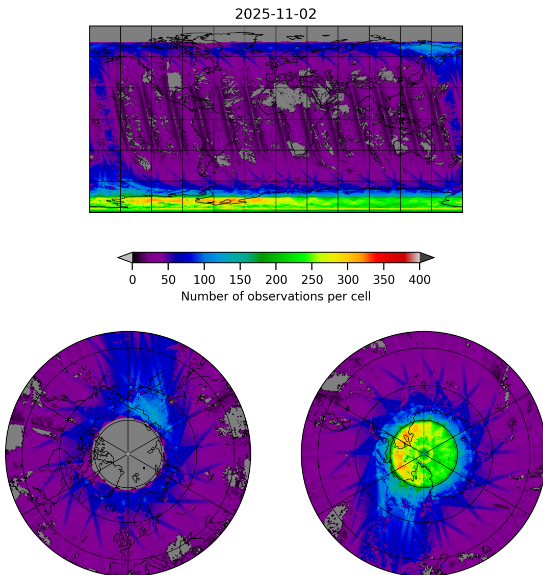
Figure 21: Map of the number of observations for 2025-11-02 to 2025-11-03
