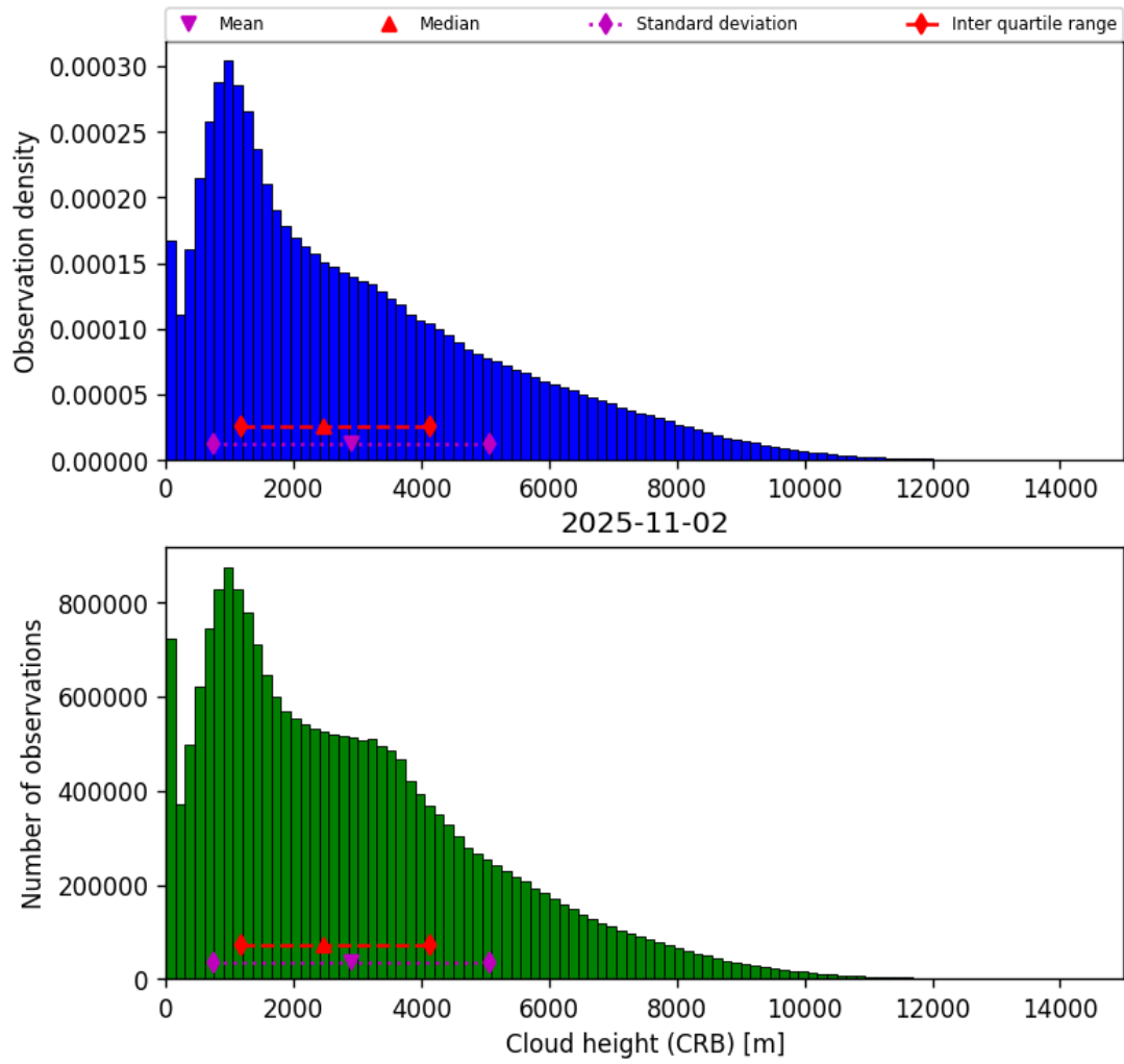
Figure 43: Histogram of “Cloud height (CRB)” for 2025-11-02 to 2025-11-03
