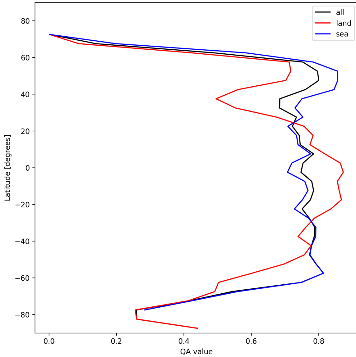
Figure 22: Zonal average of “QA value” for 2025-11-02 to 2025-11-03.
