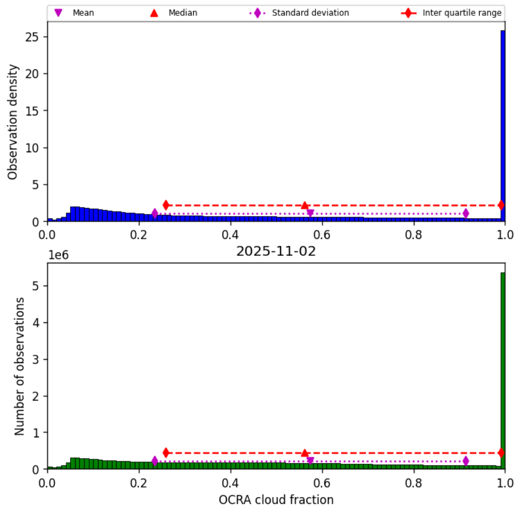
Figure 50: Histogram of “OCRA cloud fraction” for 2025-11-02 to 2025-11-03
