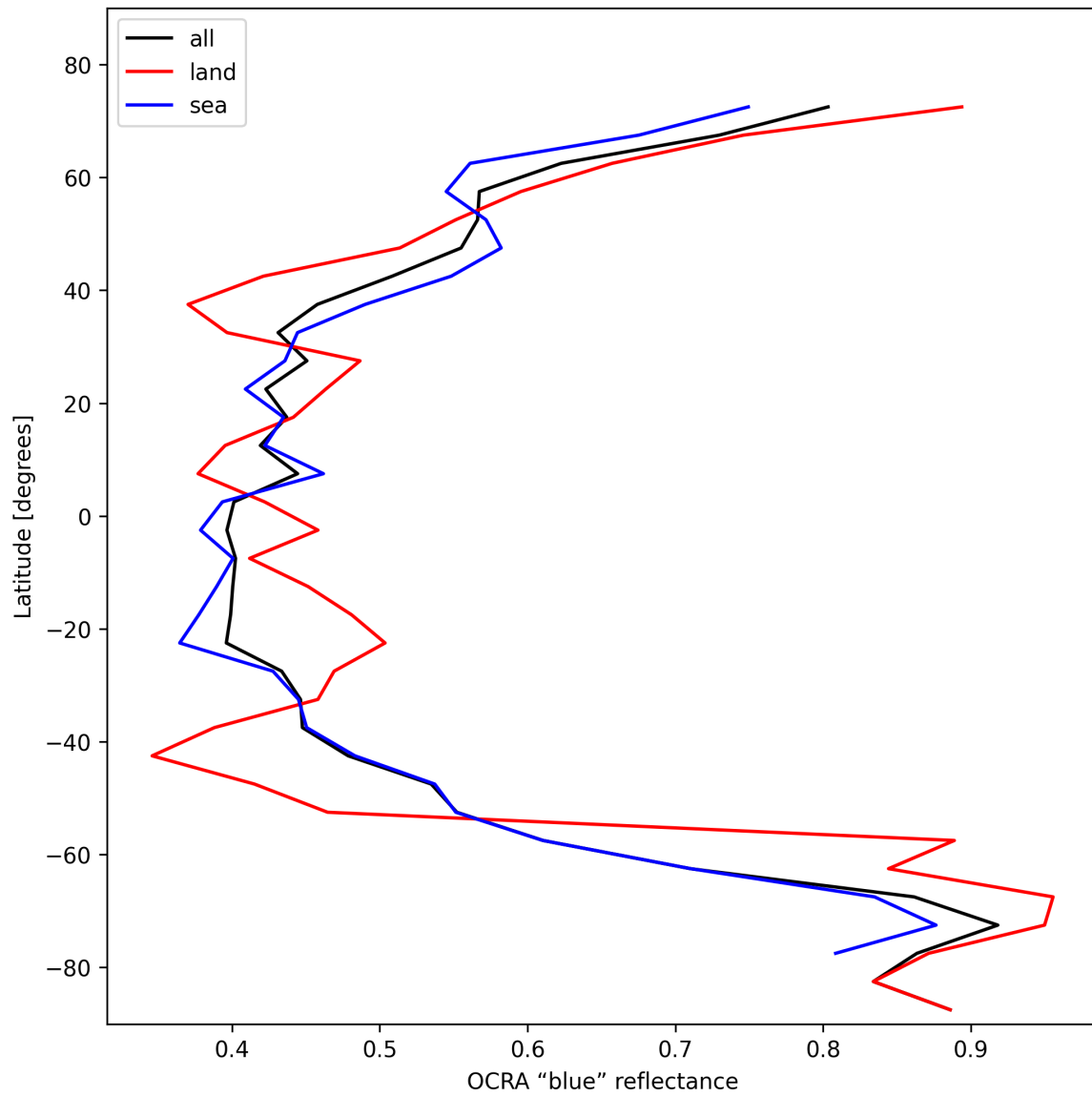
Figure 35: Zonal average of “OCRA “blue” reflectance” for 2025-11-02 to 2025-11-03.
