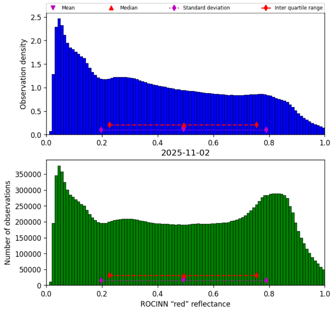
Figure 53: Histogram of “ROCINN “red” reflectance” for 2025-11-02 to 2025-11-03
