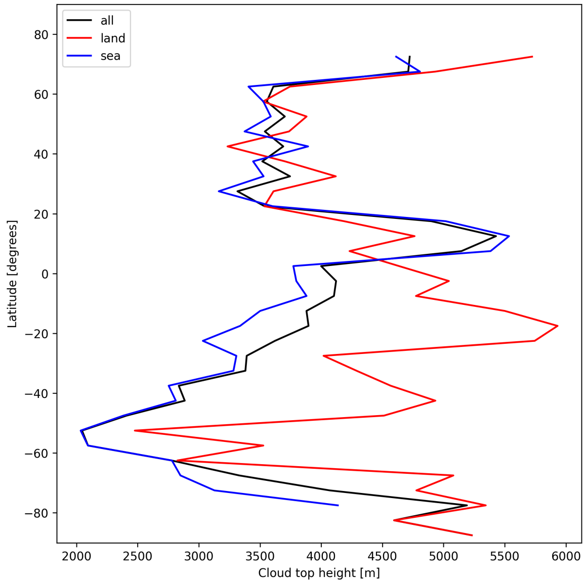
Figure 24: Zonal average of “Cloud top height” for 2025-11-02 to 2025-11-03.
