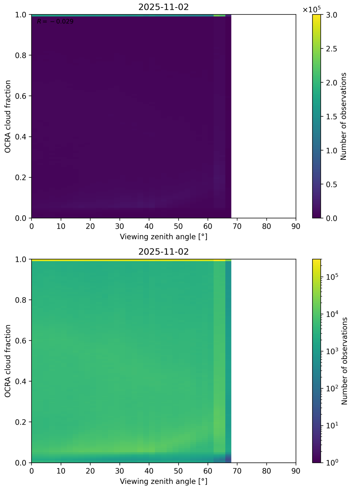
Figure 108: Scatter density plot of “Viewing zenith angle” against “OCRA cloud fraction” for 2025-11-02 to 2025-11-03.
