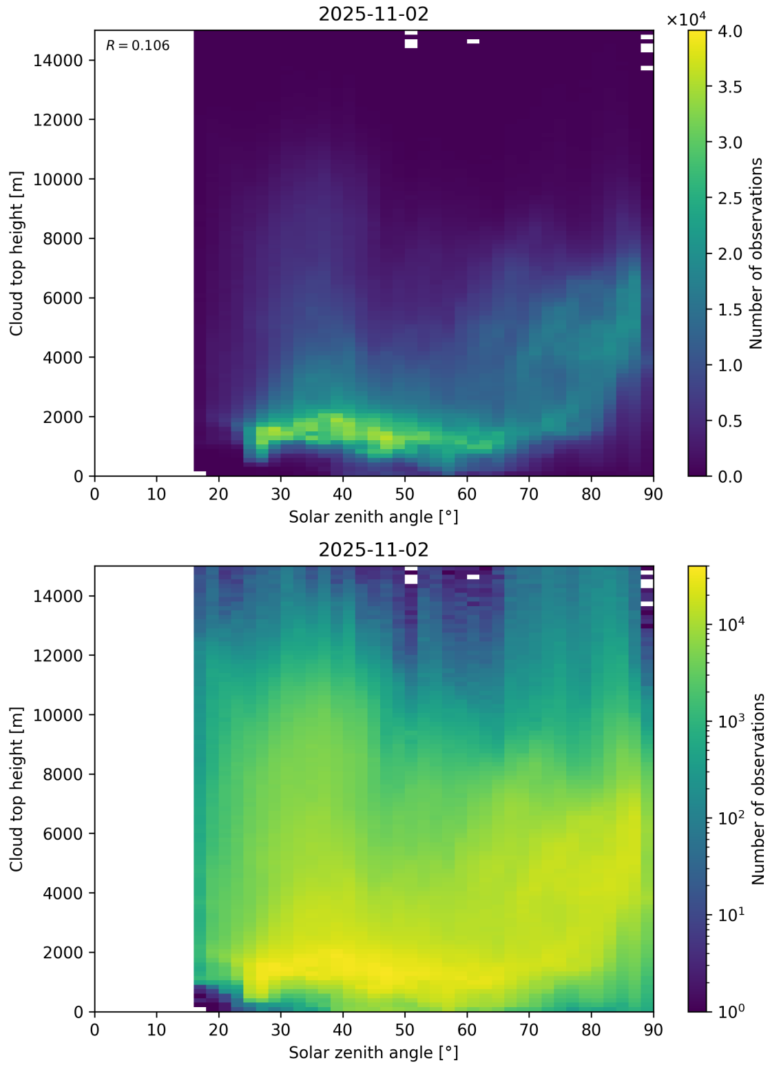
Figure 104: Scatter density plot of “Solar zenith angle” against “Cloud top height” for 2025-11-02 to 2025-11-03.
