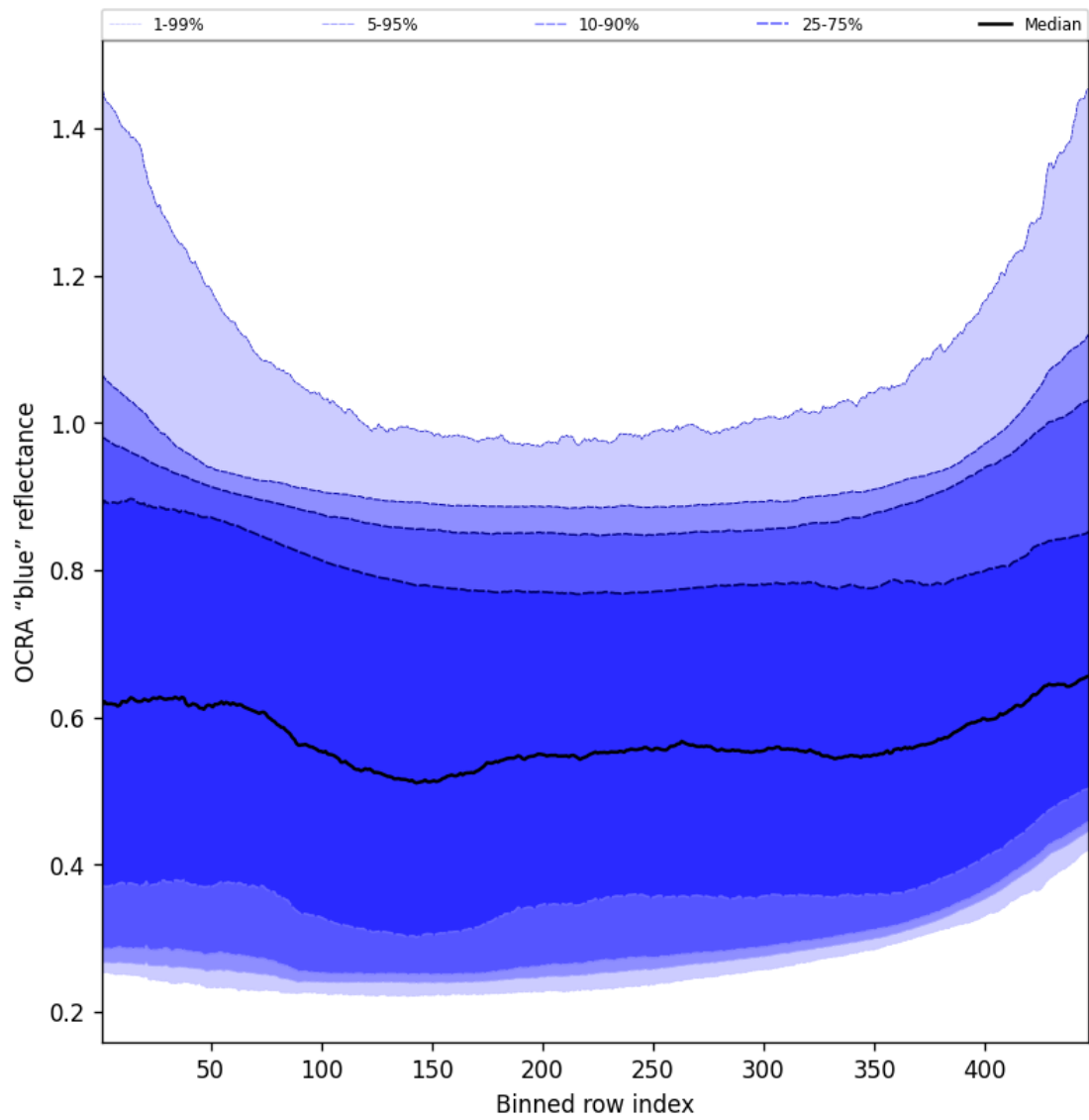
Figure 67: Along track statistics of “OCRA “blue” reflectance” for 2025-11-02 to 2025-11-03
