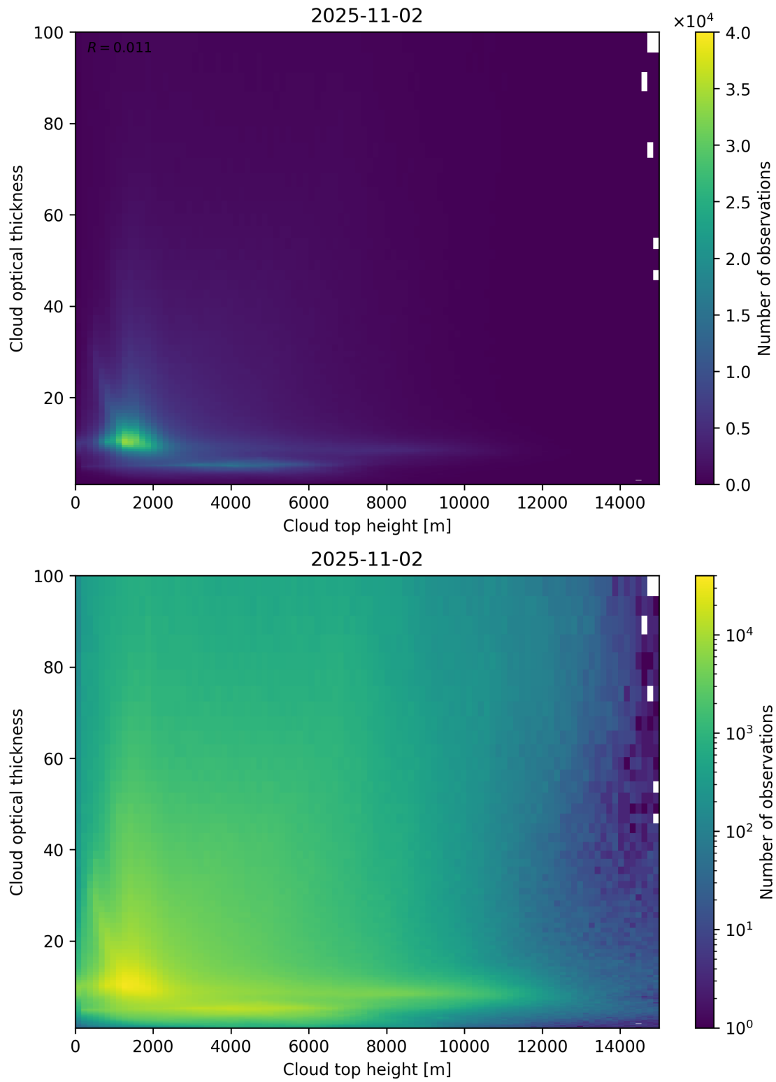
Figure 90: Scatter density plot of “Cloud top height” against “Cloud optical thickness” for 2025-11-02 to 2025-11-03.
