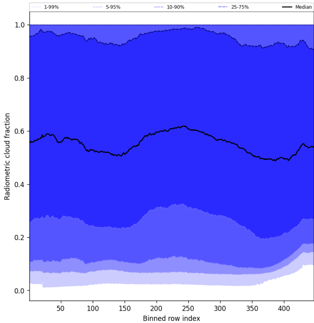
Figure 55: Along track statistics of “Radiometric cloud fraction” for 2025-11-02 to 2025-11-03
