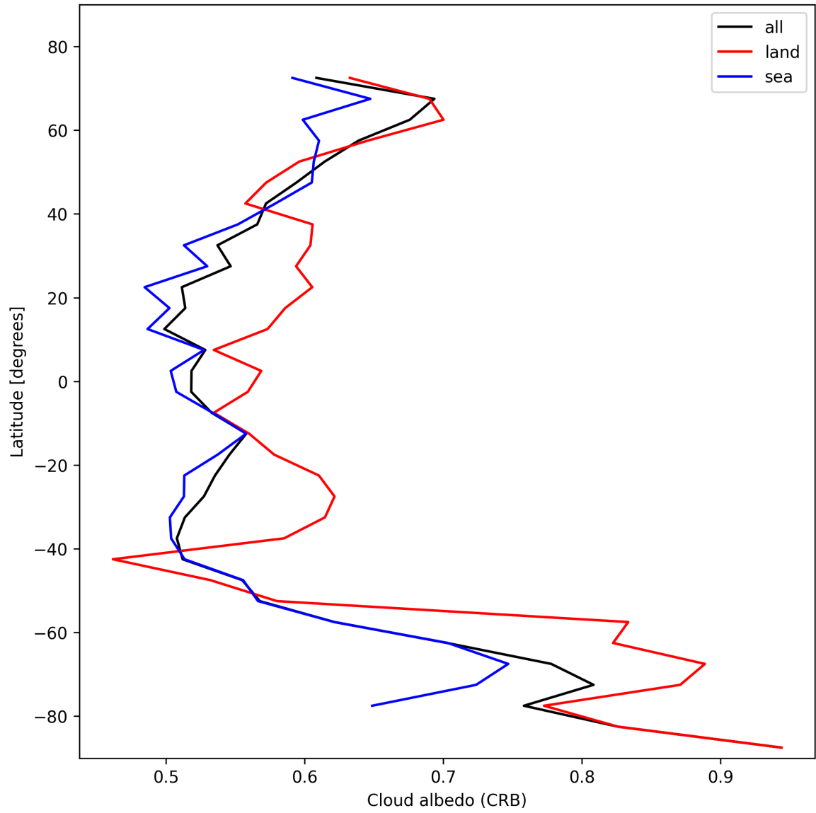
Figure 28: Zonal average of “Cloud albedo (CRB)” for 2025-11-02 to 2025-11-03.
