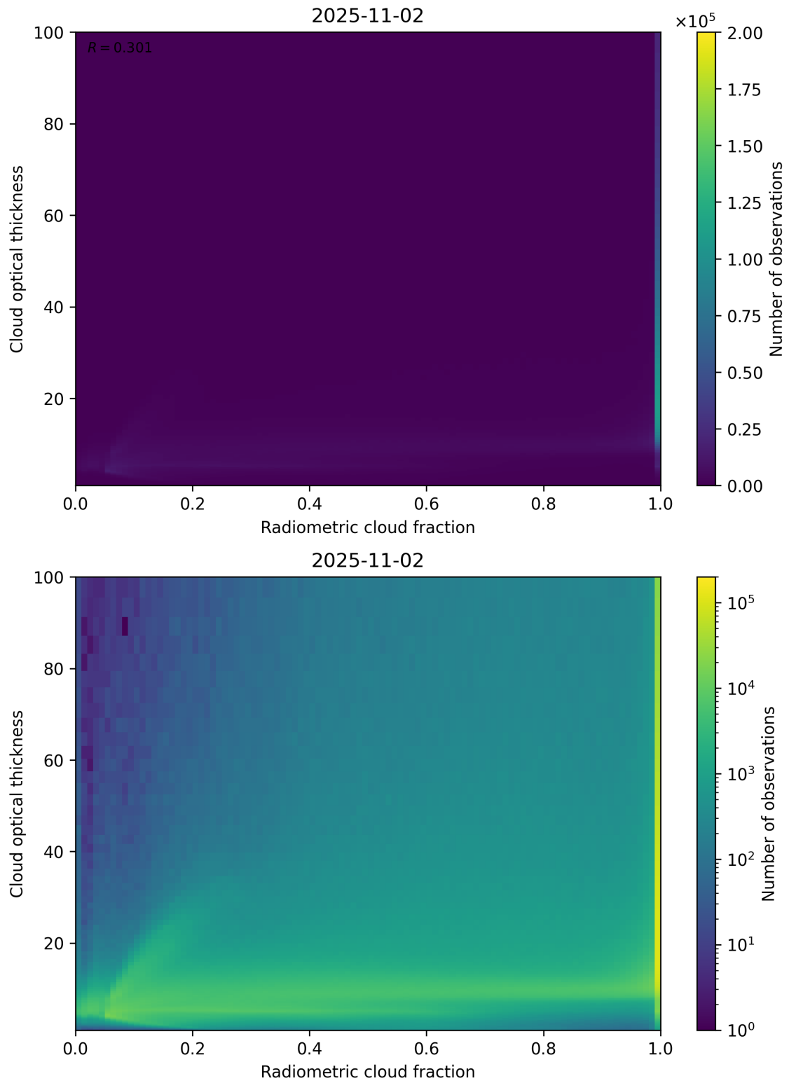
Figure 75: Scatter density plot of “Radiometric cloud fraction” against “Cloud optical thickness” for 2025-11-02 to 2025-11-03.
