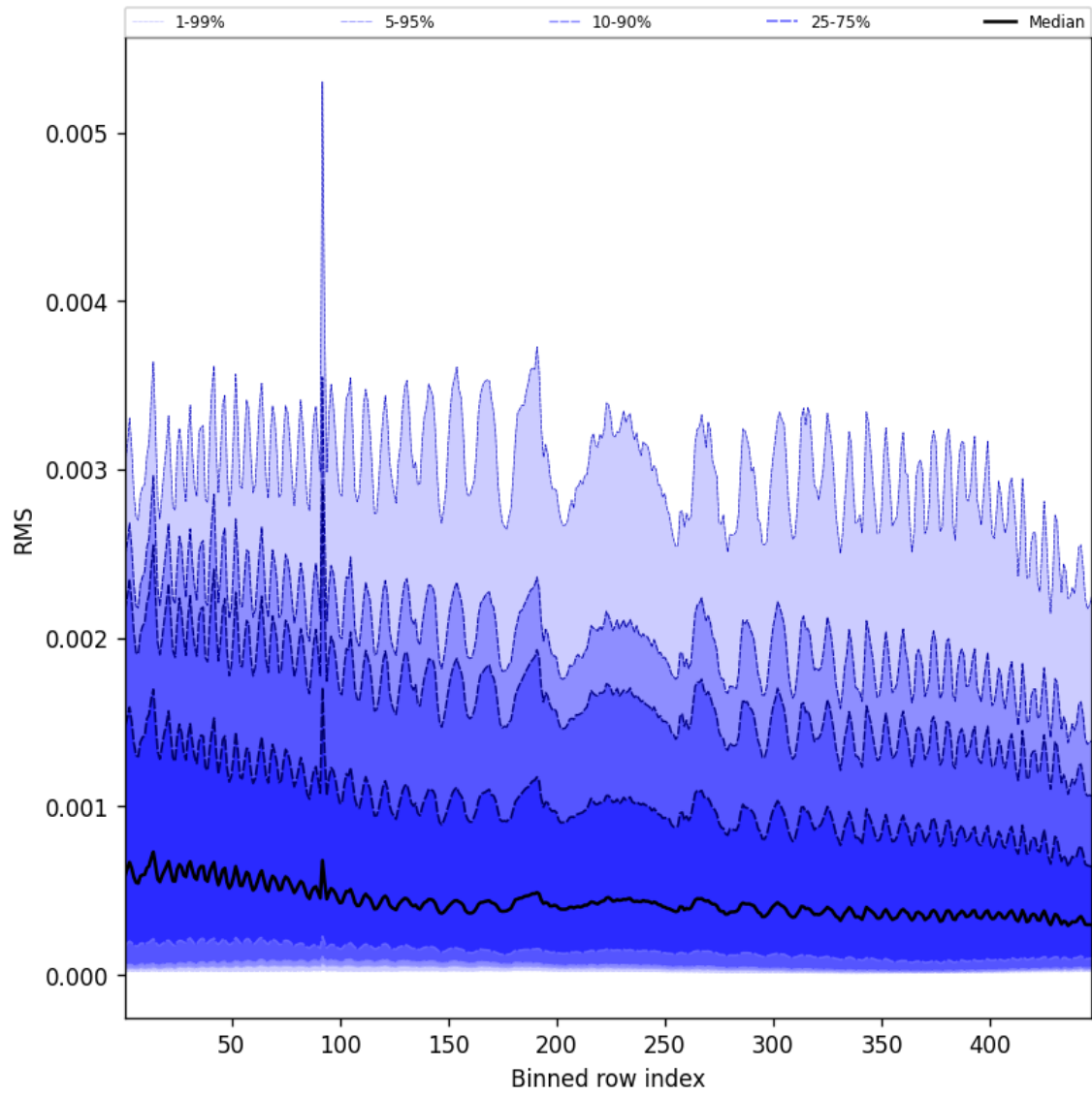
Figure 63: Along track statistics of “RMS” for 2025-11-02 to 2025-11-03
