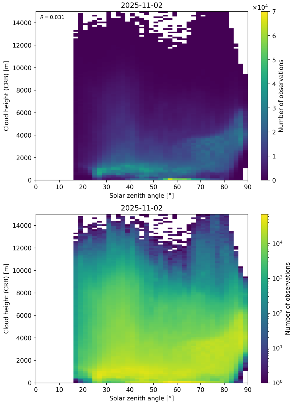
Figure 102: Scatter density plot of “Solar zenith angle” against “Cloud height (CRB)” for 2025-11-02 to 2025-11-03.
