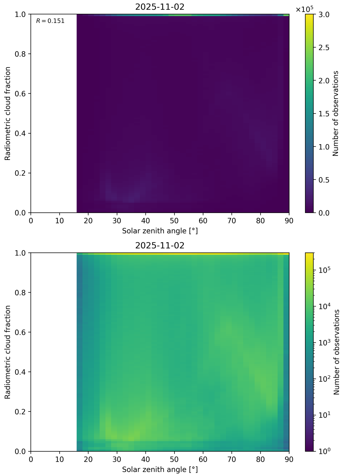
Figure 99: Scatter density plot of “Solar zenith angle” against “Radiometric cloud fraction” for 2025-11-02 to 2025-11-03.
