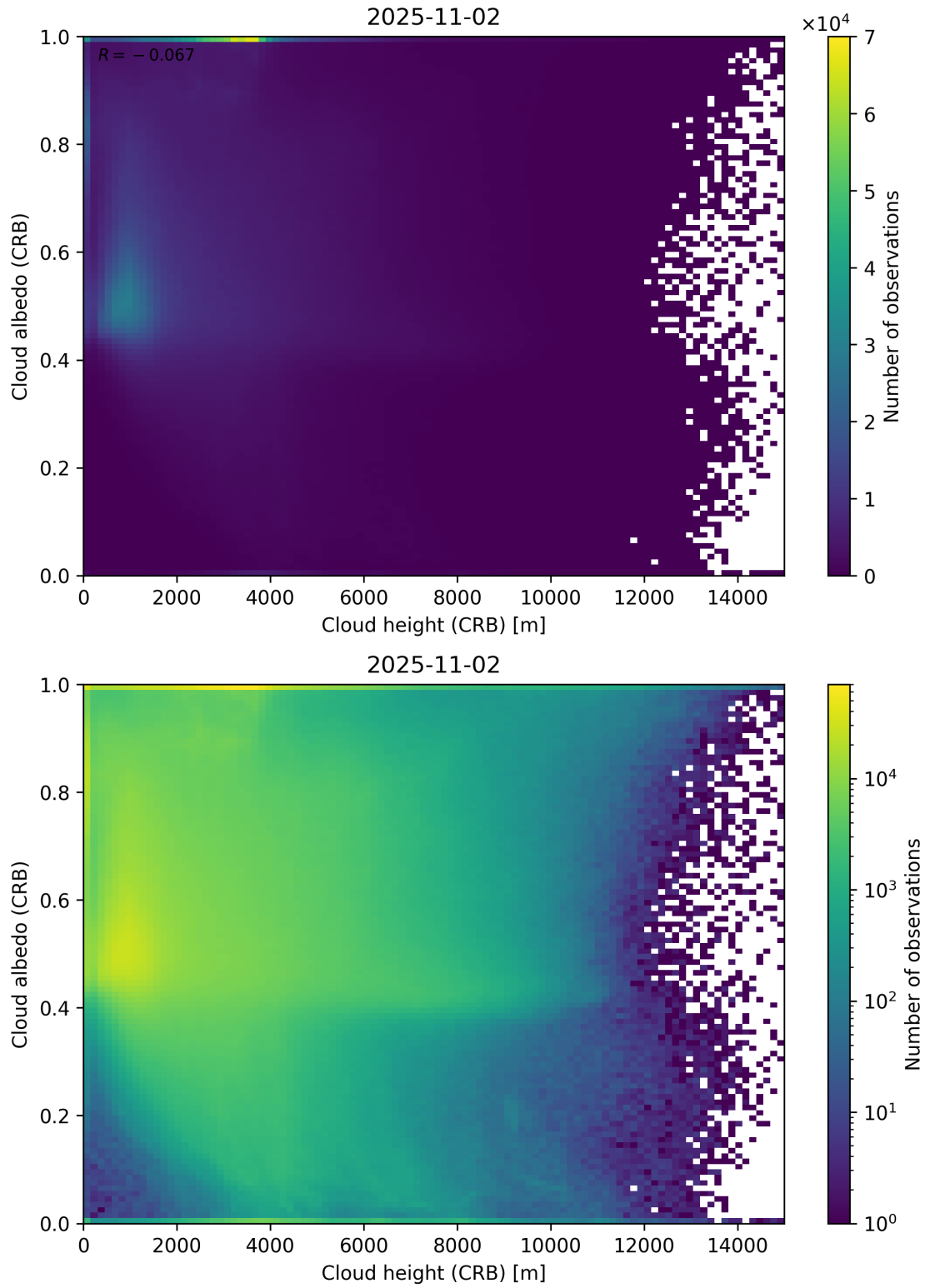
Figure 80: Scatter density plot of “Cloud height (CRB)” against “Cloud albedo (CRB)” for 2025-11-02 to 2025-11-03.
