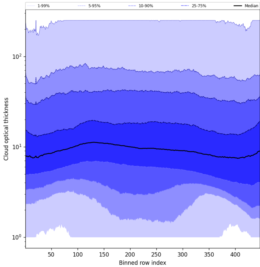
Figure 57: Along track statistics of “Cloud optical thickness” for 2025-11-02 to 2025-11-03
