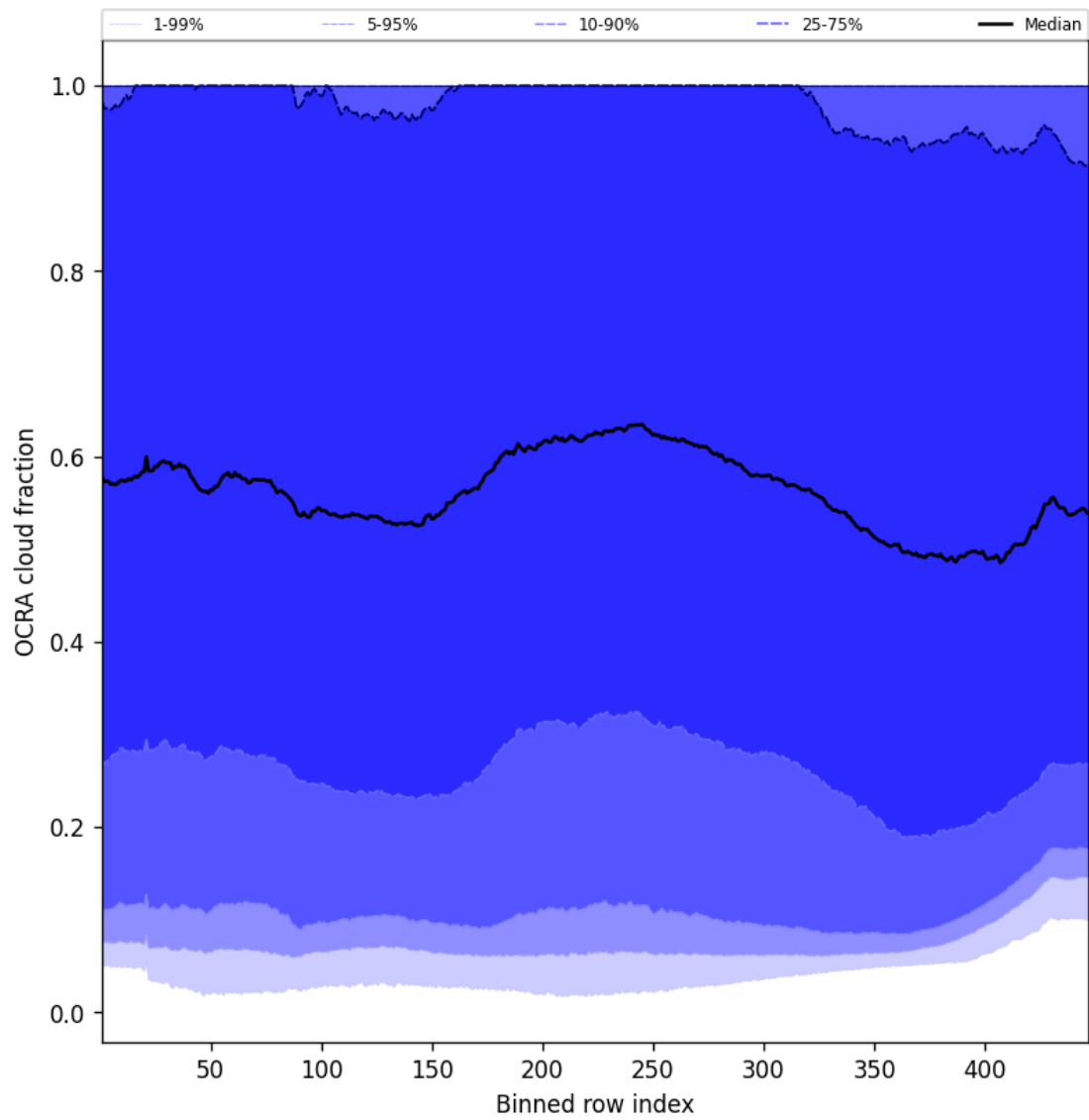
Figure 66: Along track statistics of “OCRA cloud fraction” for 2025-11-02 to 2025-11-03
