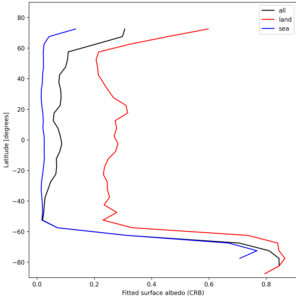
Figure 30: Zonal average of “Fitted surface albedo (CRB)” for 2025-11-02 to 2025-11-03.
