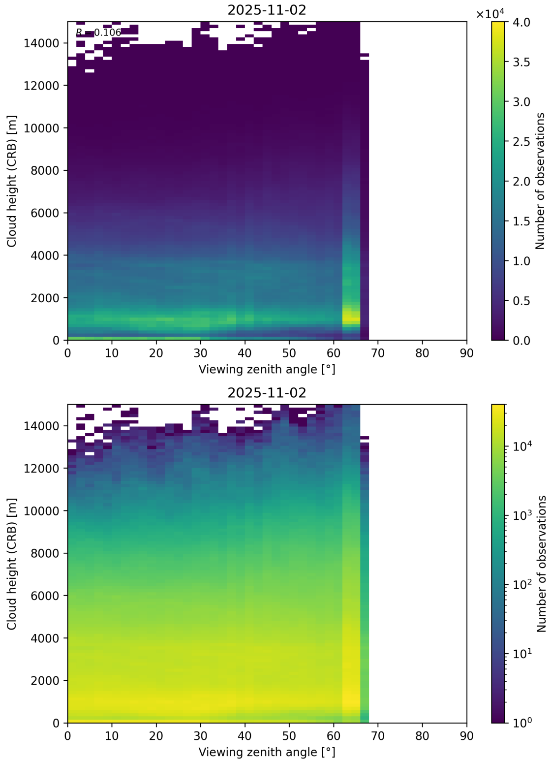
Figure 110: Scatter density plot of “Viewing zenith angle” against “Cloud height (CRB)” for 2025-11-02 to 2025-11-03.
