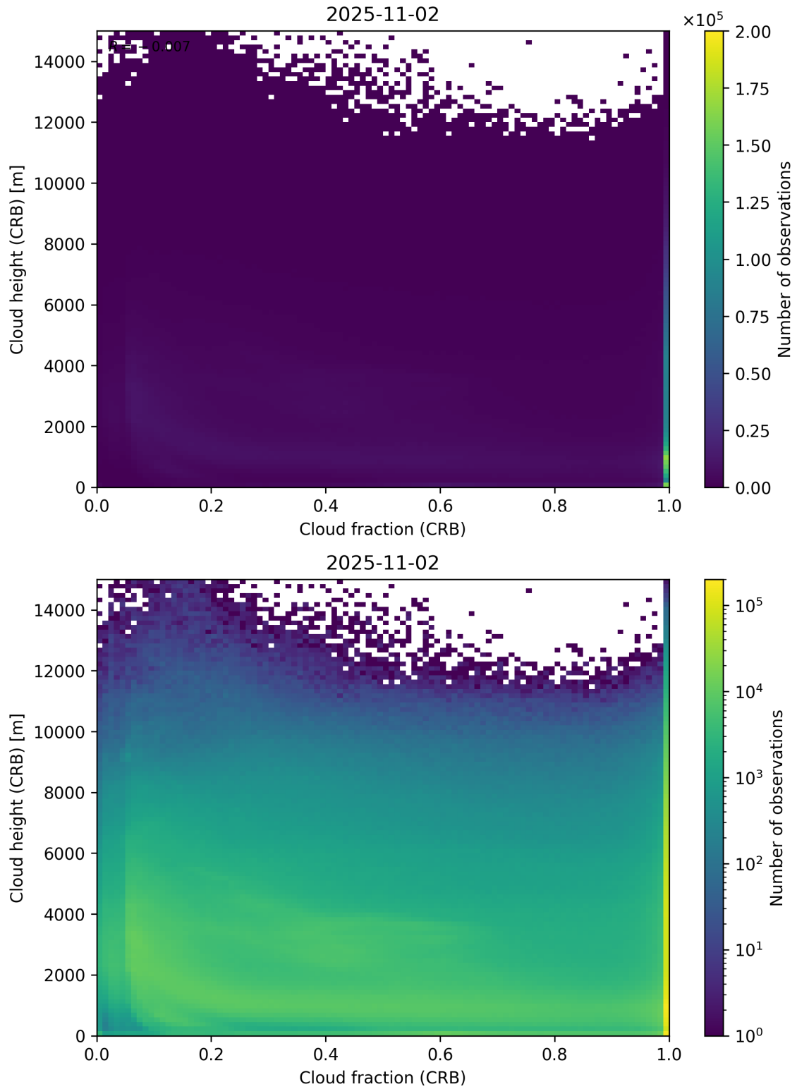
Figure 79: Scatter density plot of “Cloud fraction (CRB)” against “Cloud height (CRB)” for 2025-11-02 to 2025-11-03.
