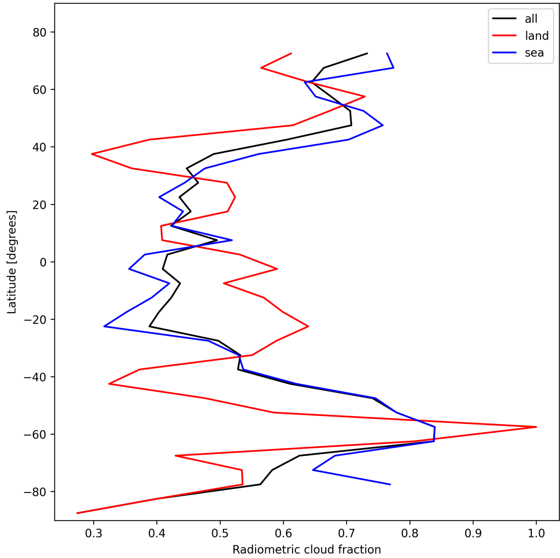
Figure 23: Zonal average of “Radiometric cloud fraction” for 2025-11-02 to 2025-11-03.
