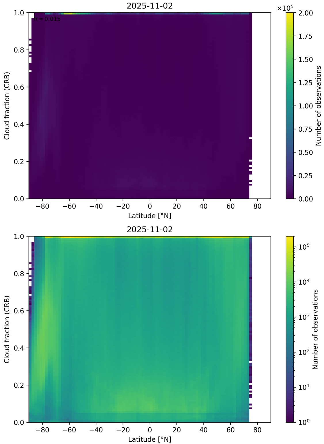
Figure 94: Scatter density plot of “Latitude” against “Cloud fraction (CRB)” for 2025-11-02 to 2025-11-03.
