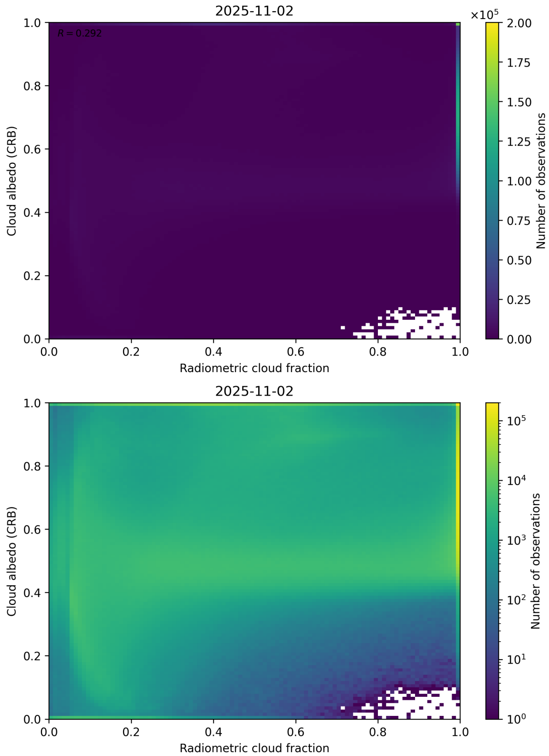
Figure 71: Scatter density plot of “Radiometric cloud fraction” against “Cloud albedo (CRB)” for 2025-11-02 to 2025-11-03.
