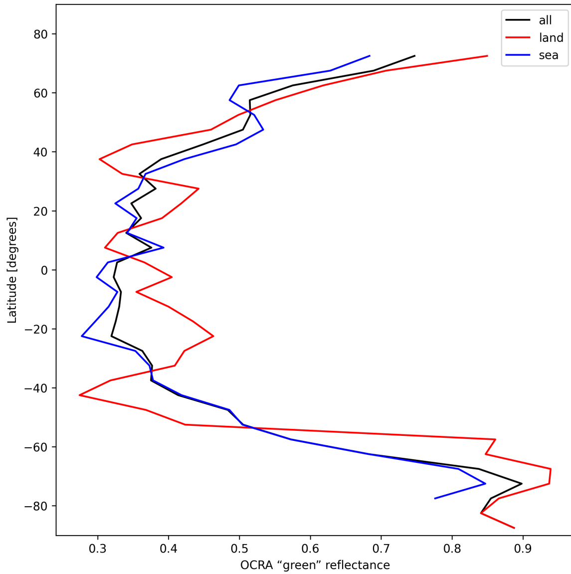
Figure 36: Zonal average of “OCRA “green” reflectance” for 2025-11-02 to 2025-11-03.
