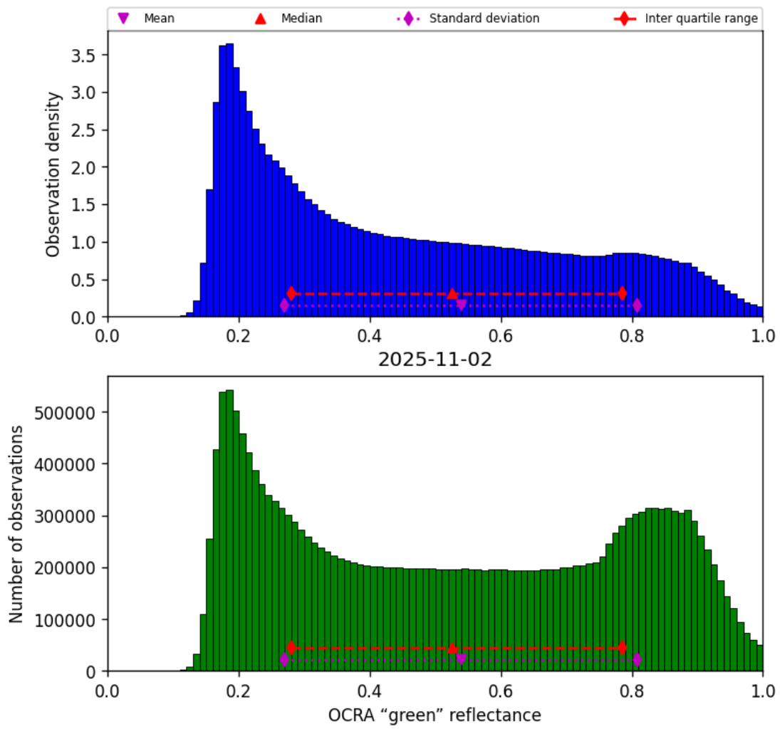
Figure 52: Histogram of “OCRA “green” reflectance” for 2025-11-02 to 2025-11-03
