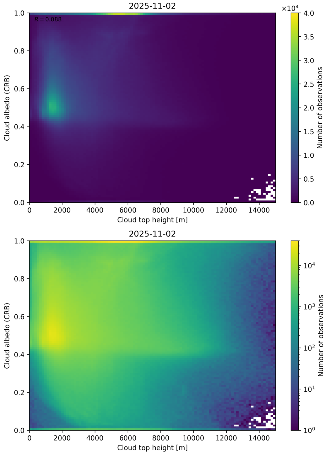
Figure 86: Scatter density plot of “Cloud top height” against “Cloud albedo (CRB)” for 2025-11-02 to 2025-11-03.
