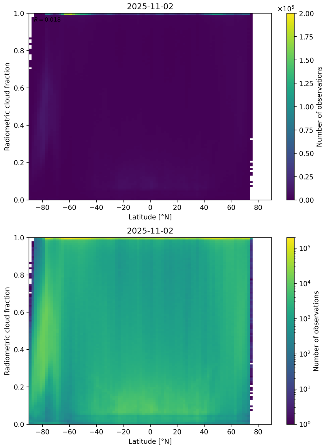
Figure 92: Scatter density plot of “Latitude” against “Radiometric cloud fraction” for 2025-11-02 to 2025-11-03.
