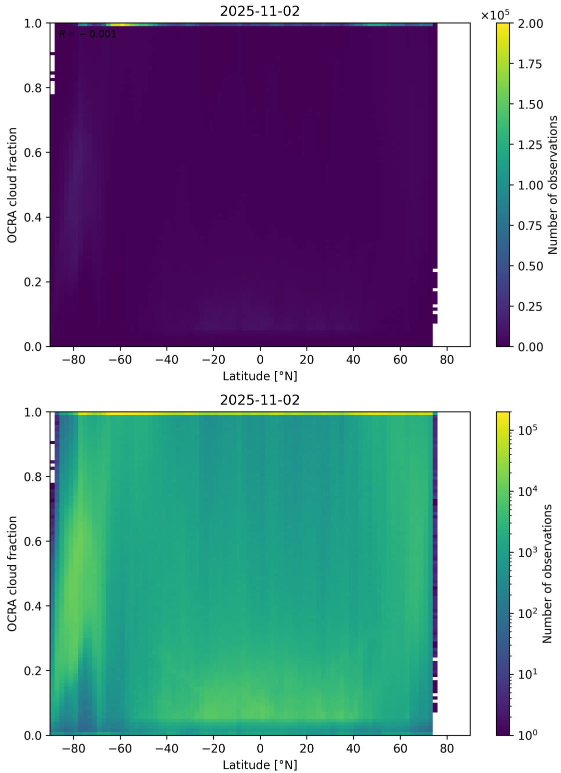
Figure 93: Scatter density plot of “Latitude” against “OCRA cloud fraction” for 2025-11-02 to 2025-11-03.
