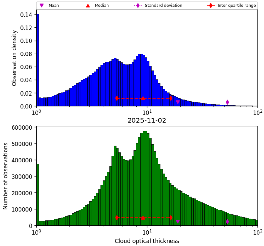
Figure 41: Histogram of “Cloud optical thickness” for 2025-11-02 to 2025-11-03
