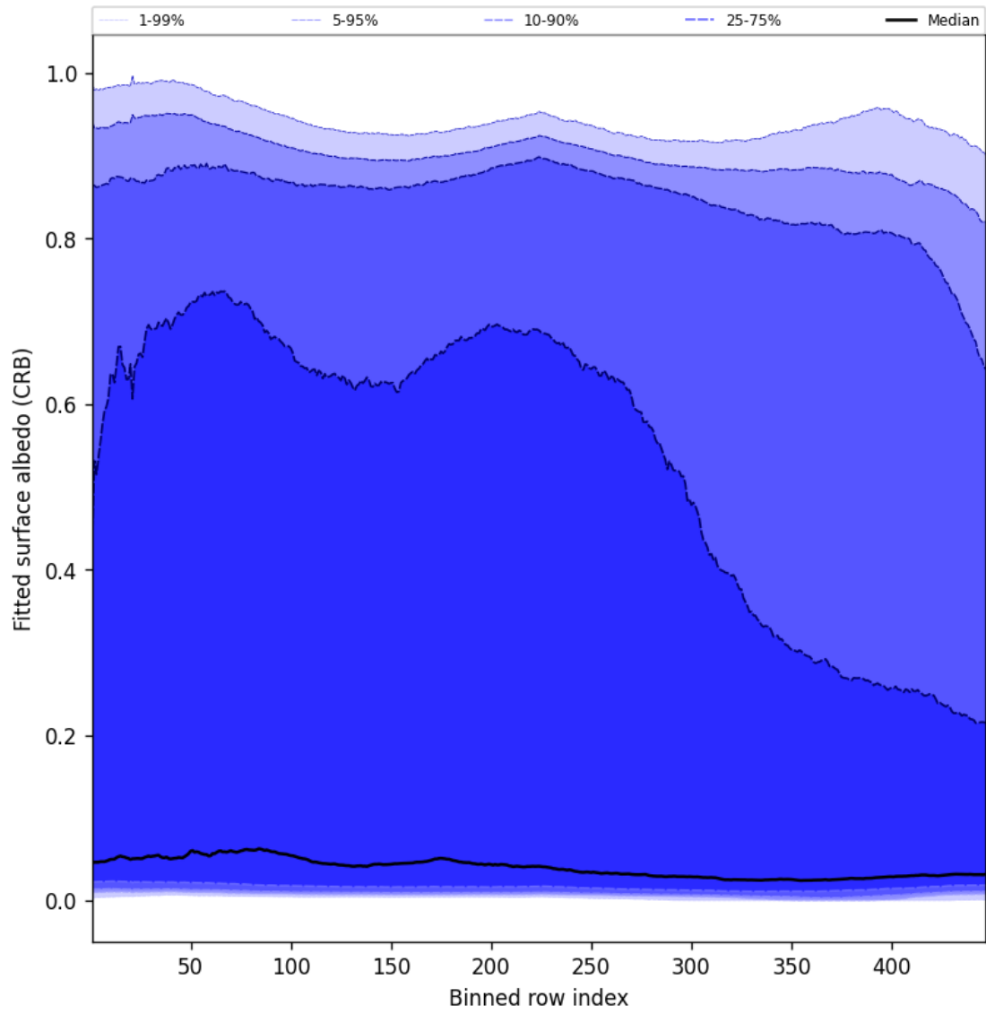
Figure 62: Along track statistics of “Fitted surface albedo (CRB)” for 2025-11-02 to 2025-11-03
