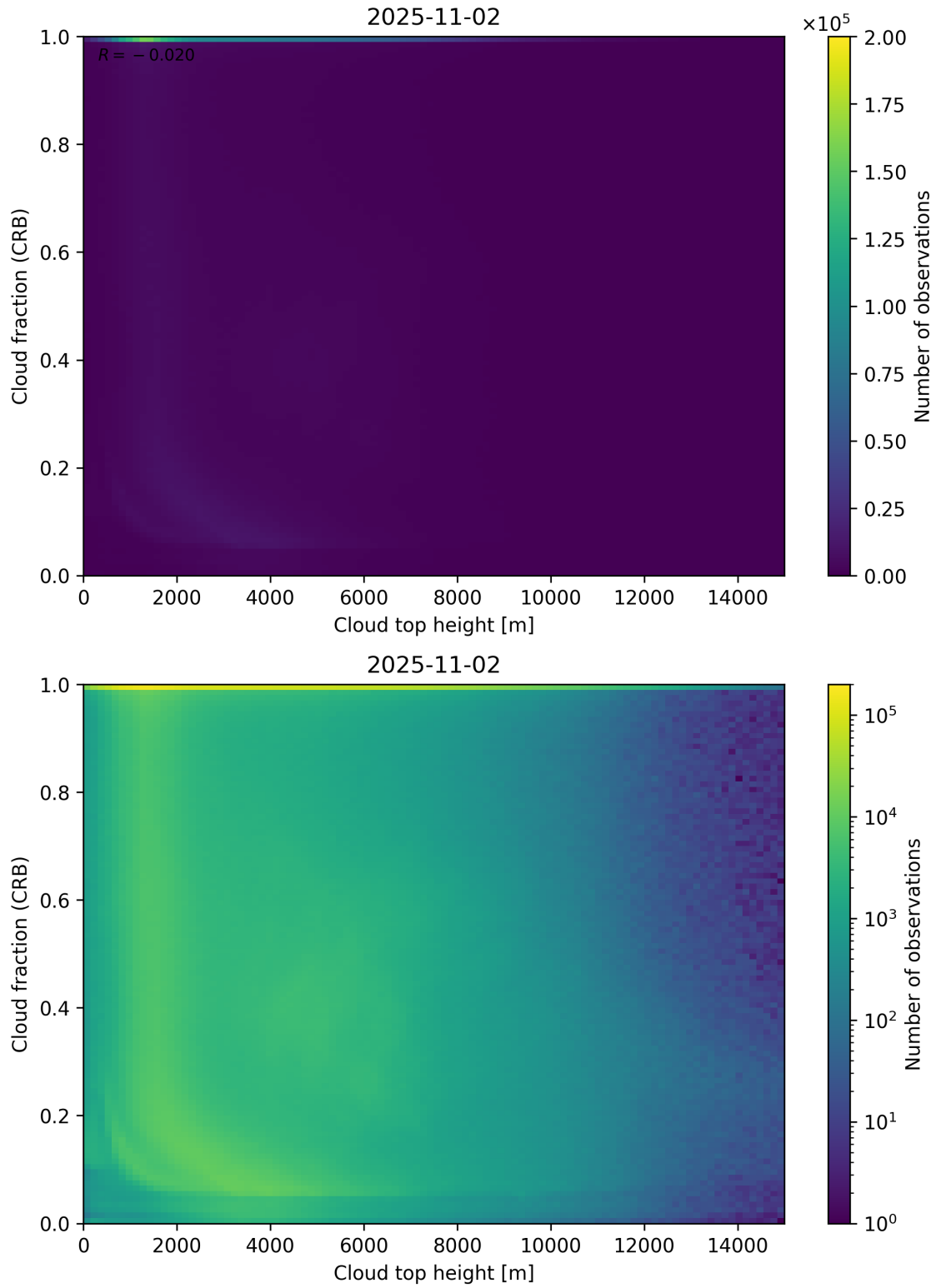
Figure 88: Scatter density plot of “Cloud top height” against “Cloud fraction (CRB)” for 2025-11-02 to 2025-11-03.
