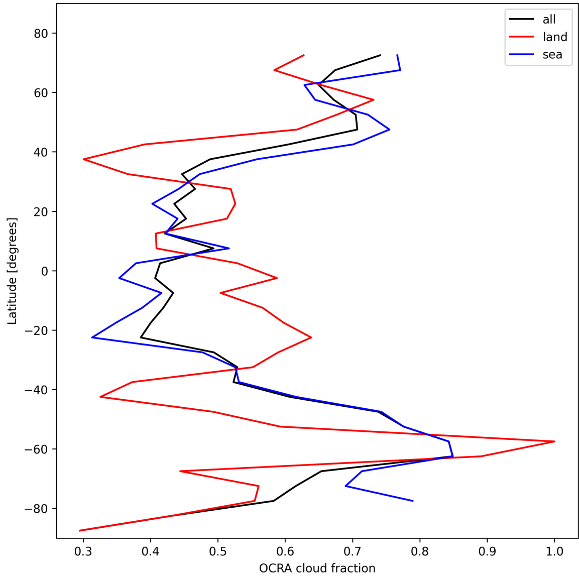
Figure 34: Zonal average of “OCRA cloud fraction” for 2025-11-02 to 2025-11-03.
