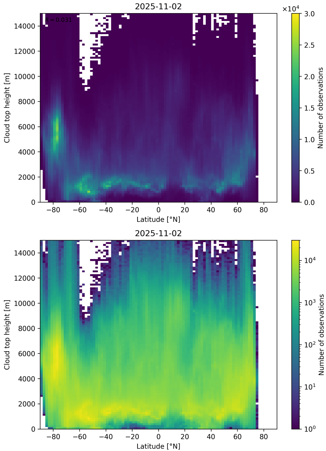
Figure 97: Scatter density plot of “Latitude” against “Cloud top height” for 2025-11-02 to 2025-11-03.
