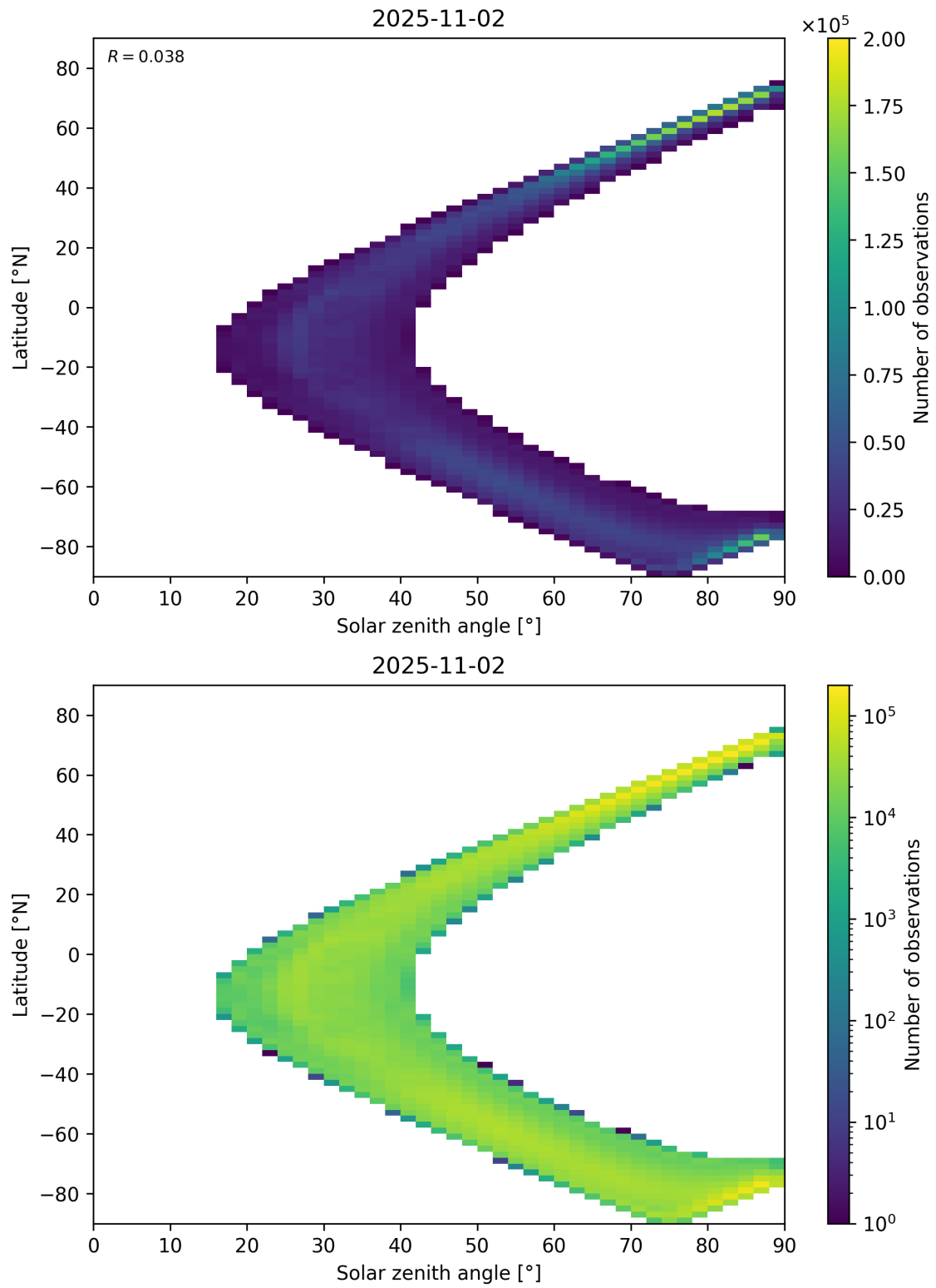
Figure 105: Scatter density plot of “Solar zenith angle” against “Latitude” for 2025-11-02 to 2025-11-03.
