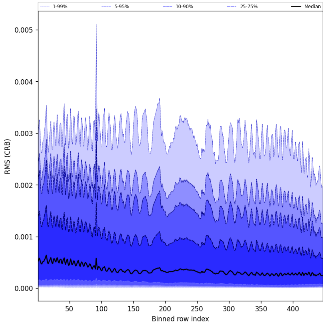
Figure 64: Along track statistics of “RMS (CRB)” for 2025-11-02 to 2025-11-03
