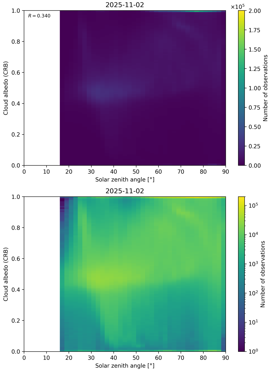
Figure 98: Scatter density plot of “Solar zenith angle” against “Cloud albedo (CRB)” for 2025-11-02 to 2025-11-03.
