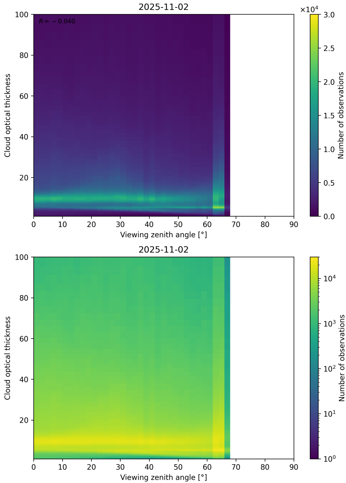
Figure 111: Scatter density plot of “Viewing zenith angle” against “Cloud optical thickness” for 2025-11-02 to 2025-11-03.
