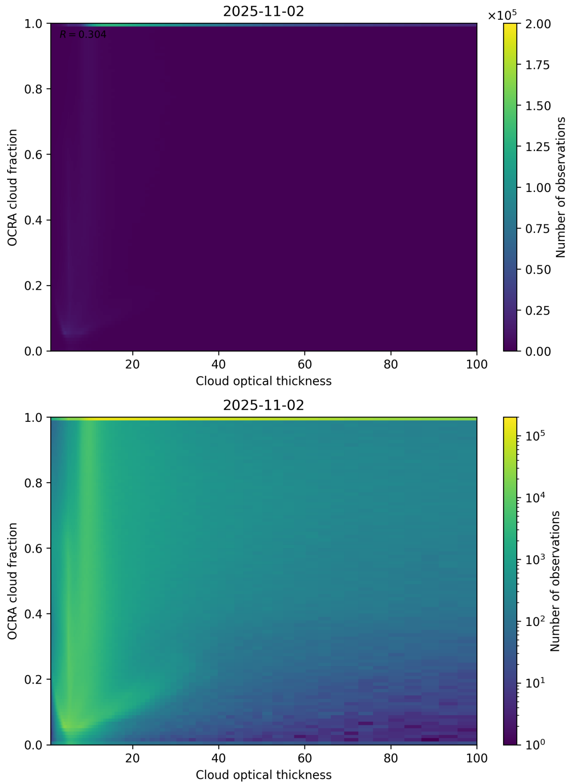
Figure 83: Scatter density plot of “Cloud optical thickness” against “OCRA cloud fraction” for 2025-11-02 to 2025-11-03.
