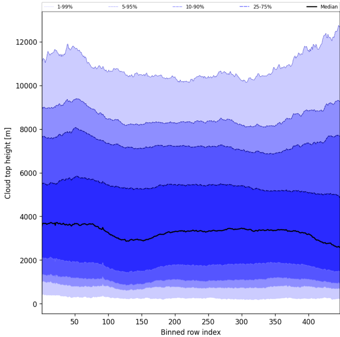
Figure 56: Along track statistics of “Cloud top height” for 2025-11-02 to 2025-11-03
