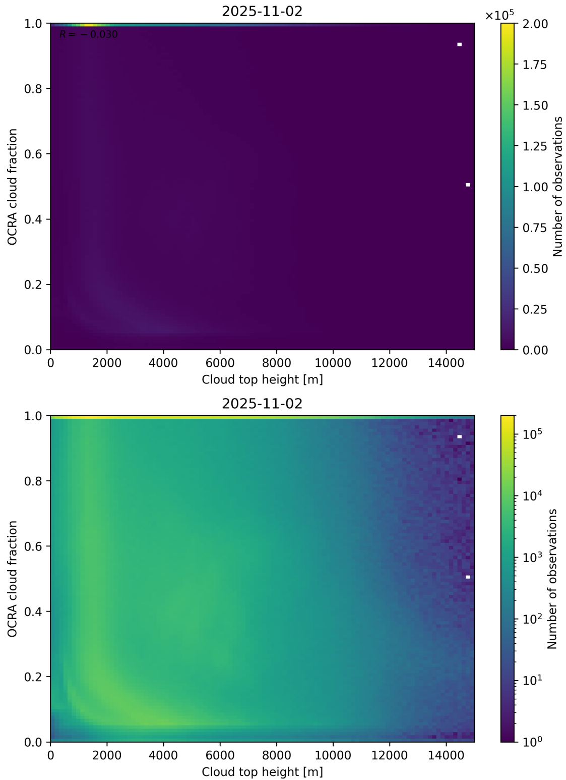
Figure 87: Scatter density plot of “Cloud top height” against “OCRA cloud fraction” for 2025-11-02 to 2025-11-03.
