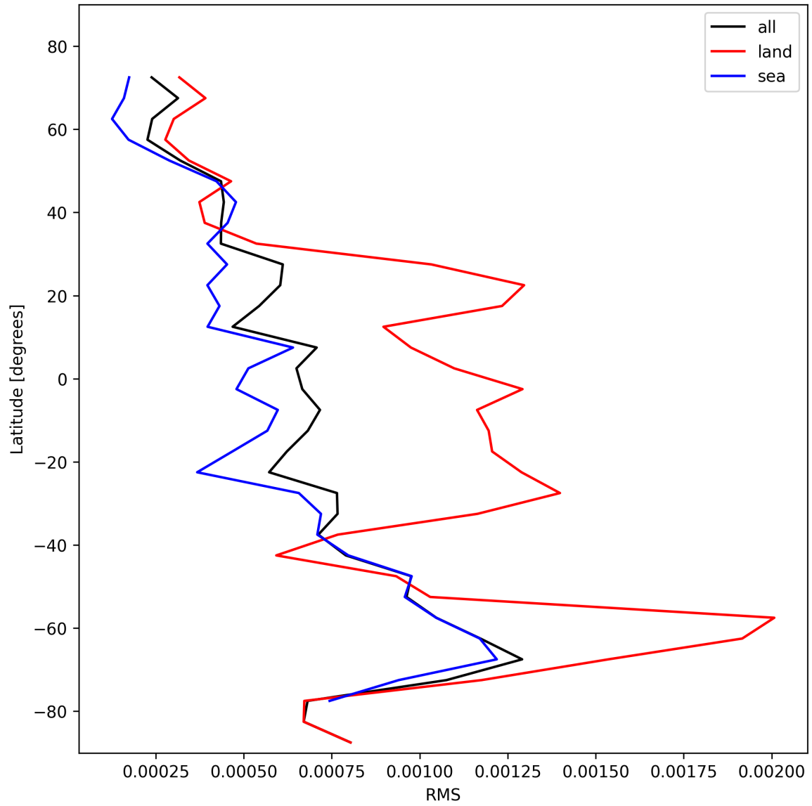
Figure 31: Zonal average of “RMS” for 2025-11-02 to 2025-11-03.
