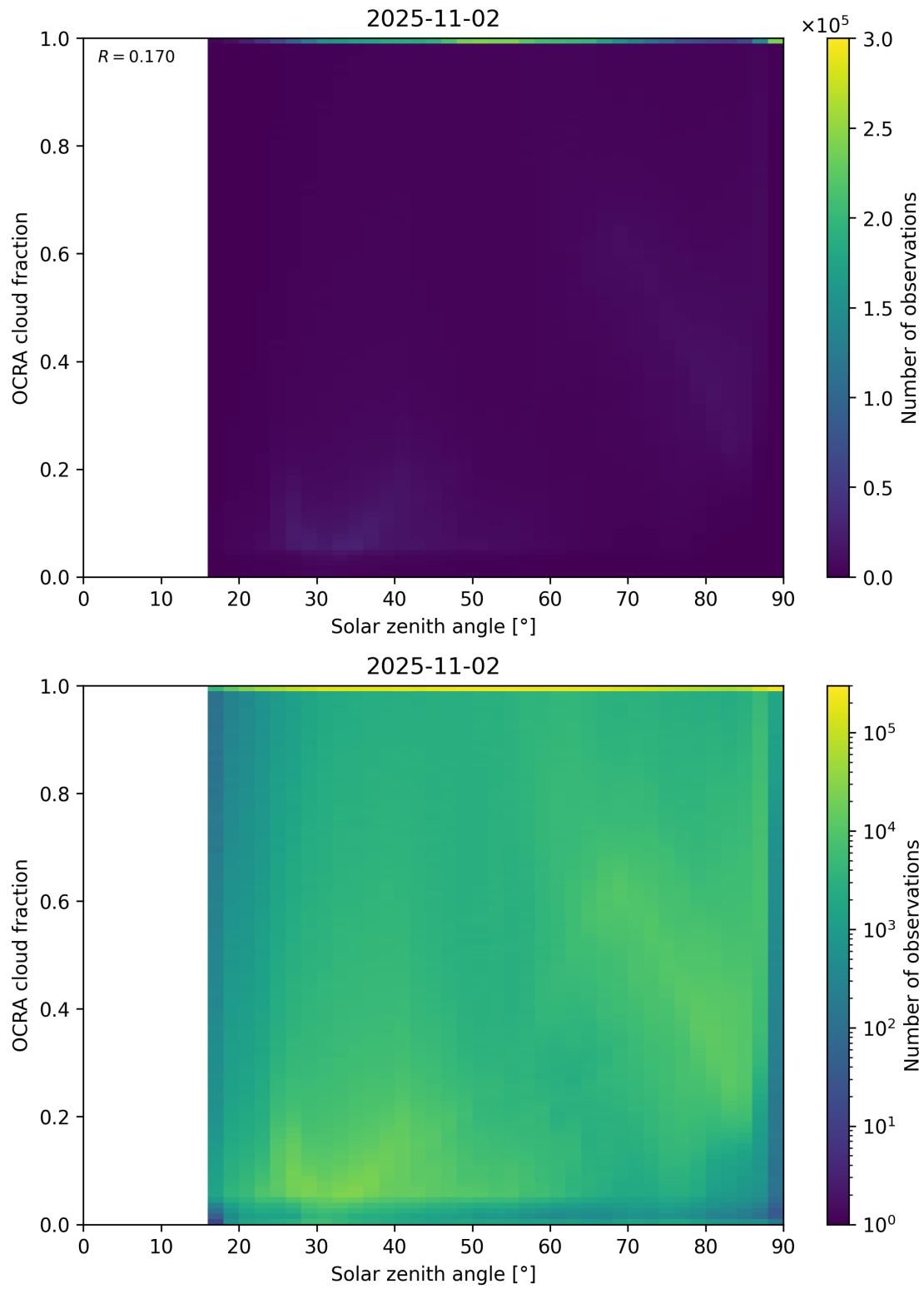
Figure 100: Scatter density plot of “Solar zenith angle” against “OCRA cloud fraction” for 2025-11-02 to 2025-11-03.
