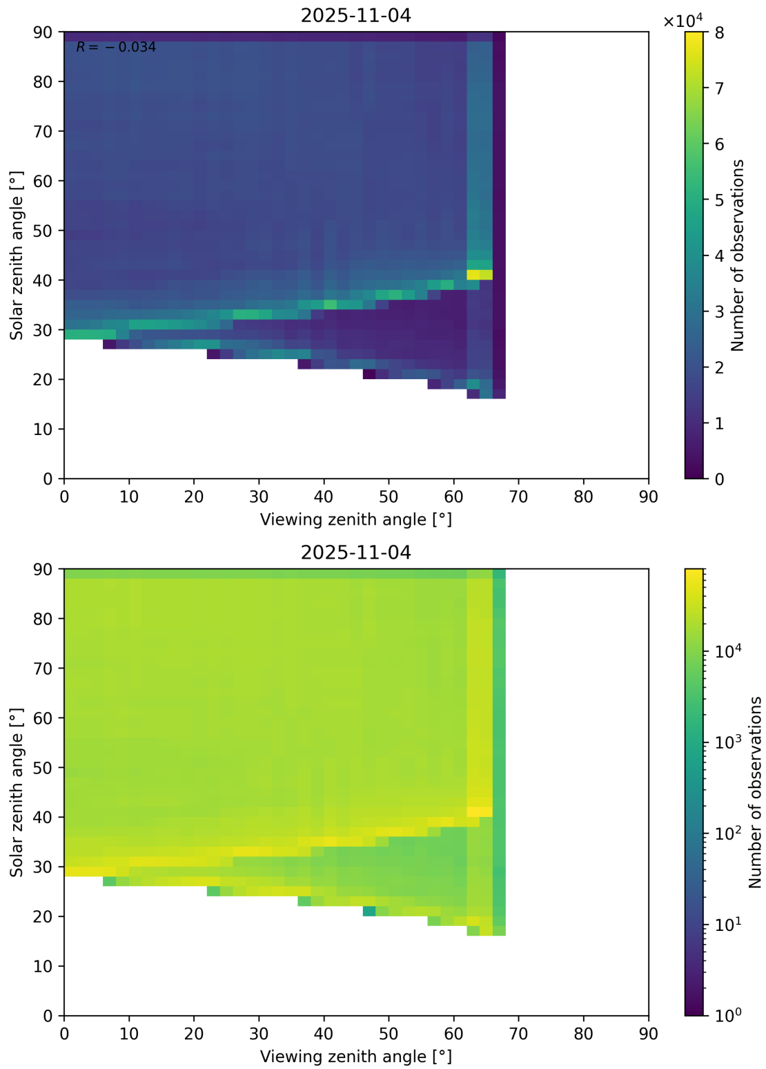
Figure 114: Scatter density plot of “Viewing zenith angle” against “Solar zenith angle” for 2025-11-03 to 2025-11-05.
