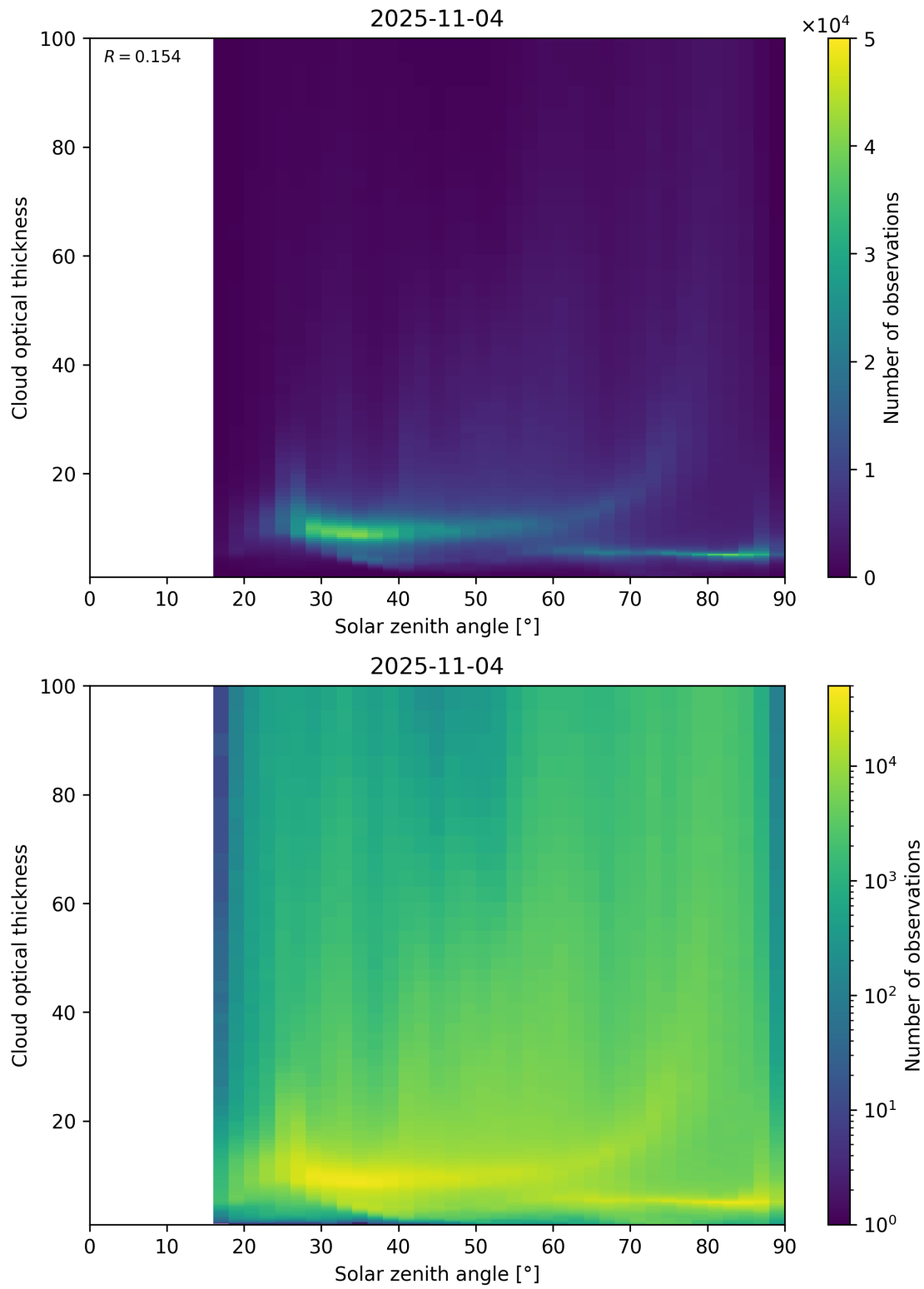
Figure 103: Scatter density plot of “Solar zenith angle” against “Cloud optical thickness” for 2025-11-03 to 2025-11-05.
