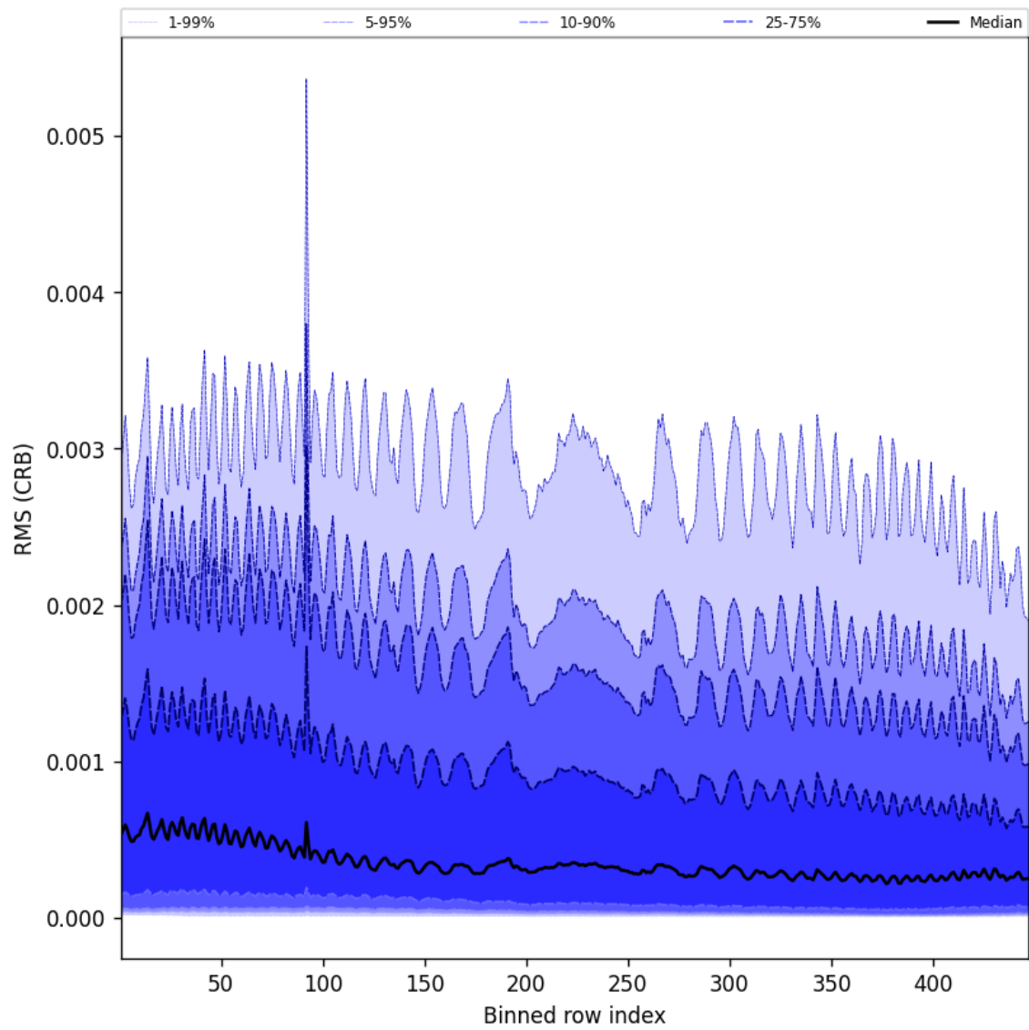
Figure 64: Along track statistics of “RMS (CRB)” for 2025-11-03 to 2025-11-05
