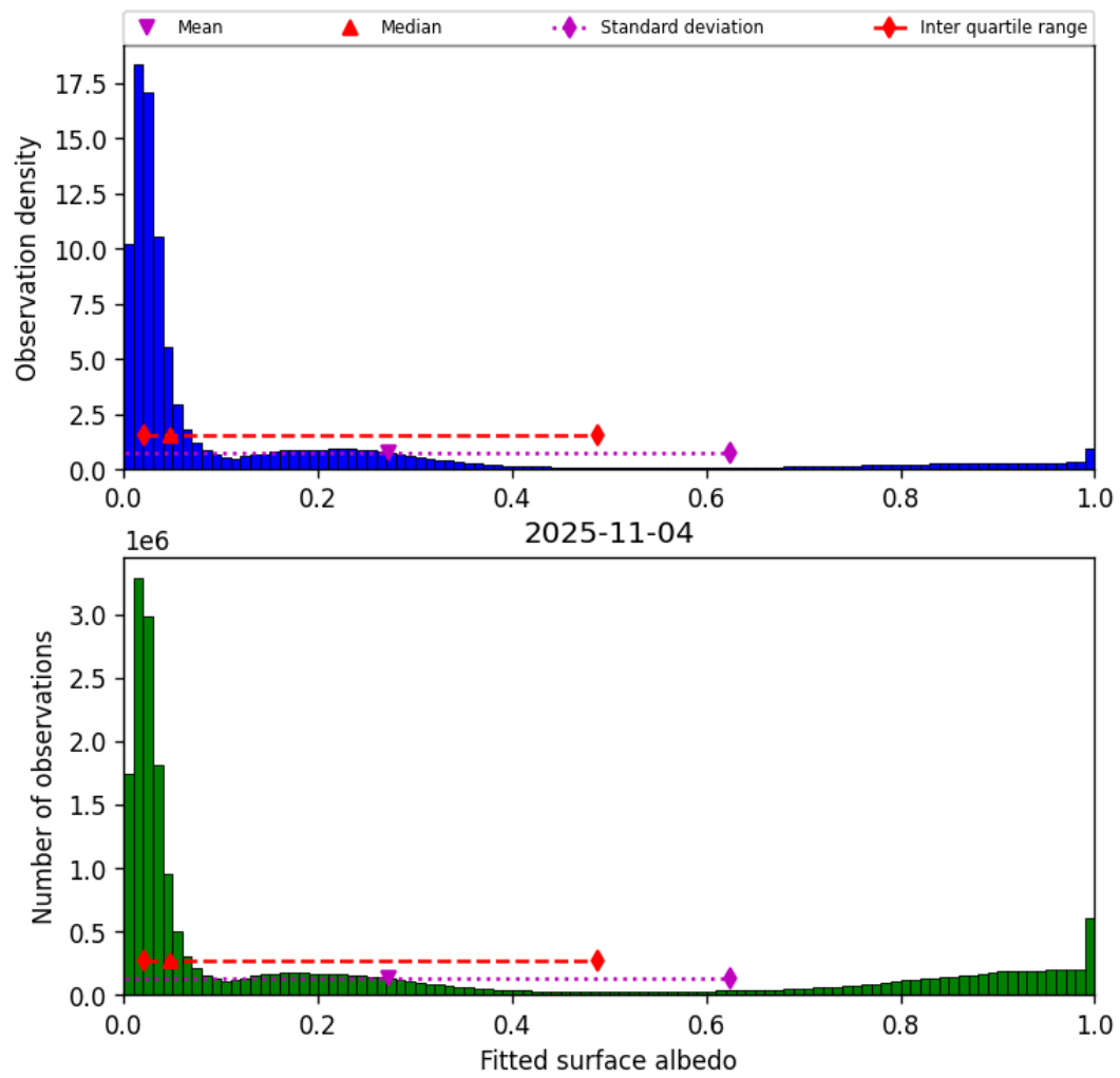
Figure 45: Histogram of “Fitted surface albedo” for 2025-11-03 to 2025-11-05
