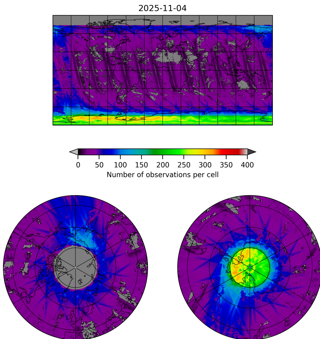
Figure 21: Map of the number of observations for 2025-11-03 to 2025-11-05
