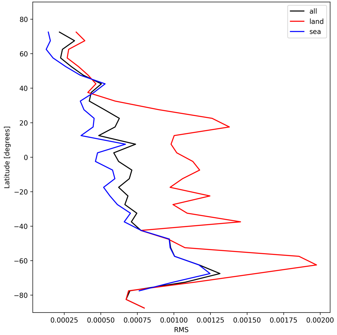
Figure 31: Zonal average of “RMS” for 2025-11-03 to 2025-11-05.
