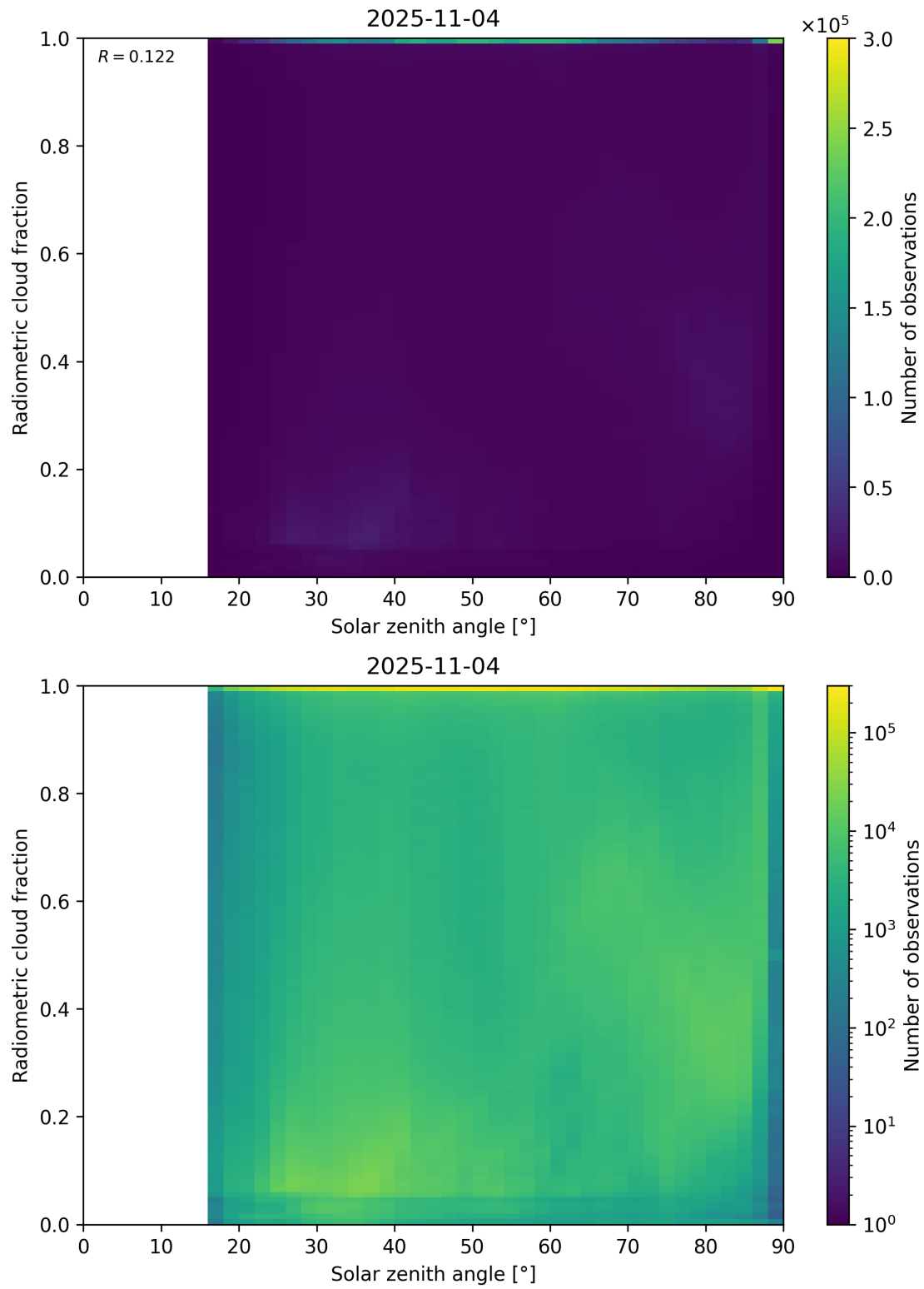
Figure 99: Scatter density plot of “Solar zenith angle” against “Radiometric cloud fraction” for 2025-11-03 to 2025-11-05.
