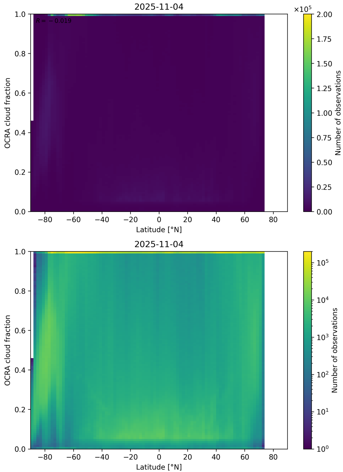
Figure 93: Scatter density plot of “Latitude” against “OCRA cloud fraction” for 2025-11-03 to 2025-11-05.
