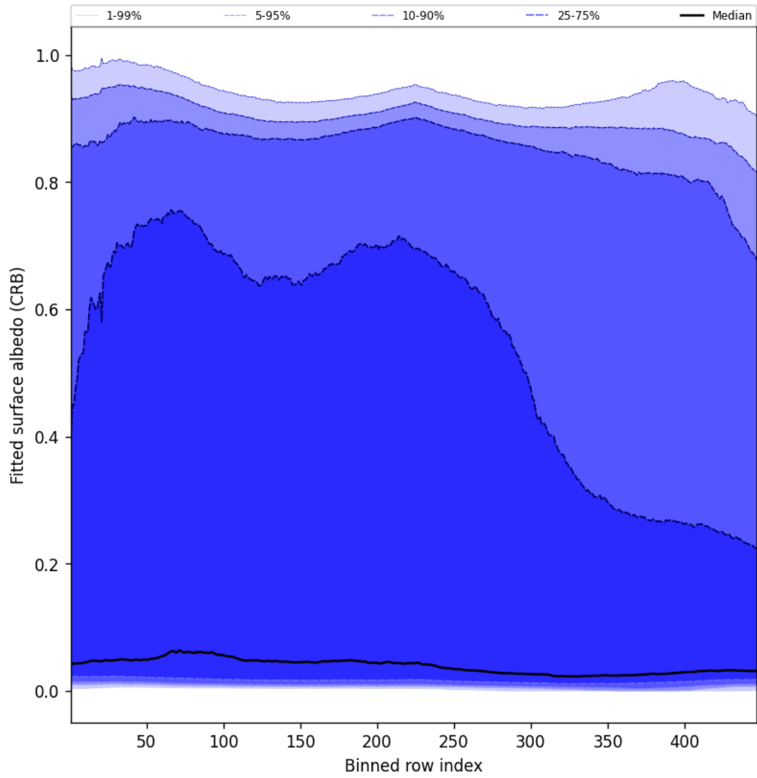
Figure 62: Along track statistics of “Fitted surface albedo (CRB)” for 2025-11-03 to 2025-11-05
