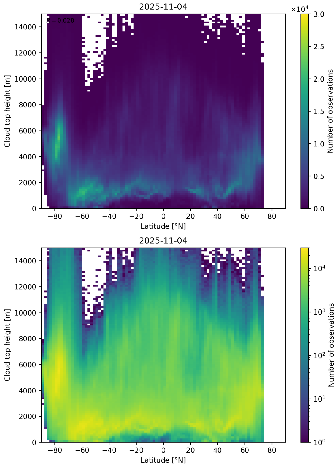
Figure 97: Scatter density plot of “Latitude” against “Cloud top height” for 2025-11-03 to 2025-11-05.
