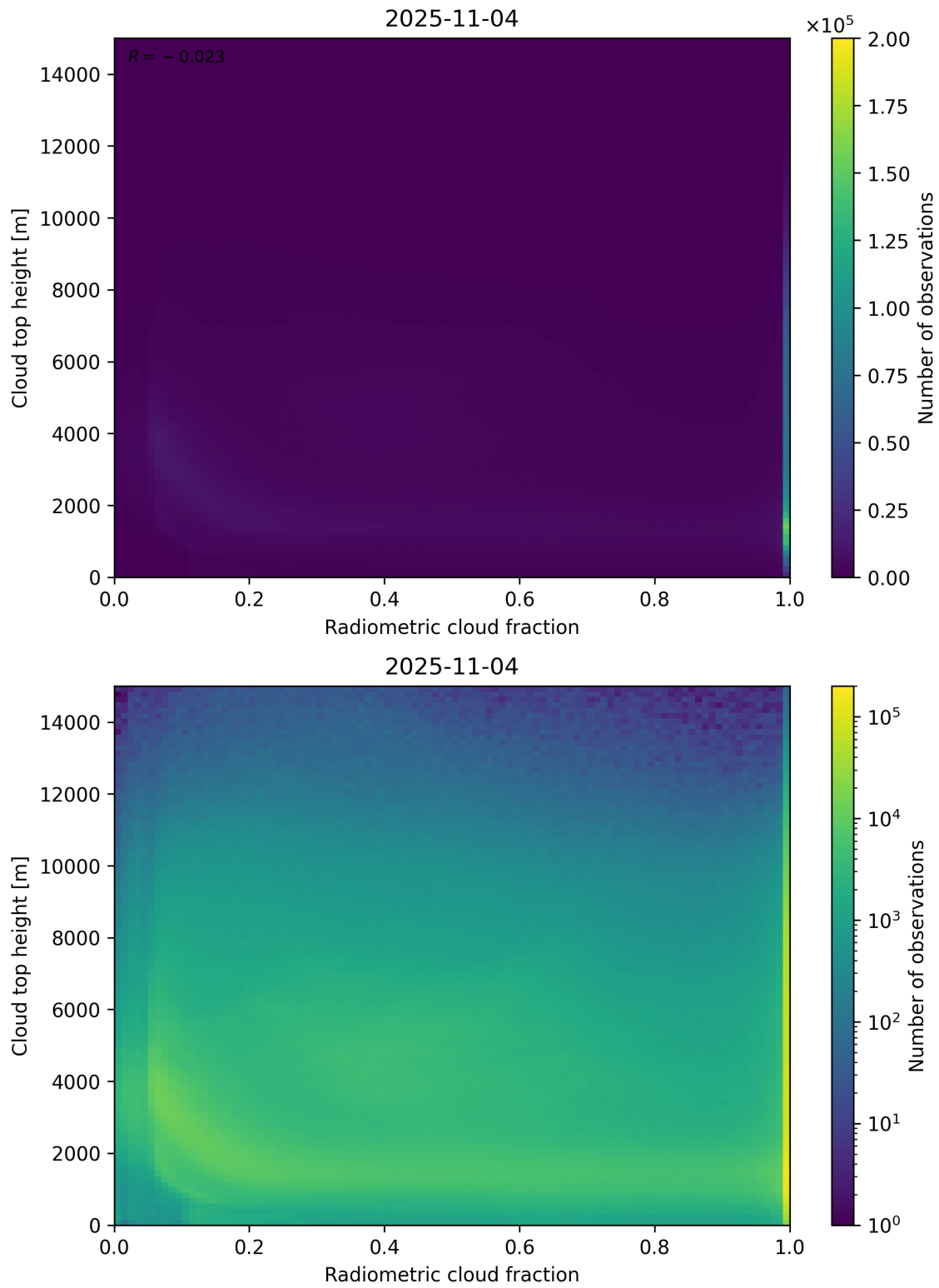
Figure 76: Scatter density plot of “Radiometric cloud fraction” against “Cloud top height” for 2025-11-03 to 2025-11-05.
