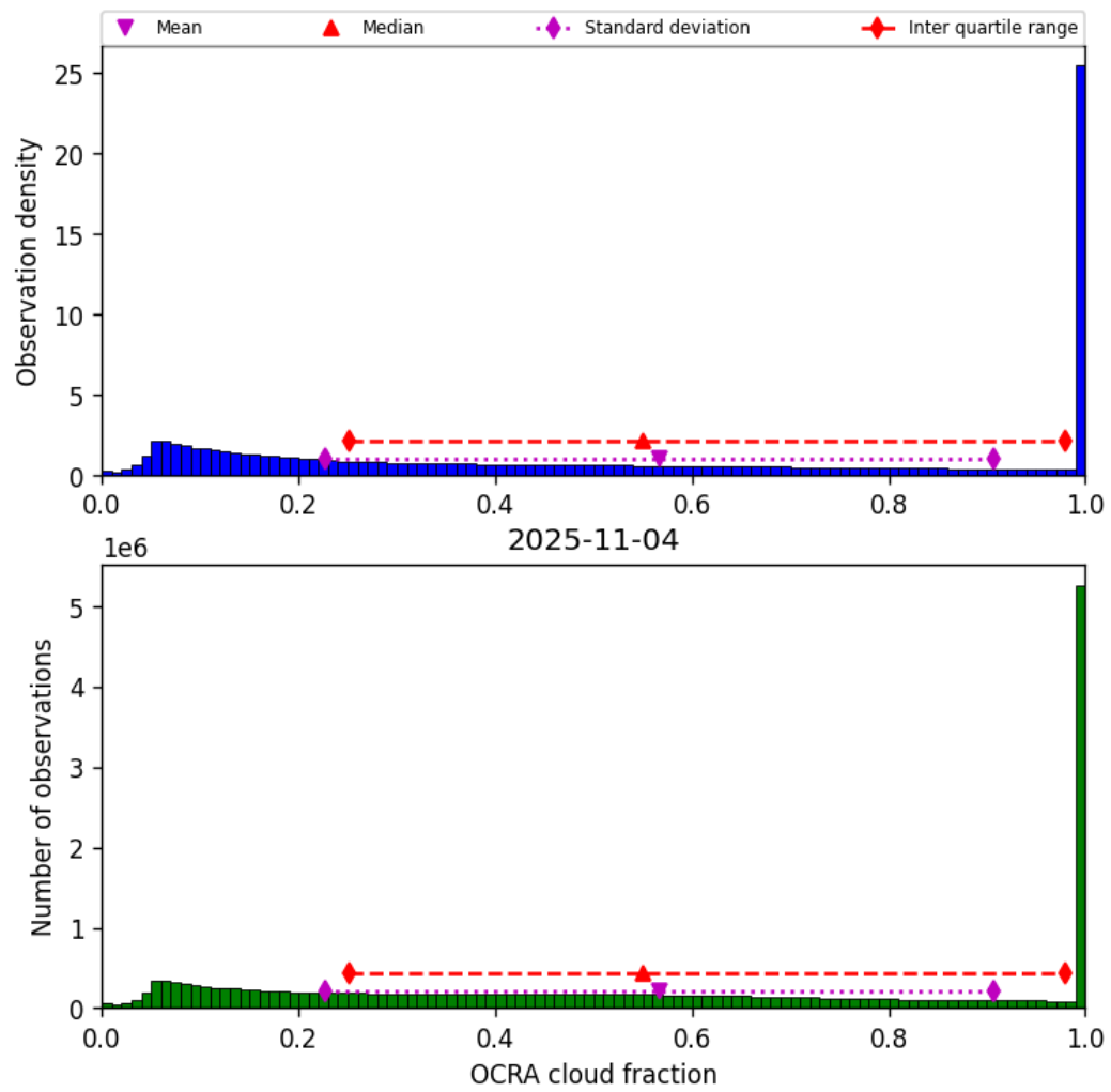
Figure 50: Histogram of “OCRA cloud fraction” for 2025-11-03 to 2025-11-05
