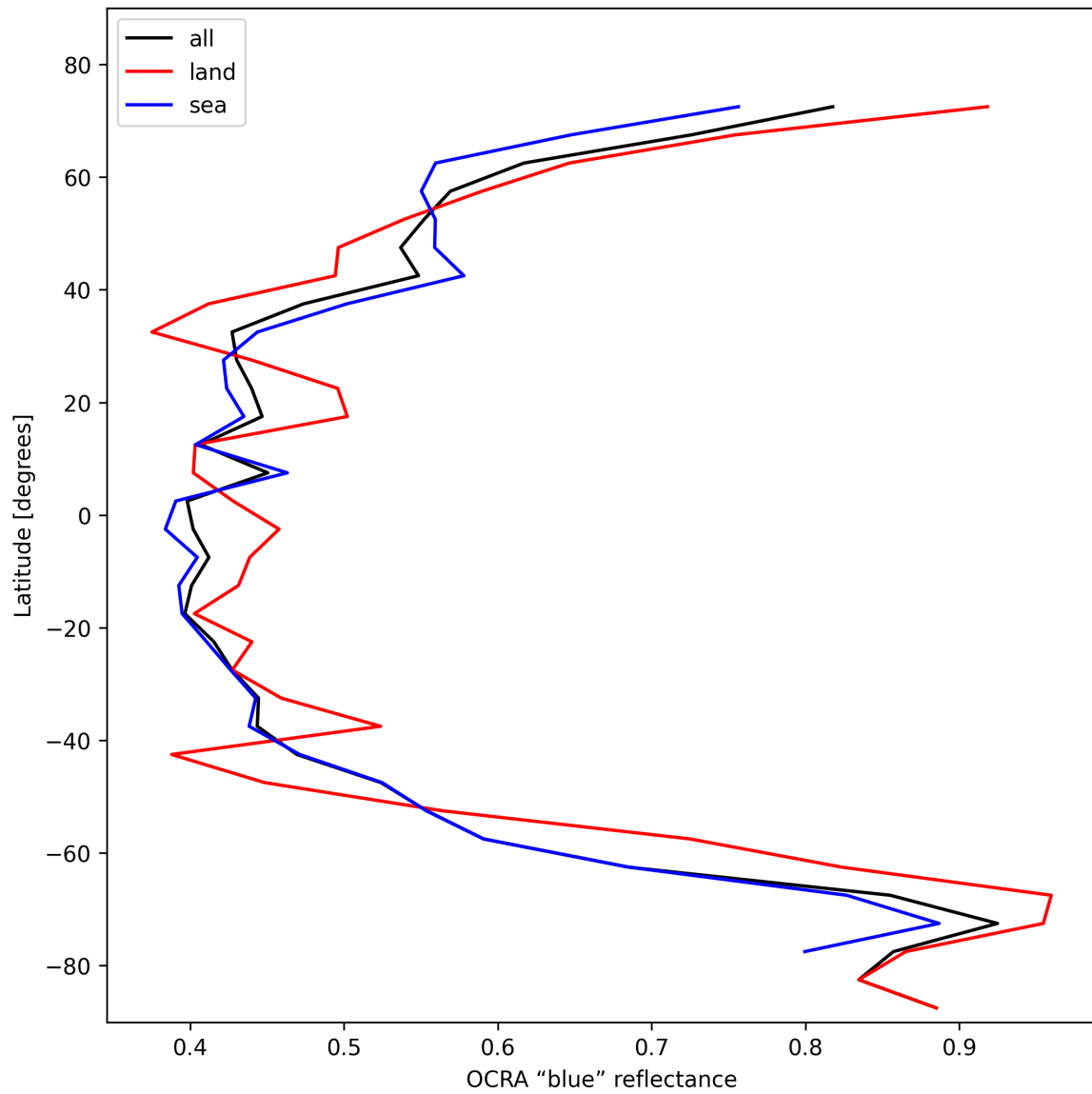
Figure 35: Zonal average of “OCRA “blue” reflectance” for 2025-11-03 to 2025-11-05.
