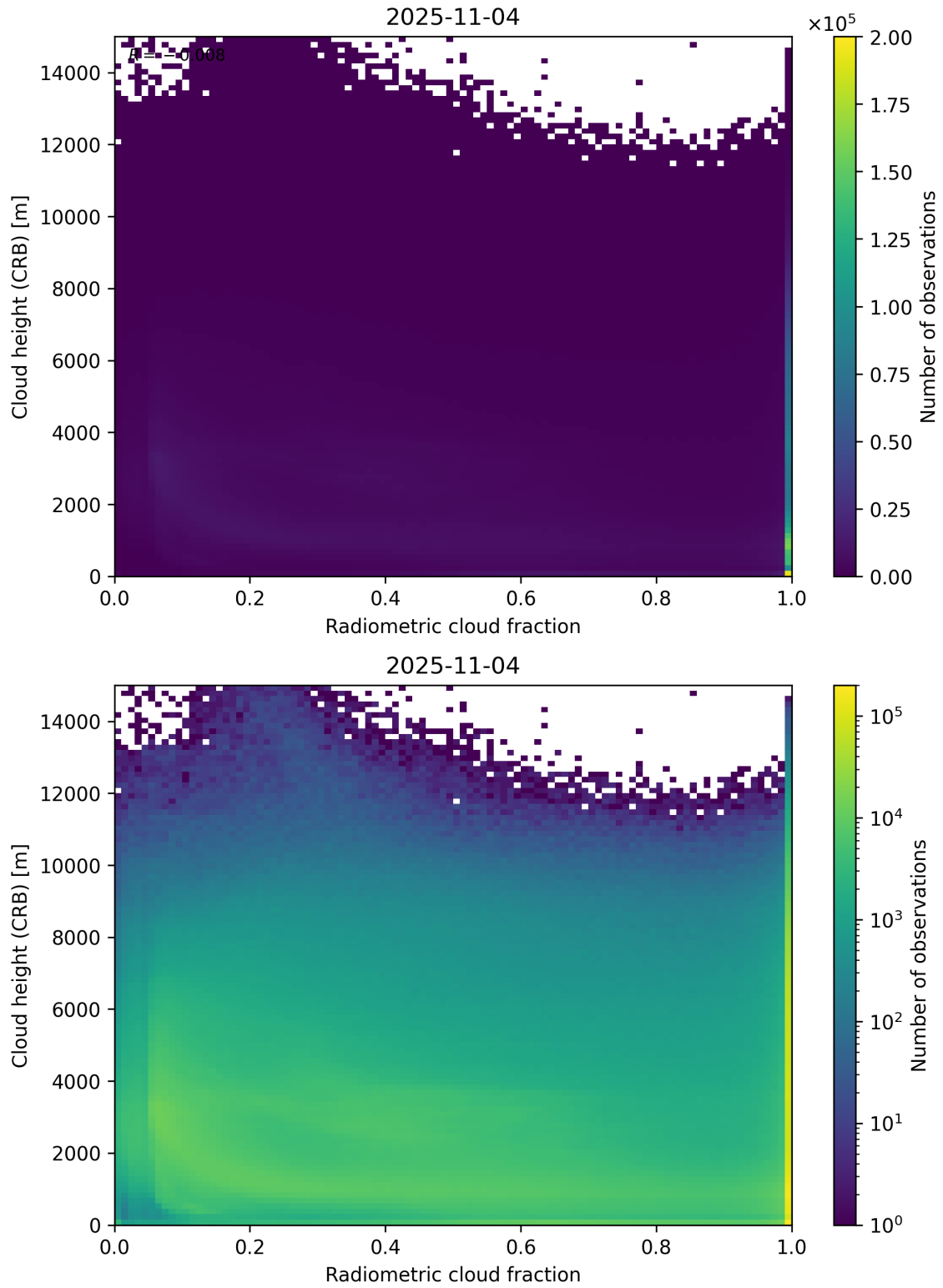
Figure 74: Scatter density plot of “Radiometric cloud fraction” against “Cloud height (CRB)” for 2025-11-03 to 2025-11-05.
