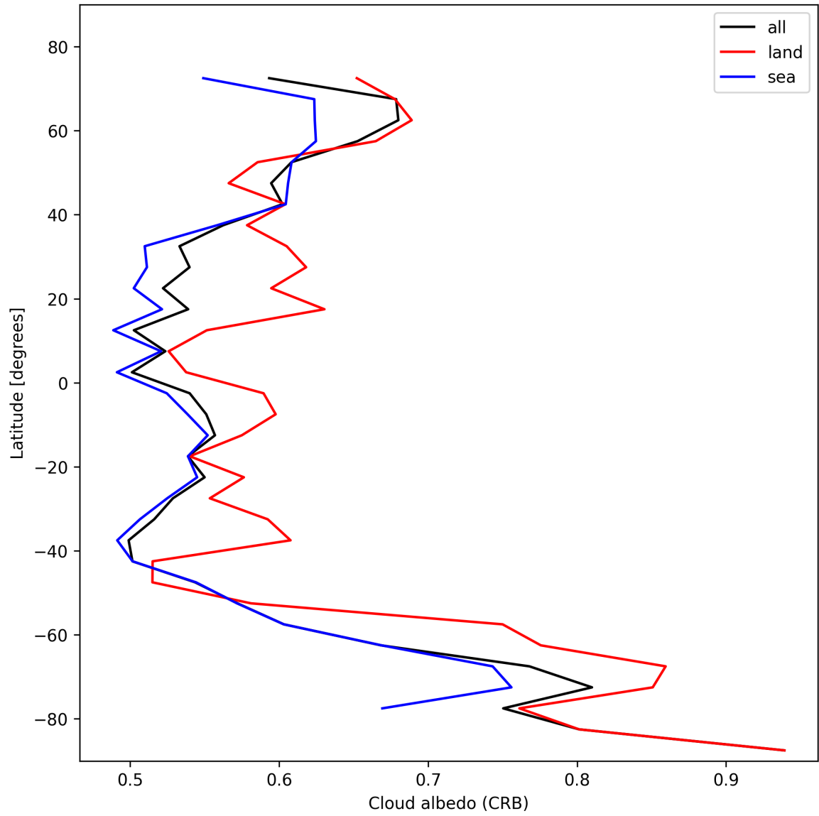
Figure 28: Zonal average of “Cloud albedo (CRB)” for 2025-11-03 to 2025-11-05.
