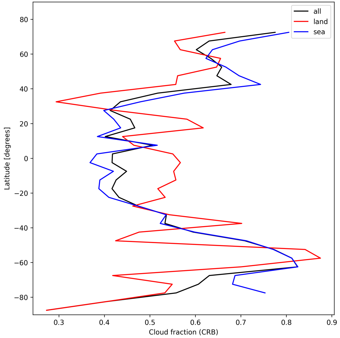
Figure 26: Zonal average of “Cloud fraction (CRB)” for 2025-11-03 to 2025-11-05.
