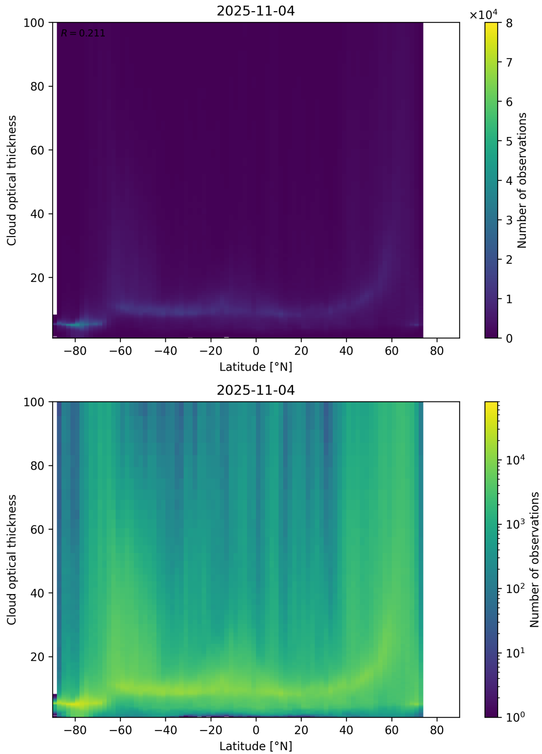
Figure 96: Scatter density plot of “Latitude” against “Cloud optical thickness” for 2025-11-03 to 2025-11-05.
