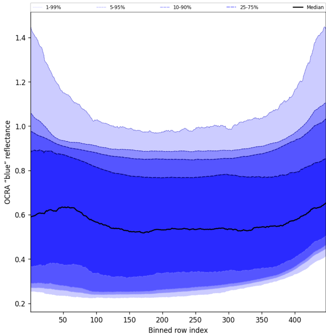
Figure 67: Along track statistics of "OCRA "blue" reflectance" for 2025-11-03 to 2025-11-05
