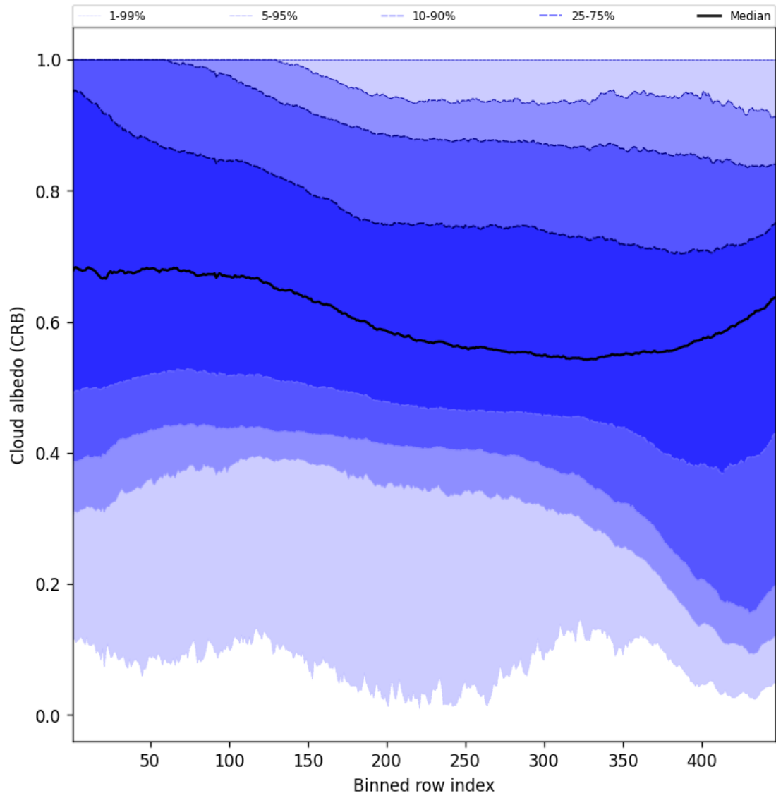
Figure 60: Along track statistics of “Cloud albedo (CRB)” for 2025-11-03 to 2025-11-05
