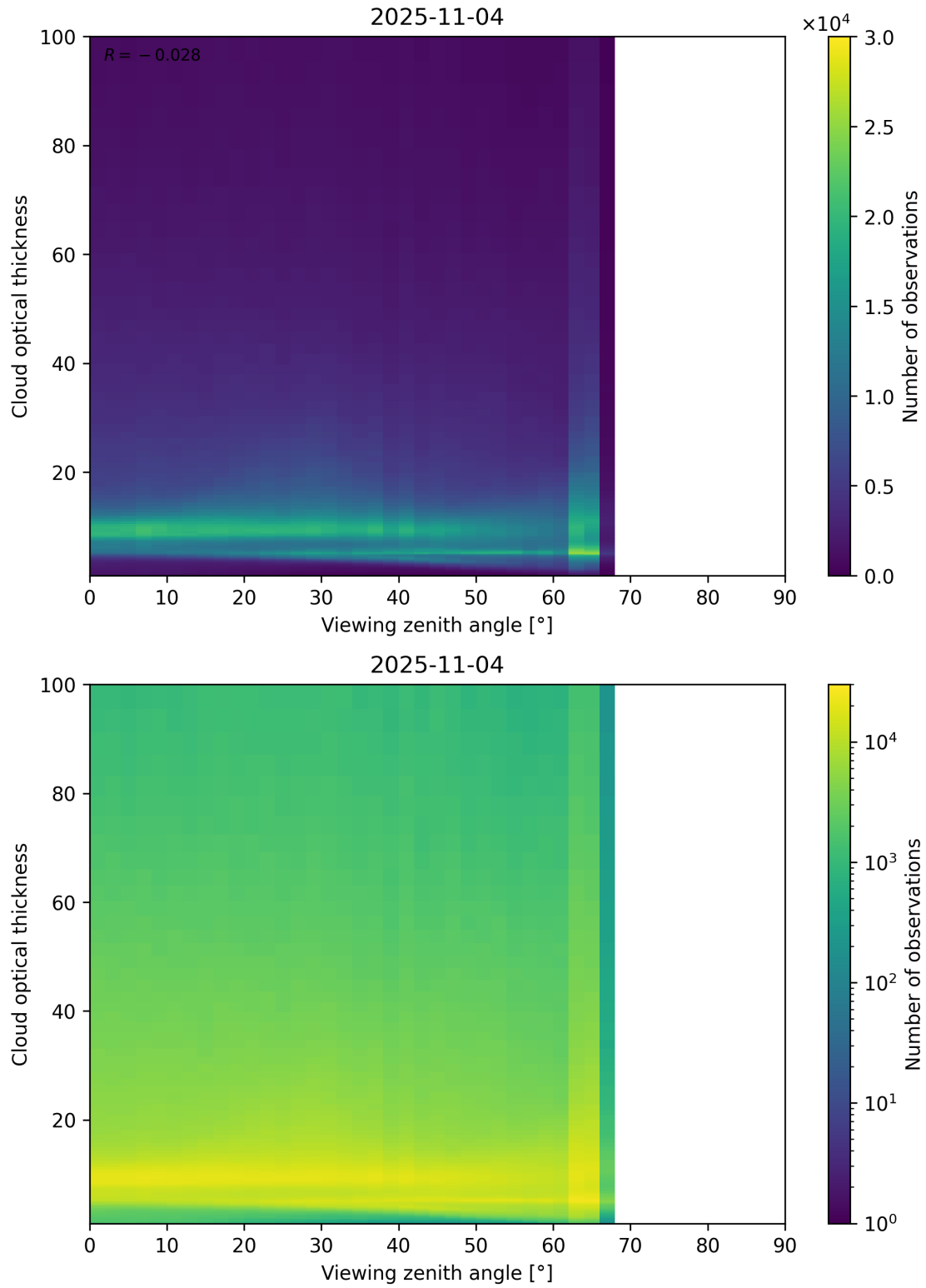
Figure 111: Scatter density plot of “Viewing zenith angle” against “Cloud optical thickness” for 2025-11-03 to 2025-11-05.
