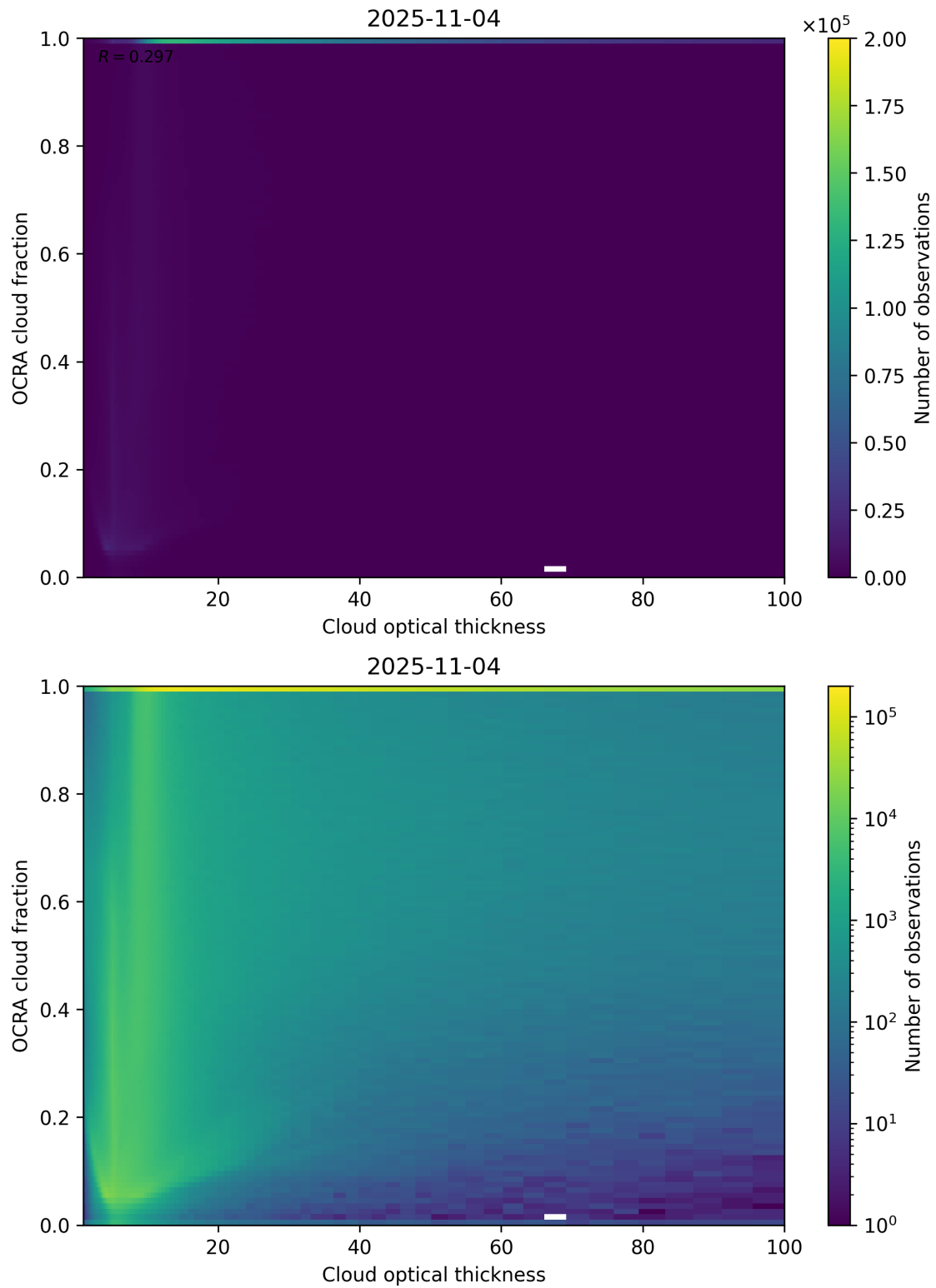
Figure 83: Scatter density plot of “Cloud optical thickness” against “OCRA cloud fraction” for 2025-11-03 to 2025-11-05.
