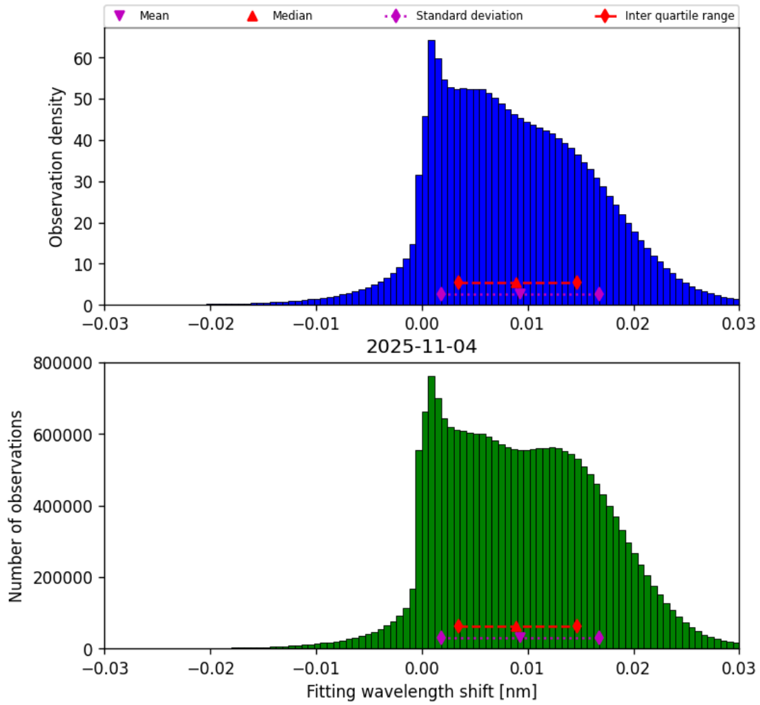
Figure 49: Histogram of “Fitting wavelength shift” for 2025-11-03 to 2025-11-05
