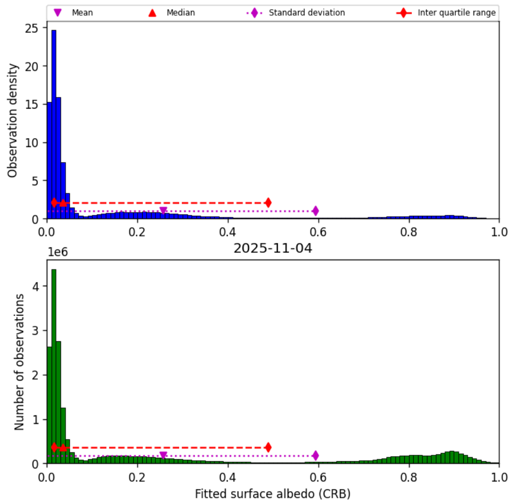
Figure 46: Histogram of “Fitted surface albedo (CRB)” for 2025-11-03 to 2025-11-05
