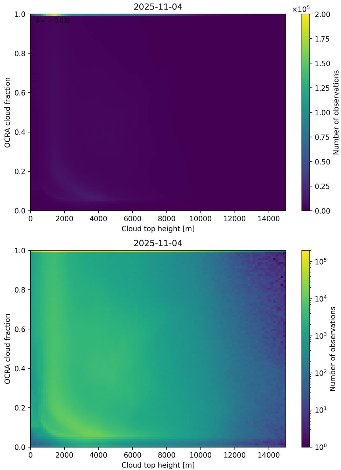
Figure 87: Scatter density plot of “Cloud top height” against “OCRA cloud fraction” for 2025-11-03 to 2025-11-05.
