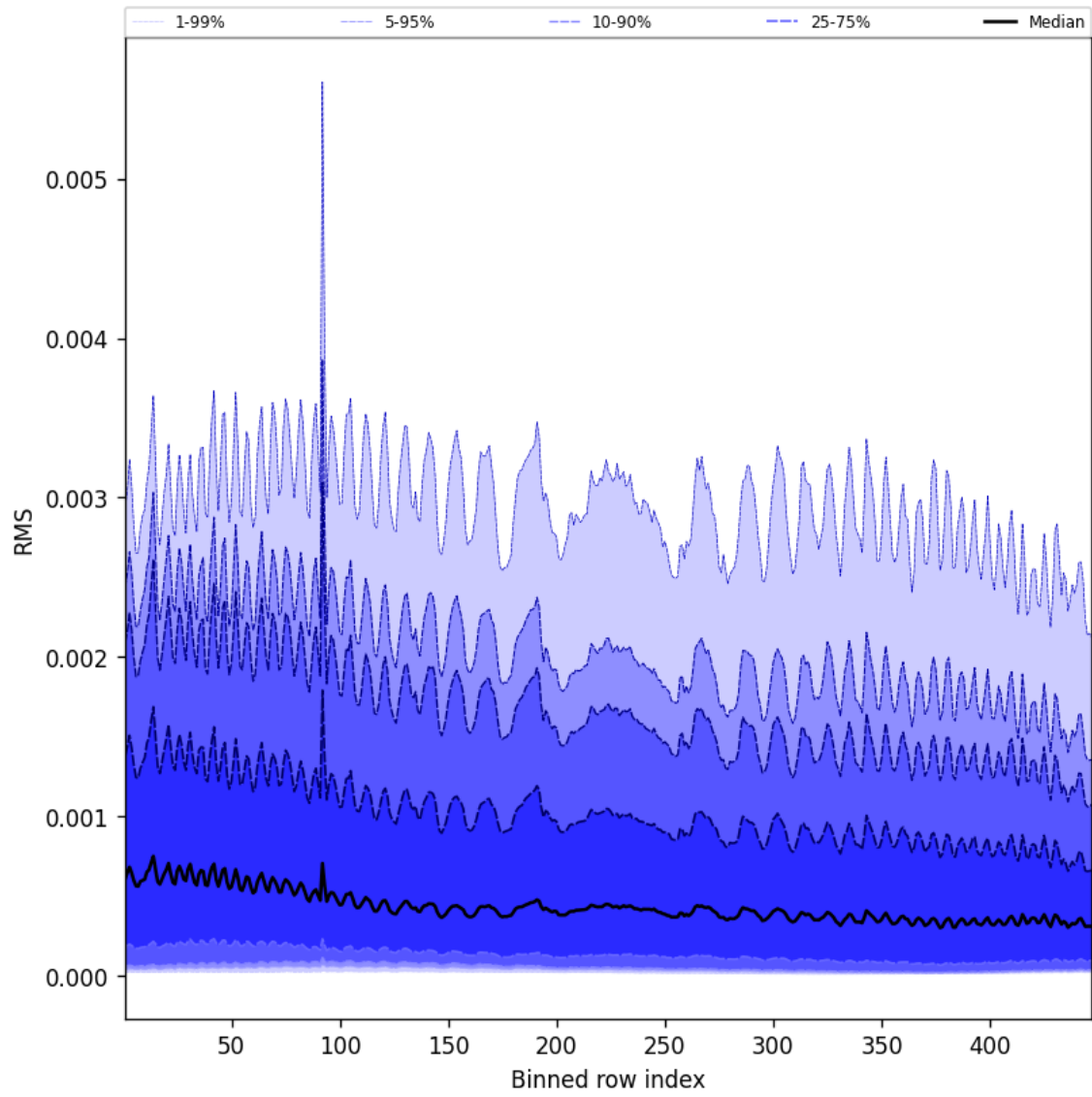
Figure 63: Along track statistics of “RMS” for 2025-11-03 to 2025-11-05
