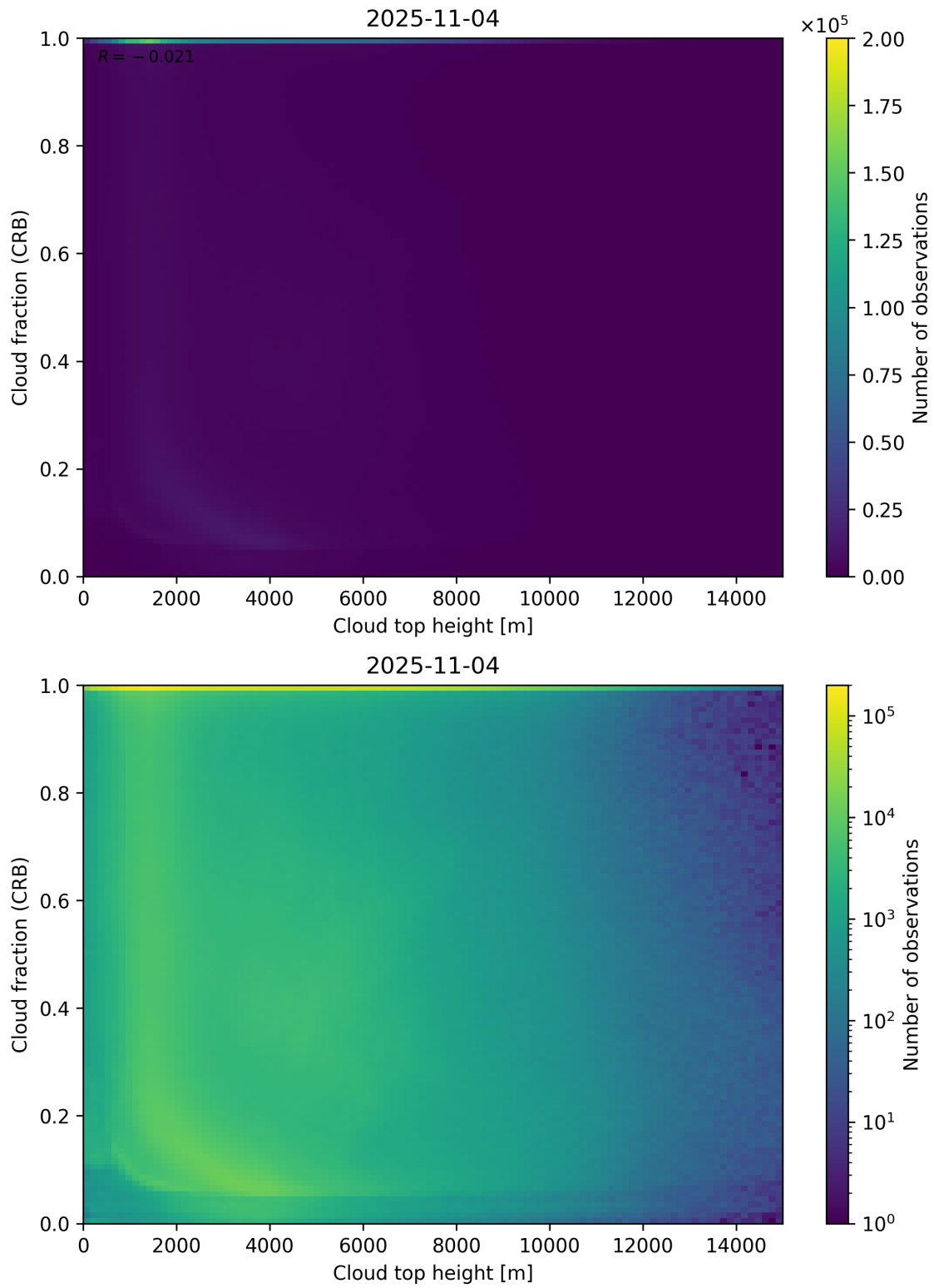
Figure 88: Scatter density plot of “Cloud top height” against “Cloud fraction (CRB)” for 2025-11-03 to 2025-11-05.
