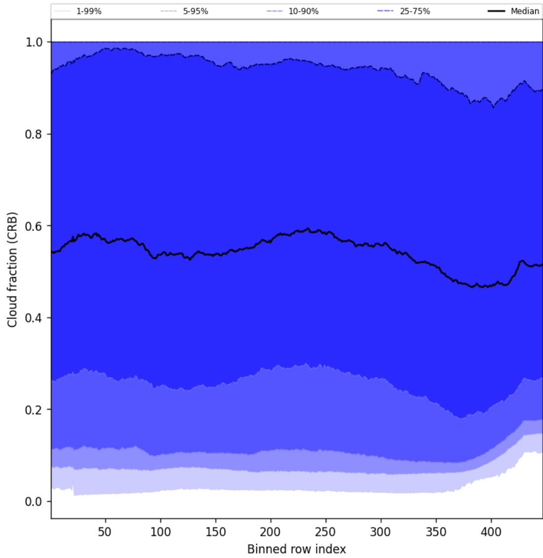
Figure 58: Along track statistics of “Cloud fraction (CRB)” for 2025-11-03 to 2025-11-05
