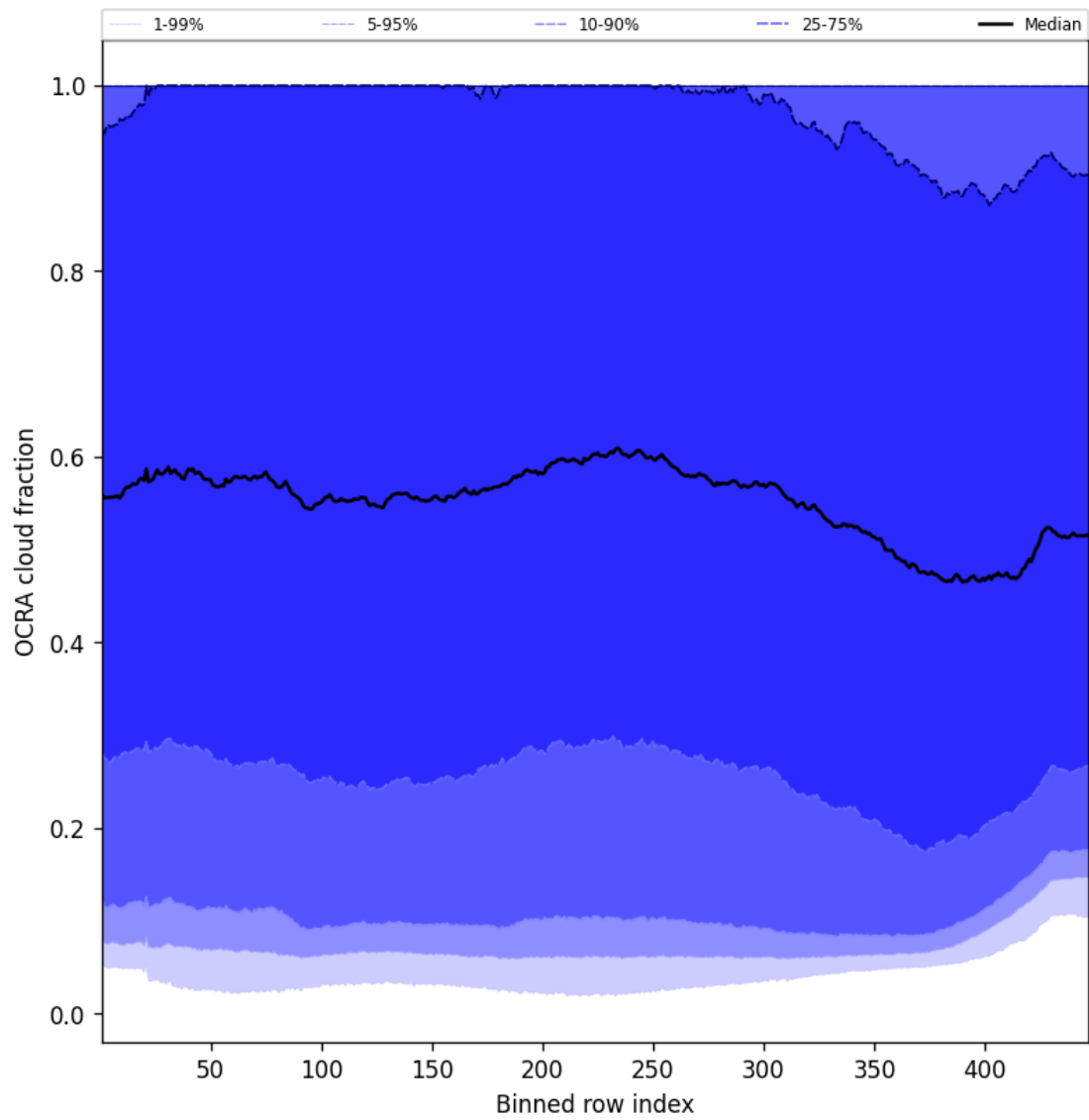
Figure 66: Along track statistics of “OCRA cloud fraction” for 2025-11-03 to 2025-11-05
