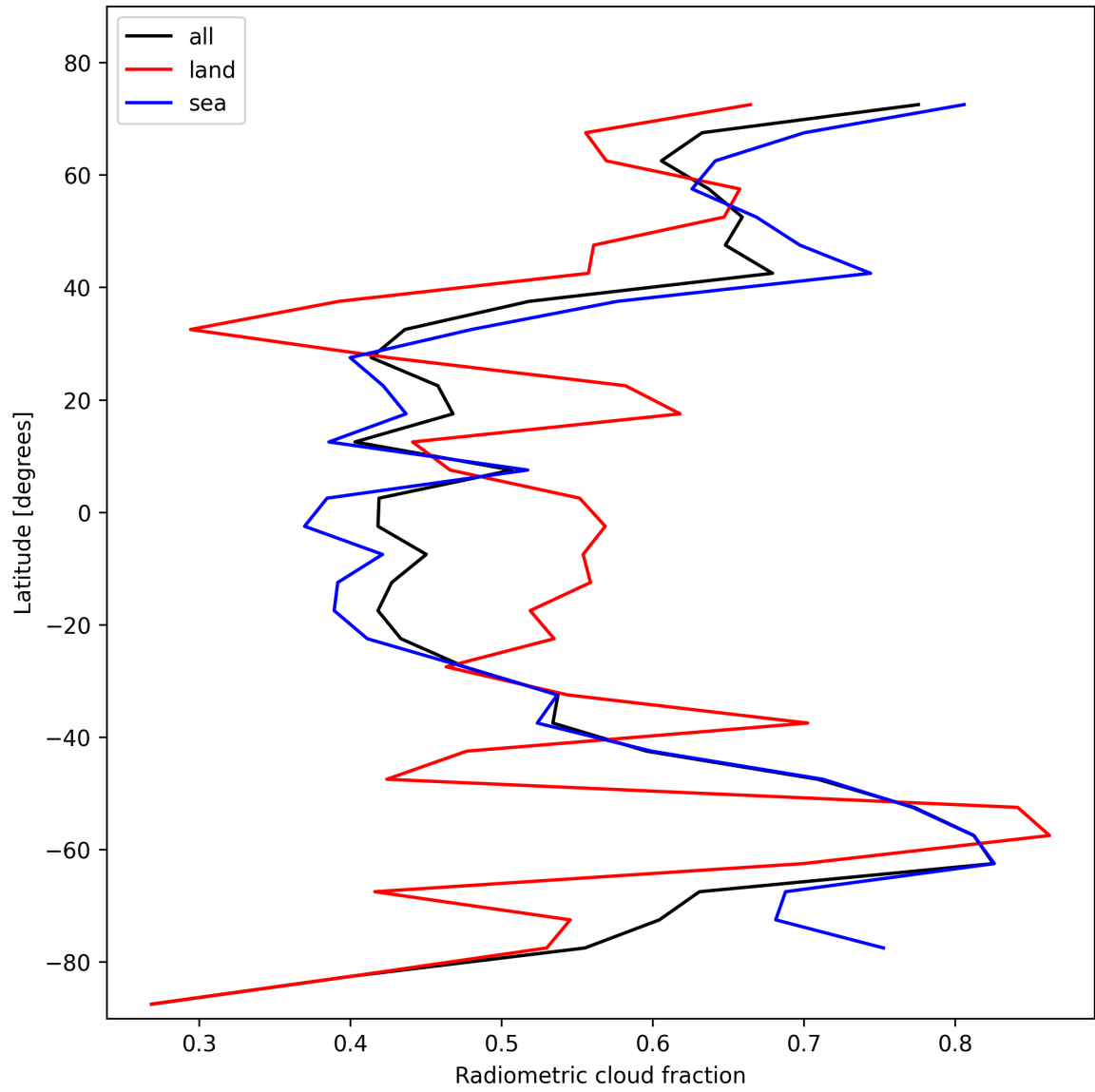
Figure 23: Zonal average of “Radiometric cloud fraction” for 2025-11-03 to 2025-11-05.
