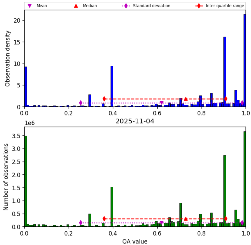
Figure 38: Histogram of “QA value” for 2025-11-03 to 2025-11-05
