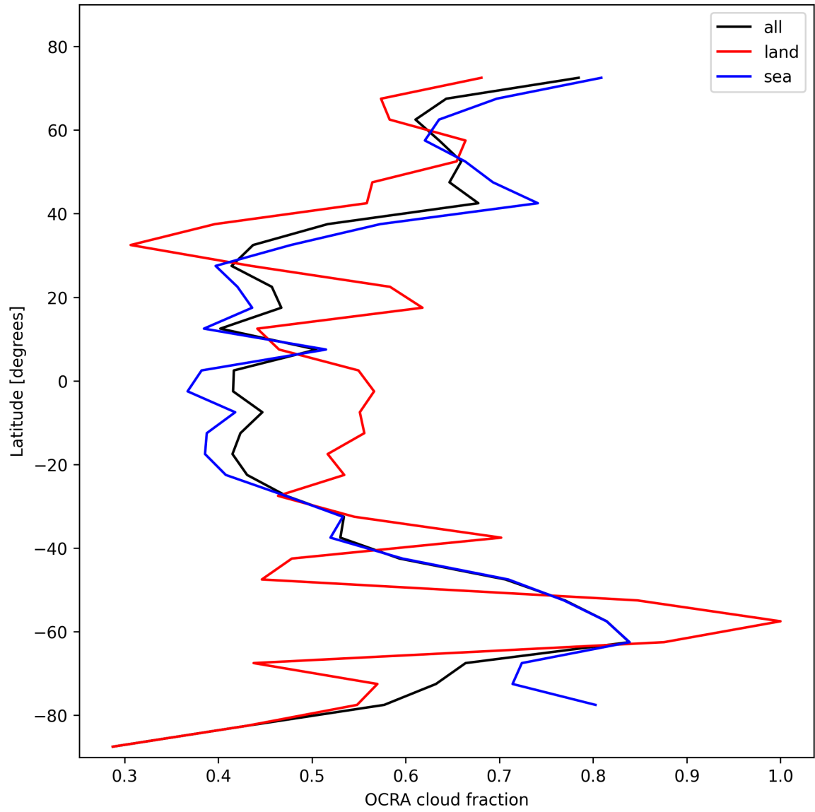
Figure 34: Zonal average of “OCRA cloud fraction” for 2025-11-03 to 2025-11-05.
