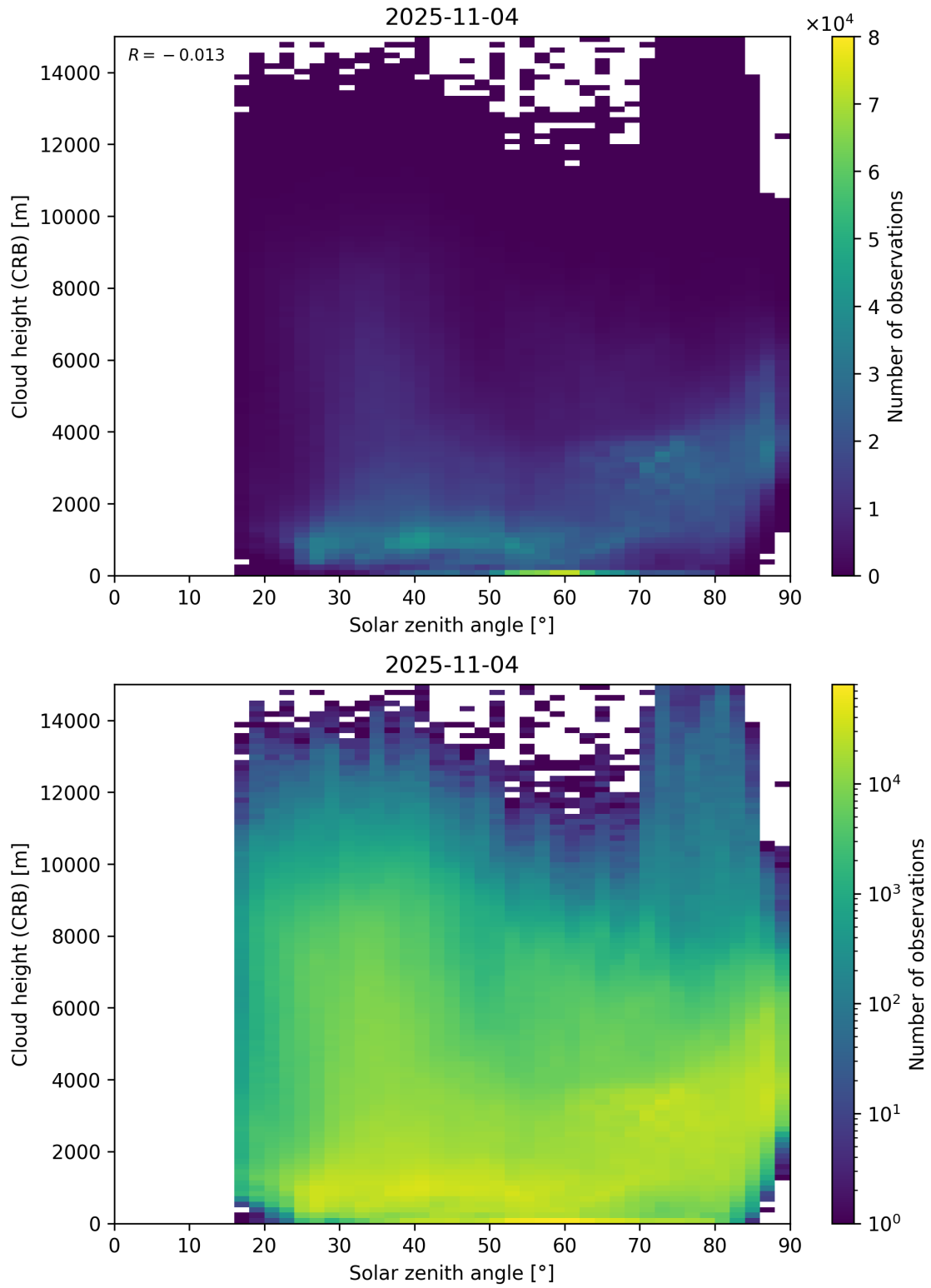
Figure 102: Scatter density plot of “Solar zenith angle” against “Cloud height (CRB)” for 2025-11-03 to 2025-11-05.
