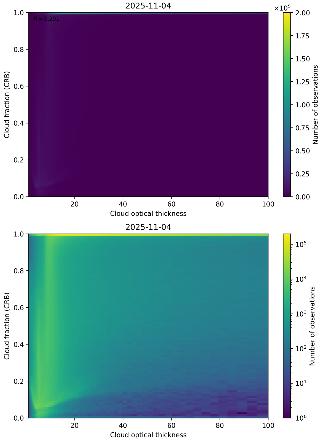
Figure 84: Scatter density plot of “Cloud optical thickness” against “Cloud fraction (CRB)” for 2025-11-03 to 2025-11-05.
