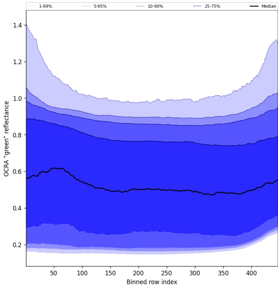
Figure 68: Along track statistics of “OCRA “green” reflectance” for 2025-11-03 to 2025-11-05
