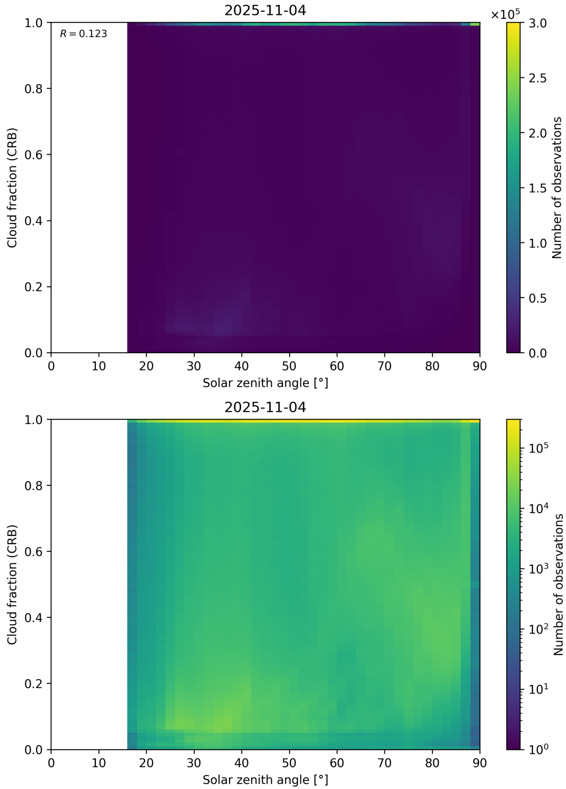
Figure 101: Scatter density plot of “Solar zenith angle” against “Cloud fraction (CRB)” for 2025-11-03 to 2025-11-05.
