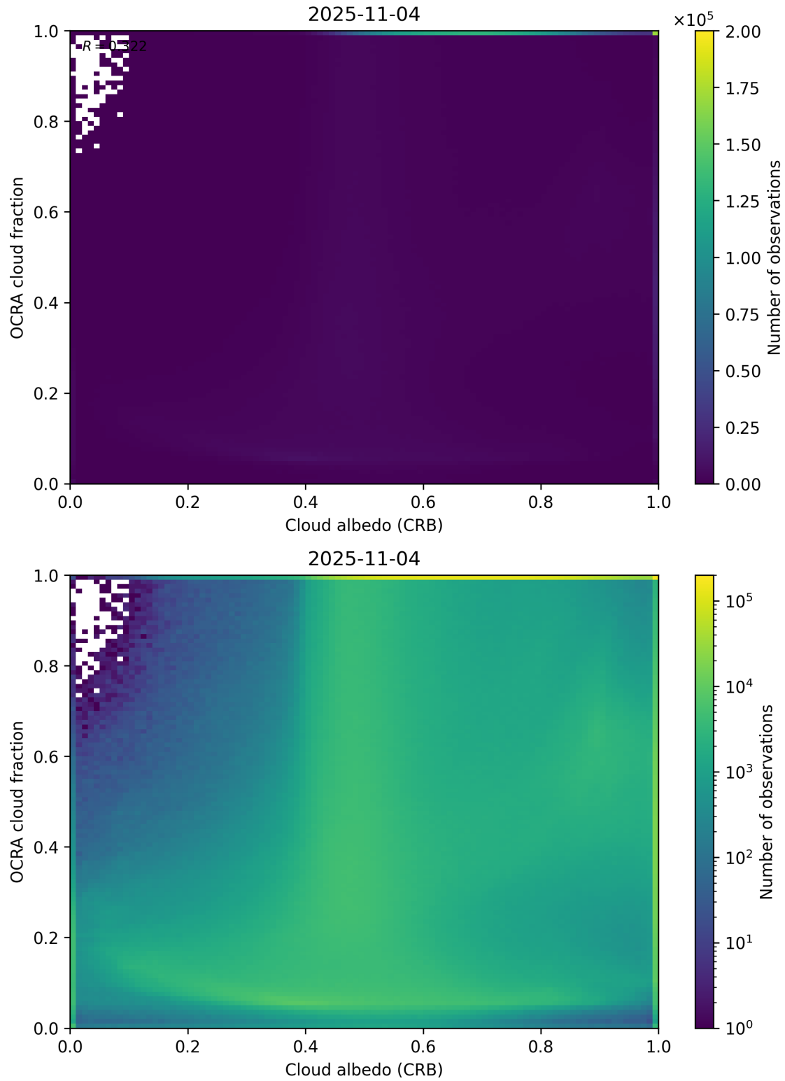
Figure 70: Scatter density plot of “Cloud albedo (CRB)” against “OCRA cloud fraction” for 2025-11-03 to 2025-11-05.
