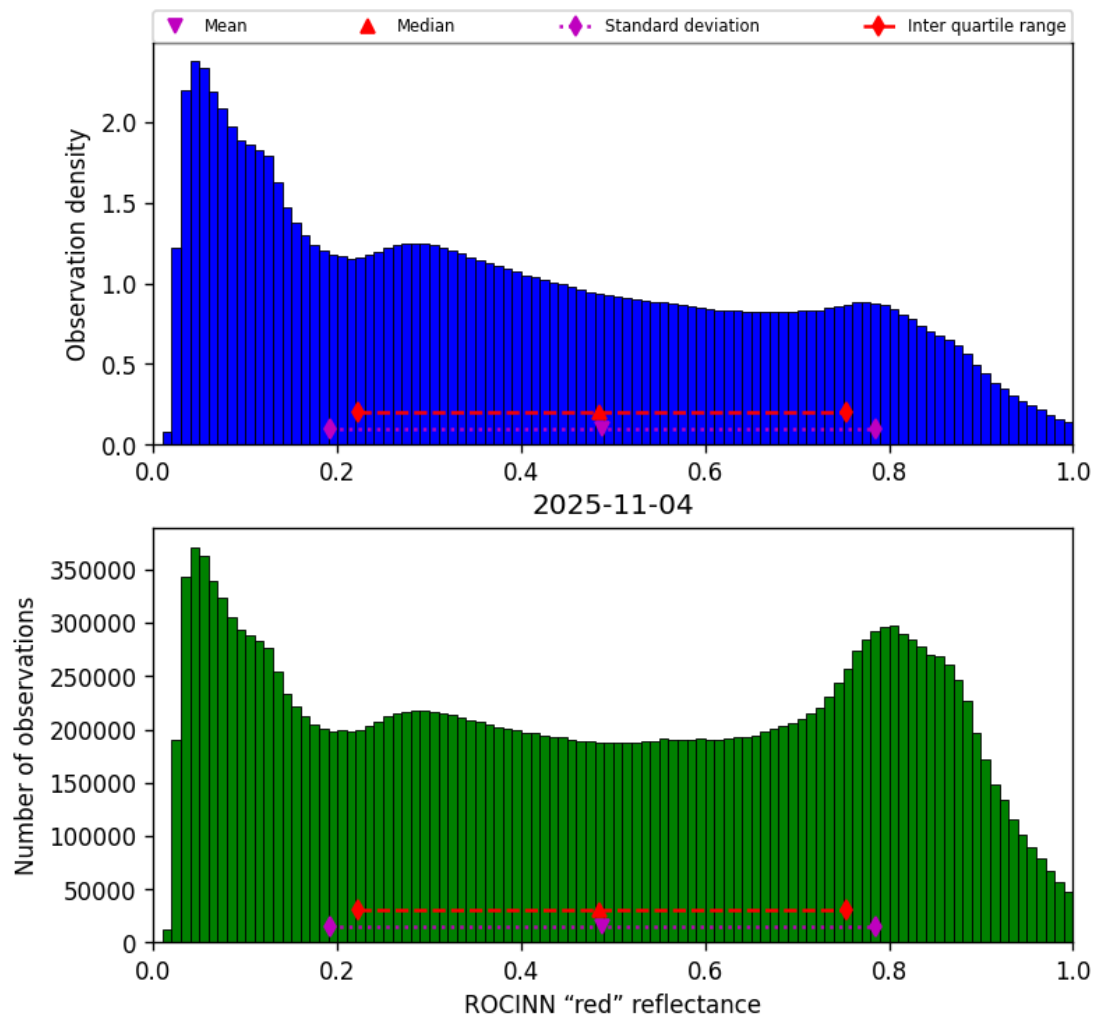
Figure 53: Histogram of “ROCINN “red” reflectance” for 2025-11-03 to 2025-11-05
