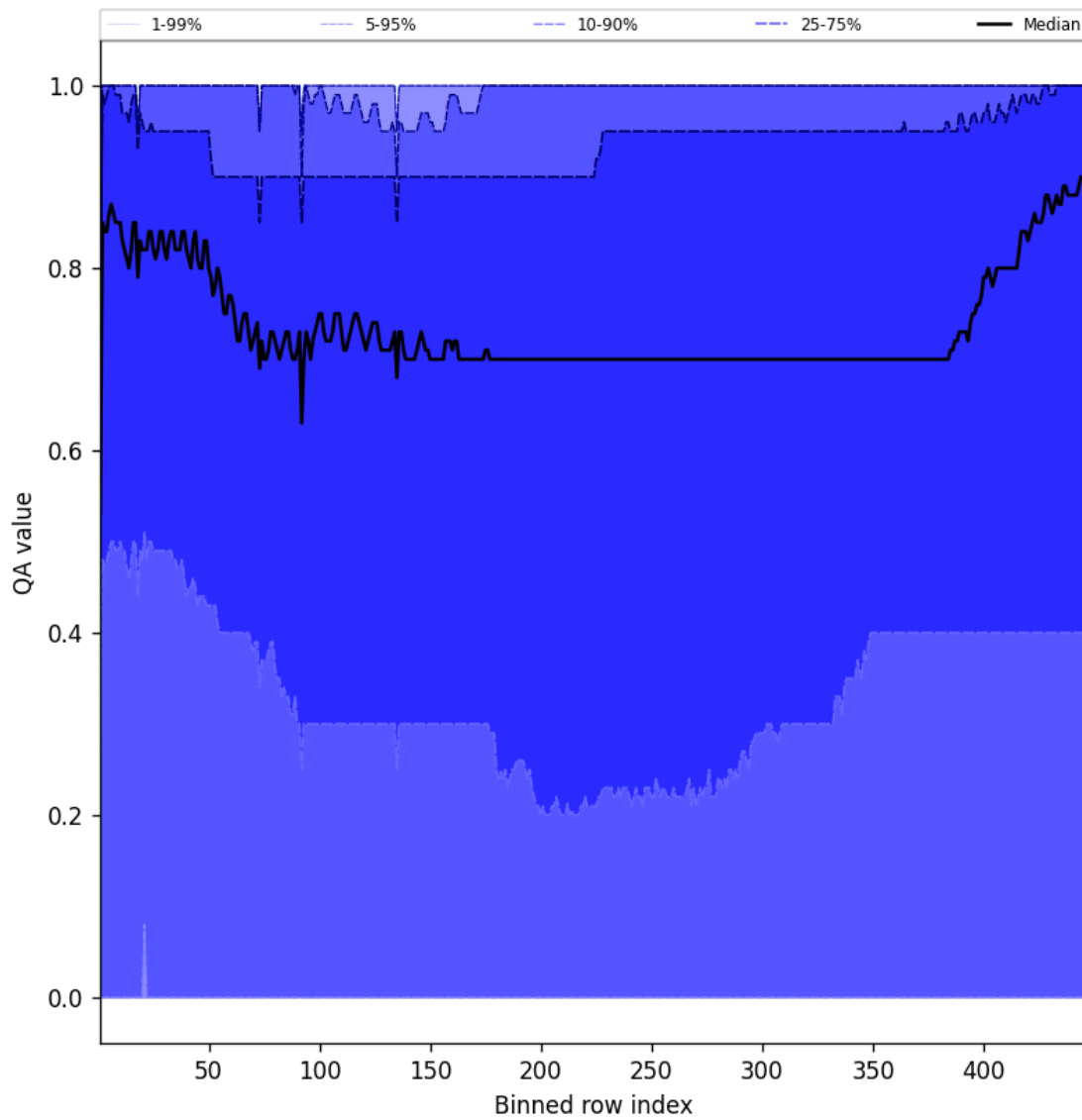
Figure 54: Along track statistics of “QA value” for 2025-11-03 to 2025-11-05
