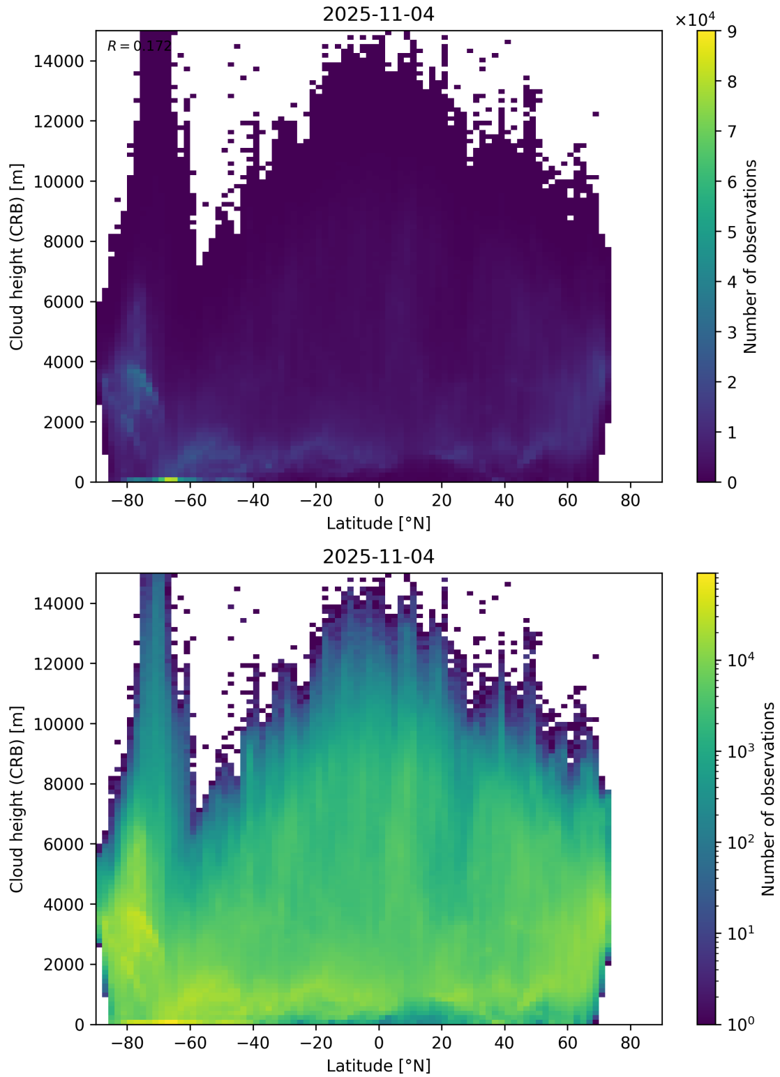
Figure 95: Scatter density plot of “Latitude” against “Cloud height (CRB)” for 2025-11-03 to 2025-11-05.
