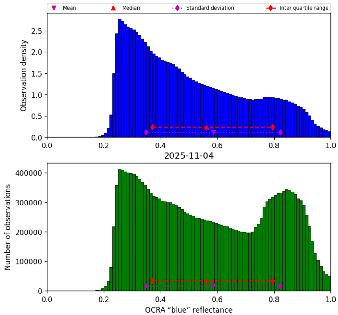
Figure 51: Histogram of “OCRA “blue” reflectance” for 2025-11-03 to 2025-11-05
