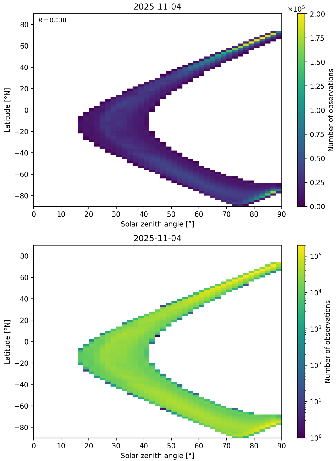
Figure 105: Scatter density plot of “Solar zenith angle” against “Latitude” for 2025-11-03 to 2025-11-05.
