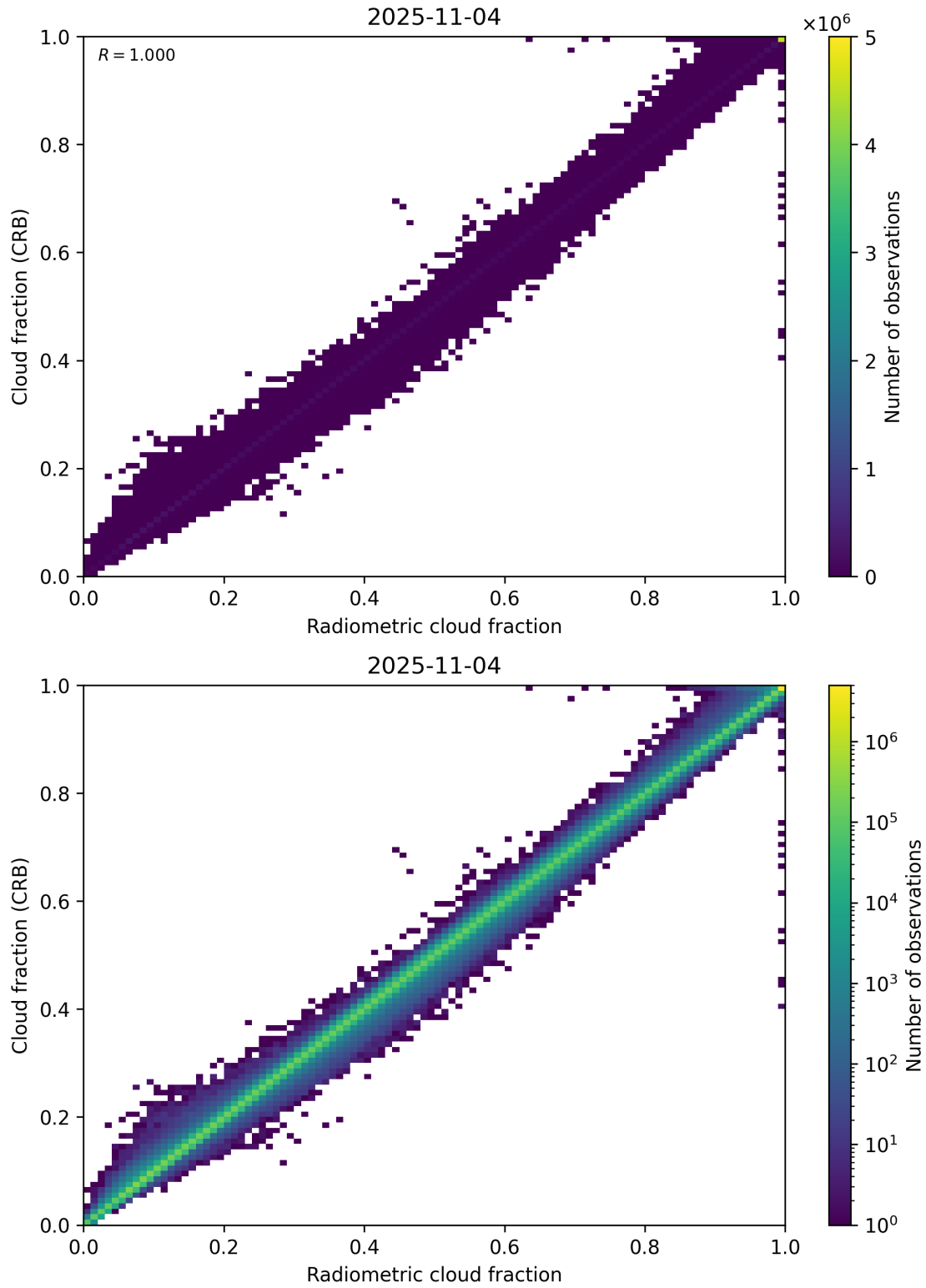
Figure 73: Scatter density plot of “Radiometric cloud fraction” against “Cloud fraction (CRB)” for 2025-11-03 to 2025-11-05.
