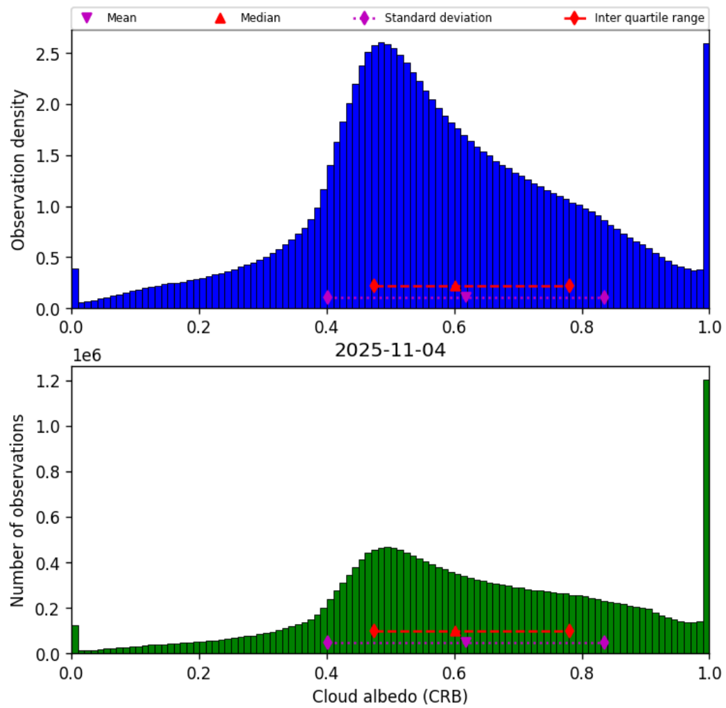
Figure 44: Histogram of “Cloud albedo (CRB)” for 2025-11-03 to 2025-11-05
