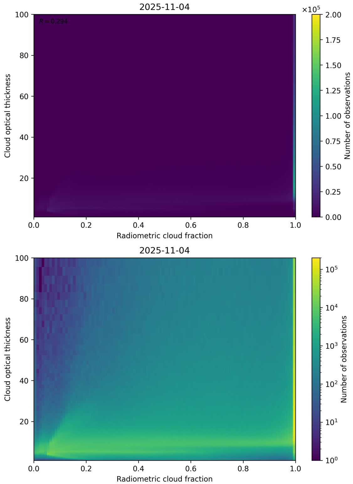
Figure 75: Scatter density plot of “Radiometric cloud fraction” against “Cloud optical thickness” for 2025-11-03 to 2025-11-05.
