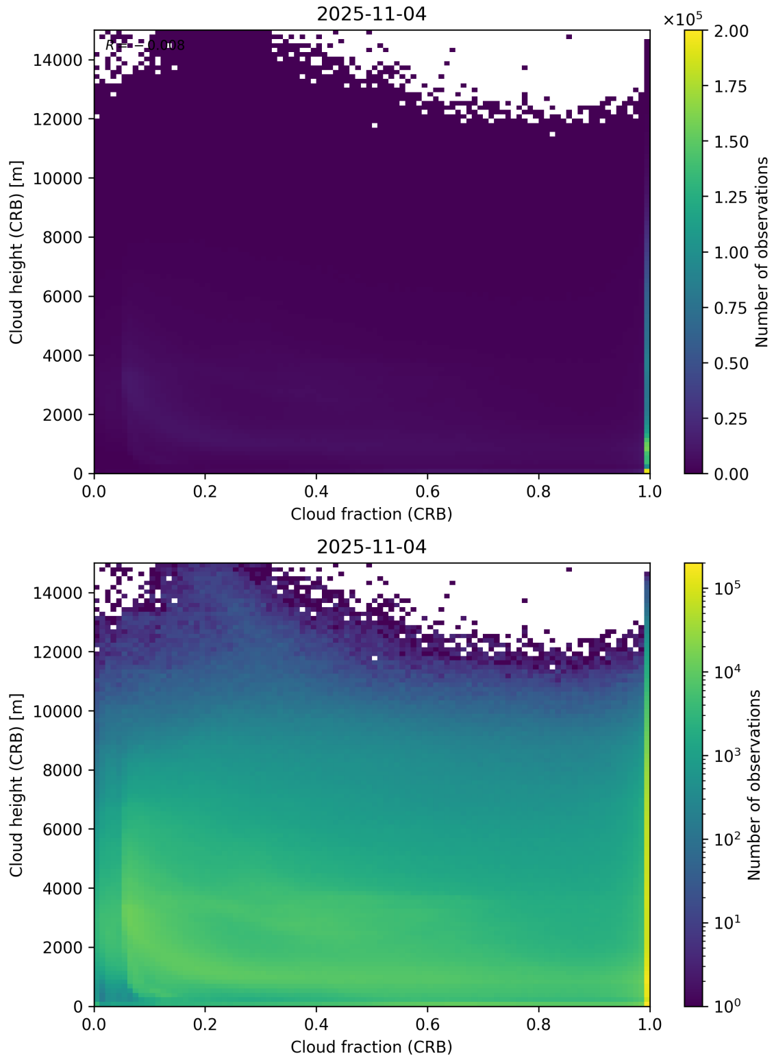
Figure 79: Scatter density plot of “Cloud fraction (CRB)” against “Cloud height (CRB)” for 2025-11-03 to 2025-11-05.
