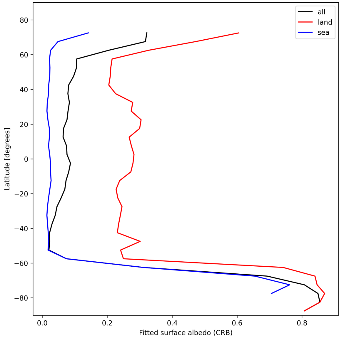
Figure 30: Zonal average of “Fitted surface albedo (CRB)” for 2025-11-03 to 2025-11-05.
