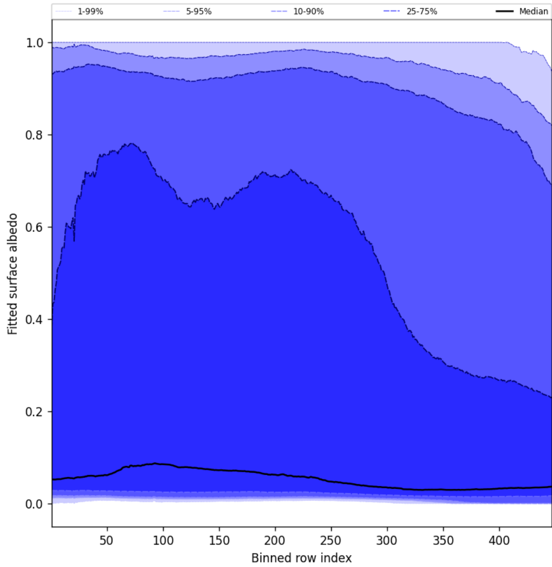
Figure 61: Along track statistics of “Fitted surface albedo” for 2025-11-03 to 2025-11-05
