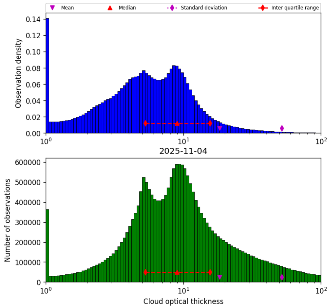
Figure 41: Histogram of “Cloud optical thickness” for 2025-11-03 to 2025-11-05
