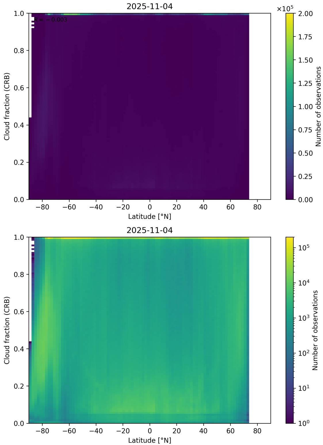
Figure 94: Scatter density plot of “Latitude” against “Cloud fraction (CRB)” for 2025-11-03 to 2025-11-05.
