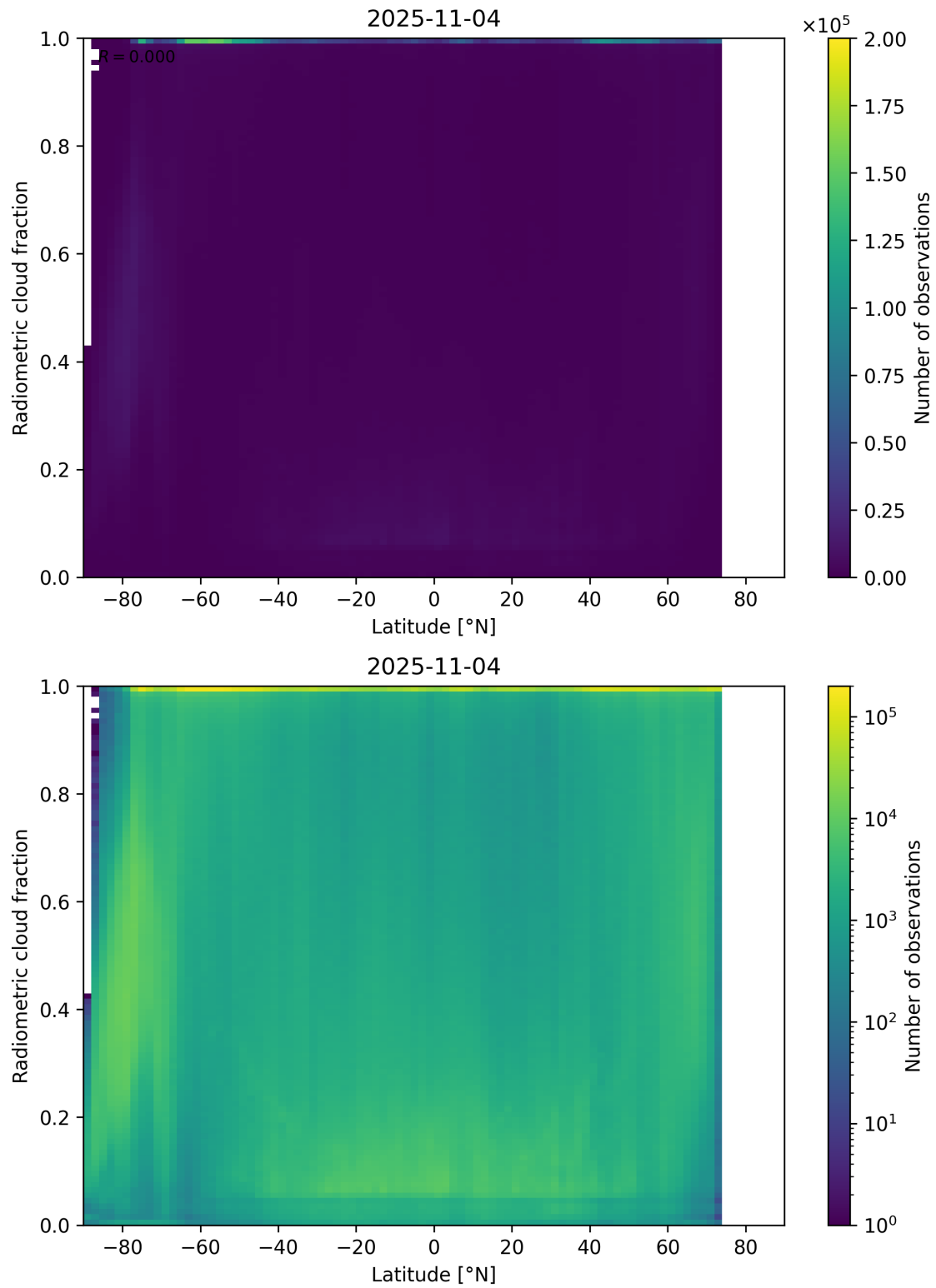
Figure 92: Scatter density plot of “Latitude” against “Radiometric cloud fraction” for 2025-11-03 to 2025-11-05.
