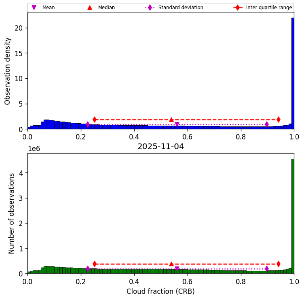
Figure 42: Histogram of “Cloud fraction (CRB)” for 2025-11-03 to 2025-11-05
