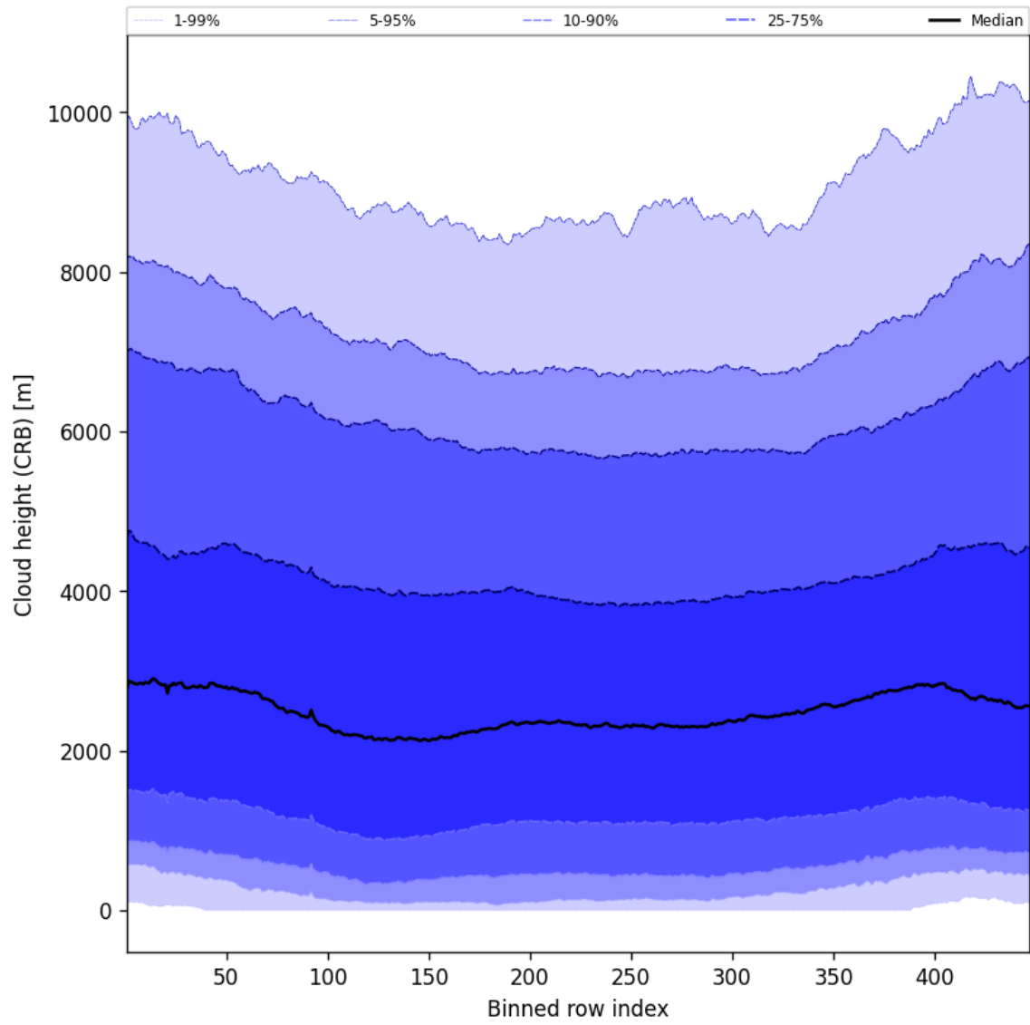
Figure 59: Along track statistics of “Cloud height (CRB)” for 2025-11-03 to 2025-11-05
