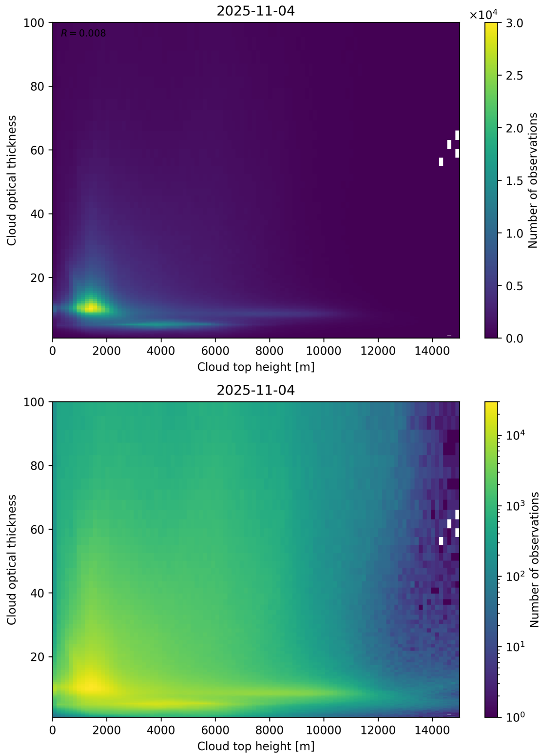
Figure 90: Scatter density plot of “Cloud top height” against “Cloud optical thickness” for 2025-11-03 to 2025-11-05.
