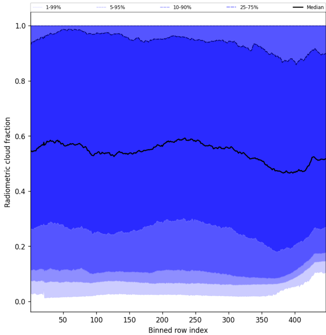
Figure 55: Along track statistics of “Radiometric cloud fraction” for 2025-11-03 to 2025-11-05
