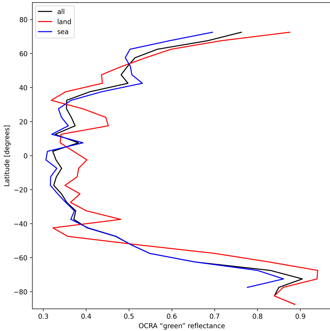
Figure 36: Zonal average of “OCRA “green” reflectance” for 2025-11-03 to 2025-11-05.
