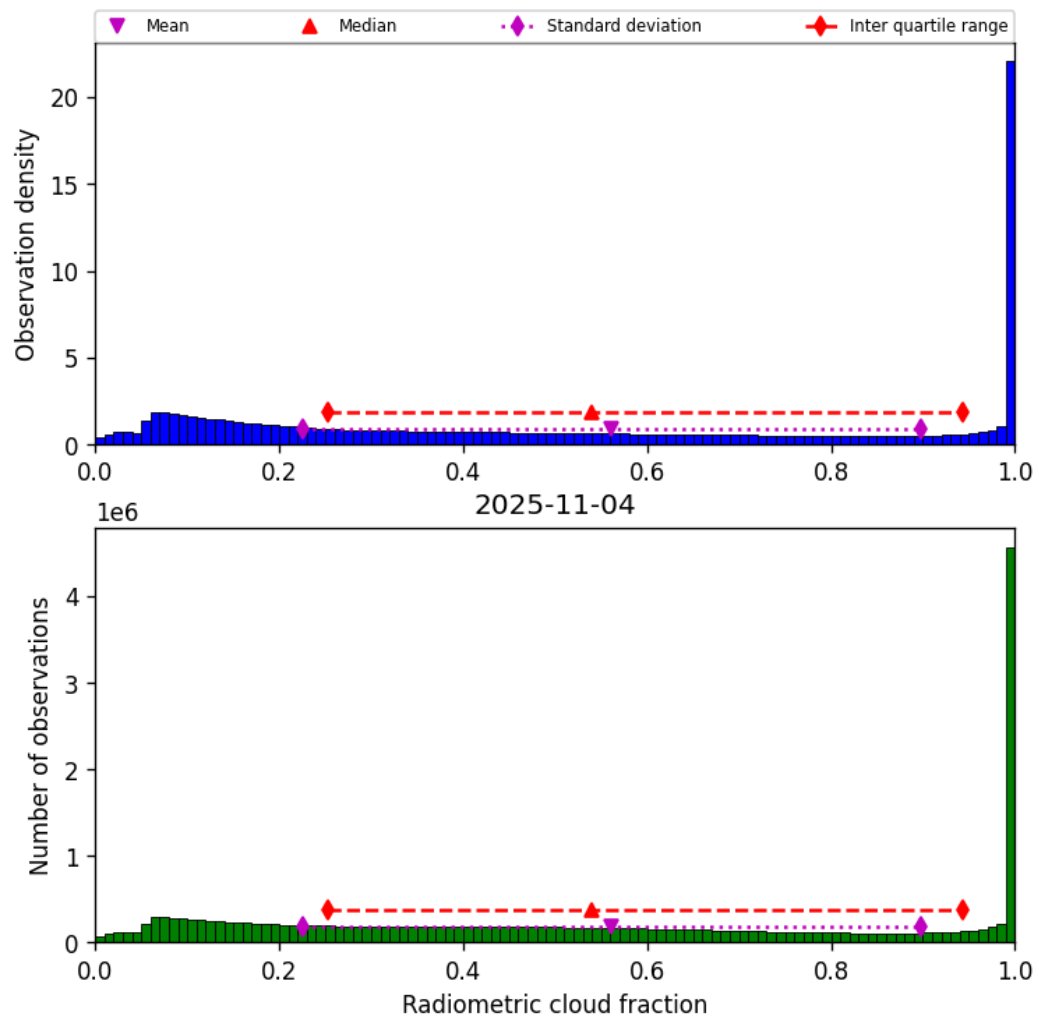
Figure 39: Histogram of “Radiometric cloud fraction” for 2025-11-03 to 2025-11-05
