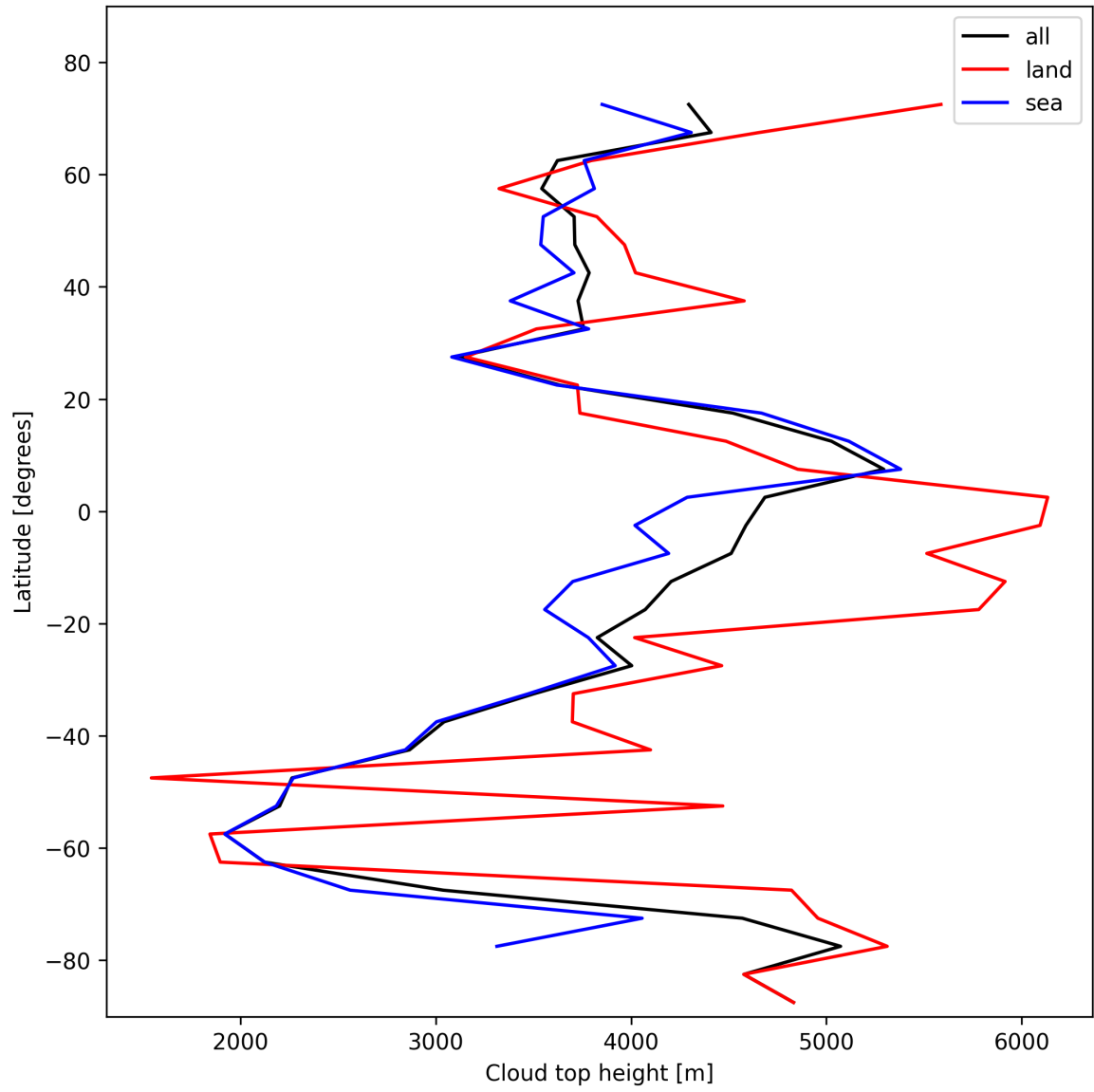
Figure 24: Zonal average of “Cloud top height” for 2025-11-03 to 2025-11-05.
