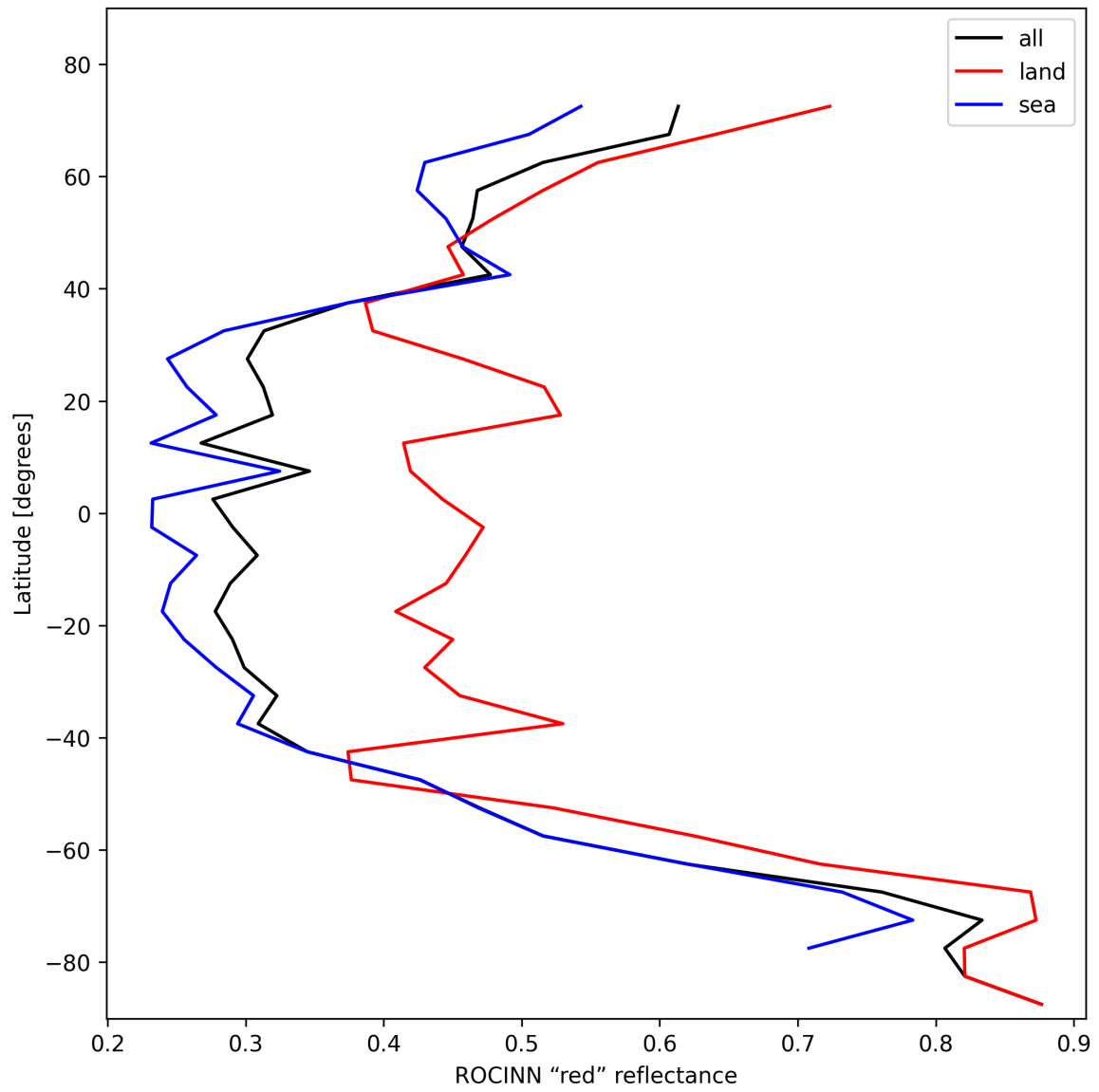
Figure 37: Zonal average of “ROCINN “red” reflectance” for 2025-11-03 to 2025-11-05.
