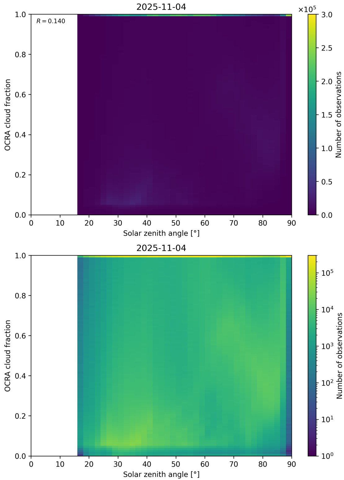
Figure 100: Scatter density plot of “Solar zenith angle” against “OCRA cloud fraction” for 2025-11-03 to 2025-11-05.
