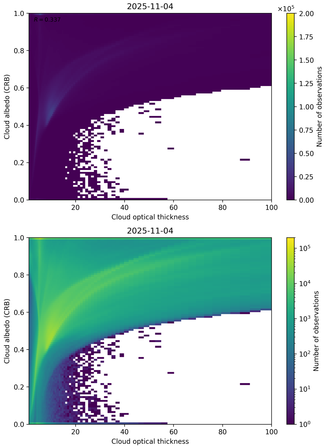
Figure 82: Scatter density plot of “Cloud optical thickness” against “Cloud albedo (CRB)” for 2025-11-03 to 2025-11-05.
