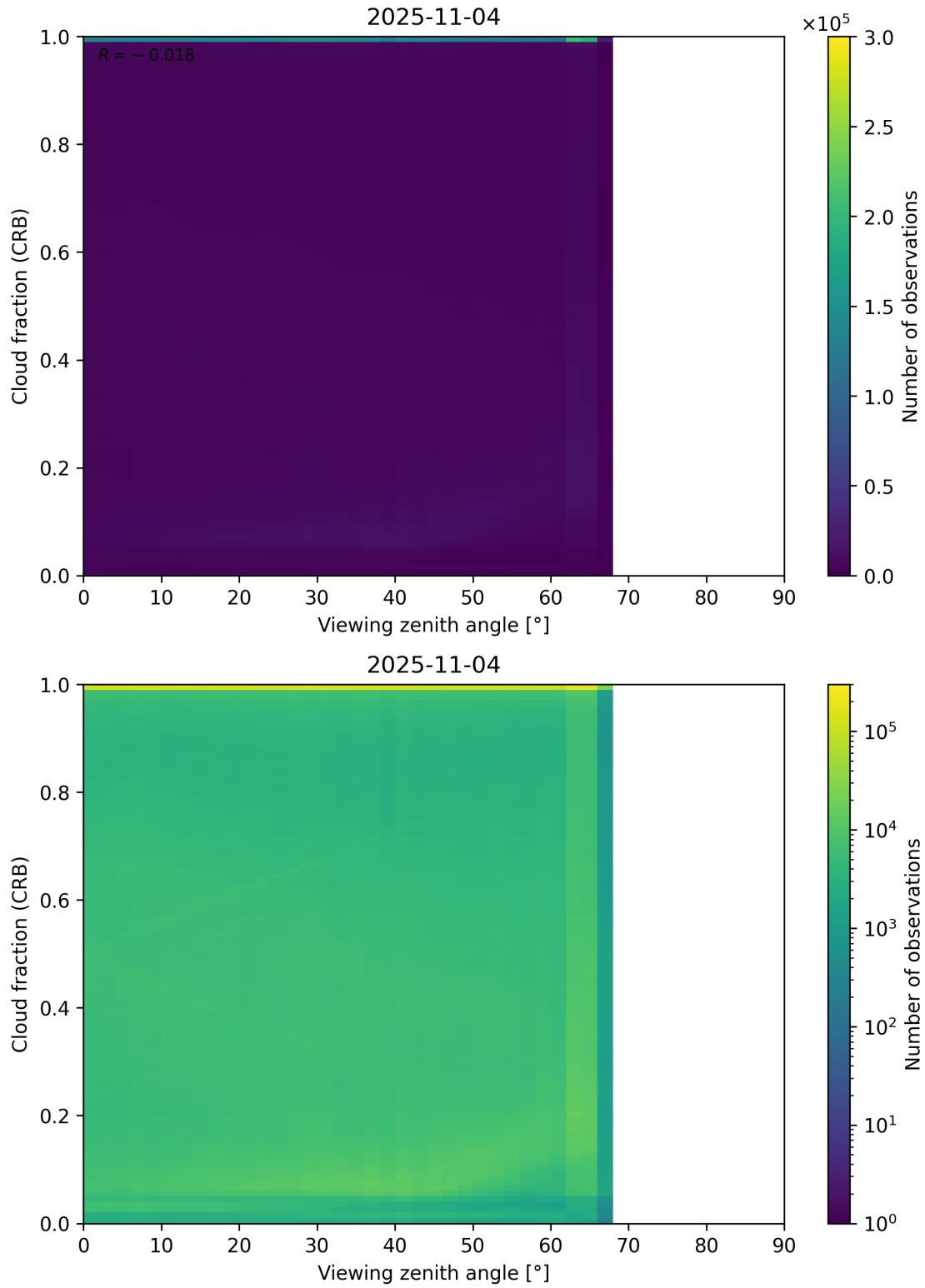
Figure 109: Scatter density plot of “Viewing zenith angle” against “Cloud fraction (CRB)” for 2025-11-03 to 2025-11-05.
