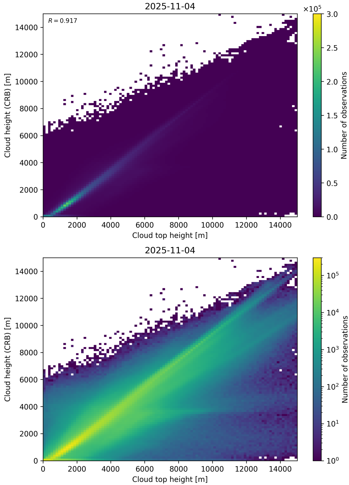
Figure 89: Scatter density plot of “Cloud top height” against “Cloud height (CRB)” for 2025-11-03 to 2025-11-05.
