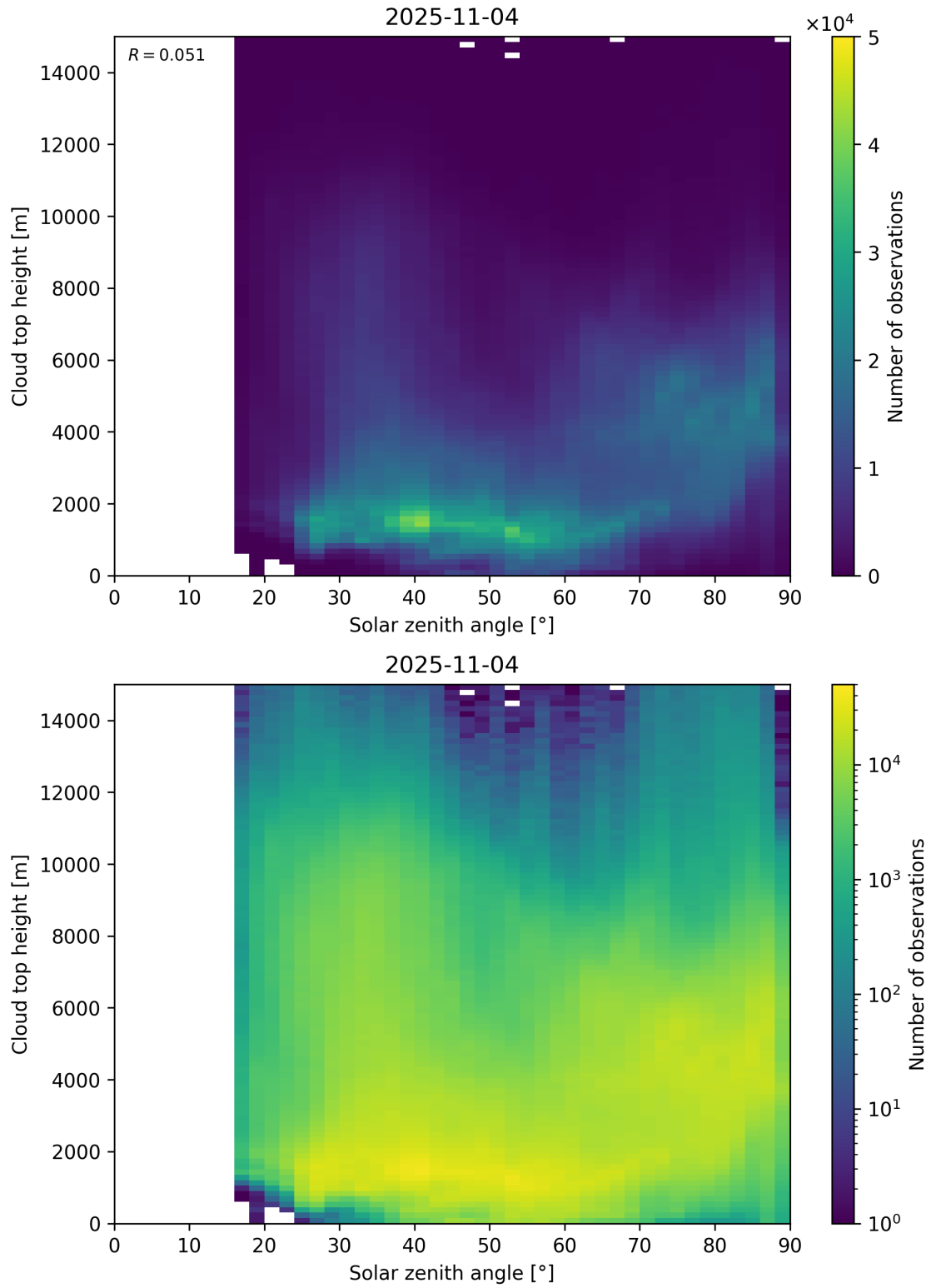
Figure 104: Scatter density plot of “Solar zenith angle” against “Cloud top height” for 2025-11-03 to 2025-11-05.
