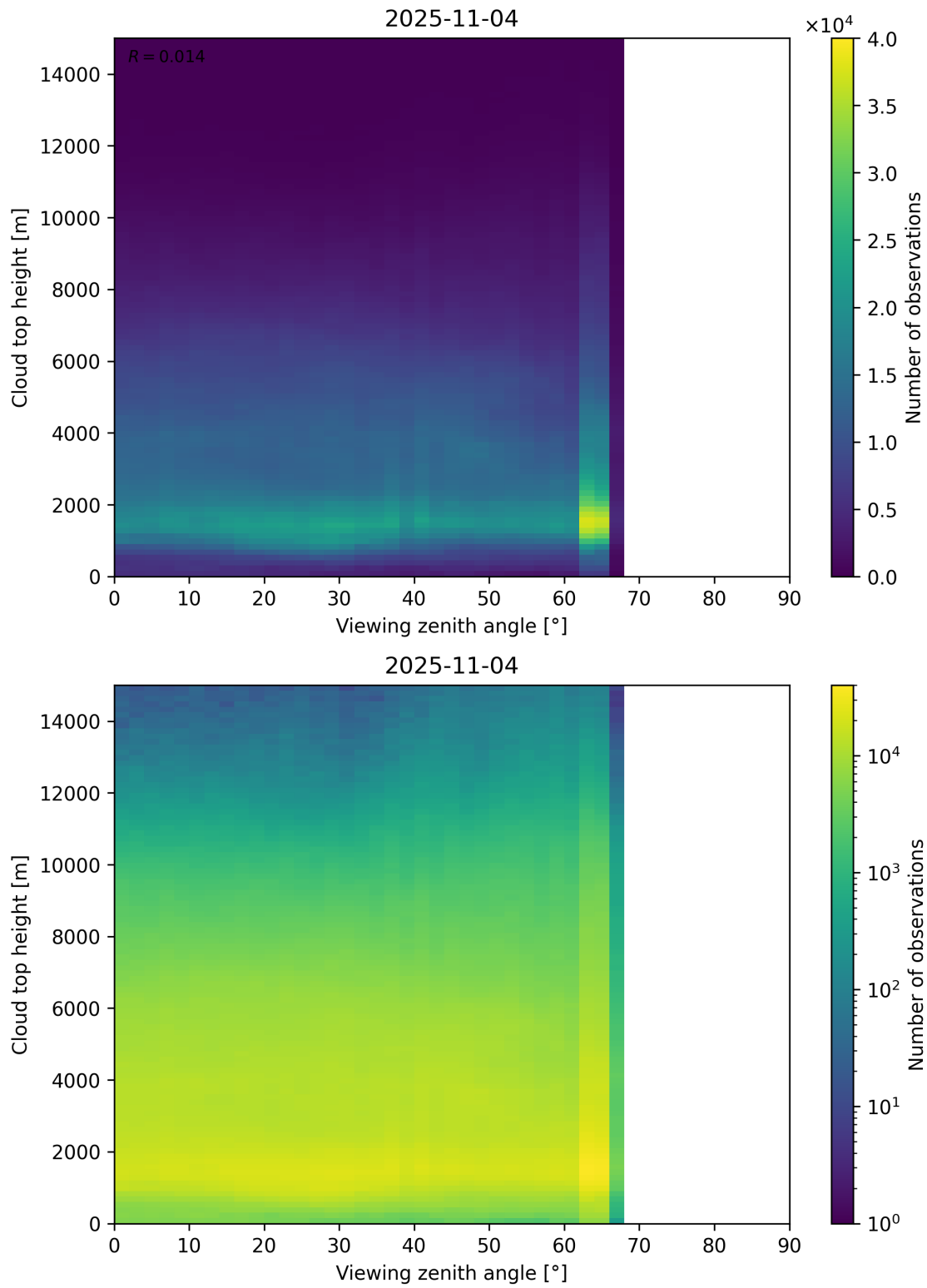
Figure 112: Scatter density plot of “Viewing zenith angle” against “Cloud top height” for 2025-11-03 to 2025-11-05.
