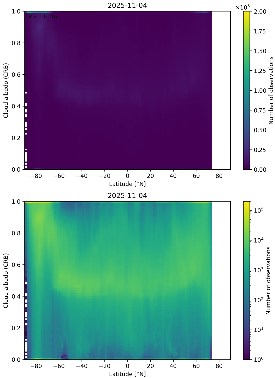
Figure 91: Scatter density plot of “Latitude” against “Cloud albedo (CRB)” for 2025-11-03 to 2025-11-05.
