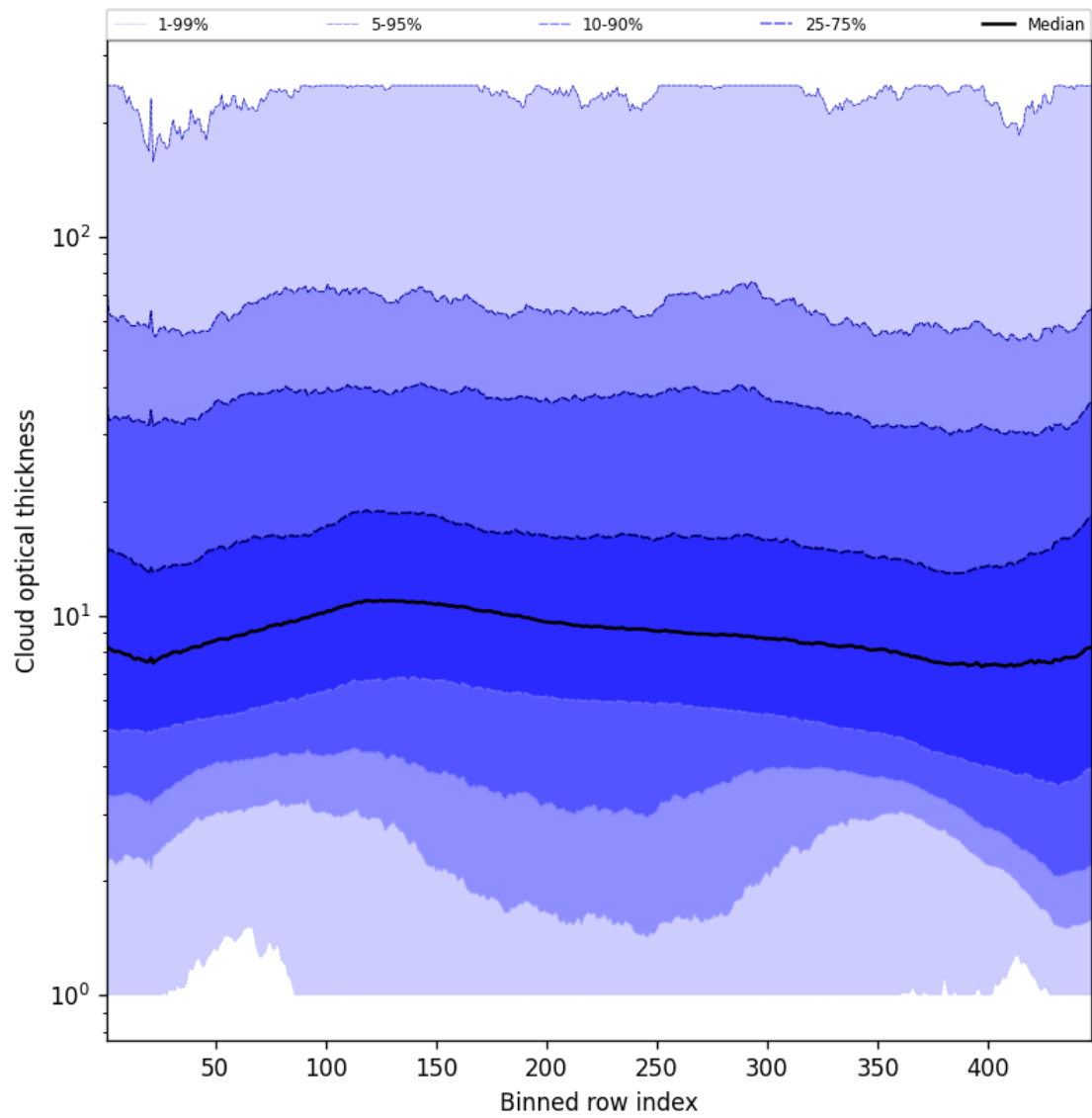
Figure 57: Along track statistics of “Cloud optical thickness” for 2025-11-03 to 2025-11-05
