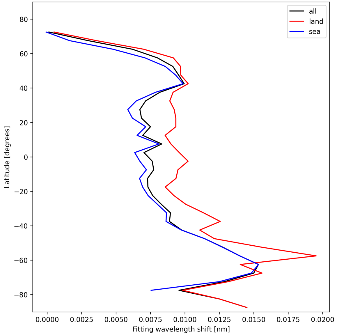
Figure 33: Zonal average of “Fitting wavelength shift” for 2025-11-03 to 2025-11-05.
