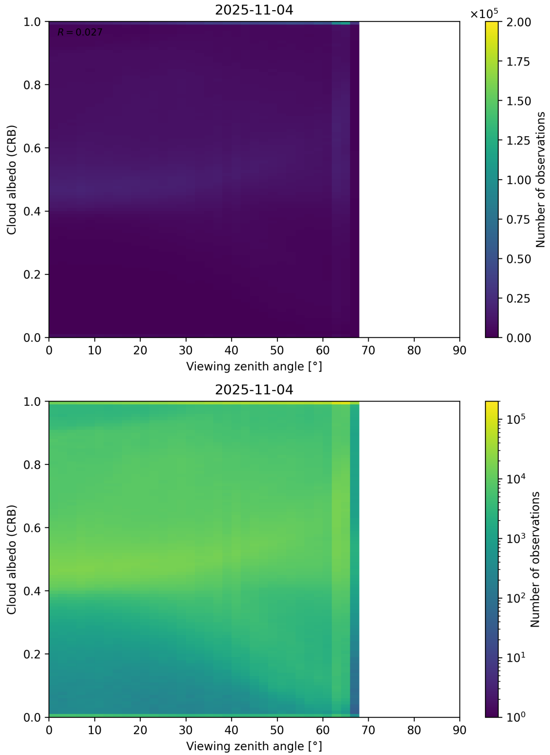
Figure 106: Scatter density plot of “Viewing zenith angle” against “Cloud albedo (CRB)” for 2025-11-03 to 2025-11-05.
