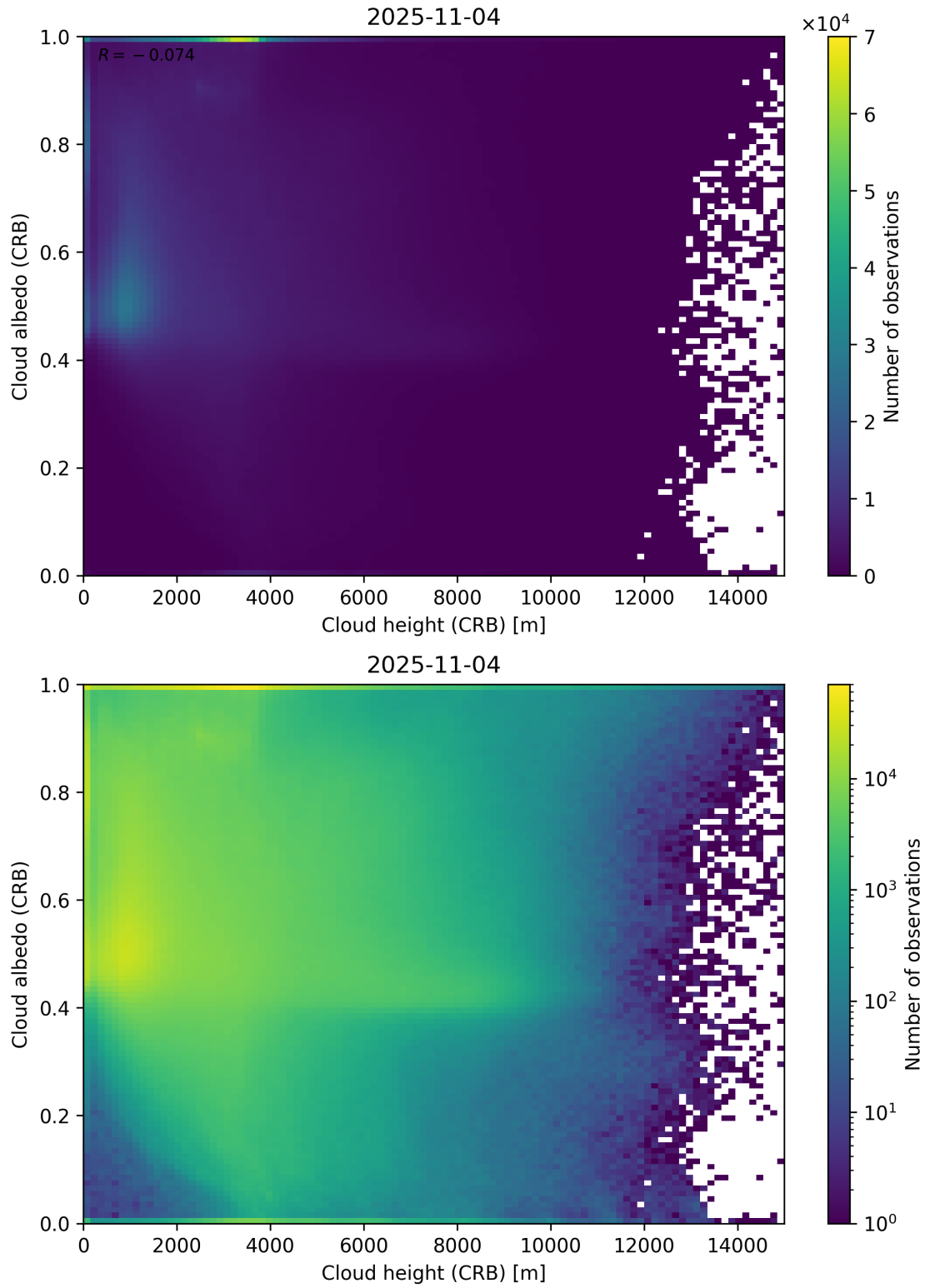
Figure 80: Scatter density plot of “Cloud height (CRB)” against “Cloud albedo (CRB)” for 2025-11-03 to 2025-11-05.
