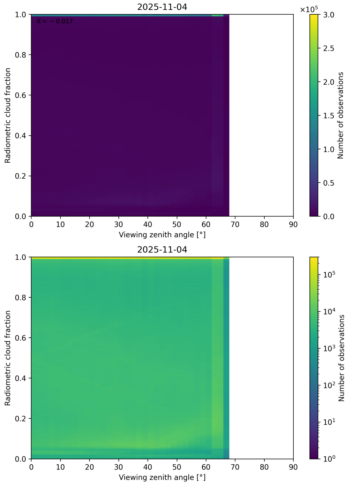
Figure 107: Scatter density plot of “Viewing zenith angle” against “Radiometric cloud fraction” for 2025-11-03 to 2025-11-05.
