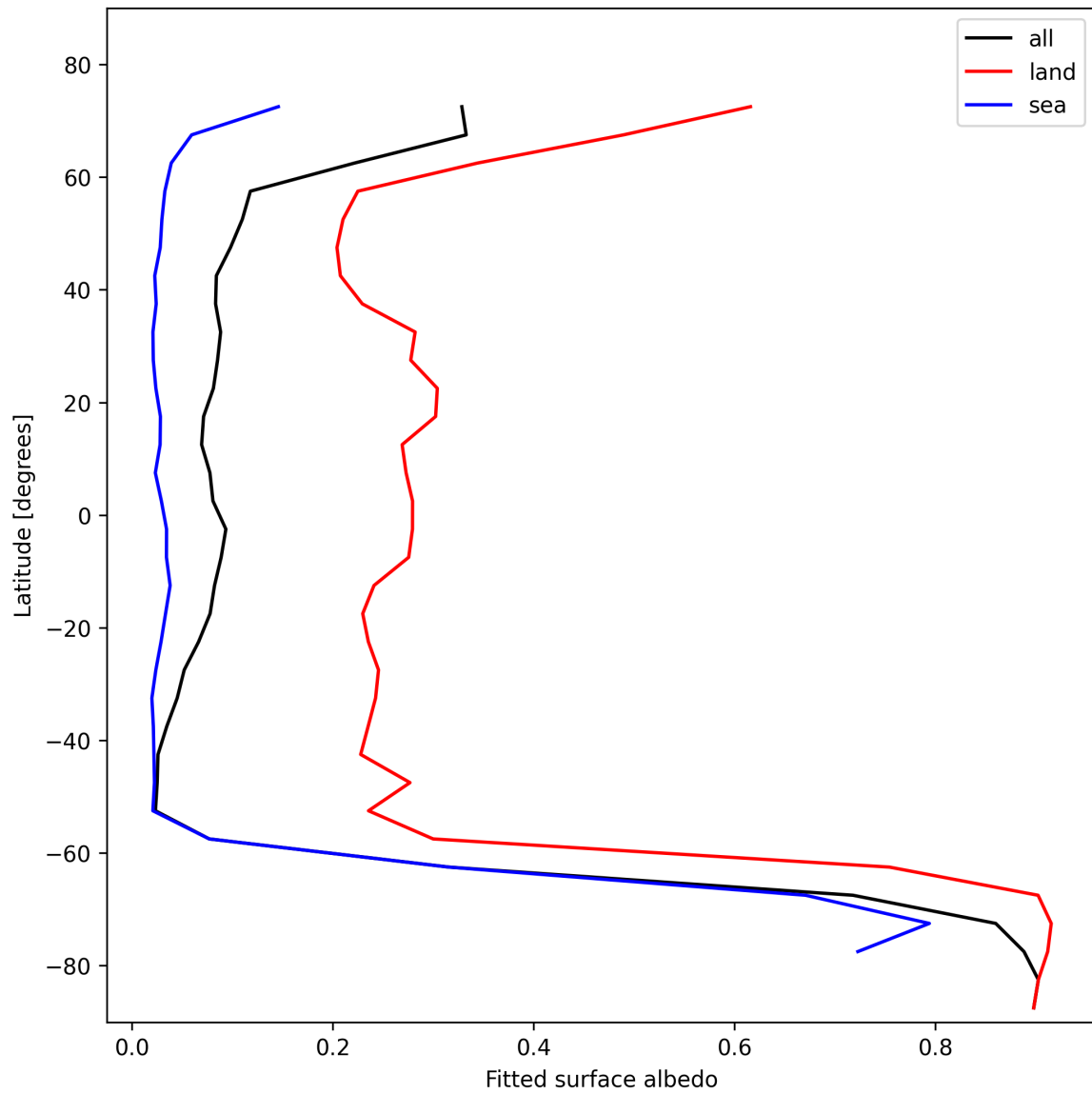
Figure 29: Zonal average of “Fitted surface albedo” for 2025-11-03 to 2025-11-05.
