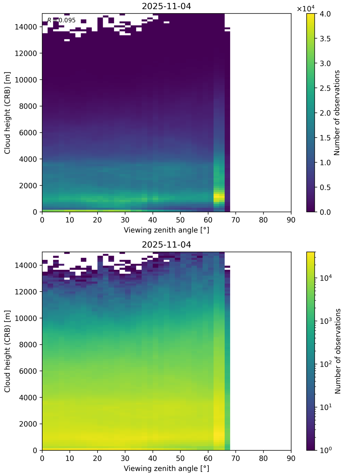
Figure 110: Scatter density plot of “Viewing zenith angle” against “Cloud height (CRB)” for 2025-11-03 to 2025-11-05.
