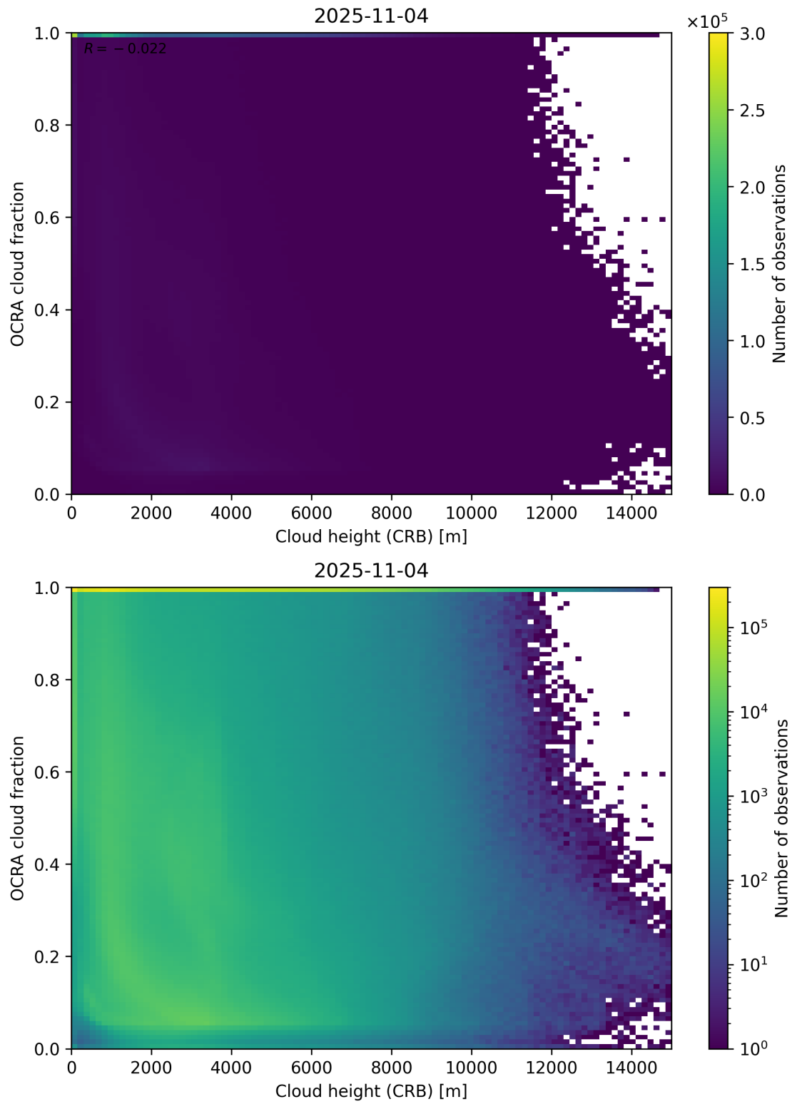
Figure 81: Scatter density plot of “Cloud height (CRB)” against “OCRA cloud fraction” for 2025-11-03 to 2025-11-05.
