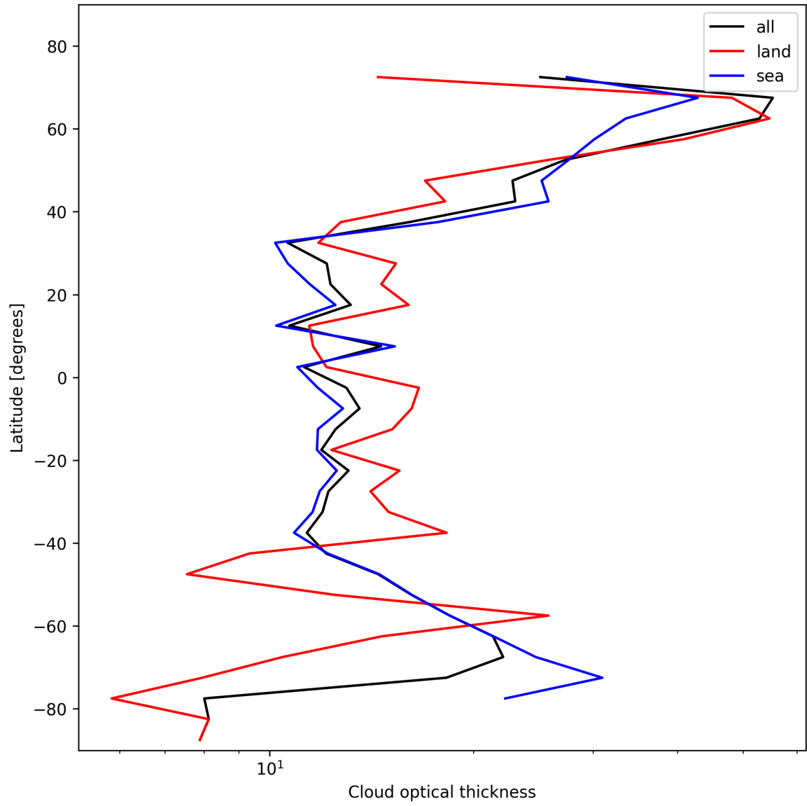
Figure 25: Zonal average of “Cloud optical thickness” for 2025-11-03 to 2025-11-05.
