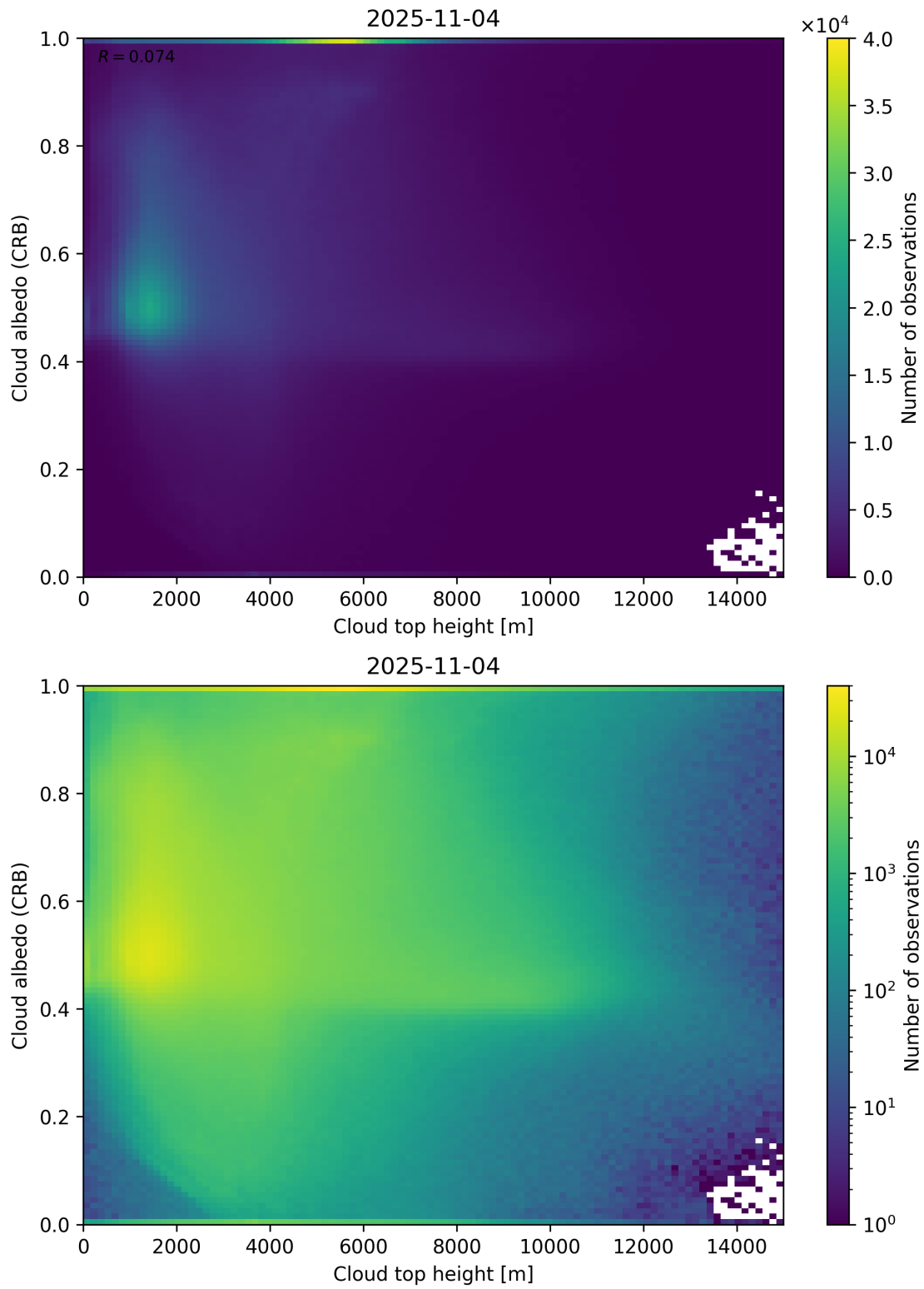
Figure 86: Scatter density plot of “Cloud top height” against “Cloud albedo (CRB)” for 2025-11-03 to 2025-11-05.
