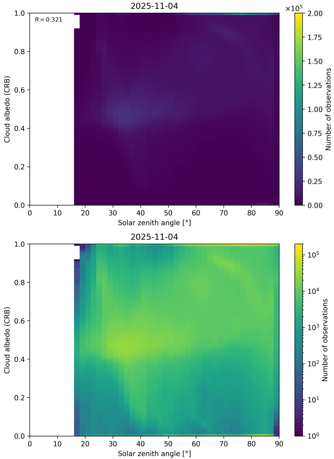
Figure 98: Scatter density plot of “Solar zenith angle” against “Cloud albedo (CRB)” for 2025-11-03 to 2025-11-05.
