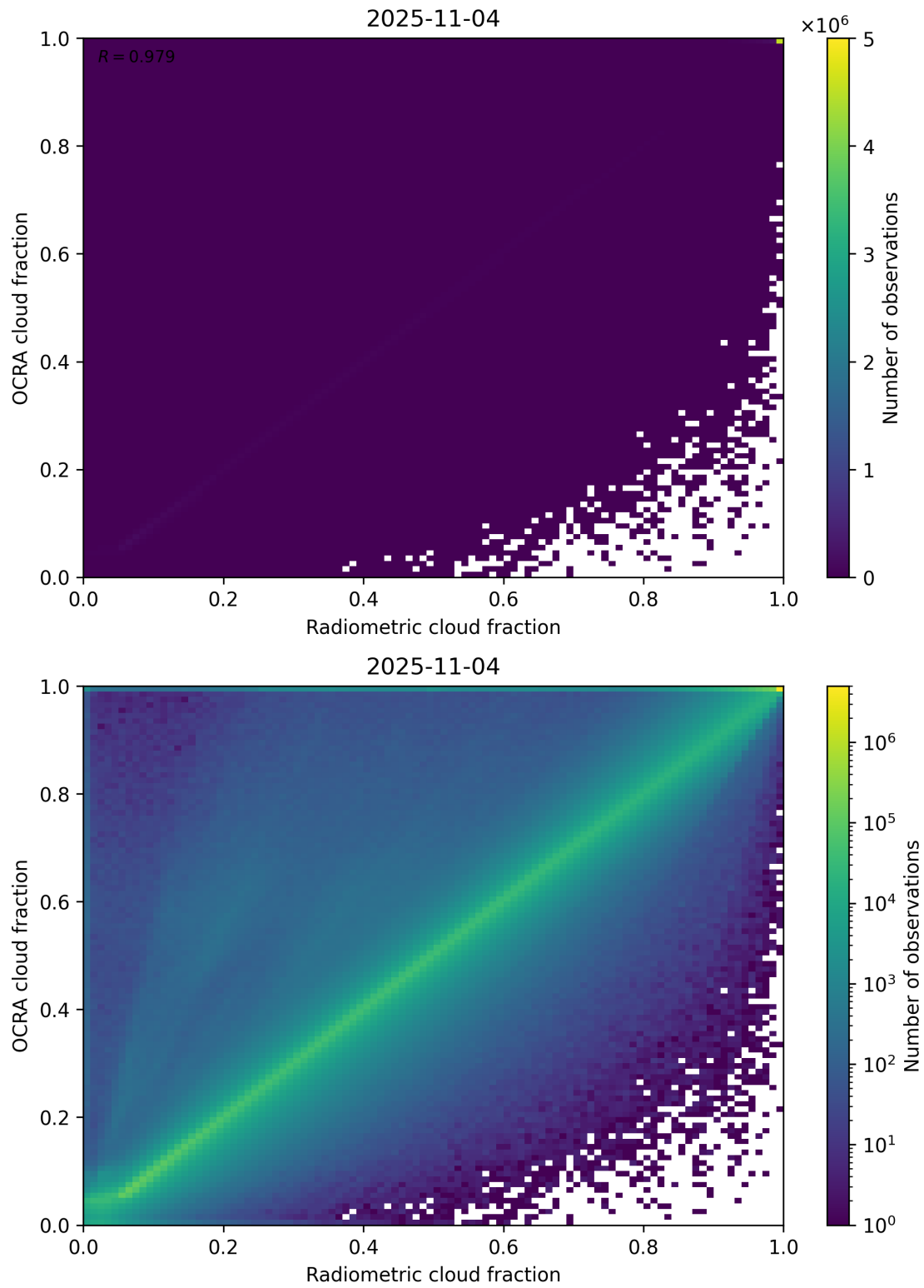
Figure 72: Scatter density plot of “Radiometric cloud fraction” against “OCRA cloud fraction” for 2025-11-03 to 2025-11-05.
