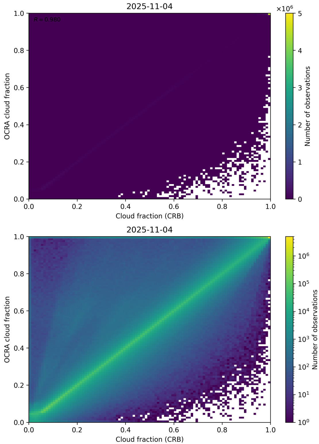
Figure 78: Scatter density plot of “Cloud fraction (CRB)” against “OCRA cloud fraction” for 2025-11-03 to 2025-11-05.
