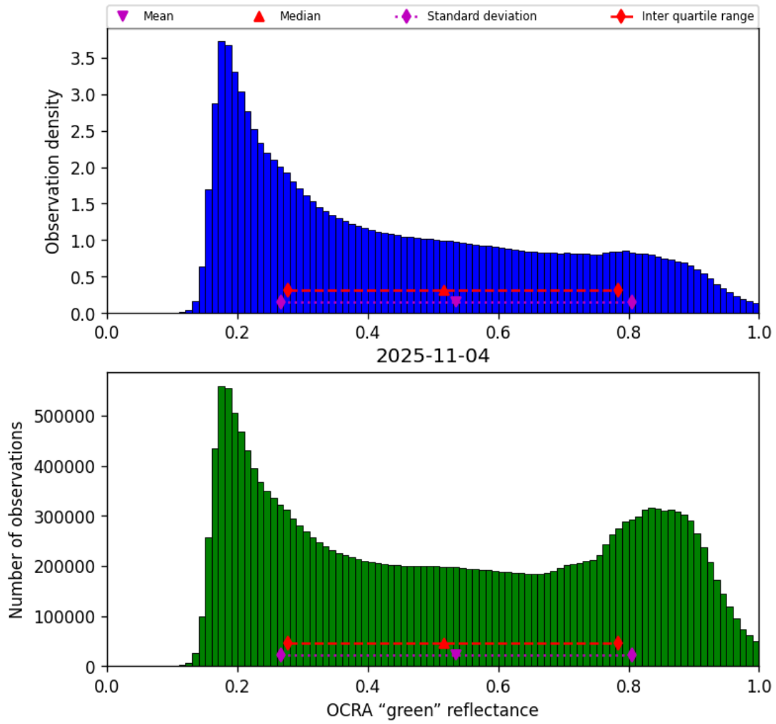
Figure 52: Histogram of “OCRA “green” reflectance” for 2025-11-03 to 2025-11-05
