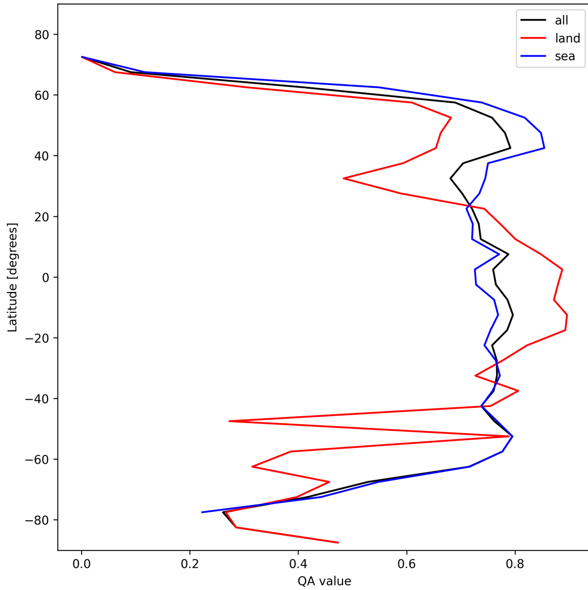
Figure 22: Zonal average of “QA value” for 2025-11-03 to 2025-11-05.
