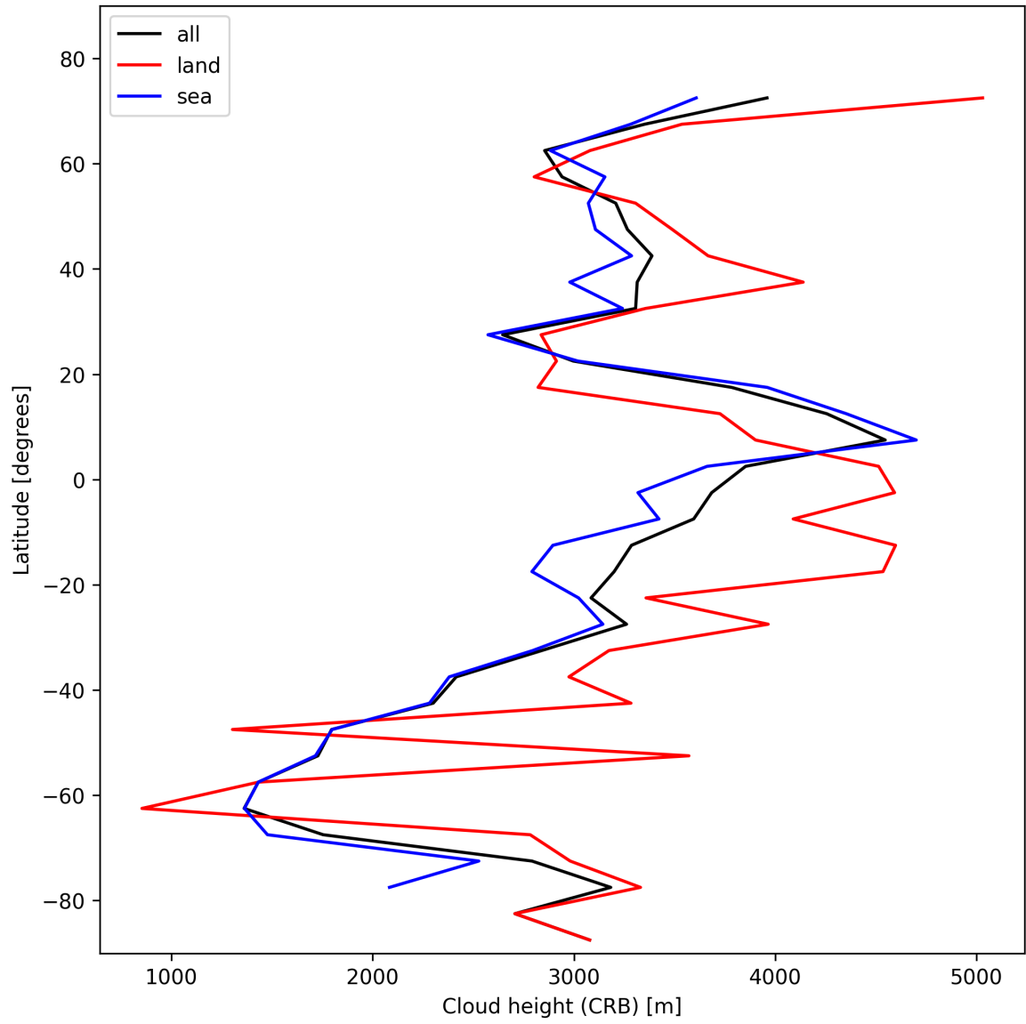
Figure 27: Zonal average of “Cloud height (CRB)” for 2025-11-03 to 2025-11-05.
