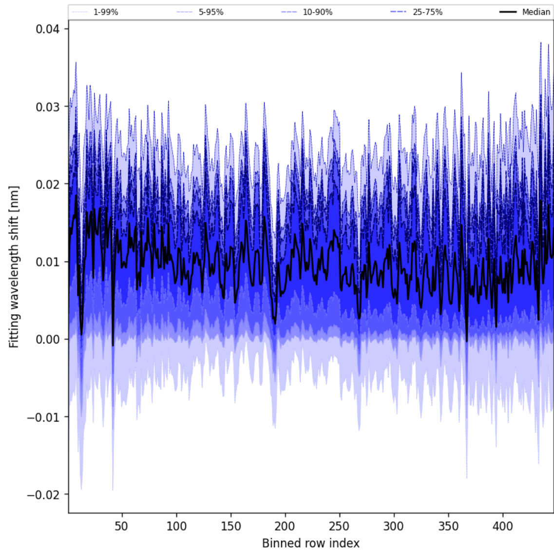
Figure 65: Along track statistics of “Fitting wavelength shift” for 2025-11-03 to 2025-11-05
