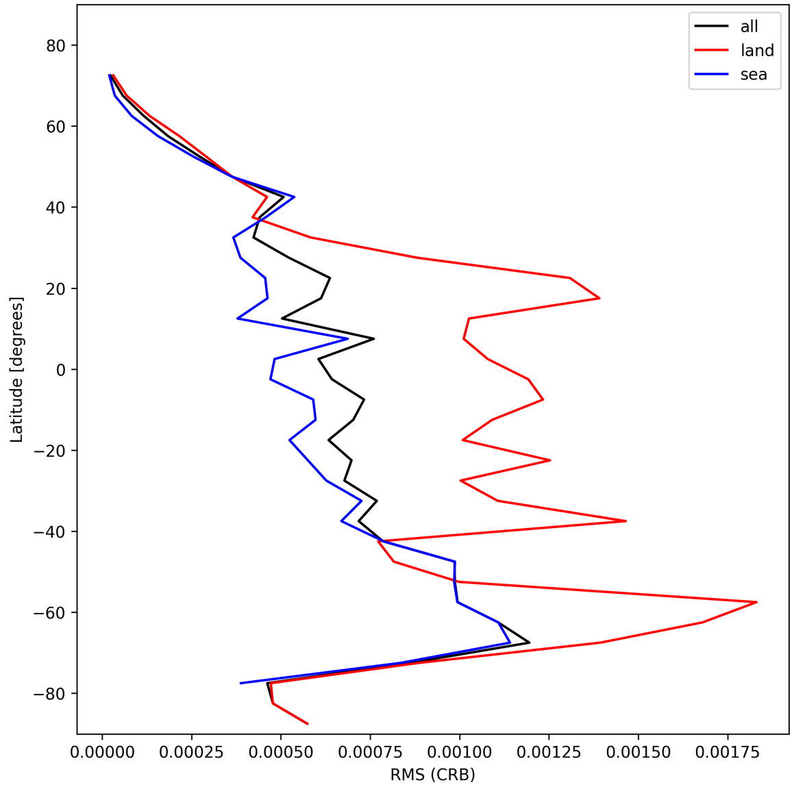
Figure 32: Zonal average of “RMS (CRB)” for 2025-11-03 to 2025-11-05.
