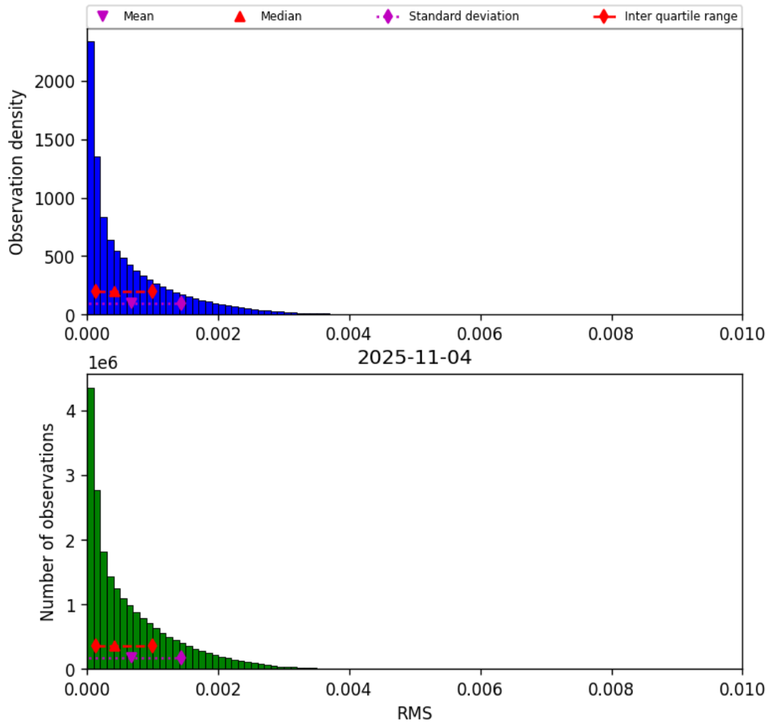
Figure 47: Histogram of “RMS” for 2025-11-03 to 2025-11-05
