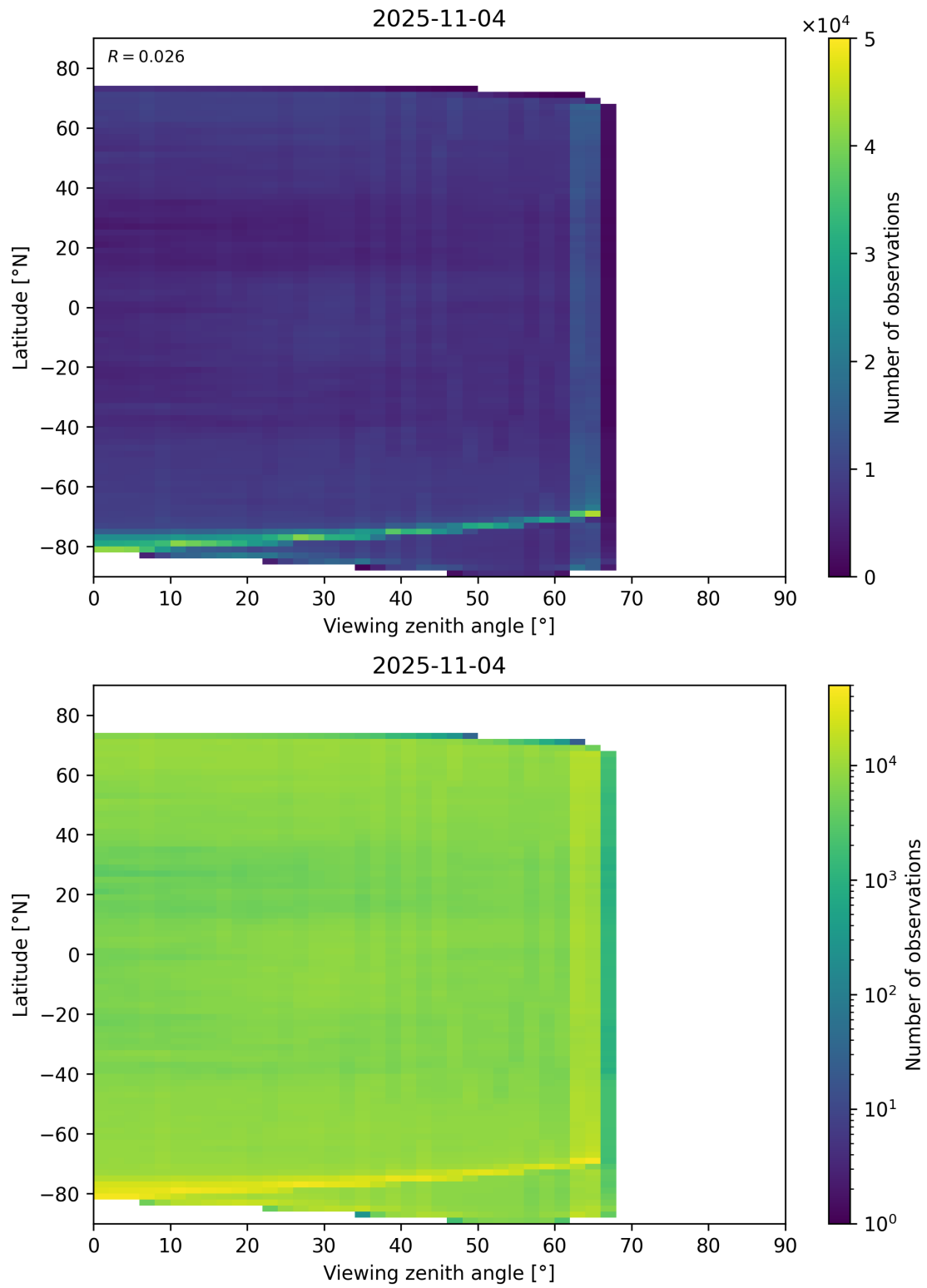
Figure 113: Scatter density plot of “Viewing zenith angle” against “Latitude” for 2025-11-03 to 2025-11-05.
