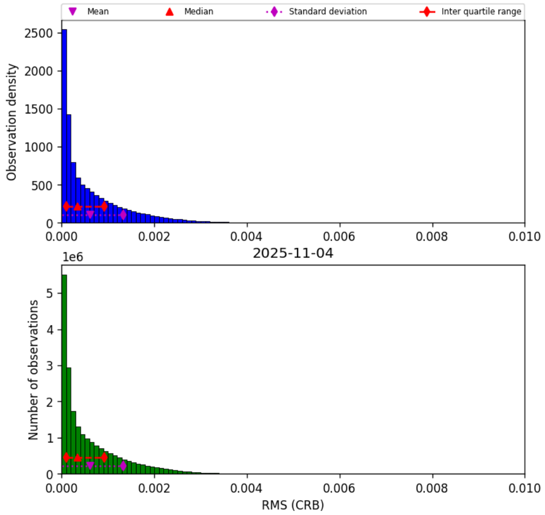
Figure 48: Histogram of “RMS (CRB)” for 2025-11-03 to 2025-11-05
