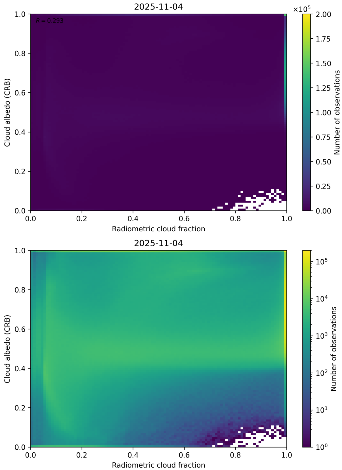
Figure 71: Scatter density plot of “Radiometric cloud fraction” against “Cloud albedo (CRB)” for 2025-11-03 to 2025-11-05.
