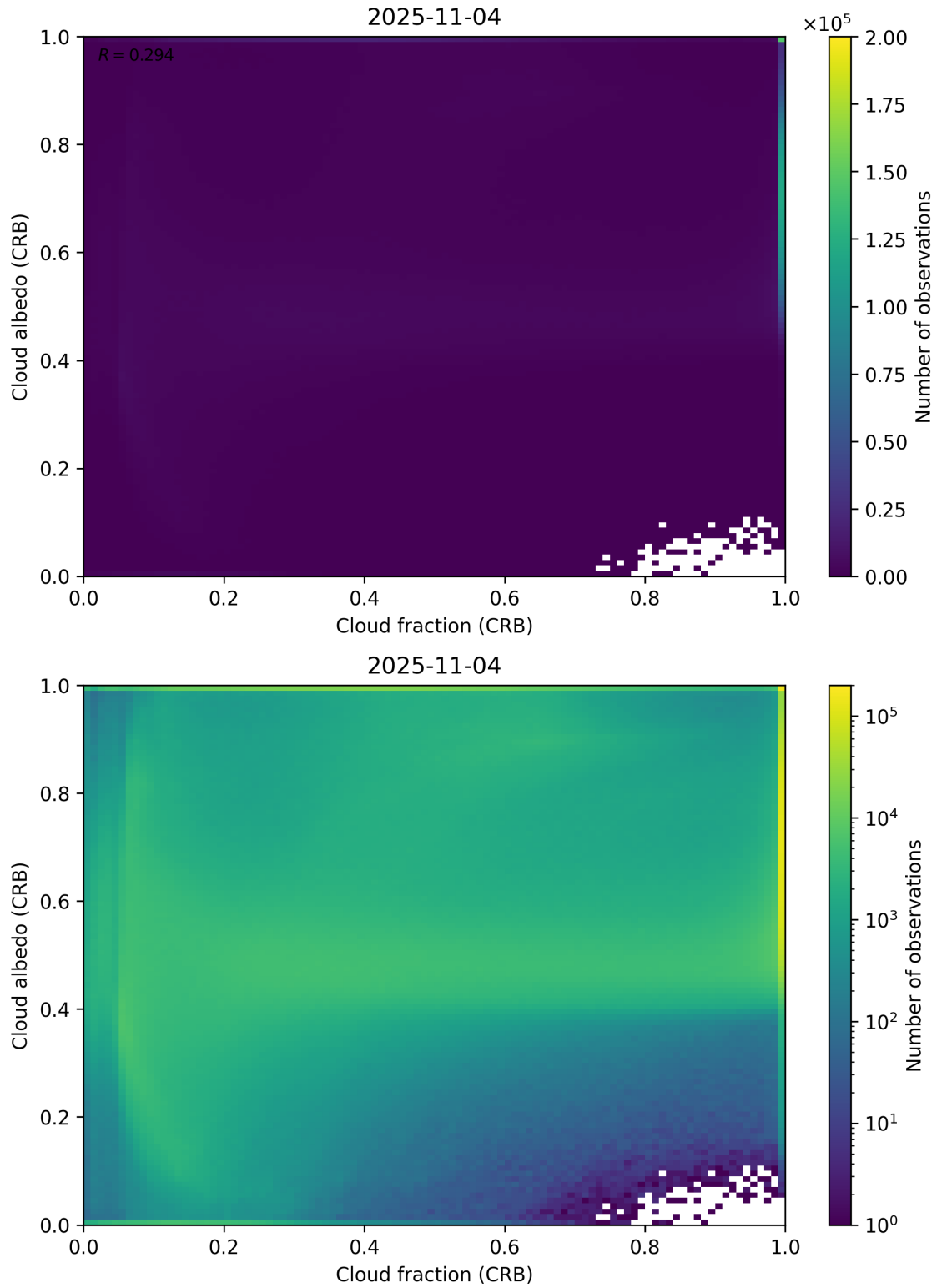
Figure 77: Scatter density plot of “Cloud fraction (CRB)” against “Cloud albedo (CRB)” for 2025-11-03 to 2025-11-05.
