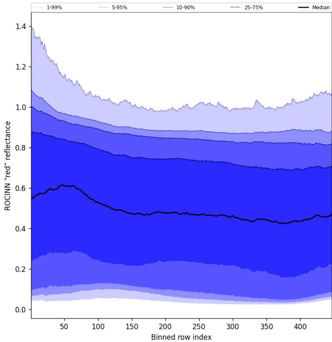
Figure 69: Along track statistics of “ROCINN “red” reflectance” for 2025-11-03 to 2025-11-05
