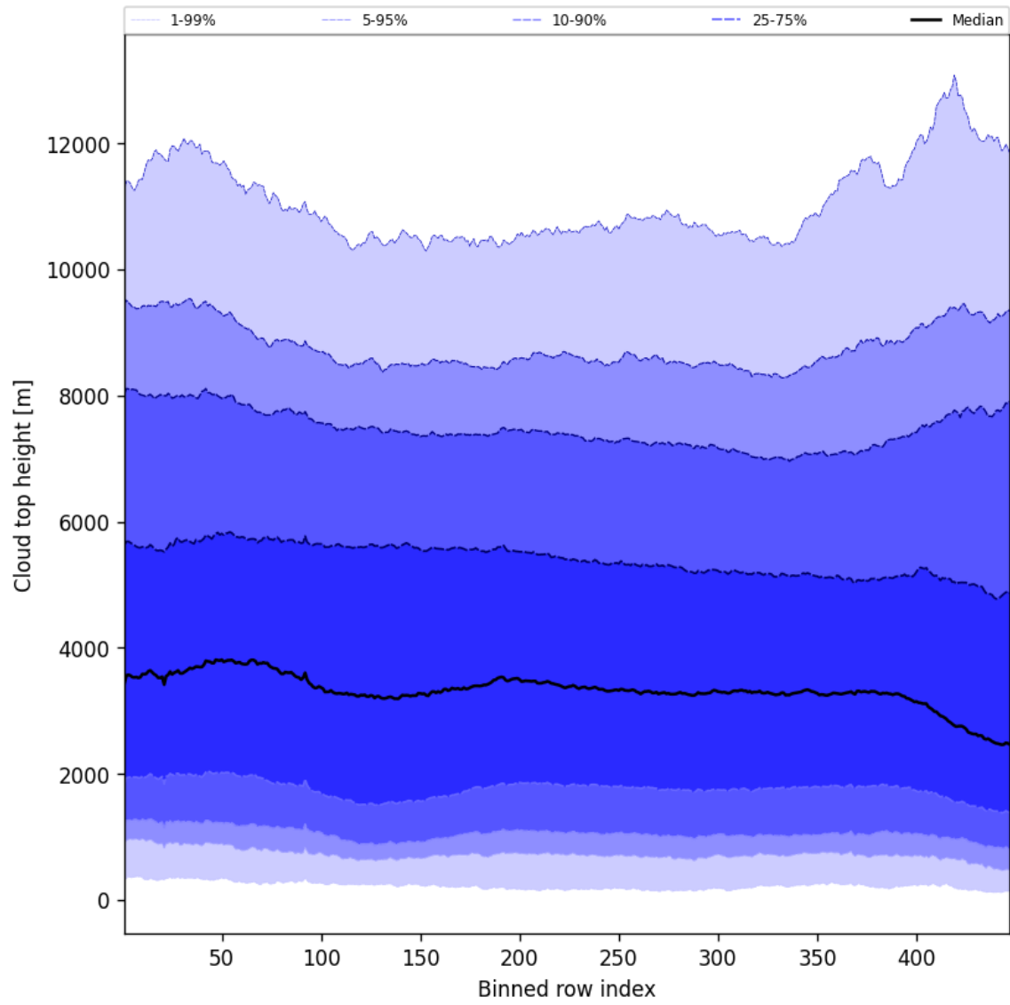
Figure 56: Along track statistics of “Cloud top height” for 2025-11-03 to 2025-11-05
