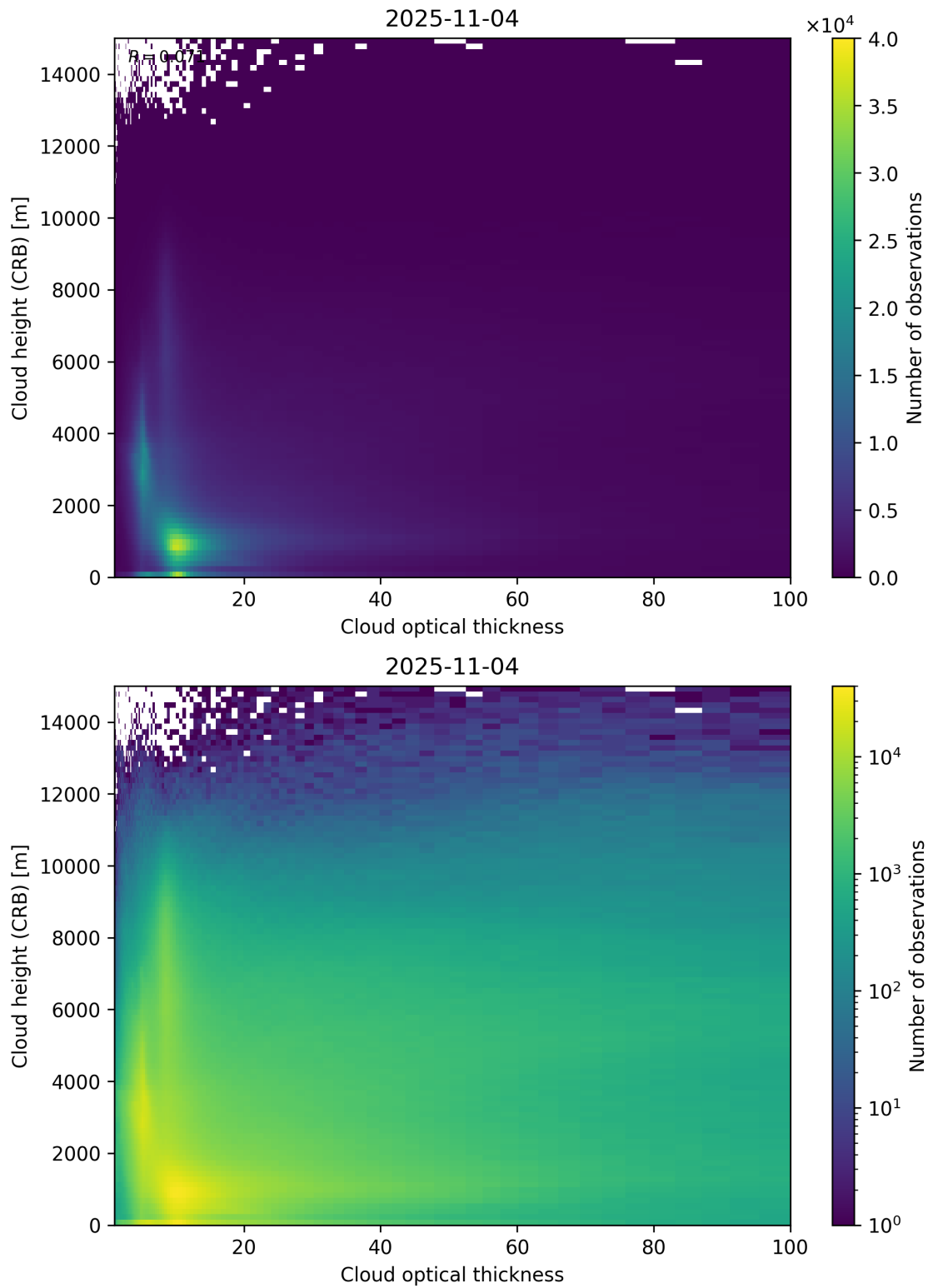
Figure 85: Scatter density plot of “Cloud optical thickness” against “Cloud height (CRB)” for 2025-11-03 to 2025-11-05.
