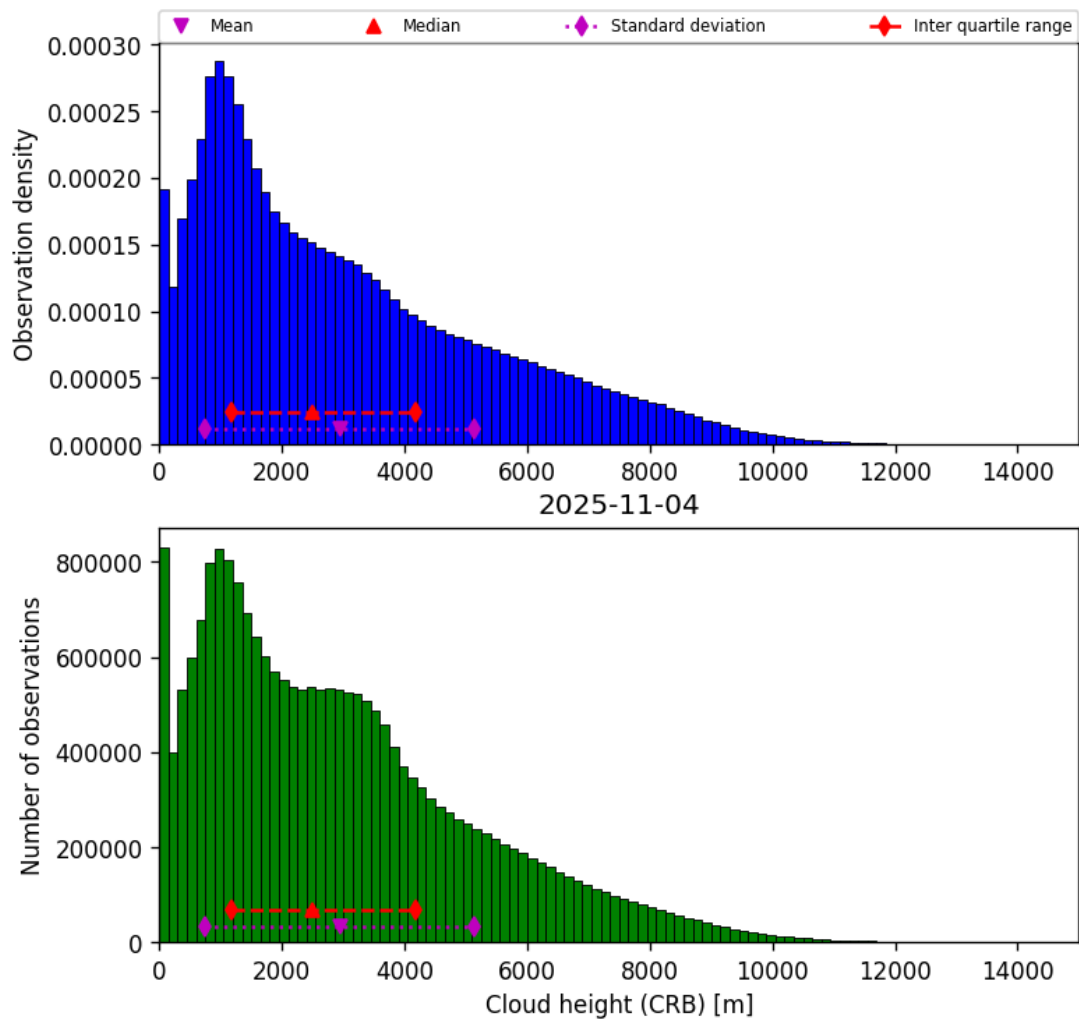
Figure 43: Histogram of “Cloud height (CRB)” for 2025-11-03 to 2025-11-05
