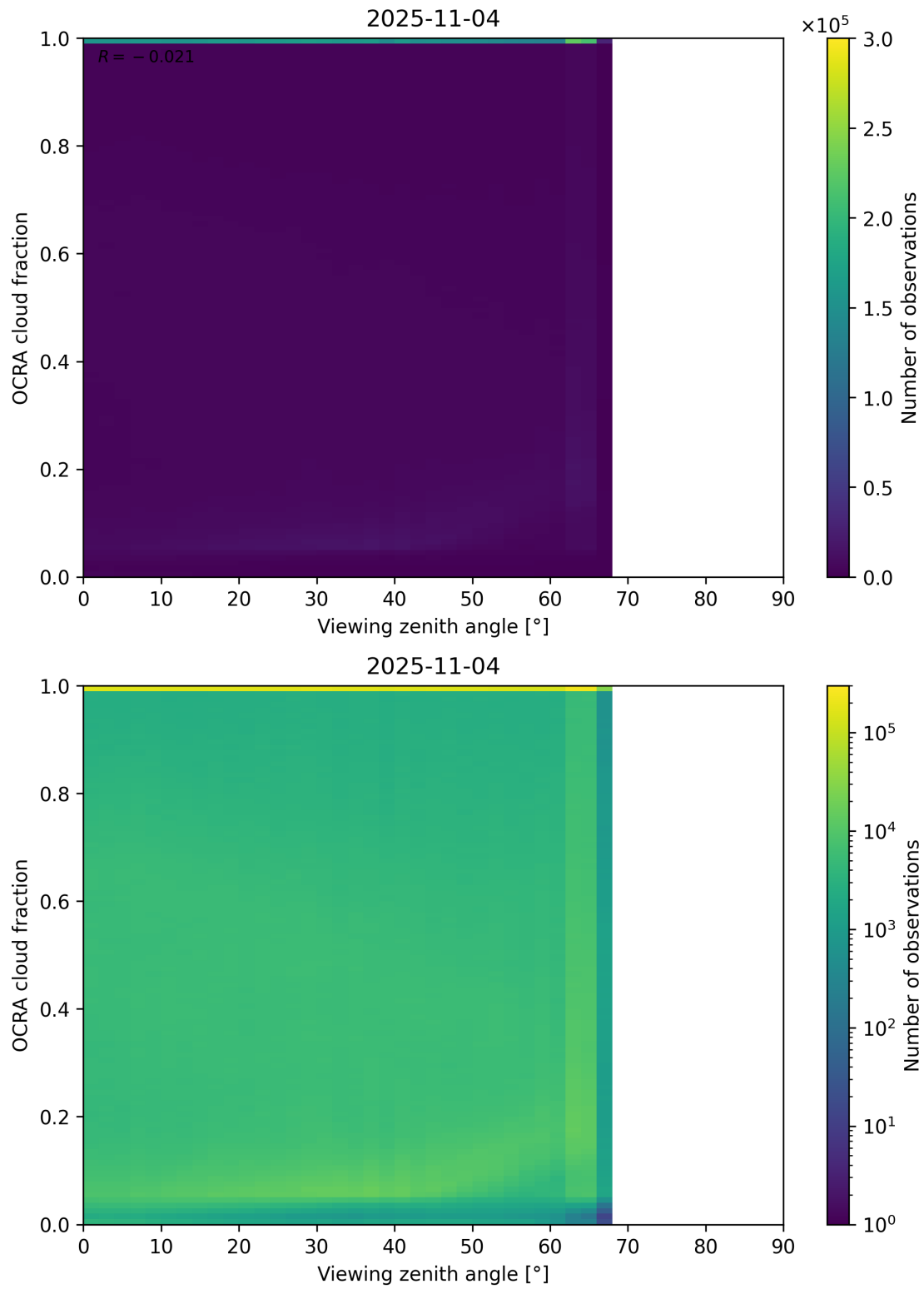
Figure 108: Scatter density plot of “Viewing zenith angle” against “OCRA cloud fraction” for 2025-11-03 to 2025-11-05.
