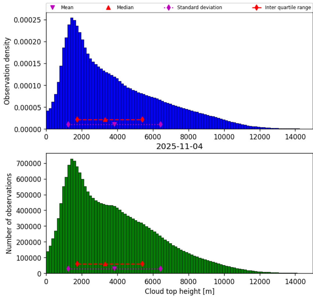
Figure 40: Histogram of “Cloud top height” for 2025-11-03 to 2025-11-05
