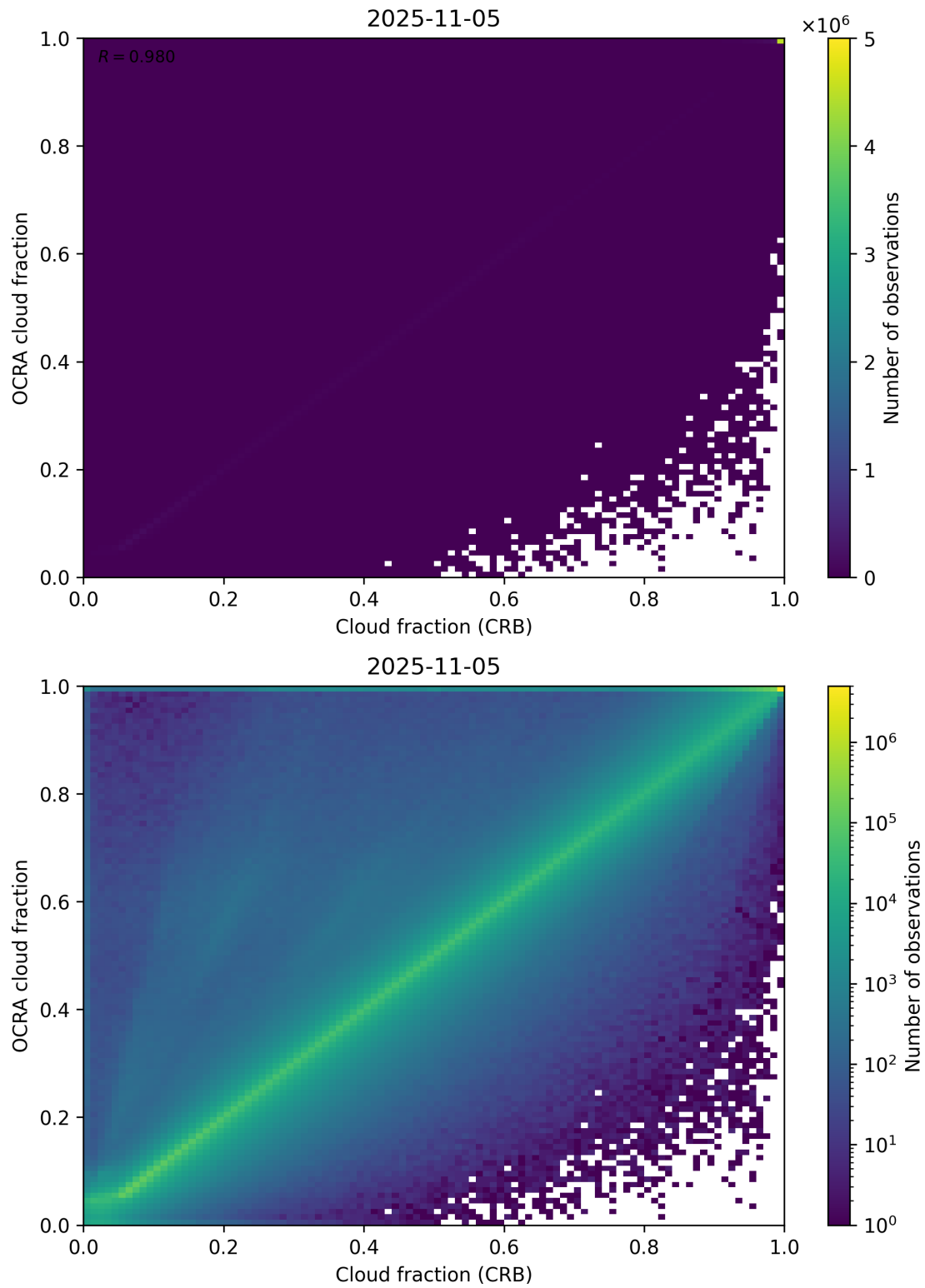
Figure 78: Scatter density plot of “Cloud fraction (CRB)” against “OCRA cloud fraction” for 2025-11-04 to 2025-11-06.
