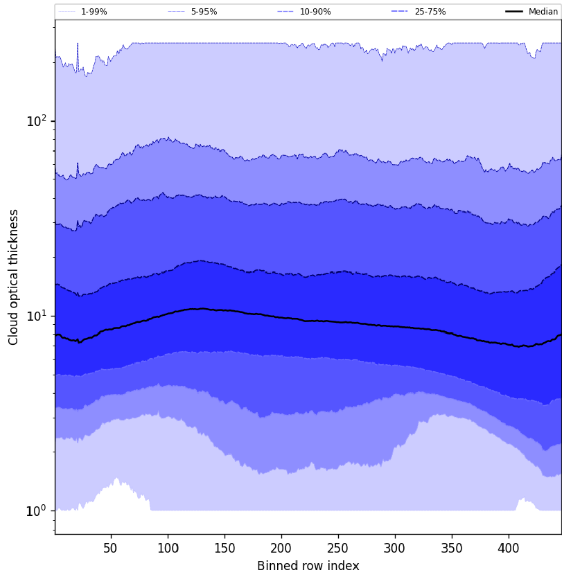
Figure 57: Along track statistics of “Cloud optical thickness” for 2025-11-04 to 2025-11-06
