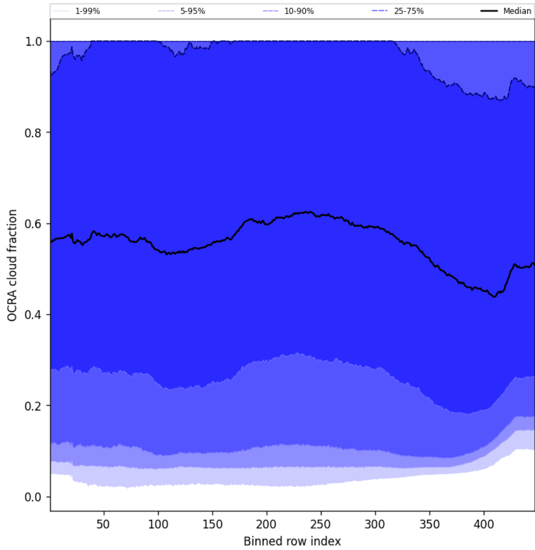
Figure 66: Along track statistics of “OCRA cloud fraction” for 2025-11-04 to 2025-11-06
