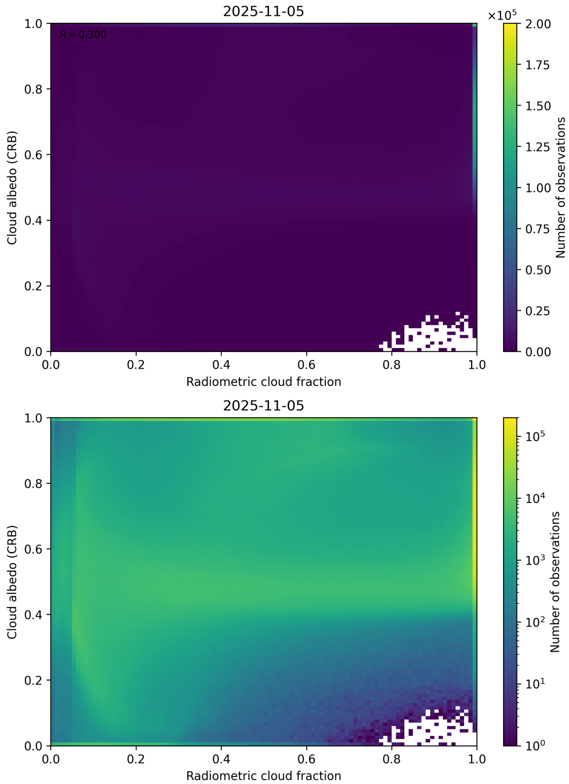
Figure 71: Scatter density plot of “Radiometric cloud fraction” against “Cloud albedo (CRB)” for 2025-11-04 to 2025-11-06.
