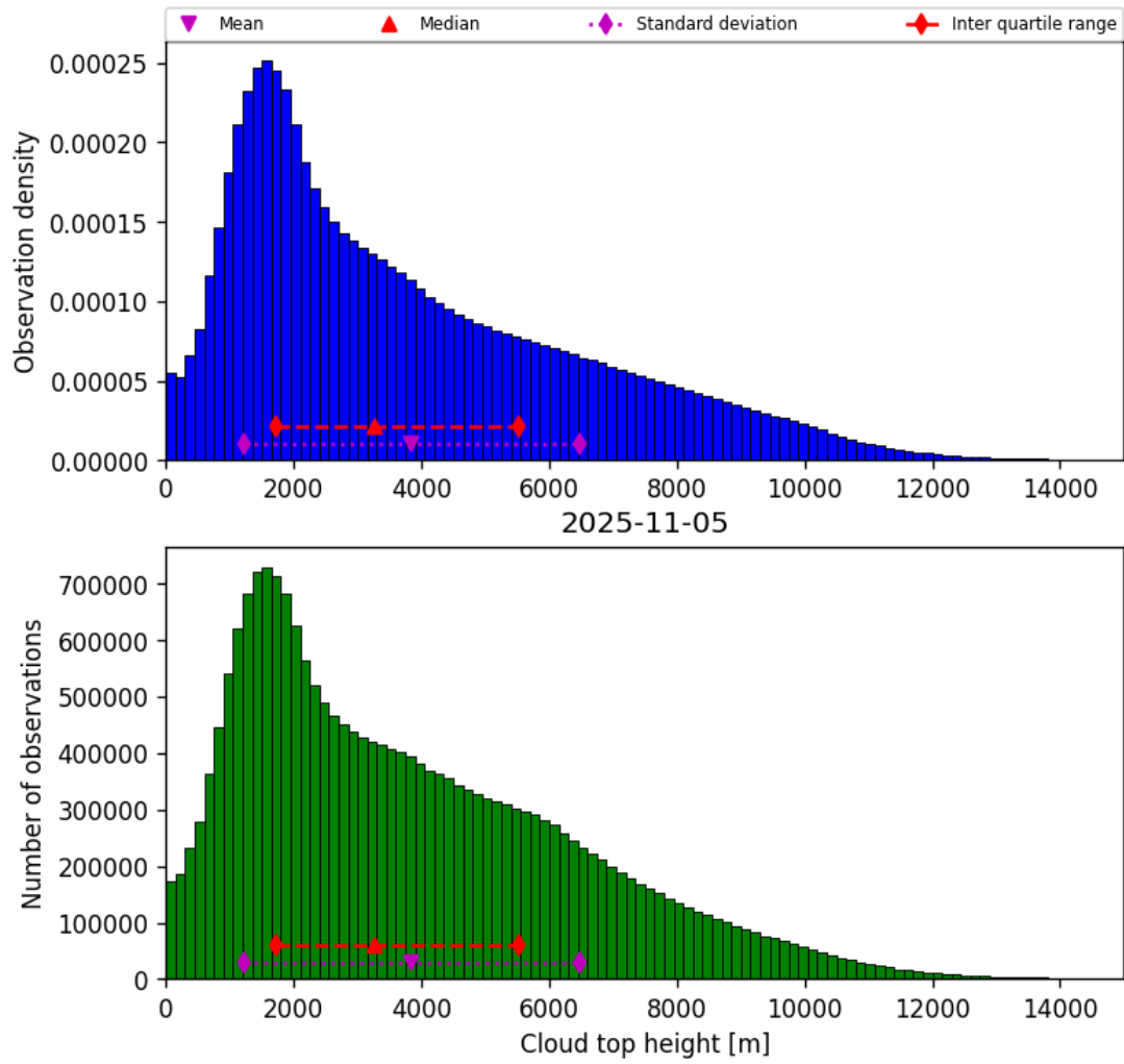
Figure 40: Histogram of “Cloud top height” for 2025-11-04 to 2025-11-06
