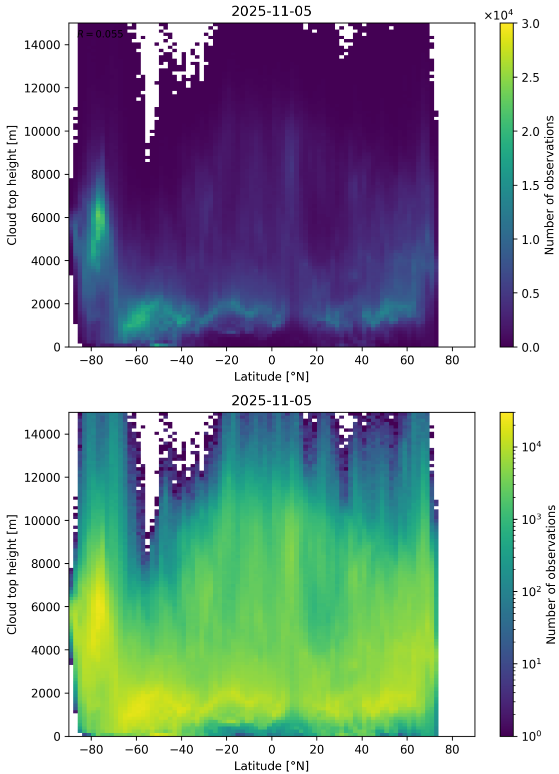
Figure 97: Scatter density plot of “Latitude” against “Cloud top height” for 2025-11-04 to 2025-11-06.
