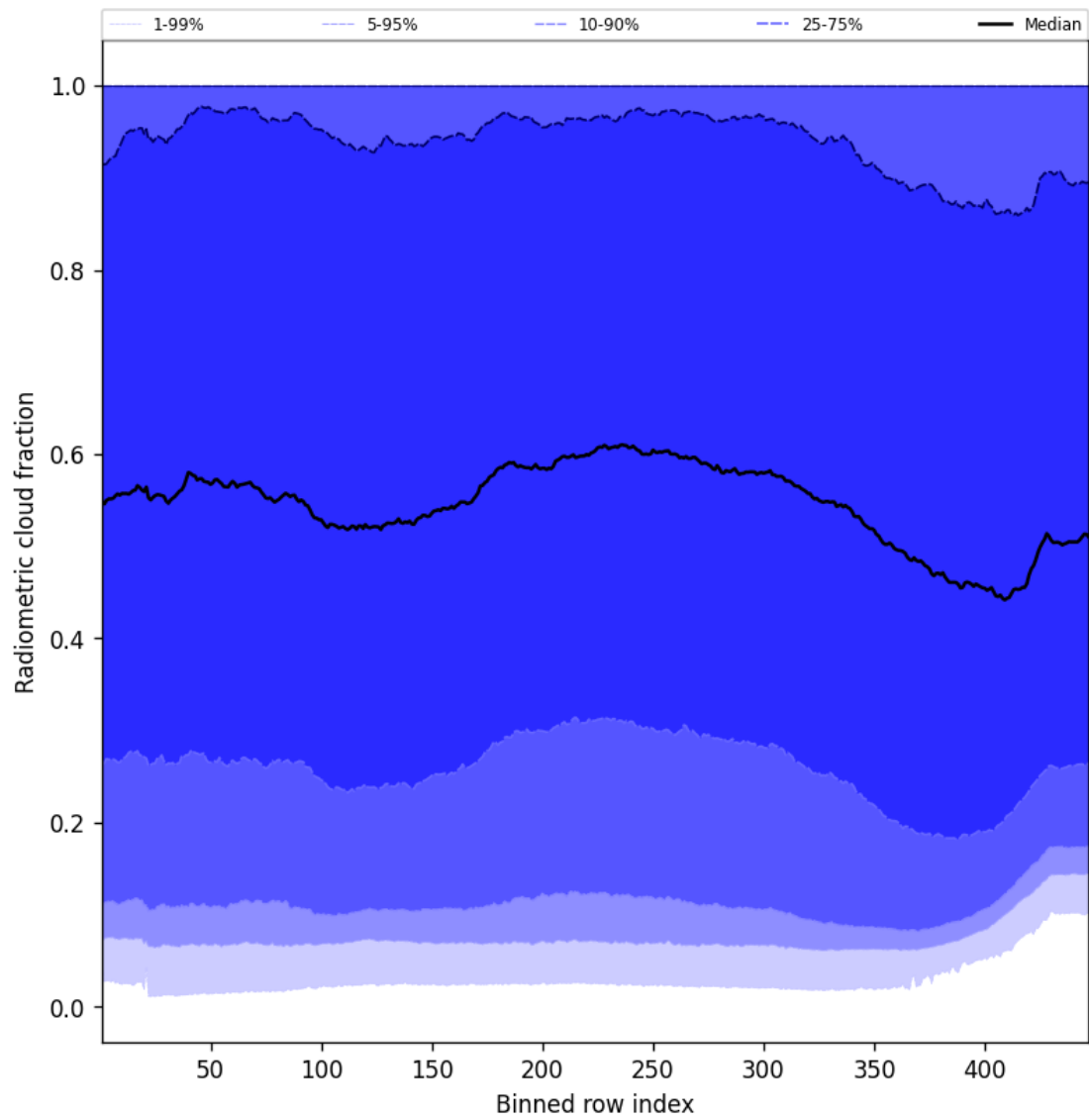
Figure 55: Along track statistics of “Radiometric cloud fraction” for 2025-11-04 to 2025-11-06
