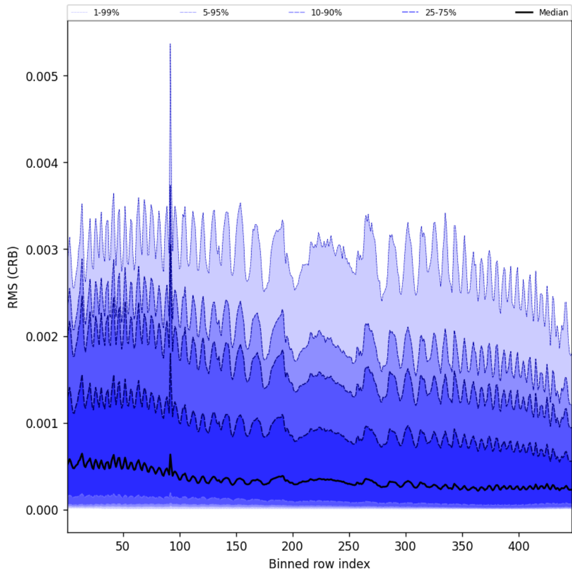
Figure 64: Along track statistics of “RMS (CRB)” for 2025-11-04 to 2025-11-06
