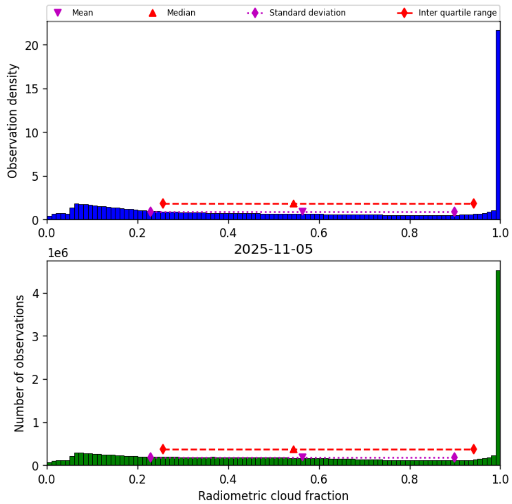
Figure 39: Histogram of “Radiometric cloud fraction” for 2025-11-04 to 2025-11-06
