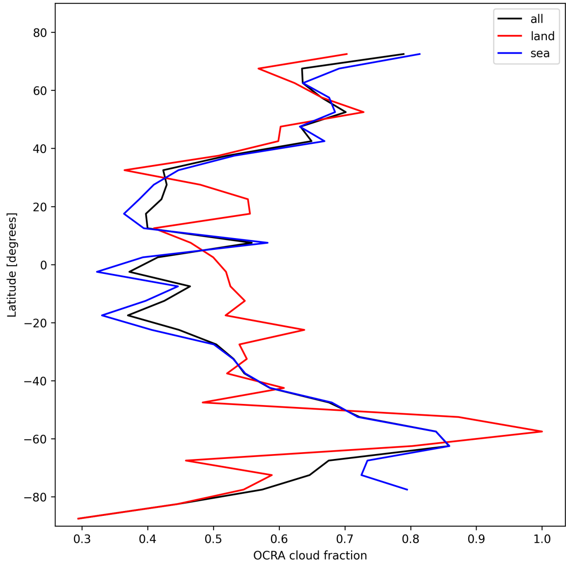
Figure 34: Zonal average of “OCRA cloud fraction” for 2025-11-04 to 2025-11-06.
