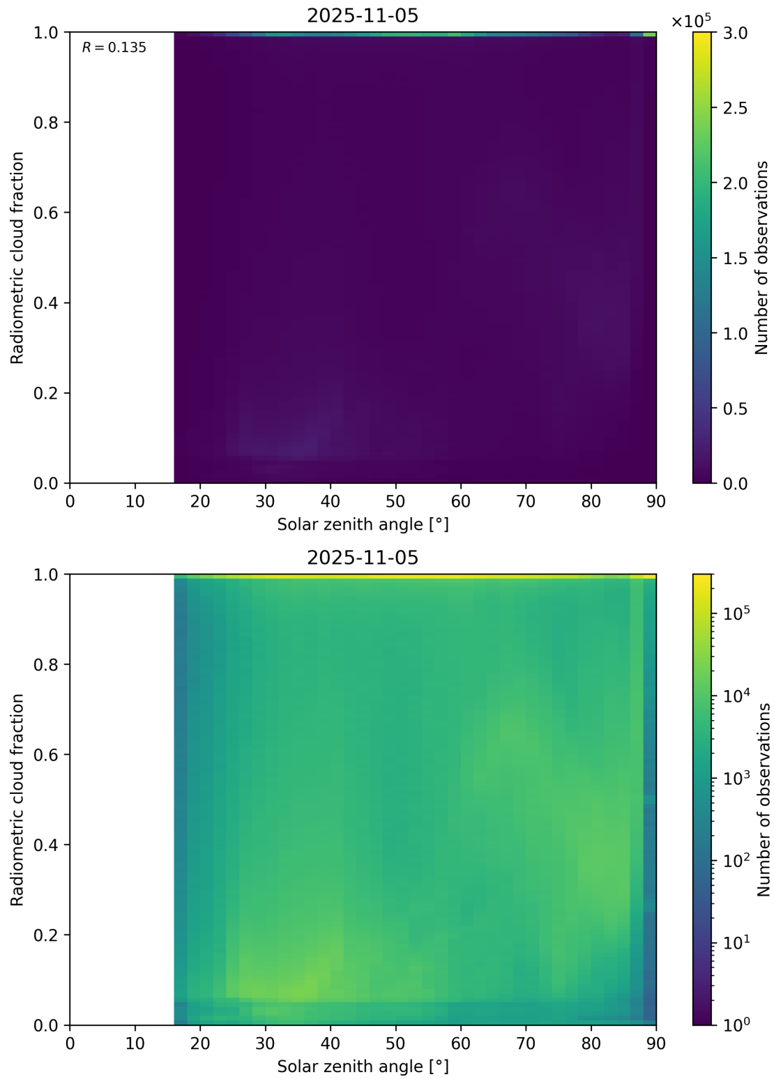
Figure 99: Scatter density plot of “Solar zenith angle” against “Radiometric cloud fraction” for 2025-11-04 to 2025-11-06.
