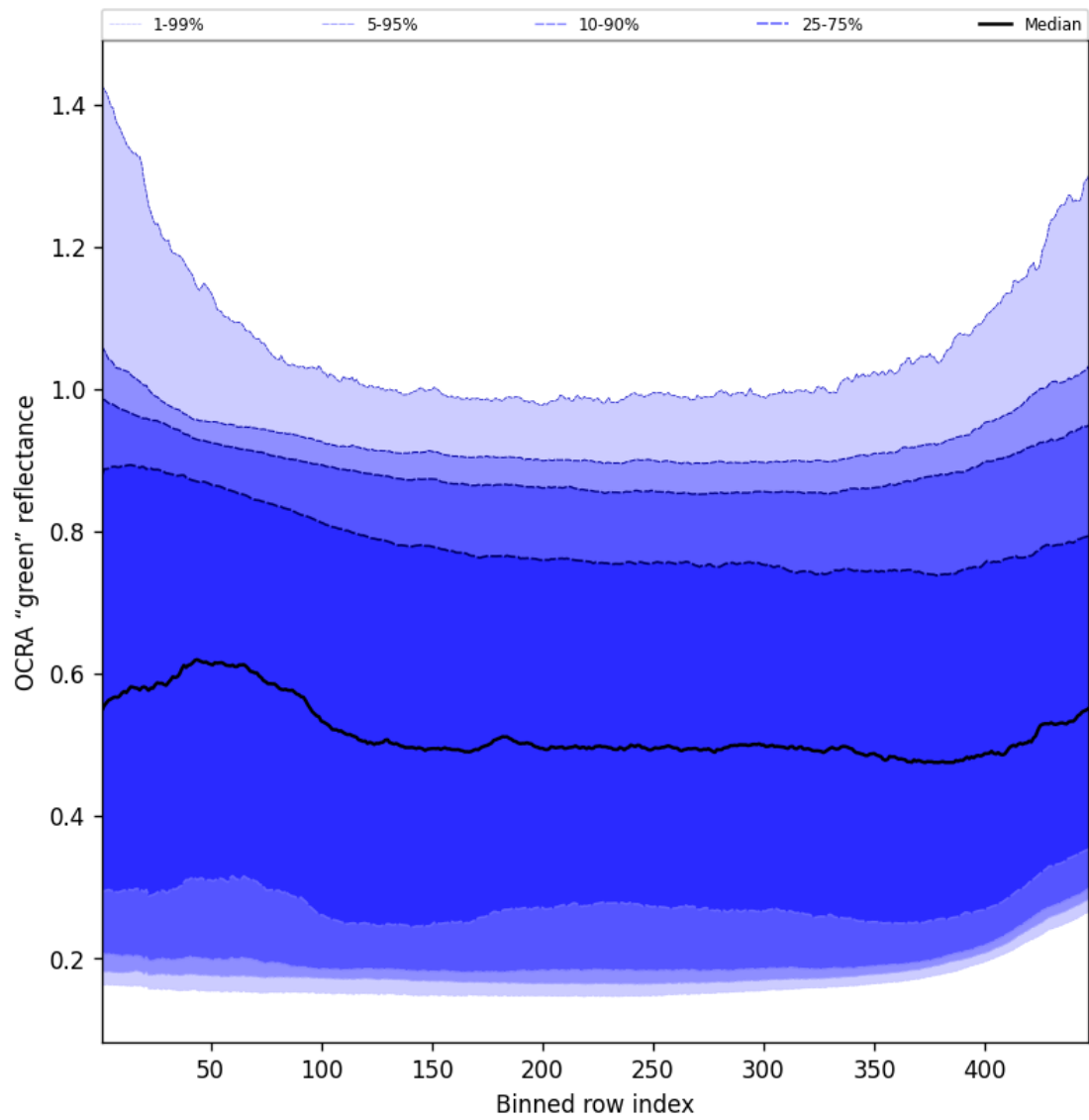
Figure 68: Along track statistics of “OCRA “green” reflectance” for 2025-11-04 to 2025-11-06
