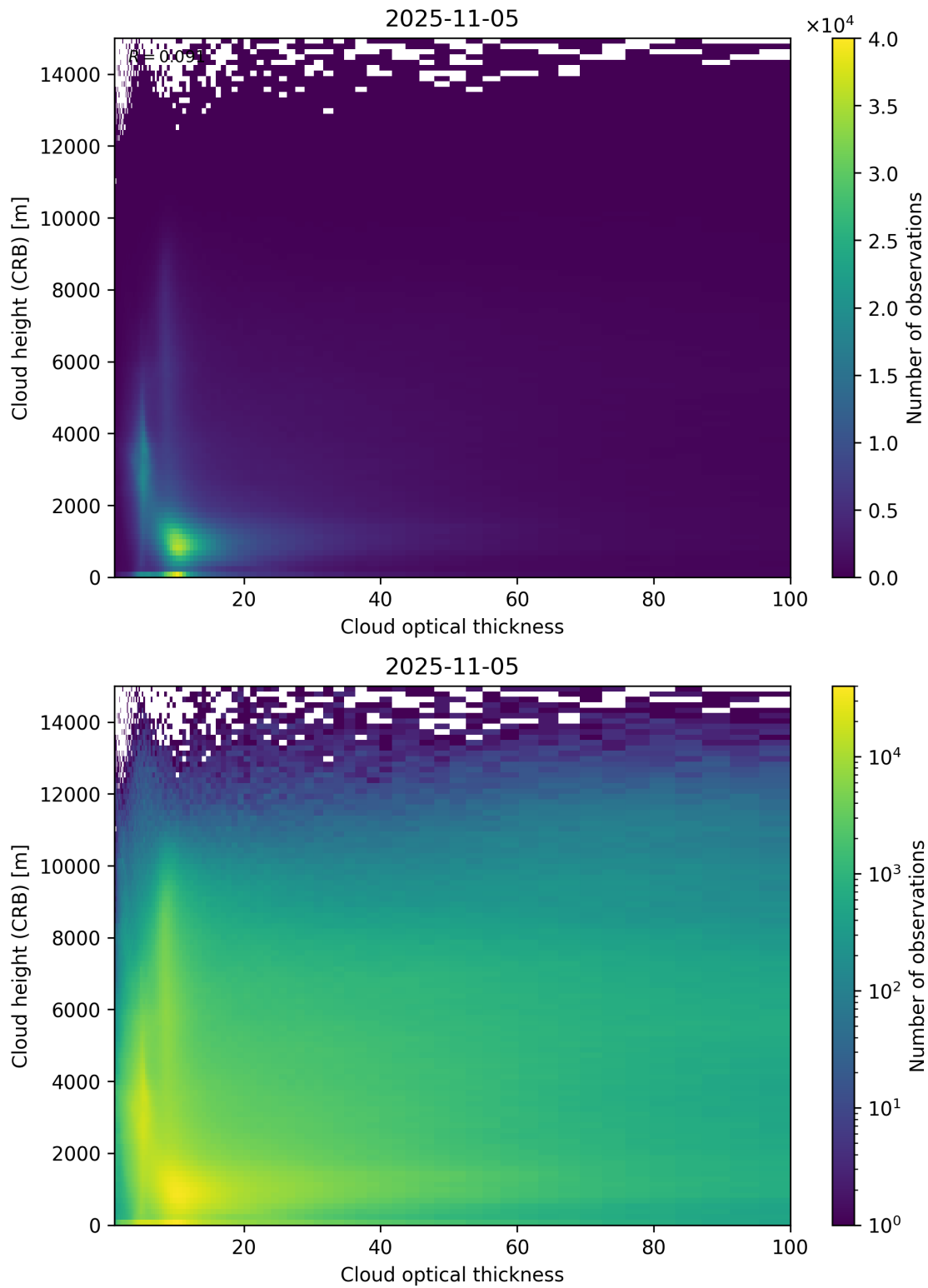
Figure 85: Scatter density plot of “Cloud optical thickness” against “Cloud height (CRB)” for 2025-11-04 to 2025-11-06.
