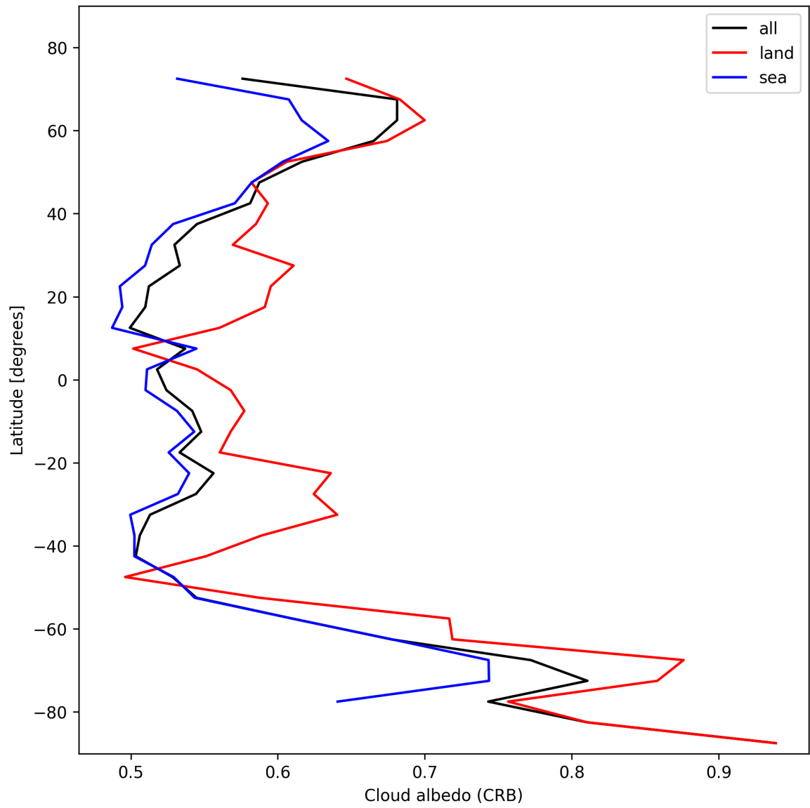
Figure 28: Zonal average of “Cloud albedo (CRB)” for 2025-11-04 to 2025-11-06.
