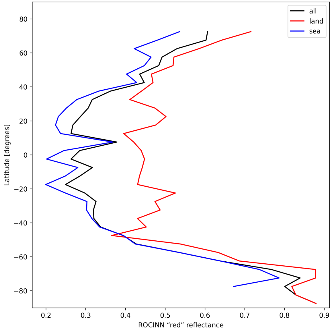
Figure 37: Zonal average of “ROCINN “red” reflectance” for 2025-11-04 to 2025-11-06.
