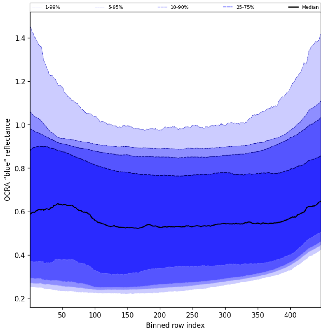
Figure 67: Along track statistics of “OCRA “blue” reflectance” for 2025-11-04 to 2025-11-06
