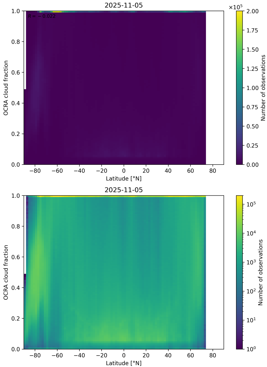
Figure 93: Scatter density plot of “Latitude” against “OCRA cloud fraction” for 2025-11-04 to 2025-11-06.
