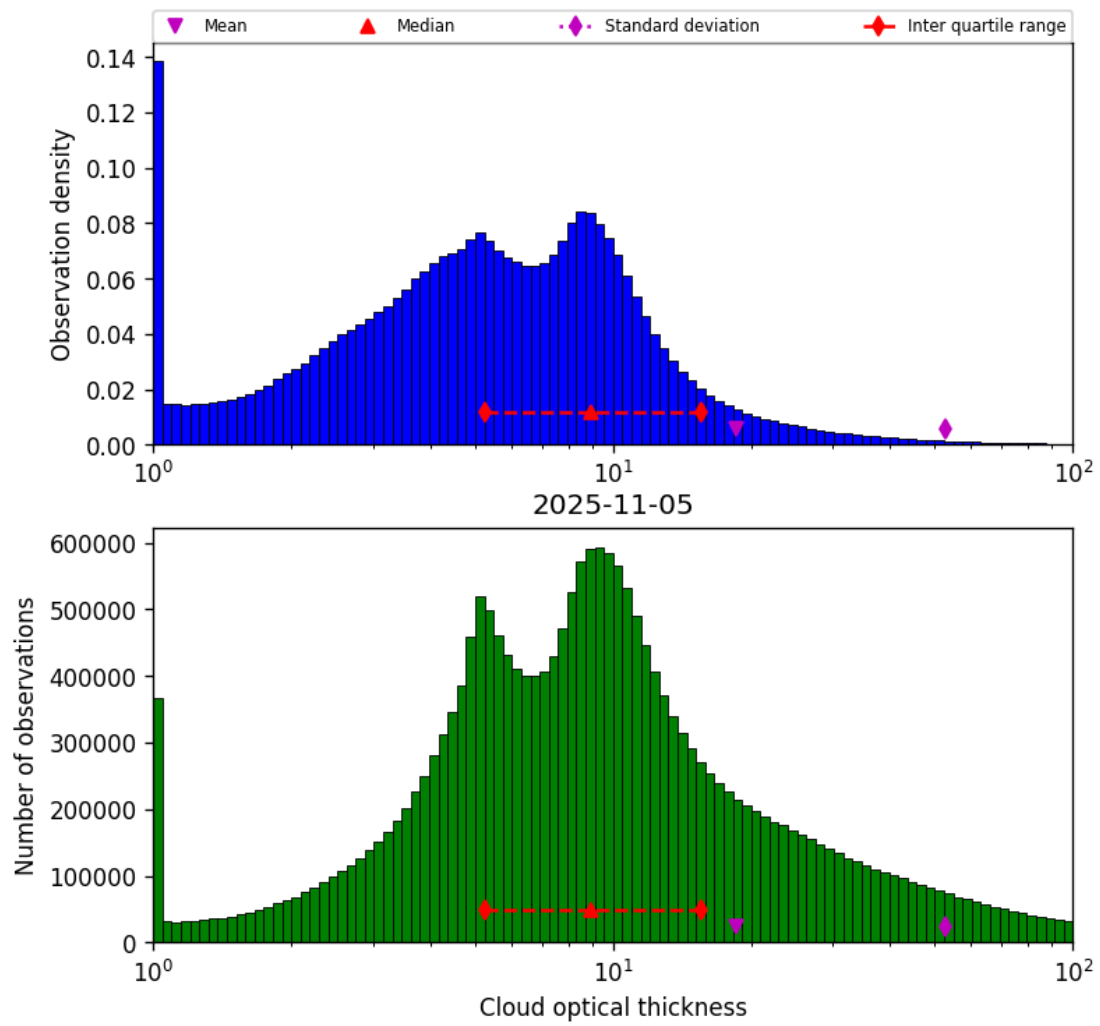
Figure 41: Histogram of “Cloud optical thickness” for 2025-11-04 to 2025-11-06
