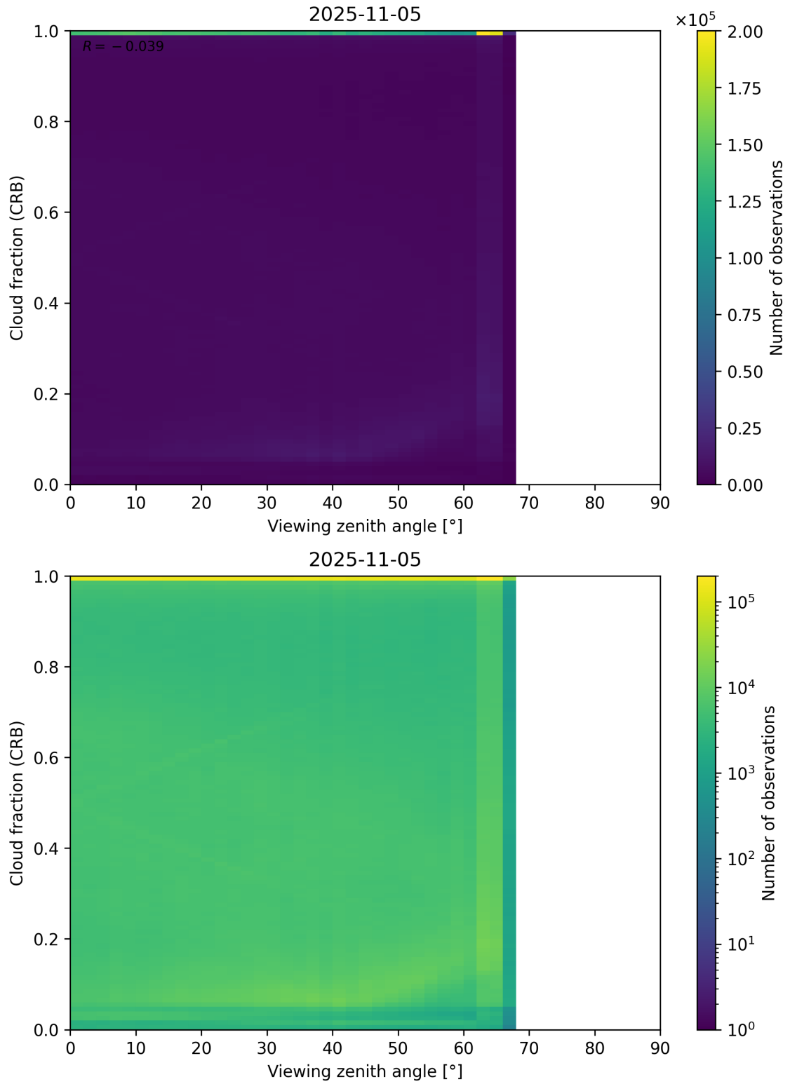
Figure 109: Scatter density plot of “Viewing zenith angle” against “Cloud fraction (CRB)” for 2025-11-04 to 2025-11-06.
