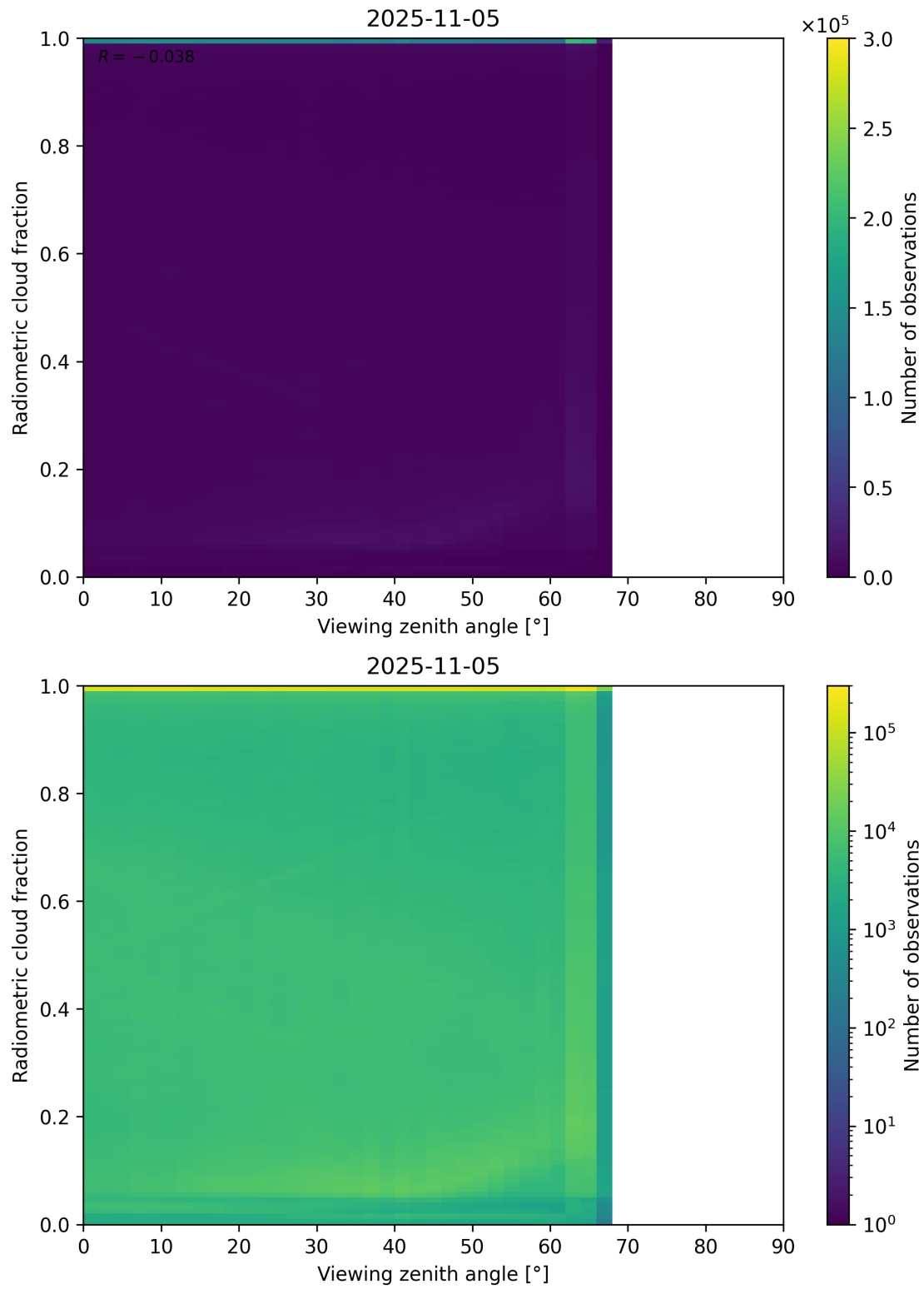
Figure 107: Scatter density plot of “Viewing zenith angle” against “Radiometric cloud fraction” for 2025-11-04 to 2025-11-06.
