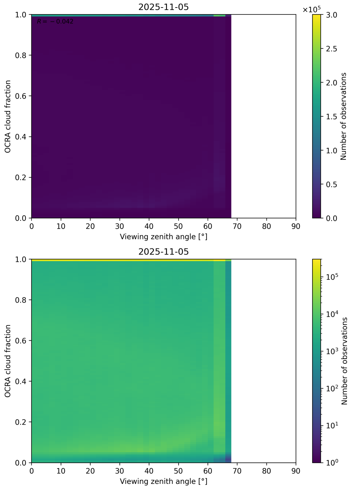
Figure 108: Scatter density plot of “Viewing zenith angle” against “OCRA cloud fraction” for 2025-11-04 to 2025-11-06.
