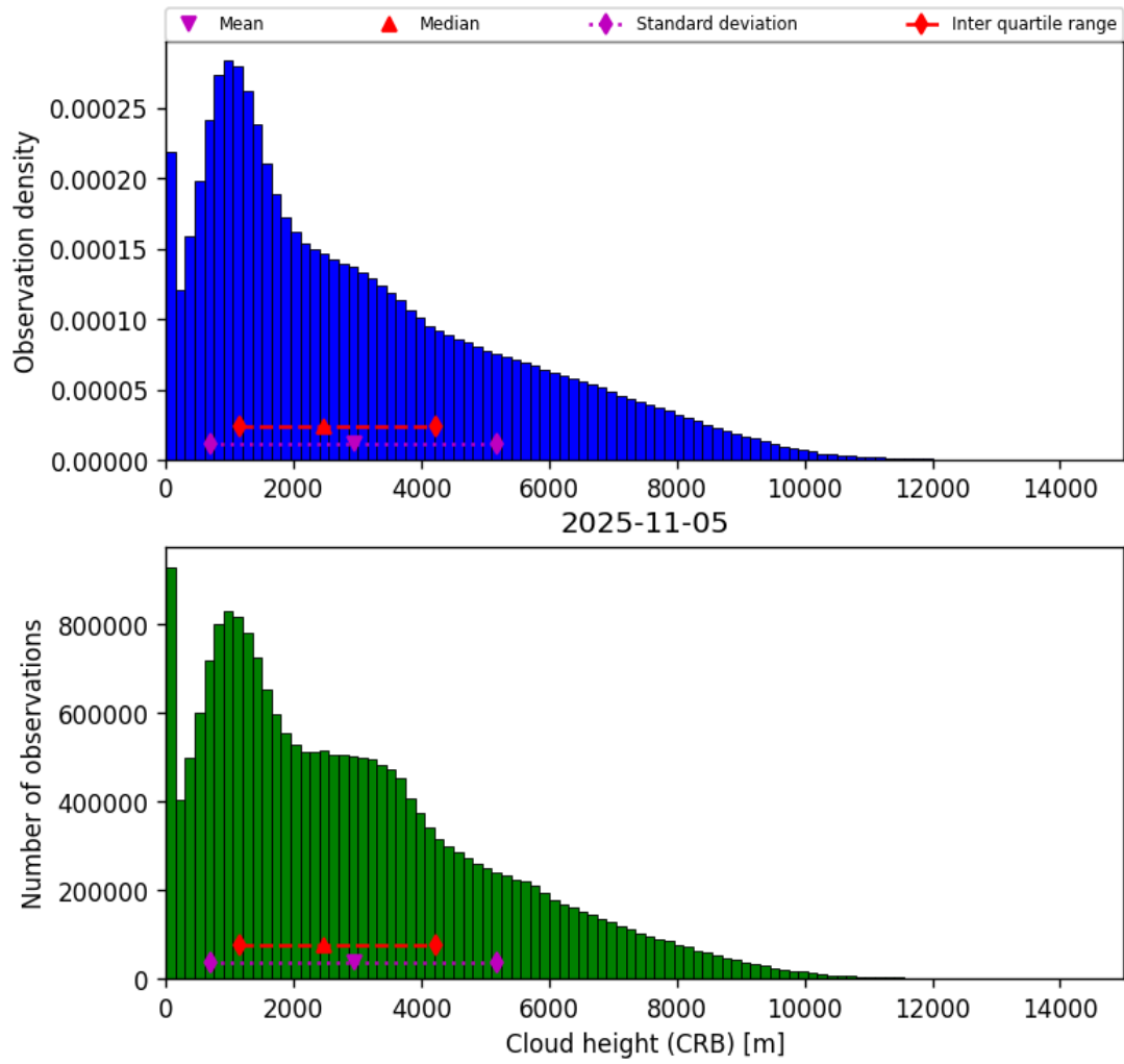
Figure 43: Histogram of “Cloud height (CRB)” for 2025-11-04 to 2025-11-06
