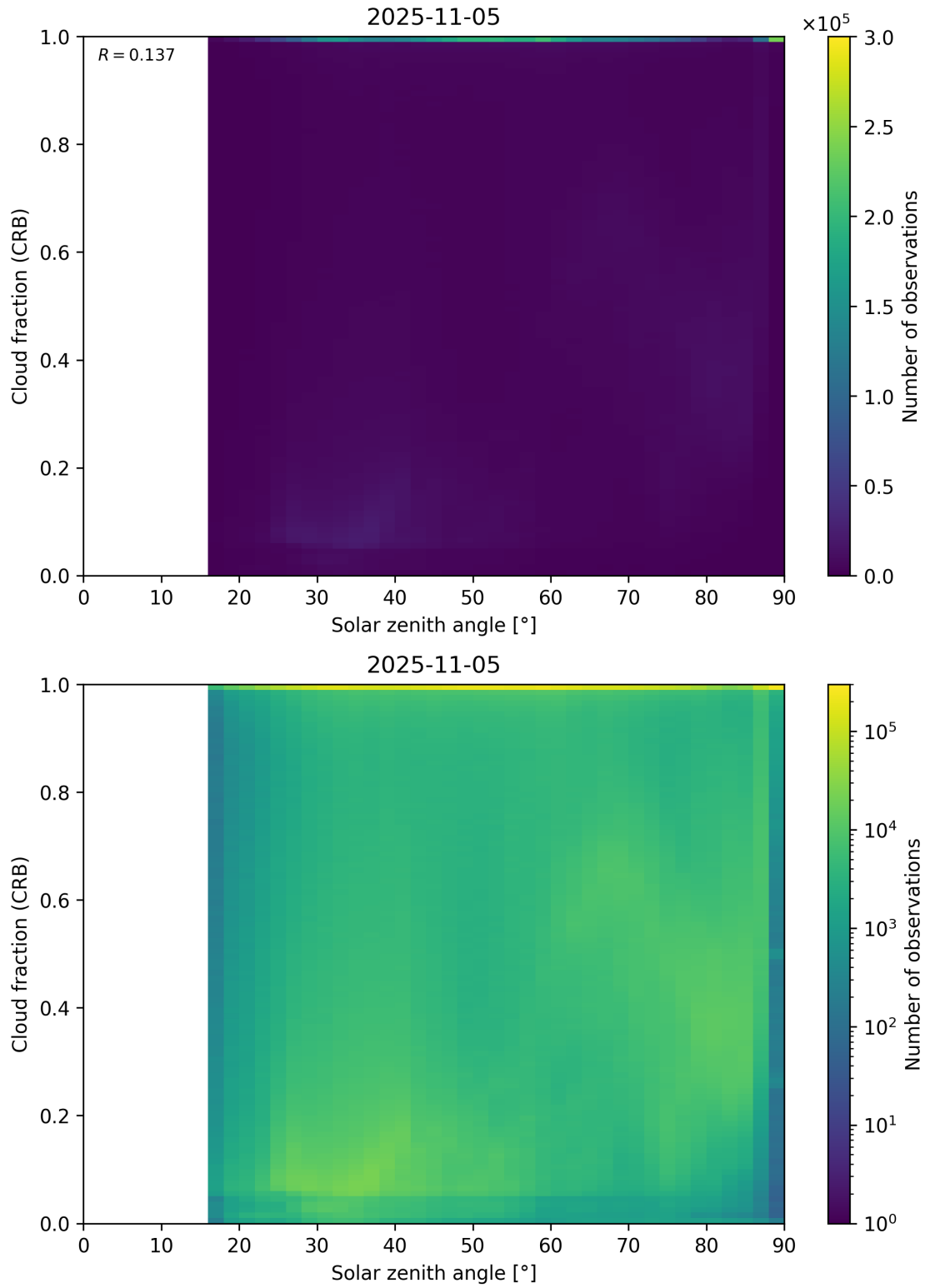
Figure 101: Scatter density plot of “Solar zenith angle” against “Cloud fraction (CRB)” for 2025-11-04 to 2025-11-06.
