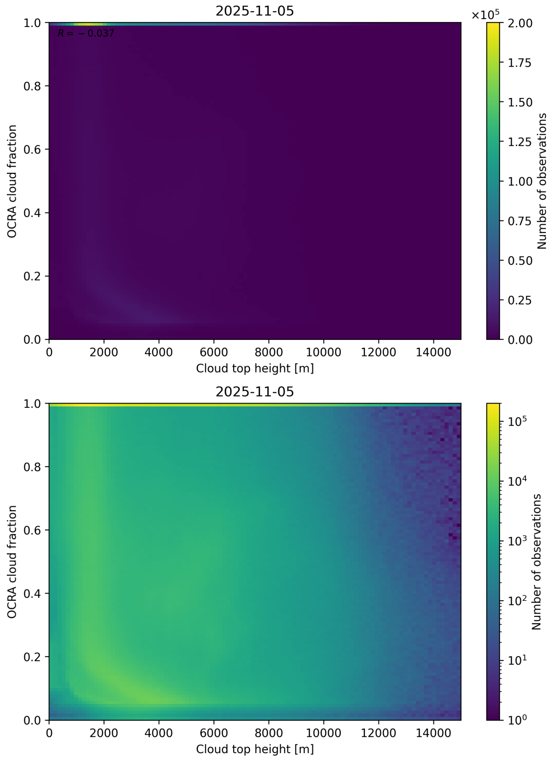
Figure 87: Scatter density plot of “Cloud top height” against “OCRA cloud fraction” for 2025-11-04 to 2025-11-06.
