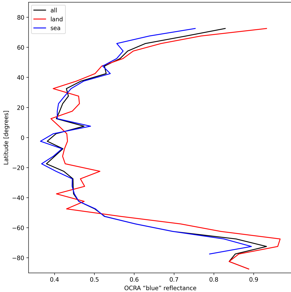
Figure 35: Zonal average of “OCRA “blue” reflectance” for 2025-11-04 to 2025-11-06.
