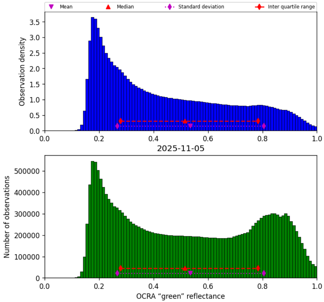
Figure 52: Histogram of “OCRA “green” reflectance” for 2025-11-04 to 2025-11-06
