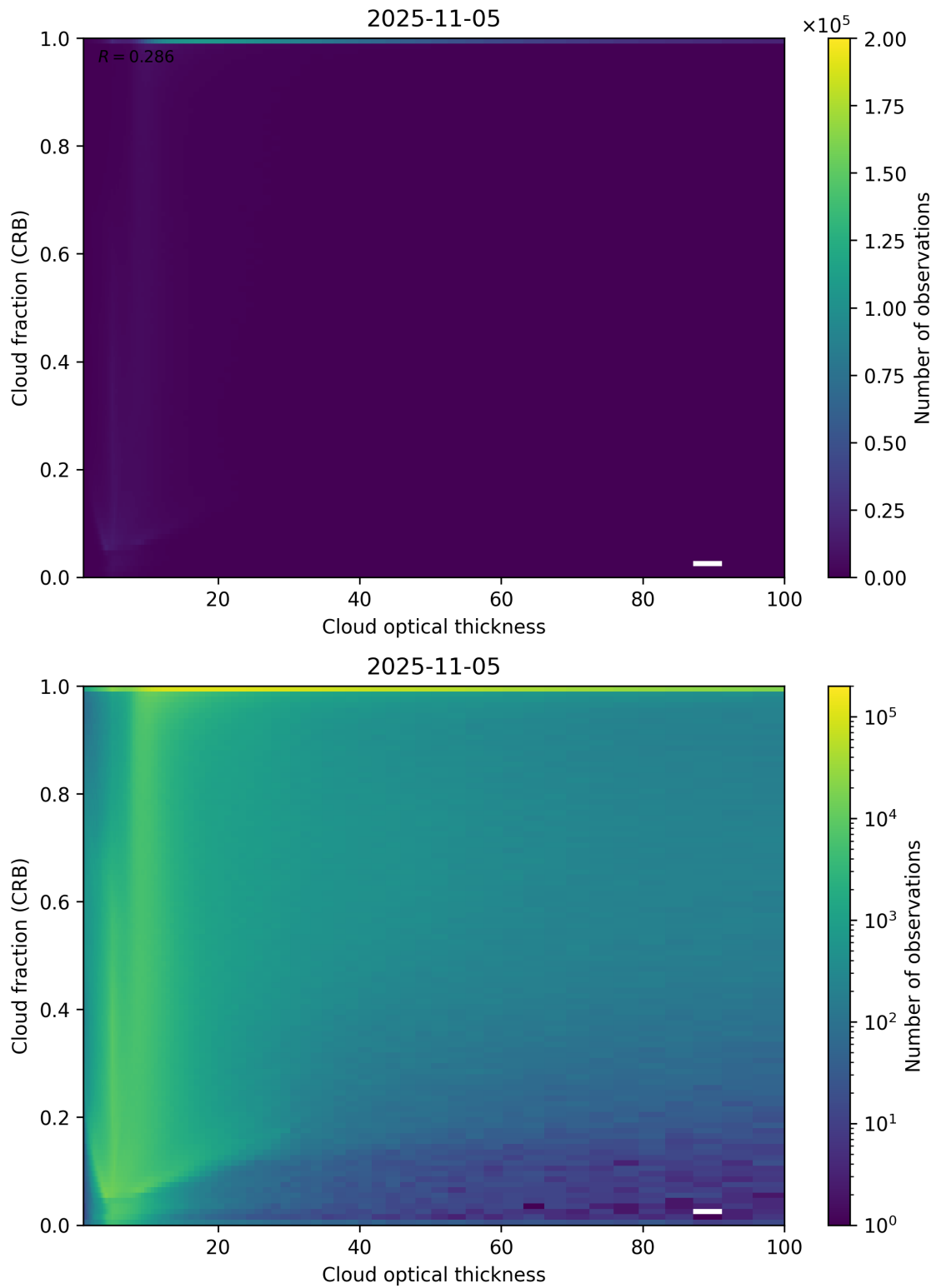
Figure 84: Scatter density plot of “Cloud optical thickness” against “Cloud fraction (CRB)” for 2025-11-04 to 2025-11-06.
