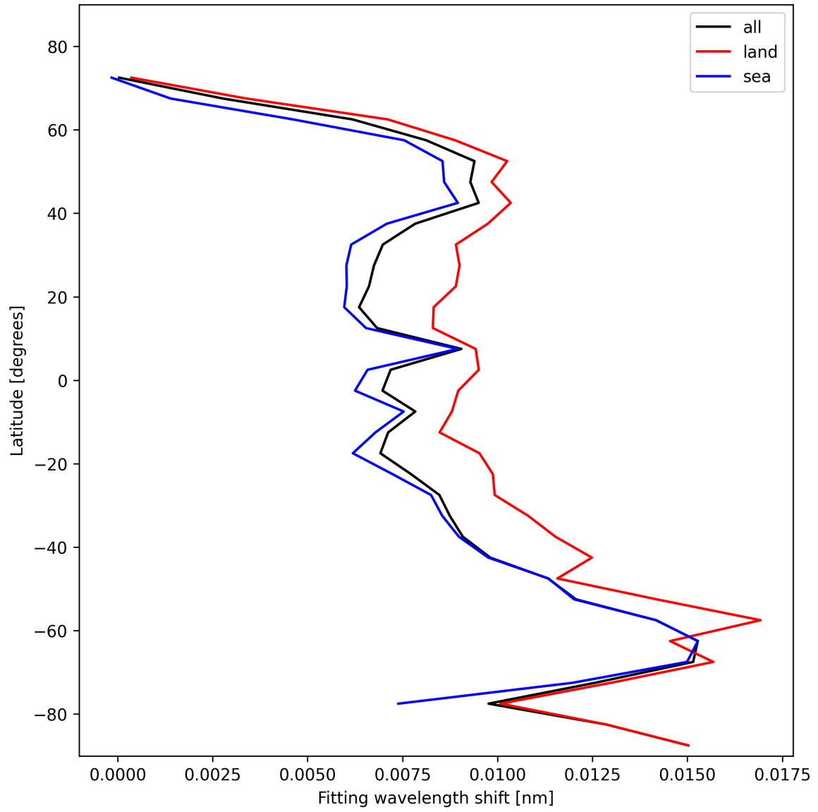
Figure 33: Zonal average of “Fitting wavelength shift” for 2025-11-04 to 2025-11-06.
