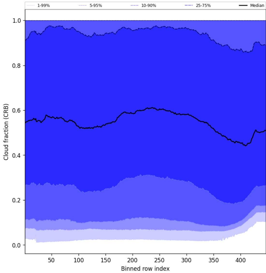
Figure 58: Along track statistics of “Cloud fraction (CRB)” for 2025-11-04 to 2025-11-06
