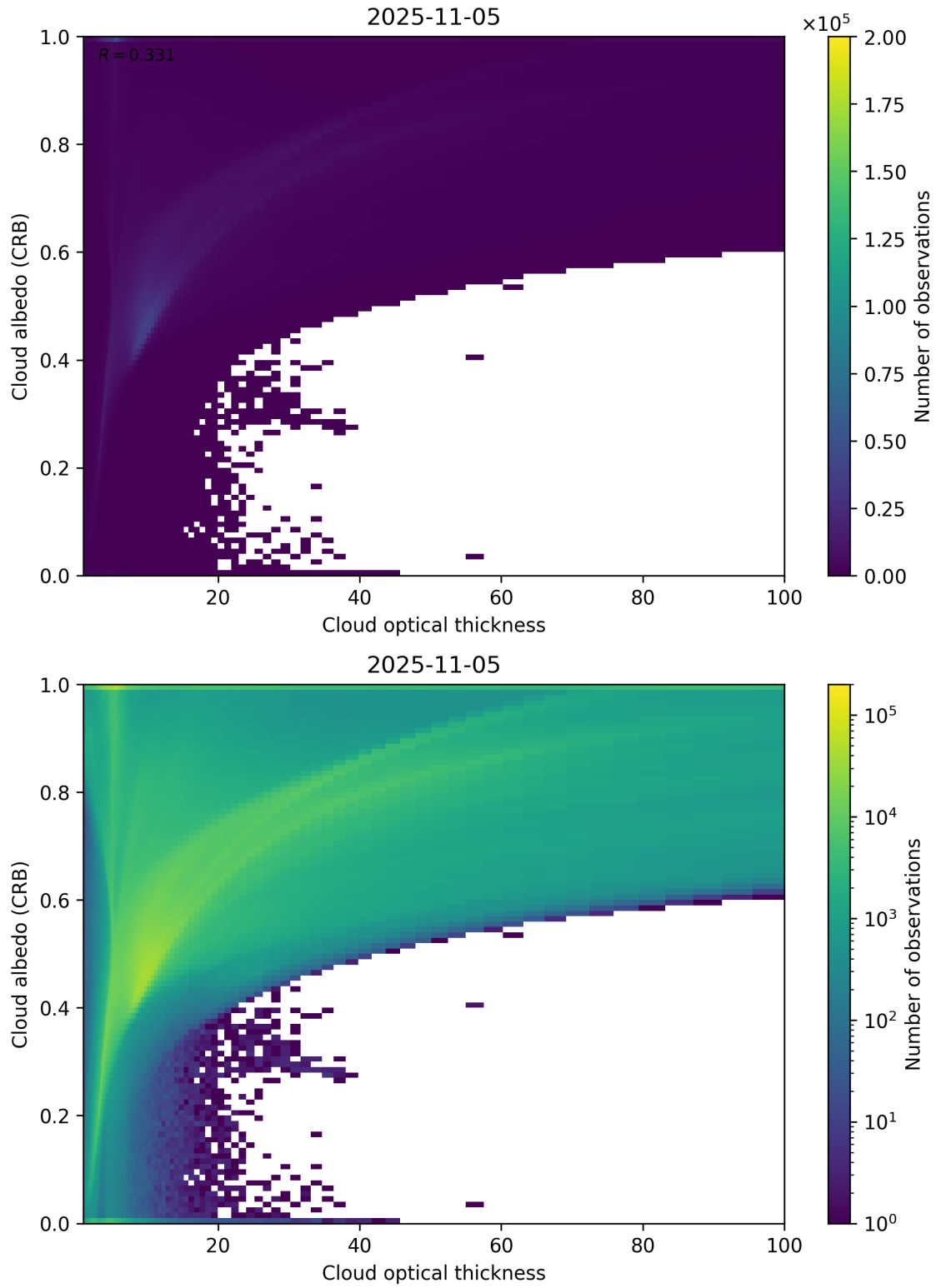
Figure 82: Scatter density plot of “Cloud optical thickness” against “Cloud albedo (CRB)” for 2025-11-04 to 2025-11-06.
