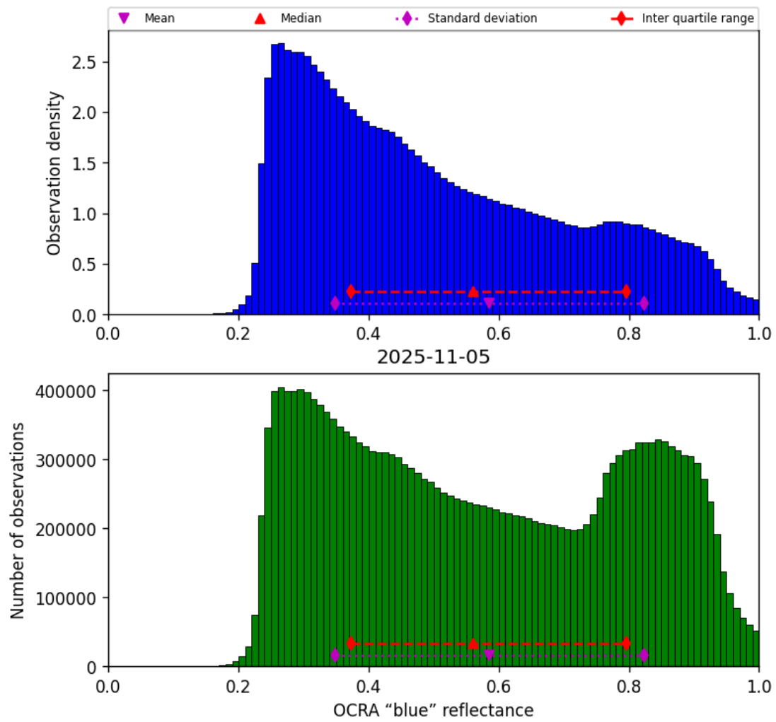
Figure 51: Histogram of “OCRA “blue” reflectance” for 2025-11-04 to 2025-11-06
