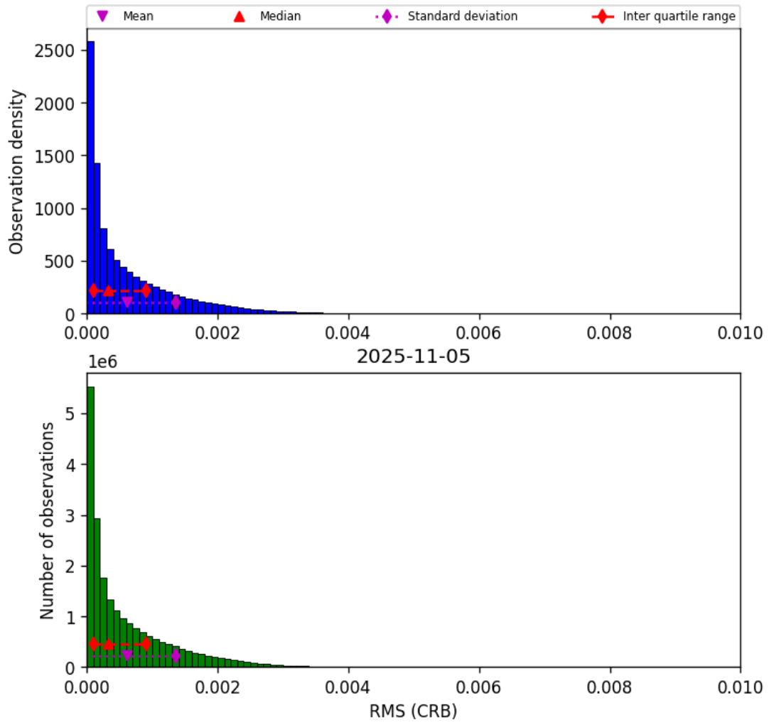
Figure 48: Histogram of “RMS (CRB)” for 2025-11-04 to 2025-11-06
