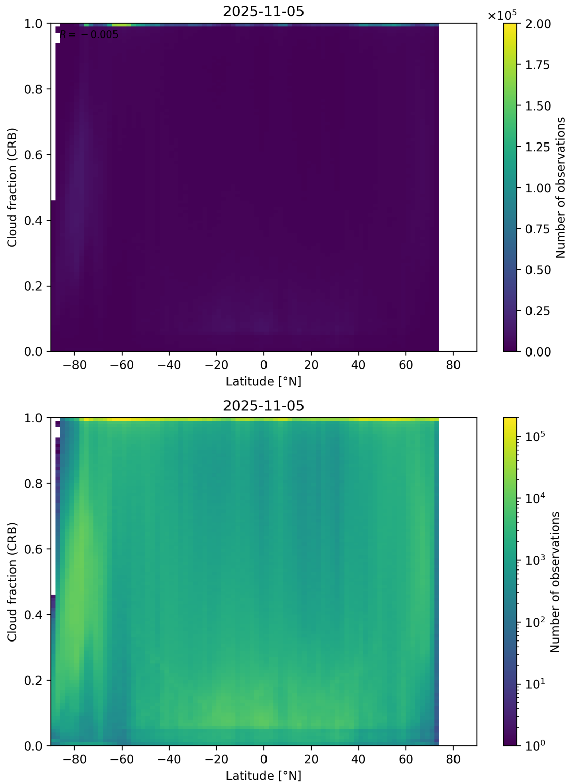
Figure 94: Scatter density plot of “Latitude” against “Cloud fraction (CRB)” for 2025-11-04 to 2025-11-06.
