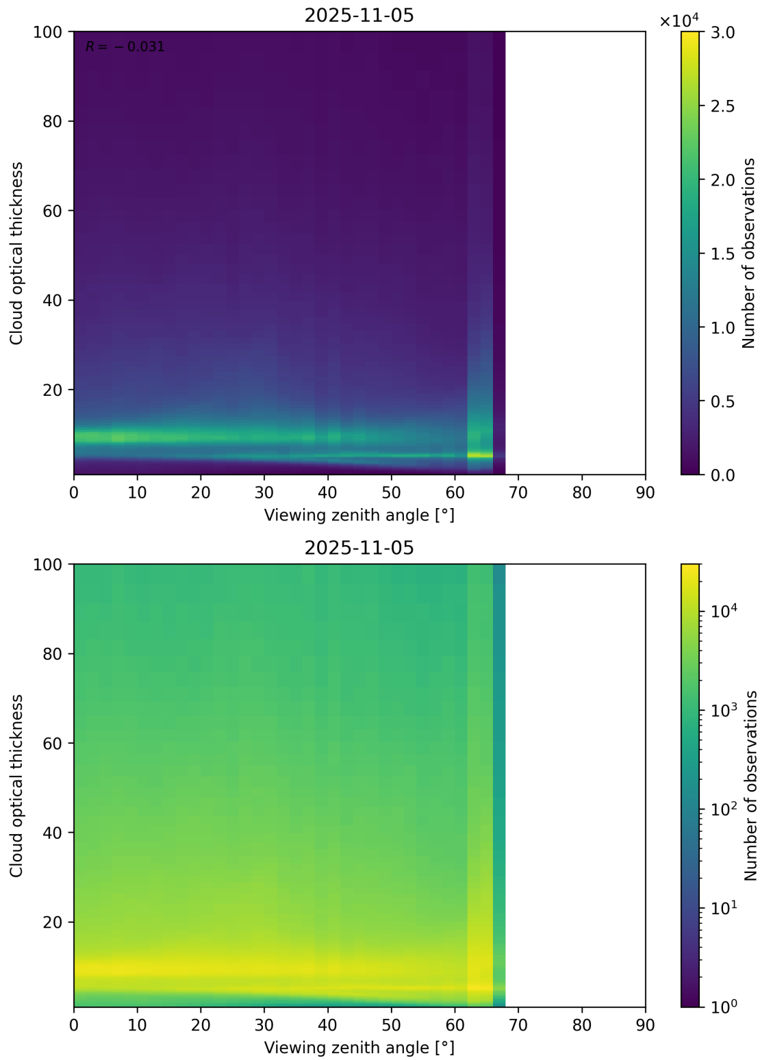
Figure 111: Scatter density plot of “Viewing zenith angle” against “Cloud optical thickness” for 2025-11-04 to 2025-11-06.
