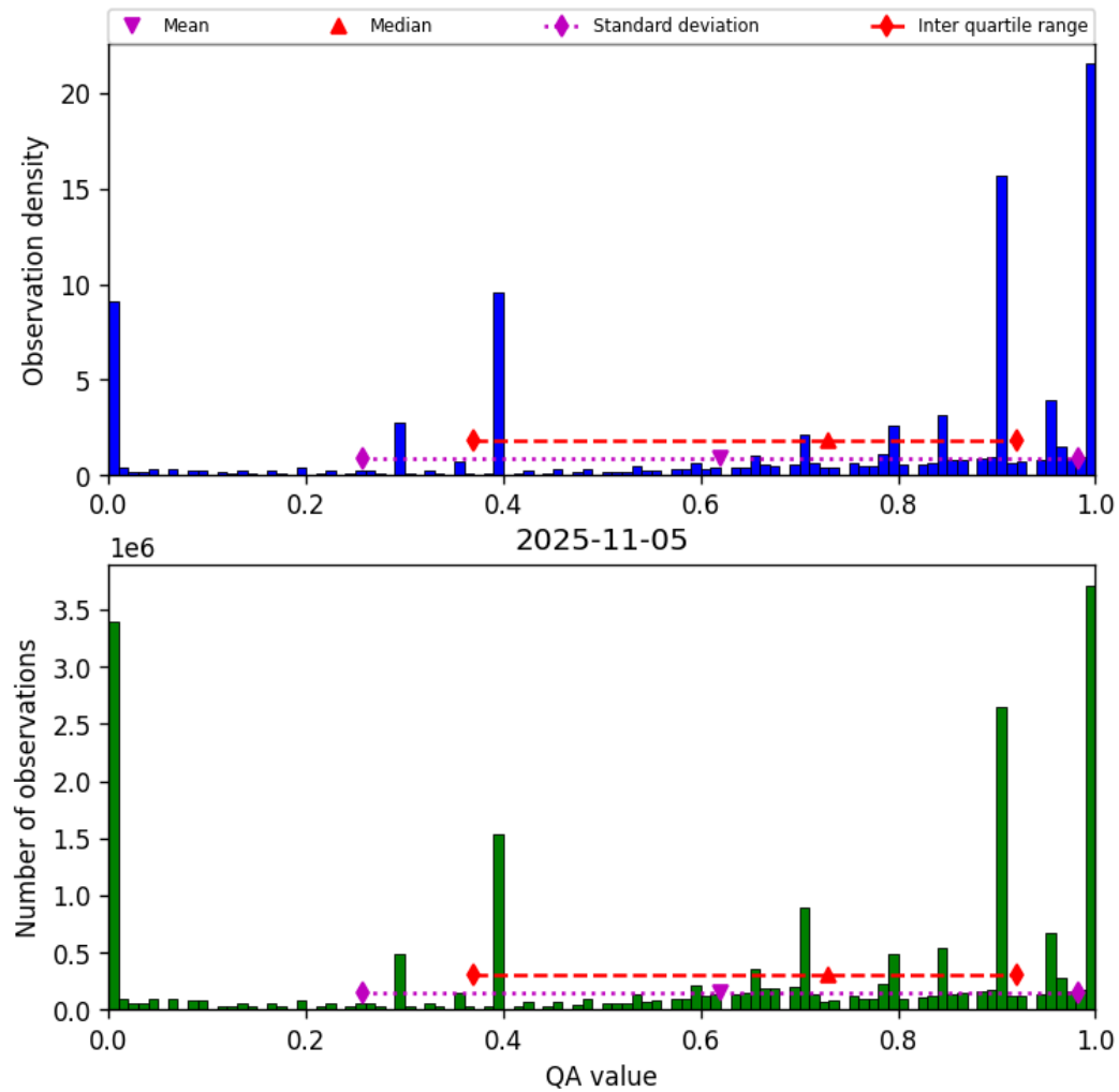
Figure 38: Histogram of “QA value” for 2025-11-04 to 2025-11-06
