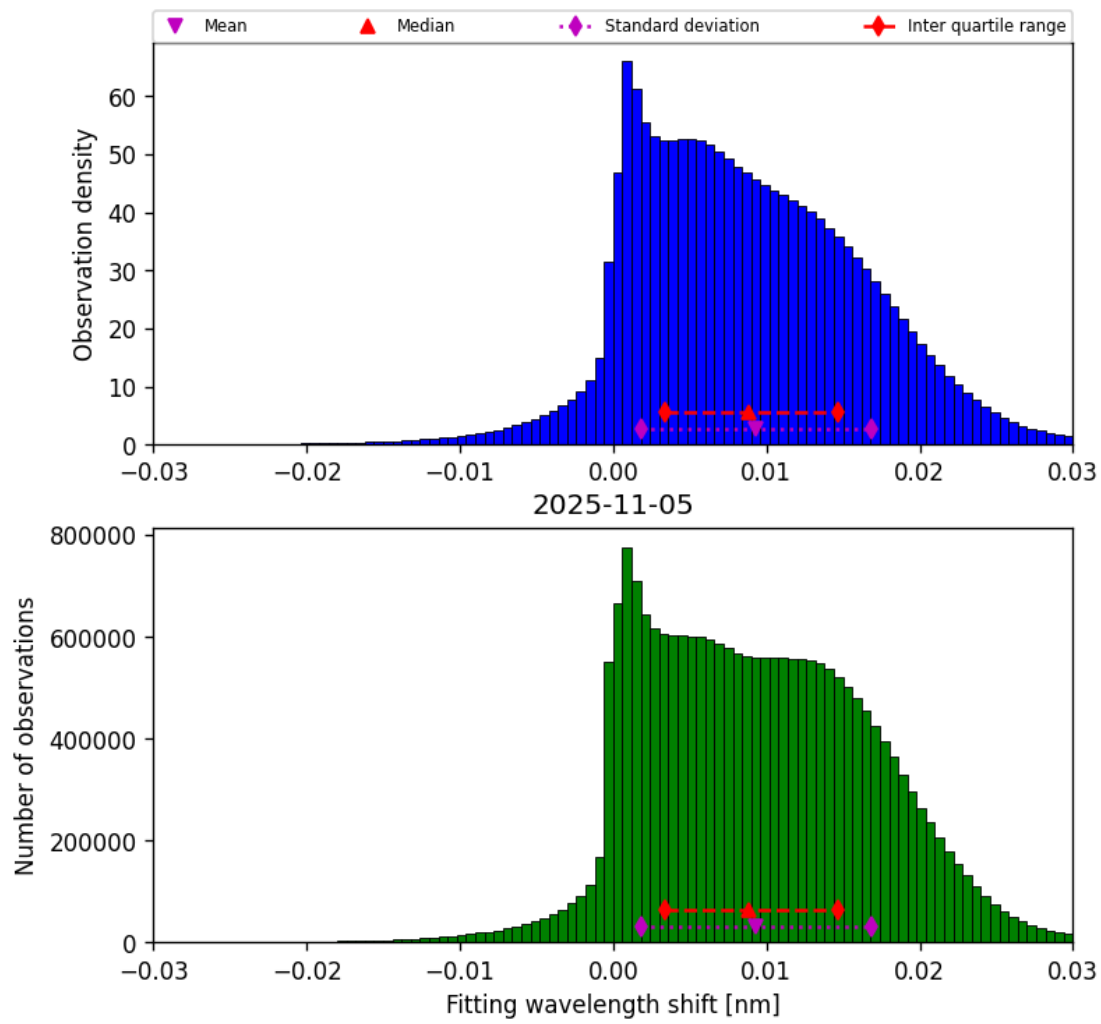
Figure 49: Histogram of “Fitting wavelength shift” for 2025-11-04 to 2025-11-06
