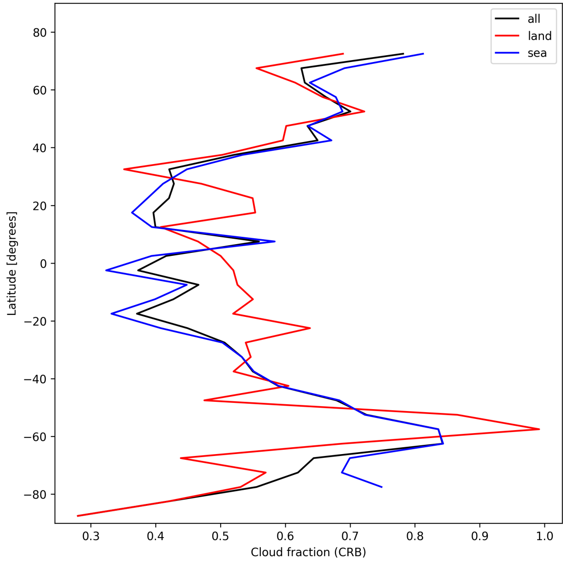
Figure 26: Zonal average of “Cloud fraction (CRB)” for 2025-11-04 to 2025-11-06.
