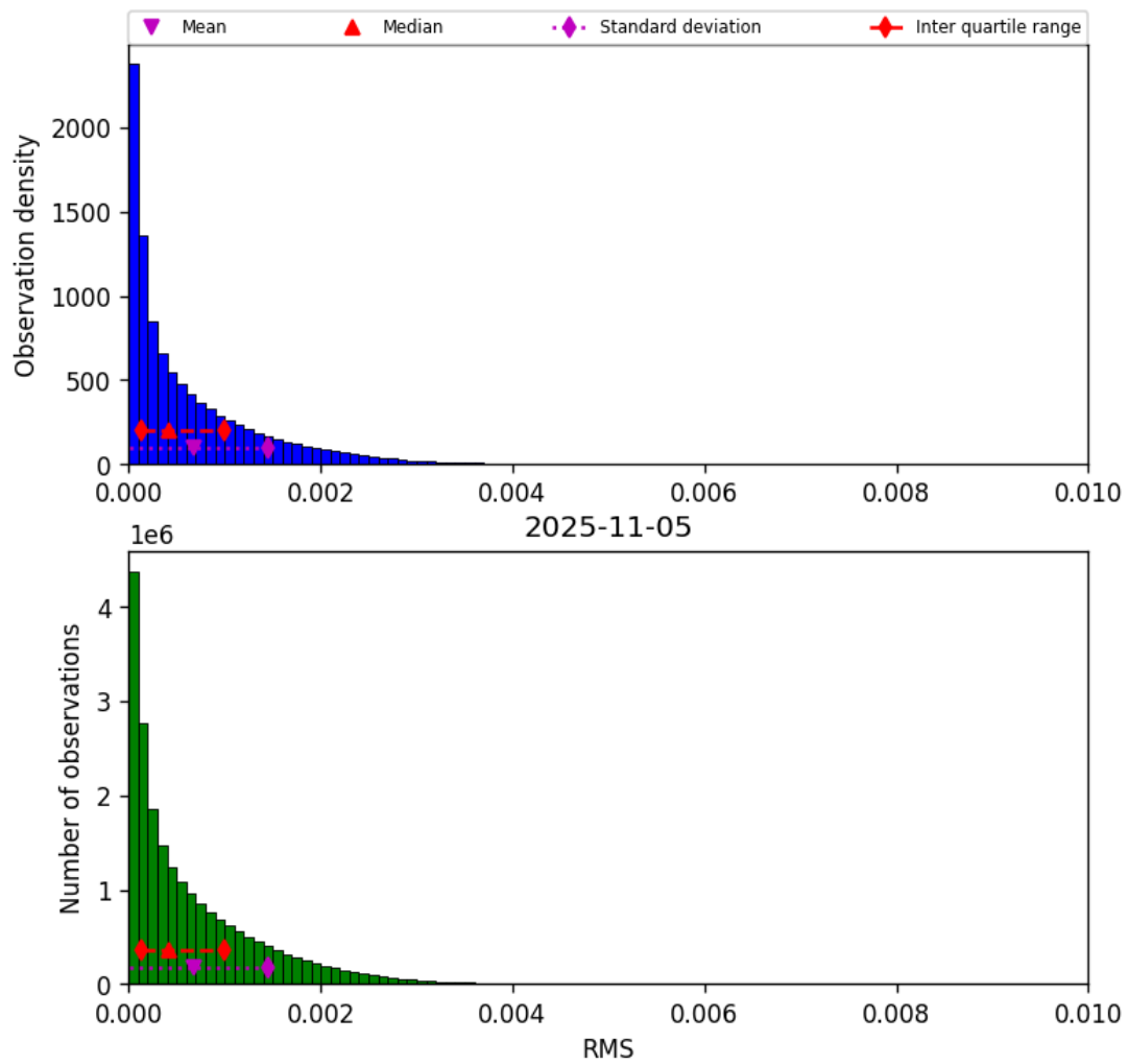
Figure 47: Histogram of “RMS” for 2025-11-04 to 2025-11-06
