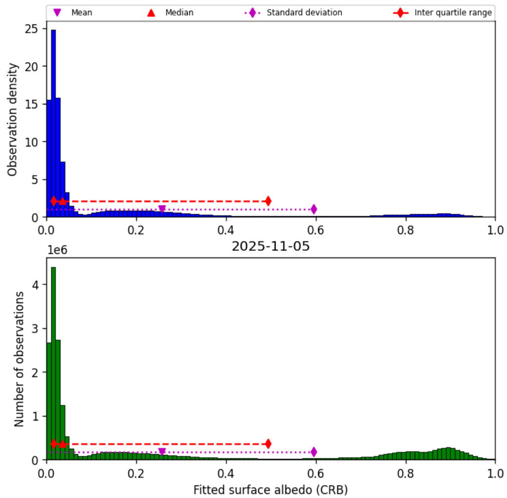
Figure 46: Histogram of “Fitted surface albedo (CRB)” for 2025-11-04 to 2025-11-06
