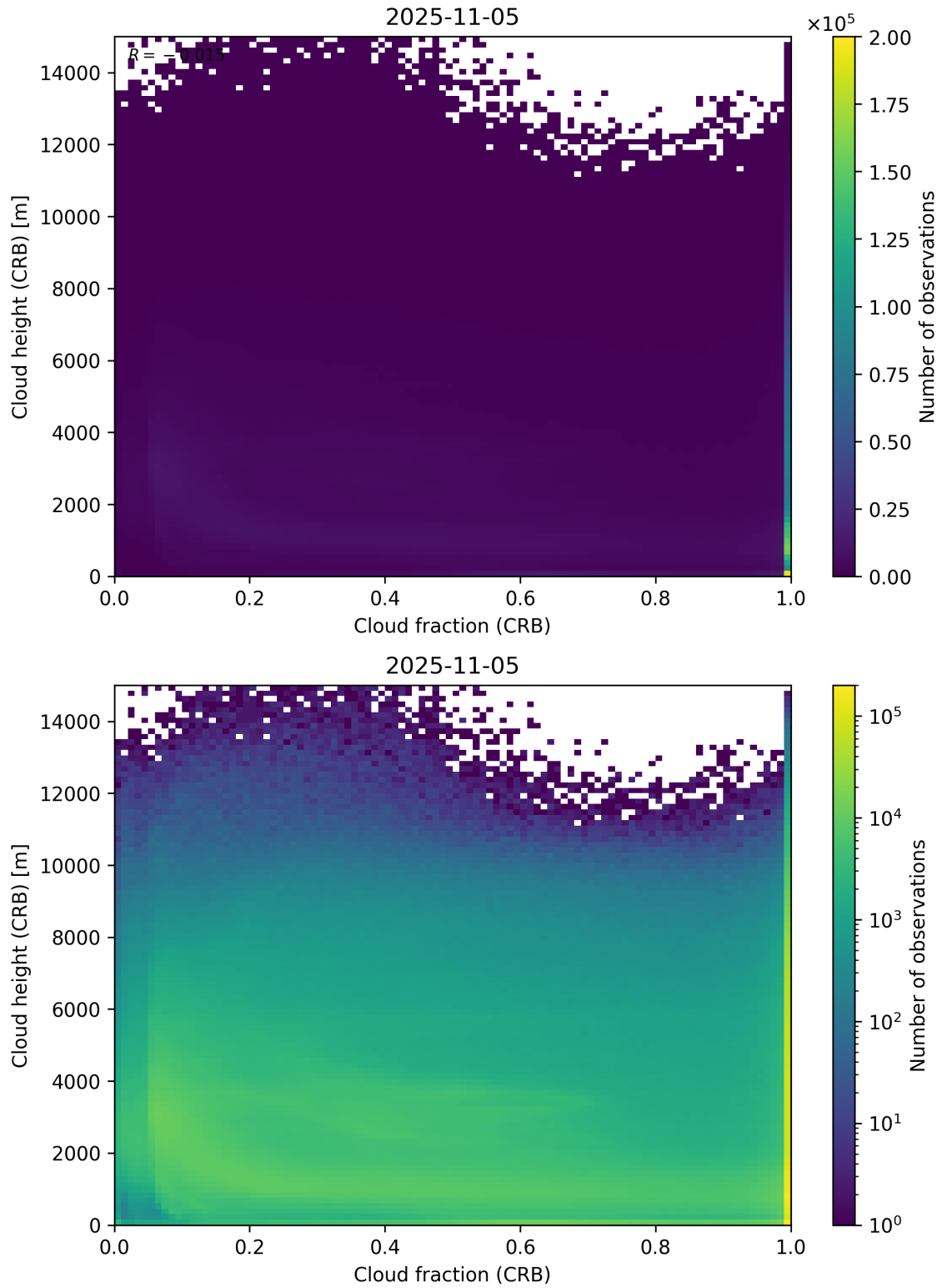
Figure 79: Scatter density plot of “Cloud fraction (CRB)” against “Cloud height (CRB)” for 2025-11-04 to 2025-11-06.
