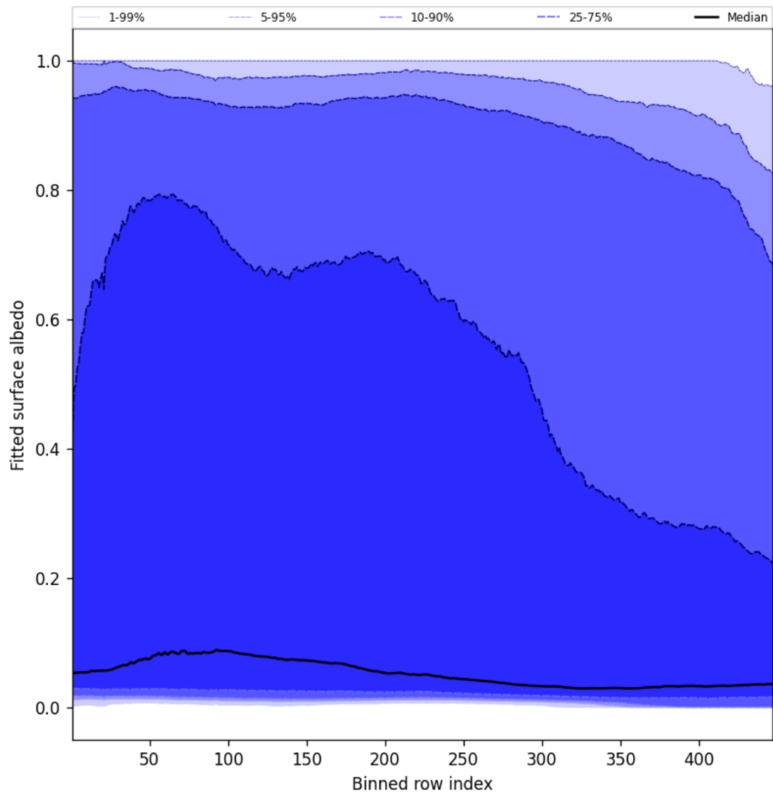
Figure 61: Along track statistics of “Fitted surface albedo” for 2025-11-04 to 2025-11-06
