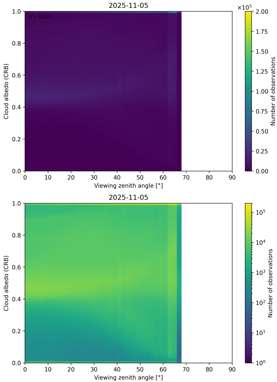
Figure 106: Scatter density plot of “Viewing zenith angle” against “Cloud albedo (CRB)” for 2025-11-04 to 2025-11-06.
