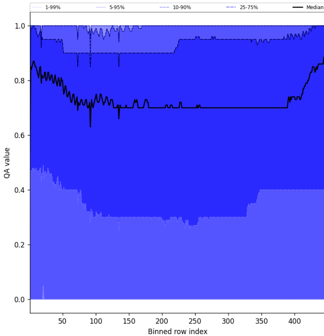
Figure 54: Along track statistics of “QA value” for 2025-11-04 to 2025-11-06
