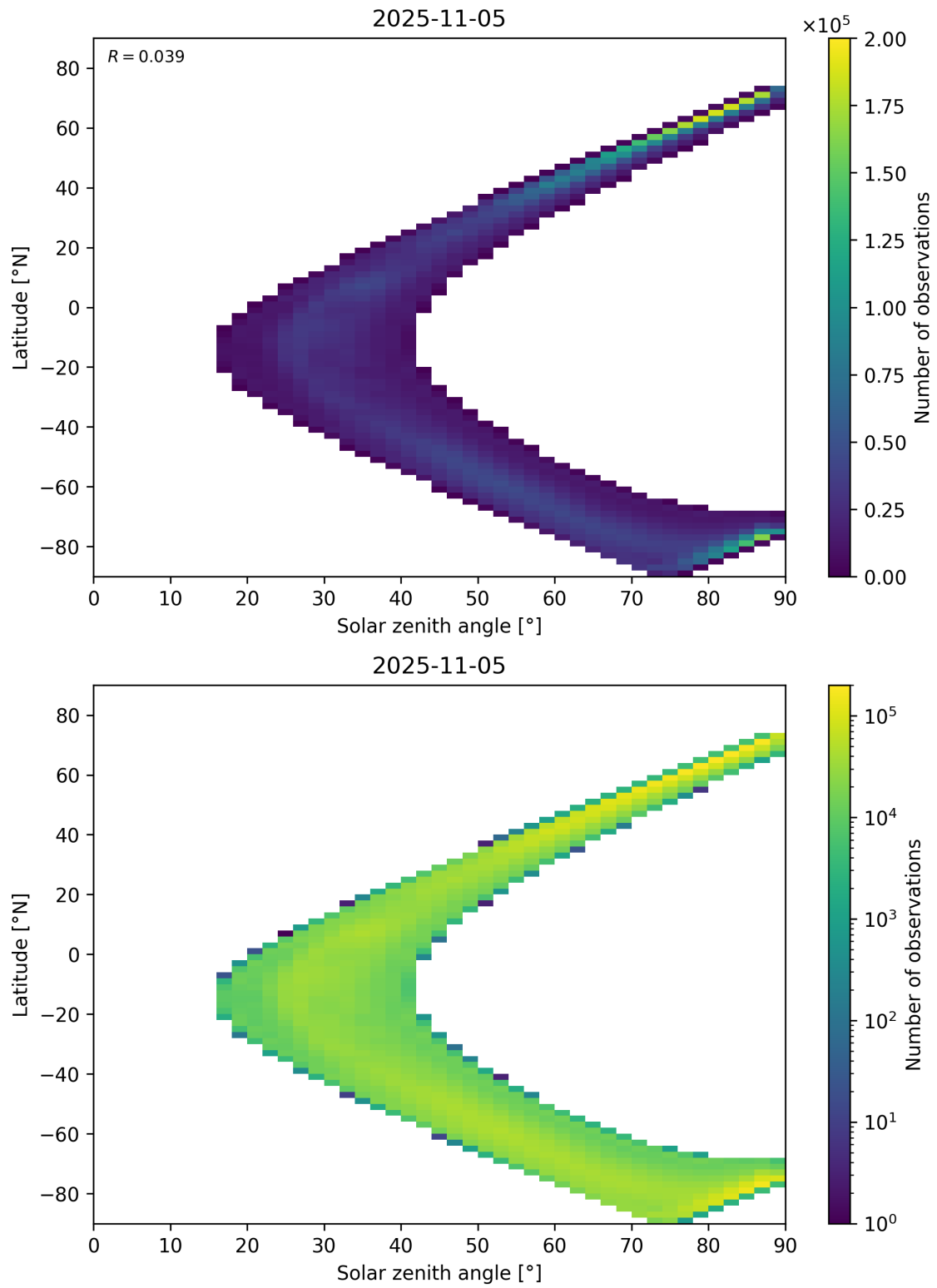
Figure 105: Scatter density plot of “Solar zenith angle” against “Latitude” for 2025-11-04 to 2025-11-06.
