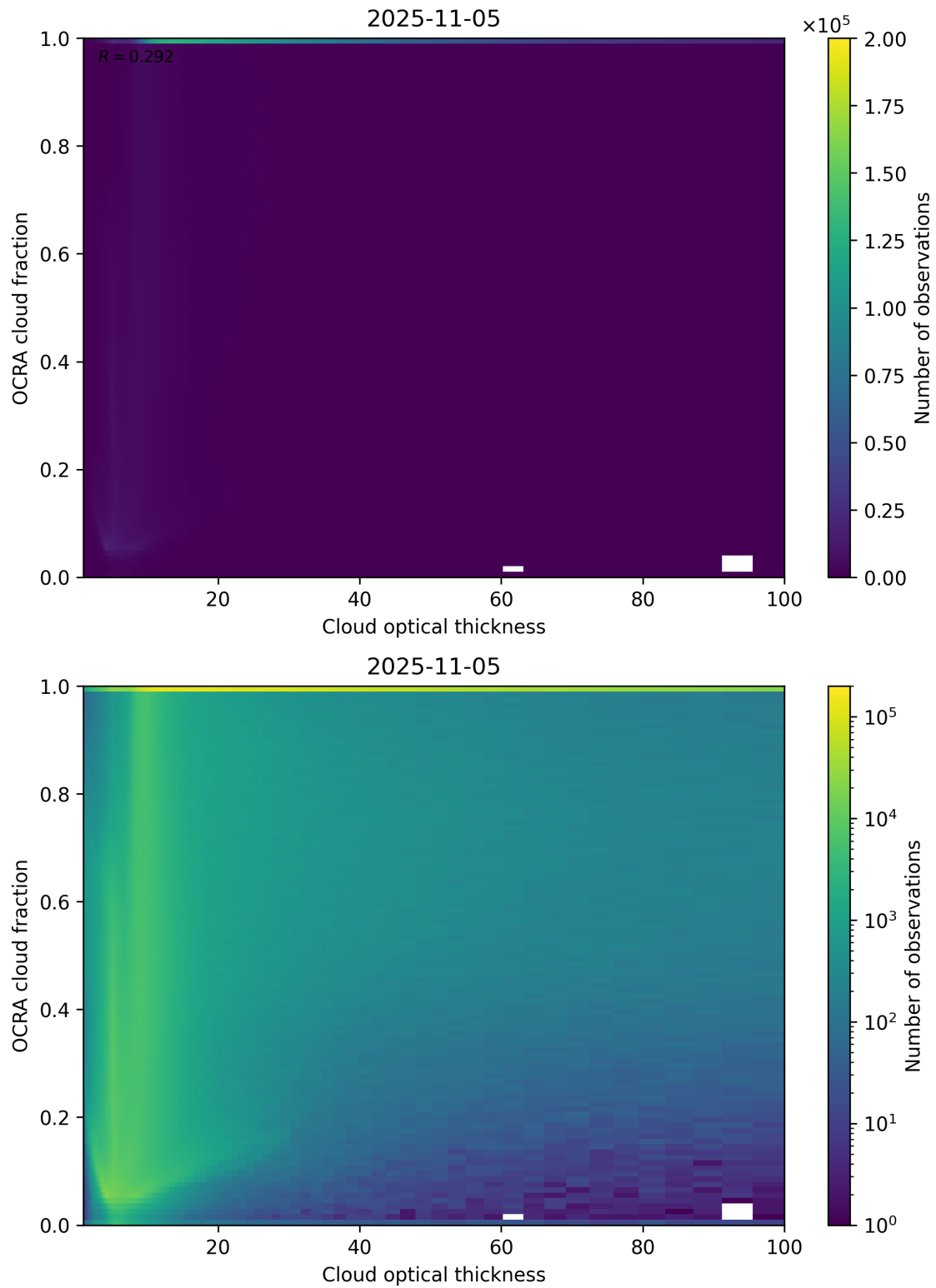
Figure 83: Scatter density plot of “Cloud optical thickness” against “OCRA cloud fraction” for 2025-11-04 to 2025-11-06.
