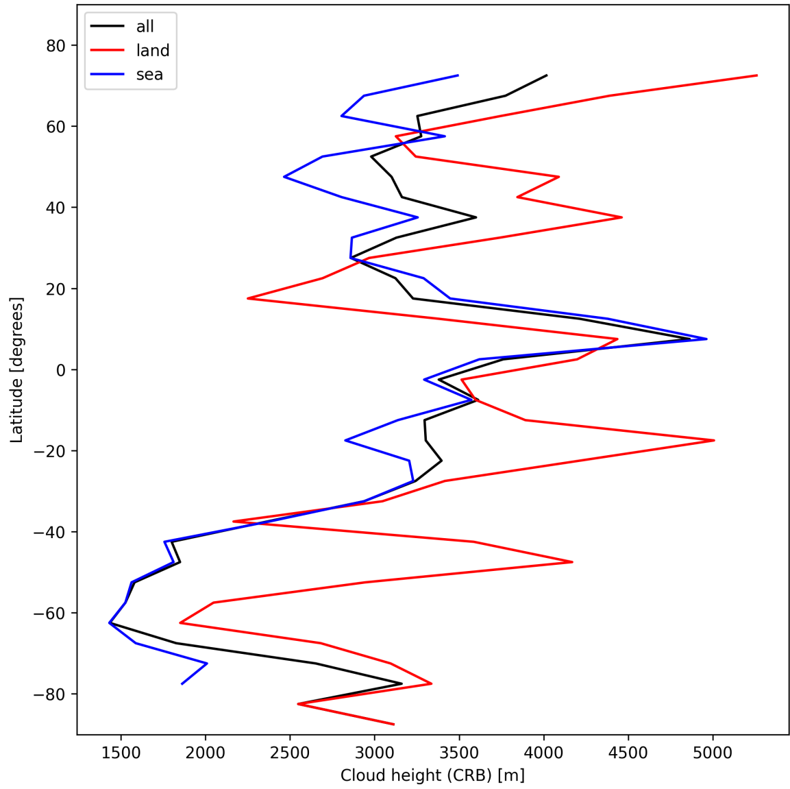
Figure 27: Zonal average of “Cloud height (CRB)” for 2025-11-04 to 2025-11-06.
