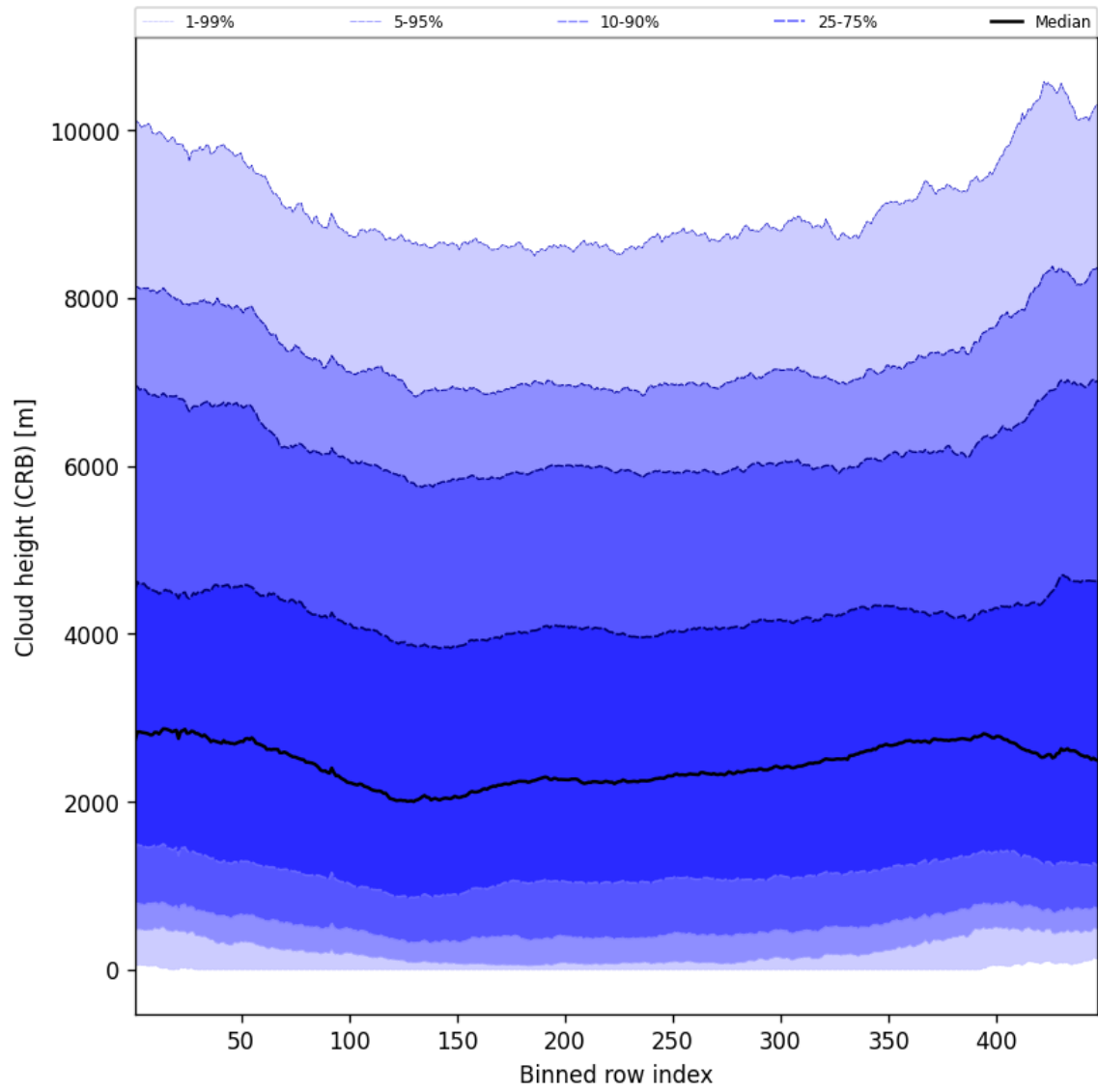
Figure 59: Along track statistics of “Cloud height (CRB)” for 2025-11-04 to 2025-11-06
