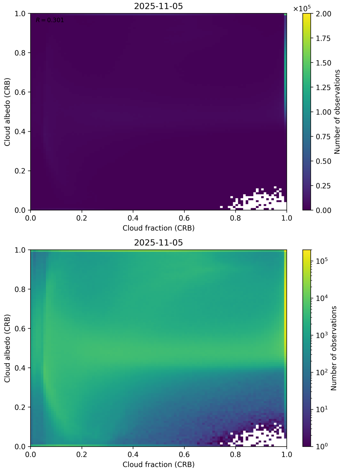
Figure 77: Scatter density plot of “Cloud fraction (CRB)” against “Cloud albedo (CRB)” for 2025-11-04 to 2025-11-06.
