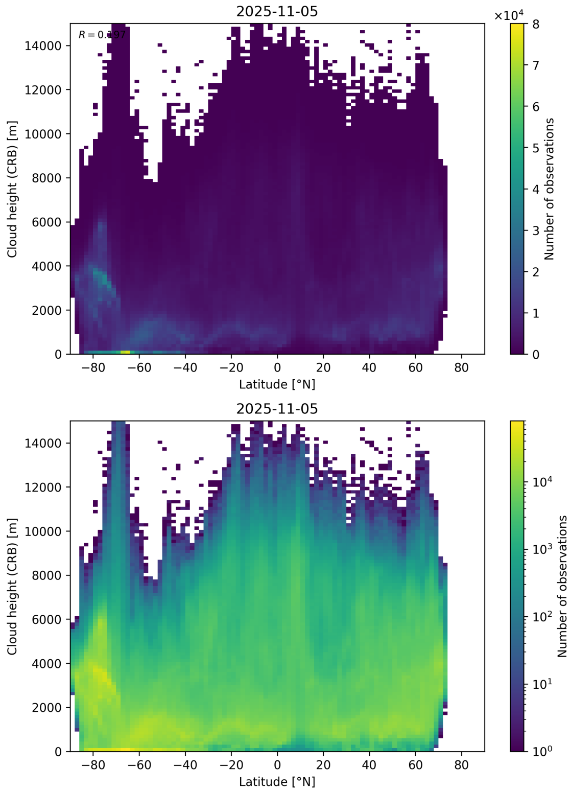
Figure 95: Scatter density plot of “Latitude” against “Cloud height (CRB)” for 2025-11-04 to 2025-11-06.
