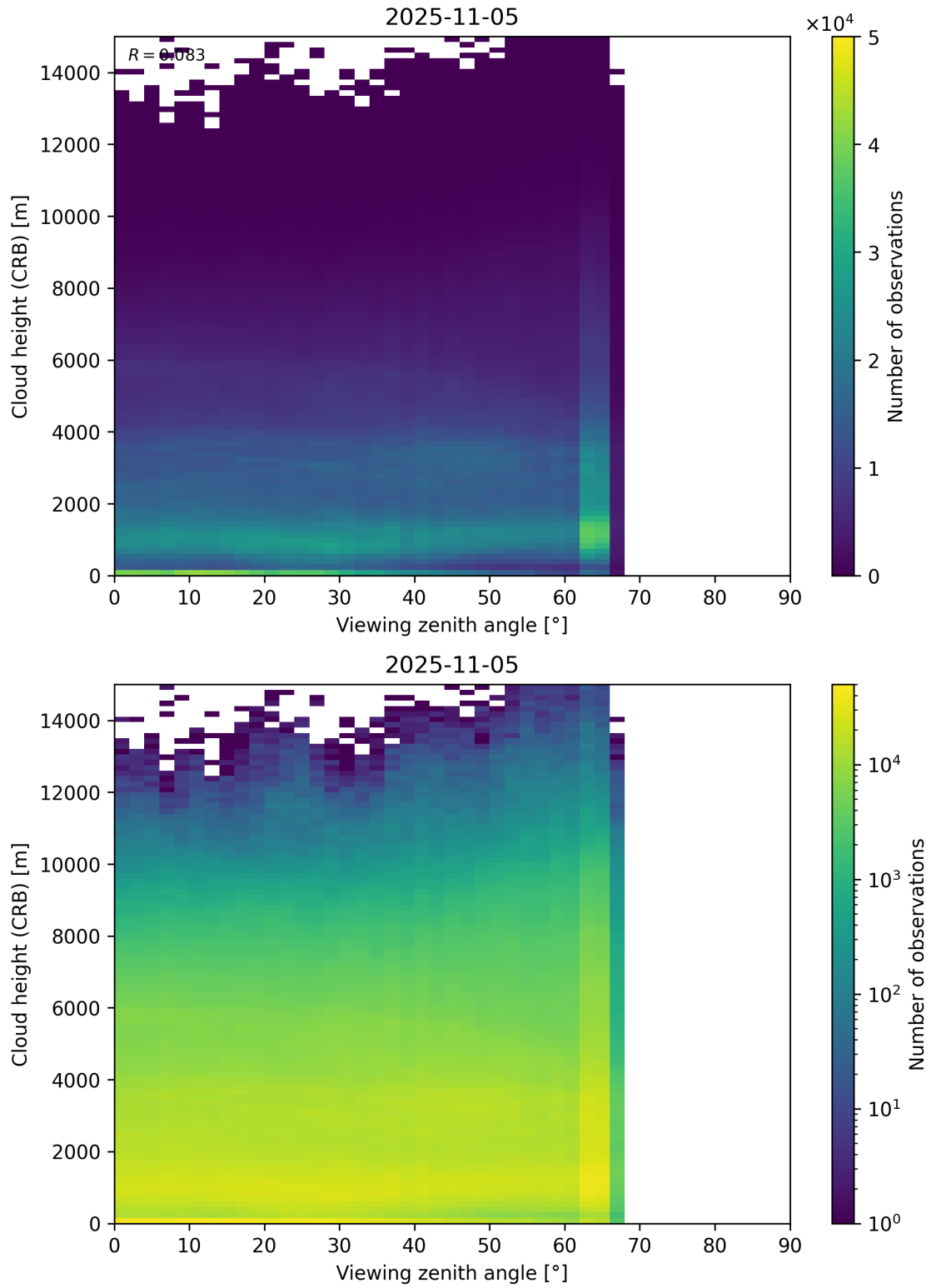
Figure 110: Scatter density plot of “Viewing zenith angle” against “Cloud height (CRB)” for 2025-11-04 to 2025-11-06.
