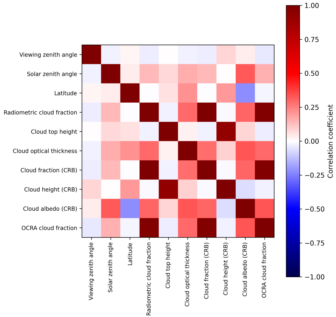
Figure 2: Map of correlation matrix for 2025-11-04 to 2025-11-06.
