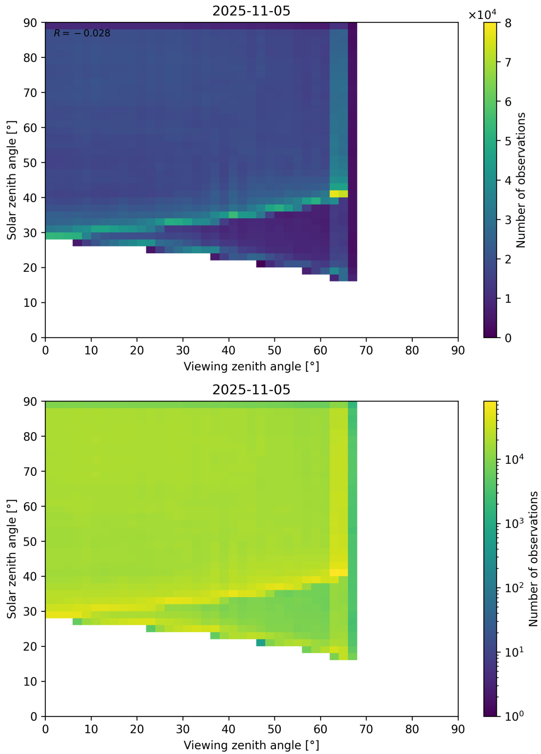
Figure 114: Scatter density plot of “Viewing zenith angle” against “Solar zenith angle” for 2025-11-04 to 2025-11-06.
