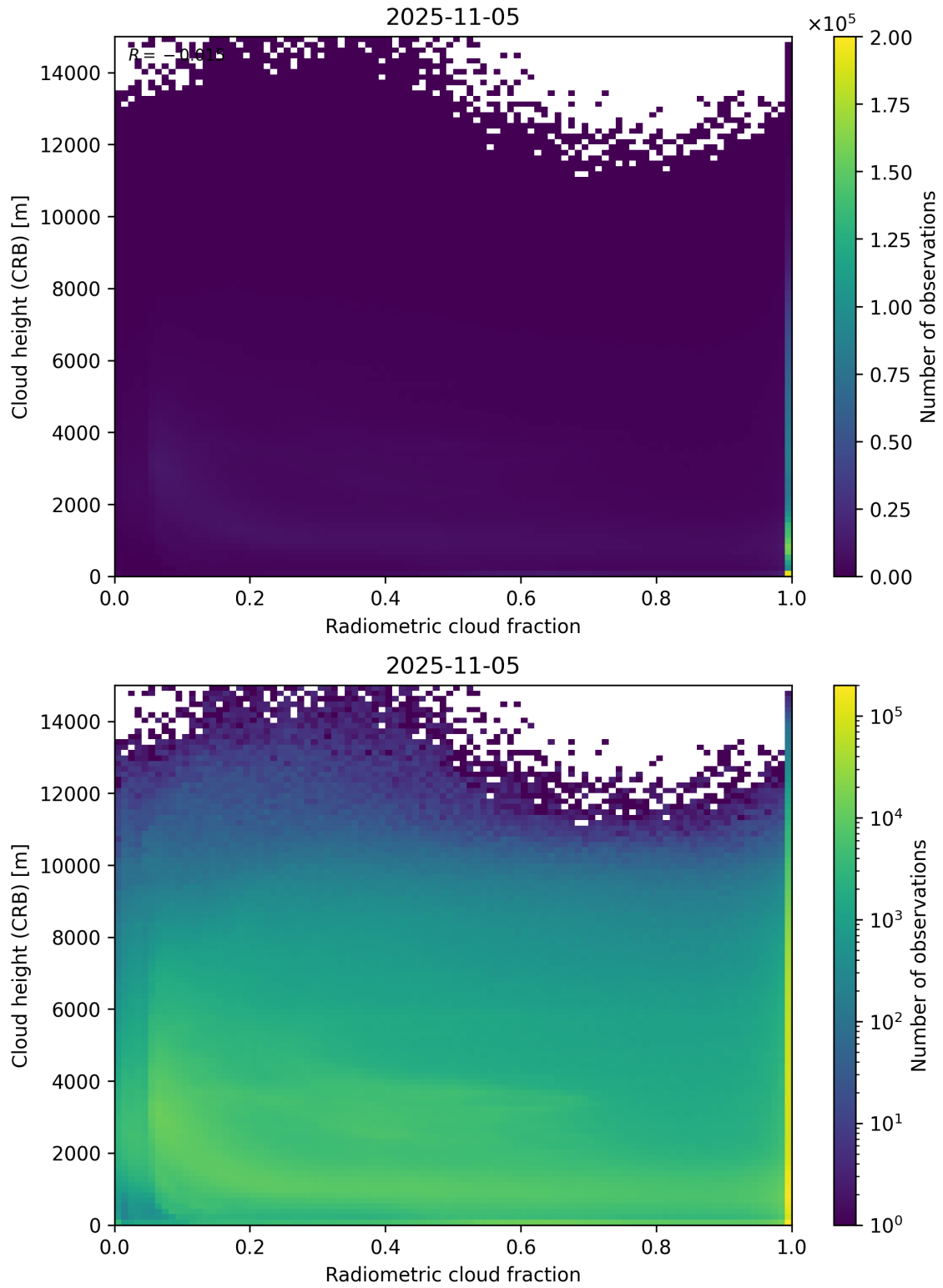
Figure 74: Scatter density plot of “Radiometric cloud fraction” against “Cloud height (CRB)” for 2025-11-04 to 2025-11-06.
