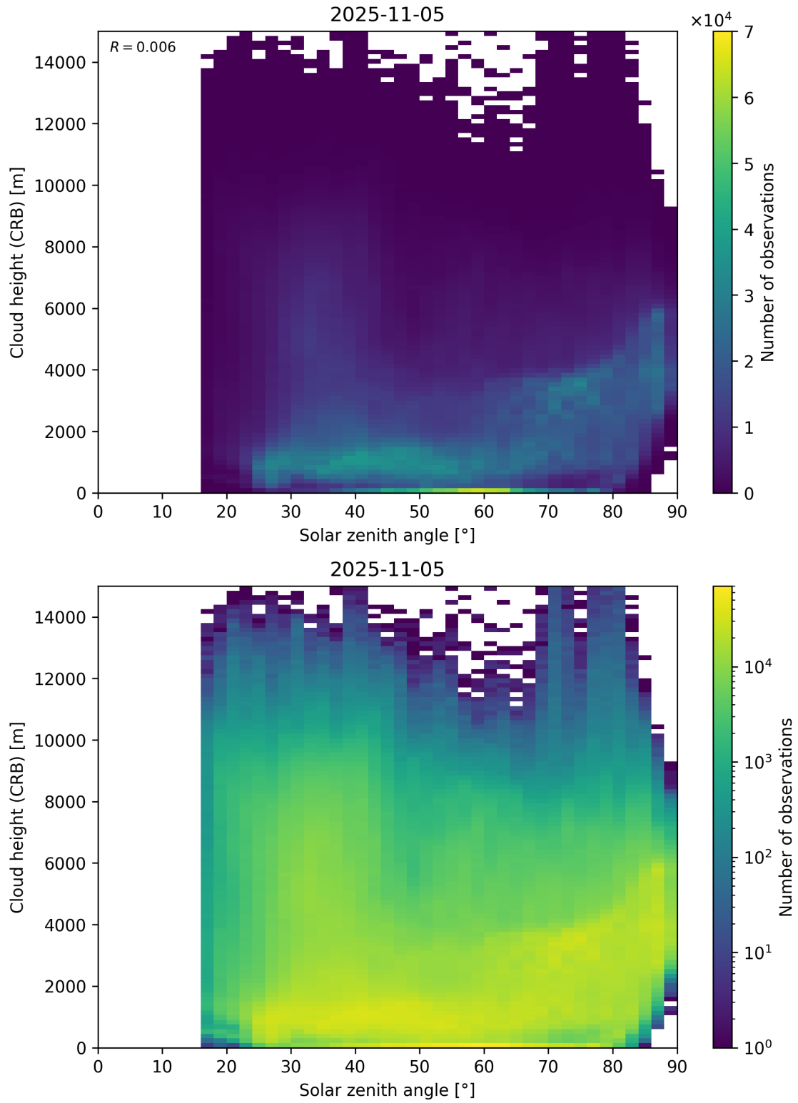
Figure 102: Scatter density plot of “Solar zenith angle” against “Cloud height (CRB)” for 2025-11-04 to 2025-11-06.
