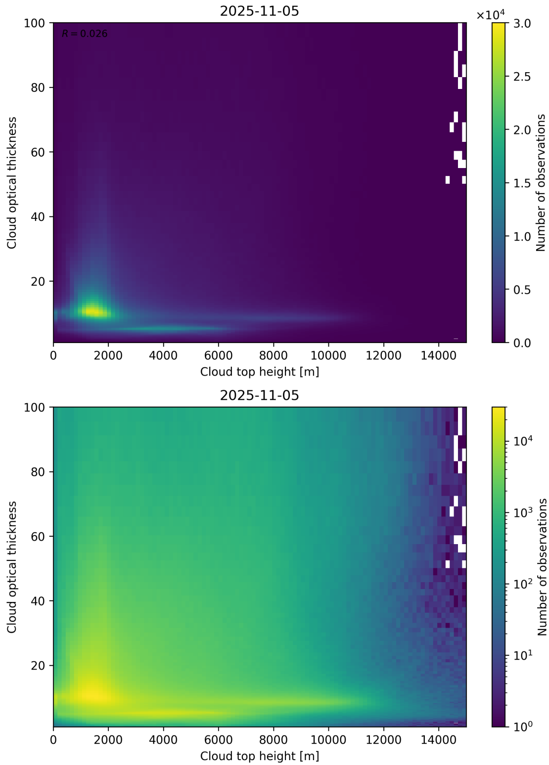
Figure 90: Scatter density plot of “Cloud top height” against “Cloud optical thickness” for 2025-11-04 to 2025-11-06.
