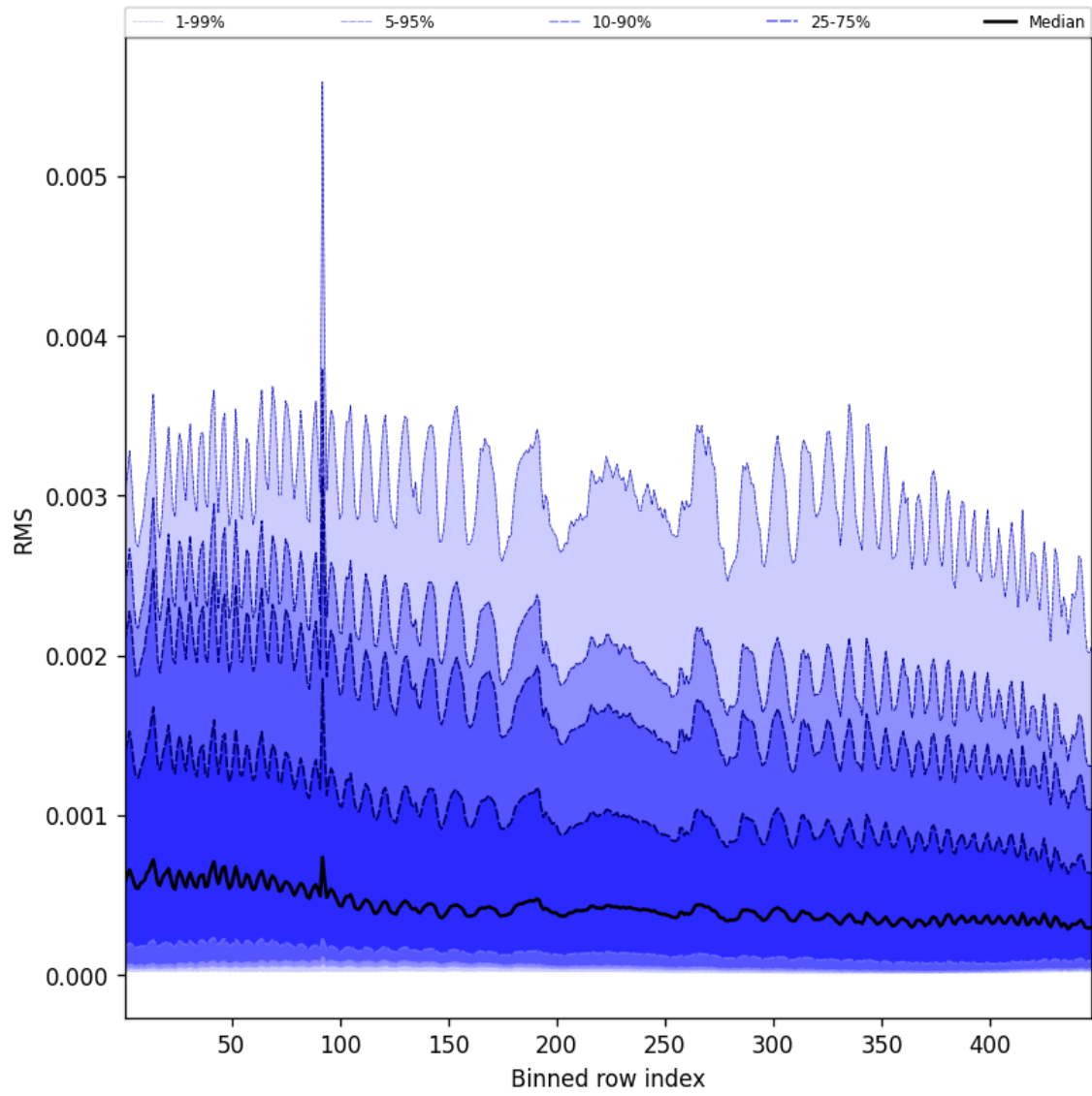
Figure 63: Along track statistics of “RMS” for 2025-11-04 to 2025-11-06
