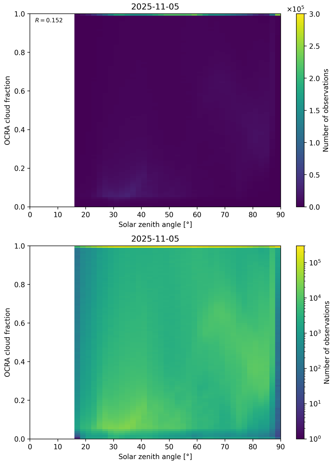
Figure 100: Scatter density plot of “Solar zenith angle” against “OCRA cloud fraction” for 2025-11-04 to 2025-11-06.
