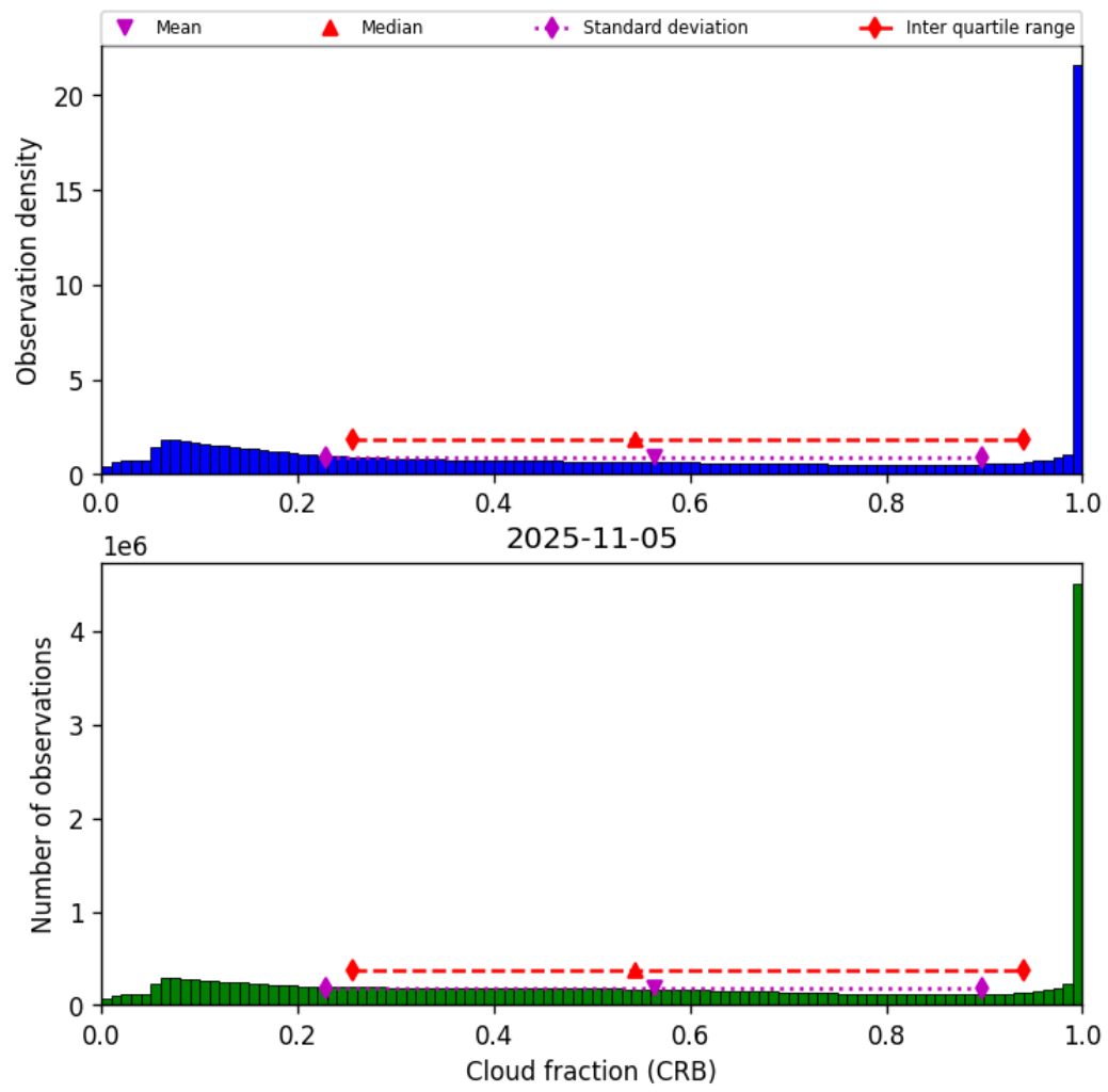
Figure 42: Histogram of “Cloud fraction (CRB)” for 2025-11-04 to 2025-11-06
