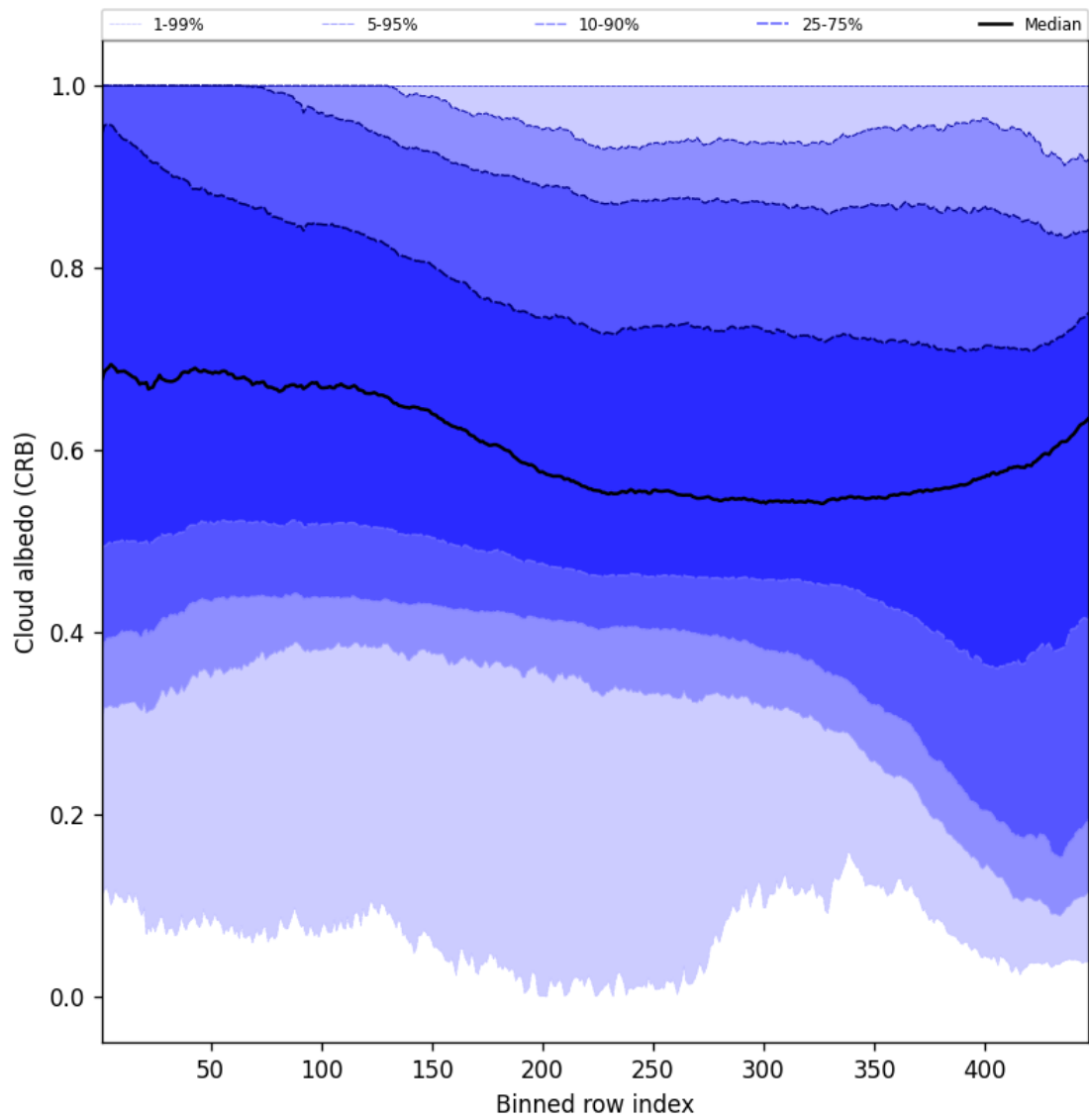
Figure 60: Along track statistics of “Cloud albedo (CRB)” for 2025-11-04 to 2025-11-06
