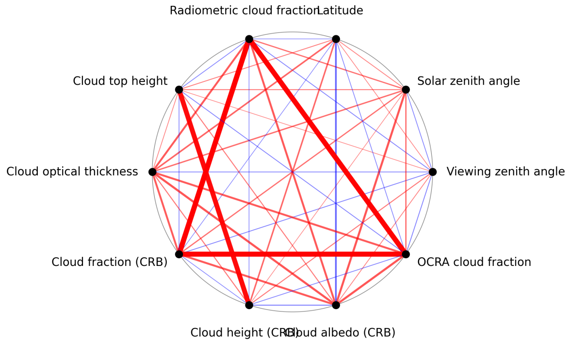
Figure 1: Map of correlation graph for 2025-11-04 to 2025-11-06.
