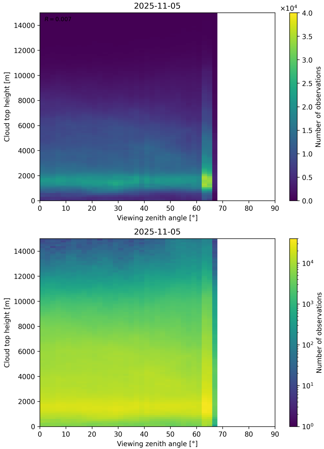
Figure 112: Scatter density plot of “Viewing zenith angle” against “Cloud top height” for 2025-11-04 to 2025-11-06.
