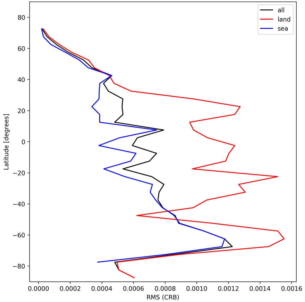
Figure 32: Zonal average of “RMS (CRB)” for 2025-11-04 to 2025-11-06.
