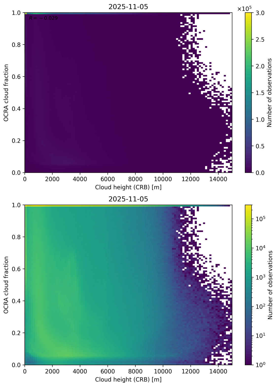
Figure 81: Scatter density plot of “Cloud height (CRB)” against “OCRA cloud fraction” for 2025-11-04 to 2025-11-06.
