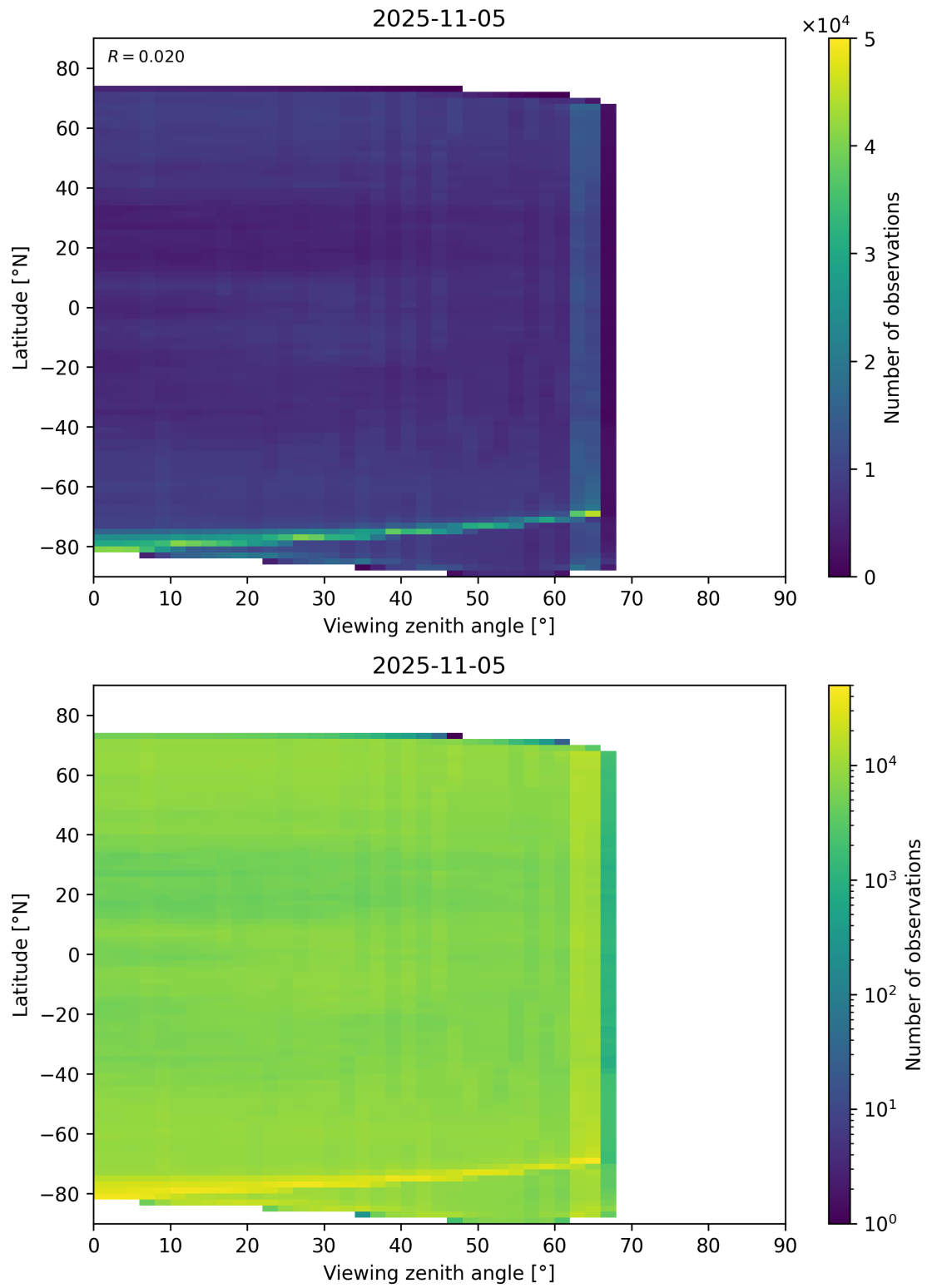
Figure 113: Scatter density plot of “Viewing zenith angle” against “Latitude” for 2025-11-04 to 2025-11-06.
