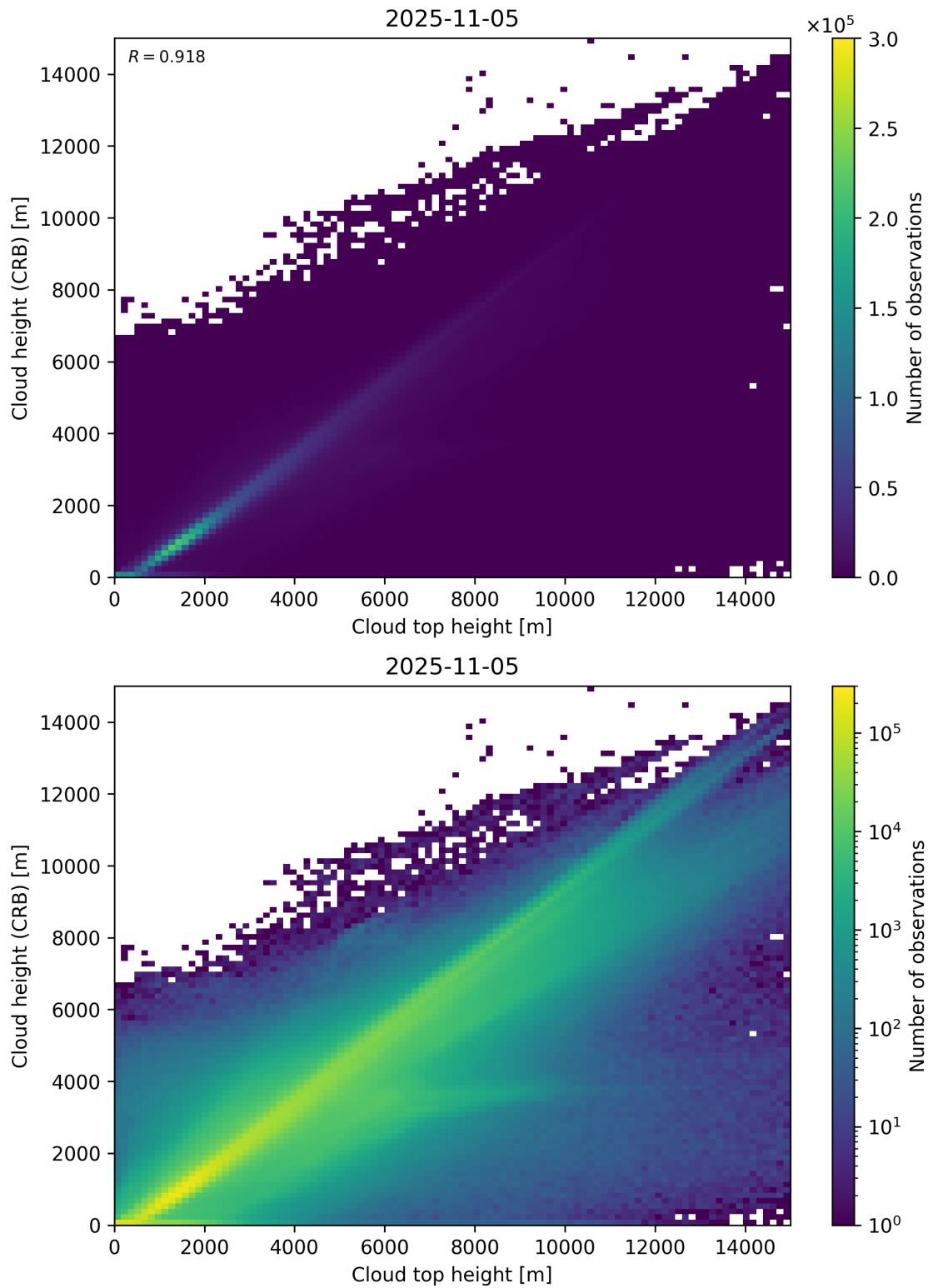
Figure 89: Scatter density plot of “Cloud top height” against “Cloud height (CRB)” for 2025-11-04 to 2025-11-06.
