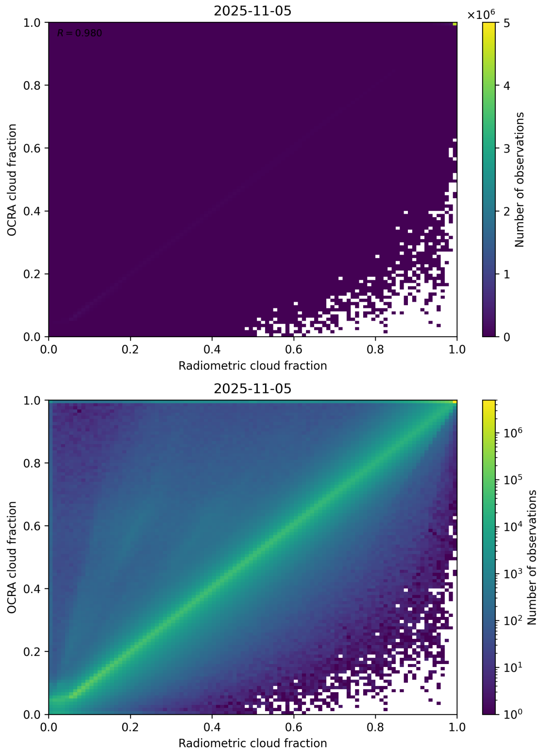
Figure 72: Scatter density plot of “Radiometric cloud fraction” against “OCRA cloud fraction” for 2025-11-04 to 2025-11-06.
