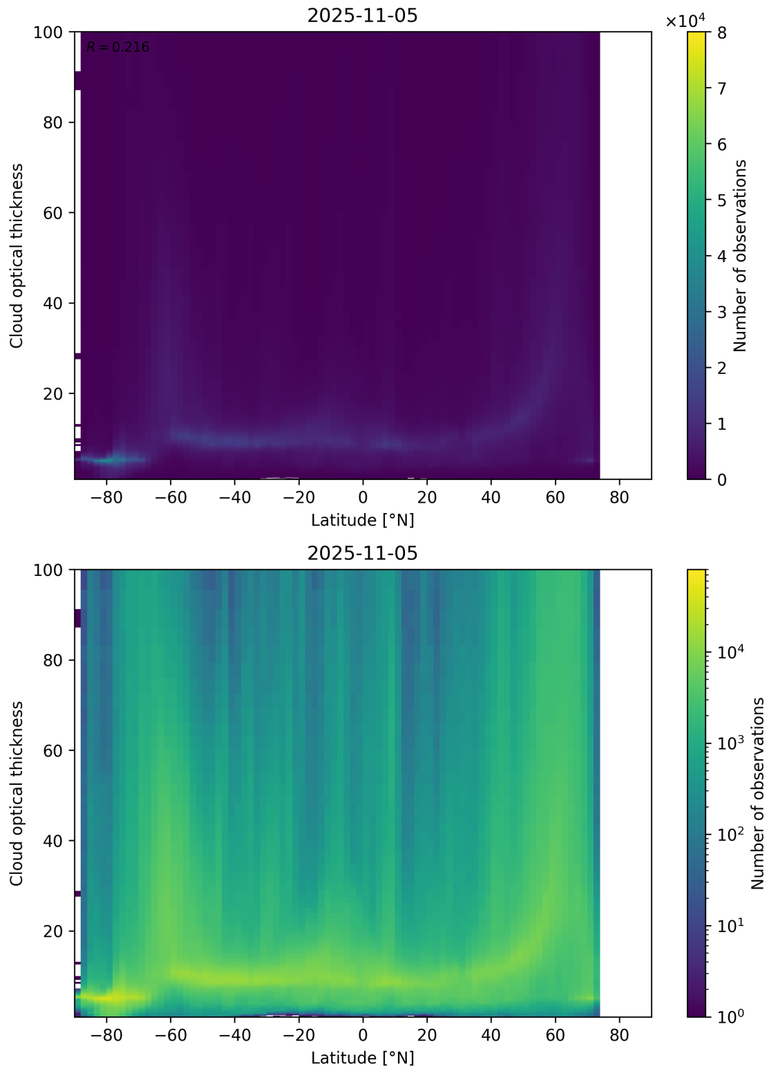
Figure 96: Scatter density plot of “Latitude” against “Cloud optical thickness” for 2025-11-04 to 2025-11-06.
