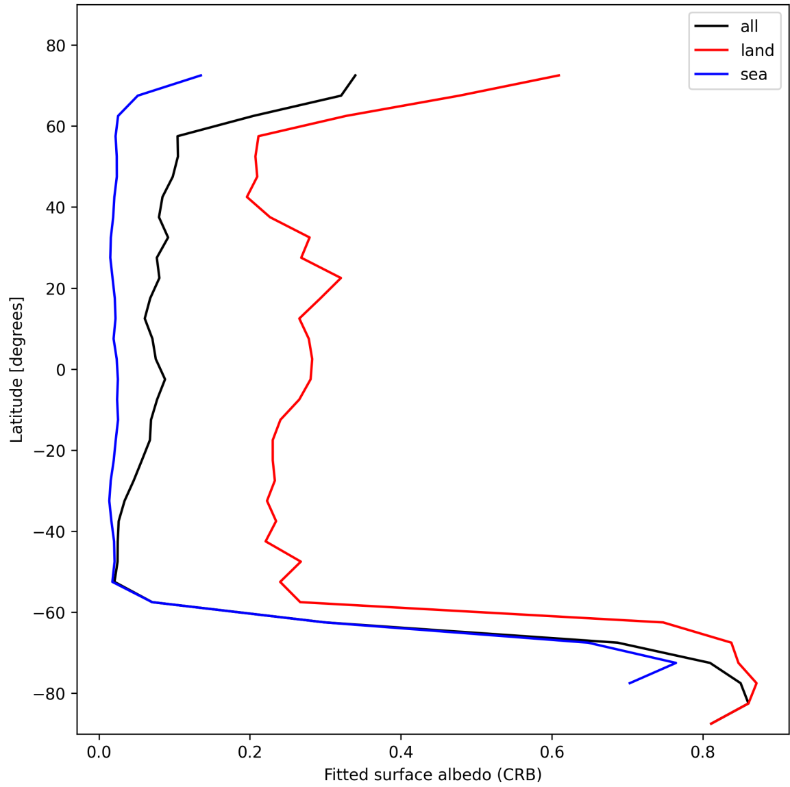
Figure 30: Zonal average of “Fitted surface albedo (CRB)” for 2025-11-04 to 2025-11-06.
