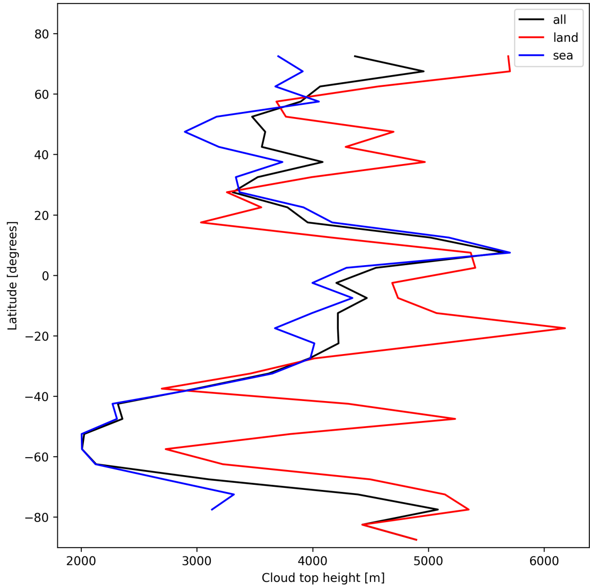
Figure 24: Zonal average of “Cloud top height” for 2025-11-04 to 2025-11-06.
