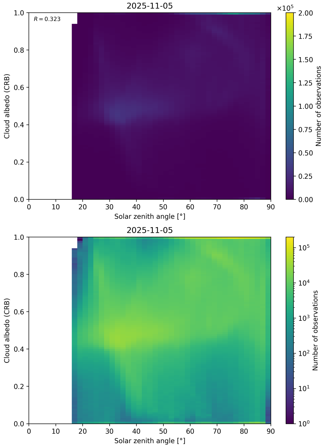
Figure 98: Scatter density plot of “Solar zenith angle” against “Cloud albedo (CRB)” for 2025-11-04 to 2025-11-06.
