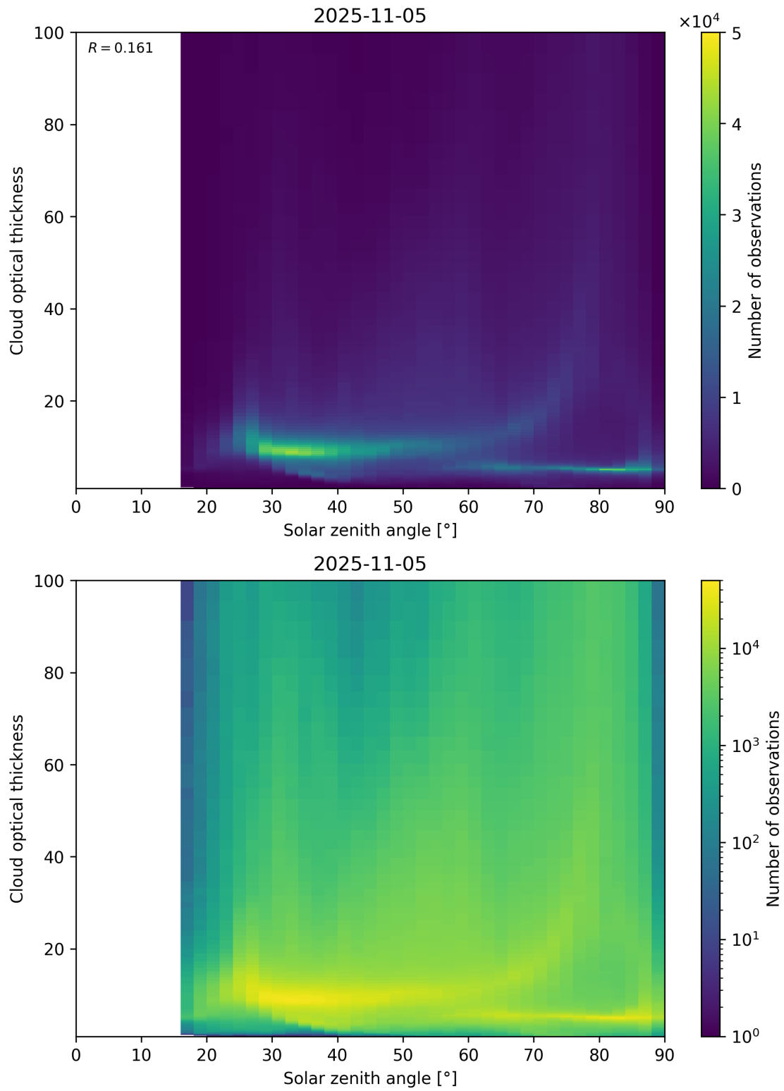
Figure 103: Scatter density plot of “Solar zenith angle” against “Cloud optical thickness” for 2025-11-04 to 2025-11-06.
