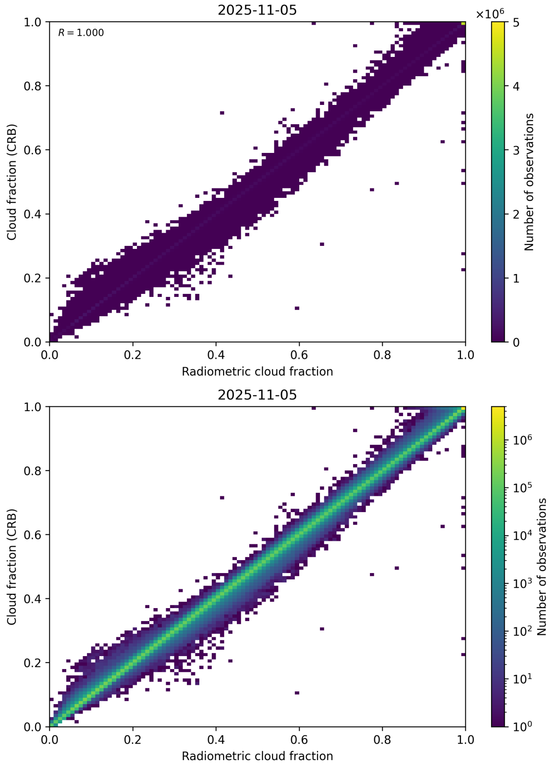
Figure 73: Scatter density plot of “Radiometric cloud fraction” against “Cloud fraction (CRB)” for 2025-11-04 to 2025-11-06.
