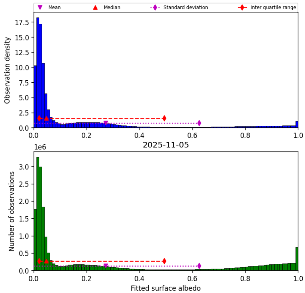
Figure 45: Histogram of “Fitted surface albedo” for 2025-11-04 to 2025-11-06
