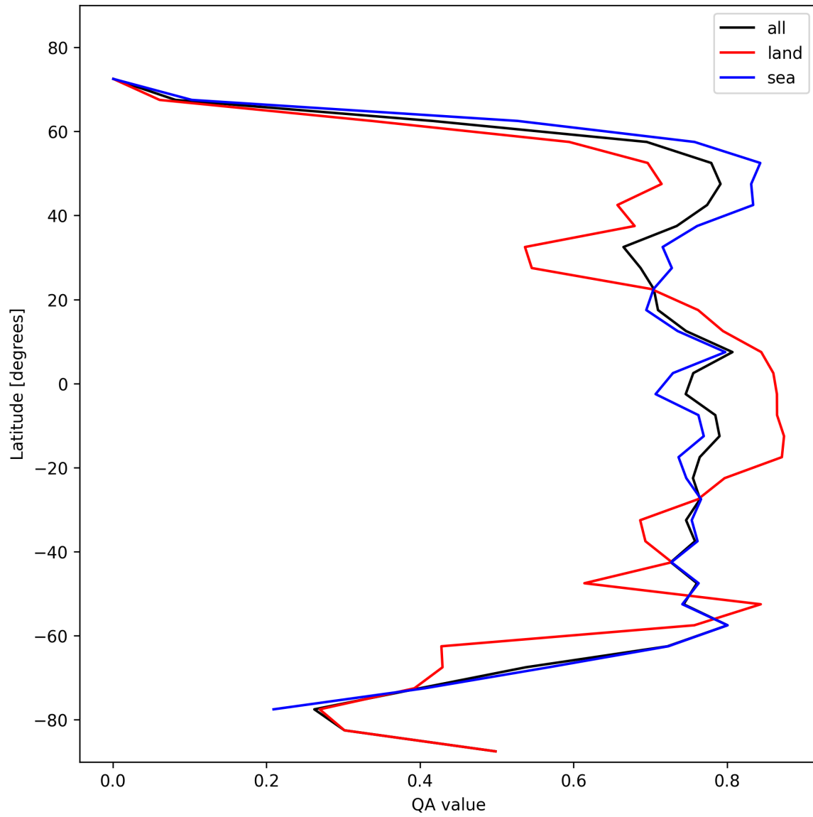
Figure 22: Zonal average of “QA value” for 2025-11-04 to 2025-11-06.
