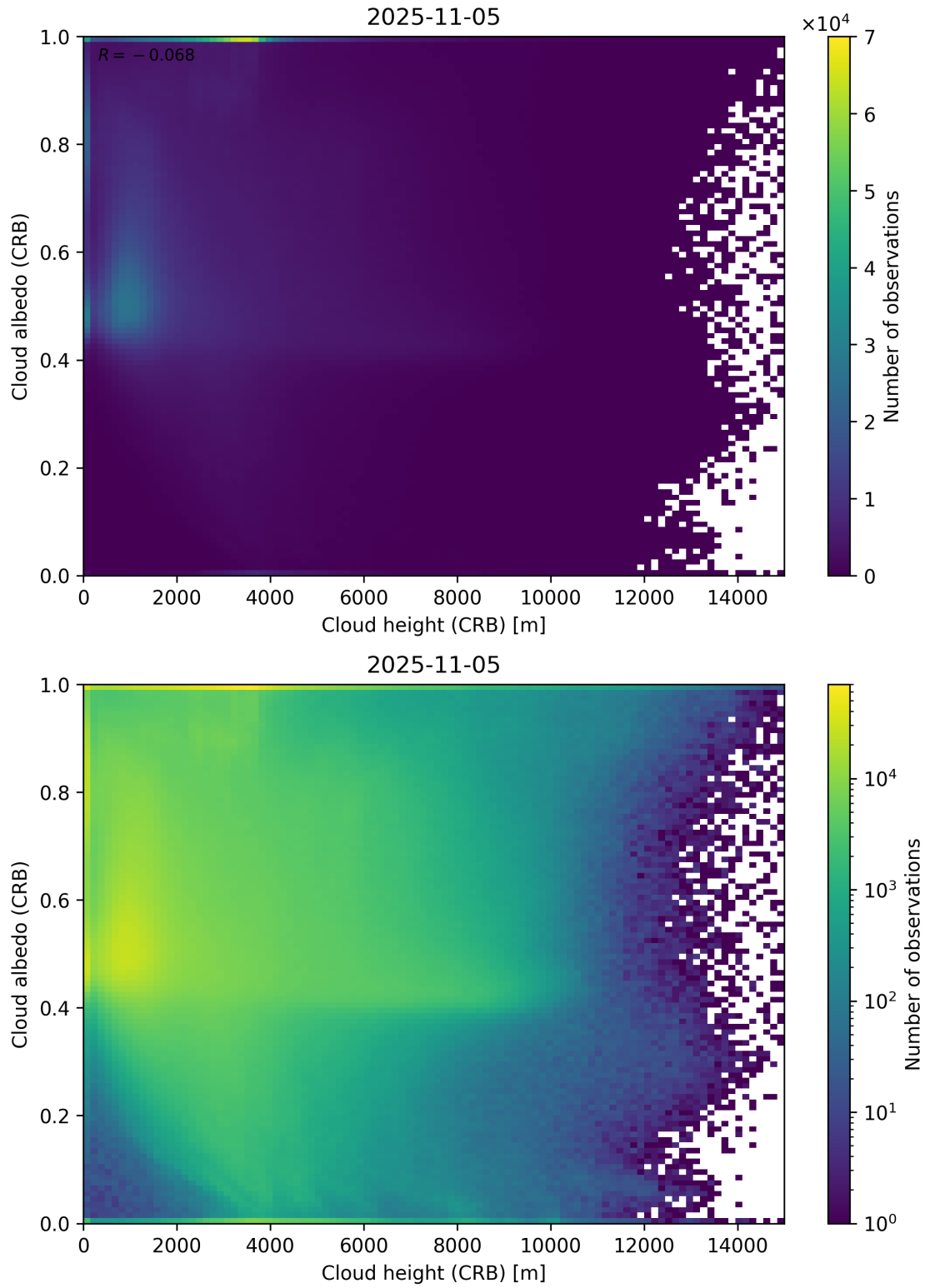
Figure 80: Scatter density plot of “Cloud height (CRB)” against “Cloud albedo (CRB)” for 2025-11-04 to 2025-11-06.
