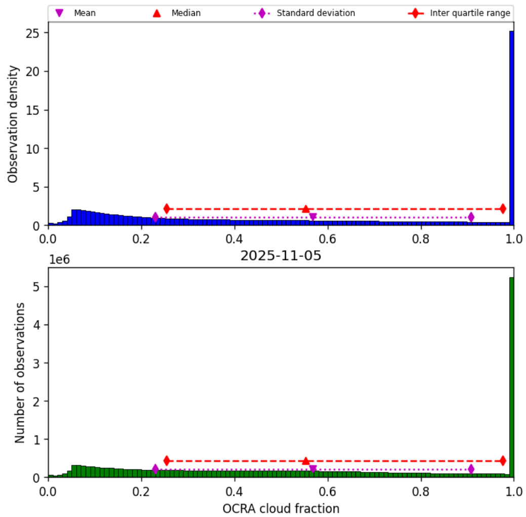
Figure 50: Histogram of “OCRA cloud fraction” for 2025-11-04 to 2025-11-06
