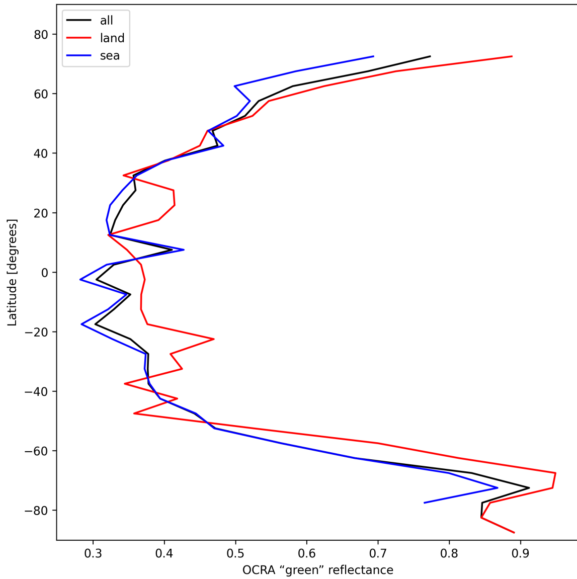
Figure 36: Zonal average of “OCRA “green” reflectance” for 2025-11-04 to 2025-11-06.
