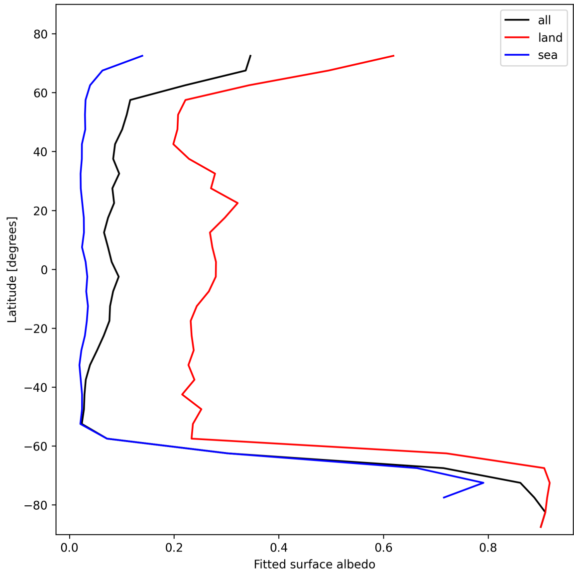
Figure 29: Zonal average of “Fitted surface albedo” for 2025-11-04 to 2025-11-06.
