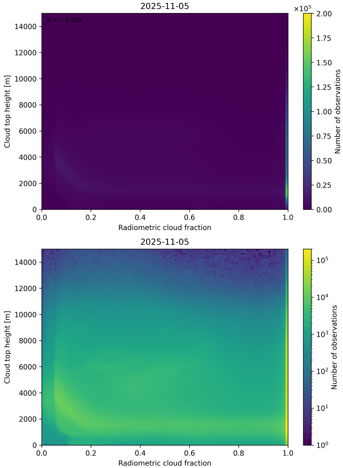
Figure 76: Scatter density plot of “Radiometric cloud fraction” against “Cloud top height” for 2025-11-04 to 2025-11-06.
