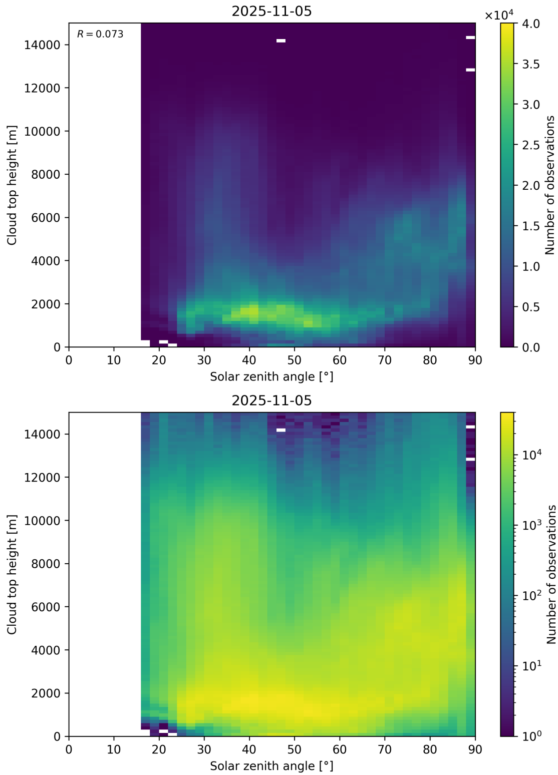
Figure 104: Scatter density plot of “Solar zenith angle” against “Cloud top height” for 2025-11-04 to 2025-11-06.
