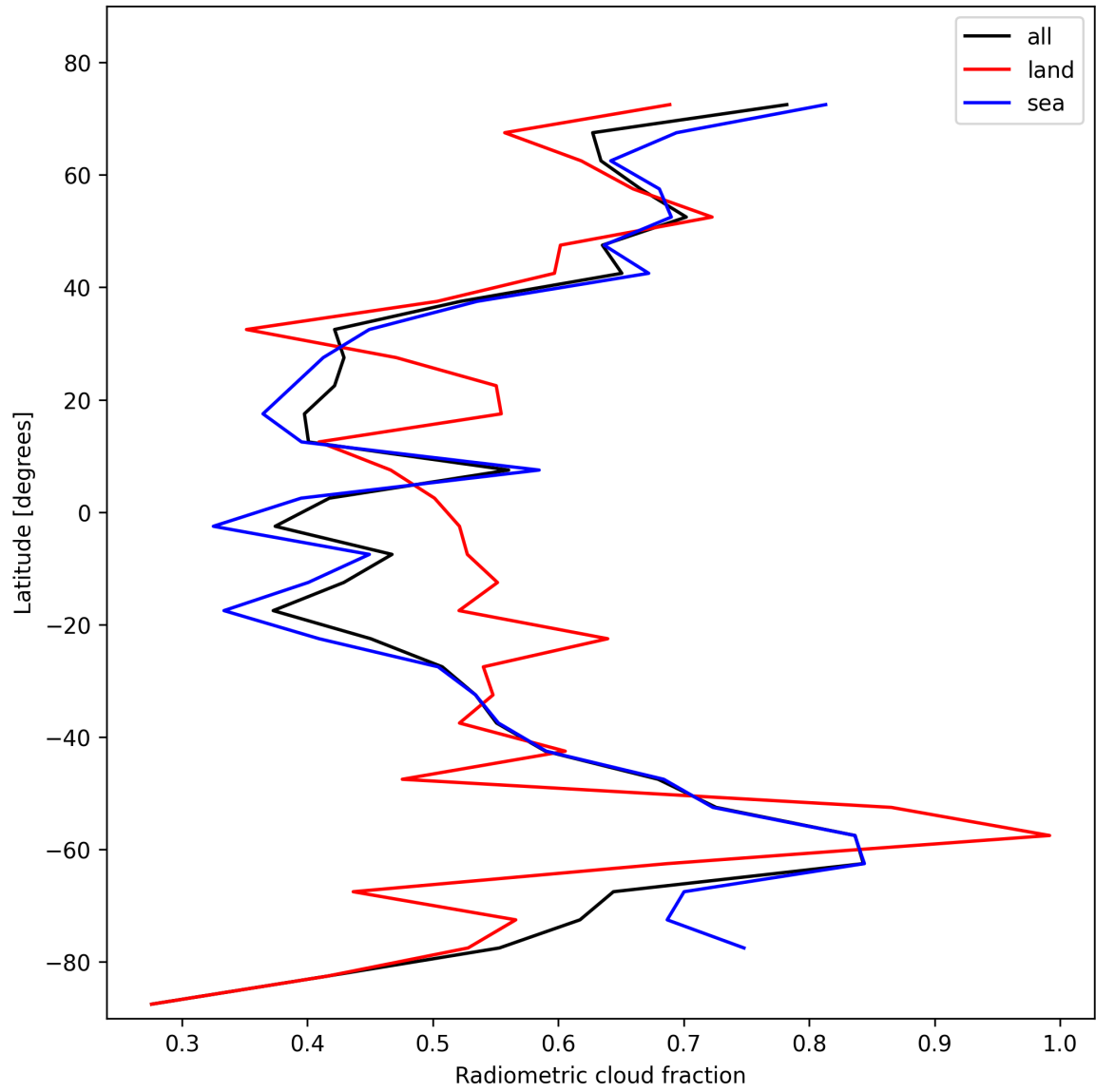
Figure 23: Zonal average of “Radiometric cloud fraction” for 2025-11-04 to 2025-11-06.
