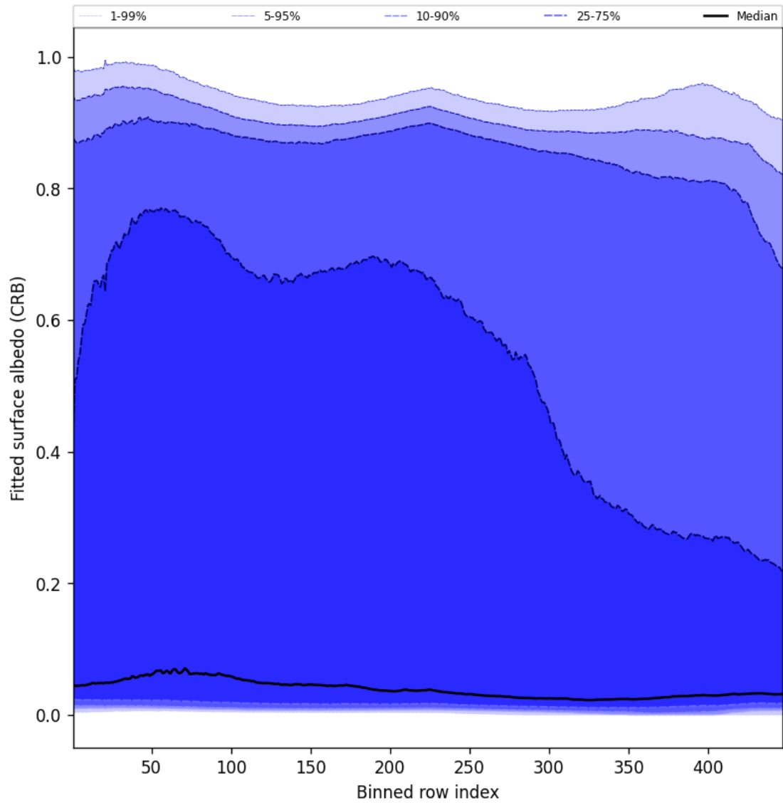
Figure 62: Along track statistics of “Fitted surface albedo (CRB)” for 2025-11-04 to 2025-11-06
