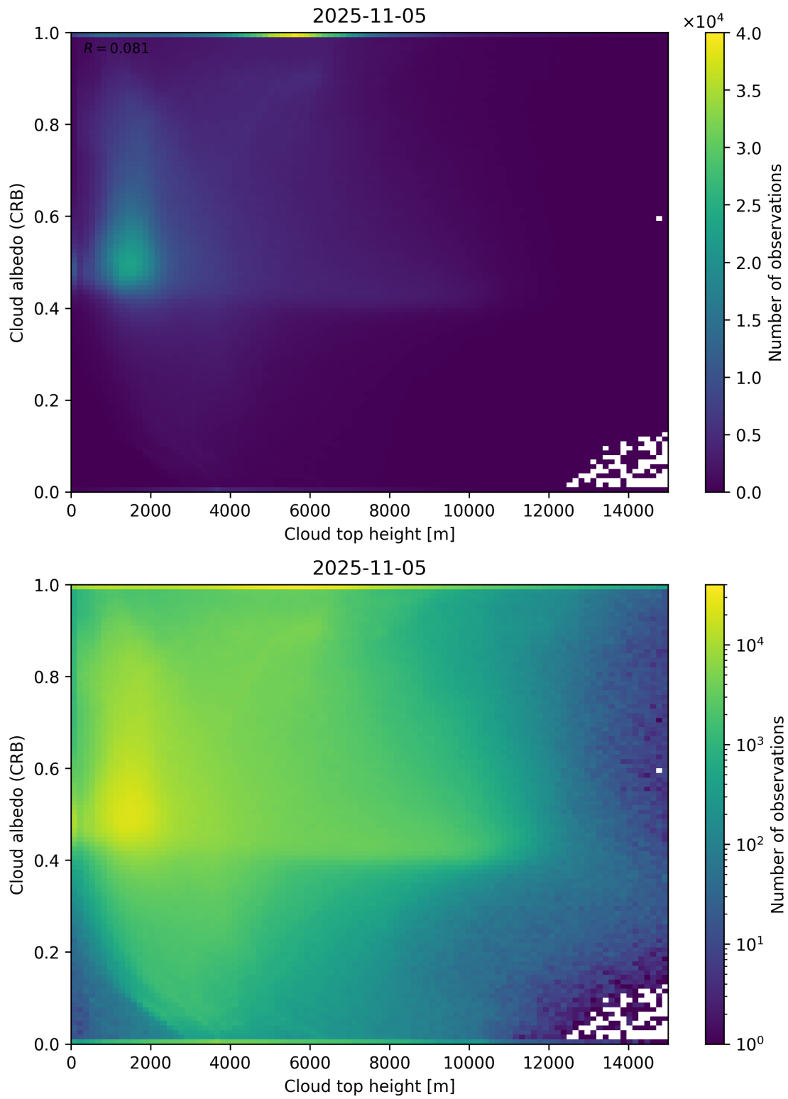
Figure 86: Scatter density plot of “Cloud top height” against “Cloud albedo (CRB)” for 2025-11-04 to 2025-11-06.
