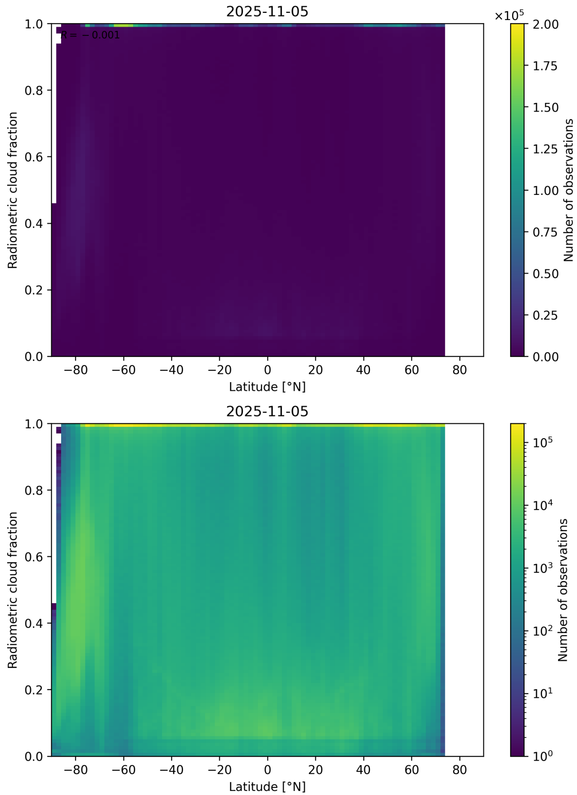
Figure 92: Scatter density plot of “Latitude” against “Radiometric cloud fraction” for 2025-11-04 to 2025-11-06.
