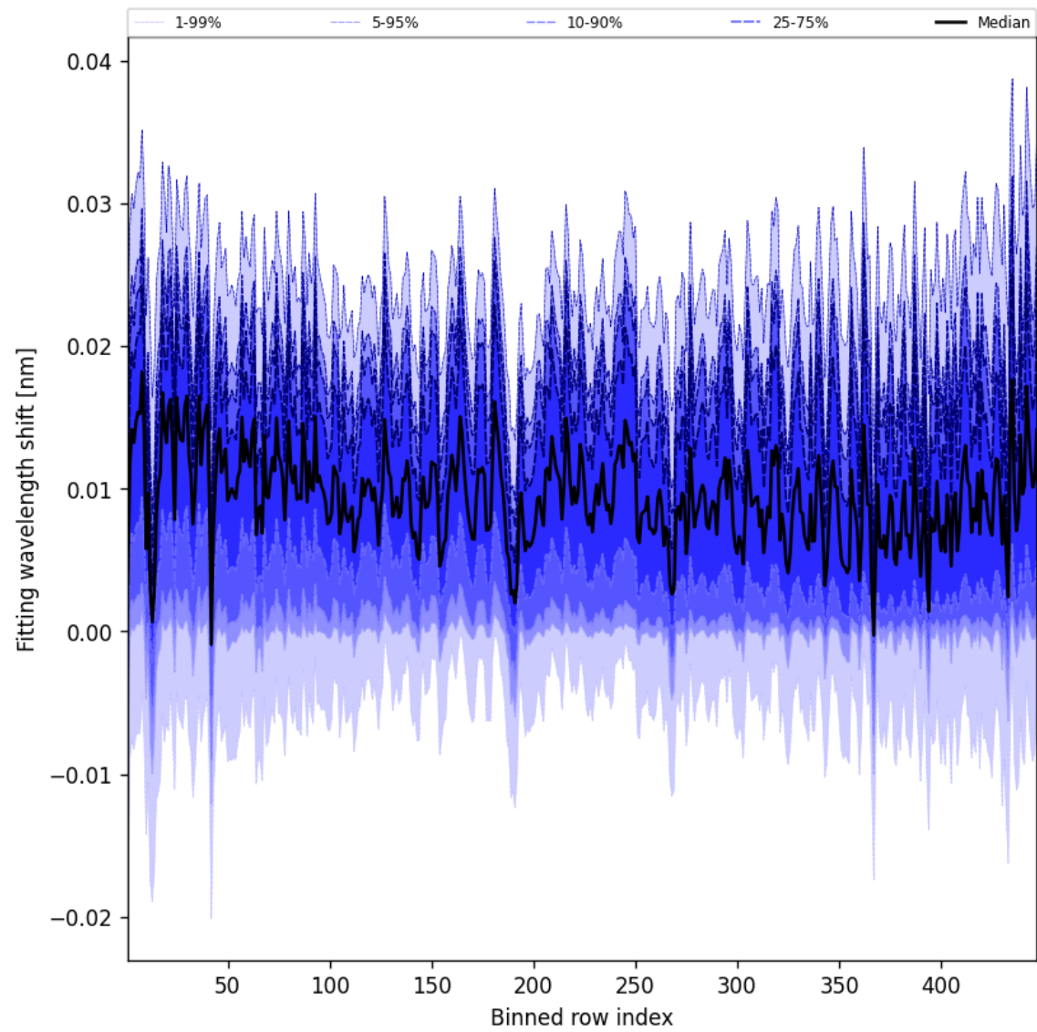
Figure 65: Along track statistics of “Fitting wavelength shift” for 2025-11-04 to 2025-11-06
