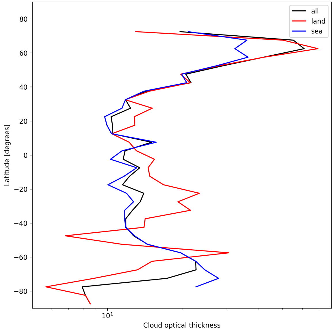
Figure 25: Zonal average of “Cloud optical thickness” for 2025-11-04 to 2025-11-06.
