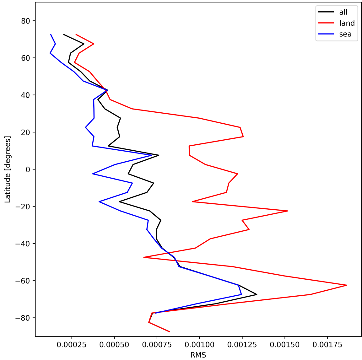
Figure 31: Zonal average of “RMS” for 2025-11-04 to 2025-11-06.
