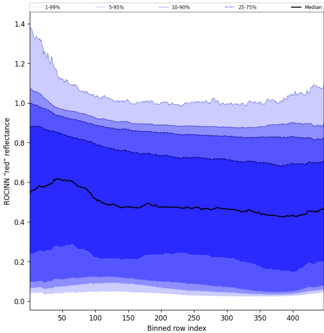
Figure 69: Along track statistics of “ROCINN “red” reflectance” for 2025-11-04 to 2025-11-06
