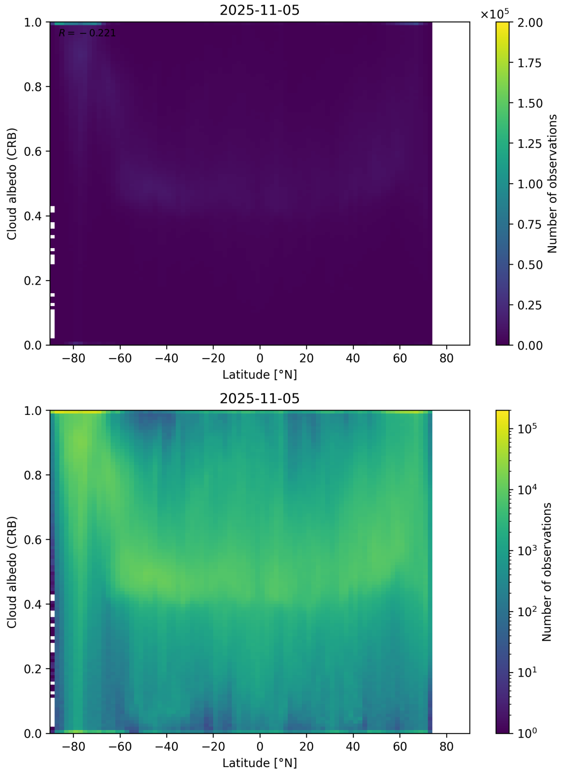
Figure 91: Scatter density plot of “Latitude” against “Cloud albedo (CRB)” for 2025-11-04 to 2025-11-06.
