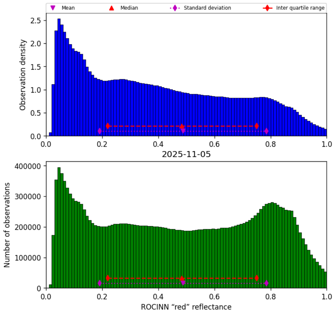
Figure 53: Histogram of “ROCINN “red” reflectance” for 2025-11-04 to 2025-11-06
