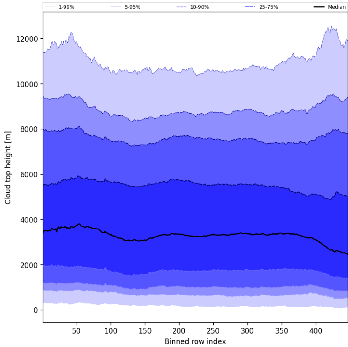
Figure 56: Along track statistics of “Cloud top height” for 2025-11-04 to 2025-11-06
