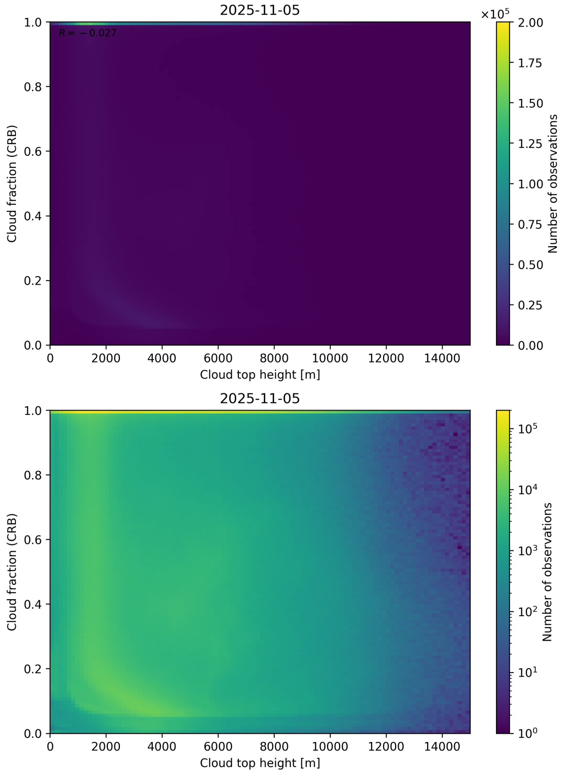
Figure 88: Scatter density plot of “Cloud top height” against “Cloud fraction (CRB)” for 2025-11-04 to 2025-11-06.
