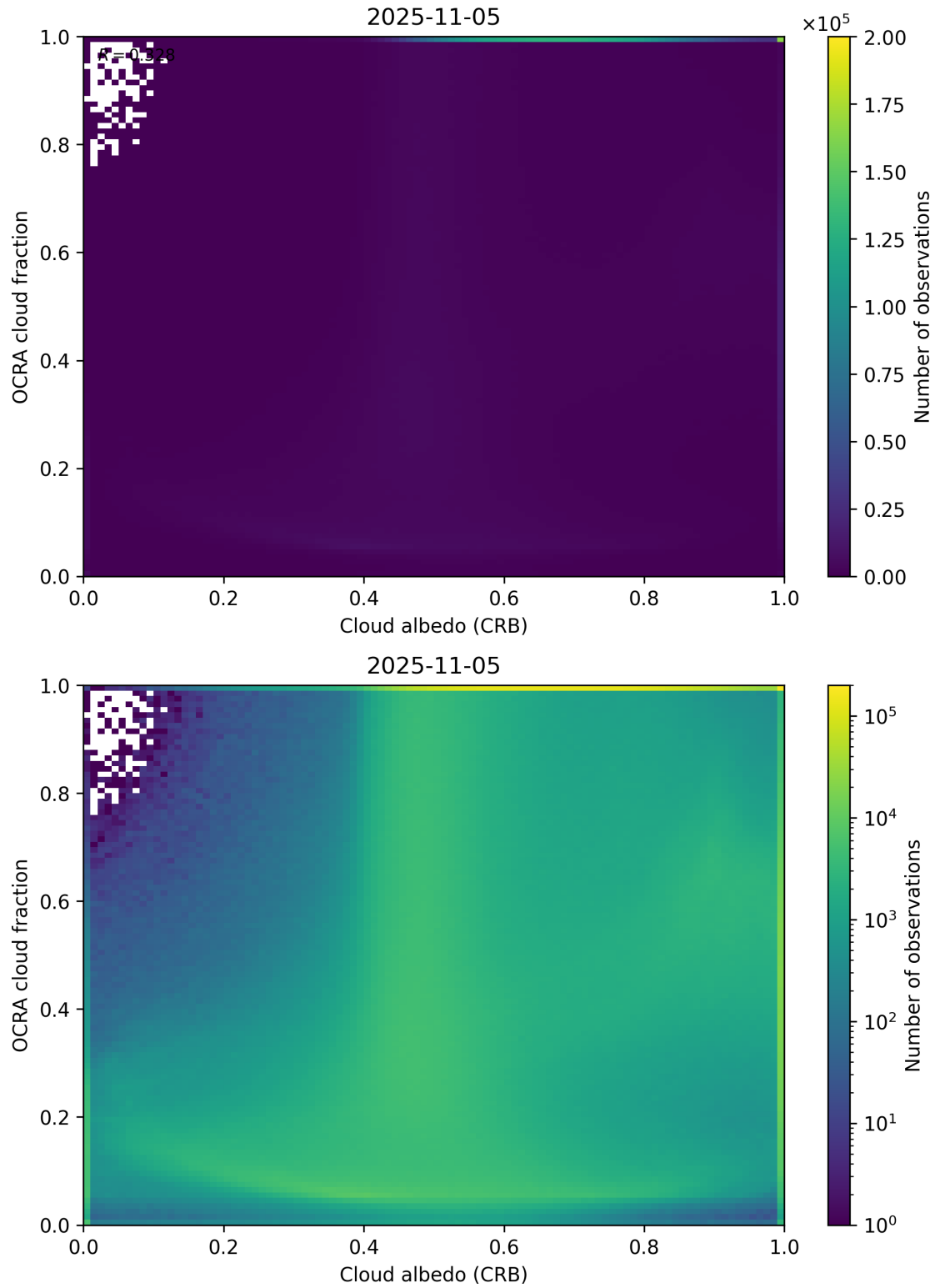
Figure 70: Scatter density plot of “Cloud albedo (CRB)” against “OCRA cloud fraction” for 2025-11-04 to 2025-11-06.
