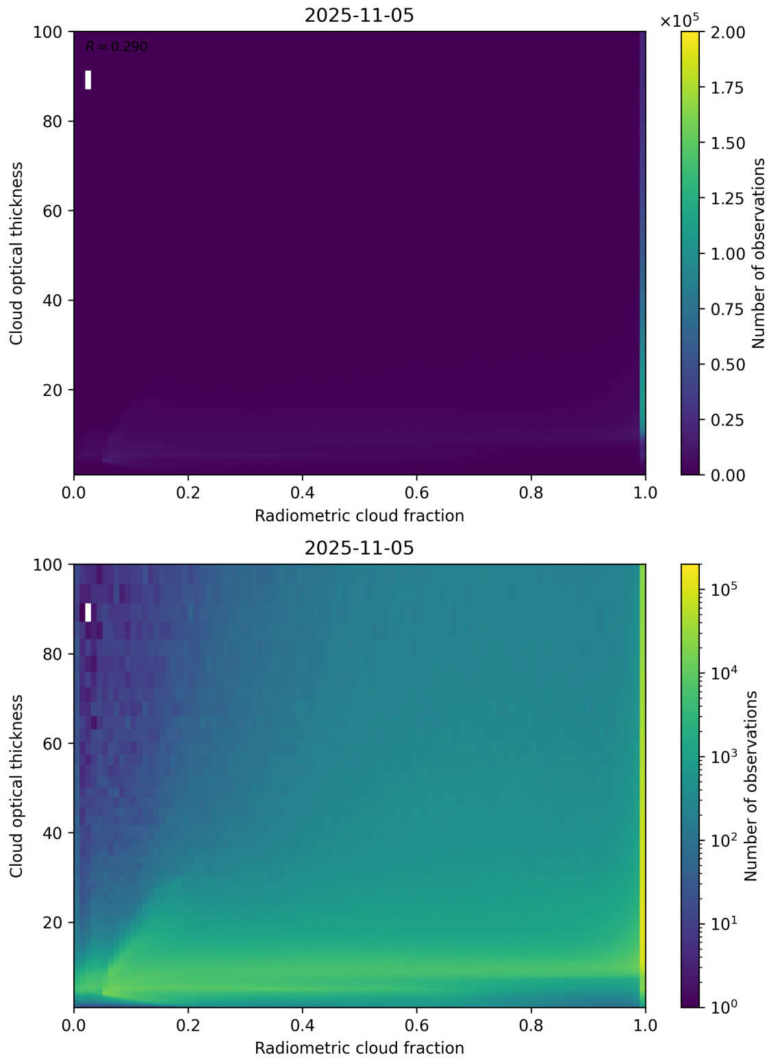
Figure 75: Scatter density plot of “Radiometric cloud fraction” against “Cloud optical thickness” for 2025-11-04 to 2025-11-06.
