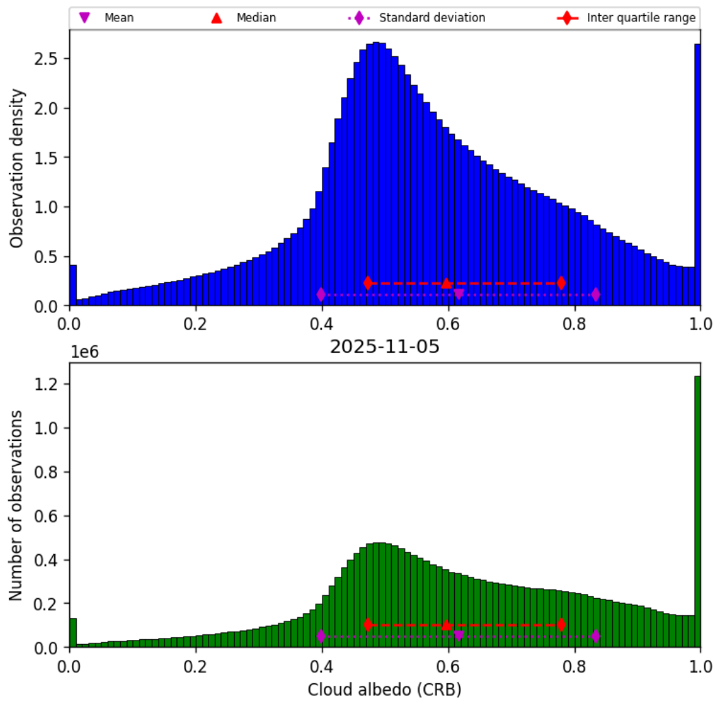
Figure 44: Histogram of “Cloud albedo (CRB)” for 2025-11-04 to 2025-11-06
