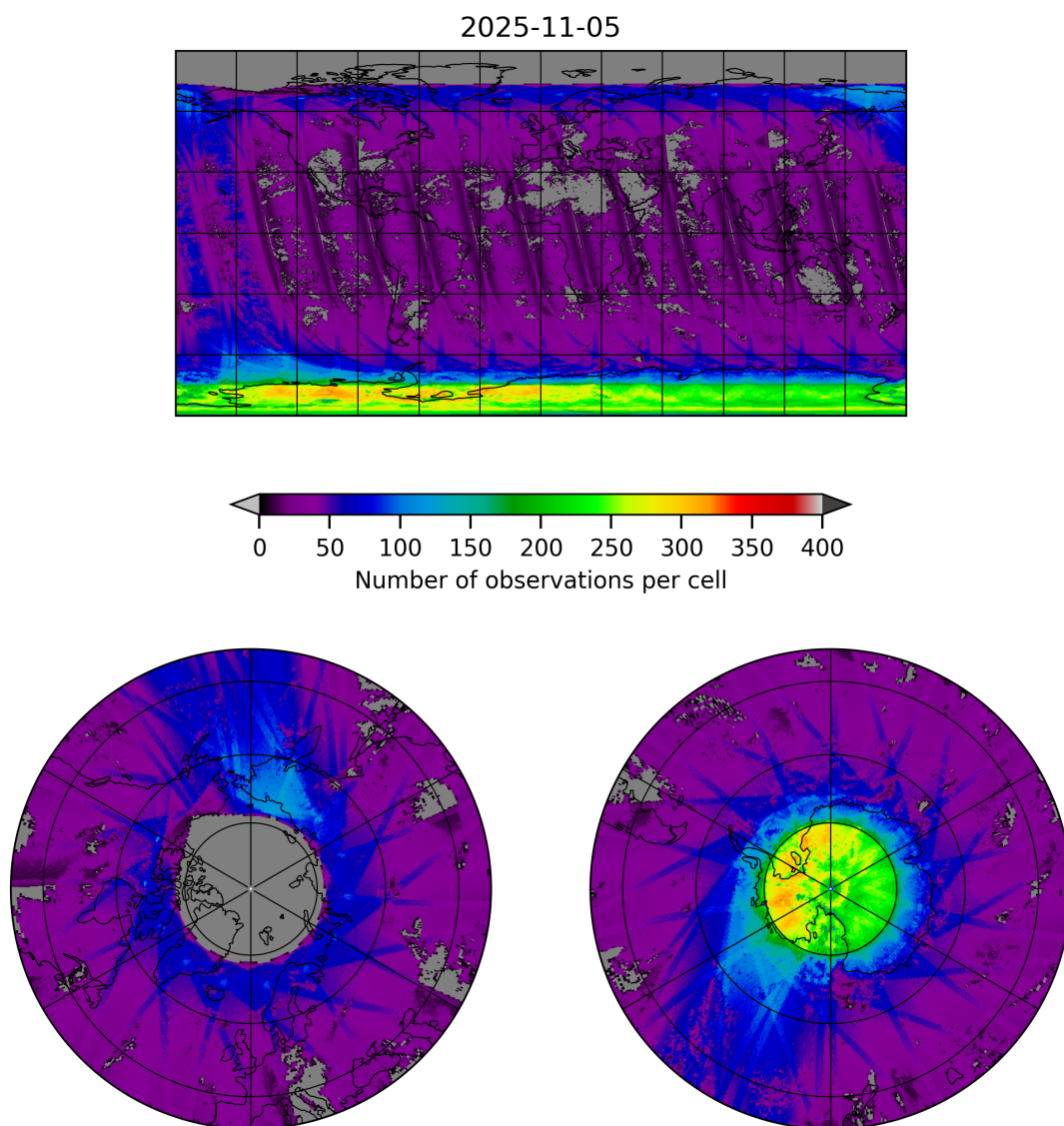
Figure 21: Map of the number of observations for 2025-11-04 to 2025-11-06
