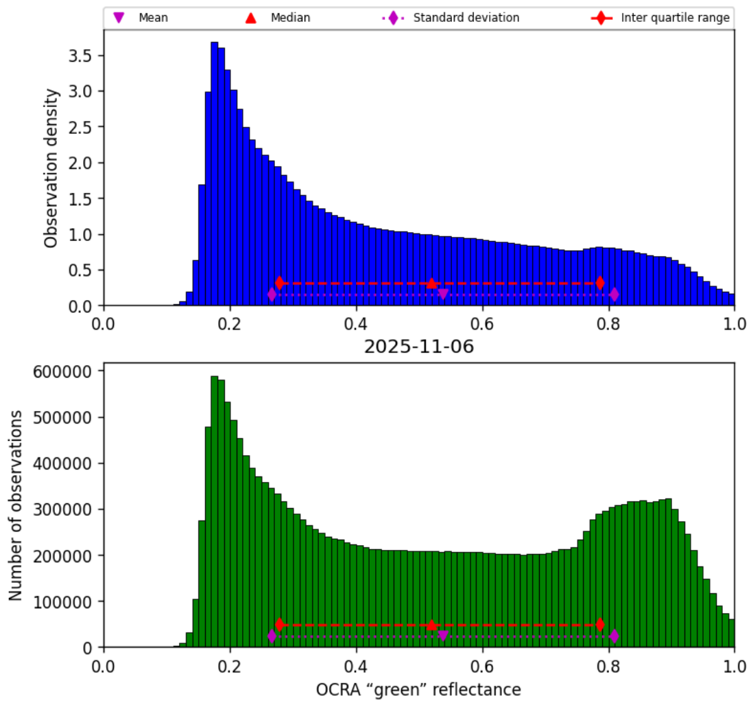
Figure 52: Histogram of “OCRA “green” reflectance” for 2025-11-05 to 2025-11-07
