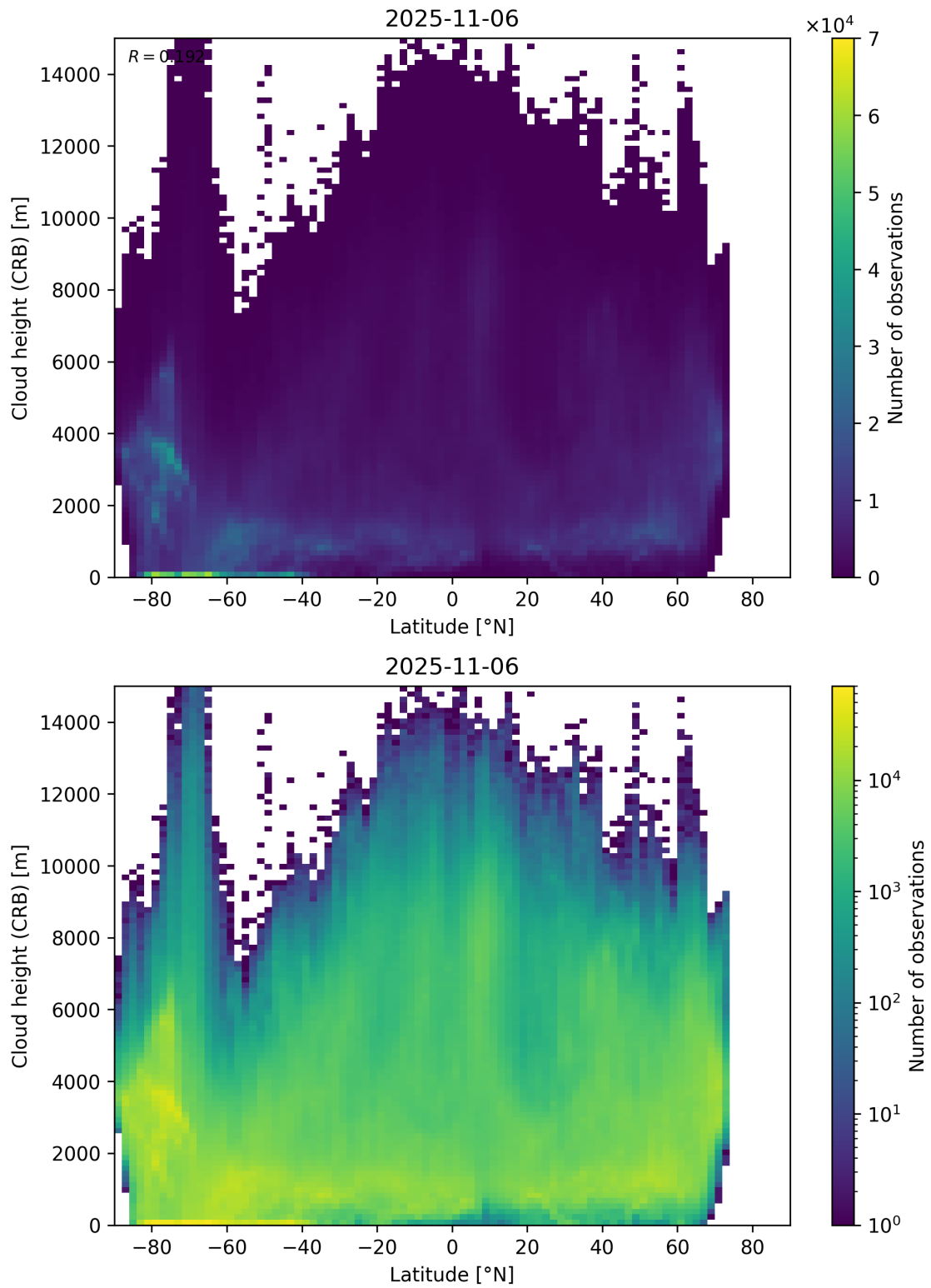
Figure 95: Scatter density plot of “Latitude” against “Cloud height (CRB)” for 2025-11-05 to 2025-11-07.
