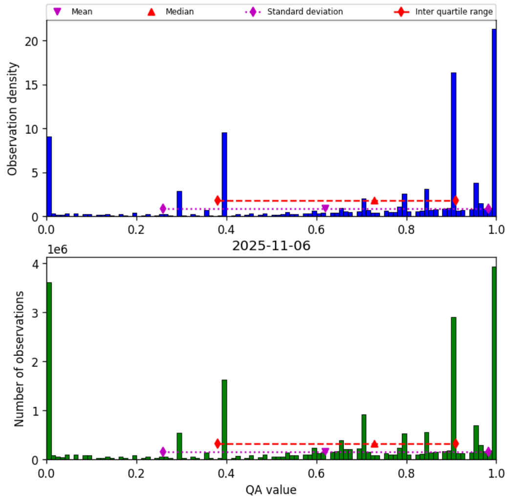
Figure 38: Histogram of “QA value” for 2025-11-05 to 2025-11-07
