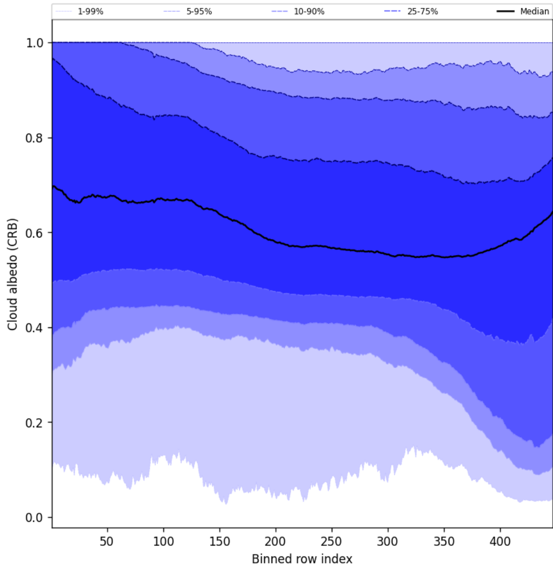
Figure 60: Along track statistics of “Cloud albedo (CRB)” for 2025-11-05 to 2025-11-07
