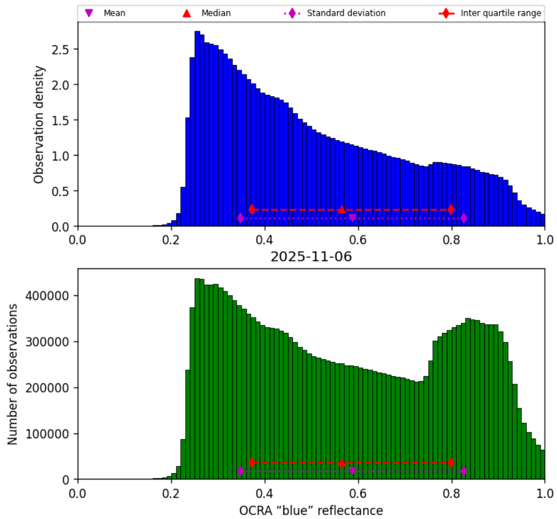
Figure 51: Histogram of “OCRA “blue” reflectance” for 2025-11-05 to 2025-11-07
