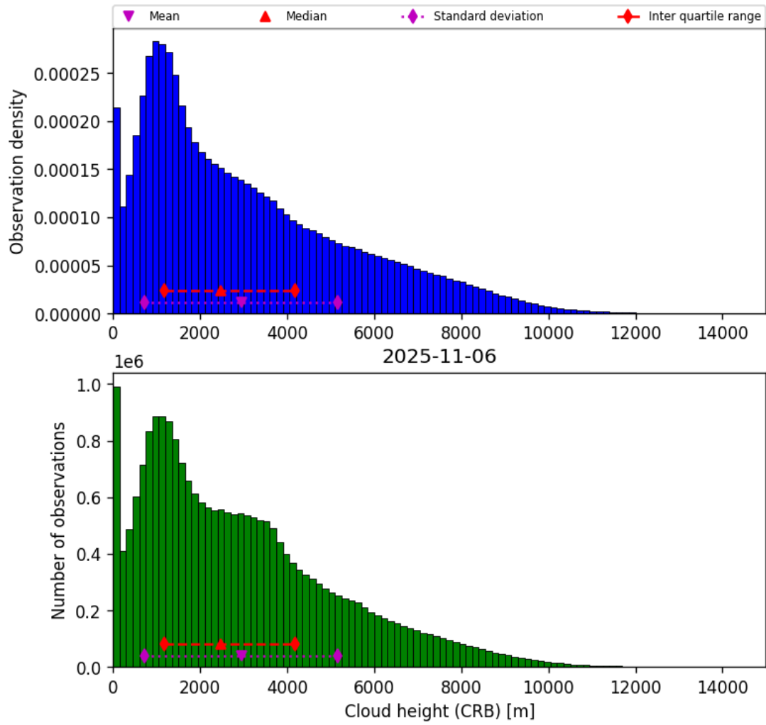
Figure 43: Histogram of “Cloud height (CRB)” for 2025-11-05 to 2025-11-07
