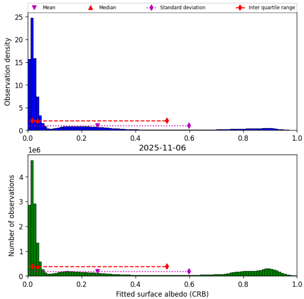
Figure 46: Histogram of “Fitted surface albedo (CRB)” for 2025-11-05 to 2025-11-07
