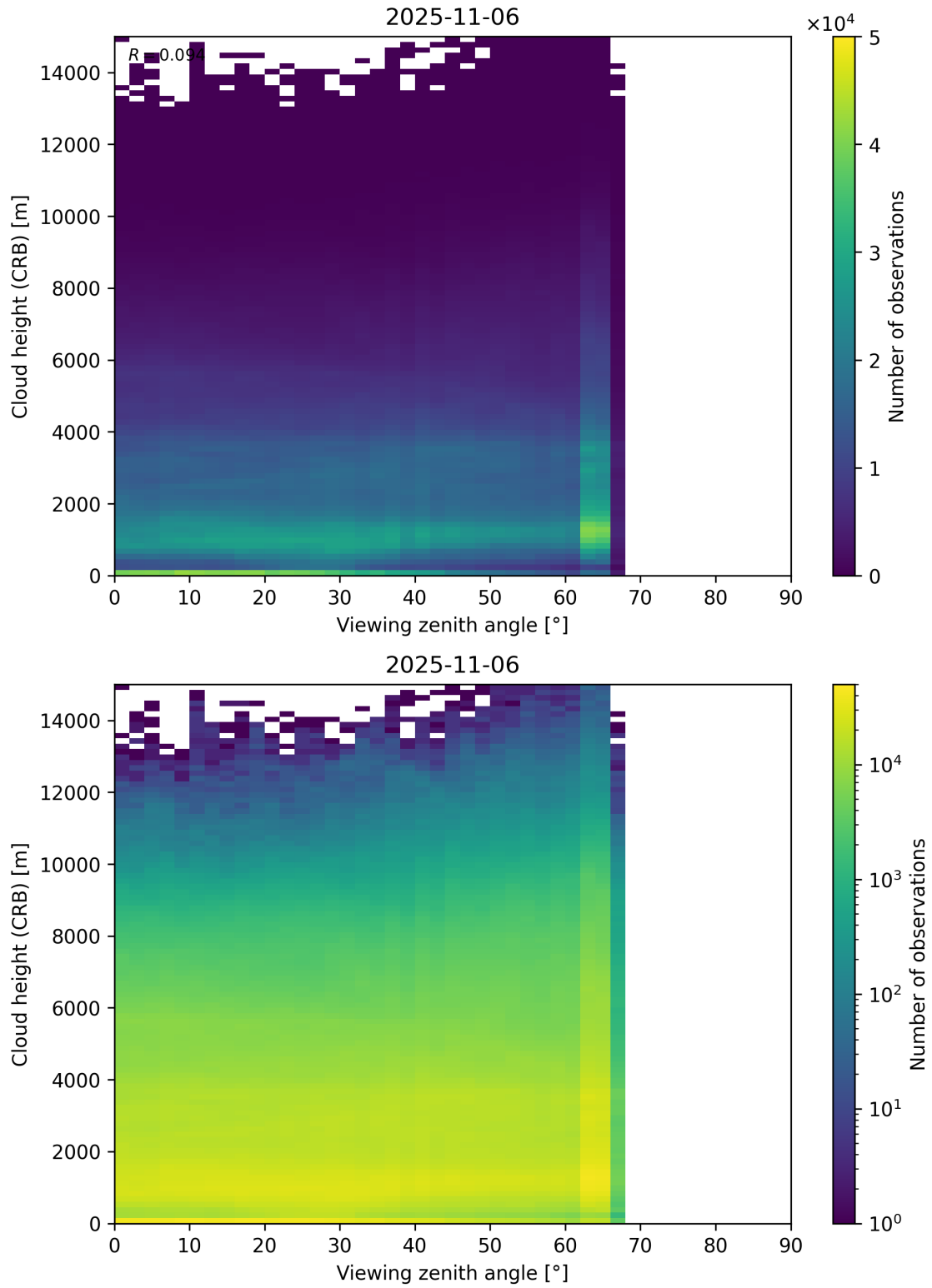
Figure 110: Scatter density plot of “Viewing zenith angle” against “Cloud height (CRB)” for 2025-11-05 to 2025-11-07.
