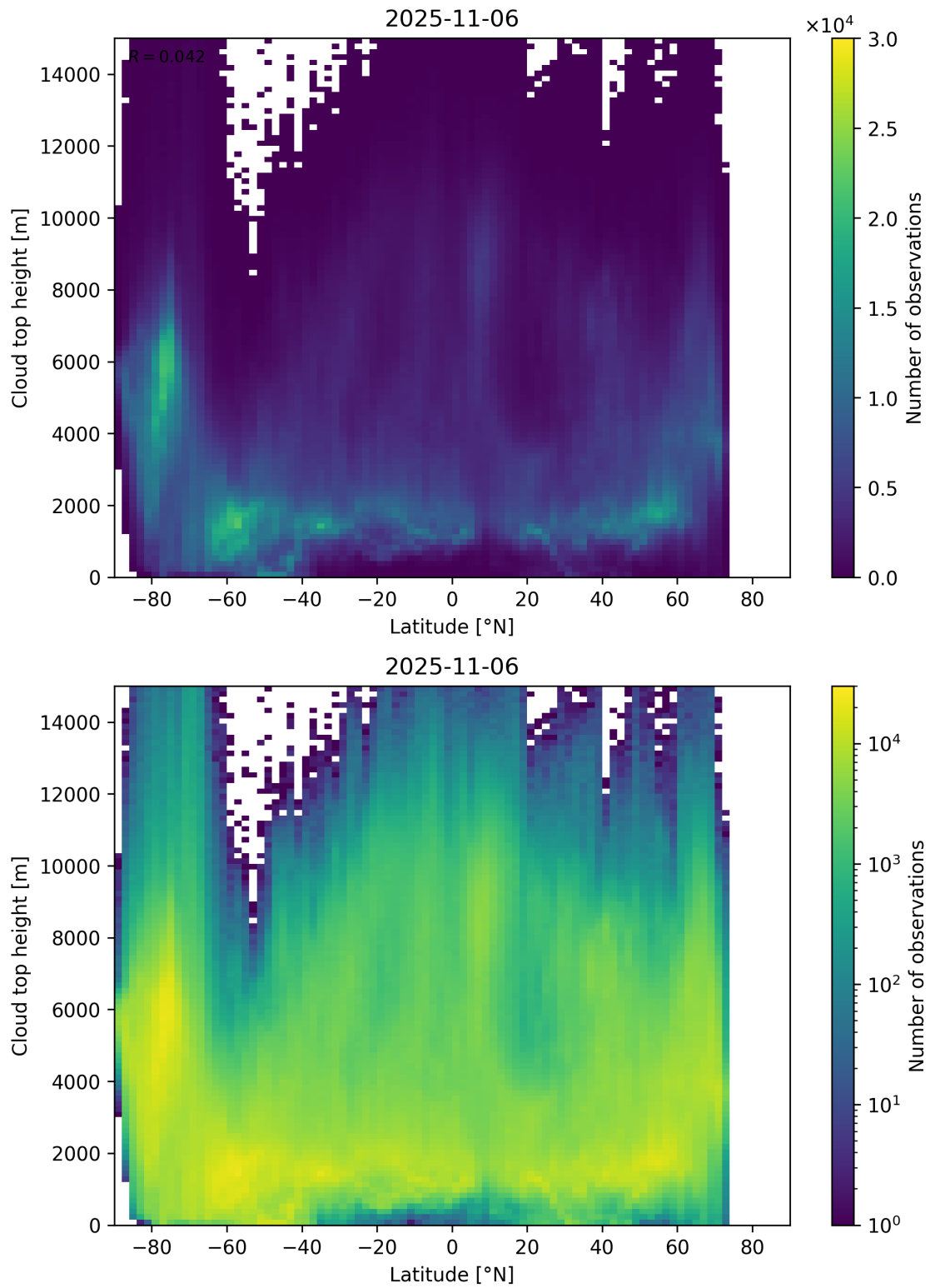
Figure 97: Scatter density plot of “Latitude” against “Cloud top height” for 2025-11-05 to 2025-11-07.
