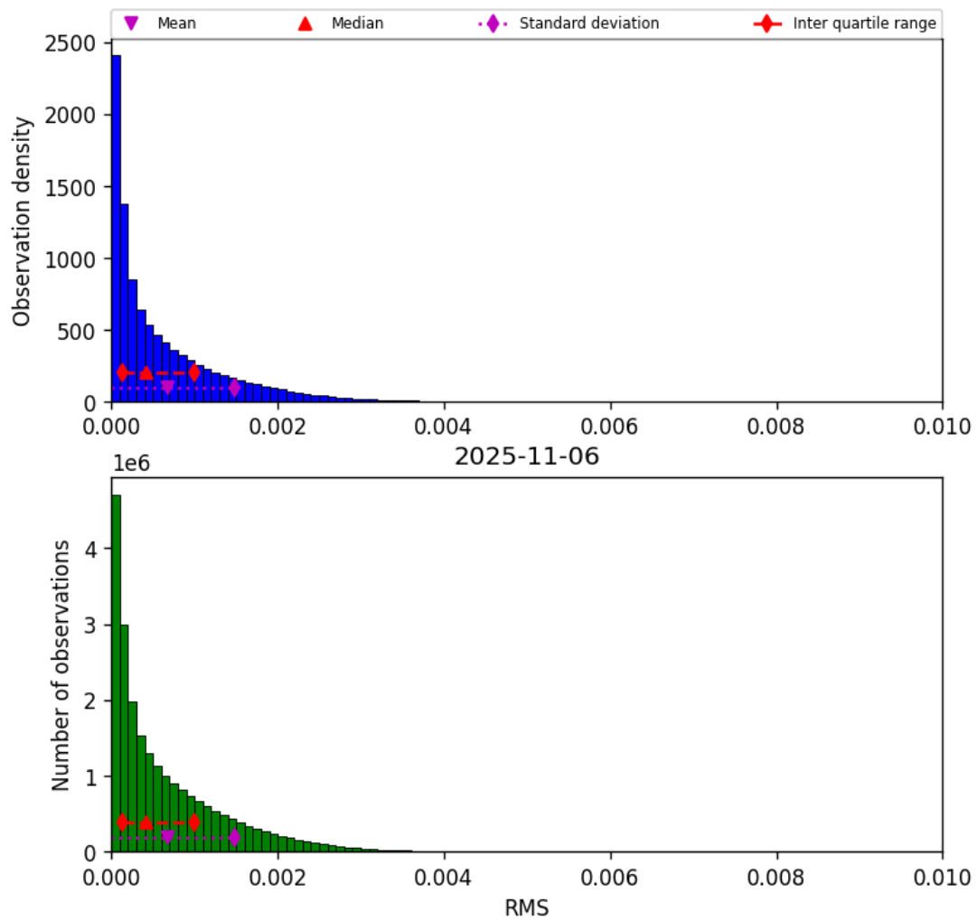
Figure 47: Histogram of “RMS” for 2025-11-05 to 2025-11-07
