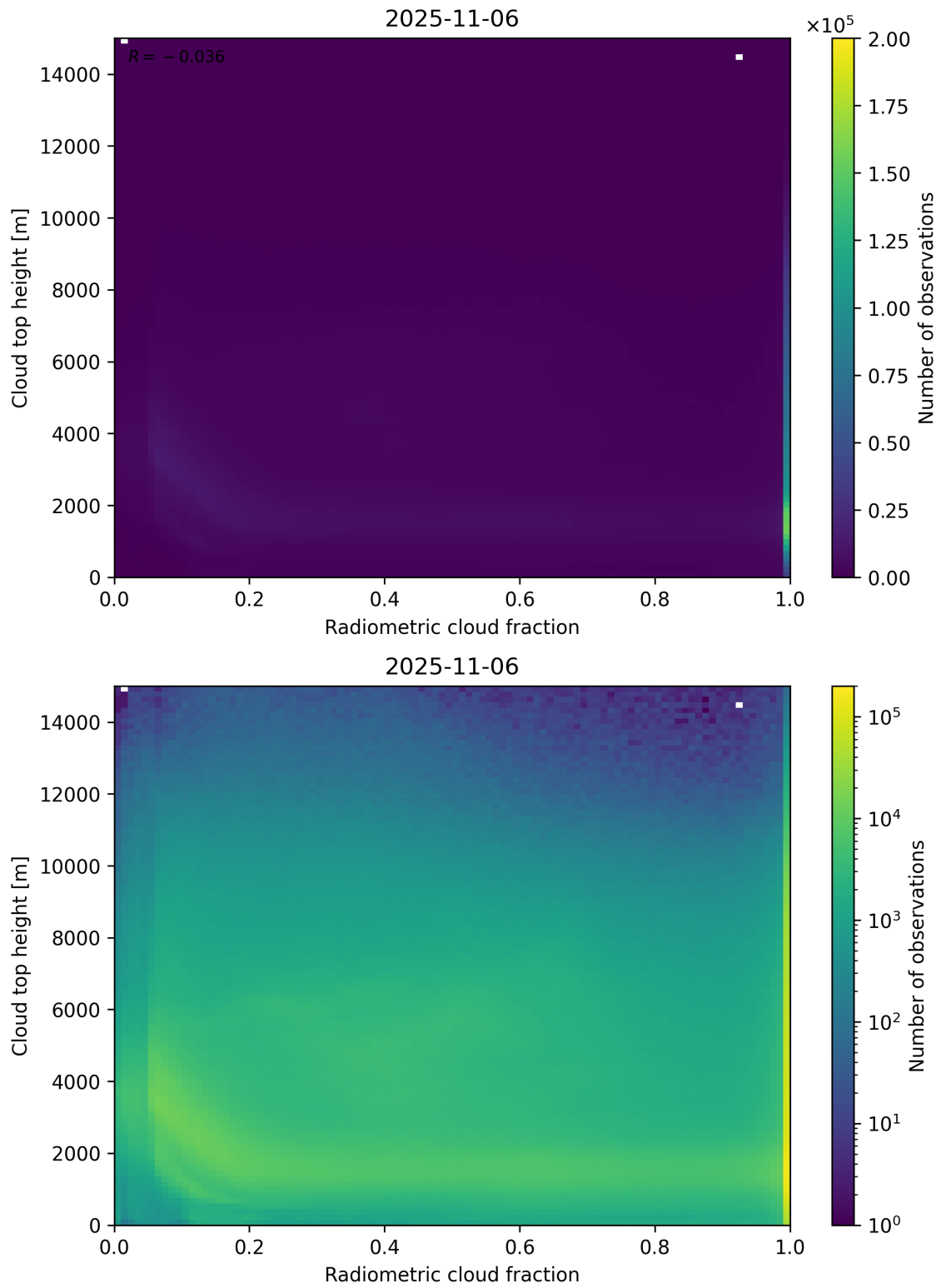
Figure 76: Scatter density plot of “Radiometric cloud fraction” against “Cloud top height” for 2025-11-05 to 2025-11-07.
