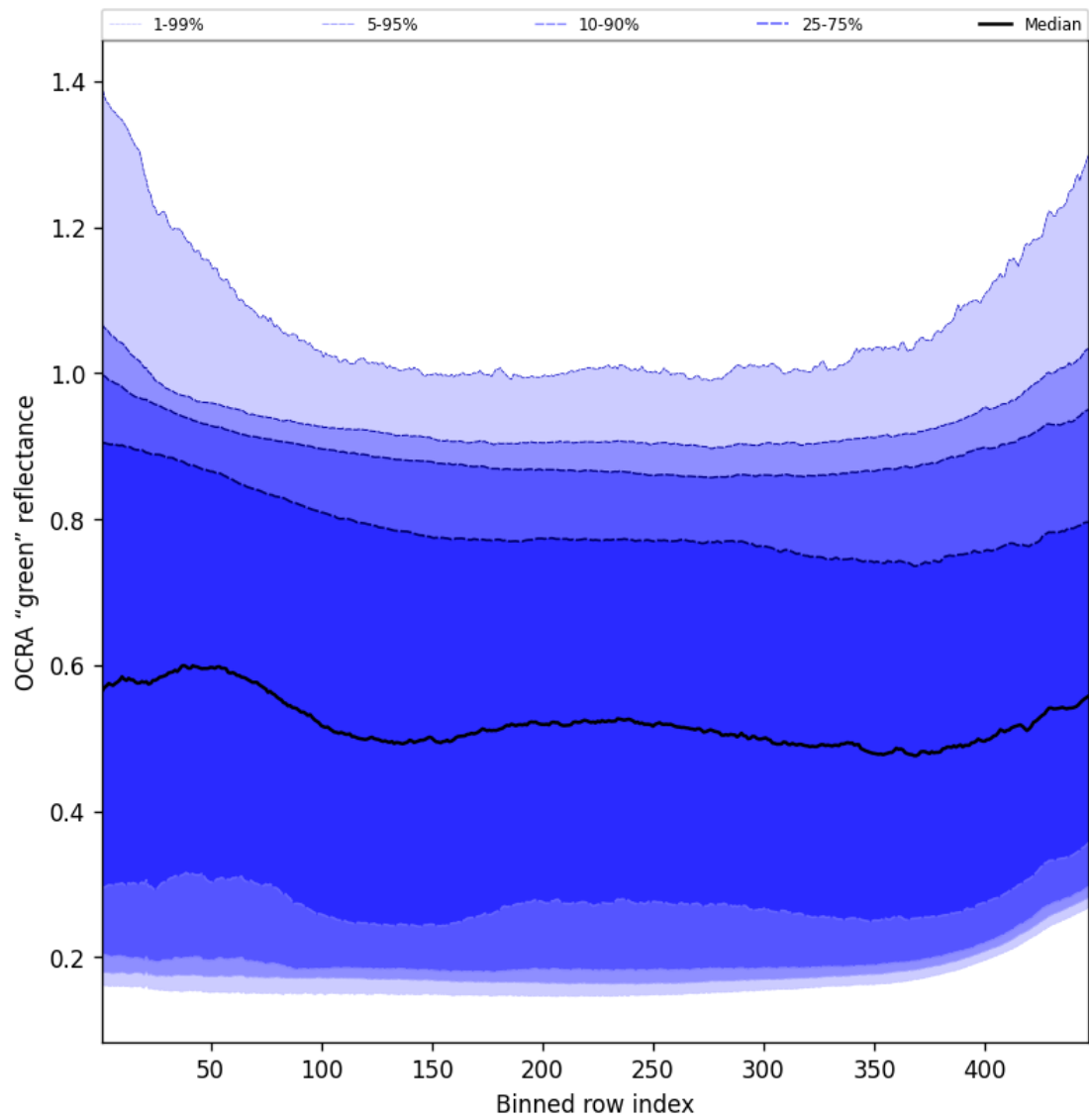
Figure 68: Along track statistics of “OCRA “green” reflectance” for 2025-11-05 to 2025-11-07
