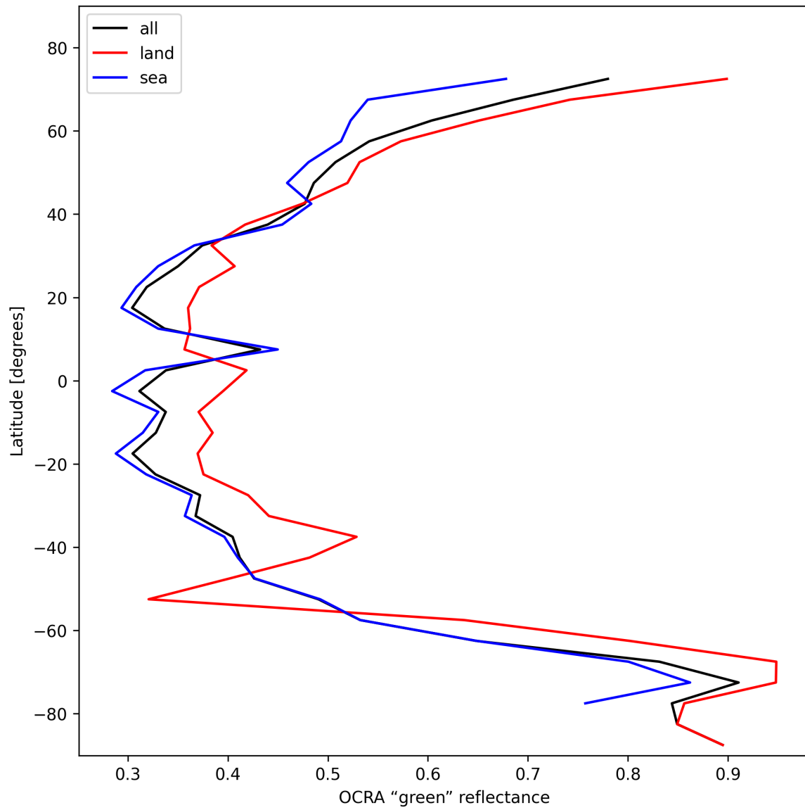
Figure 36: Zonal average of “OCRA “green” reflectance” for 2025-11-05 to 2025-11-07.
