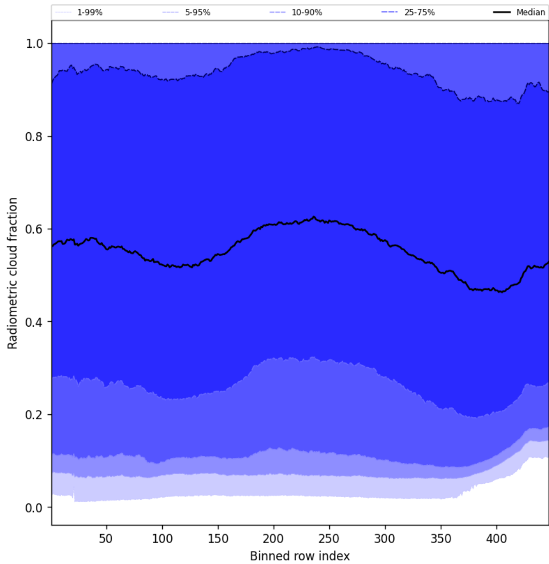
Figure 55: Along track statistics of “Radiometric cloud fraction” for 2025-11-05 to 2025-11-07
