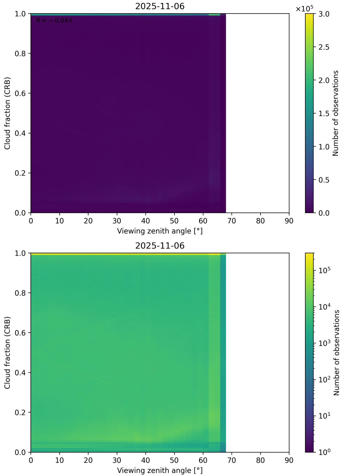
Figure 109: Scatter density plot of “Viewing zenith angle” against “Cloud fraction (CRB)” for 2025-11-05 to 2025-11-07.
