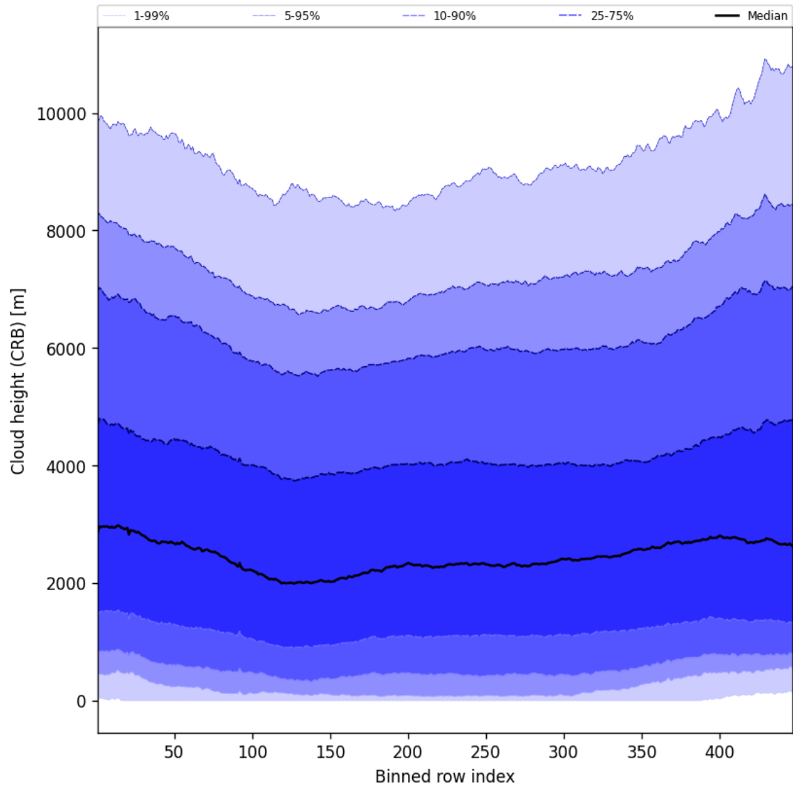
Figure 59: Along track statistics of “Cloud height (CRB)” for 2025-11-05 to 2025-11-07
