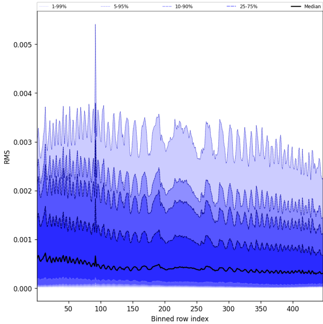
Figure 63: Along track statistics of “RMS” for 2025-11-05 to 2025-11-07
