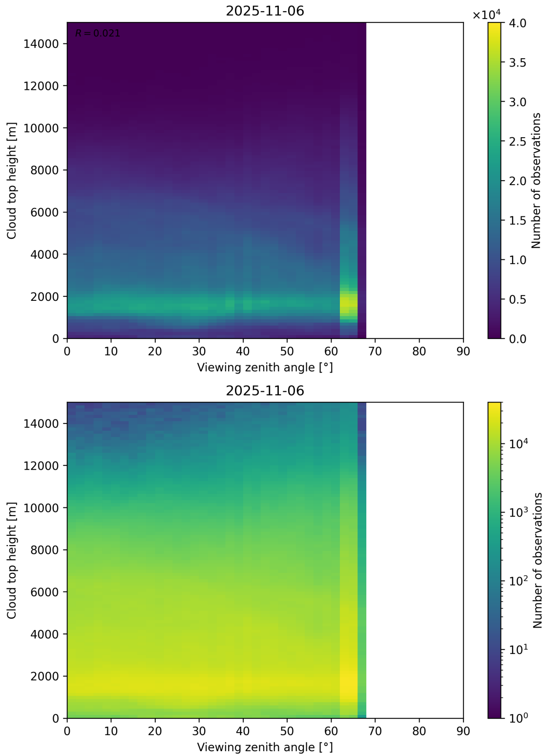
Figure 112: Scatter density plot of “Viewing zenith angle” against “Cloud top height” for 2025-11-05 to 2025-11-07.
