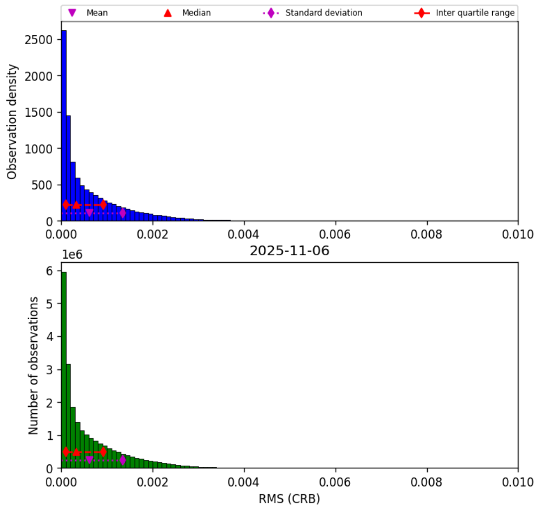
Figure 48: Histogram of “RMS (CRB)” for 2025-11-05 to 2025-11-07
