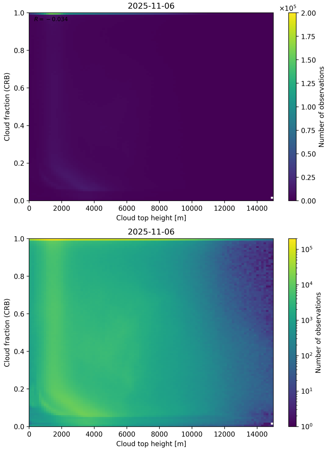
Figure 88: Scatter density plot of “Cloud top height” against “Cloud fraction (CRB)” for 2025-11-05 to 2025-11-07.
