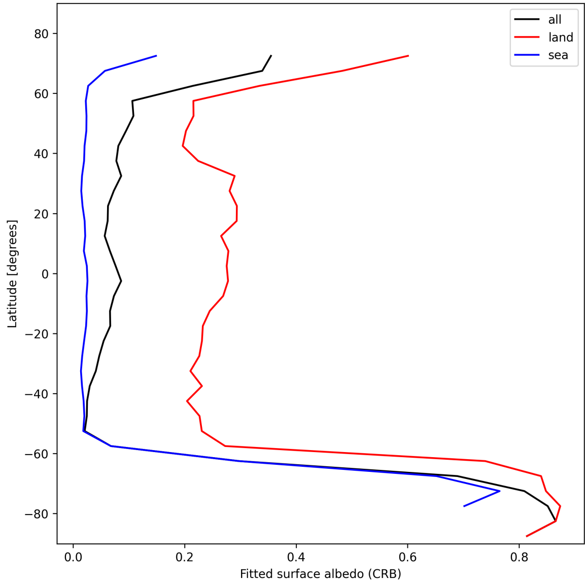
Figure 30: Zonal average of “Fitted surface albedo (CRB)” for 2025-11-05 to 2025-11-07.
