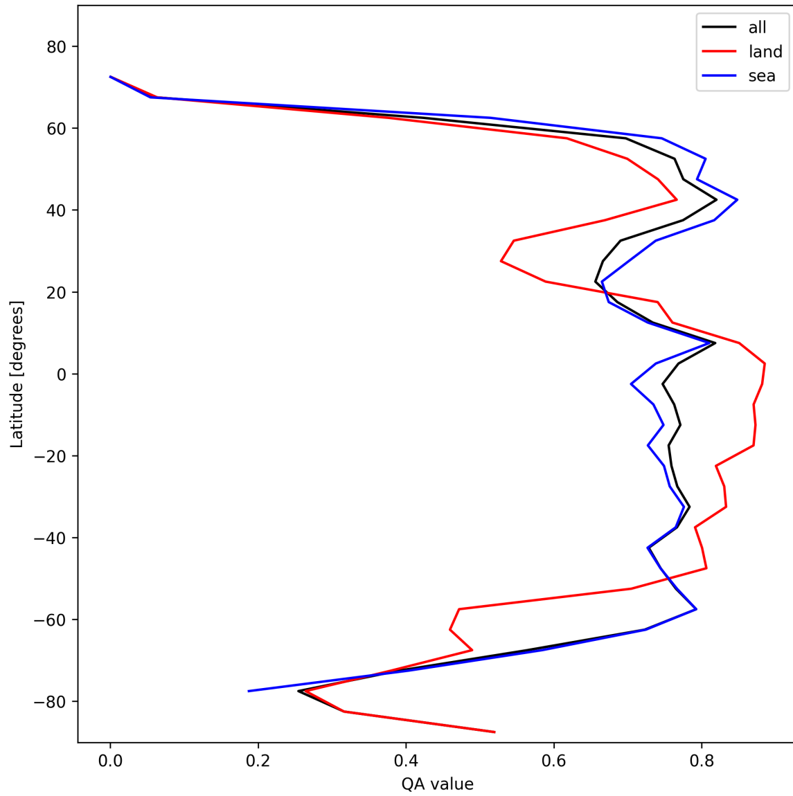
Figure 22: Zonal average of “QA value” for 2025-11-05 to 2025-11-07.
