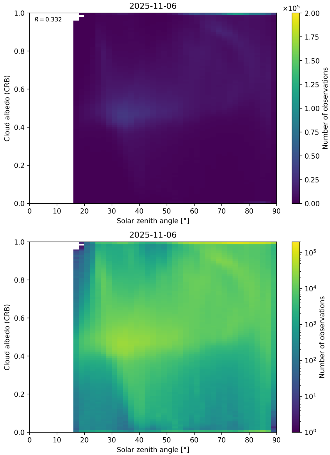
Figure 98: Scatter density plot of “Solar zenith angle” against “Cloud albedo (CRB)” for 2025-11-05 to 2025-11-07.
