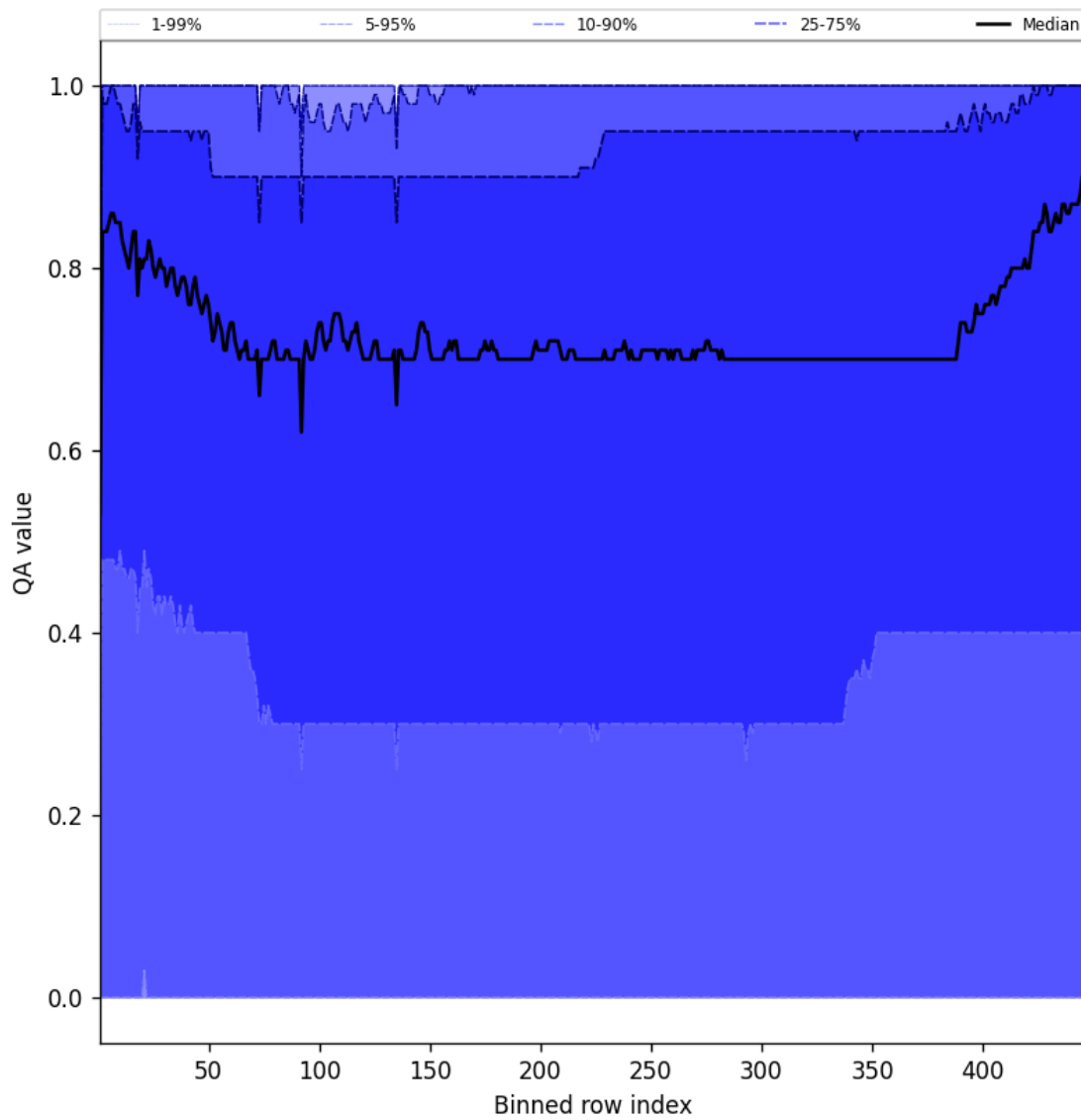
Figure 54: Along track statistics of “QA value” for 2025-11-05 to 2025-11-07
