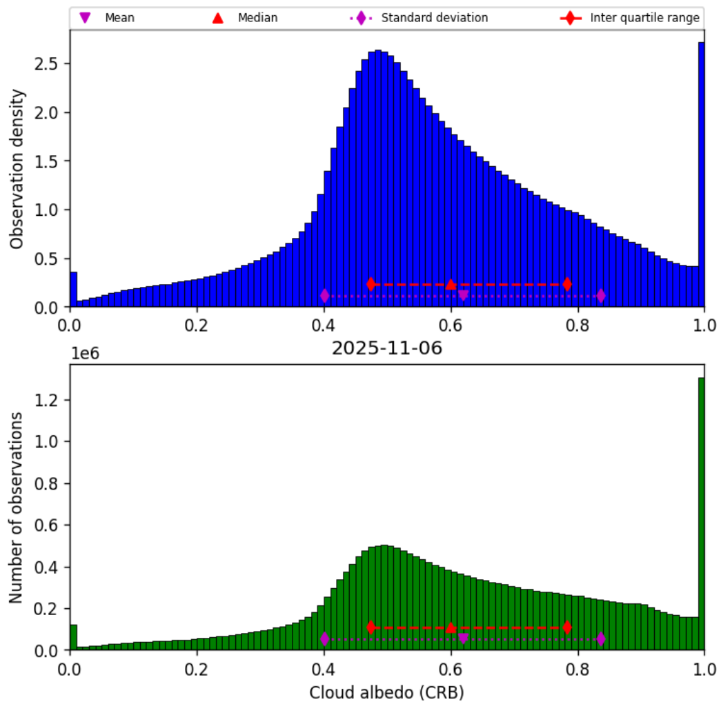
Figure 44: Histogram of “Cloud albedo (CRB)” for 2025-11-05 to 2025-11-07
