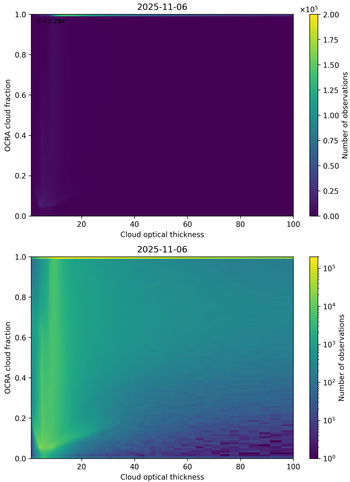
Figure 83: Scatter density plot of “Cloud optical thickness” against “OCRA cloud fraction” for 2025-11-05 to 2025-11-07.
