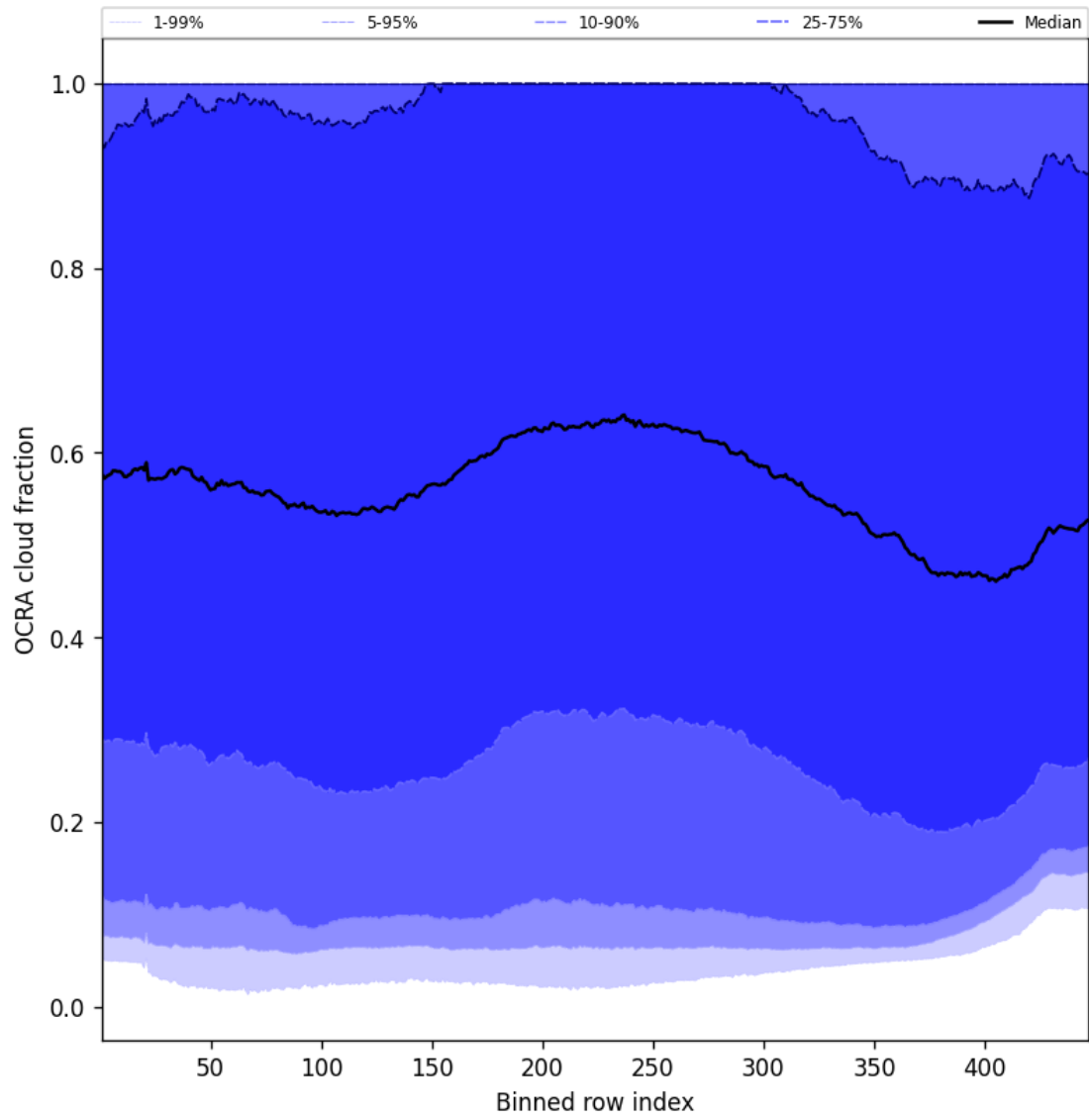
Figure 66: Along track statistics of “OCRA cloud fraction” for 2025-11-05 to 2025-11-07
