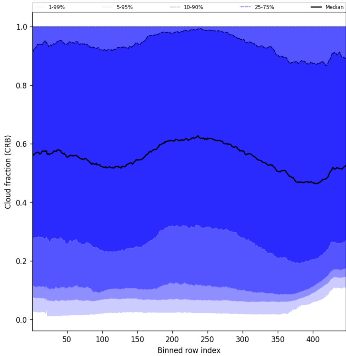
Figure 58: Along track statistics of “Cloud fraction (CRB)” for 2025-11-05 to 2025-11-07
