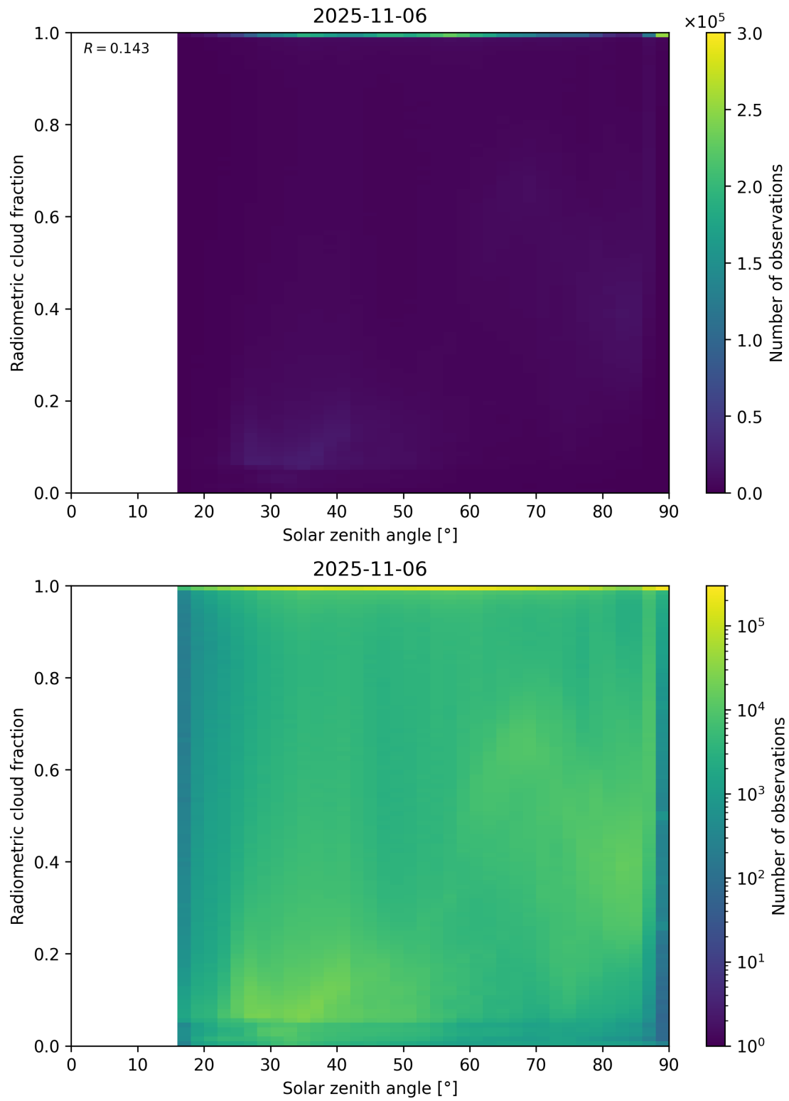
Figure 99: Scatter density plot of “Solar zenith angle” against “Radiometric cloud fraction” for 2025-11-05 to 2025-11-07.
