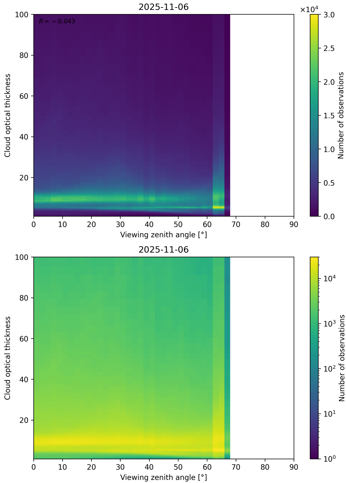
Figure 111: Scatter density plot of “Viewing zenith angle” against “Cloud optical thickness” for 2025-11-05 to 2025-11-07.
