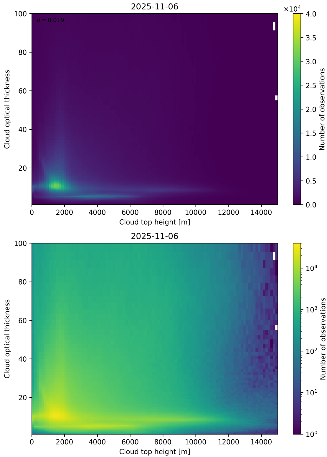
Figure 90: Scatter density plot of “Cloud top height” against “Cloud optical thickness” for 2025-11-05 to 2025-11-07.
