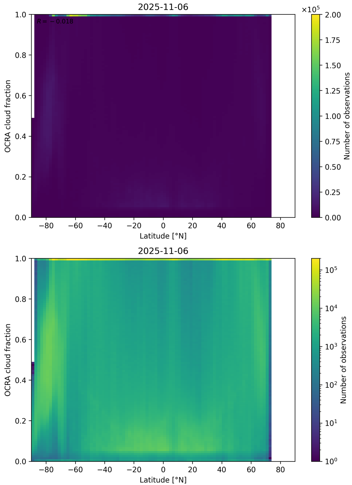
Figure 93: Scatter density plot of “Latitude” against “OCRA cloud fraction” for 2025-11-05 to 2025-11-07.
