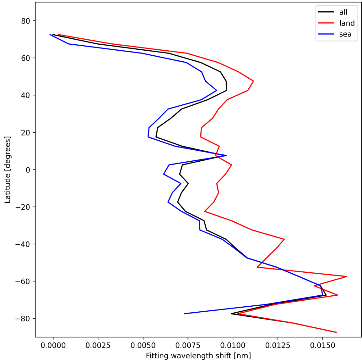
Figure 33: Zonal average of “Fitting wavelength shift” for 2025-11-05 to 2025-11-07.
