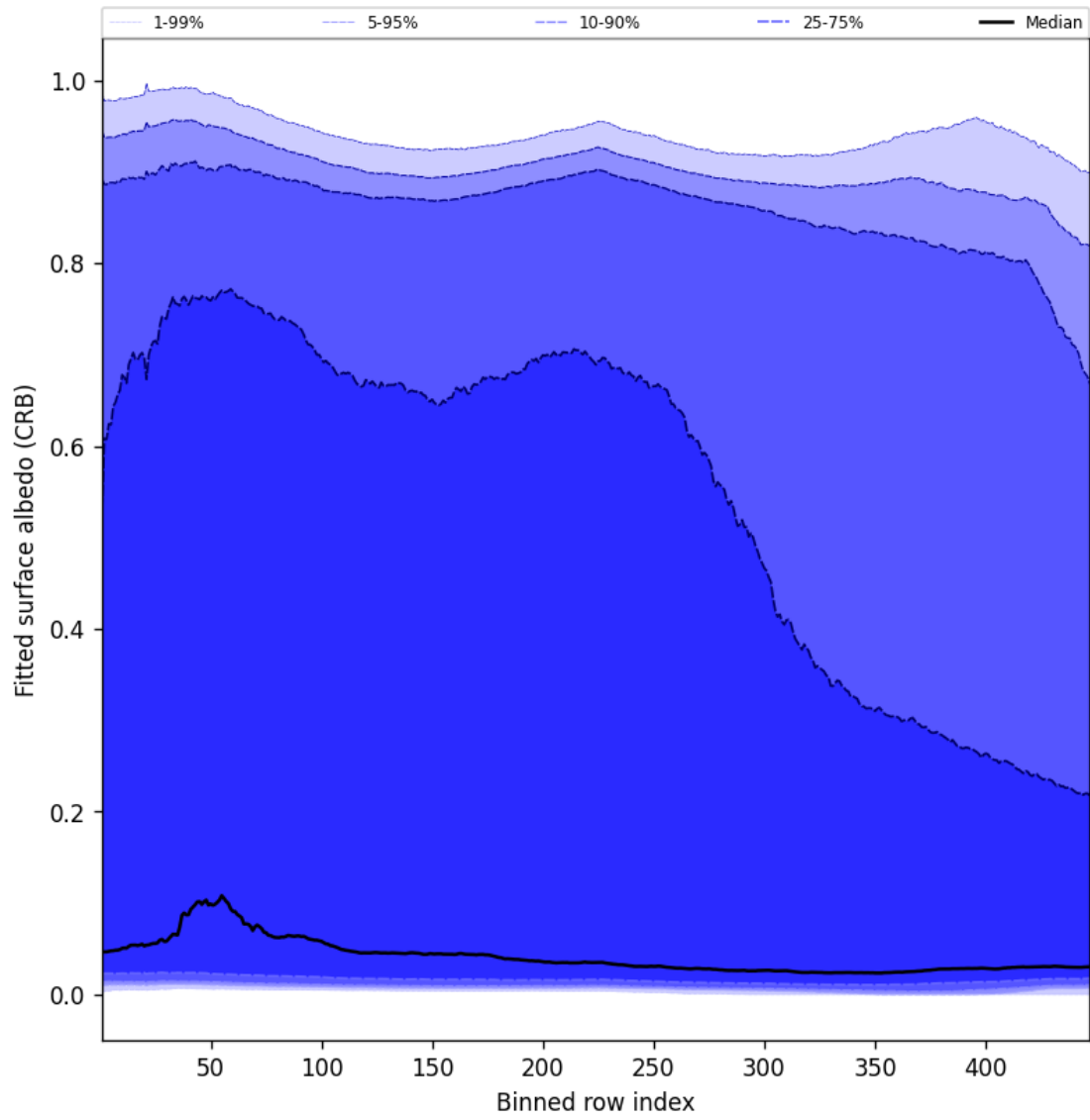
Figure 62: Along track statistics of “Fitted surface albedo (CRB)” for 2025-11-05 to 2025-11-07
