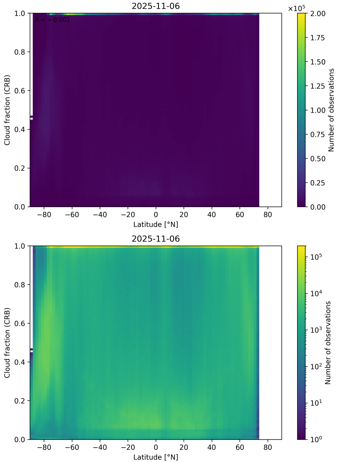
Figure 94: Scatter density plot of “Latitude” against “Cloud fraction (CRB)” for 2025-11-05 to 2025-11-07.
