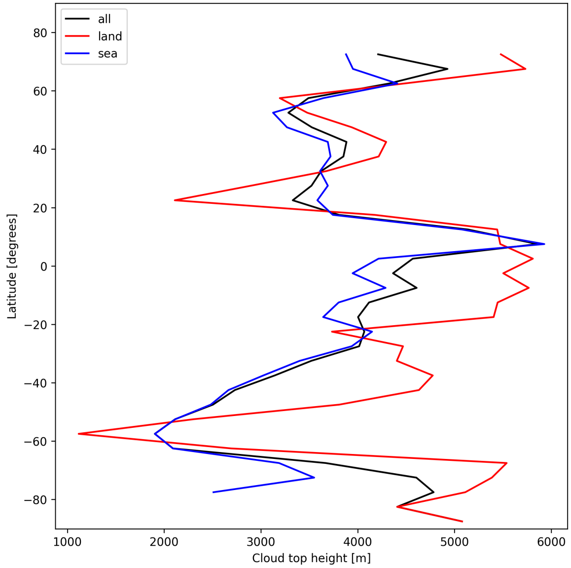
Figure 24: Zonal average of “Cloud top height” for 2025-11-05 to 2025-11-07.
