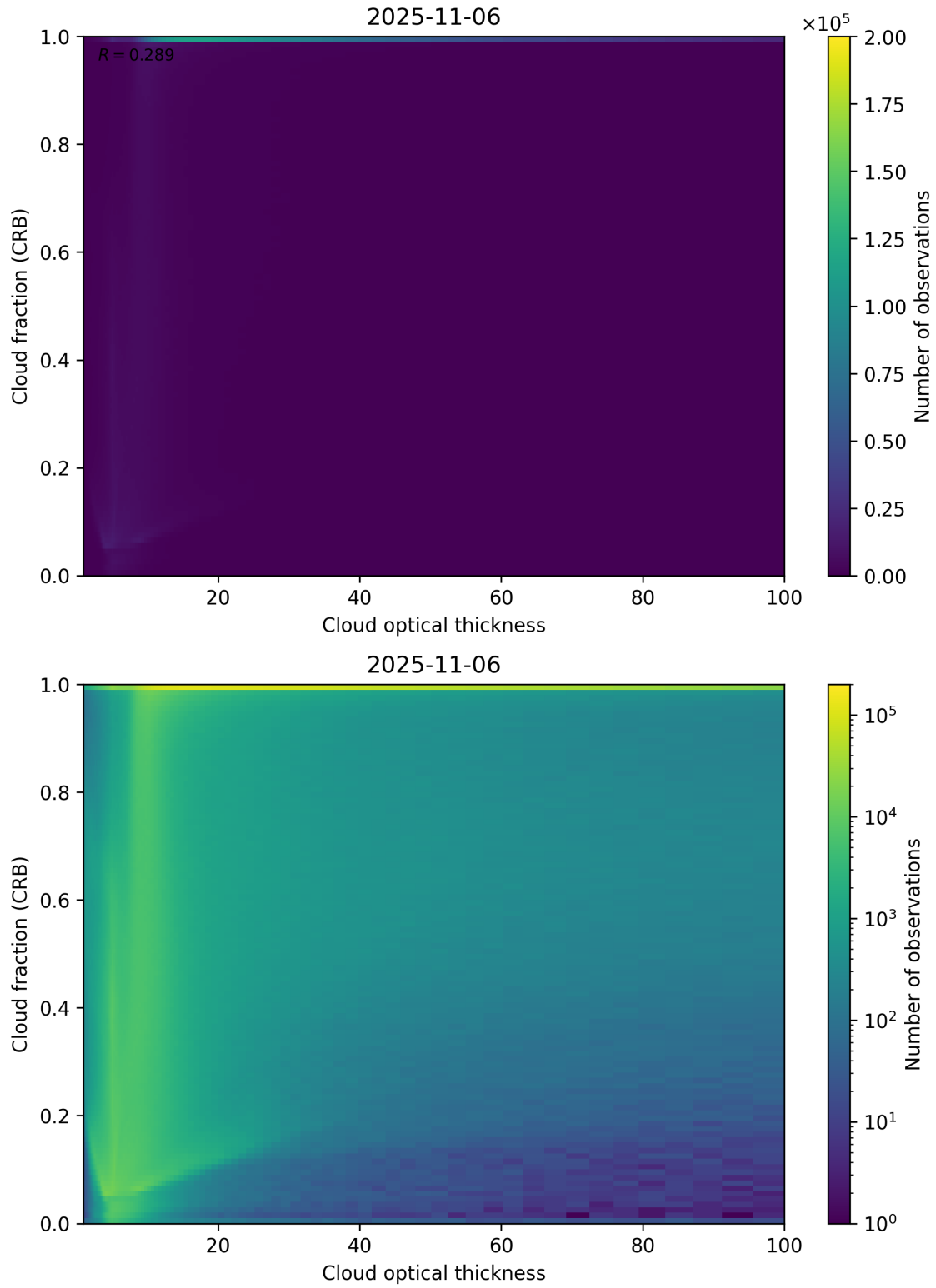
Figure 84: Scatter density plot of “Cloud optical thickness” against “Cloud fraction (CRB)” for 2025-11-05 to 2025-11-07.
