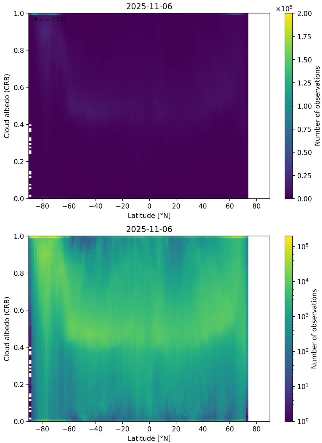
Figure 91: Scatter density plot of “Latitude” against “Cloud albedo (CRB)” for 2025-11-05 to 2025-11-07.
