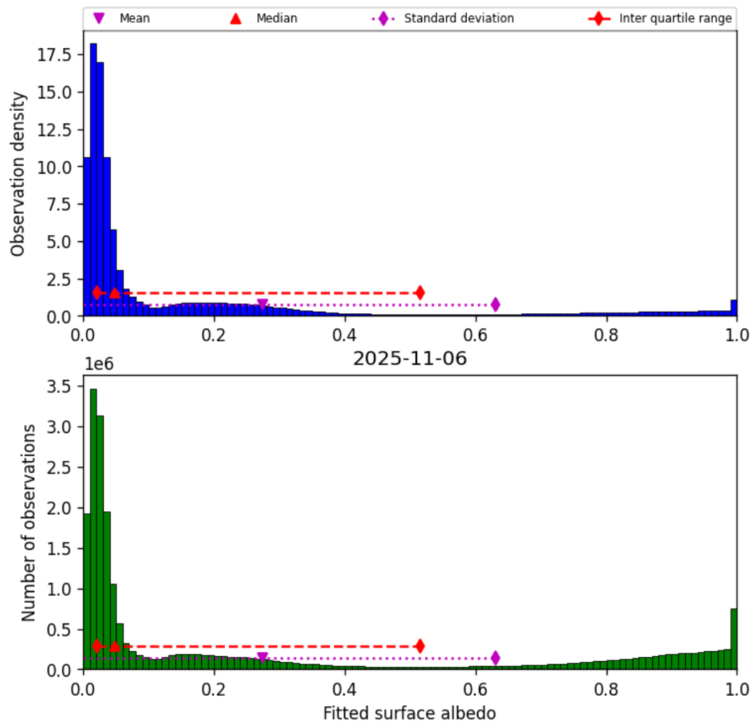
Figure 45: Histogram of “Fitted surface albedo” for 2025-11-05 to 2025-11-07
