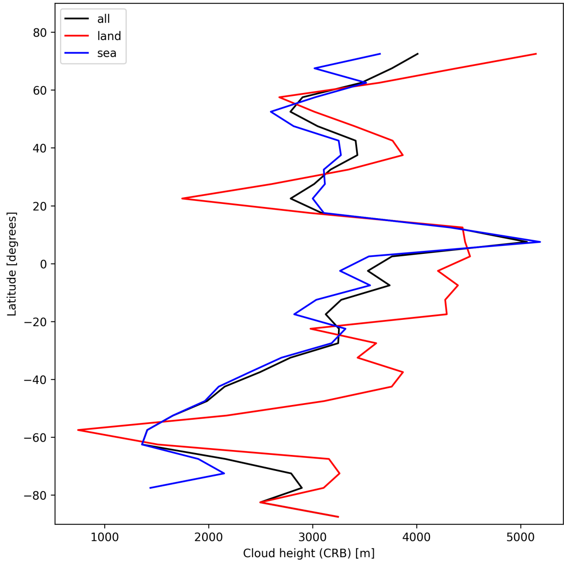
Figure 27: Zonal average of “Cloud height (CRB)” for 2025-11-05 to 2025-11-07.
