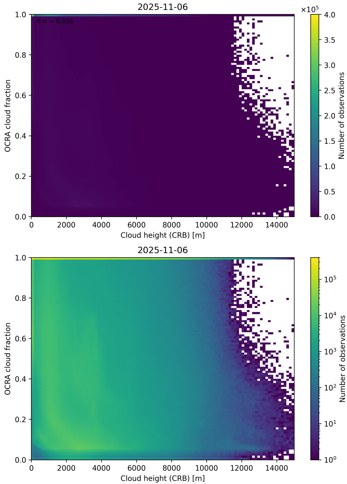
Figure 81: Scatter density plot of “Cloud height (CRB)” against “OCRA cloud fraction” for 2025-11-05 to 2025-11-07.
