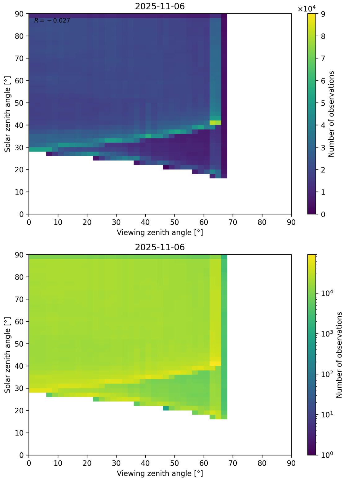
Figure 114: Scatter density plot of “Viewing zenith angle” against “Solar zenith angle” for 2025-11-05 to 2025-11-07.
