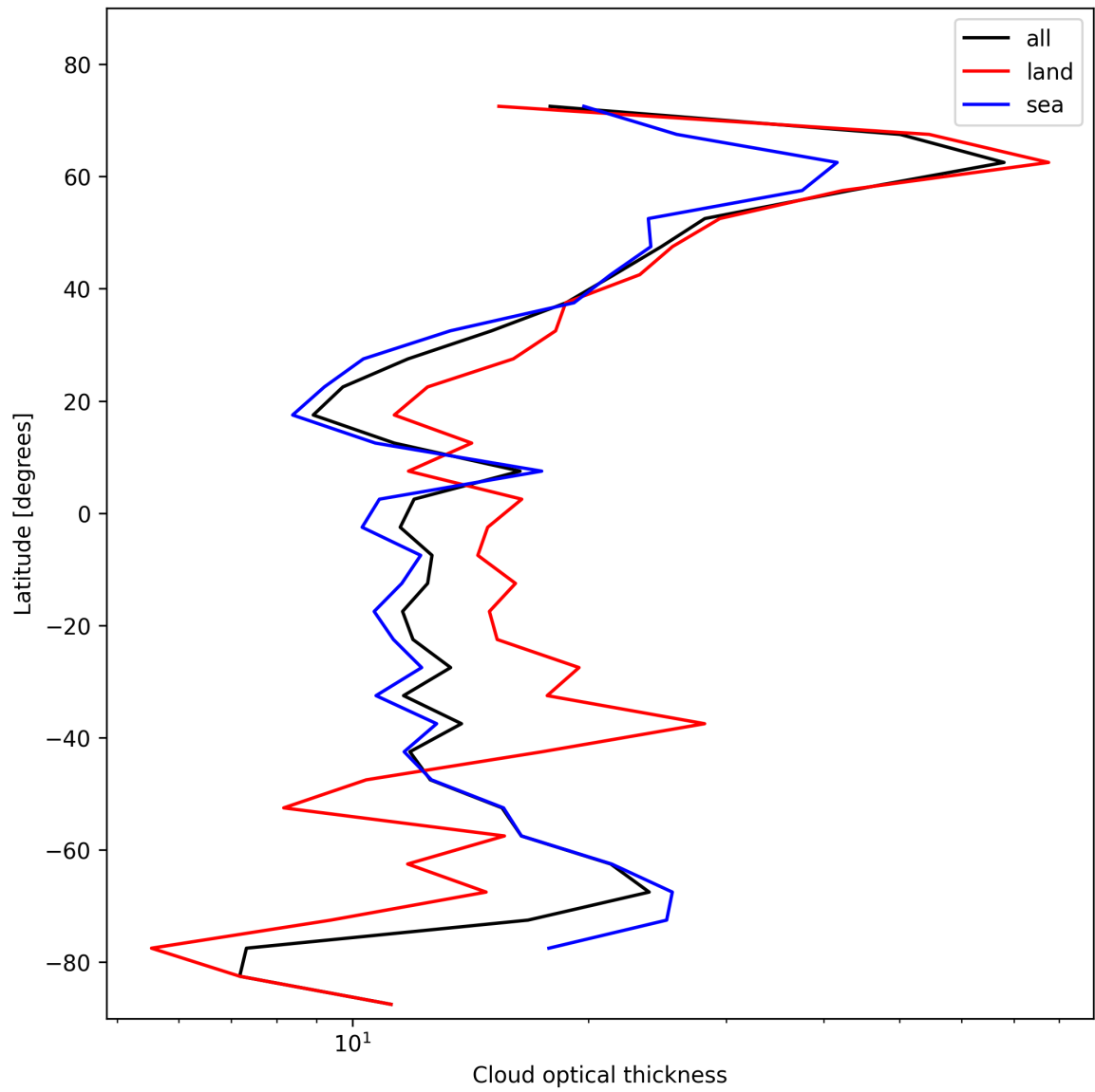
Figure 25: Zonal average of “Cloud optical thickness” for 2025-11-05 to 2025-11-07.
