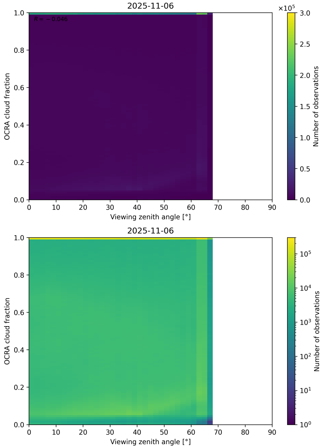
Figure 108: Scatter density plot of “Viewing zenith angle” against “OCRA cloud fraction” for 2025-11-05 to 2025-11-07.
