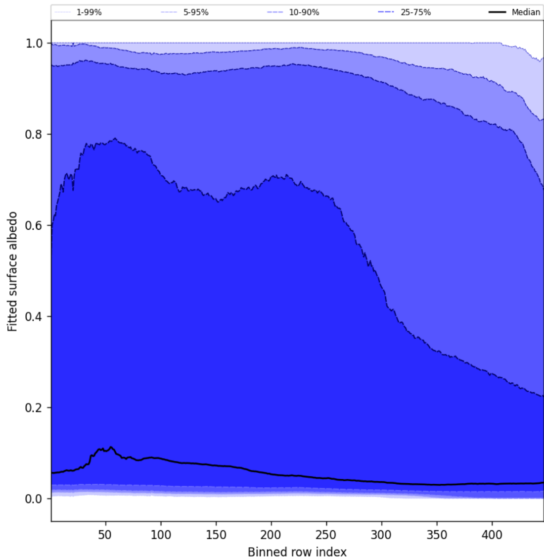
Figure 61: Along track statistics of “Fitted surface albedo” for 2025-11-05 to 2025-11-07
