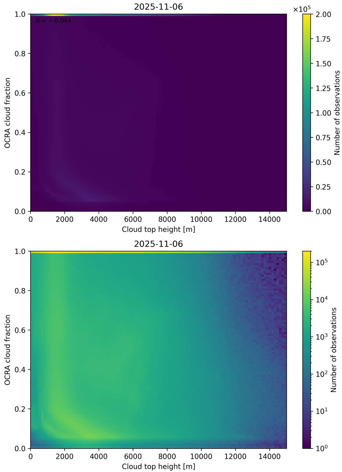
Figure 87: Scatter density plot of “Cloud top height” against “OCRA cloud fraction” for 2025-11-05 to 2025-11-07.
