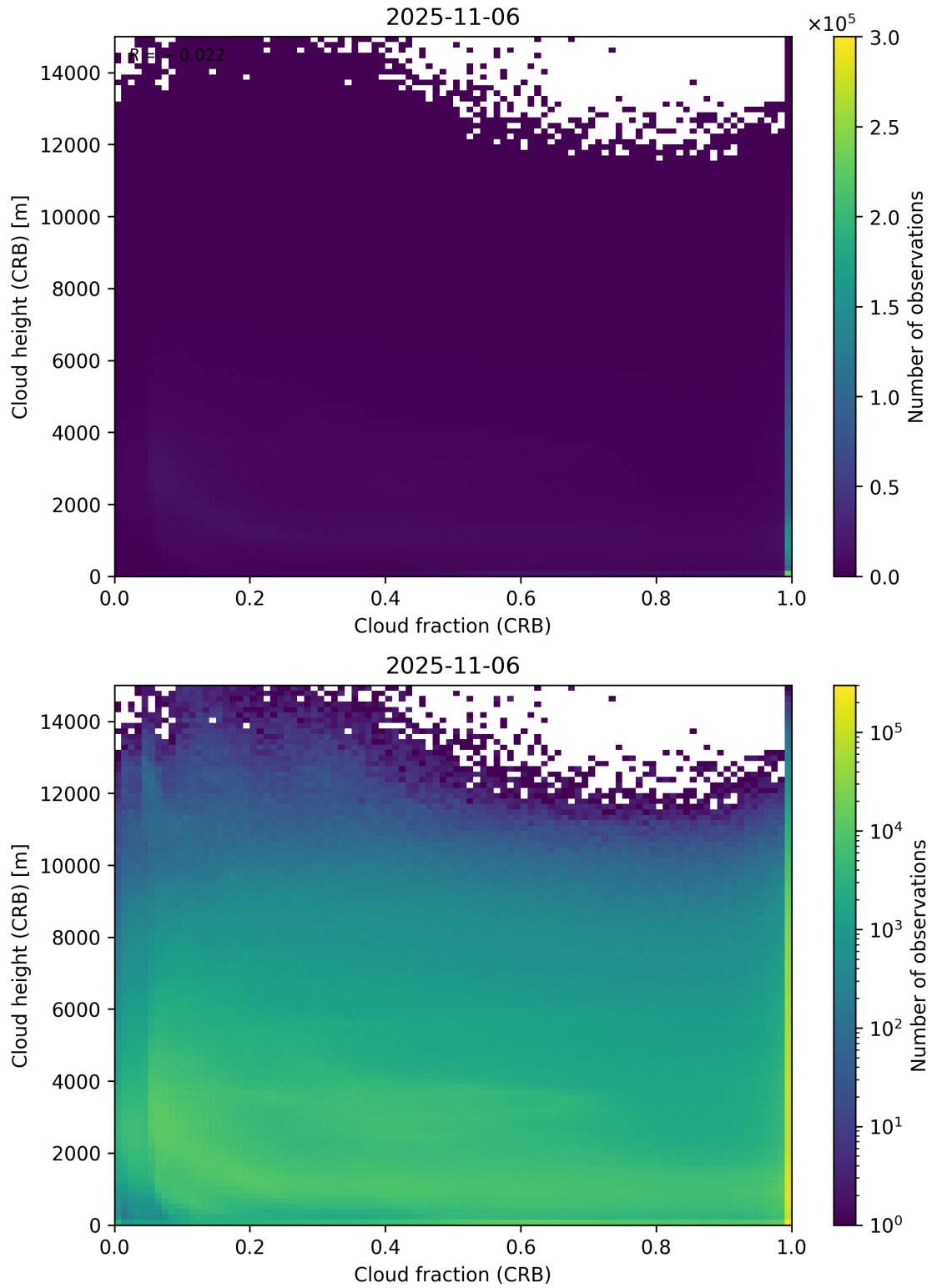
Figure 79: Scatter density plot of “Cloud fraction (CRB)” against “Cloud height (CRB)” for 2025-11-05 to 2025-11-07.
