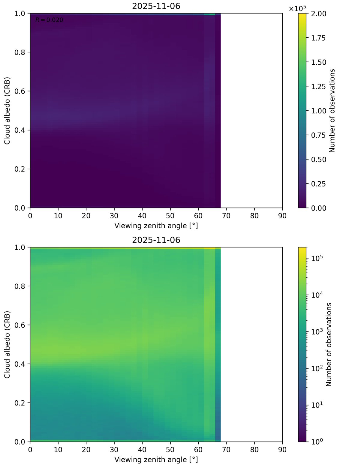
Figure 106: Scatter density plot of “Viewing zenith angle” against “Cloud albedo (CRB)” for 2025-11-05 to 2025-11-07.
