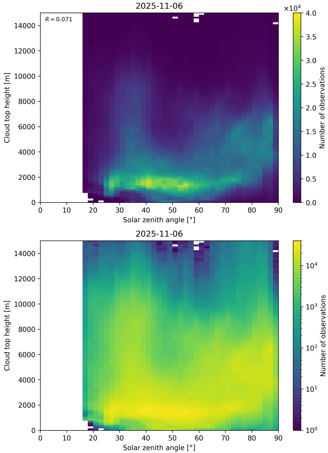
Figure 104: Scatter density plot of “Solar zenith angle” against “Cloud top height” for 2025-11-05 to 2025-11-07.
