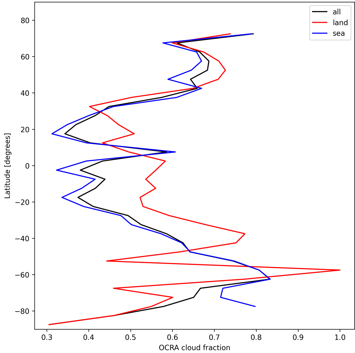
Figure 34: Zonal average of “OCRA cloud fraction” for 2025-11-05 to 2025-11-07.
