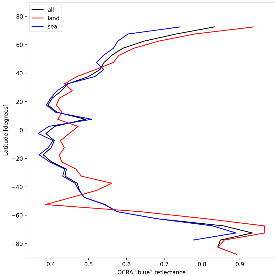
Figure 35: Zonal average of “OCRA “blue” reflectance” for 2025-11-05 to 2025-11-07.
