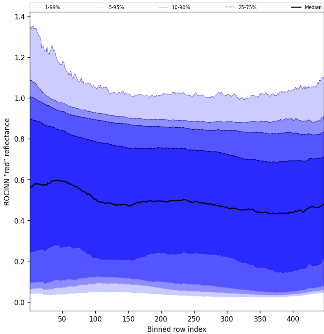
Figure 69: Along track statistics of “ROCINN “red” reflectance” for 2025-11-05 to 2025-11-07
