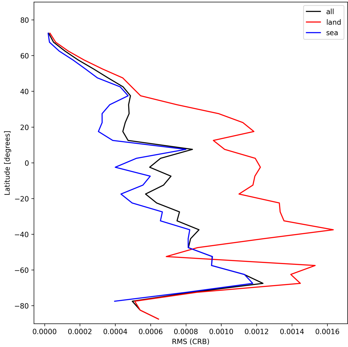
Figure 32: Zonal average of “RMS (CRB)” for 2025-11-05 to 2025-11-07.
