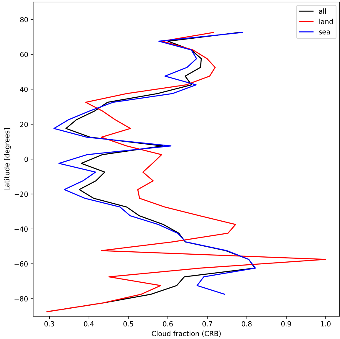
Figure 26: Zonal average of “Cloud fraction (CRB)” for 2025-11-05 to 2025-11-07.
