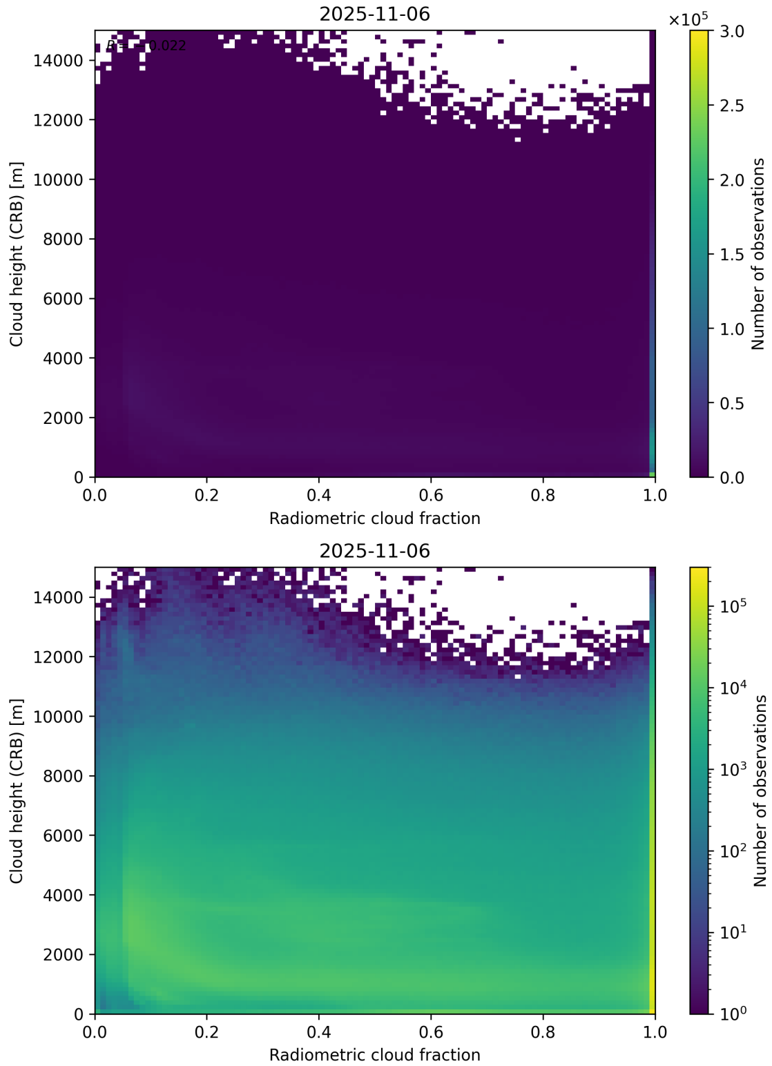
Figure 74: Scatter density plot of “Radiometric cloud fraction” against “Cloud height (CRB)” for 2025-11-05 to 2025-11-07.
