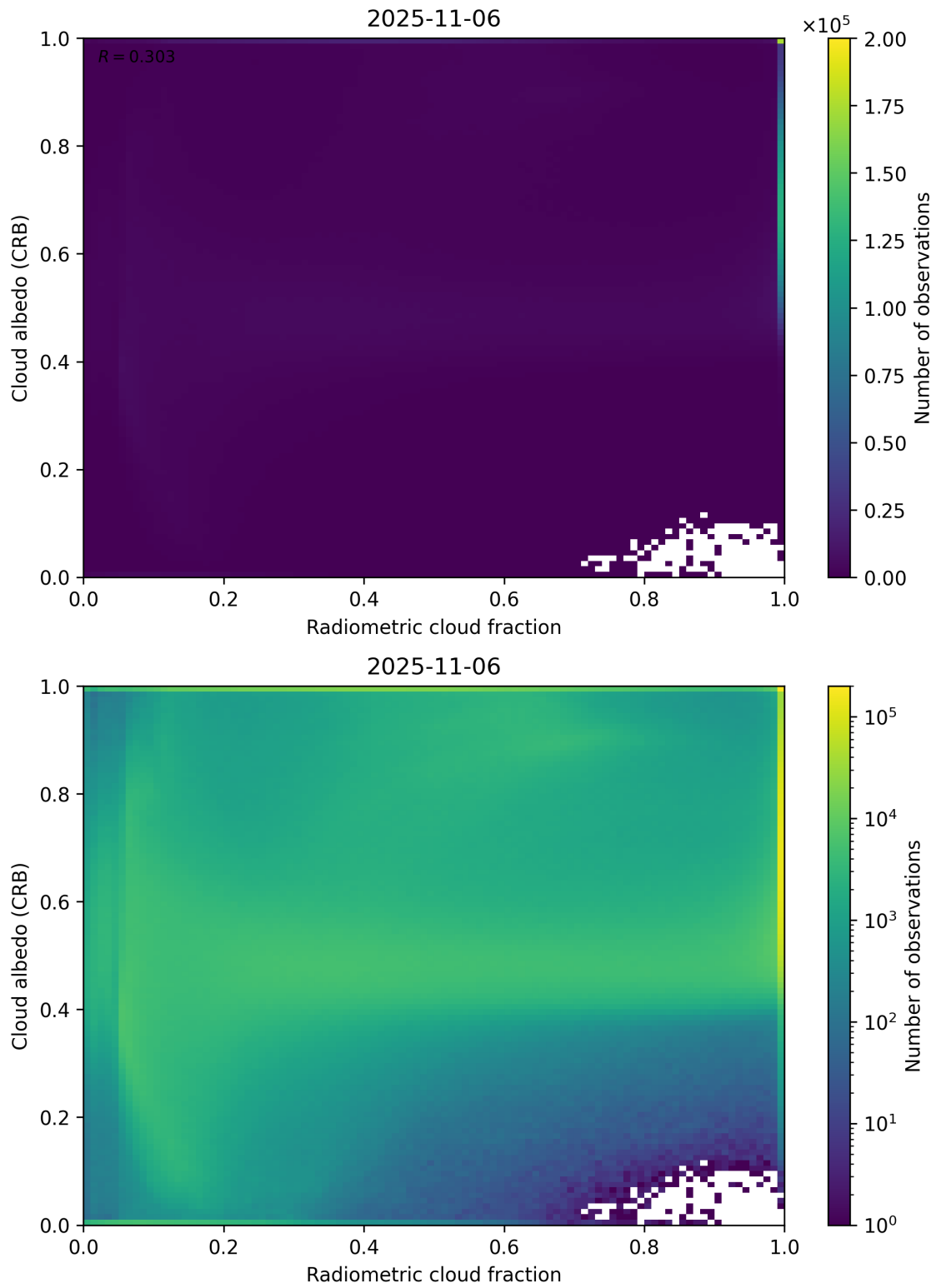
Figure 71: Scatter density plot of “Radiometric cloud fraction” against “Cloud albedo (CRB)” for 2025-11-05 to 2025-11-07.
