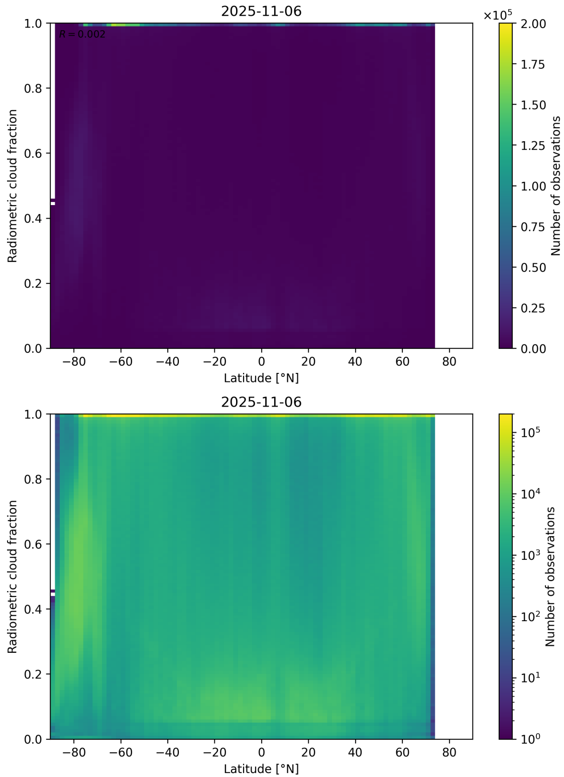
Figure 92: Scatter density plot of “Latitude” against “Radiometric cloud fraction” for 2025-11-05 to 2025-11-07.
