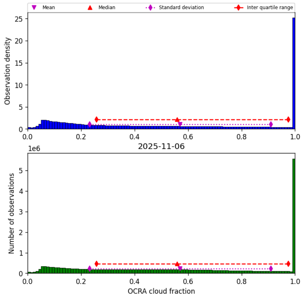
Figure 50: Histogram of “OCRA cloud fraction” for 2025-11-05 to 2025-11-07
