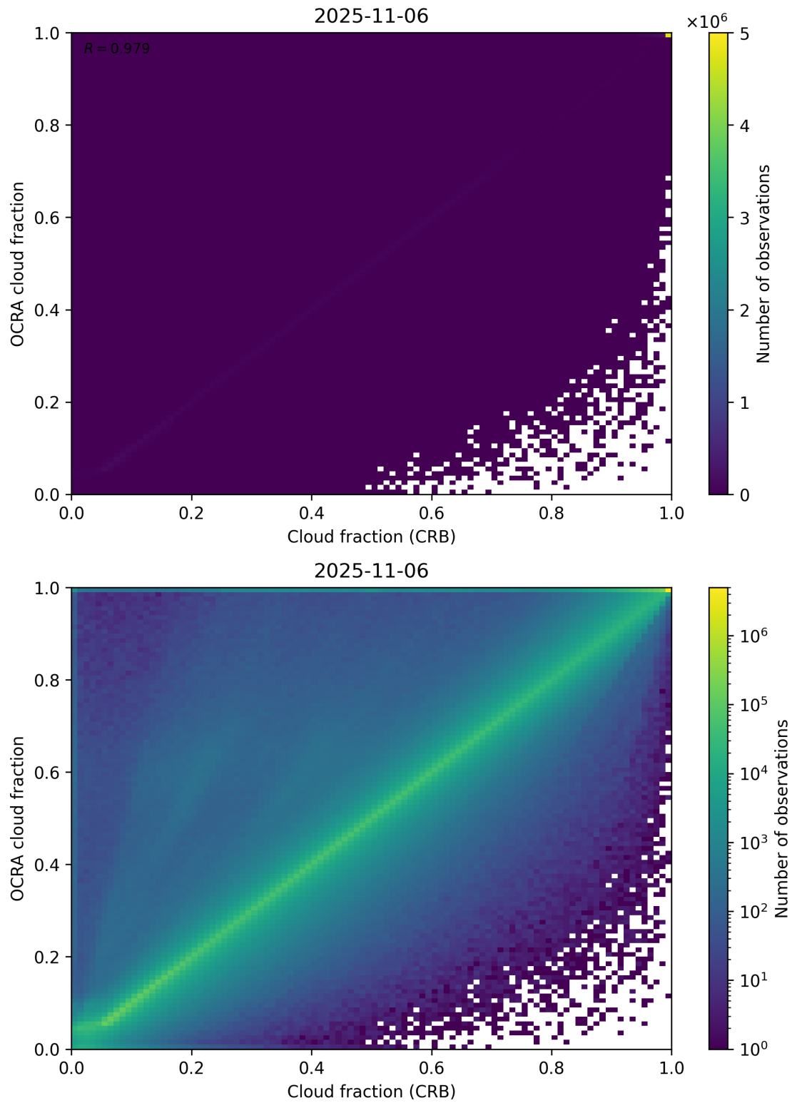
Figure 78: Scatter density plot of “Cloud fraction (CRB)” against “OCRA cloud fraction” for 2025-11-05 to 2025-11-07.
