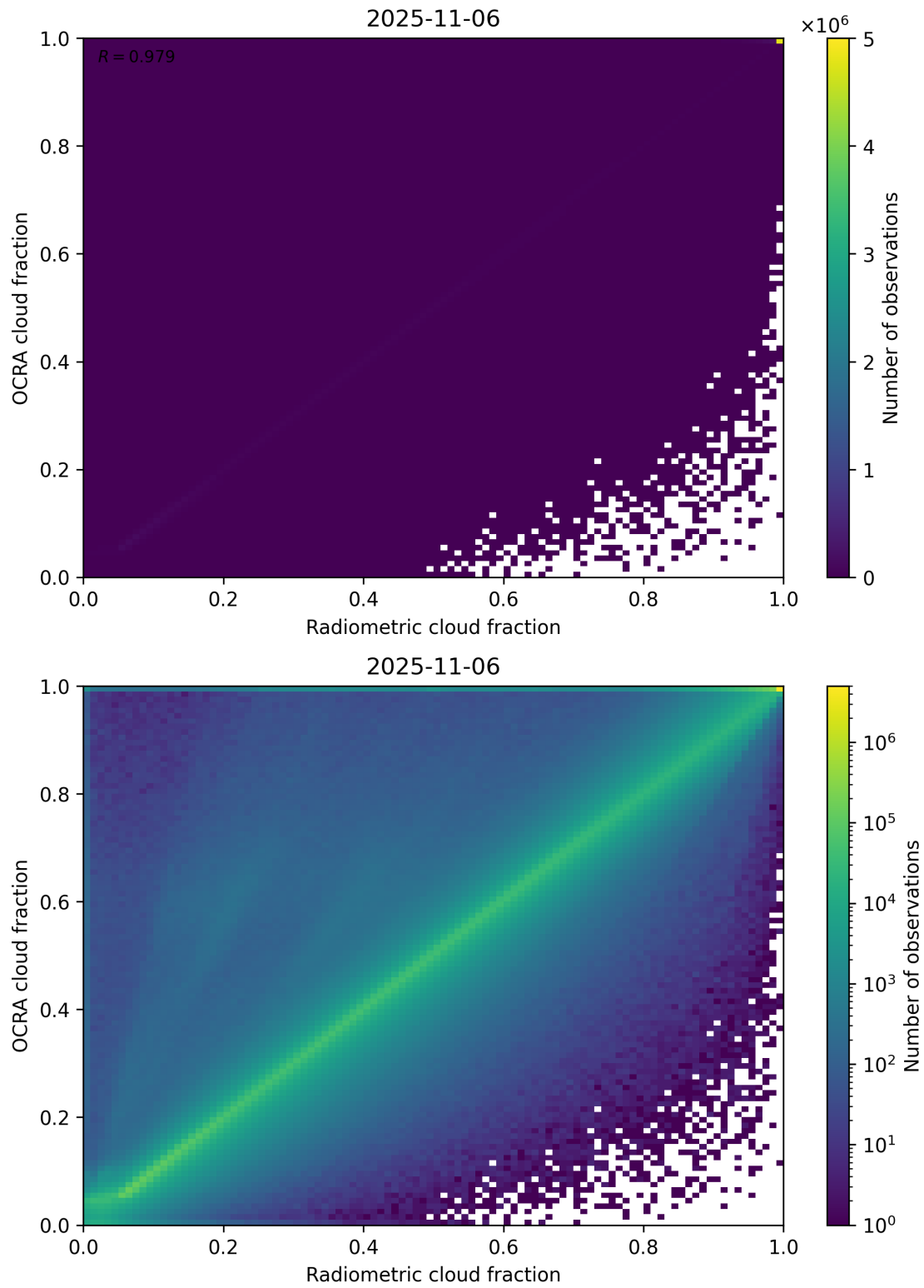
Figure 72: Scatter density plot of “Radiometric cloud fraction” against “OCRA cloud fraction” for 2025-11-05 to 2025-11-07.
