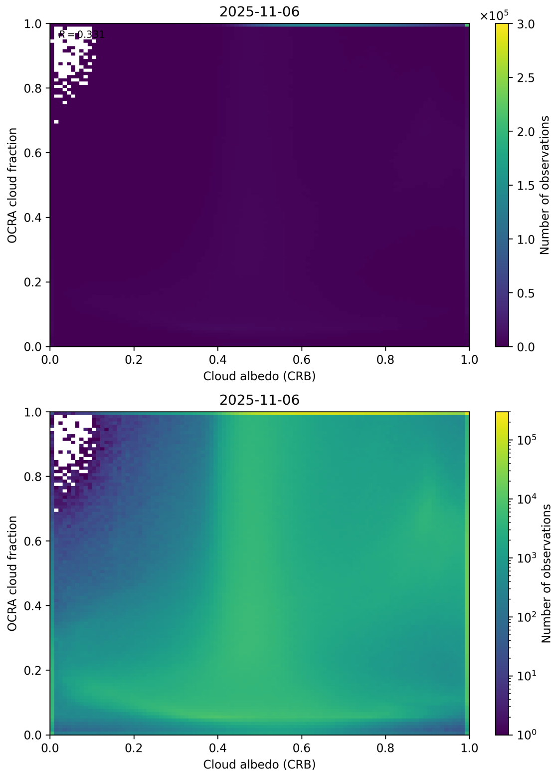
Figure 70: Scatter density plot of “Cloud albedo (CRB)” against “OCRA cloud fraction” for 2025-11-05 to 2025-11-07.
