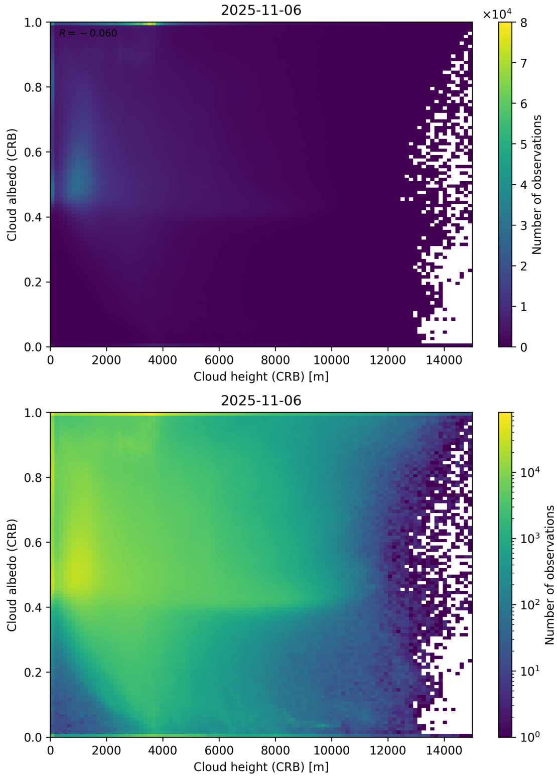
Figure 80: Scatter density plot of “Cloud height (CRB)” against “Cloud albedo (CRB)” for 2025-11-05 to 2025-11-07.
