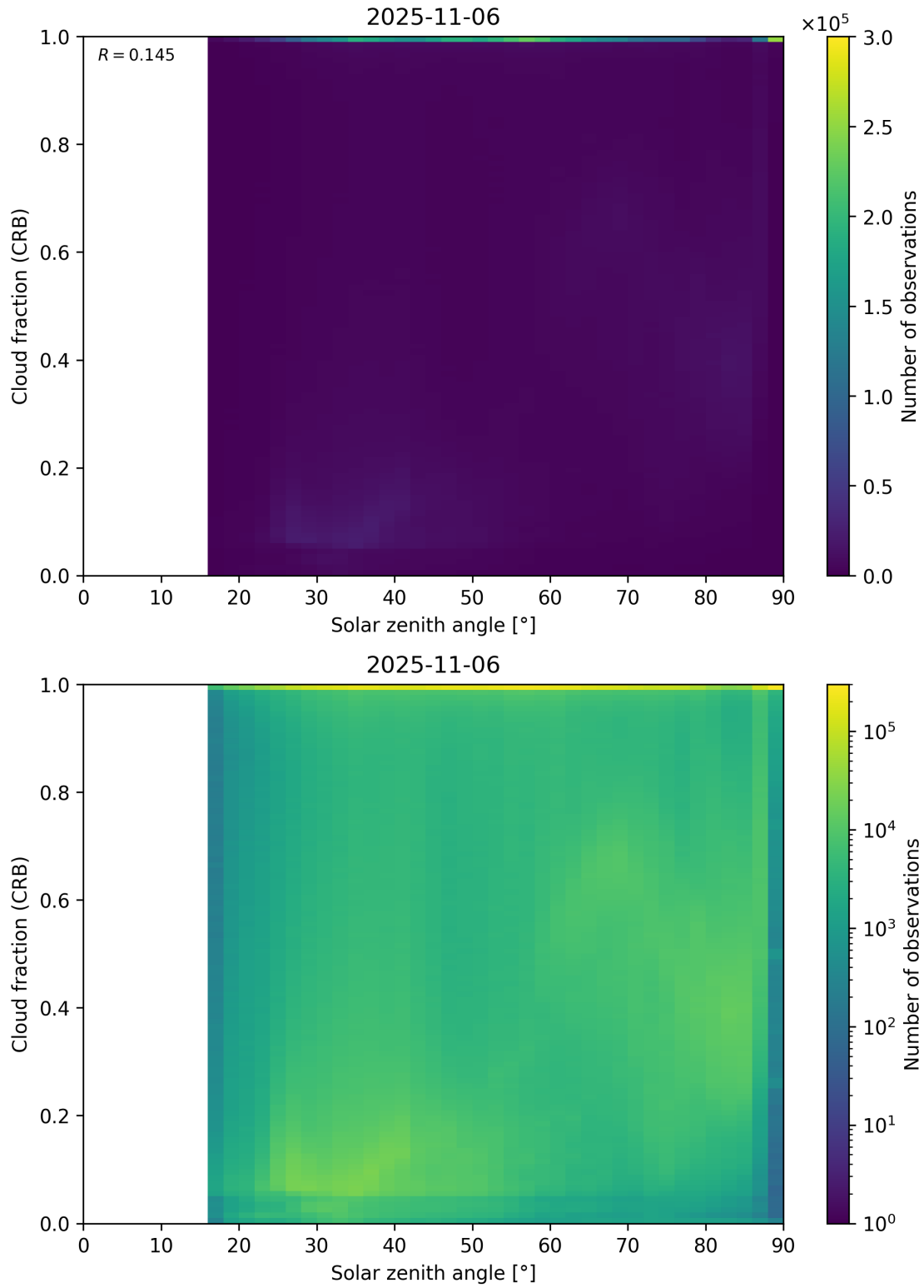
Figure 101: Scatter density plot of “Solar zenith angle” against “Cloud fraction (CRB)” for 2025-11-05 to 2025-11-07.
