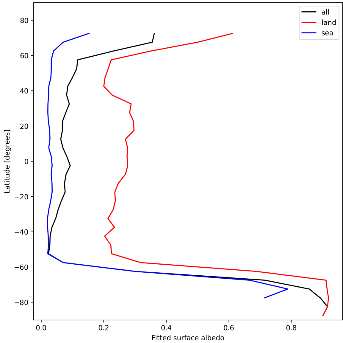
Figure 29: Zonal average of “Fitted surface albedo” for 2025-11-05 to 2025-11-07.
