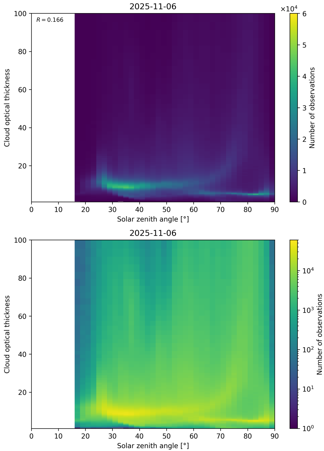
Figure 103: Scatter density plot of “Solar zenith angle” against “Cloud optical thickness” for 2025-11-05 to 2025-11-07.
