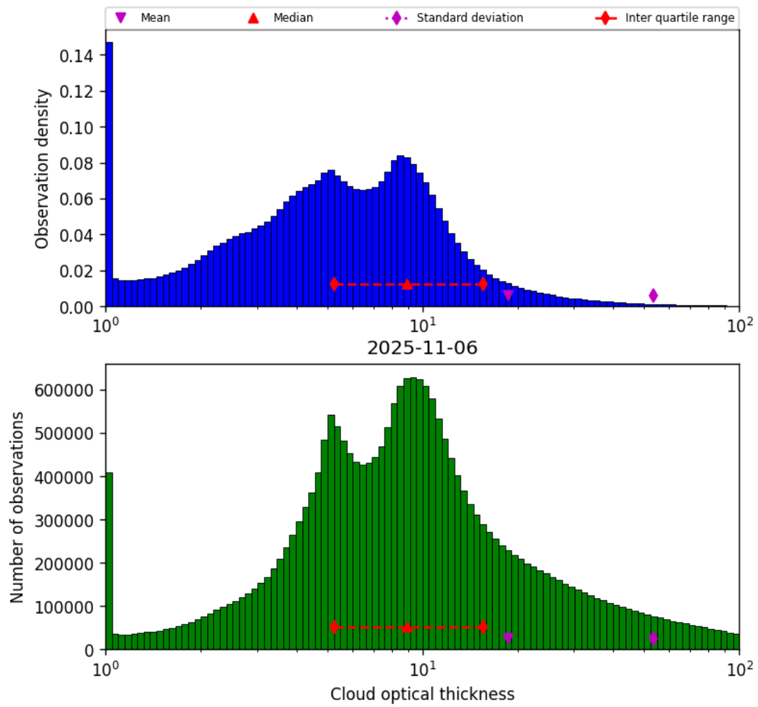
Figure 41: Histogram of “Cloud optical thickness” for 2025-11-05 to 2025-11-07
