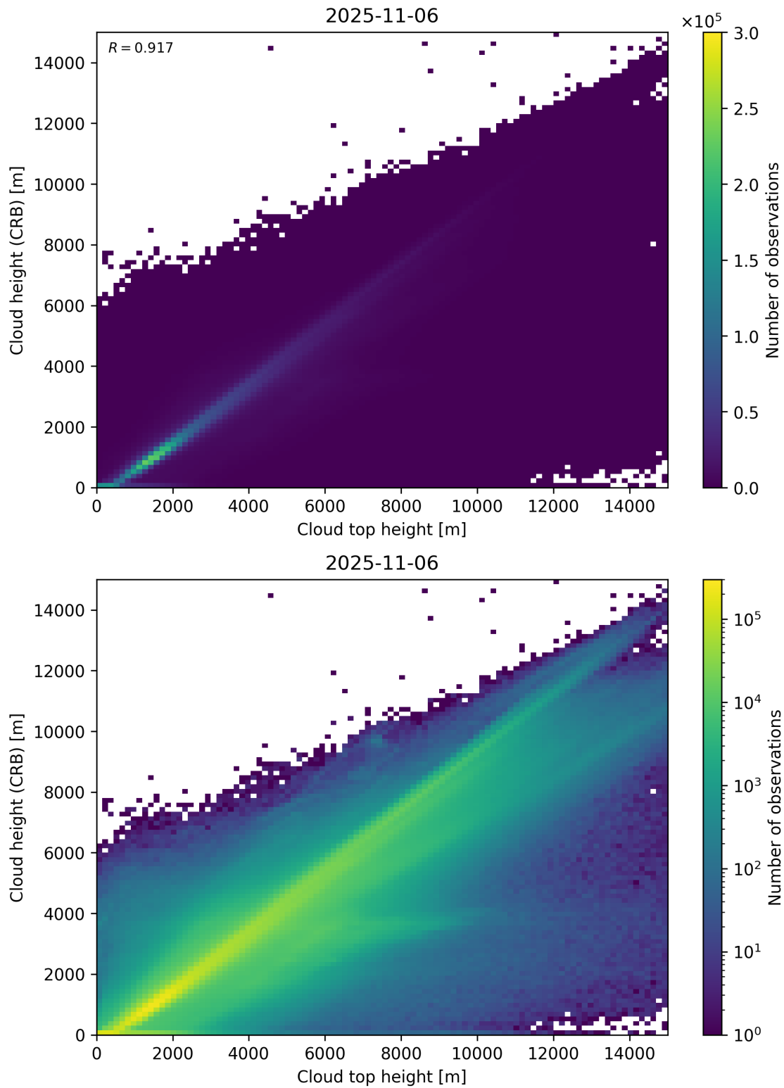
Figure 89: Scatter density plot of “Cloud top height” against “Cloud height (CRB)” for 2025-11-05 to 2025-11-07.
