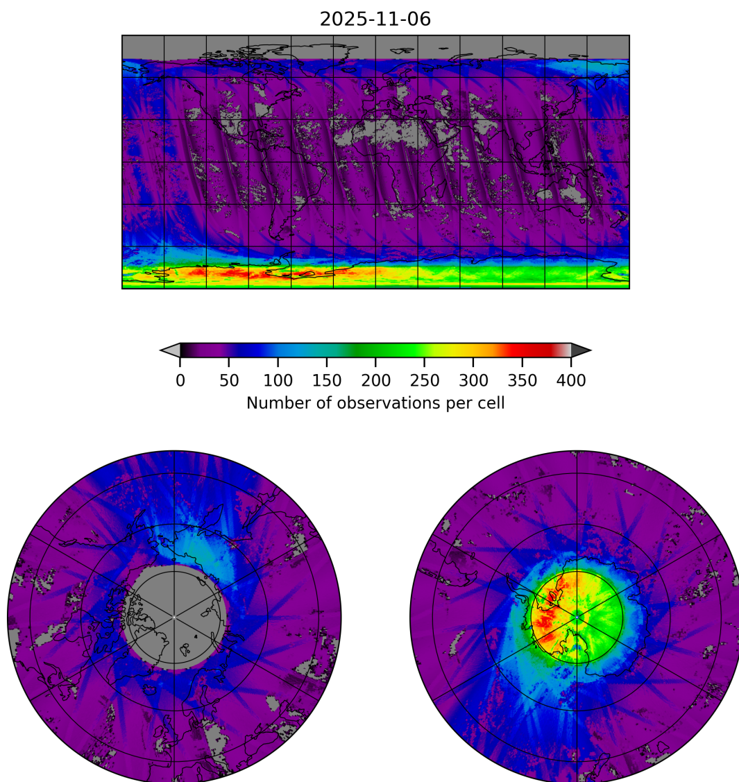
Figure 21: Map of the number of observations for 2025-11-05 to 2025-11-07
