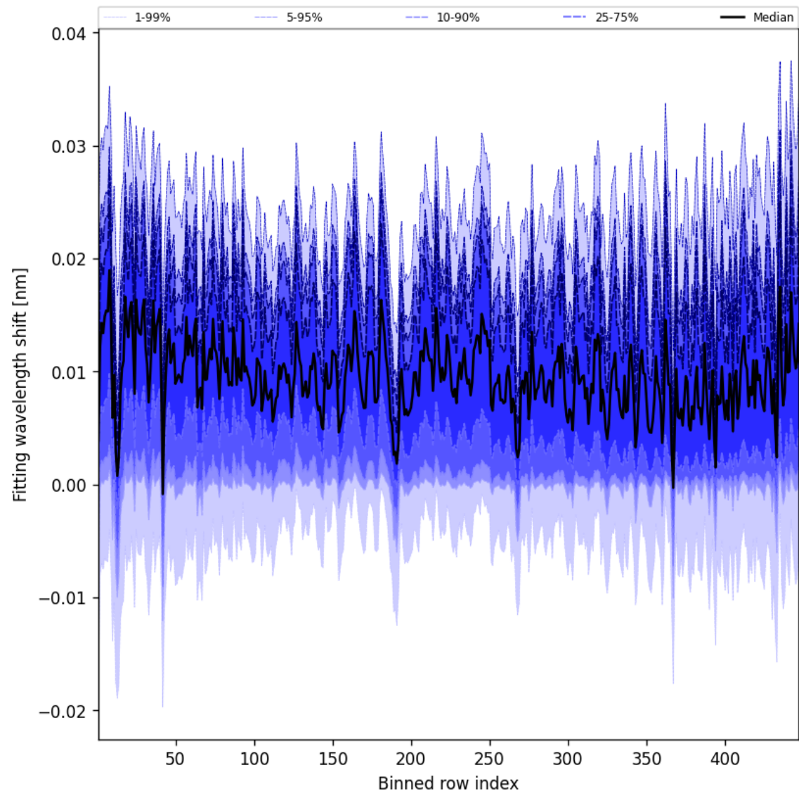
Figure 65: Along track statistics of “Fitting wavelength shift” for 2025-11-05 to 2025-11-07
