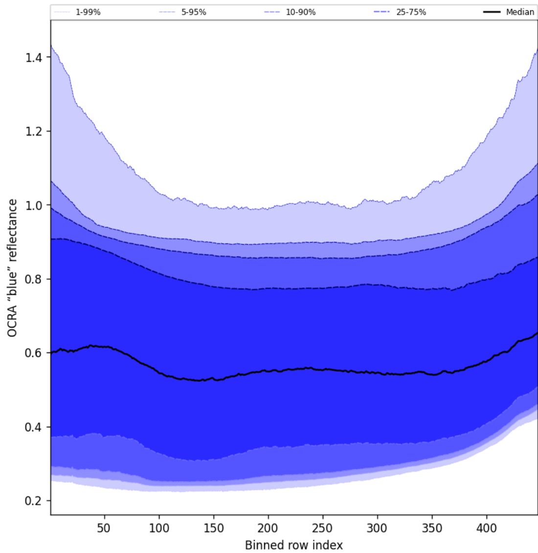
Figure 67: Along track statistics of “OCRA “blue” reflectance” for 2025-11-05 to 2025-11-07
