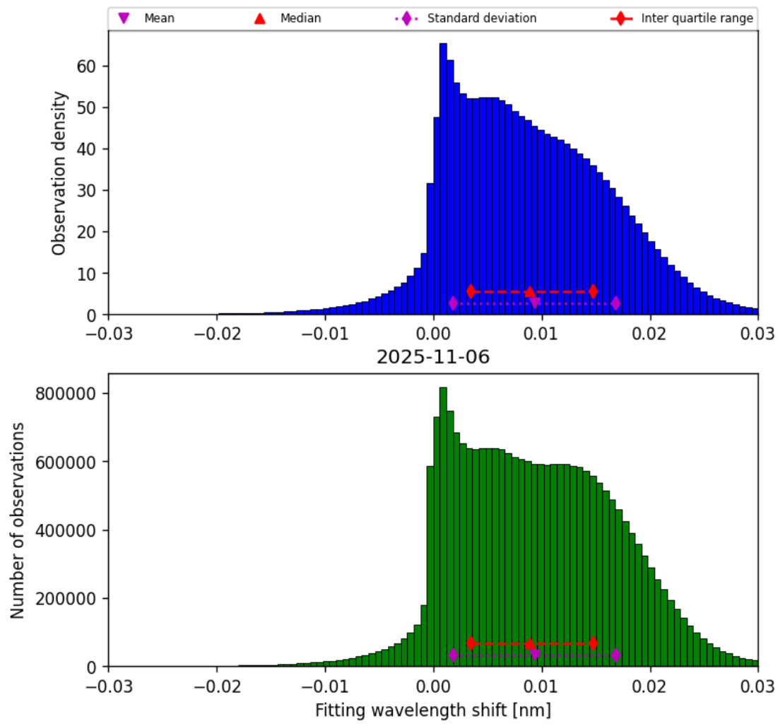
Figure 49: Histogram of “Fitting wavelength shift” for 2025-11-05 to 2025-11-07
