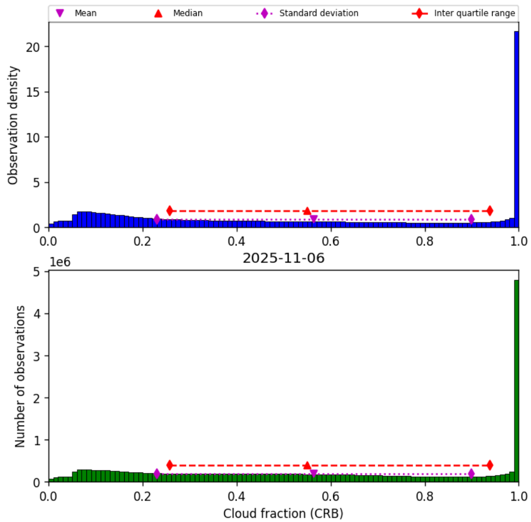
Figure 42: Histogram of “Cloud fraction (CRB)” for 2025-11-05 to 2025-11-07
