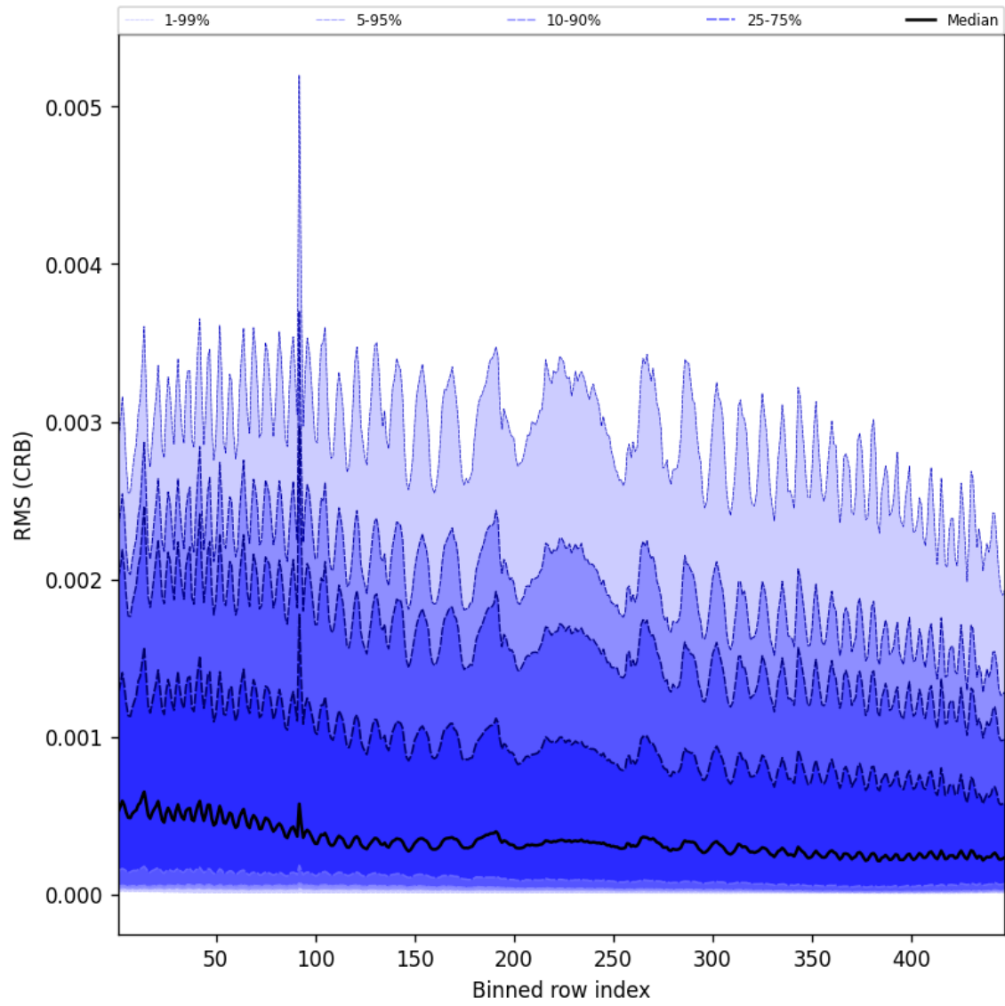
Figure 64: Along track statistics of “RMS (CRB)” for 2025-11-05 to 2025-11-07
