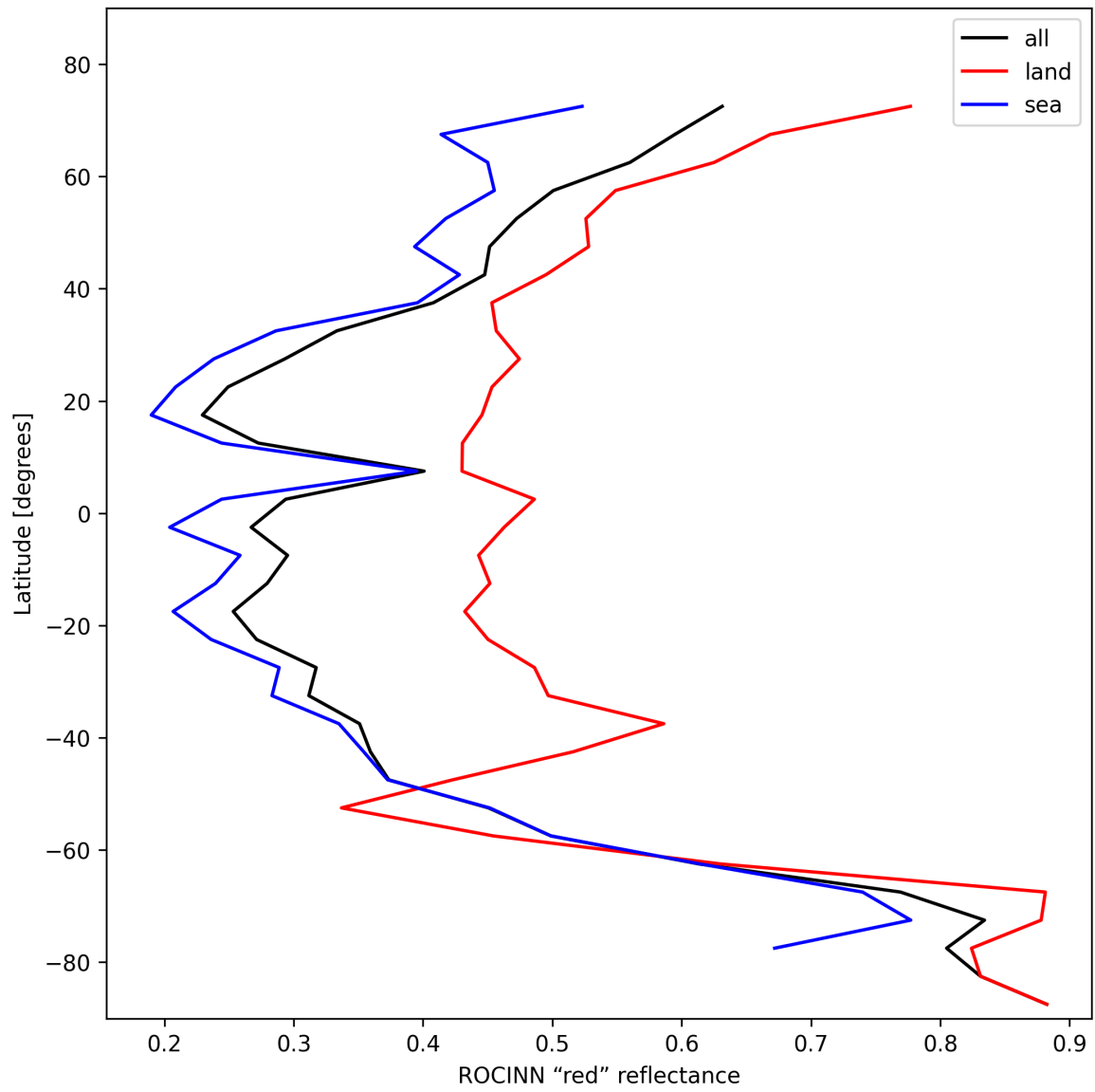
Figure 37: Zonal average of “ROCINN “red” reflectance” for 2025-11-05 to 2025-11-07.
