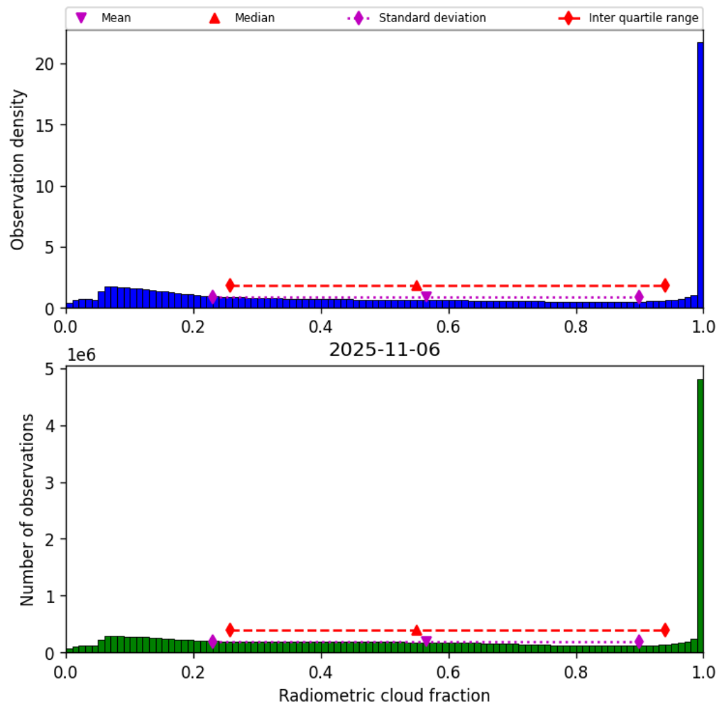
Figure 39: Histogram of “Radiometric cloud fraction” for 2025-11-05 to 2025-11-07
