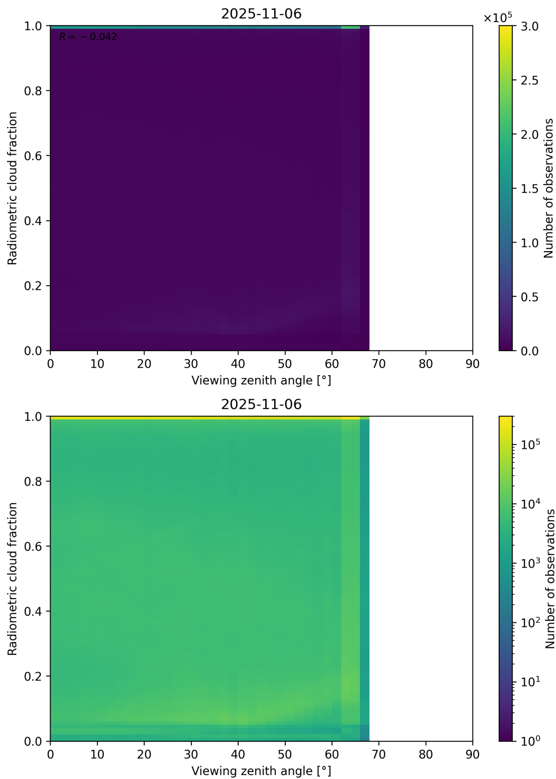
Figure 107: Scatter density plot of “Viewing zenith angle” against “Radiometric cloud fraction” for 2025-11-05 to 2025-11-07.
