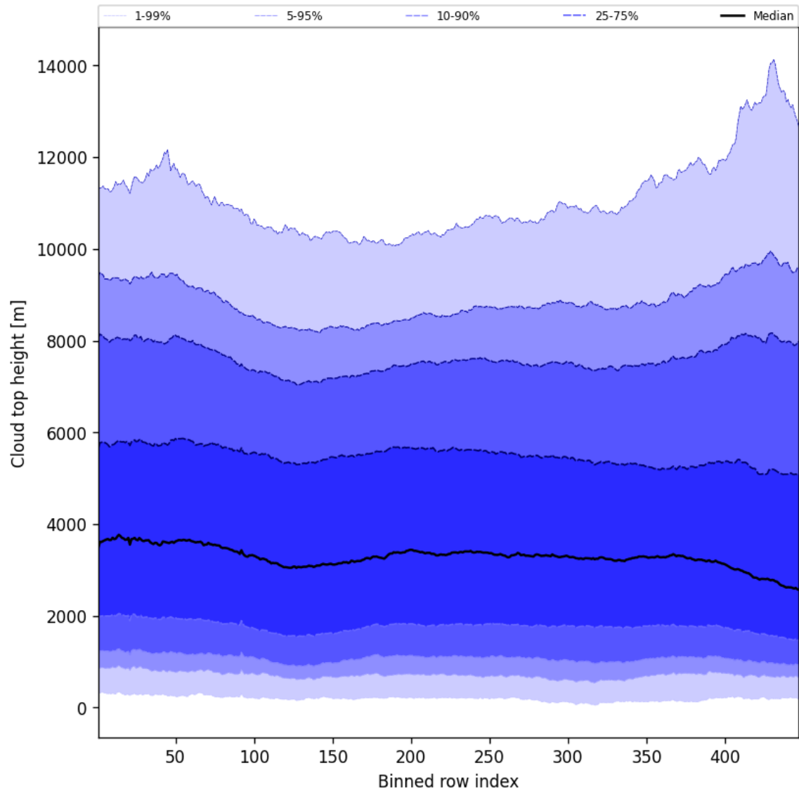
Figure 56: Along track statistics of “Cloud top height” for 2025-11-05 to 2025-11-07
