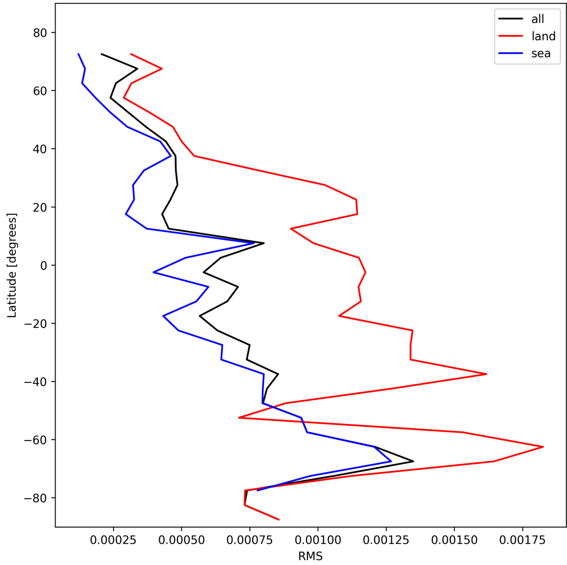
Figure 31: Zonal average of “RMS” for 2025-11-05 to 2025-11-07.
