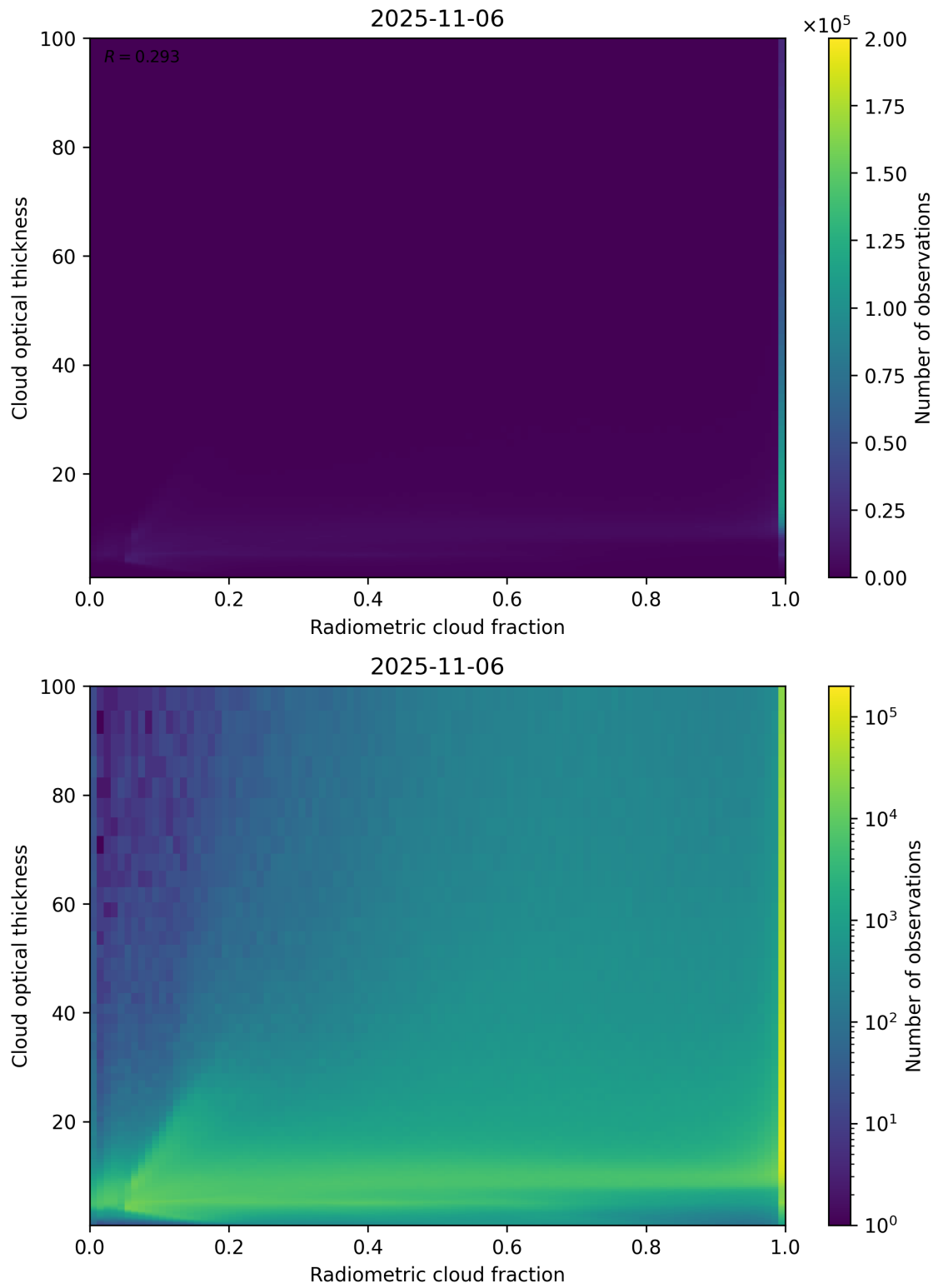
Figure 75: Scatter density plot of “Radiometric cloud fraction” against “Cloud optical thickness” for 2025-11-05 to 2025-11-07.
