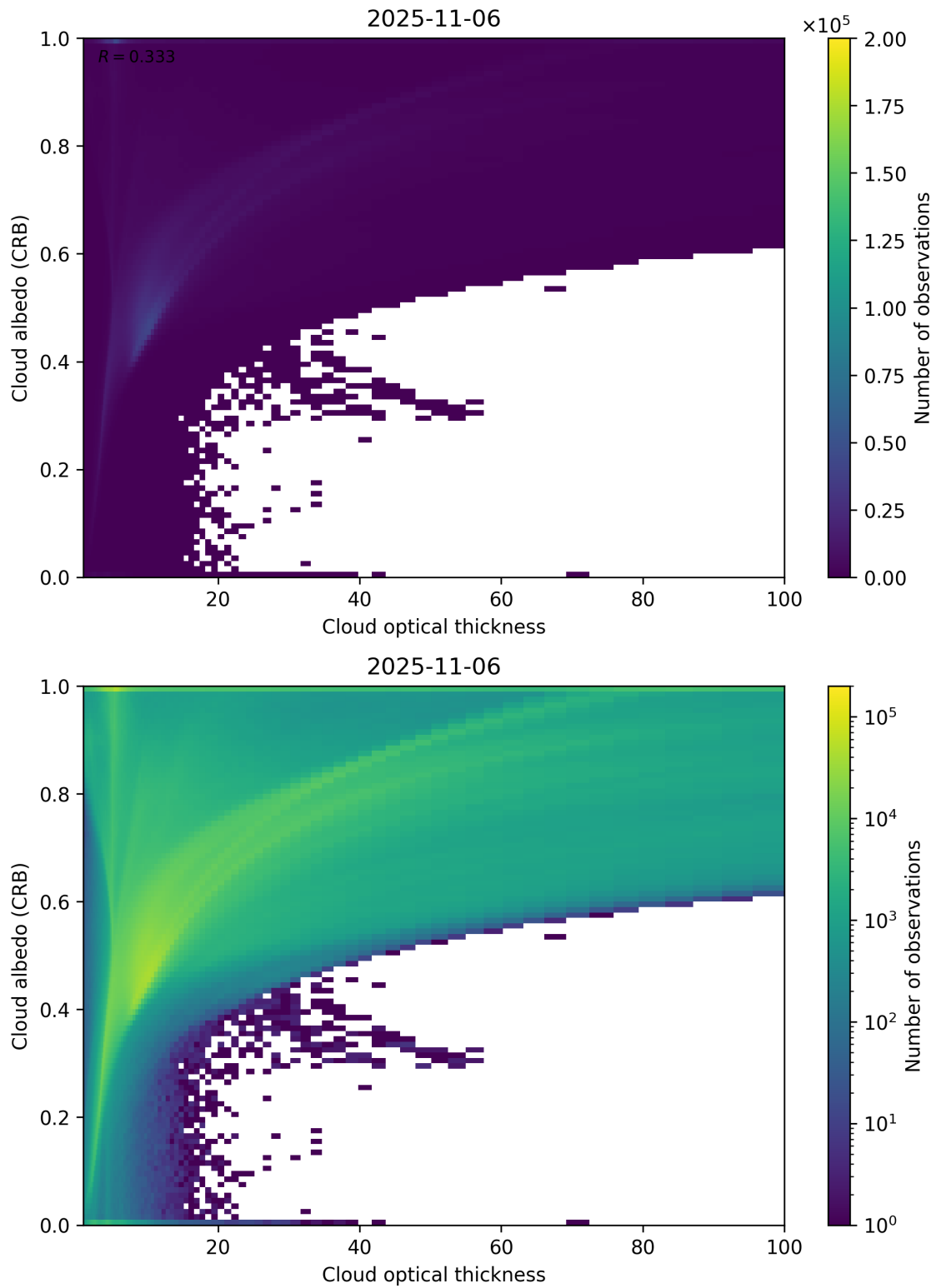
Figure 82: Scatter density plot of “Cloud optical thickness” against “Cloud albedo (CRB)” for 2025-11-05 to 2025-11-07.
