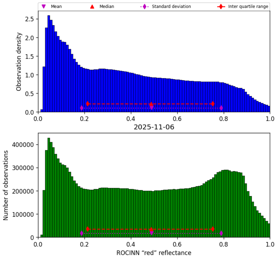
Figure 53: Histogram of “ROCINN “red” reflectance” for 2025-11-05 to 2025-11-07
