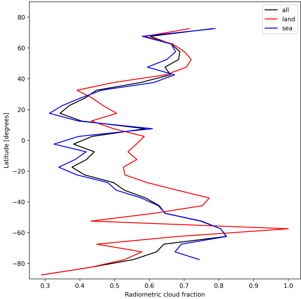
Figure 23: Zonal average of “Radiometric cloud fraction” for 2025-11-05 to 2025-11-07.
