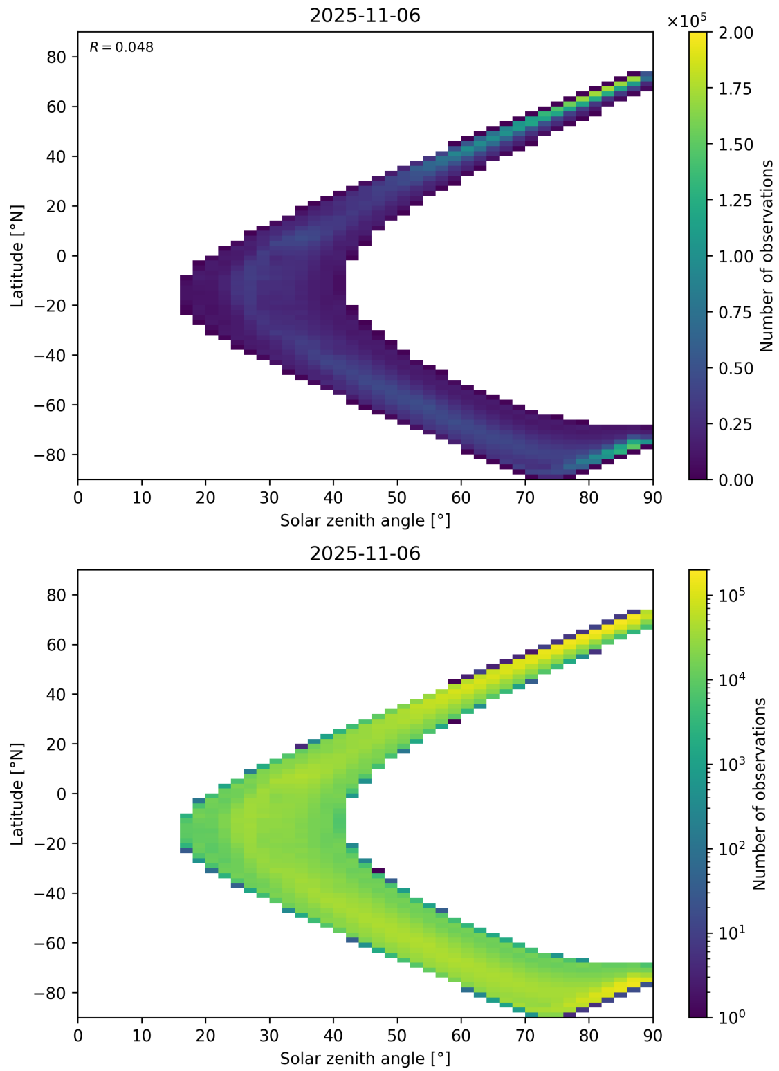
Figure 105: Scatter density plot of “Solar zenith angle” against “Latitude” for 2025-11-05 to 2025-11-07.
