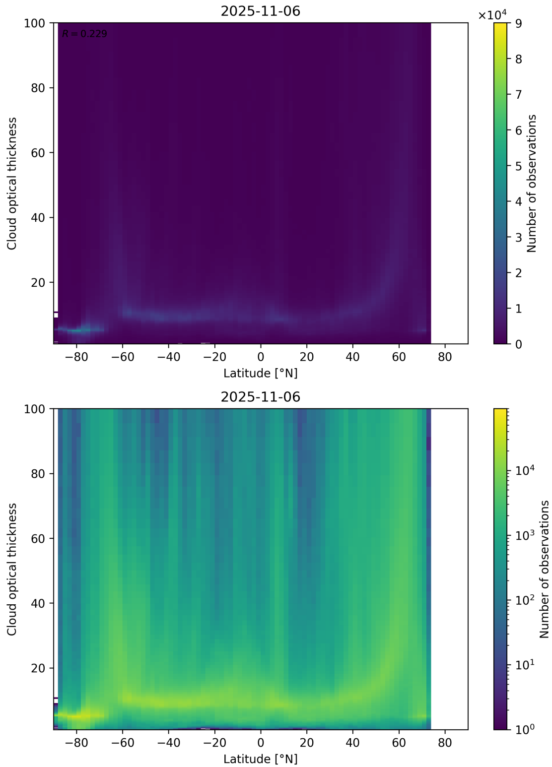
Figure 96: Scatter density plot of “Latitude” against “Cloud optical thickness” for 2025-11-05 to 2025-11-07.
