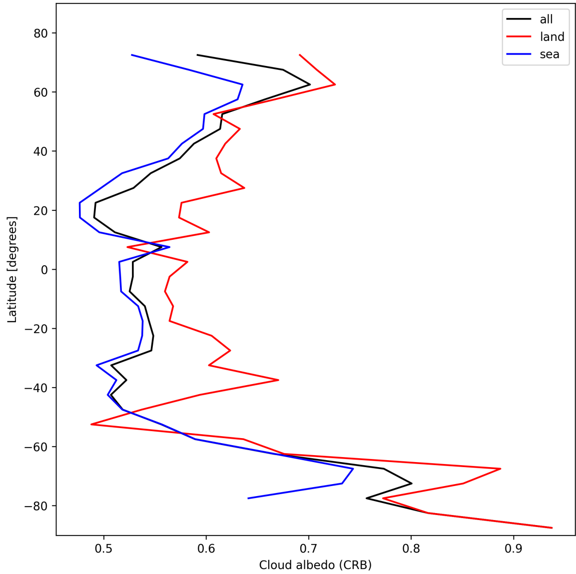
Figure 28: Zonal average of “Cloud albedo (CRB)” for 2025-11-05 to 2025-11-07.
