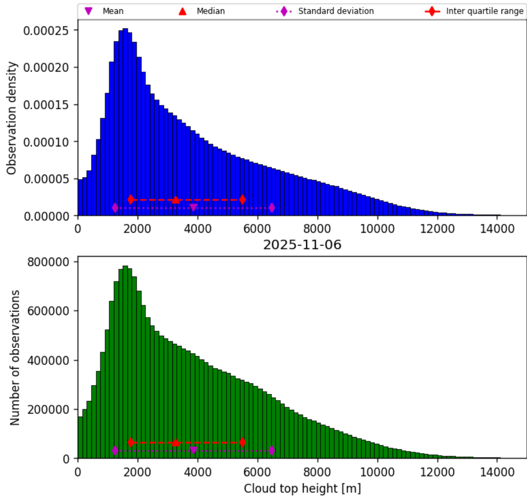
Figure 40: Histogram of “Cloud top height” for 2025-11-05 to 2025-11-07
