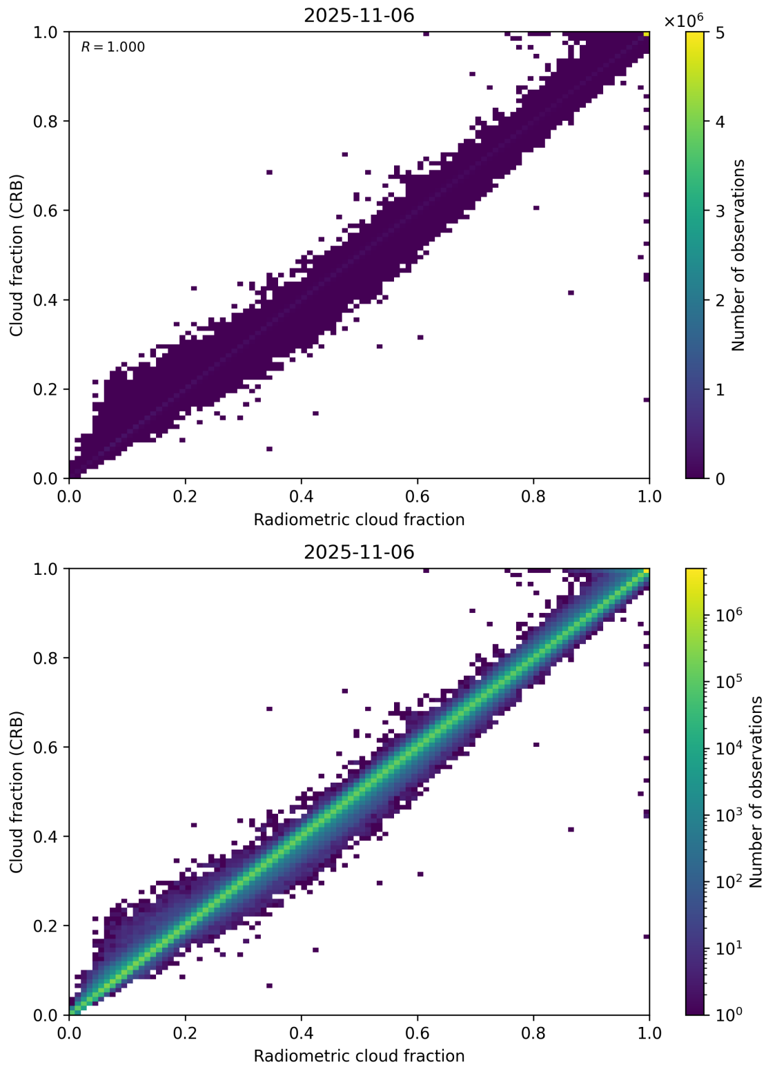
Figure 73: Scatter density plot of “Radiometric cloud fraction” against “Cloud fraction (CRB)” for 2025-11-05 to 2025-11-07.
