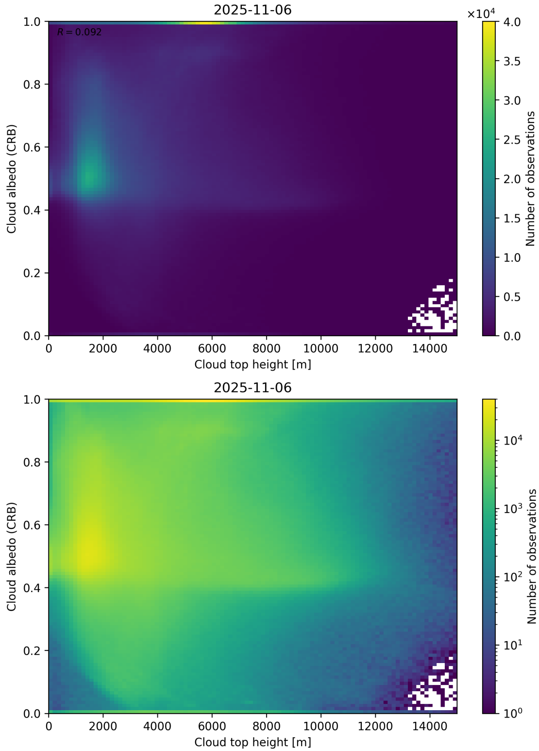
Figure 86: Scatter density plot of “Cloud top height” against “Cloud albedo (CRB)” for 2025-11-05 to 2025-11-07.
