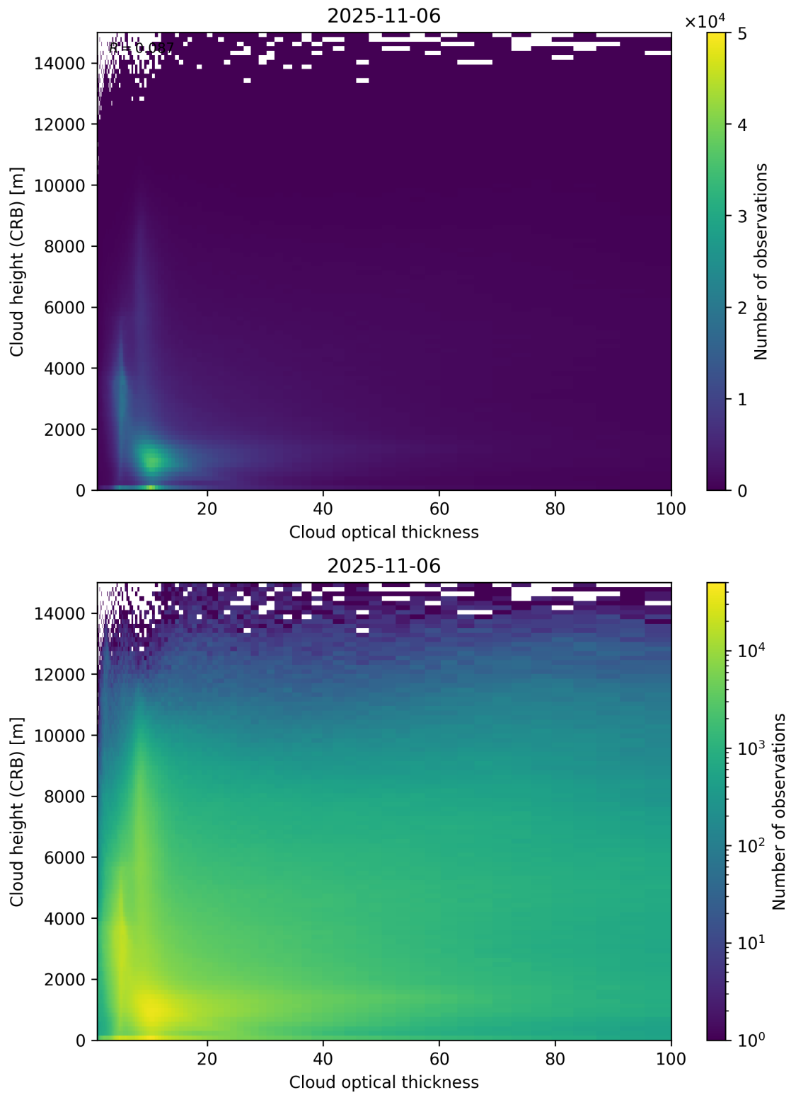
Figure 85: Scatter density plot of “Cloud optical thickness” against “Cloud height (CRB)” for 2025-11-05 to 2025-11-07.
