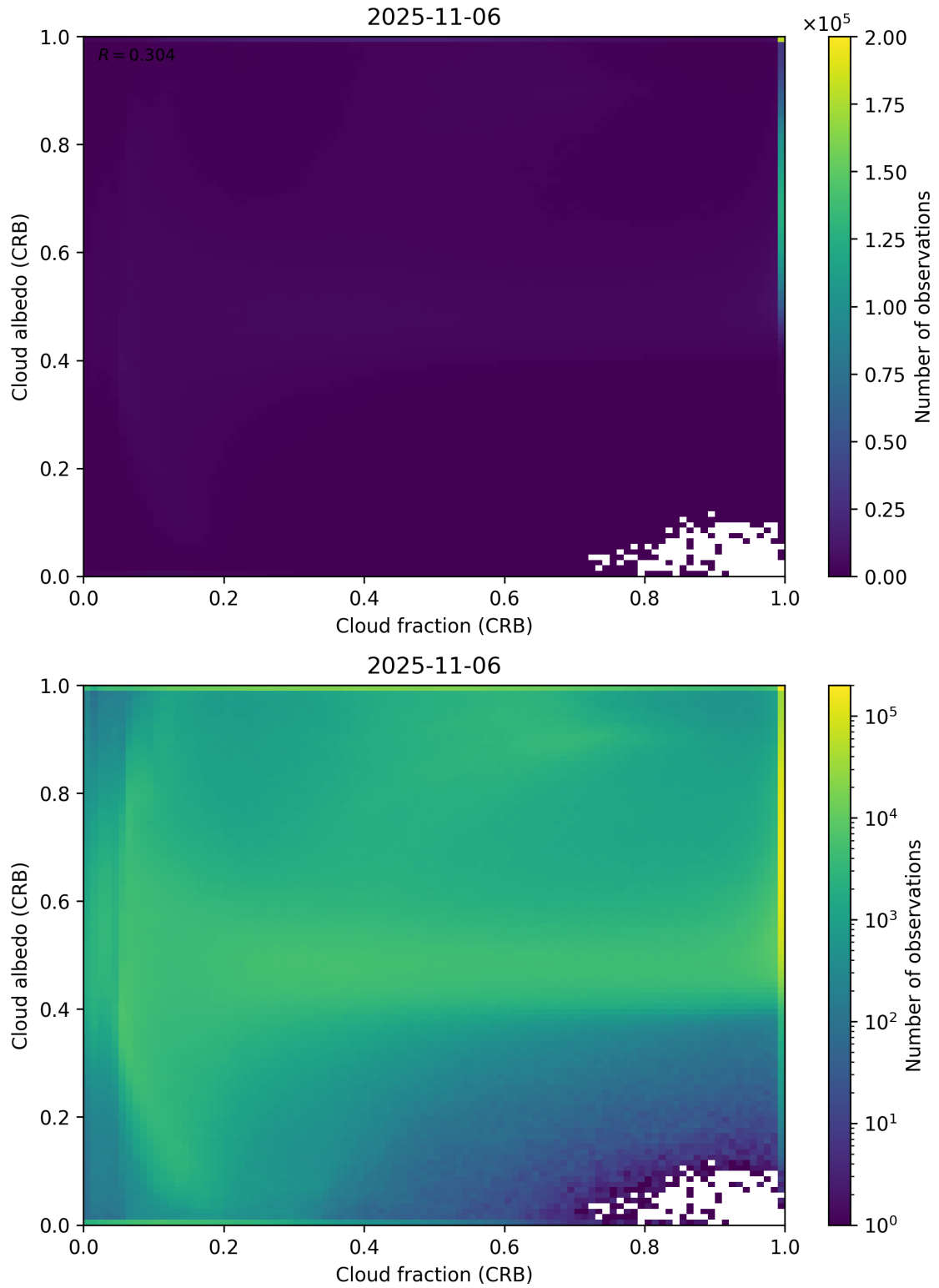
Figure 77: Scatter density plot of “Cloud fraction (CRB)” against “Cloud albedo (CRB)” for 2025-11-05 to 2025-11-07.
