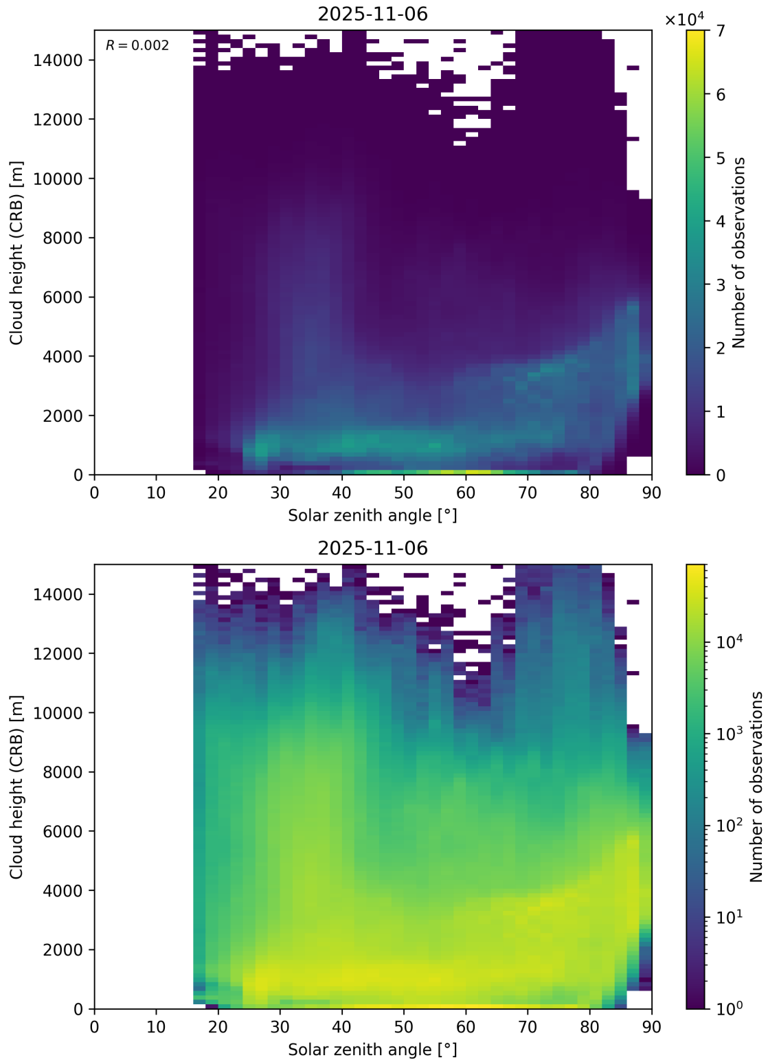
Figure 102: Scatter density plot of “Solar zenith angle” against “Cloud height (CRB)” for 2025-11-05 to 2025-11-07.
