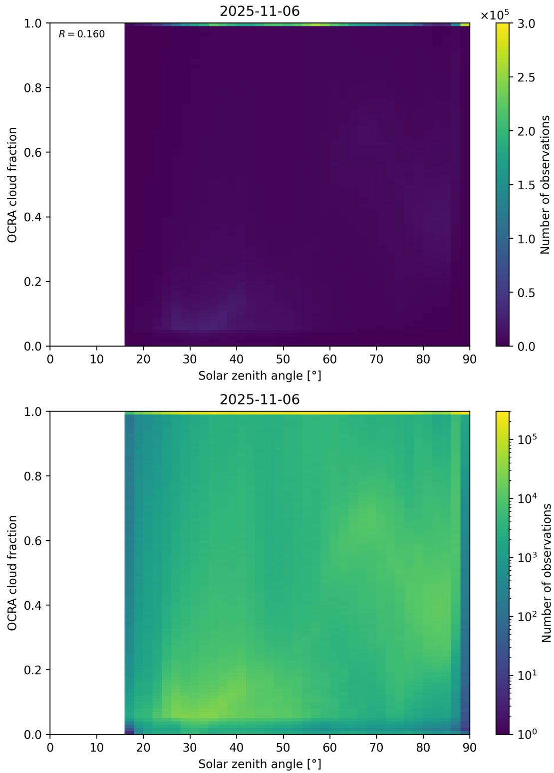
Figure 100: Scatter density plot of “Solar zenith angle” against “OCRA cloud fraction” for 2025-11-05 to 2025-11-07.
