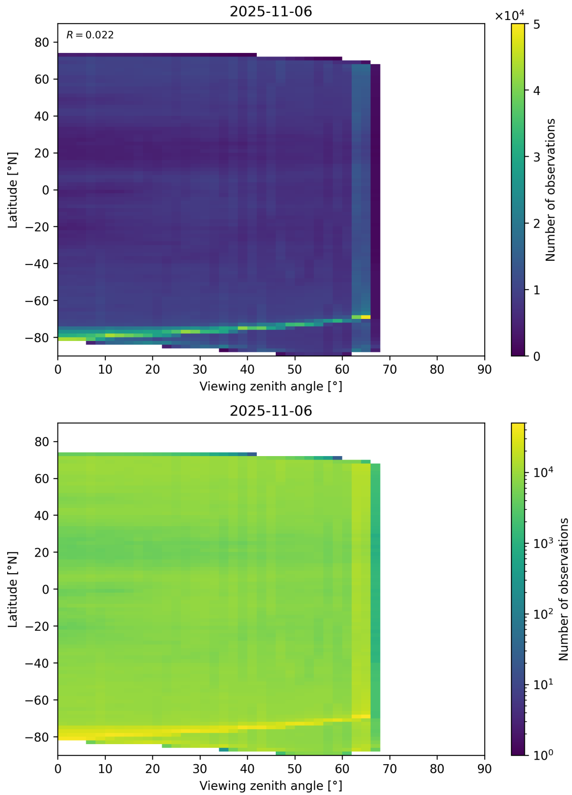
Figure 113: Scatter density plot of “Viewing zenith angle” against “Latitude” for 2025-11-05 to 2025-11-07.
