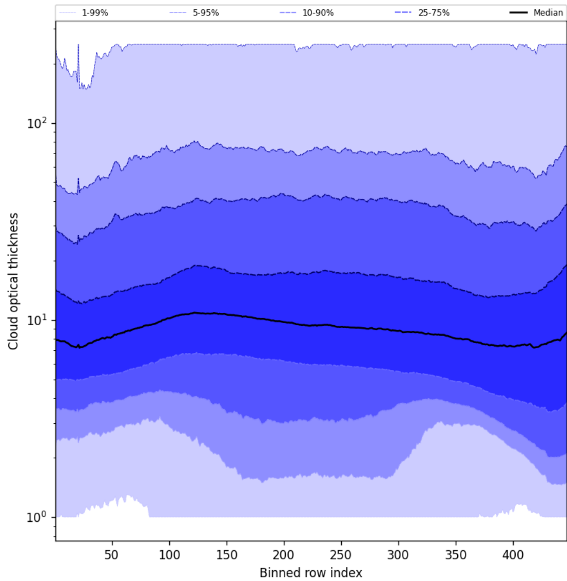
Figure 57: Along track statistics of “Cloud optical thickness” for 2025-11-05 to 2025-11-07
