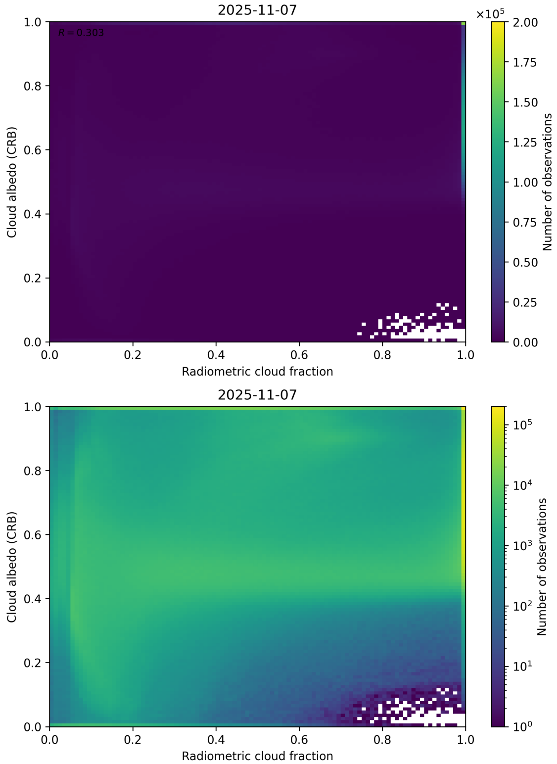
Figure 71: Scatter density plot of “Radiometric cloud fraction” against “Cloud albedo (CRB)” for 2025-11-07 to 2025-11-08.
