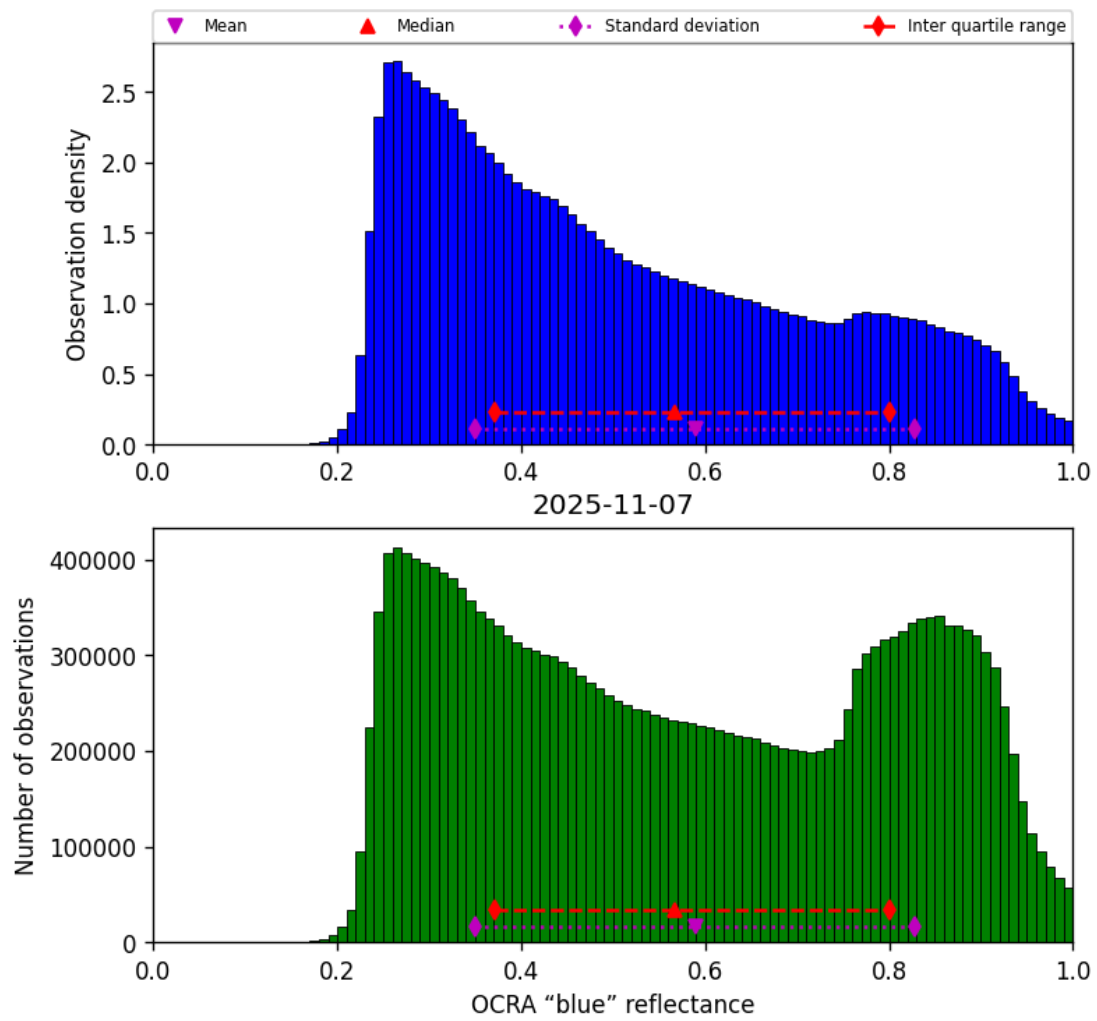
Figure 51: Histogram of “OCRA “blue” reflectance” for 2025-11-07 to 2025-11-08
