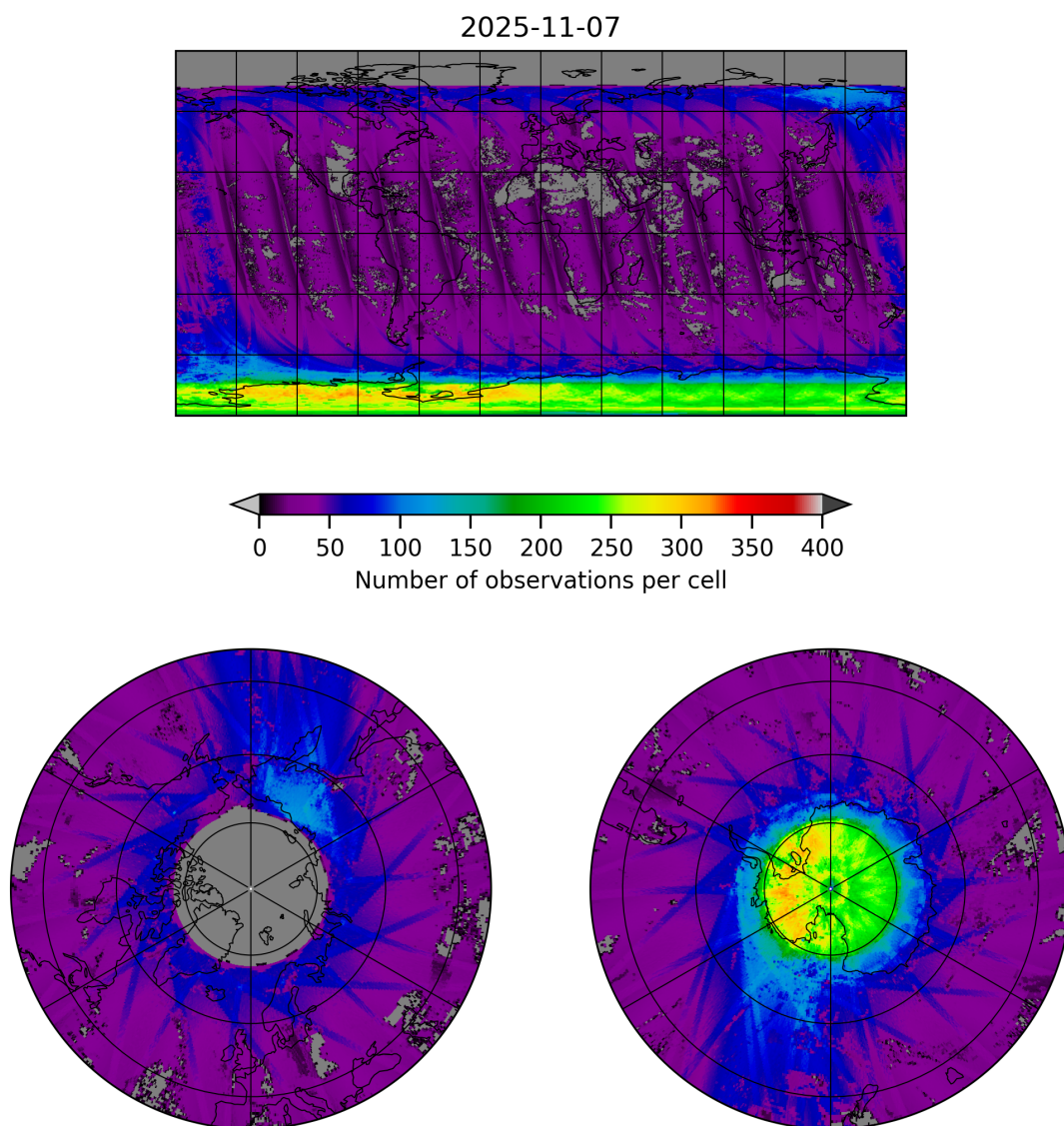
Figure 21: Map of the number of observations for 2025-11-07 to 2025-11-08
