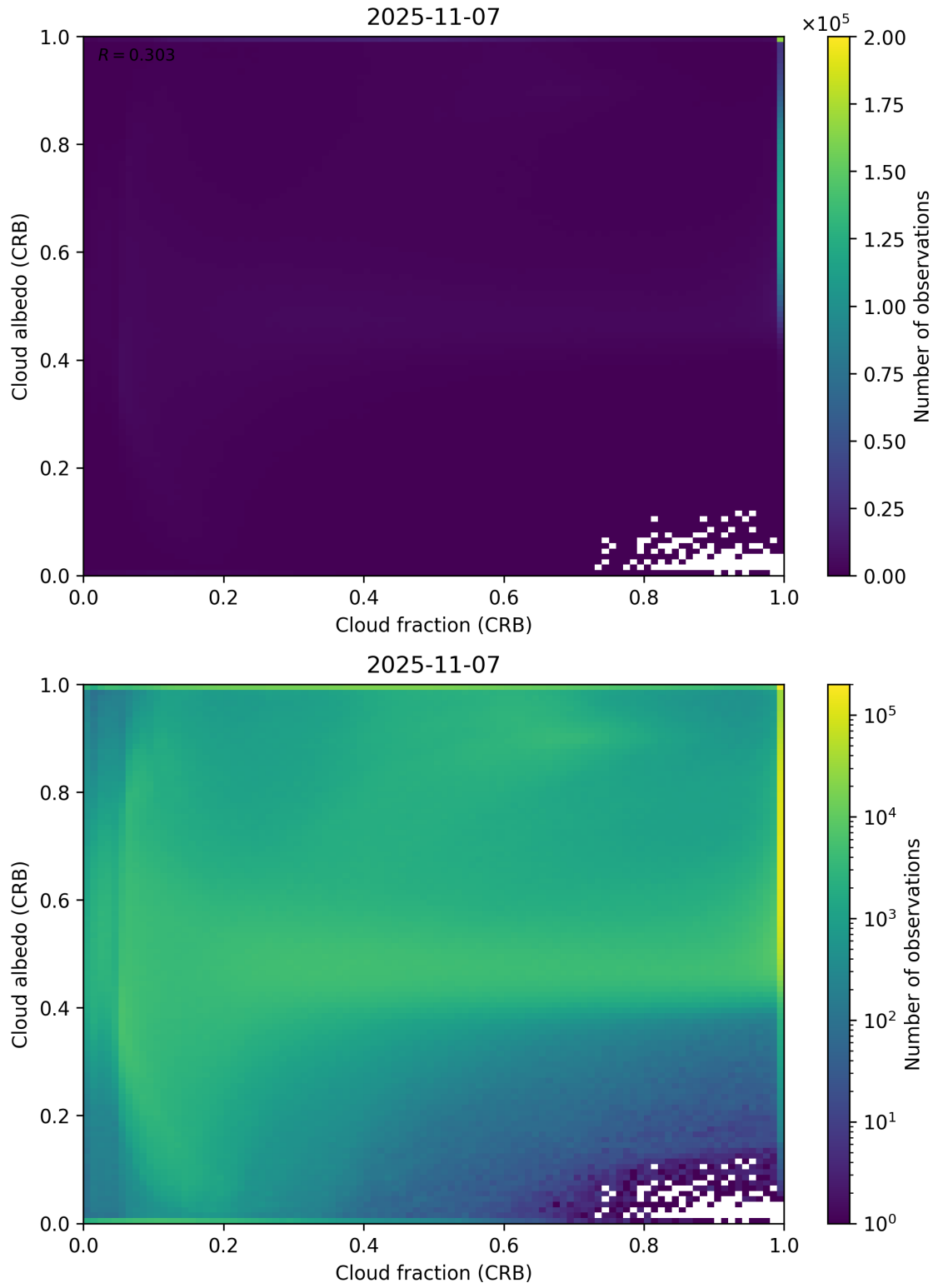
Figure 77: Scatter density plot of “Cloud fraction (CRB)” against “Cloud albedo (CRB)” for 2025-11-07 to 2025-11-08.
