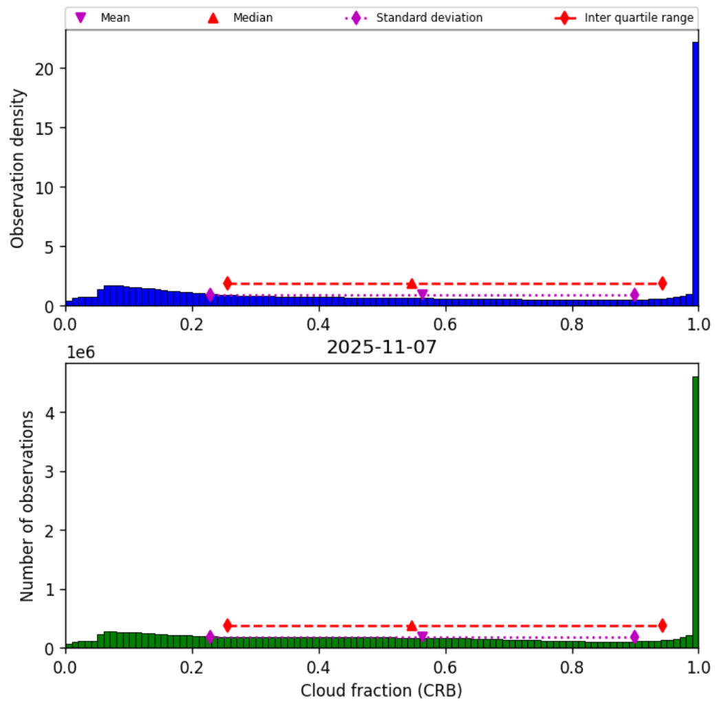
Figure 42: Histogram of “Cloud fraction (CRB)” for 2025-11-07 to 2025-11-08
