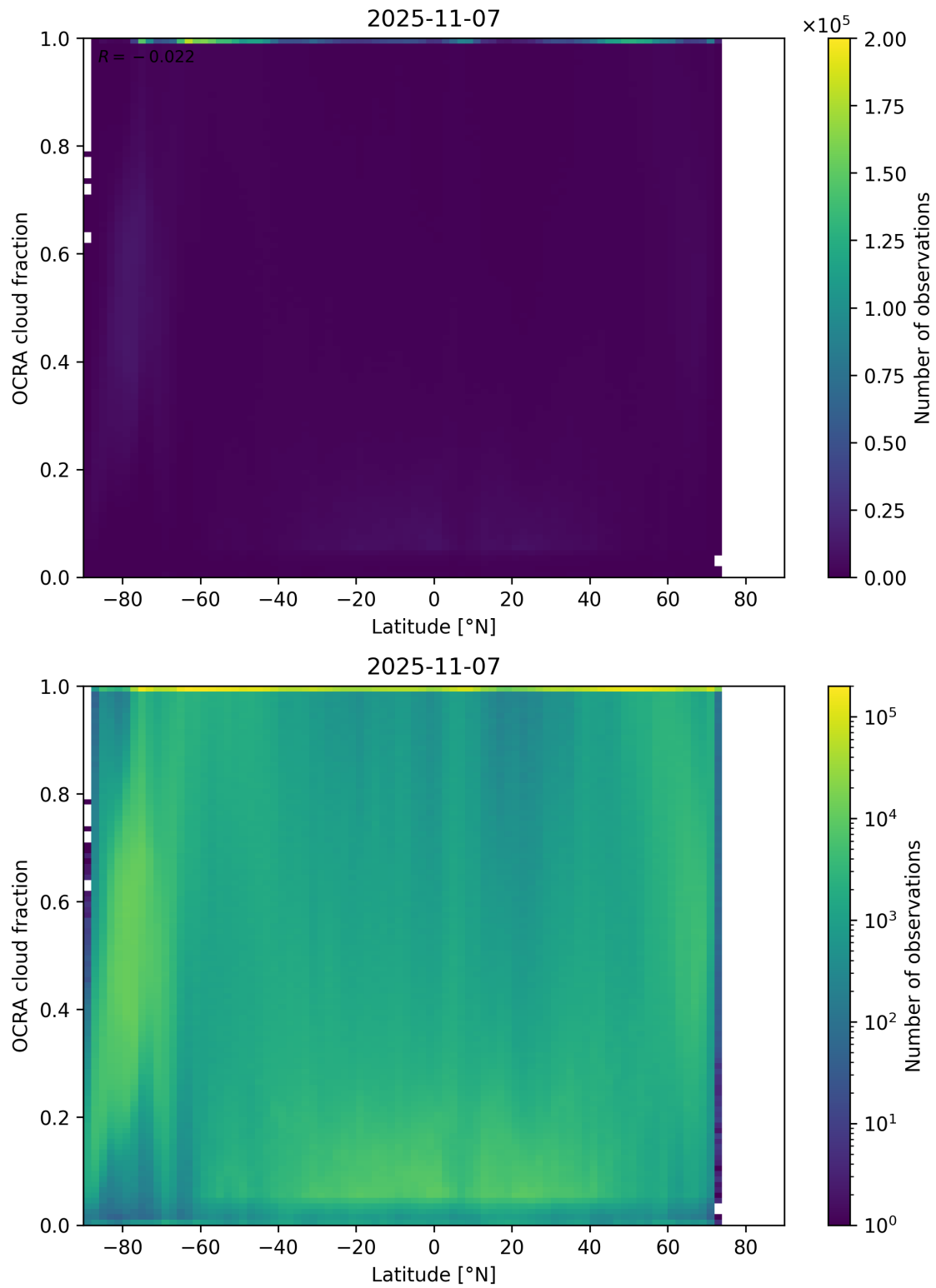
Figure 93: Scatter density plot of “Latitude” against “OCRA cloud fraction” for 2025-11-07 to 2025-11-08.
