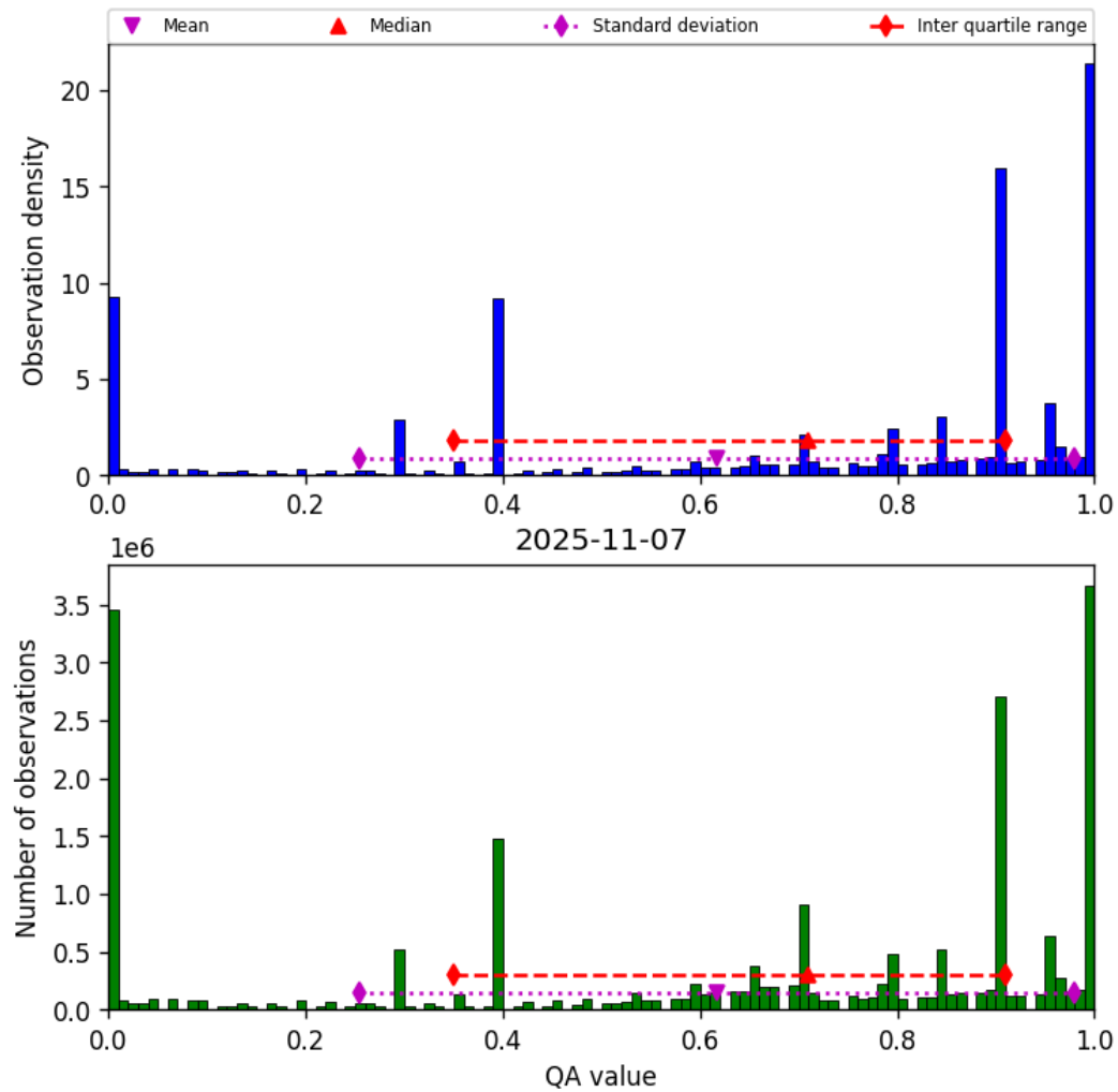
Figure 38: Histogram of “QA value” for 2025-11-07 to 2025-11-08
