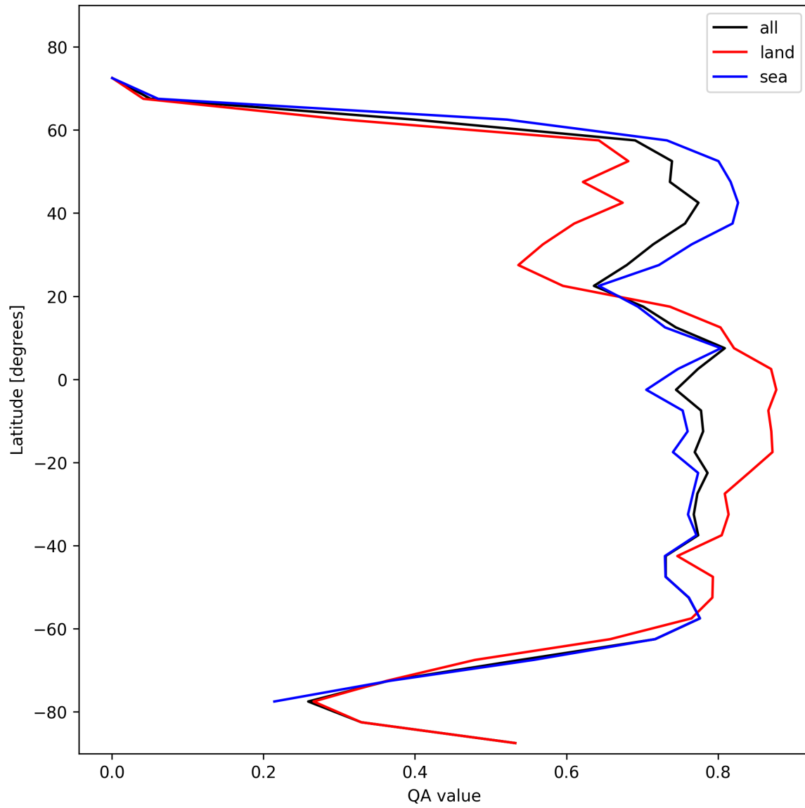
Figure 22: Zonal average of “QA value” for 2025-11-07 to 2025-11-08.
