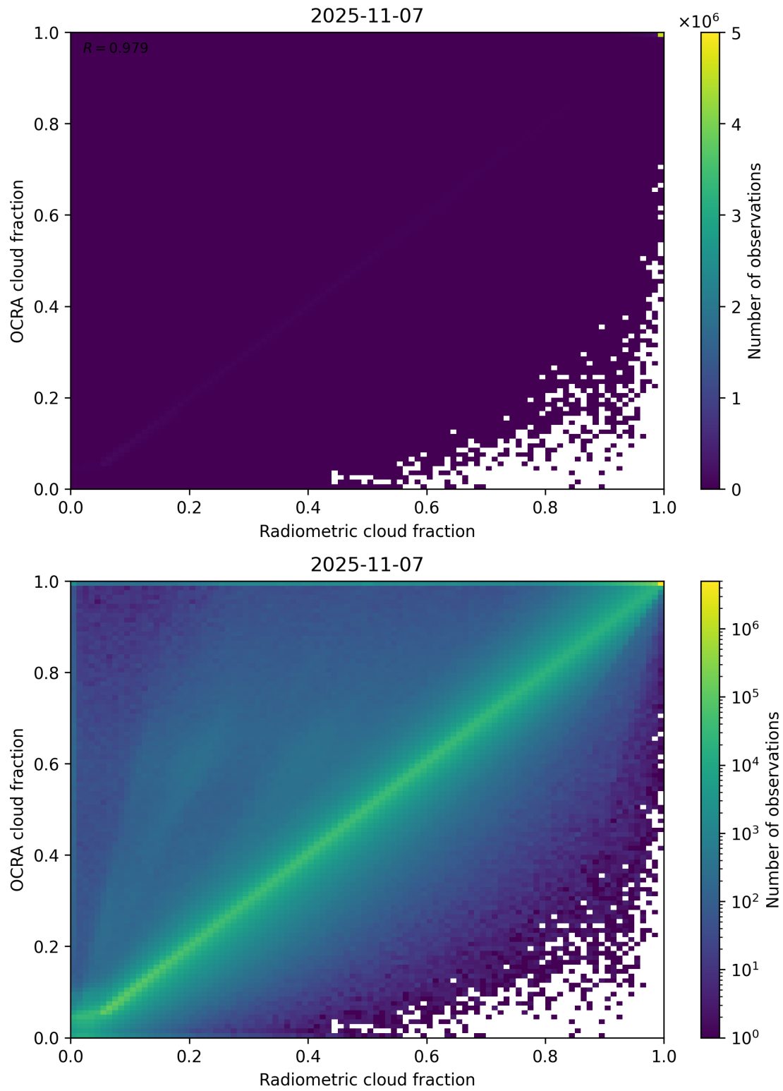
Figure 72: Scatter density plot of “Radiometric cloud fraction” against “OCRA cloud fraction” for 2025-11-07 to 2025-11-08.
