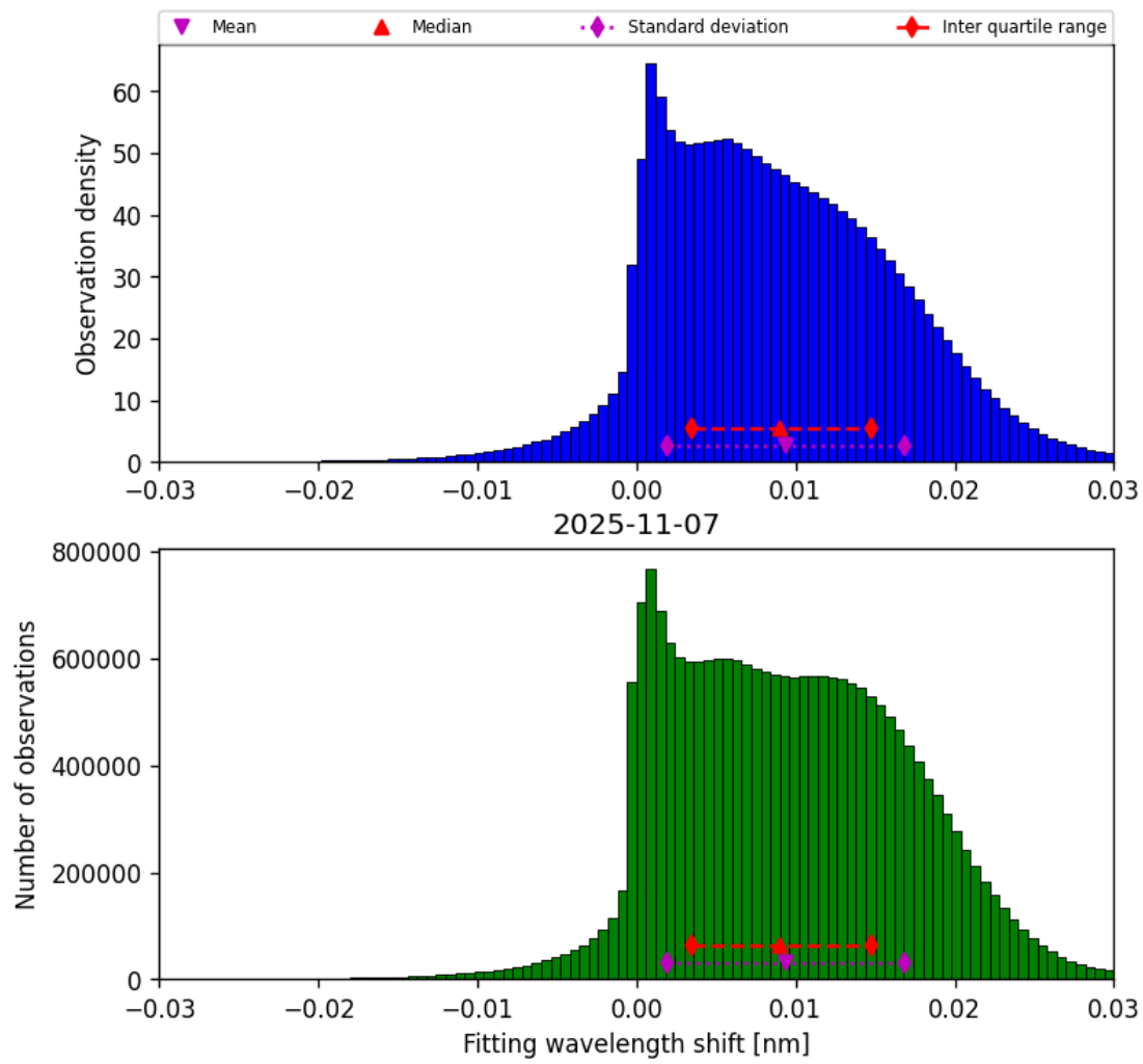
Figure 49: Histogram of “Fitting wavelength shift” for 2025-11-07 to 2025-11-08
