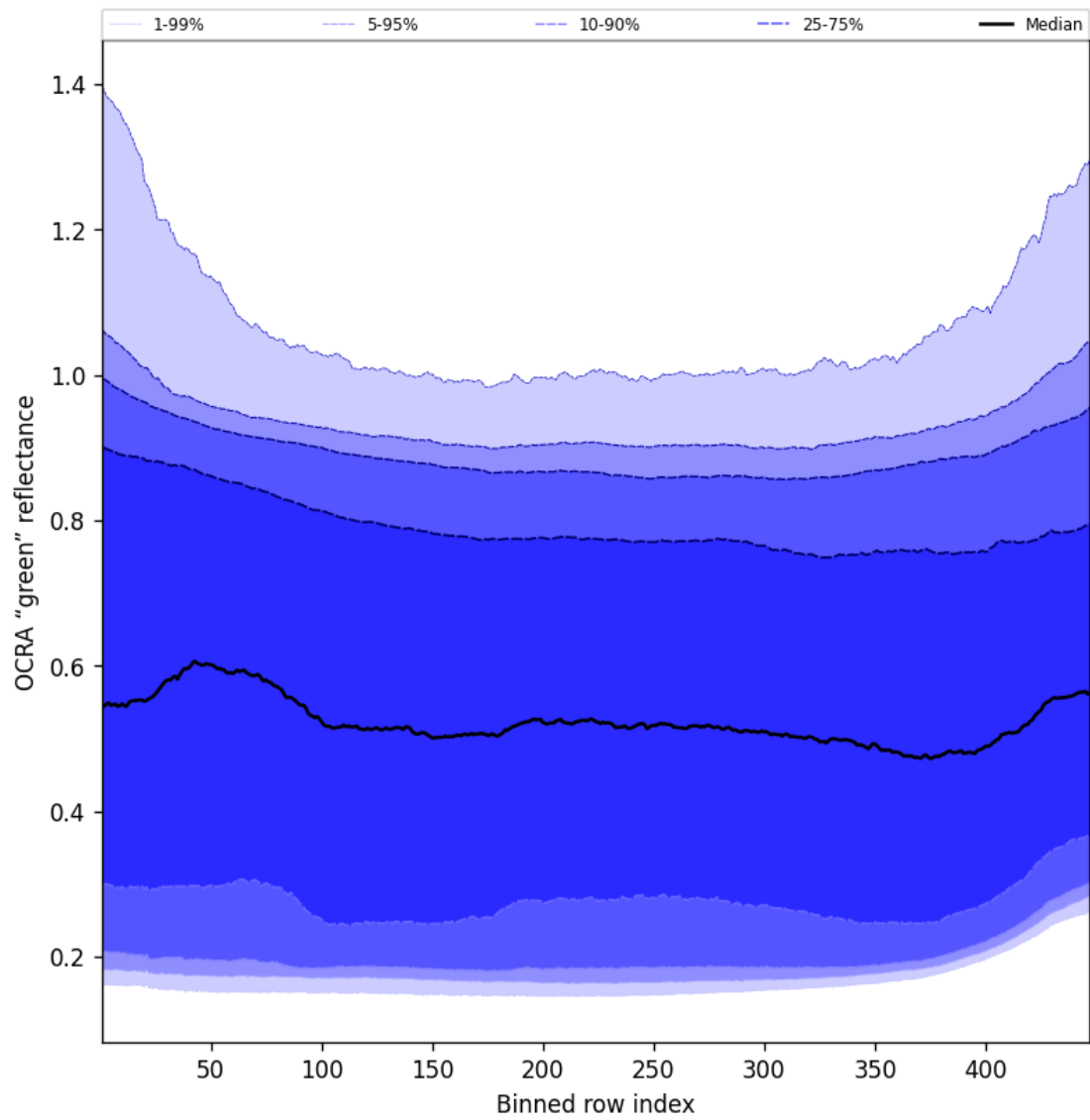
Figure 68: Along track statistics of “OCRA “green” reflectance” for 2025-11-07 to 2025-11-08
