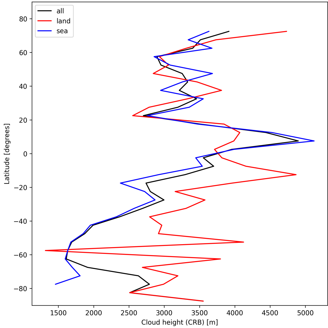
Figure 27: Zonal average of “Cloud height (CRB)” for 2025-11-07 to 2025-11-08.
