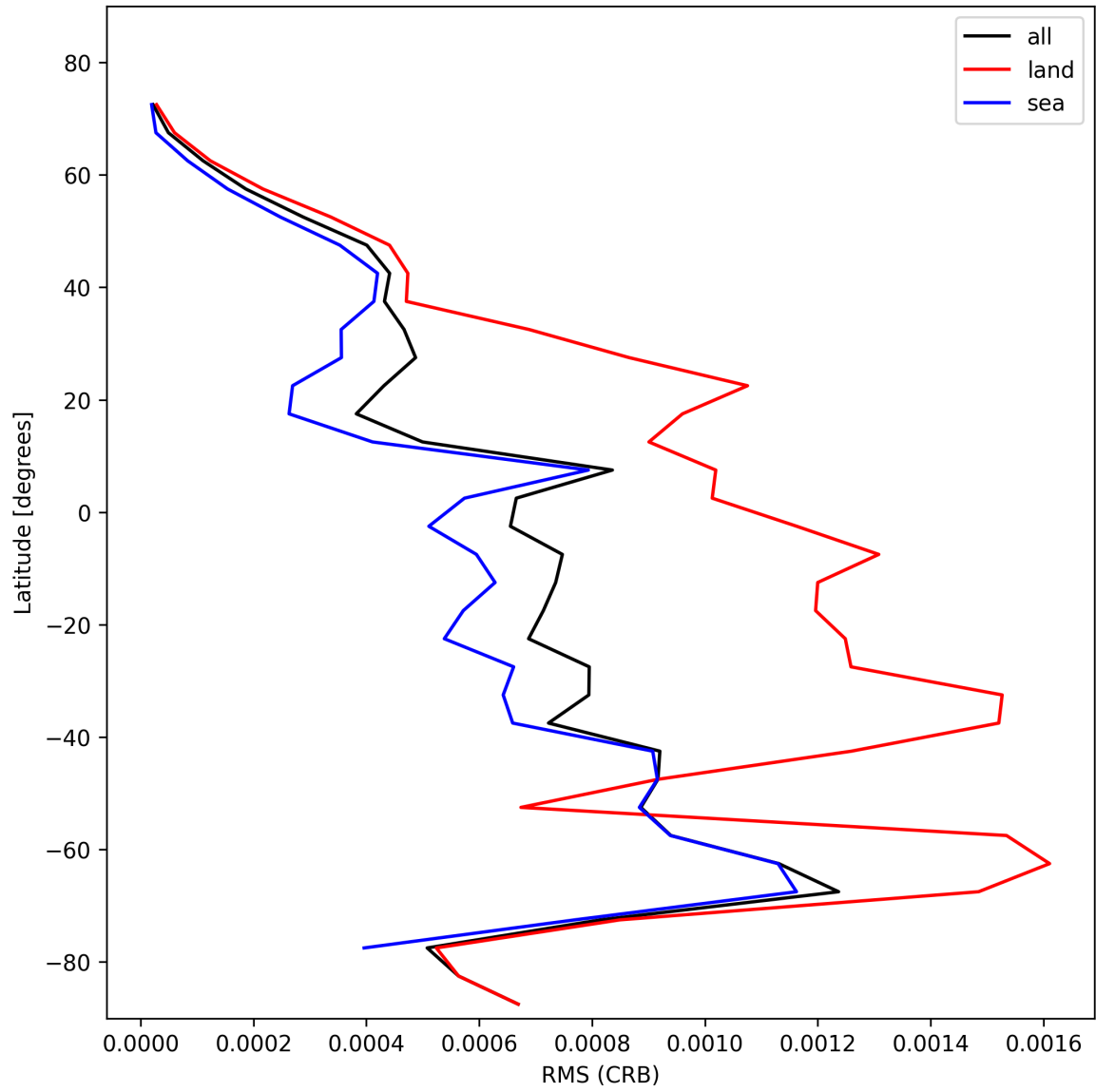
Figure 32: Zonal average of “RMS (CRB)” for 2025-11-07 to 2025-11-08.
