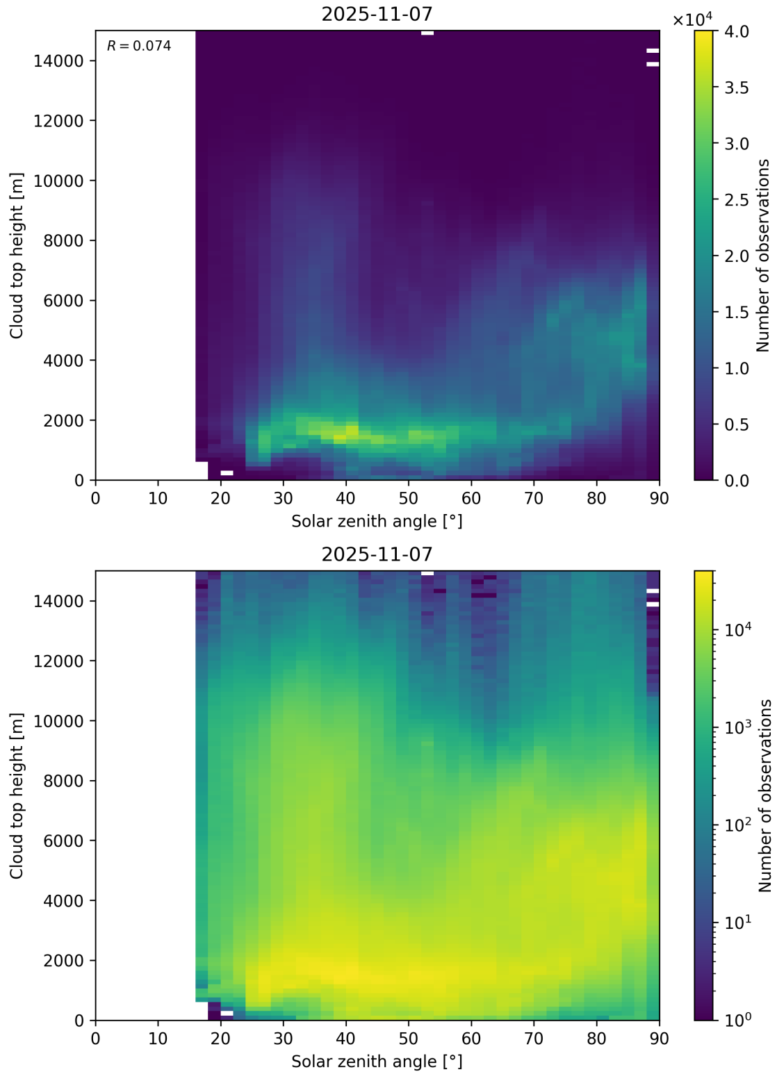
Figure 104: Scatter density plot of “Solar zenith angle” against “Cloud top height” for 2025-11-07 to 2025-11-08.
