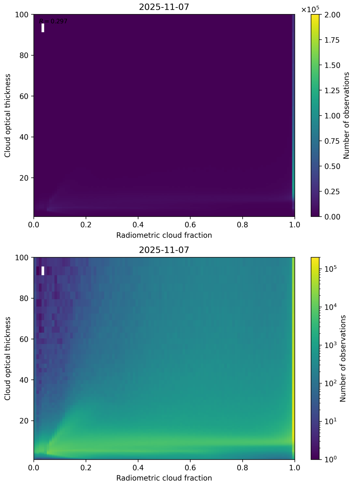
Figure 75: Scatter density plot of “Radiometric cloud fraction” against “Cloud optical thickness” for 2025-11-07 to 2025-11-08.
