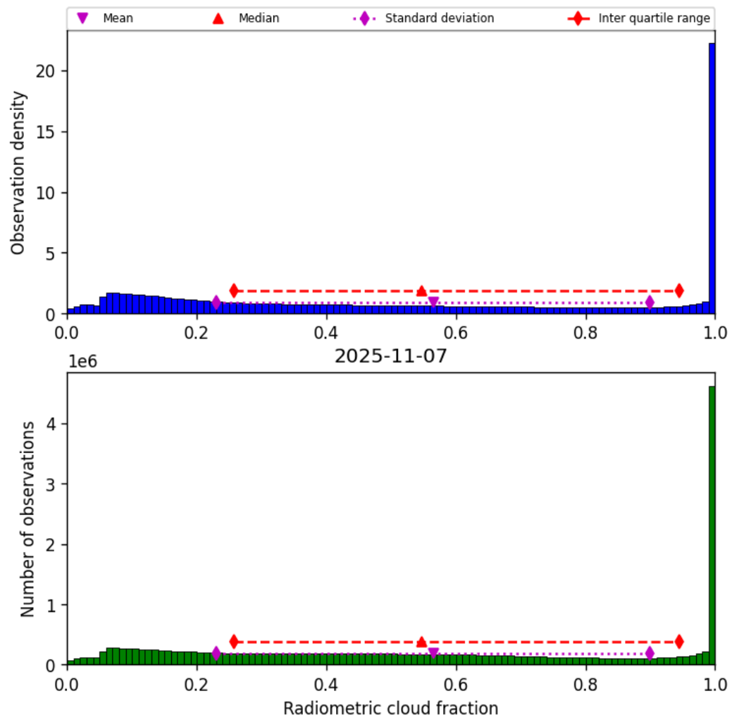
Figure 39: Histogram of “Radiometric cloud fraction” for 2025-11-07 to 2025-11-08
