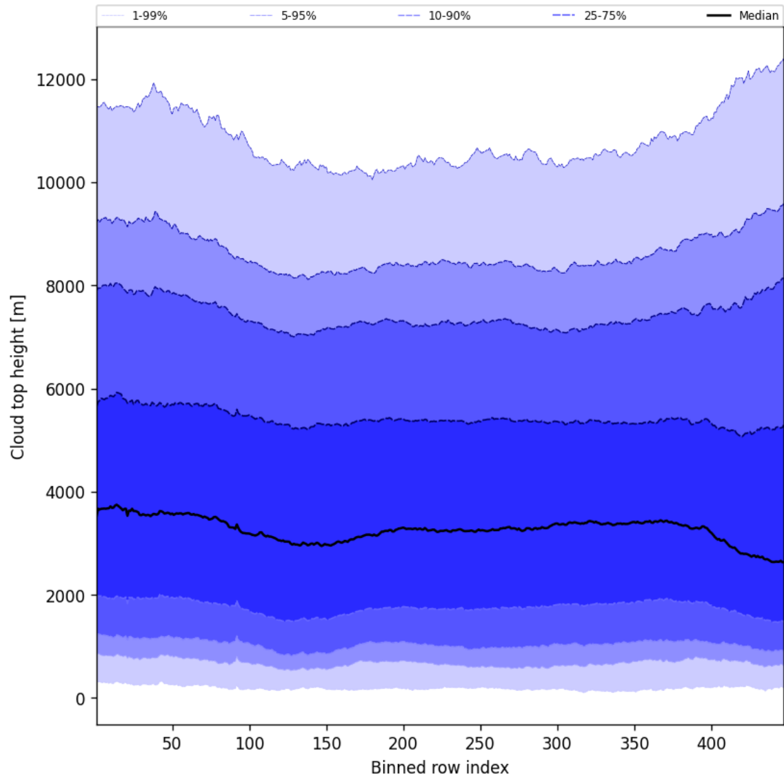
Figure 56: Along track statistics of “Cloud top height” for 2025-11-07 to 2025-11-08
