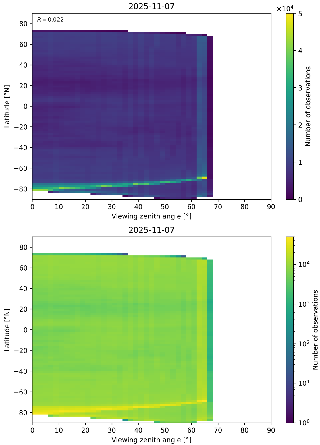
Figure 113: Scatter density plot of “Viewing zenith angle” against “Latitude” for 2025-11-07 to 2025-11-08.
