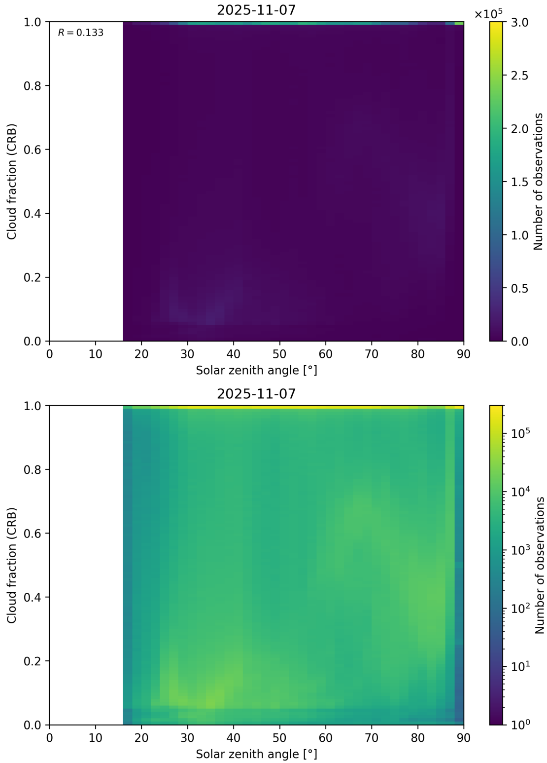
Figure 101: Scatter density plot of “Solar zenith angle” against “Cloud fraction (CRB)” for 2025-11-07 to 2025-11-08.
