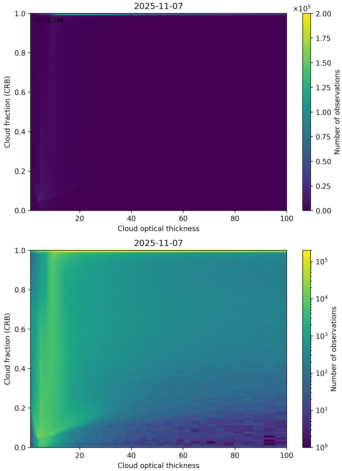
Figure 84: Scatter density plot of “Cloud optical thickness” against “Cloud fraction (CRB)” for 2025-11-07 to 2025-11-08.
