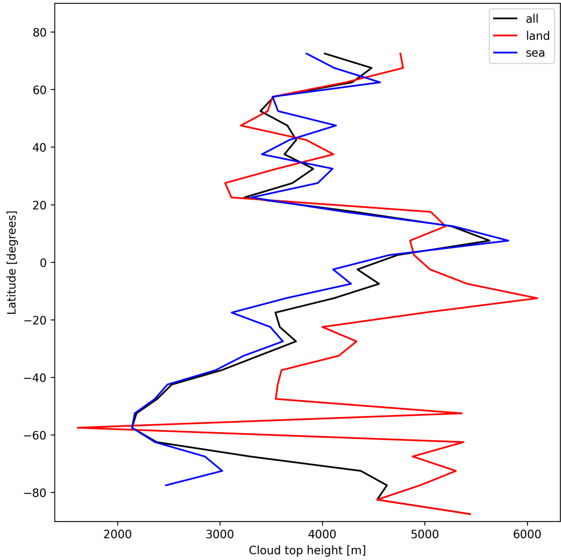
Figure 24: Zonal average of “Cloud top height” for 2025-11-07 to 2025-11-08.
