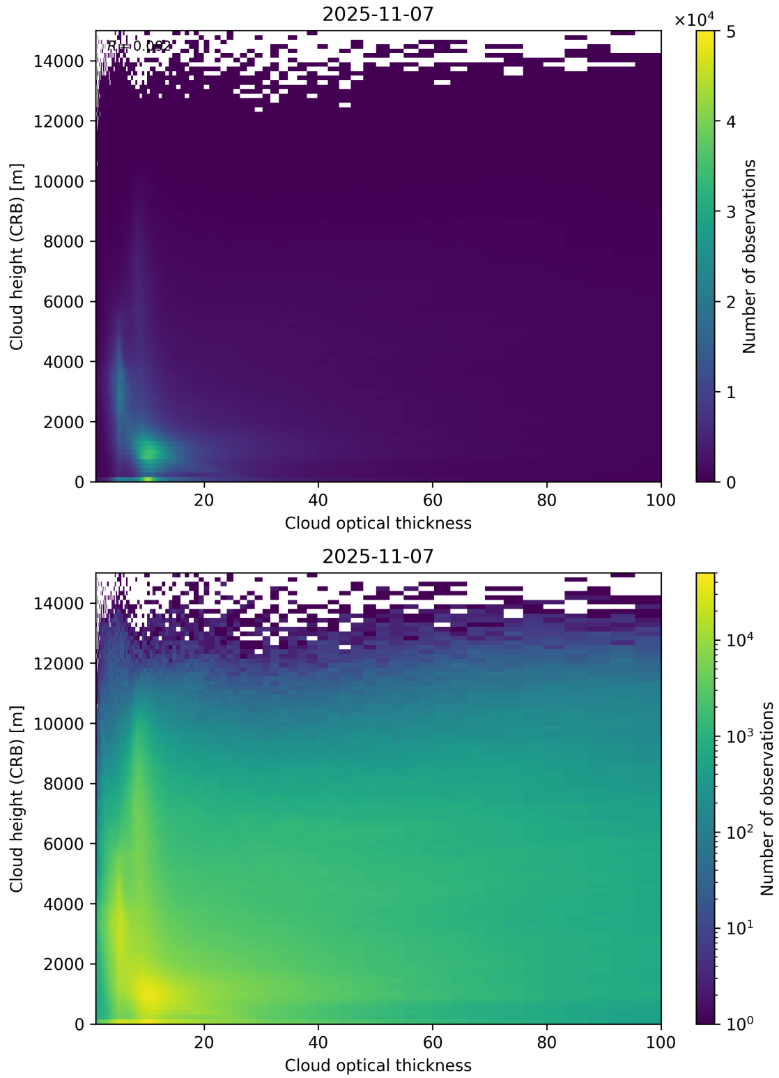
Figure 85: Scatter density plot of “Cloud optical thickness” against “Cloud height (CRB)” for 2025-11-07 to 2025-11-08.
