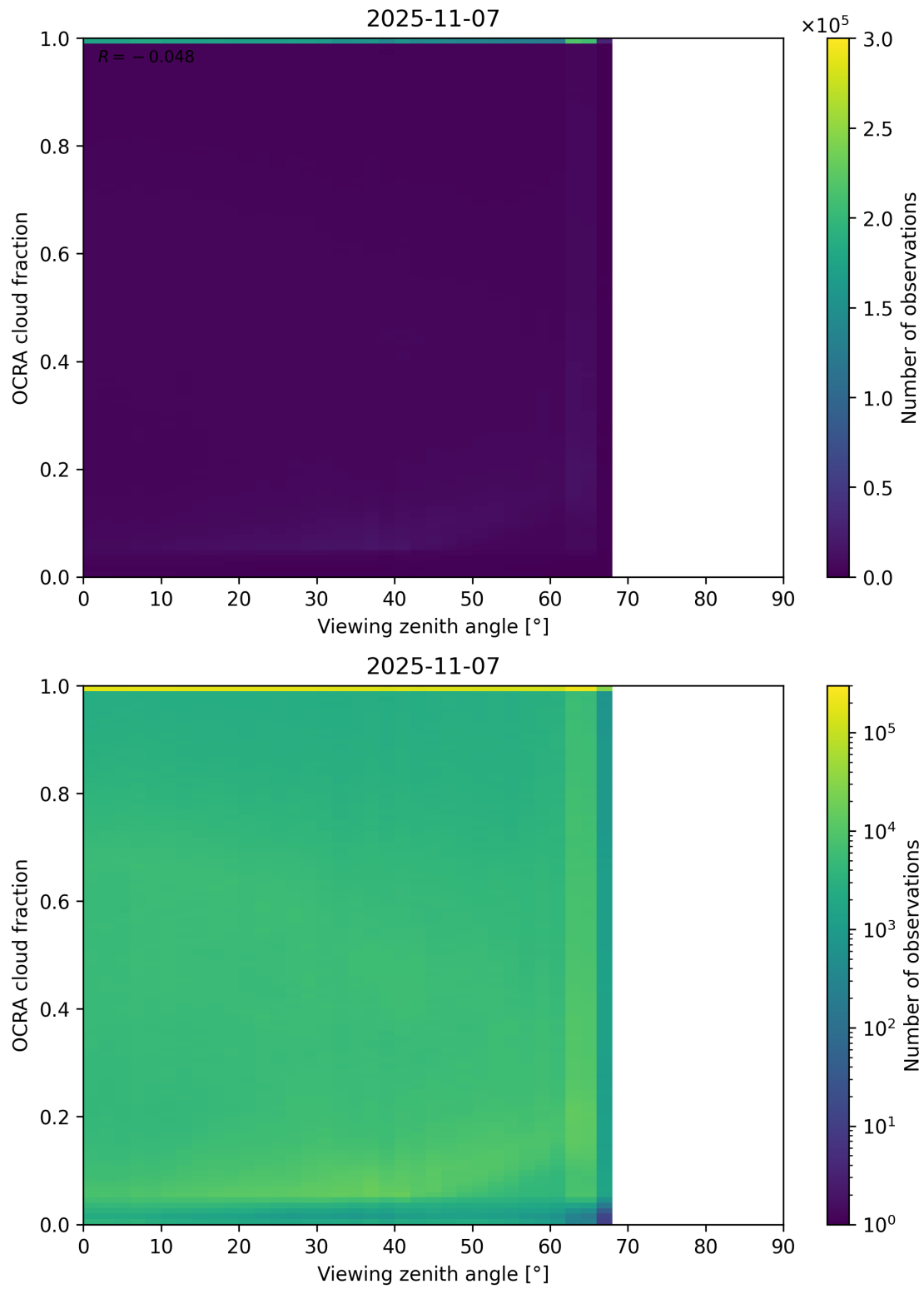
Figure 108: Scatter density plot of “Viewing zenith angle” against “OCRA cloud fraction” for 2025-11-07 to 2025-11-08.
