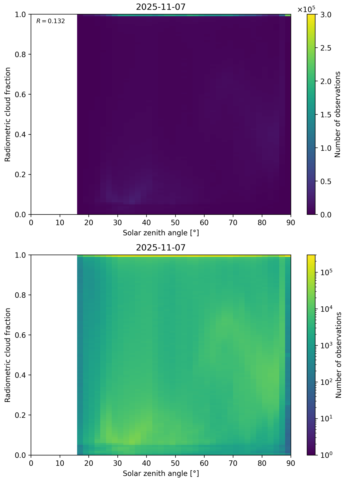
Figure 99: Scatter density plot of “Solar zenith angle” against “Radiometric cloud fraction” for 2025-11-07 to 2025-11-08.
