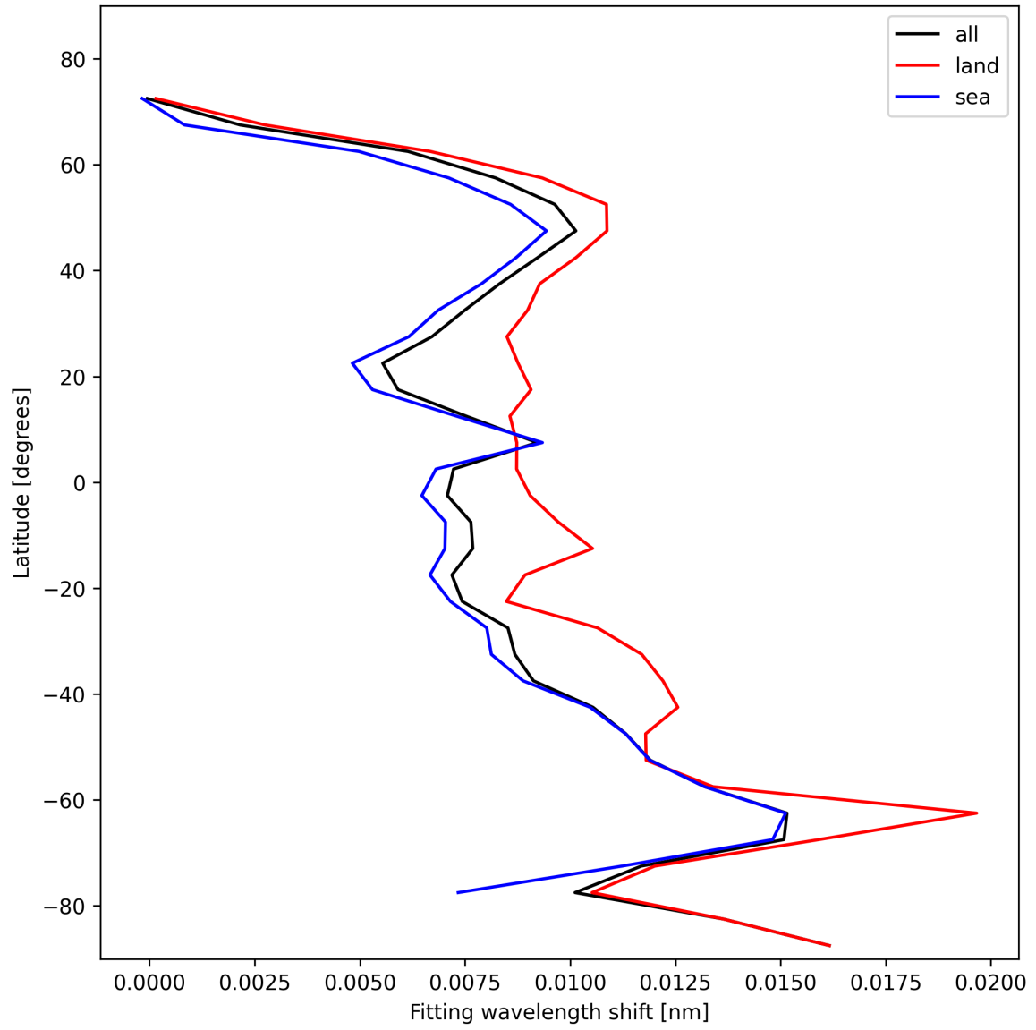
Figure 33: Zonal average of “Fitting wavelength shift” for 2025-11-07 to 2025-11-08.
