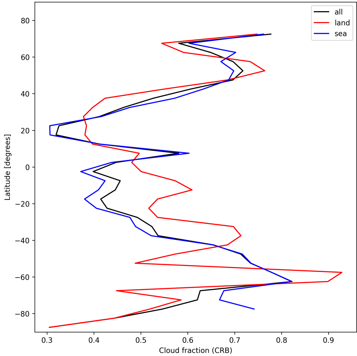
Figure 26: Zonal average of “Cloud fraction (CRB)” for 2025-11-07 to 2025-11-08.
