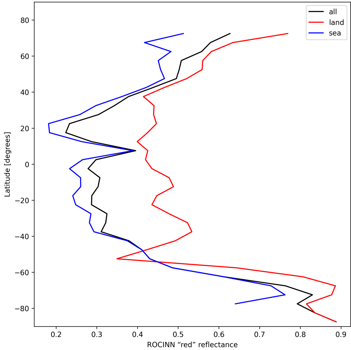
Figure 37: Zonal average of “ROCINN “red” reflectance” for 2025-11-07 to 2025-11-08.
