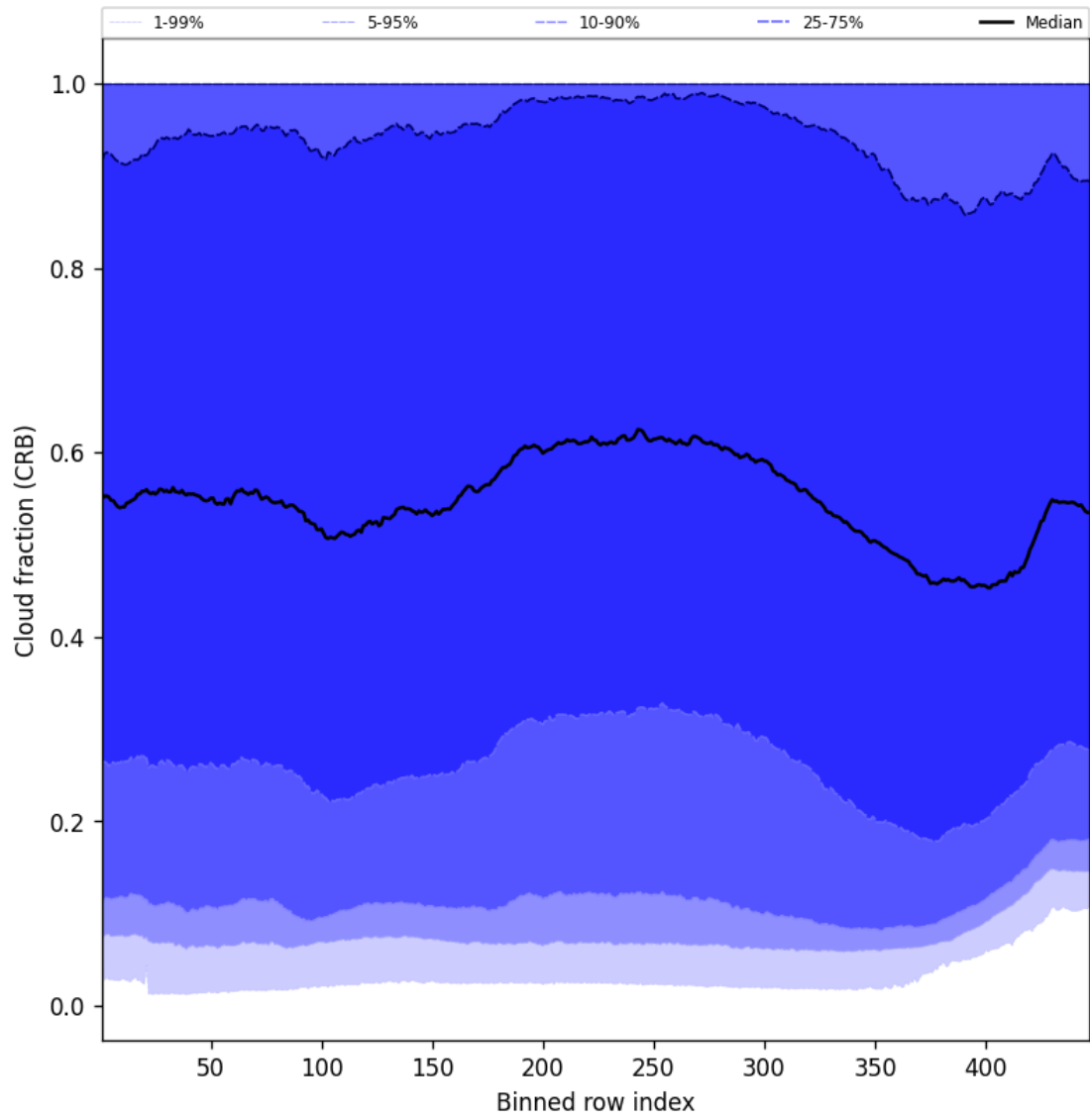
Figure 58: Along track statistics of “Cloud fraction (CRB)” for 2025-11-07 to 2025-11-08
