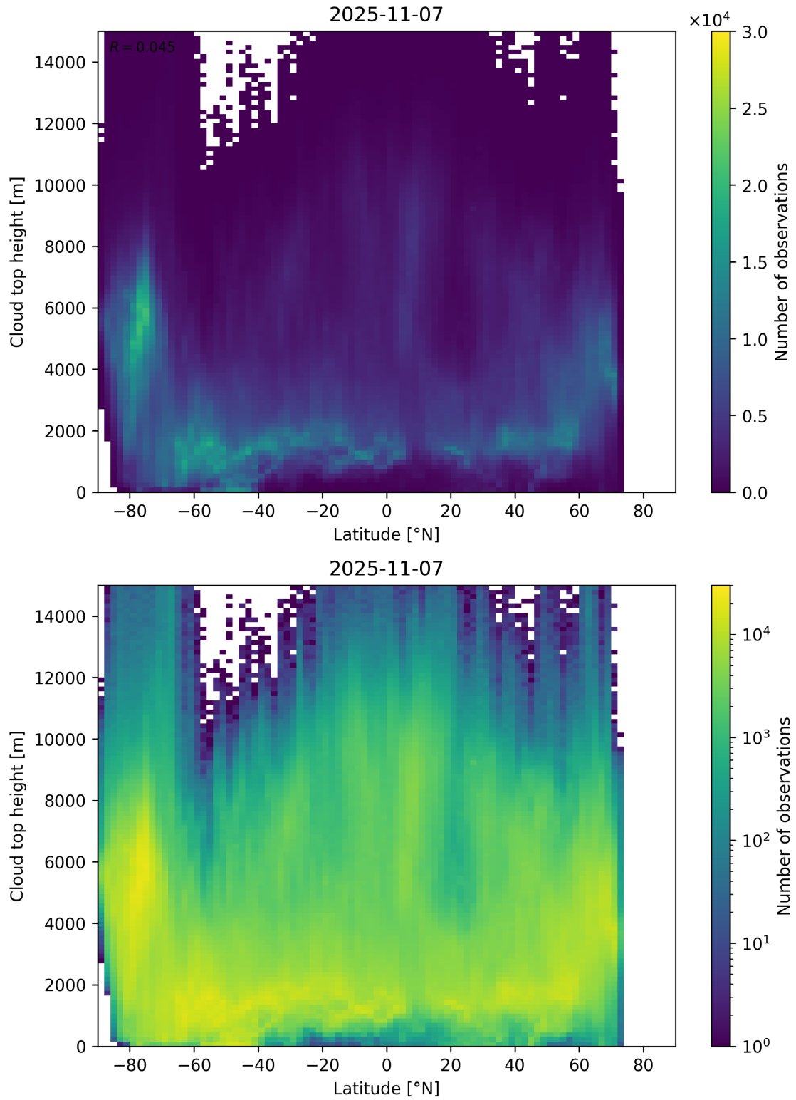
Figure 97: Scatter density plot of “Latitude” against “Cloud top height” for 2025-11-07 to 2025-11-08.
