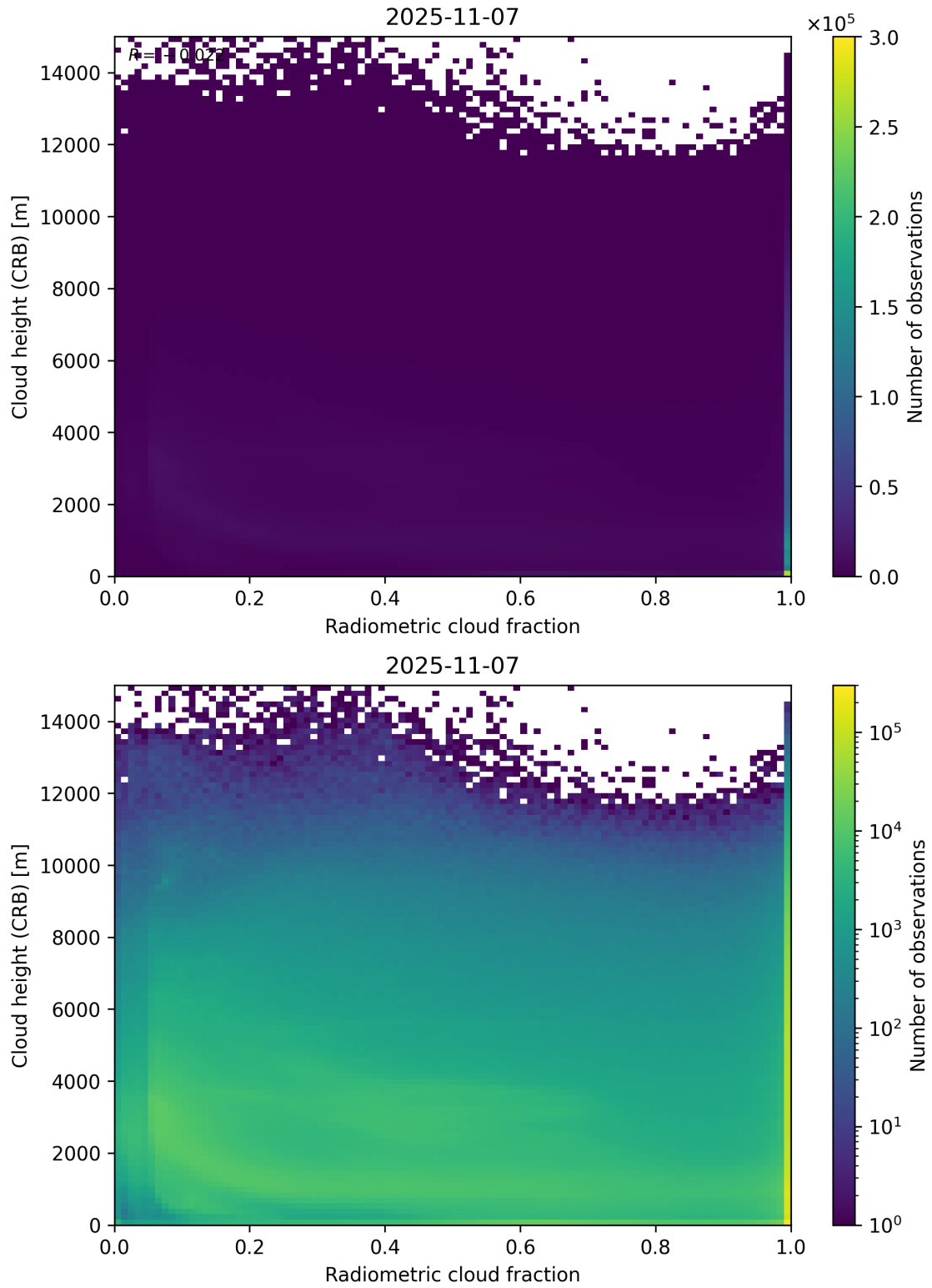
Figure 74: Scatter density plot of “Radiometric cloud fraction” against “Cloud height (CRB)” for 2025-11-07 to 2025-11-08.
