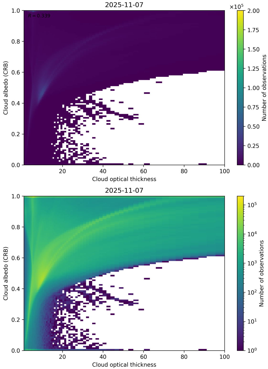
Figure 82: Scatter density plot of “Cloud optical thickness” against “Cloud albedo (CRB)” for 2025-11-07 to 2025-11-08.
