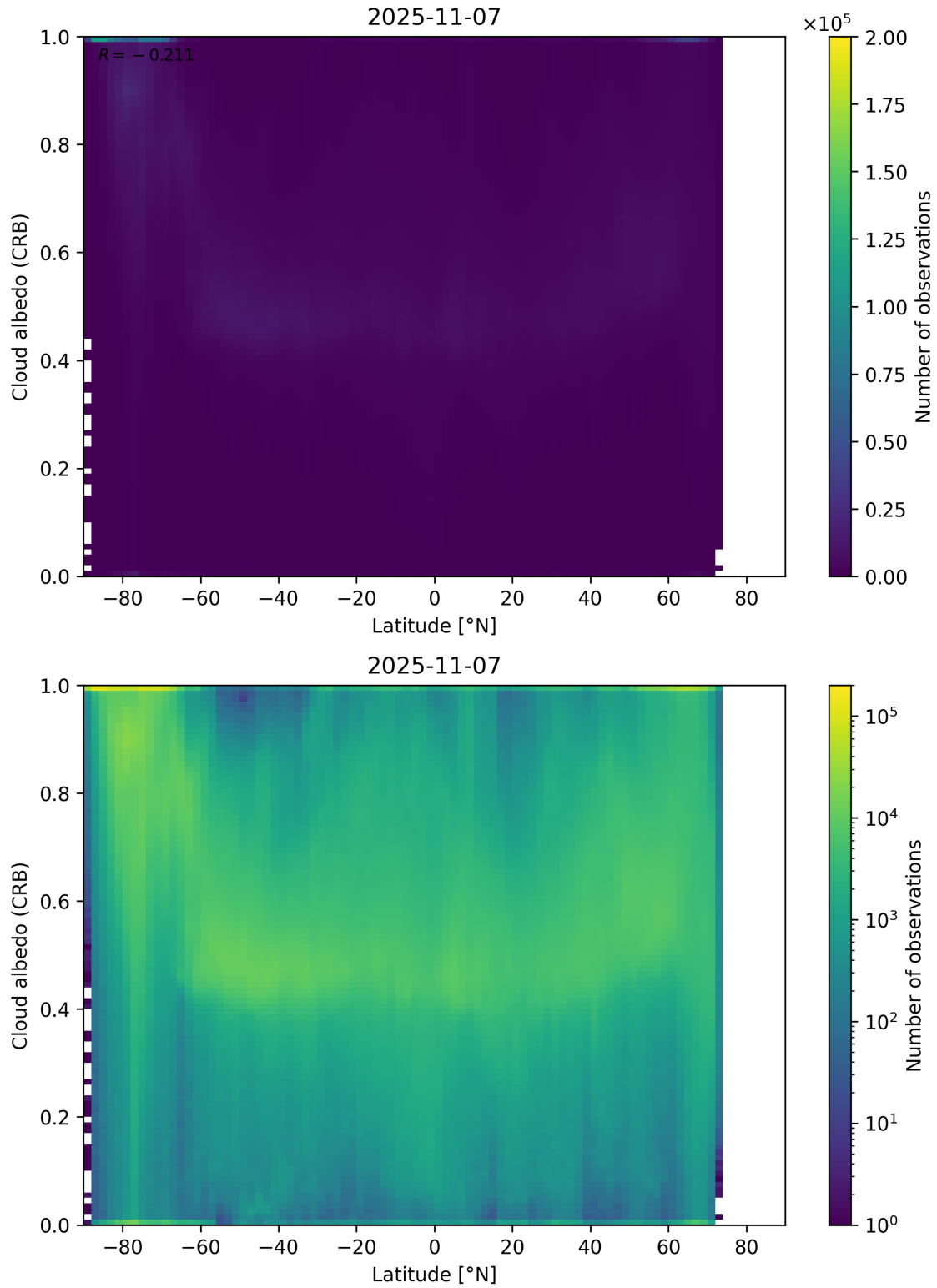
Figure 91: Scatter density plot of “Latitude” against “Cloud albedo (CRB)” for 2025-11-07 to 2025-11-08.
