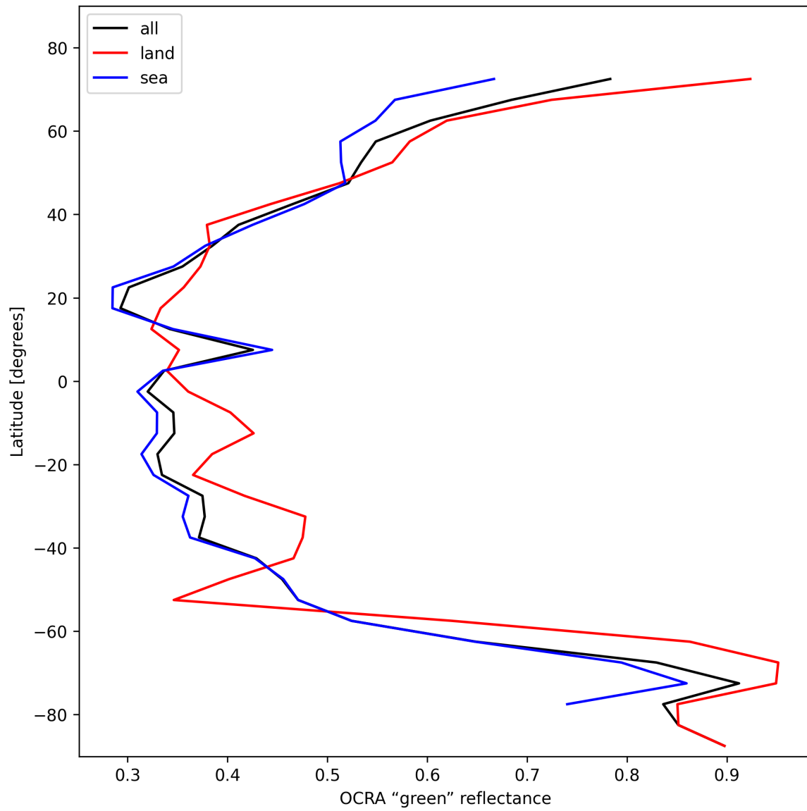
Figure 36: Zonal average of “OCRA “green” reflectance” for 2025-11-07 to 2025-11-08.
