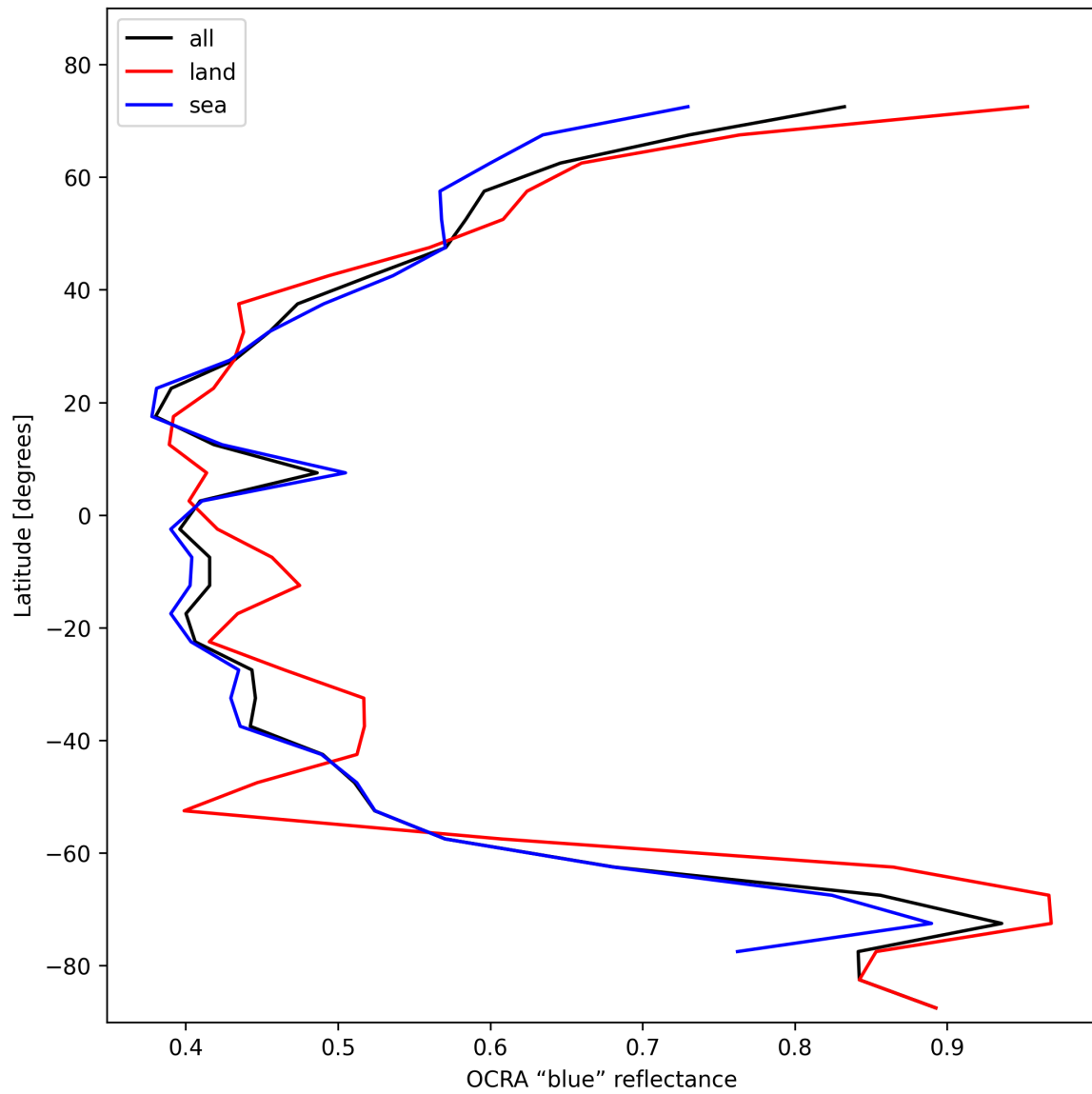
Figure 35: Zonal average of “OCRA “blue” reflectance” for 2025-11-07 to 2025-11-08.
