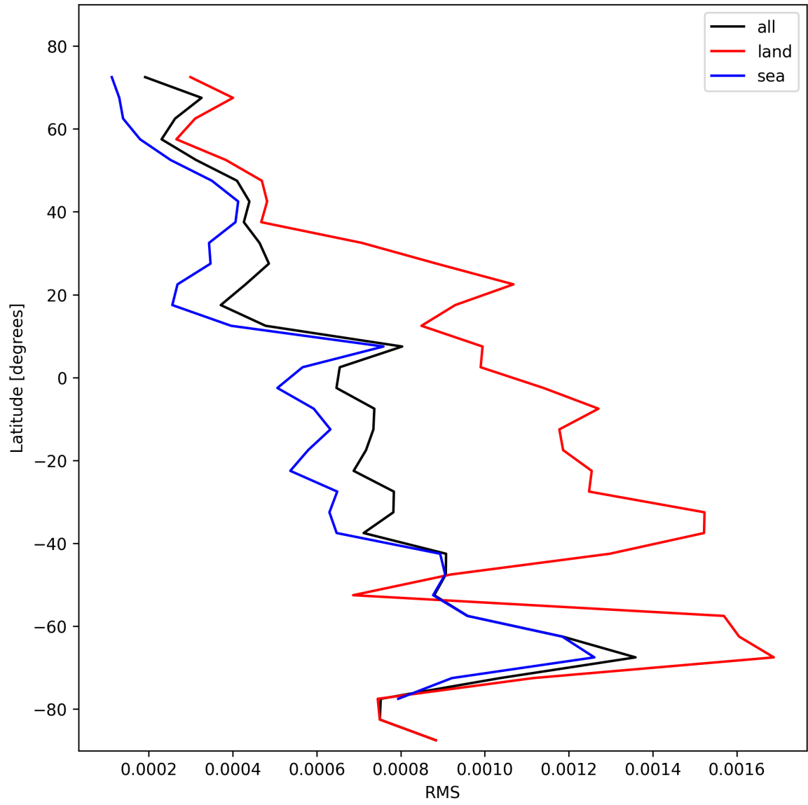
Figure 31: Zonal average of “RMS” for 2025-11-07 to 2025-11-08.
