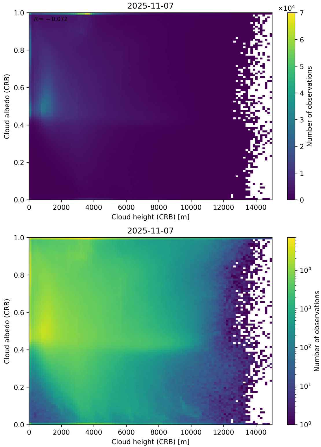
Figure 80: Scatter density plot of “Cloud height (CRB)” against “Cloud albedo (CRB)” for 2025-11-07 to 2025-11-08.
