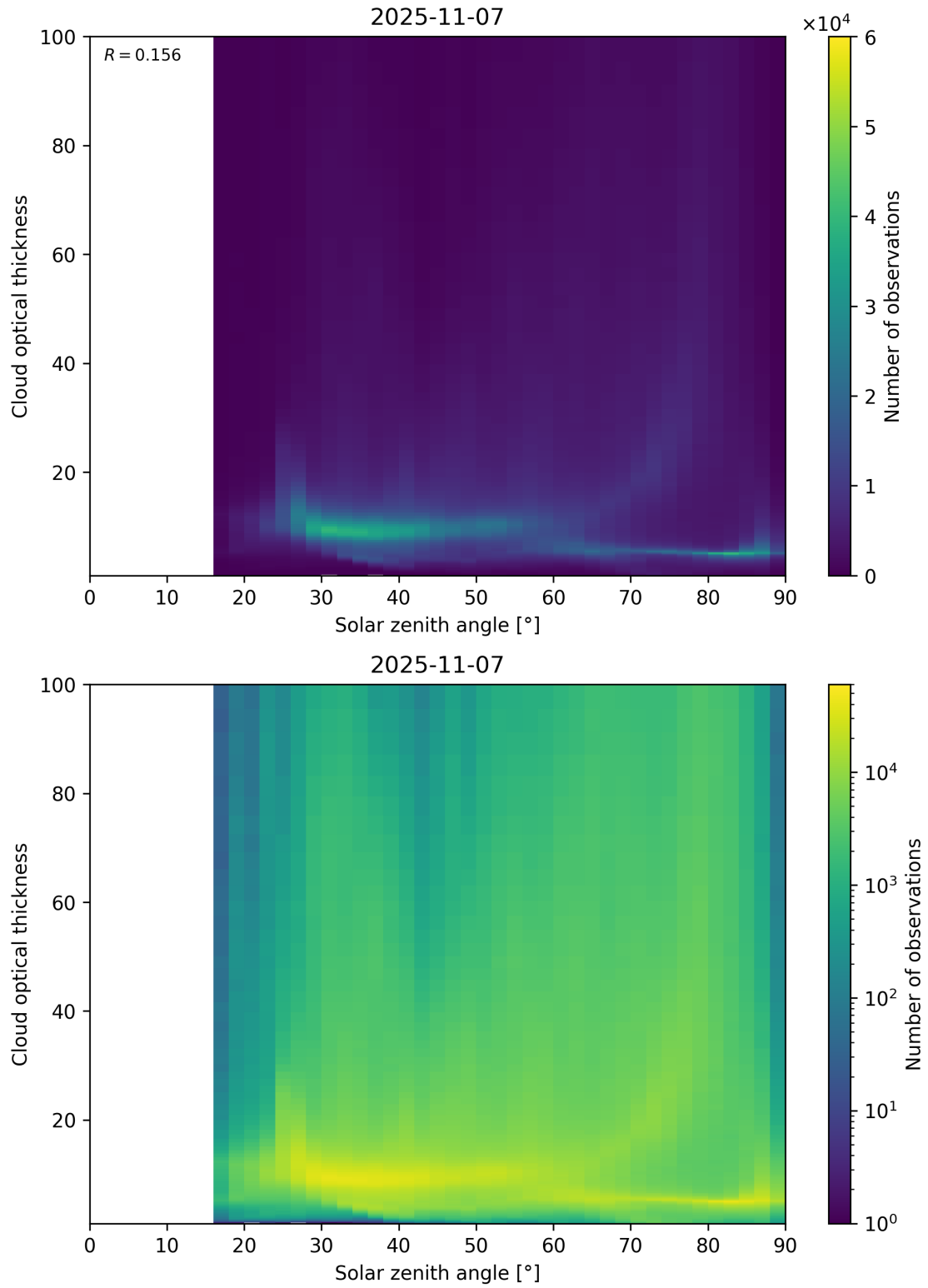
Figure 103: Scatter density plot of “Solar zenith angle” against “Cloud optical thickness” for 2025-11-07 to 2025-11-08.
