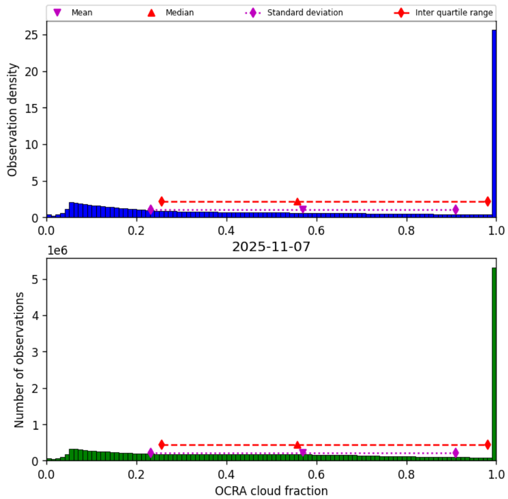
Figure 50: Histogram of “OCRA cloud fraction” for 2025-11-07 to 2025-11-08
