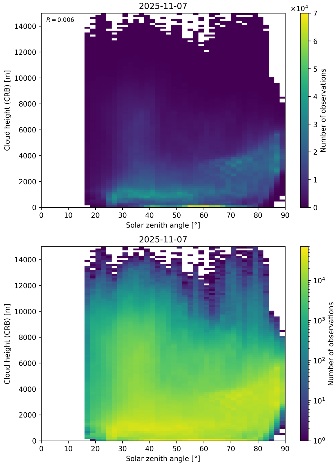
Figure 102: Scatter density plot of “Solar zenith angle” against “Cloud height (CRB)” for 2025-11-07 to 2025-11-08.
