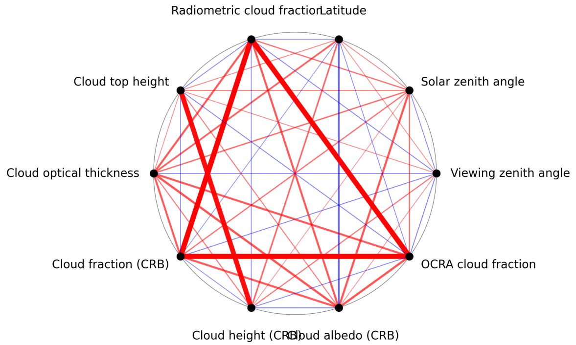
Figure 1: Map of correlation graph for 2025-11-07 to 2025-11-08.
