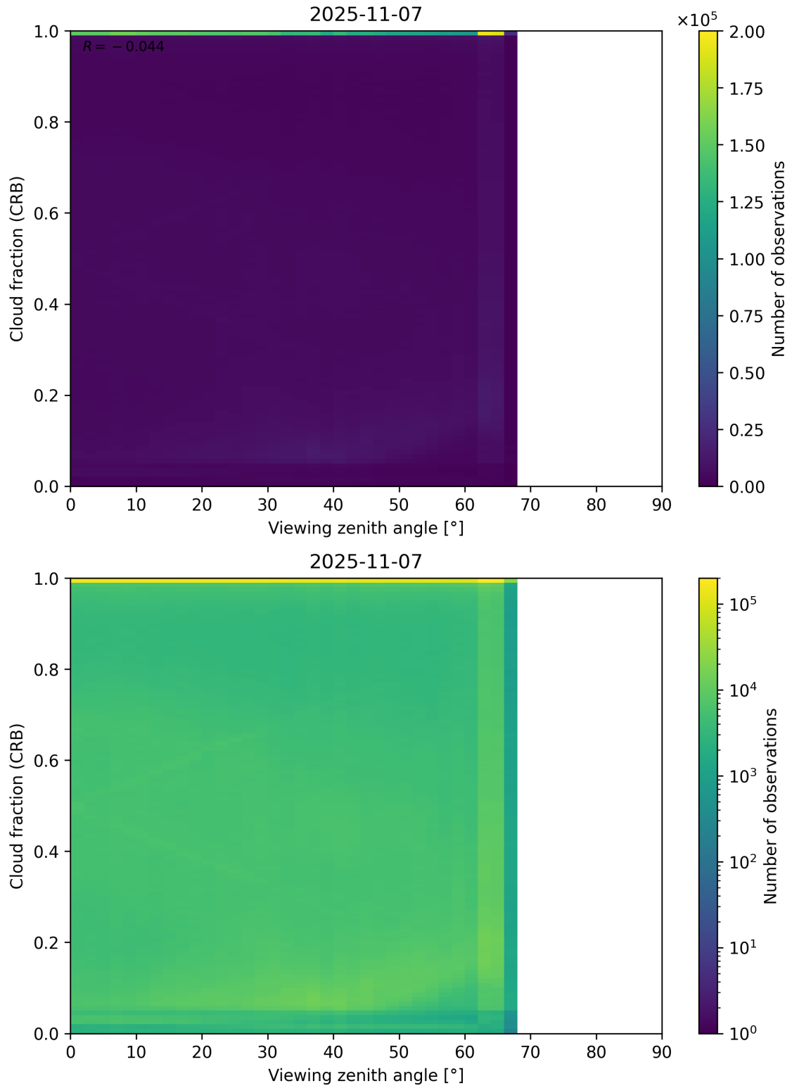
Figure 109: Scatter density plot of “Viewing zenith angle” against “Cloud fraction (CRB)” for 2025-11-07 to 2025-11-08.
