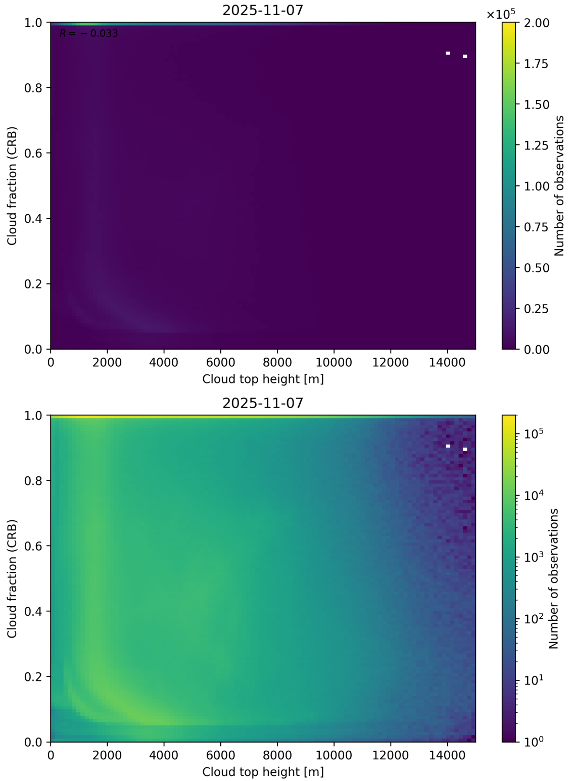
Figure 88: Scatter density plot of “Cloud top height” against “Cloud fraction (CRB)” for 2025-11-07 to 2025-11-08.
