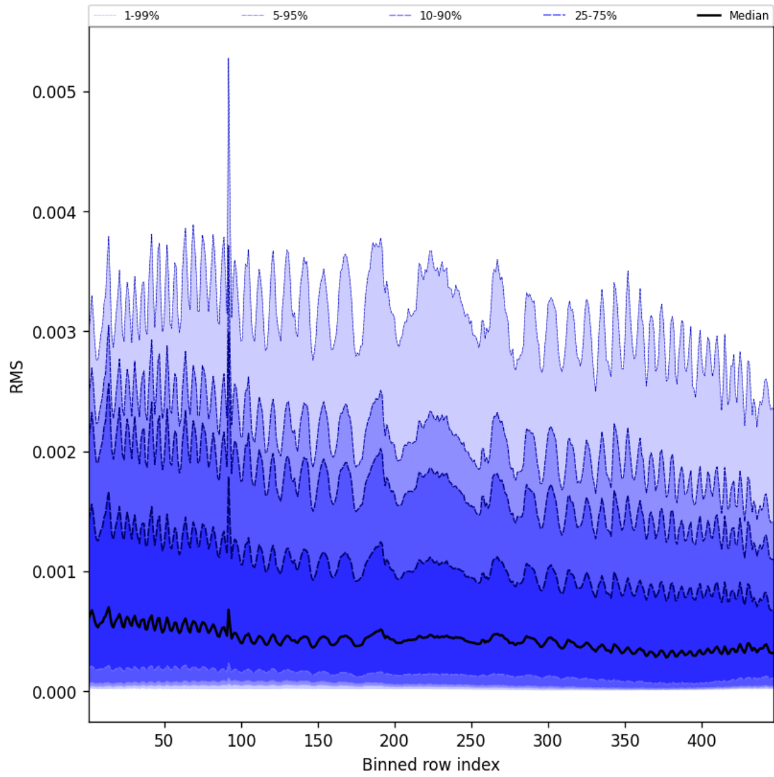
Figure 63: Along track statistics of “RMS” for 2025-11-07 to 2025-11-08
