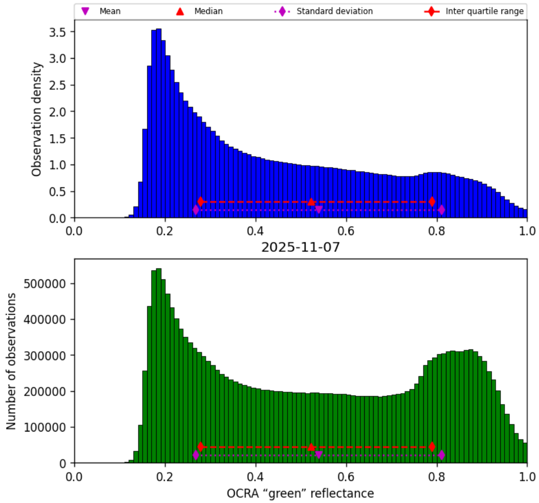
Figure 52: Histogram of “OCRA “green” reflectance” for 2025-11-07 to 2025-11-08
