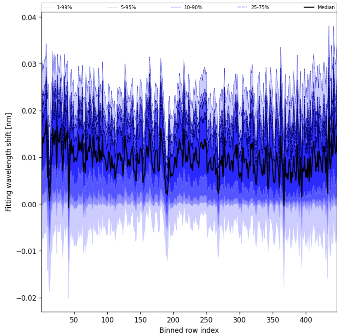
Figure 65: Along track statistics of “Fitting wavelength shift” for 2025-11-07 to 2025-11-08
