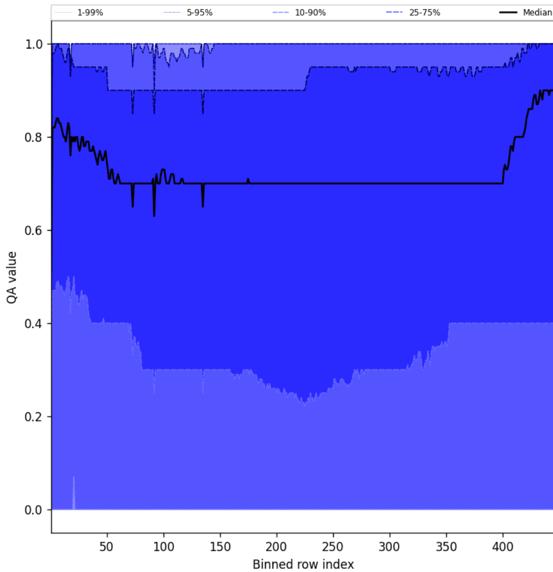
Figure 54: Along track statistics of “QA value” for 2025-11-07 to 2025-11-08
