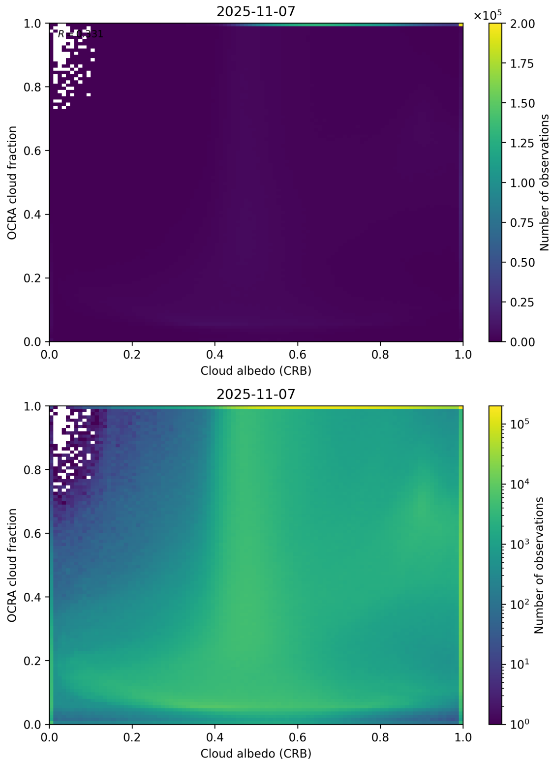
Figure 70: Scatter density plot of “Cloud albedo (CRB)” against “OCRA cloud fraction” for 2025-11-07 to 2025-11-08.
