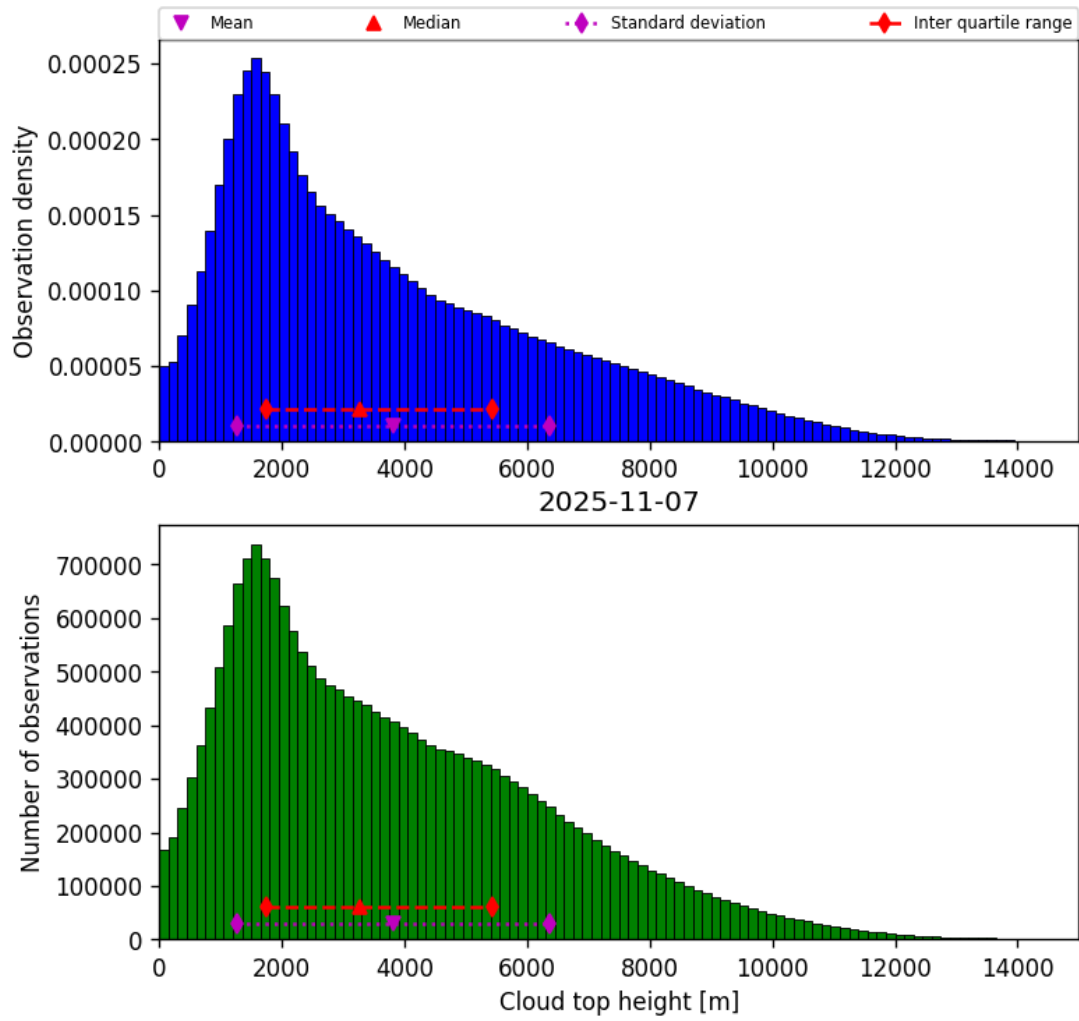
Figure 40: Histogram of “Cloud top height” for 2025-11-07 to 2025-11-08
