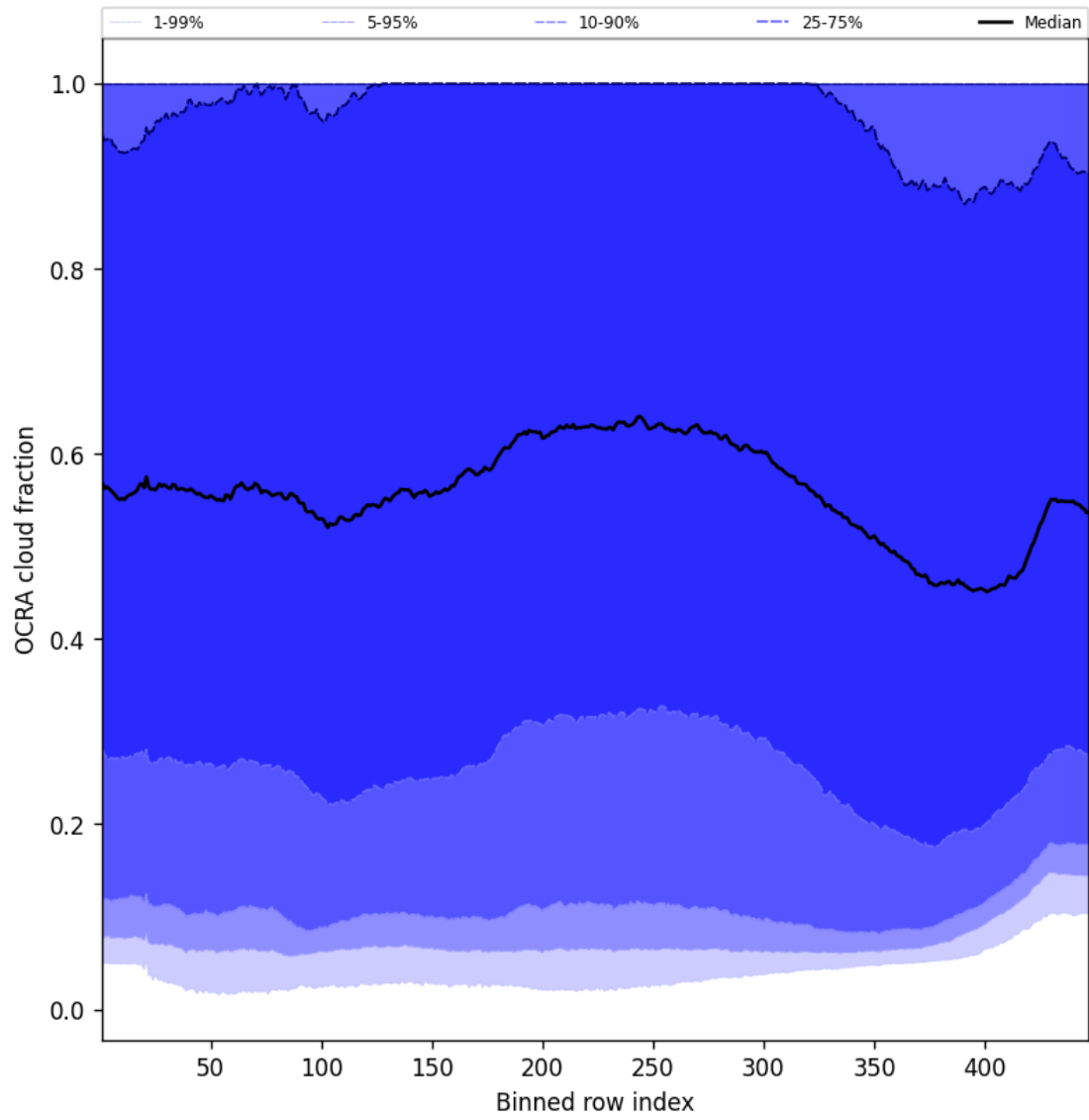
Figure 66: Along track statistics of “OCRA cloud fraction” for 2025-11-07 to 2025-11-08
