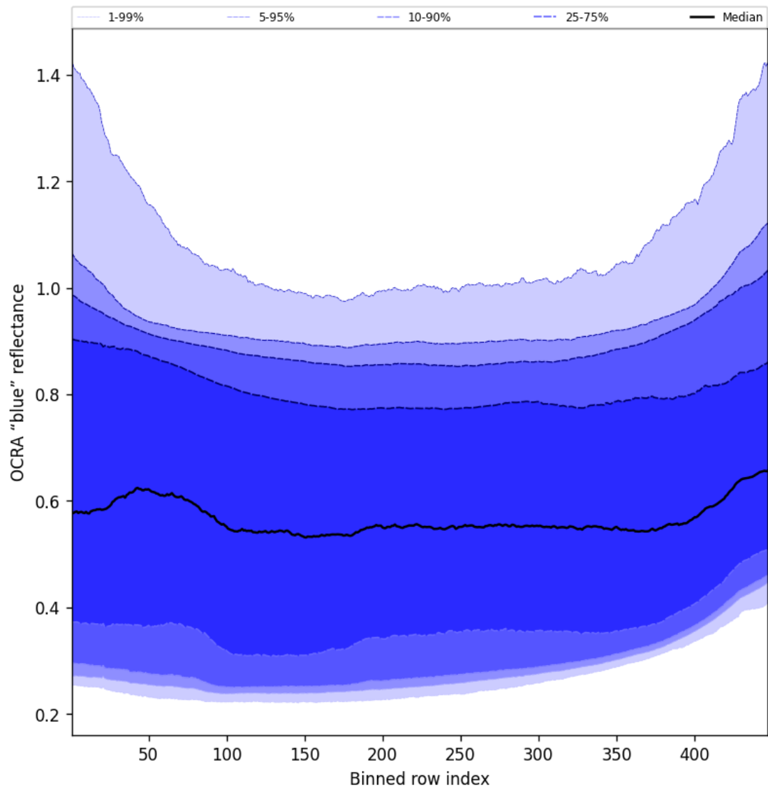
Figure 67: Along track statistics of “OCRA “blue” reflectance” for 2025-11-07 to 2025-11-08
