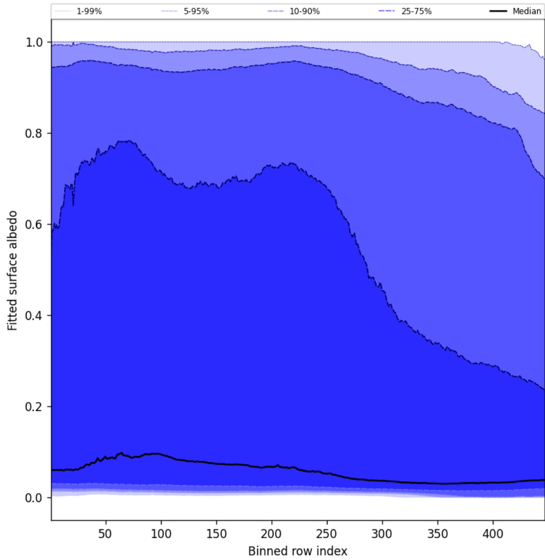
Figure 61: Along track statistics of “Fitted surface albedo” for 2025-11-07 to 2025-11-08
