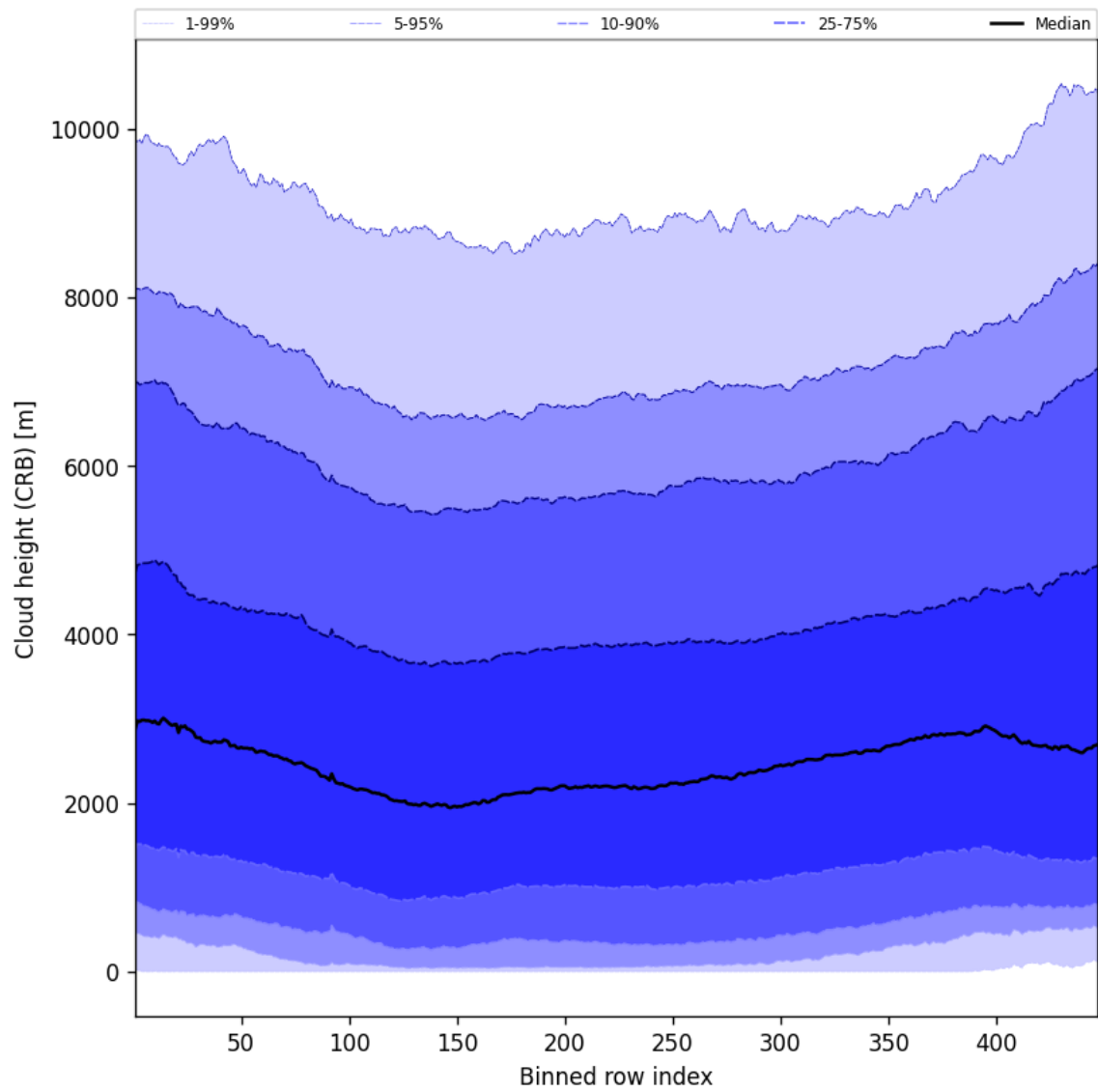
Figure 59: Along track statistics of “Cloud height (CRB)” for 2025-11-07 to 2025-11-08
