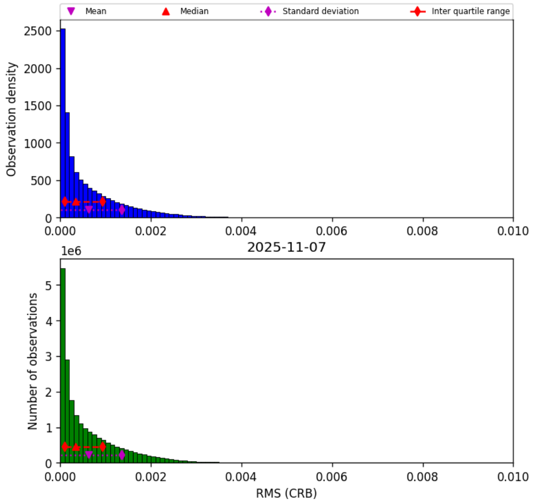
Figure 48: Histogram of “RMS (CRB)” for 2025-11-07 to 2025-11-08
