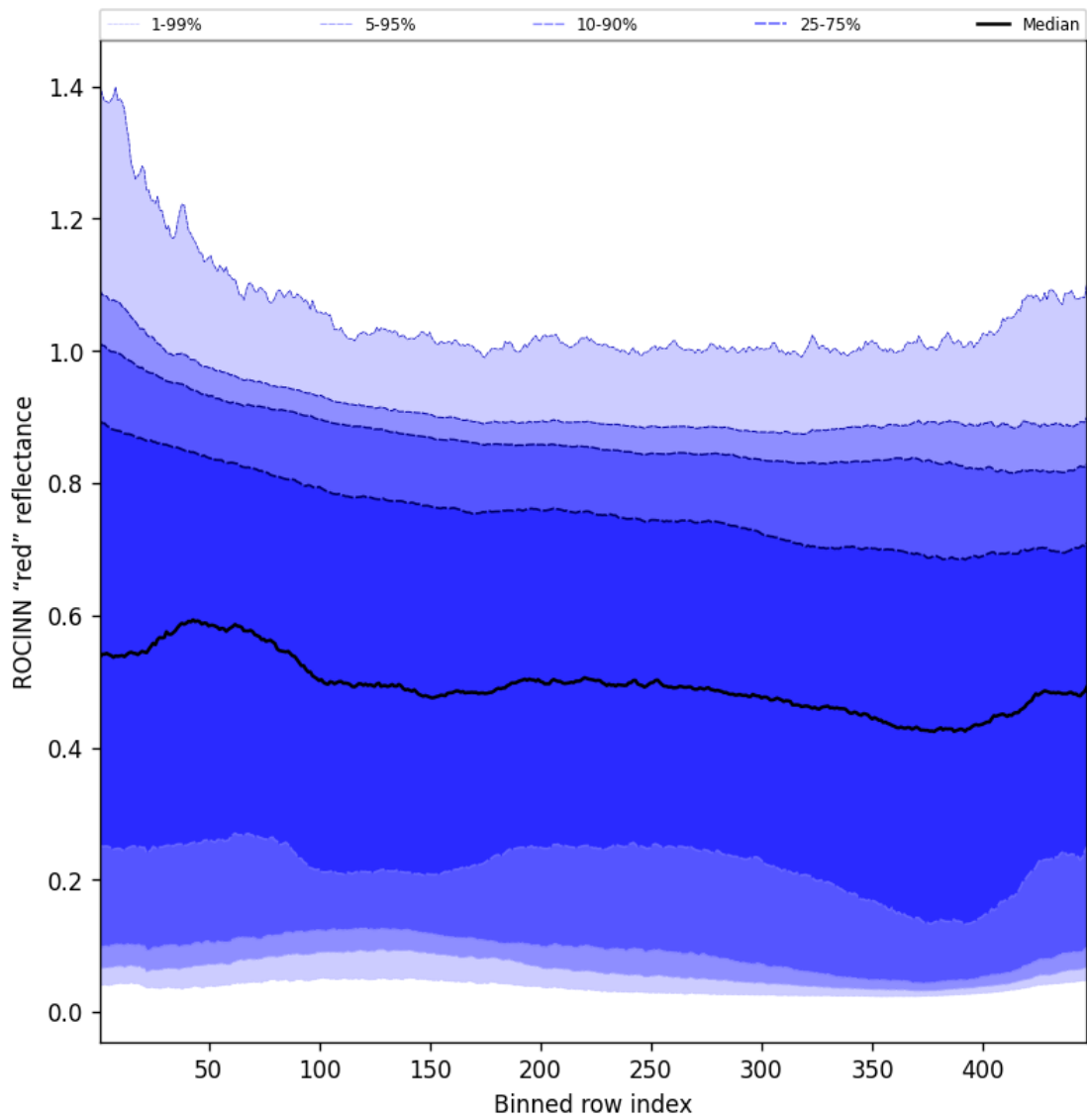
Figure 69: Along track statistics of “ROCINN “red” reflectance” for 2025-11-07 to 2025-11-08
