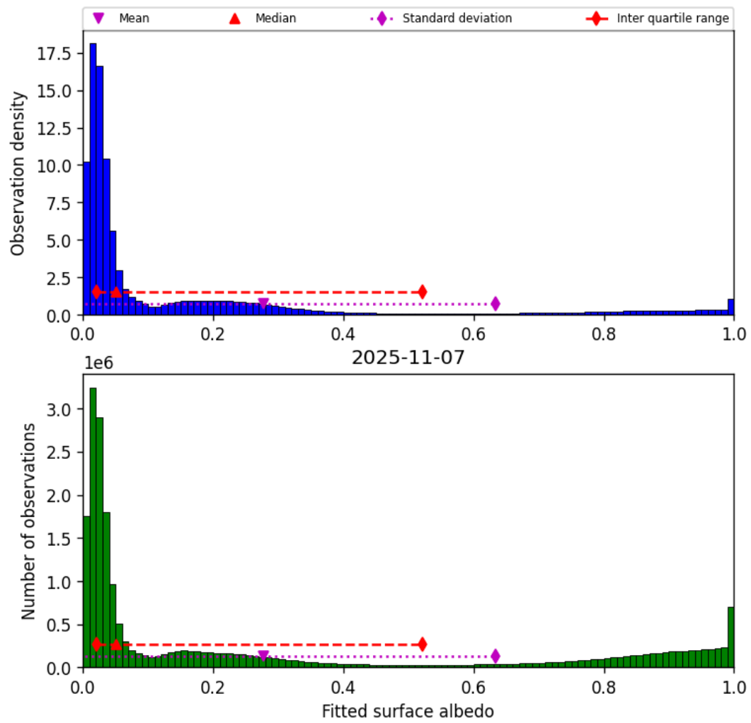
Figure 45: Histogram of “Fitted surface albedo” for 2025-11-07 to 2025-11-08
