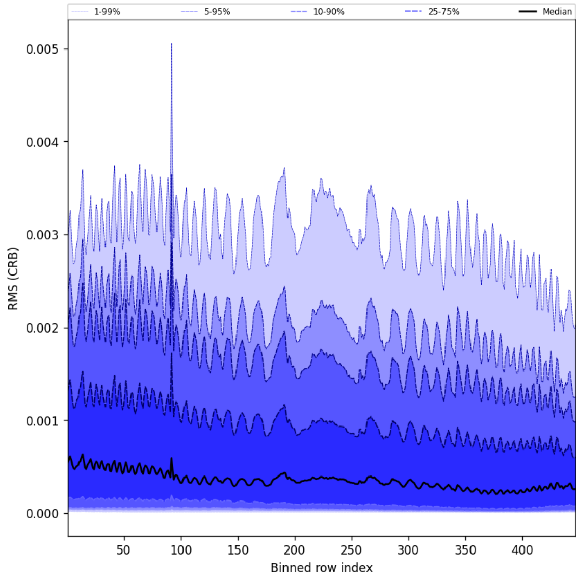
Figure 64: Along track statistics of “RMS (CRB)” for 2025-11-07 to 2025-11-08
