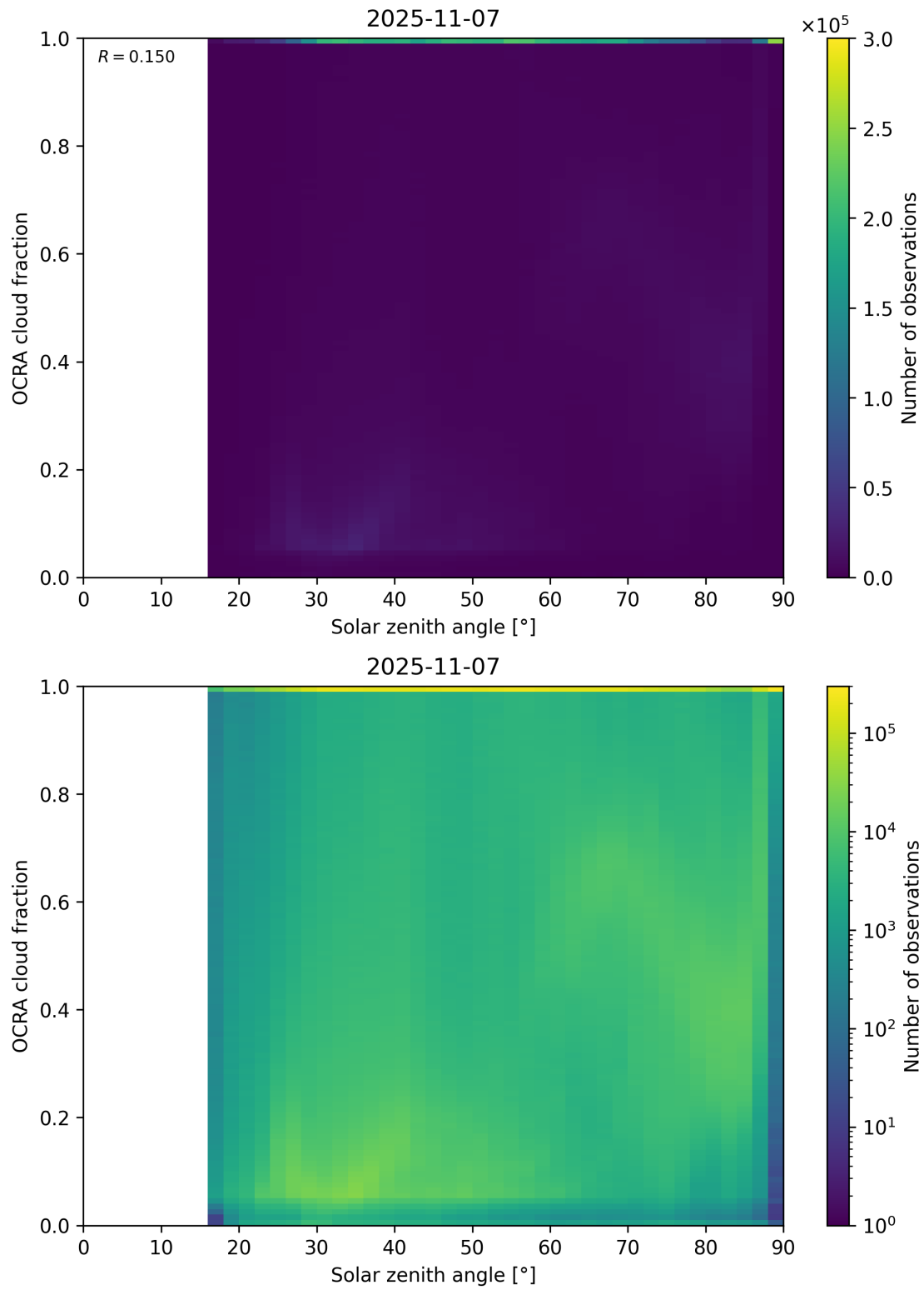
Figure 100: Scatter density plot of “Solar zenith angle” against “OCRA cloud fraction” for 2025-11-07 to 2025-11-08.
