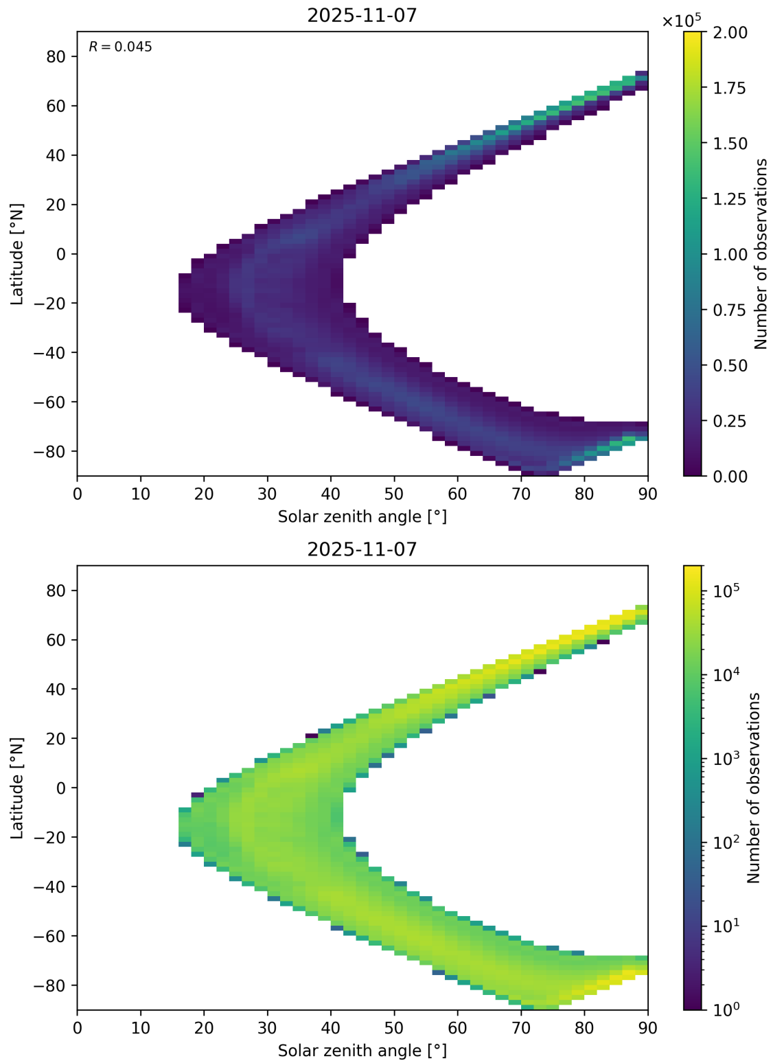
Figure 105: Scatter density plot of “Solar zenith angle” against “Latitude” for 2025-11-07 to 2025-11-08.
