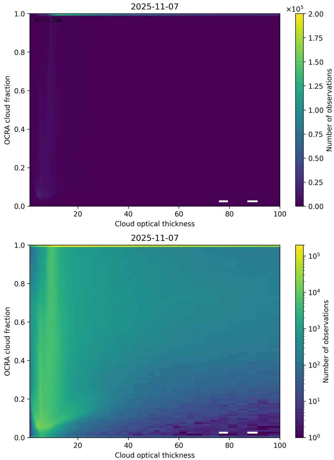
Figure 83: Scatter density plot of “Cloud optical thickness” against “OCRA cloud fraction” for 2025-11-07 to 2025-11-08.
