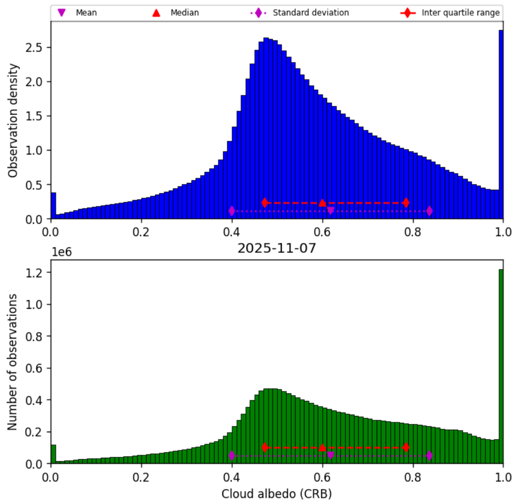
Figure 44: Histogram of “Cloud albedo (CRB)” for 2025-11-07 to 2025-11-08
