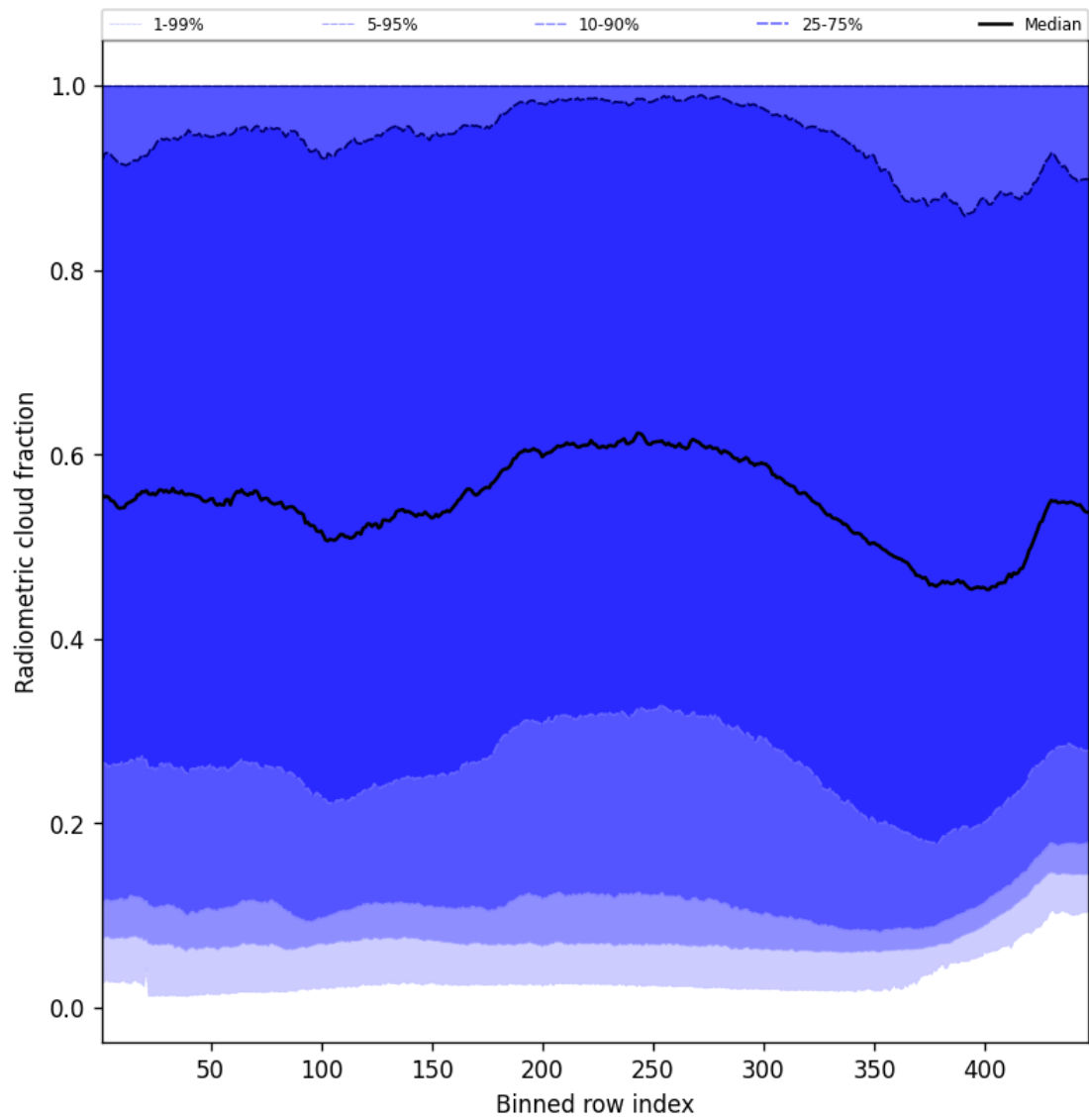
Figure 55: Along track statistics of “Radiometric cloud fraction” for 2025-11-07 to 2025-11-08
