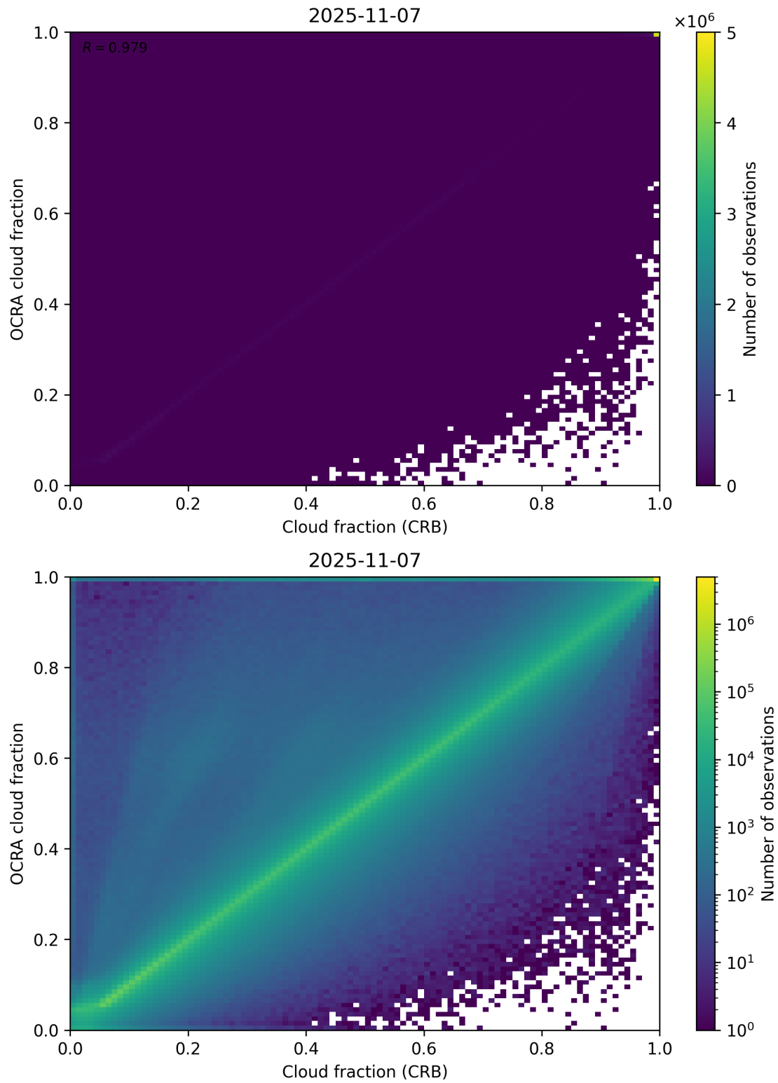
Figure 78: Scatter density plot of “Cloud fraction (CRB)” against “OCRA cloud fraction” for 2025-11-07 to 2025-11-08.
