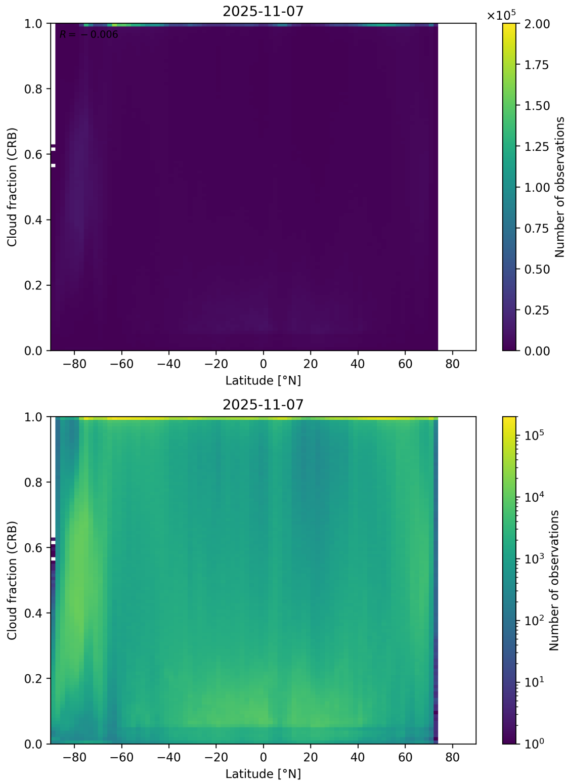
Figure 94: Scatter density plot of “Latitude” against “Cloud fraction (CRB)” for 2025-11-07 to 2025-11-08.
