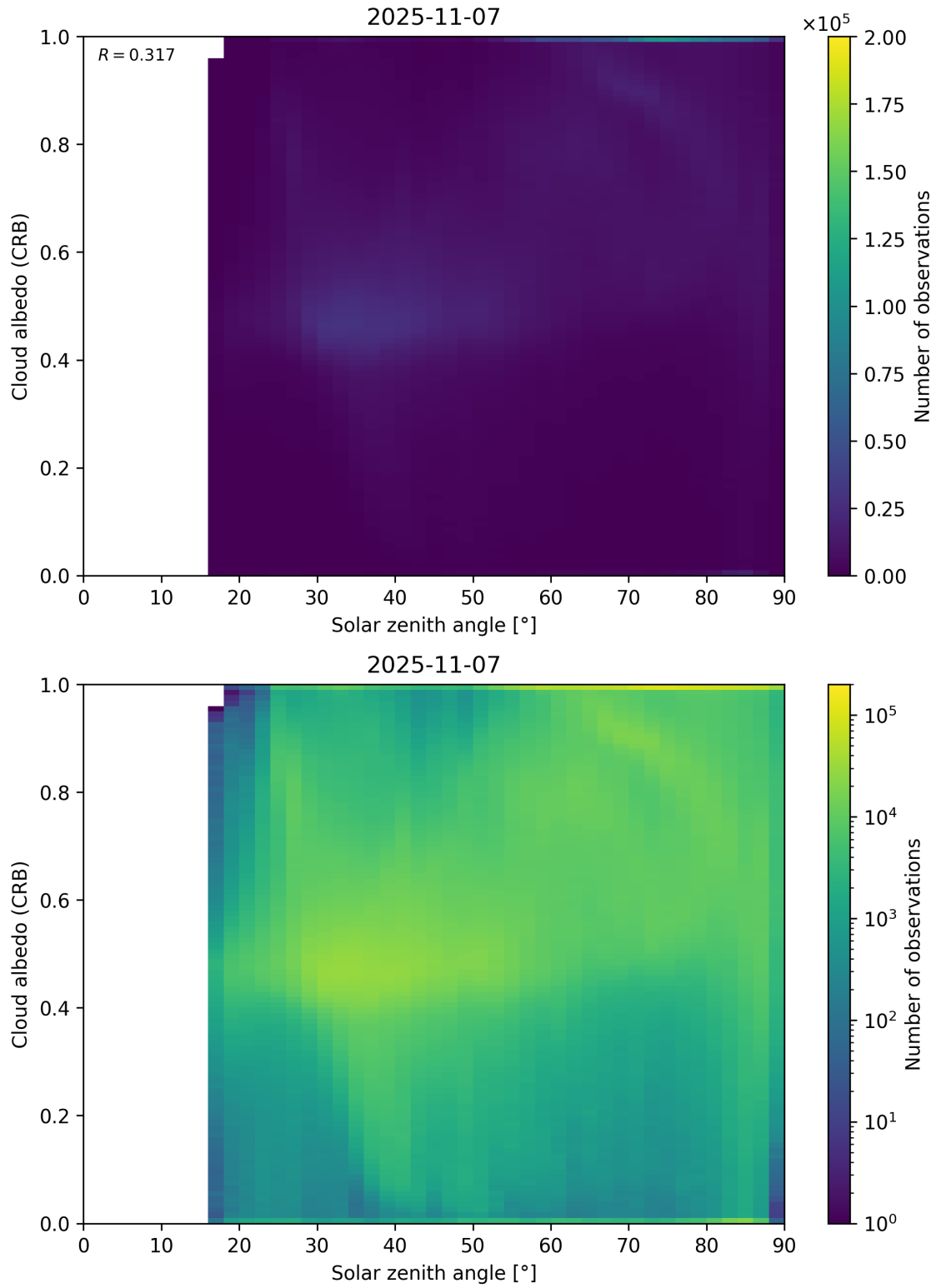
Figure 98: Scatter density plot of “Solar zenith angle” against “Cloud albedo (CRB)” for 2025-11-07 to 2025-11-08.
