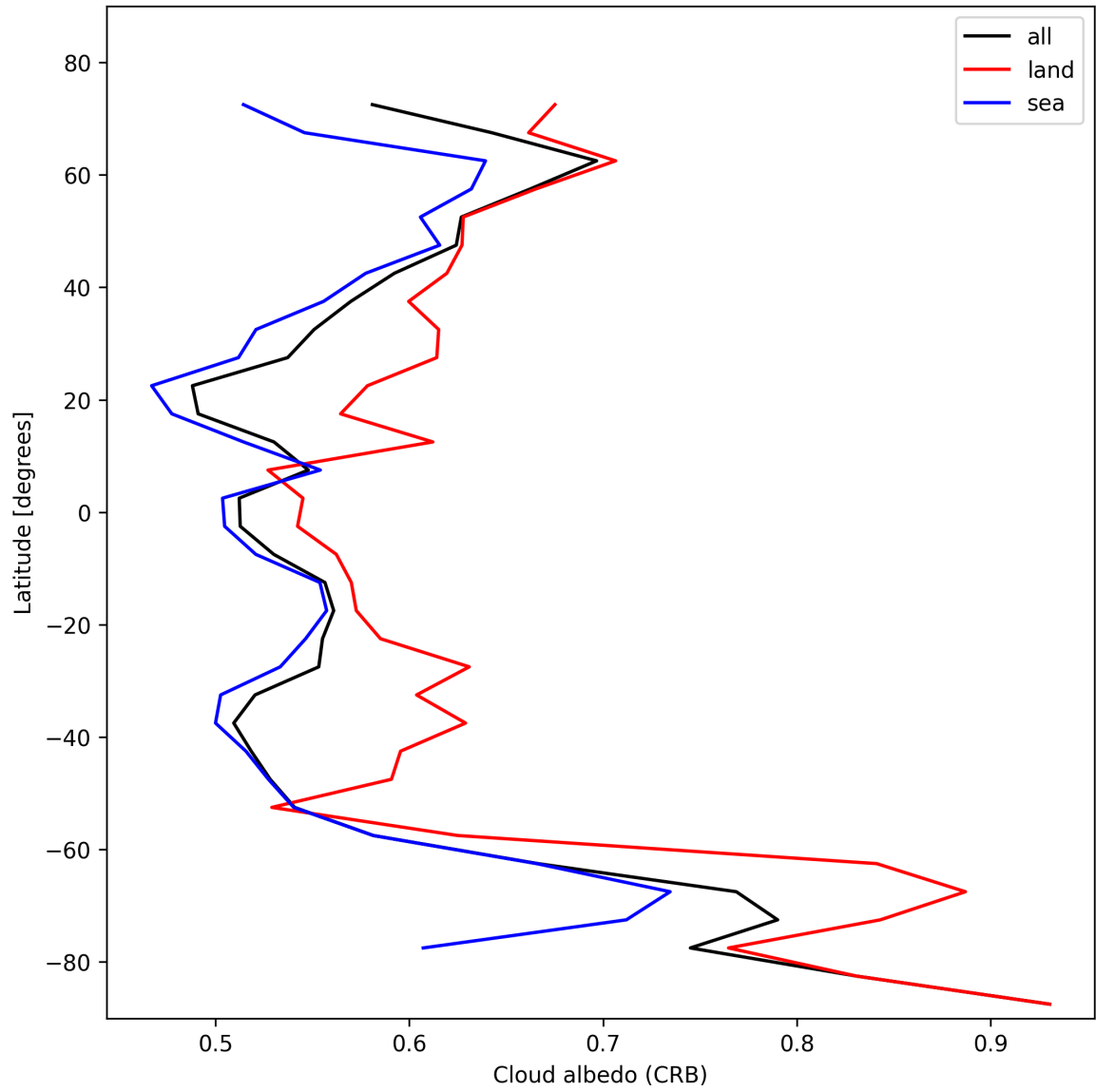
Figure 28: Zonal average of “Cloud albedo (CRB)” for 2025-11-07 to 2025-11-08.
