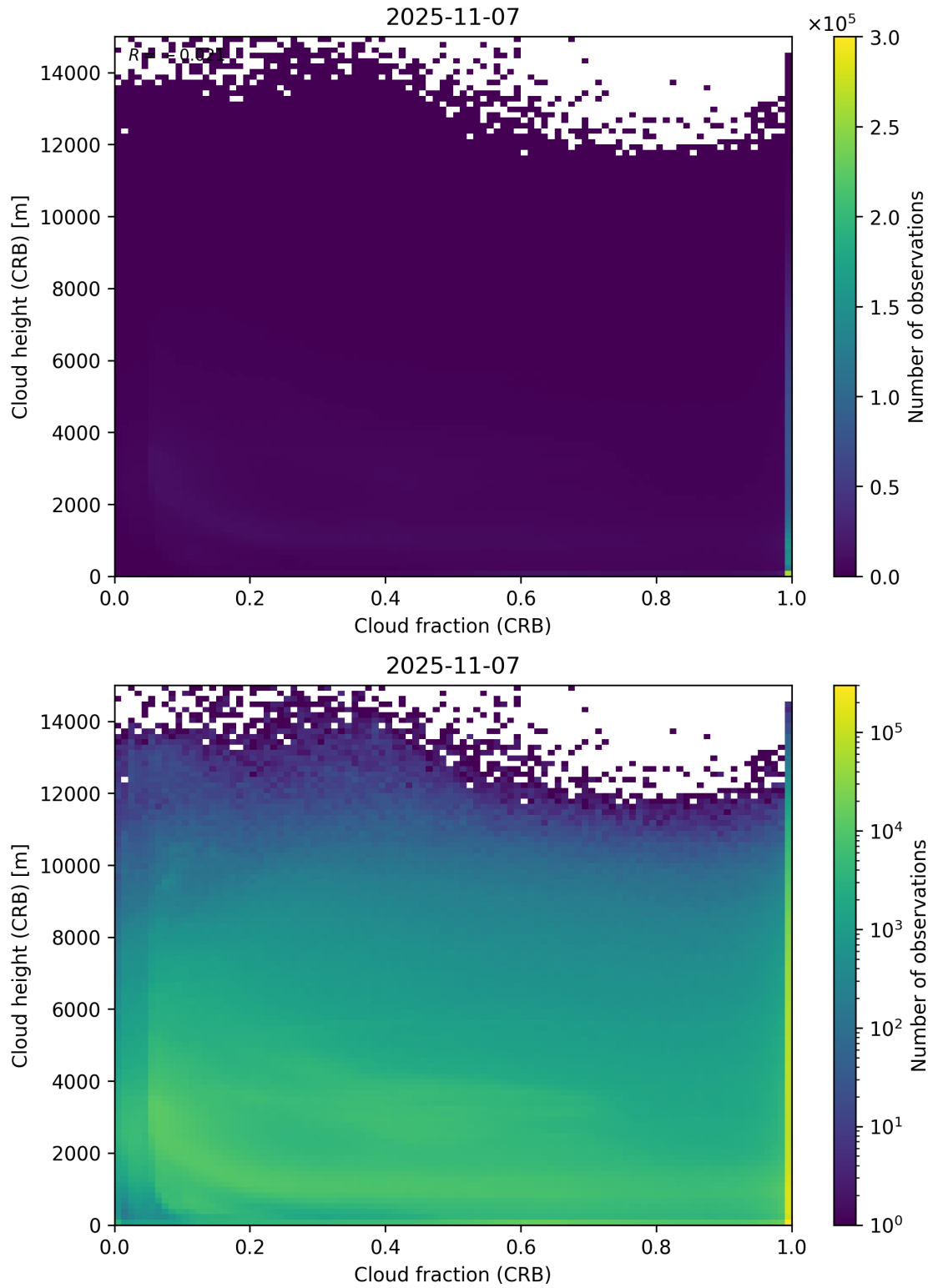
Figure 79: Scatter density plot of “Cloud fraction (CRB)” against “Cloud height (CRB)” for 2025-11-07 to 2025-11-08.
