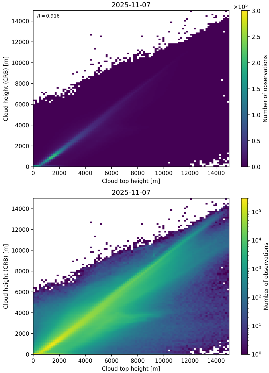
Figure 89: Scatter density plot of “Cloud top height” against “Cloud height (CRB)” for 2025-11-07 to 2025-11-08.
