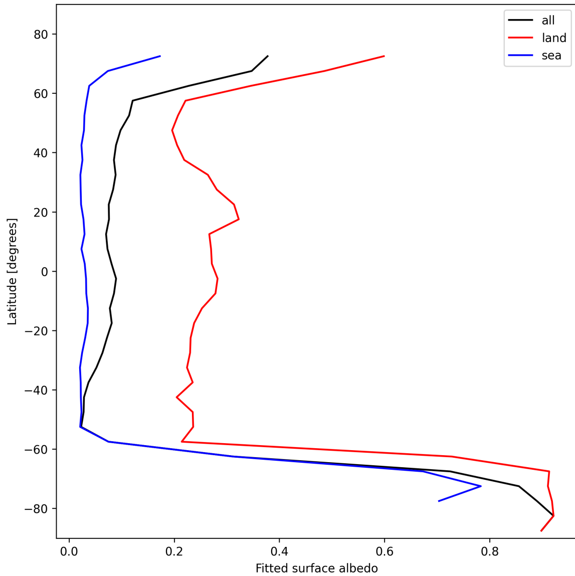
Figure 29: Zonal average of “Fitted surface albedo” for 2025-11-07 to 2025-11-08.
