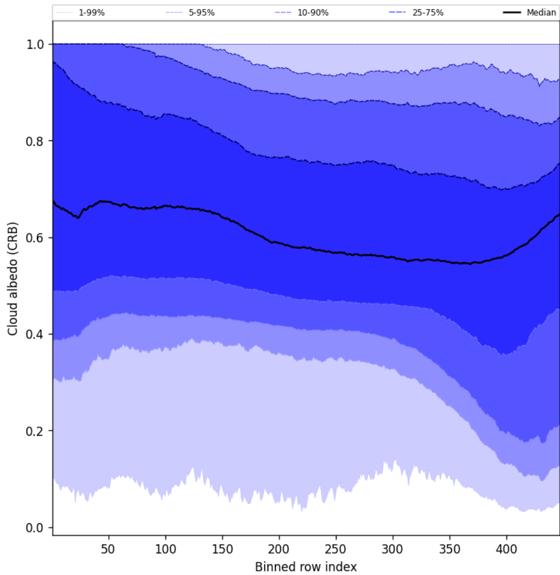
Figure 60: Along track statistics of “Cloud albedo (CRB)” for 2025-11-07 to 2025-11-08
