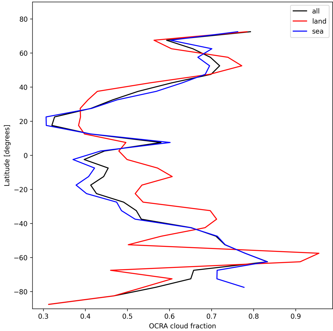
Figure 34: Zonal average of “OCRA cloud fraction” for 2025-11-07 to 2025-11-08.
