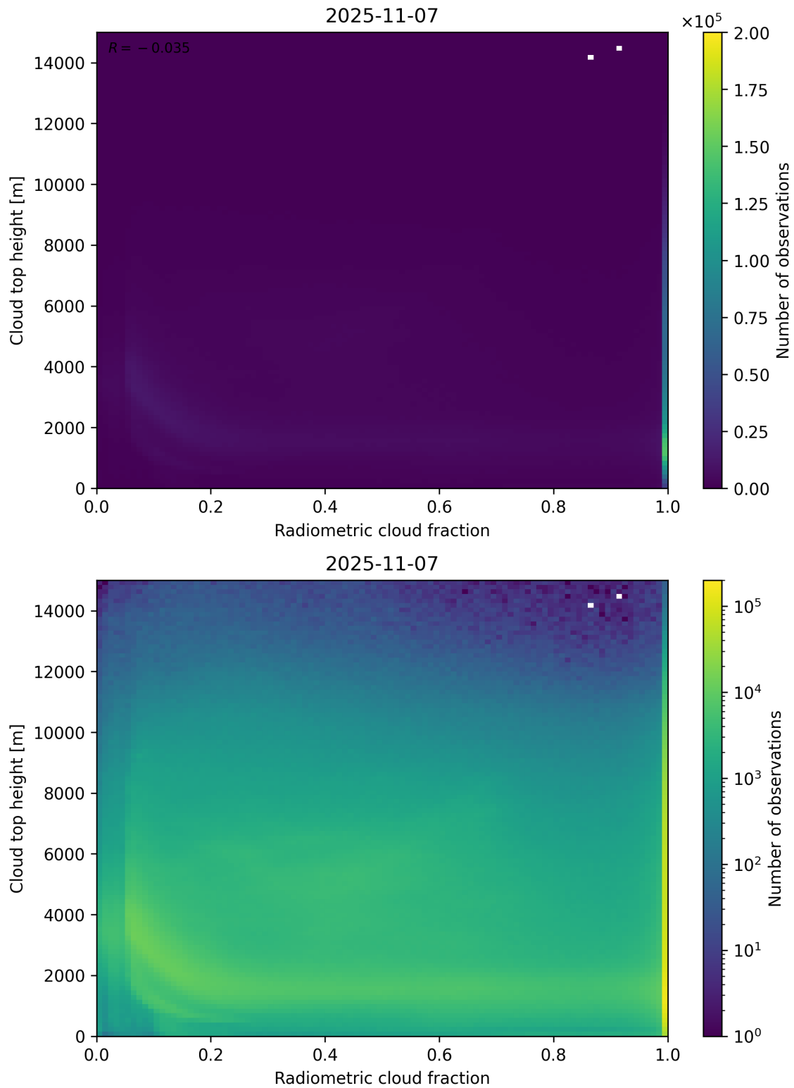
Figure 76: Scatter density plot of “Radiometric cloud fraction” against “Cloud top height” for 2025-11-07 to 2025-11-08.
