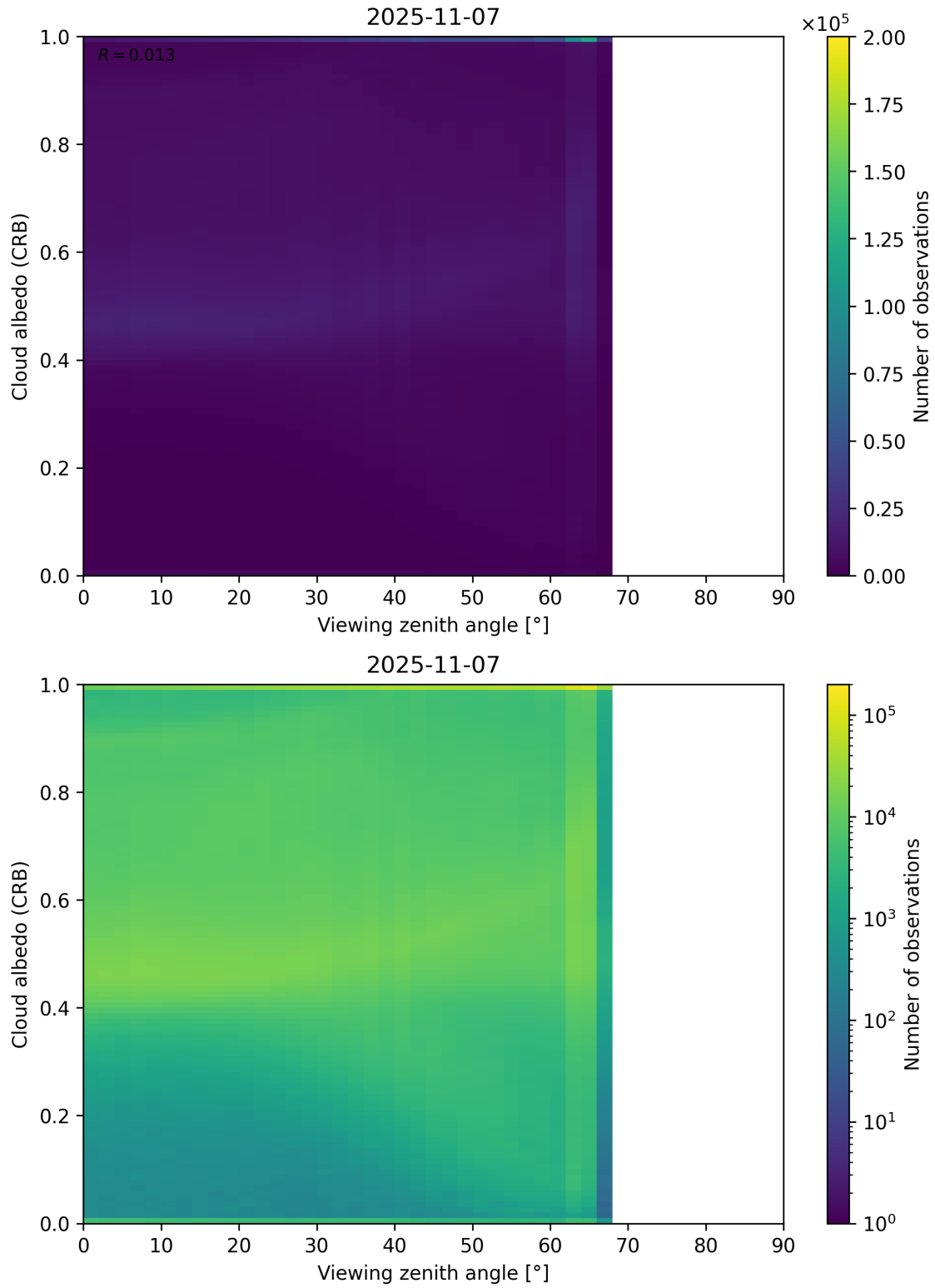
Figure 106: Scatter density plot of “Viewing zenith angle” against “Cloud albedo (CRB)” for 2025-11-07 to 2025-11-08.
