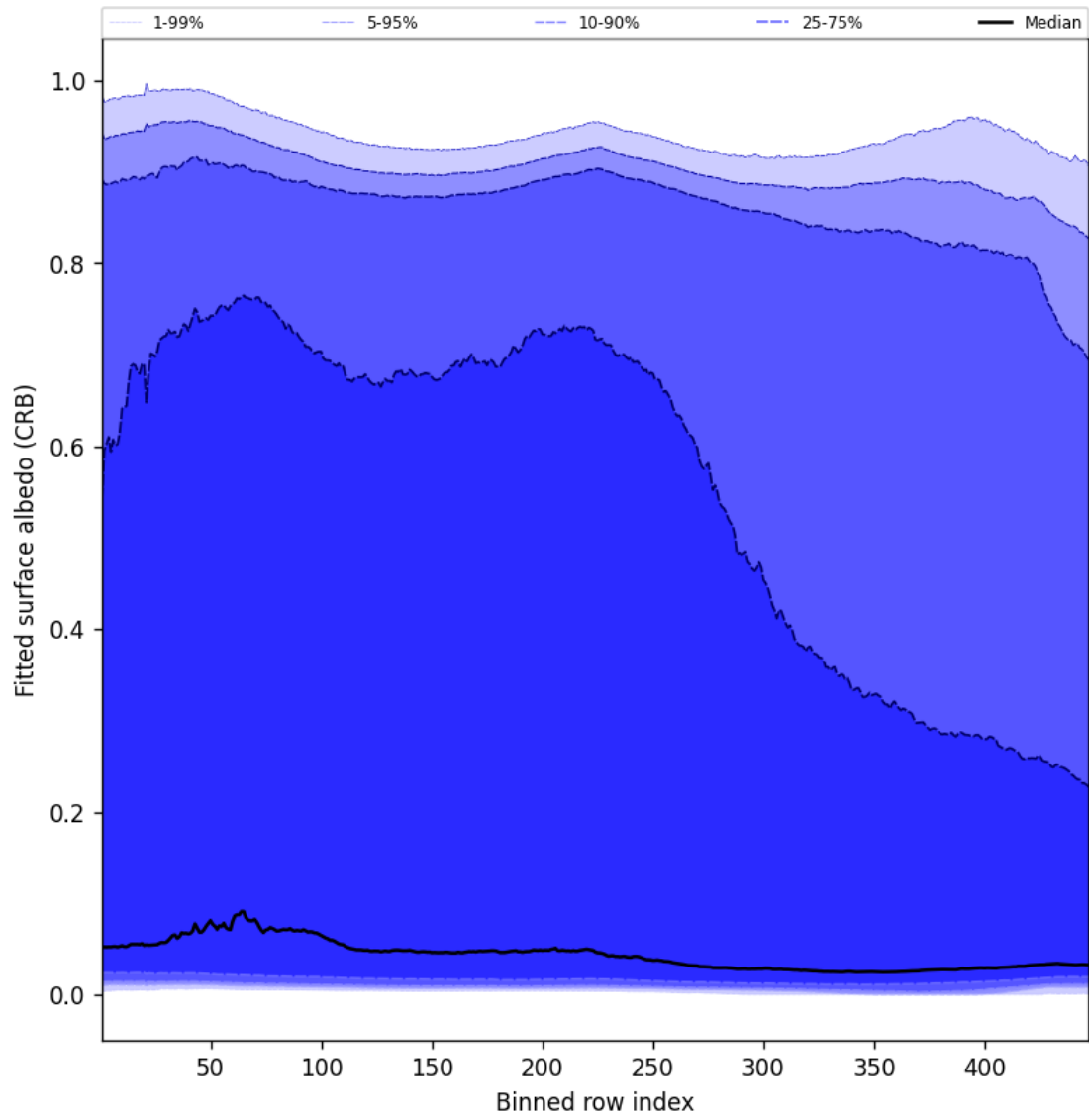
Figure 62: Along track statistics of “Fitted surface albedo (CRB)” for 2025-11-07 to 2025-11-08
