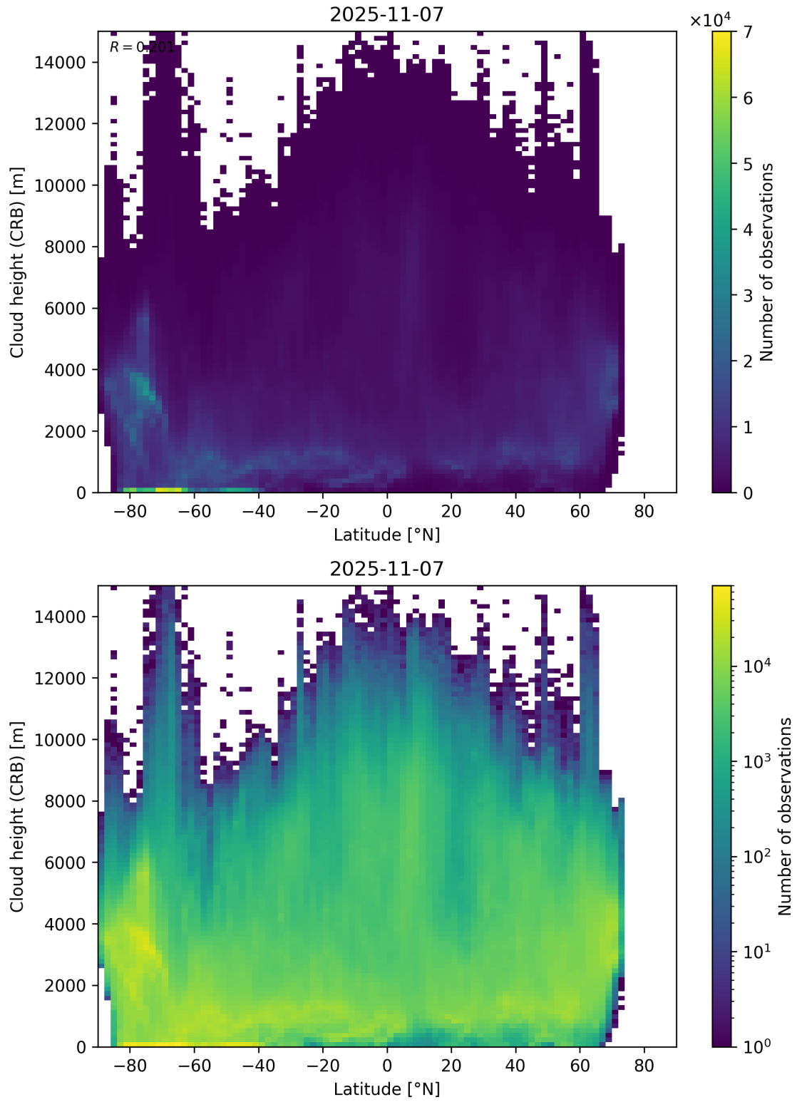
Figure 95: Scatter density plot of “Latitude” against “Cloud height (CRB)” for 2025-11-07 to 2025-11-08.
