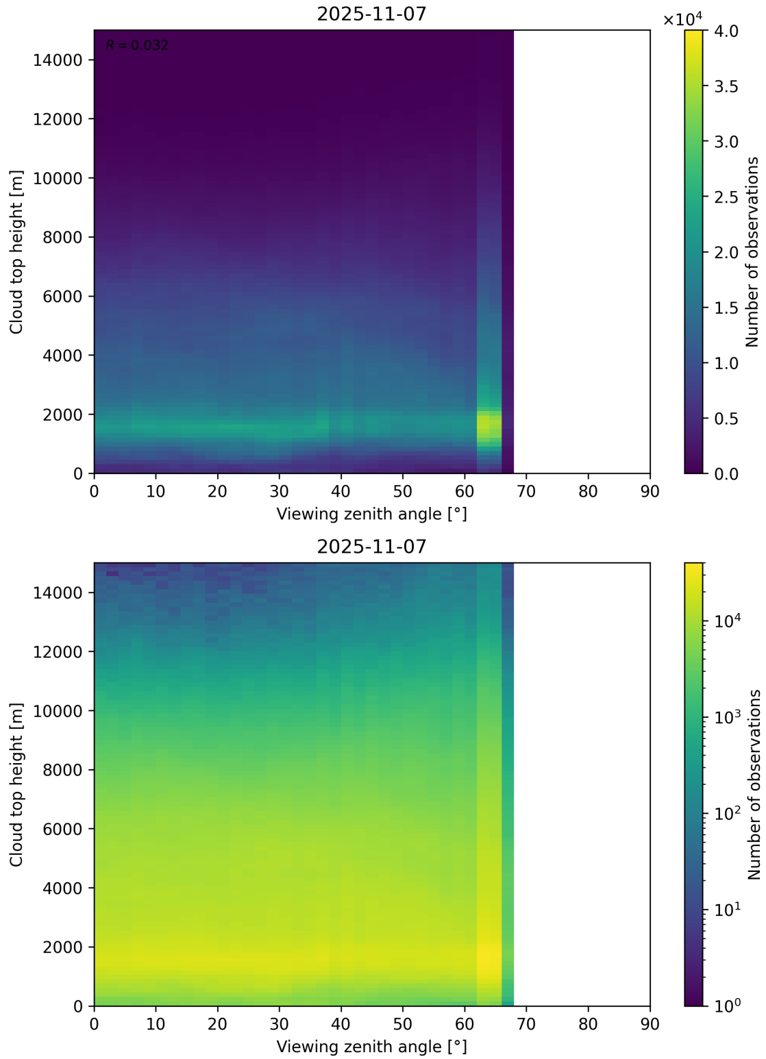
Figure 112: Scatter density plot of “Viewing zenith angle” against “Cloud top height” for 2025-11-07 to 2025-11-08.
