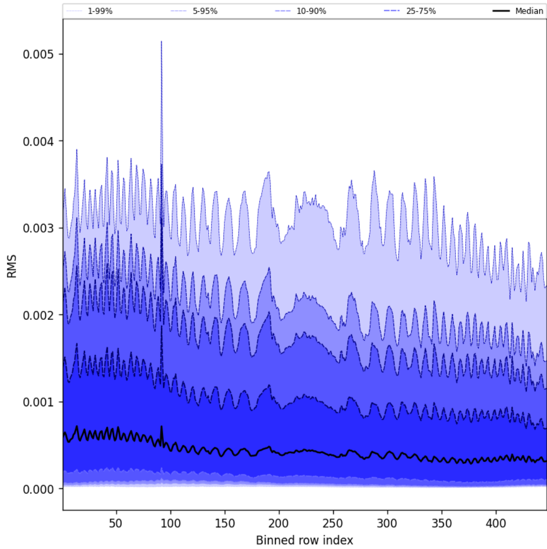
Figure 63: Along track statistics of “RMS” for 2025-11-07 to 2025-11-09
