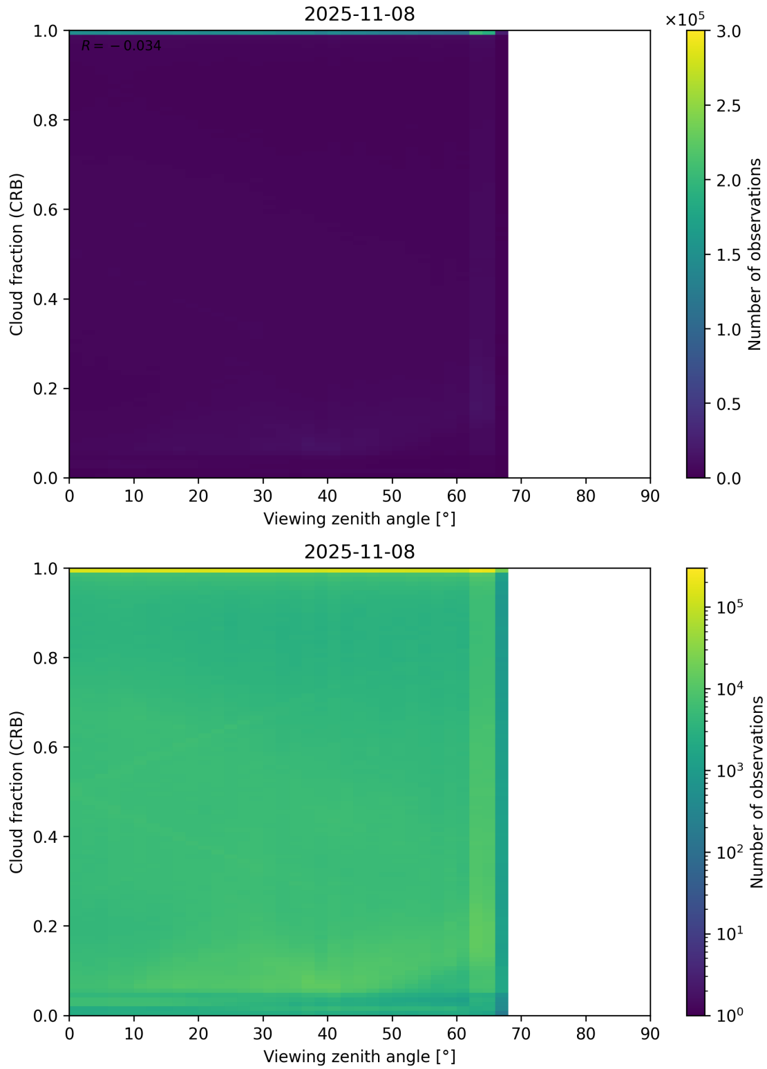
Figure 109: Scatter density plot of “Viewing zenith angle” against “Cloud fraction (CRB)” for 2025-11-07 to 2025-11-09.
