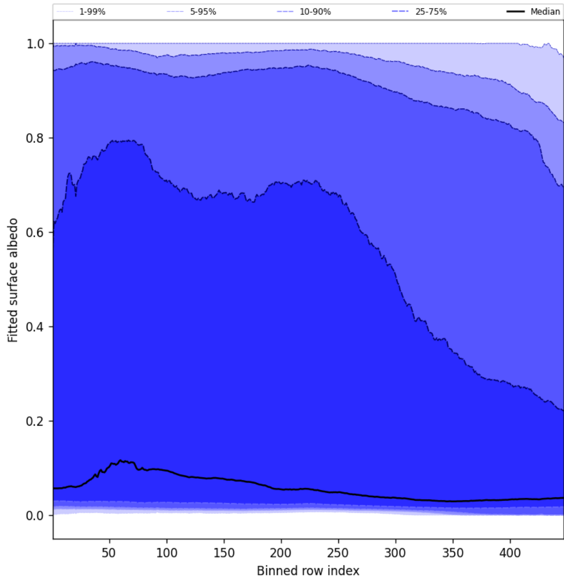
Figure 61: Along track statistics of “Fitted surface albedo” for 2025-11-07 to 2025-11-09
