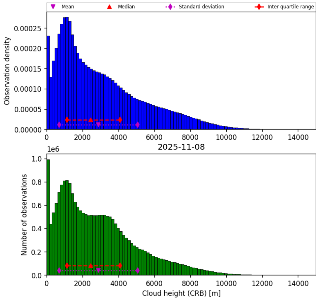
Figure 43: Histogram of “Cloud height (CRB)” for 2025-11-07 to 2025-11-09
