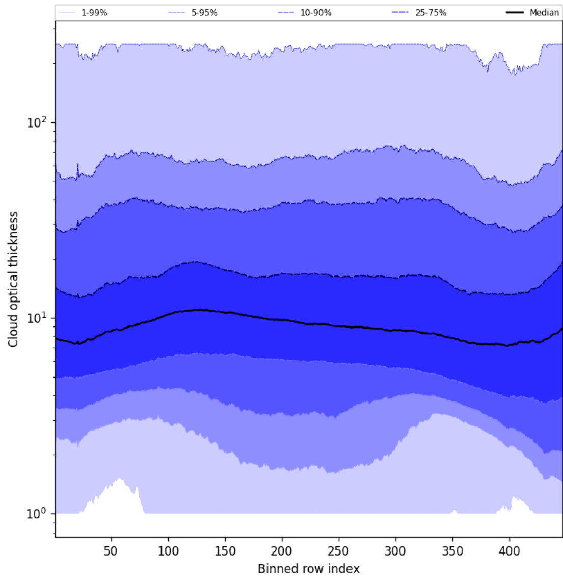
Figure 57: Along track statistics of “Cloud optical thickness” for 2025-11-07 to 2025-11-09
