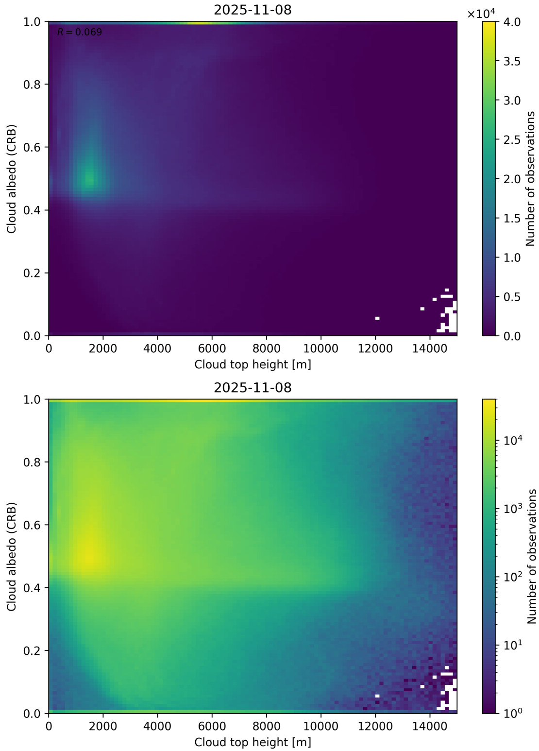
Figure 86: Scatter density plot of “Cloud top height” against “Cloud albedo (CRB)” for 2025-11-07 to 2025-11-09.
