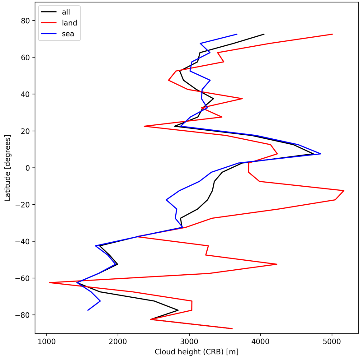
Figure 27: Zonal average of “Cloud height (CRB)” for 2025-11-07 to 2025-11-09.
