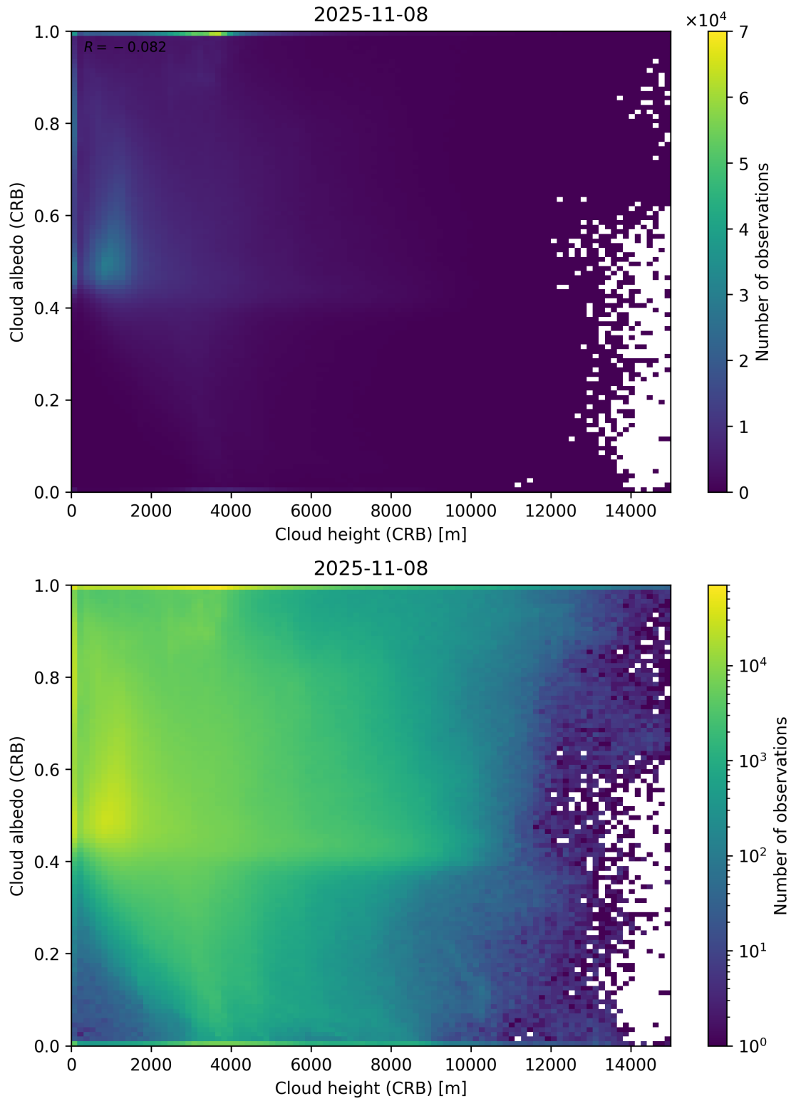
Figure 80: Scatter density plot of “Cloud height (CRB)” against “Cloud albedo (CRB)” for 2025-11-07 to 2025-11-09.
