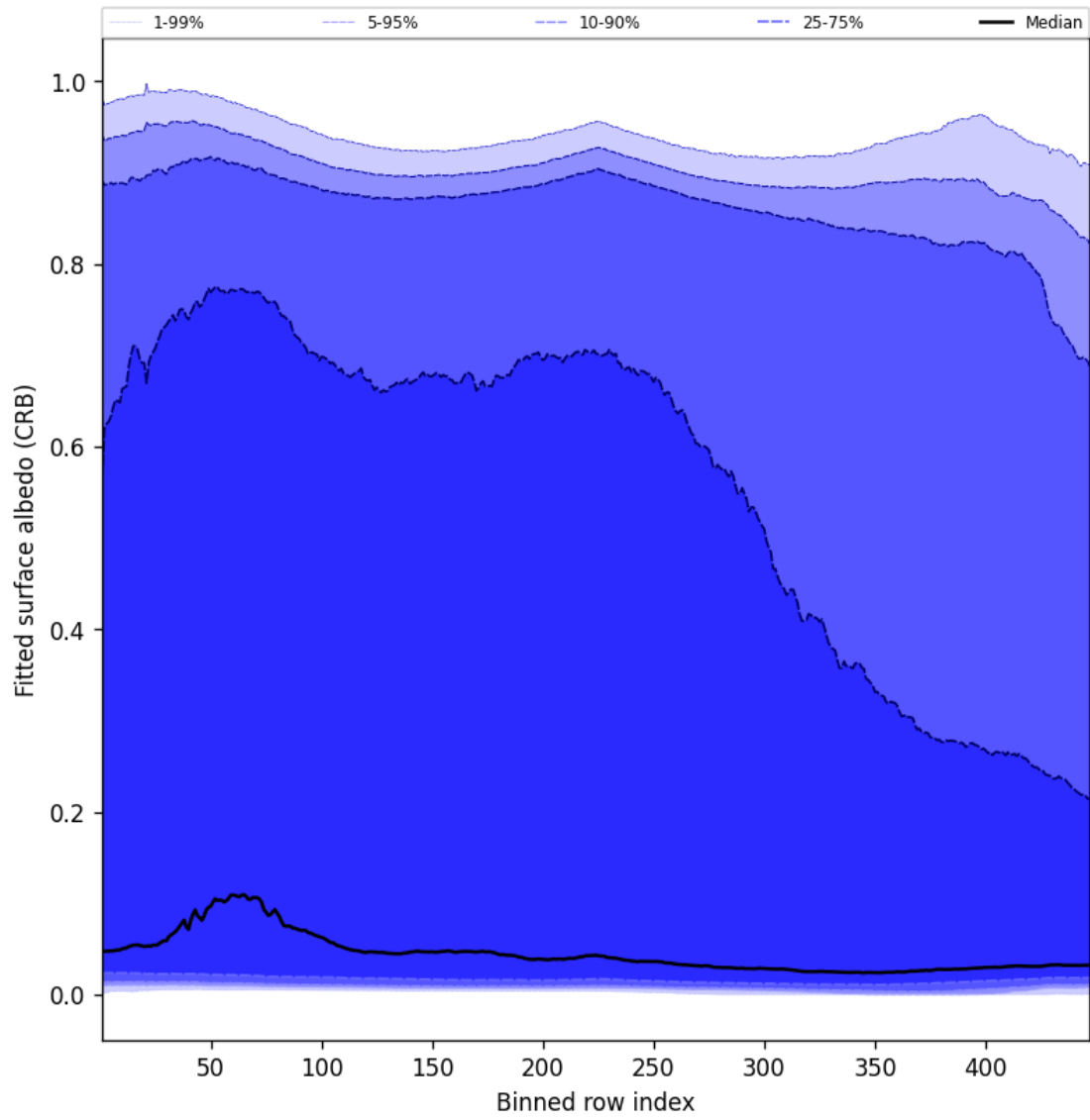
Figure 62: Along track statistics of “Fitted surface albedo (CRB)” for 2025-11-07 to 2025-11-09
