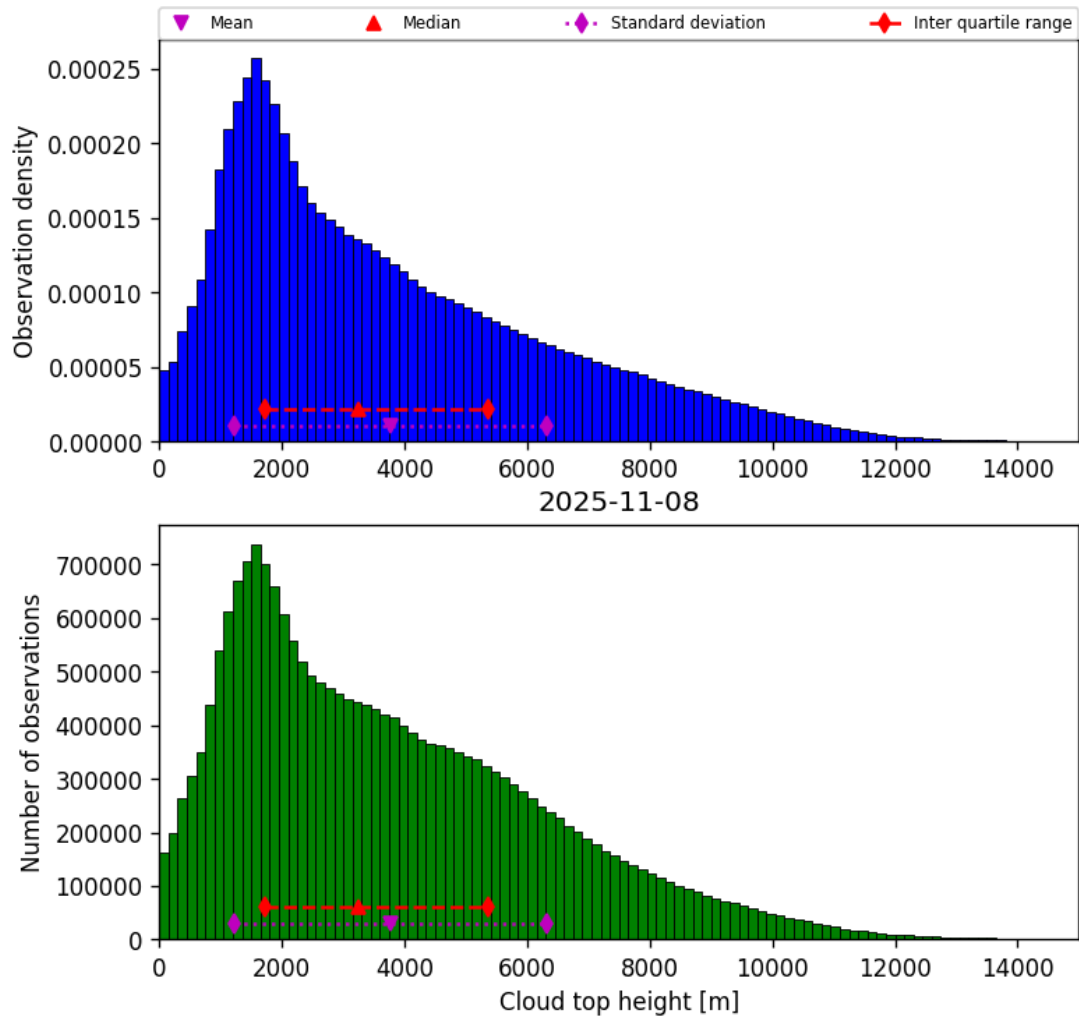
Figure 40: Histogram of “Cloud top height” for 2025-11-07 to 2025-11-09
