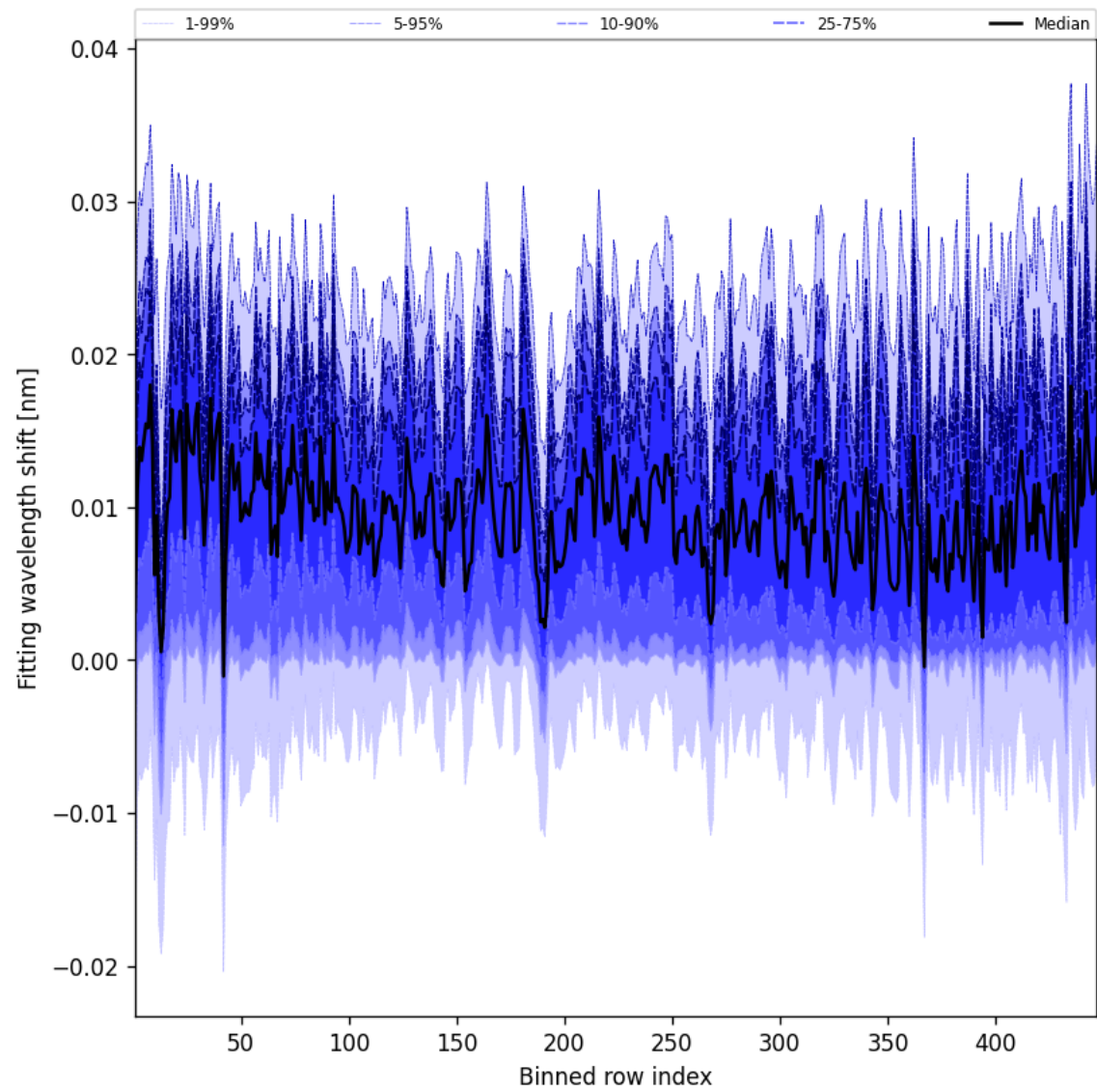
Figure 65: Along track statistics of “Fitting wavelength shift” for 2025-11-07 to 2025-11-09
