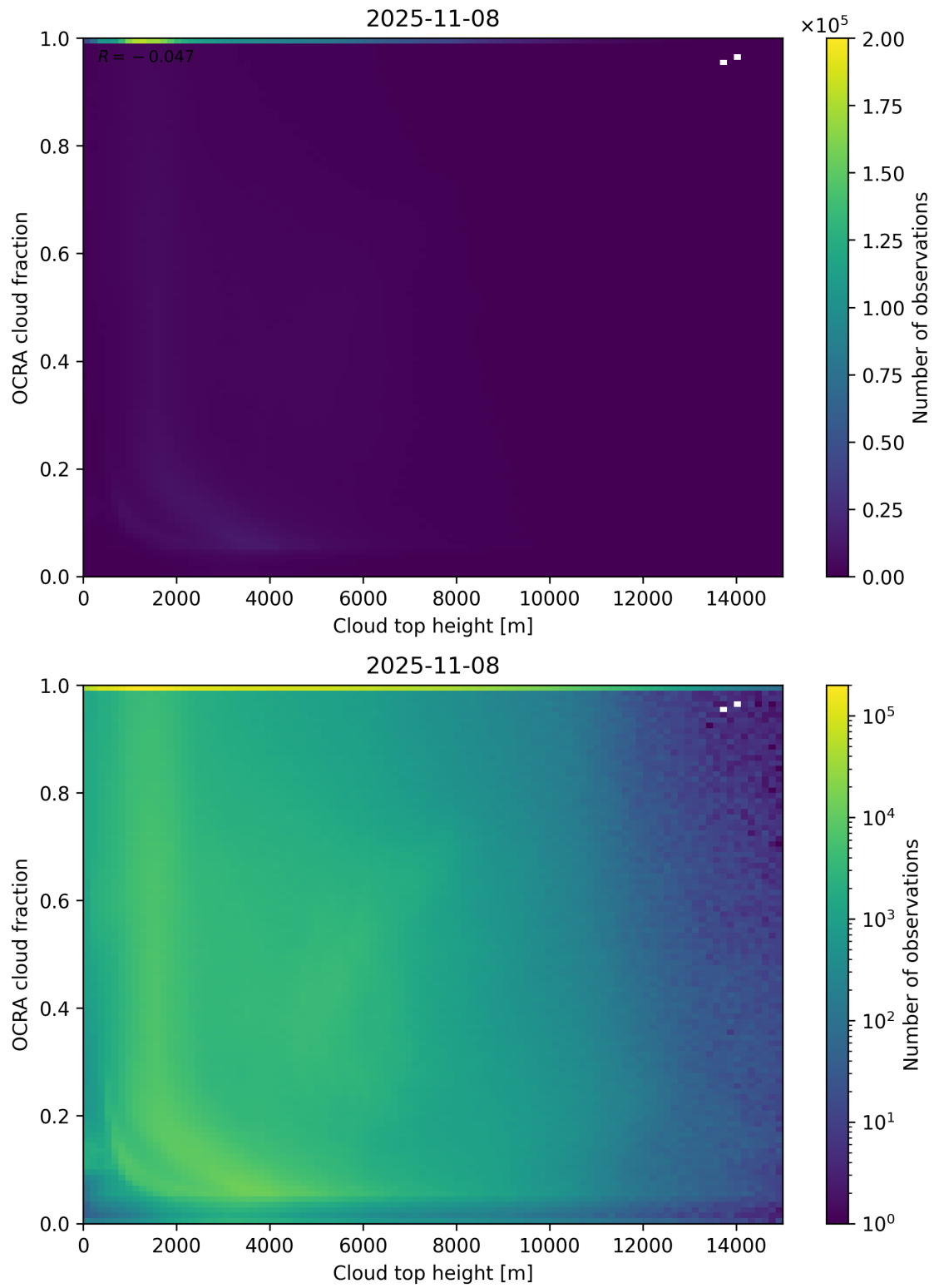
Figure 87: Scatter density plot of “Cloud top height” against “OCRA cloud fraction” for 2025-11-07 to 2025-11-09.
