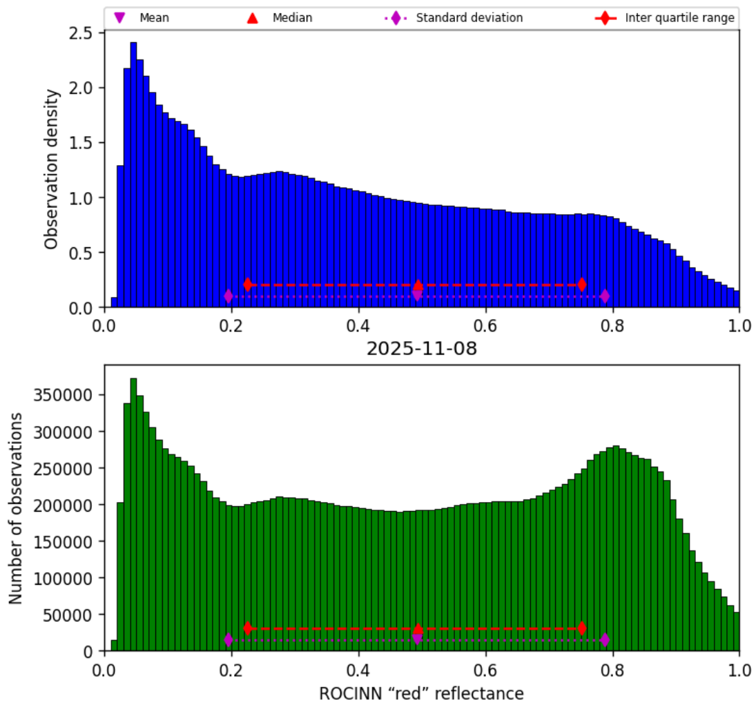
Figure 53: Histogram of “ROCINN “red” reflectance” for 2025-11-07 to 2025-11-09
