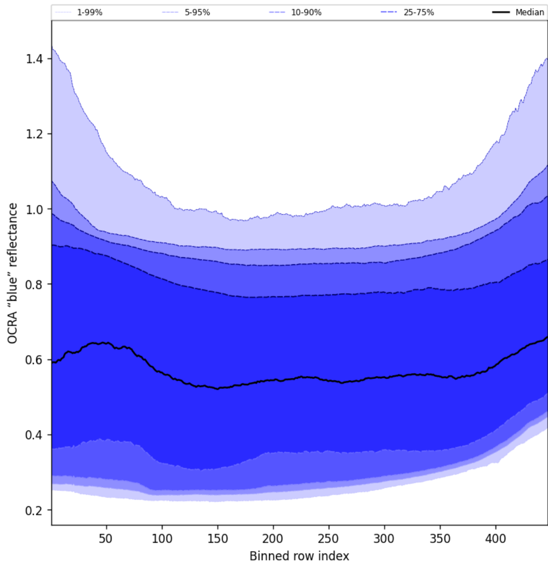
Figure 67: Along track statistics of “OCRA “blue” reflectance” for 2025-11-07 to 2025-11-09
