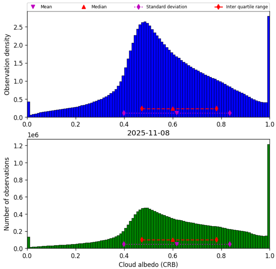
Figure 44: Histogram of “Cloud albedo (CRB)” for 2025-11-07 to 2025-11-09
