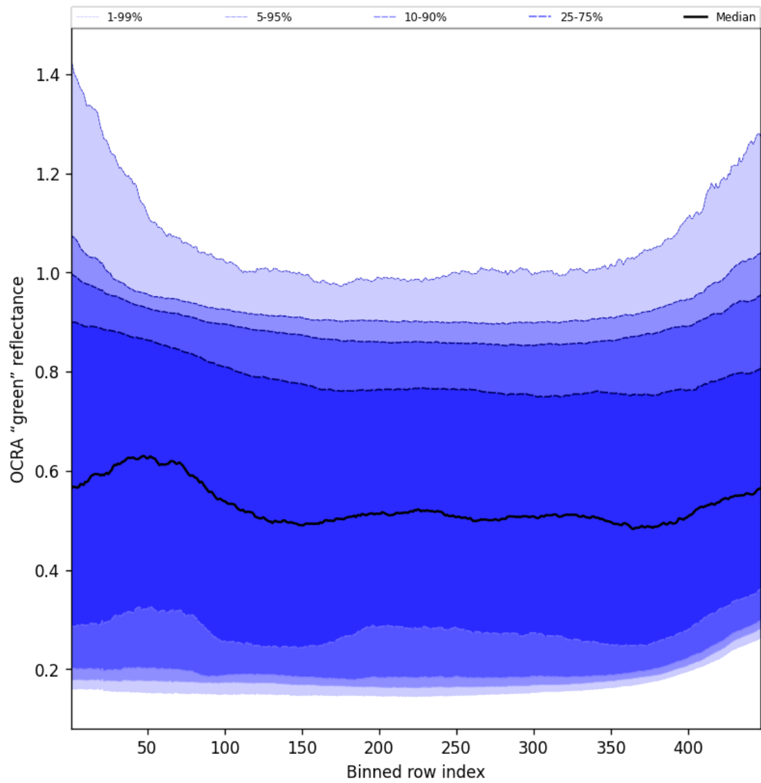
Figure 68: Along track statistics of "OCRA "green" reflectance" for 2025-11-07 to 2025-11-09
