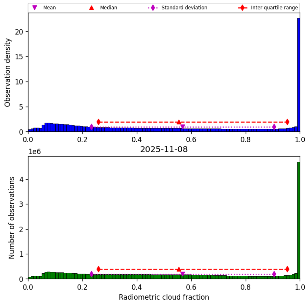
Figure 39: Histogram of “Radiometric cloud fraction” for 2025-11-07 to 2025-11-09
