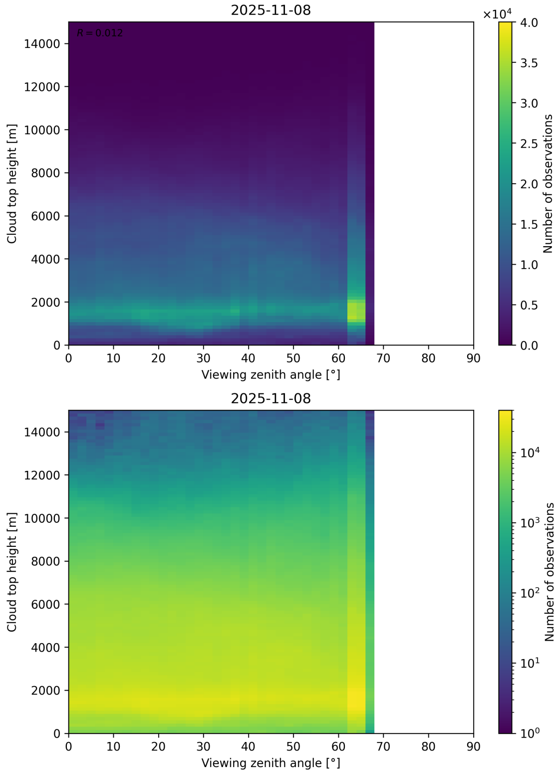
Figure 112: Scatter density plot of “Viewing zenith angle” against “Cloud top height” for 2025-11-07 to 2025-11-09.
