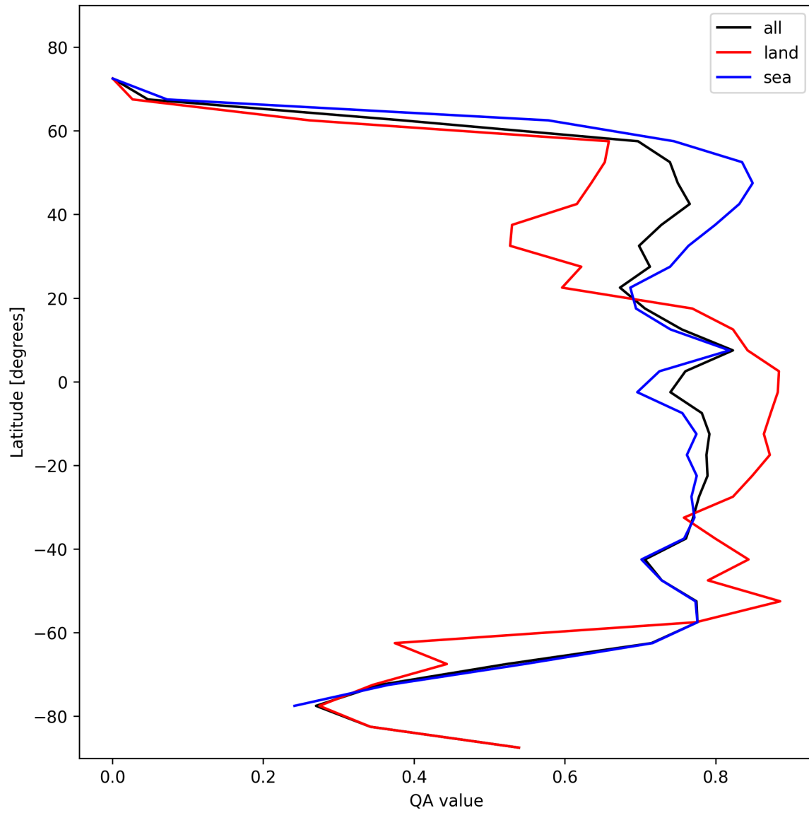
Figure 22: Zonal average of “QA value” for 2025-11-07 to 2025-11-09.
