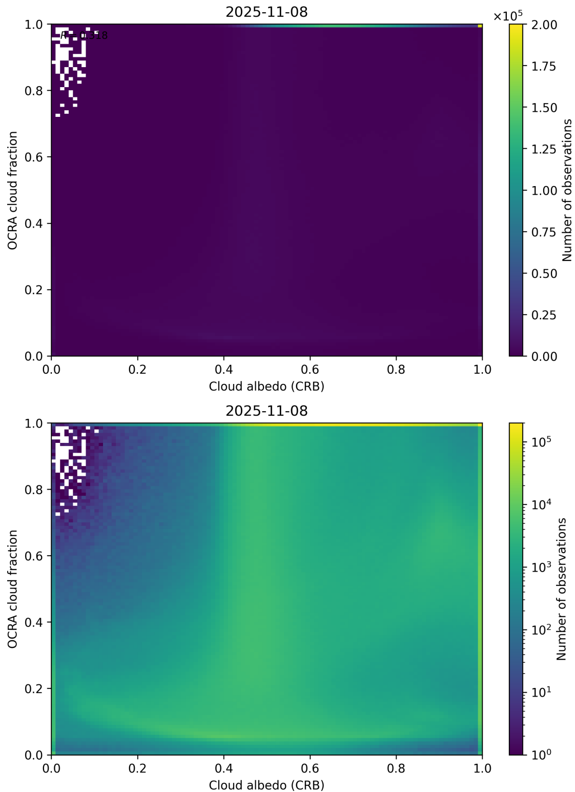
Figure 70: Scatter density plot of “Cloud albedo (CRB)” against “OCRA cloud fraction” for 2025-11-07 to 2025-11-09.
