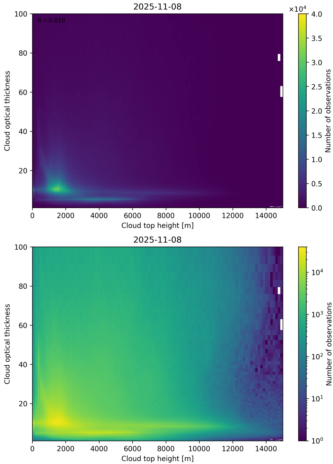
Figure 90: Scatter density plot of “Cloud top height” against “Cloud optical thickness” for 2025-11-07 to 2025-11-09.
