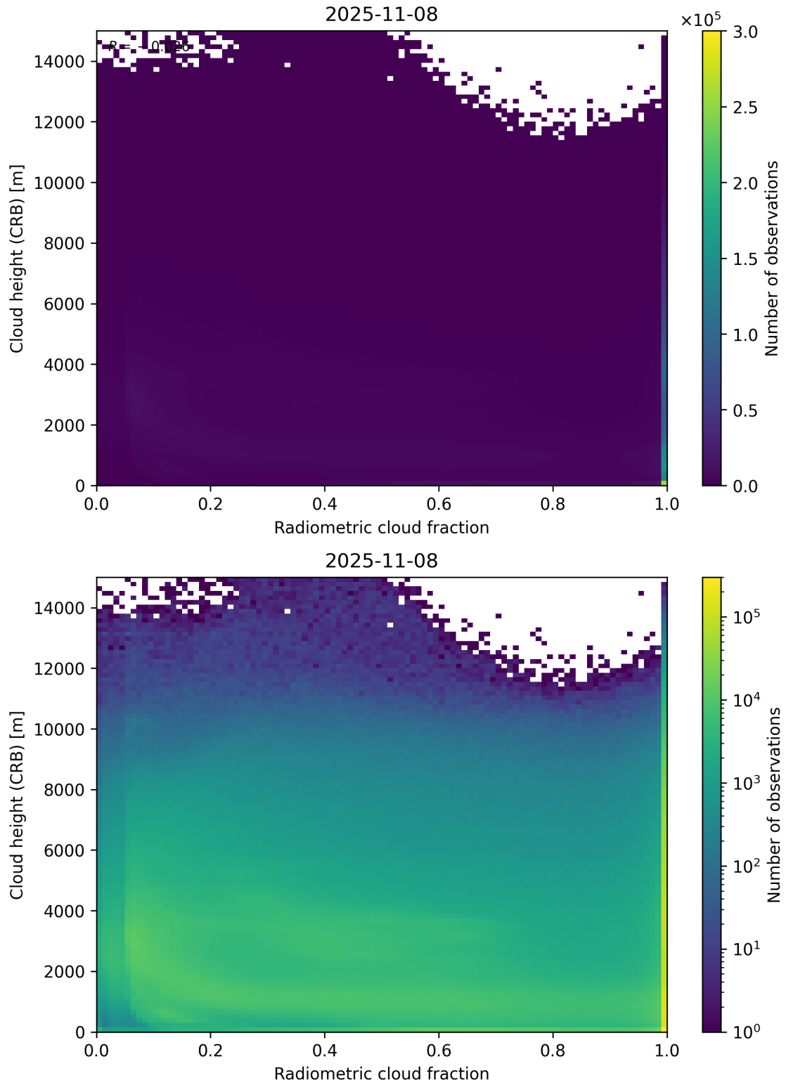
Figure 74: Scatter density plot of “Radiometric cloud fraction” against “Cloud height (CRB)” for 2025-11-07 to 2025-11-09.
