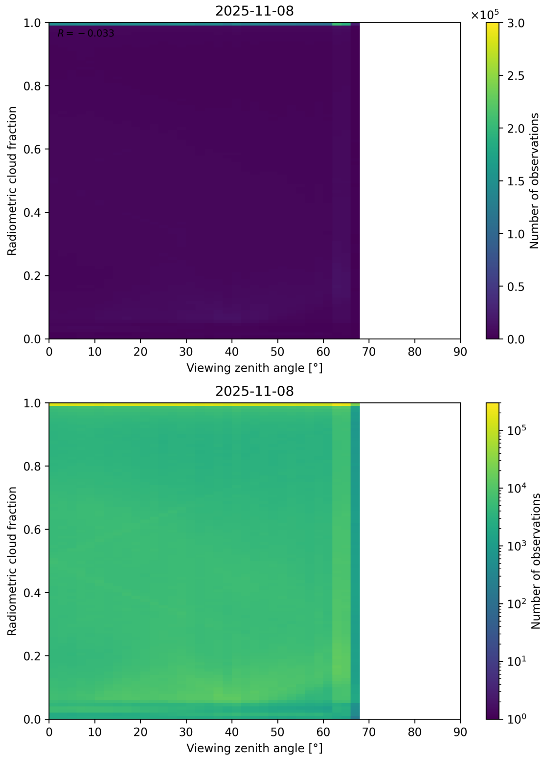
Figure 107: Scatter density plot of “Viewing zenith angle” against “Radiometric cloud fraction” for 2025-11-07 to 2025-11-09.
