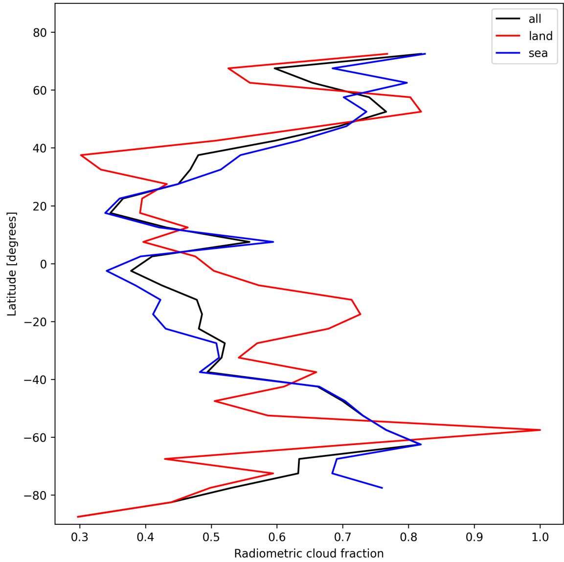
Figure 23: Zonal average of “Radiometric cloud fraction” for 2025-11-07 to 2025-11-09.
