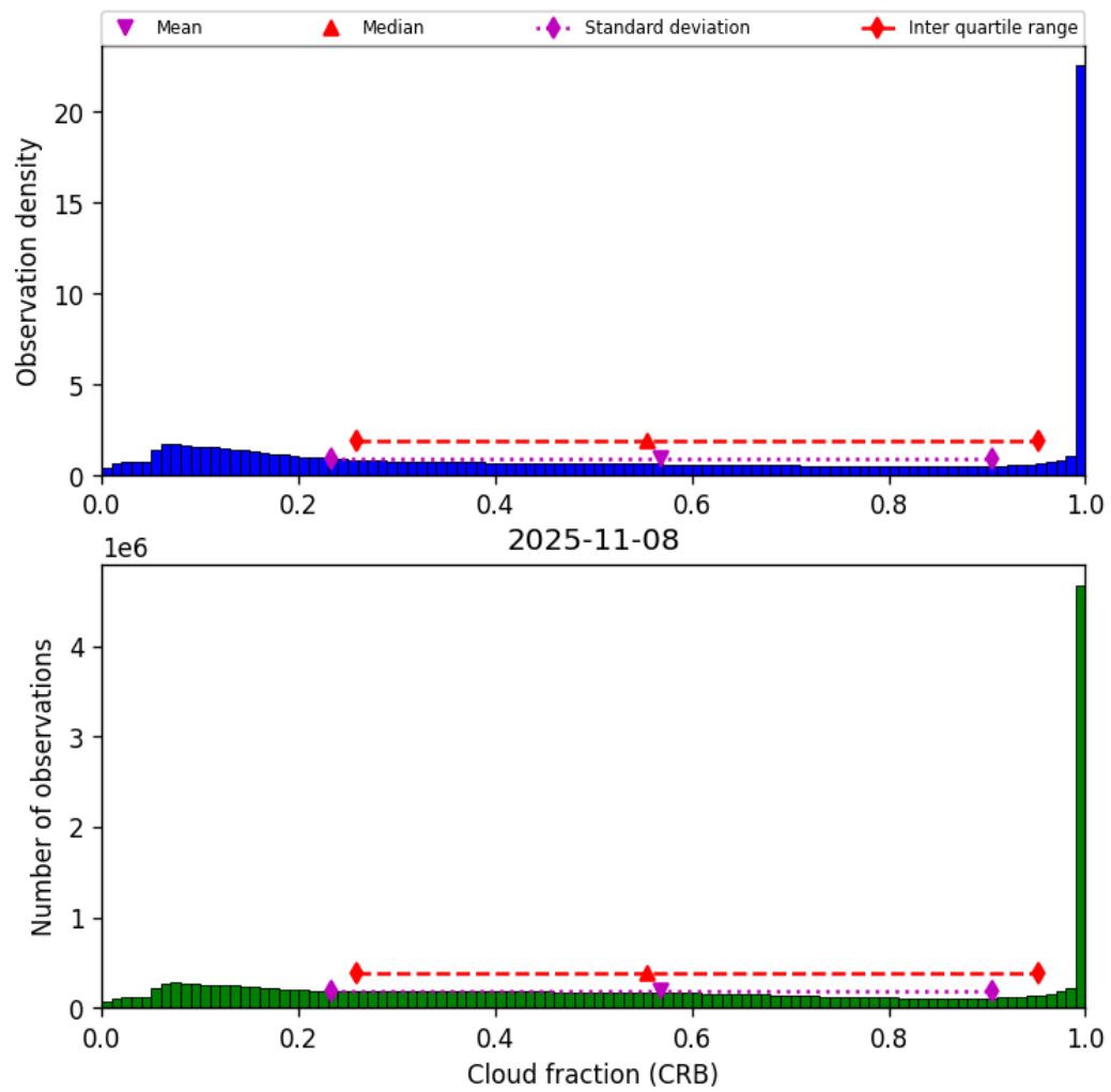
Figure 42: Histogram of “Cloud fraction (CRB)” for 2025-11-07 to 2025-11-09
