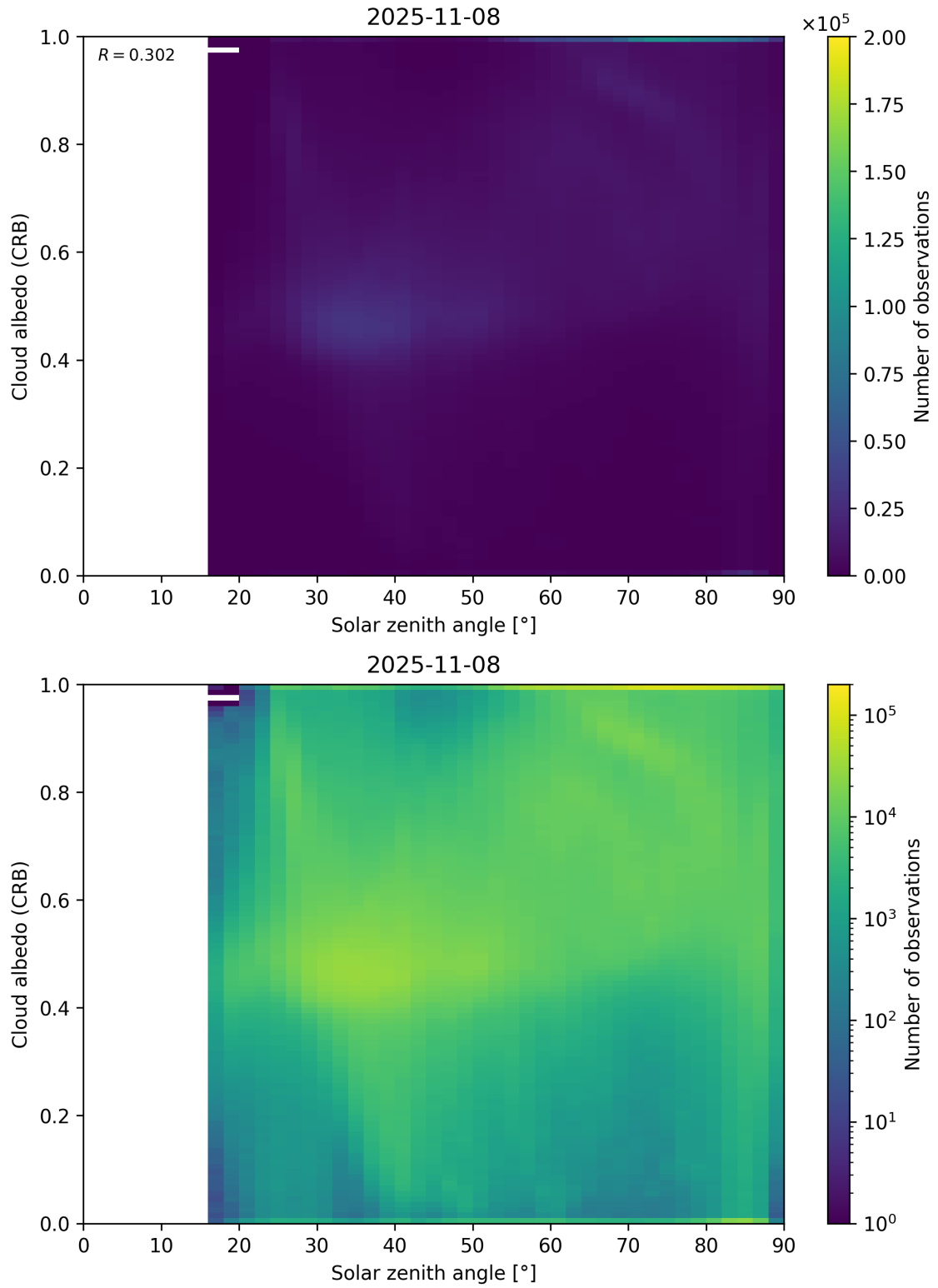
Figure 98: Scatter density plot of “Solar zenith angle” against “Cloud albedo (CRB)” for 2025-11-07 to 2025-11-09.
