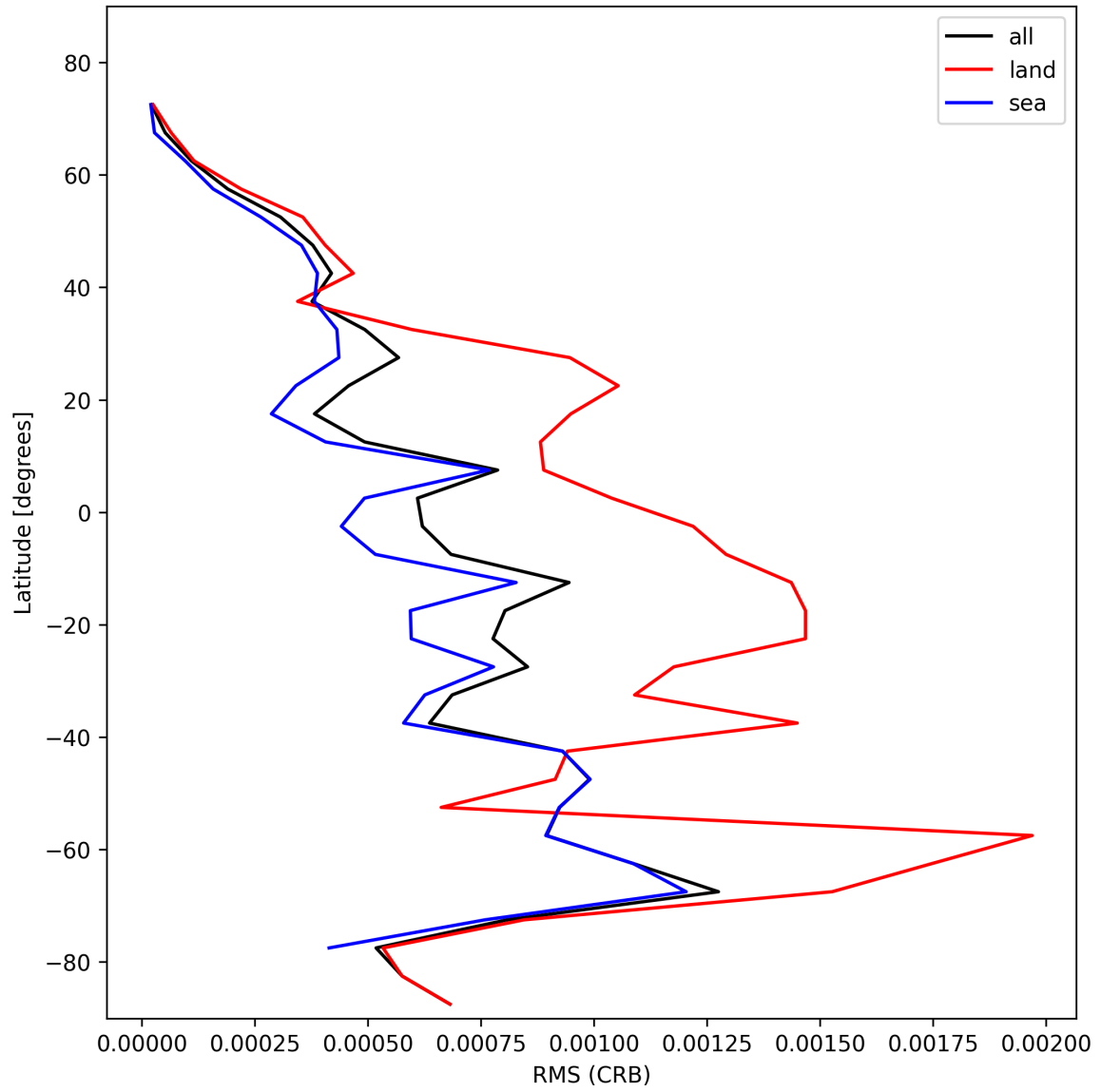
Figure 32: Zonal average of “RMS (CRB)” for 2025-11-07 to 2025-11-09.
