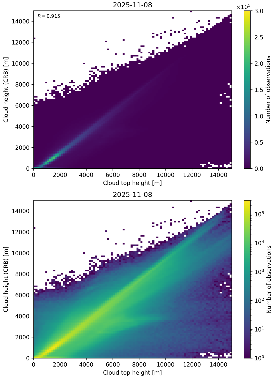
Figure 89: Scatter density plot of “Cloud top height” against “Cloud height (CRB)” for 2025-11-07 to 2025-11-09.
