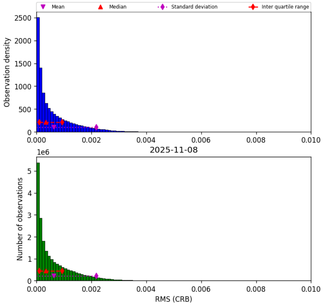
Figure 48: Histogram of “RMS (CRB)” for 2025-11-07 to 2025-11-09
