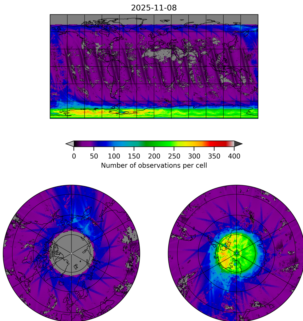
Figure 21: Map of the number of observations for 2025-11-07 to 2025-11-09
