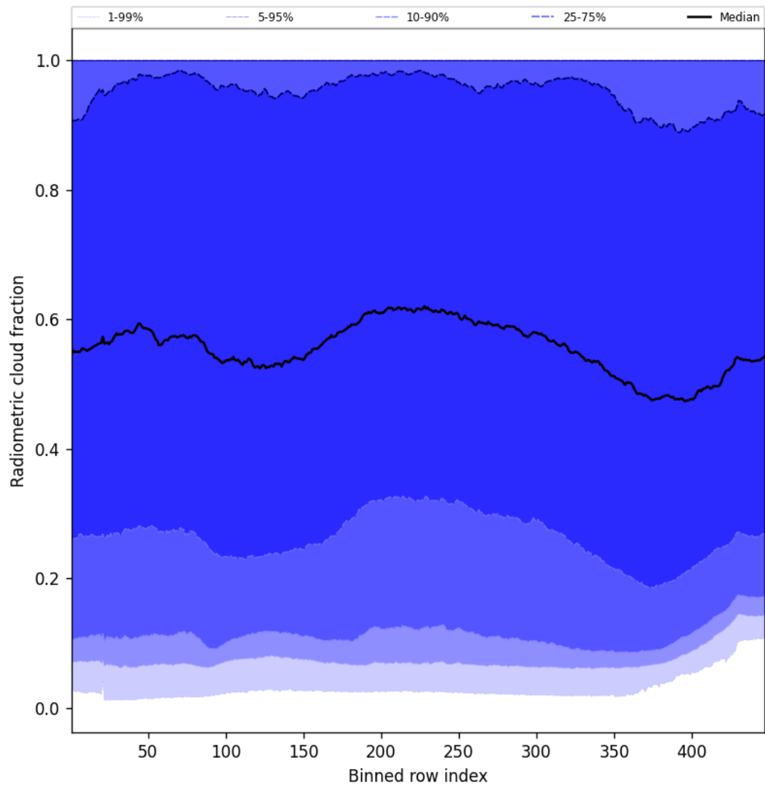
Figure 55: Along track statistics of “Radiometric cloud fraction” for 2025-11-07 to 2025-11-09
