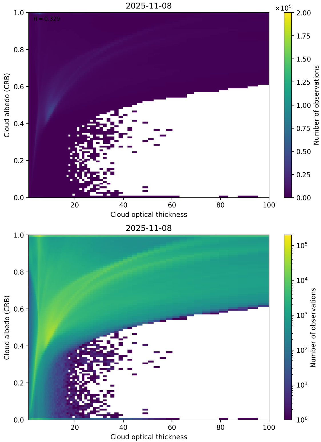
Figure 82: Scatter density plot of “Cloud optical thickness” against “Cloud albedo (CRB)” for 2025-11-07 to 2025-11-09.
