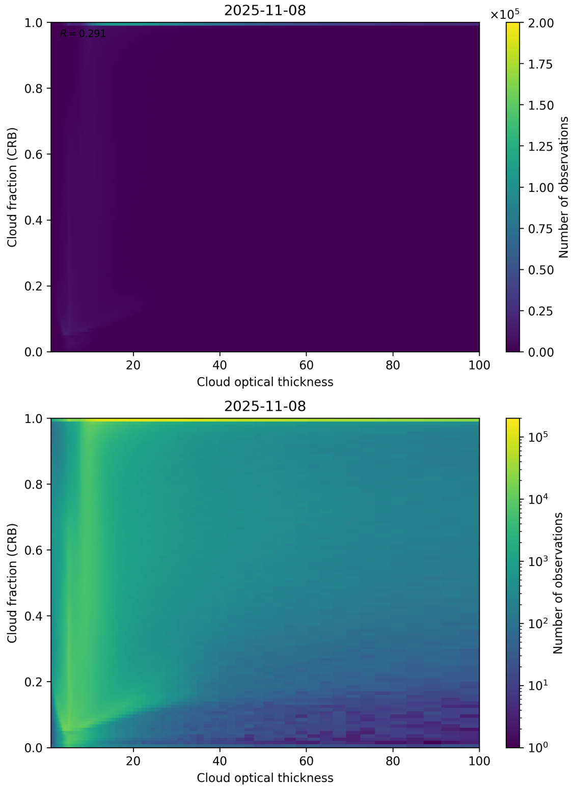
Figure 84: Scatter density plot of “Cloud optical thickness” against “Cloud fraction (CRB)” for 2025-11-07 to 2025-11-09.
