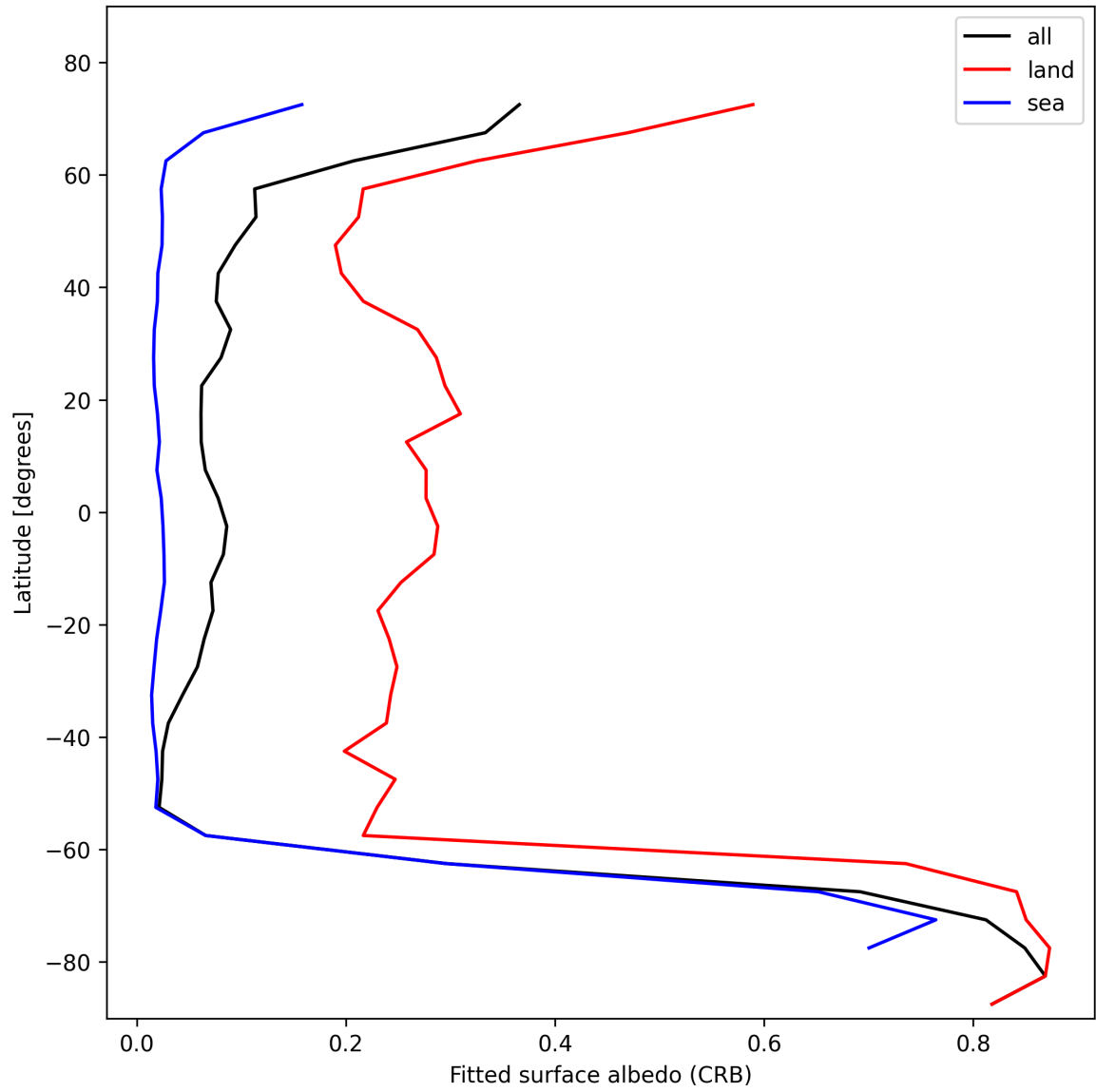
Figure 30: Zonal average of “Fitted surface albedo (CRB)” for 2025-11-07 to 2025-11-09.
