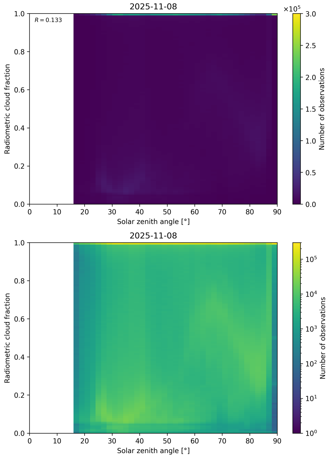
Figure 99: Scatter density plot of “Solar zenith angle” against “Radiometric cloud fraction” for 2025-11-07 to 2025-11-09.
