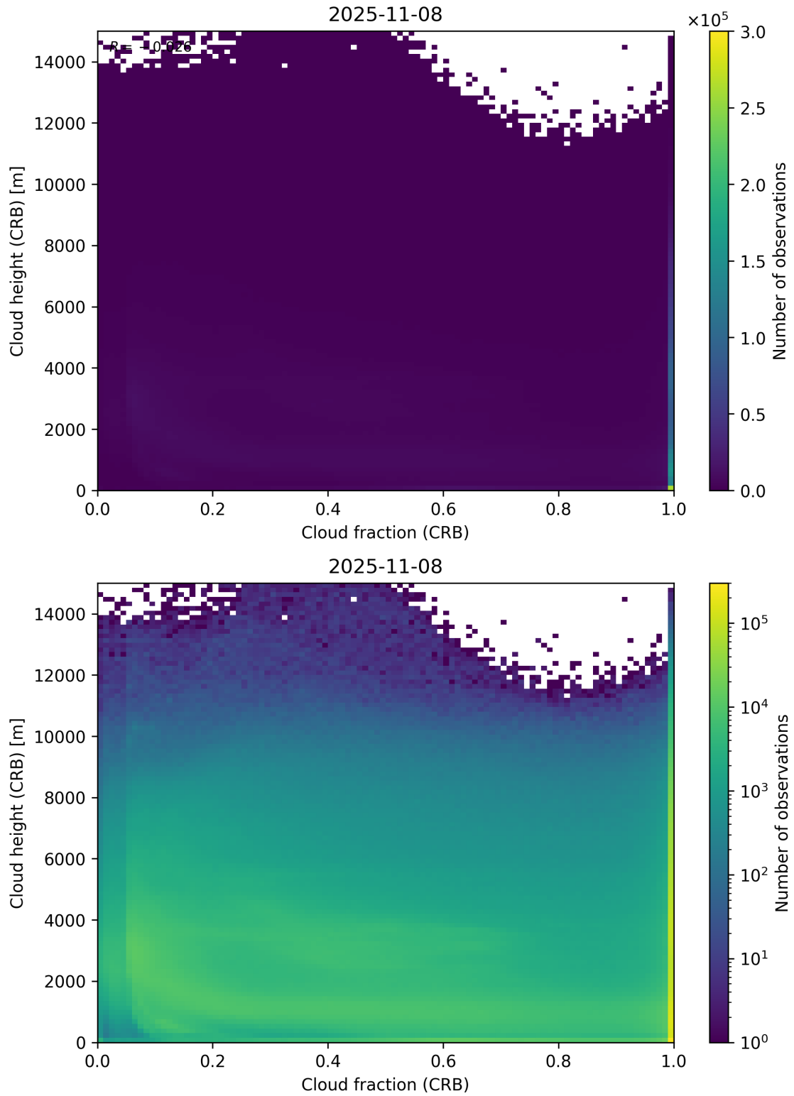
Figure 79: Scatter density plot of “Cloud fraction (CRB)” against “Cloud height (CRB)” for 2025-11-07 to 2025-11-09.
