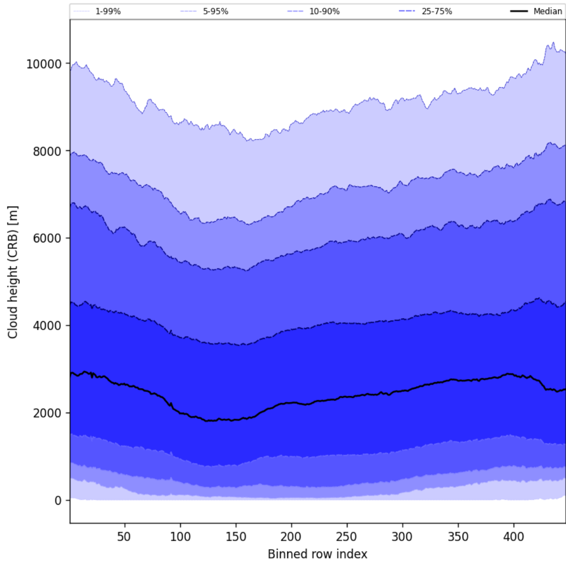
Figure 59: Along track statistics of “Cloud height (CRB)” for 2025-11-07 to 2025-11-09
