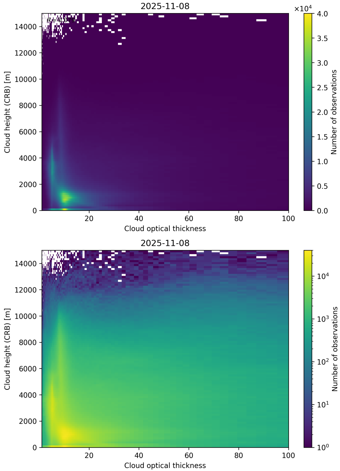
Figure 85: Scatter density plot of “Cloud optical thickness” against “Cloud height (CRB)” for 2025-11-07 to 2025-11-09.
