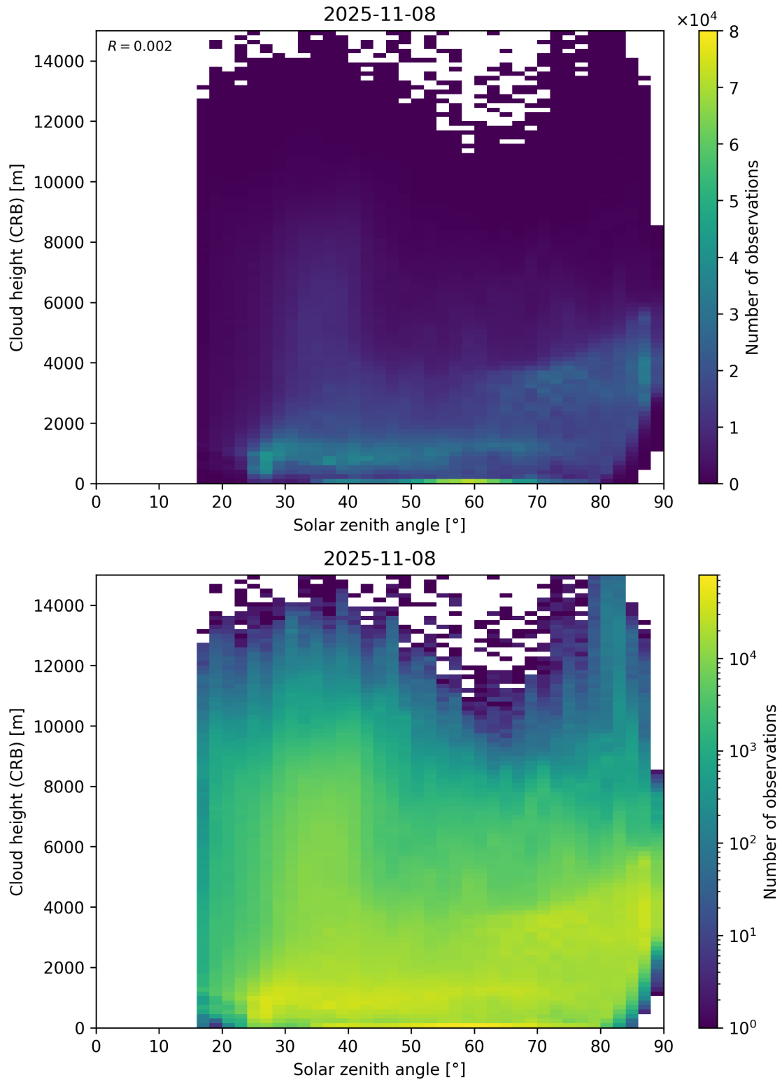
Figure 102: Scatter density plot of “Solar zenith angle” against “Cloud height (CRB)” for 2025-11-07 to 2025-11-09.
