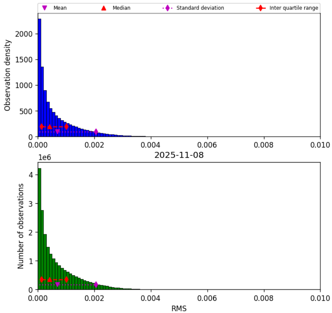
Figure 47: Histogram of “RMS” for 2025-11-07 to 2025-11-09
