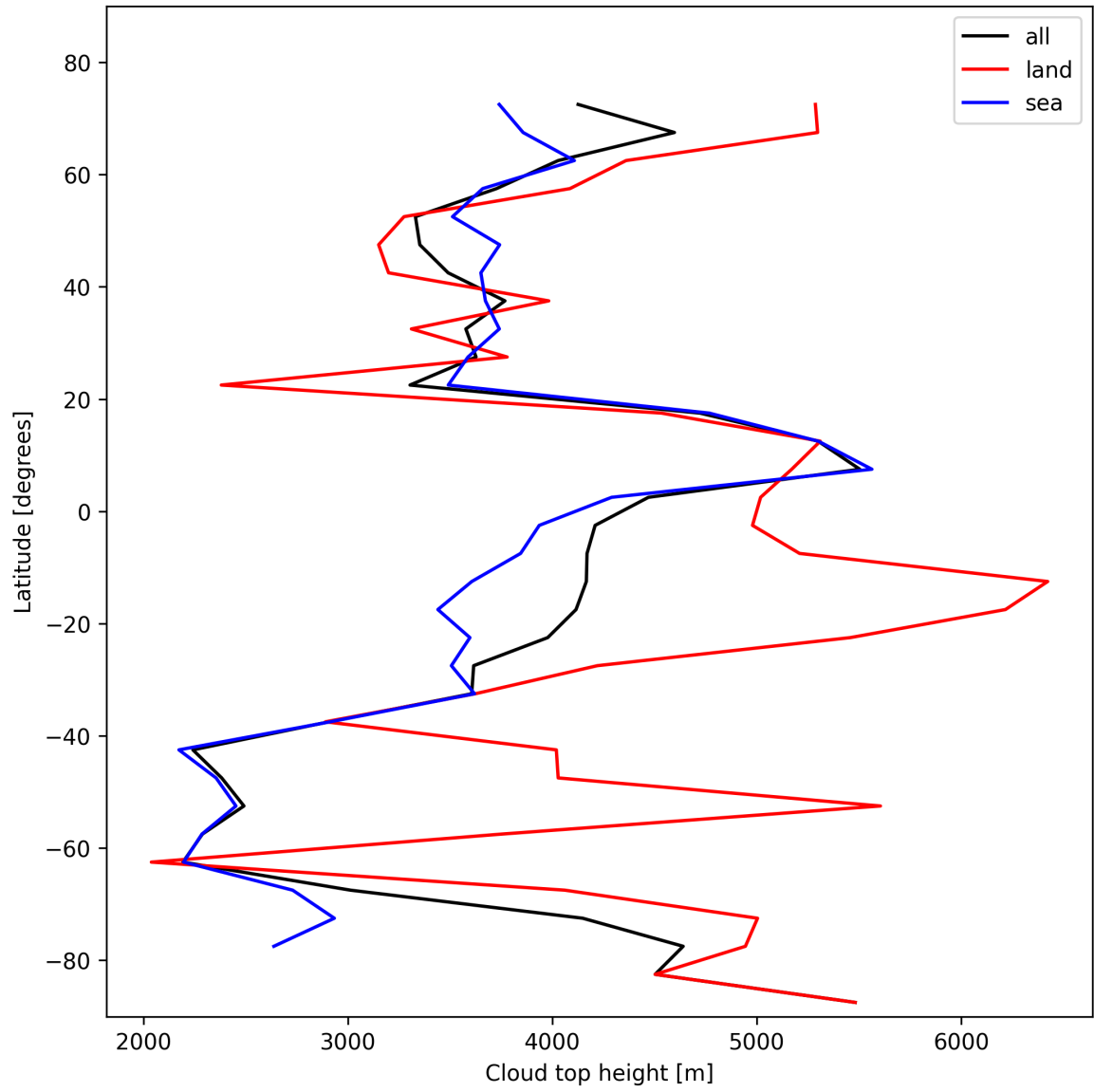
Figure 24: Zonal average of “Cloud top height” for 2025-11-07 to 2025-11-09.
