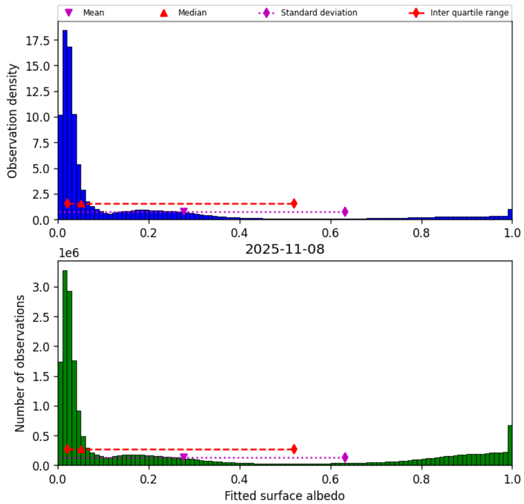
Figure 45: Histogram of “Fitted surface albedo” for 2025-11-07 to 2025-11-09
