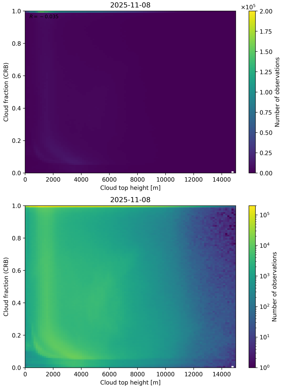
Figure 88: Scatter density plot of “Cloud top height” against “Cloud fraction (CRB)” for 2025-11-07 to 2025-11-09.
