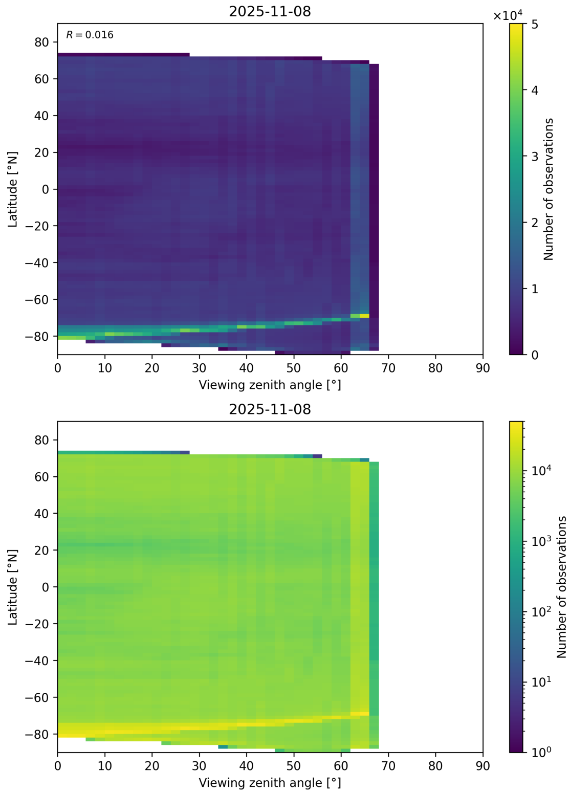
Figure 113: Scatter density plot of “Viewing zenith angle” against “Latitude” for 2025-11-07 to 2025-11-09.
