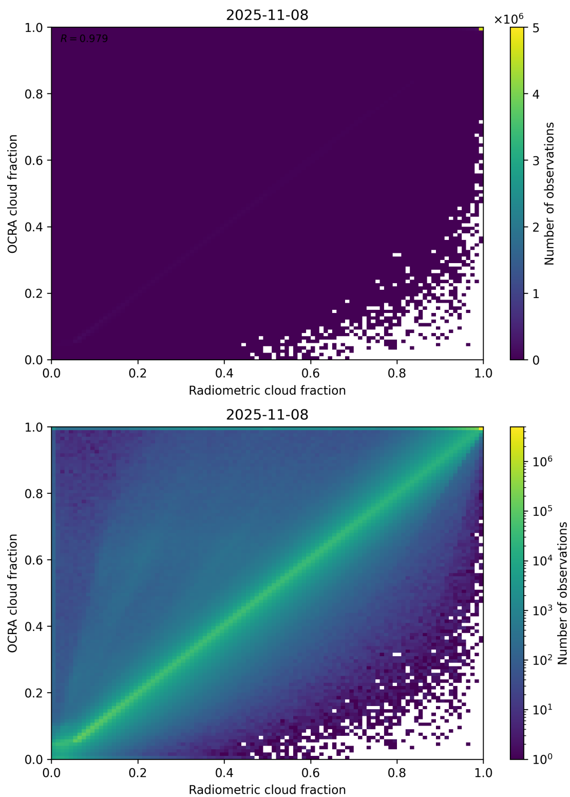
Figure 72: Scatter density plot of “Radiometric cloud fraction” against “OCRA cloud fraction” for 2025-11-07 to 2025-11-09.
