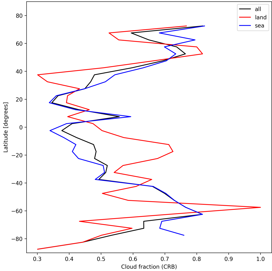
Figure 26: Zonal average of “Cloud fraction (CRB)” for 2025-11-07 to 2025-11-09.
