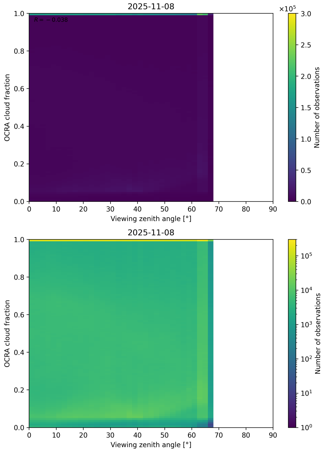
Figure 108: Scatter density plot of “Viewing zenith angle” against “OCRA cloud fraction” for 2025-11-07 to 2025-11-09.
