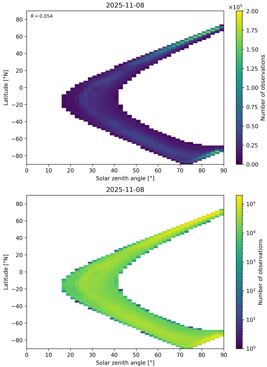
Figure 105: Scatter density plot of “Solar zenith angle” against “Latitude” for 2025-11-07 to 2025-11-09.
