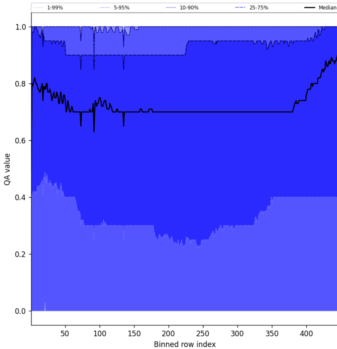
Figure 54: Along track statistics of “QA value” for 2025-11-07 to 2025-11-09
