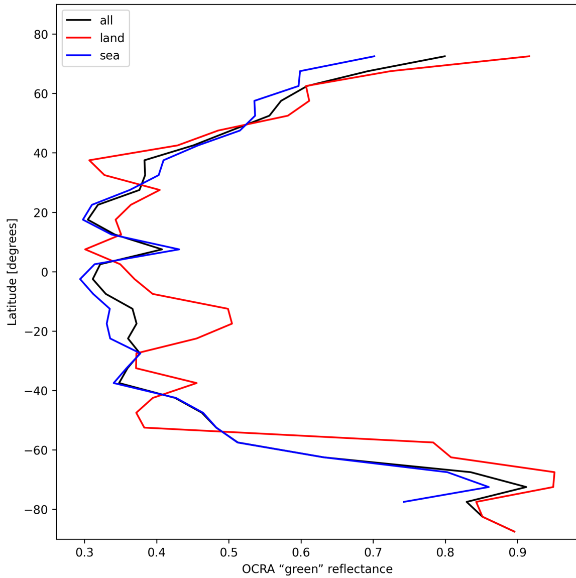
Figure 36: Zonal average of “OCRA “green” reflectance” for 2025-11-07 to 2025-11-09.
