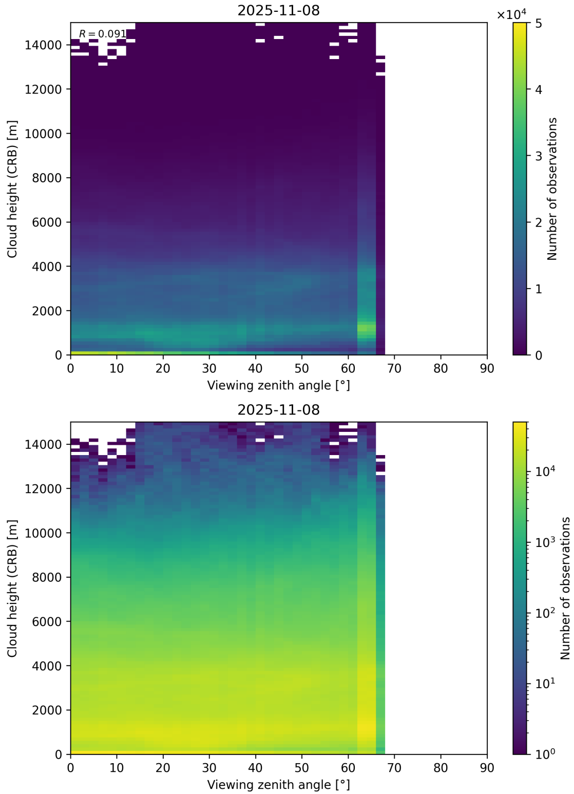
Figure 110: Scatter density plot of “Viewing zenith angle” against “Cloud height (CRB)” for 2025-11-07 to 2025-11-09.
