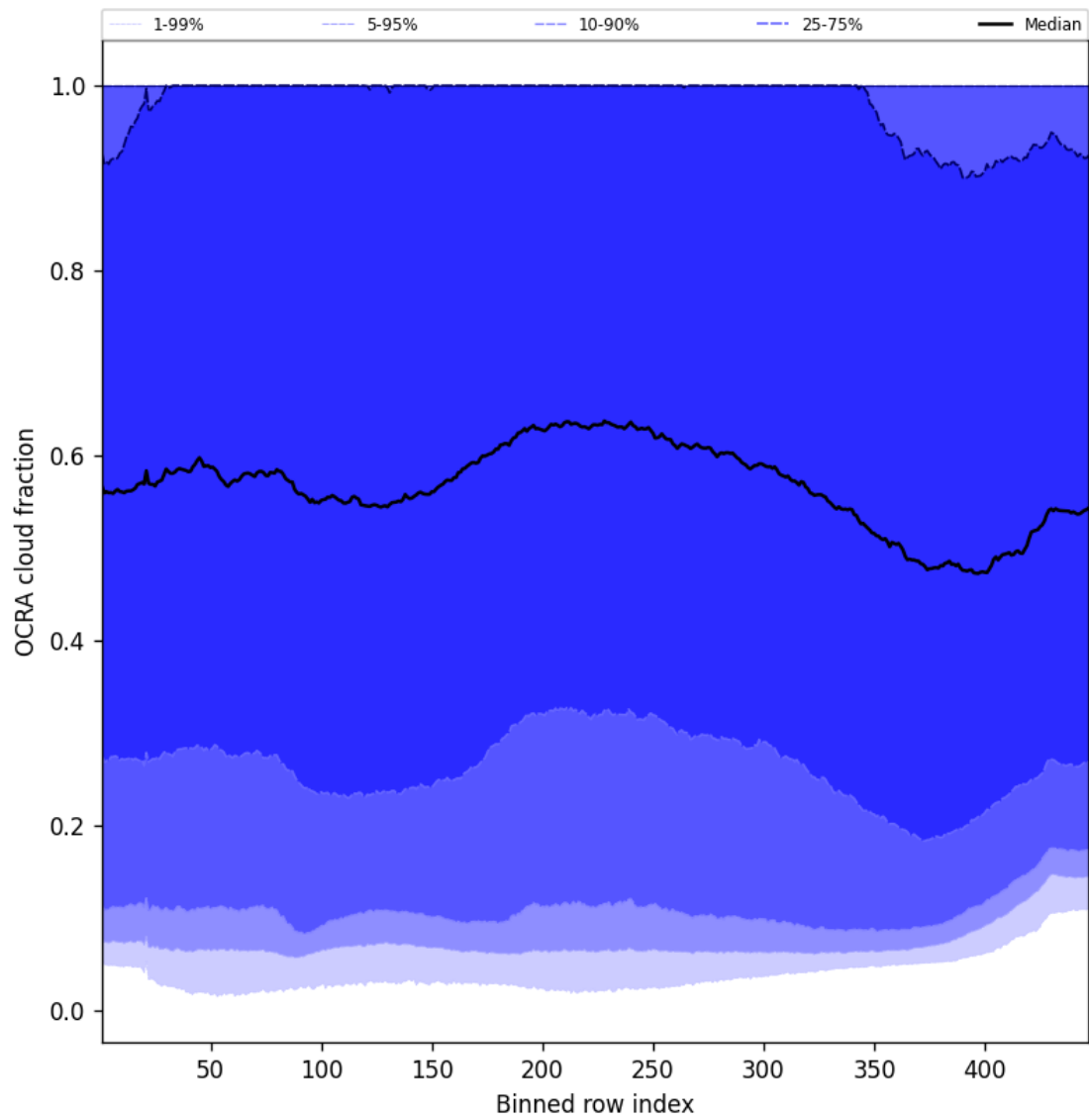
Figure 66: Along track statistics of “OCRA cloud fraction” for 2025-11-07 to 2025-11-09
