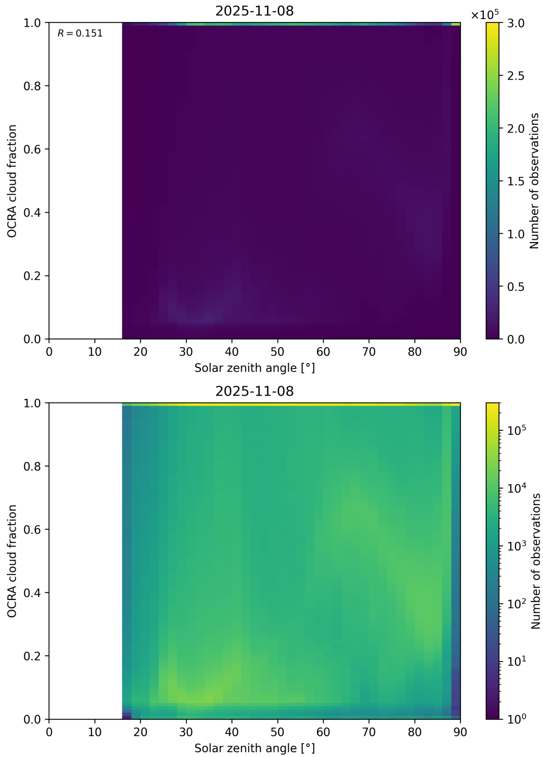
Figure 100: Scatter density plot of “Solar zenith angle” against “OCRA cloud fraction” for 2025-11-07 to 2025-11-09.
