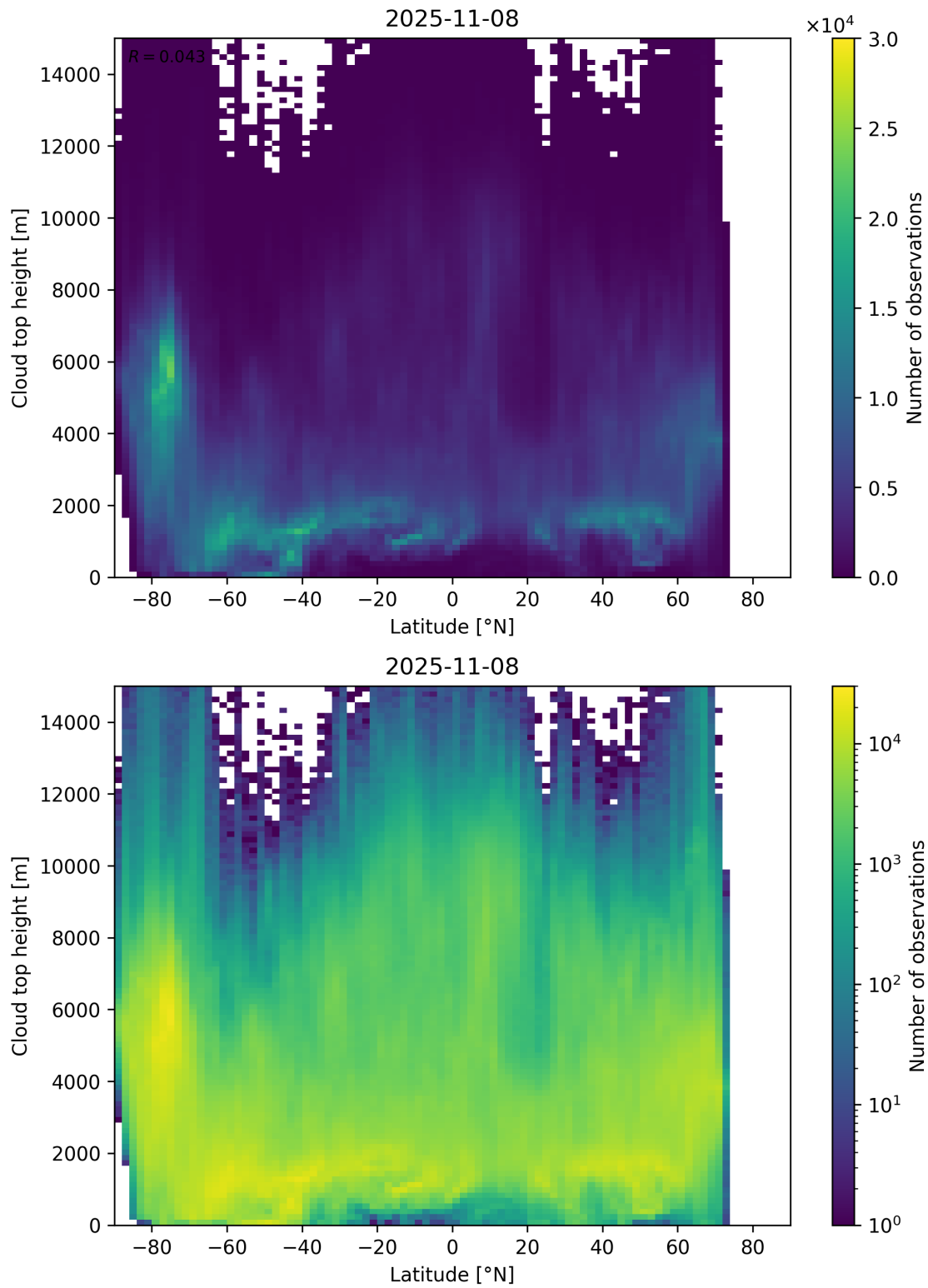
Figure 97: Scatter density plot of “Latitude” against “Cloud top height” for 2025-11-07 to 2025-11-09.
