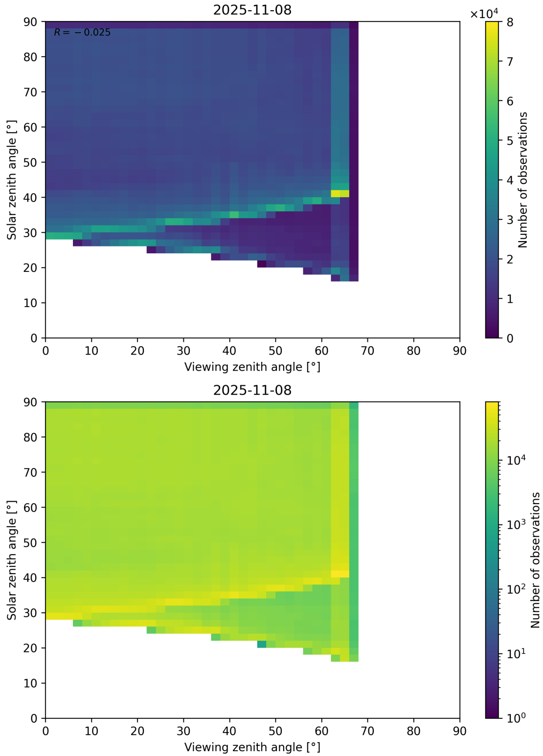
Figure 114: Scatter density plot of “Viewing zenith angle” against “Solar zenith angle” for 2025-11-07 to 2025-11-09.
