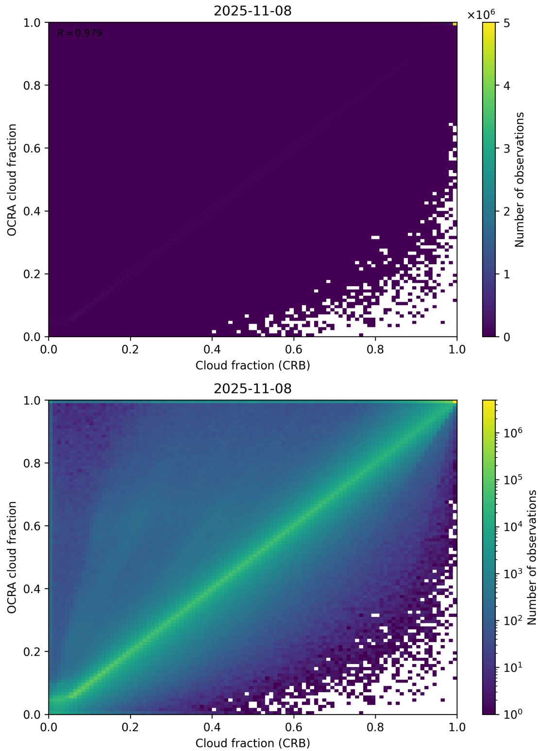
Figure 78: Scatter density plot of “Cloud fraction (CRB)” against “OCRA cloud fraction” for 2025-11-07 to 2025-11-09.
