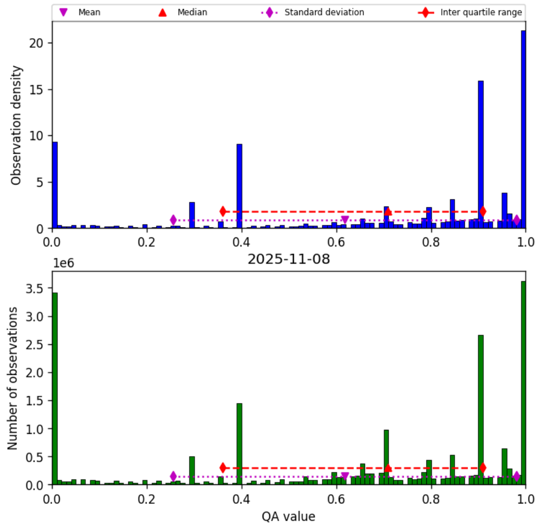
Figure 38: Histogram of “QA value” for 2025-11-07 to 2025-11-09
