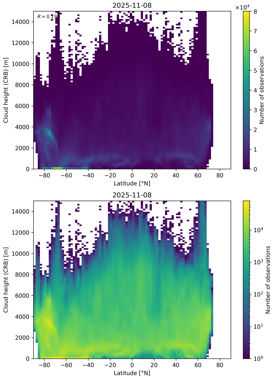
Figure 95: Scatter density plot of “Latitude” against “Cloud height (CRB)” for 2025-11-07 to 2025-11-09.
