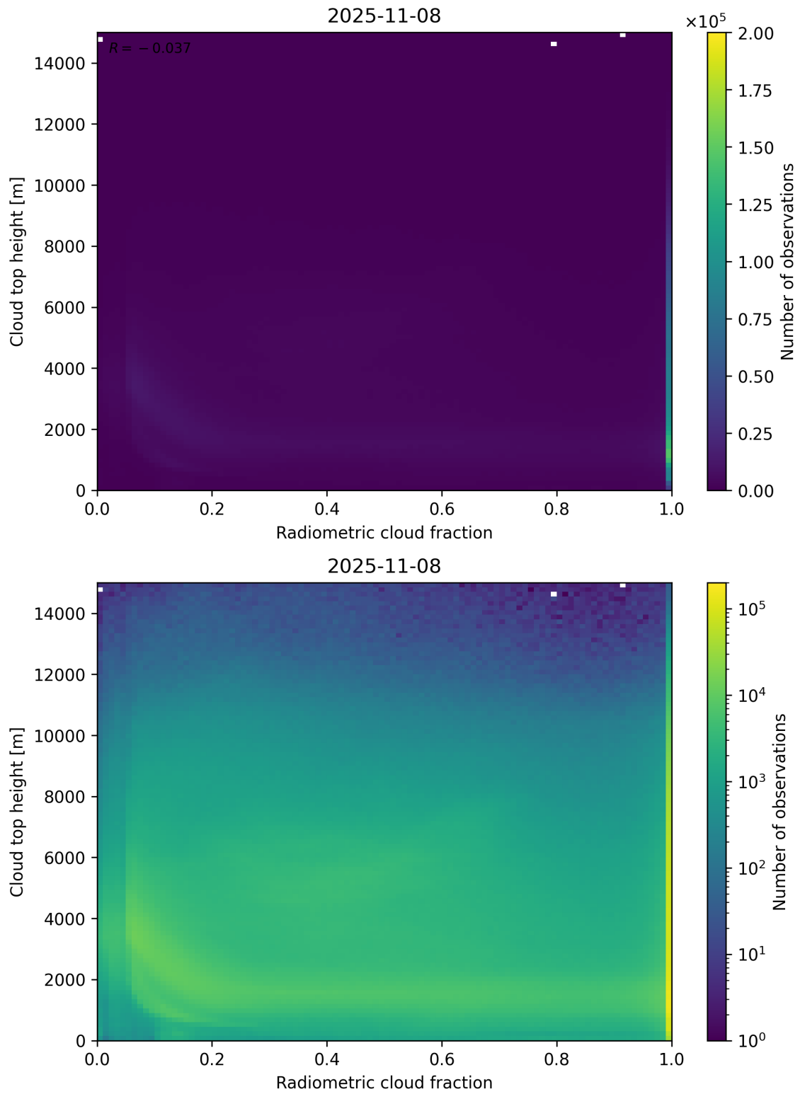
Figure 76: Scatter density plot of “Radiometric cloud fraction” against “Cloud top height” for 2025-11-07 to 2025-11-09.
