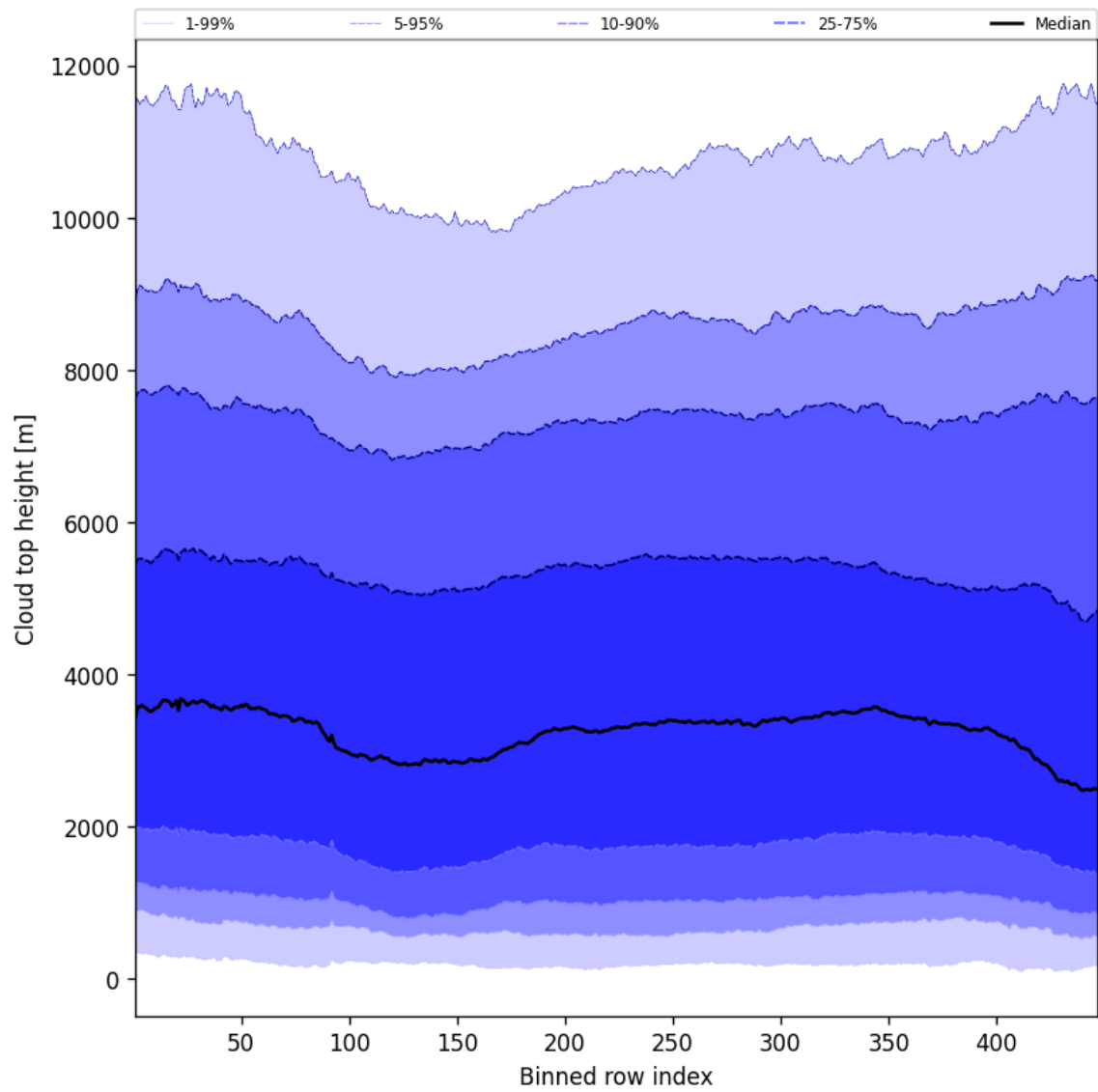
Figure 56: Along track statistics of “Cloud top height” for 2025-11-07 to 2025-11-09
