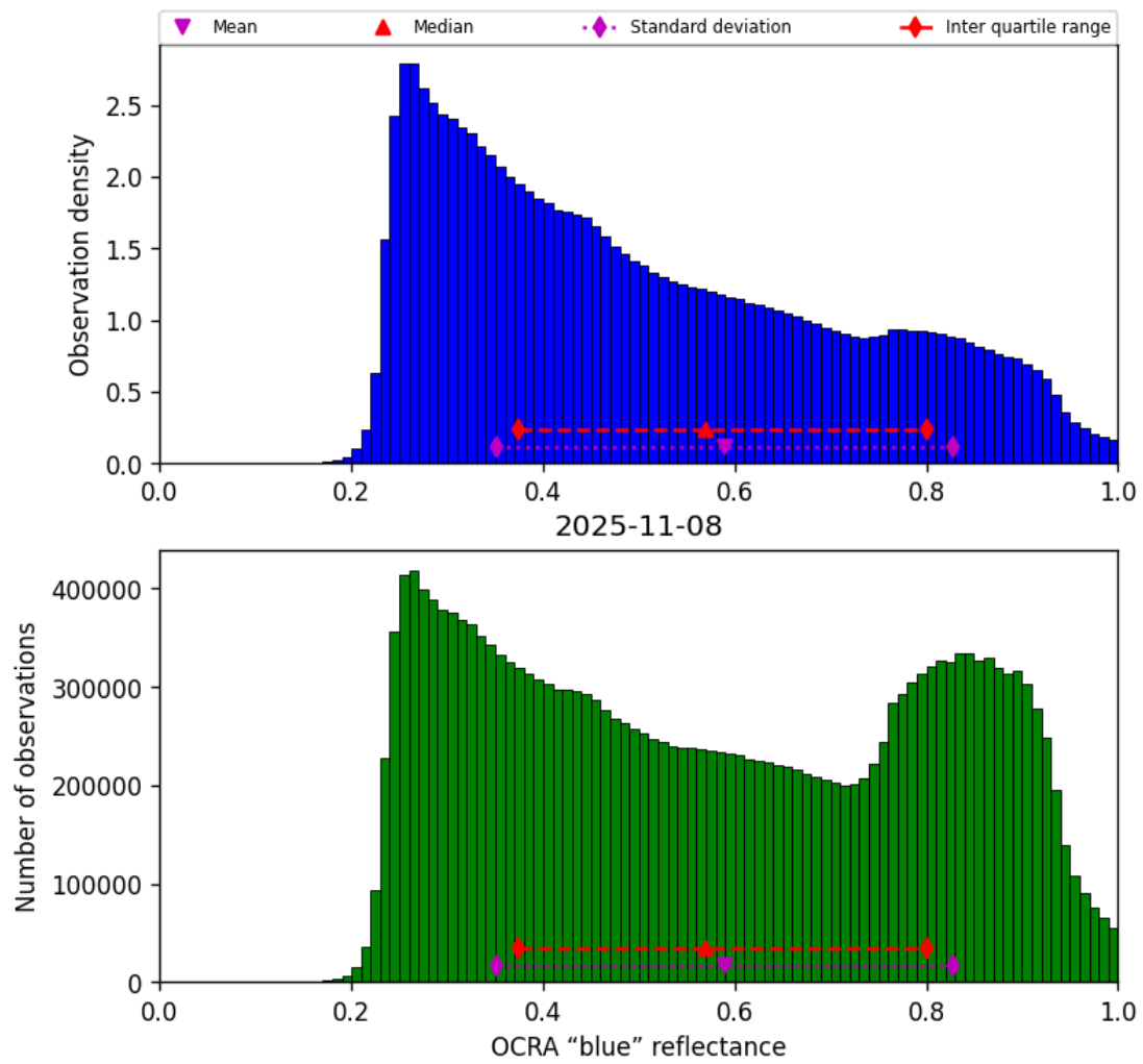
Figure 51: Histogram of “OCRA “blue” reflectance” for 2025-11-07 to 2025-11-09
