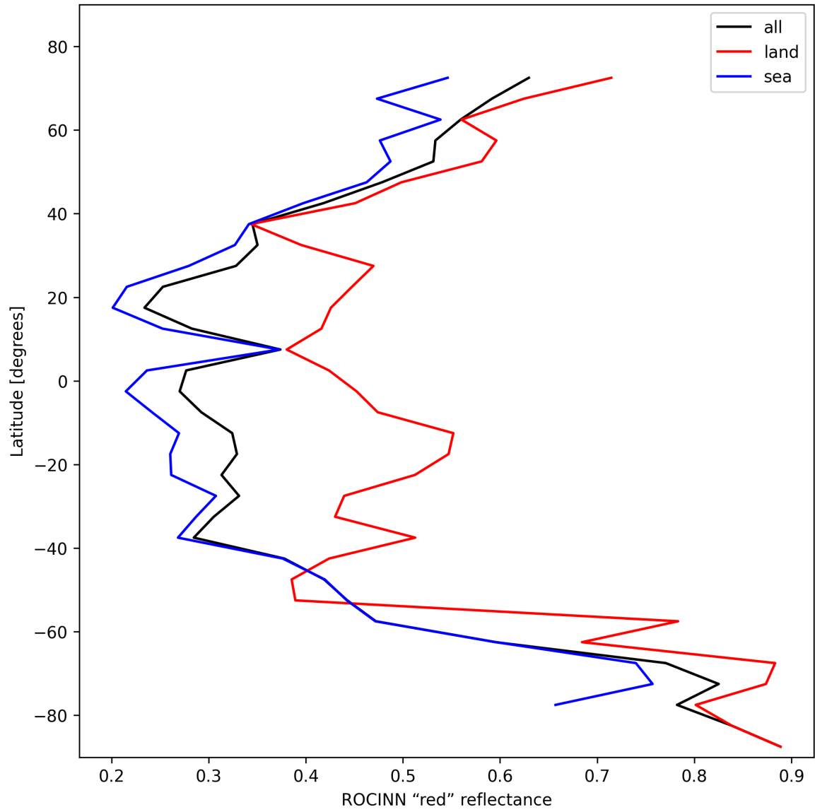
Figure 37: Zonal average of “ROCINN “red” reflectance” for 2025-11-07 to 2025-11-09.
