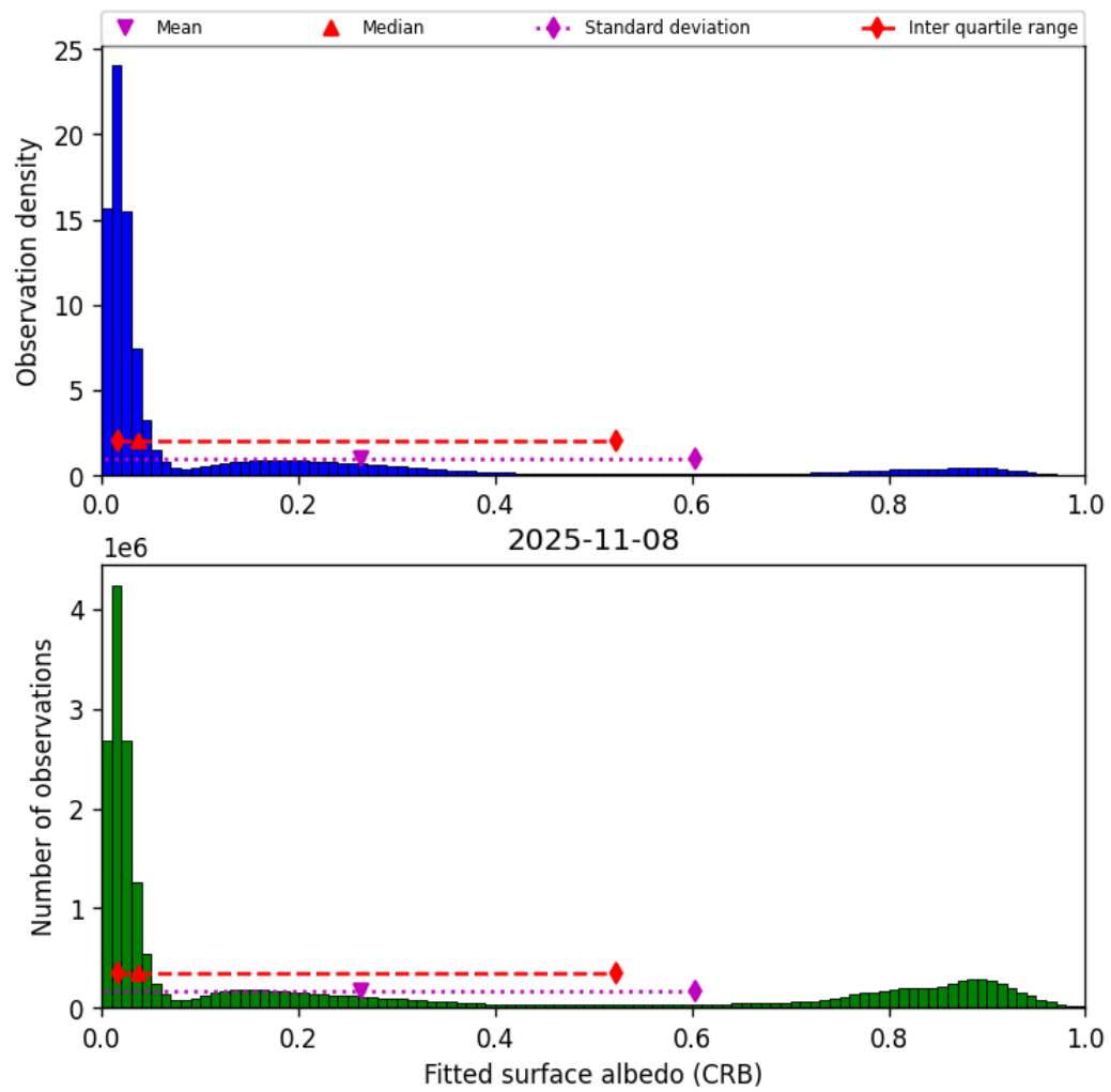
Figure 46: Histogram of “Fitted surface albedo (CRB)” for 2025-11-07 to 2025-11-09
