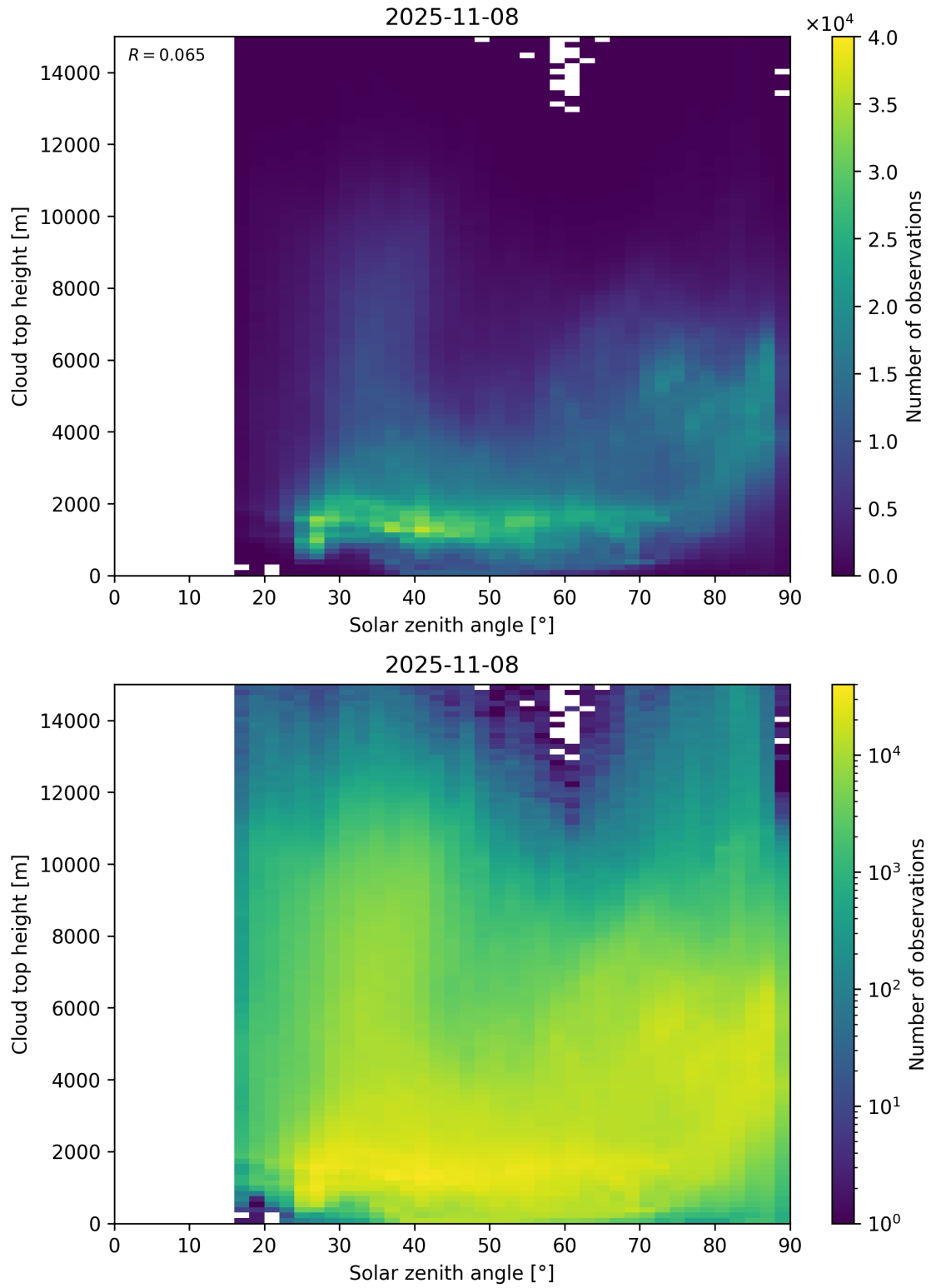
Figure 104: Scatter density plot of “Solar zenith angle” against “Cloud top height” for 2025-11-07 to 2025-11-09.
