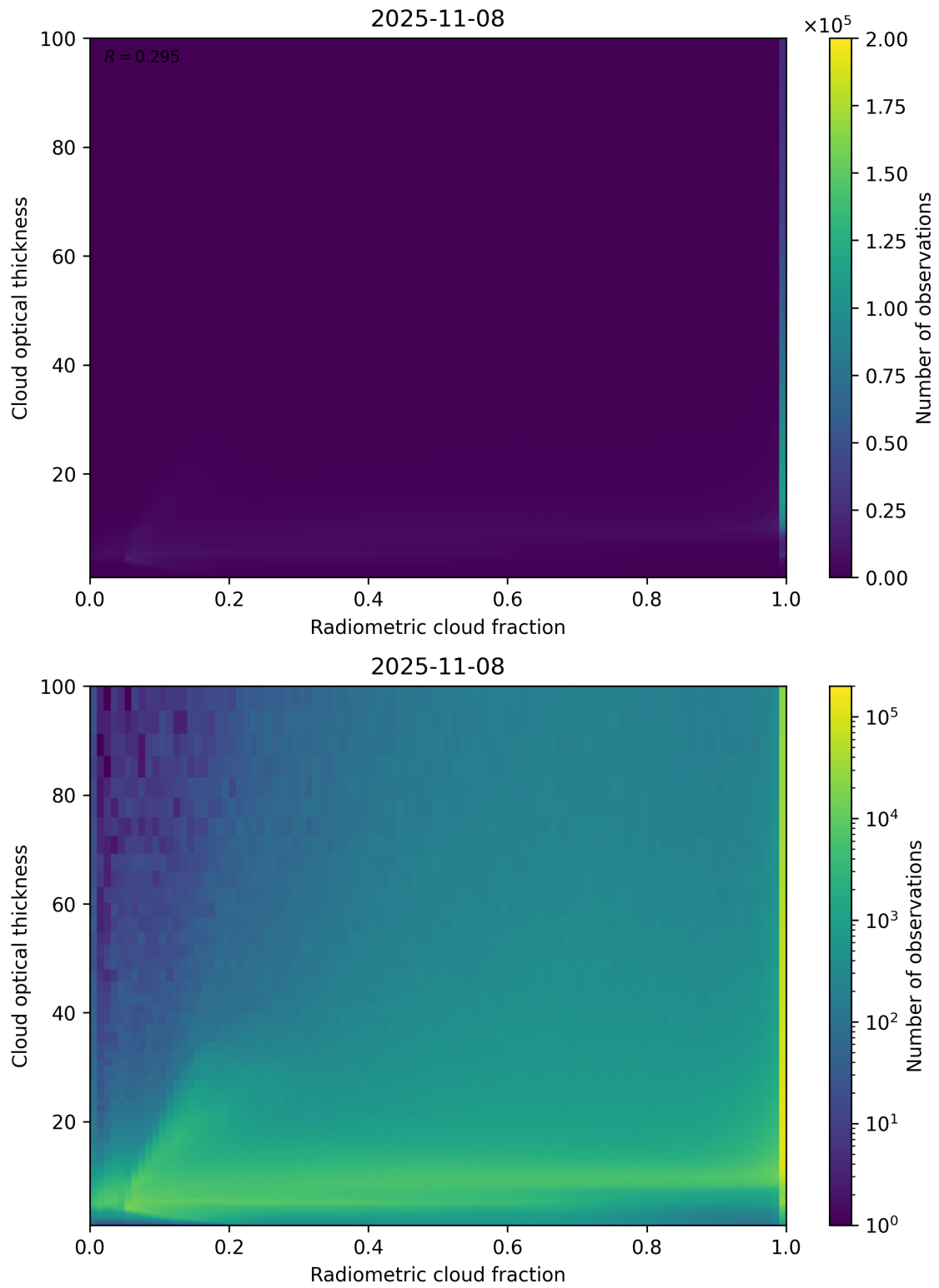
Figure 75: Scatter density plot of “Radiometric cloud fraction” against “Cloud optical thickness” for 2025-11-07 to 2025-11-09.
