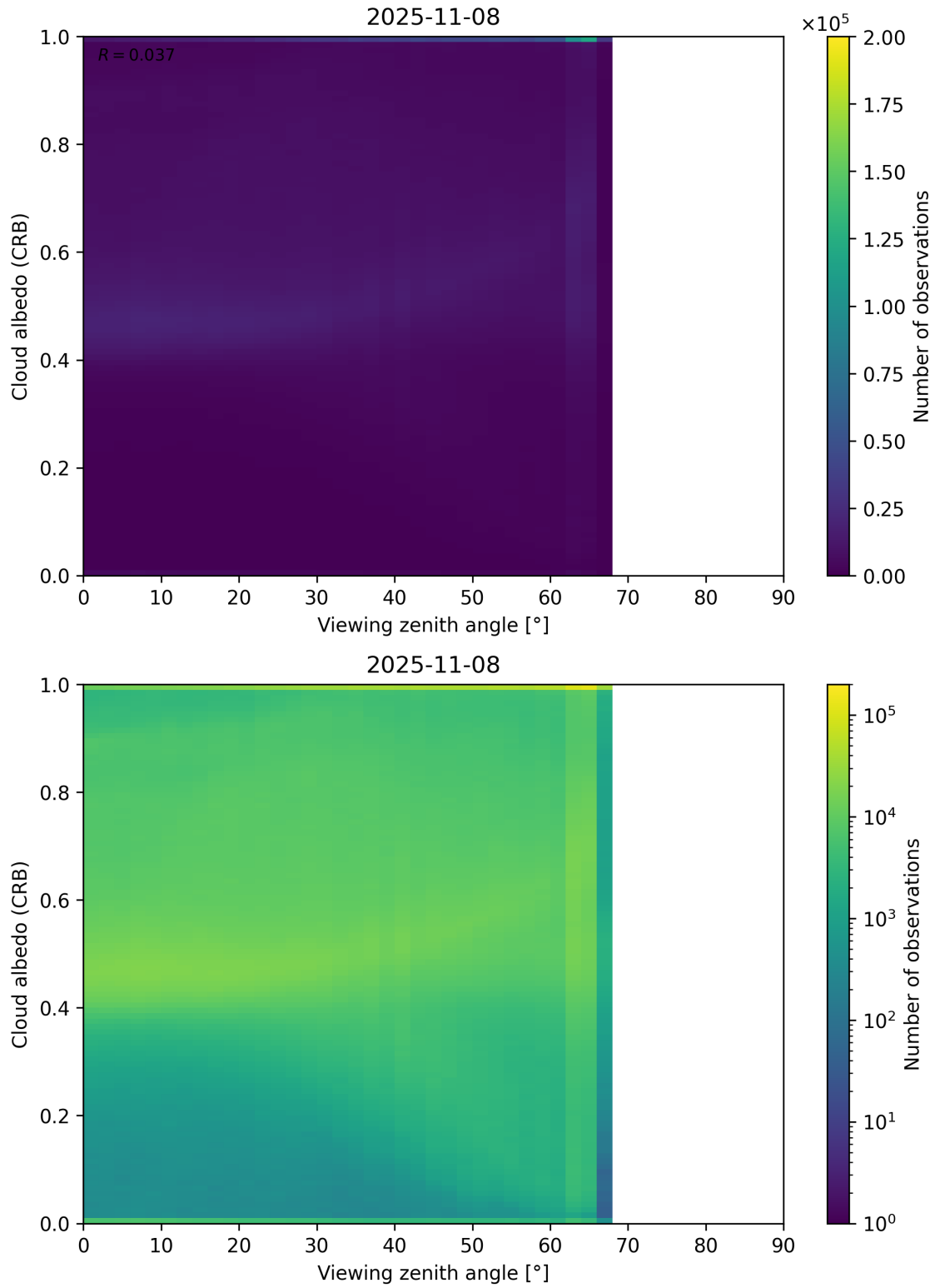
Figure 106: Scatter density plot of “Viewing zenith angle” against “Cloud albedo (CRB)” for 2025-11-07 to 2025-11-09.
