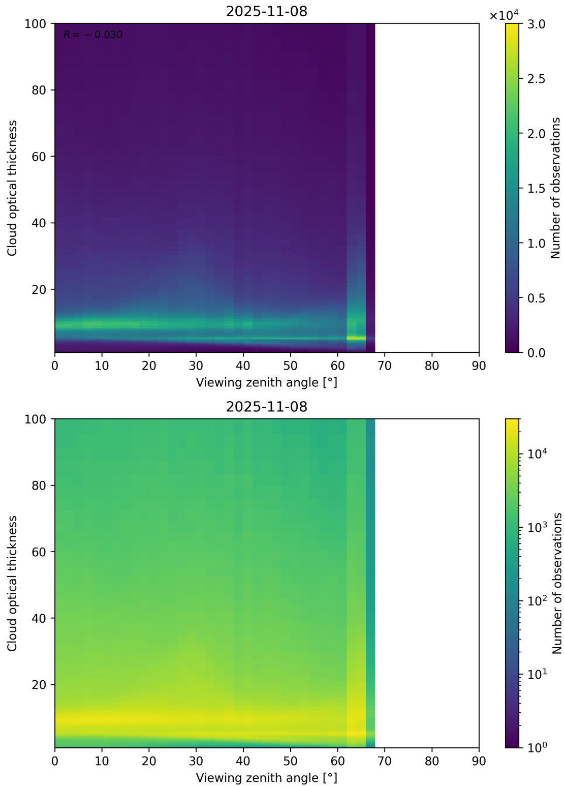
Figure 111: Scatter density plot of “Viewing zenith angle” against “Cloud optical thickness” for 2025-11-07 to 2025-11-09.
