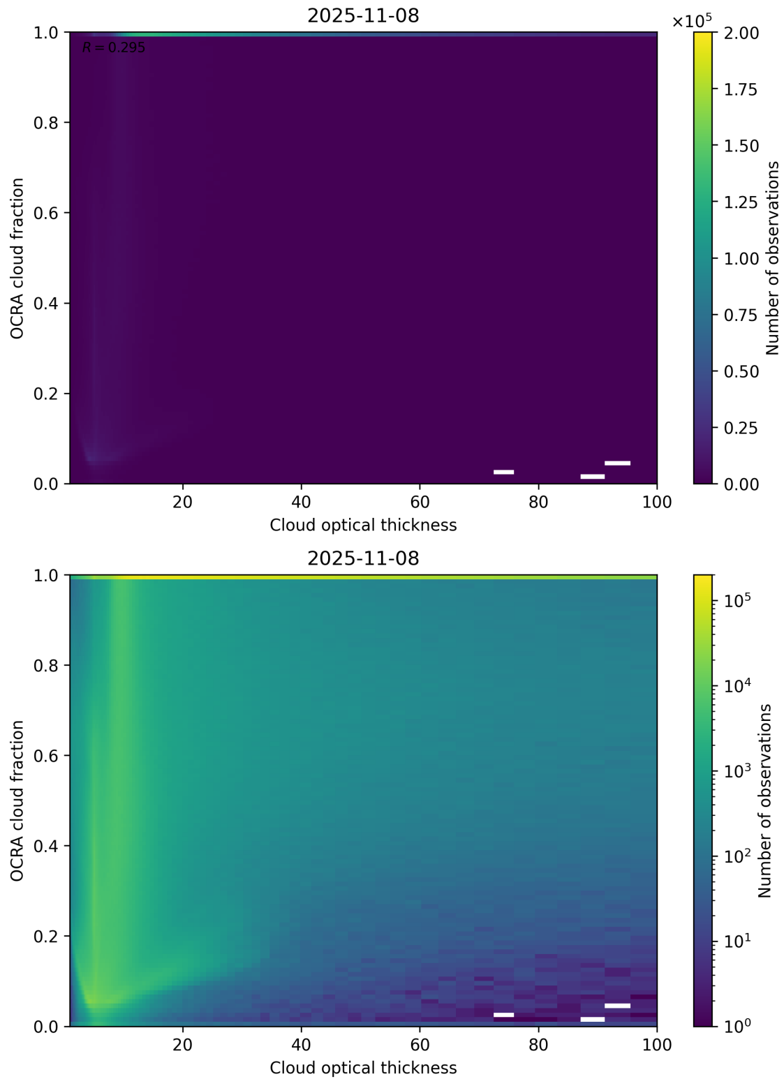
Figure 83: Scatter density plot of “Cloud optical thickness” against “OCRA cloud fraction” for 2025-11-07 to 2025-11-09.
