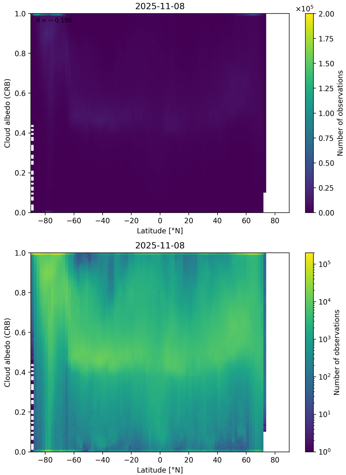
Figure 91: Scatter density plot of “Latitude” against “Cloud albedo (CRB)” for 2025-11-07 to 2025-11-09.
