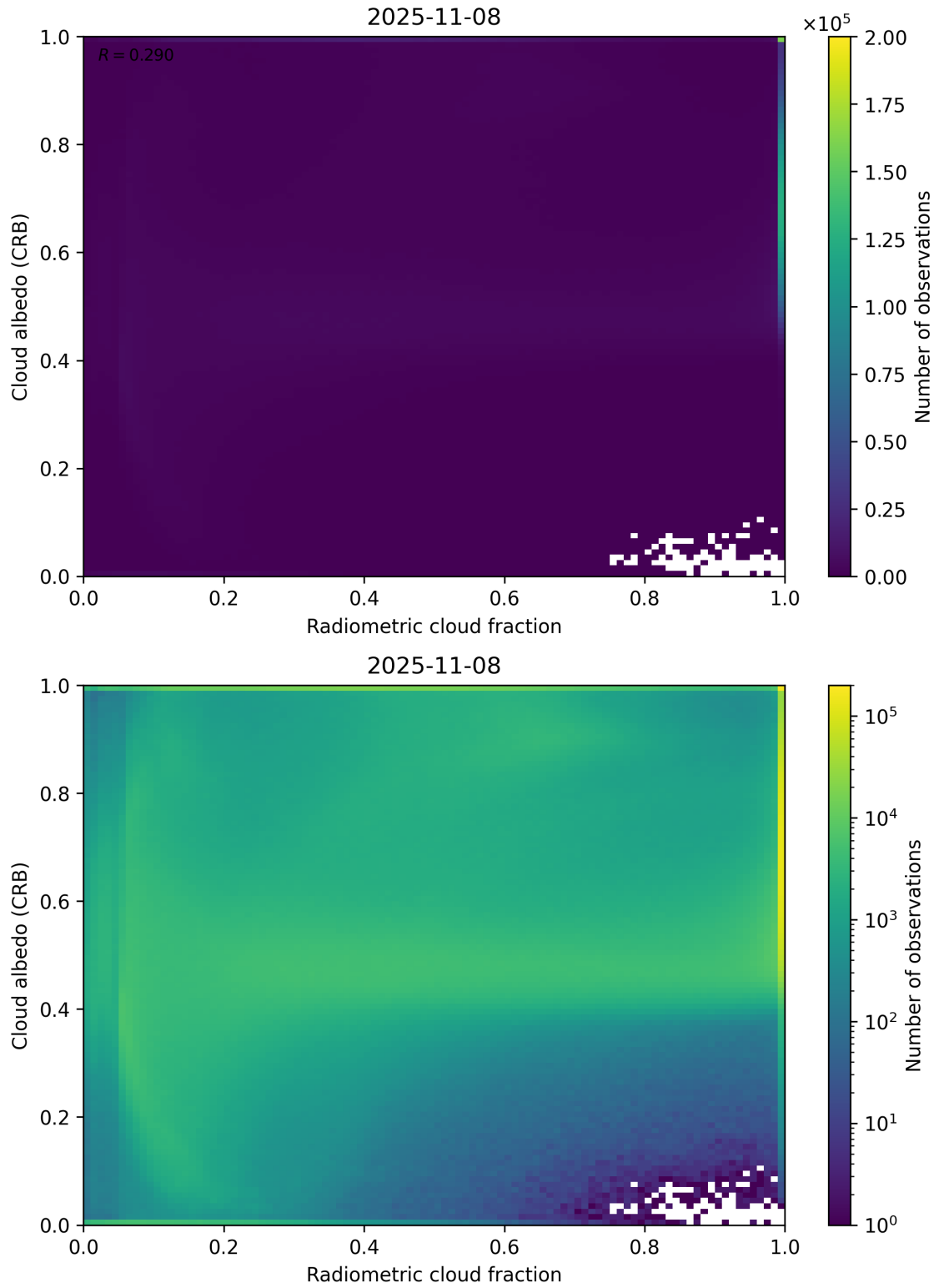
Figure 71: Scatter density plot of “Radiometric cloud fraction” against “Cloud albedo (CRB)” for 2025-11-07 to 2025-11-09.
