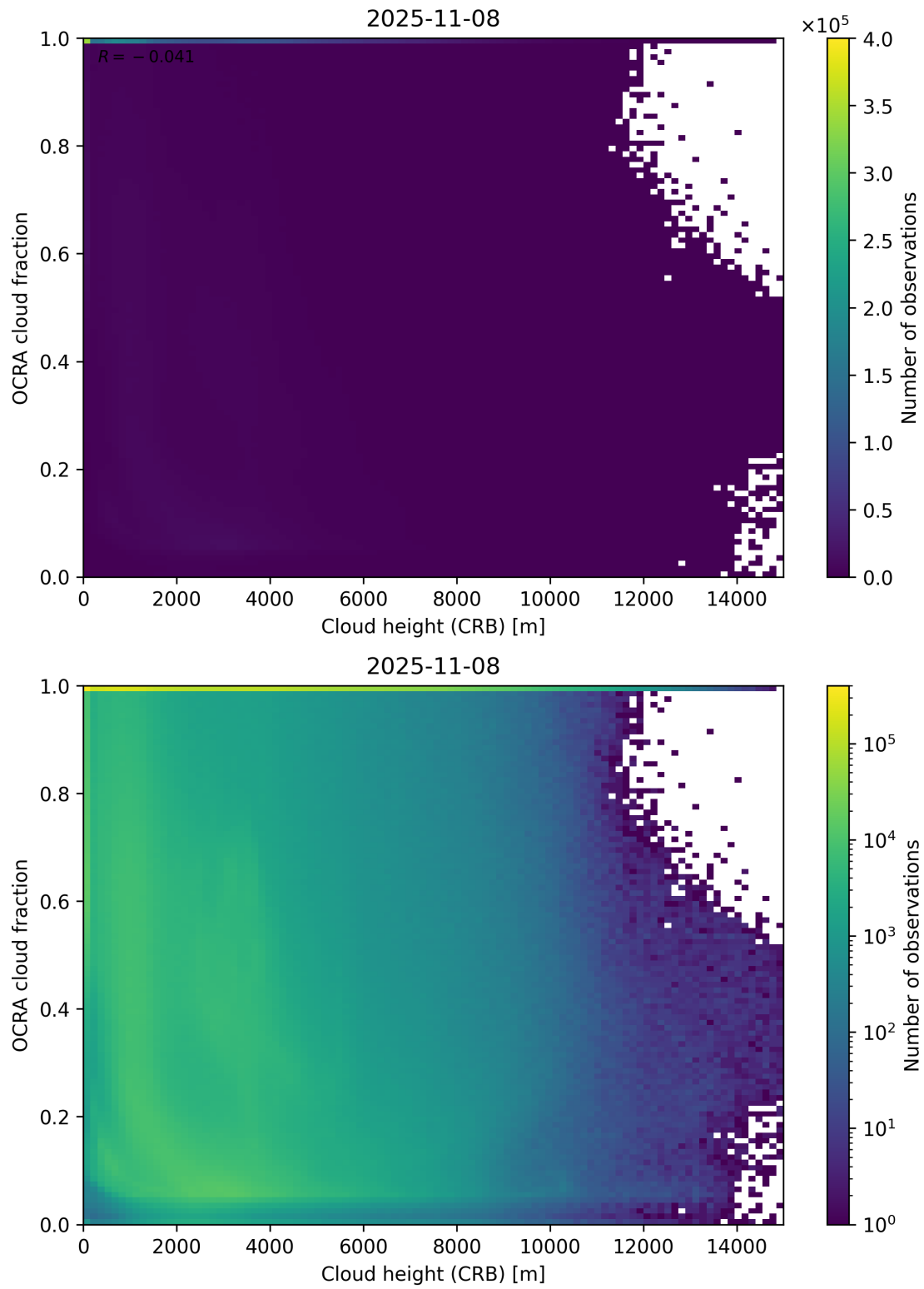
Figure 81: Scatter density plot of “Cloud height (CRB)” against “OCRA cloud fraction” for 2025-11-07 to 2025-11-09.
