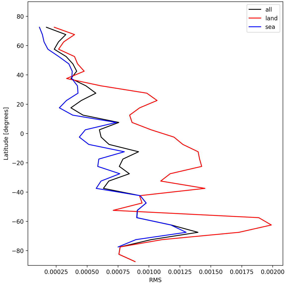
Figure 31: Zonal average of “RMS” for 2025-11-07 to 2025-11-09.
