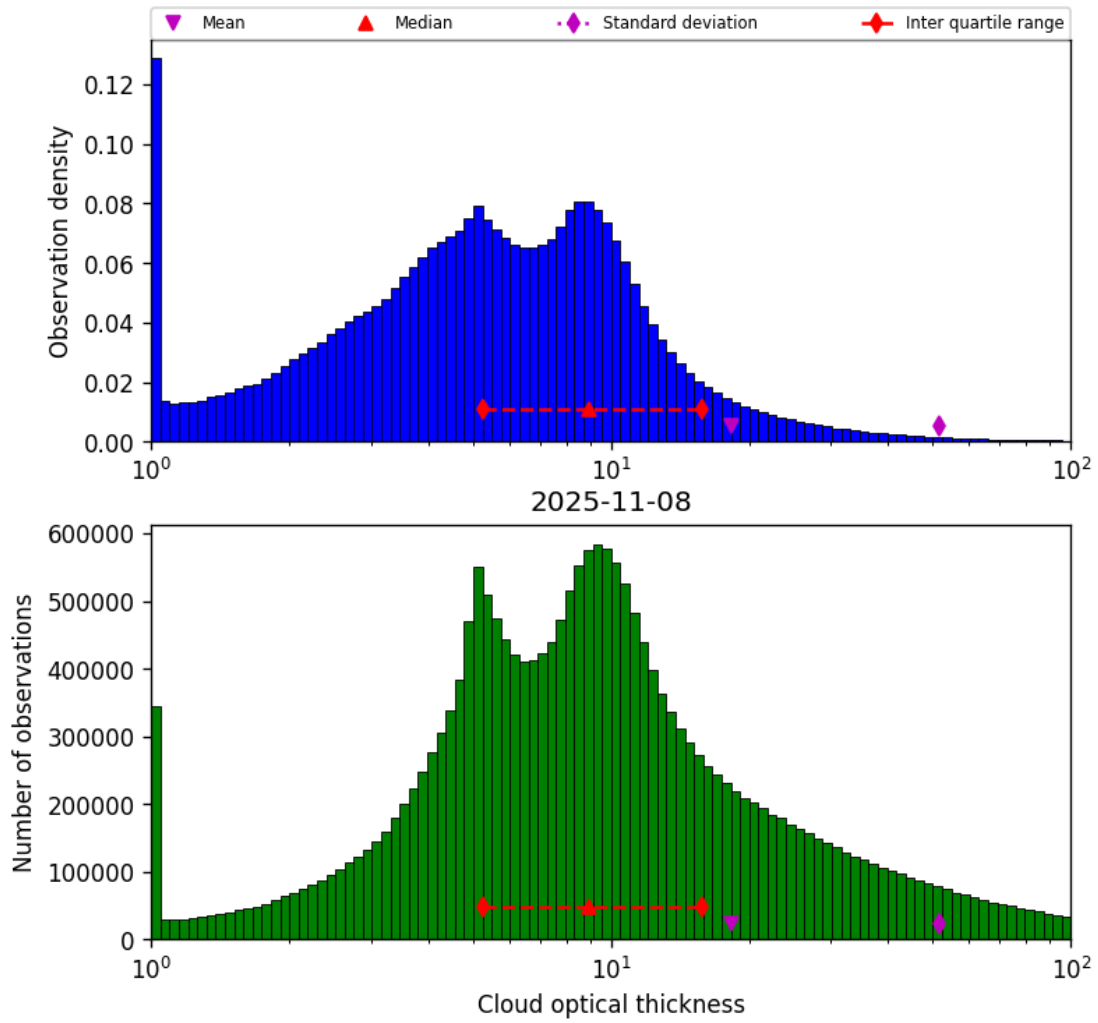
Figure 41: Histogram of “Cloud optical thickness” for 2025-11-07 to 2025-11-09
