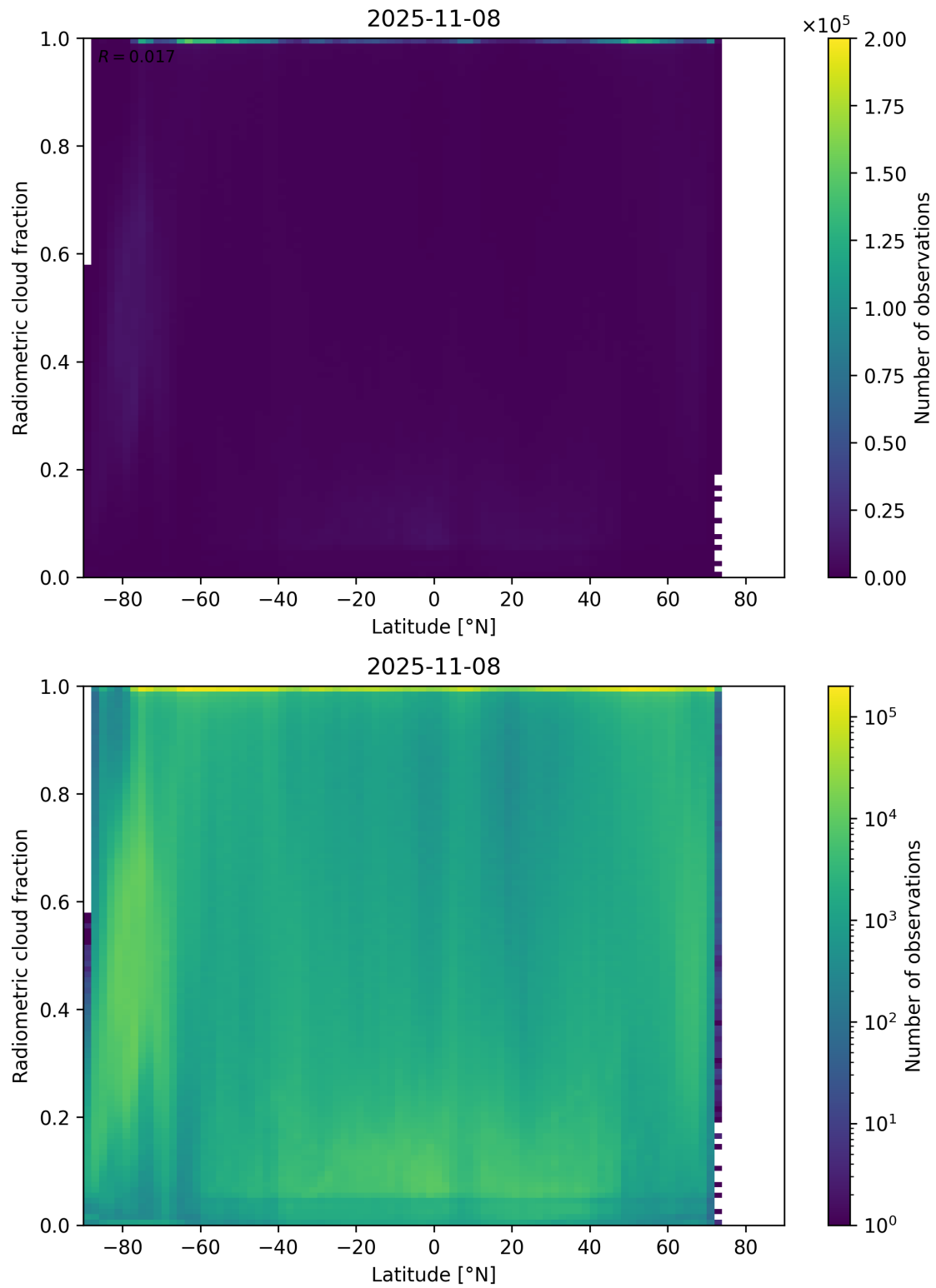
Figure 92: Scatter density plot of “Latitude” against “Radiometric cloud fraction” for 2025-11-07 to 2025-11-09.
