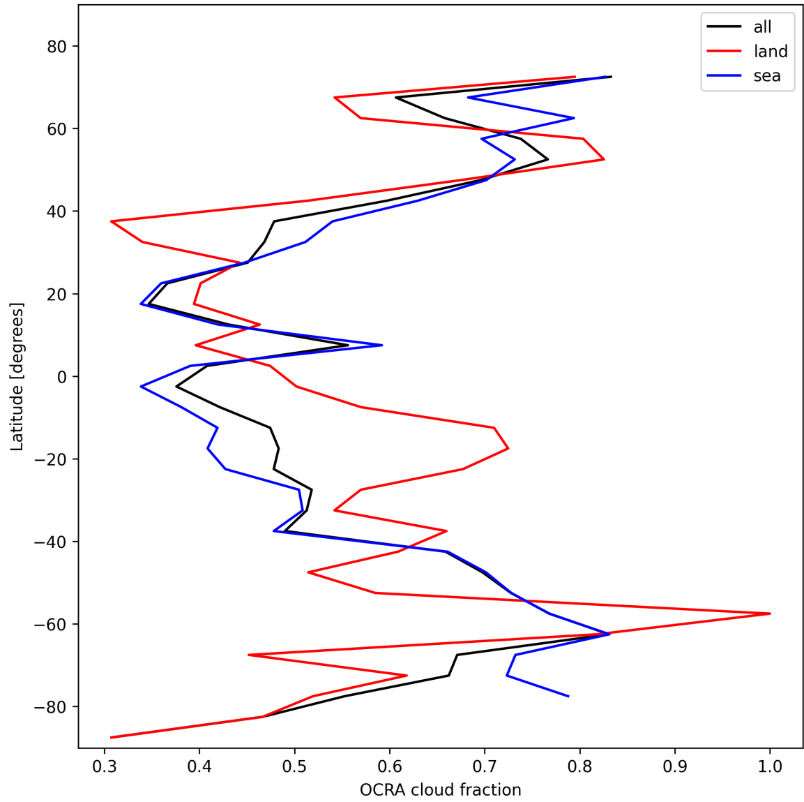
Figure 34: Zonal average of “OCRA cloud fraction” for 2025-11-07 to 2025-11-09.
