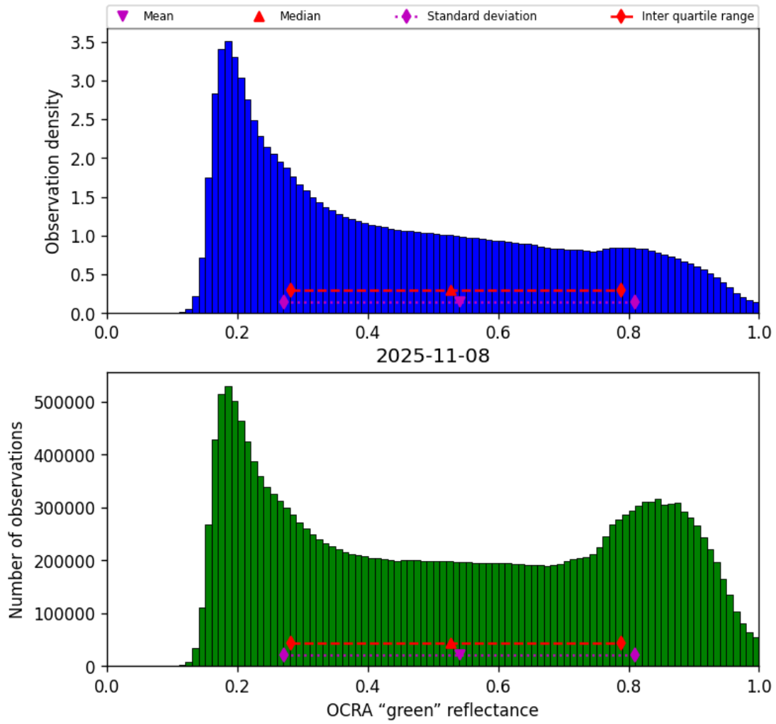
Figure 52: Histogram of “OCRA “green” reflectance” for 2025-11-07 to 2025-11-09
