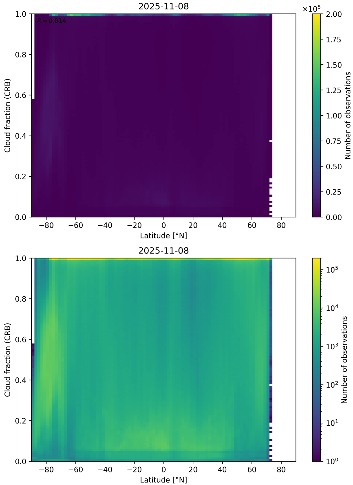
Figure 94: Scatter density plot of “Latitude” against “Cloud fraction (CRB)” for 2025-11-07 to 2025-11-09.
