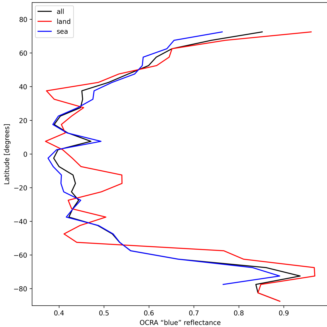
Figure 35: Zonal average of “OCRA “blue” reflectance” for 2025-11-07 to 2025-11-09.
