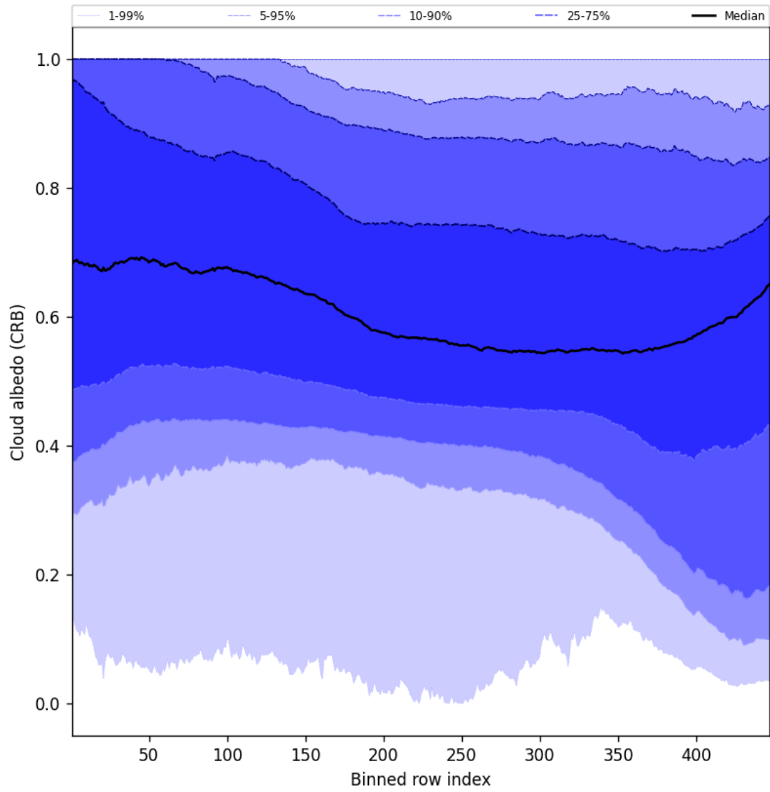
Figure 60: Along track statistics of “Cloud albedo (CRB)” for 2025-11-07 to 2025-11-09
