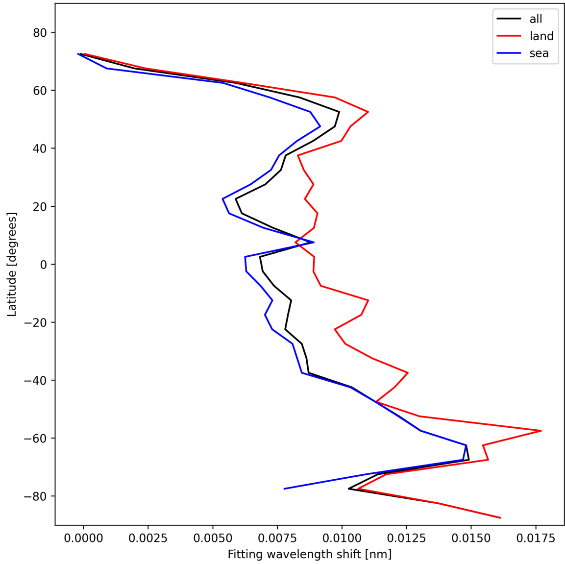
Figure 33: Zonal average of “Fitting wavelength shift” for 2025-11-07 to 2025-11-09.
