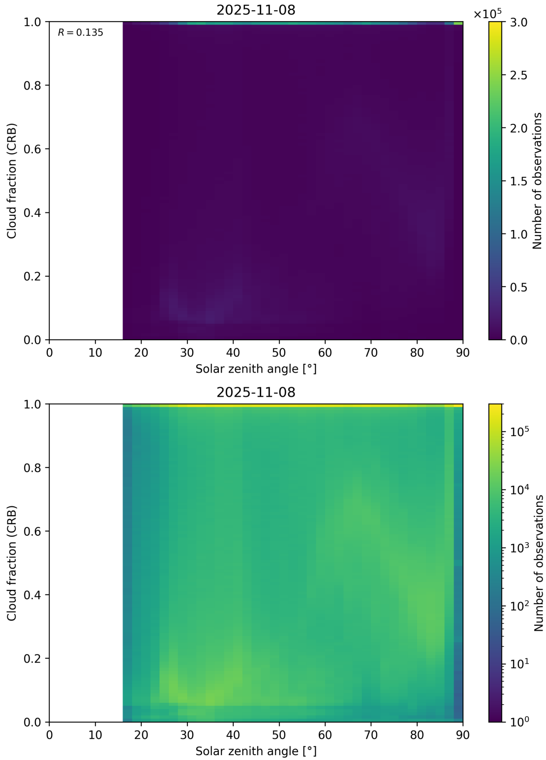
Figure 101: Scatter density plot of “Solar zenith angle” against “Cloud fraction (CRB)” for 2025-11-07 to 2025-11-09.
