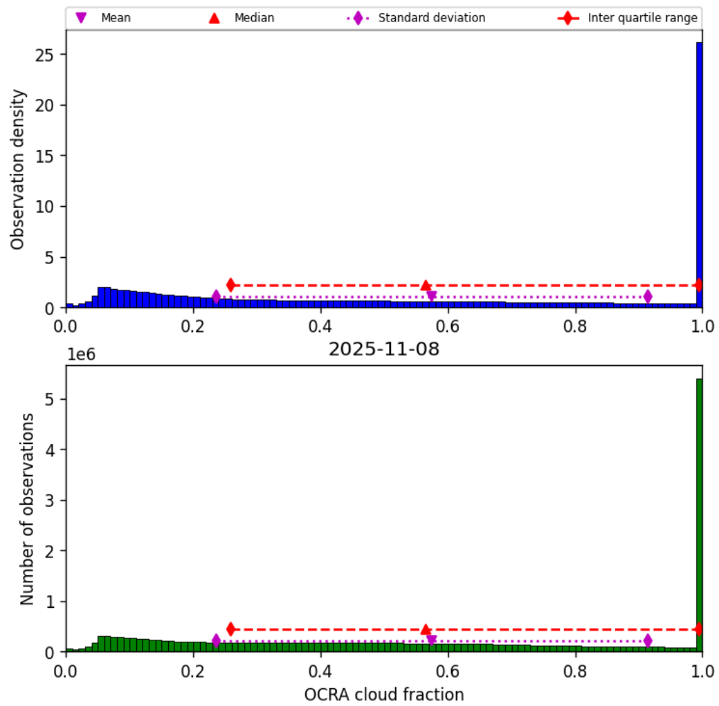
Figure 50: Histogram of “OCRA cloud fraction” for 2025-11-07 to 2025-11-09
