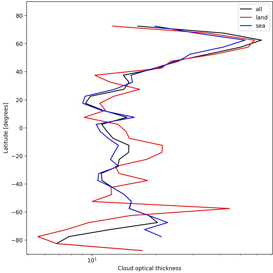
Figure 25: Zonal average of “Cloud optical thickness” for 2025-11-07 to 2025-11-09.
