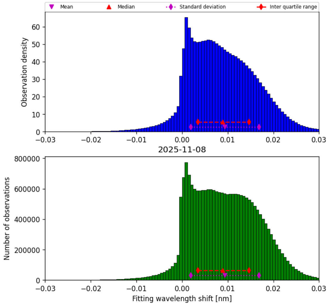
Figure 49: Histogram of “Fitting wavelength shift” for 2025-11-07 to 2025-11-09
