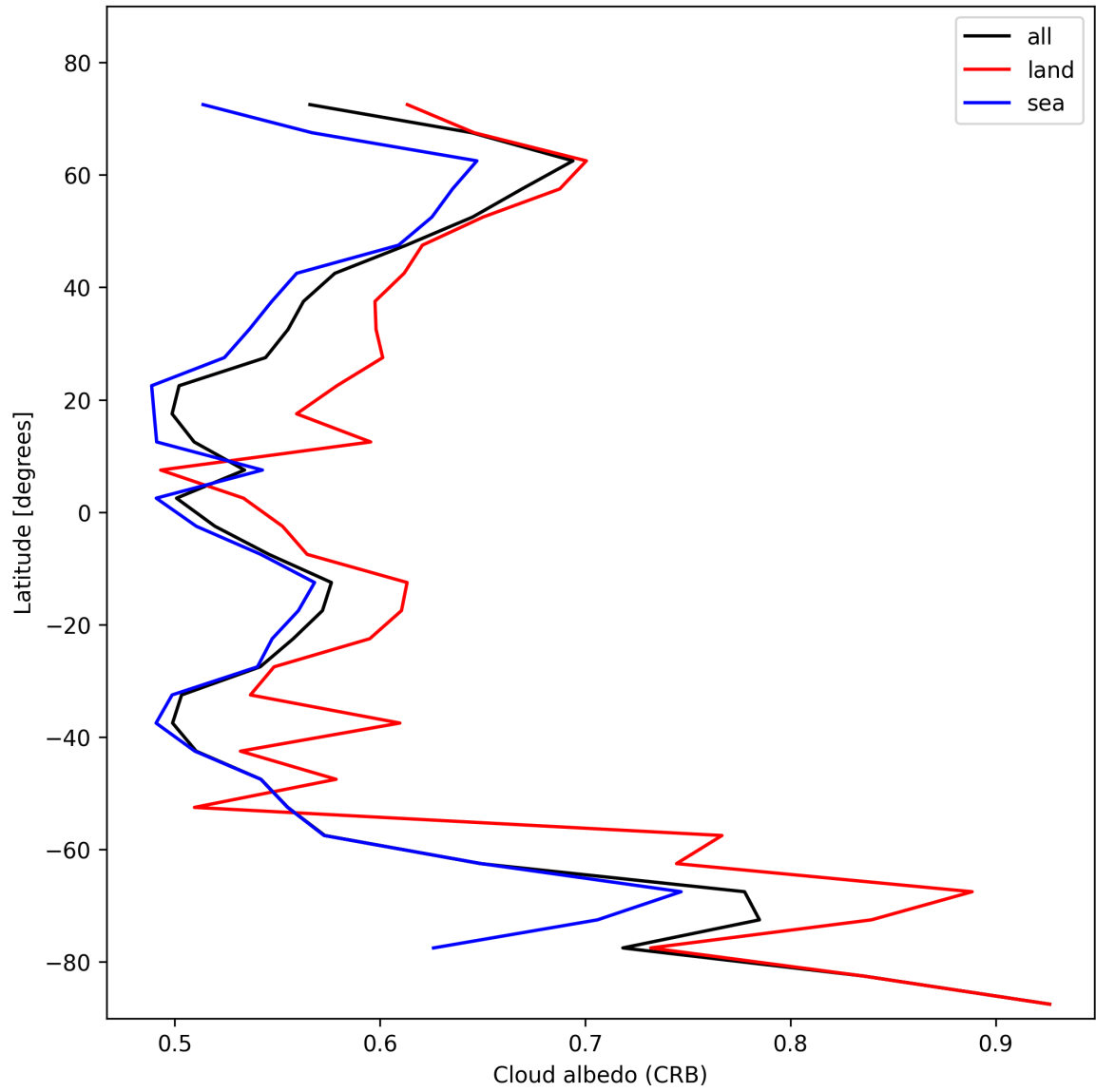
Figure 28: Zonal average of “Cloud albedo (CRB)” for 2025-11-07 to 2025-11-09.
