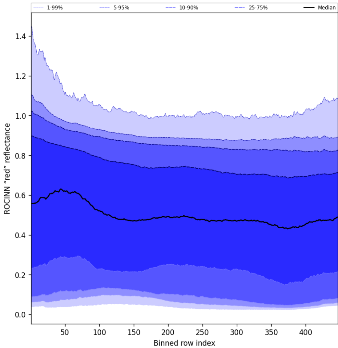
Figure 69: Along track statistics of “ROCINN “red” reflectance” for 2025-11-07 to 2025-11-09
