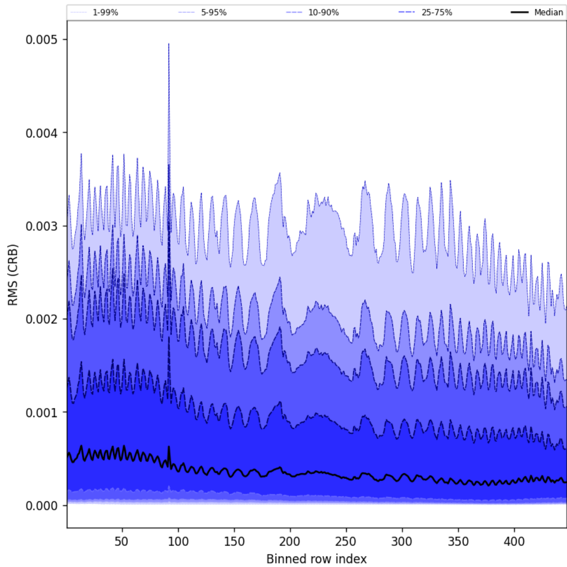
Figure 64: Along track statistics of “RMS (CRB)” for 2025-11-07 to 2025-11-09
