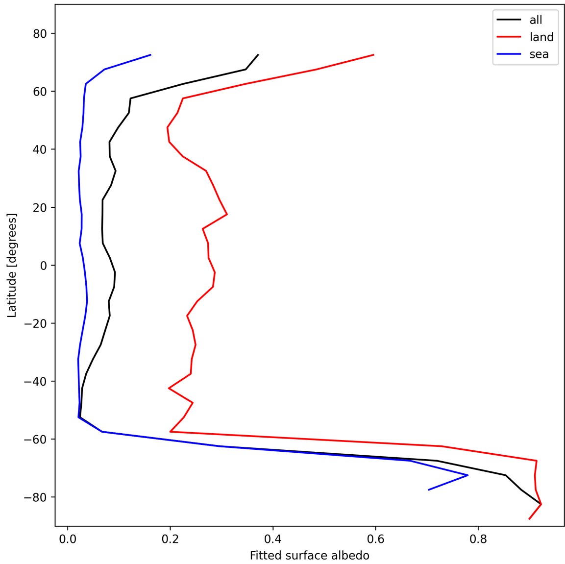
Figure 29: Zonal average of “Fitted surface albedo” for 2025-11-07 to 2025-11-09.
