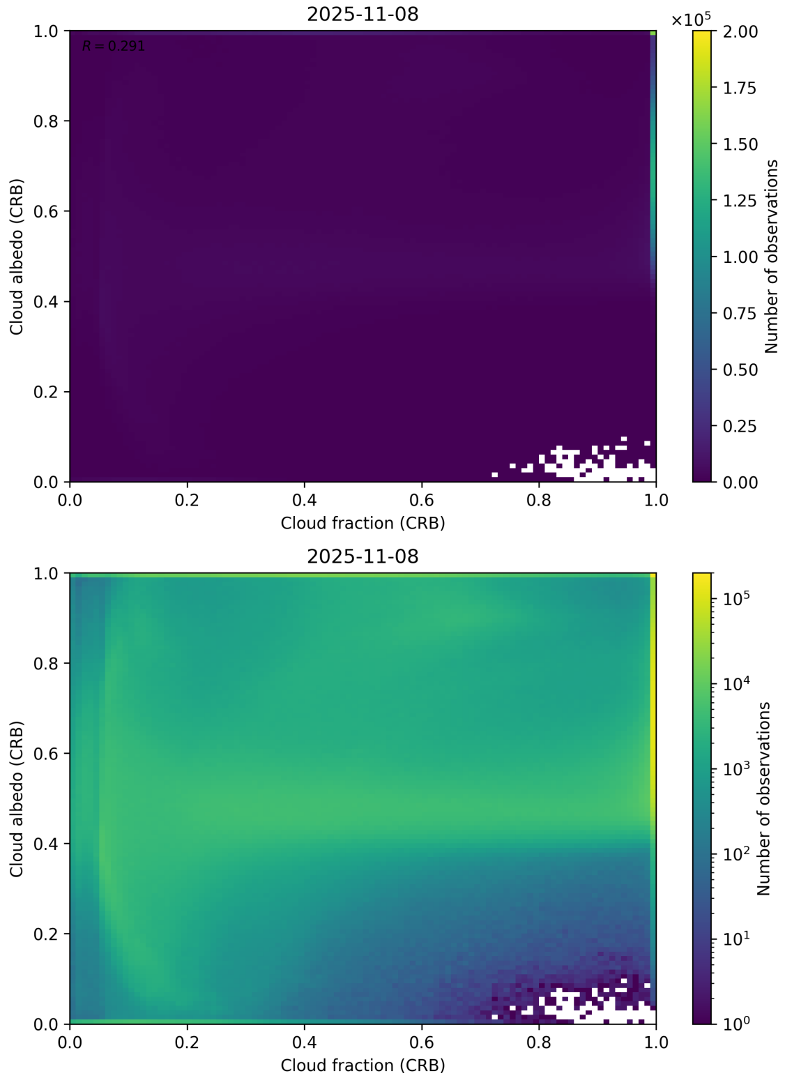
Figure 77: Scatter density plot of “Cloud fraction (CRB)” against “Cloud albedo (CRB)” for 2025-11-07 to 2025-11-09.
