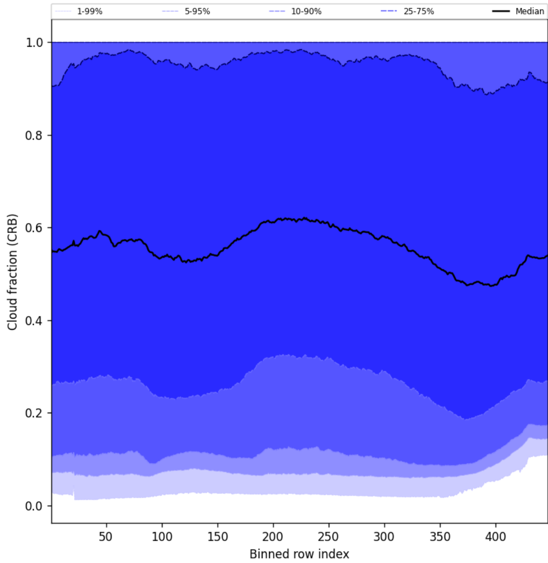
Figure 58: Along track statistics of “Cloud fraction (CRB)” for 2025-11-07 to 2025-11-09
