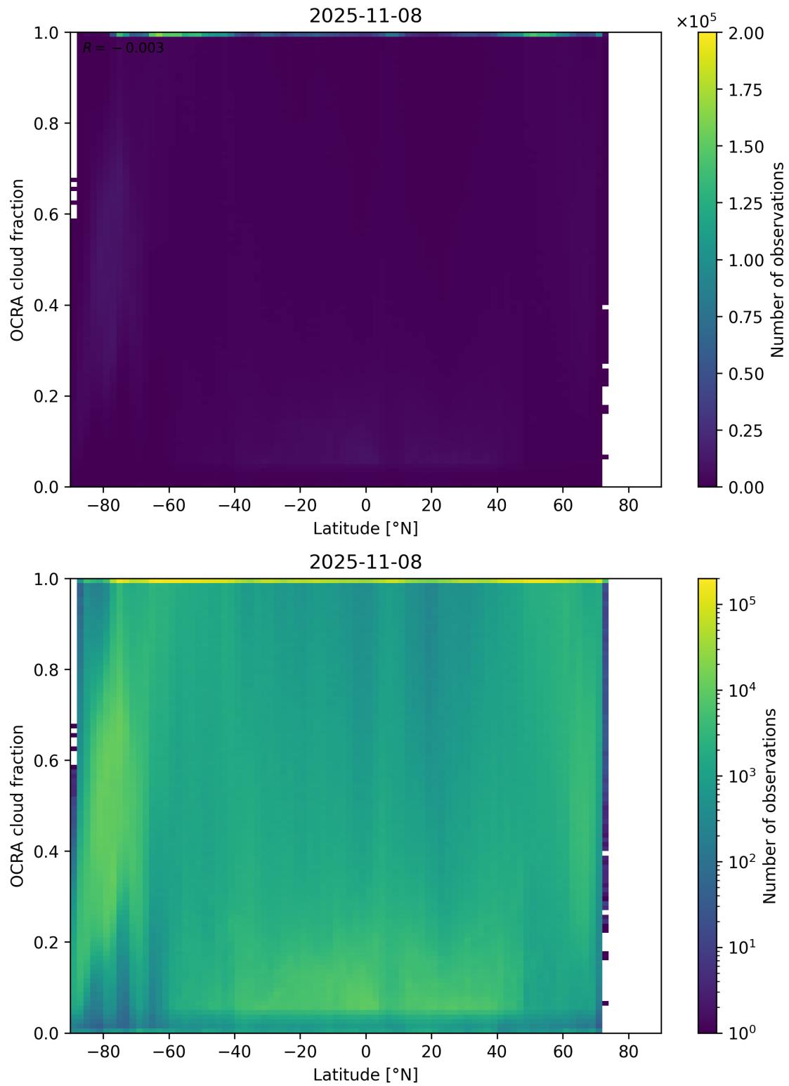
Figure 93: Scatter density plot of “Latitude” against “OCRA cloud fraction” for 2025-11-07 to 2025-11-09.
