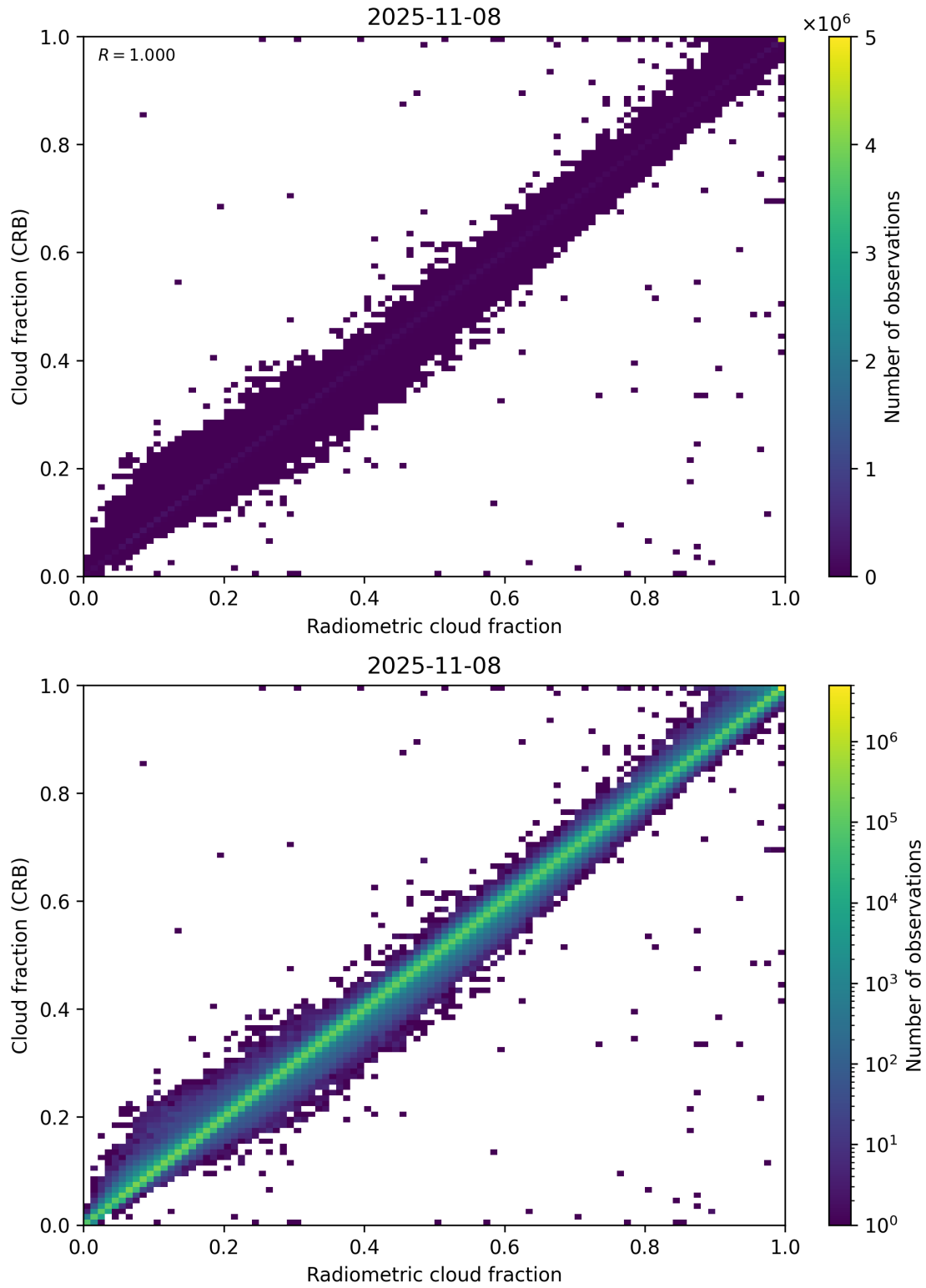
Figure 73: Scatter density plot of “Radiometric cloud fraction” against “Cloud fraction (CRB)” for 2025-11-07 to 2025-11-09.
