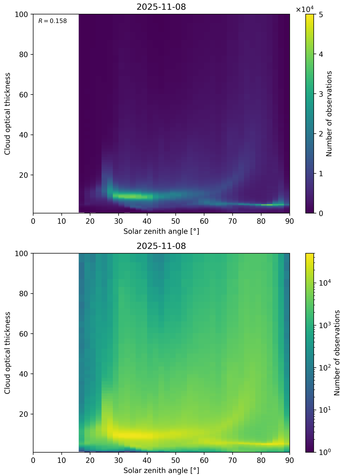
Figure 103: Scatter density plot of “Solar zenith angle” against “Cloud optical thickness” for 2025-11-07 to 2025-11-09.
