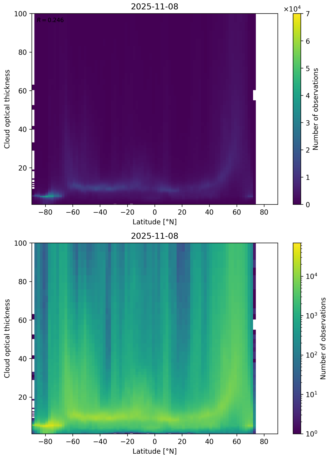
Figure 96: Scatter density plot of “Latitude” against “Cloud optical thickness” for 2025-11-07 to 2025-11-09.
