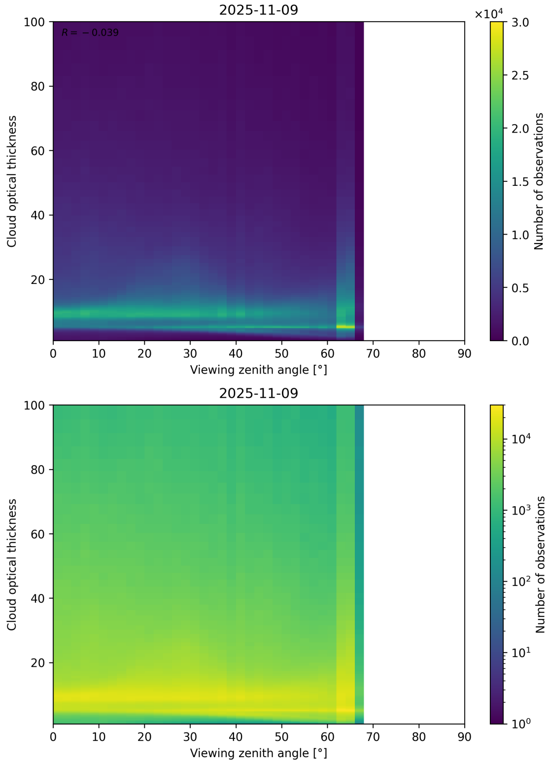
Figure 111: Scatter density plot of “Viewing zenith angle” against “Cloud optical thickness” for 2025-11-08 to 2025-11-10.
