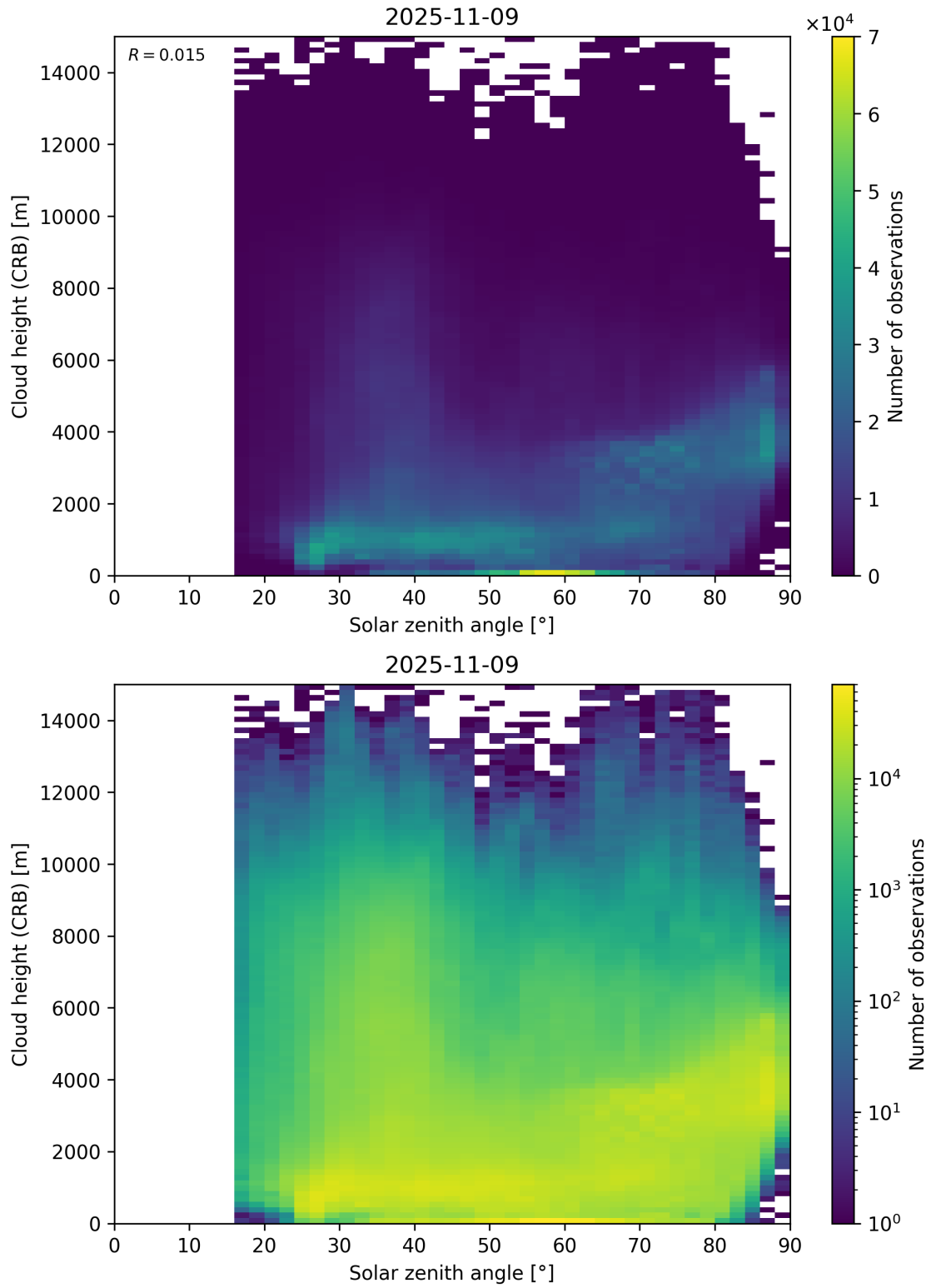
Figure 102: Scatter density plot of “Solar zenith angle” against “Cloud height (CRB)” for 2025-11-08 to 2025-11-10.
