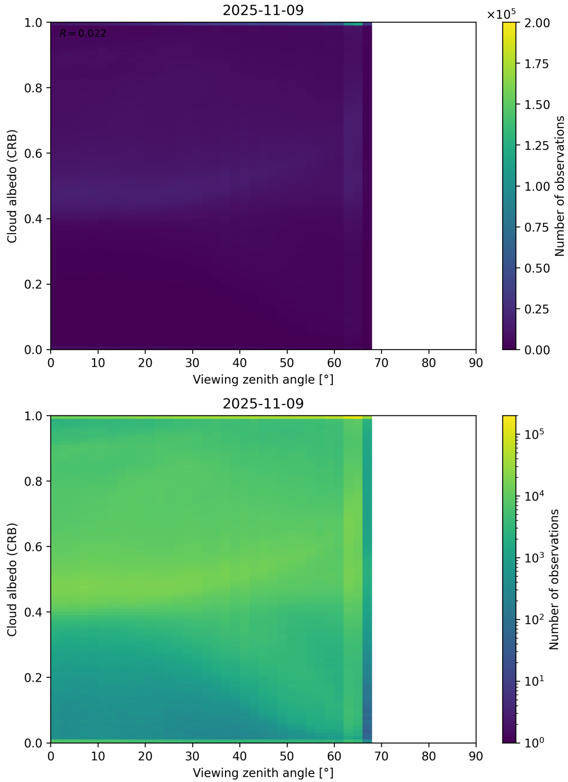
Figure 106: Scatter density plot of “Viewing zenith angle” against “Cloud albedo (CRB)” for 2025-11-08 to 2025-11-10.
