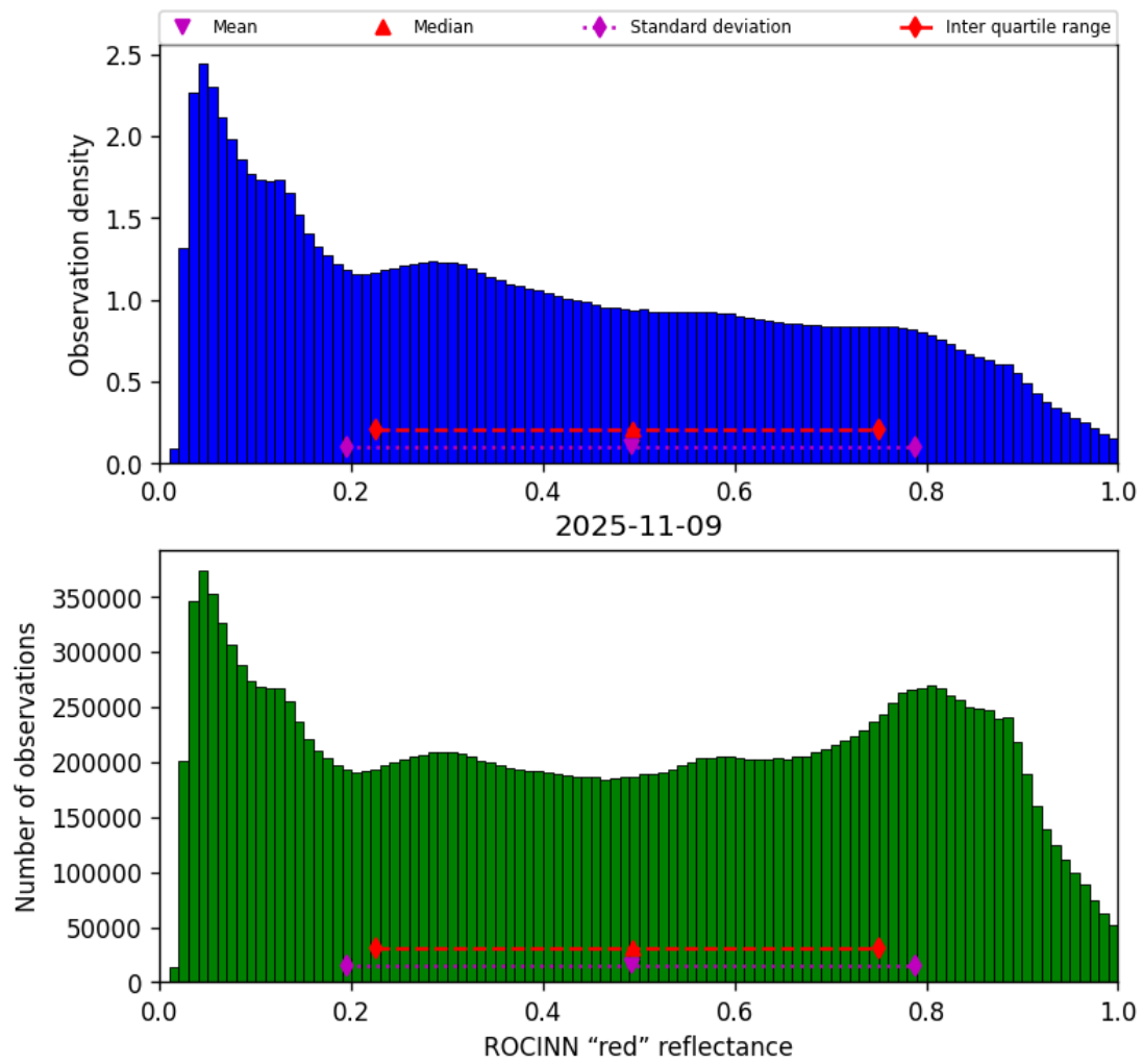
Figure 53: Histogram of “ROCINN “red” reflectance” for 2025-11-08 to 2025-11-10
