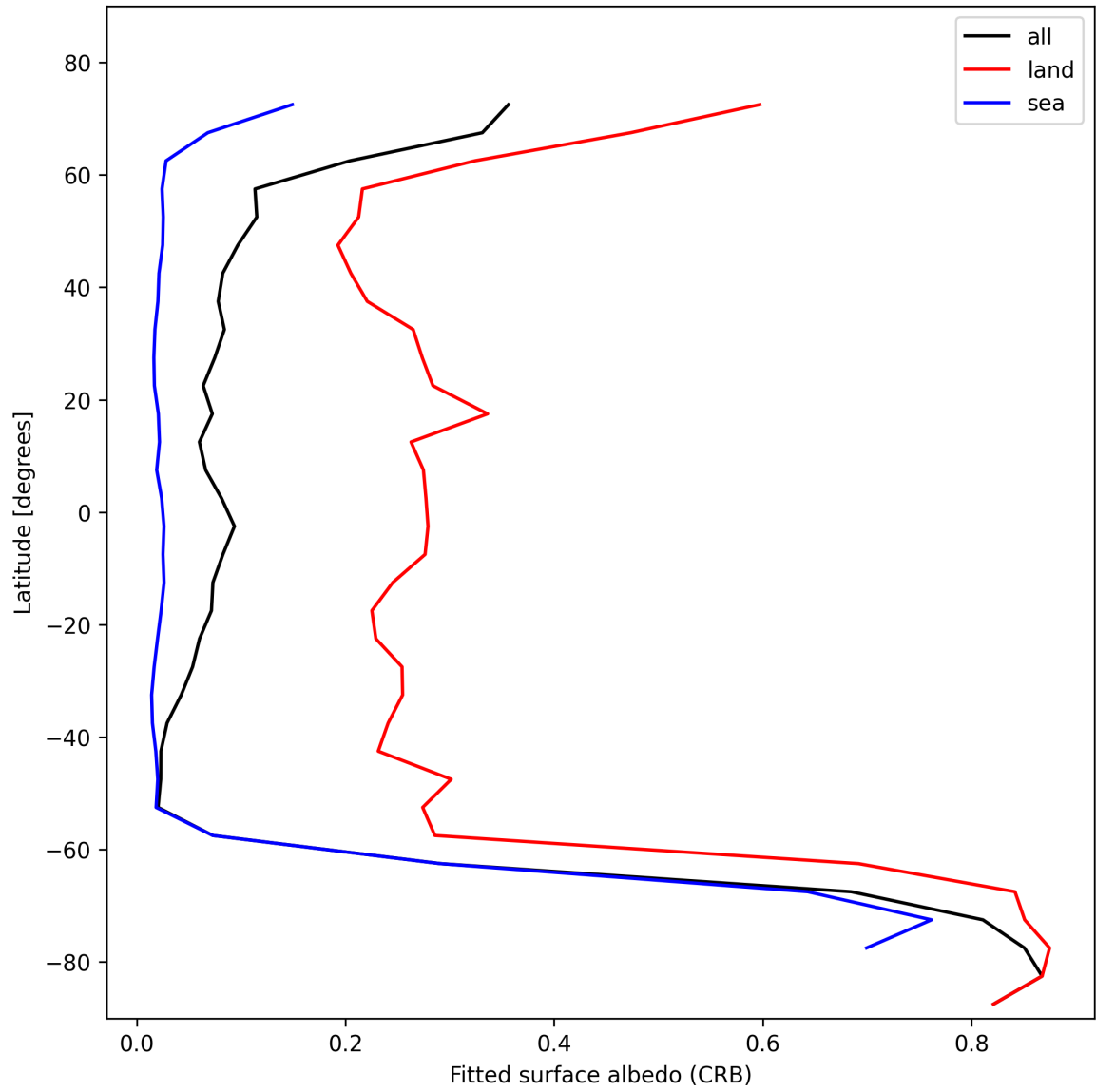
Figure 30: Zonal average of “Fitted surface albedo (CRB)” for 2025-11-08 to 2025-11-10.
