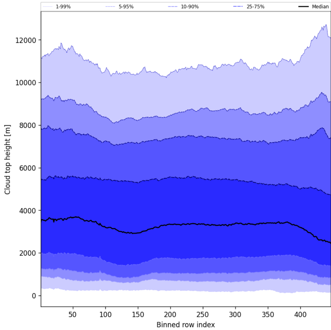
Figure 56: Along track statistics of “Cloud top height” for 2025-11-08 to 2025-11-10
