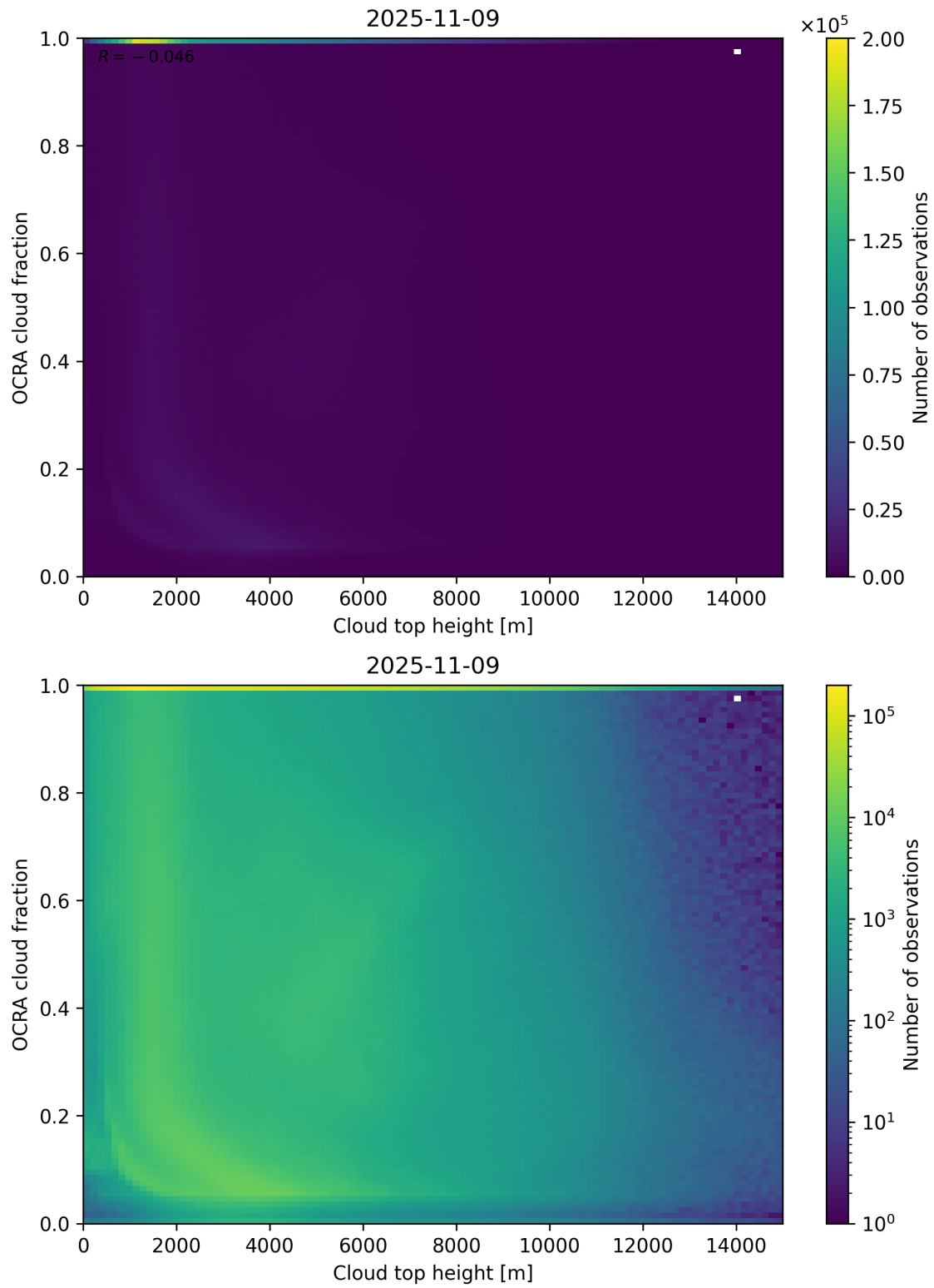
Figure 87: Scatter density plot of “Cloud top height” against “OCRA cloud fraction” for 2025-11-08 to 2025-11-10.
