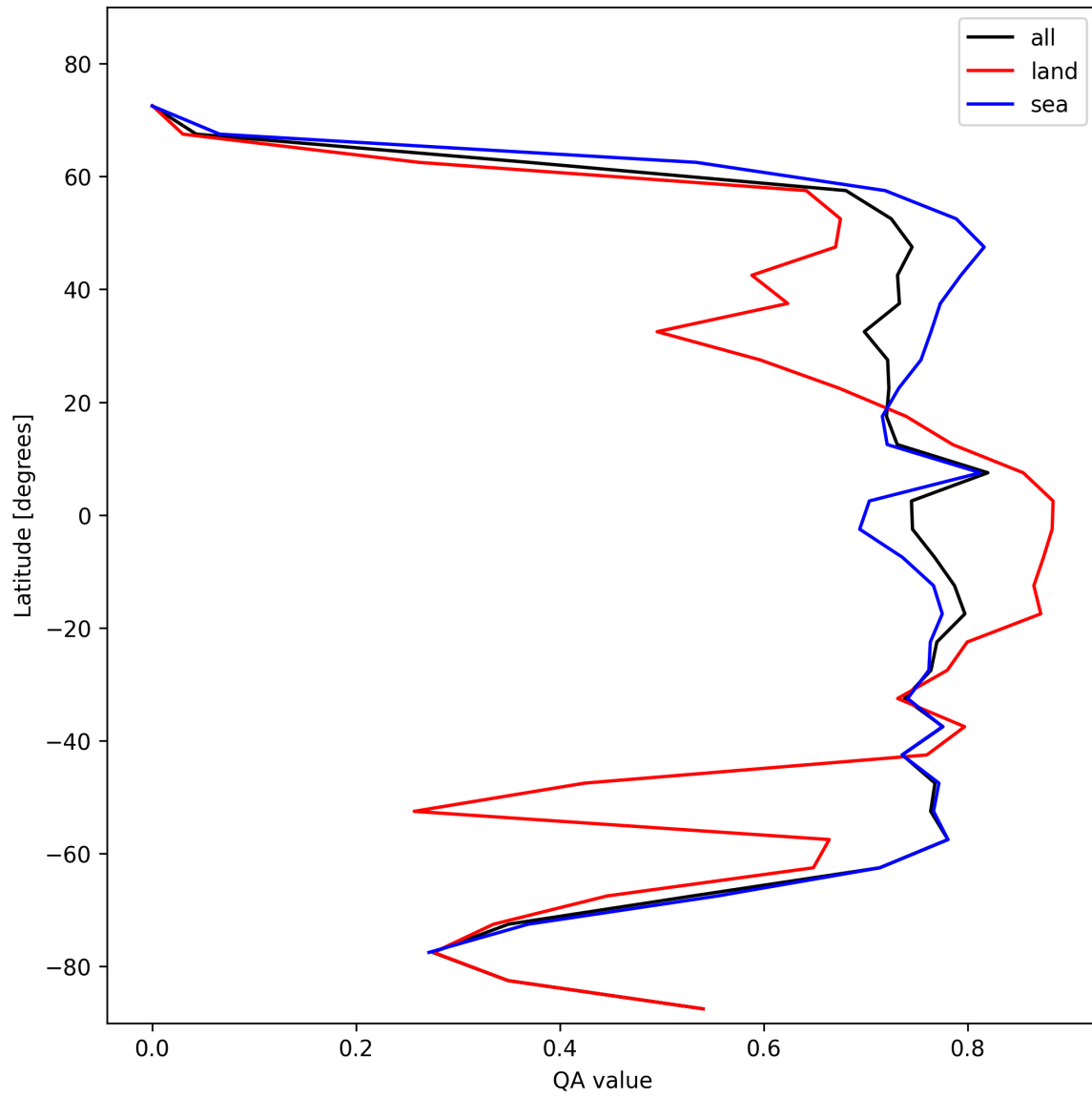
Figure 22: Zonal average of “QA value” for 2025-11-08 to 2025-11-10.
