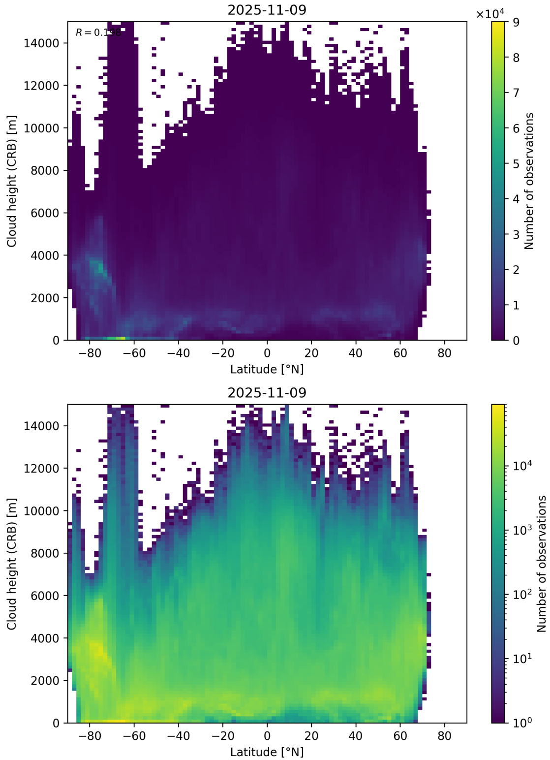
Figure 95: Scatter density plot of “Latitude” against “Cloud height (CRB)” for 2025-11-08 to 2025-11-10.
