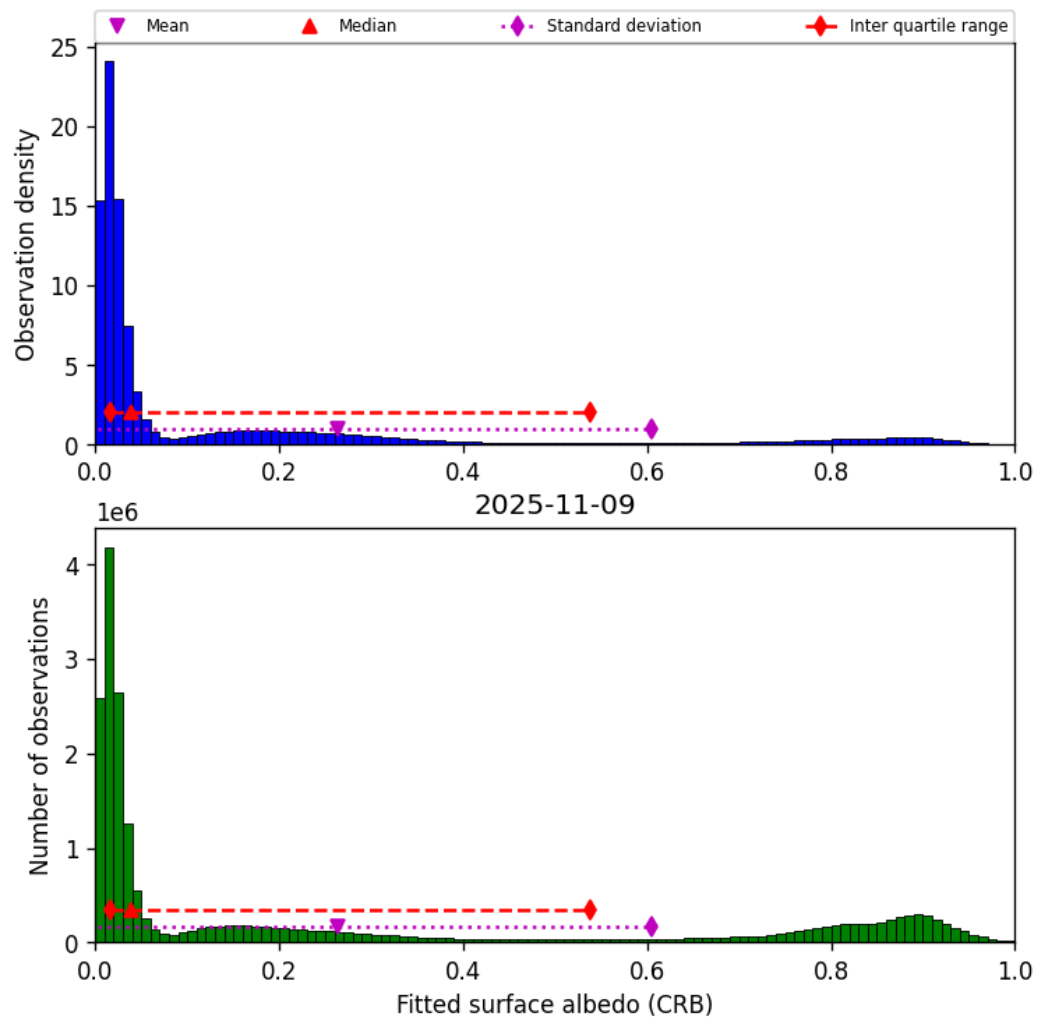
Figure 46: Histogram of “Fitted surface albedo (CRB)” for 2025-11-08 to 2025-11-10
