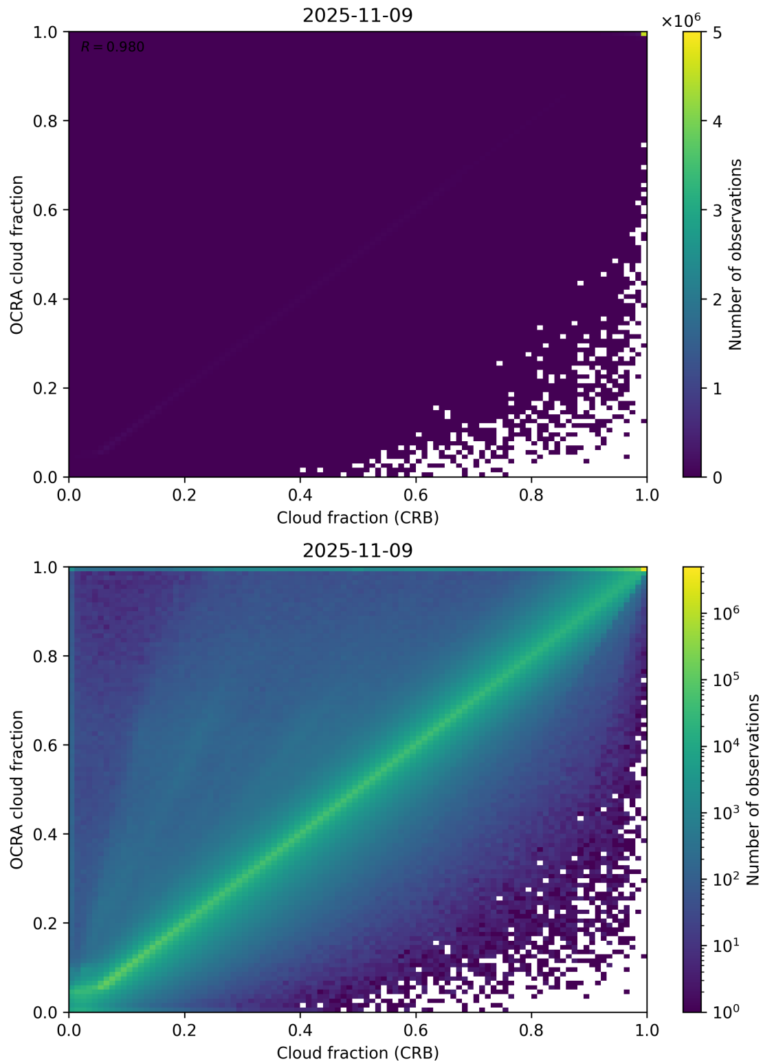
Figure 78: Scatter density plot of “Cloud fraction (CRB)” against “OCRA cloud fraction” for 2025-11-08 to 2025-11-10.
