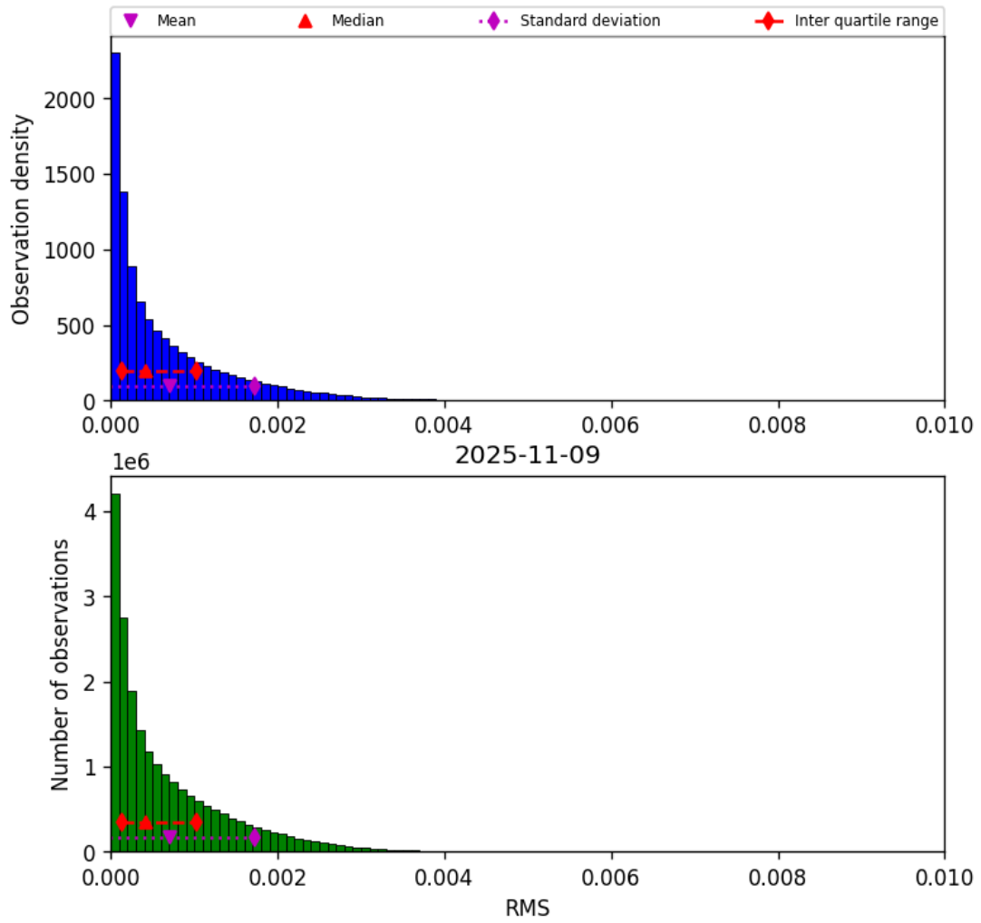
Figure 47: Histogram of “RMS” for 2025-11-08 to 2025-11-10
