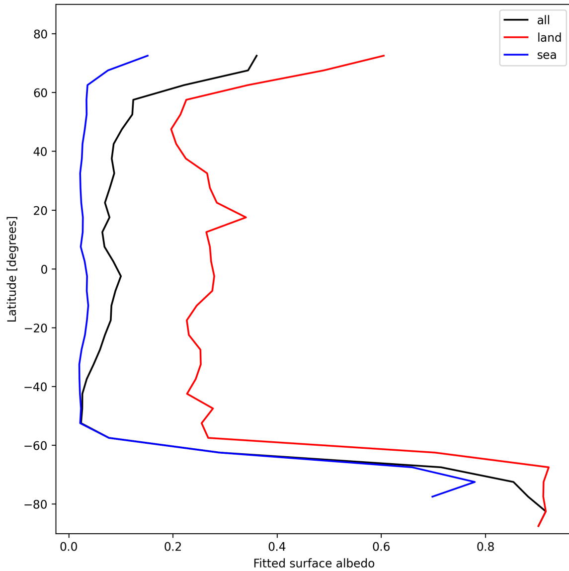
Figure 29: Zonal average of “Fitted surface albedo” for 2025-11-08 to 2025-11-10.
