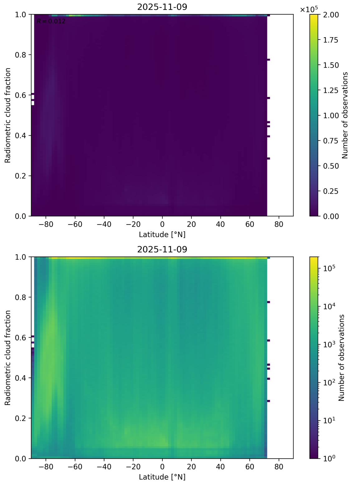
Figure 92: Scatter density plot of “Latitude” against “Radiometric cloud fraction” for 2025-11-08 to 2025-11-10.
