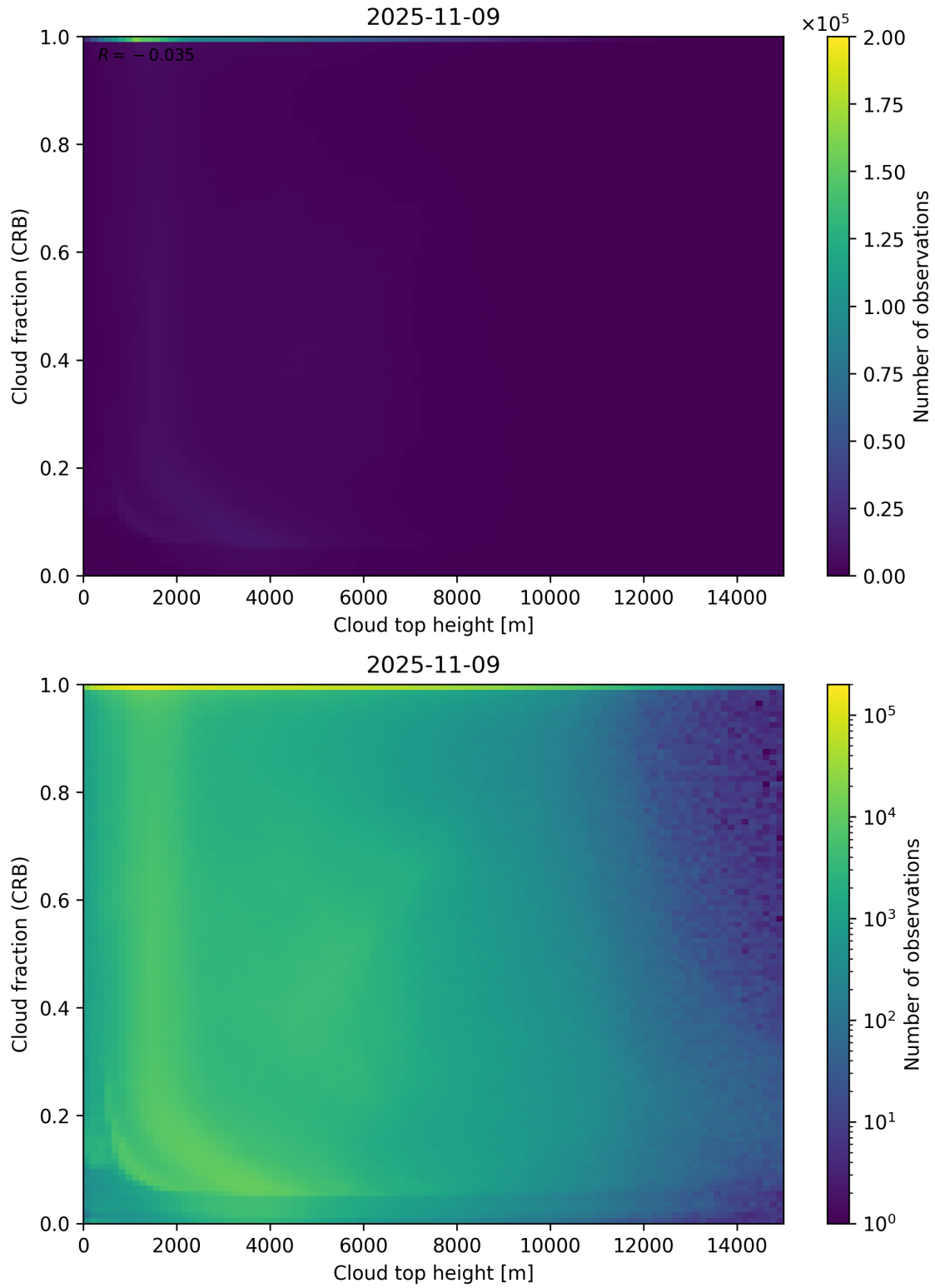
Figure 88: Scatter density plot of “Cloud top height” against “Cloud fraction (CRB)” for 2025-11-08 to 2025-11-10.
