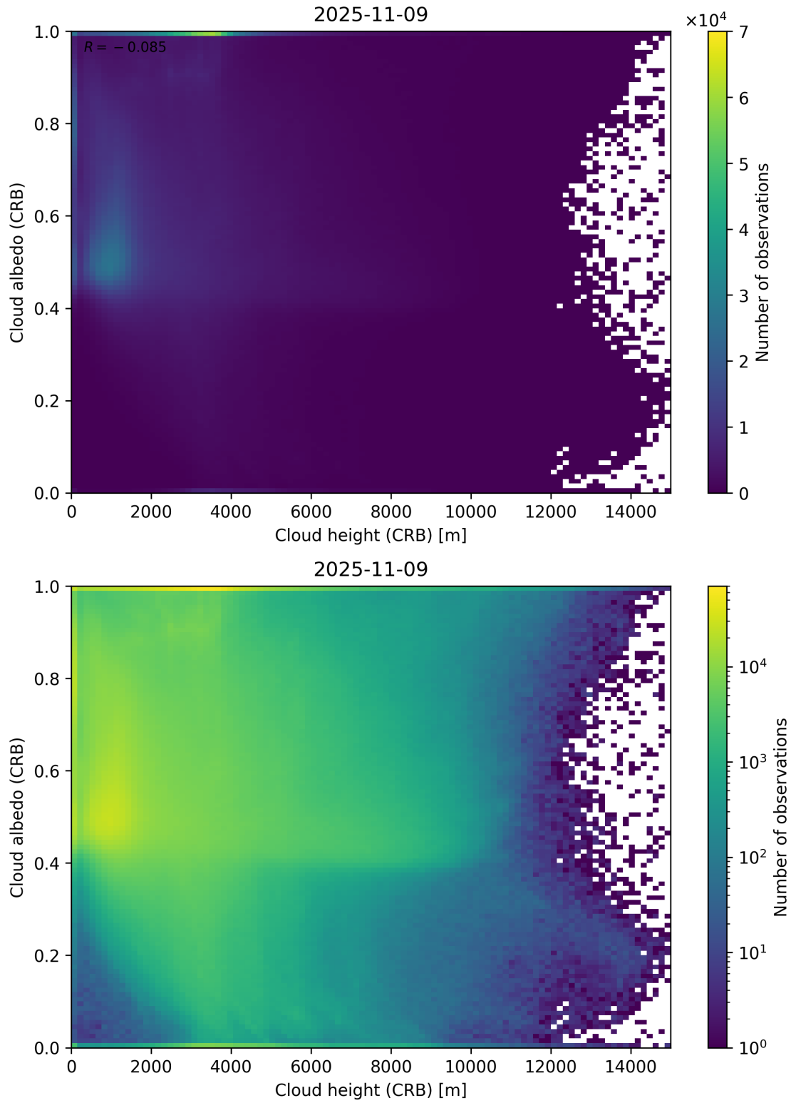
Figure 80: Scatter density plot of “Cloud height (CRB)” against “Cloud albedo (CRB)” for 2025-11-08 to 2025-11-10.
