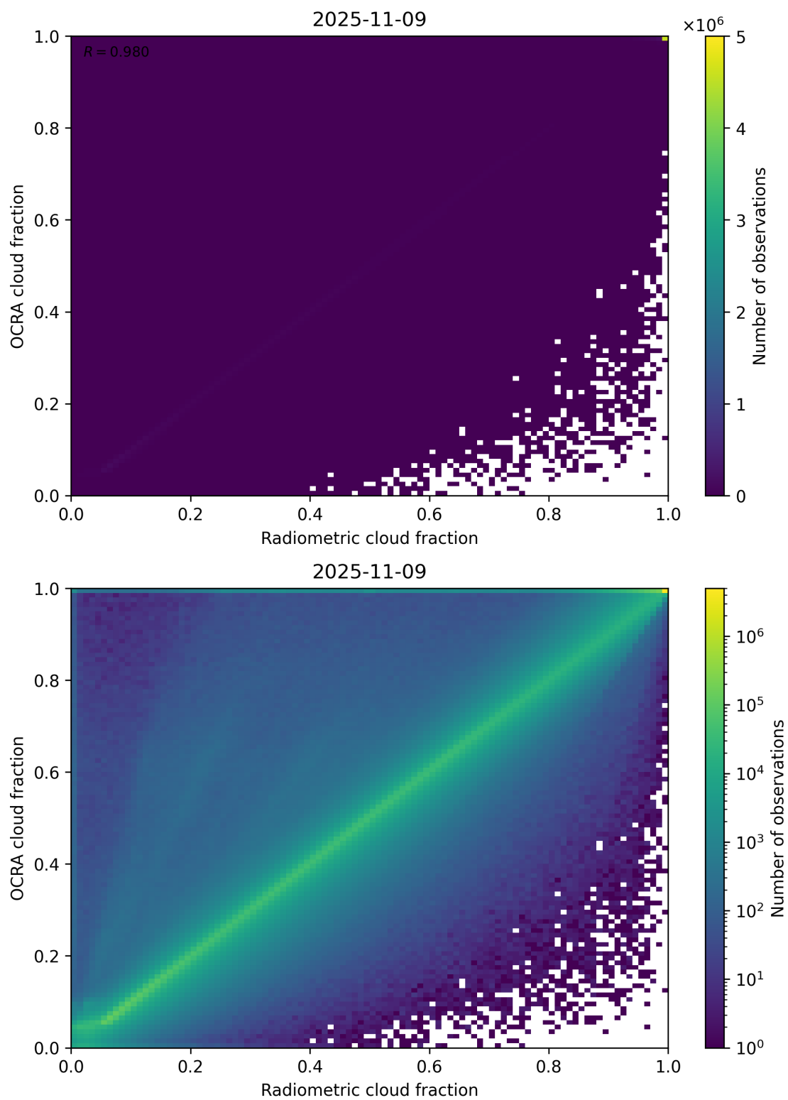
Figure 72: Scatter density plot of “Radiometric cloud fraction” against “OCRA cloud fraction” for 2025-11-08 to 2025-11-10.
