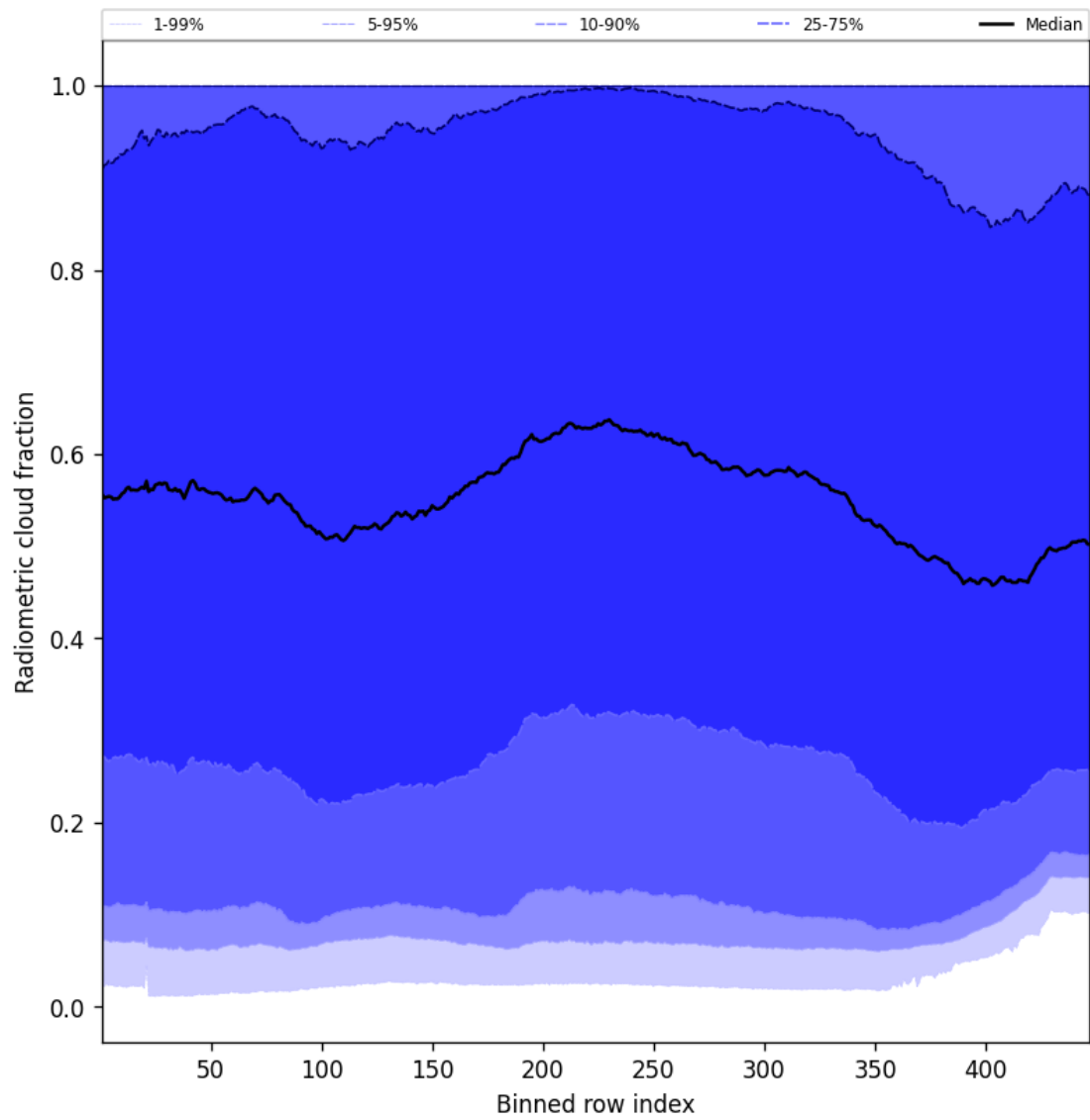
Figure 55: Along track statistics of “Radiometric cloud fraction” for 2025-11-08 to 2025-11-10
