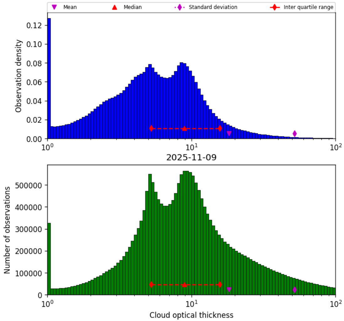
Figure 41: Histogram of “Cloud optical thickness” for 2025-11-08 to 2025-11-10
