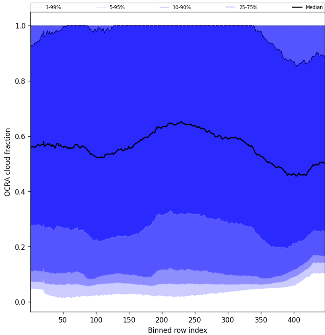
Figure 66: Along track statistics of “OCRA cloud fraction” for 2025-11-08 to 2025-11-10
