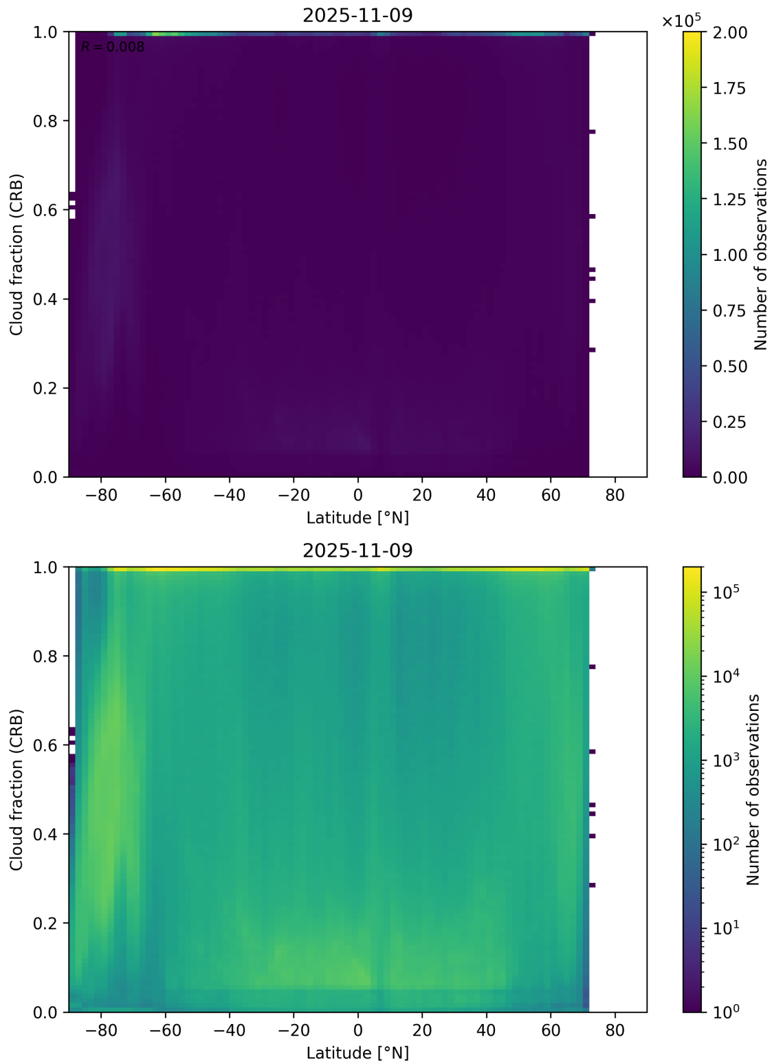
Figure 94: Scatter density plot of “Latitude” against “Cloud fraction (CRB)” for 2025-11-08 to 2025-11-10.
