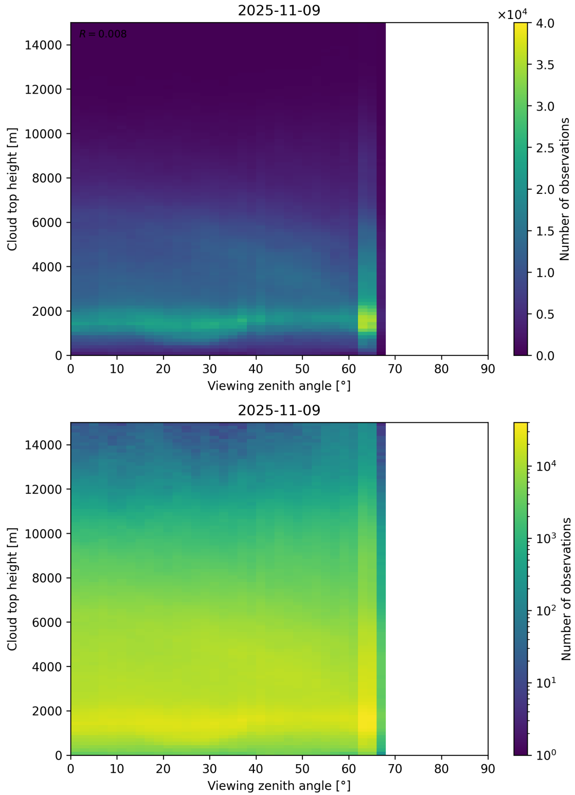
Figure 112: Scatter density plot of “Viewing zenith angle” against “Cloud top height” for 2025-11-08 to 2025-11-10.
