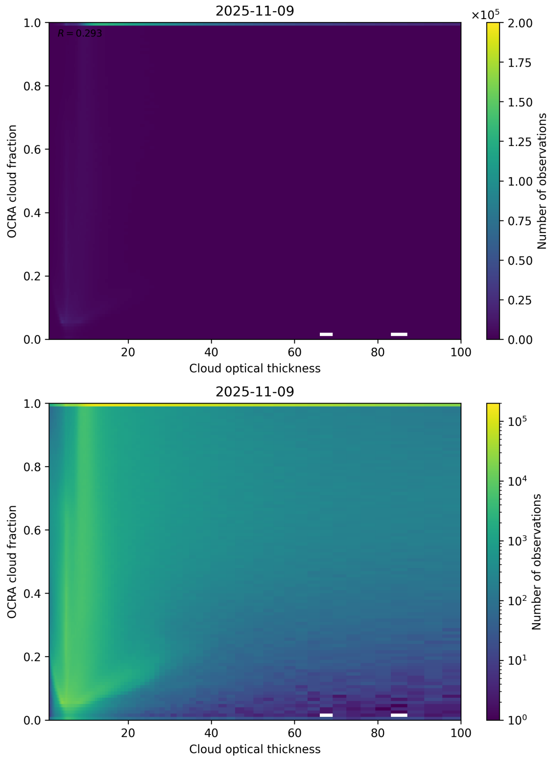
Figure 83: Scatter density plot of “Cloud optical thickness” against “OCRA cloud fraction” for 2025-11-08 to 2025-11-10.
