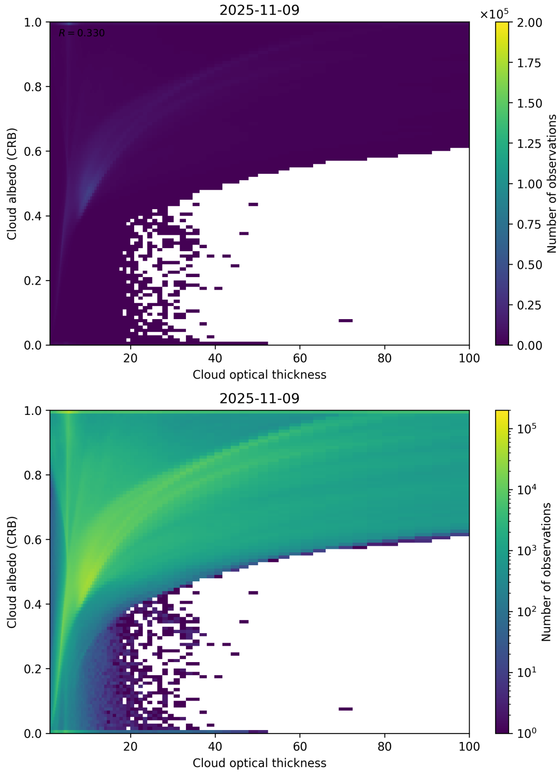
Figure 82: Scatter density plot of “Cloud optical thickness” against “Cloud albedo (CRB)” for 2025-11-08 to 2025-11-10.
