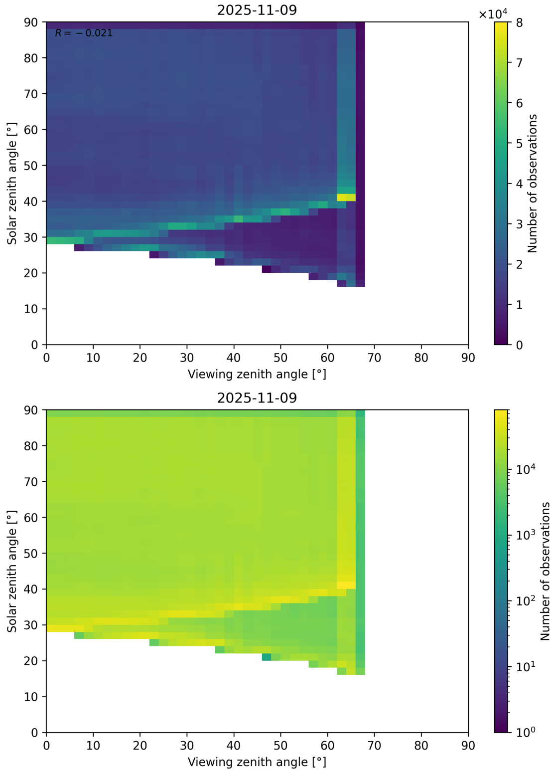
Figure 114: Scatter density plot of “Viewing zenith angle” against “Solar zenith angle” for 2025-11-08 to 2025-11-10.
