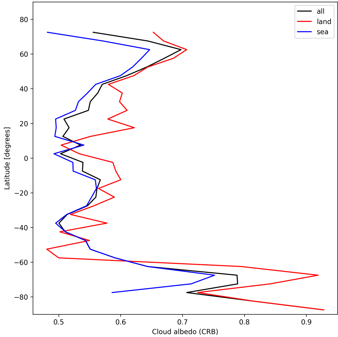
Figure 28: Zonal average of “Cloud albedo (CRB)” for 2025-11-08 to 2025-11-10.
