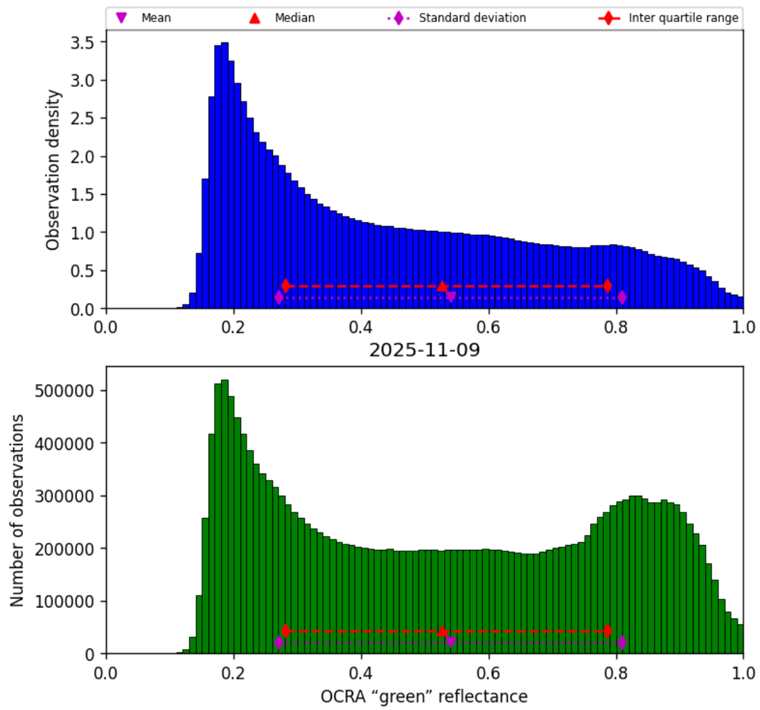
Figure 52: Histogram of “OCRA “green” reflectance” for 2025-11-08 to 2025-11-10
