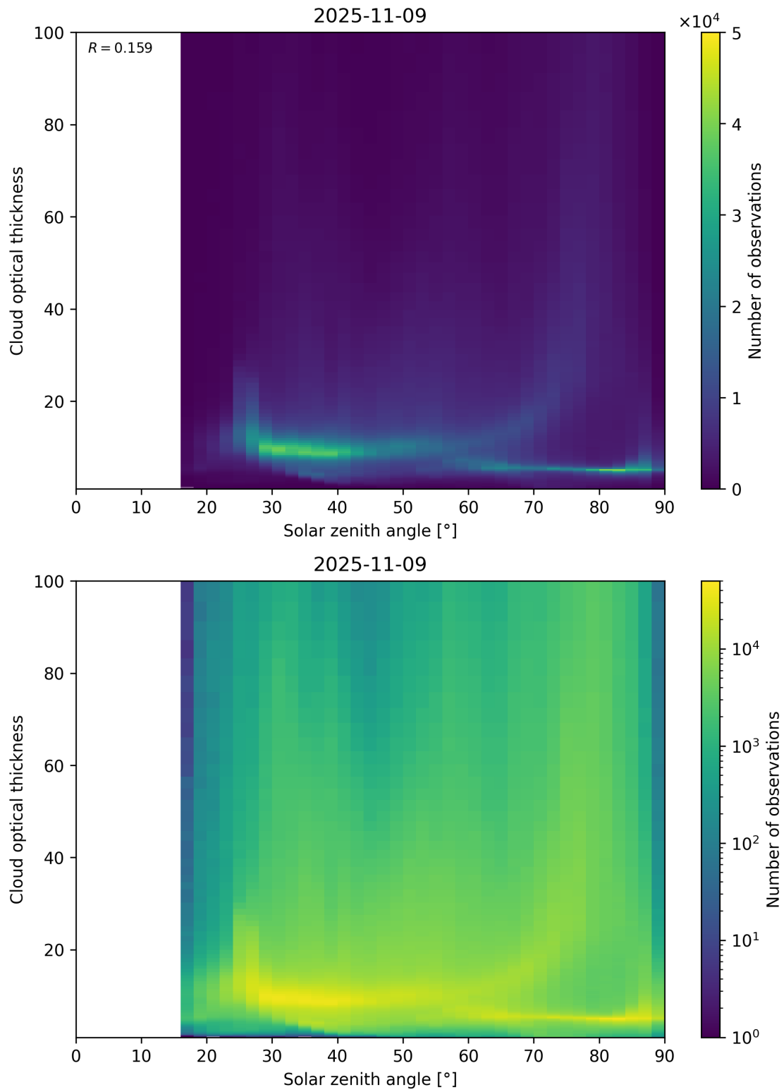
Figure 103: Scatter density plot of “Solar zenith angle” against “Cloud optical thickness” for 2025-11-08 to 2025-11-10.
