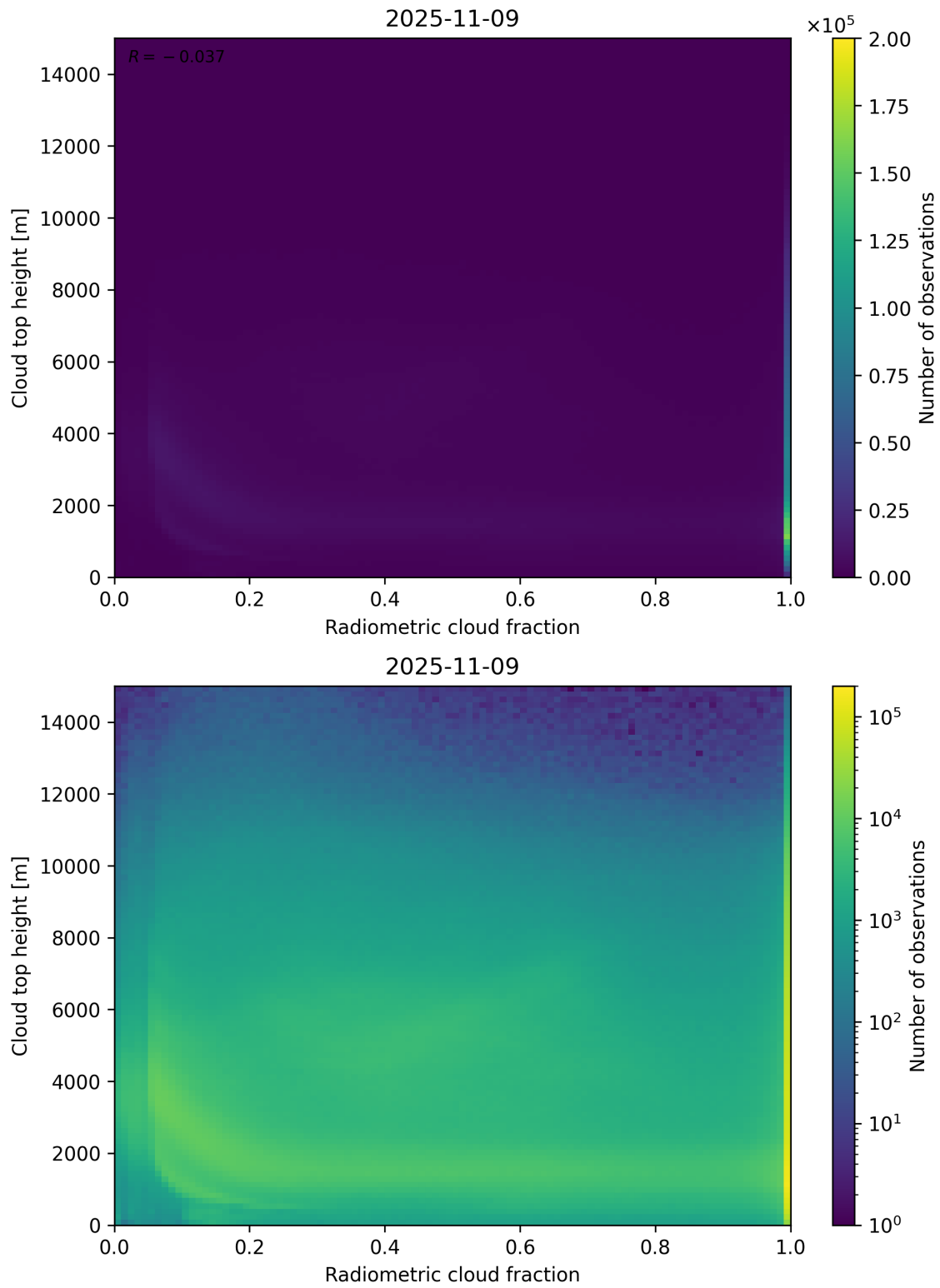
Figure 76: Scatter density plot of “Radiometric cloud fraction” against “Cloud top height” for 2025-11-08 to 2025-11-10.
