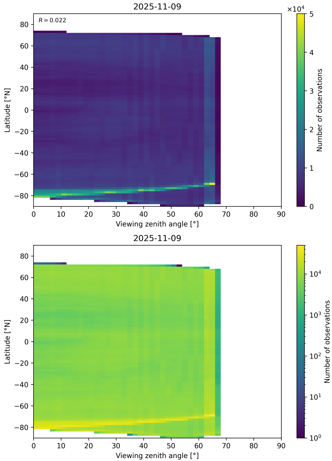
Figure 113: Scatter density plot of “Viewing zenith angle” against “Latitude” for 2025-11-08 to 2025-11-10.
