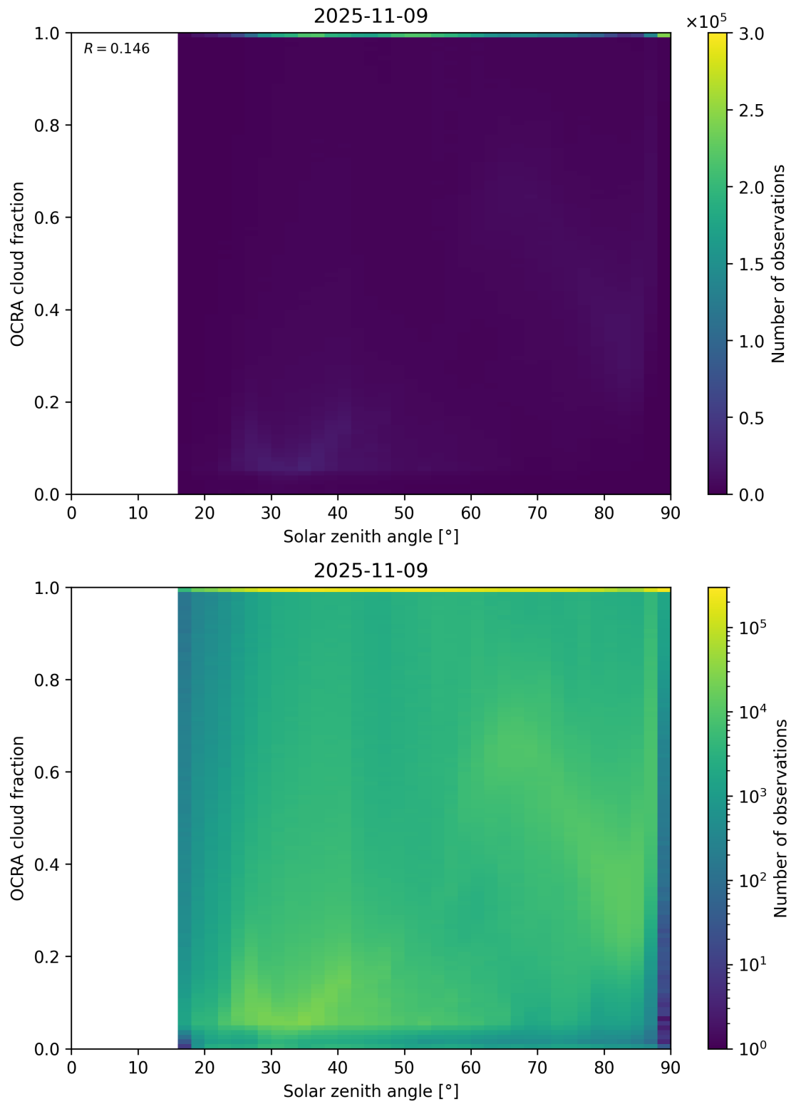
Figure 100: Scatter density plot of “Solar zenith angle” against “OCRA cloud fraction” for 2025-11-08 to 2025-11-10.
