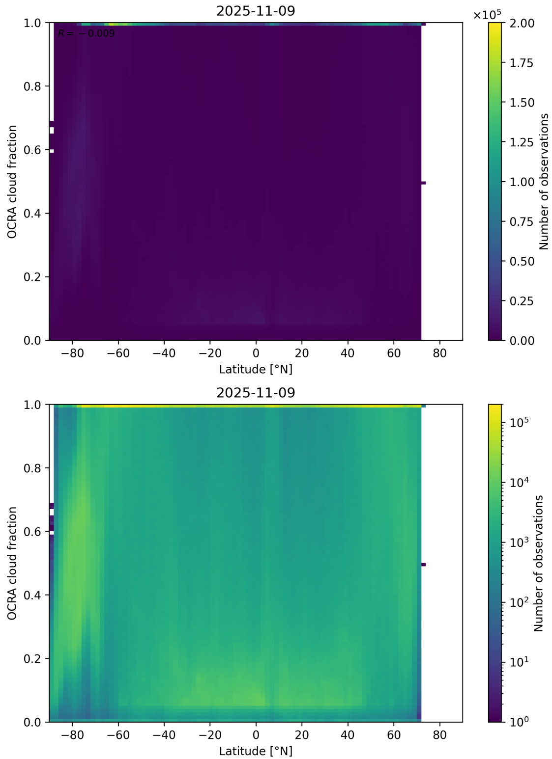
Figure 93: Scatter density plot of “Latitude” against “OCRA cloud fraction” for 2025-11-08 to 2025-11-10.
