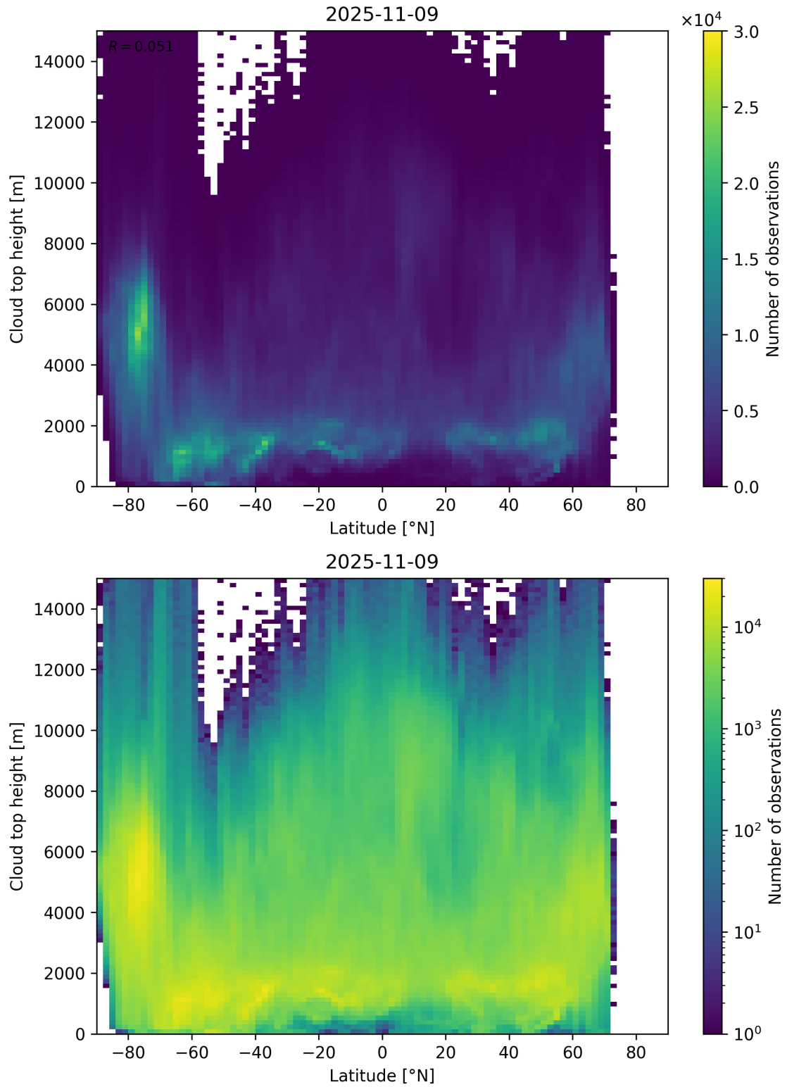
Figure 97: Scatter density plot of “Latitude” against “Cloud top height” for 2025-11-08 to 2025-11-10.
