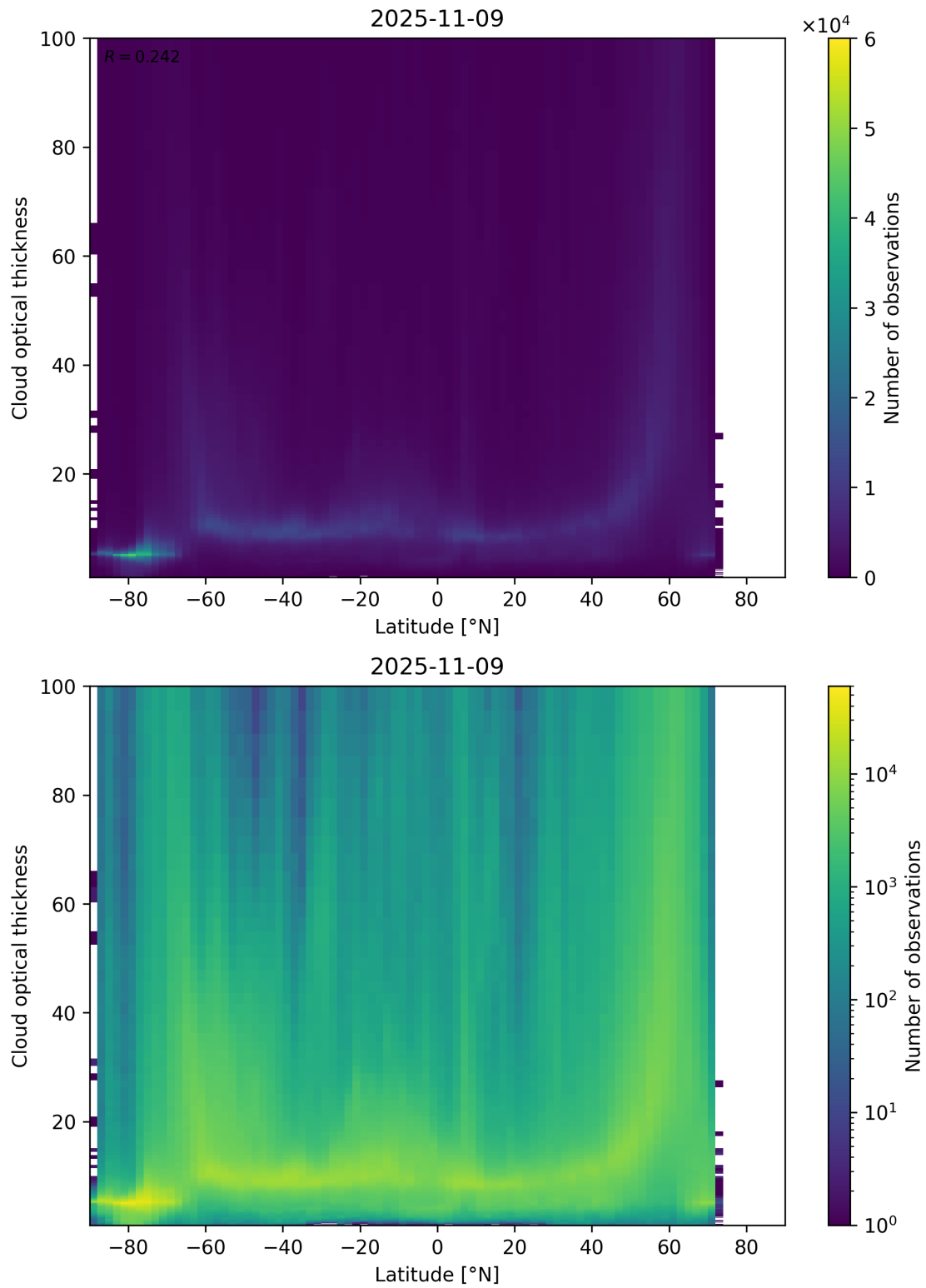
Figure 96: Scatter density plot of “Latitude” against “Cloud optical thickness” for 2025-11-08 to 2025-11-10.
