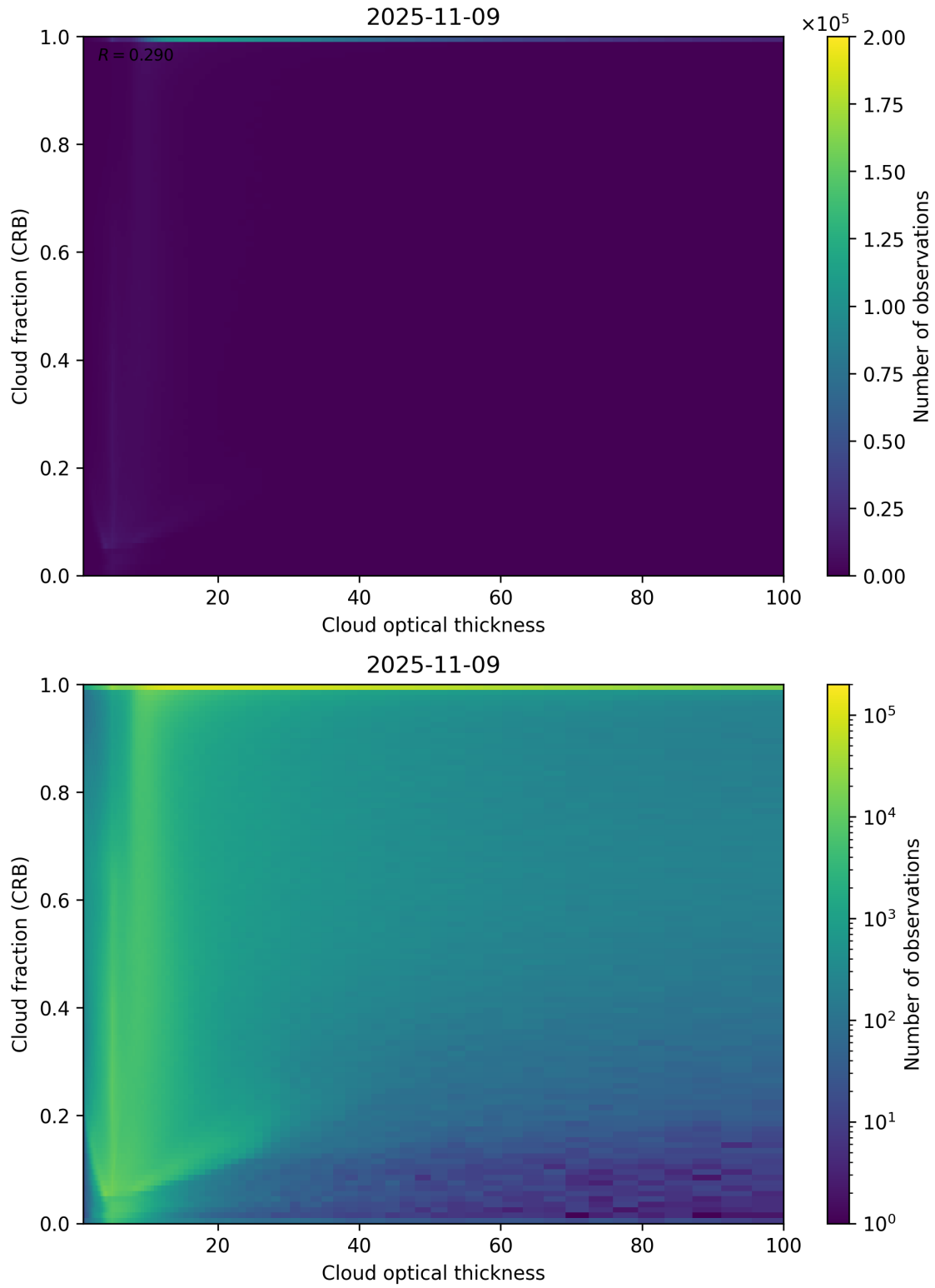
Figure 84: Scatter density plot of “Cloud optical thickness” against “Cloud fraction (CRB)” for 2025-11-08 to 2025-11-10.
