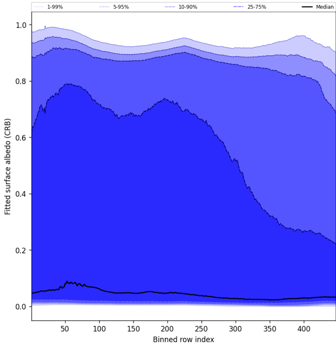
Figure 62: Along track statistics of “Fitted surface albedo (CRB)” for 2025-11-08 to 2025-11-10
