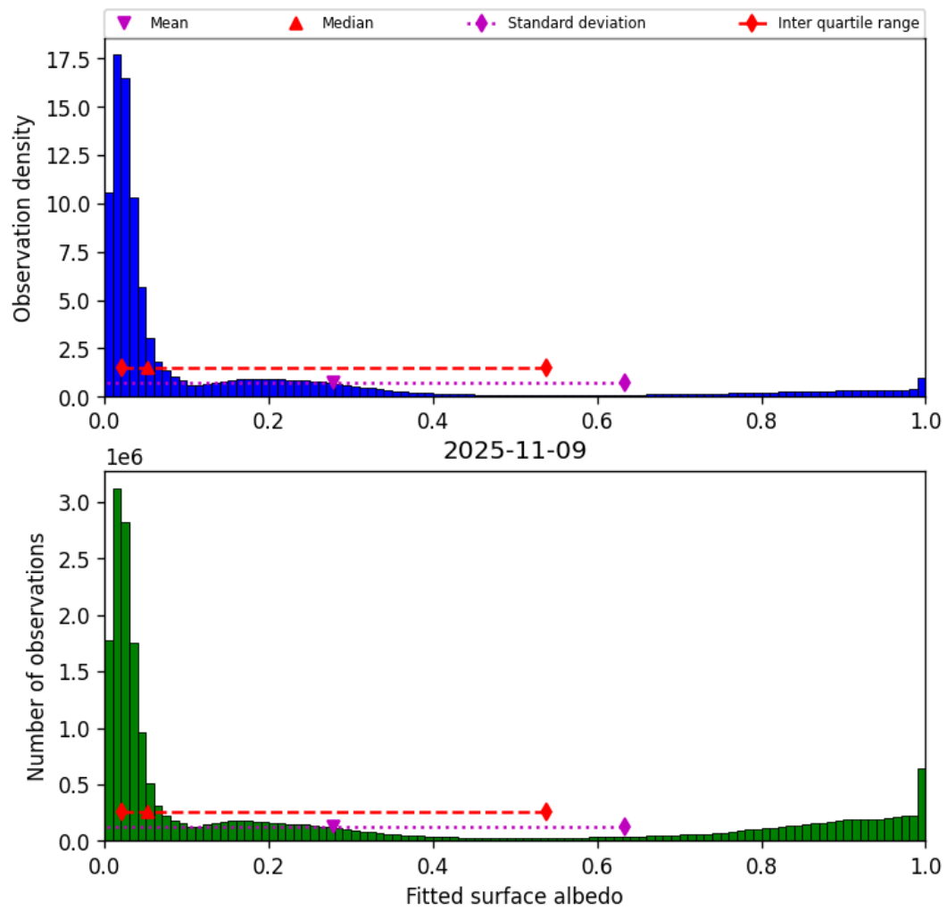
Figure 45: Histogram of “Fitted surface albedo” for 2025-11-08 to 2025-11-10
