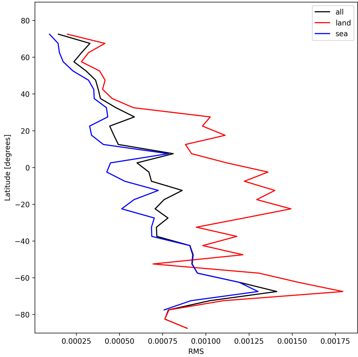
Figure 31: Zonal average of “RMS” for 2025-11-08 to 2025-11-10.
