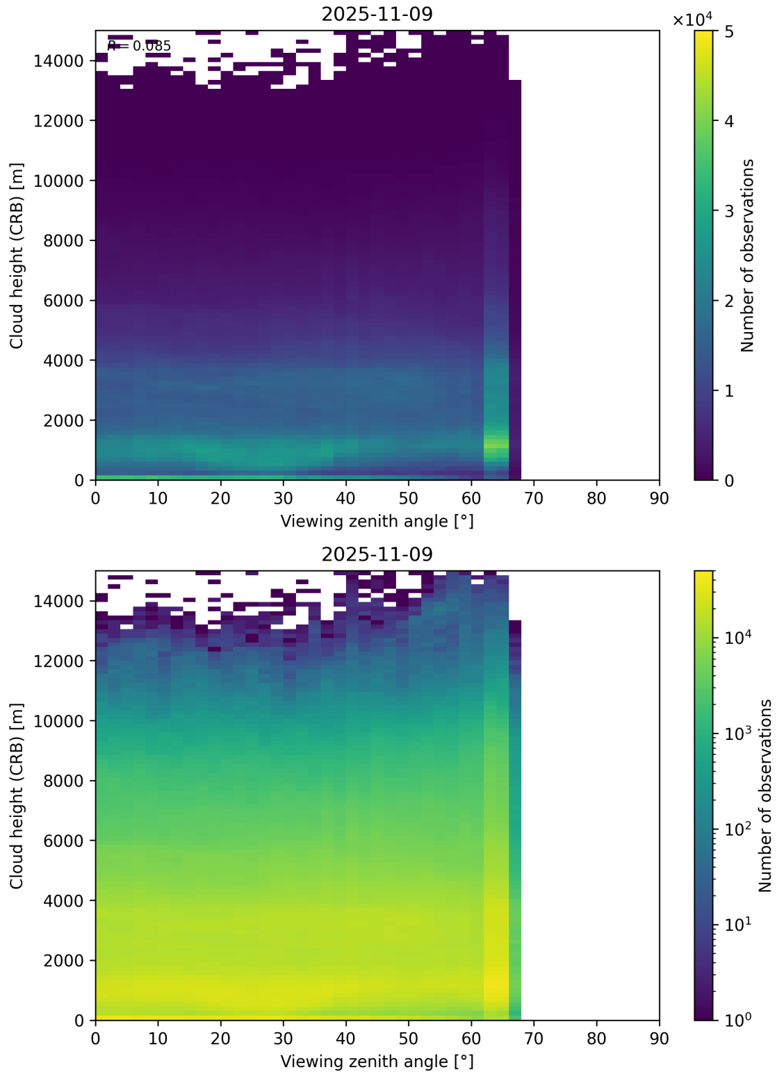
Figure 110: Scatter density plot of “Viewing zenith angle” against “Cloud height (CRB)” for 2025-11-08 to 2025-11-10.
