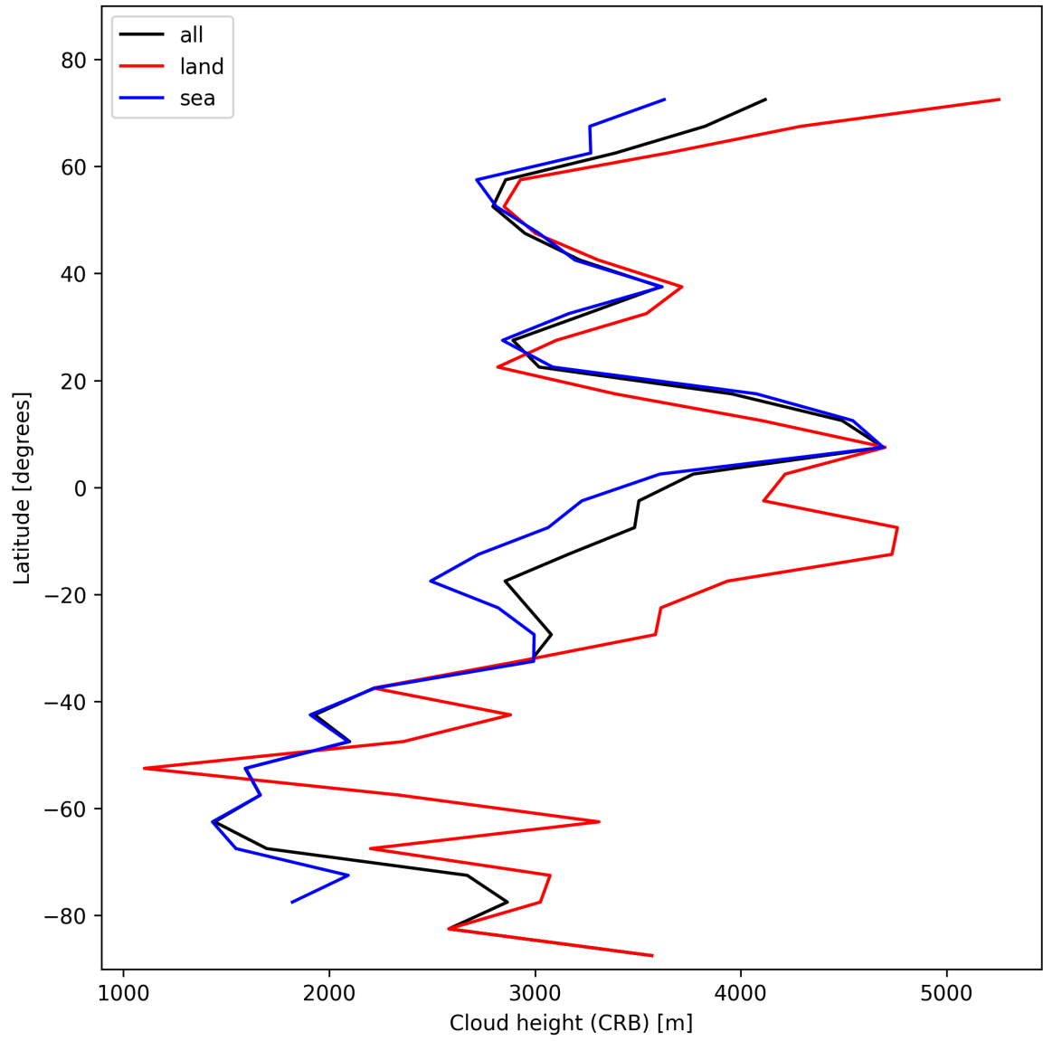
Figure 27: Zonal average of “Cloud height (CRB)” for 2025-11-08 to 2025-11-10.
