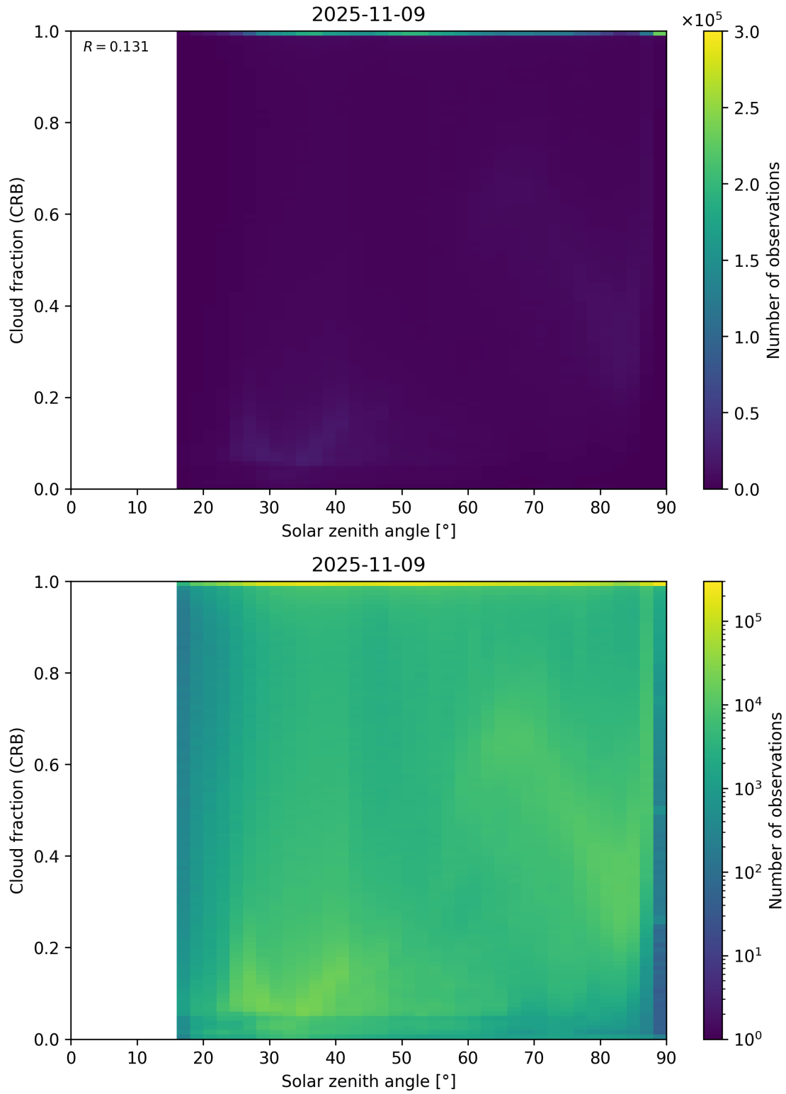
Figure 101: Scatter density plot of “Solar zenith angle” against “Cloud fraction (CRB)” for 2025-11-08 to 2025-11-10.
