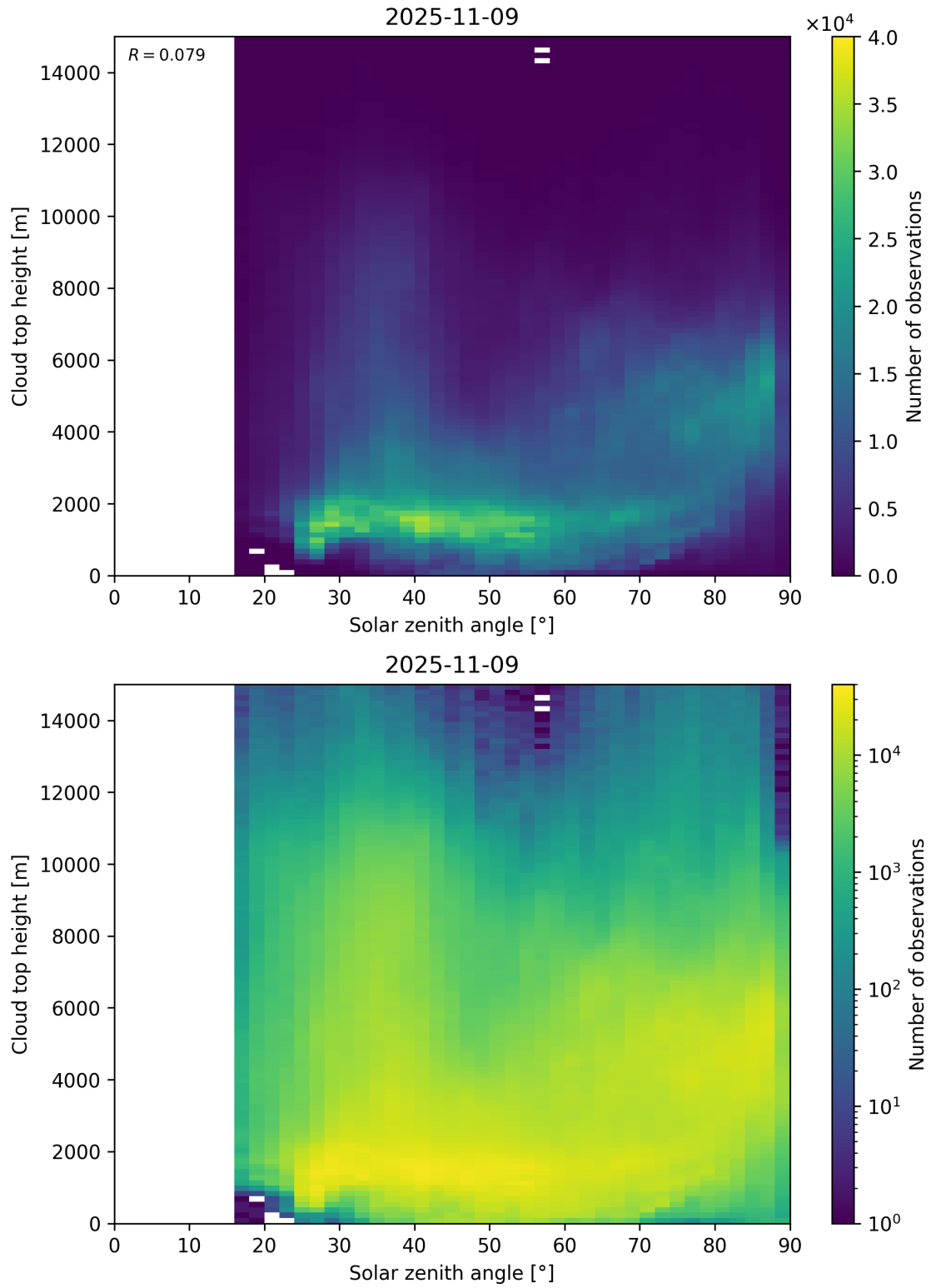
Figure 104: Scatter density plot of “Solar zenith angle” against “Cloud top height” for 2025-11-08 to 2025-11-10.
