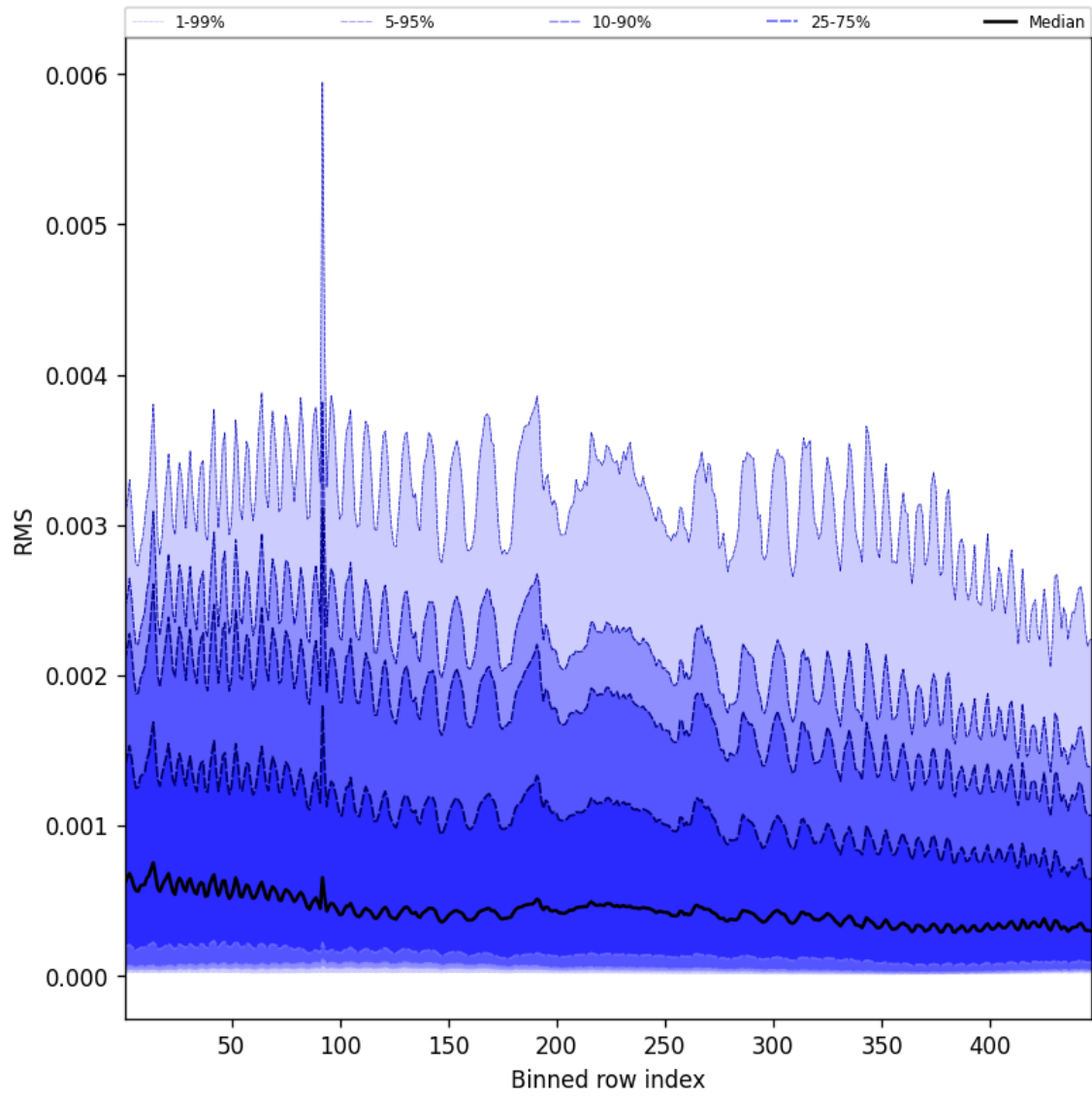
Figure 63: Along track statistics of “RMS” for 2025-11-08 to 2025-11-10
