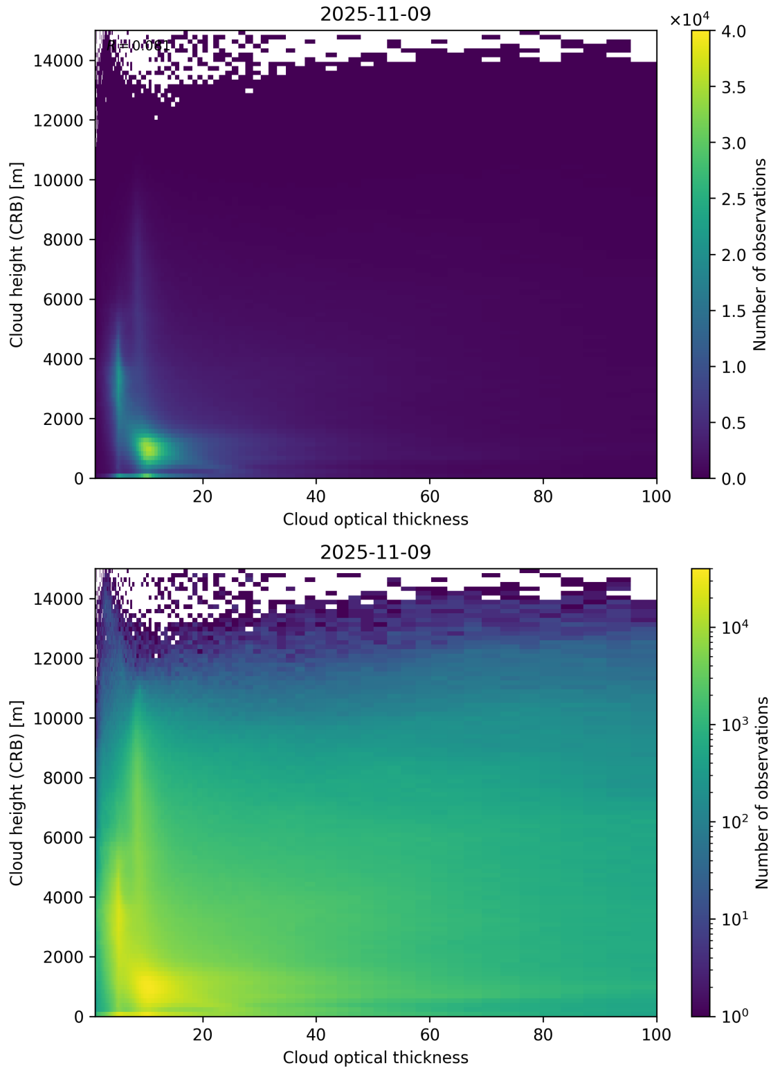
Figure 85: Scatter density plot of “Cloud optical thickness” against “Cloud height (CRB)” for 2025-11-08 to 2025-11-10.
