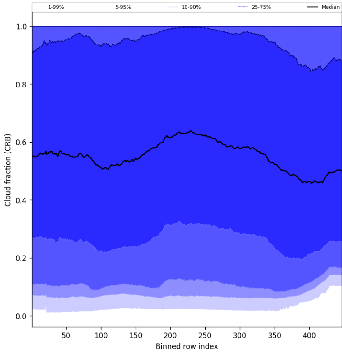
Figure 58: Along track statistics of “Cloud fraction (CRB)” for 2025-11-08 to 2025-11-10
