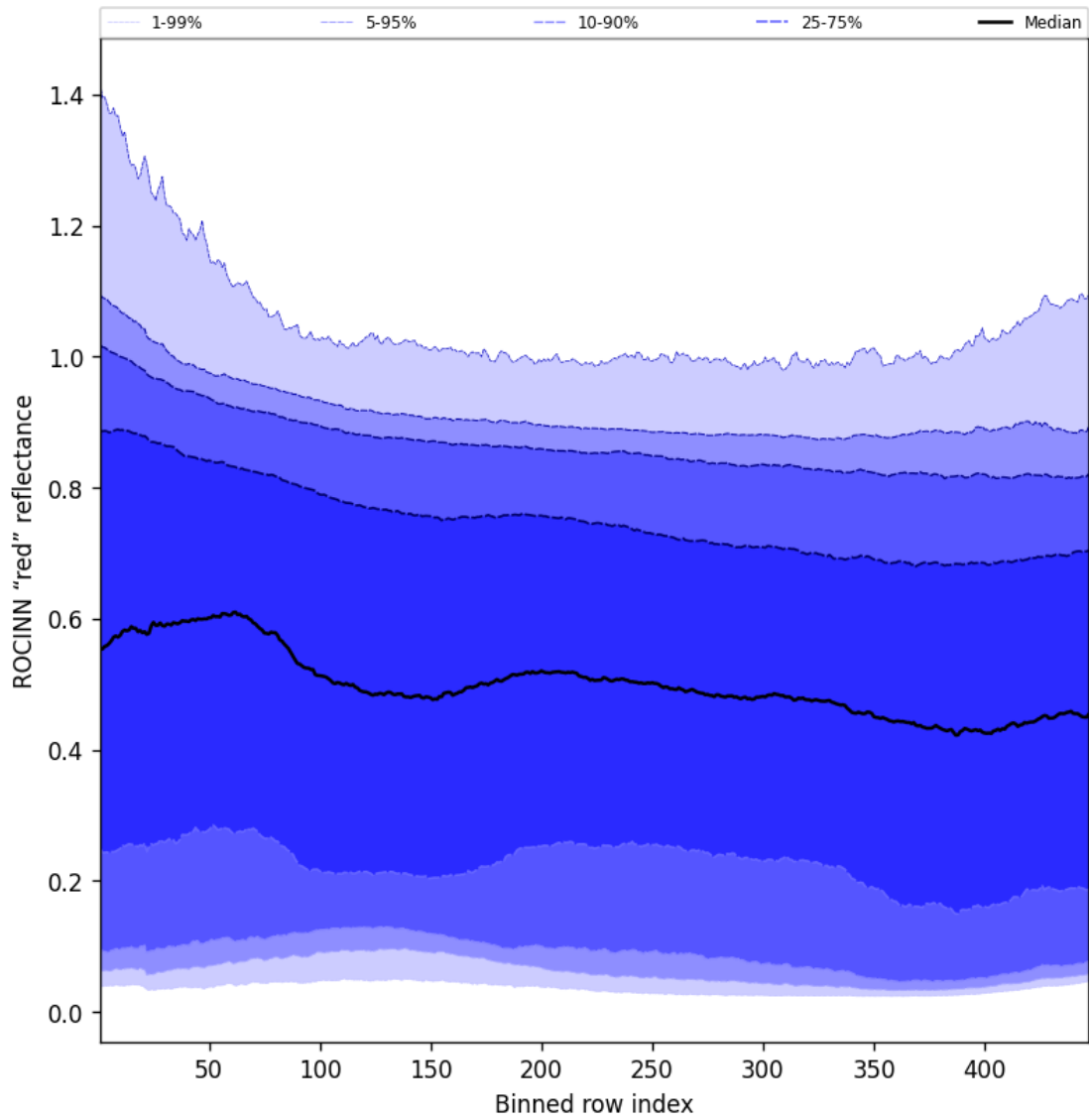
Figure 69: Along track statistics of "ROCINN "red" reflectance" for 2025-11-08 to 2025-11-10
