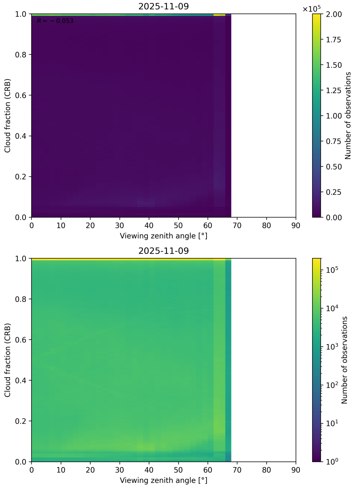
Figure 109: Scatter density plot of “Viewing zenith angle” against “Cloud fraction (CRB)” for 2025-11-08 to 2025-11-10.
