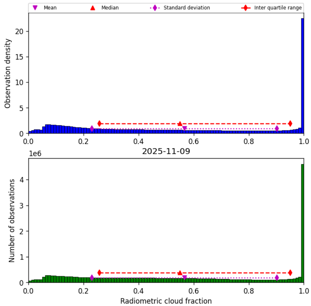
Figure 39: Histogram of “Radiometric cloud fraction” for 2025-11-08 to 2025-11-10
