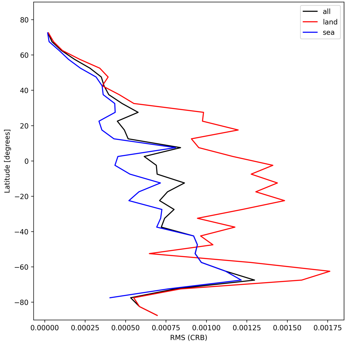
Figure 32: Zonal average of “RMS (CRB)” for 2025-11-08 to 2025-11-10.
