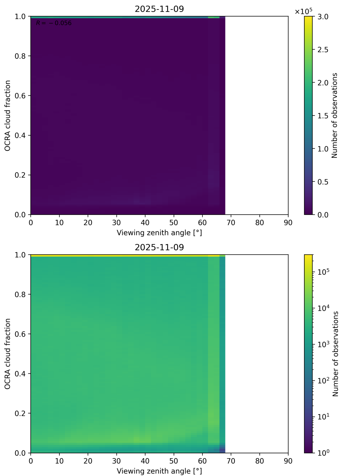
Figure 108: Scatter density plot of “Viewing zenith angle” against “OCRA cloud fraction” for 2025-11-08 to 2025-11-10.
