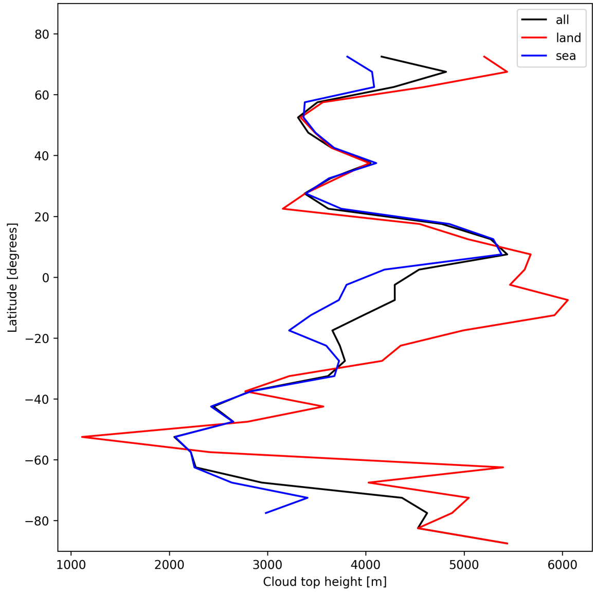
Figure 24: Zonal average of “Cloud top height” for 2025-11-08 to 2025-11-10.
