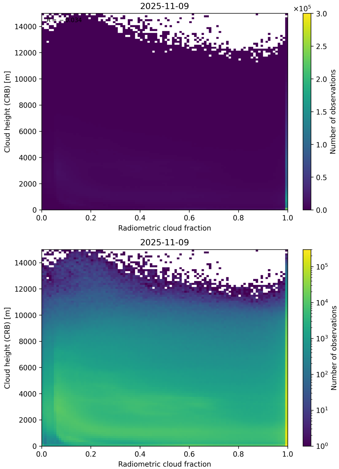
Figure 74: Scatter density plot of “Radiometric cloud fraction” against “Cloud height (CRB)” for 2025-11-08 to 2025-11-10.
