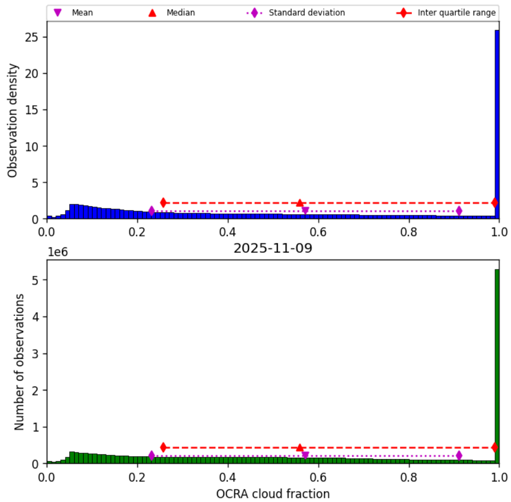
Figure 50: Histogram of “OCRA cloud fraction” for 2025-11-08 to 2025-11-10
