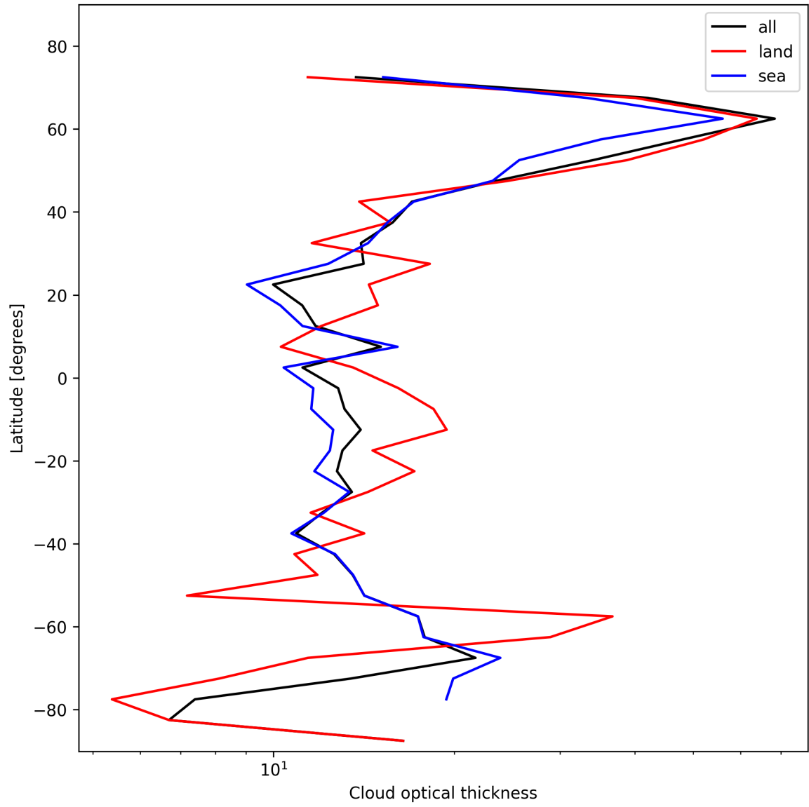
Figure 25: Zonal average of “Cloud optical thickness” for 2025-11-08 to 2025-11-10.
