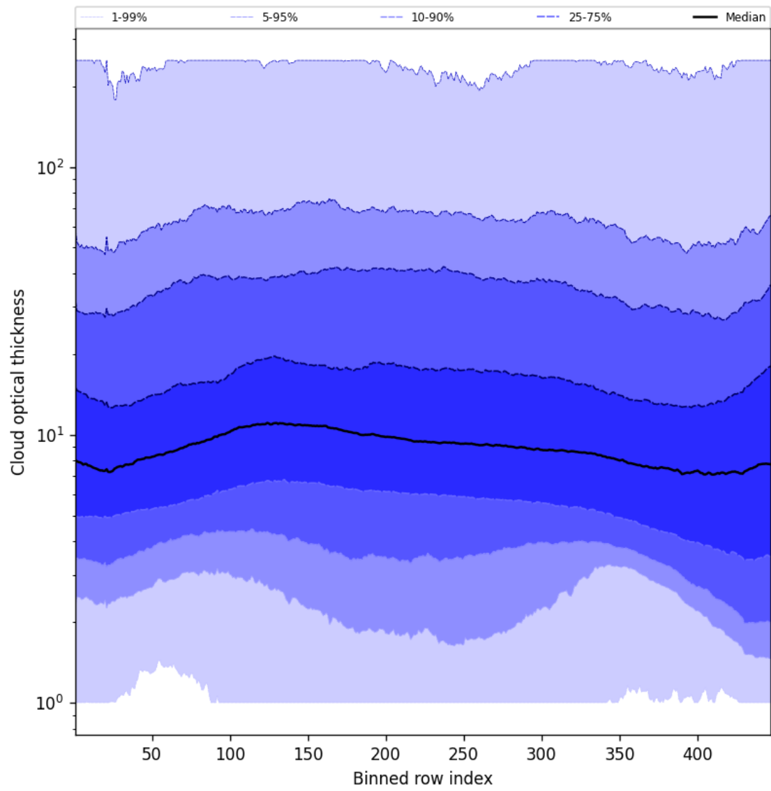
Figure 57: Along track statistics of “Cloud optical thickness” for 2025-11-08 to 2025-11-10
