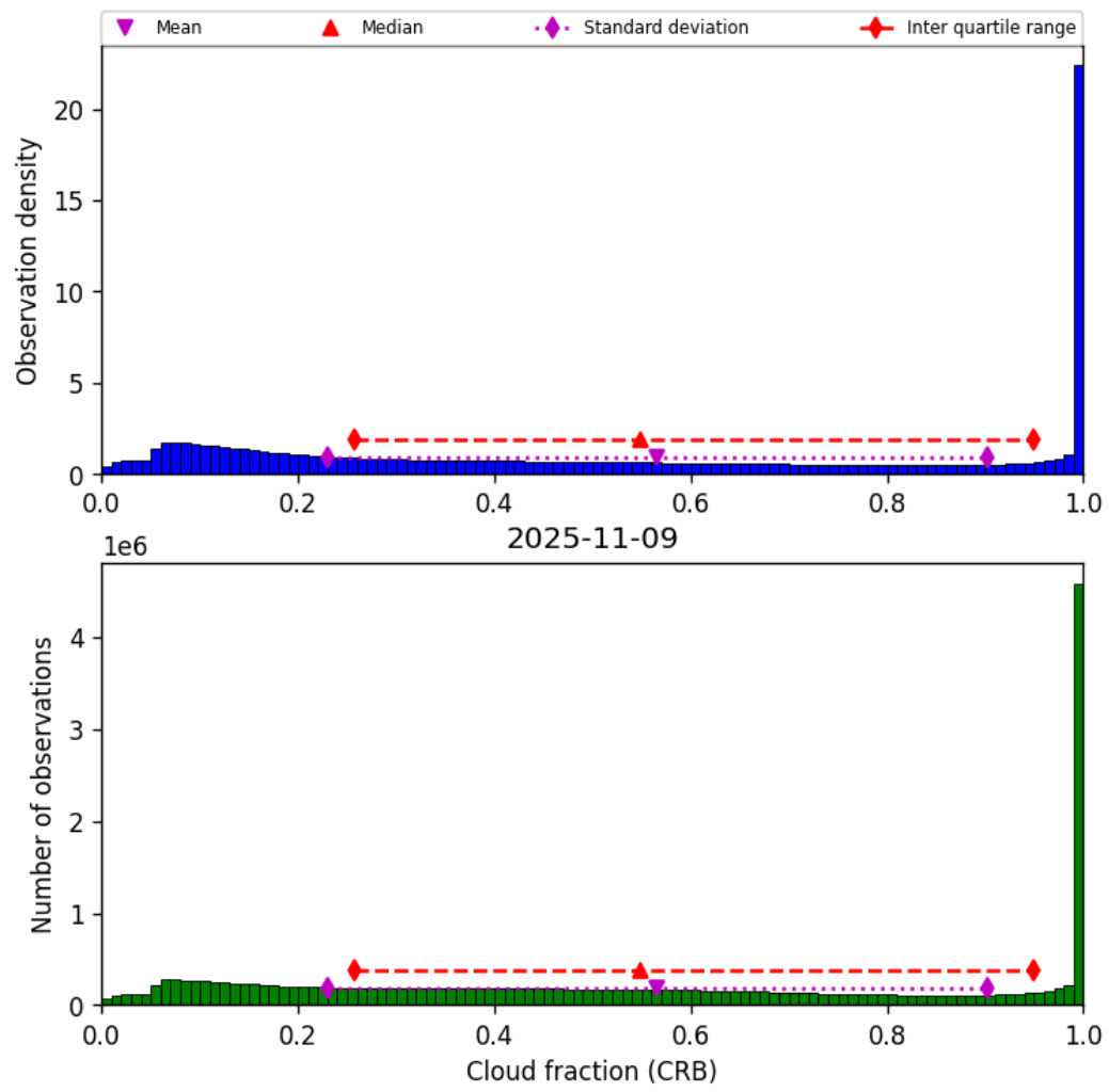
Figure 42: Histogram of “Cloud fraction (CRB)” for 2025-11-08 to 2025-11-10
