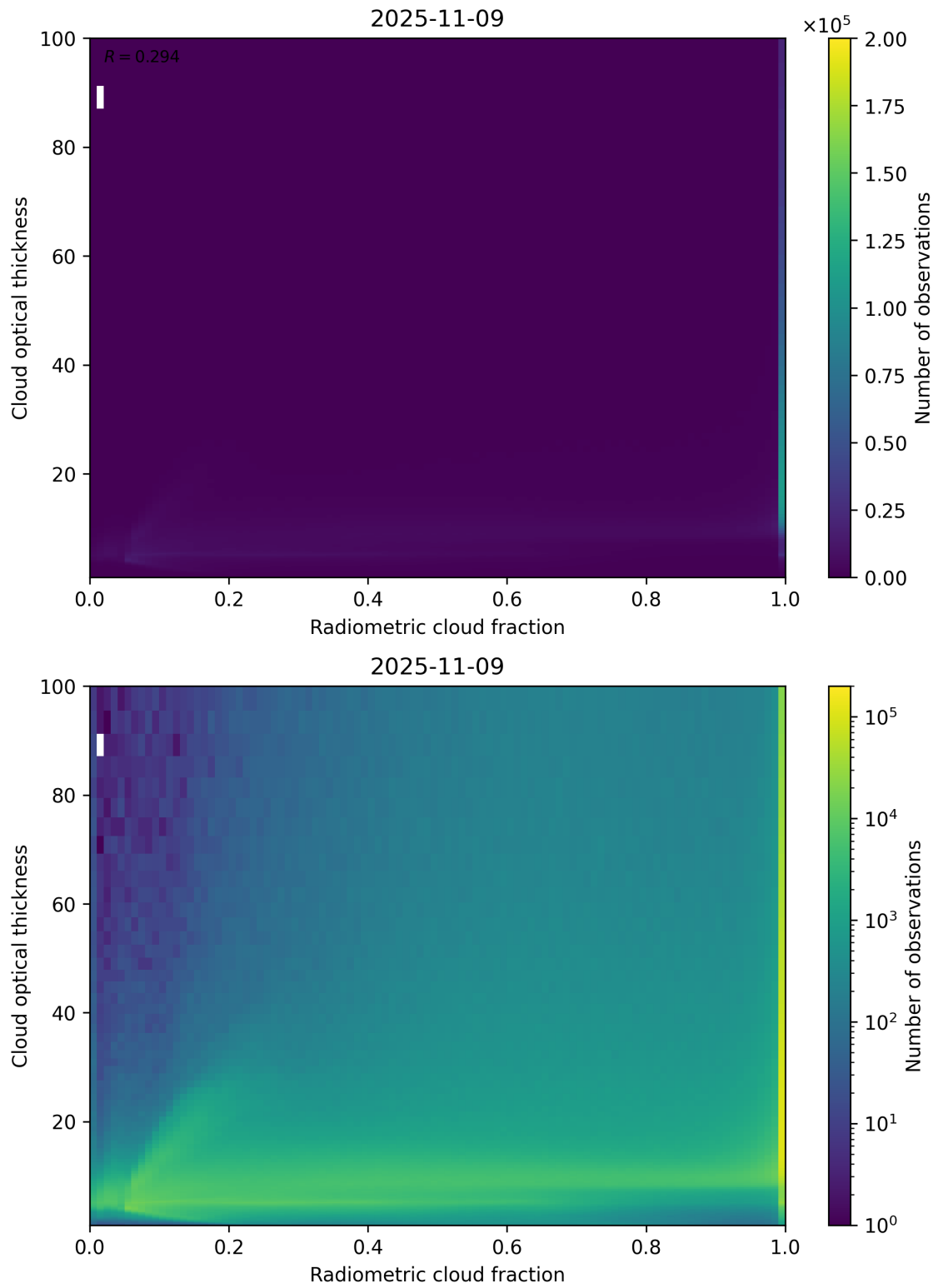
Figure 75: Scatter density plot of “Radiometric cloud fraction” against “Cloud optical thickness” for 2025-11-08 to 2025-11-10.
