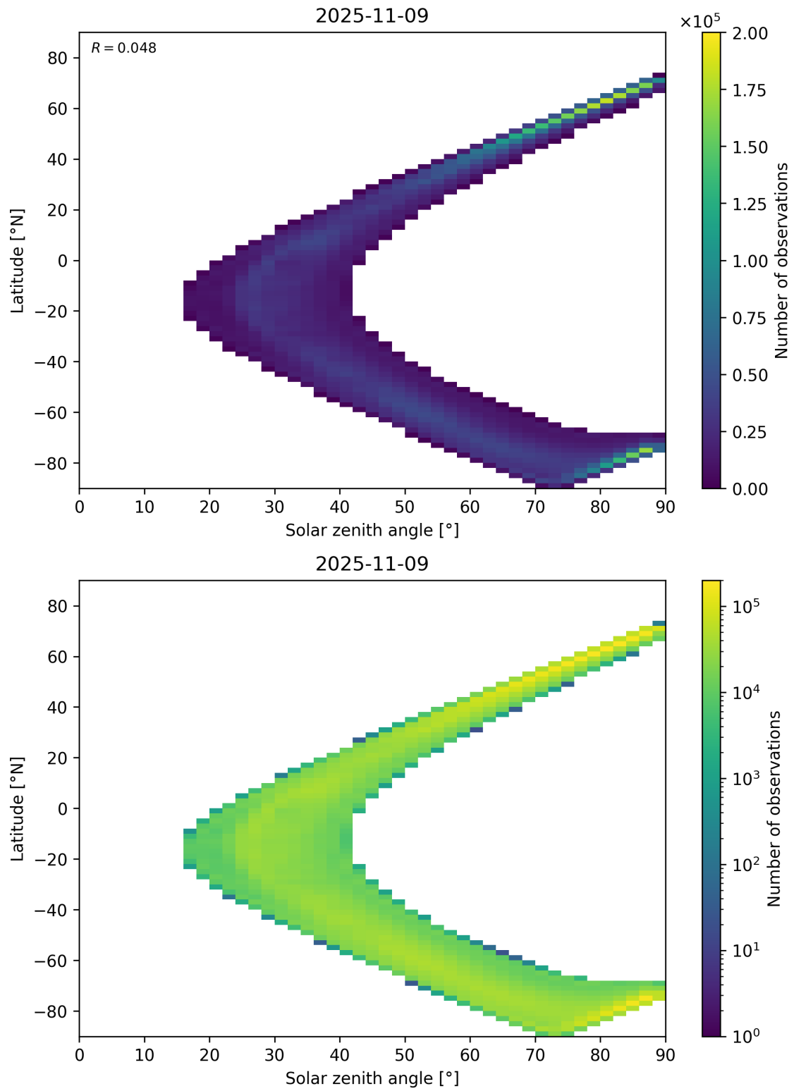
Figure 105: Scatter density plot of “Solar zenith angle” against “Latitude” for 2025-11-08 to 2025-11-10.
