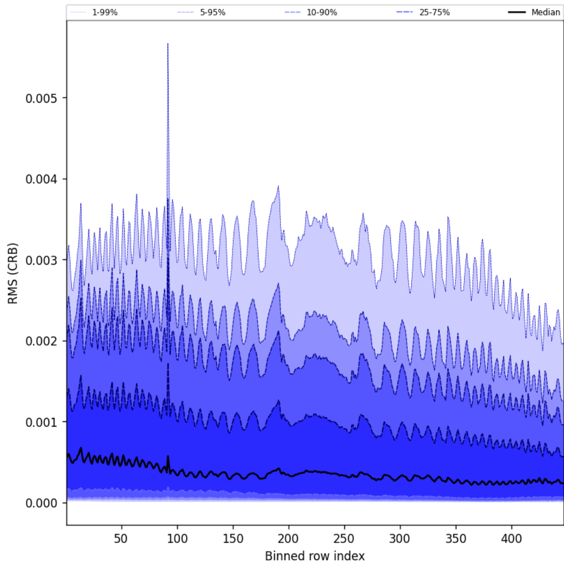
Figure 64: Along track statistics of “RMS (CRB)” for 2025-11-08 to 2025-11-10
