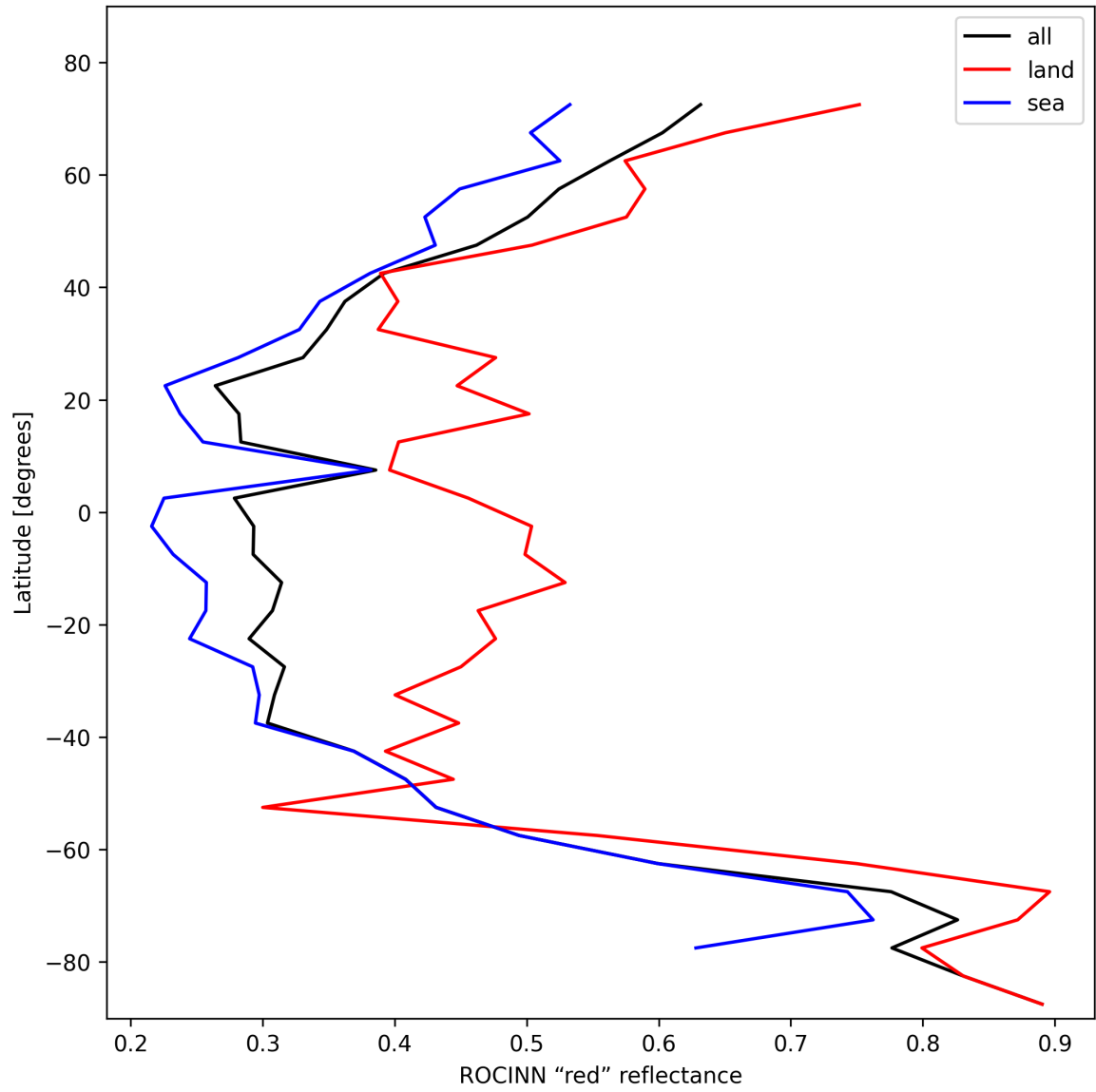
Figure 37: Zonal average of "ROCINN "red" reflectance" for 2025-11-08 to 2025-11-10.
