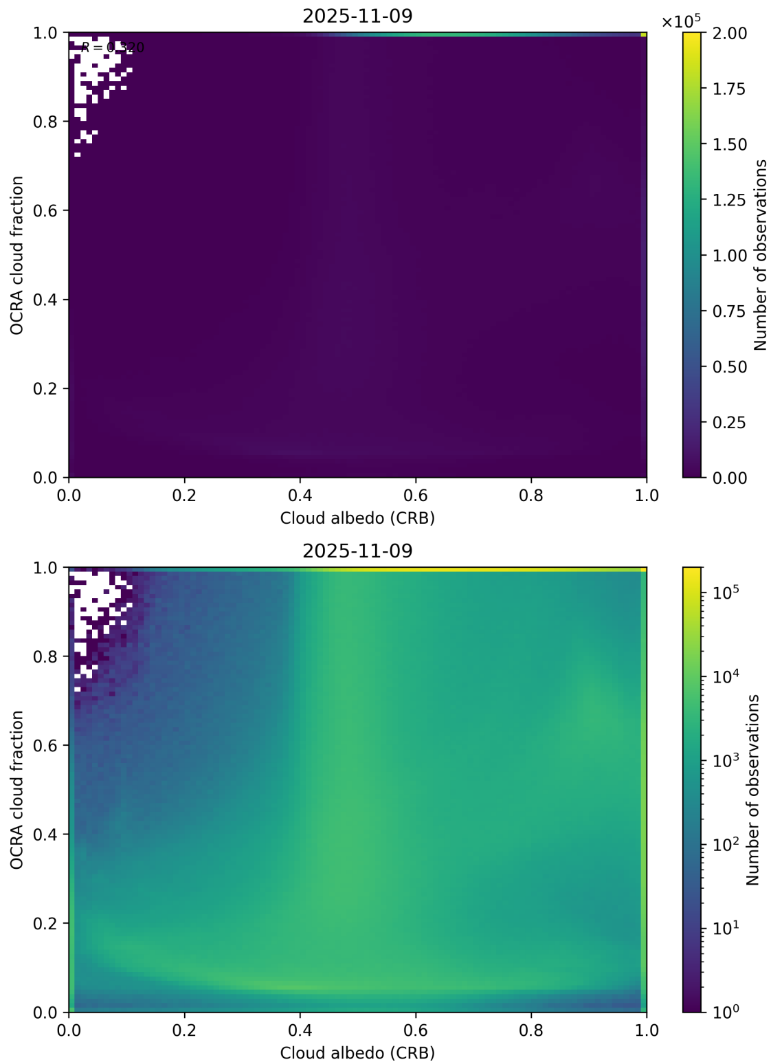
Figure 70: Scatter density plot of “Cloud albedo (CRB)” against “OCRA cloud fraction” for 2025-11-08 to 2025-11-10.
