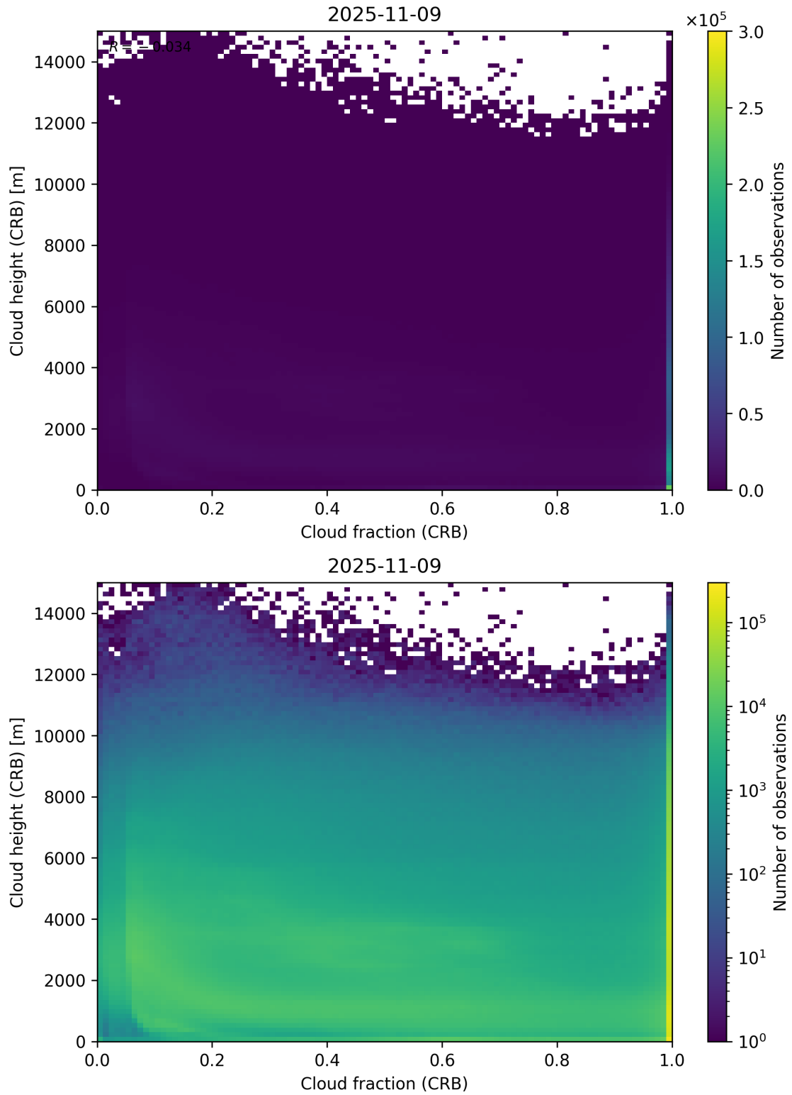
Figure 79: Scatter density plot of “Cloud fraction (CRB)” against “Cloud height (CRB)” for 2025-11-08 to 2025-11-10.
