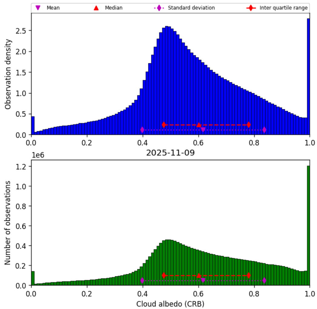
Figure 44: Histogram of “Cloud albedo (CRB)” for 2025-11-08 to 2025-11-10
