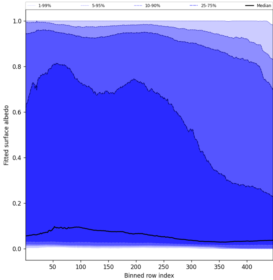
Figure 61: Along track statistics of “Fitted surface albedo” for 2025-11-08 to 2025-11-10
