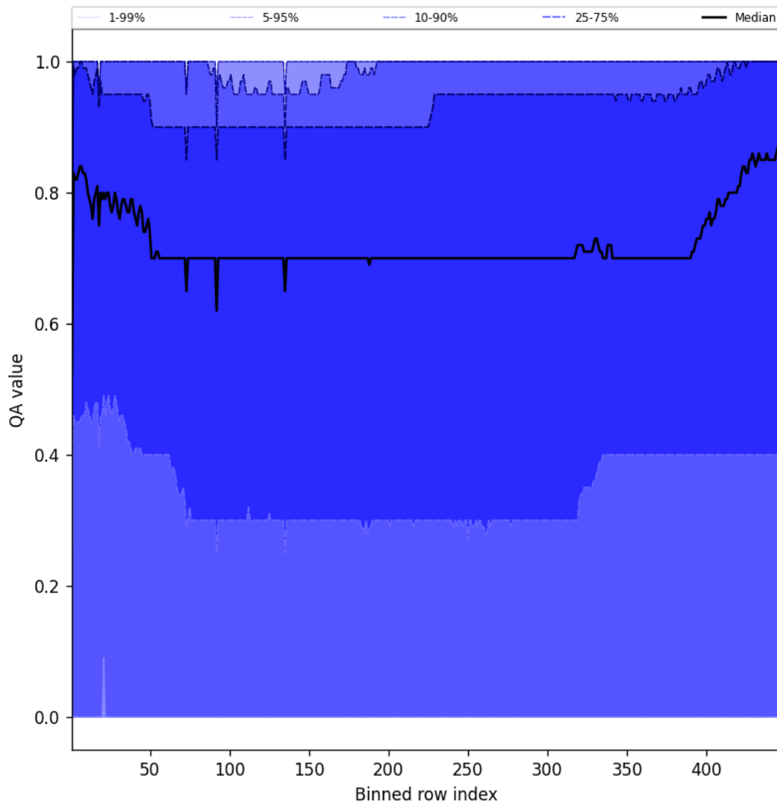
Figure 54: Along track statistics of “QA value” for 2025-11-08 to 2025-11-10
