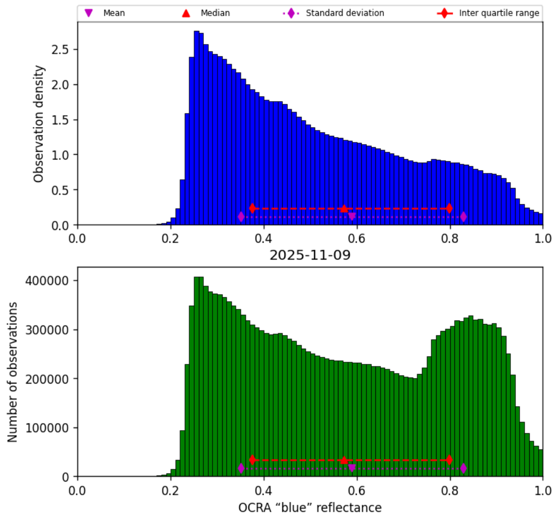
Figure 51: Histogram of "OCRA "blue" reflectance" for 2025-11-08 to 2025-11-10
