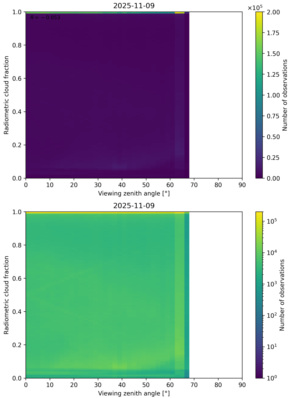
Figure 107: Scatter density plot of “Viewing zenith angle” against “Radiometric cloud fraction” for 2025-11-08 to 2025-11-10.
