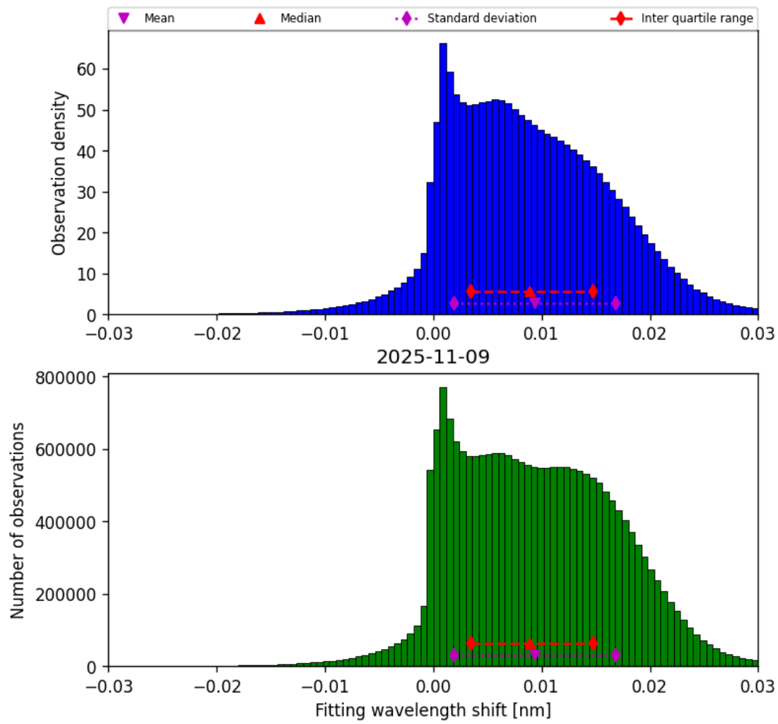
Figure 49: Histogram of “Fitting wavelength shift” for 2025-11-08 to 2025-11-10
