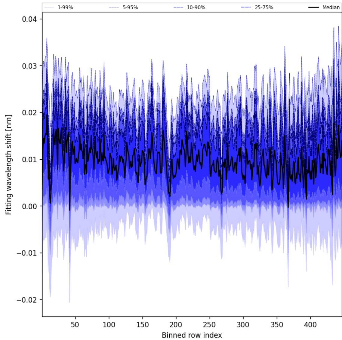
Figure 65: Along track statistics of “Fitting wavelength shift” for 2025-11-08 to 2025-11-10
