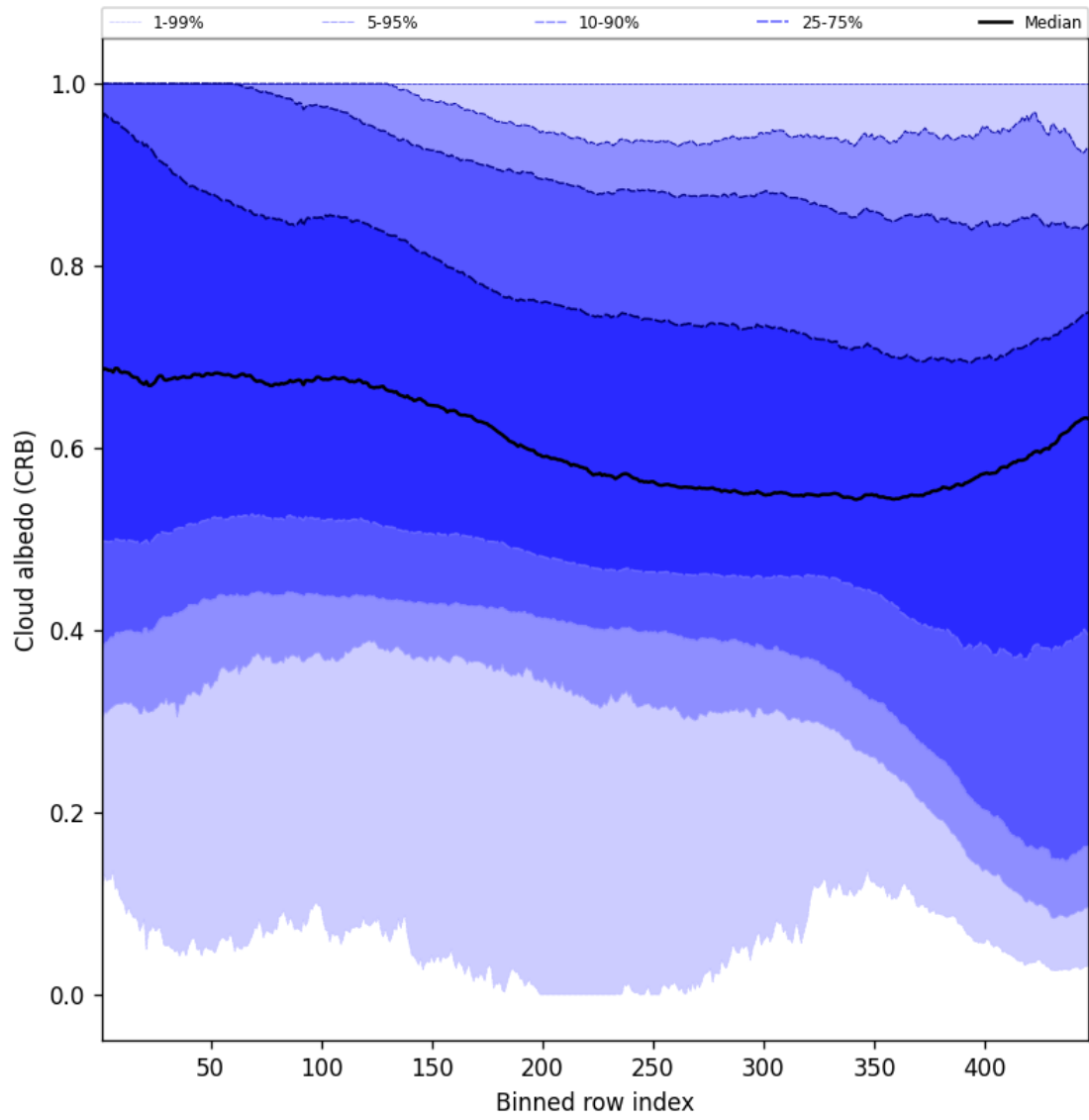
Figure 60: Along track statistics of “Cloud albedo (CRB)” for 2025-11-08 to 2025-11-10
