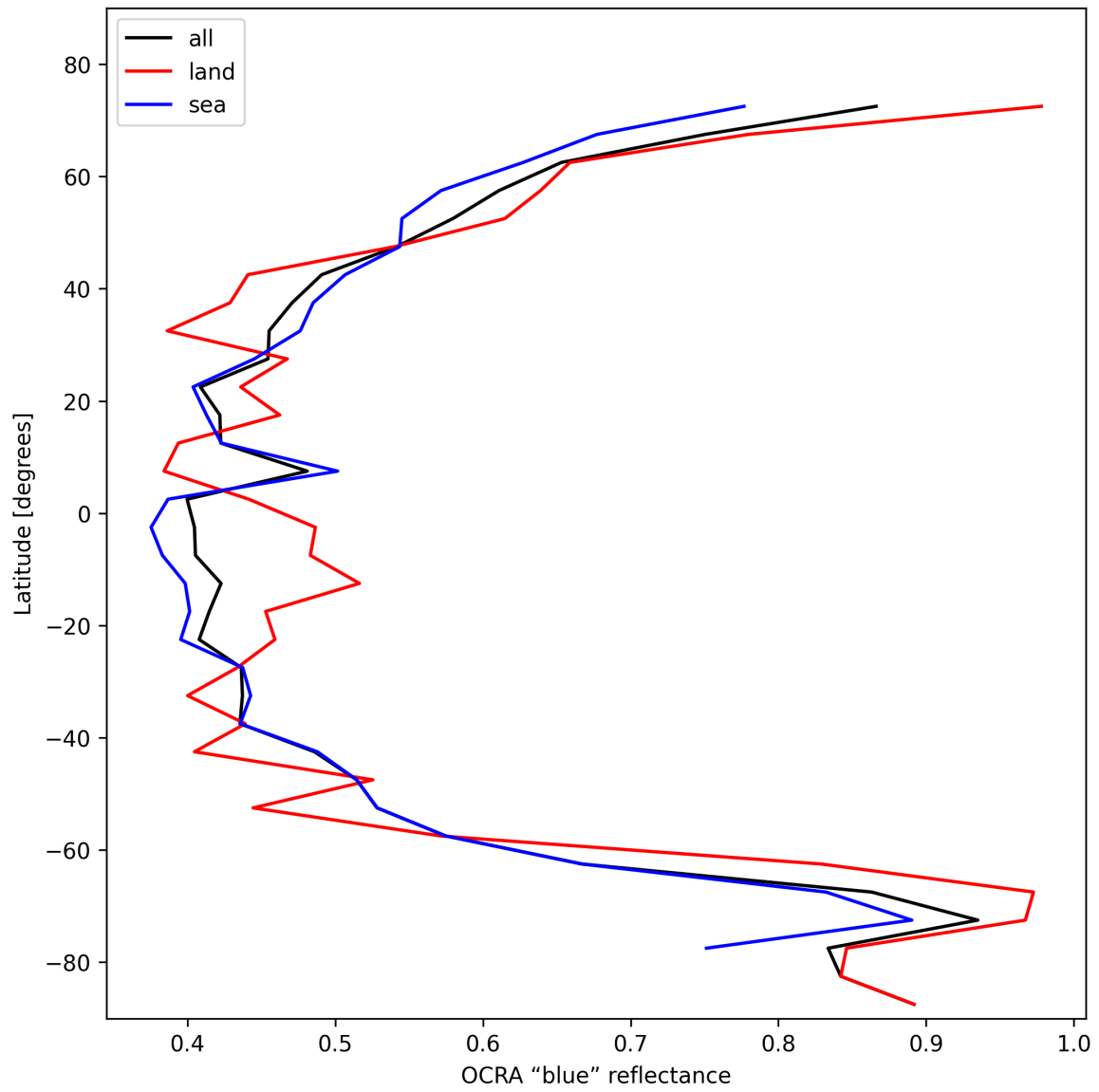
Figure 35: Zonal average of “OCRA “blue” reflectance” for 2025-11-08 to 2025-11-10.
