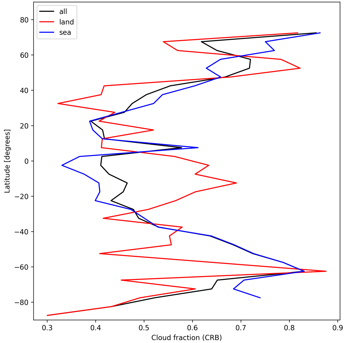
Figure 26: Zonal average of “Cloud fraction (CRB)” for 2025-11-08 to 2025-11-10.
