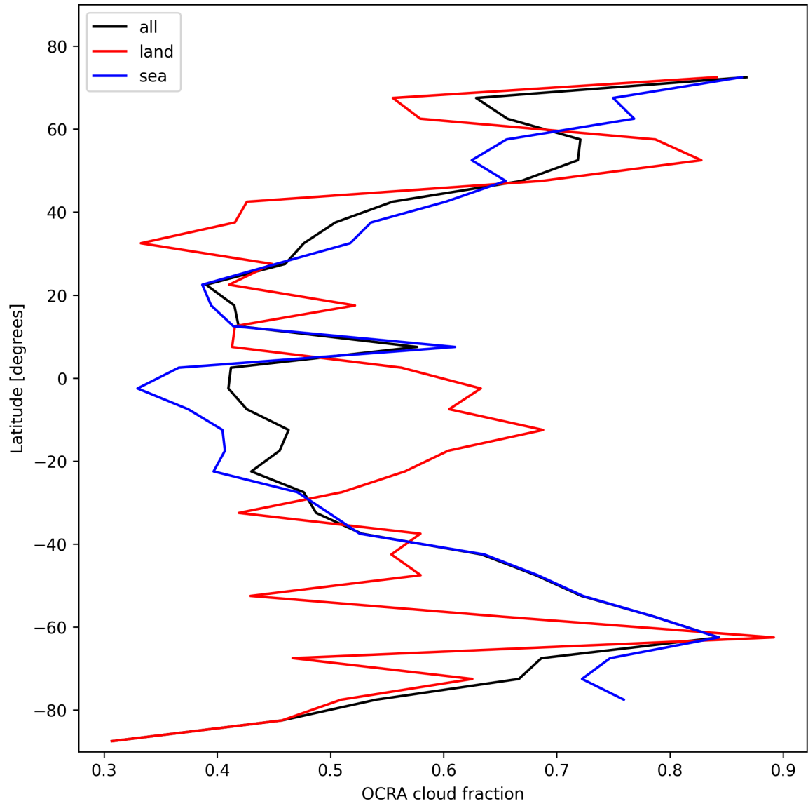
Figure 34: Zonal average of “OCRA cloud fraction” for 2025-11-08 to 2025-11-10.
