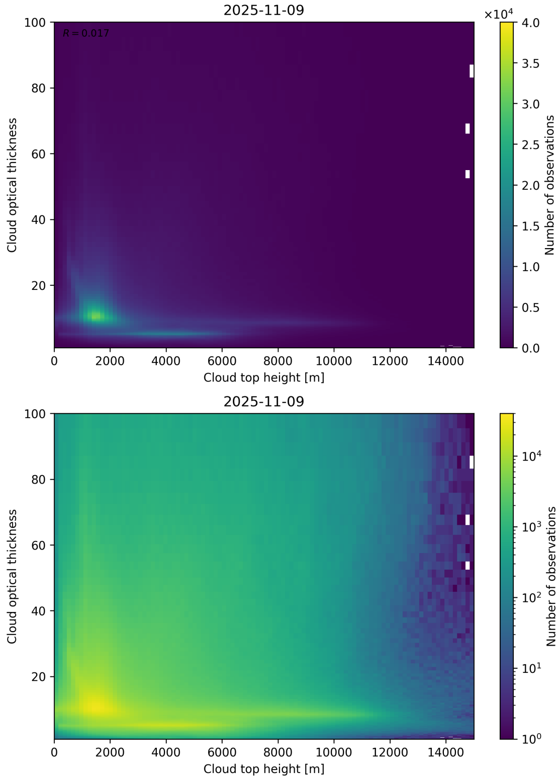
Figure 90: Scatter density plot of “Cloud top height” against “Cloud optical thickness” for 2025-11-08 to 2025-11-10.
