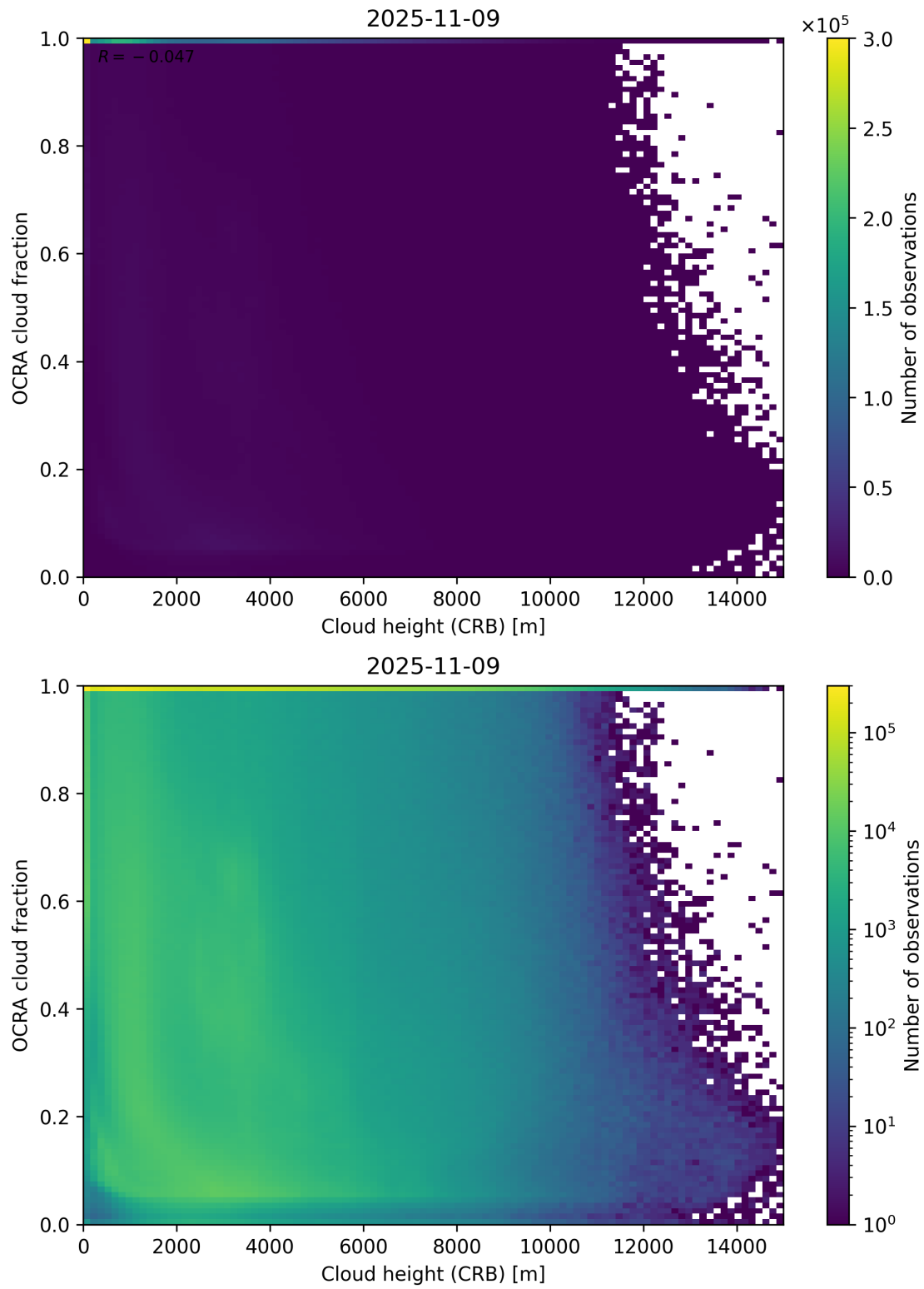
Figure 81: Scatter density plot of “Cloud height (CRB)” against “OCRA cloud fraction” for 2025-11-08 to 2025-11-10.
