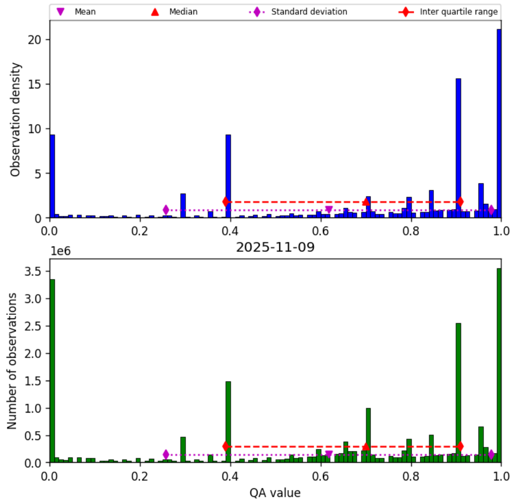
Figure 38: Histogram of “QA value” for 2025-11-08 to 2025-11-10
