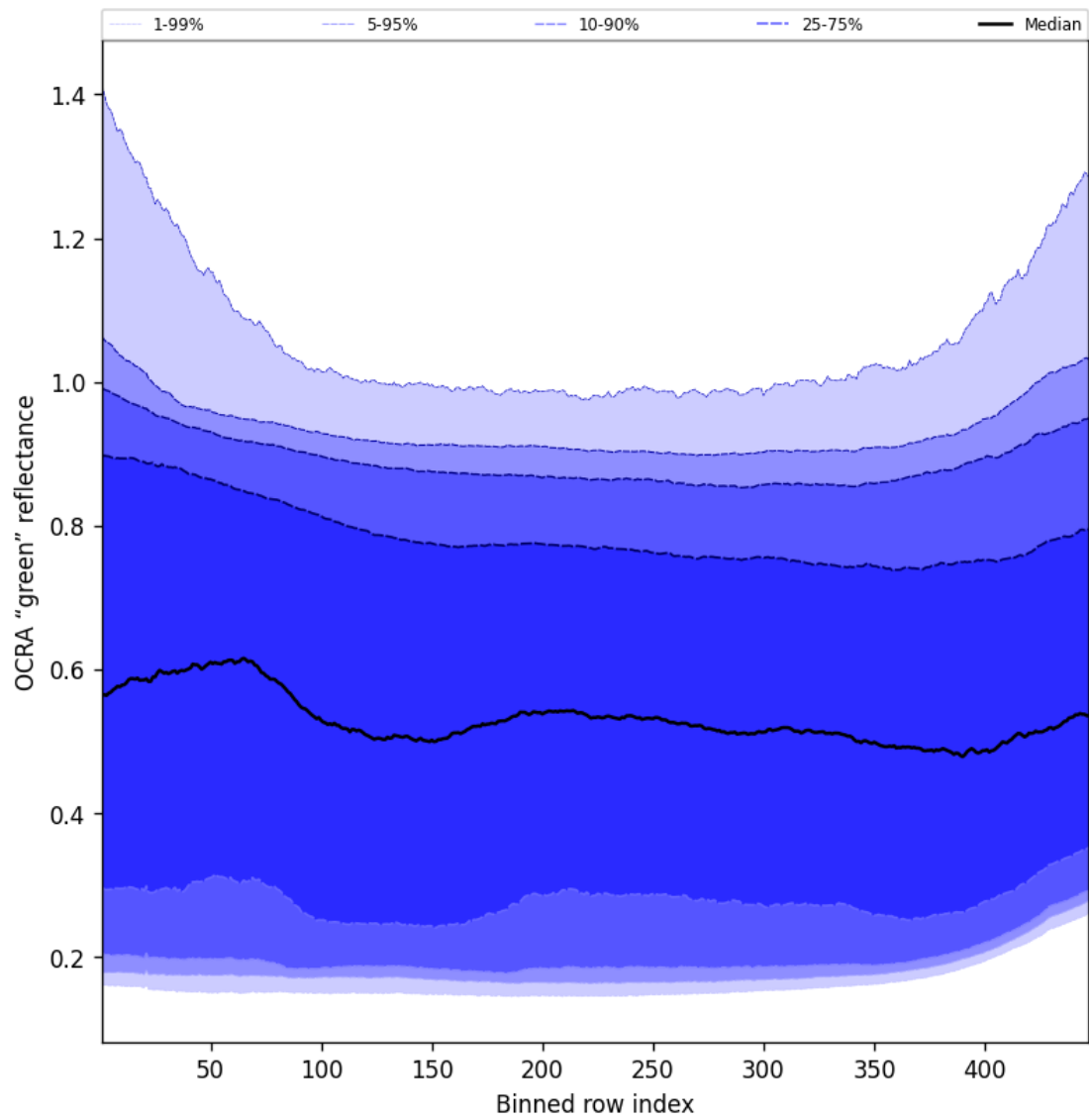
Figure 68: Along track statistics of “OCRA “green” reflectance” for 2025-11-08 to 2025-11-10
