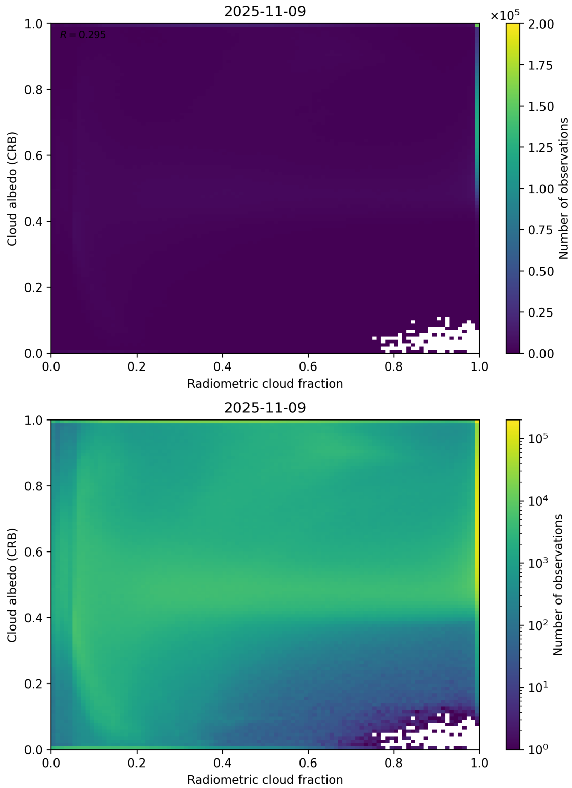
Figure 71: Scatter density plot of “Radiometric cloud fraction” against “Cloud albedo (CRB)” for 2025-11-08 to 2025-11-10.
