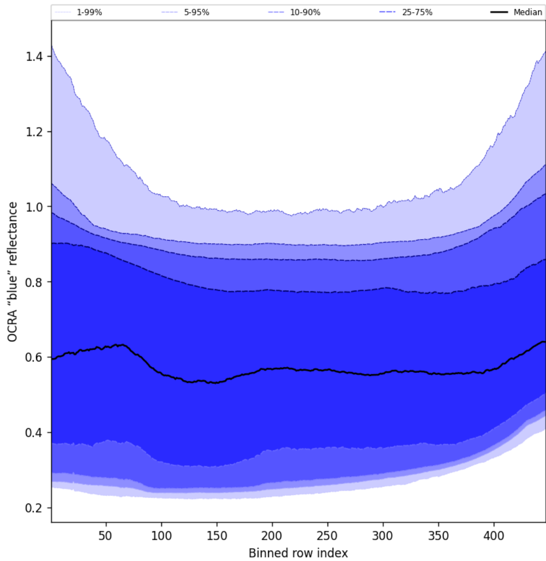
Figure 67: Along track statistics of "OCRA "blue" reflectance" for 2025-11-08 to 2025-11-10
