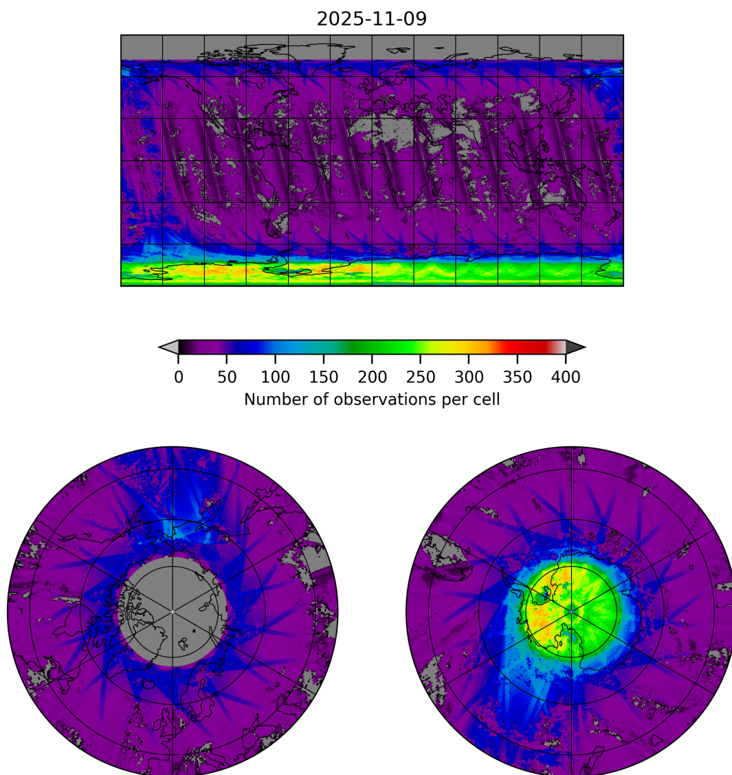
Figure 21: Map of the number of observations for 2025-11-08 to 2025-11-10
