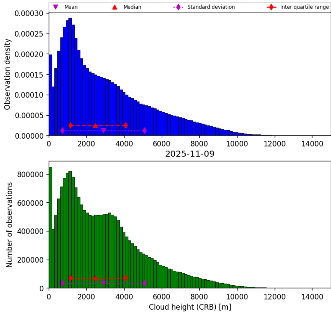
Figure 43: Histogram of “Cloud height (CRB)” for 2025-11-08 to 2025-11-10
