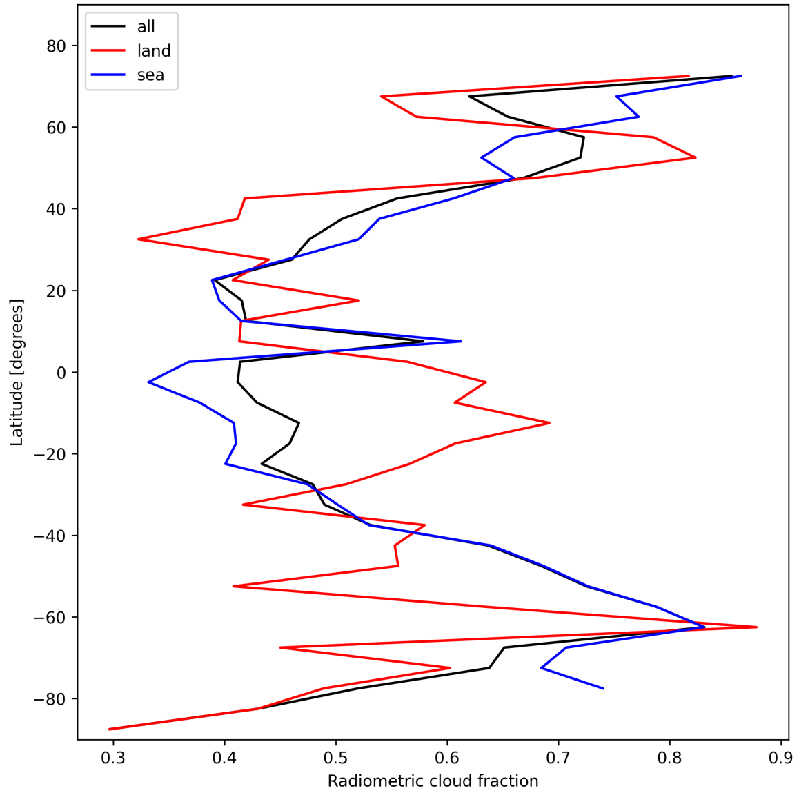
Figure 23: Zonal average of “Radiometric cloud fraction” for 2025-11-08 to 2025-11-10.
