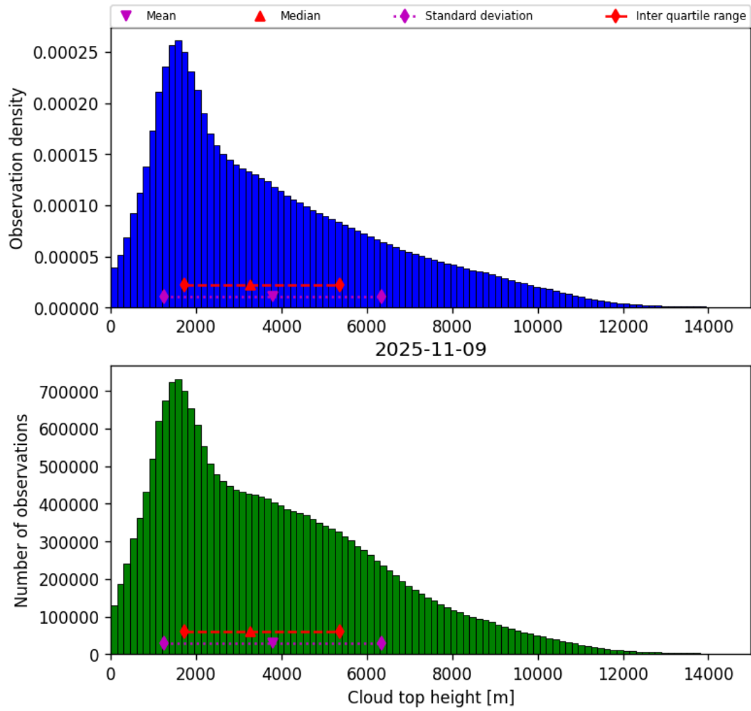
Figure 40: Histogram of “Cloud top height” for 2025-11-08 to 2025-11-10
