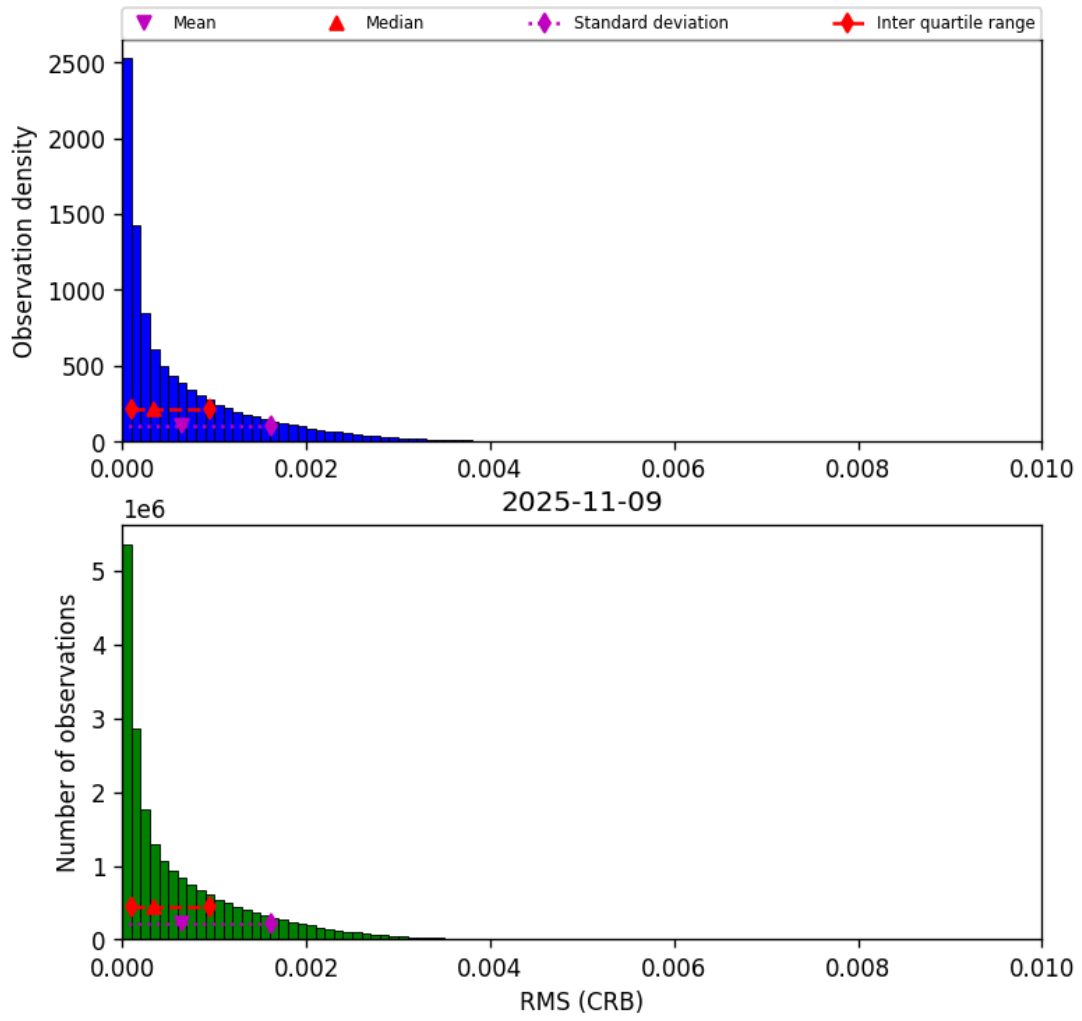
Figure 48: Histogram of “RMS (CRB)” for 2025-11-08 to 2025-11-10
