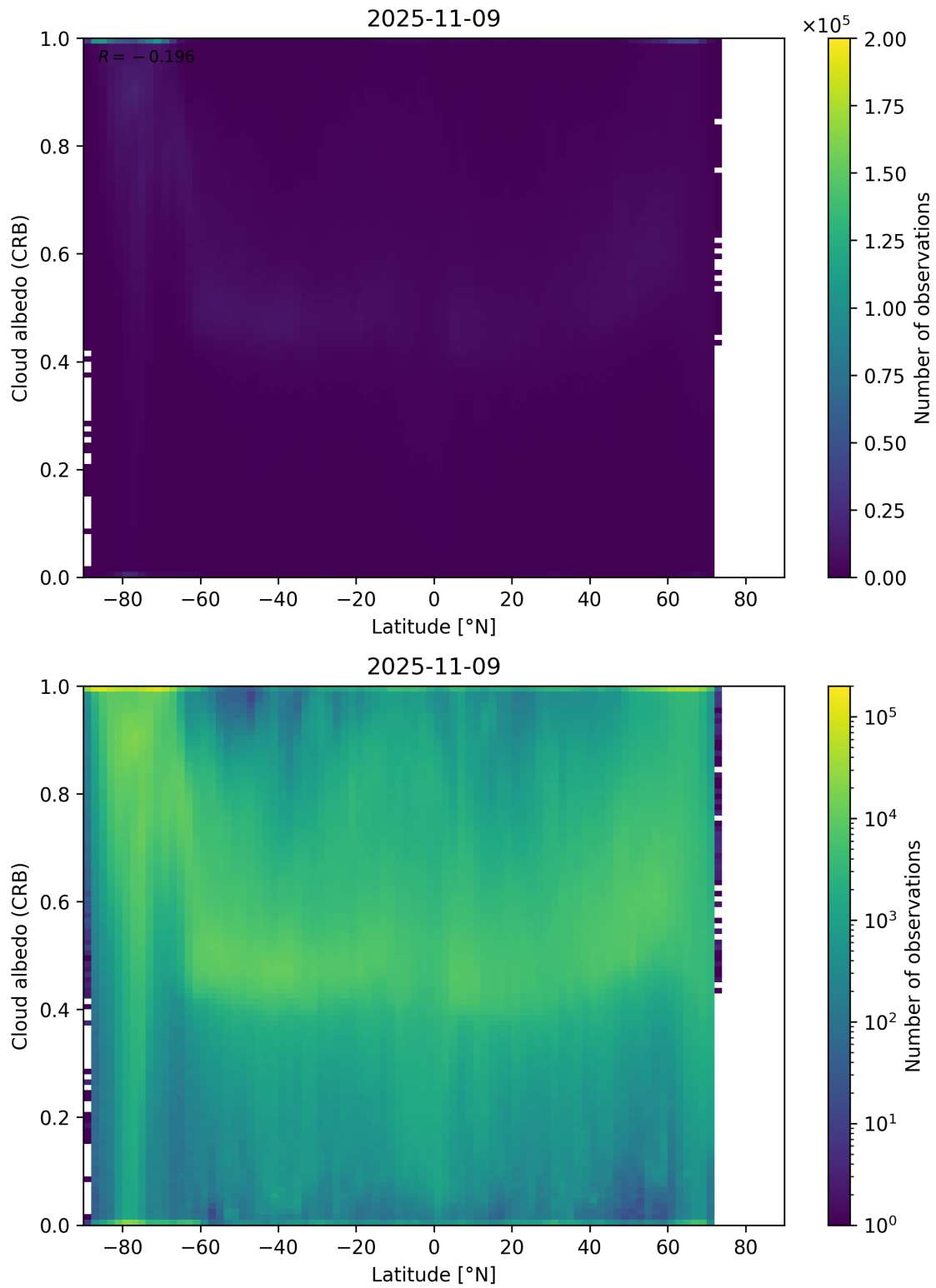
Figure 91: Scatter density plot of “Latitude” against “Cloud albedo (CRB)” for 2025-11-08 to 2025-11-10.
