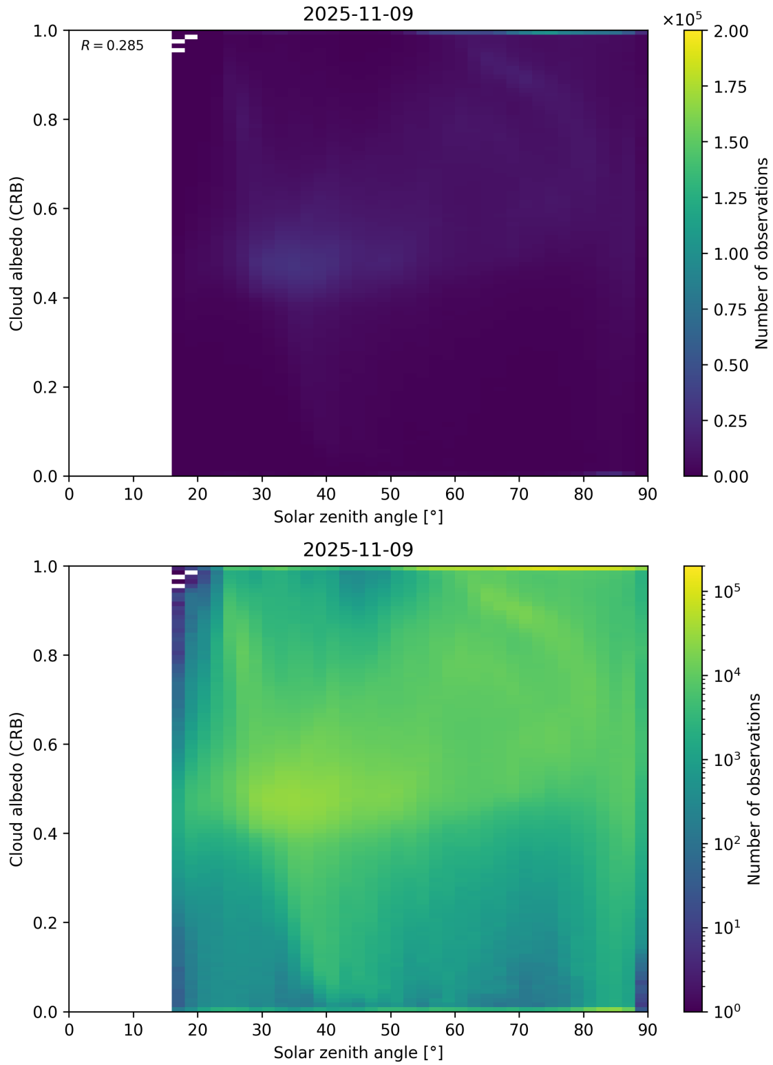
Figure 98: Scatter density plot of “Solar zenith angle” against “Cloud albedo (CRB)” for 2025-11-08 to 2025-11-10.
