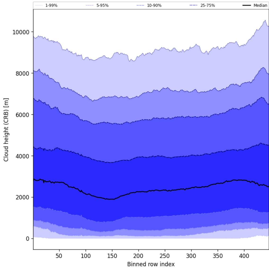
Figure 59: Along track statistics of “Cloud height (CRB)” for 2025-11-08 to 2025-11-10
