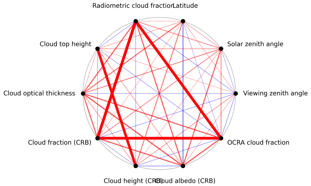
Figure 1: Map of correlation graph for 2025-11-08 to 2025-11-10.
