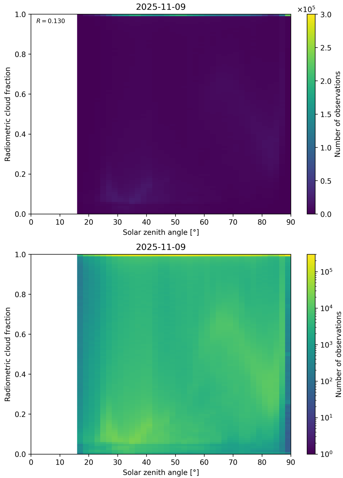
Figure 99: Scatter density plot of “Solar zenith angle” against “Radiometric cloud fraction” for 2025-11-08 to 2025-11-10.
