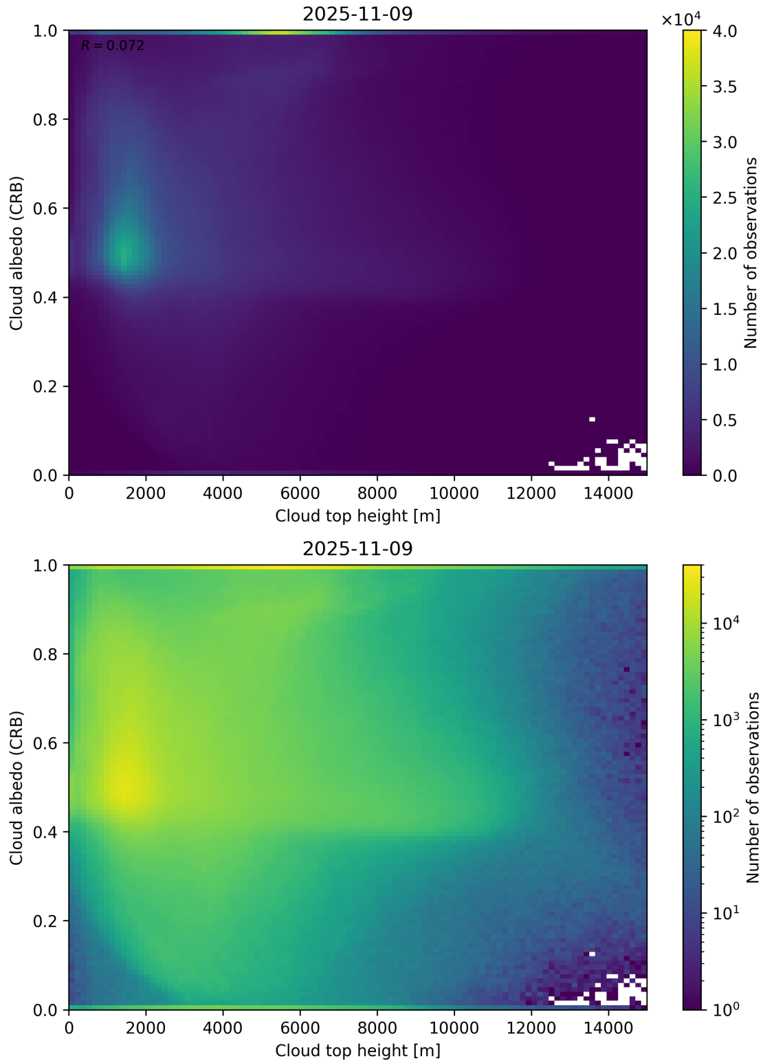
Figure 86: Scatter density plot of “Cloud top height” against “Cloud albedo (CRB)” for 2025-11-08 to 2025-11-10.
