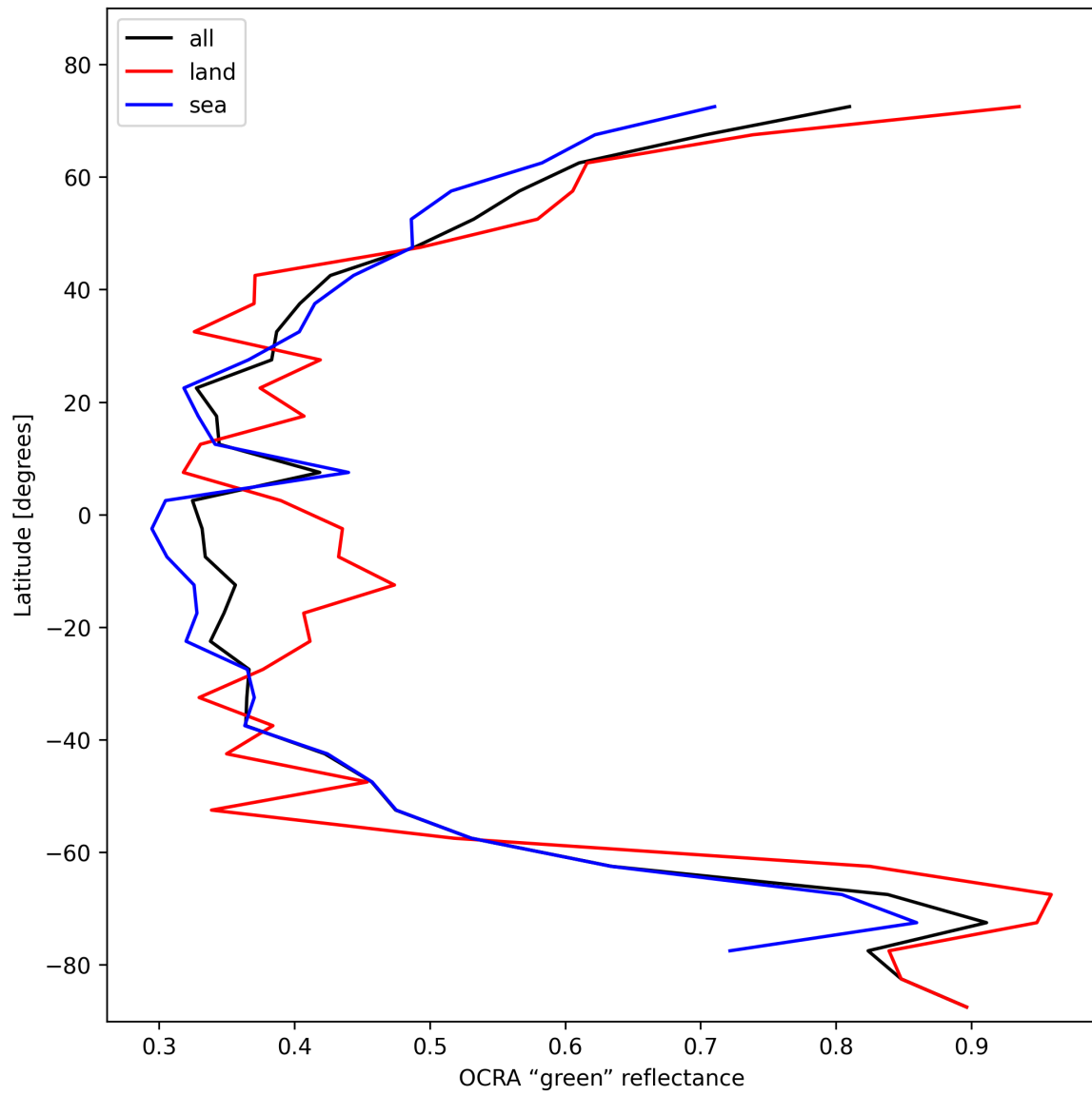
Figure 36: Zonal average of “OCRA “green” reflectance” for 2025-11-08 to 2025-11-10.
