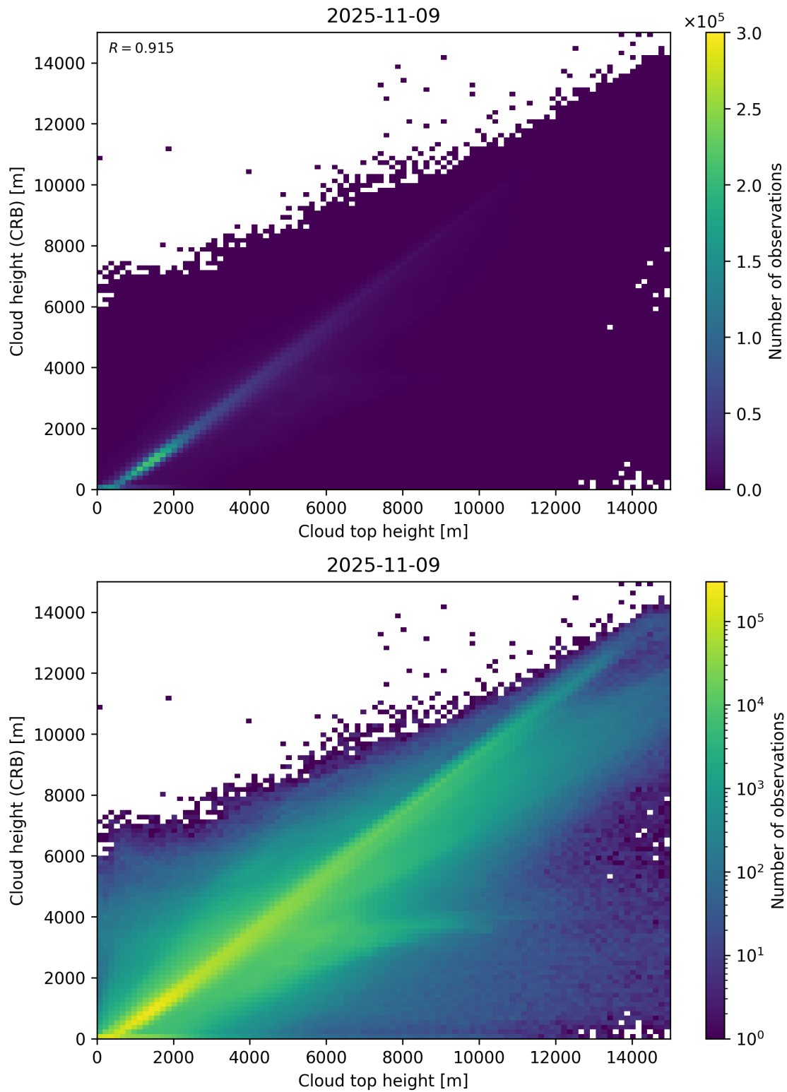
Figure 89: Scatter density plot of “Cloud top height” against “Cloud height (CRB)” for 2025-11-08 to 2025-11-10.
