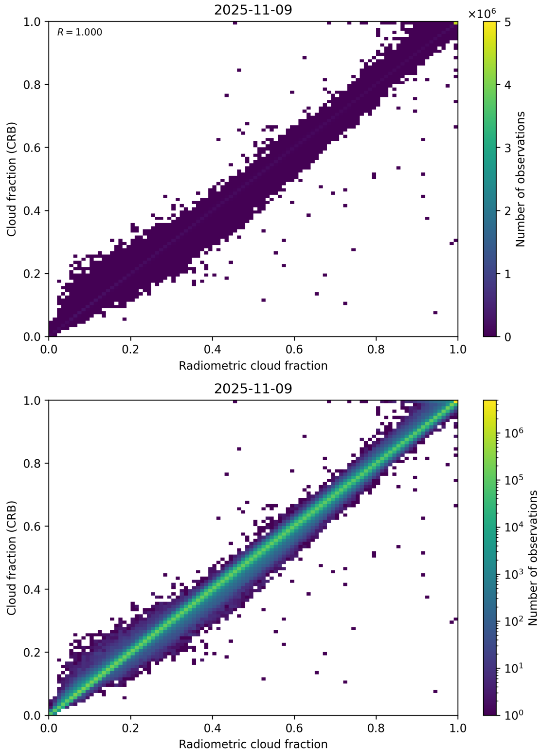
Figure 73: Scatter density plot of “Radiometric cloud fraction” against “Cloud fraction (CRB)” for 2025-11-08 to 2025-11-10.
