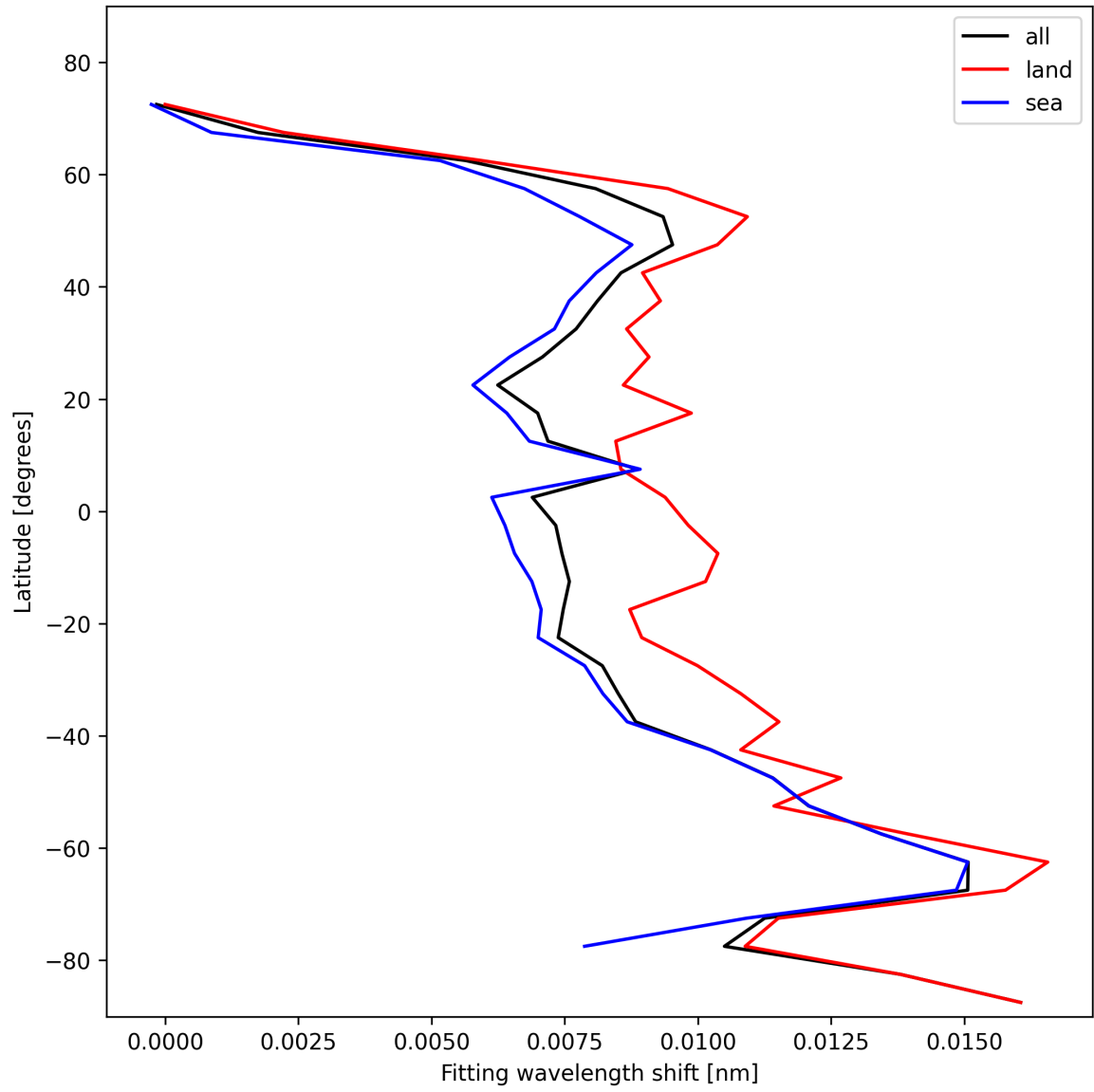
Figure 33: Zonal average of “Fitting wavelength shift” for 2025-11-08 to 2025-11-10.
