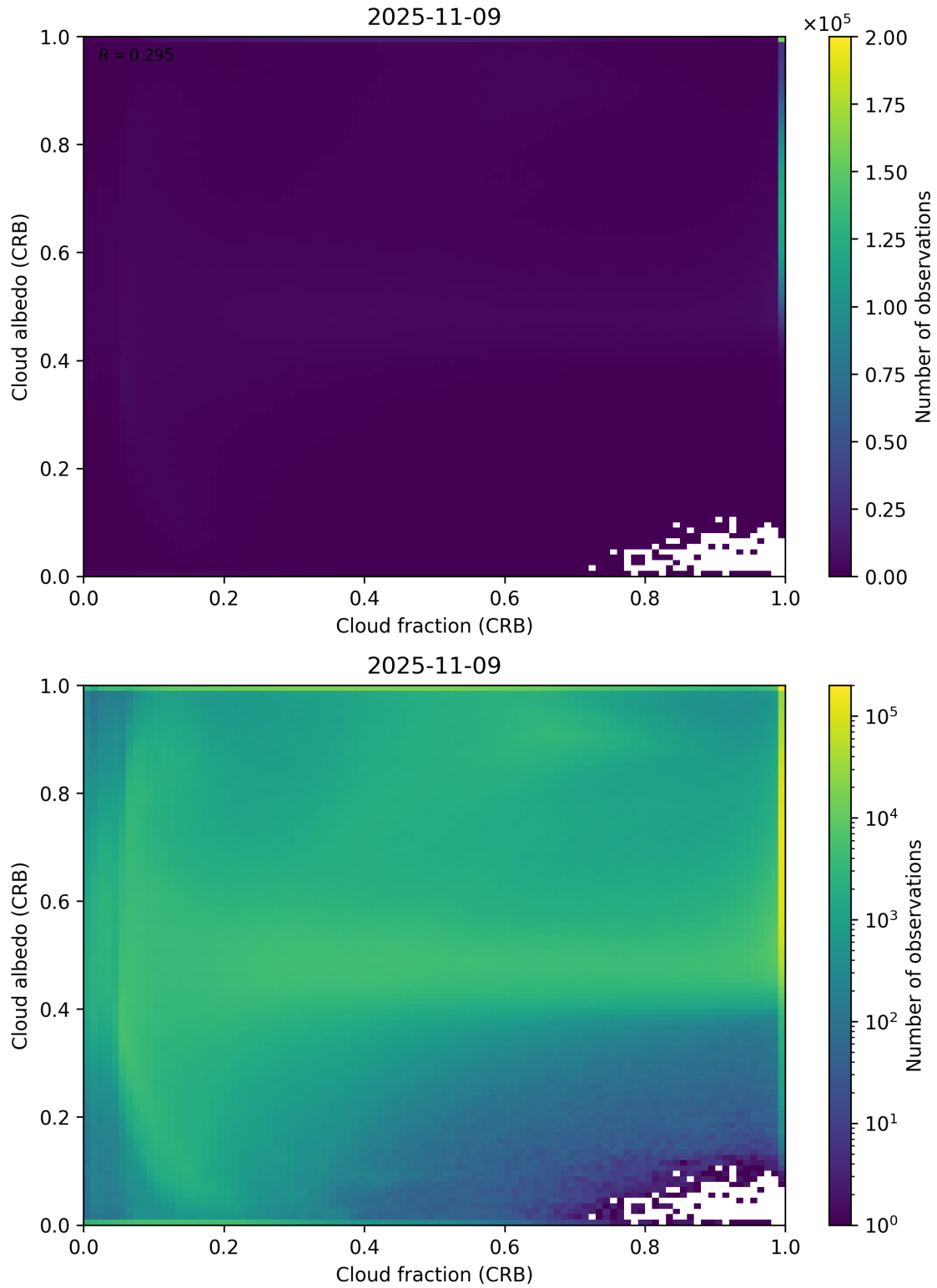
Figure 77: Scatter density plot of “Cloud fraction (CRB)” against “Cloud albedo (CRB)” for 2025-11-08 to 2025-11-10.
