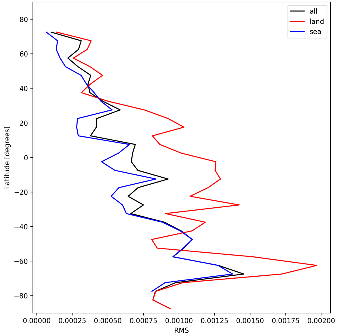
Figure 31: Zonal average of “RMS” for 2025-11-12 to 2025-11-13.
