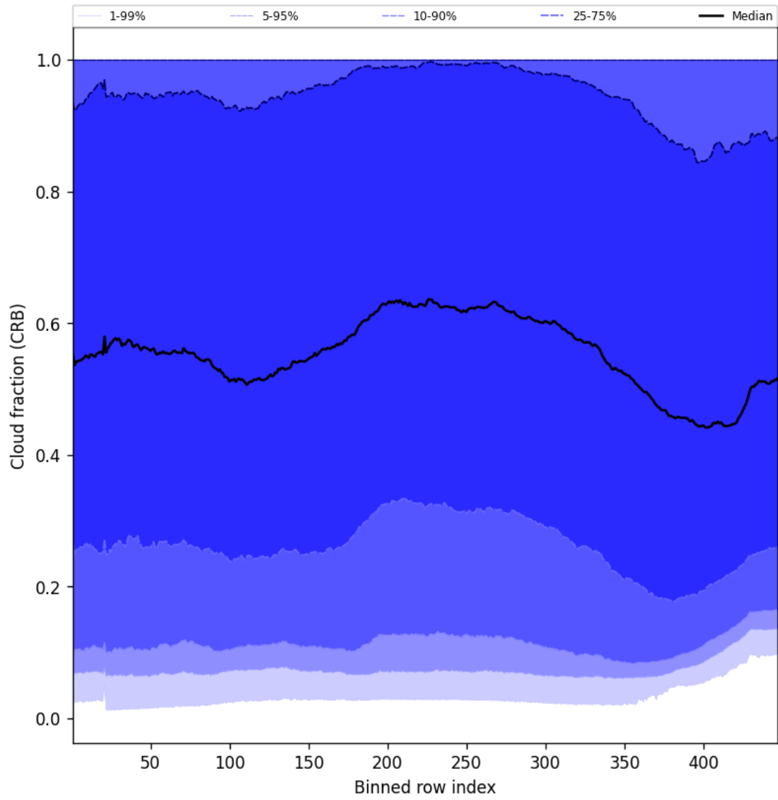
Figure 58: Along track statistics of “Cloud fraction (CRB)” for 2025-11-12 to 2025-11-13
