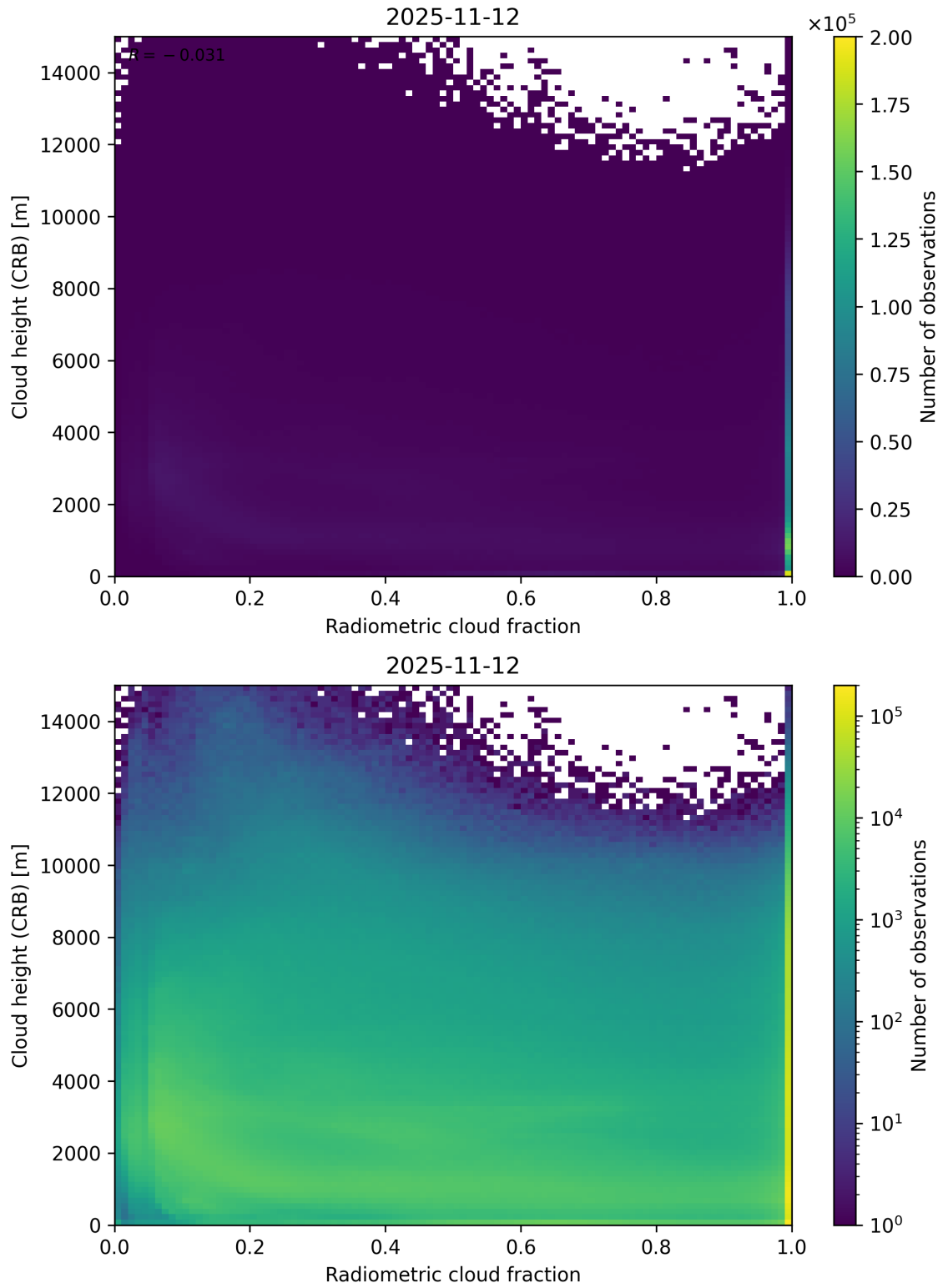
Figure 74: Scatter density plot of “Radiometric cloud fraction” against “Cloud height (CRB)” for 2025-11-12 to 2025-11-13.
