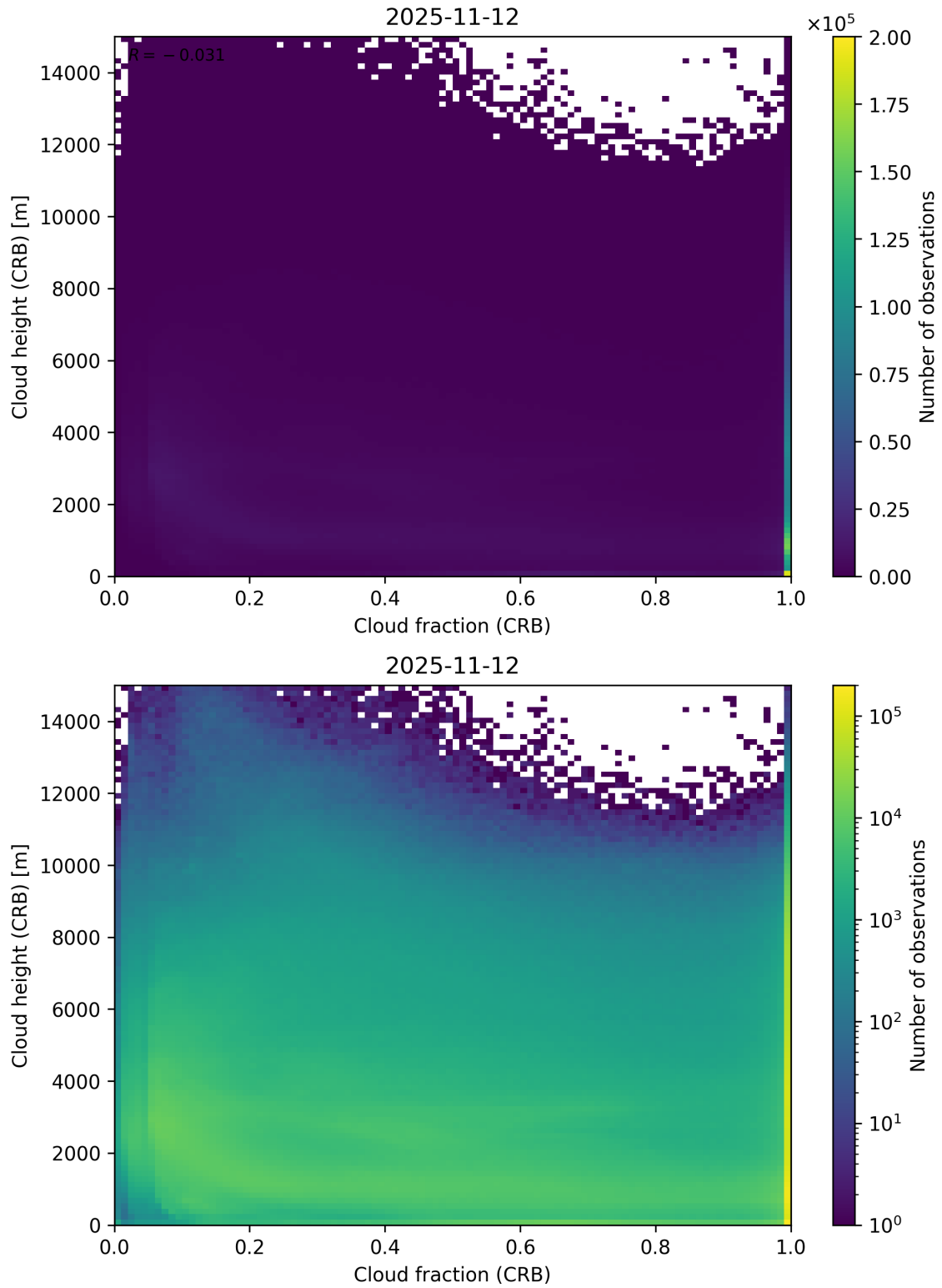
Figure 79: Scatter density plot of “Cloud fraction (CRB)” against “Cloud height (CRB)” for 2025-11-12 to 2025-11-13.
