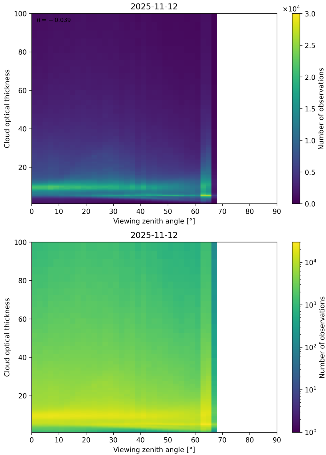
Figure 111: Scatter density plot of “Viewing zenith angle” against “Cloud optical thickness” for 2025-11-12 to 2025-11-13.
