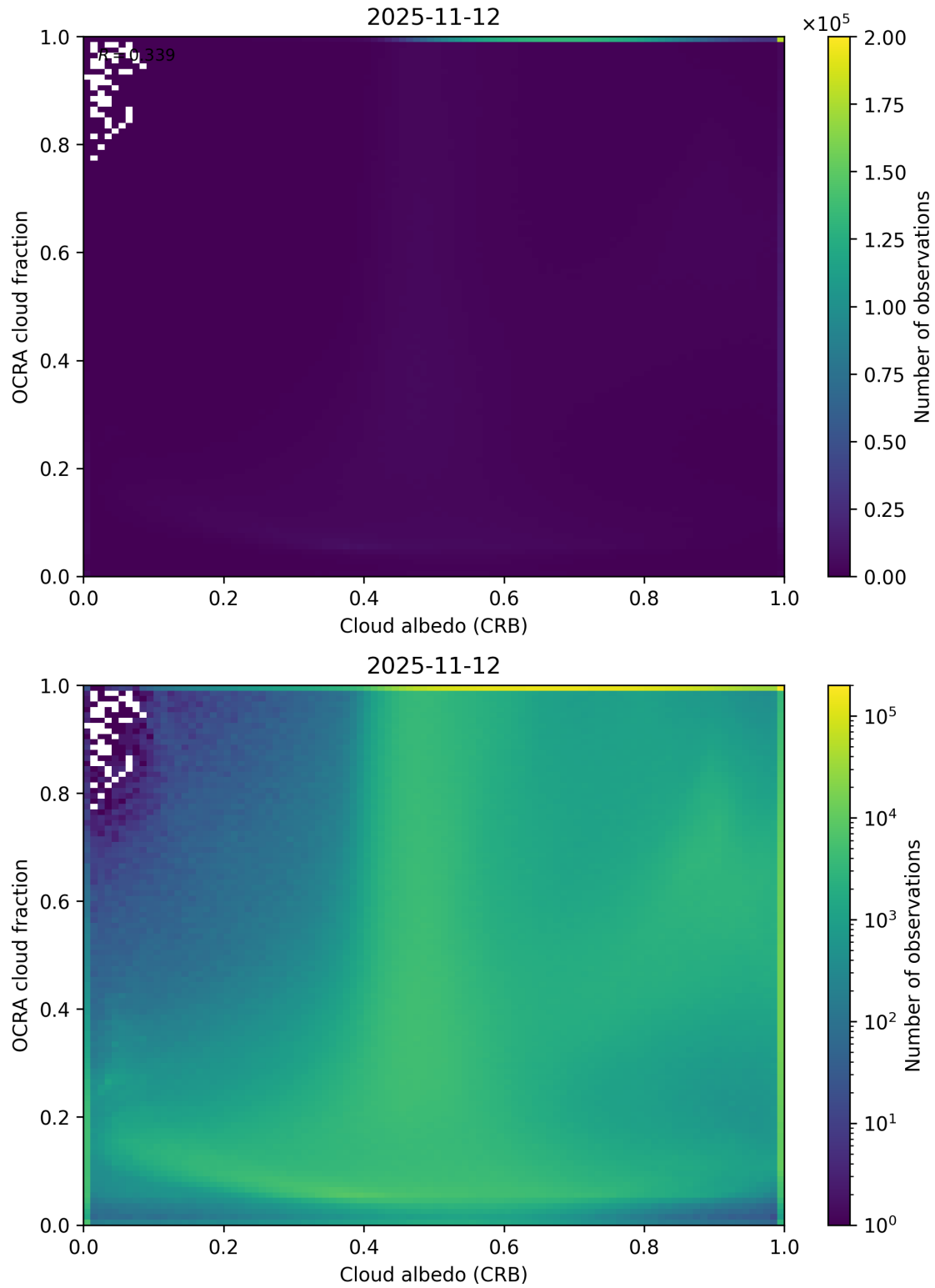
Figure 70: Scatter density plot of “Cloud albedo (CRB)” against “OCRA cloud fraction” for 2025-11-12 to 2025-11-13.
