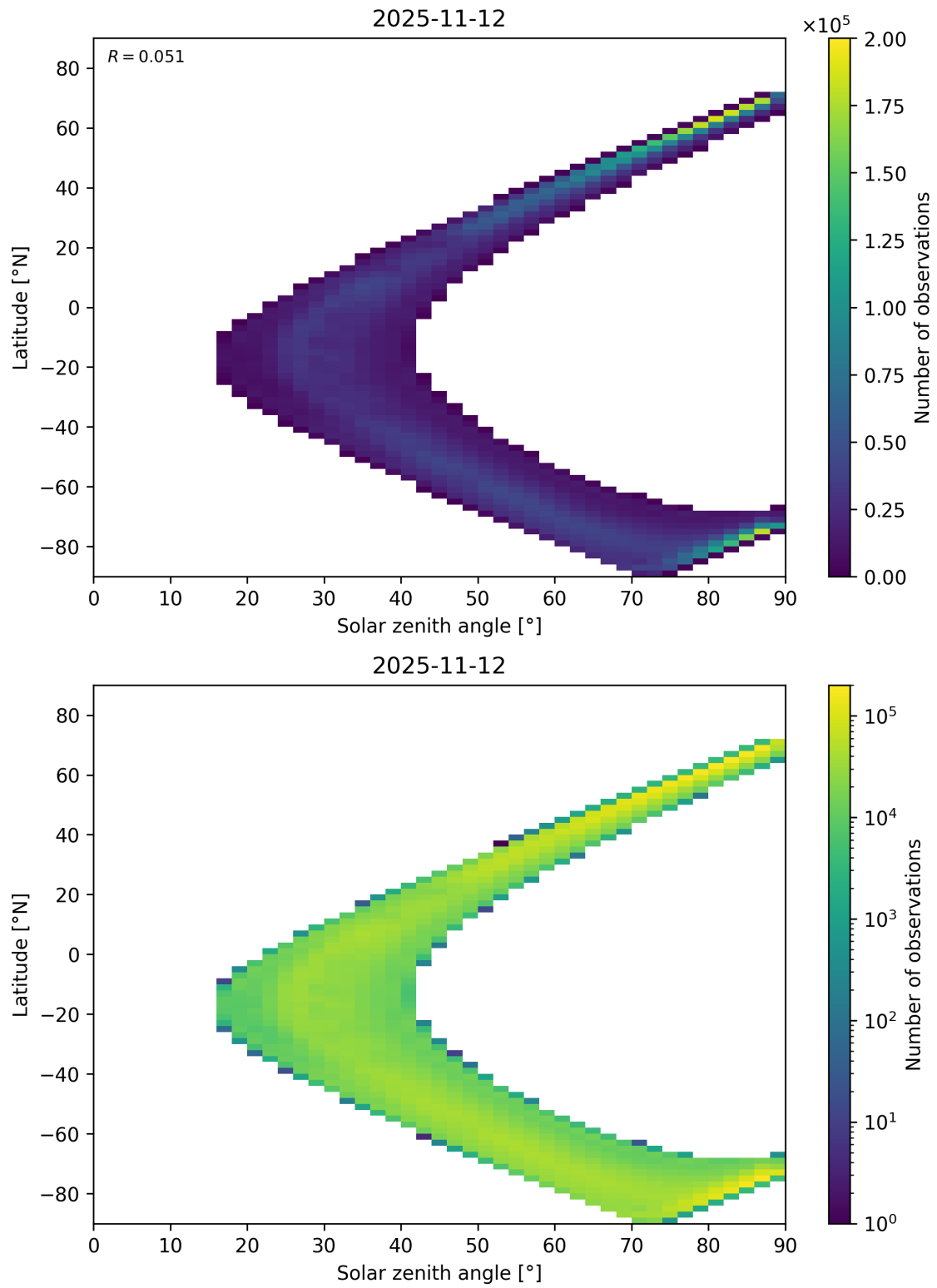
Figure 105: Scatter density plot of “Solar zenith angle” against “Latitude” for 2025-11-12 to 2025-11-13.
