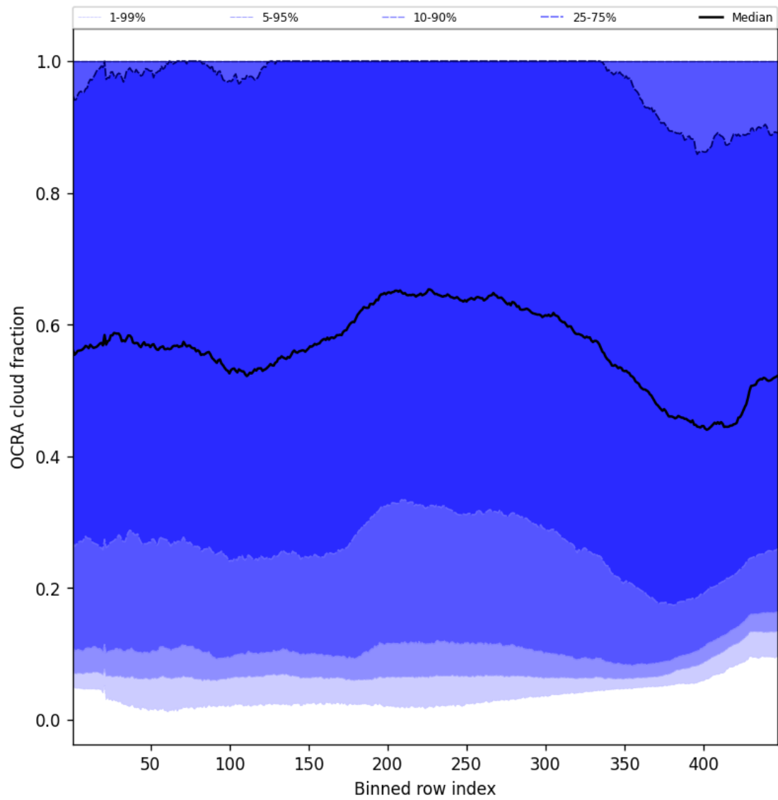
Figure 66: Along track statistics of “OCRA cloud fraction” for 2025-11-12 to 2025-11-13
