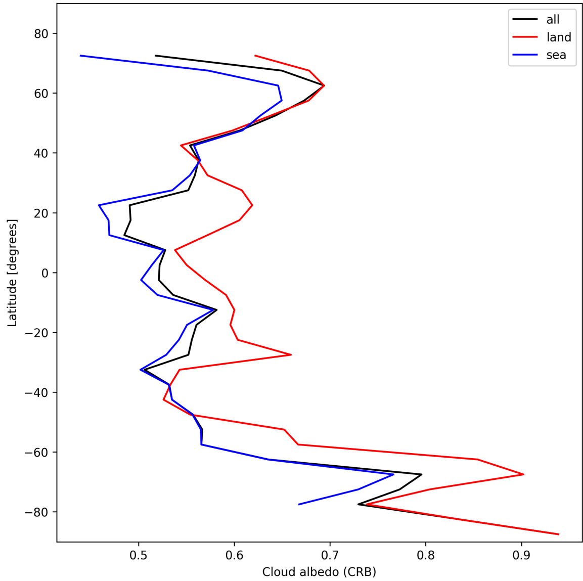
Figure 28: Zonal average of “Cloud albedo (CRB)” for 2025-11-12 to 2025-11-13.
