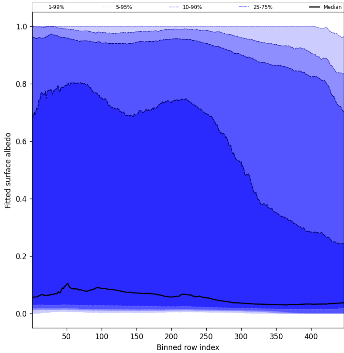
Figure 61: Along track statistics of “Fitted surface albedo” for 2025-11-12 to 2025-11-13
