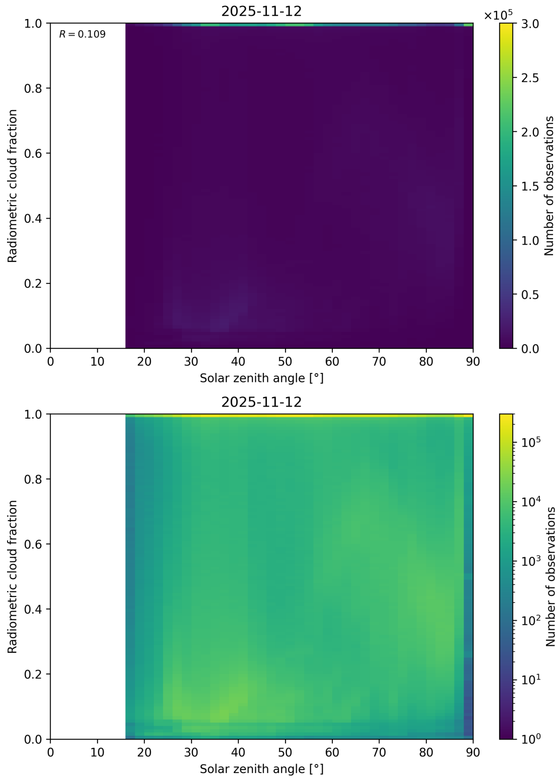
Figure 99: Scatter density plot of “Solar zenith angle” against “Radiometric cloud fraction” for 2025-11-12 to 2025-11-13.
