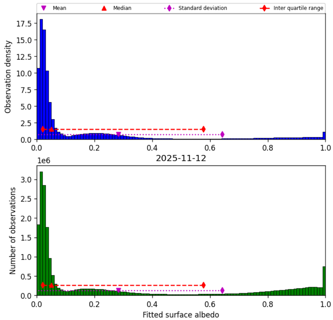
Figure 45: Histogram of “Fitted surface albedo” for 2025-11-12 to 2025-11-13
