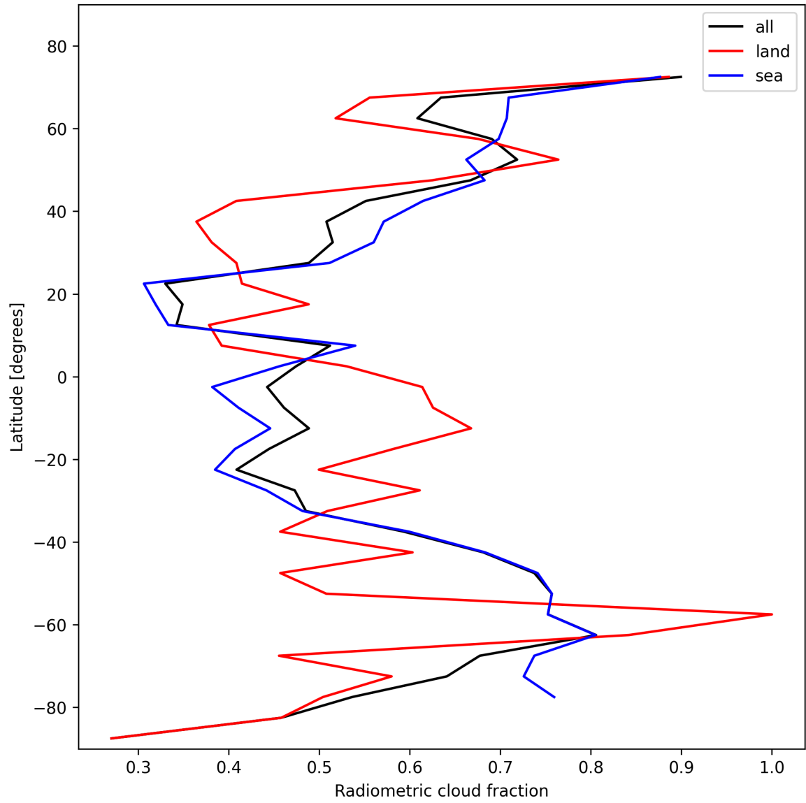
Figure 23: Zonal average of “Radiometric cloud fraction” for 2025-11-12 to 2025-11-13.
