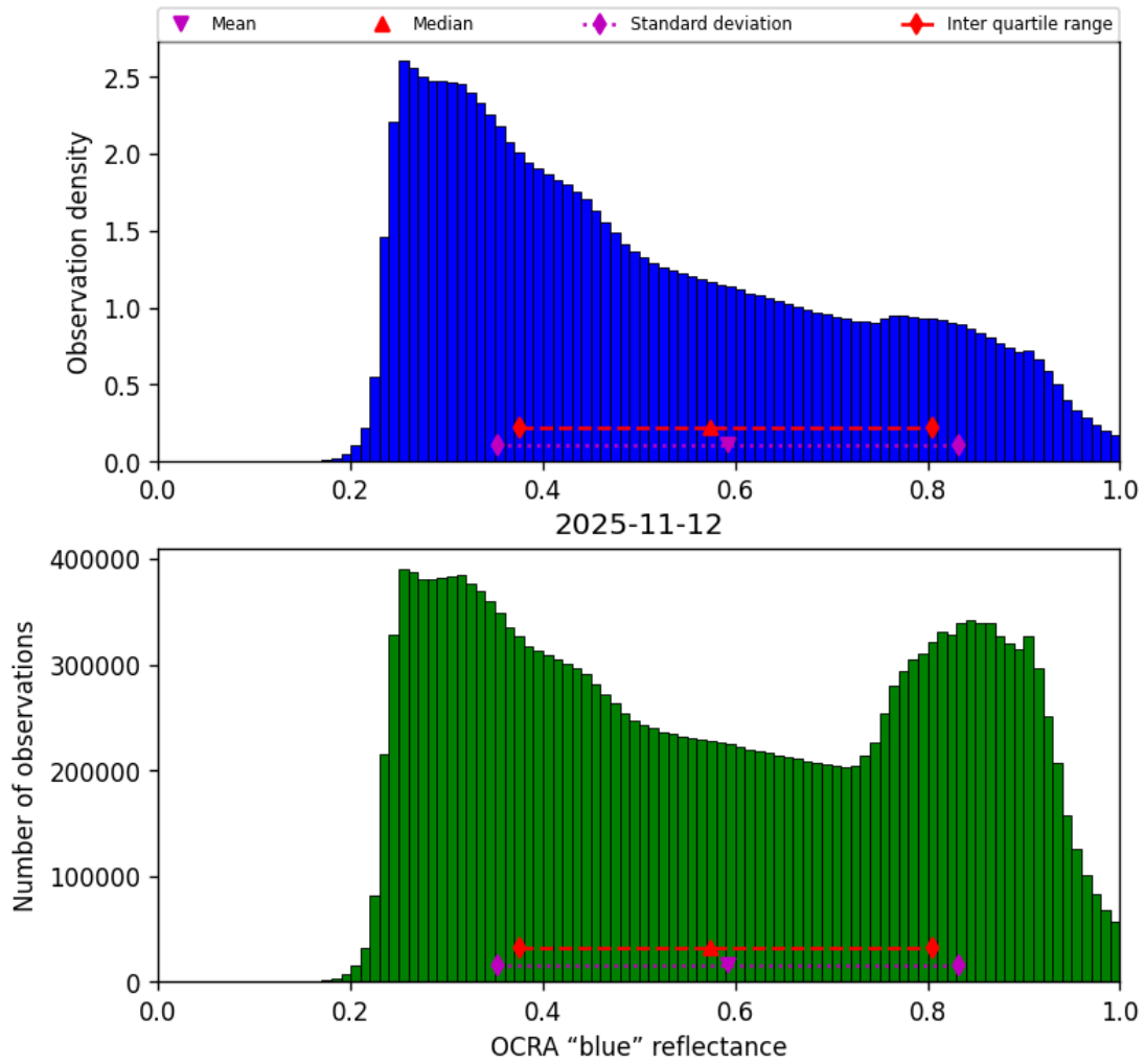
Figure 51: Histogram of “OCRA “blue” reflectance” for 2025-11-12 to 2025-11-13
