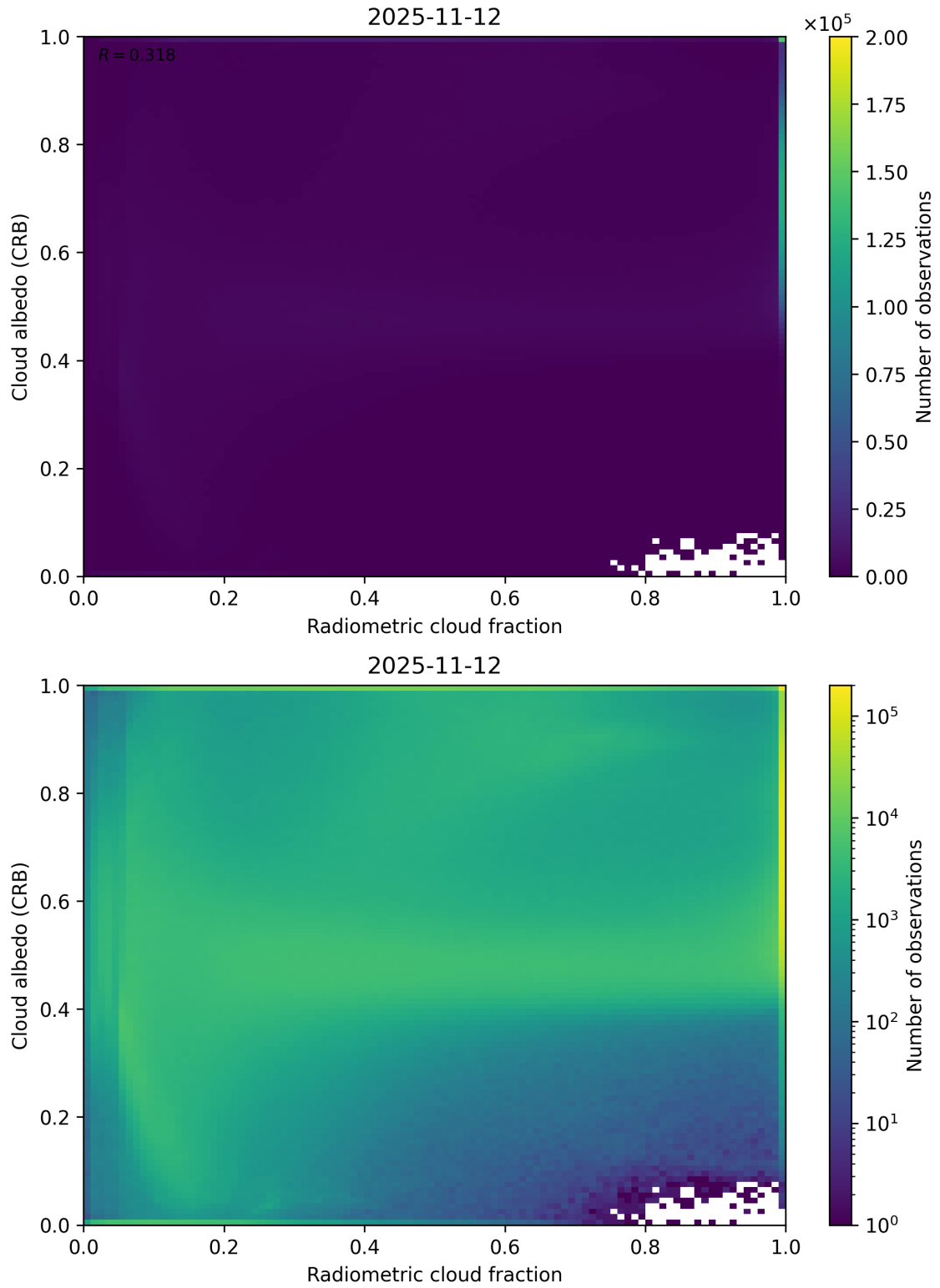
Figure 71: Scatter density plot of “Radiometric cloud fraction” against “Cloud albedo (CRB)” for 2025-11-12 to 2025-11-13.
