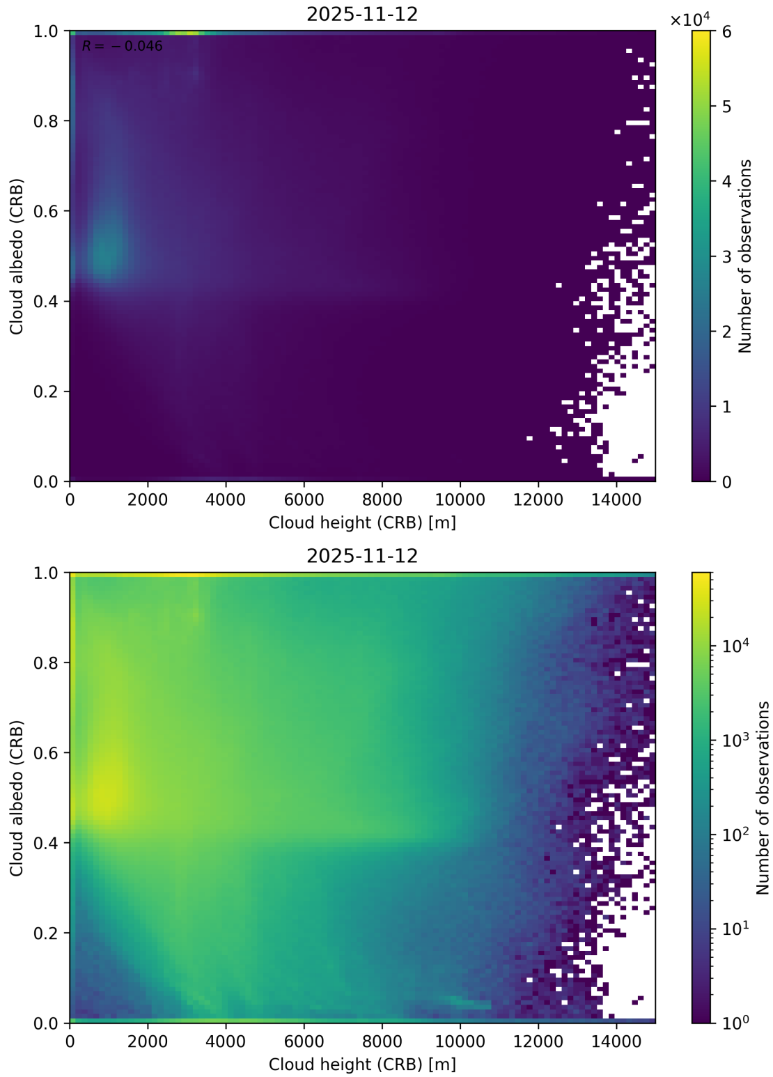
Figure 80: Scatter density plot of “Cloud height (CRB)” against “Cloud albedo (CRB)” for 2025-11-12 to 2025-11-13.
