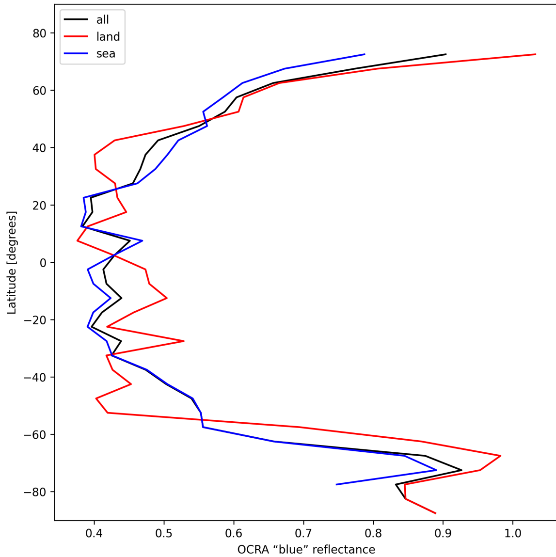
Figure 35: Zonal average of “OCRA “blue” reflectance” for 2025-11-12 to 2025-11-13.
