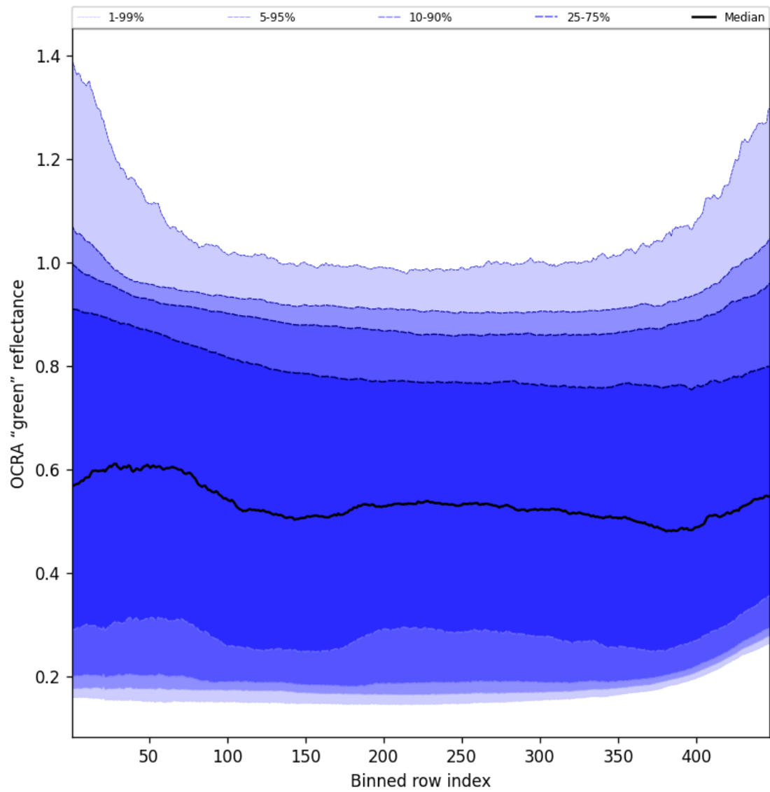
Figure 68: Along track statistics of “OCRA “green” reflectance” for 2025-11-12 to 2025-11-13
