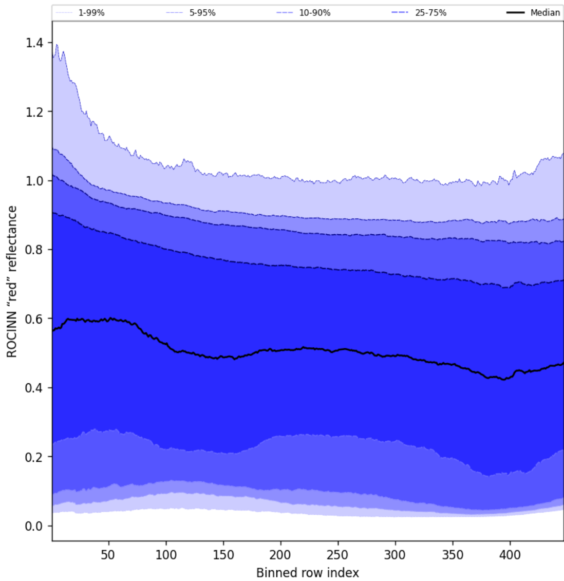
Figure 69: Along track statistics of “ROCINN “red” reflectance” for 2025-11-12 to 2025-11-13
