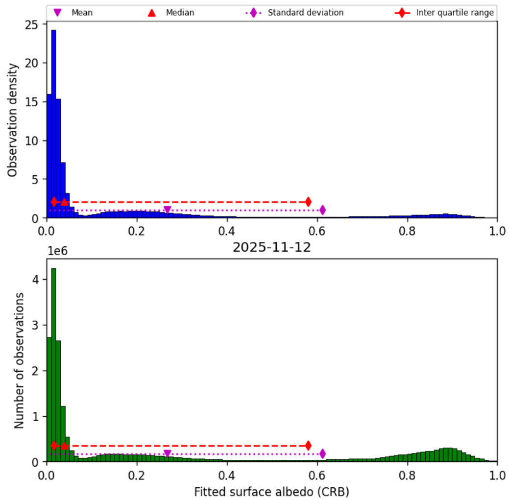
Figure 46: Histogram of “Fitted surface albedo (CRB)” for 2025-11-12 to 2025-11-13
