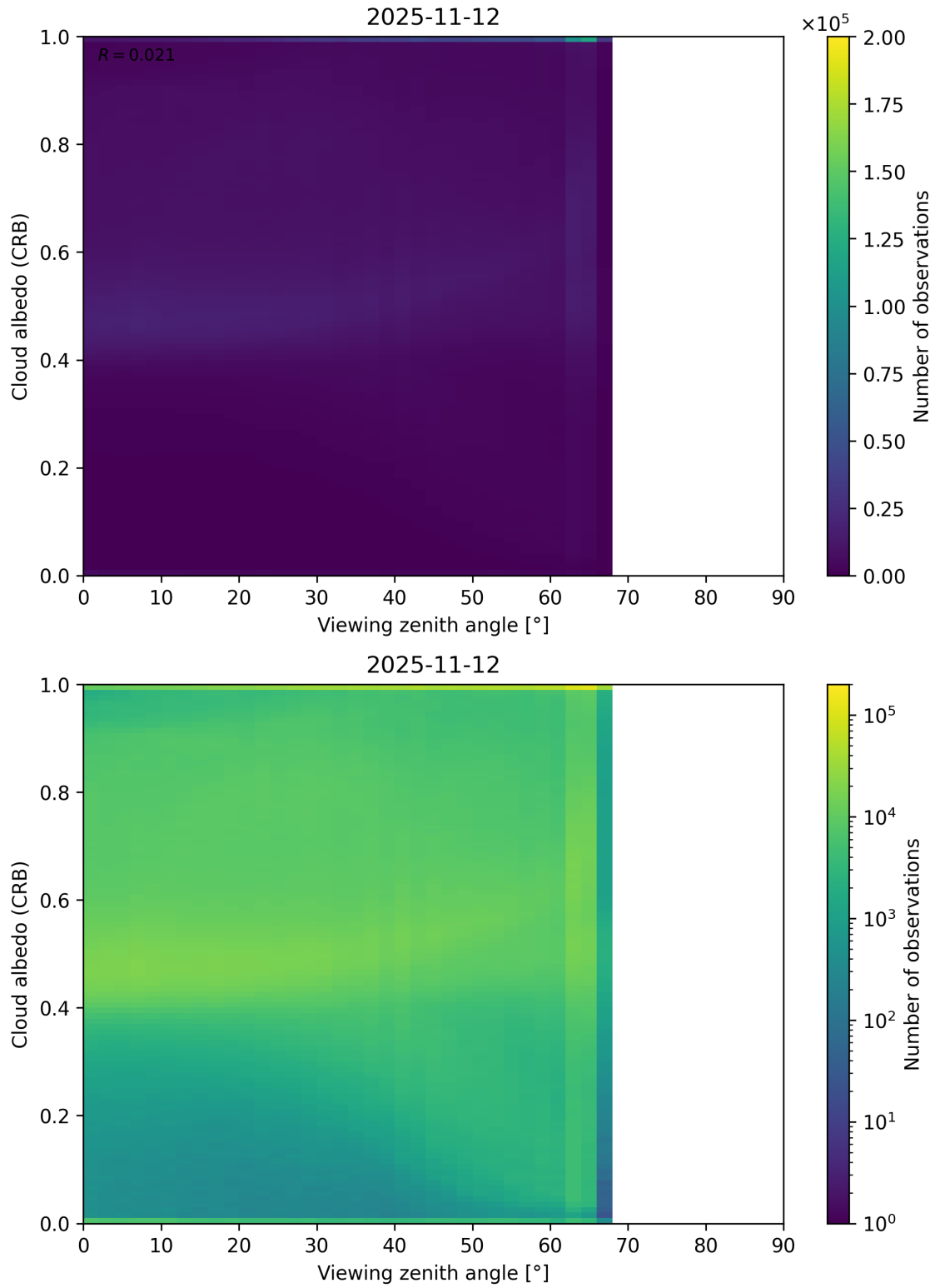
Figure 106: Scatter density plot of “Viewing zenith angle” against “Cloud albedo (CRB)” for 2025-11-12 to 2025-11-13.
