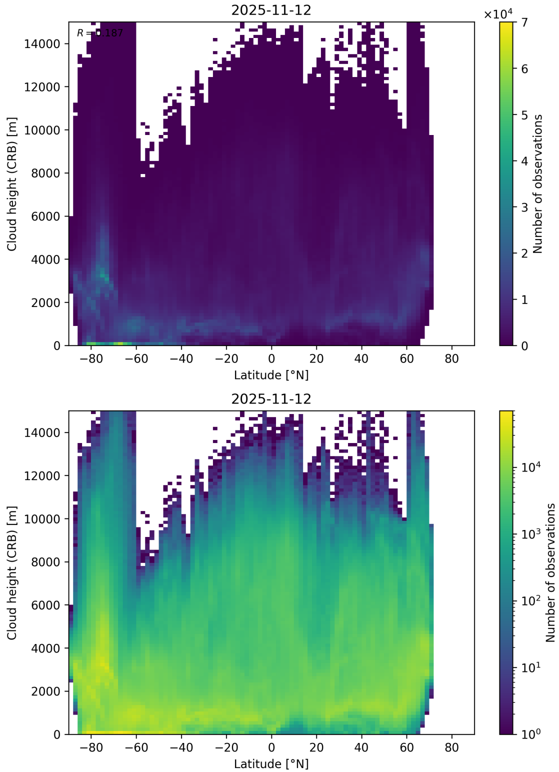
Figure 95: Scatter density plot of “Latitude” against “Cloud height (CRB)” for 2025-11-12 to 2025-11-13.
