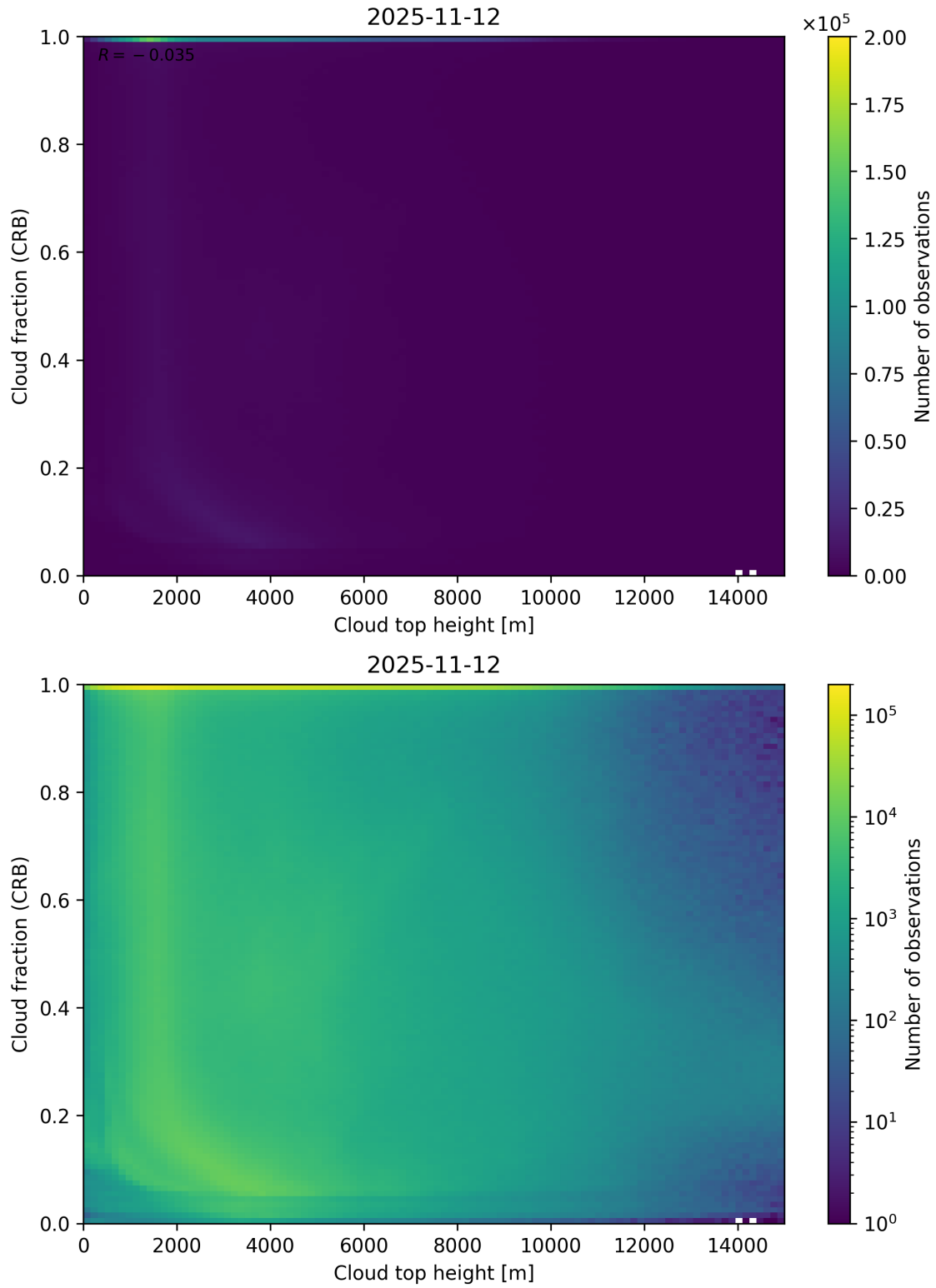
Figure 88: Scatter density plot of “Cloud top height” against “Cloud fraction (CRB)” for 2025-11-12 to 2025-11-13.
