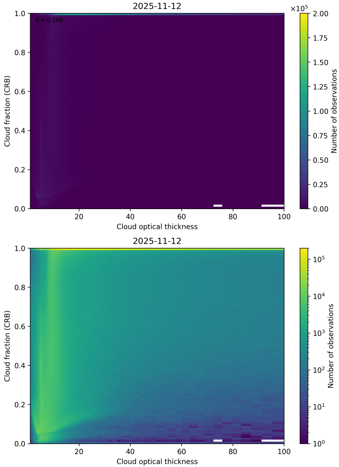
Figure 84: Scatter density plot of “Cloud optical thickness” against “Cloud fraction (CRB)” for 2025-11-12 to 2025-11-13.
