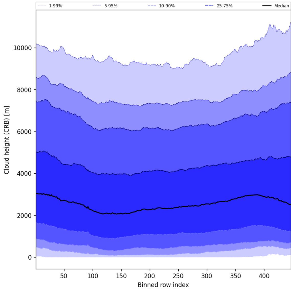
Figure 59: Along track statistics of “Cloud height (CRB)” for 2025-11-12 to 2025-11-13
