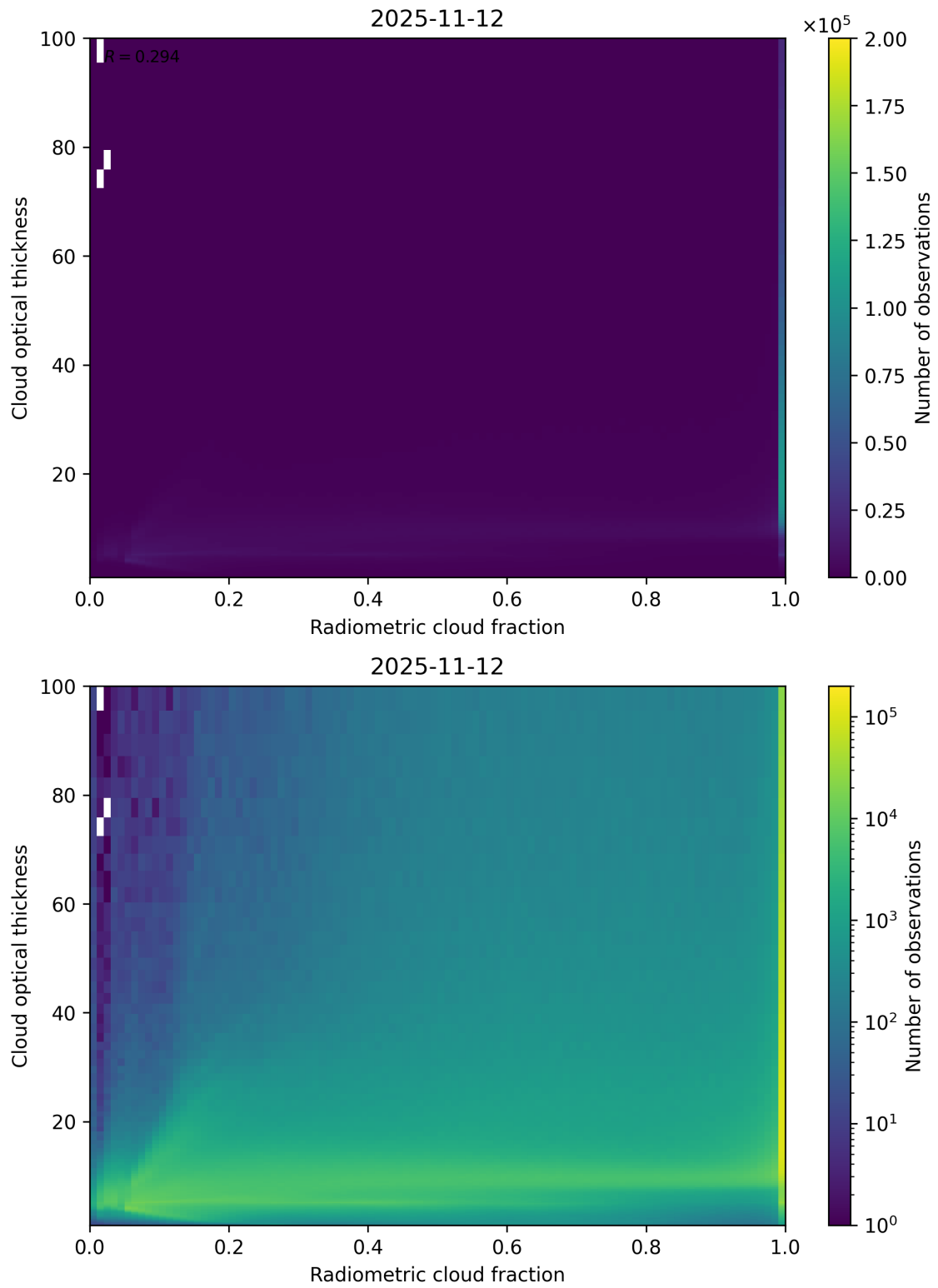
Figure 75: Scatter density plot of “Radiometric cloud fraction” against “Cloud optical thickness” for 2025-11-12 to 2025-11-13.
