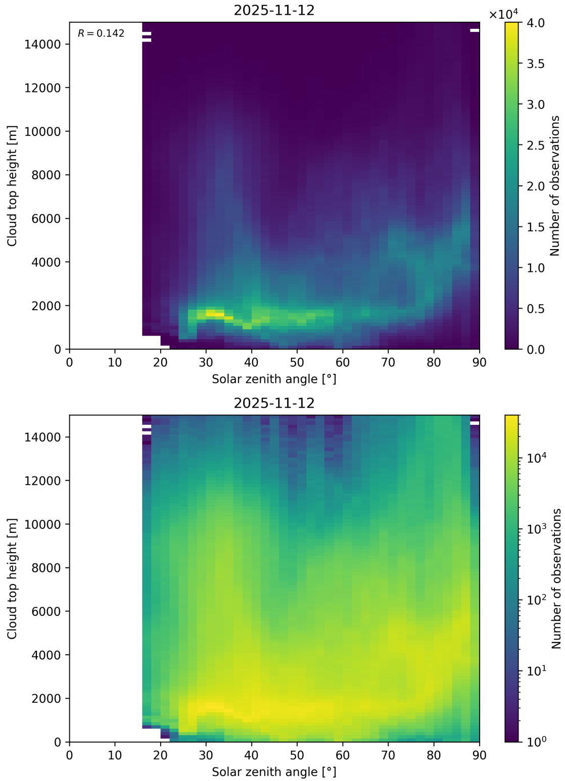
Figure 104: Scatter density plot of “Solar zenith angle” against “Cloud top height” for 2025-11-12 to 2025-11-13.
