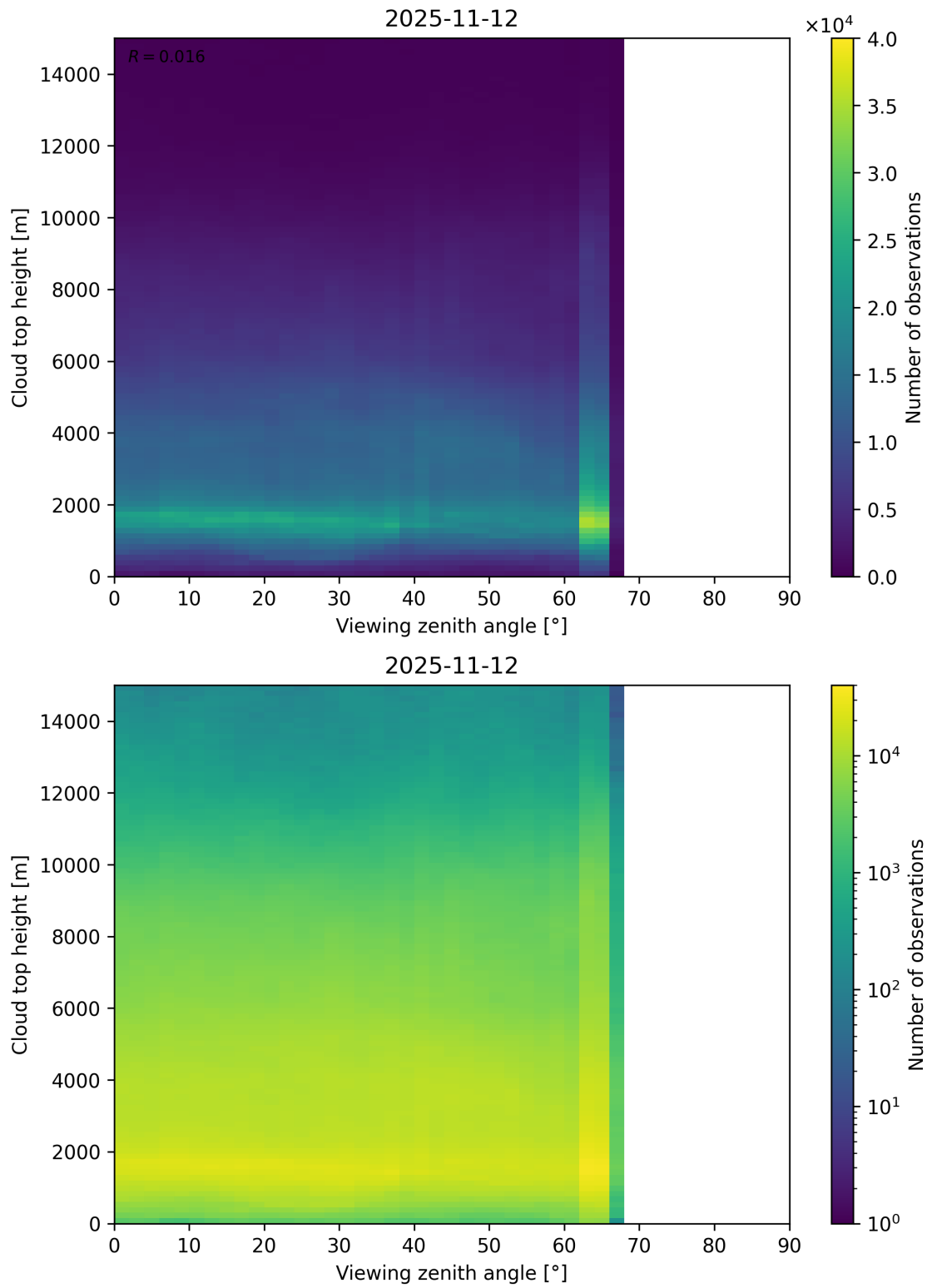
Figure 112: Scatter density plot of “Viewing zenith angle” against “Cloud top height” for 2025-11-12 to 2025-11-13.
