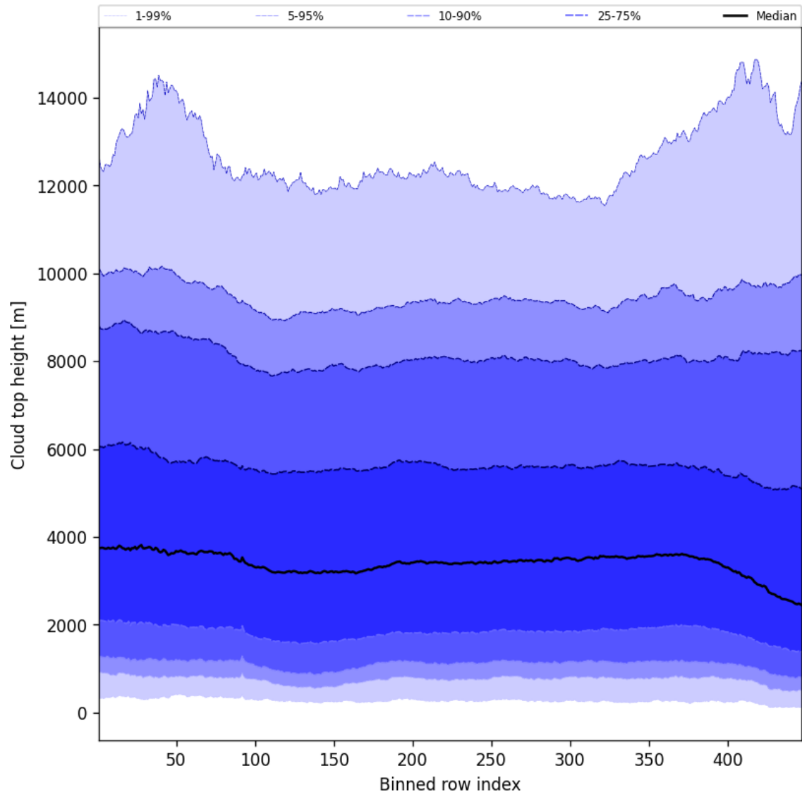
Figure 56: Along track statistics of “Cloud top height” for 2025-11-12 to 2025-11-13
