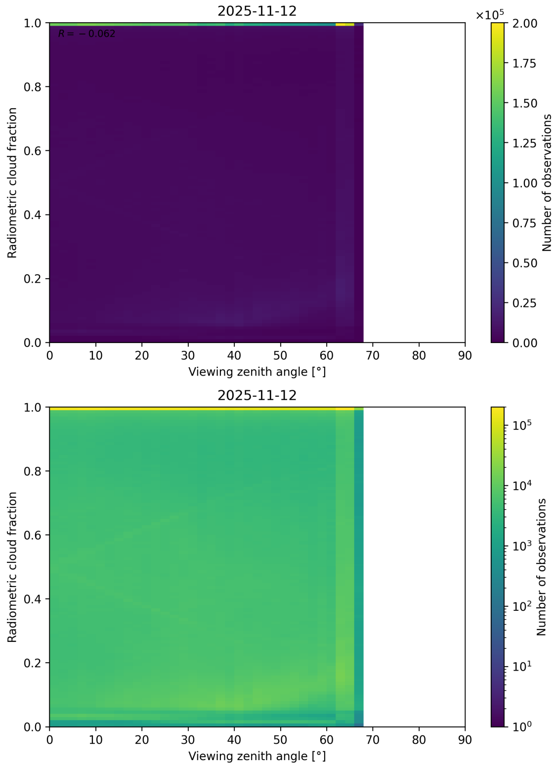
Figure 107: Scatter density plot of “Viewing zenith angle” against “Radiometric cloud fraction” for 2025-11-12 to 2025-11-13.
