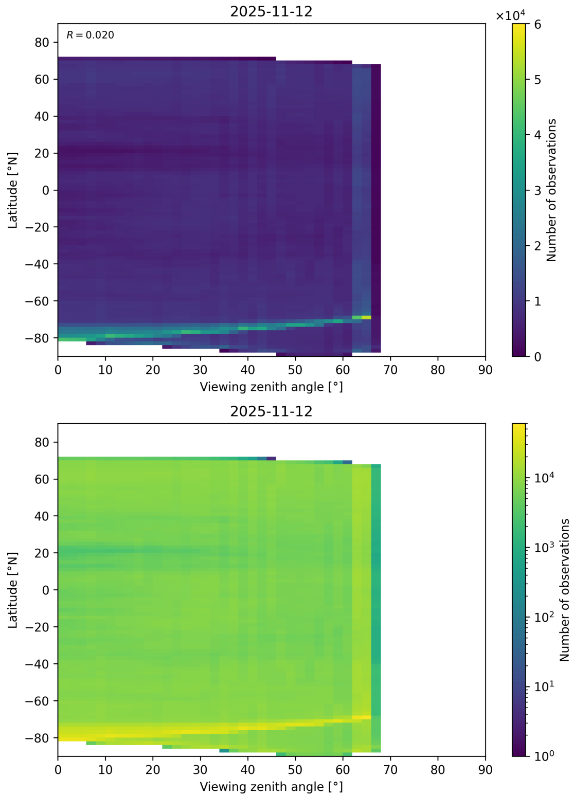
Figure 113: Scatter density plot of “Viewing zenith angle” against “Latitude” for 2025-11-12 to 2025-11-13.
