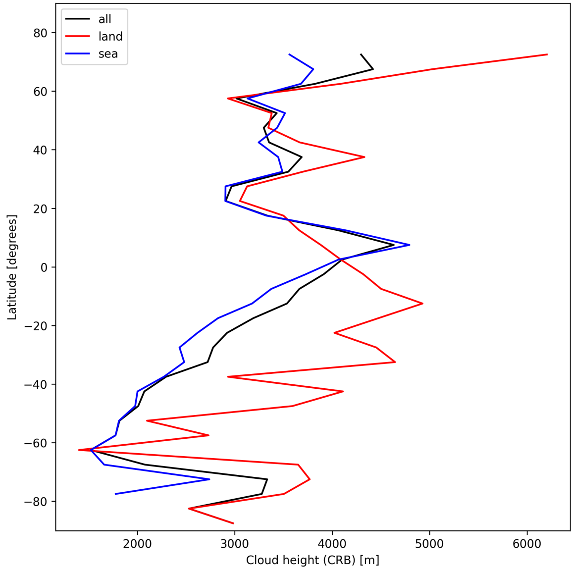
Figure 27: Zonal average of “Cloud height (CRB)” for 2025-11-12 to 2025-11-13.
