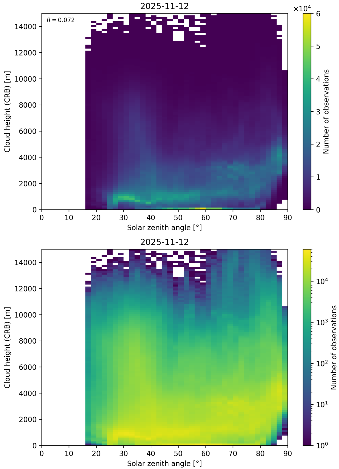
Figure 102: Scatter density plot of “Solar zenith angle” against “Cloud height (CRB)” for 2025-11-12 to 2025-11-13.
