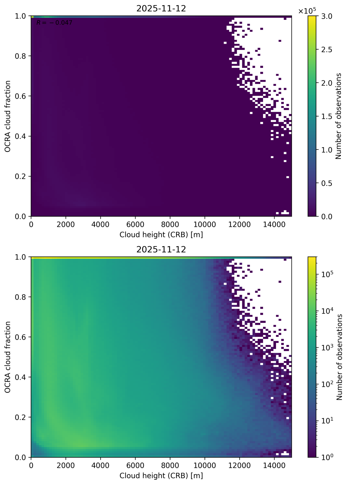
Figure 81: Scatter density plot of “Cloud height (CRB)” against “OCRA cloud fraction” for 2025-11-12 to 2025-11-13.
