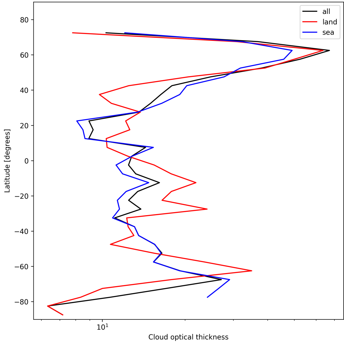
Figure 25: Zonal average of “Cloud optical thickness” for 2025-11-12 to 2025-11-13.
