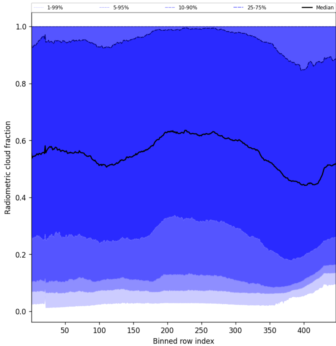
Figure 55: Along track statistics of “Radiometric cloud fraction” for 2025-11-12 to 2025-11-13
