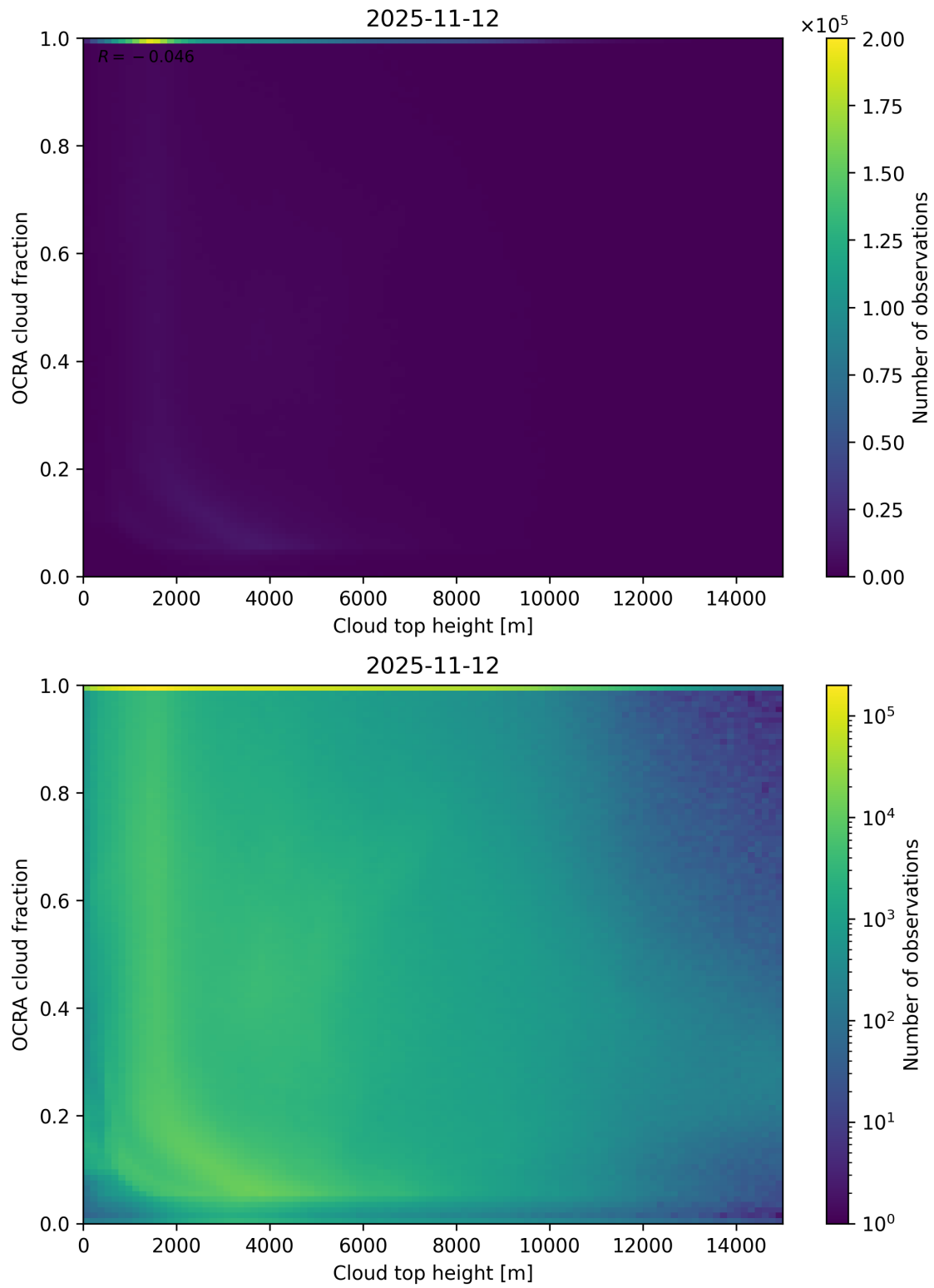
Figure 87: Scatter density plot of “Cloud top height” against “OCRA cloud fraction” for 2025-11-12 to 2025-11-13.
