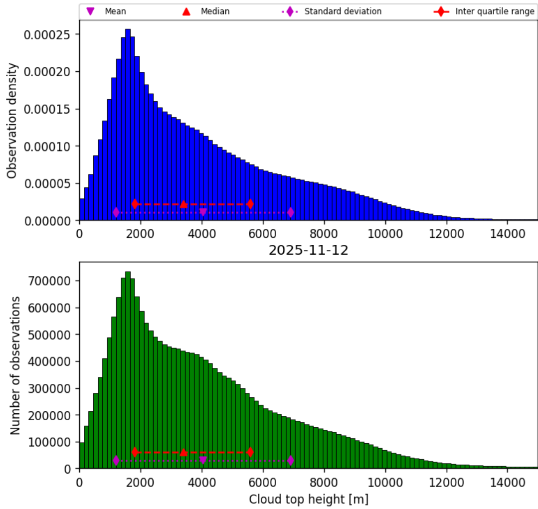
Figure 40: Histogram of “Cloud top height” for 2025-11-12 to 2025-11-13
