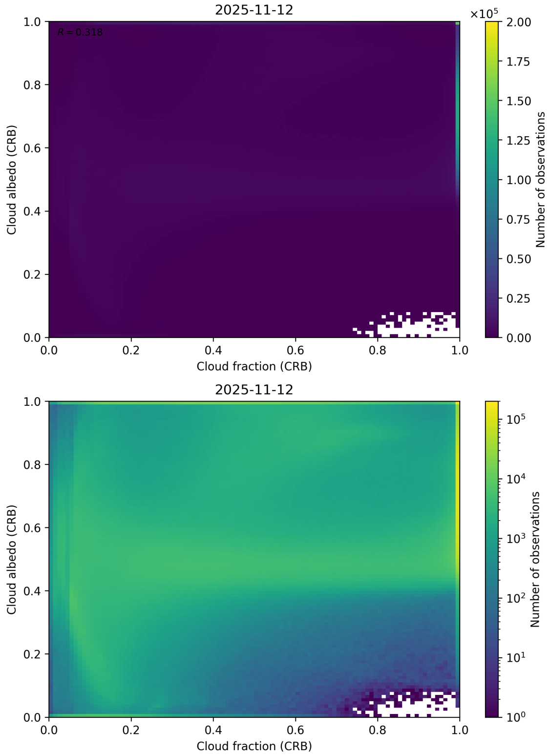
Figure 77: Scatter density plot of “Cloud fraction (CRB)” against “Cloud albedo (CRB)” for 2025-11-12 to 2025-11-13.
