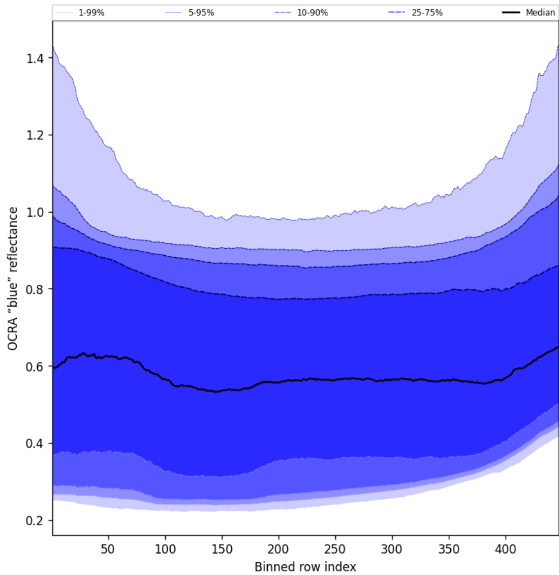
Figure 67: Along track statistics of “OCRA “blue” reflectance” for 2025-11-12 to 2025-11-13
