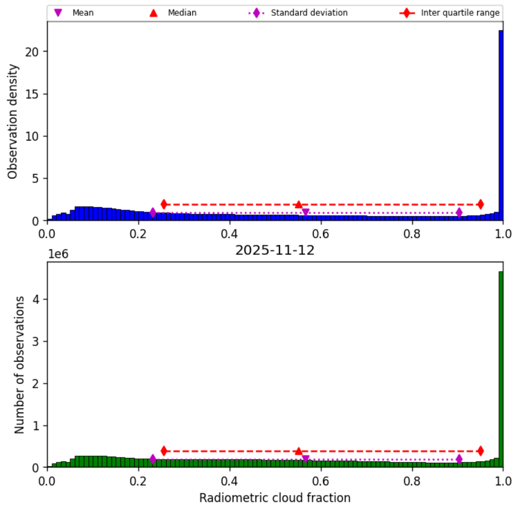
Figure 39: Histogram of “Radiometric cloud fraction” for 2025-11-12 to 2025-11-13
