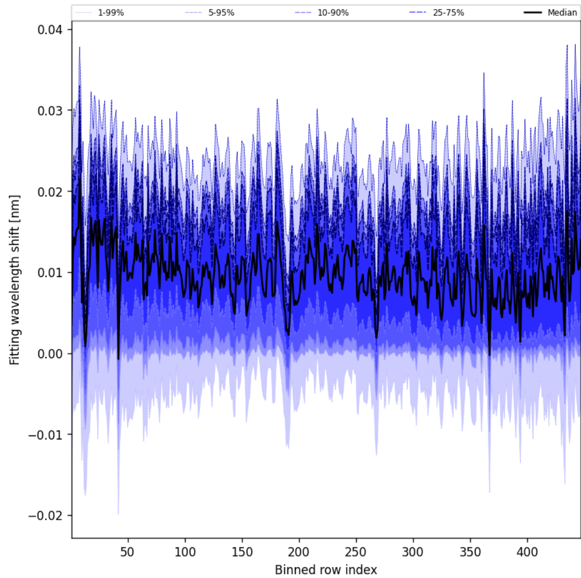
Figure 65: Along track statistics of “Fitting wavelength shift” for 2025-11-12 to 2025-11-13
