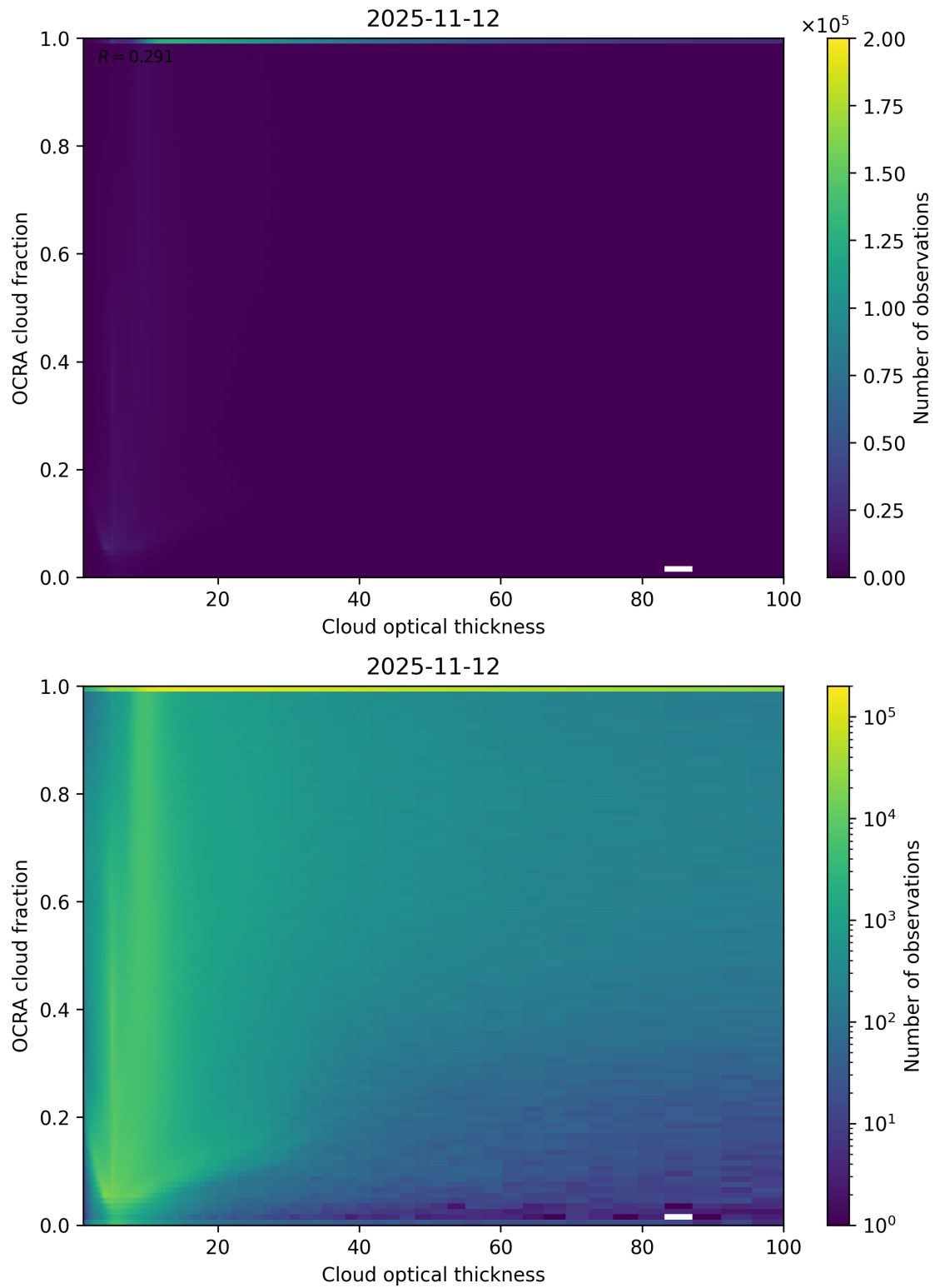
Figure 83: Scatter density plot of “Cloud optical thickness” against “OCRA cloud fraction” for 2025-11-12 to 2025-11-13.
