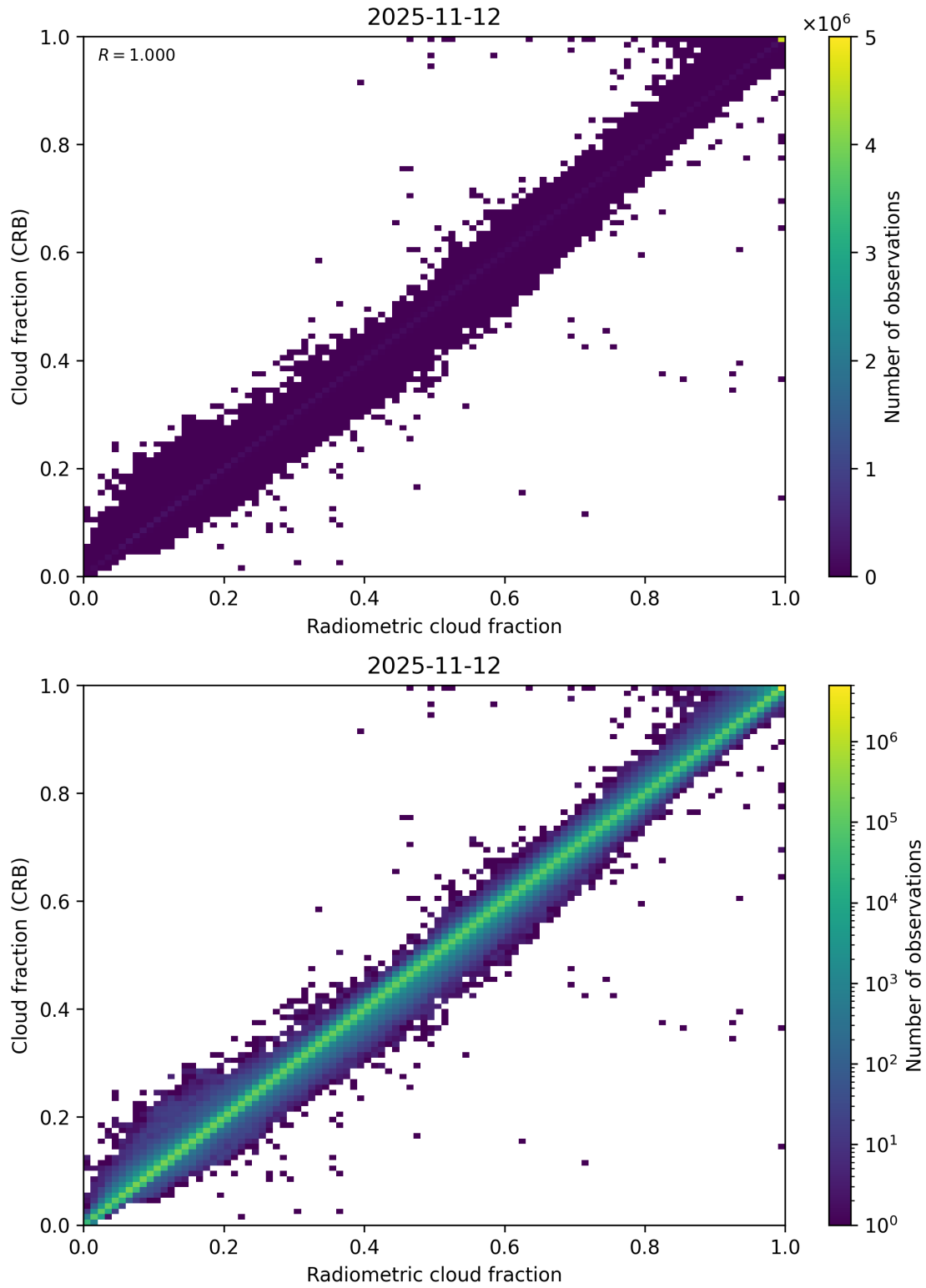
Figure 73: Scatter density plot of “Radiometric cloud fraction” against “Cloud fraction (CRB)” for 2025-11-12 to 2025-11-13.
