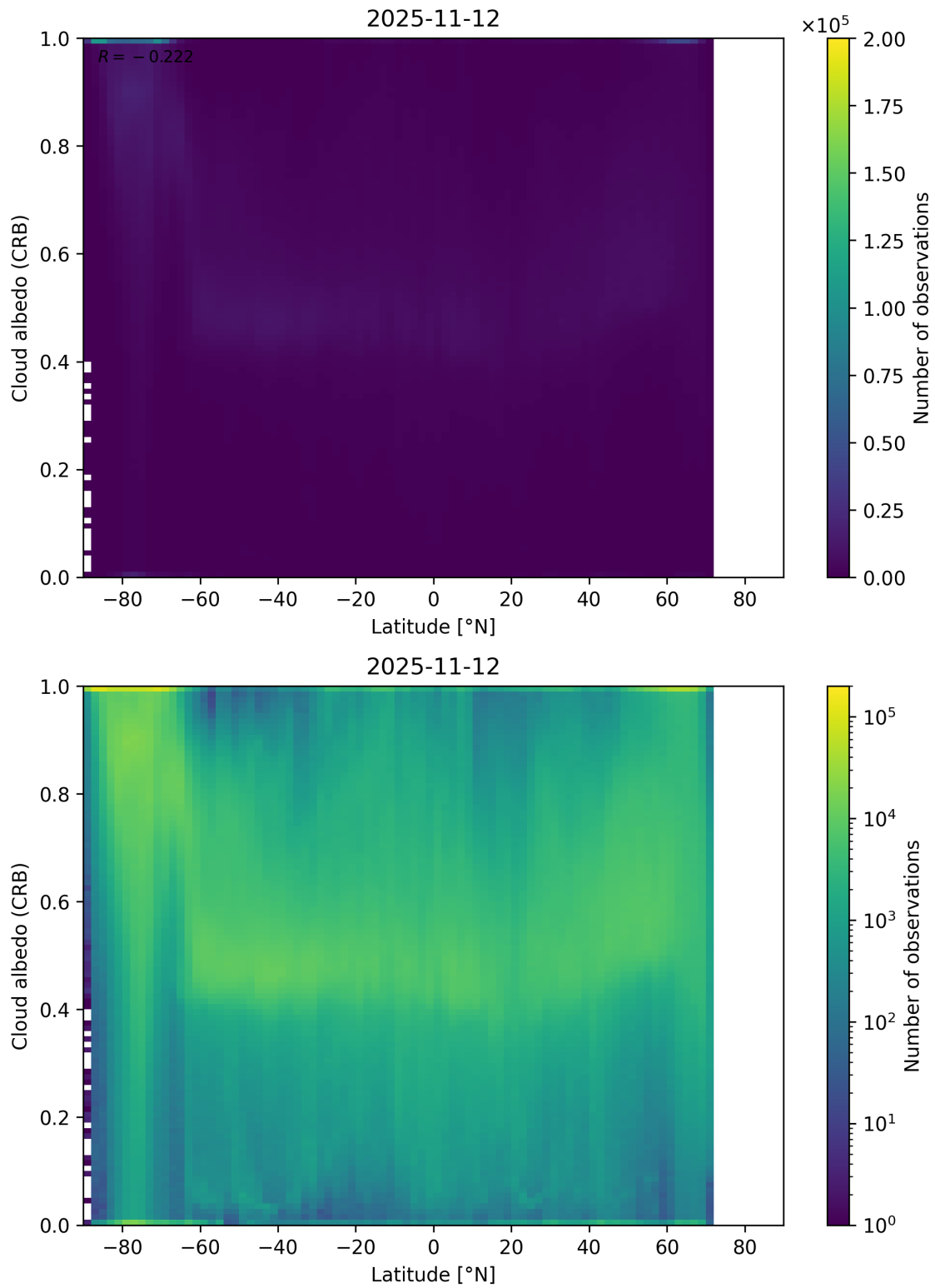
Figure 91: Scatter density plot of “Latitude” against “Cloud albedo (CRB)” for 2025-11-12 to 2025-11-13.
