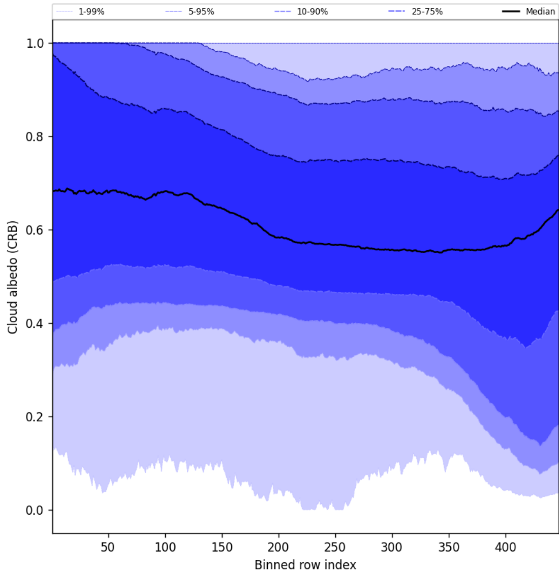
Figure 60: Along track statistics of “Cloud albedo (CRB)” for 2025-11-12 to 2025-11-13
