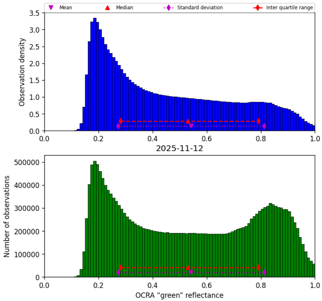
Figure 52: Histogram of “OCRA “green” reflectance” for 2025-11-12 to 2025-11-13
