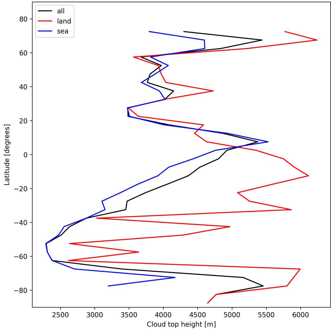
Figure 24: Zonal average of “Cloud top height” for 2025-11-12 to 2025-11-13.
