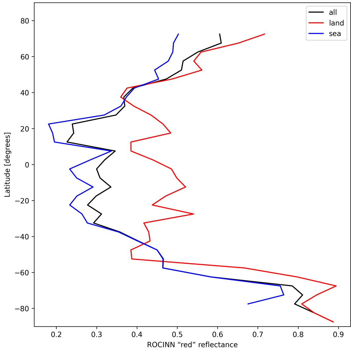
Figure 37: Zonal average of “ROCINN “red” reflectance” for 2025-11-12 to 2025-11-13.
