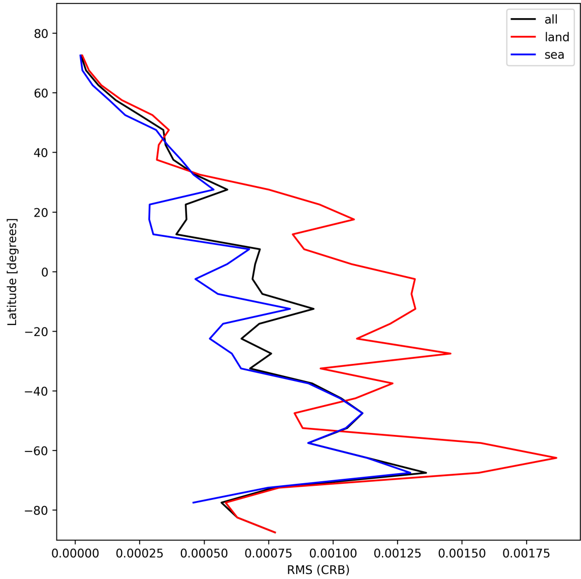
Figure 32: Zonal average of “RMS (CRB)” for 2025-11-12 to 2025-11-13.
