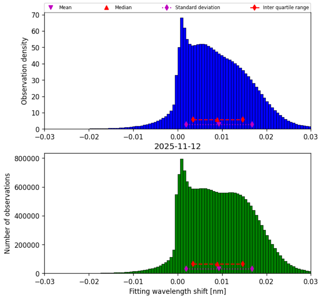
Figure 49: Histogram of “Fitting wavelength shift” for 2025-11-12 to 2025-11-13
