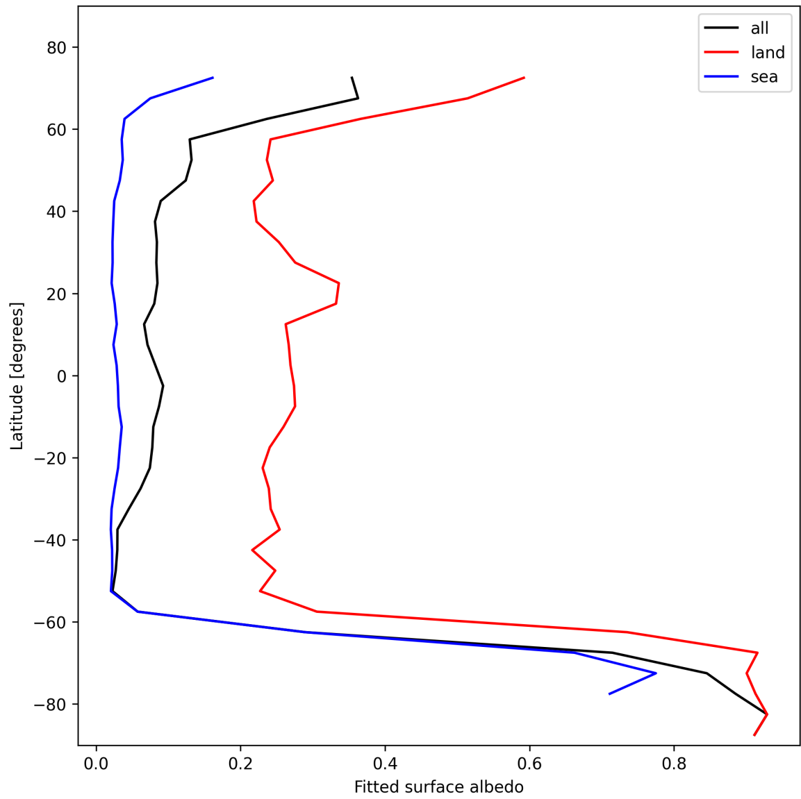
Figure 29: Zonal average of “Fitted surface albedo” for 2025-11-12 to 2025-11-13.
