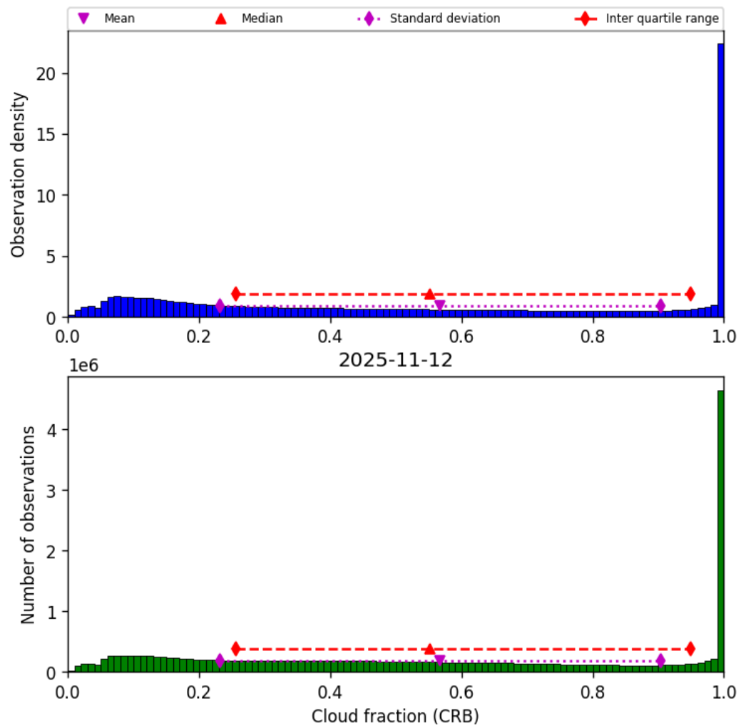
Figure 42: Histogram of “Cloud fraction (CRB)” for 2025-11-12 to 2025-11-13
