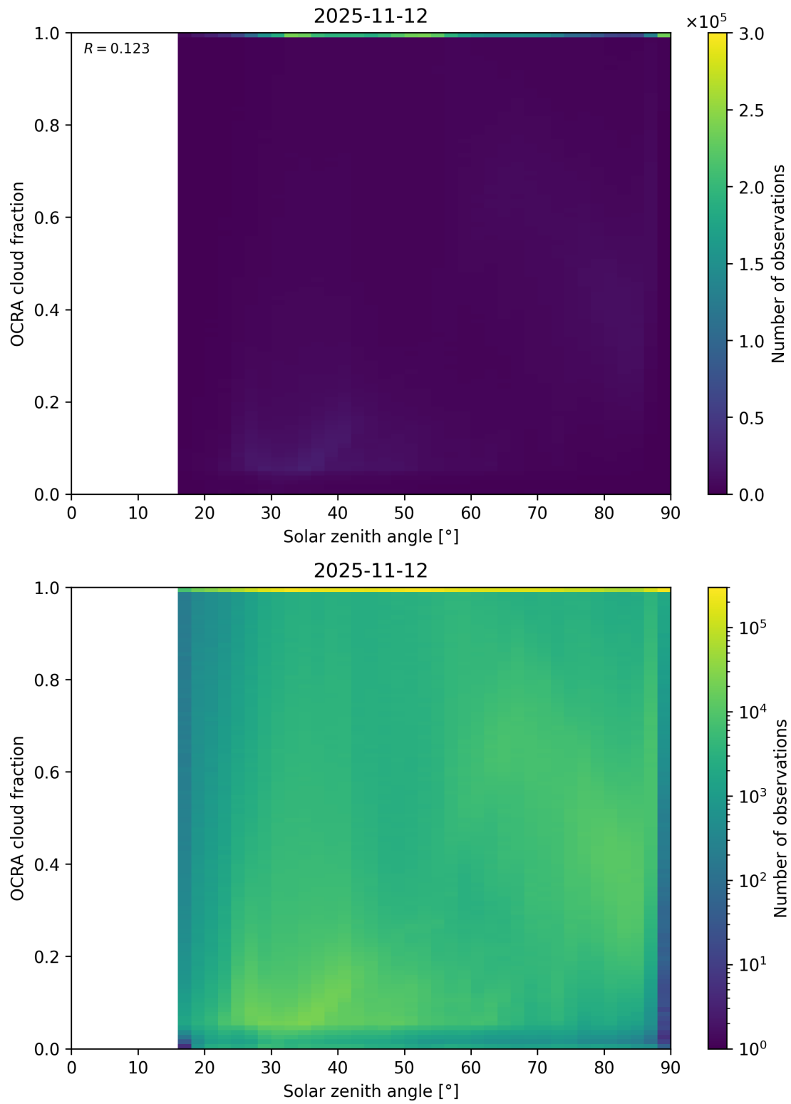
Figure 100: Scatter density plot of “Solar zenith angle” against “OCRA cloud fraction” for 2025-11-12 to 2025-11-13.
