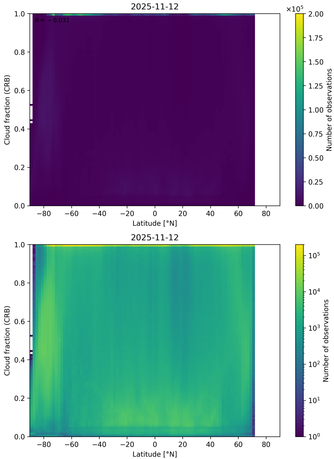
Figure 94: Scatter density plot of “Latitude” against “Cloud fraction (CRB)” for 2025-11-12 to 2025-11-13.
