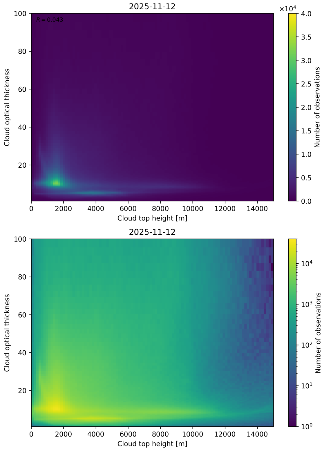
Figure 90: Scatter density plot of “Cloud top height” against “Cloud optical thickness” for 2025-11-12 to 2025-11-13.
