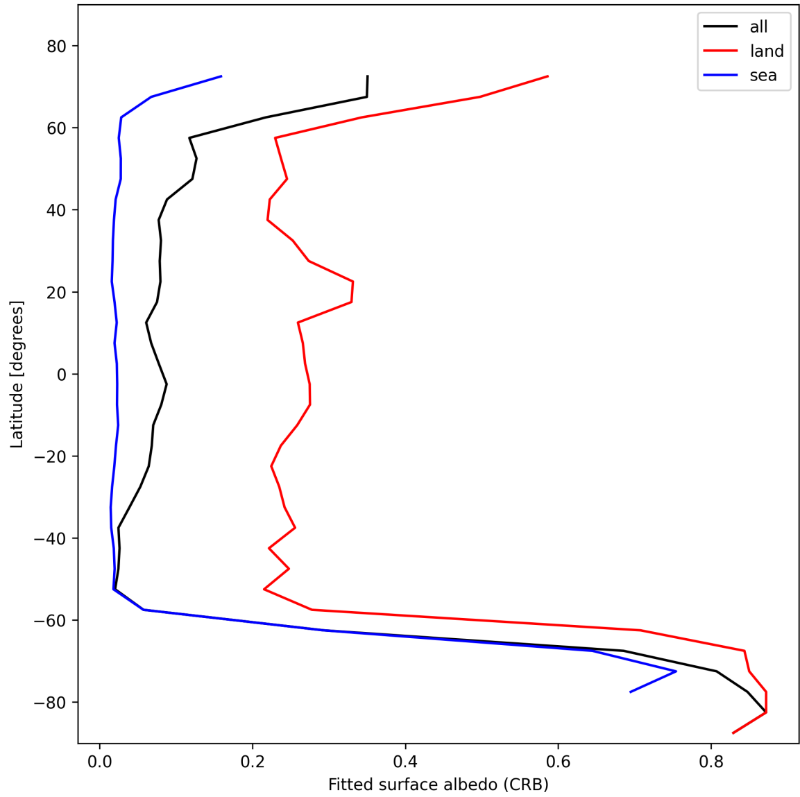
Figure 30: Zonal average of “Fitted surface albedo (CRB)” for 2025-11-12 to 2025-11-13.
