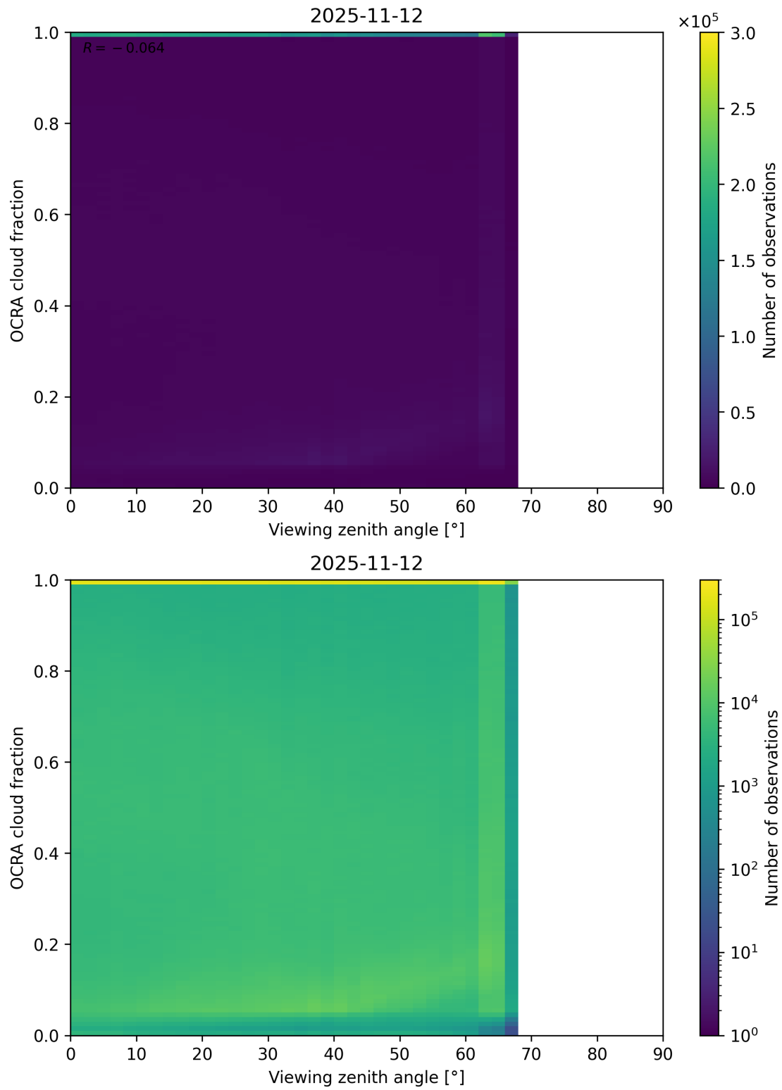
Figure 108: Scatter density plot of “Viewing zenith angle” against “OCRA cloud fraction” for 2025-11-12 to 2025-11-13.
