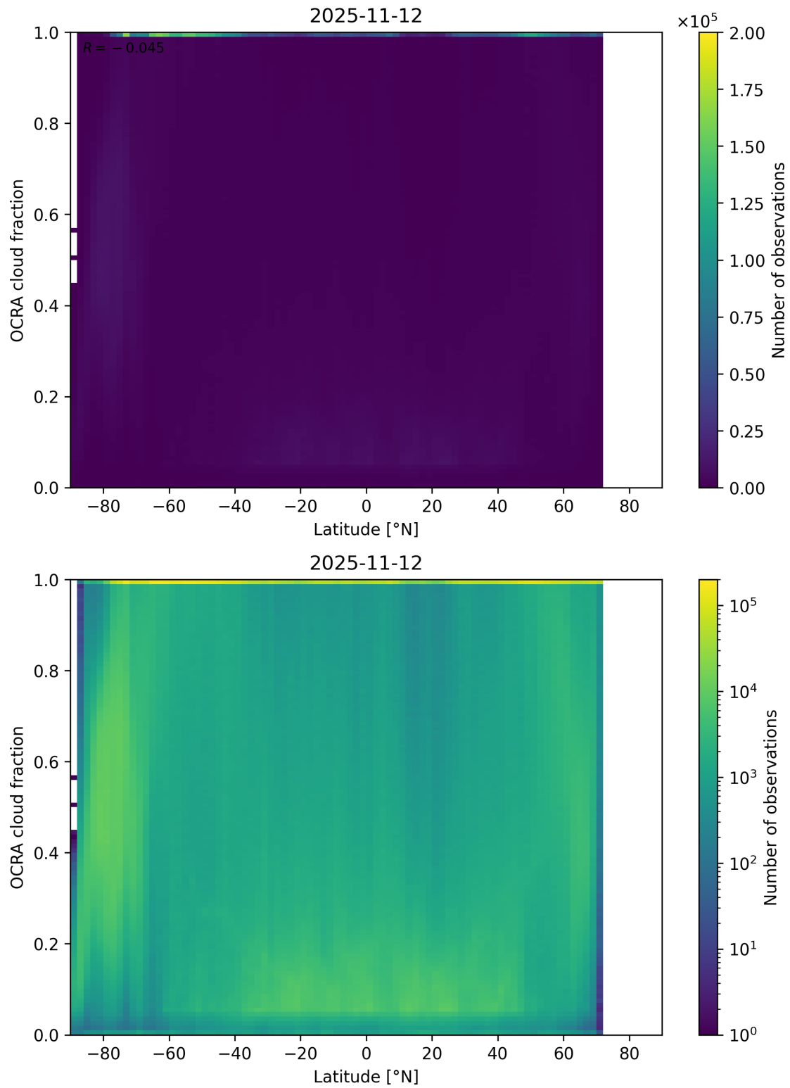
Figure 93: Scatter density plot of “Latitude” against “OCRA cloud fraction” for 2025-11-12 to 2025-11-13.
