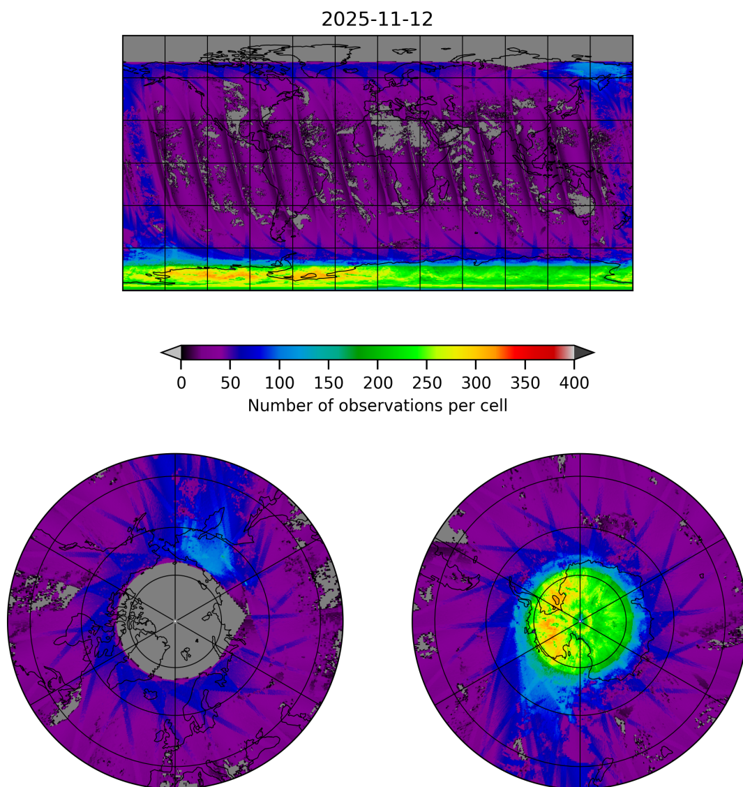
Figure 21: Map of the number of observations for 2025-11-12 to 2025-11-13
