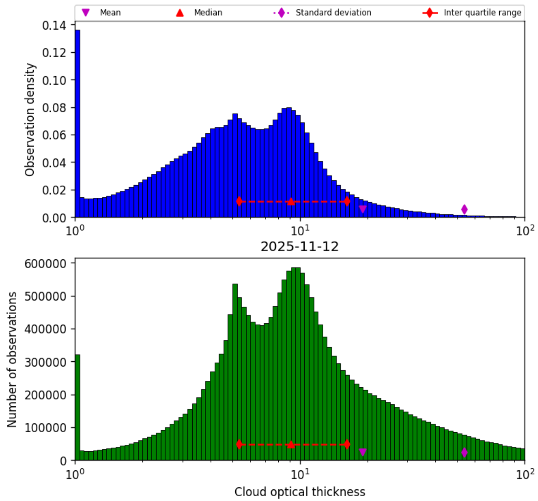
Figure 41: Histogram of “Cloud optical thickness” for 2025-11-12 to 2025-11-13
