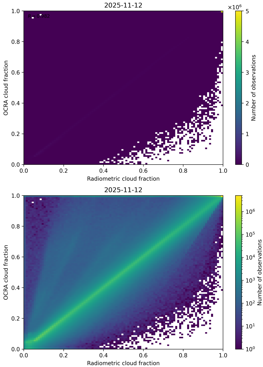
Figure 72: Scatter density plot of “Radiometric cloud fraction” against “OCRA cloud fraction” for 2025-11-12 to 2025-11-13.
