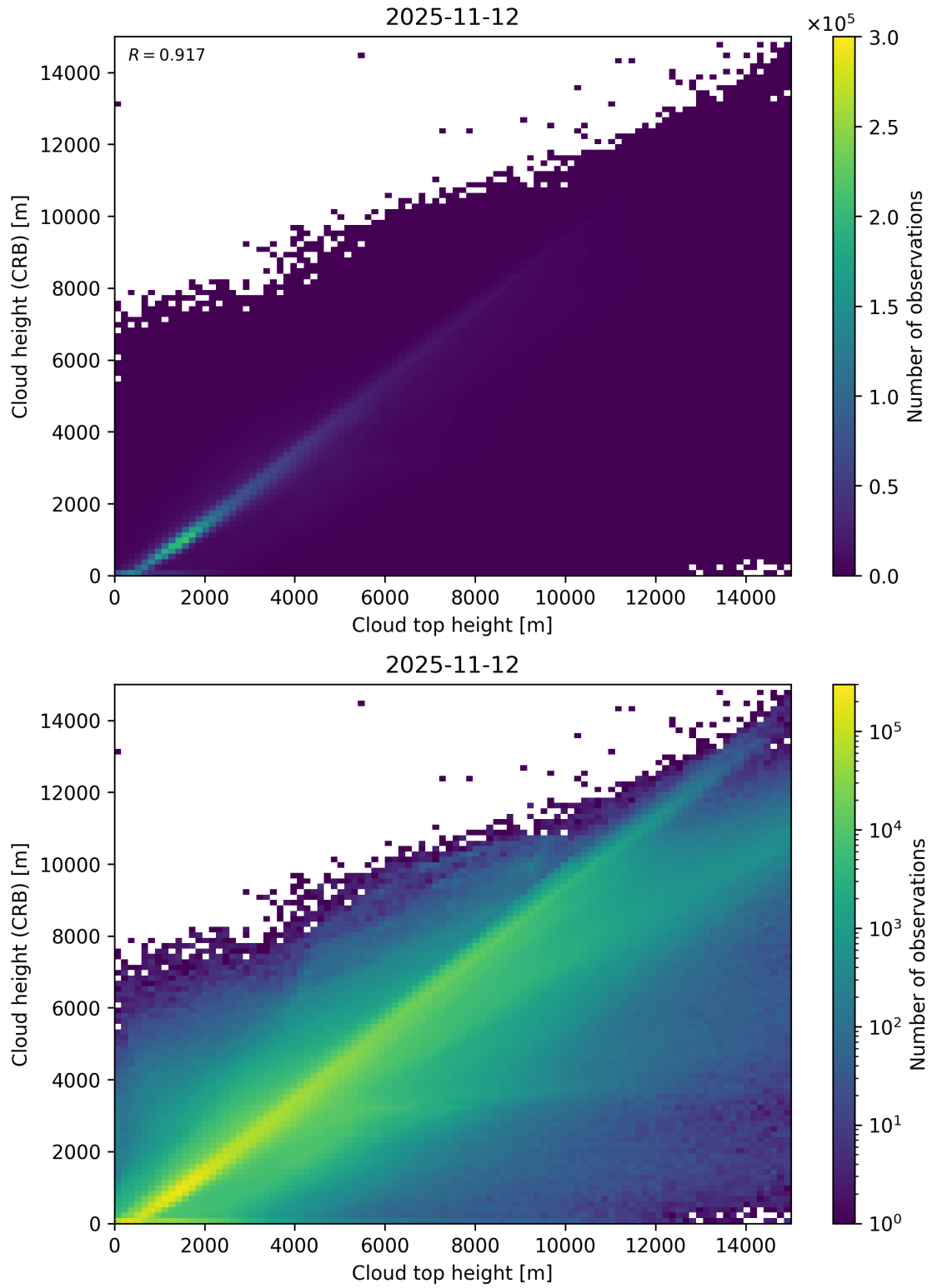
Figure 89: Scatter density plot of “Cloud top height” against “Cloud height (CRB)” for 2025-11-12 to 2025-11-13.
