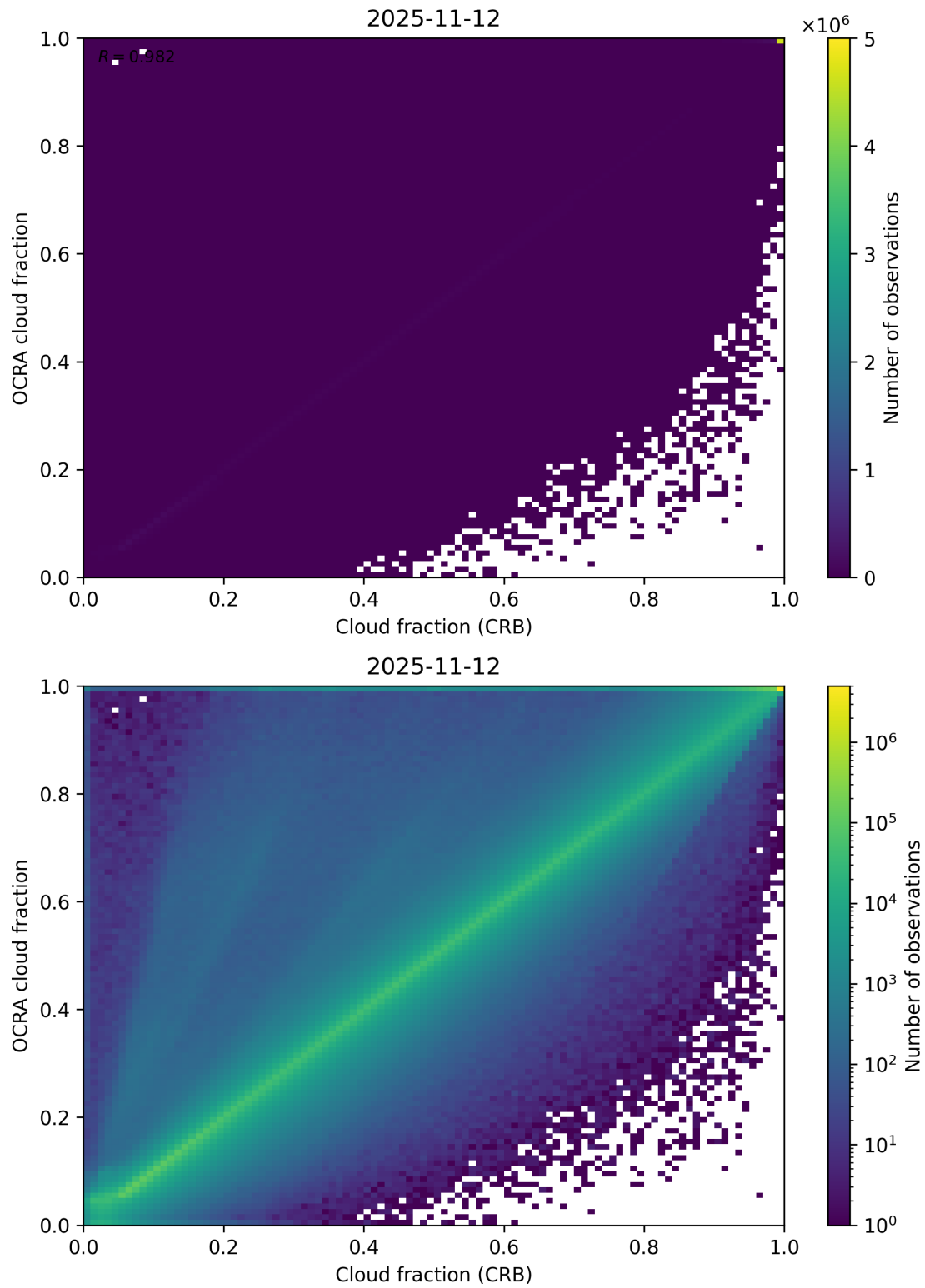
Figure 78: Scatter density plot of “Cloud fraction (CRB)” against “OCRA cloud fraction” for 2025-11-12 to 2025-11-13.
