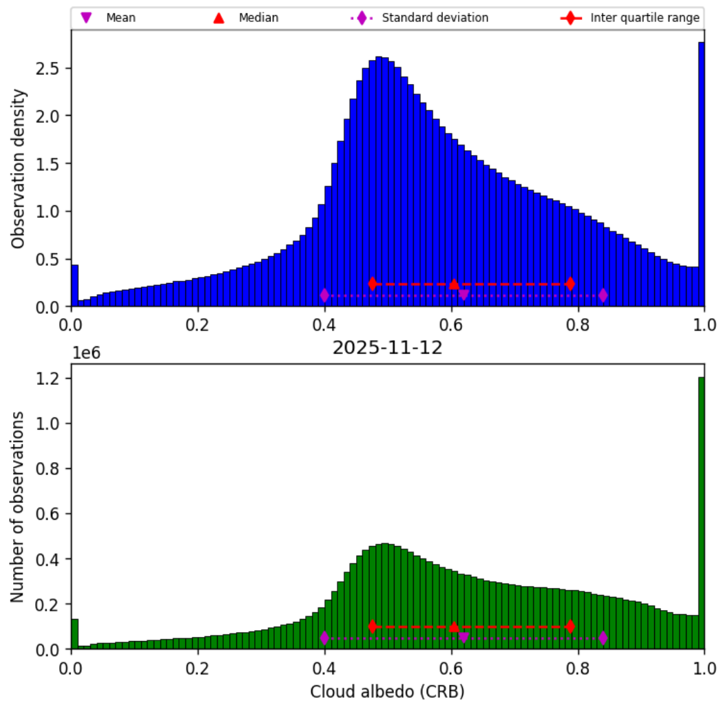
Figure 44: Histogram of “Cloud albedo (CRB)” for 2025-11-12 to 2025-11-13
