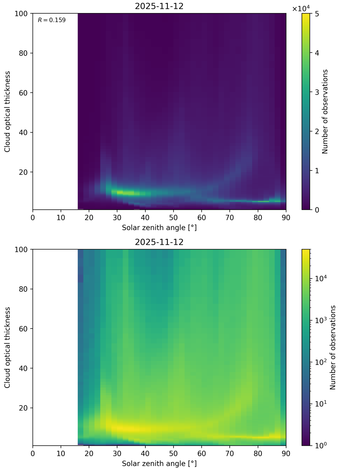
Figure 103: Scatter density plot of “Solar zenith angle” against “Cloud optical thickness” for 2025-11-12 to 2025-11-13.
