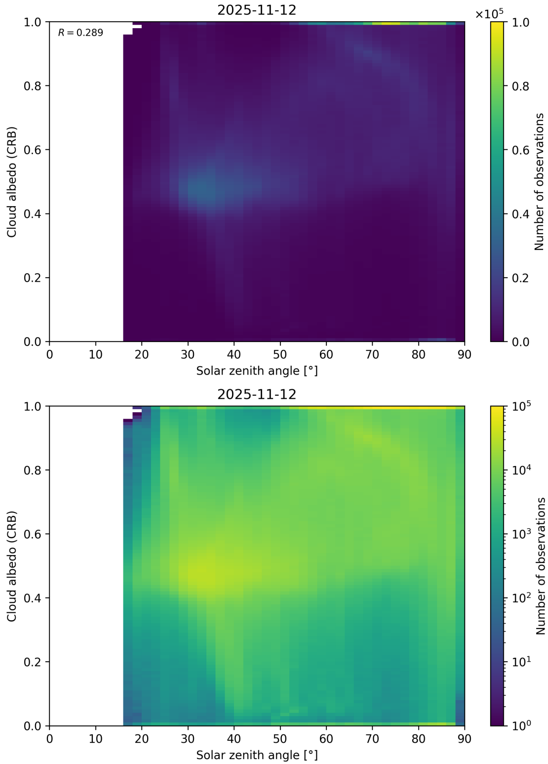
Figure 98: Scatter density plot of “Solar zenith angle” against “Cloud albedo (CRB)” for 2025-11-12 to 2025-11-13.
