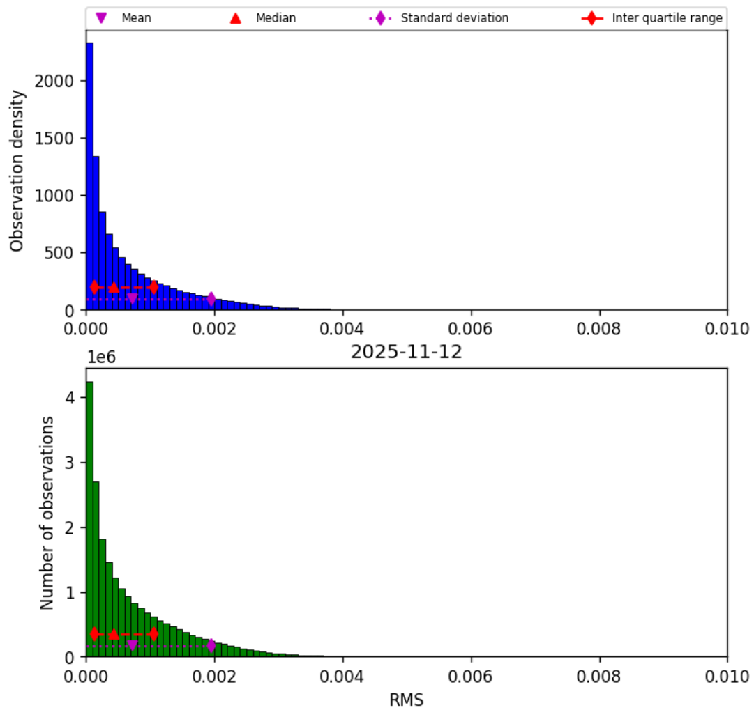
Figure 47: Histogram of “RMS” for 2025-11-12 to 2025-11-13
