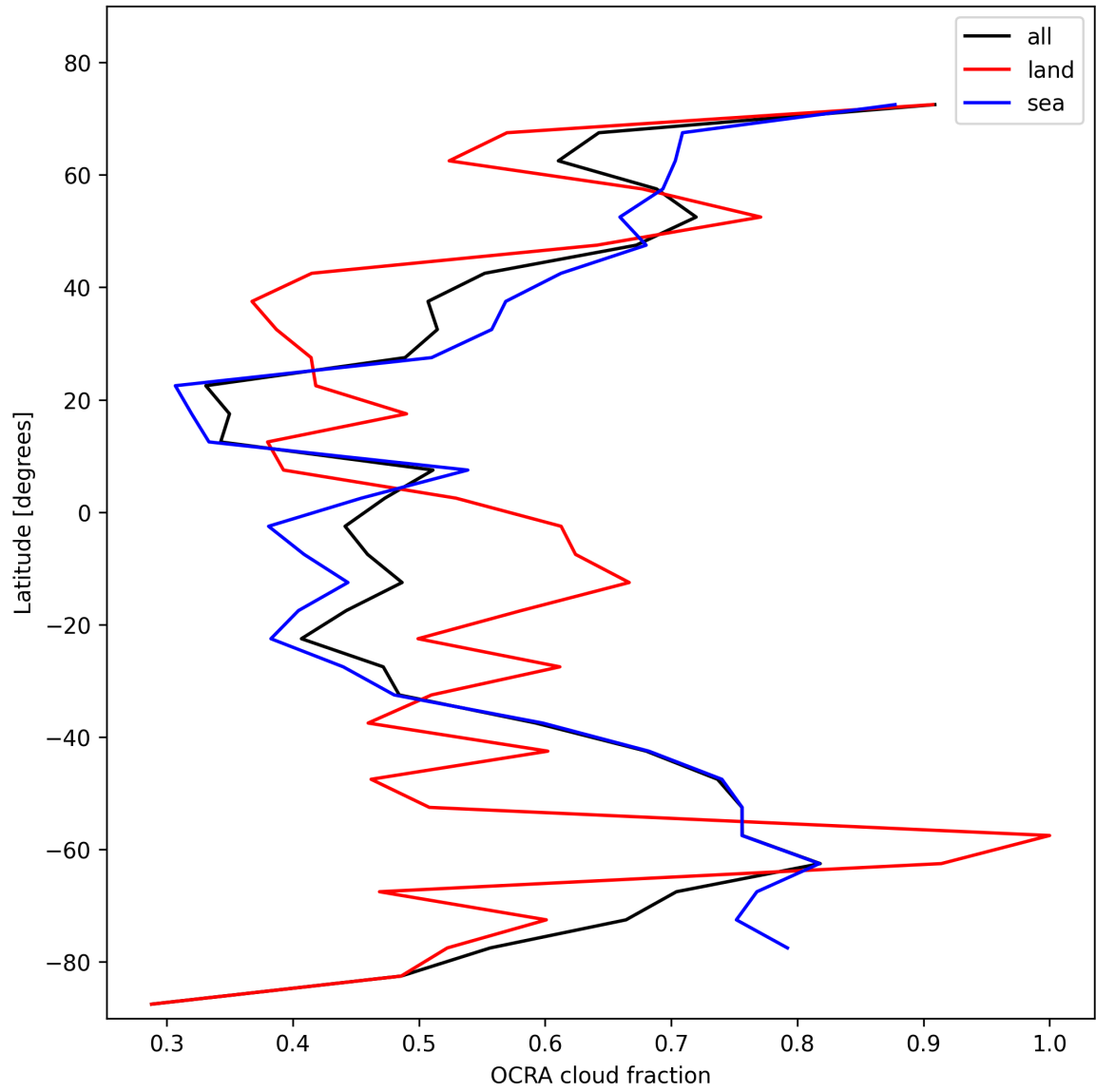
Figure 34: Zonal average of “OCRA cloud fraction” for 2025-11-12 to 2025-11-13.
