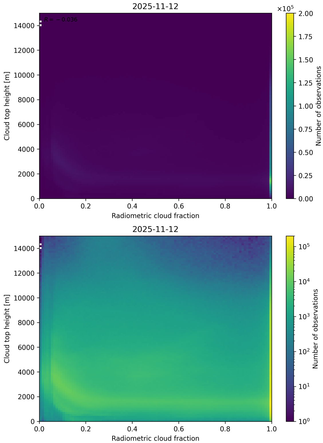
Figure 76: Scatter density plot of “Radiometric cloud fraction” against “Cloud top height” for 2025-11-12 to 2025-11-13.
