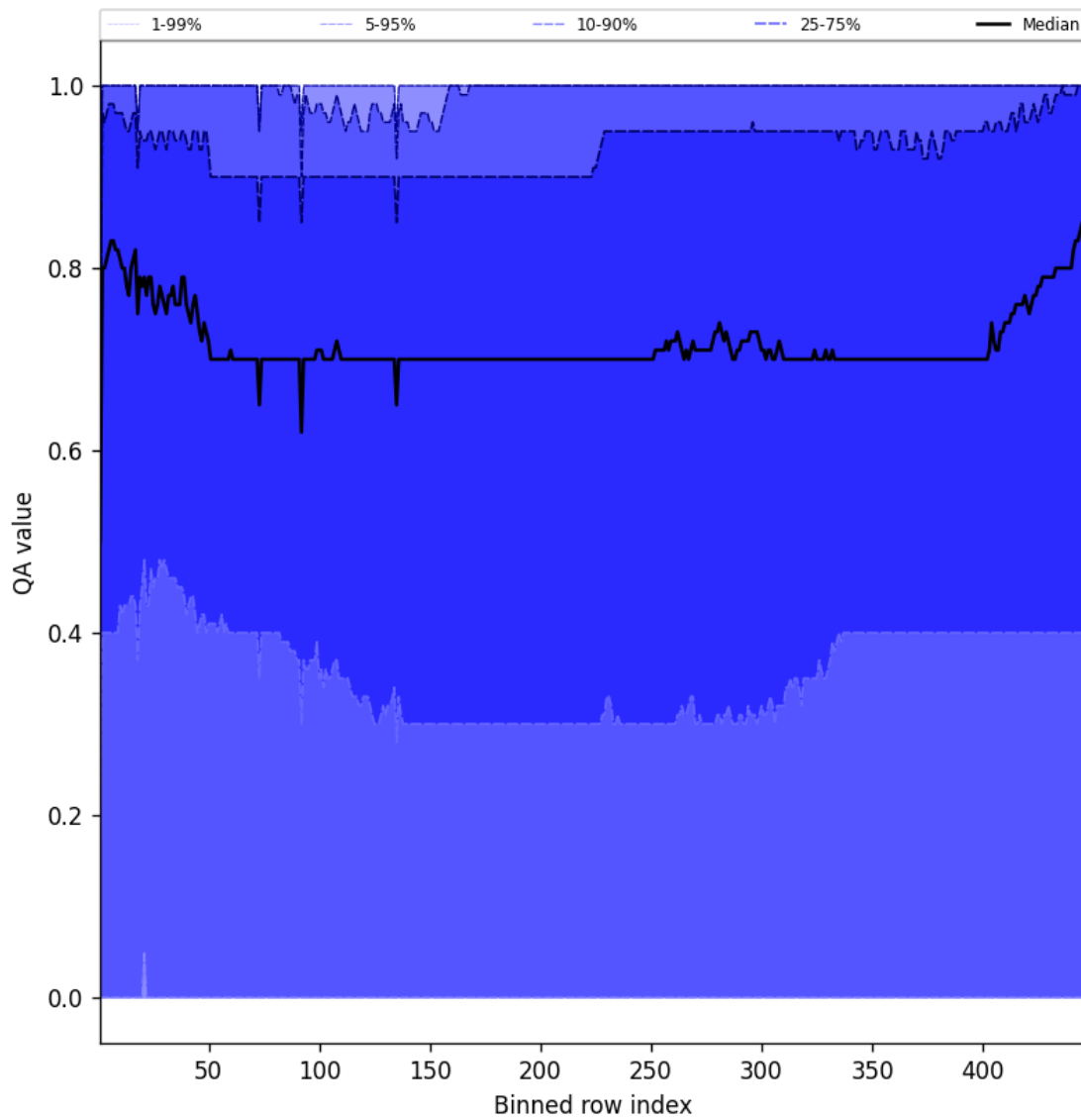
Figure 54: Along track statistics of “QA value” for 2025-11-12 to 2025-11-13
