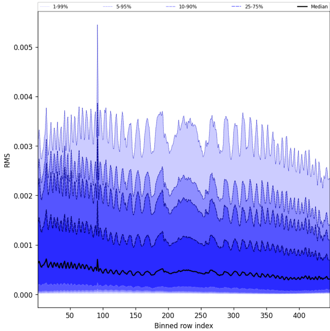
Figure 63: Along track statistics of “RMS” for 2025-11-12 to 2025-11-13
