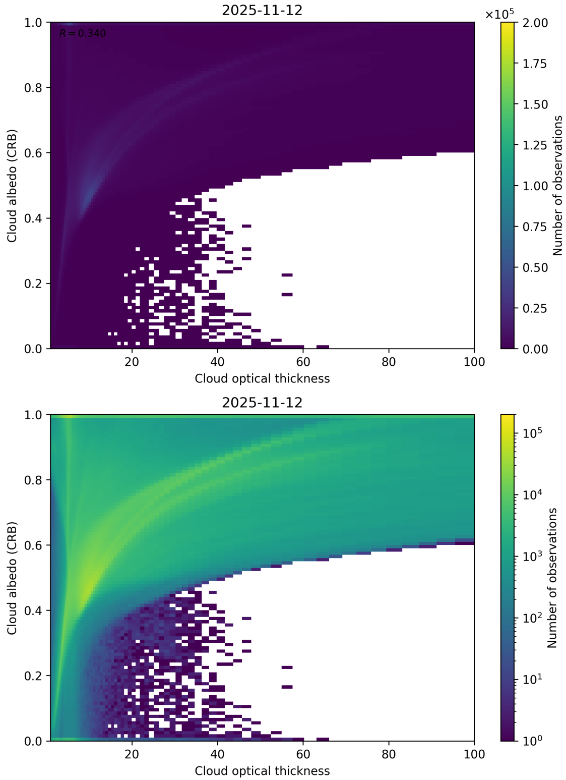
Figure 82: Scatter density plot of “Cloud optical thickness” against “Cloud albedo (CRB)” for 2025-11-12 to 2025-11-13.
