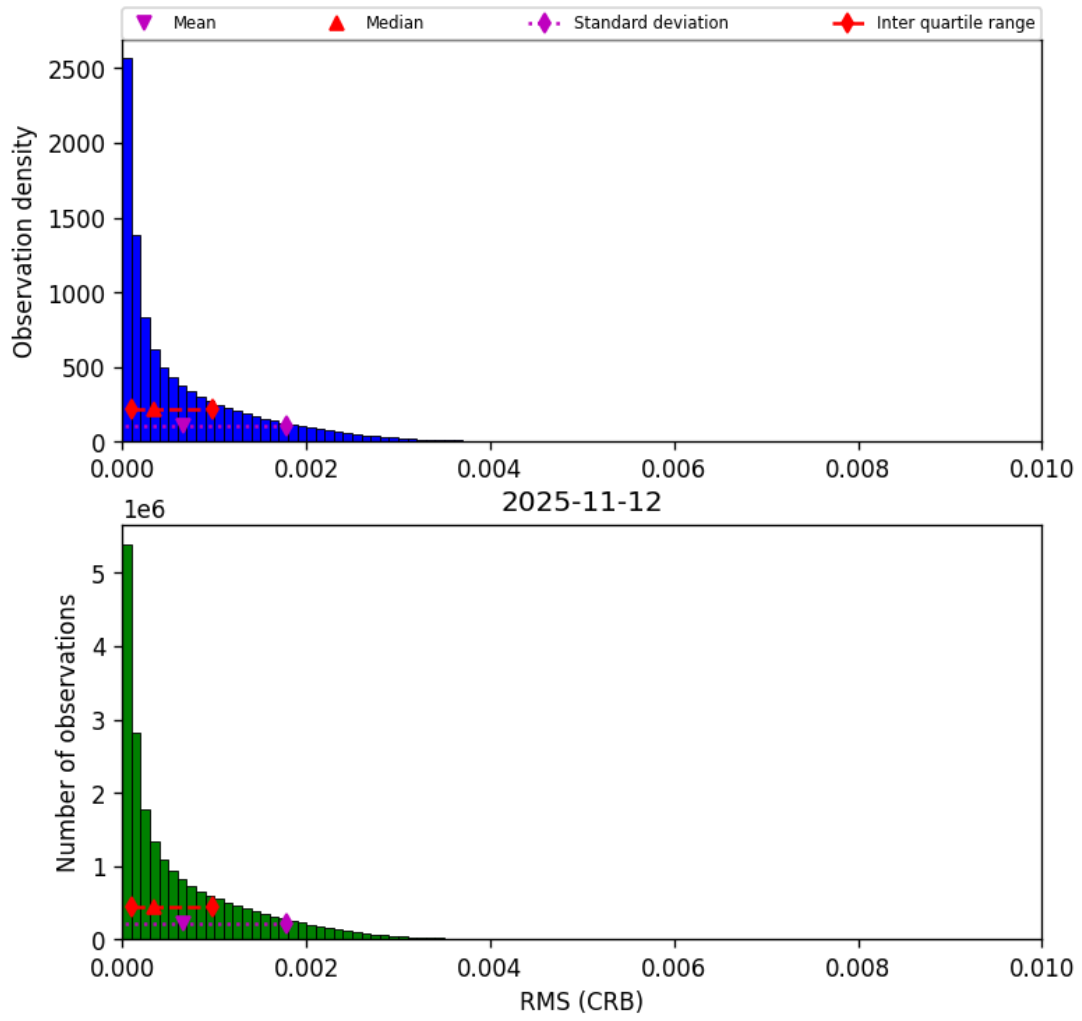
Figure 48: Histogram of “RMS (CRB)” for 2025-11-12 to 2025-11-13
