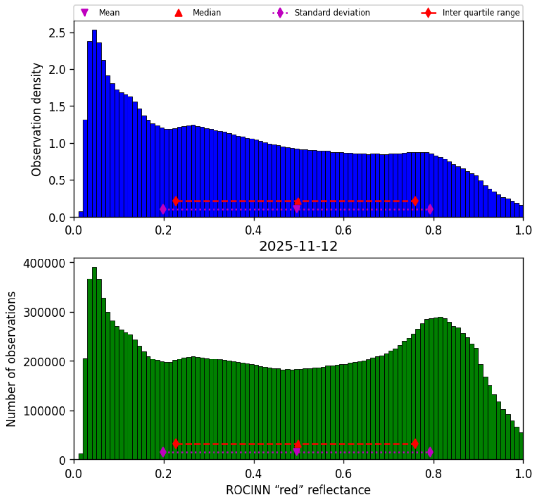
Figure 53: Histogram of “ROCINN “red” reflectance” for 2025-11-12 to 2025-11-13
