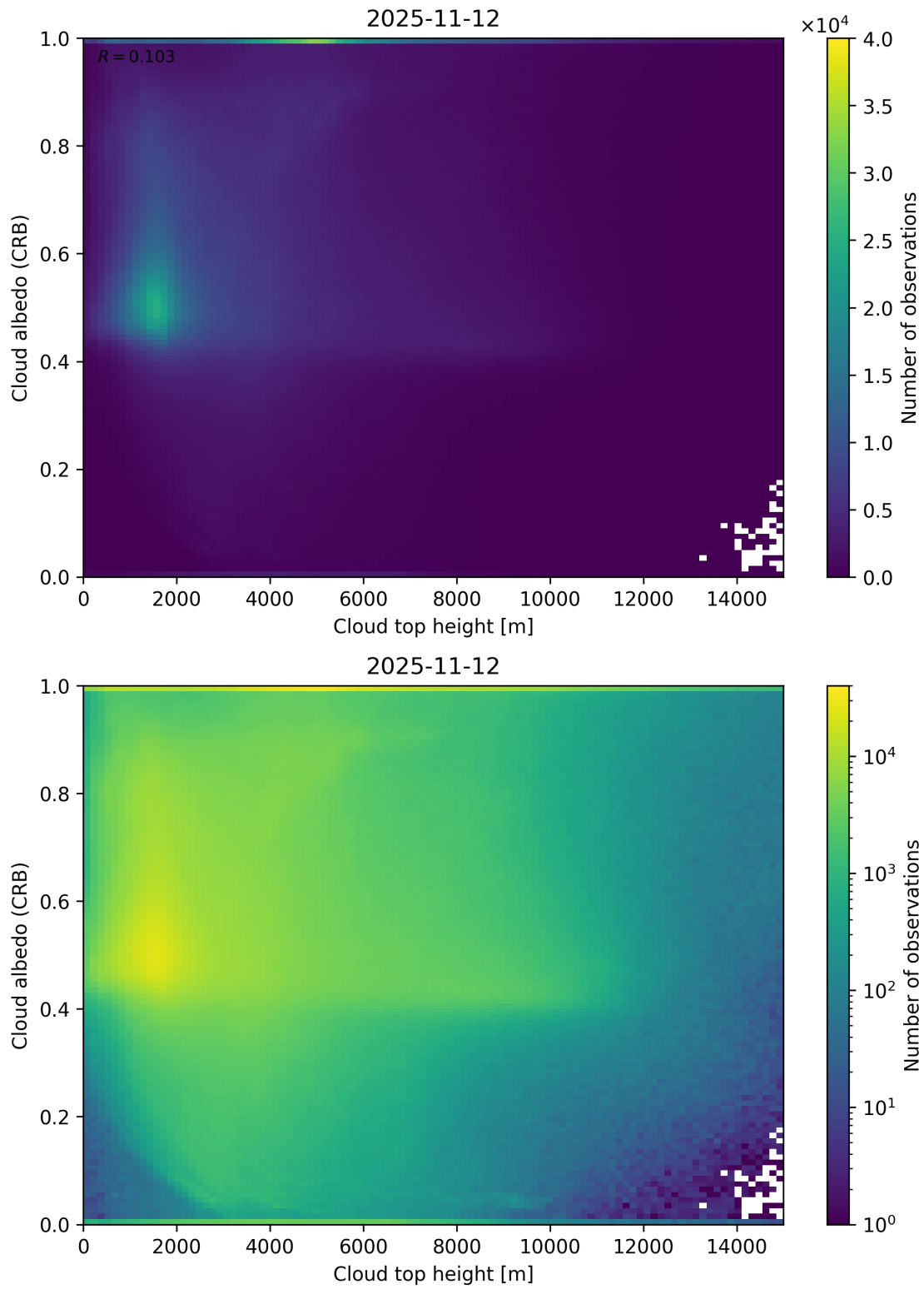
Figure 86: Scatter density plot of “Cloud top height” against “Cloud albedo (CRB)” for 2025-11-12 to 2025-11-13.
