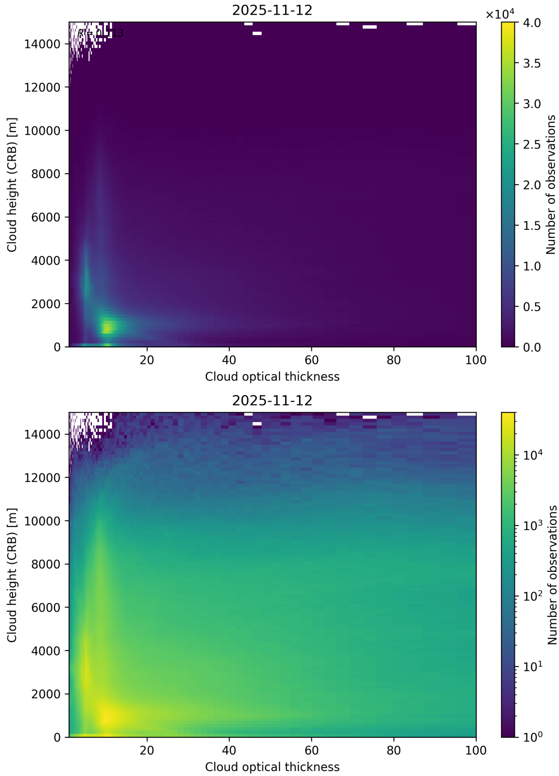
Figure 85: Scatter density plot of “Cloud optical thickness” against “Cloud height (CRB)” for 2025-11-12 to 2025-11-13.
