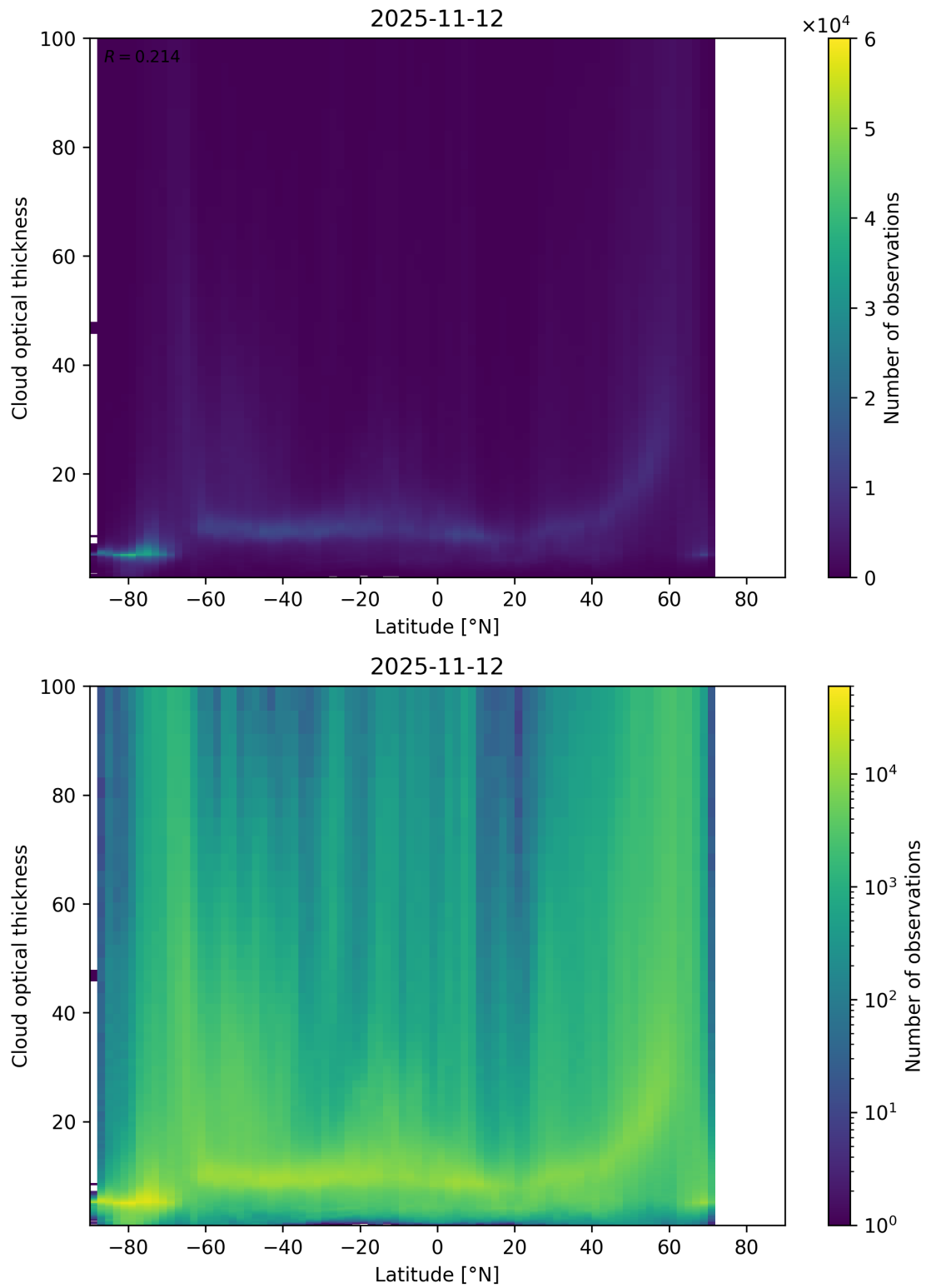
Figure 96: Scatter density plot of “Latitude” against “Cloud optical thickness” for 2025-11-12 to 2025-11-13.
