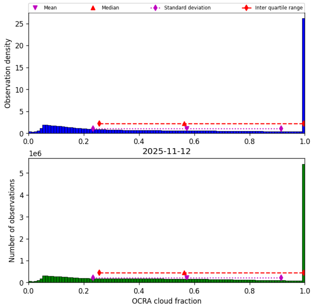
Figure 50: Histogram of “OCRA cloud fraction” for 2025-11-12 to 2025-11-13
