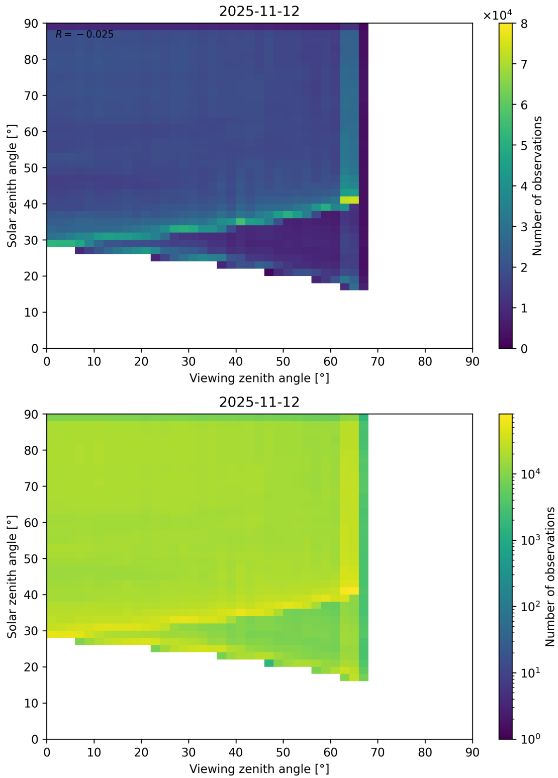
Figure 114: Scatter density plot of “Viewing zenith angle” against “Solar zenith angle” for 2025-11-12 to 2025-11-13.
