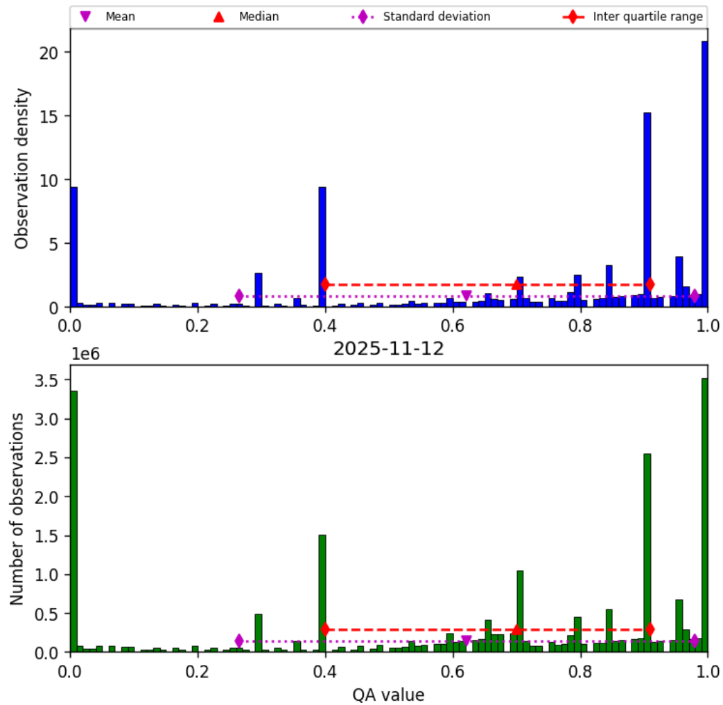
Figure 38: Histogram of “QA value” for 2025-11-12 to 2025-11-13
