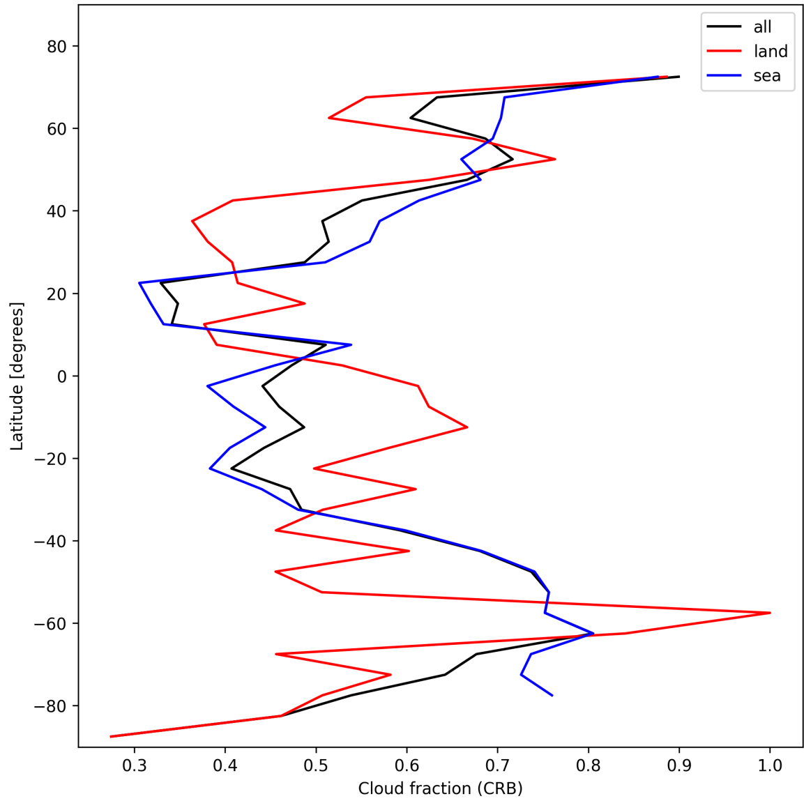
Figure 26: Zonal average of “Cloud fraction (CRB)” for 2025-11-12 to 2025-11-13.
