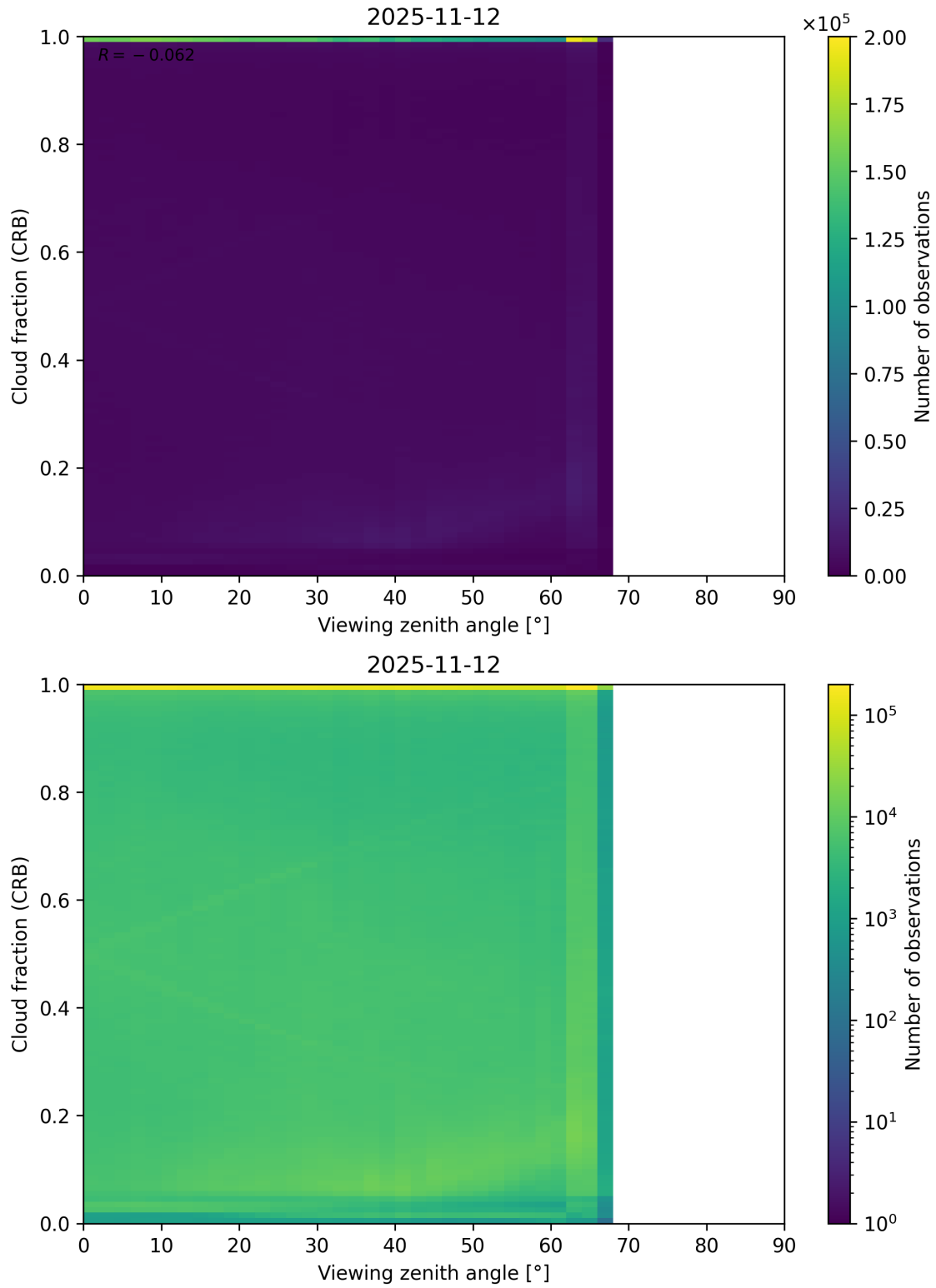
Figure 109: Scatter density plot of “Viewing zenith angle” against “Cloud fraction (CRB)” for 2025-11-12 to 2025-11-13.
