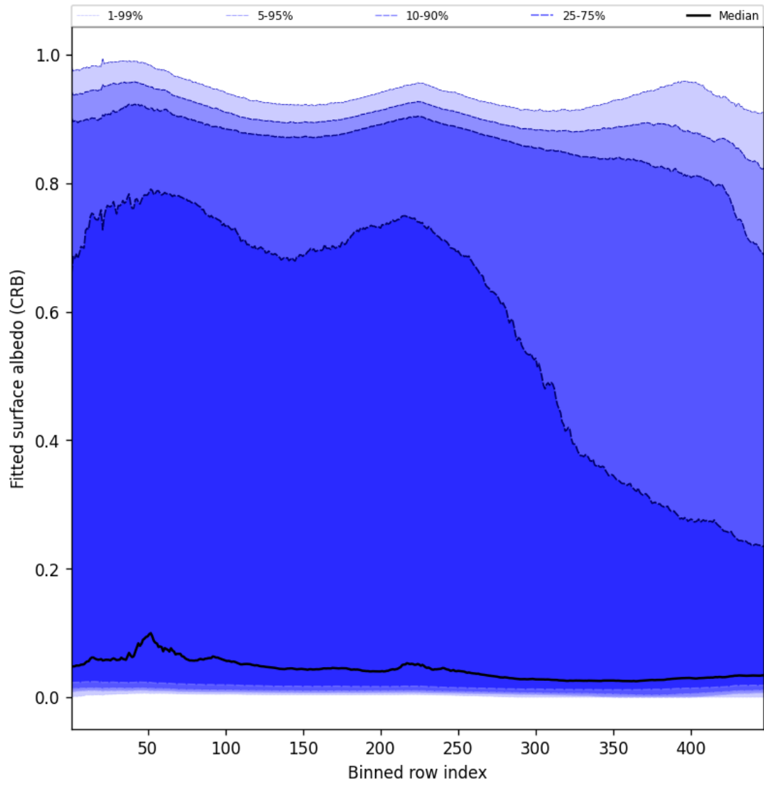
Figure 62: Along track statistics of “Fitted surface albedo (CRB)” for 2025-11-12 to 2025-11-13
