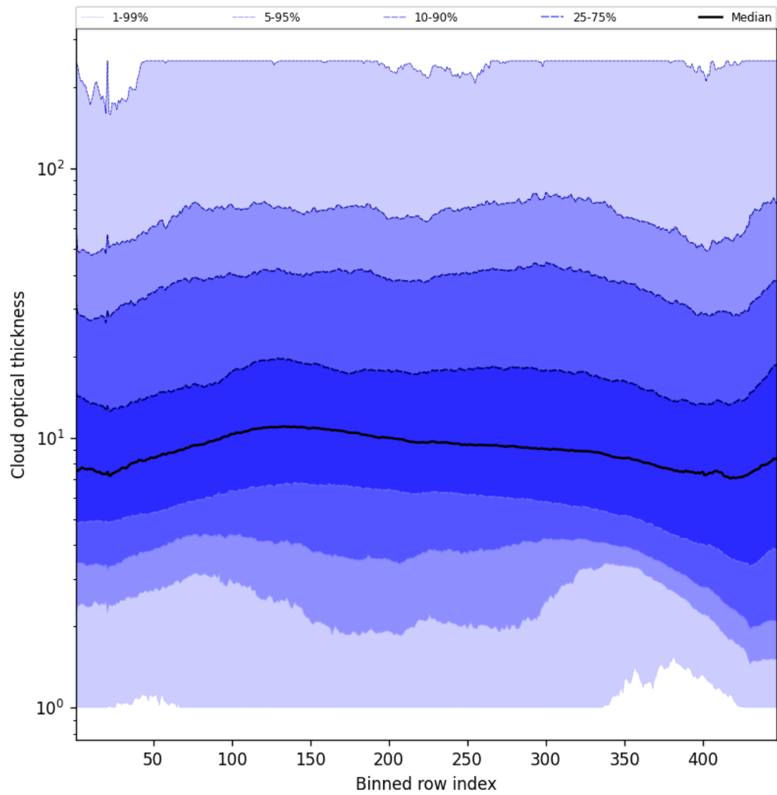
Figure 57: Along track statistics of “Cloud optical thickness” for 2025-11-12 to 2025-11-13
