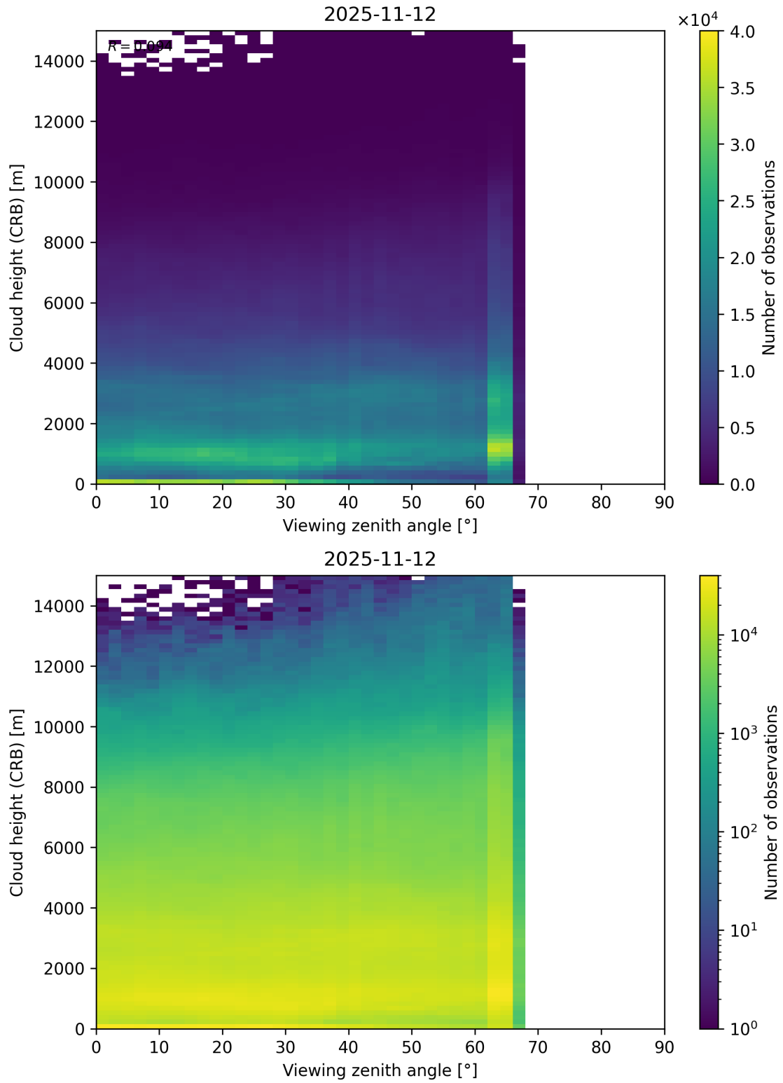
Figure 110: Scatter density plot of “Viewing zenith angle” against “Cloud height (CRB)” for 2025-11-12 to 2025-11-13.
