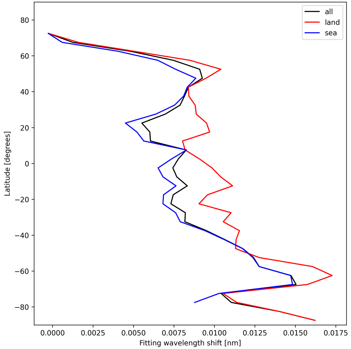
Figure 33: Zonal average of “Fitting wavelength shift” for 2025-11-12 to 2025-11-13.
