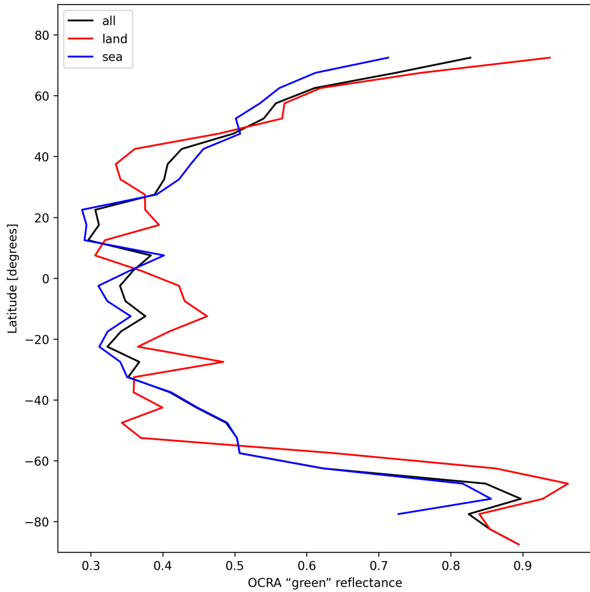
Figure 36: Zonal average of “OCRA “green” reflectance” for 2025-11-12 to 2025-11-13.
