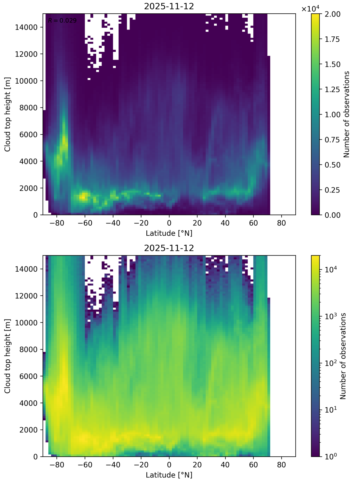
Figure 97: Scatter density plot of “Latitude” against “Cloud top height” for 2025-11-12 to 2025-11-13.
