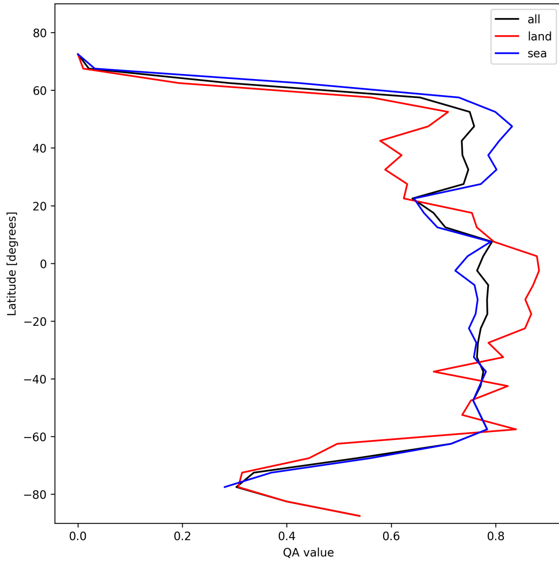
Figure 22: Zonal average of “QA value” for 2025-11-12 to 2025-11-13.
