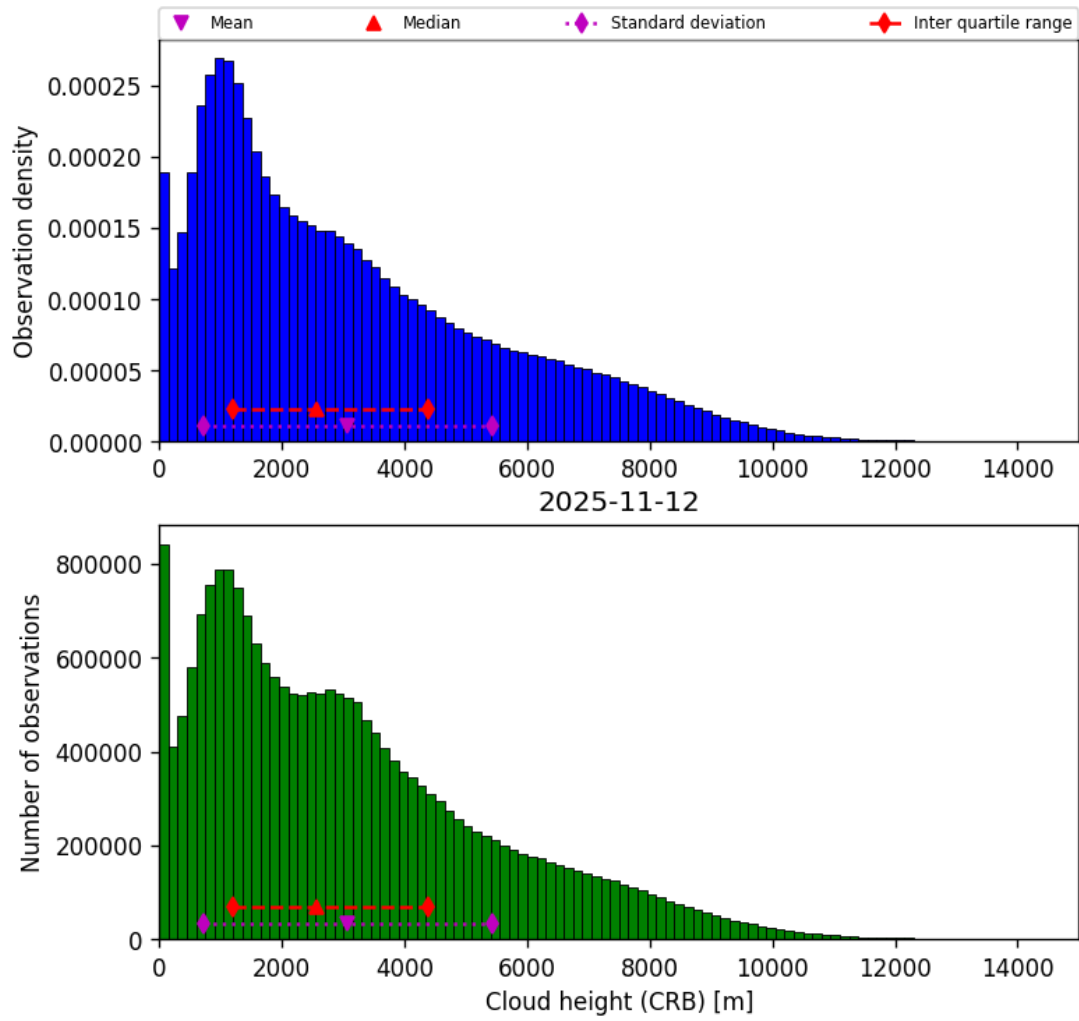
Figure 43: Histogram of “Cloud height (CRB)” for 2025-11-12 to 2025-11-13
