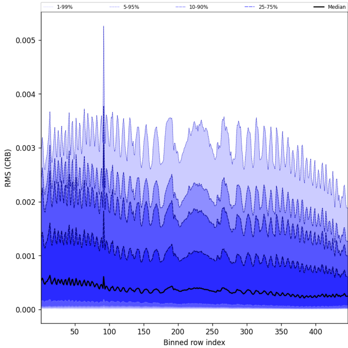
Figure 64: Along track statistics of “RMS (CRB)” for 2025-11-12 to 2025-11-13
