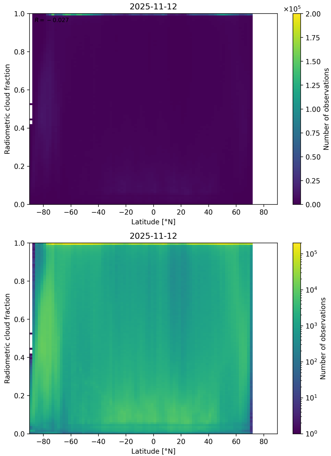
Figure 92: Scatter density plot of “Latitude” against “Radiometric cloud fraction” for 2025-11-12 to 2025-11-13.
