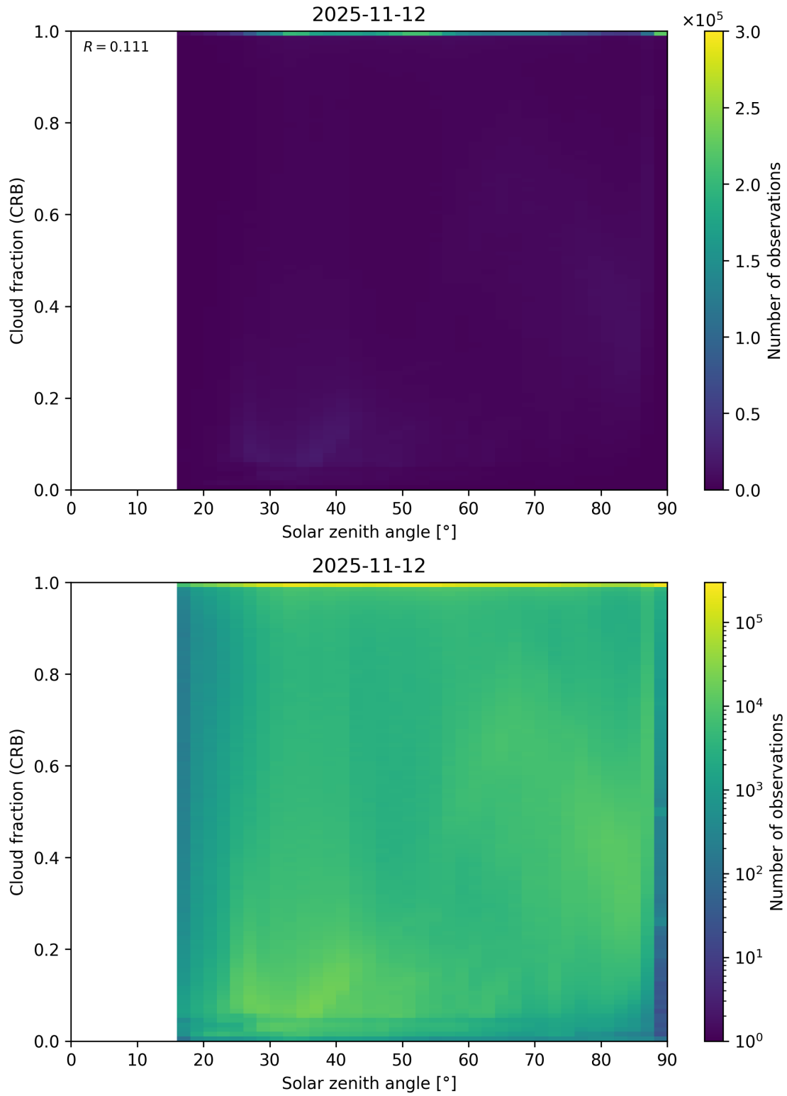
Figure 101: Scatter density plot of “Solar zenith angle” against “Cloud fraction (CRB)” for 2025-11-12 to 2025-11-13.
