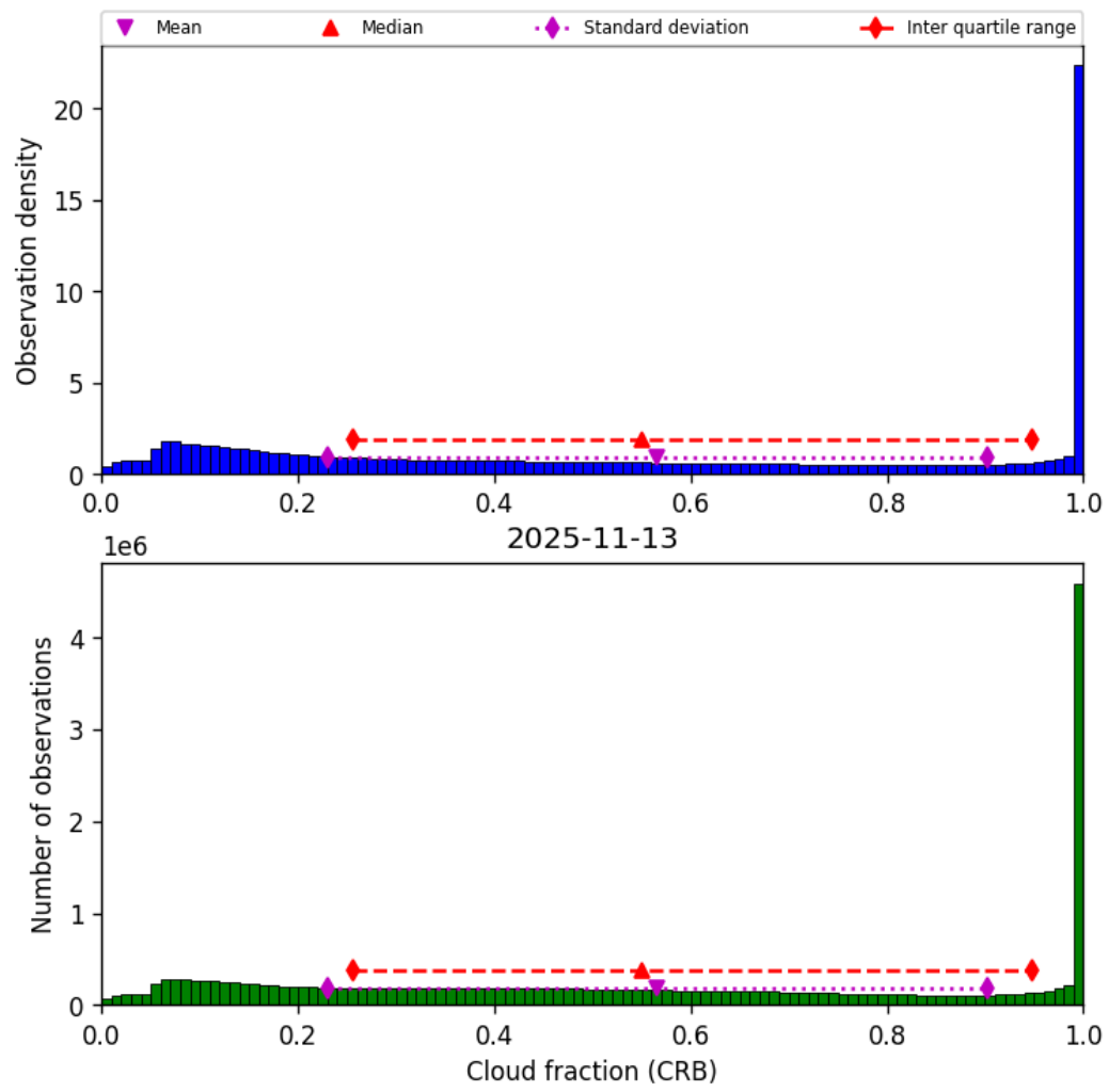
Figure 42: Histogram of “Cloud fraction (CRB)” for 2025-11-12 to 2025-11-14
