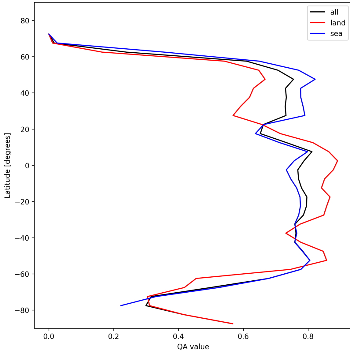
Figure 22: Zonal average of “QA value” for 2025-11-12 to 2025-11-14.
