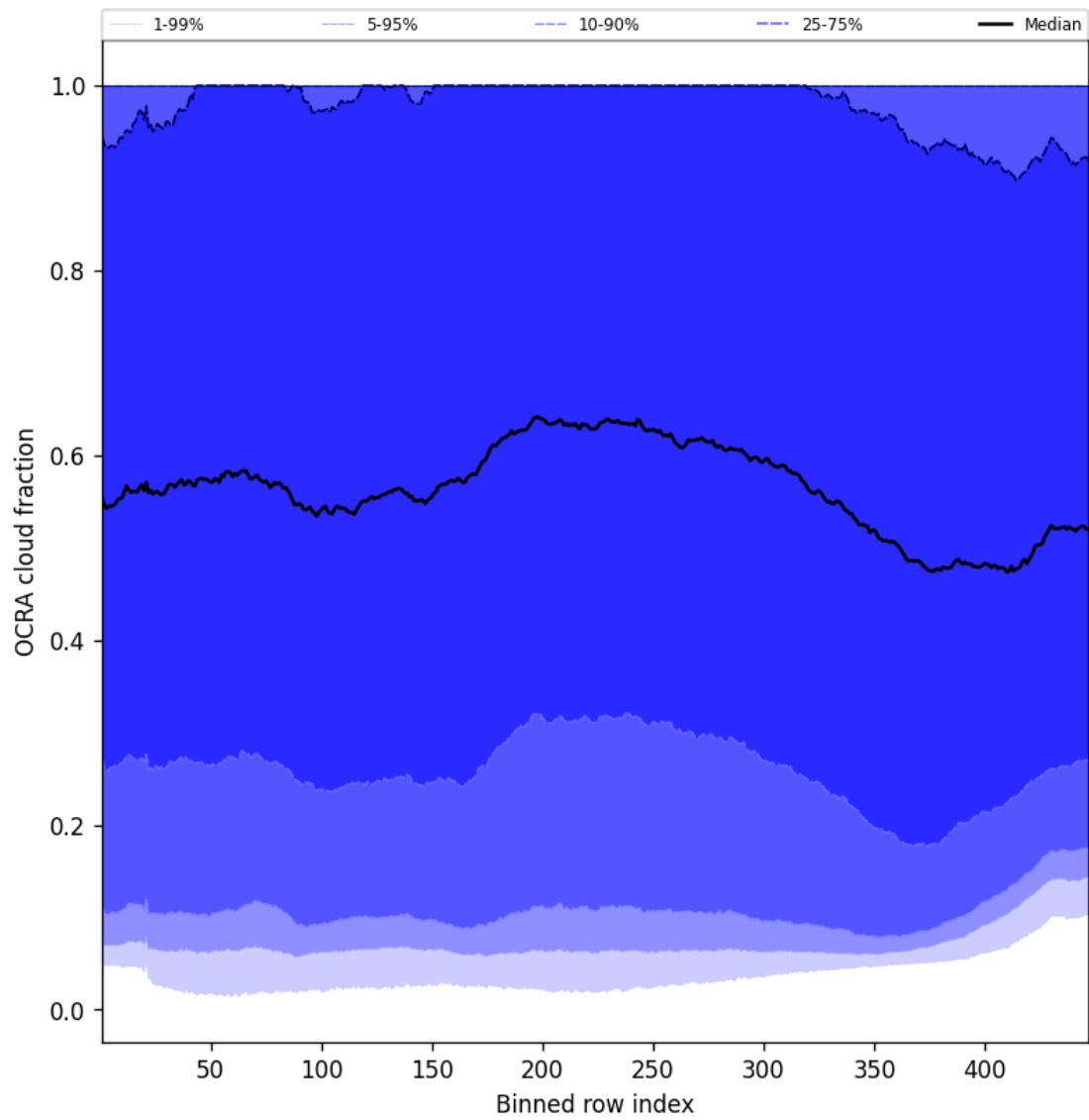
Figure 66: Along track statistics of “OCRA cloud fraction” for 2025-11-12 to 2025-11-14
