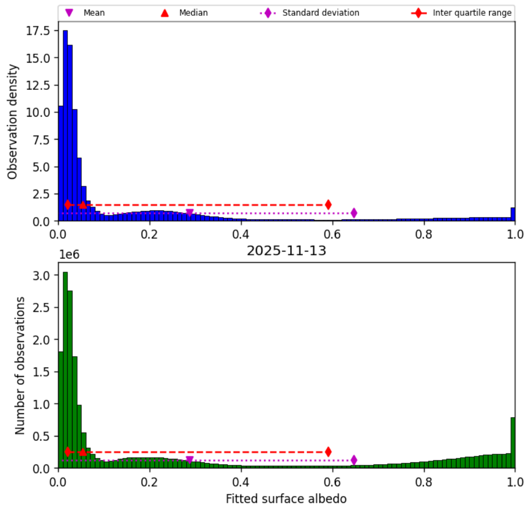
Figure 45: Histogram of “Fitted surface albedo” for 2025-11-12 to 2025-11-14
