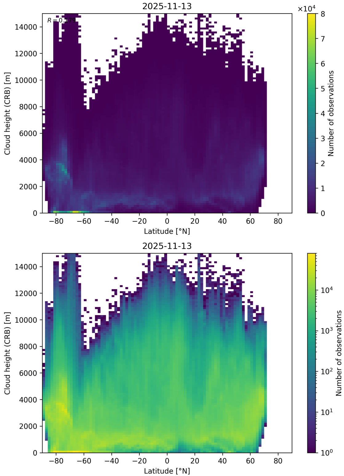
Figure 95: Scatter density plot of “Latitude” against “Cloud height (CRB)” for 2025-11-12 to 2025-11-14.
