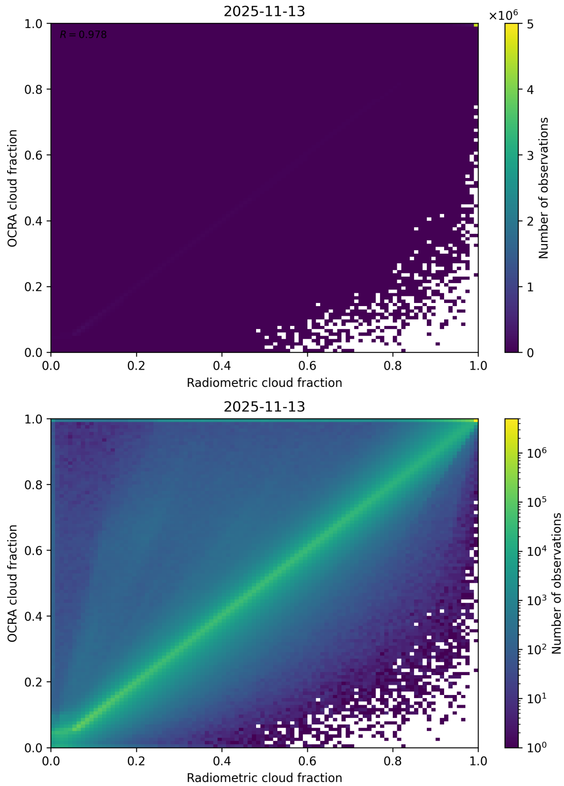
Figure 72: Scatter density plot of “Radiometric cloud fraction” against “OCRA cloud fraction” for 2025-11-12 to 2025-11-14.
