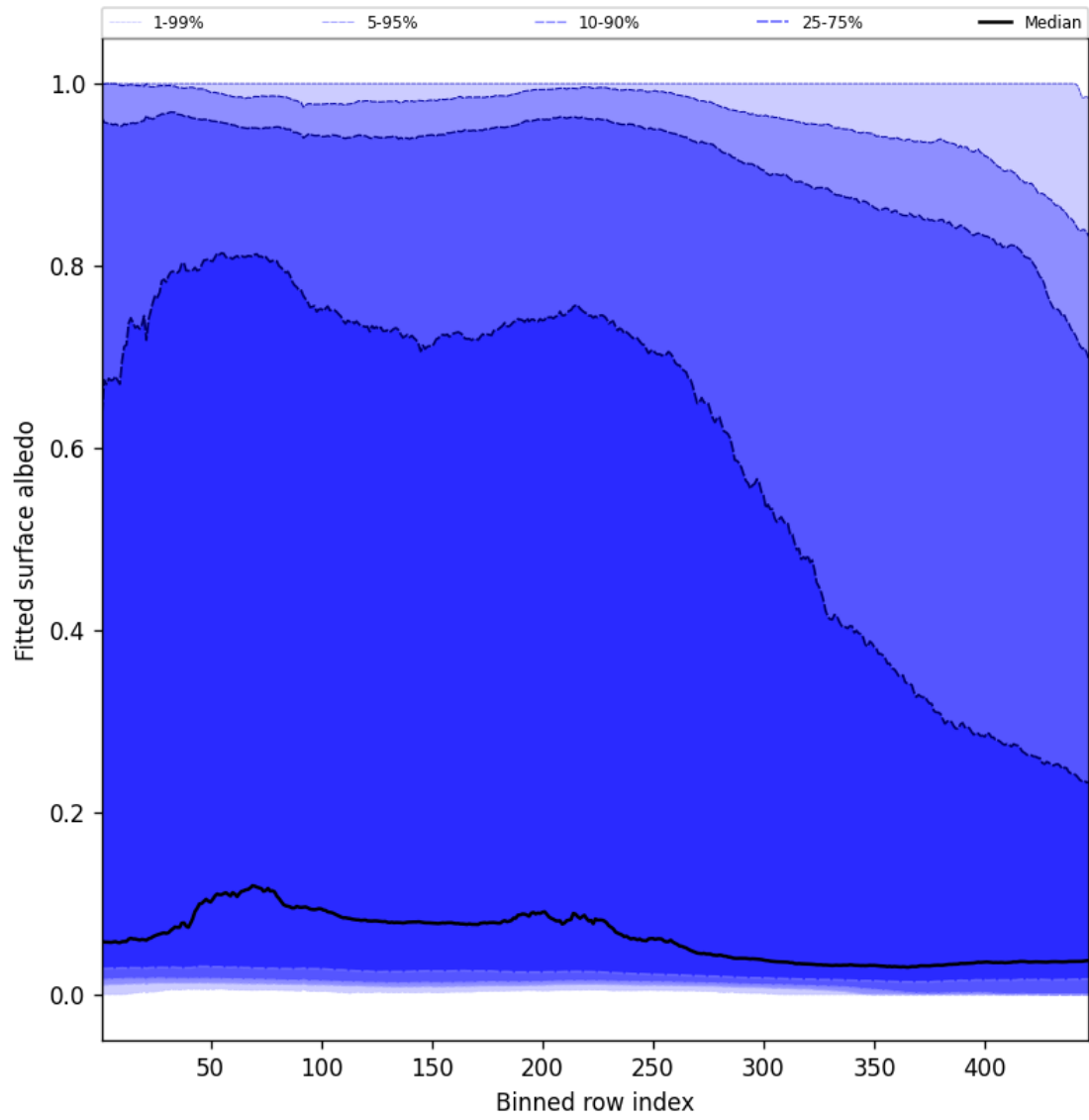
Figure 61: Along track statistics of “Fitted surface albedo” for 2025-11-12 to 2025-11-14
