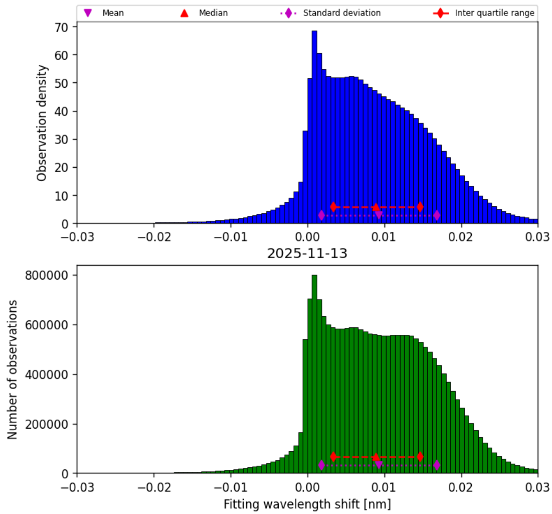
Figure 49: Histogram of “Fitting wavelength shift” for 2025-11-12 to 2025-11-14
