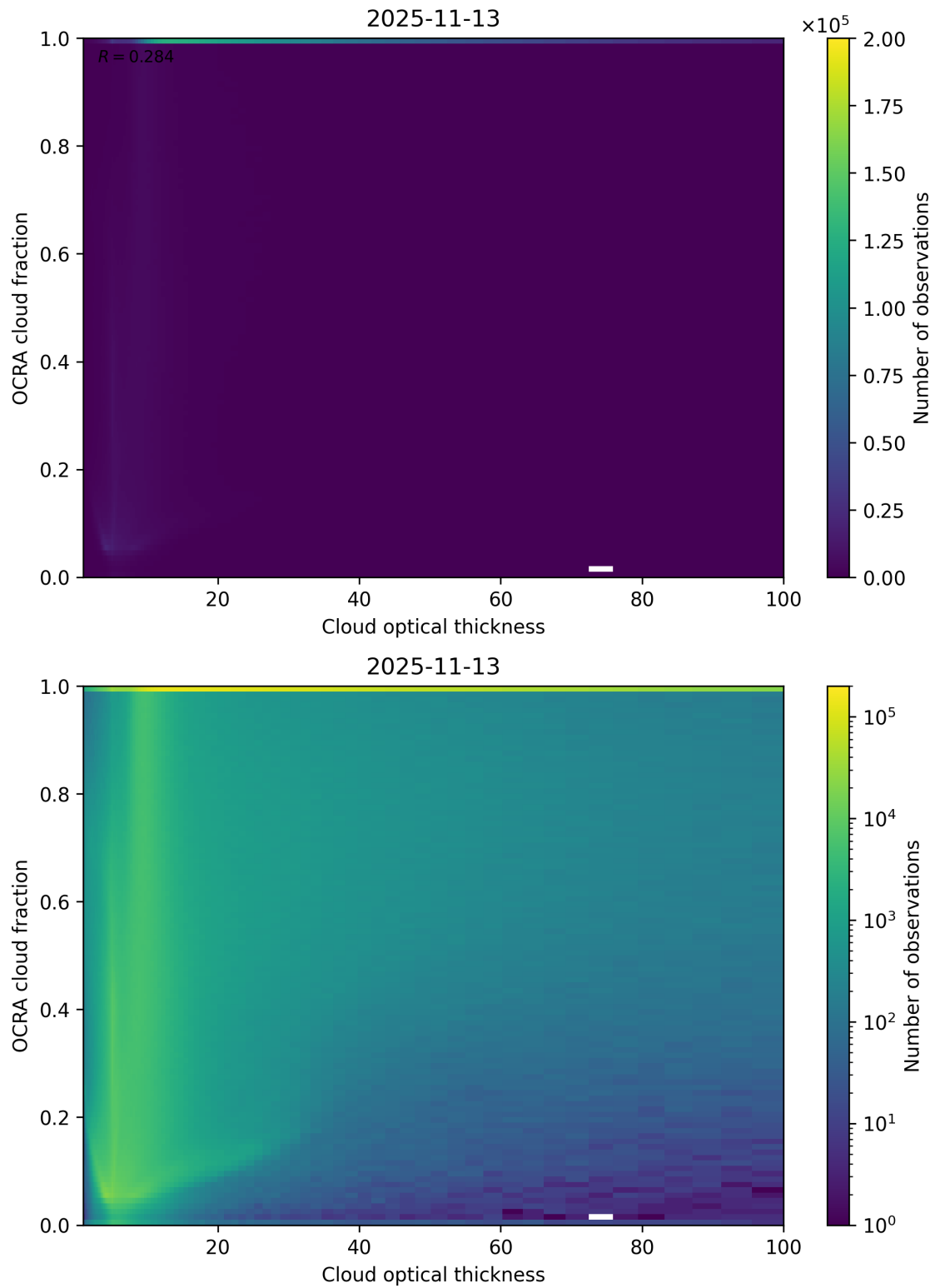
Figure 83: Scatter density plot of “Cloud optical thickness” against “OCRA cloud fraction” for 2025-11-12 to 2025-11-14.
