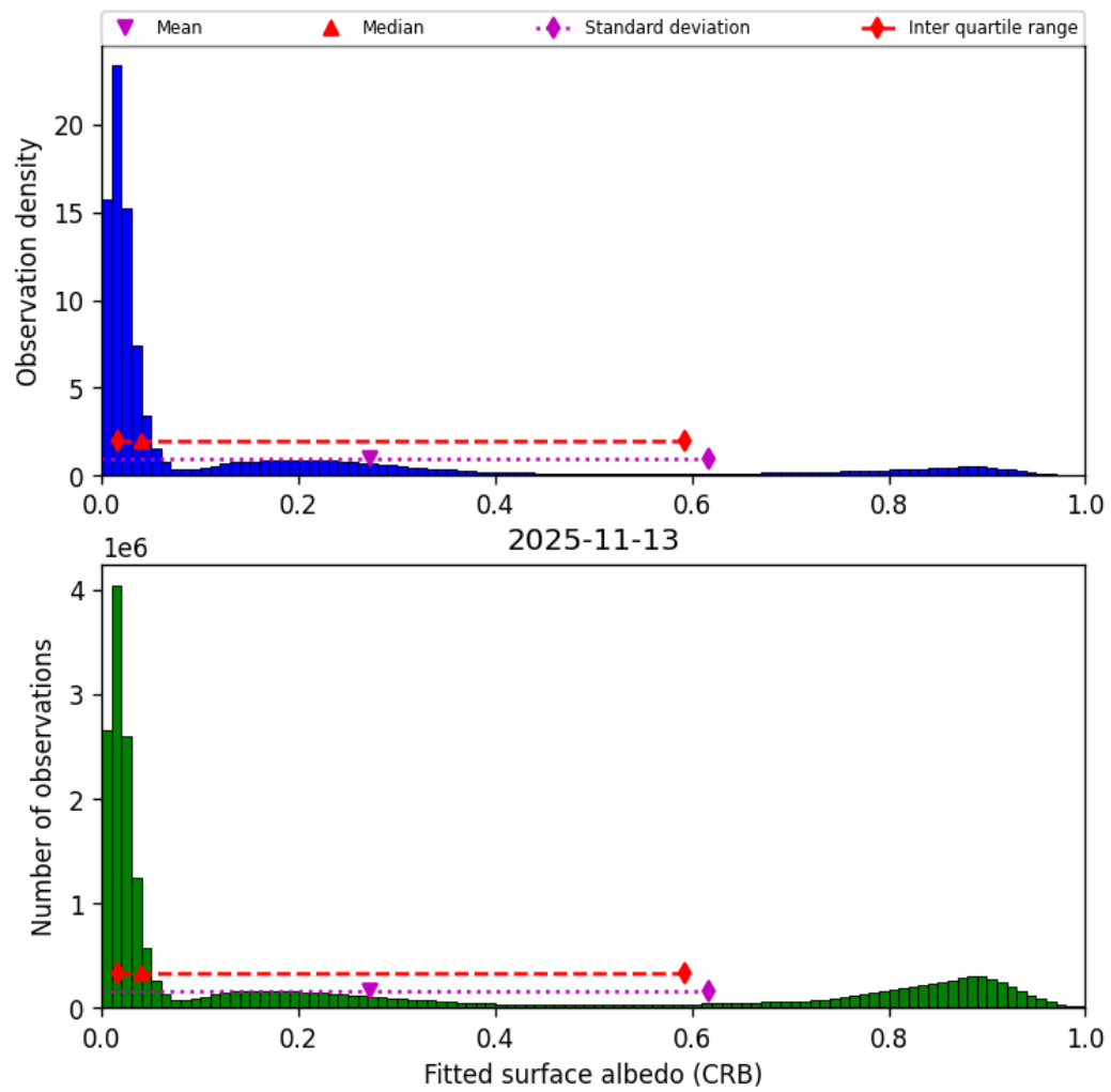
Figure 46: Histogram of “Fitted surface albedo (CRB)” for 2025-11-12 to 2025-11-14
