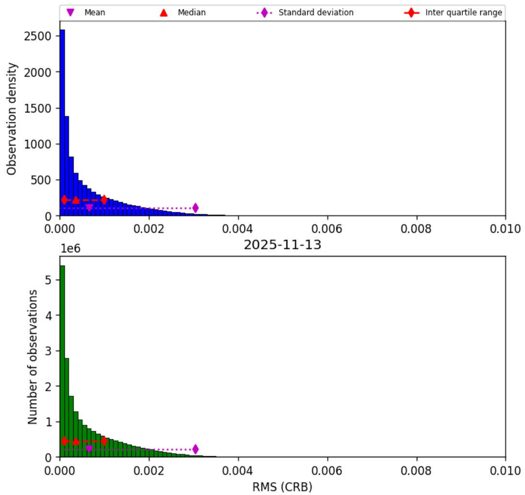
Figure 48: Histogram of “RMS (CRB)” for 2025-11-12 to 2025-11-14
