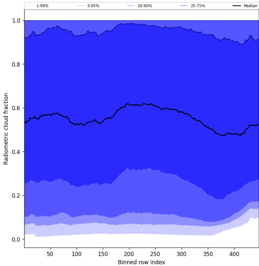
Figure 55: Along track statistics of “Radiometric cloud fraction” for 2025-11-12 to 2025-11-14
