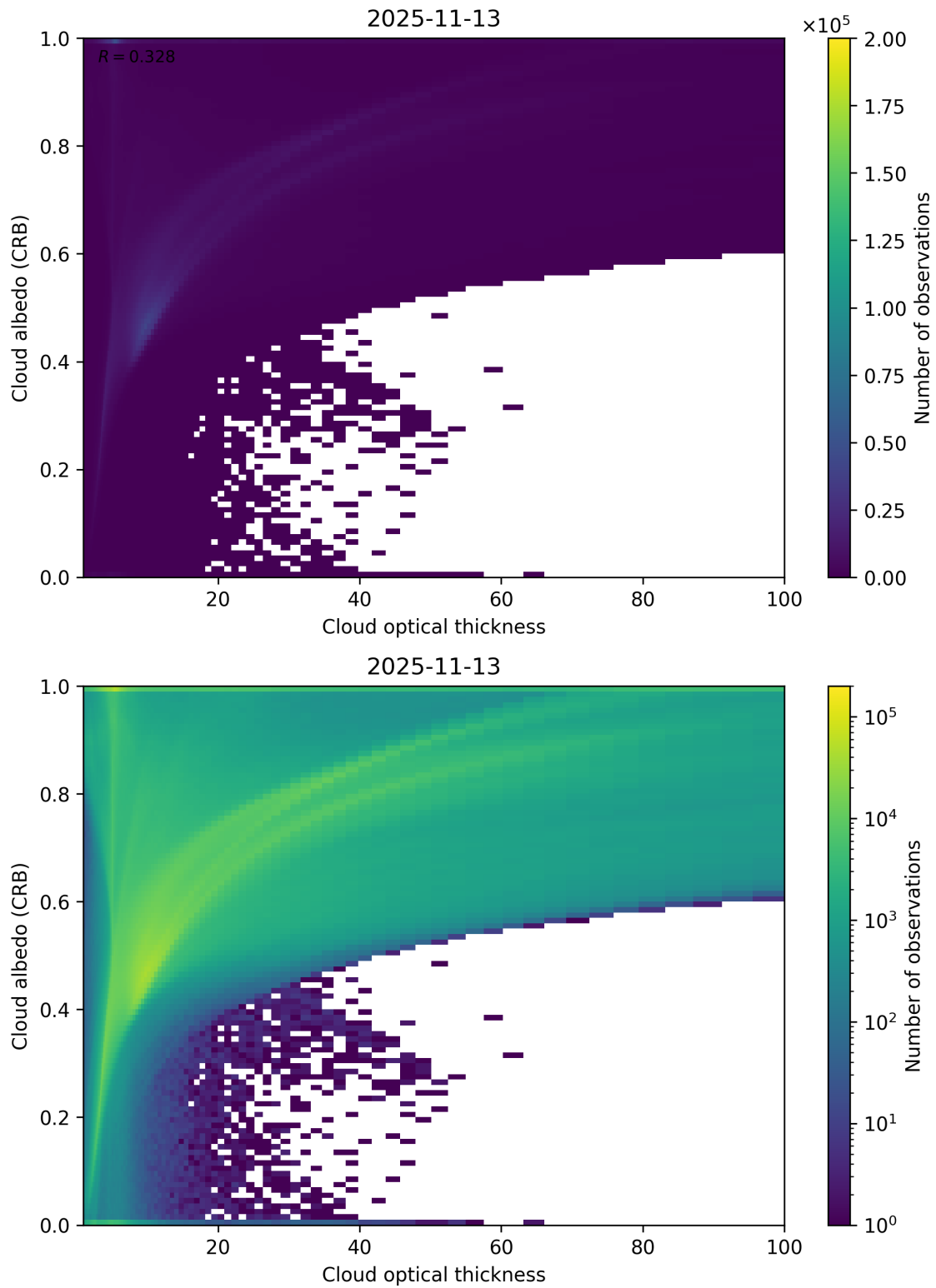
Figure 82: Scatter density plot of “Cloud optical thickness” against “Cloud albedo (CRB)” for 2025-11-12 to 2025-11-14.
