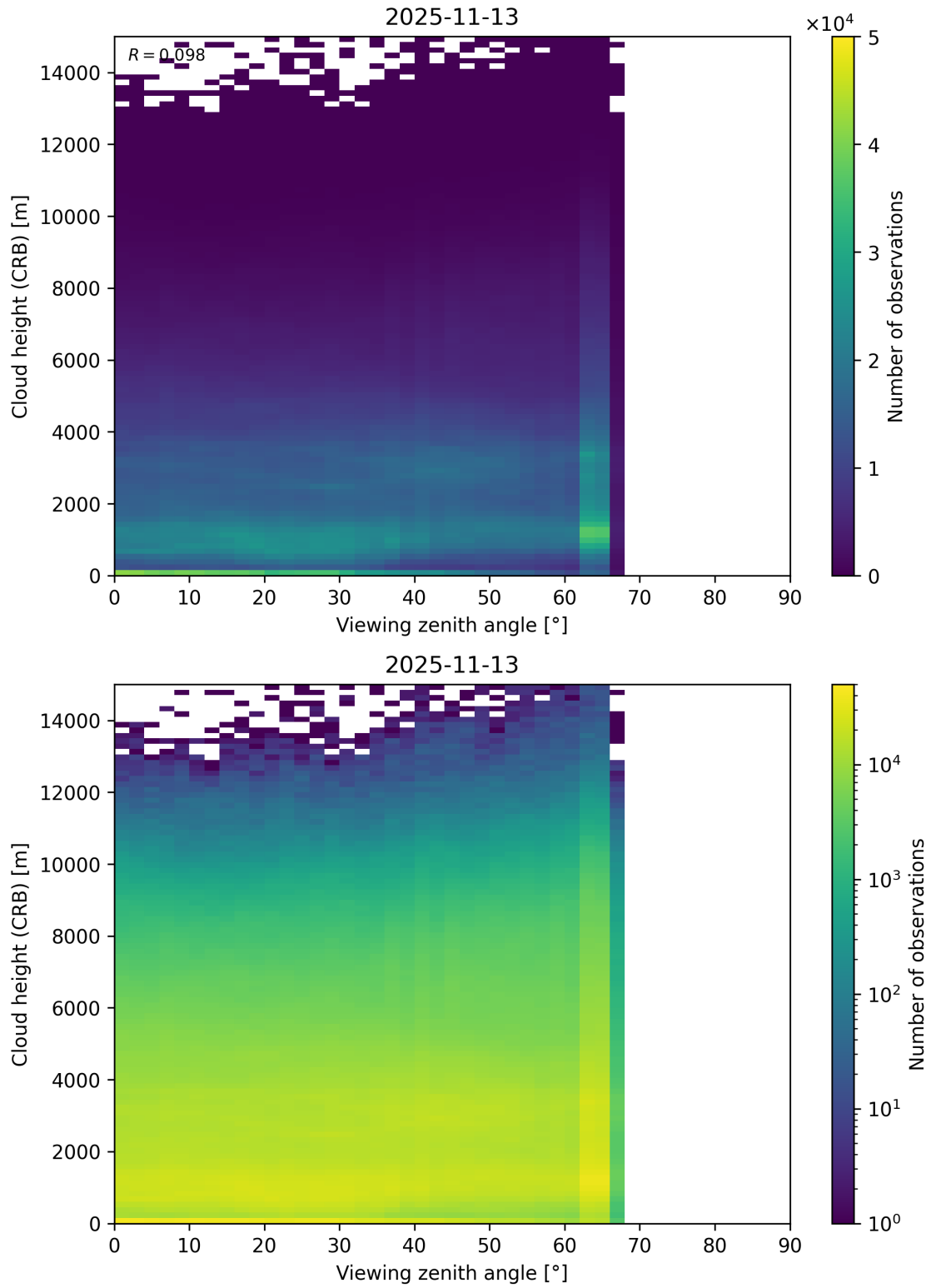
Figure 110: Scatter density plot of “Viewing zenith angle” against “Cloud height (CRB)” for 2025-11-12 to 2025-11-14.
