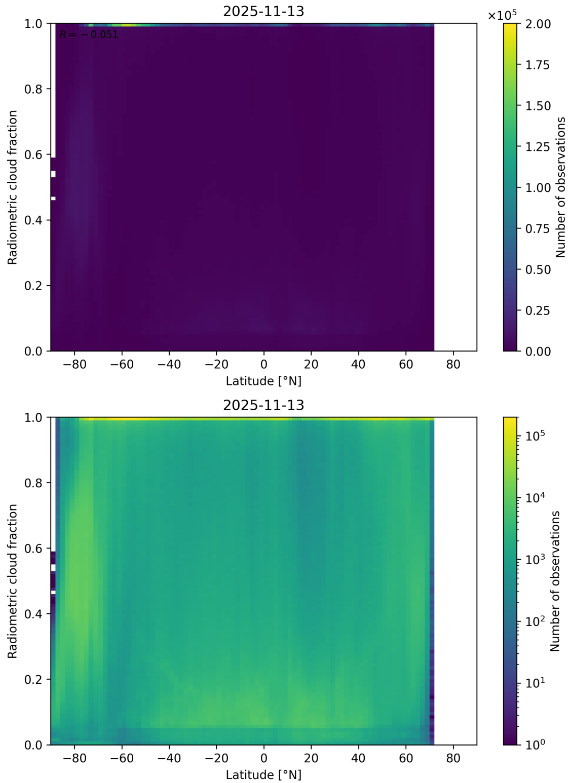
Figure 92: Scatter density plot of “Latitude” against “Radiometric cloud fraction” for 2025-11-12 to 2025-11-14.
