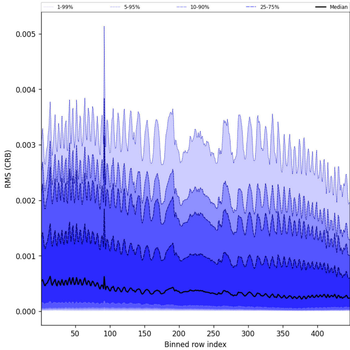
Figure 64: Along track statistics of “RMS (CRB)” for 2025-11-12 to 2025-11-14
