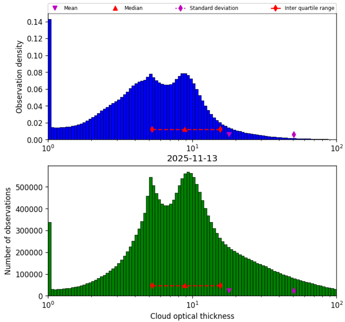
Figure 41: Histogram of “Cloud optical thickness” for 2025-11-12 to 2025-11-14
