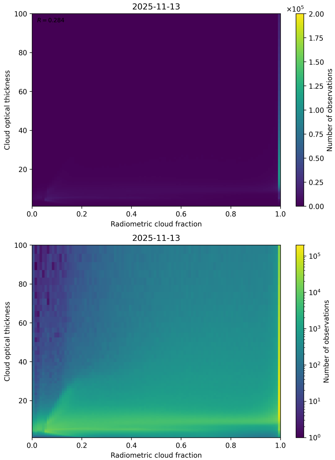
Figure 75: Scatter density plot of “Radiometric cloud fraction” against “Cloud optical thickness” for 2025-11-12 to 2025-11-14.
