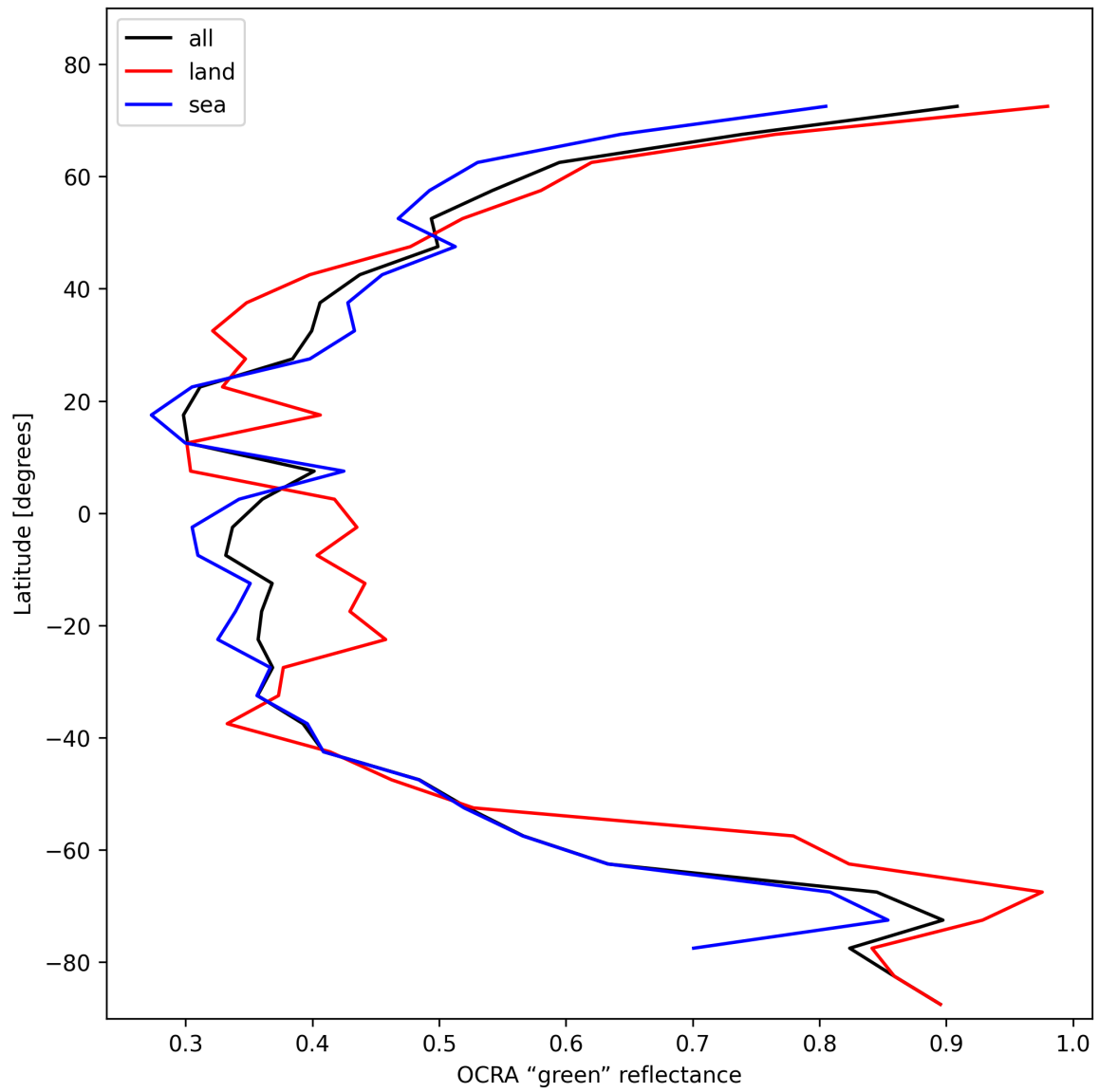
Figure 36: Zonal average of “OCRA “green” reflectance” for 2025-11-12 to 2025-11-14.
