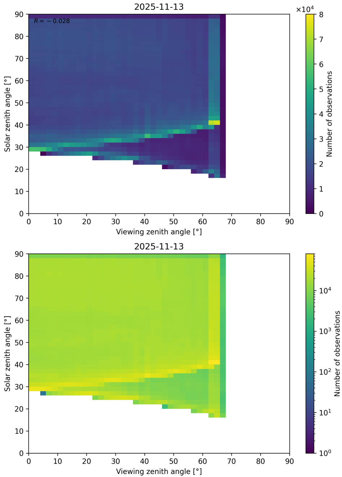
Figure 114: Scatter density plot of “Viewing zenith angle” against “Solar zenith angle” for 2025-11-12 to 2025-11-14.
