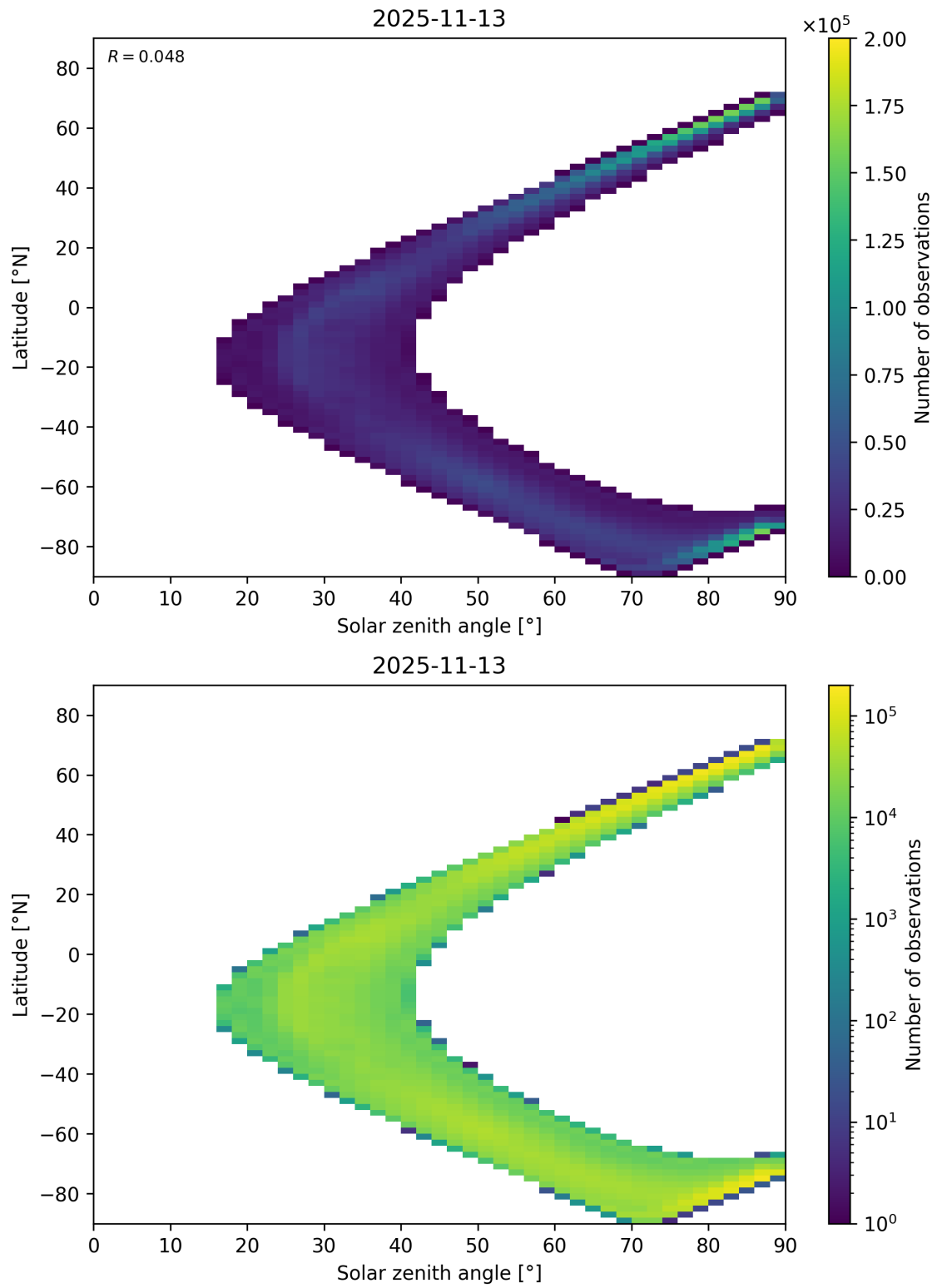
Figure 105: Scatter density plot of “Solar zenith angle” against “Latitude” for 2025-11-12 to 2025-11-14.
