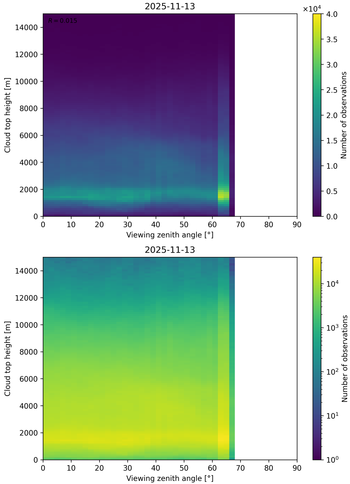
Figure 112: Scatter density plot of “Viewing zenith angle” against “Cloud top height” for 2025-11-12 to 2025-11-14.
