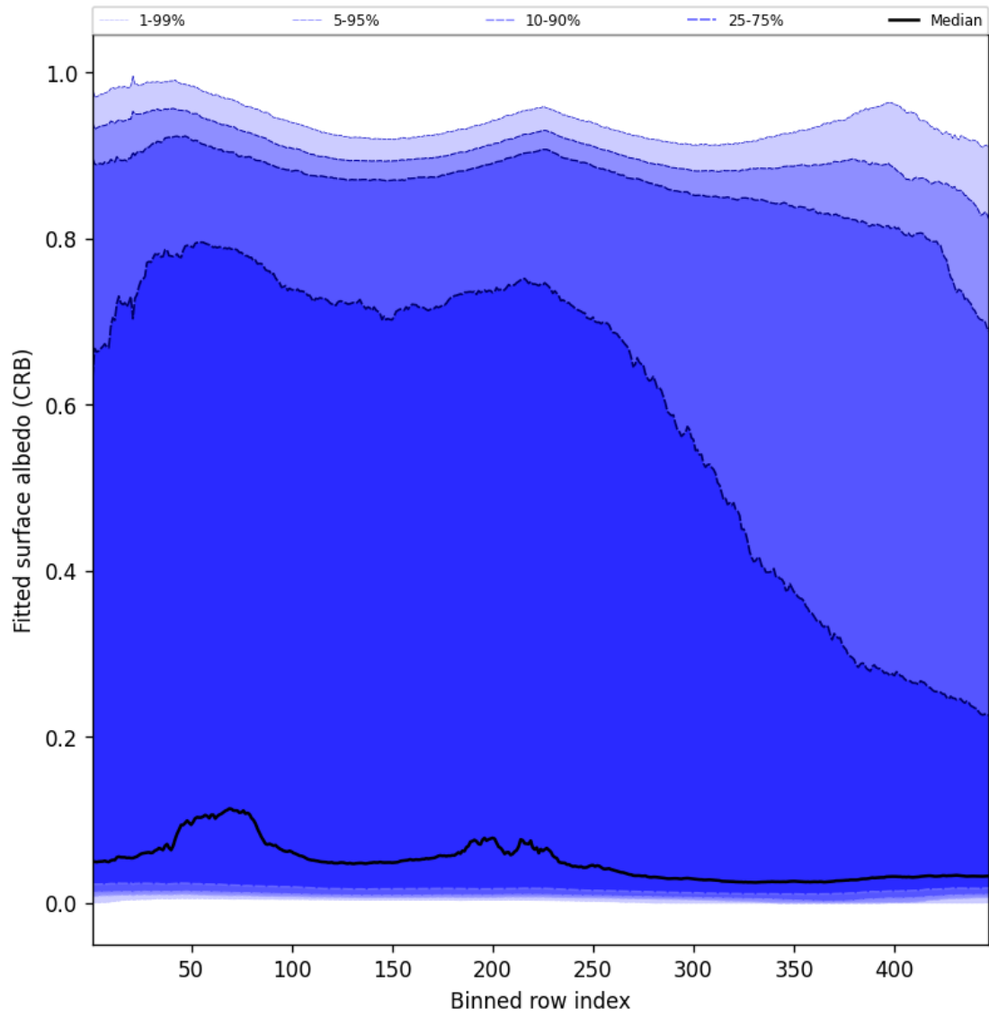
Figure 62: Along track statistics of “Fitted surface albedo (CRB)” for 2025-11-12 to 2025-11-14
