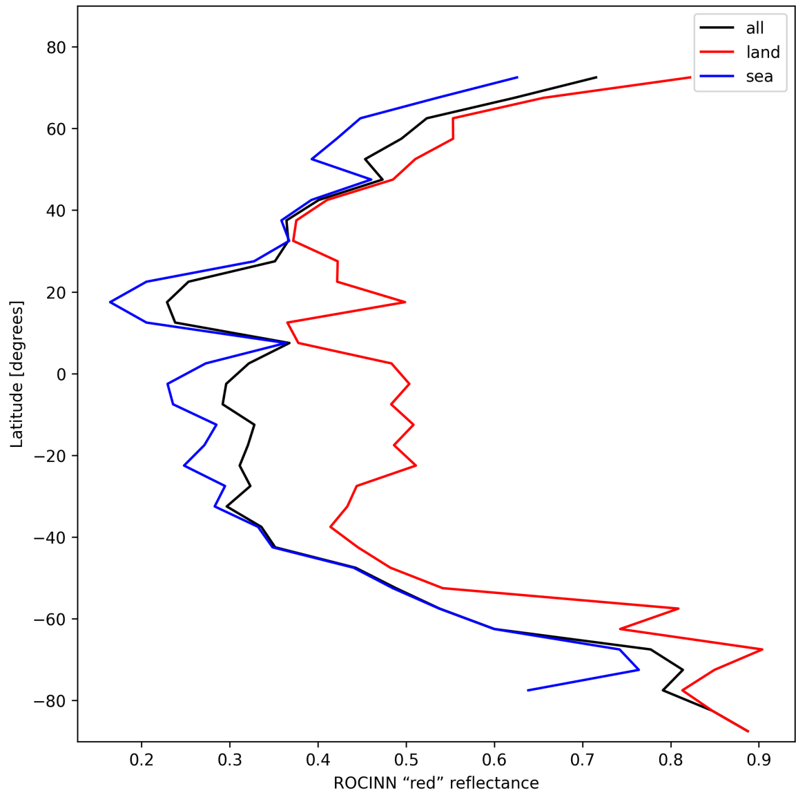
Figure 37: Zonal average of “ROCINN “red” reflectance” for 2025-11-12 to 2025-11-14.
