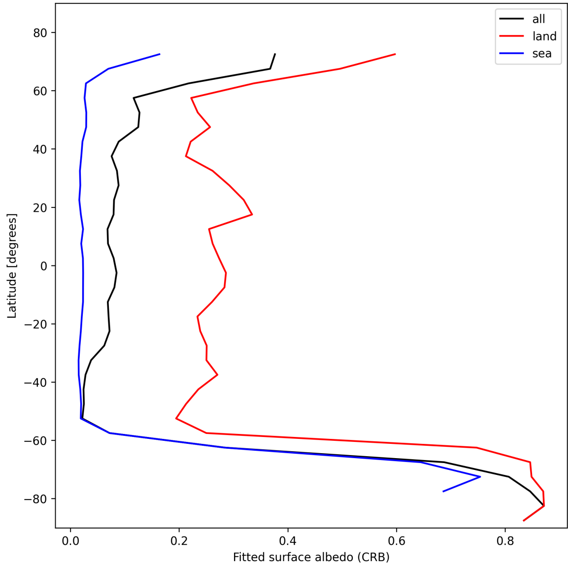
Figure 30: Zonal average of “Fitted surface albedo (CRB)” for 2025-11-12 to 2025-11-14.
