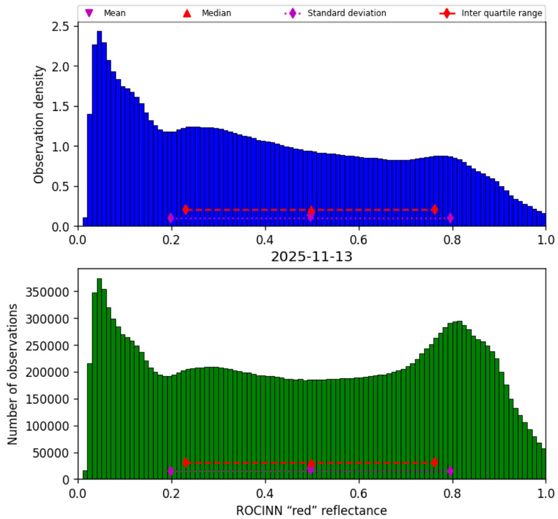
Figure 53: Histogram of “ROCINN “red” reflectance” for 2025-11-12 to 2025-11-14
