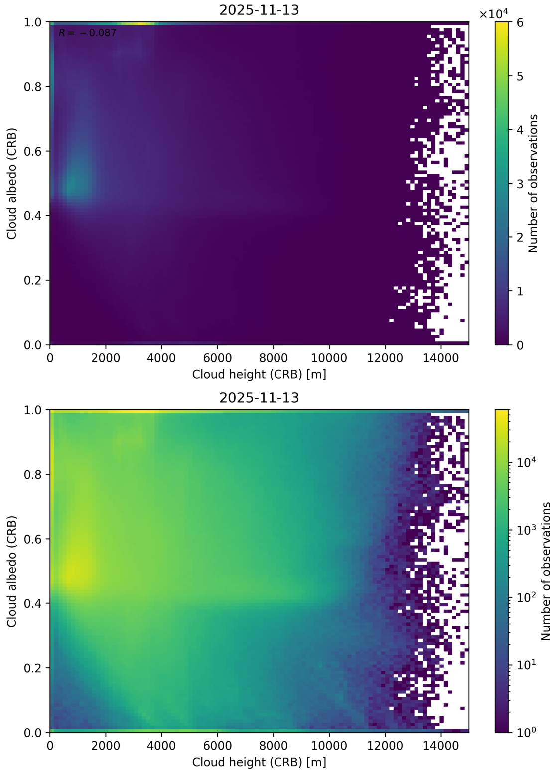
Figure 80: Scatter density plot of “Cloud height (CRB)” against “Cloud albedo (CRB)” for 2025-11-12 to 2025-11-14.
