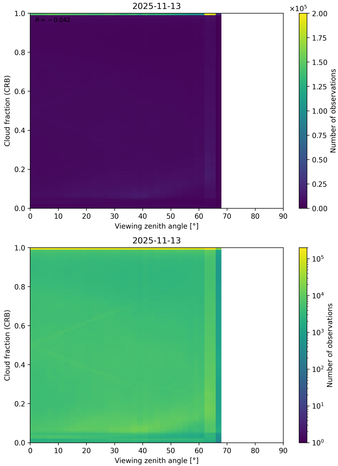
Figure 109: Scatter density plot of “Viewing zenith angle” against “Cloud fraction (CRB)” for 2025-11-12 to 2025-11-14.
