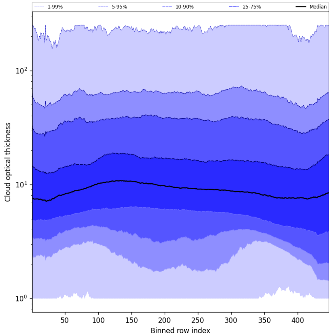
Figure 57: Along track statistics of “Cloud optical thickness” for 2025-11-12 to 2025-11-14
