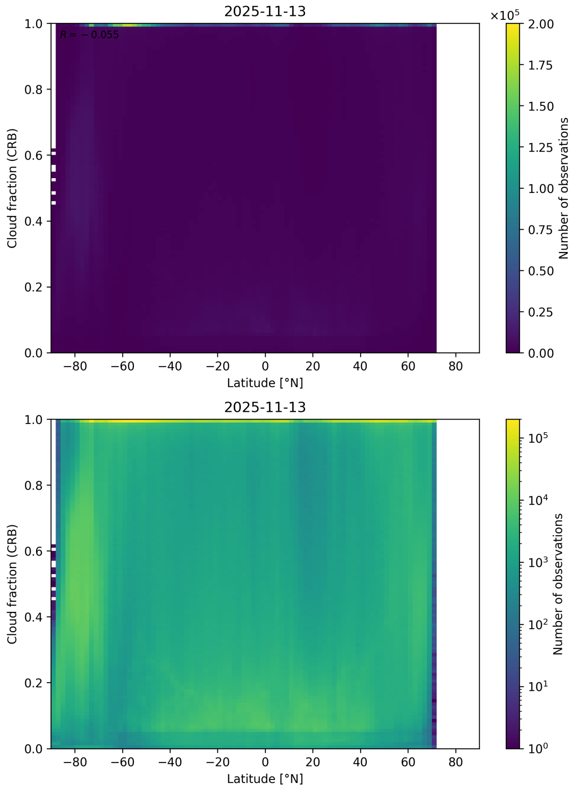
Figure 94: Scatter density plot of “Latitude” against “Cloud fraction (CRB)” for 2025-11-12 to 2025-11-14.
