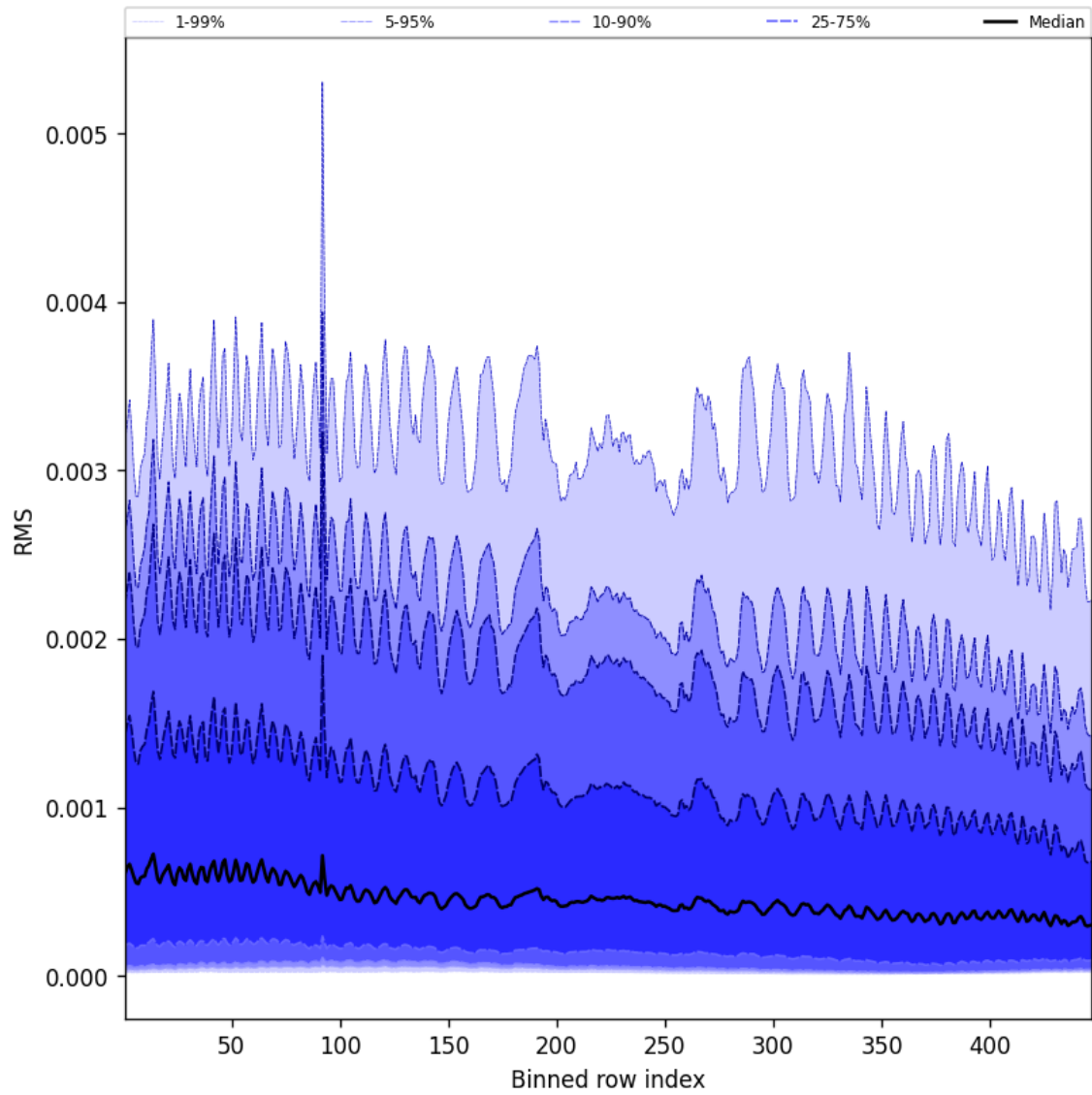
Figure 63: Along track statistics of “RMS” for 2025-11-12 to 2025-11-14
