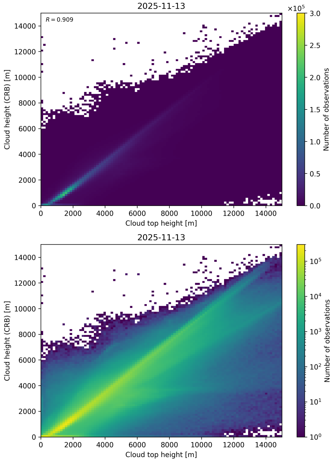
Figure 89: Scatter density plot of “Cloud top height” against “Cloud height (CRB)” for 2025-11-12 to 2025-11-14.
