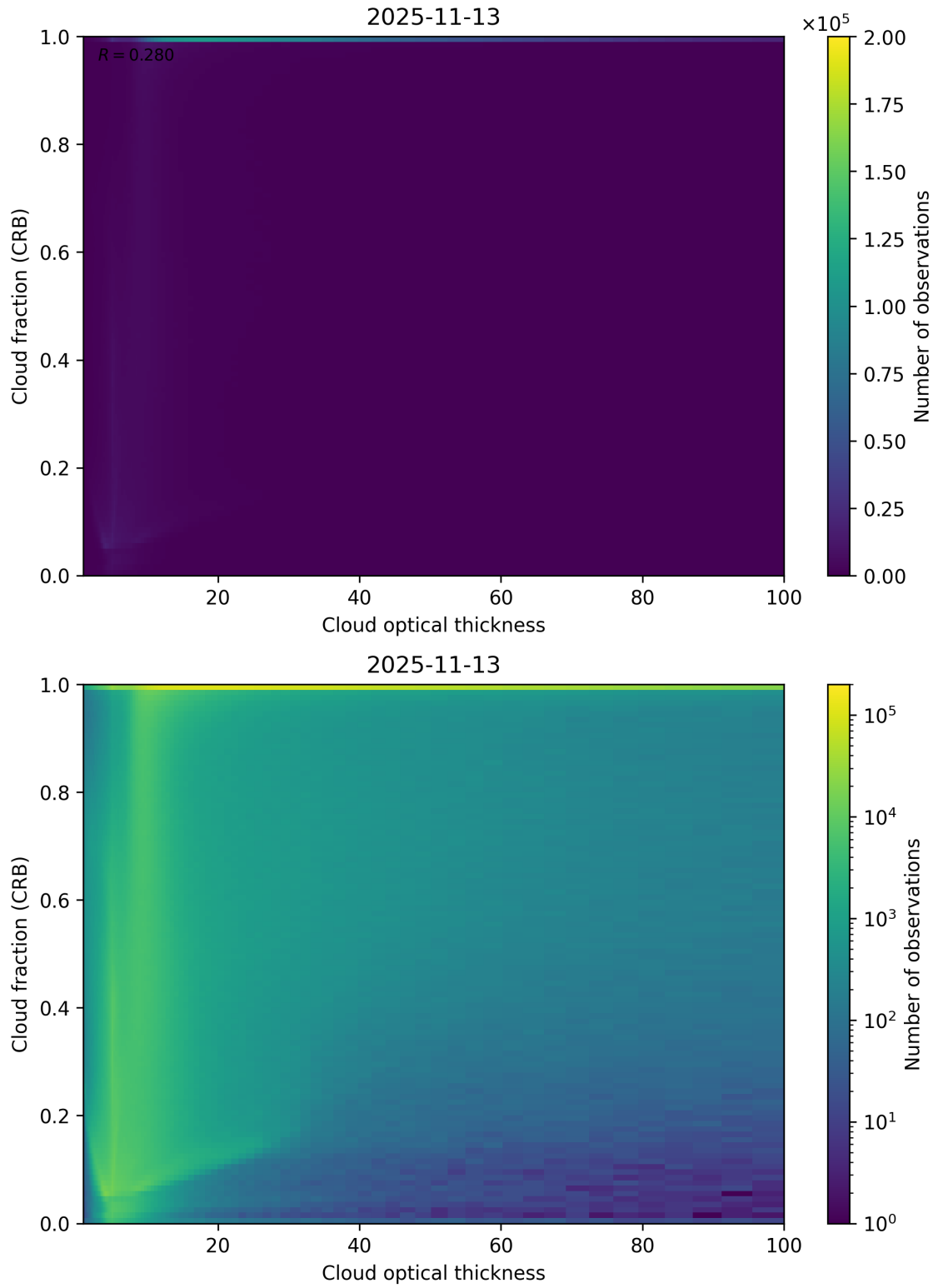
Figure 84: Scatter density plot of “Cloud optical thickness” against “Cloud fraction (CRB)” for 2025-11-12 to 2025-11-14.
