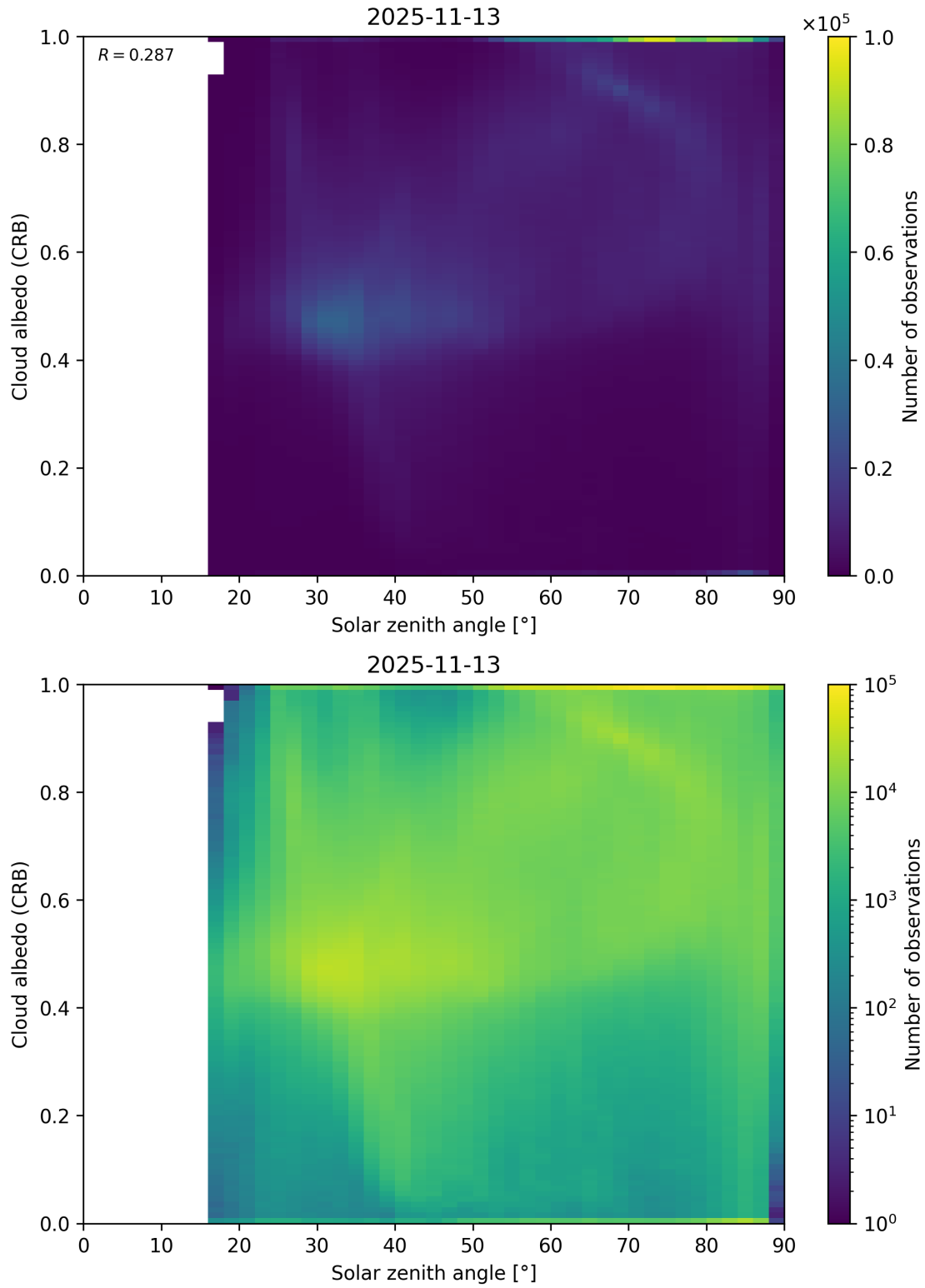
Figure 98: Scatter density plot of “Solar zenith angle” against “Cloud albedo (CRB)” for 2025-11-12 to 2025-11-14.
