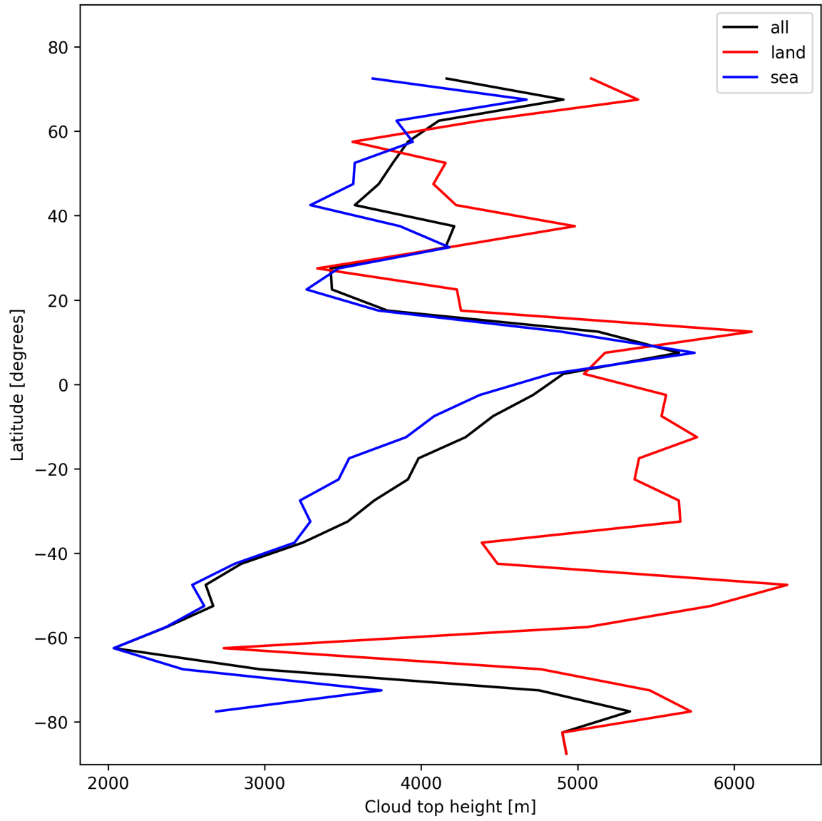
Figure 24: Zonal average of “Cloud top height” for 2025-11-12 to 2025-11-14.
