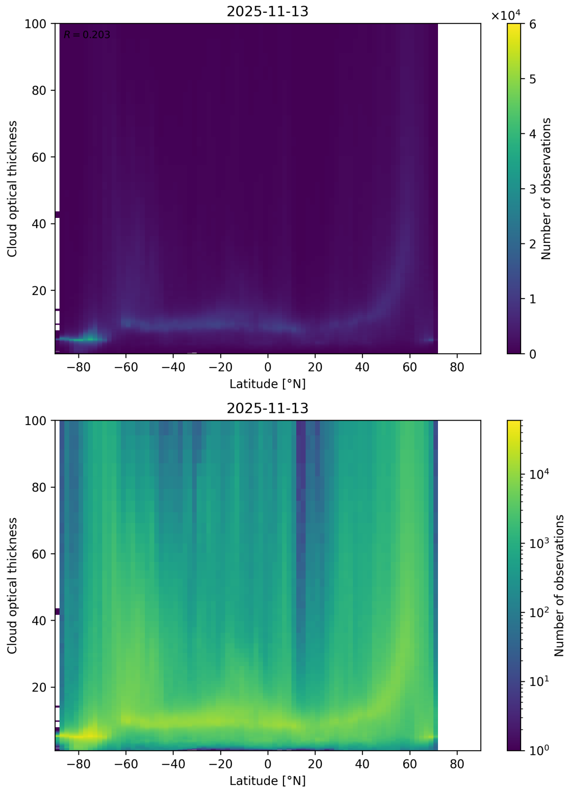
Figure 96: Scatter density plot of “Latitude” against “Cloud optical thickness” for 2025-11-12 to 2025-11-14.
