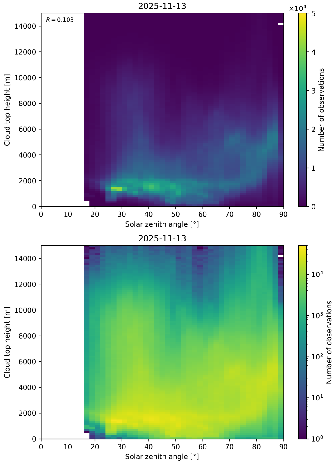
Figure 104: Scatter density plot of “Solar zenith angle” against “Cloud top height” for 2025-11-12 to 2025-11-14.
