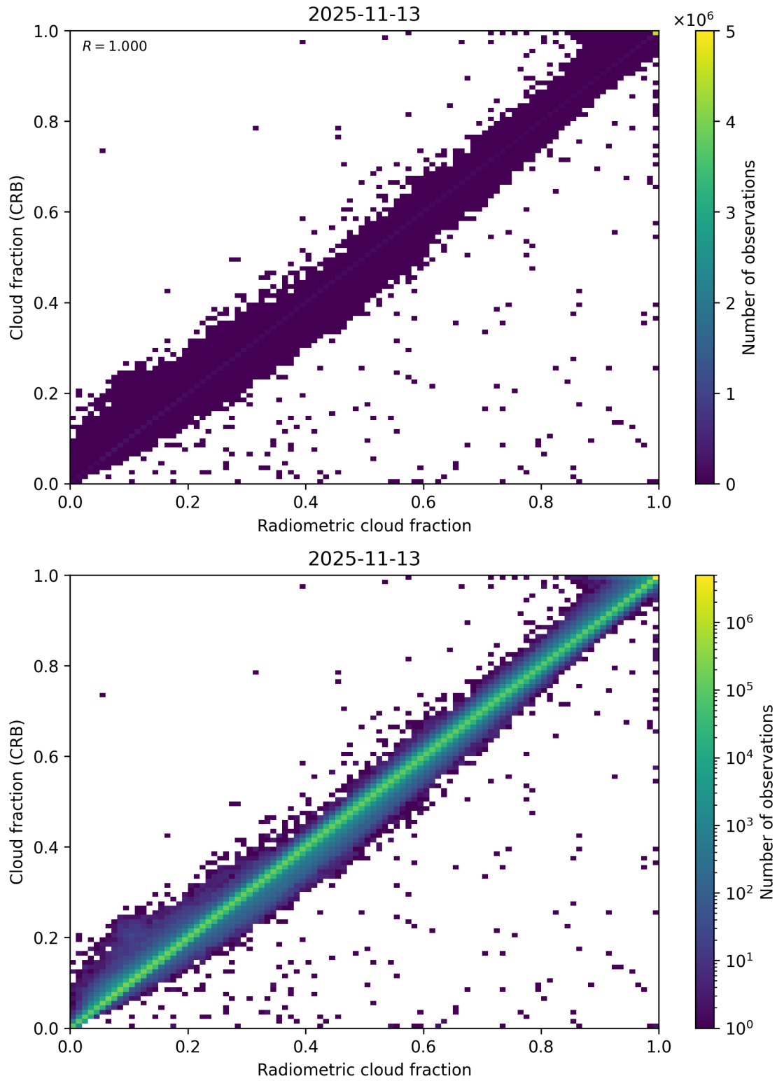
Figure 73: Scatter density plot of “Radiometric cloud fraction” against “Cloud fraction (CRB)” for 2025-11-12 to 2025-11-14.
