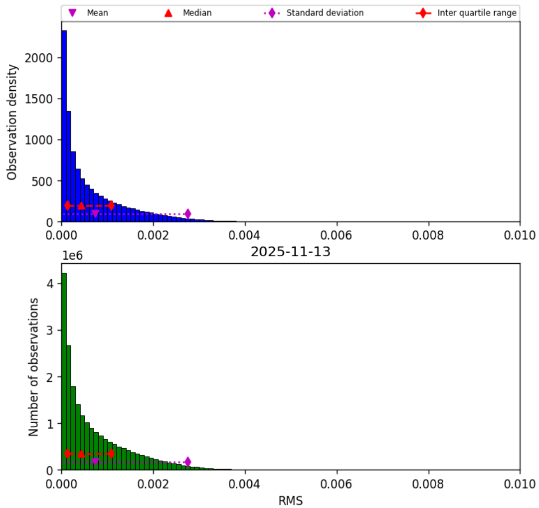
Figure 47: Histogram of “RMS” for 2025-11-12 to 2025-11-14
