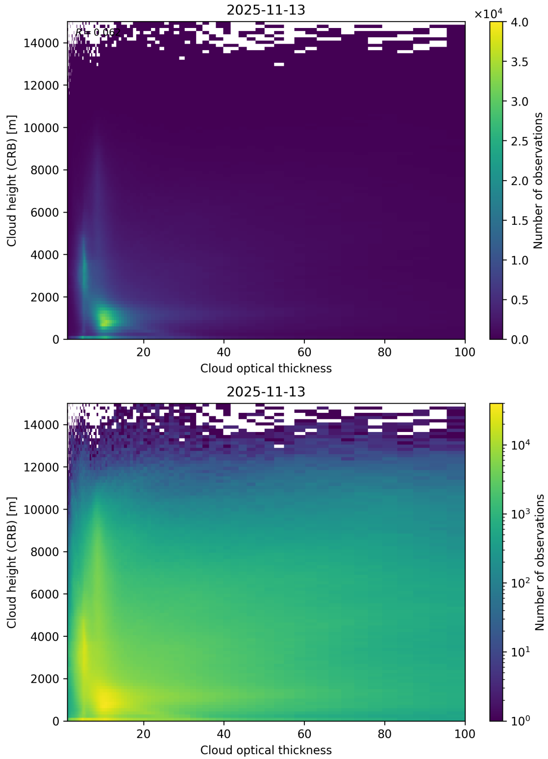
Figure 85: Scatter density plot of “Cloud optical thickness” against “Cloud height (CRB)” for 2025-11-12 to 2025-11-14.
