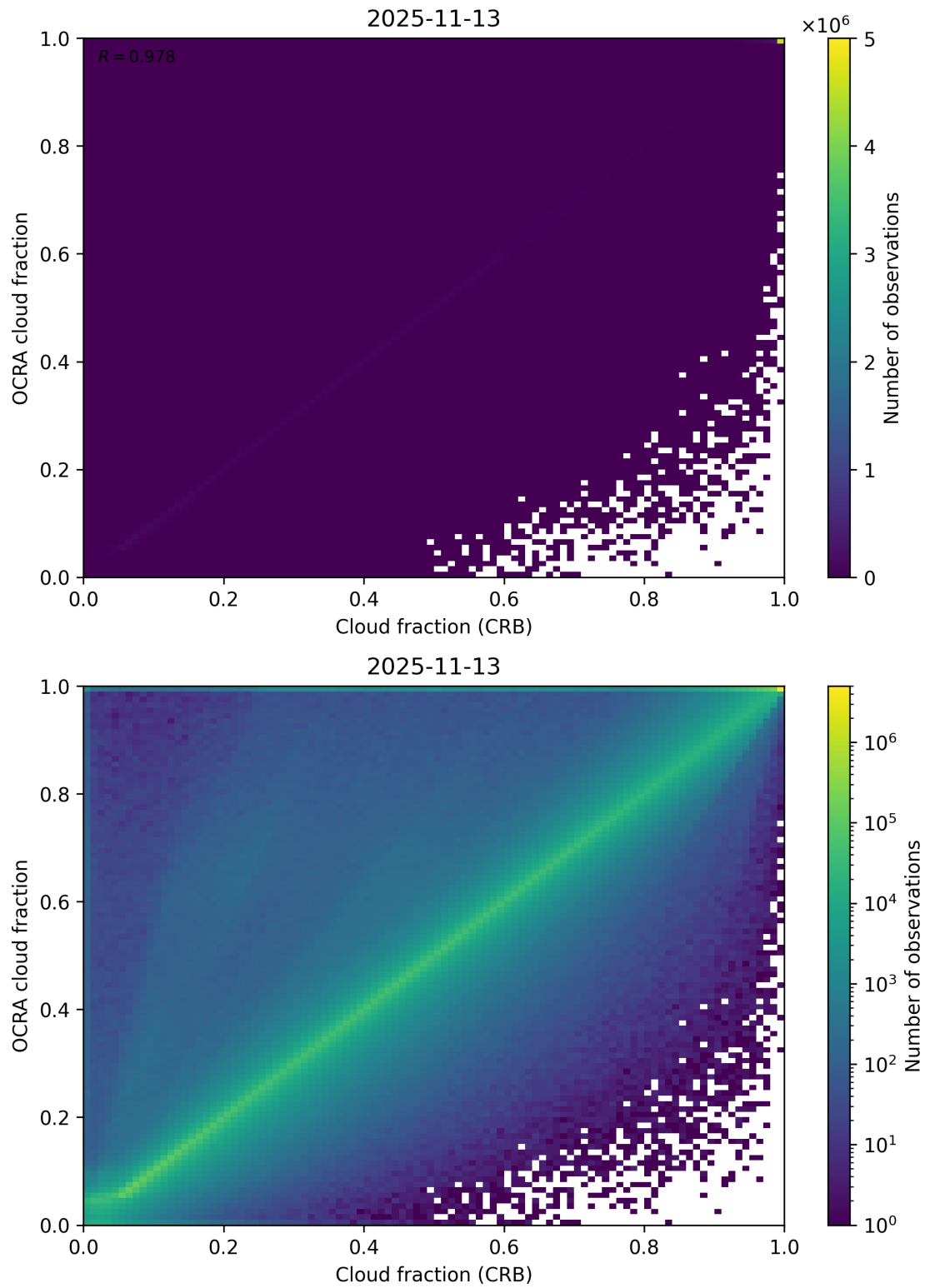
Figure 78: Scatter density plot of “Cloud fraction (CRB)” against “OCRA cloud fraction” for 2025-11-12 to 2025-11-14.
