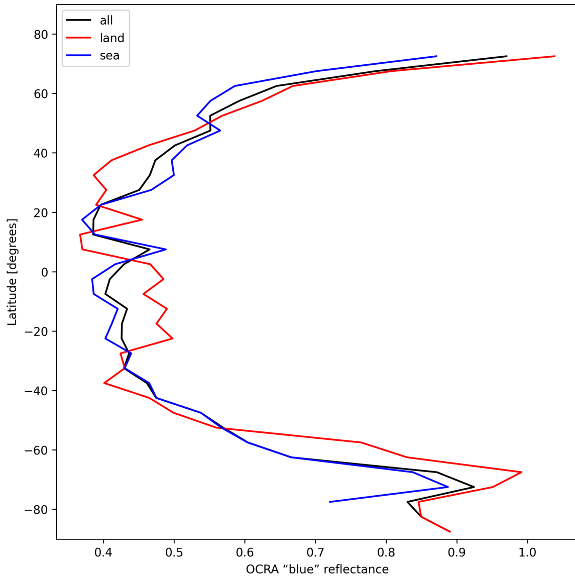
Figure 35: Zonal average of “OCRA “blue” reflectance” for 2025-11-12 to 2025-11-14.
