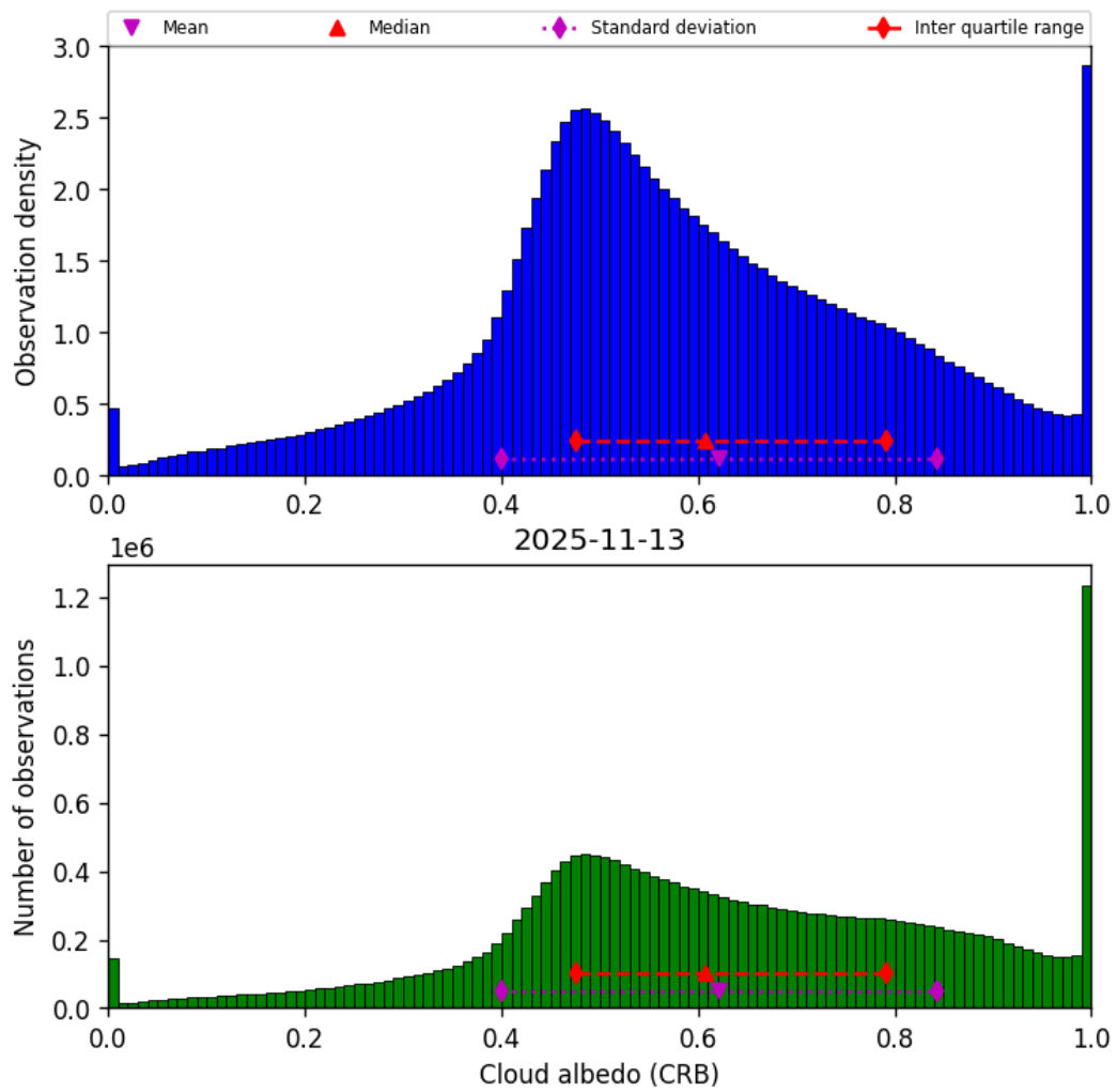
Figure 44: Histogram of “Cloud albedo (CRB)” for 2025-11-12 to 2025-11-14
