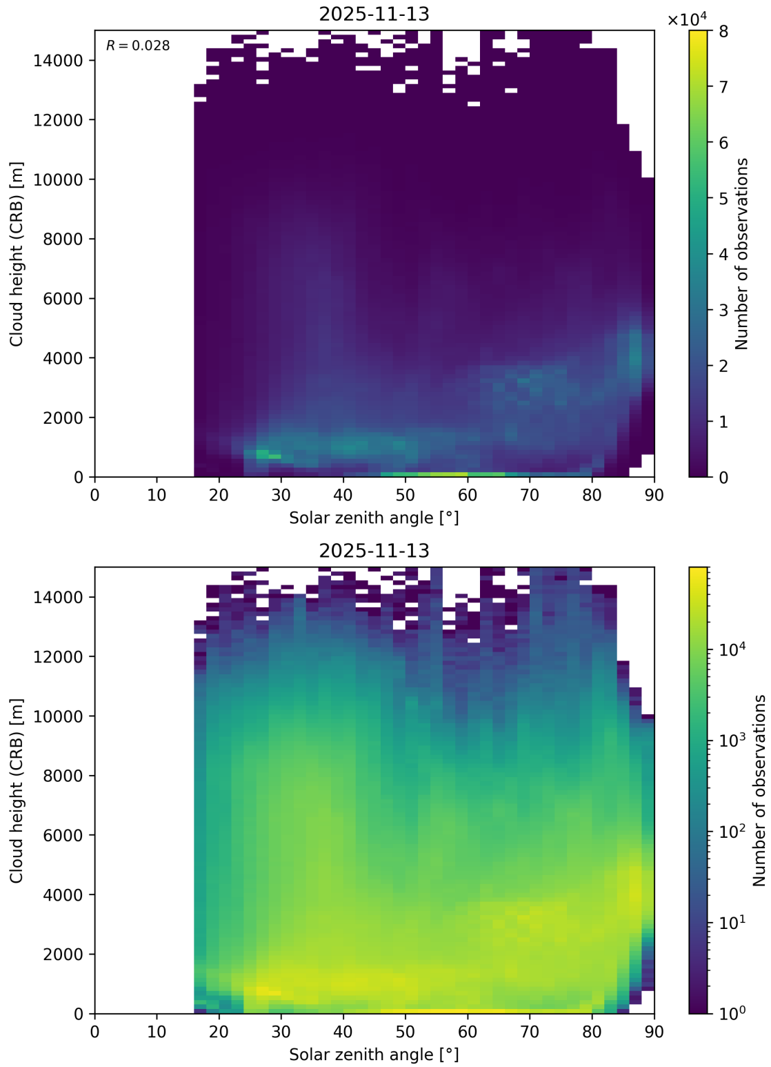
Figure 102: Scatter density plot of “Solar zenith angle” against “Cloud height (CRB)” for 2025-11-12 to 2025-11-14.
