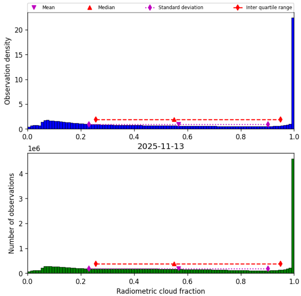
Figure 39: Histogram of “Radiometric cloud fraction” for 2025-11-12 to 2025-11-14
