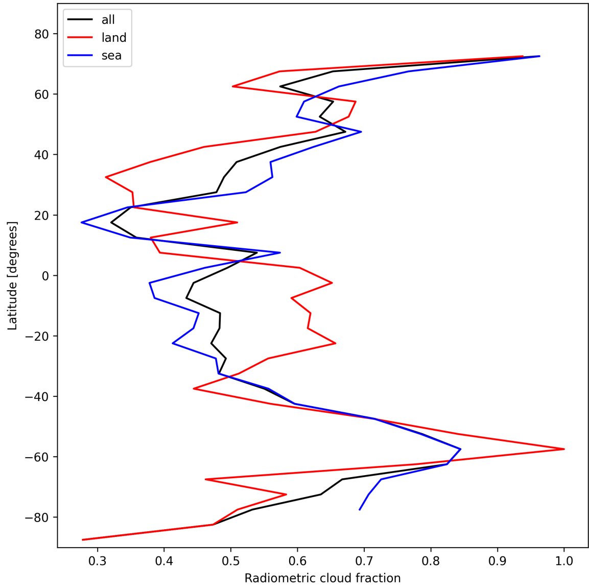
Figure 23: Zonal average of “Radiometric cloud fraction” for 2025-11-12 to 2025-11-14.
