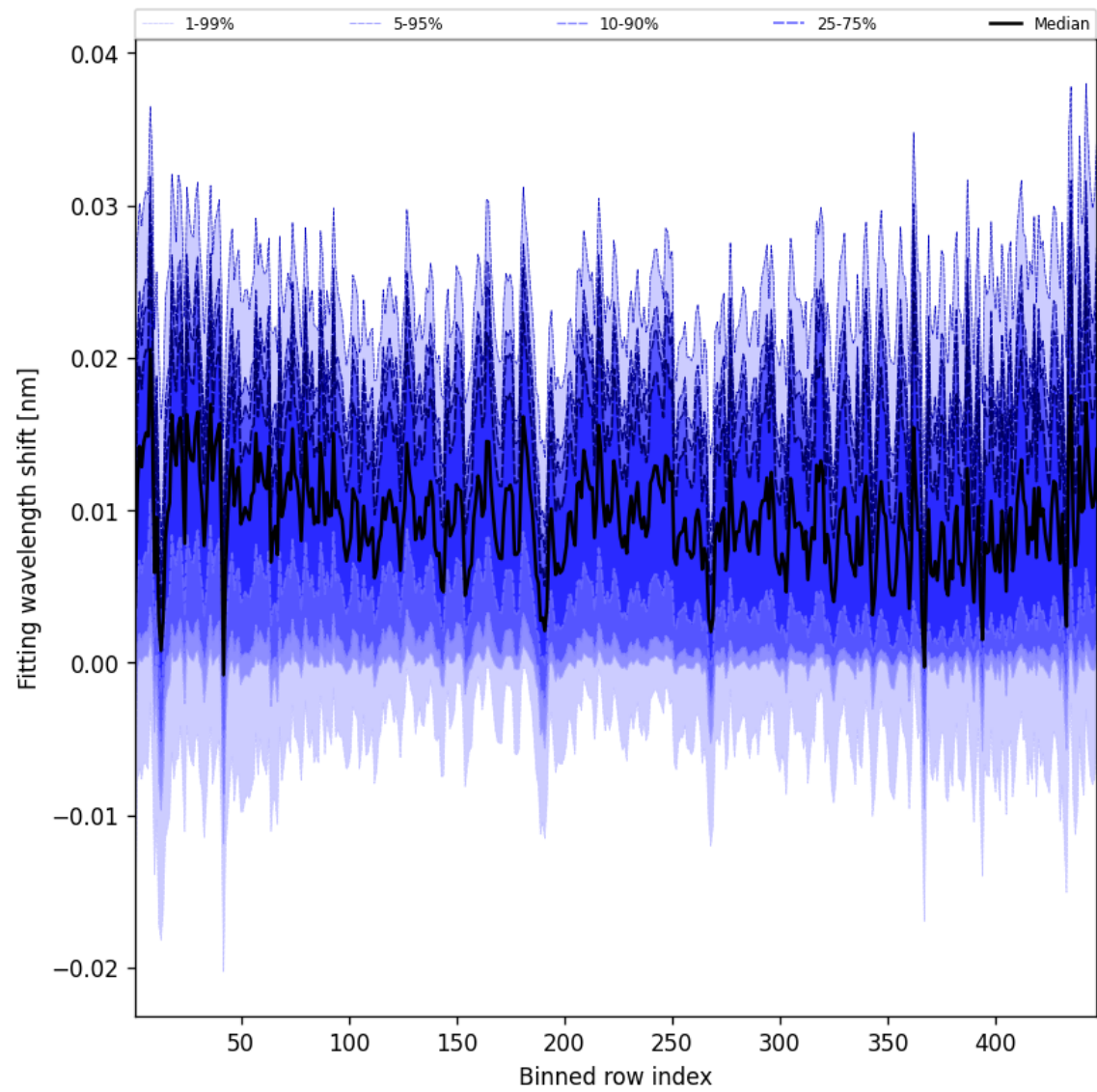
Figure 65: Along track statistics of “Fitting wavelength shift” for 2025-11-12 to 2025-11-14
