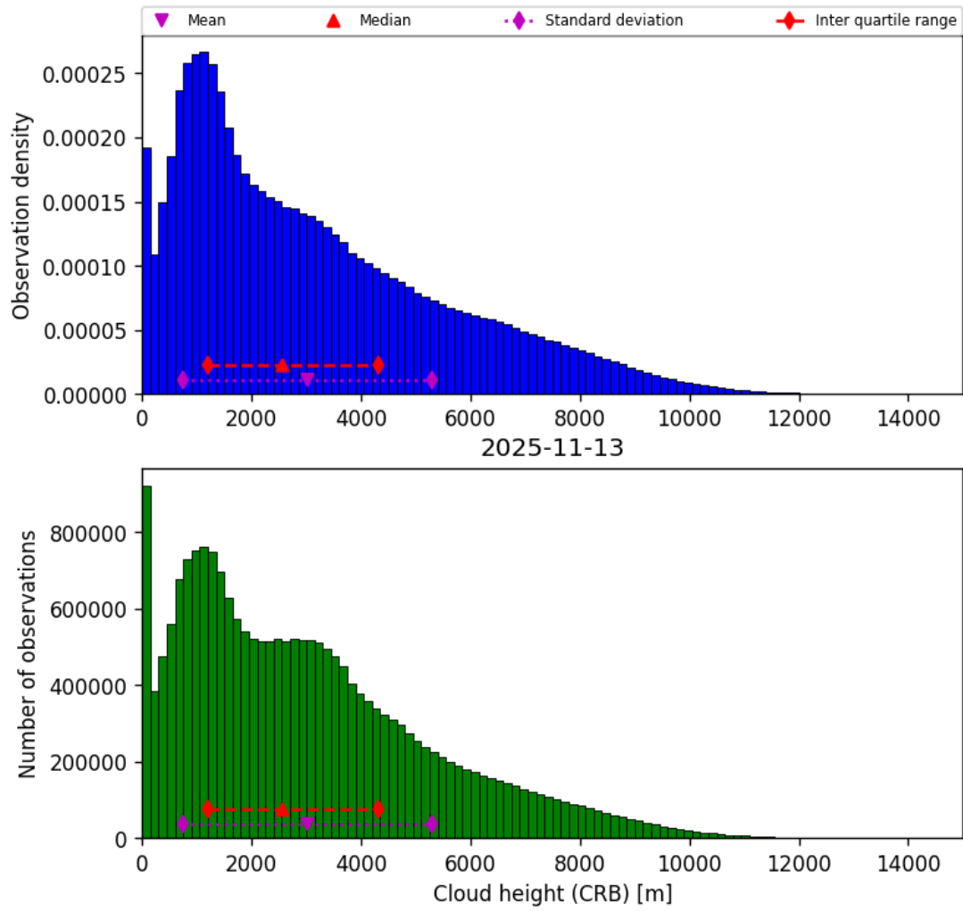
Figure 43: Histogram of “Cloud height (CRB)” for 2025-11-12 to 2025-11-14
