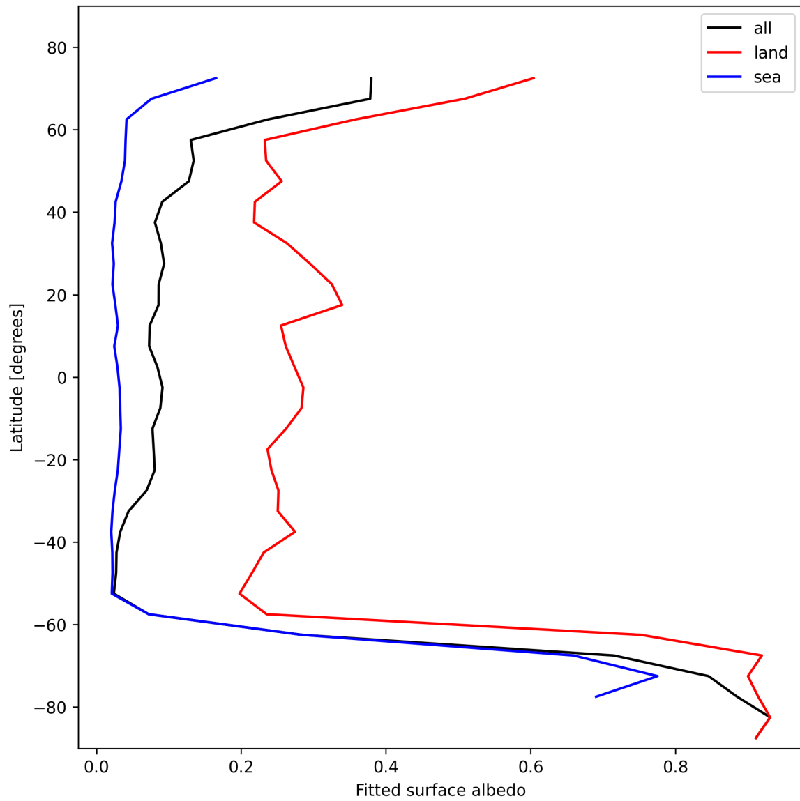
Figure 29: Zonal average of “Fitted surface albedo” for 2025-11-12 to 2025-11-14.
