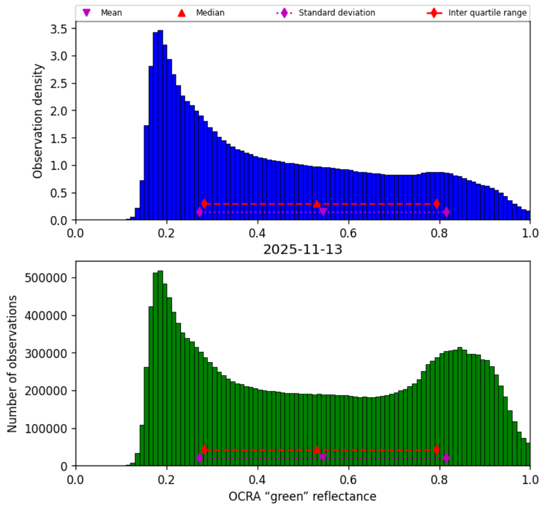
Figure 52: Histogram of “OCRA “green” reflectance” for 2025-11-12 to 2025-11-14
