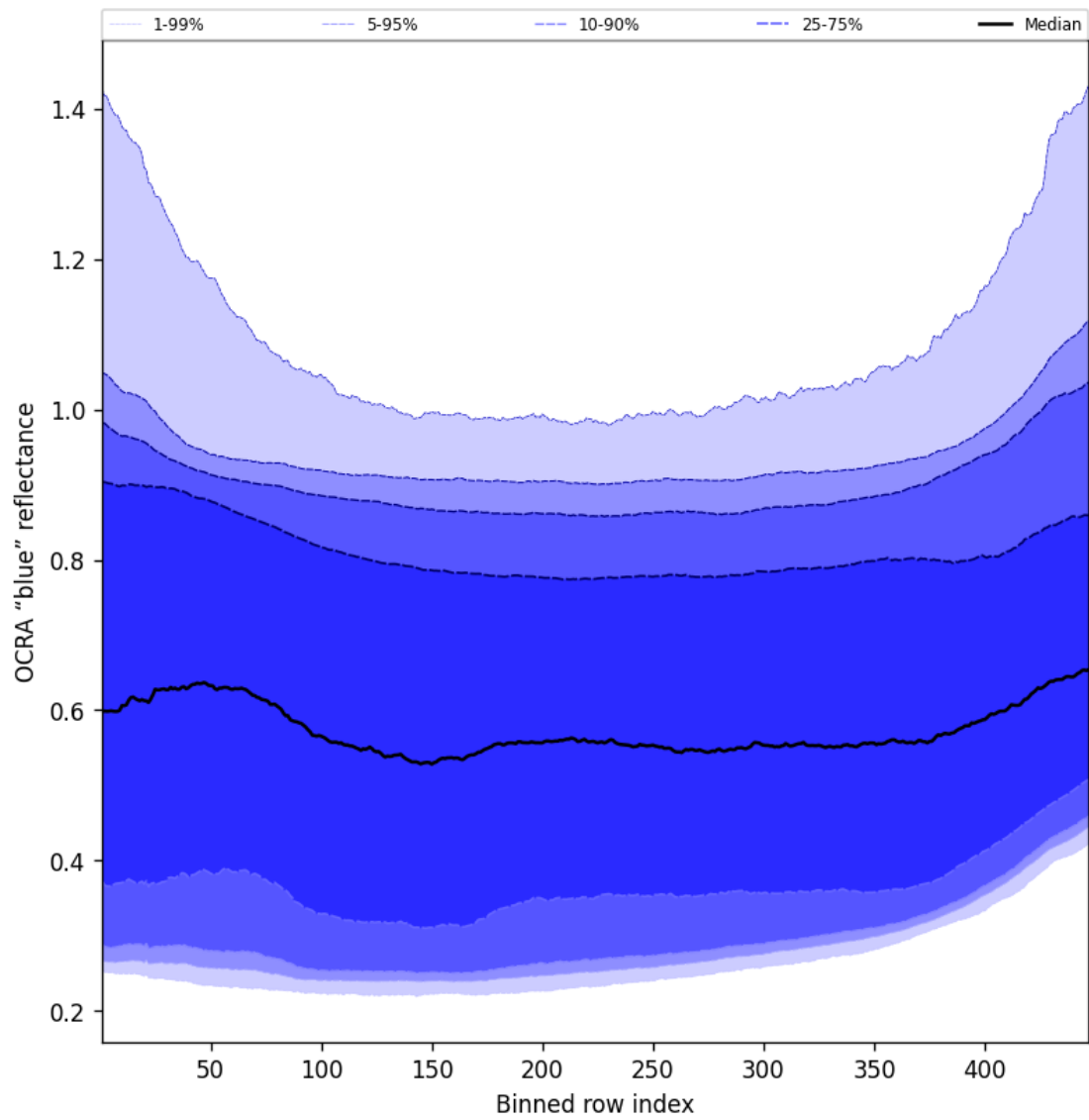
Figure 67: Along track statistics of “OCRA “blue” reflectance” for 2025-11-12 to 2025-11-14
