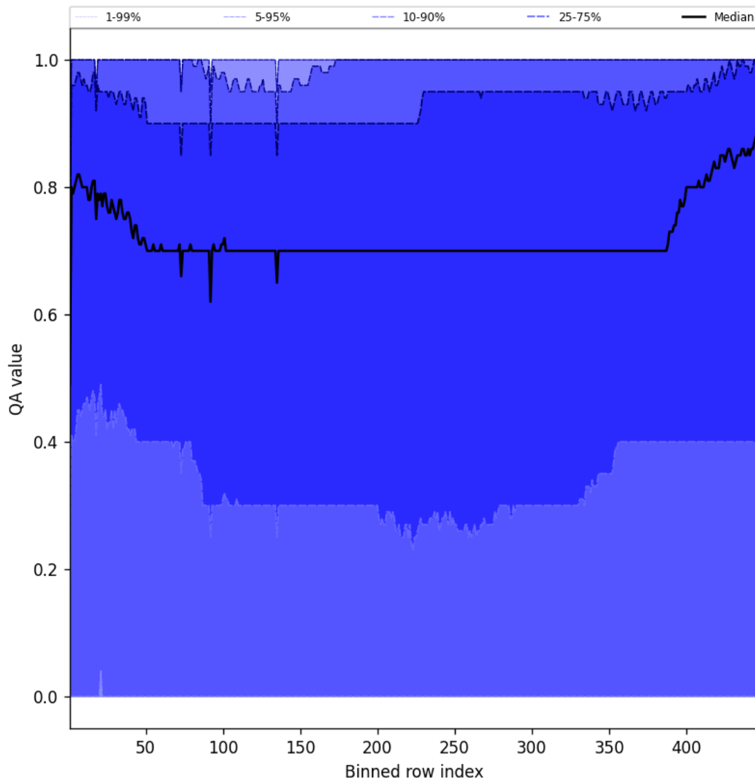
Figure 54: Along track statistics of “QA value” for 2025-11-12 to 2025-11-14
