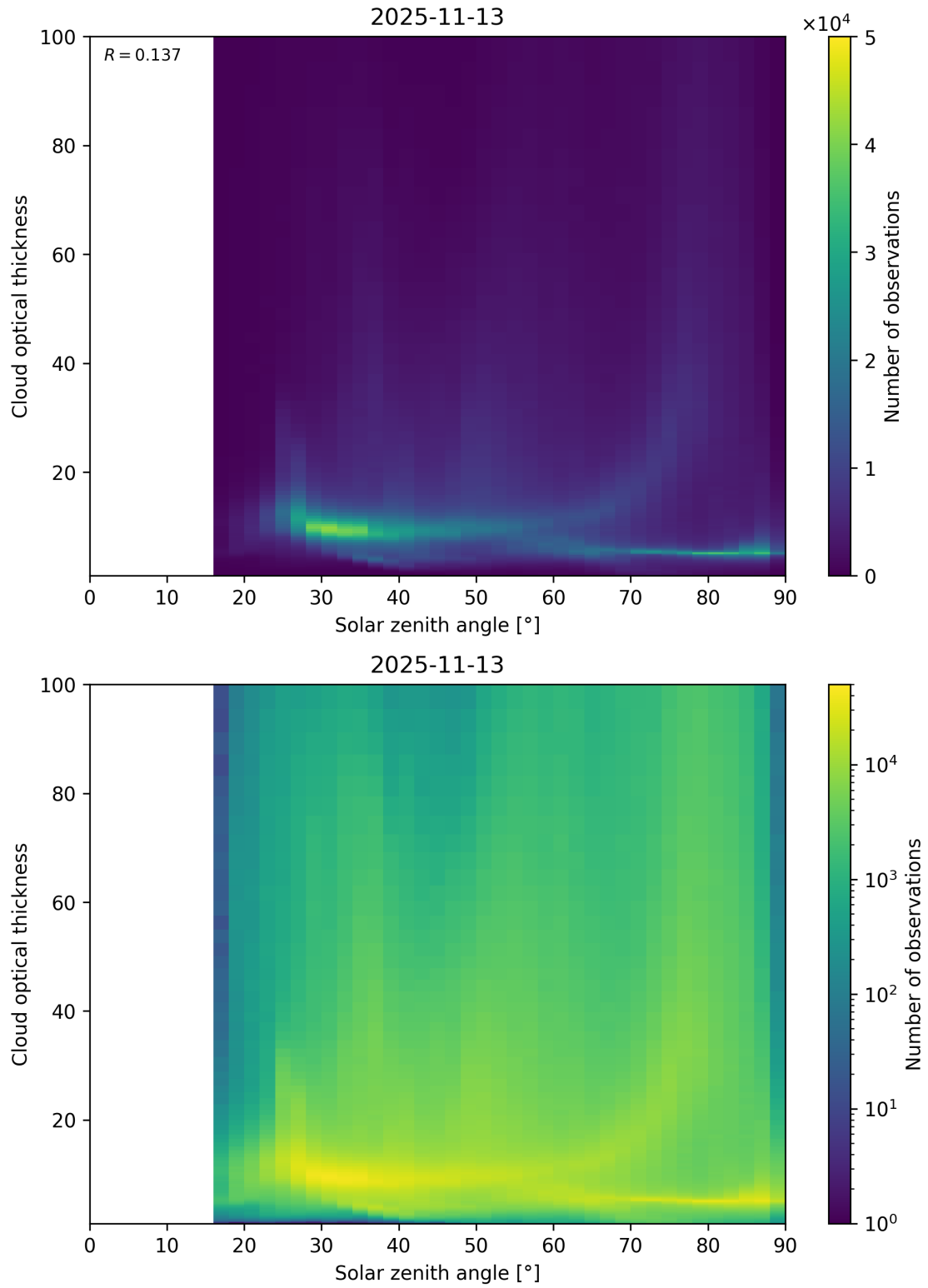
Figure 103: Scatter density plot of “Solar zenith angle” against “Cloud optical thickness” for 2025-11-12 to 2025-11-14.
