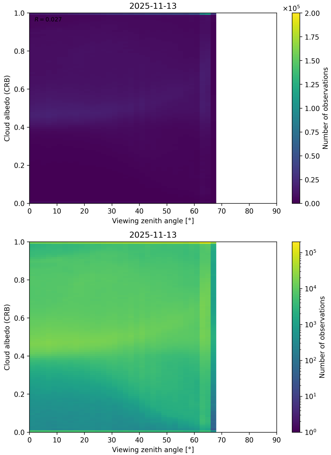
Figure 106: Scatter density plot of “Viewing zenith angle” against “Cloud albedo (CRB)” for 2025-11-12 to 2025-11-14.
