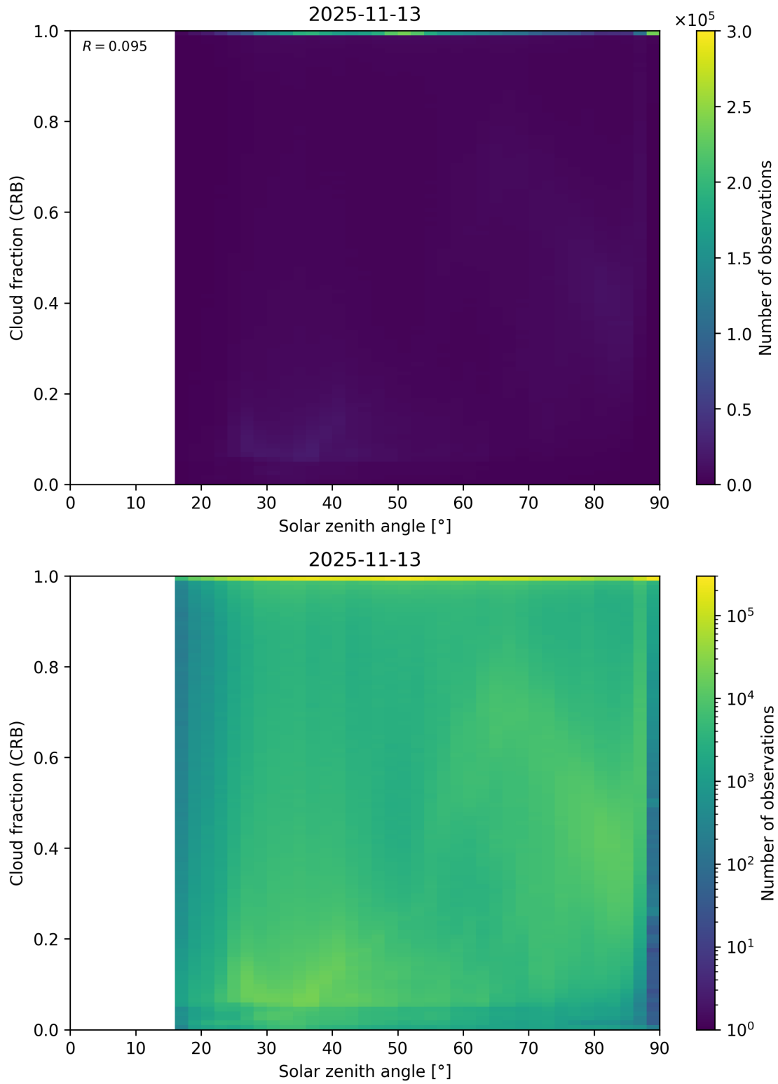
Figure 101: Scatter density plot of “Solar zenith angle” against “Cloud fraction (CRB)” for 2025-11-12 to 2025-11-14.
