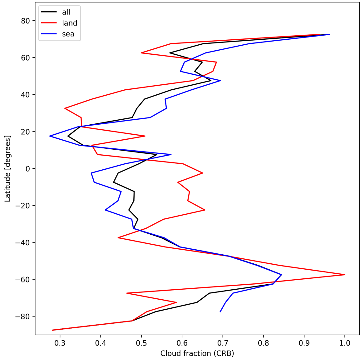
Figure 26: Zonal average of “Cloud fraction (CRB)” for 2025-11-12 to 2025-11-14.
