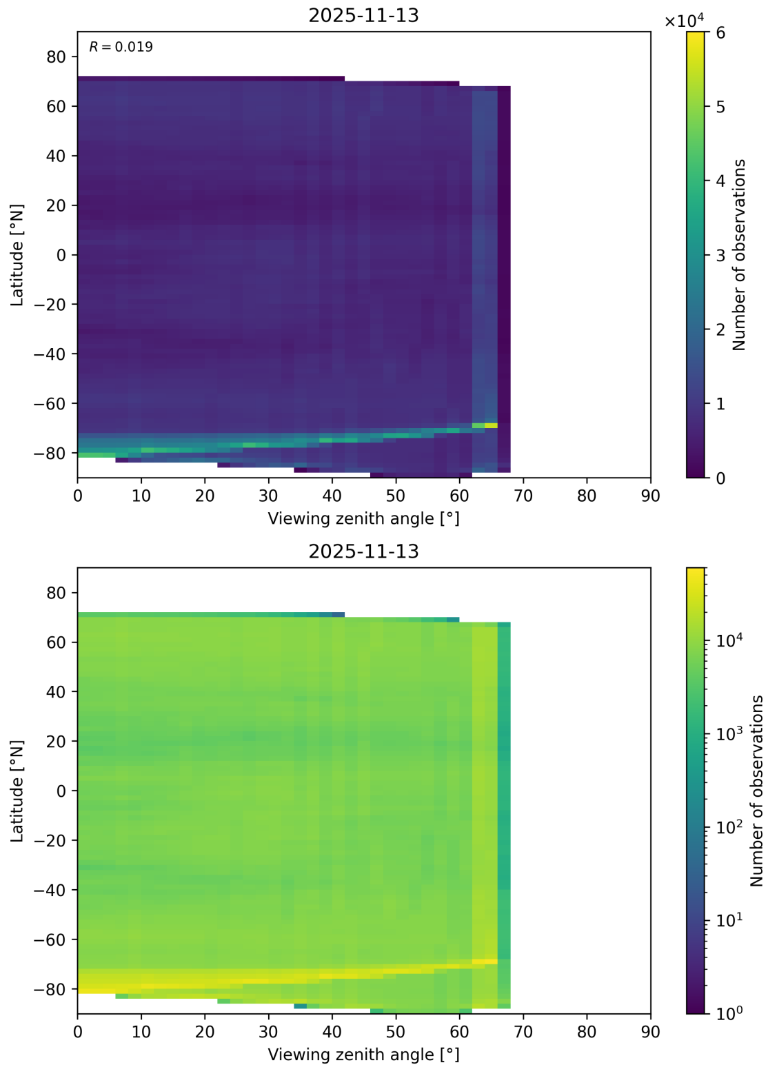
Figure 113: Scatter density plot of “Viewing zenith angle” against “Latitude” for 2025-11-12 to 2025-11-14.
