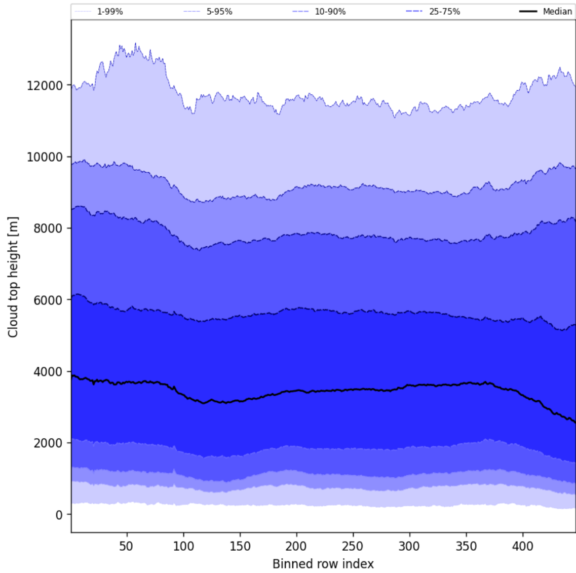
Figure 56: Along track statistics of “Cloud top height” for 2025-11-12 to 2025-11-14
