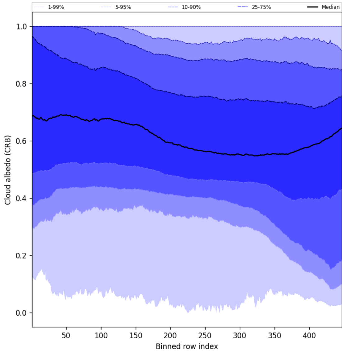
Figure 60: Along track statistics of “Cloud albedo (CRB)” for 2025-11-12 to 2025-11-14
