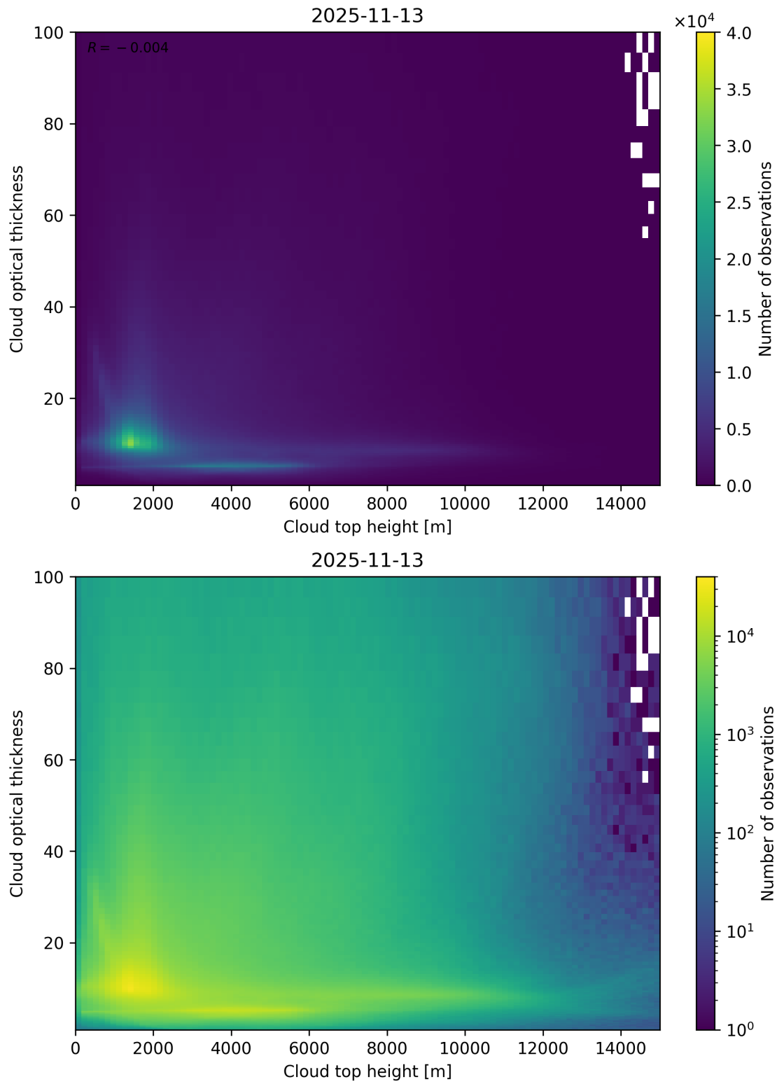
Figure 90: Scatter density plot of “Cloud top height” against “Cloud optical thickness” for 2025-11-12 to 2025-11-14.
