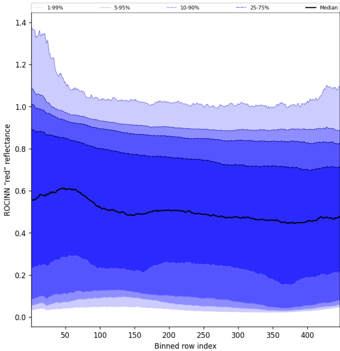
Figure 69: Along track statistics of “ROCINN “red” reflectance” for 2025-11-12 to 2025-11-14
