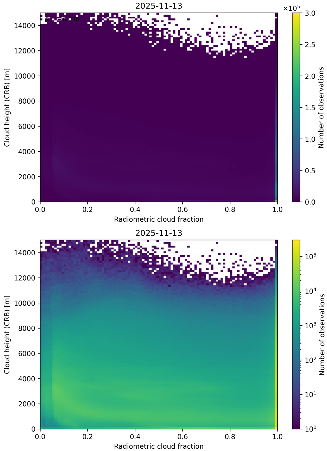
Figure 74: Scatter density plot of “Radiometric cloud fraction” against “Cloud height (CRB)” for 2025-11-12 to 2025-11-14.
