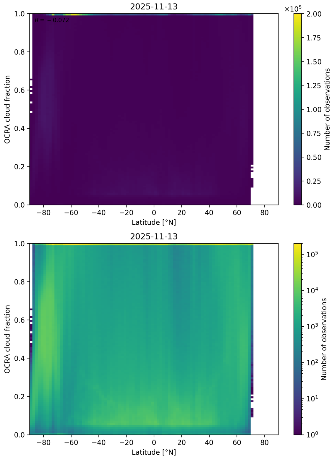
Figure 93: Scatter density plot of “Latitude” against “OCRA cloud fraction” for 2025-11-12 to 2025-11-14.
