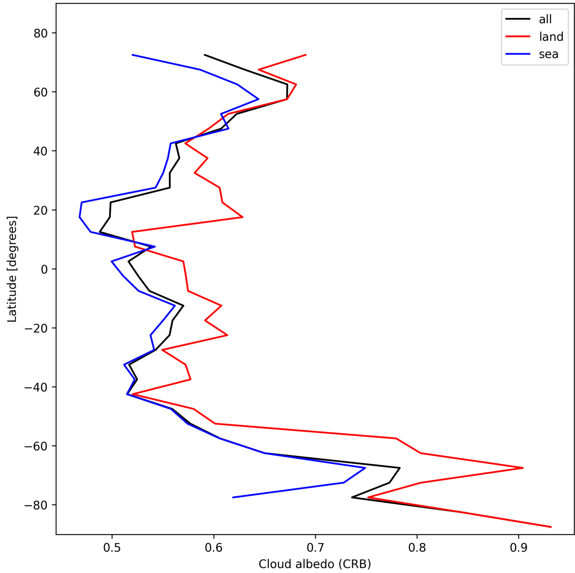
Figure 28: Zonal average of “Cloud albedo (CRB)” for 2025-11-12 to 2025-11-14.
