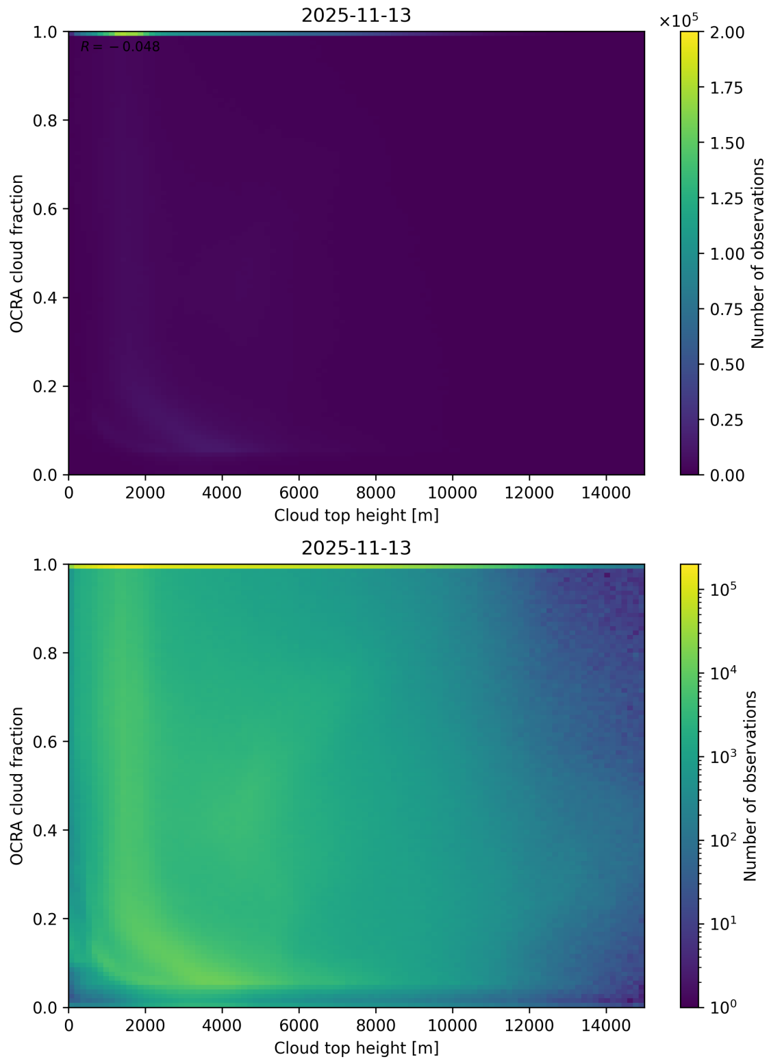
Figure 87: Scatter density plot of “Cloud top height” against “OCRA cloud fraction” for 2025-11-12 to 2025-11-14.
