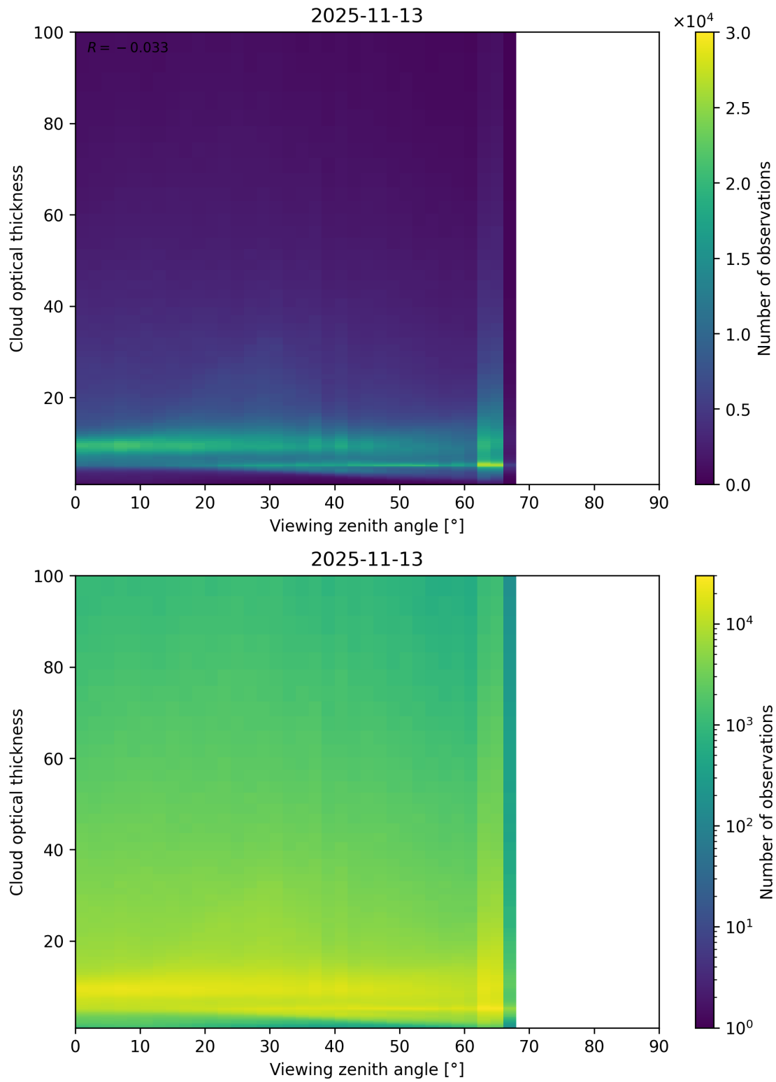
Figure 111: Scatter density plot of “Viewing zenith angle” against “Cloud optical thickness” for 2025-11-12 to 2025-11-14.
