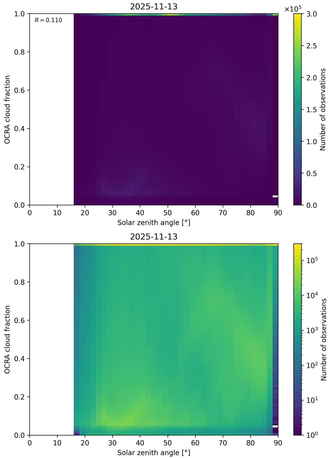
Figure 100: Scatter density plot of “Solar zenith angle” against “OCRA cloud fraction” for 2025-11-12 to 2025-11-14.
