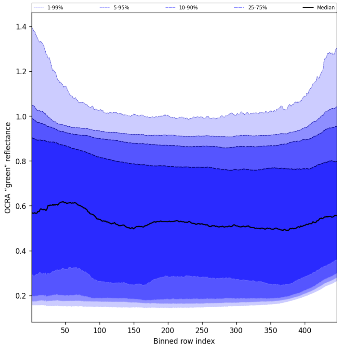
Figure 68: Along track statistics of “OCRA “green” reflectance” for 2025-11-12 to 2025-11-14
