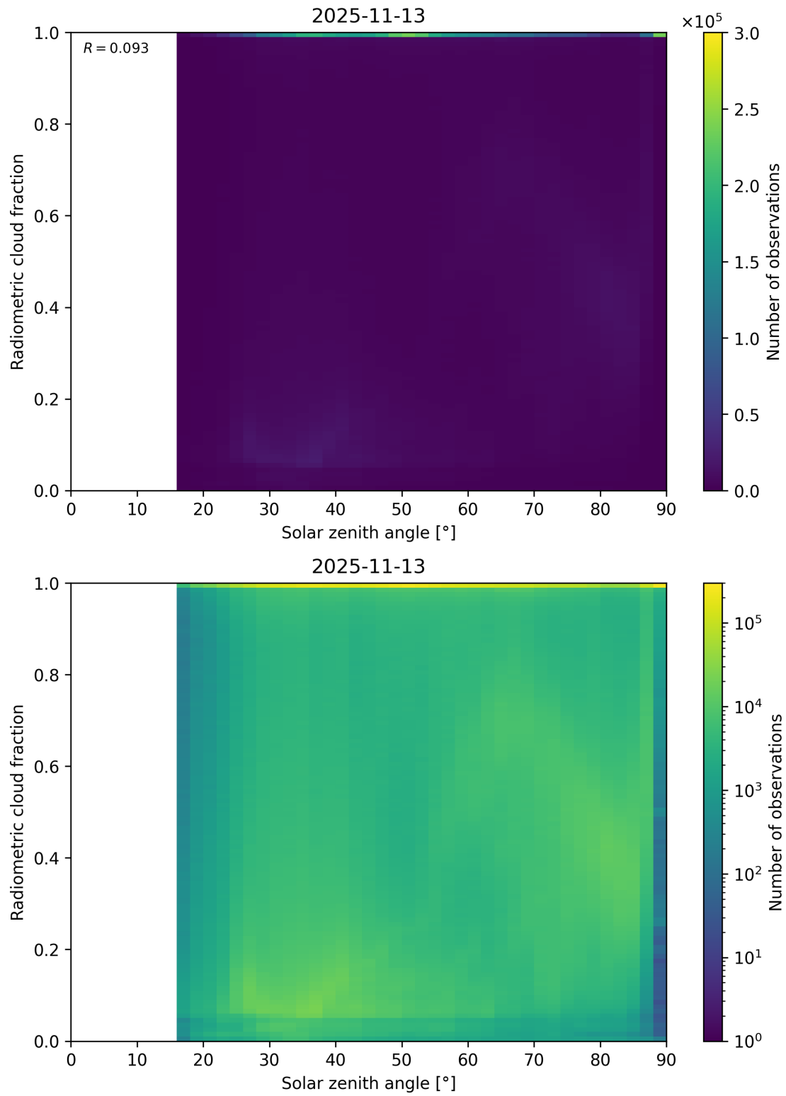
Figure 99: Scatter density plot of “Solar zenith angle” against “Radiometric cloud fraction” for 2025-11-12 to 2025-11-14.
