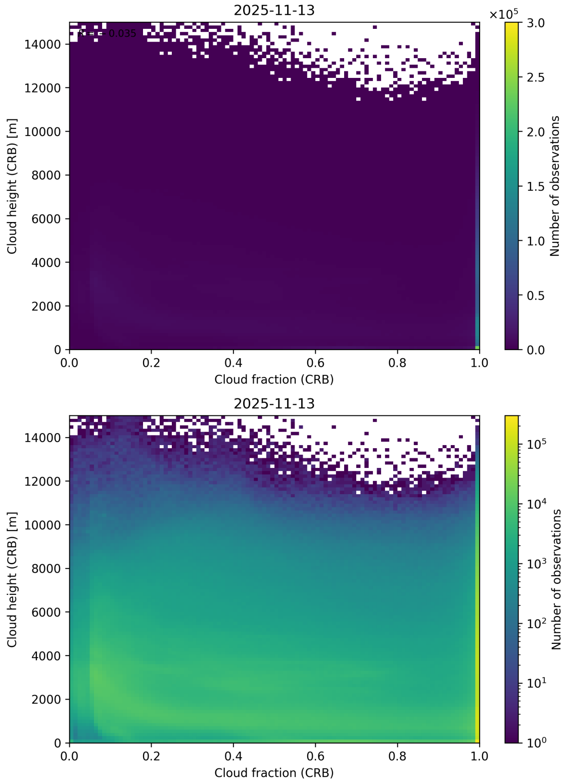
Figure 79: Scatter density plot of “Cloud fraction (CRB)” against “Cloud height (CRB)” for 2025-11-12 to 2025-11-14.
