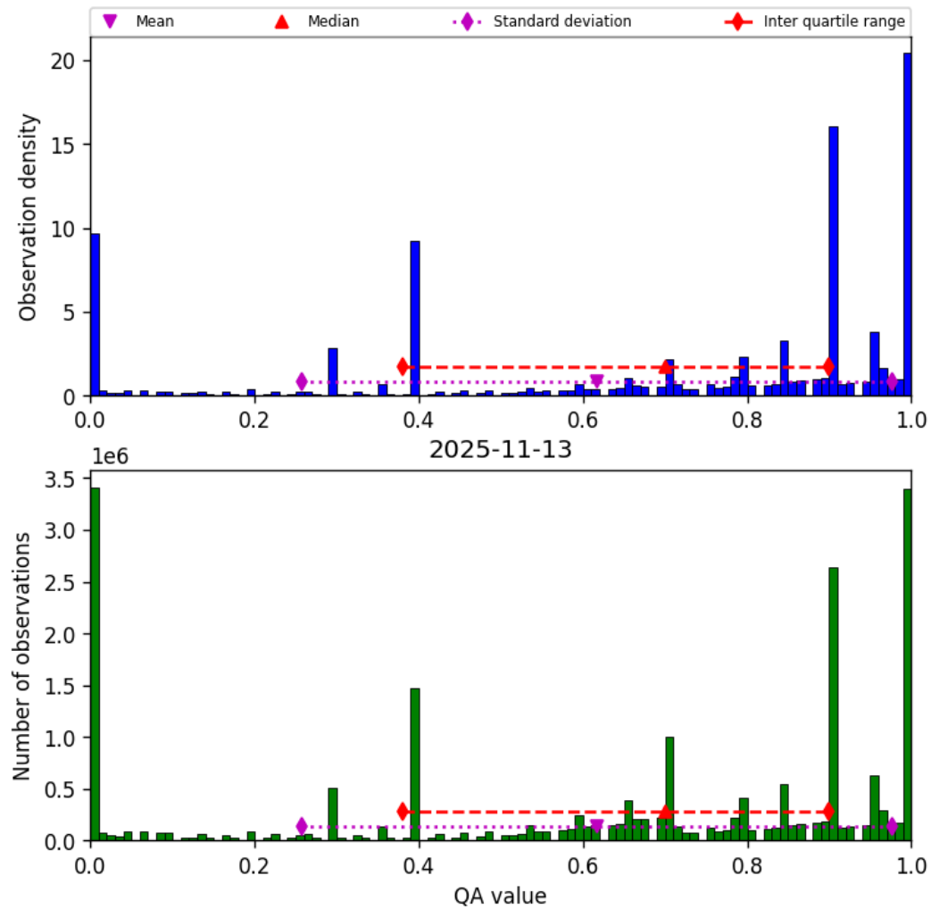
Figure 38: Histogram of “QA value” for 2025-11-12 to 2025-11-14
