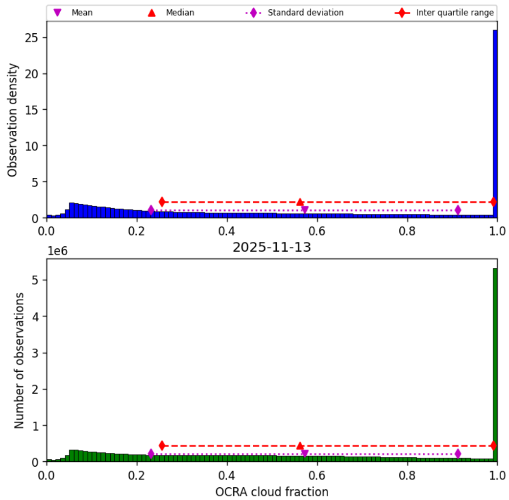
Figure 50: Histogram of “OCRA cloud fraction” for 2025-11-12 to 2025-11-14
