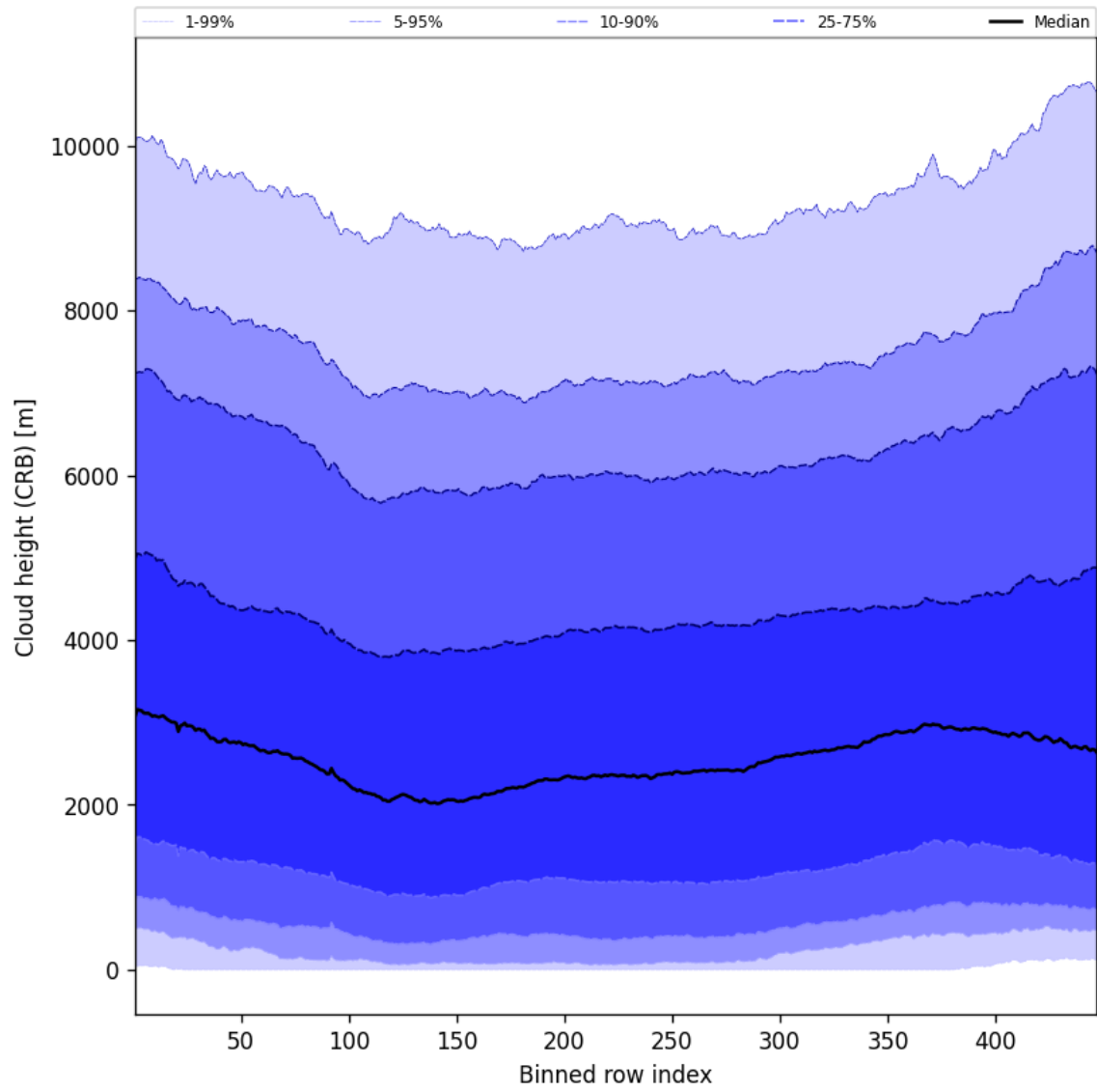
Figure 59: Along track statistics of “Cloud height (CRB)” for 2025-11-12 to 2025-11-14
