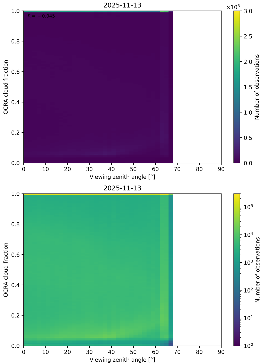
Figure 108: Scatter density plot of “Viewing zenith angle” against “OCRA cloud fraction” for 2025-11-12 to 2025-11-14.
