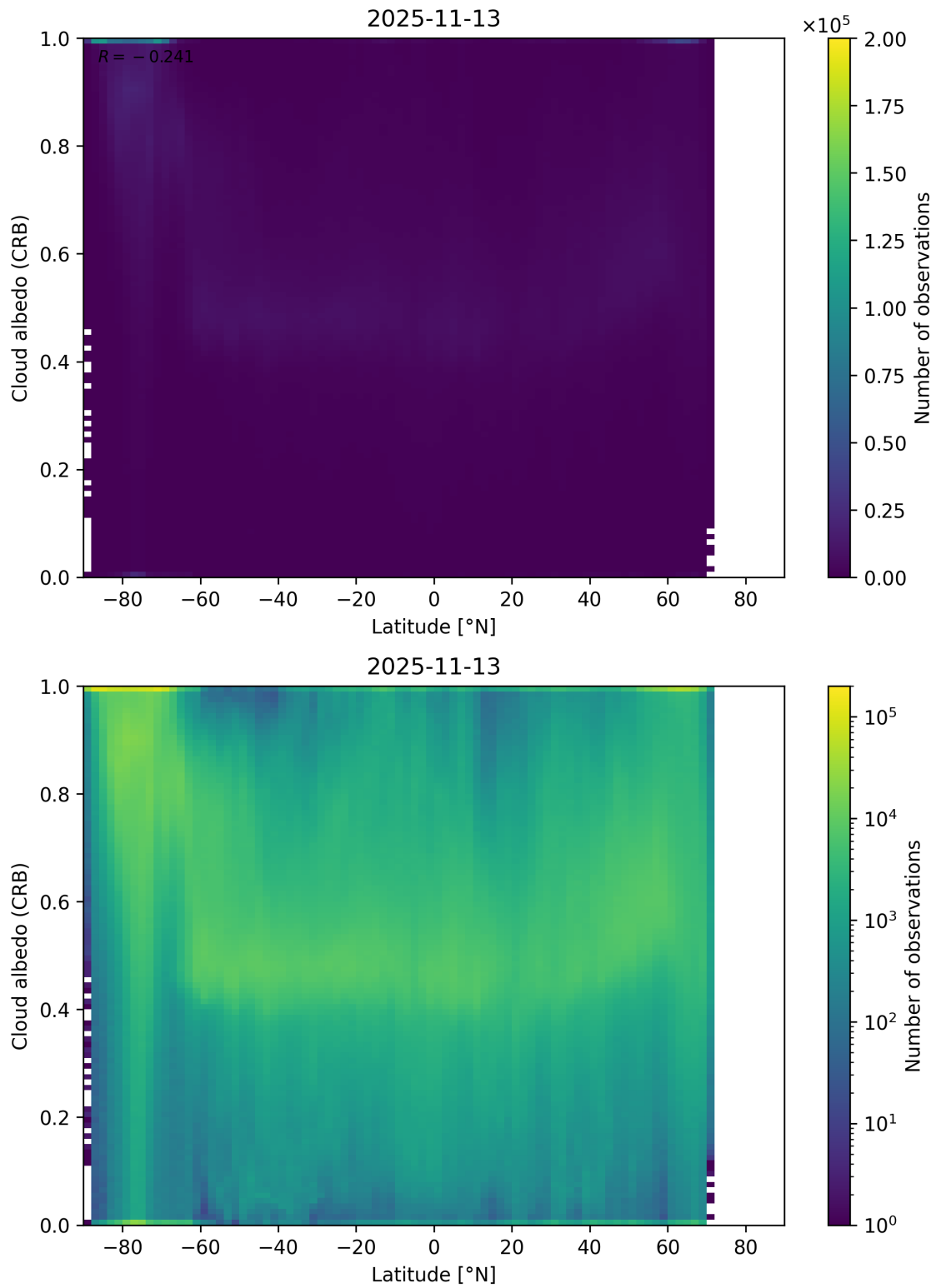
Figure 91: Scatter density plot of “Latitude” against “Cloud albedo (CRB)” for 2025-11-12 to 2025-11-14.
