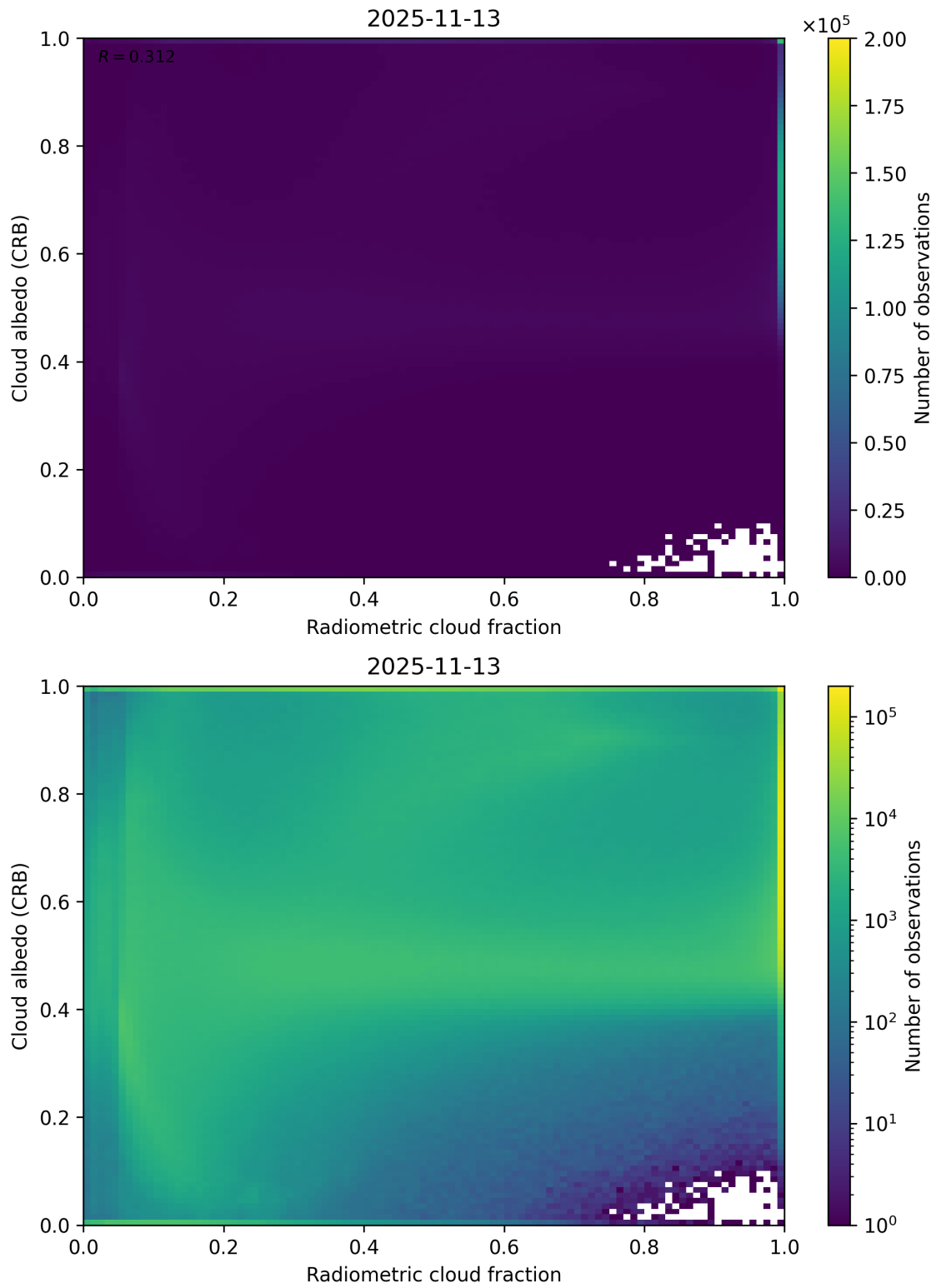
Figure 71: Scatter density plot of “Radiometric cloud fraction” against “Cloud albedo (CRB)” for 2025-11-12 to 2025-11-14.
