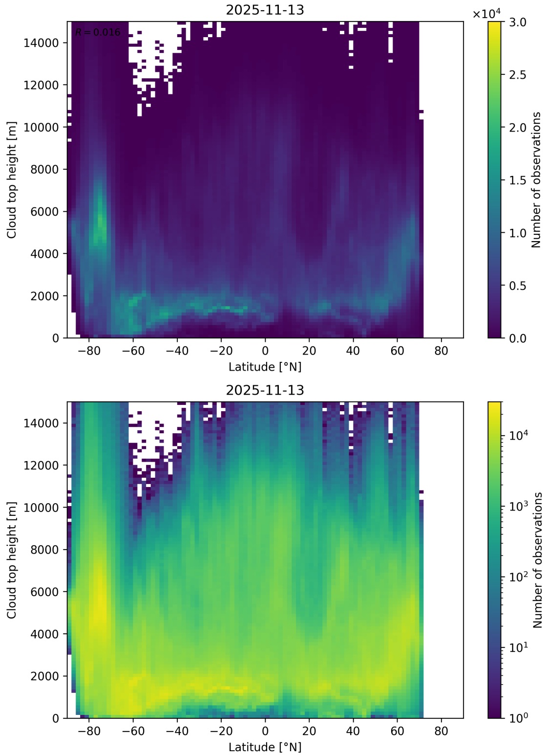
Figure 97: Scatter density plot of “Latitude” against “Cloud top height” for 2025-11-12 to 2025-11-14.
