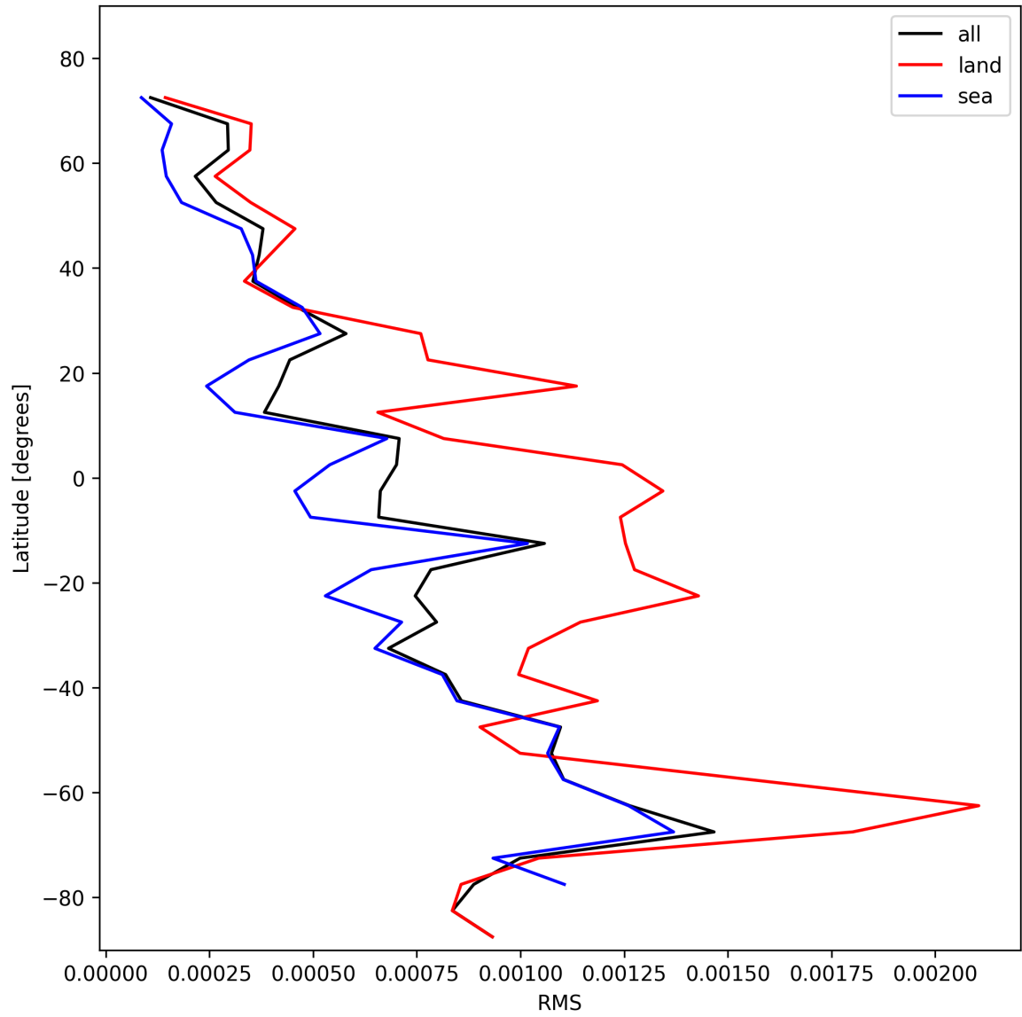
Figure 31: Zonal average of “RMS” for 2025-11-12 to 2025-11-14.
