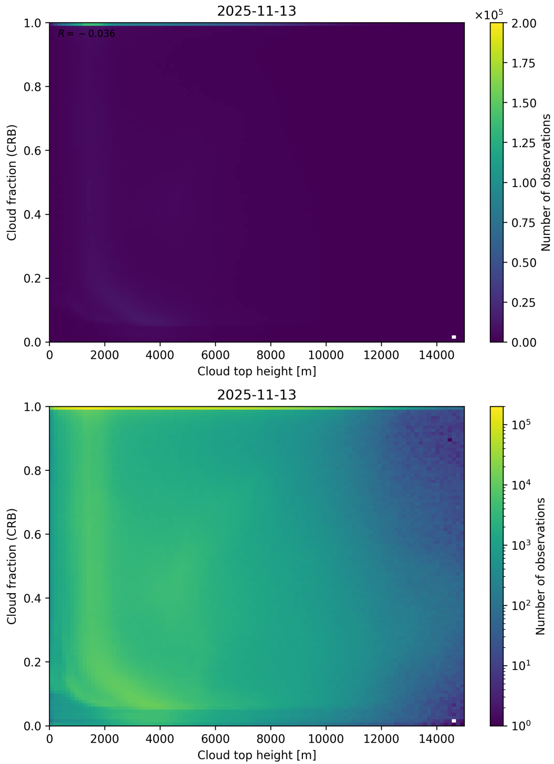
Figure 88: Scatter density plot of “Cloud top height” against “Cloud fraction (CRB)” for 2025-11-12 to 2025-11-14.
