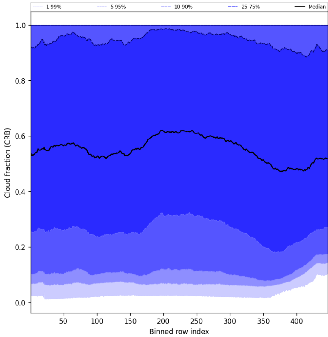
Figure 58: Along track statistics of “Cloud fraction (CRB)” for 2025-11-12 to 2025-11-14
