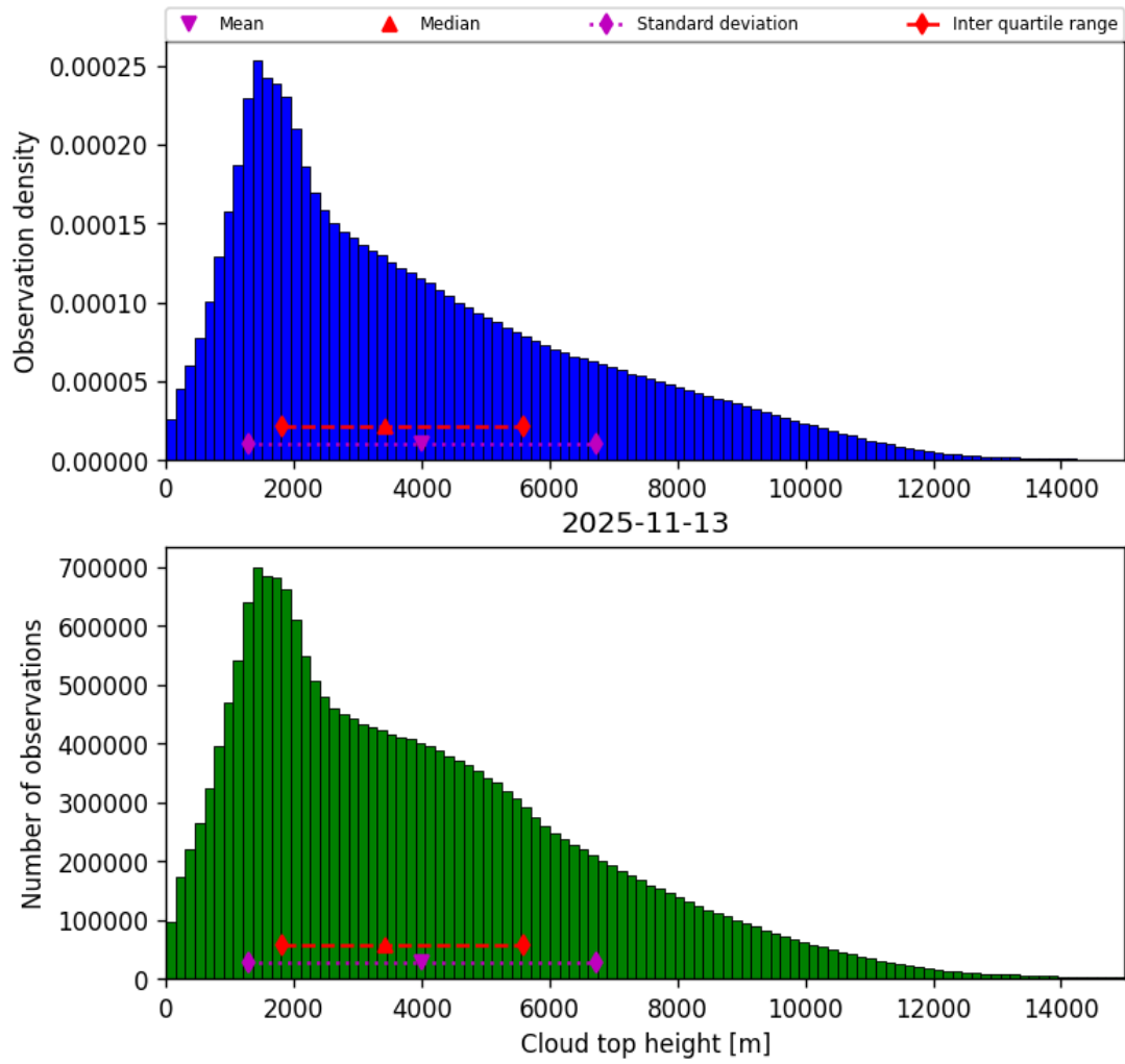
Figure 40: Histogram of “Cloud top height” for 2025-11-12 to 2025-11-14
