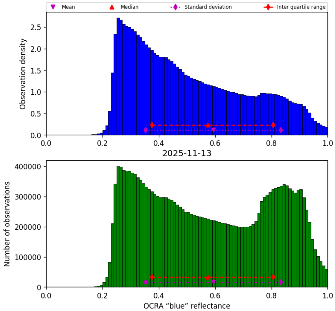
Figure 51: Histogram of “OCRA “blue” reflectance” for 2025-11-12 to 2025-11-14
