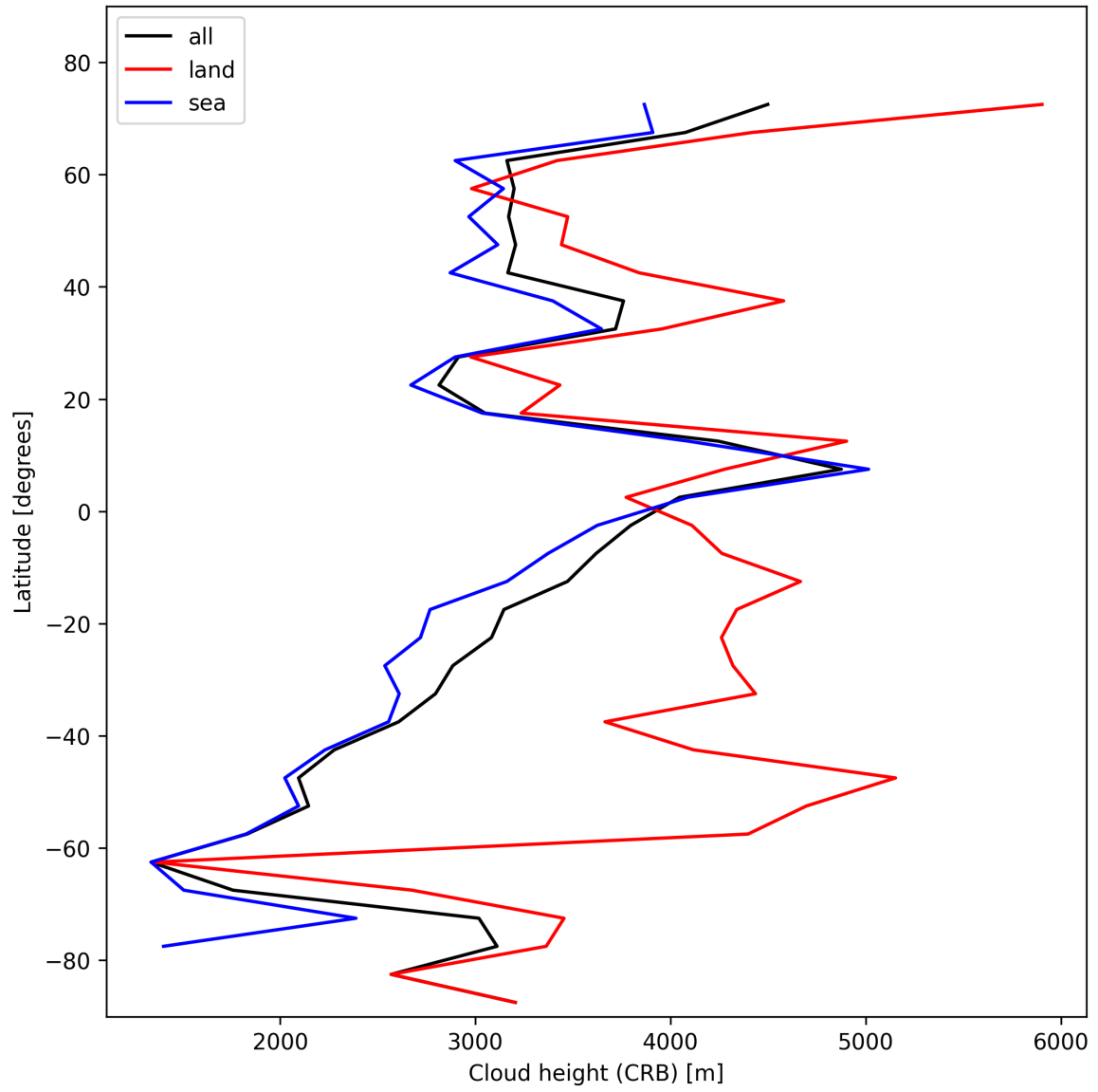
Figure 27: Zonal average of “Cloud height (CRB)” for 2025-11-12 to 2025-11-14.
