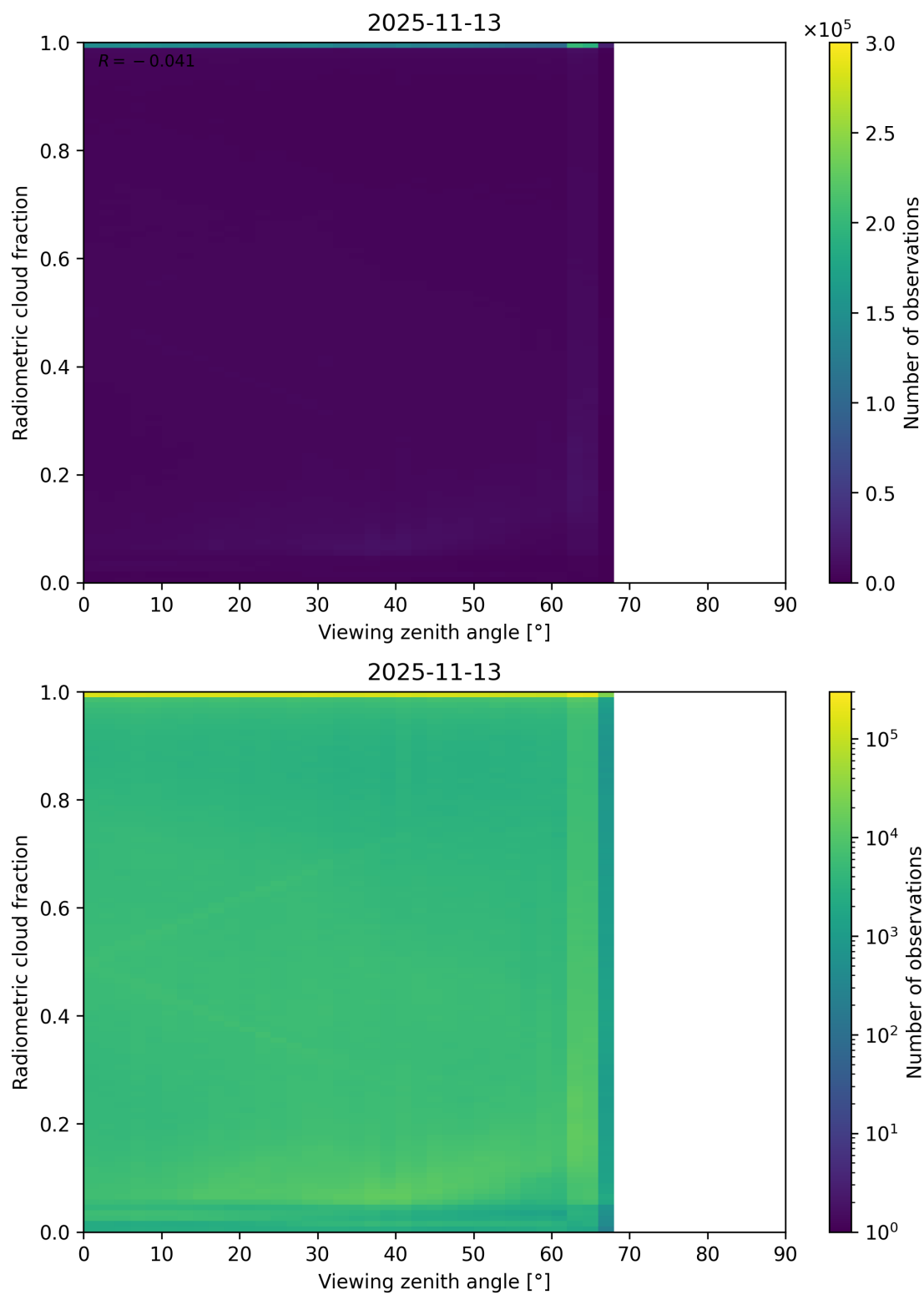
Figure 107: Scatter density plot of “Viewing zenith angle” against “Radiometric cloud fraction” for 2025-11-12 to 2025-11-14.
