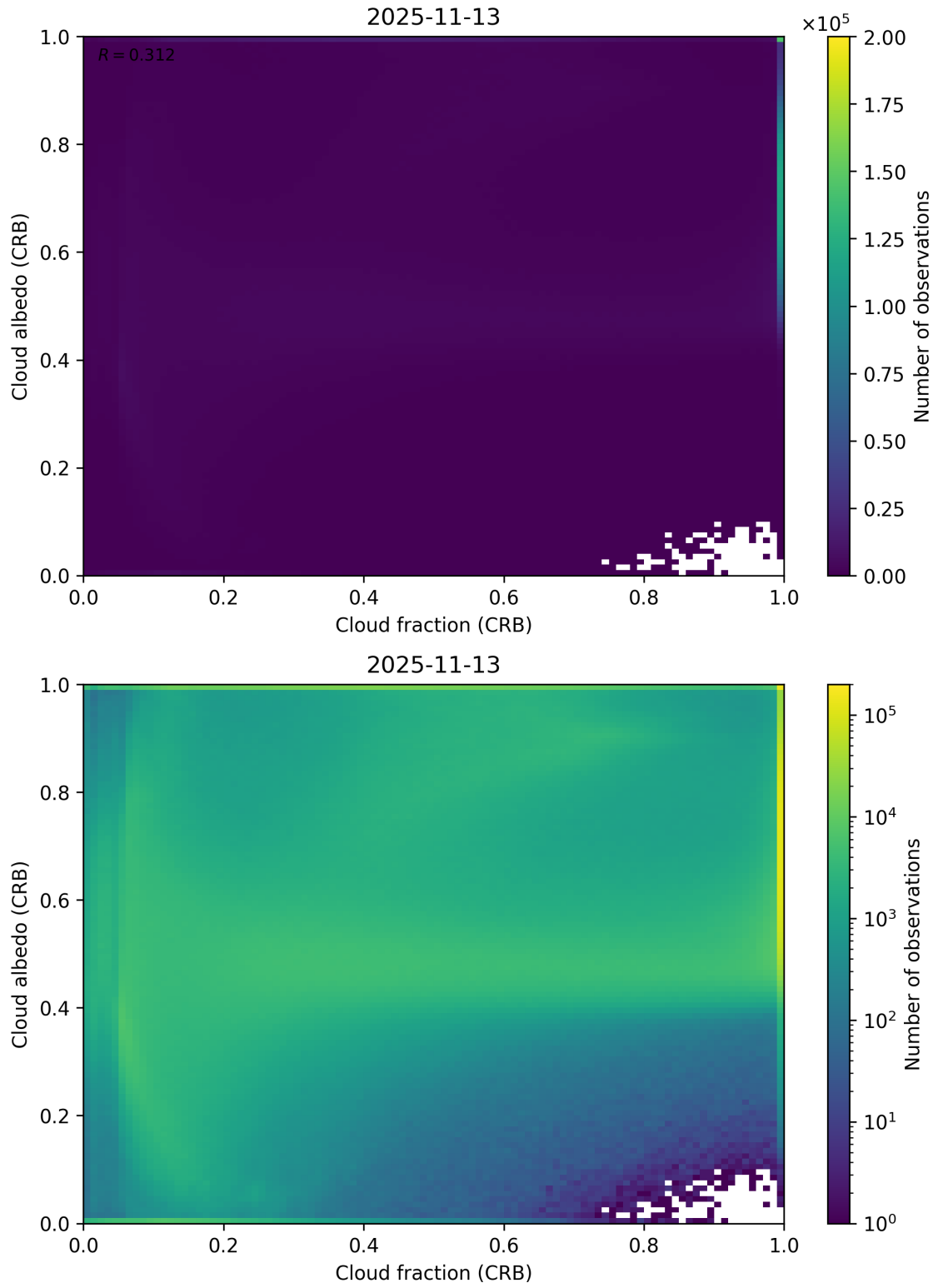
Figure 77: Scatter density plot of “Cloud fraction (CRB)” against “Cloud albedo (CRB)” for 2025-11-12 to 2025-11-14.
