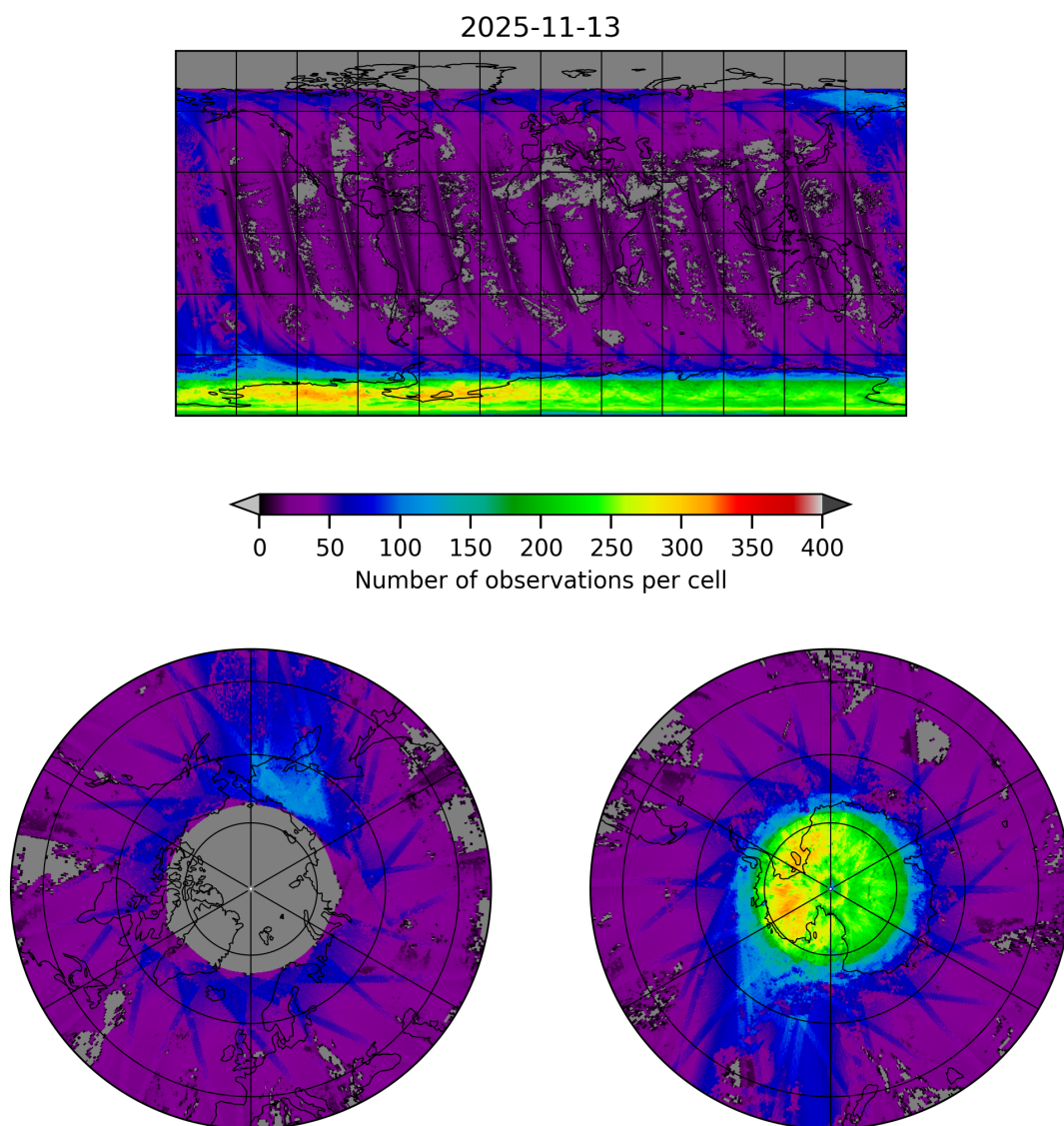
Figure 21: Map of the number of observations for 2025-11-12 to 2025-11-14
