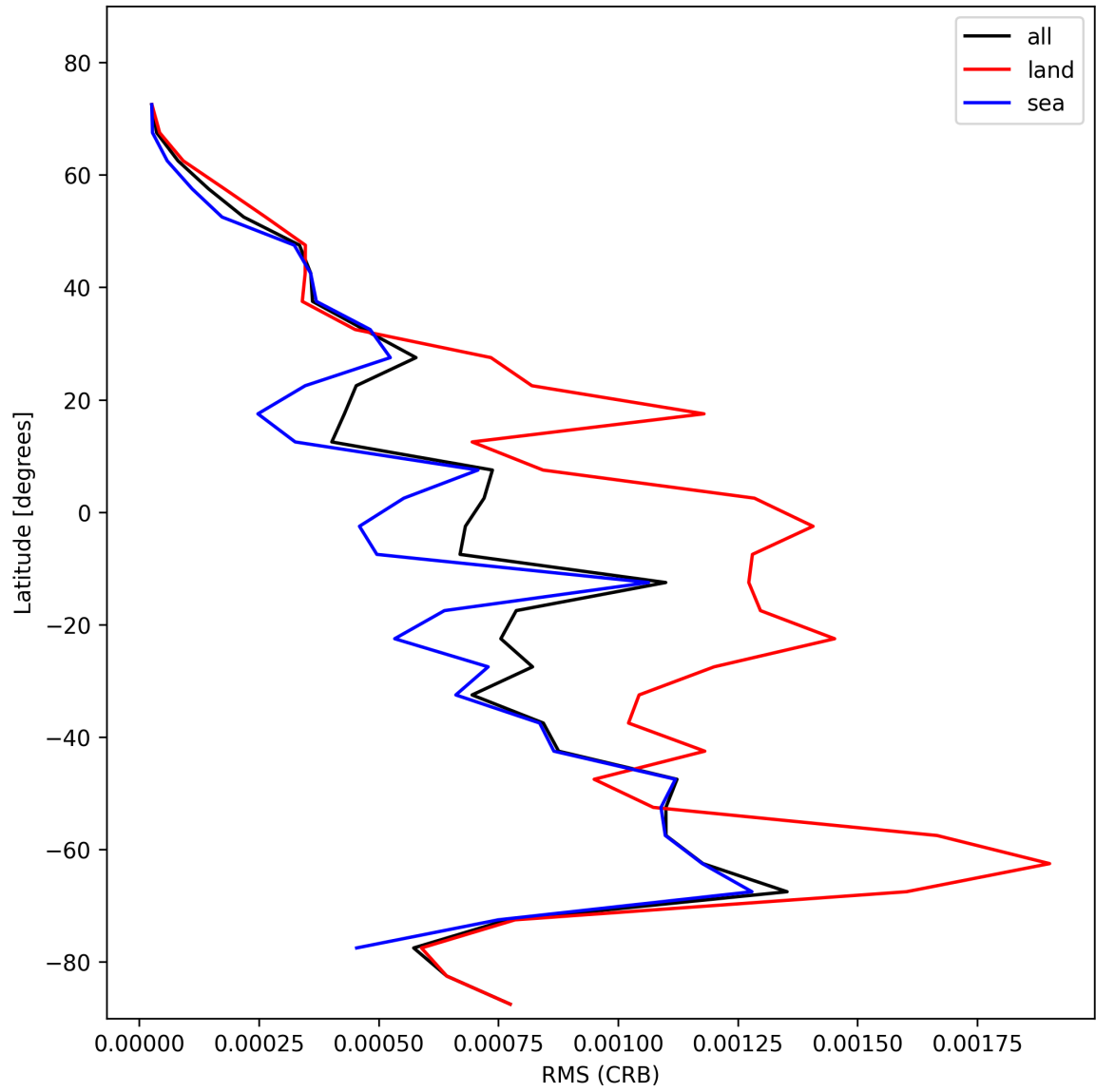
Figure 32: Zonal average of “RMS (CRB)” for 2025-11-12 to 2025-11-14.
