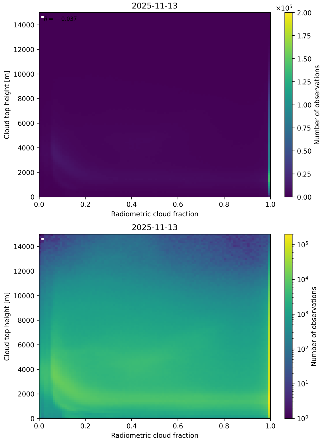
Figure 76: Scatter density plot of “Radiometric cloud fraction” against “Cloud top height” for 2025-11-12 to 2025-11-14.
