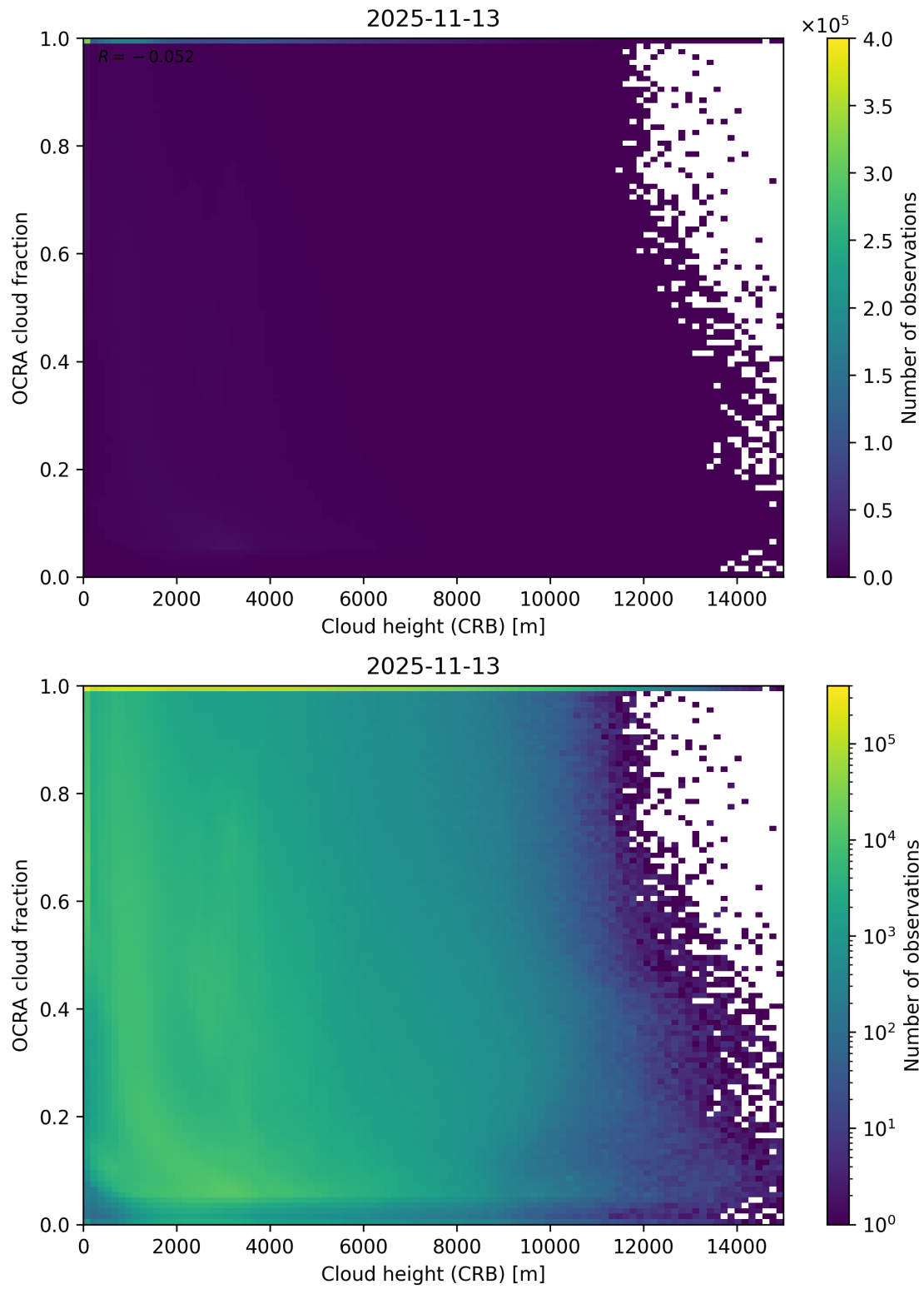
Figure 81: Scatter density plot of “Cloud height (CRB)” against “OCRA cloud fraction” for 2025-11-12 to 2025-11-14.
