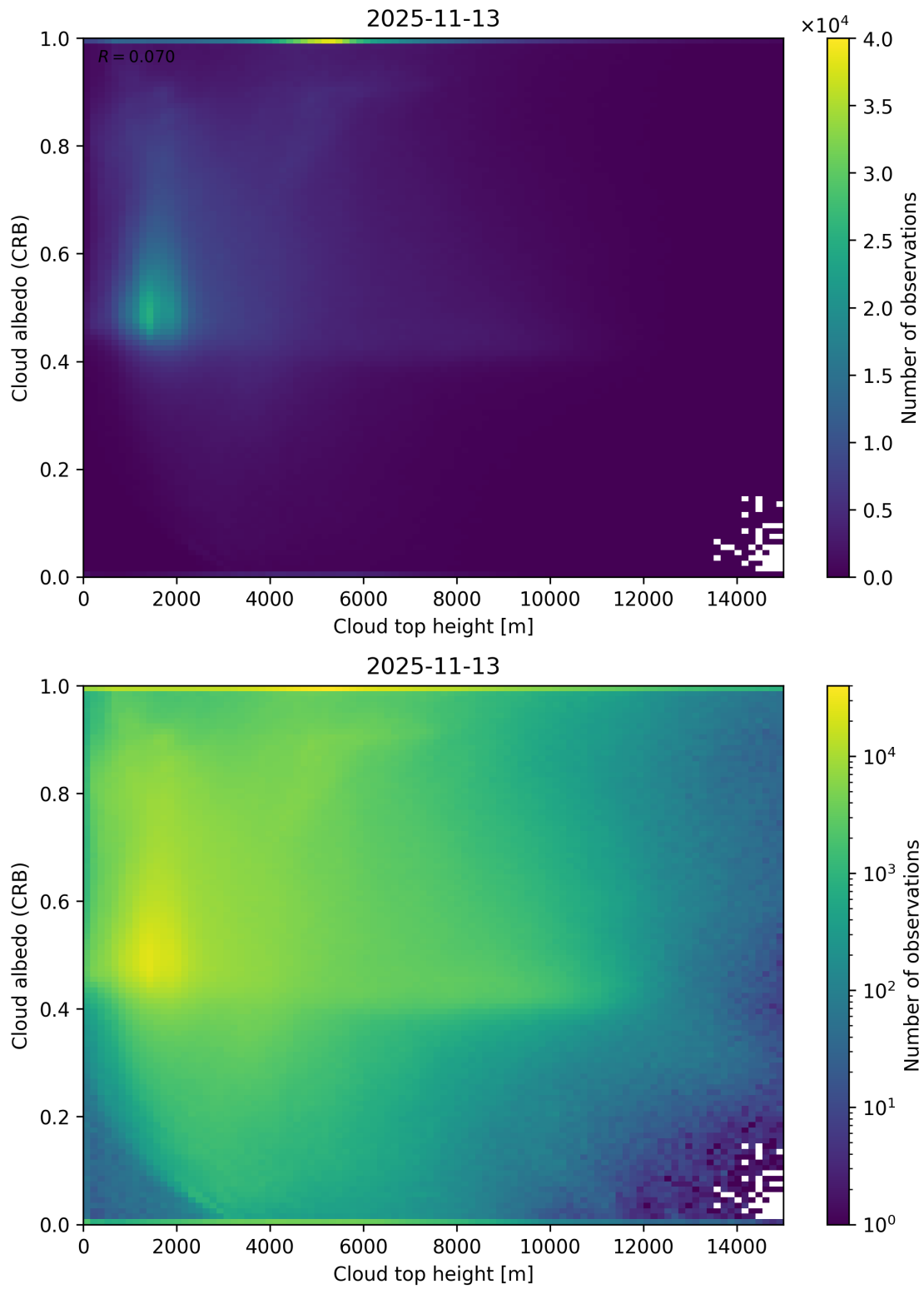
Figure 86: Scatter density plot of “Cloud top height” against “Cloud albedo (CRB)” for 2025-11-12 to 2025-11-14.
