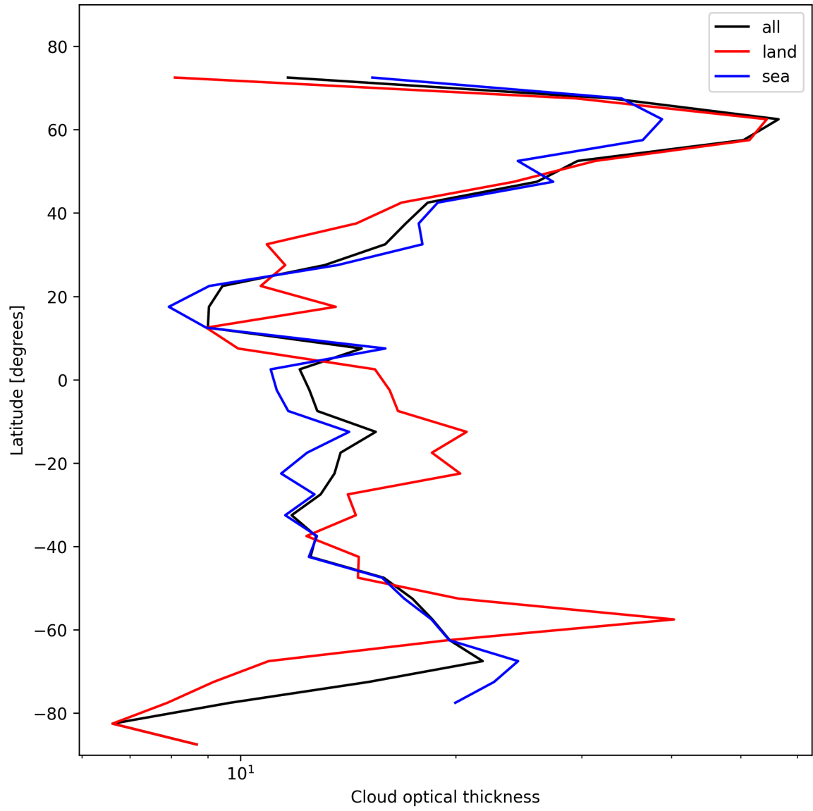
Figure 25: Zonal average of “Cloud optical thickness” for 2025-11-12 to 2025-11-14.
