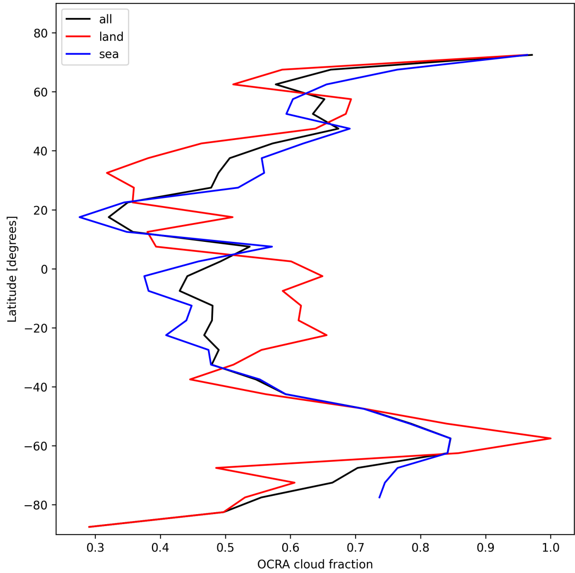
Figure 34: Zonal average of “OCRA cloud fraction” for 2025-11-12 to 2025-11-14.
