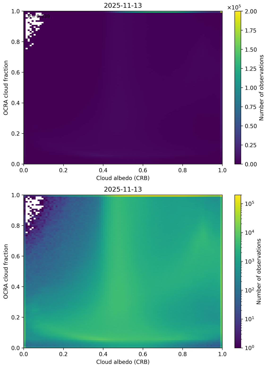
Figure 70: Scatter density plot of “Cloud albedo (CRB)” against “OCRA cloud fraction” for 2025-11-12 to 2025-11-14.
