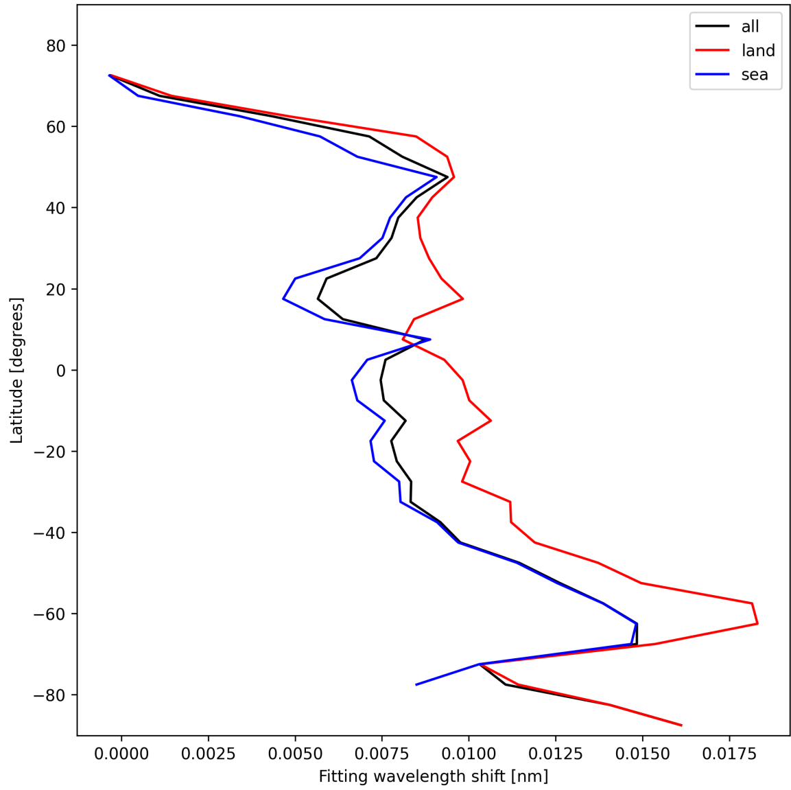
Figure 33: Zonal average of “Fitting wavelength shift” for 2025-11-12 to 2025-11-14.
