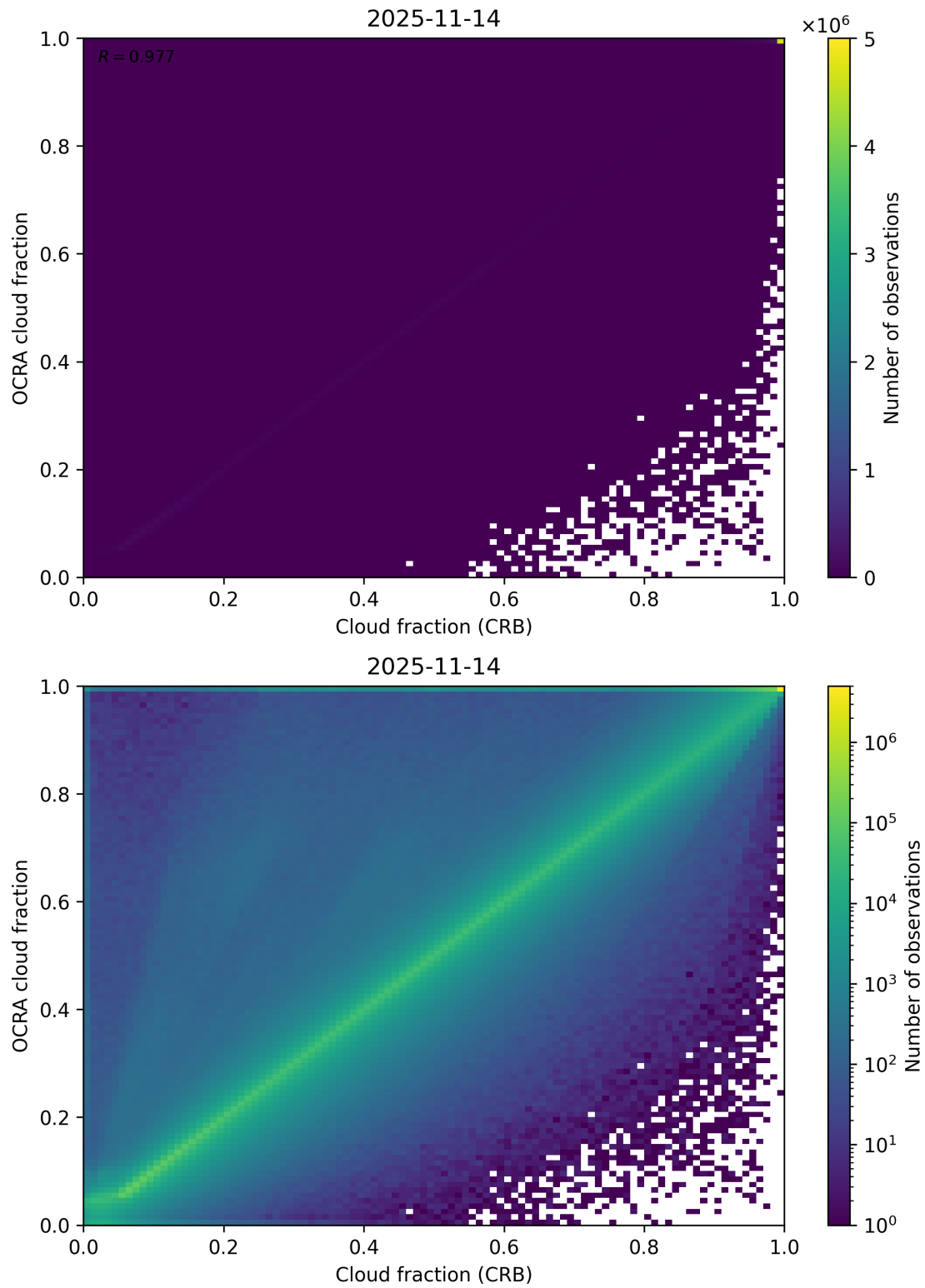
Figure 78: Scatter density plot of “Cloud fraction (CRB)” against “OCRA cloud fraction” for 2025-11-13 to 2025-11-15.
