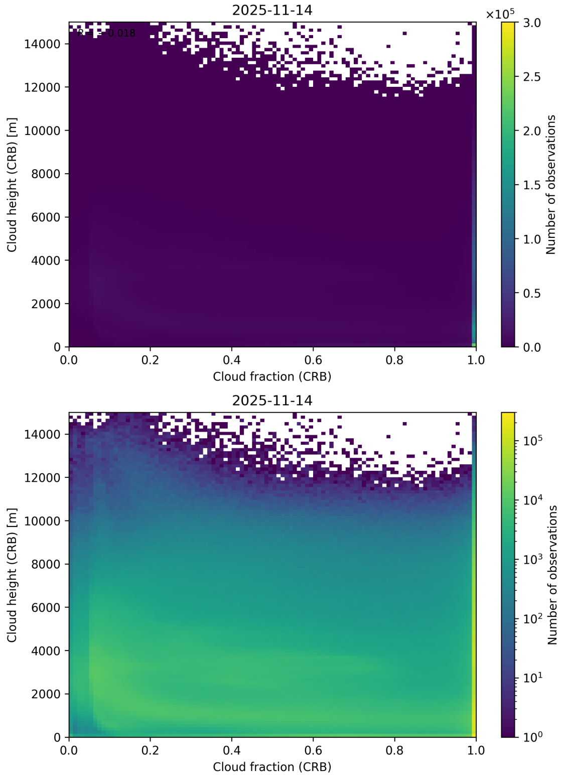
Figure 79: Scatter density plot of “Cloud fraction (CRB)” against “Cloud height (CRB)” for 2025-11-13 to 2025-11-15.
