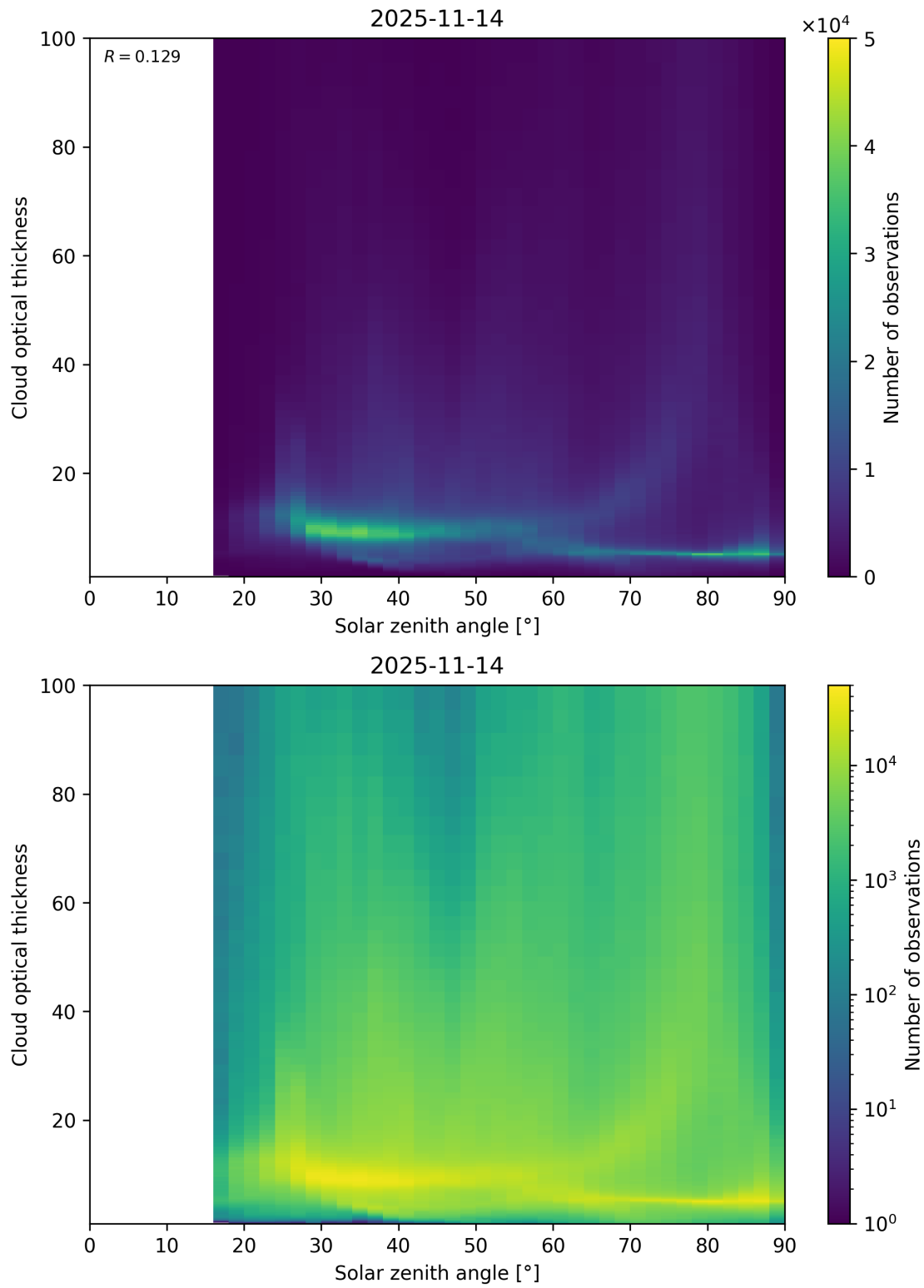
Figure 103: Scatter density plot of “Solar zenith angle” against “Cloud optical thickness” for 2025-11-13 to 2025-11-15.
