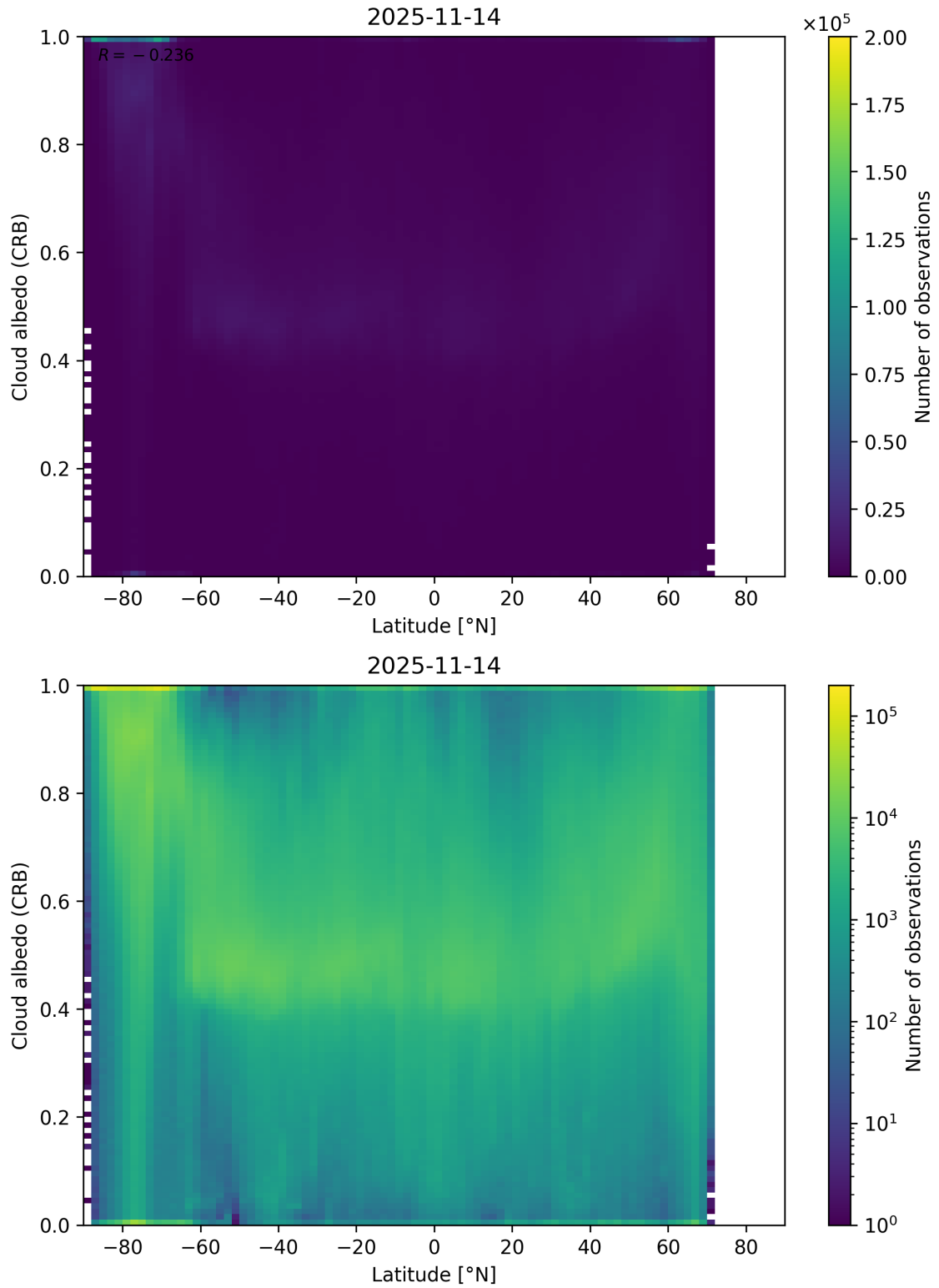
Figure 91: Scatter density plot of “Latitude” against “Cloud albedo (CRB)” for 2025-11-13 to 2025-11-15.
