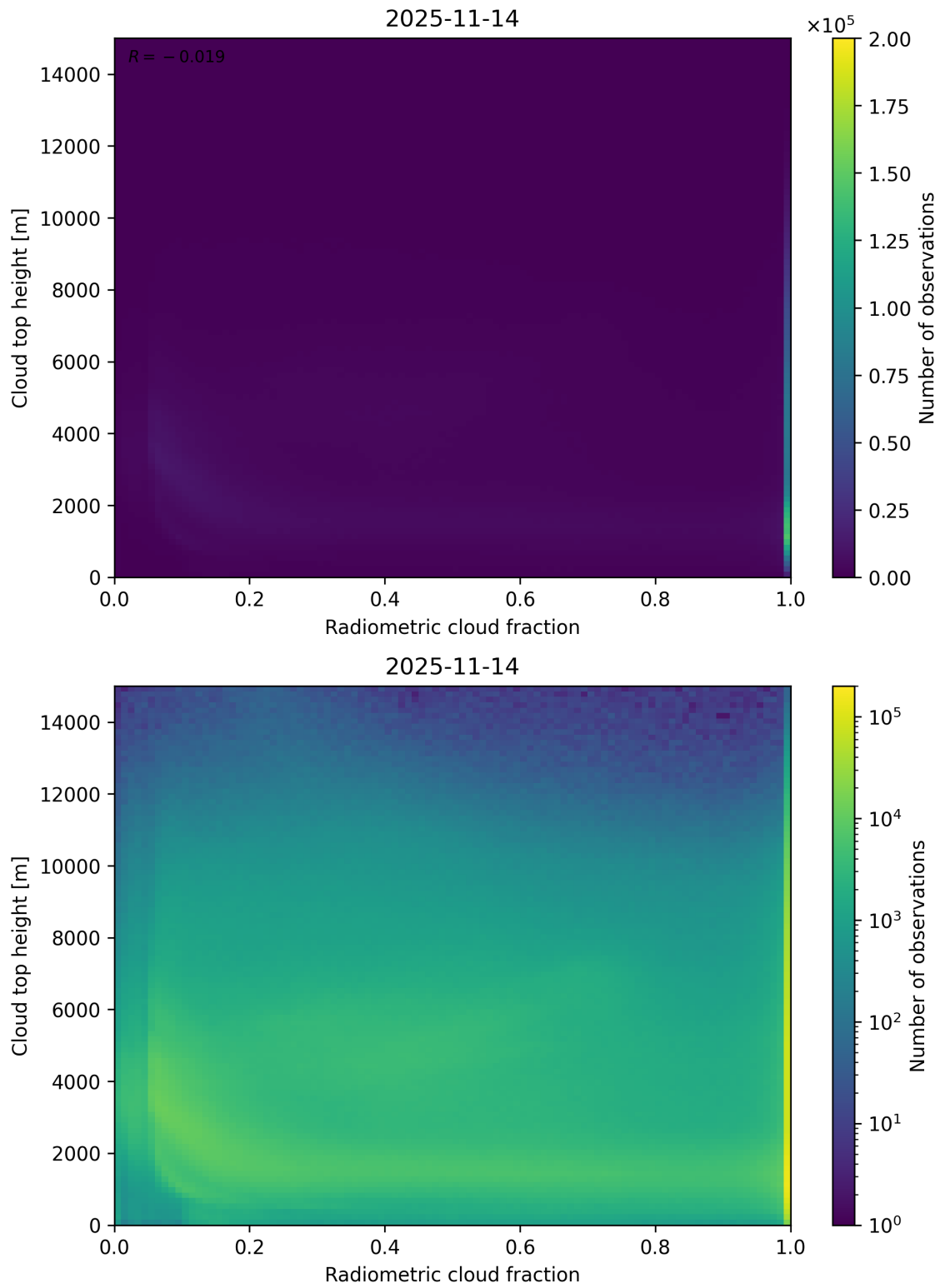
Figure 76: Scatter density plot of “Radiometric cloud fraction” against “Cloud top height” for 2025-11-13 to 2025-11-15.
