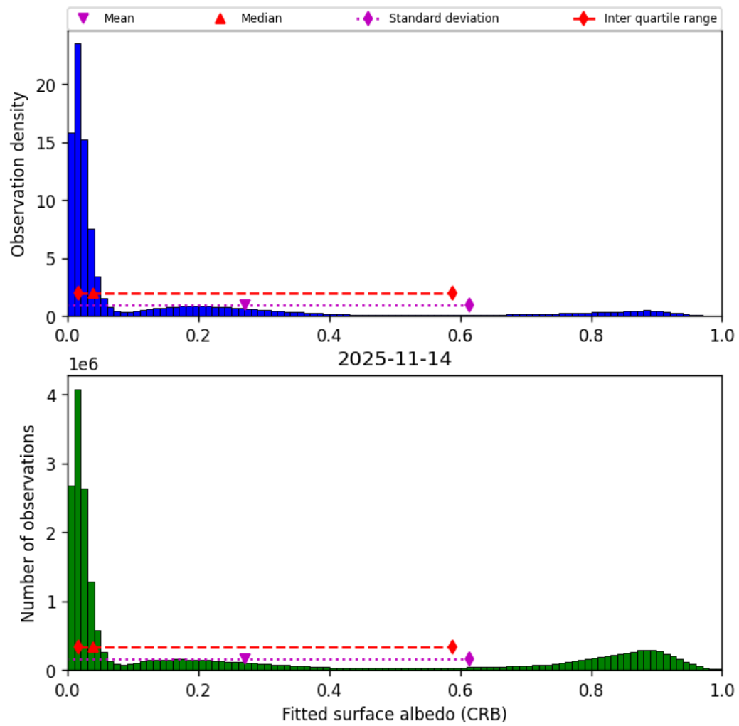
Figure 46: Histogram of “Fitted surface albedo (CRB)” for 2025-11-13 to 2025-11-15
