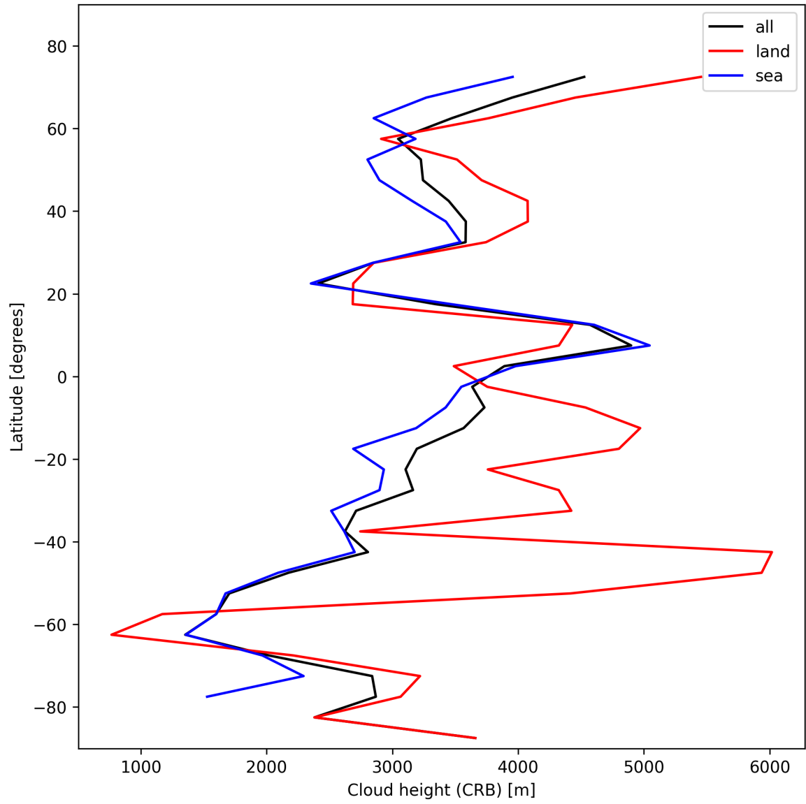
Figure 27: Zonal average of “Cloud height (CRB)” for 2025-11-13 to 2025-11-15.
