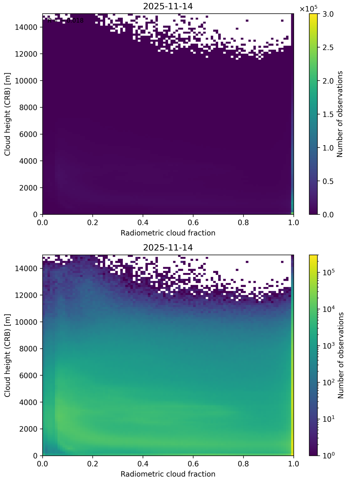
Figure 74: Scatter density plot of “Radiometric cloud fraction” against “Cloud height (CRB)” for 2025-11-13 to 2025-11-15.
