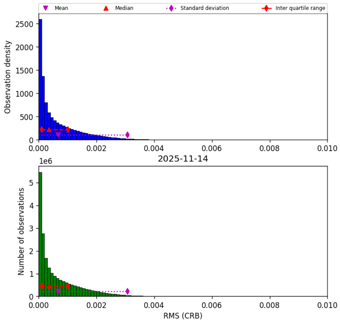
Figure 48: Histogram of “RMS (CRB)” for 2025-11-13 to 2025-11-15
