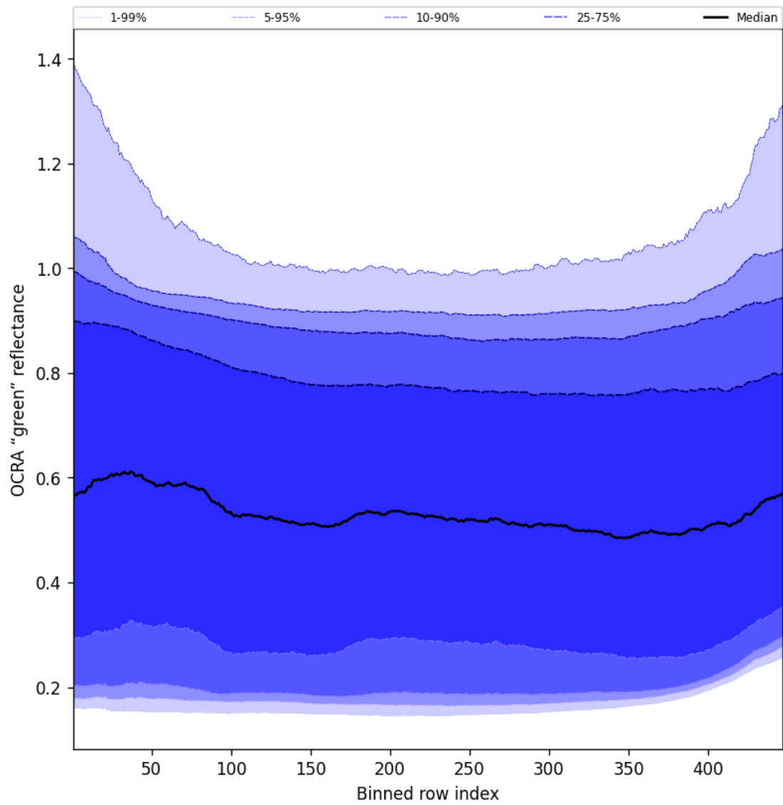
Figure 68: Along track statistics of “OCRA “green” reflectance” for 2025-11-13 to 2025-11-15
