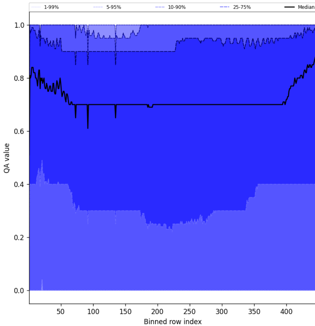
Figure 54: Along track statistics of “QA value” for 2025-11-13 to 2025-11-15
