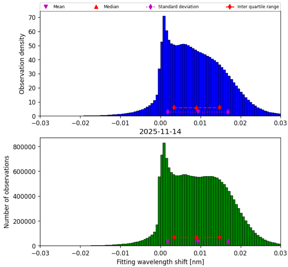
Figure 49: Histogram of “Fitting wavelength shift” for 2025-11-13 to 2025-11-15
