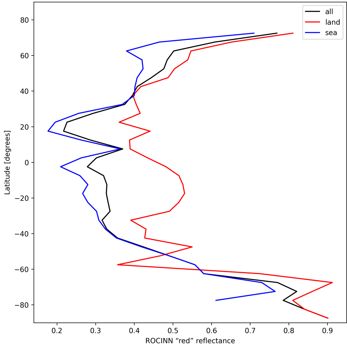
Figure 37: Zonal average of “ROCINN “red” reflectance” for 2025-11-13 to 2025-11-15.
