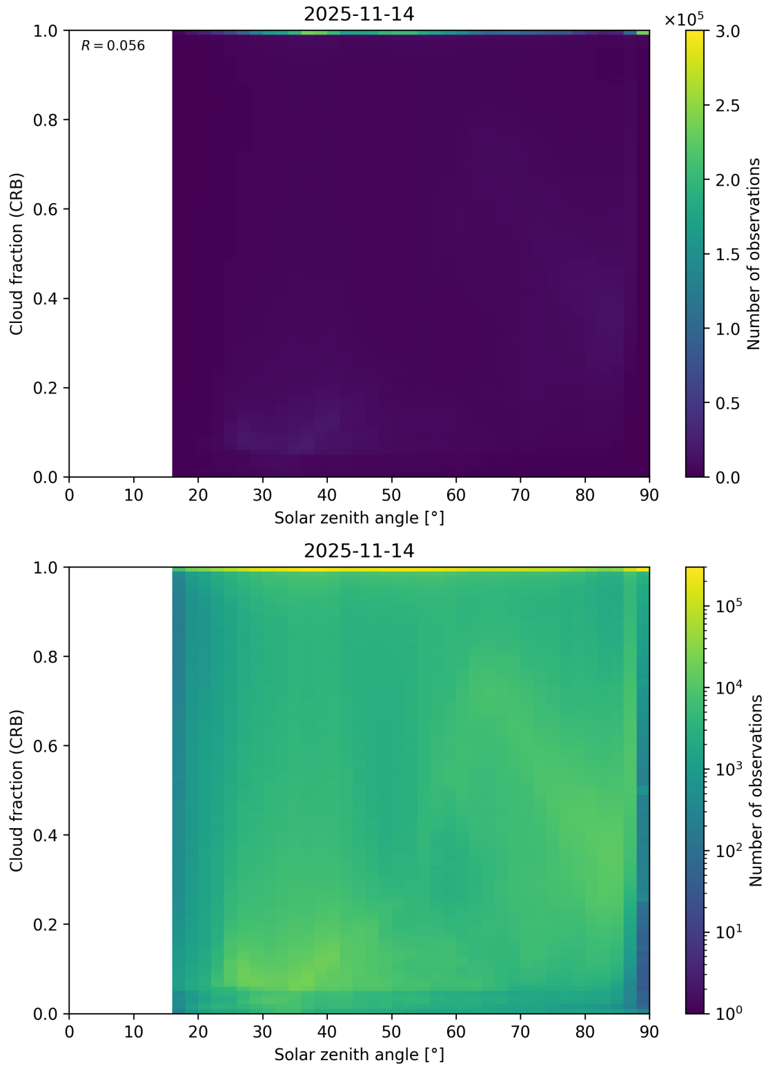
Figure 101: Scatter density plot of “Solar zenith angle” against “Cloud fraction (CRB)” for 2025-11-13 to 2025-11-15.
