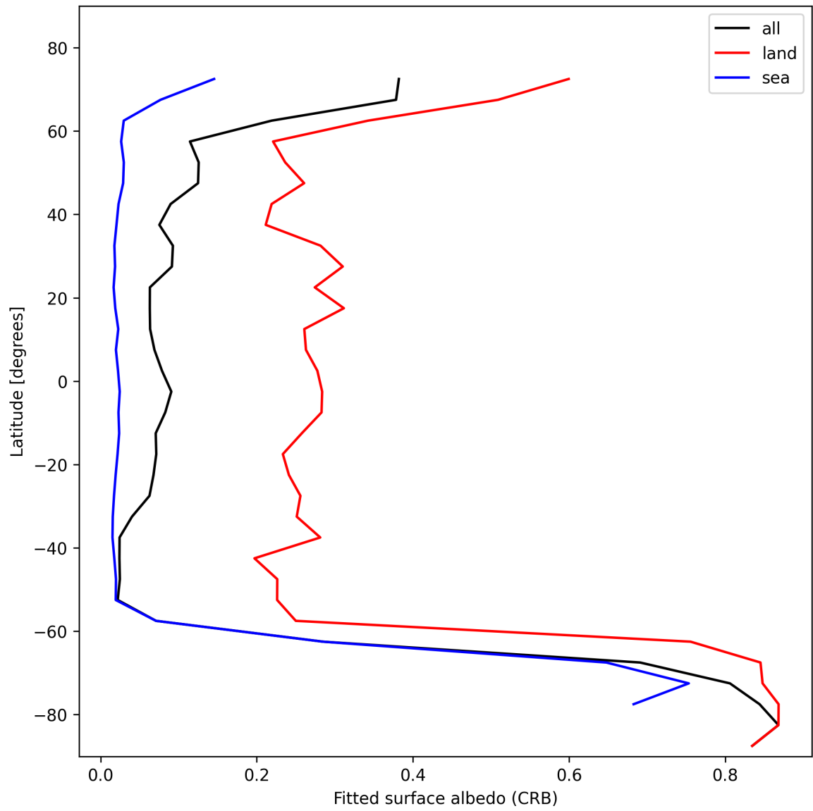
Figure 30: Zonal average of “Fitted surface albedo (CRB)” for 2025-11-13 to 2025-11-15.
