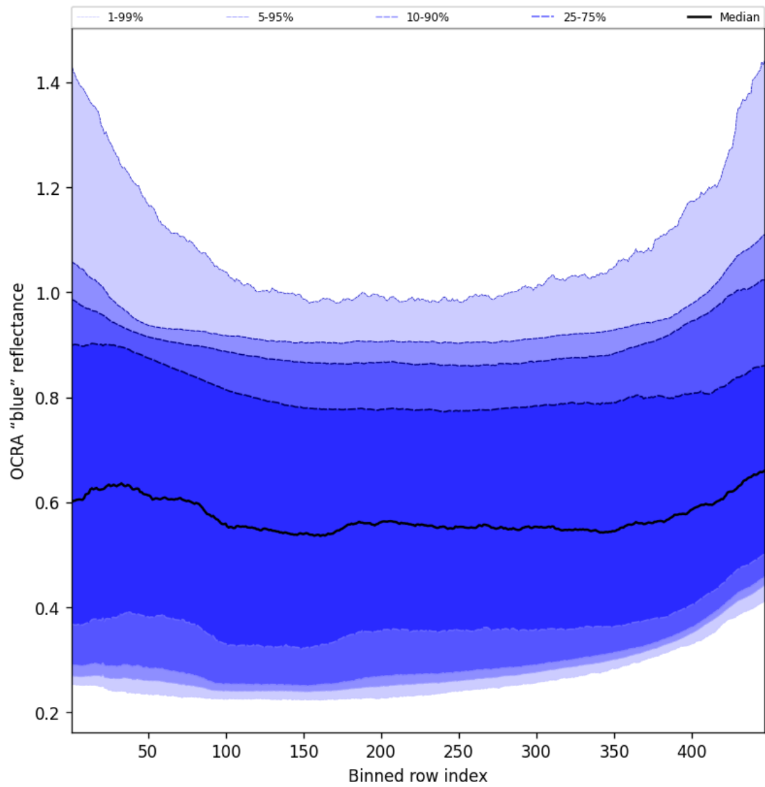
Figure 67: Along track statistics of “OCRA “blue” reflectance” for 2025-11-13 to 2025-11-15
