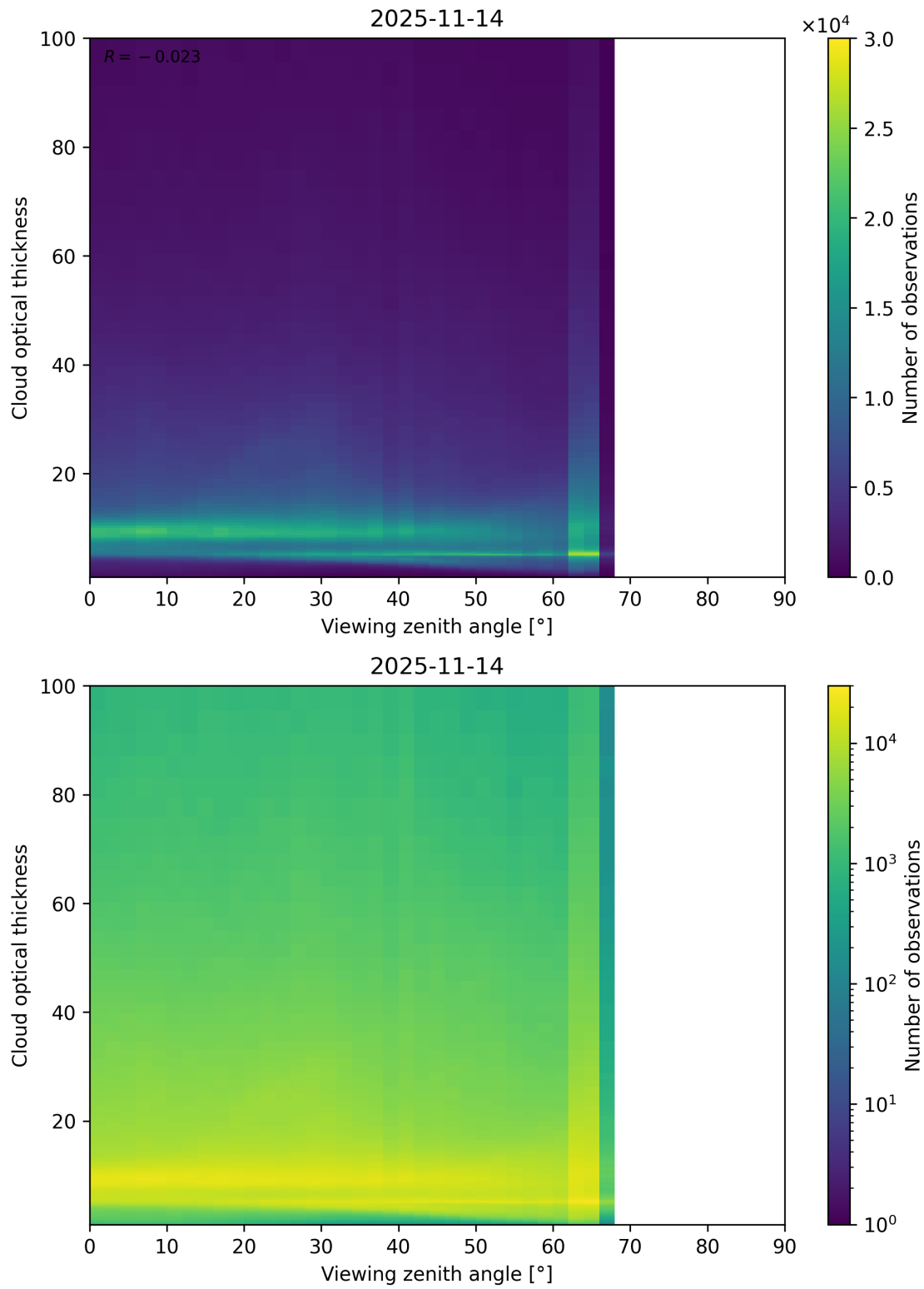
Figure 111: Scatter density plot of “Viewing zenith angle” against “Cloud optical thickness” for 2025-11-13 to 2025-11-15.
