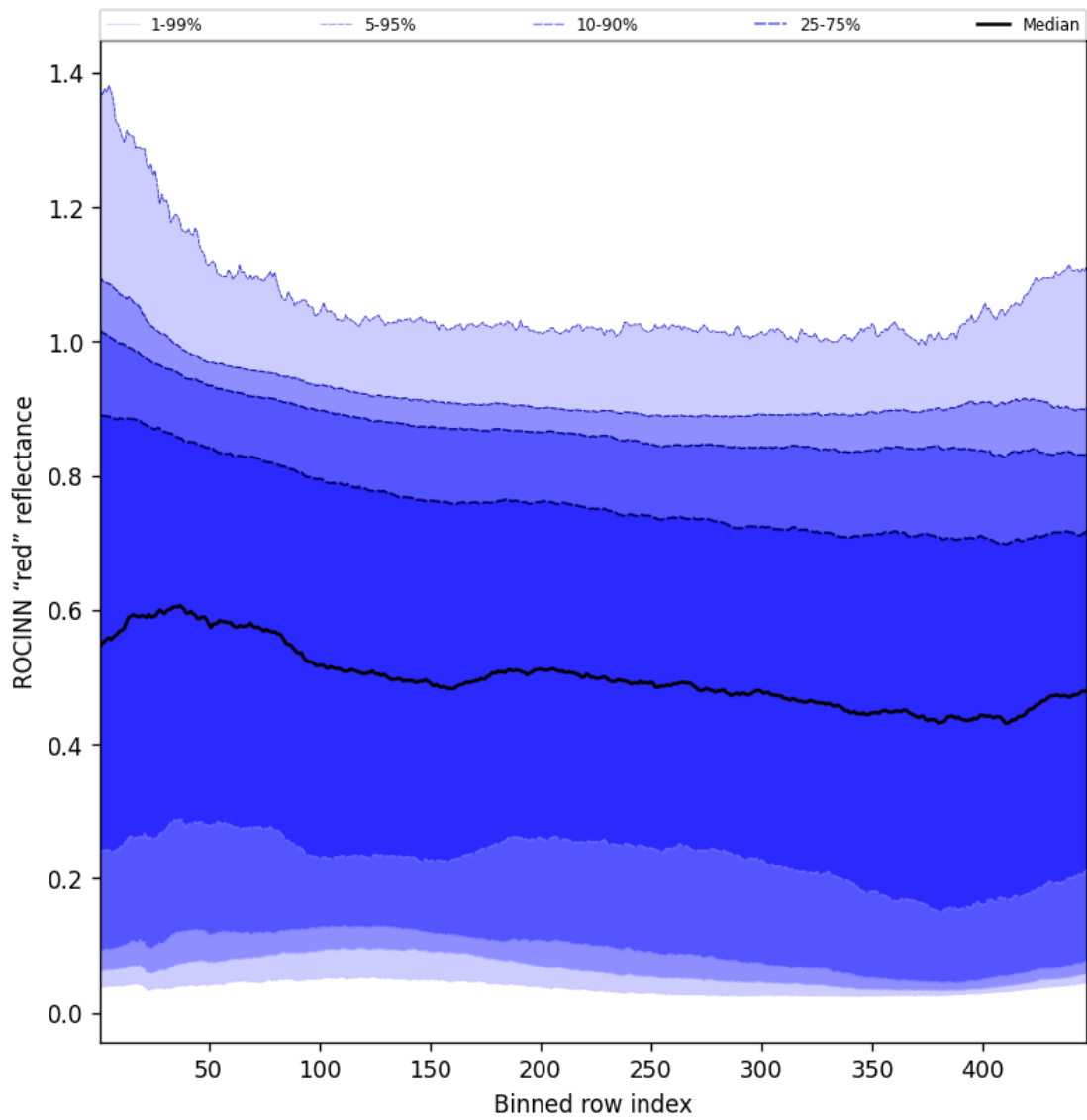
Figure 69: Along track statistics of “ROCINN “red” reflectance” for 2025-11-13 to 2025-11-15
