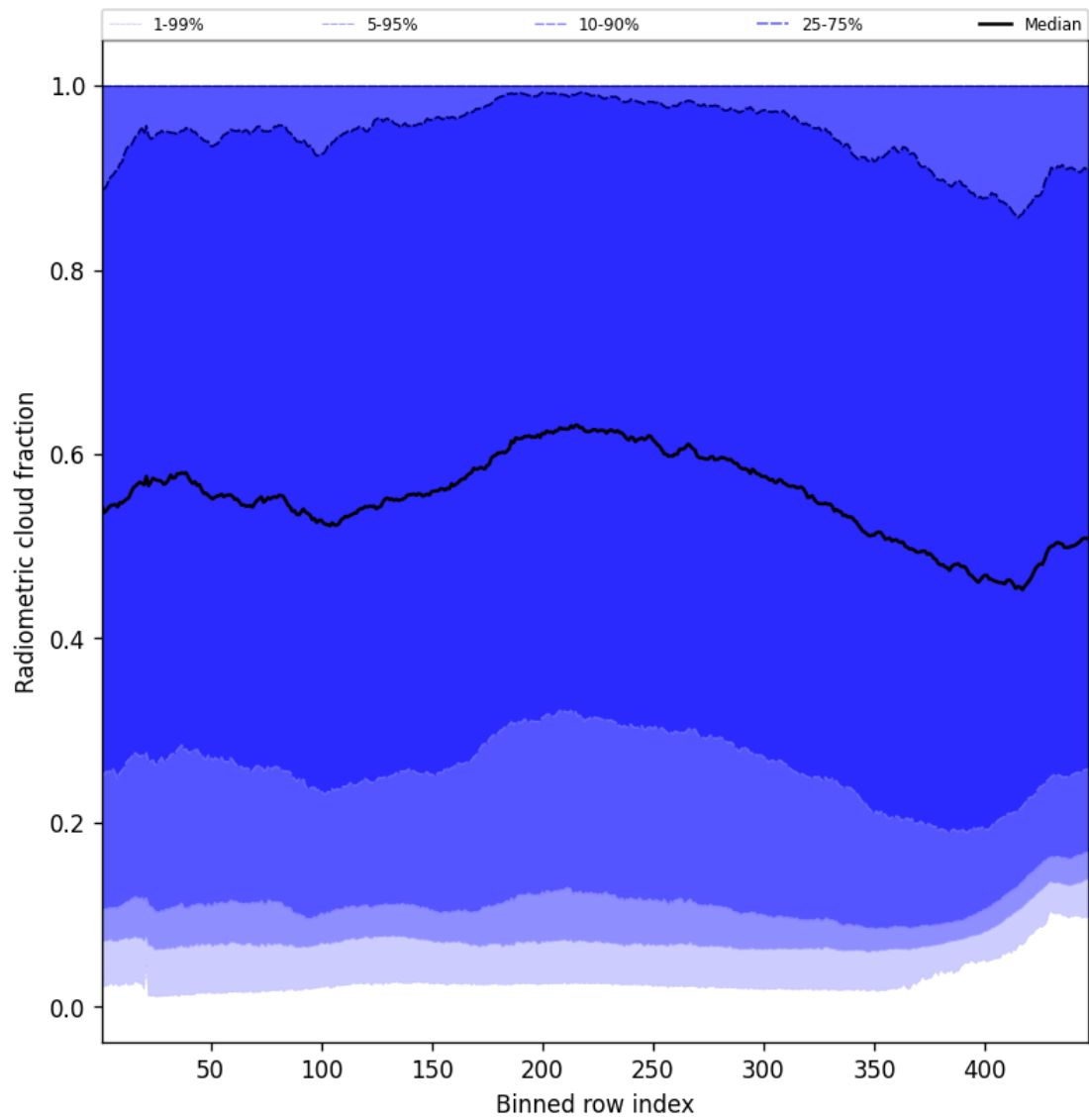
Figure 55: Along track statistics of “Radiometric cloud fraction” for 2025-11-13 to 2025-11-15
