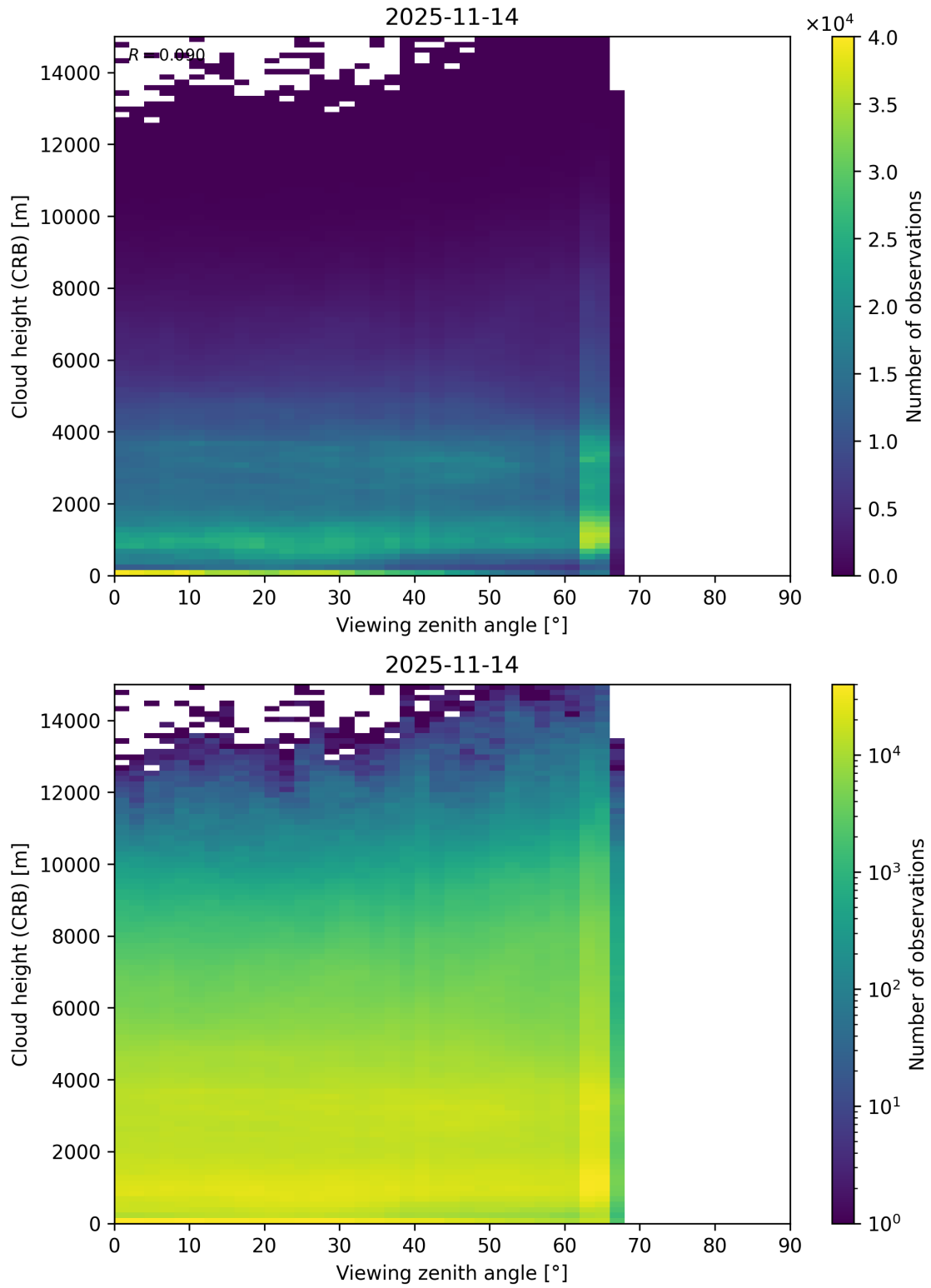
Figure 110: Scatter density plot of “Viewing zenith angle” against “Cloud height (CRB)” for 2025-11-13 to 2025-11-15.
