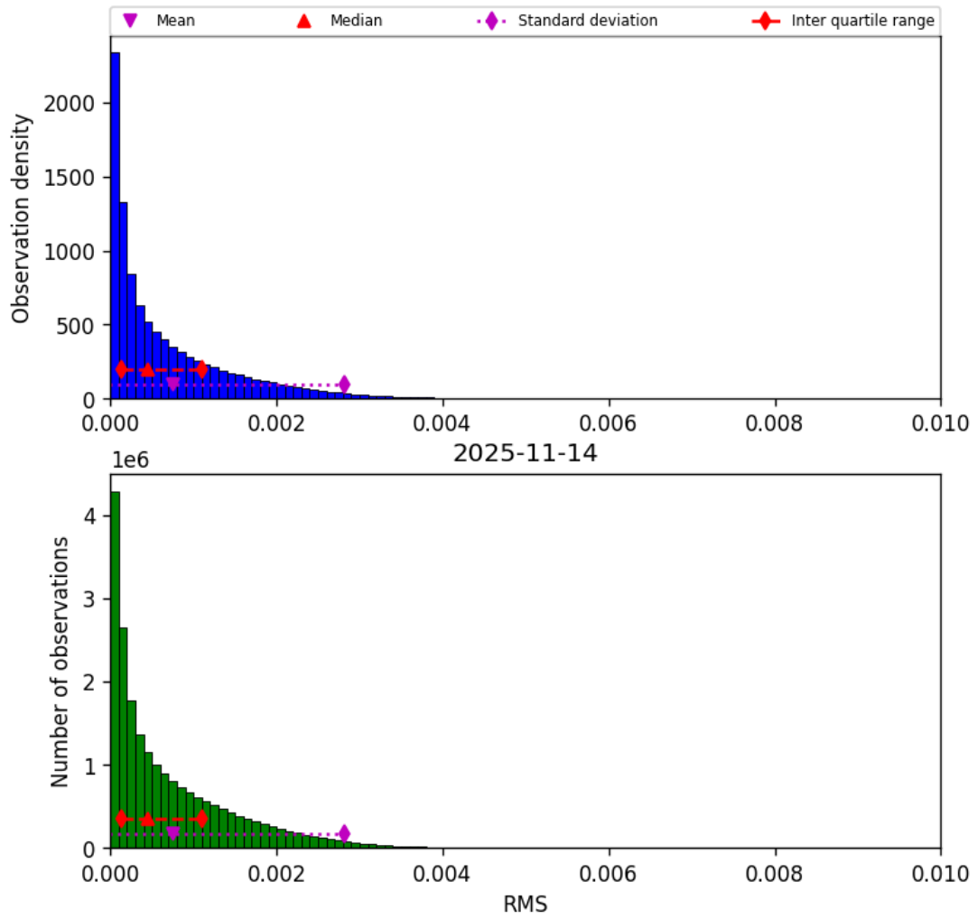
Figure 47: Histogram of “RMS” for 2025-11-13 to 2025-11-15
