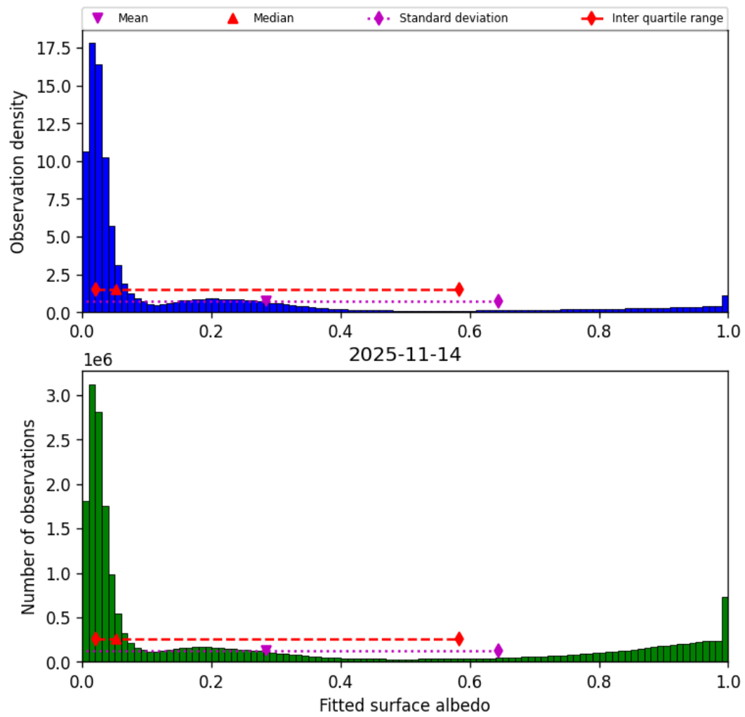
Figure 45: Histogram of “Fitted surface albedo” for 2025-11-13 to 2025-11-15
