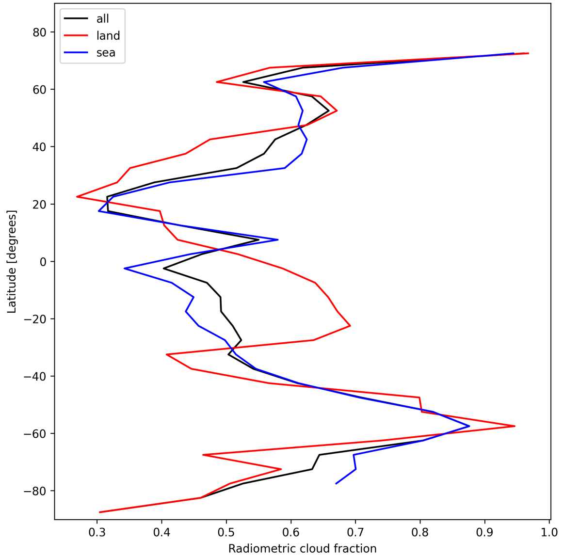
Figure 23: Zonal average of “Radiometric cloud fraction” for 2025-11-13 to 2025-11-15.
