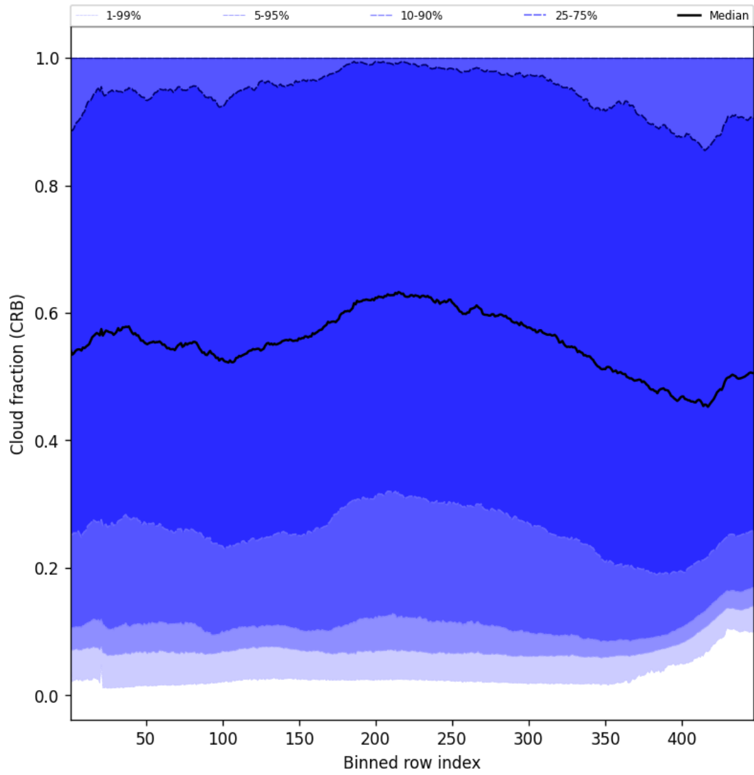
Figure 58: Along track statistics of “Cloud fraction (CRB)” for 2025-11-13 to 2025-11-15
