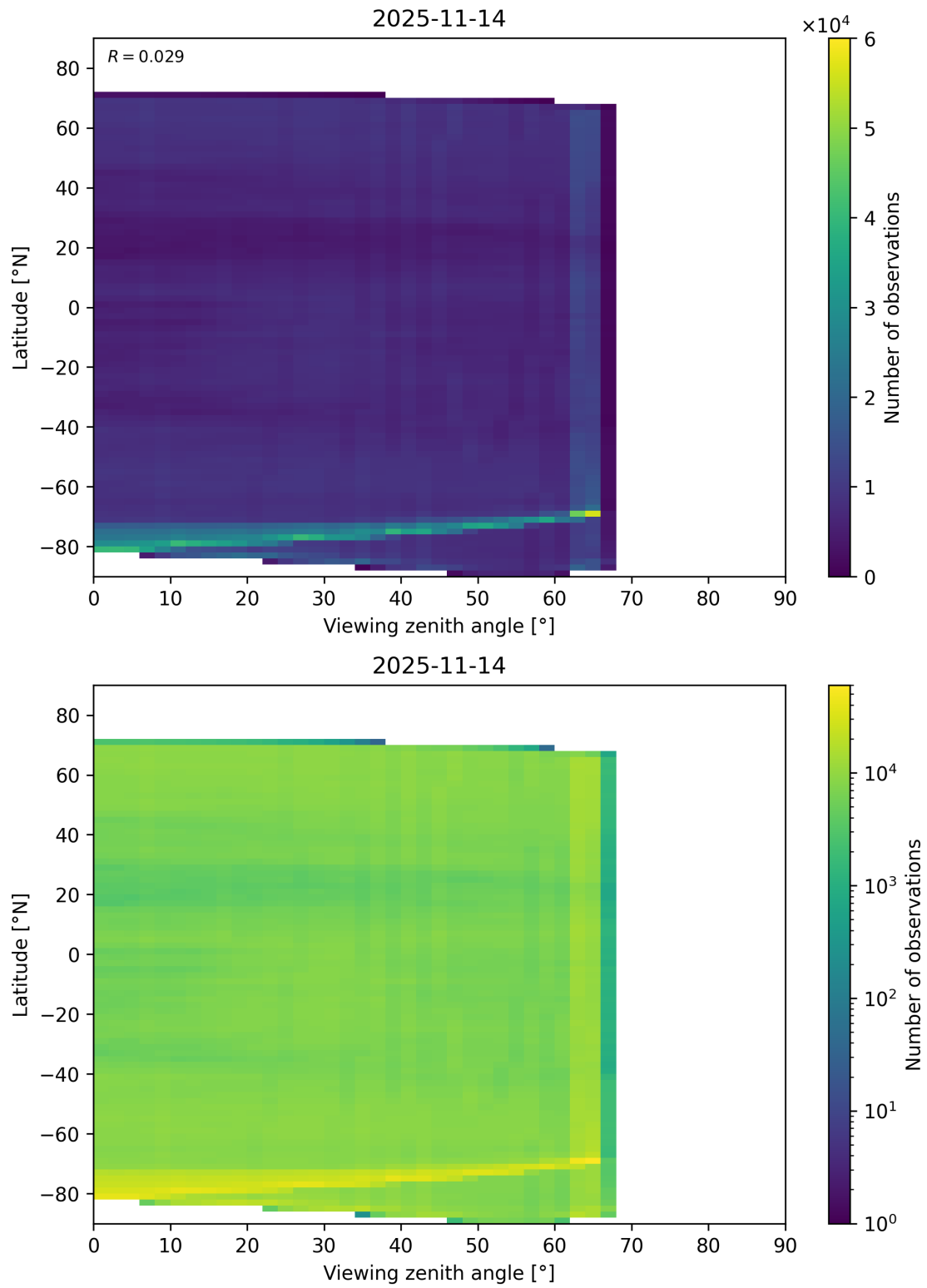
Figure 113: Scatter density plot of “Viewing zenith angle” against “Latitude” for 2025-11-13 to 2025-11-15.
