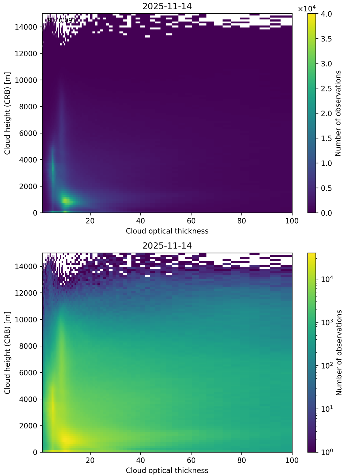
Figure 85: Scatter density plot of “Cloud optical thickness” against “Cloud height (CRB)” for 2025-11-13 to 2025-11-15.
