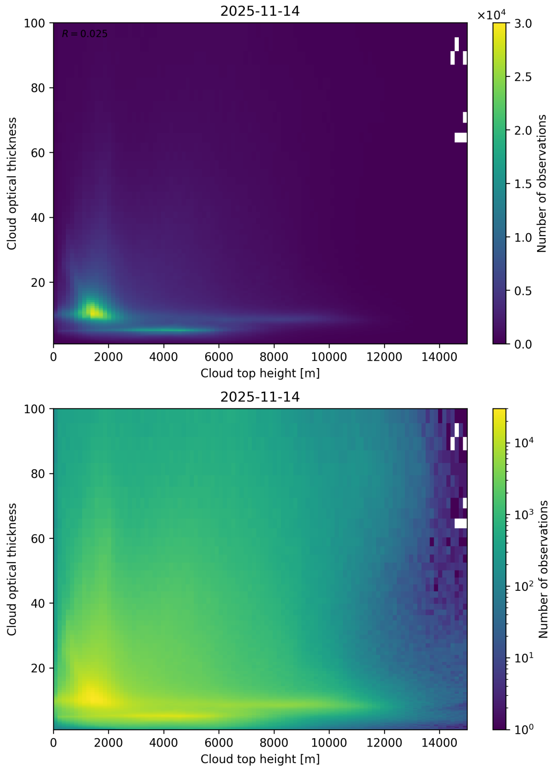
Figure 90: Scatter density plot of “Cloud top height” against “Cloud optical thickness” for 2025-11-13 to 2025-11-15.
