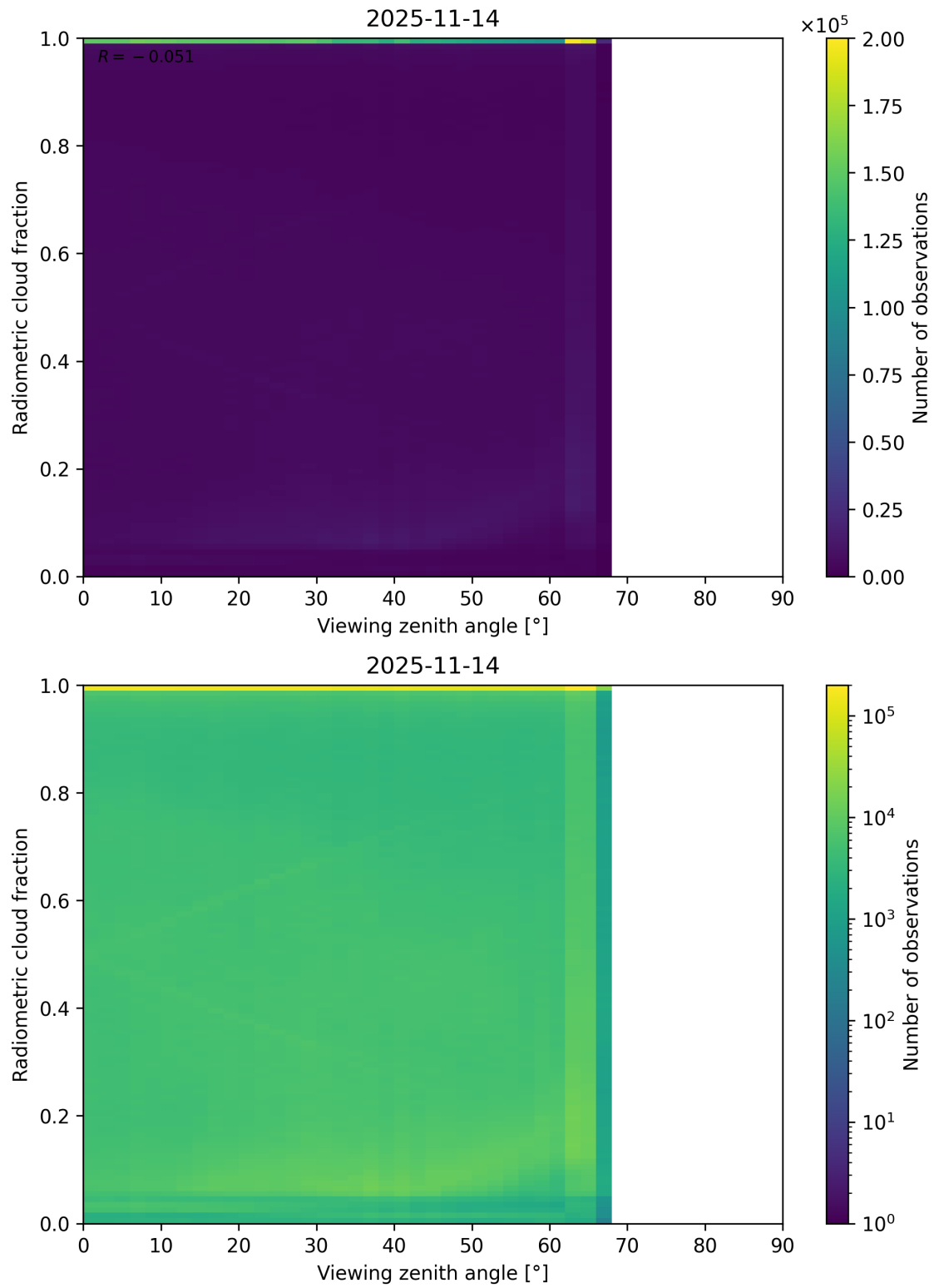
Figure 107: Scatter density plot of “Viewing zenith angle” against “Radiometric cloud fraction” for 2025-11-13 to 2025-11-15.
