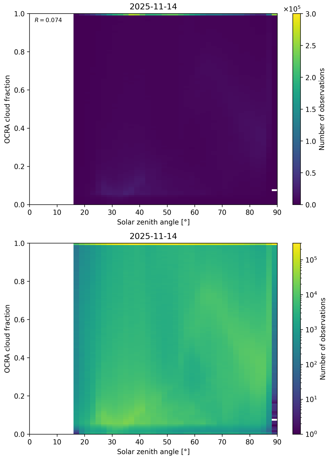
Figure 100: Scatter density plot of “Solar zenith angle” against “OCRA cloud fraction” for 2025-11-13 to 2025-11-15.
