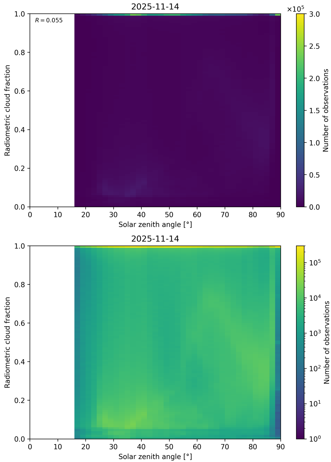
Figure 99: Scatter density plot of “Solar zenith angle” against “Radiometric cloud fraction” for 2025-11-13 to 2025-11-15.
