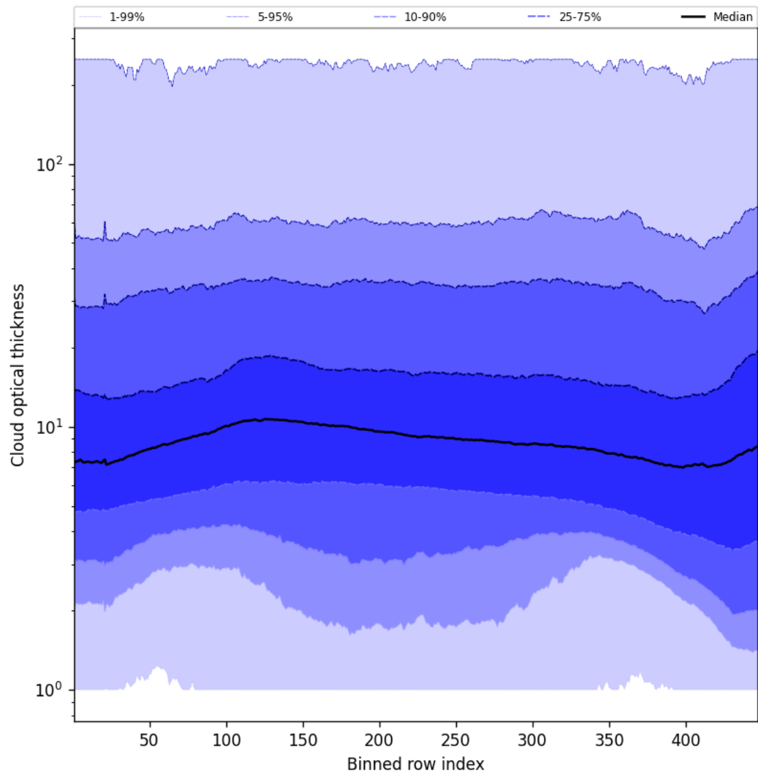
Figure 57: Along track statistics of “Cloud optical thickness” for 2025-11-13 to 2025-11-15
