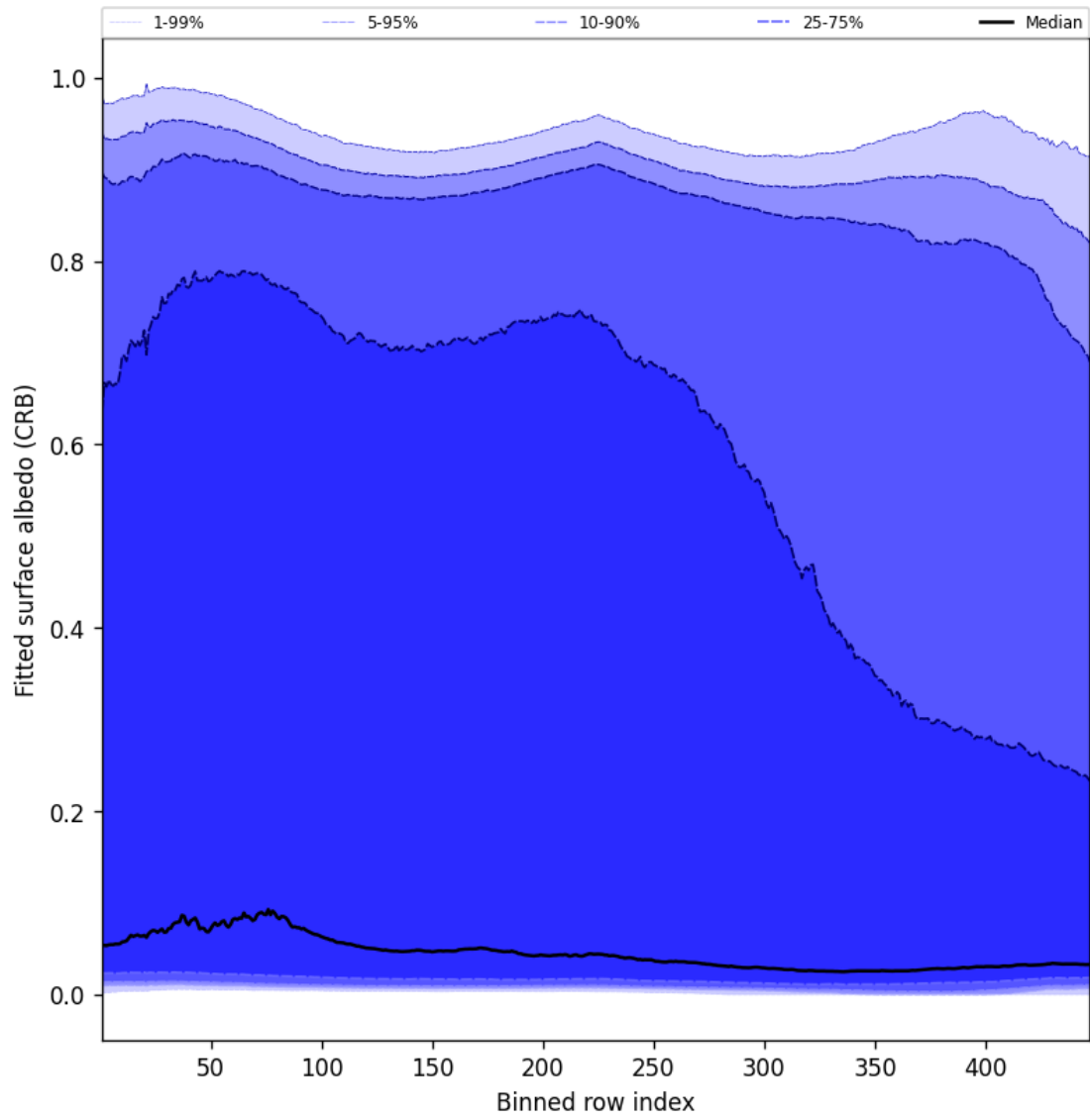
Figure 62: Along track statistics of “Fitted surface albedo (CRB)” for 2025-11-13 to 2025-11-15
