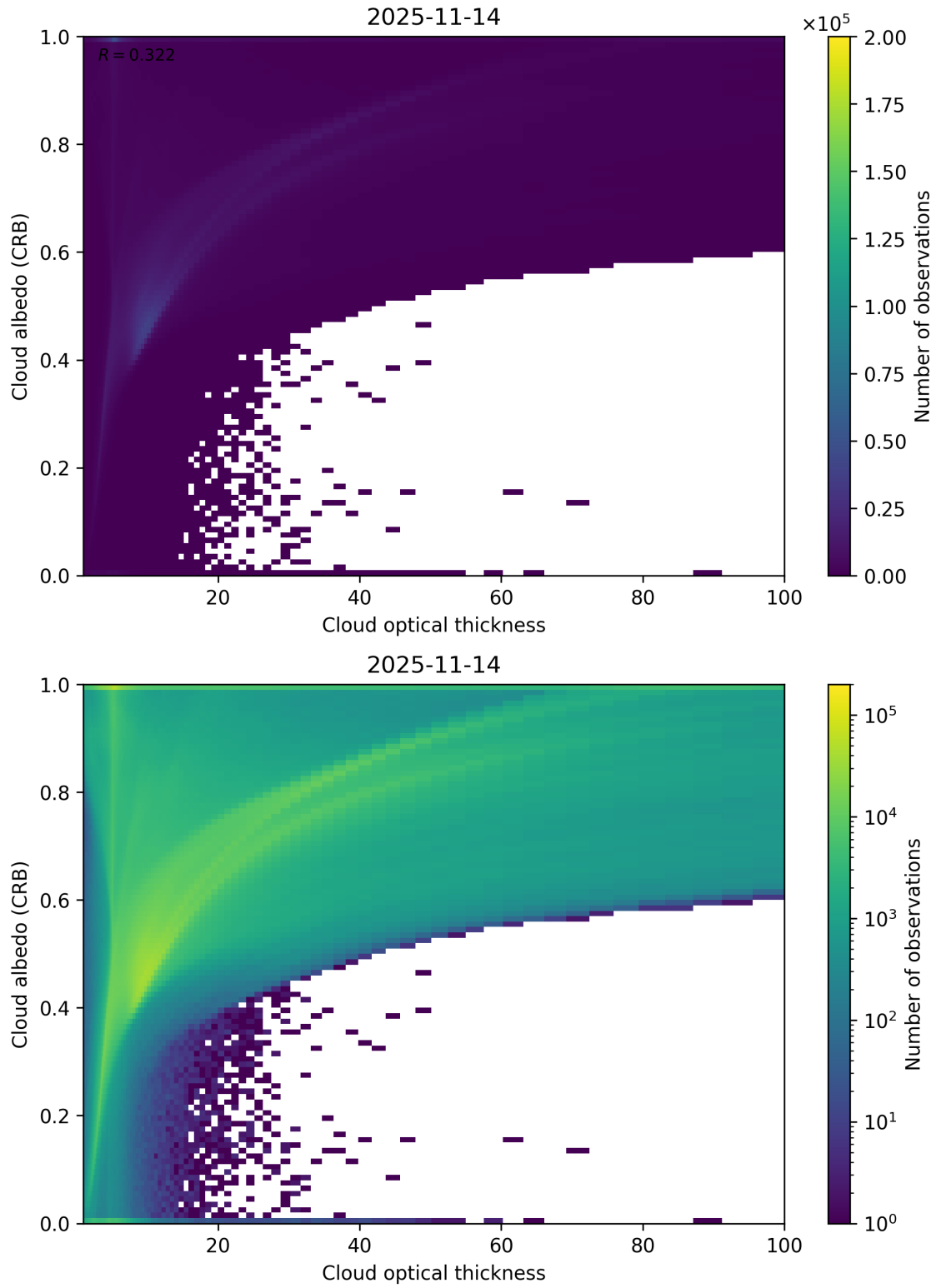
Figure 82: Scatter density plot of “Cloud optical thickness” against “Cloud albedo (CRB)” for 2025-11-13 to 2025-11-15.
