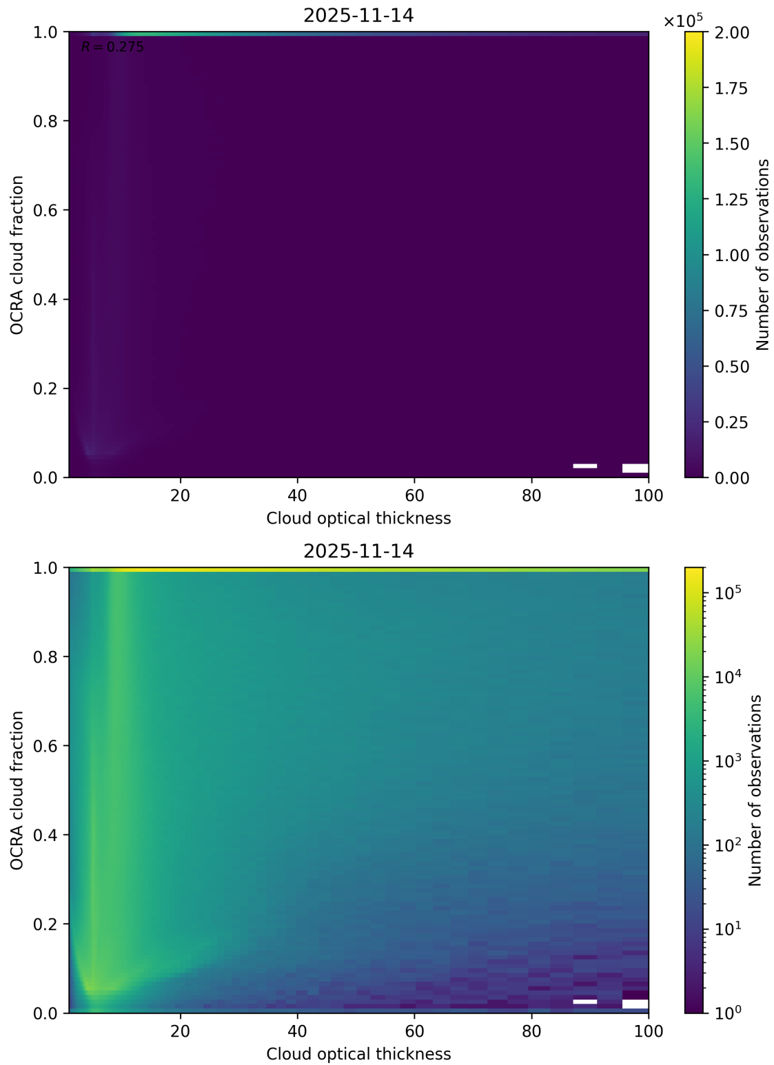
Figure 83: Scatter density plot of “Cloud optical thickness” against “OCRA cloud fraction” for 2025-11-13 to 2025-11-15.
