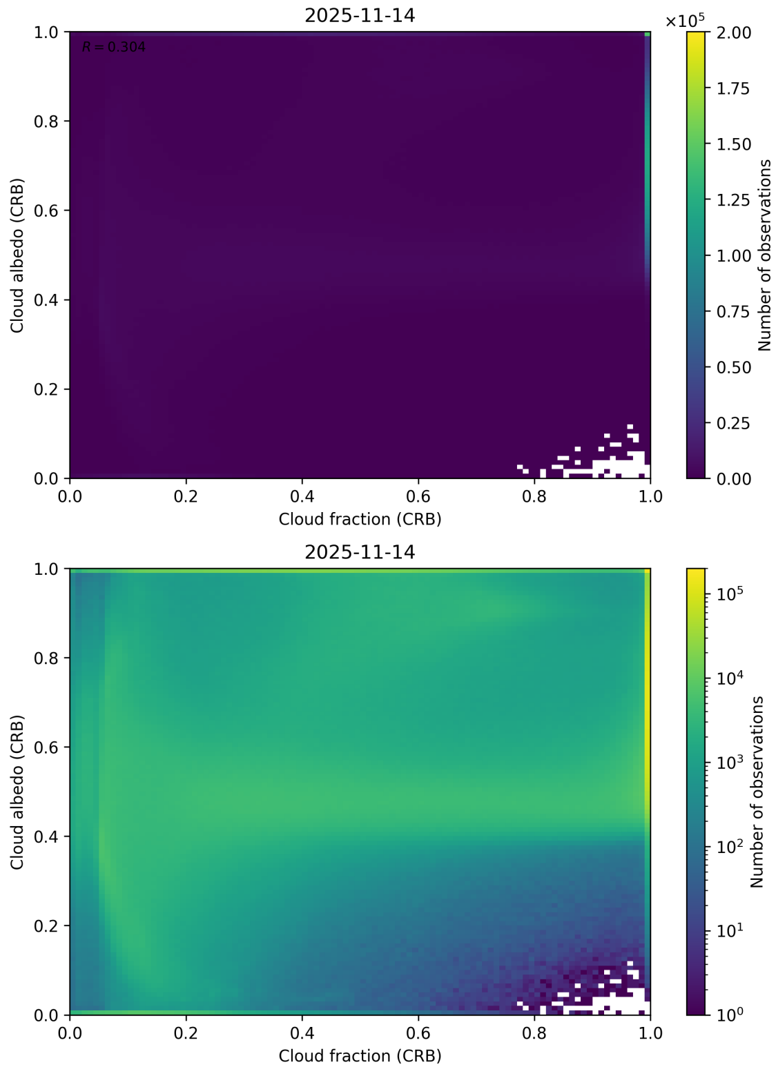
Figure 77: Scatter density plot of “Cloud fraction (CRB)” against “Cloud albedo (CRB)” for 2025-11-13 to 2025-11-15.
