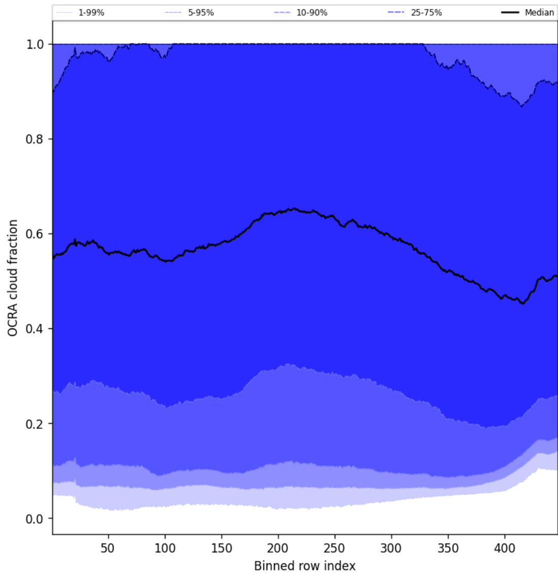
Figure 66: Along track statistics of “OCRA cloud fraction” for 2025-11-13 to 2025-11-15
