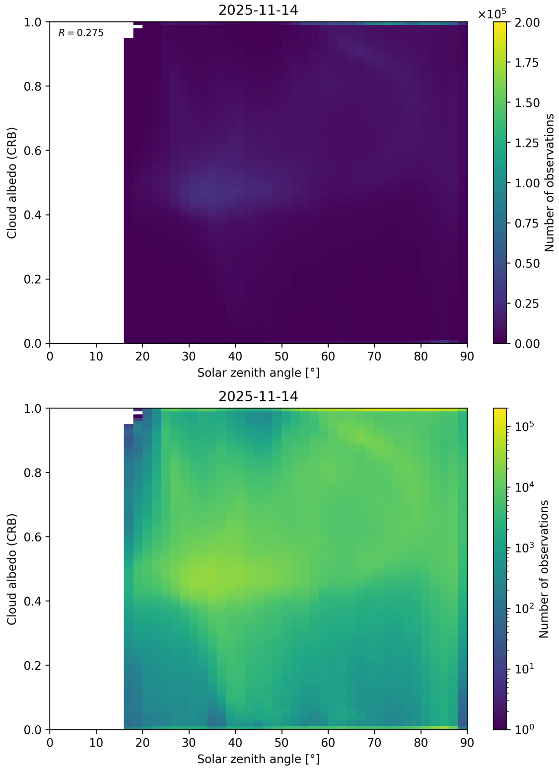
Figure 98: Scatter density plot of “Solar zenith angle” against “Cloud albedo (CRB)” for 2025-11-13 to 2025-11-15.
