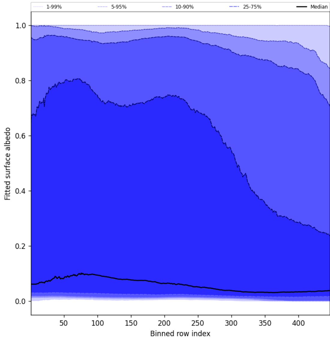
Figure 61: Along track statistics of “Fitted surface albedo” for 2025-11-13 to 2025-11-15
