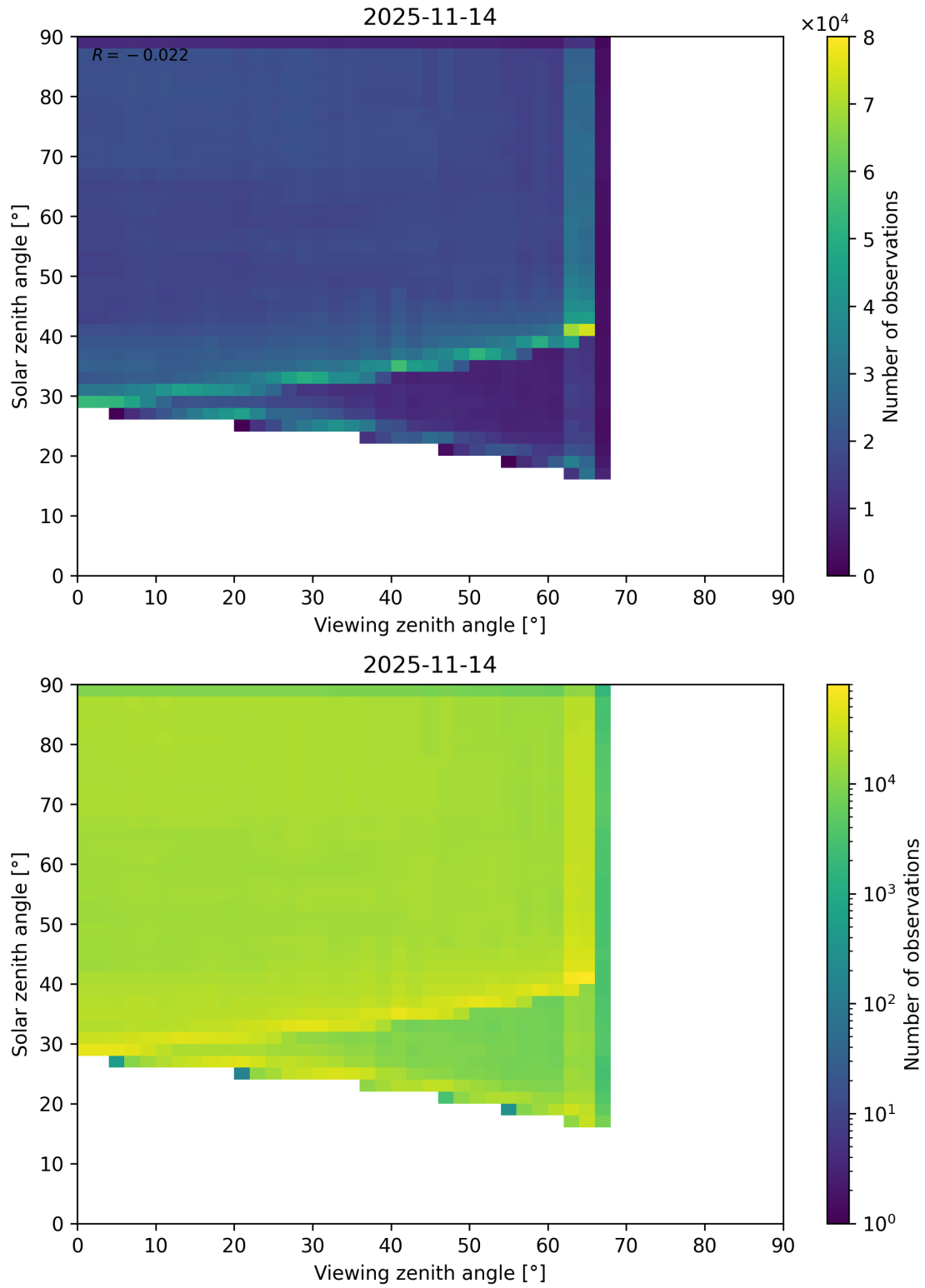
Figure 114: Scatter density plot of “Viewing zenith angle” against “Solar zenith angle” for 2025-11-13 to 2025-11-15.
