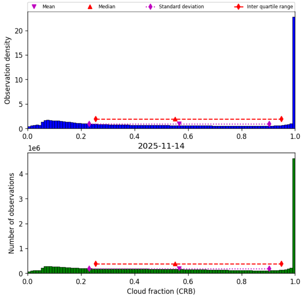
Figure 42: Histogram of “Cloud fraction (CRB)” for 2025-11-13 to 2025-11-15
