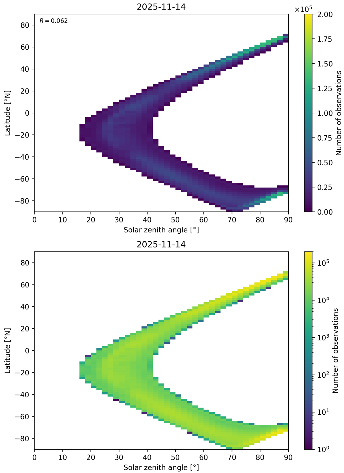
Figure 105: Scatter density plot of “Solar zenith angle” against “Latitude” for 2025-11-13 to 2025-11-15.
