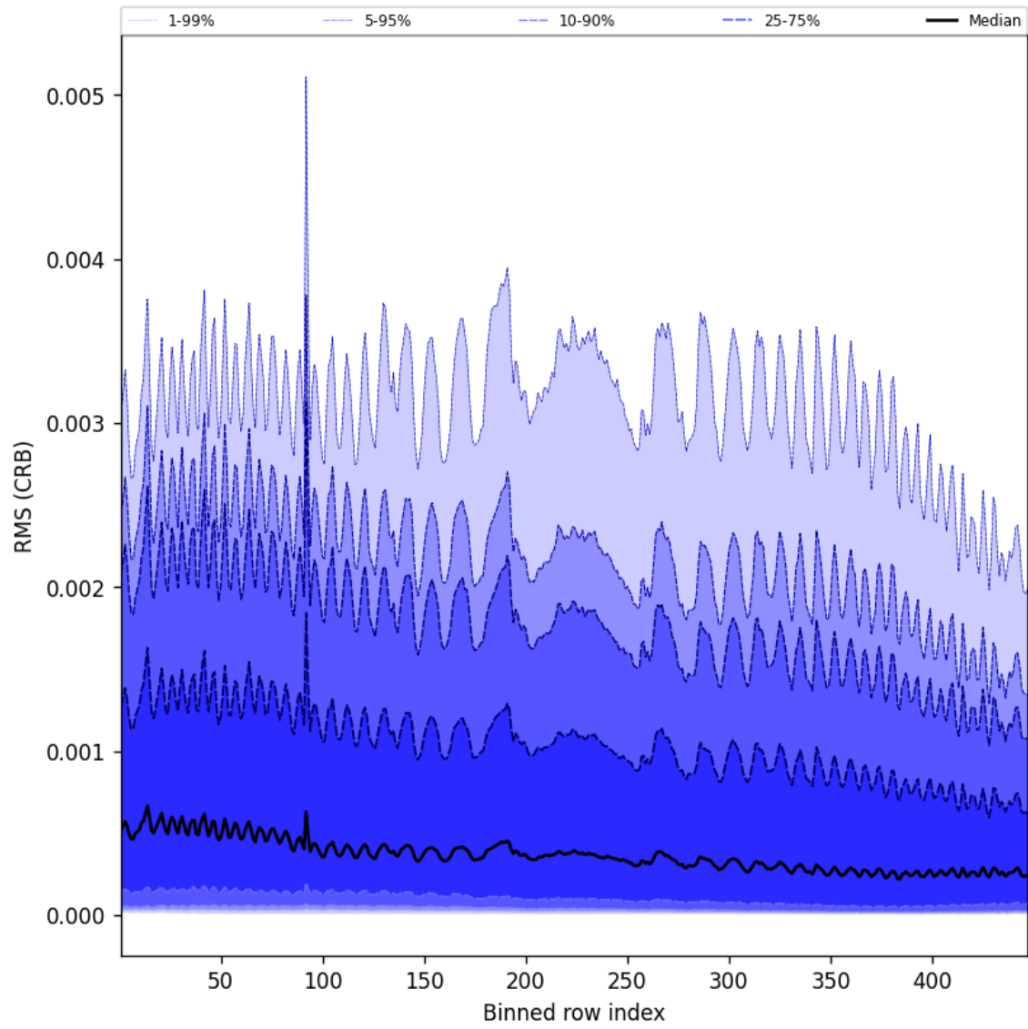
Figure 64: Along track statistics of “RMS (CRB)” for 2025-11-13 to 2025-11-15
