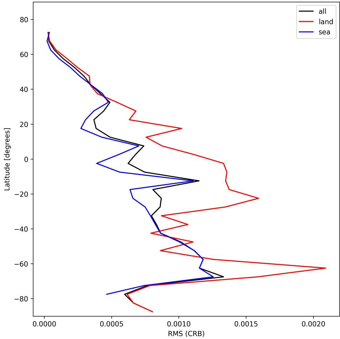
Figure 32: Zonal average of “RMS (CRB)” for 2025-11-13 to 2025-11-15.
