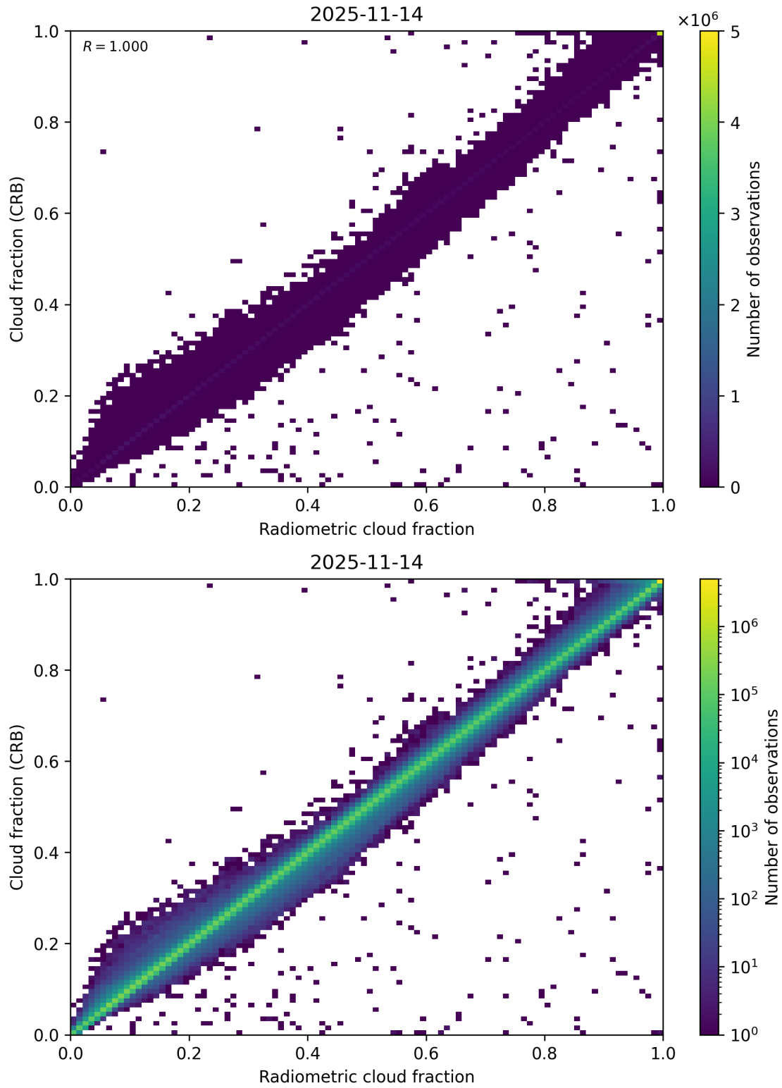
Figure 73: Scatter density plot of “Radiometric cloud fraction” against “Cloud fraction (CRB)” for 2025-11-13 to 2025-11-15.
