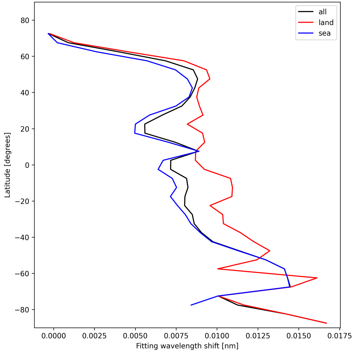
Figure 33: Zonal average of “Fitting wavelength shift” for 2025-11-13 to 2025-11-15.
