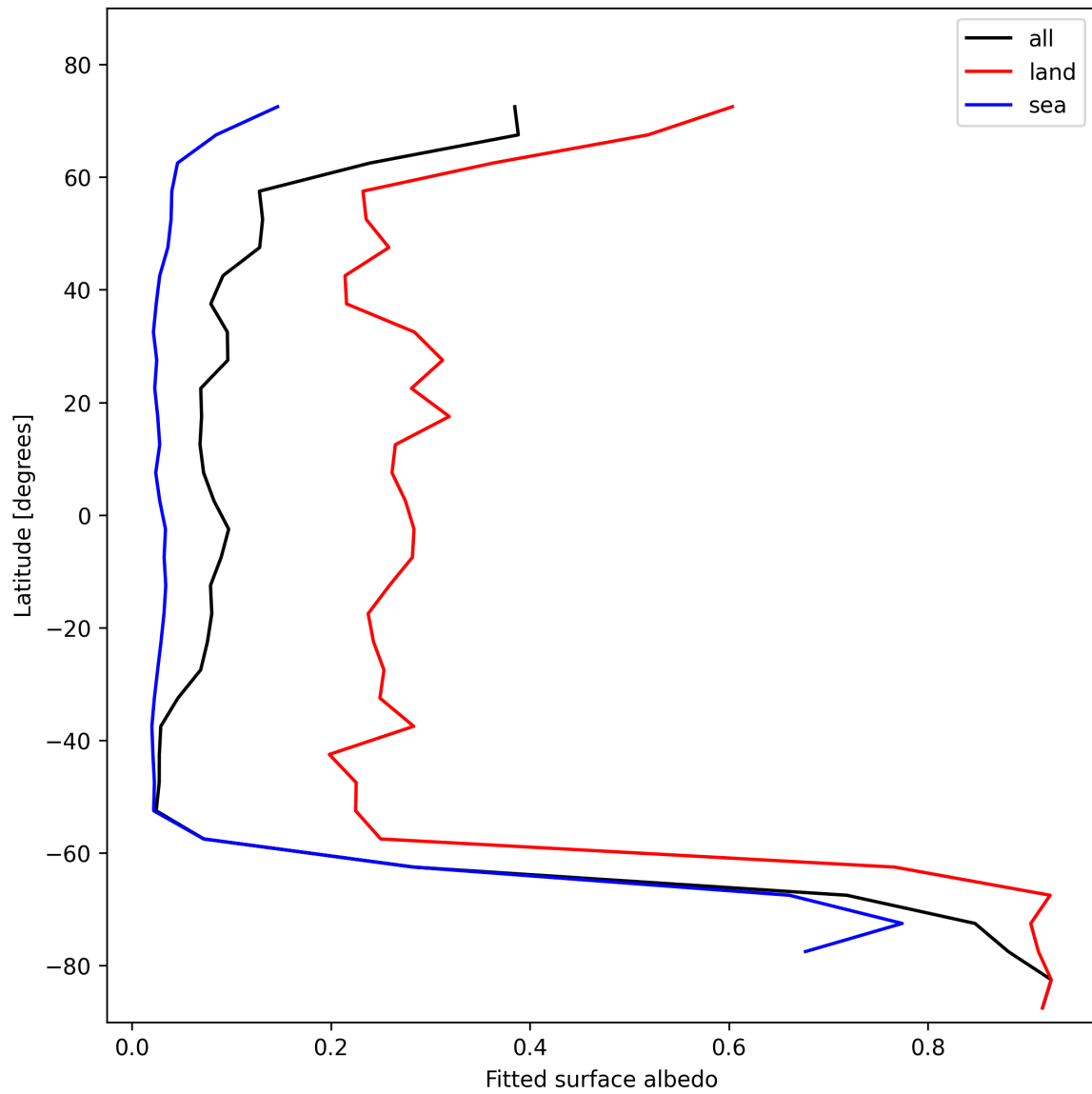
Figure 29: Zonal average of “Fitted surface albedo” for 2025-11-13 to 2025-11-15.
