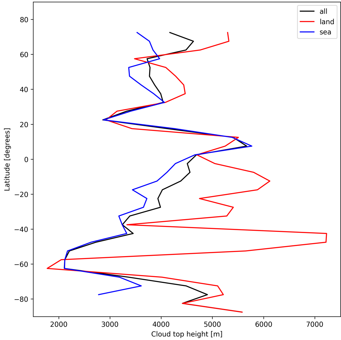
Figure 24: Zonal average of “Cloud top height” for 2025-11-13 to 2025-11-15.
