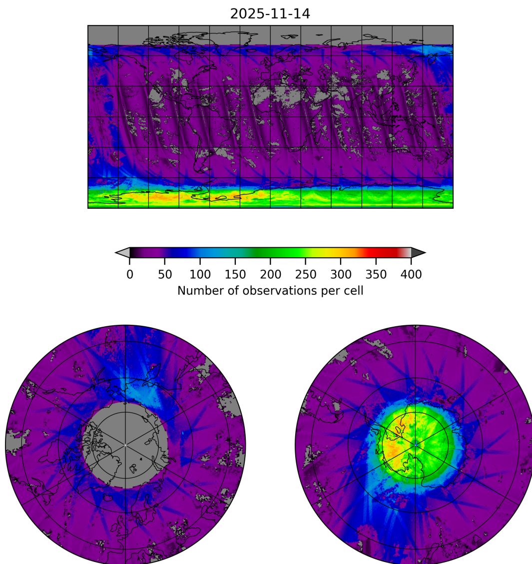
Figure 21: Map of the number of observations for 2025-11-13 to 2025-11-15
