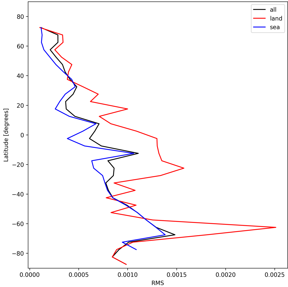
Figure 31: Zonal average of “RMS” for 2025-11-13 to 2025-11-15.
