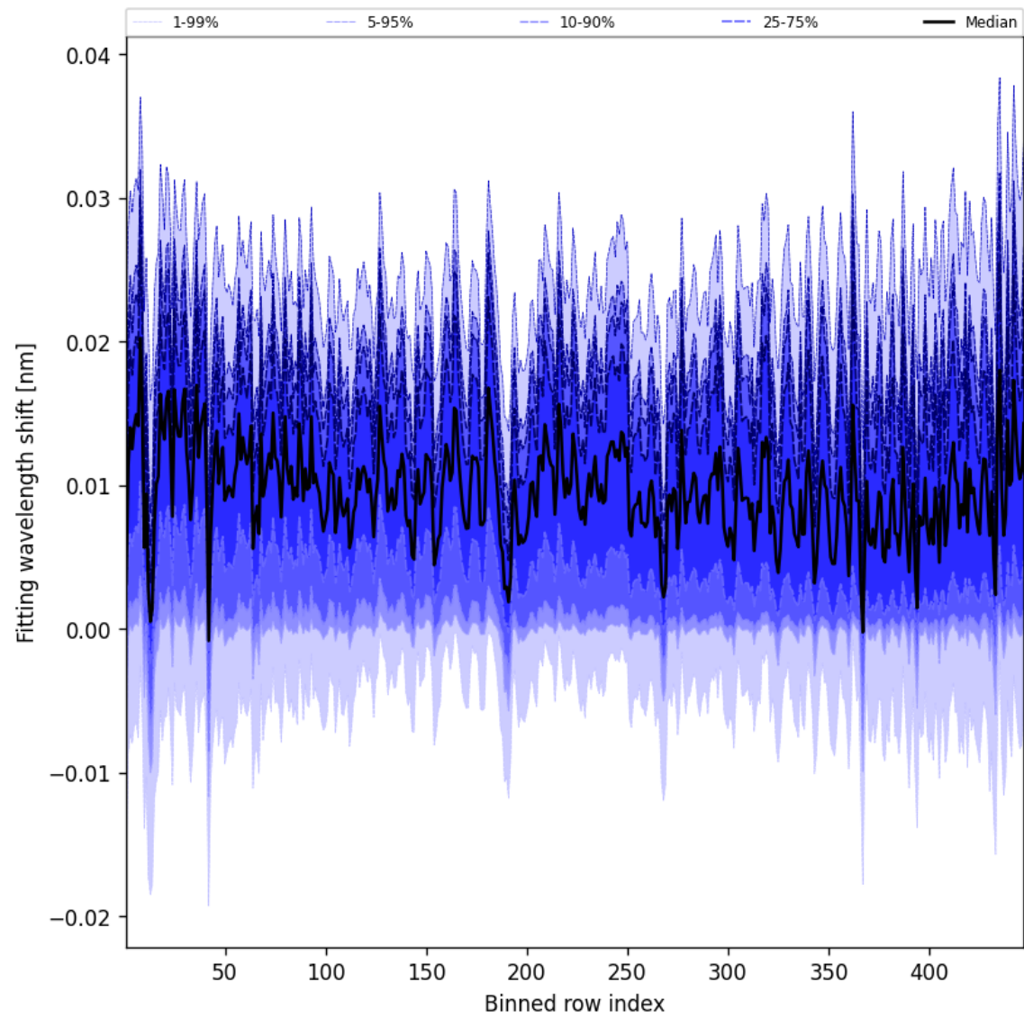
Figure 65: Along track statistics of “Fitting wavelength shift” for 2025-11-13 to 2025-11-15
