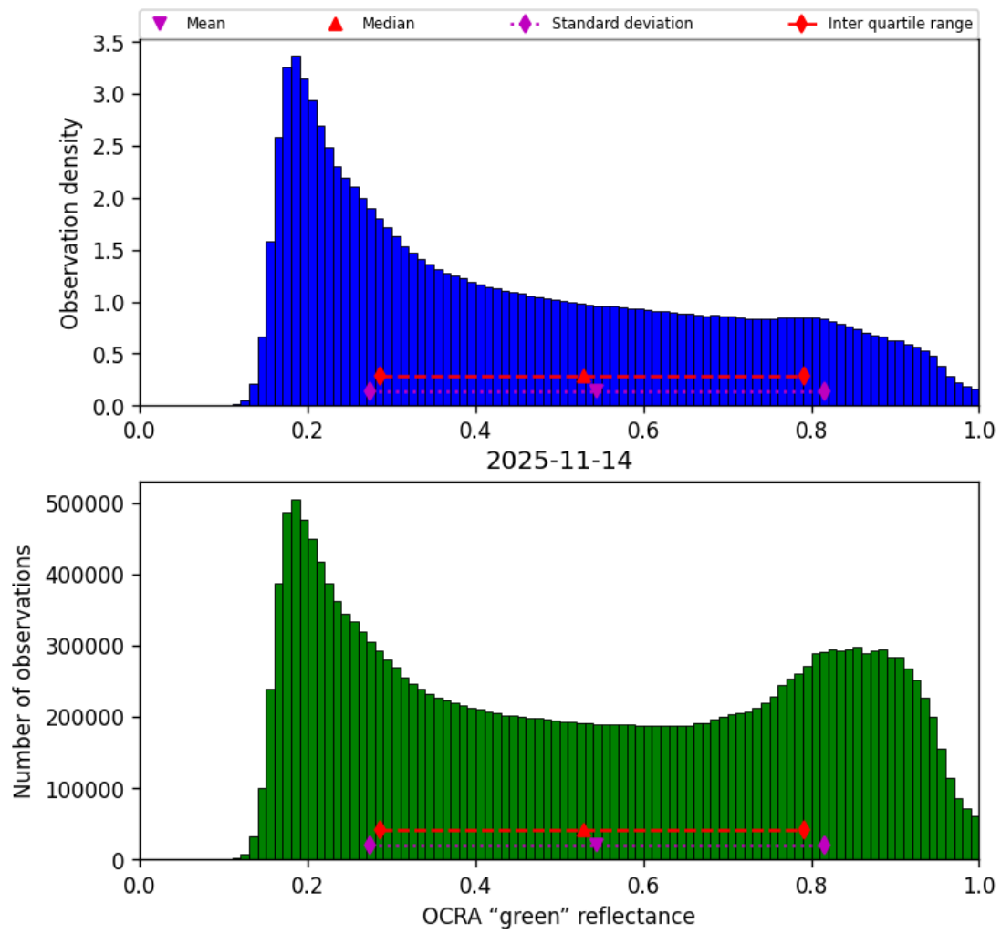
Figure 52: Histogram of “OCRA “green” reflectance” for 2025-11-13 to 2025-11-15
