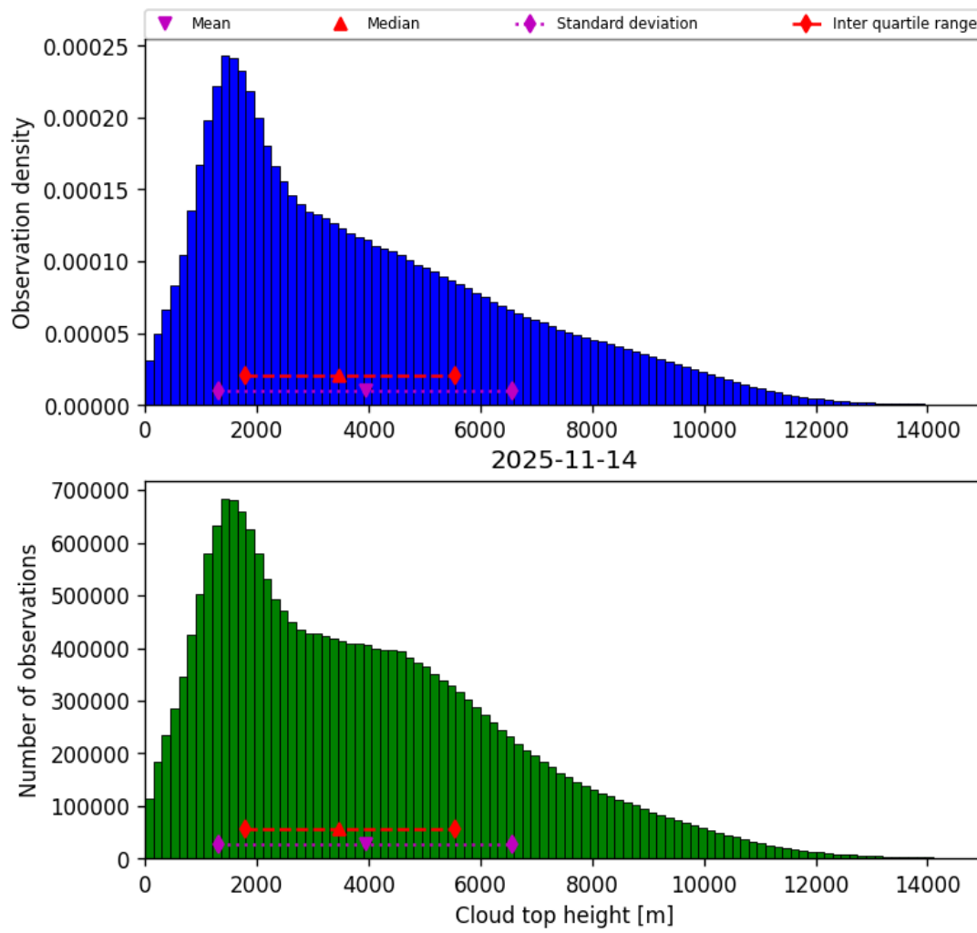
Figure 40: Histogram of “Cloud top height” for 2025-11-13 to 2025-11-15
