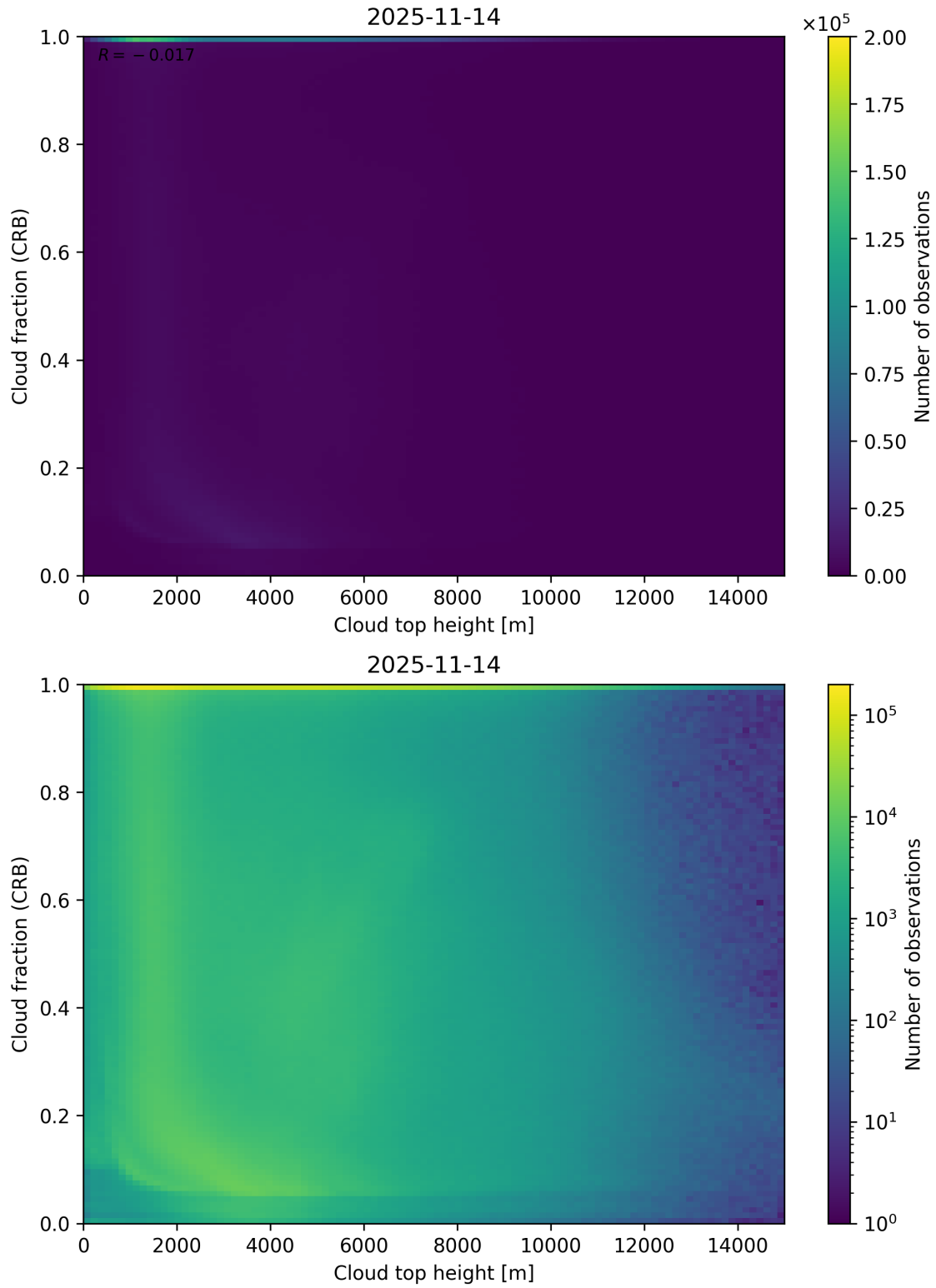
Figure 88: Scatter density plot of “Cloud top height” against “Cloud fraction (CRB)” for 2025-11-13 to 2025-11-15.
