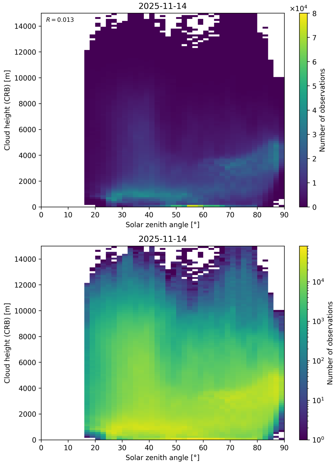
Figure 102: Scatter density plot of “Solar zenith angle” against “Cloud height (CRB)” for 2025-11-13 to 2025-11-15.
