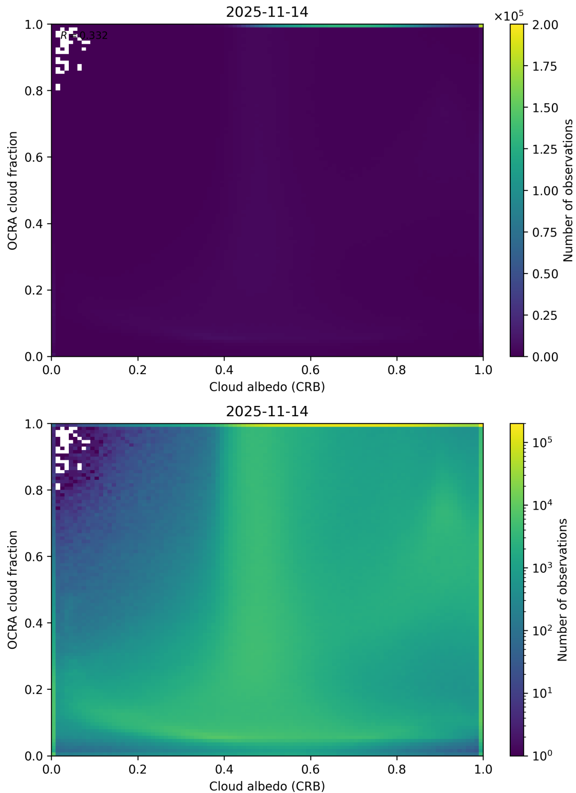
Figure 70: Scatter density plot of “Cloud albedo (CRB)” against “OCRA cloud fraction” for 2025-11-13 to 2025-11-15.
