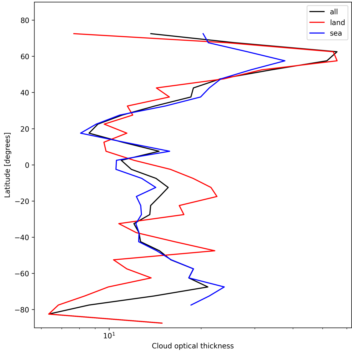
Figure 25: Zonal average of “Cloud optical thickness” for 2025-11-13 to 2025-11-15.
