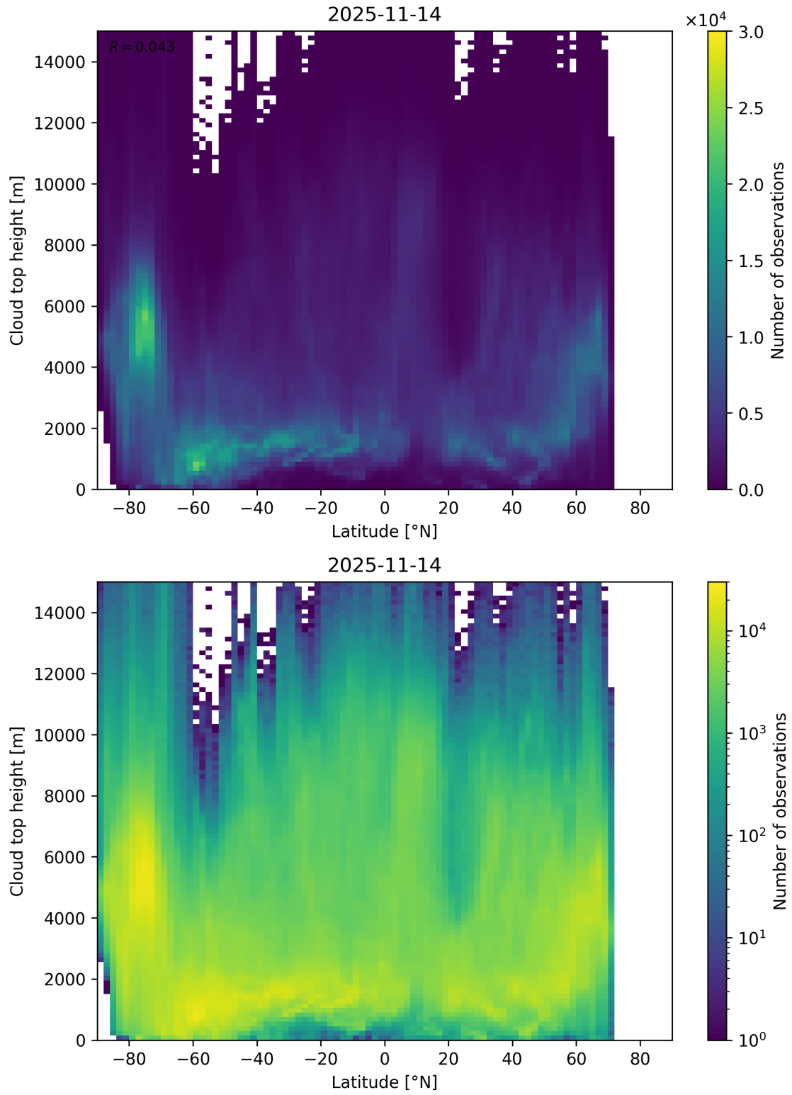
Figure 97: Scatter density plot of “Latitude” against “Cloud top height” for 2025-11-13 to 2025-11-15.
