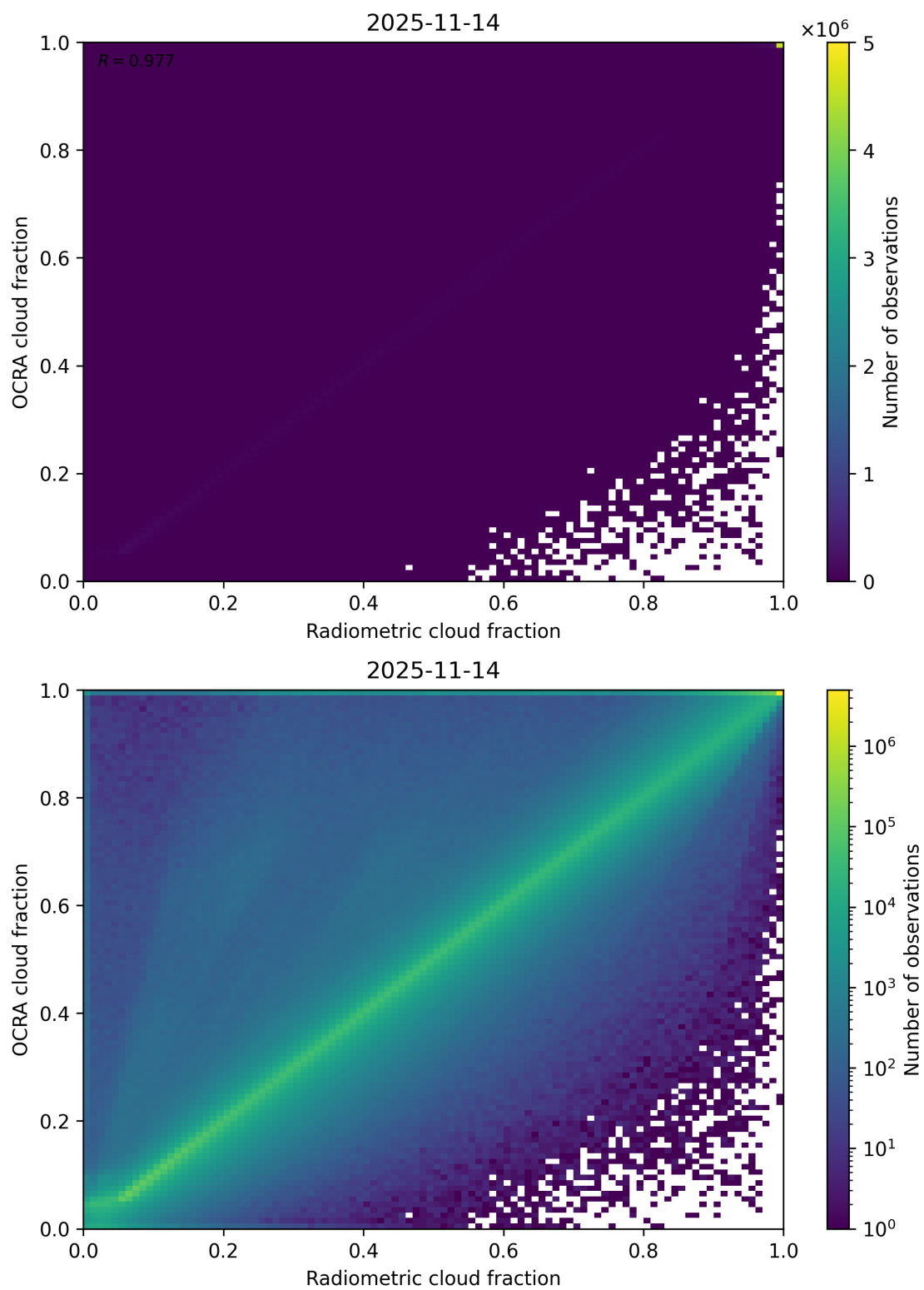
Figure 72: Scatter density plot of “Radiometric cloud fraction” against “OCRA cloud fraction” for 2025-11-13 to 2025-11-15.
