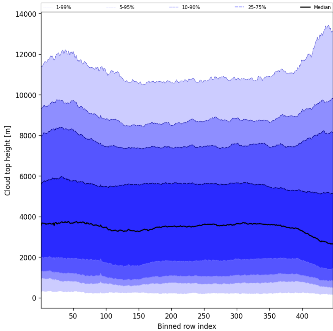
Figure 56: Along track statistics of “Cloud top height” for 2025-11-13 to 2025-11-15
