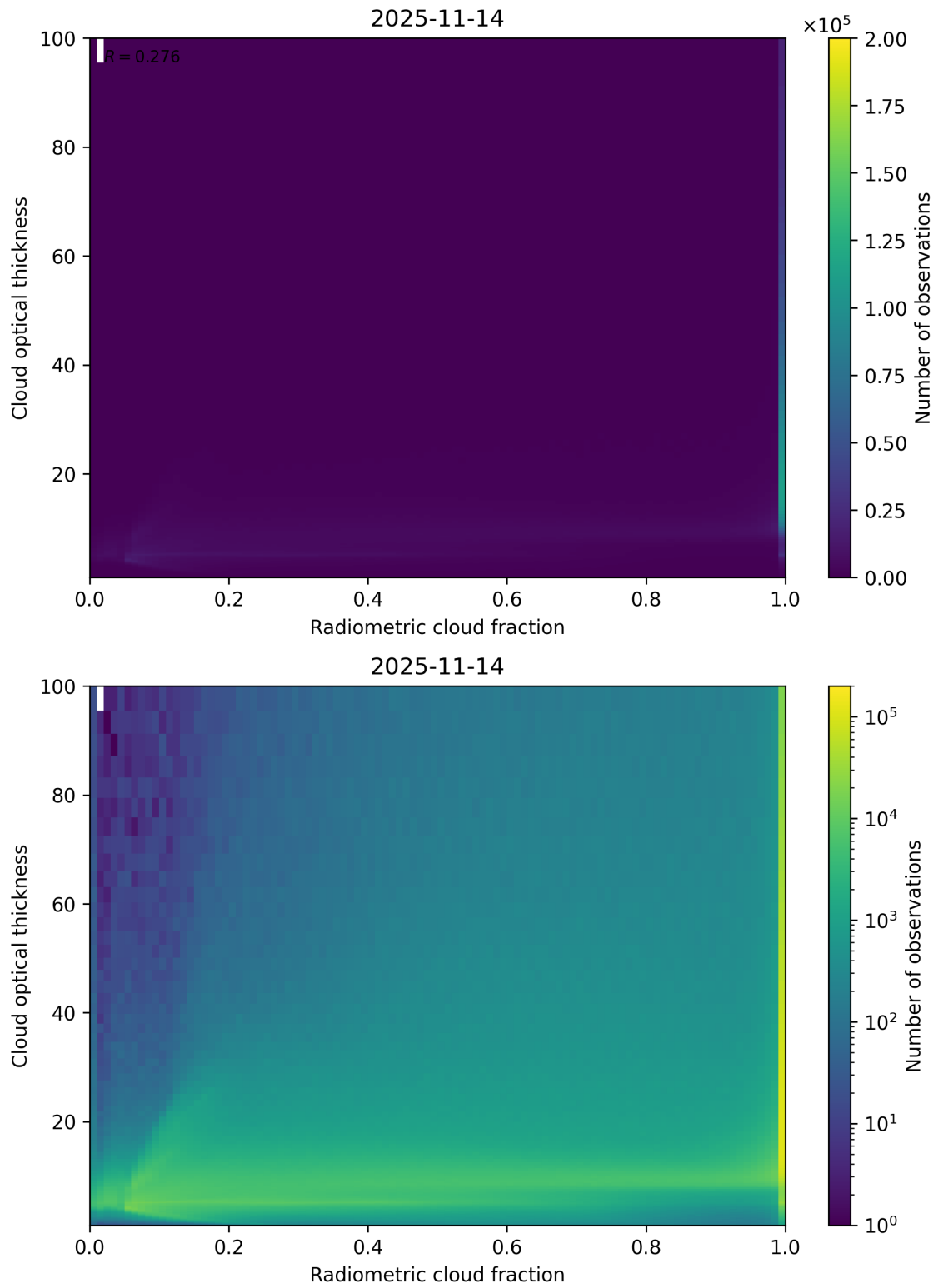
Figure 75: Scatter density plot of “Radiometric cloud fraction” against “Cloud optical thickness” for 2025-11-13 to 2025-11-15.
