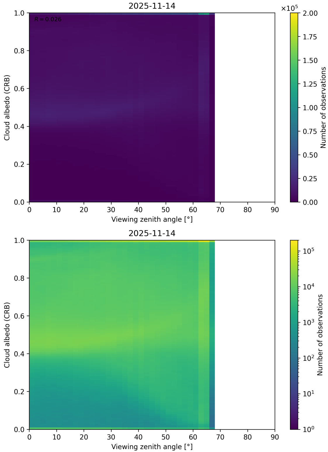
Figure 106: Scatter density plot of “Viewing zenith angle” against “Cloud albedo (CRB)” for 2025-11-13 to 2025-11-15.
