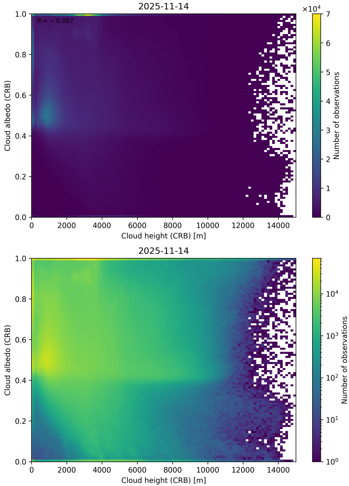
Figure 80: Scatter density plot of “Cloud height (CRB)” against “Cloud albedo (CRB)” for 2025-11-13 to 2025-11-15.
