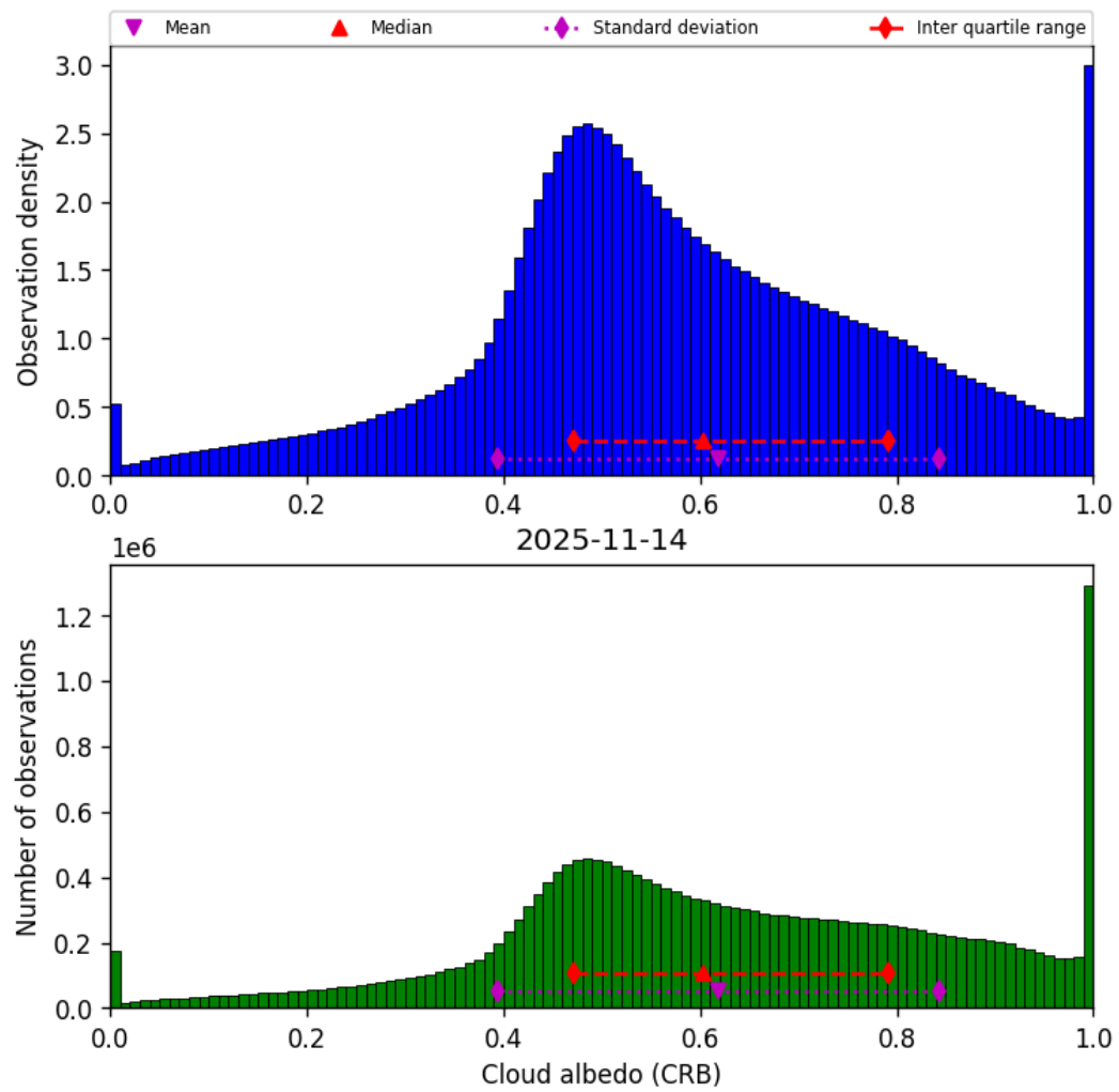
Figure 44: Histogram of “Cloud albedo (CRB)” for 2025-11-13 to 2025-11-15
