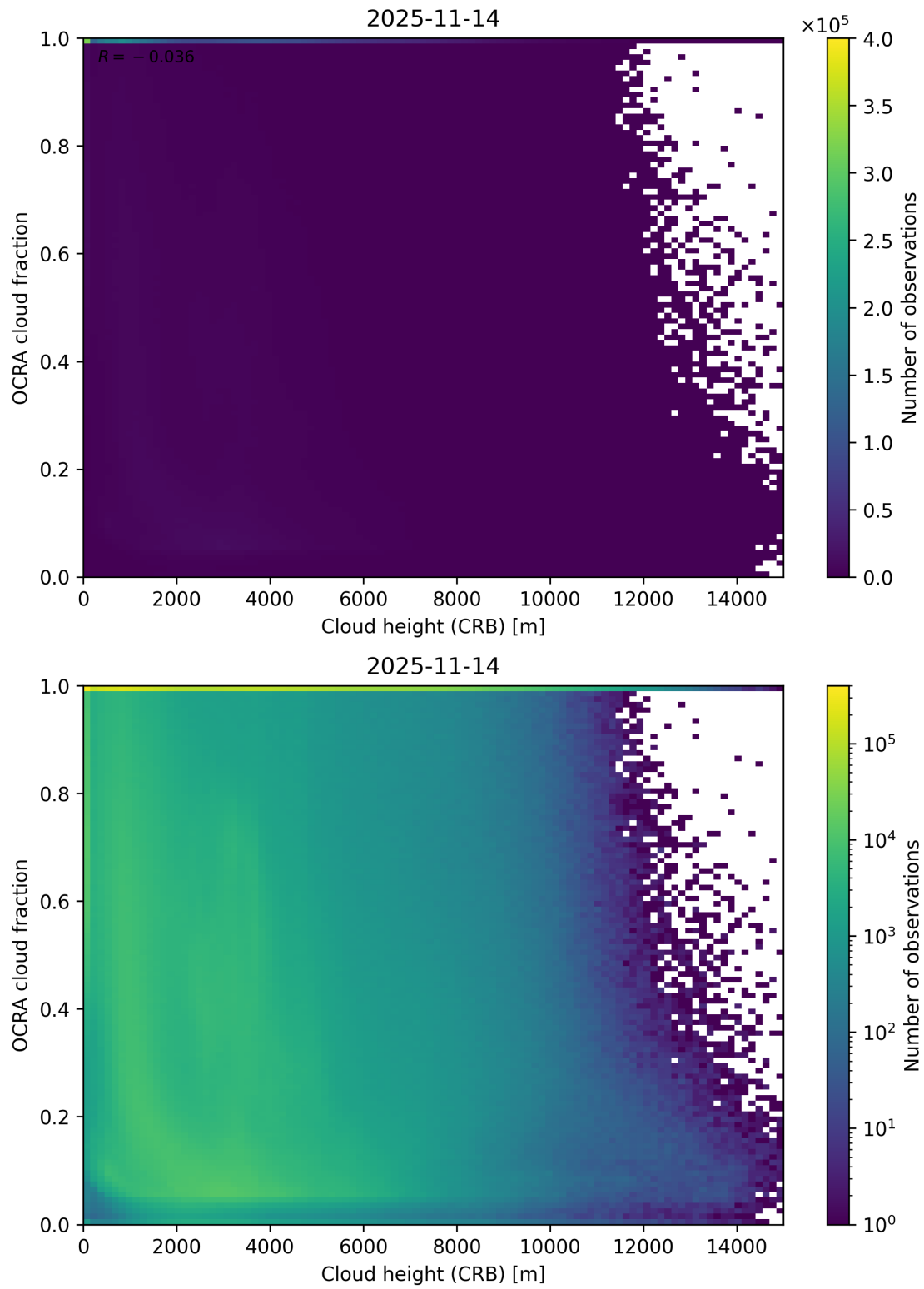
Figure 81: Scatter density plot of “Cloud height (CRB)” against “OCRA cloud fraction” for 2025-11-13 to 2025-11-15.
