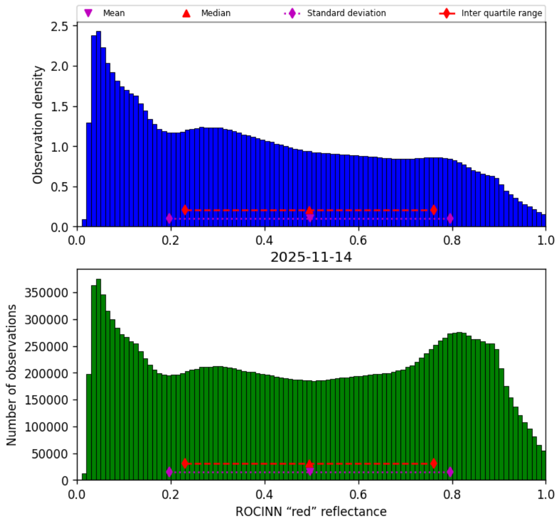
Figure 53: Histogram of “ROCINN “red” reflectance” for 2025-11-13 to 2025-11-15
