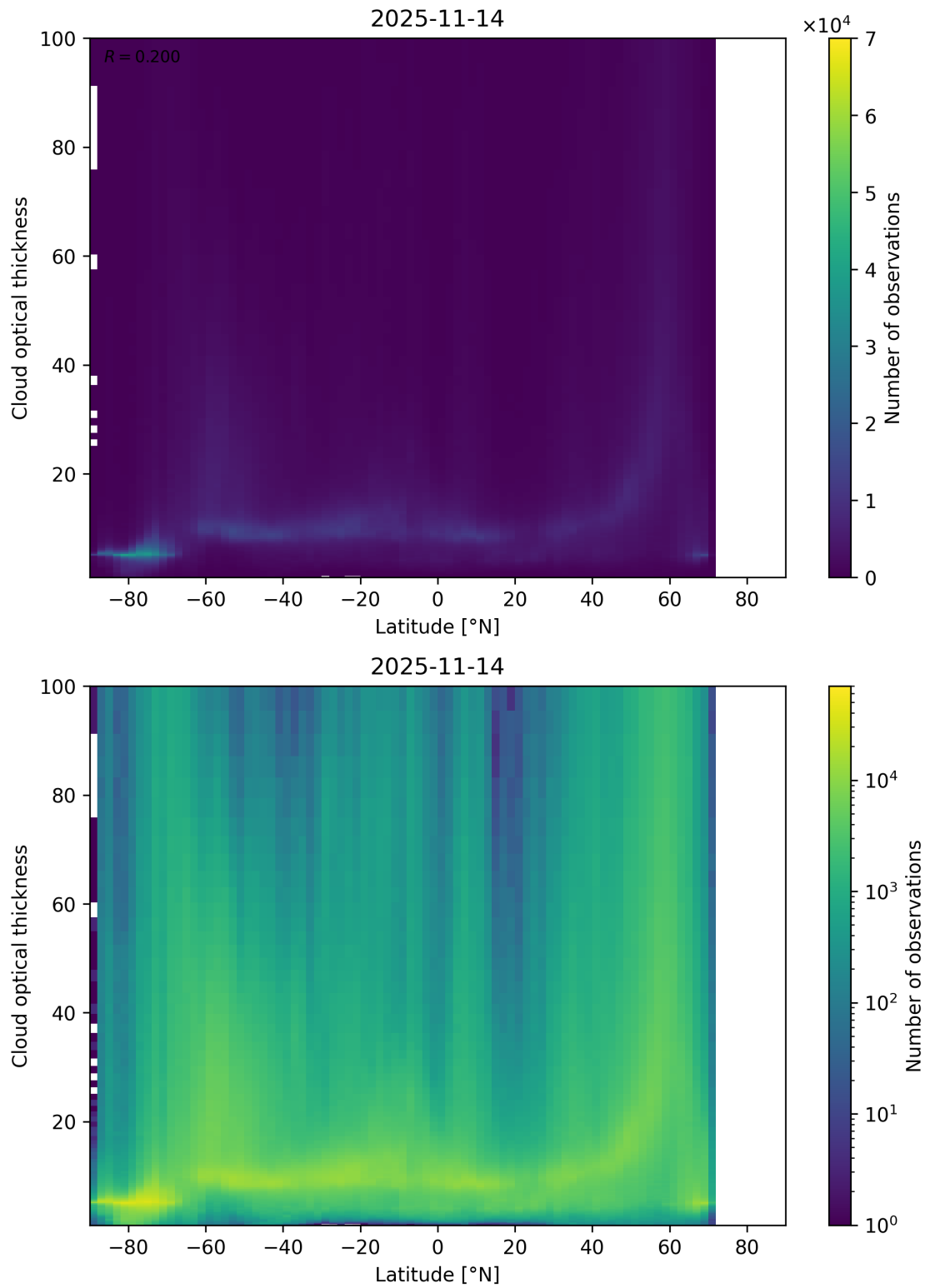
Figure 96: Scatter density plot of “Latitude” against “Cloud optical thickness” for 2025-11-13 to 2025-11-15.
