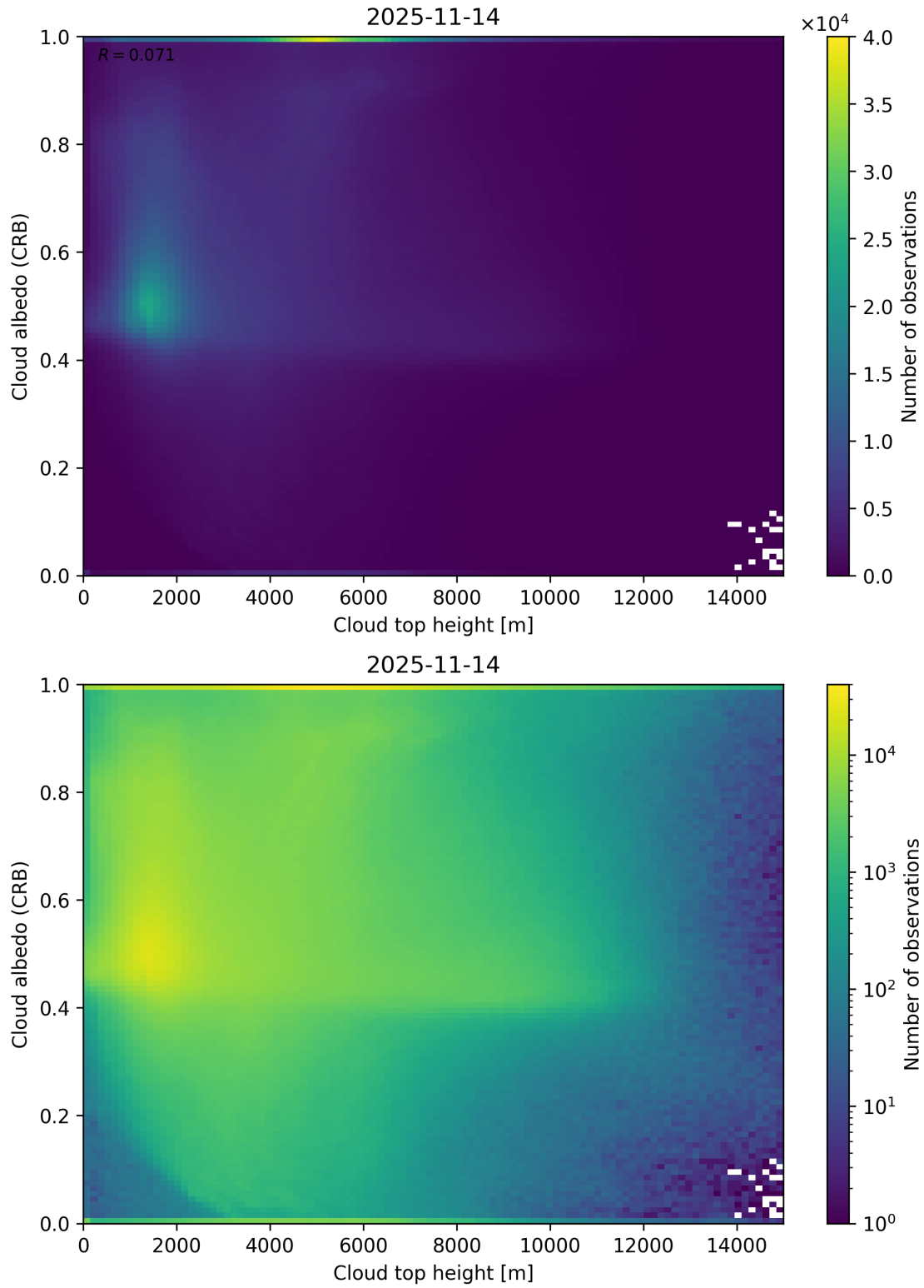
Figure 86: Scatter density plot of “Cloud top height” against “Cloud albedo (CRB)” for 2025-11-13 to 2025-11-15.
