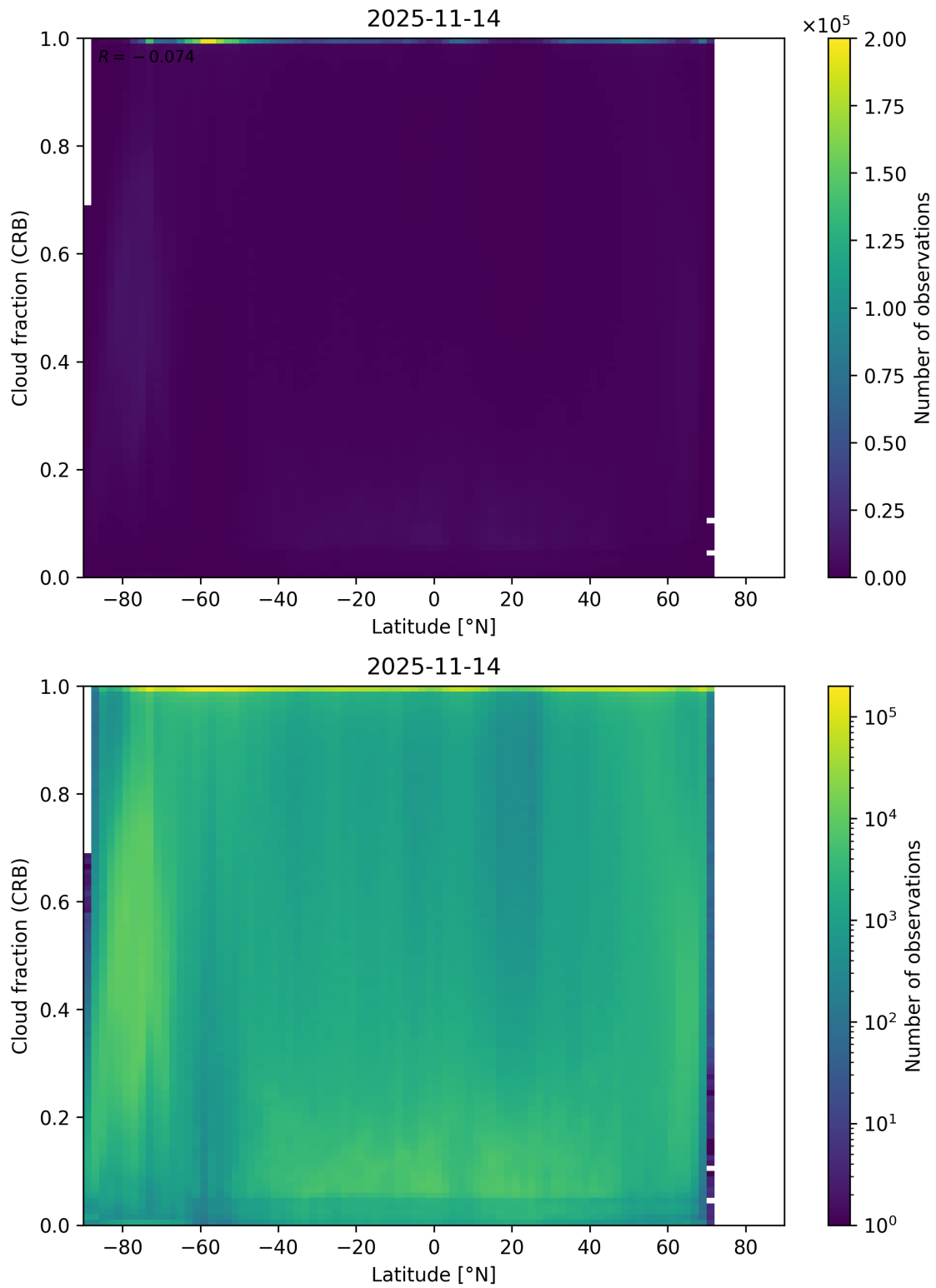
Figure 94: Scatter density plot of “Latitude” against “Cloud fraction (CRB)” for 2025-11-13 to 2025-11-15.
