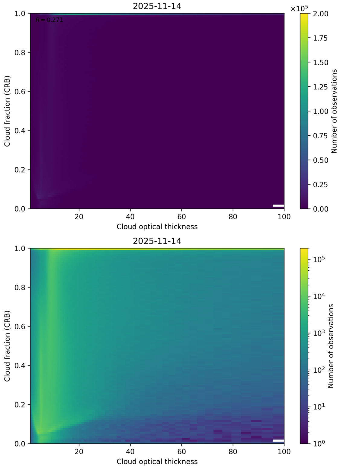
Figure 84: Scatter density plot of “Cloud optical thickness” against “Cloud fraction (CRB)” for 2025-11-13 to 2025-11-15.
