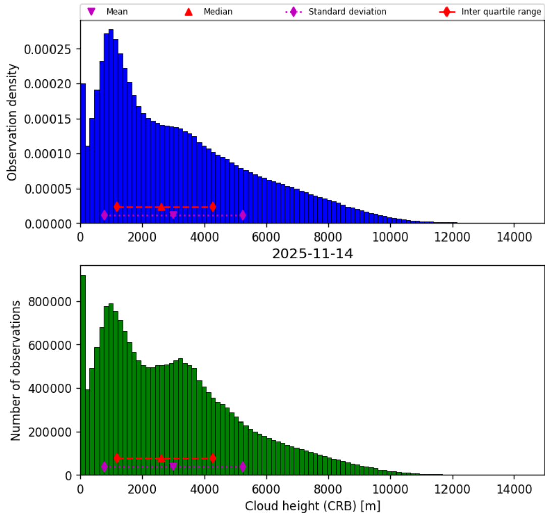
Figure 43: Histogram of “Cloud height (CRB)” for 2025-11-13 to 2025-11-15
