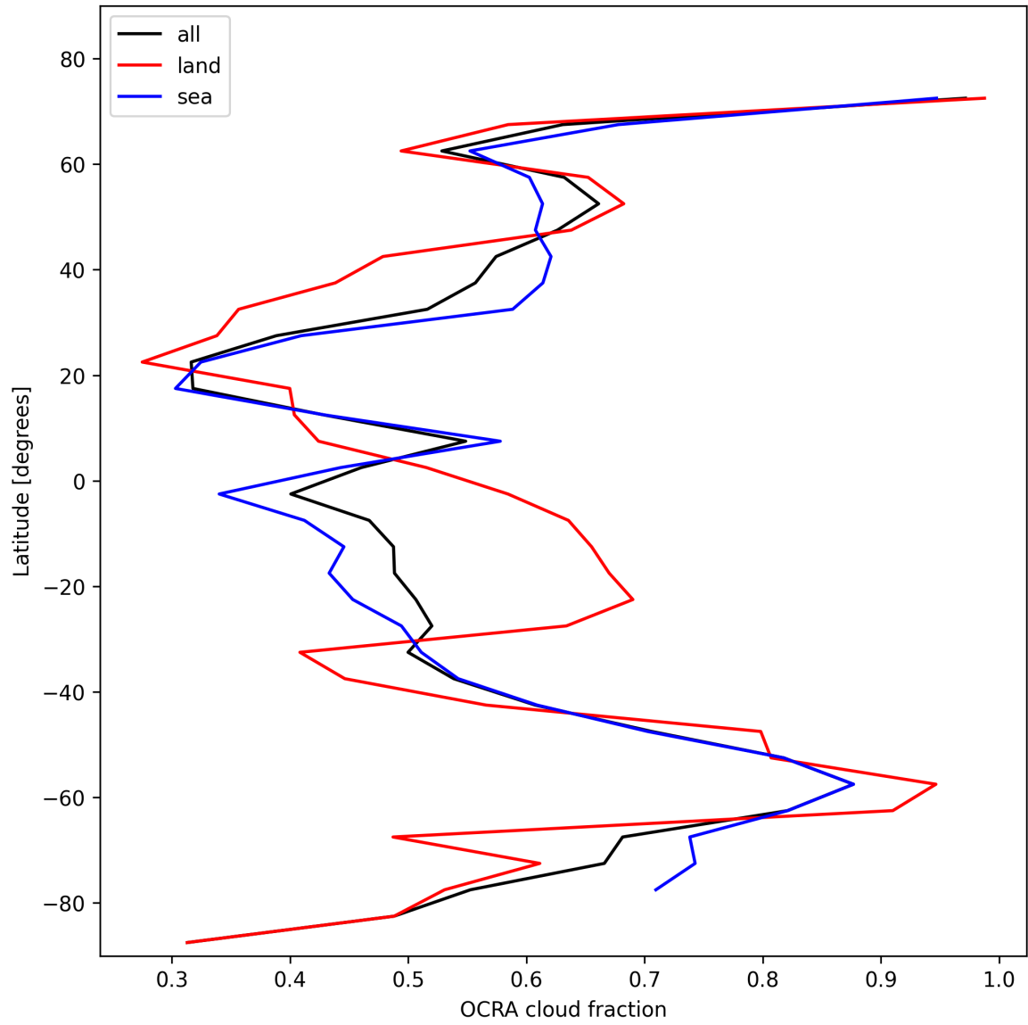
Figure 34: Zonal average of “OCRA cloud fraction” for 2025-11-13 to 2025-11-15.
