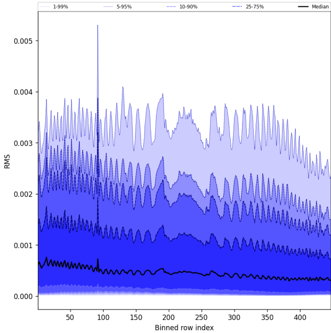
Figure 63: Along track statistics of “RMS” for 2025-11-13 to 2025-11-15
