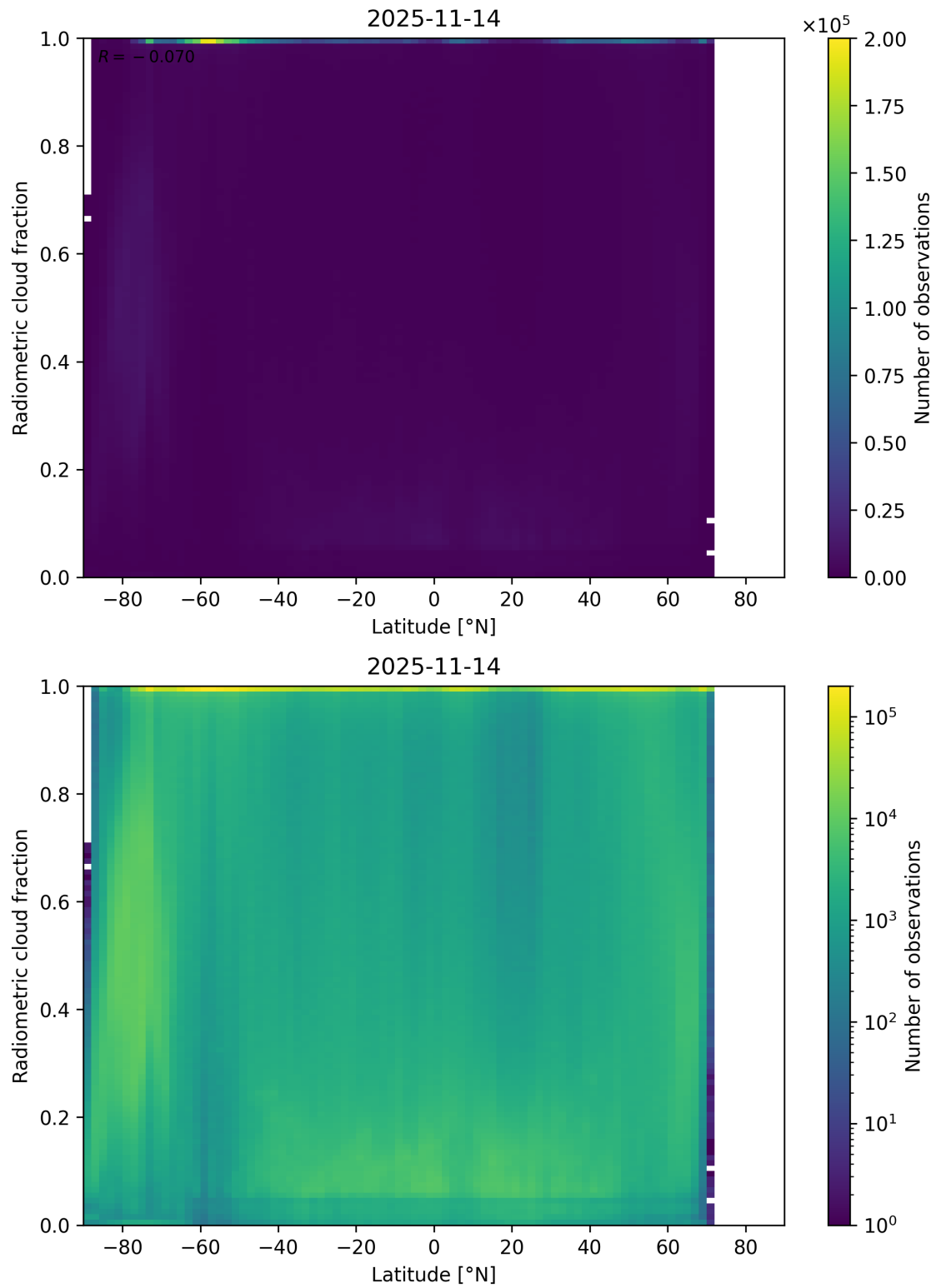
Figure 92: Scatter density plot of “Latitude” against “Radiometric cloud fraction” for 2025-11-13 to 2025-11-15.
