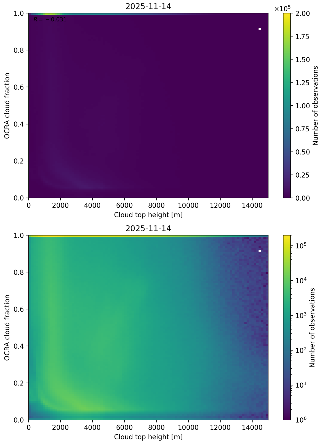
Figure 87: Scatter density plot of “Cloud top height” against “OCRA cloud fraction” for 2025-11-13 to 2025-11-15.
