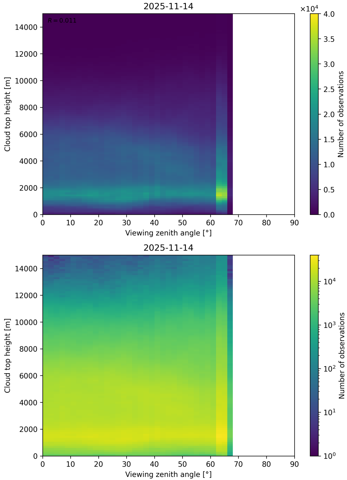
Figure 112: Scatter density plot of “Viewing zenith angle” against “Cloud top height” for 2025-11-13 to 2025-11-15.
