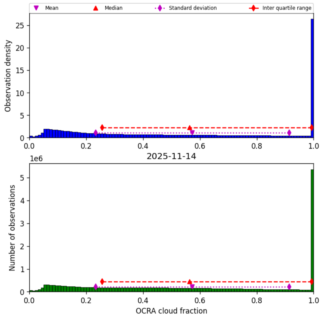
Figure 50: Histogram of “OCRA cloud fraction” for 2025-11-13 to 2025-11-15
