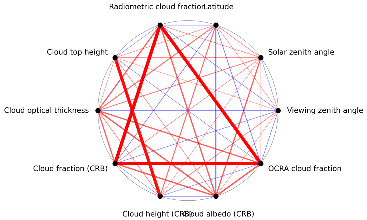
Figure 1: Map of correlation graph for 2025-11-13 to 2025-11-15.
