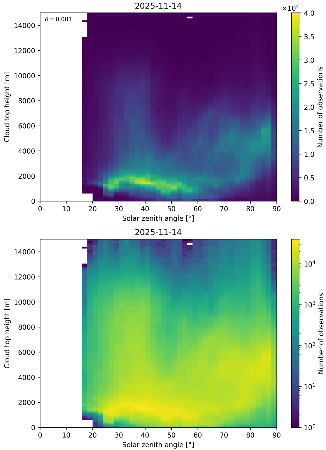
Figure 104: Scatter density plot of “Solar zenith angle” against “Cloud top height” for 2025-11-13 to 2025-11-15.
