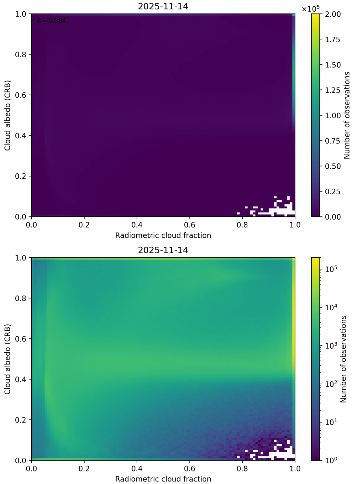
Figure 71: Scatter density plot of “Radiometric cloud fraction” against “Cloud albedo (CRB)” for 2025-11-13 to 2025-11-15.
