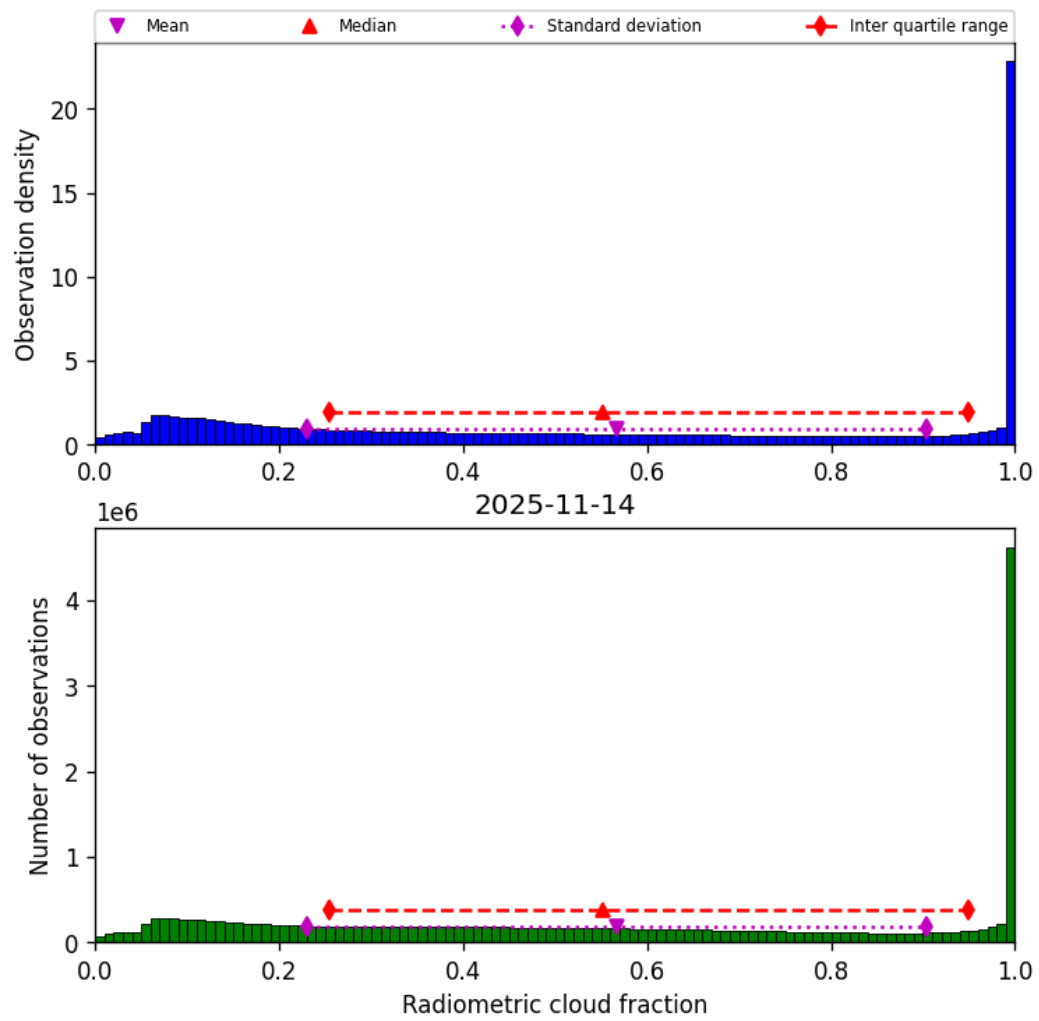
Figure 39: Histogram of “Radiometric cloud fraction” for 2025-11-13 to 2025-11-15
