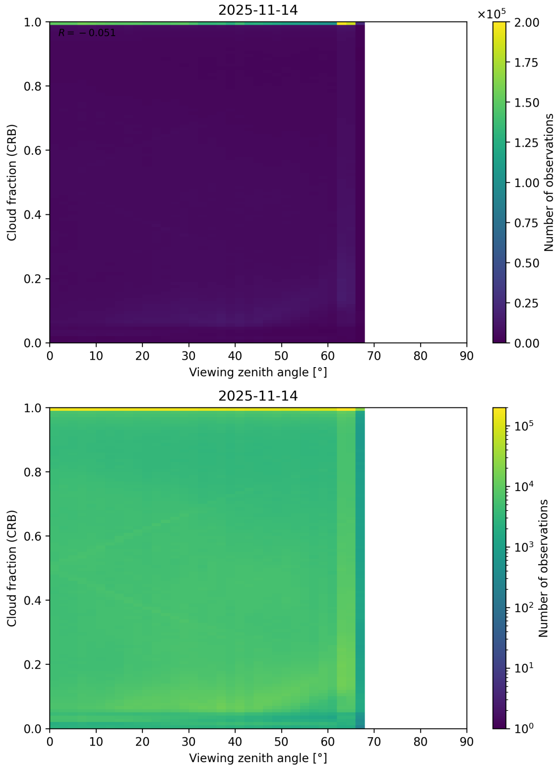
Figure 109: Scatter density plot of “Viewing zenith angle” against “Cloud fraction (CRB)” for 2025-11-13 to 2025-11-15.
