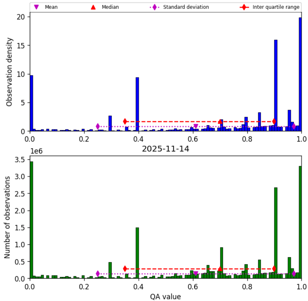
Figure 38: Histogram of “QA value” for 2025-11-13 to 2025-11-15
