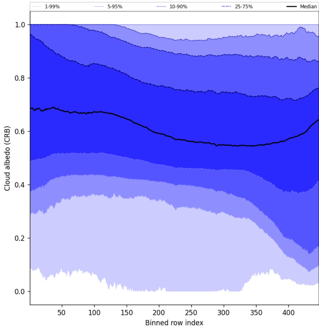
Figure 60: Along track statistics of “Cloud albedo (CRB)” for 2025-11-13 to 2025-11-15
