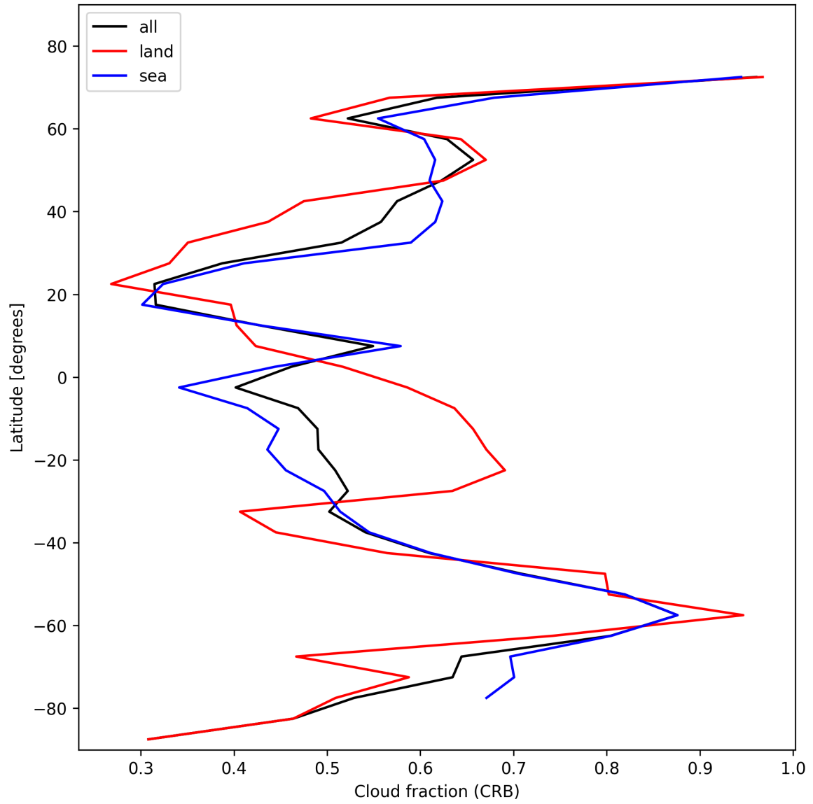
Figure 26: Zonal average of “Cloud fraction (CRB)” for 2025-11-13 to 2025-11-15.
