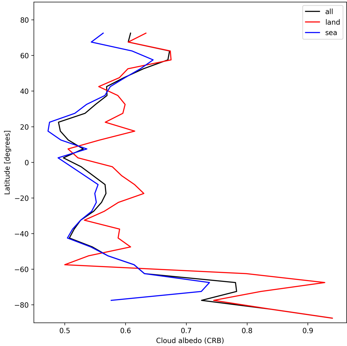
Figure 28: Zonal average of “Cloud albedo (CRB)” for 2025-11-13 to 2025-11-15.
