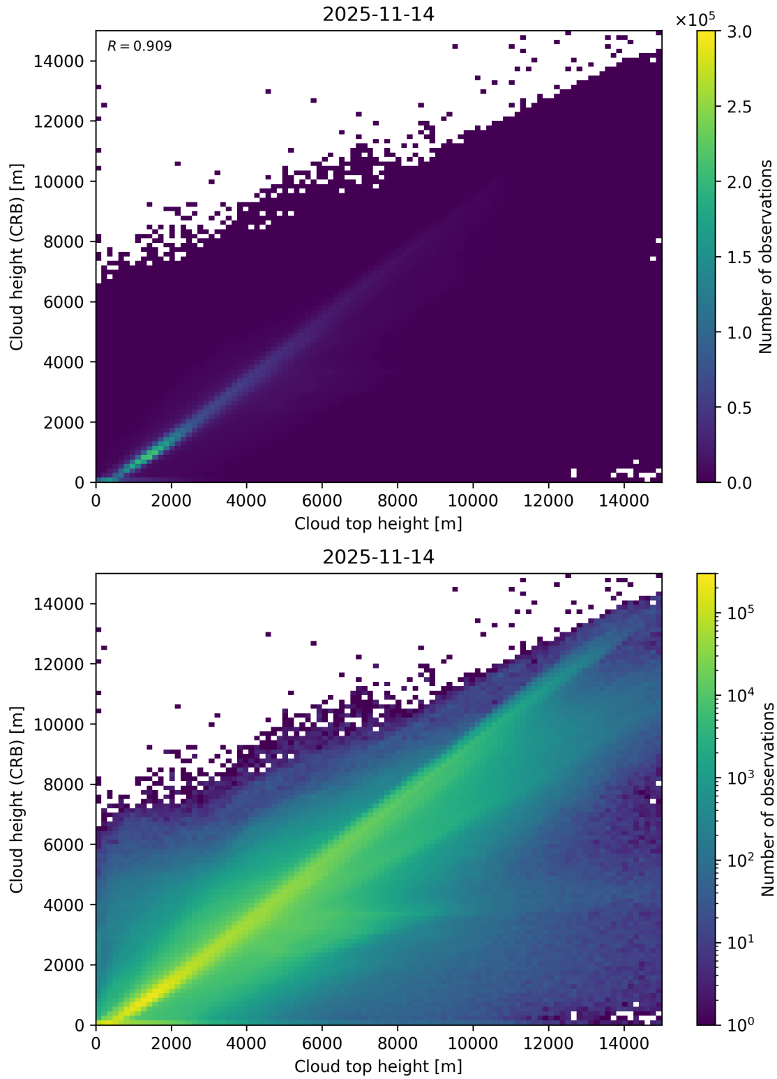
Figure 89: Scatter density plot of “Cloud top height” against “Cloud height (CRB)” for 2025-11-13 to 2025-11-15.
