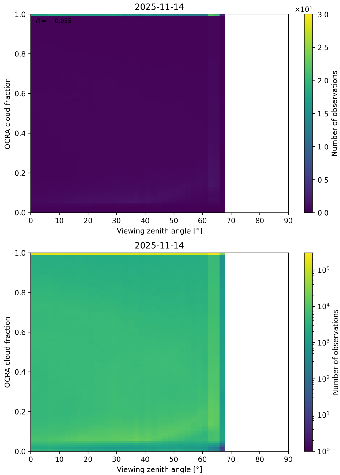
Figure 108: Scatter density plot of “Viewing zenith angle” against “OCRA cloud fraction” for 2025-11-13 to 2025-11-15.
