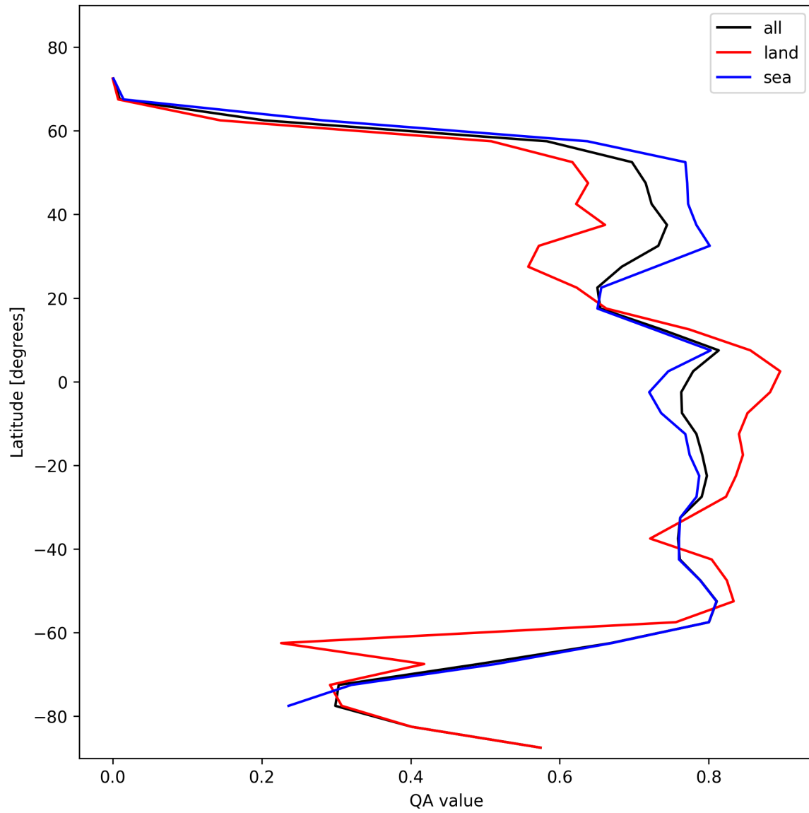
Figure 22: Zonal average of “QA value” for 2025-11-13 to 2025-11-15.
