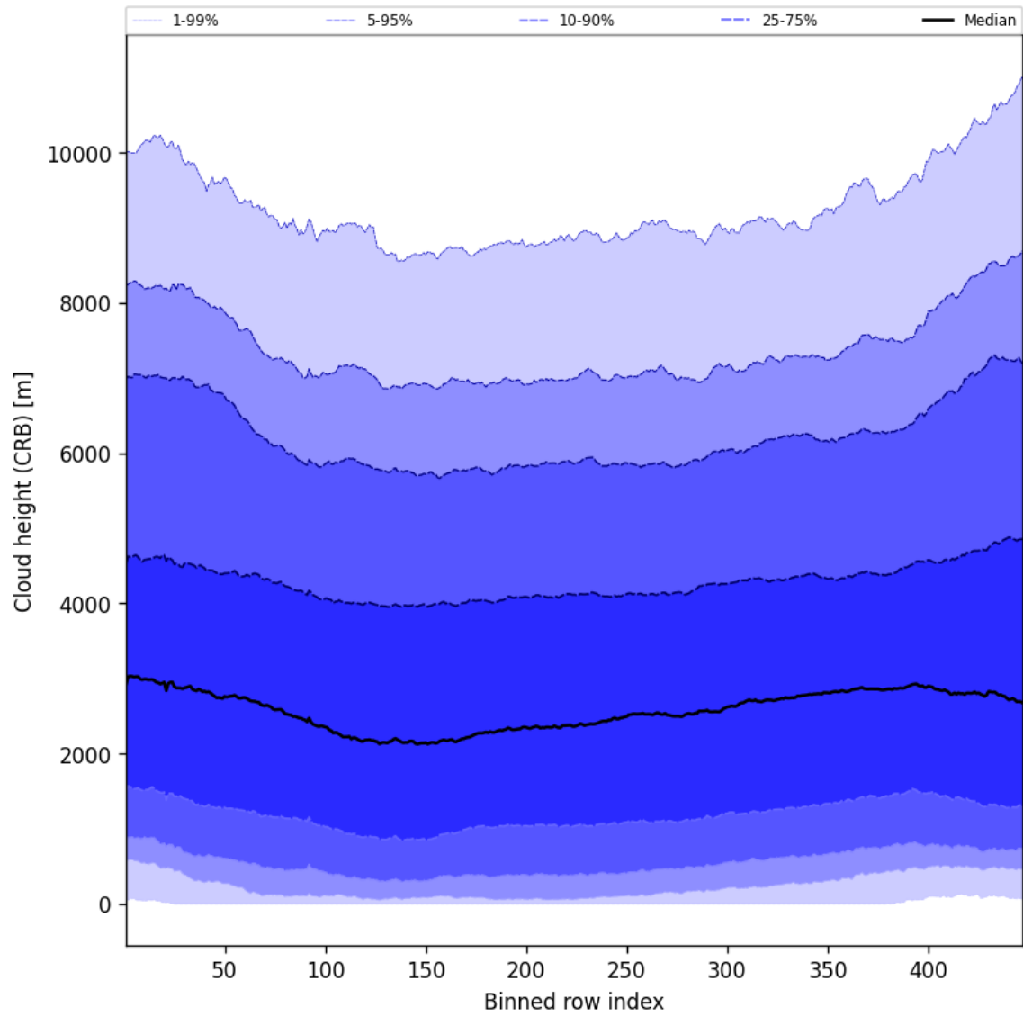
Figure 59: Along track statistics of “Cloud height (CRB)” for 2025-11-13 to 2025-11-15
