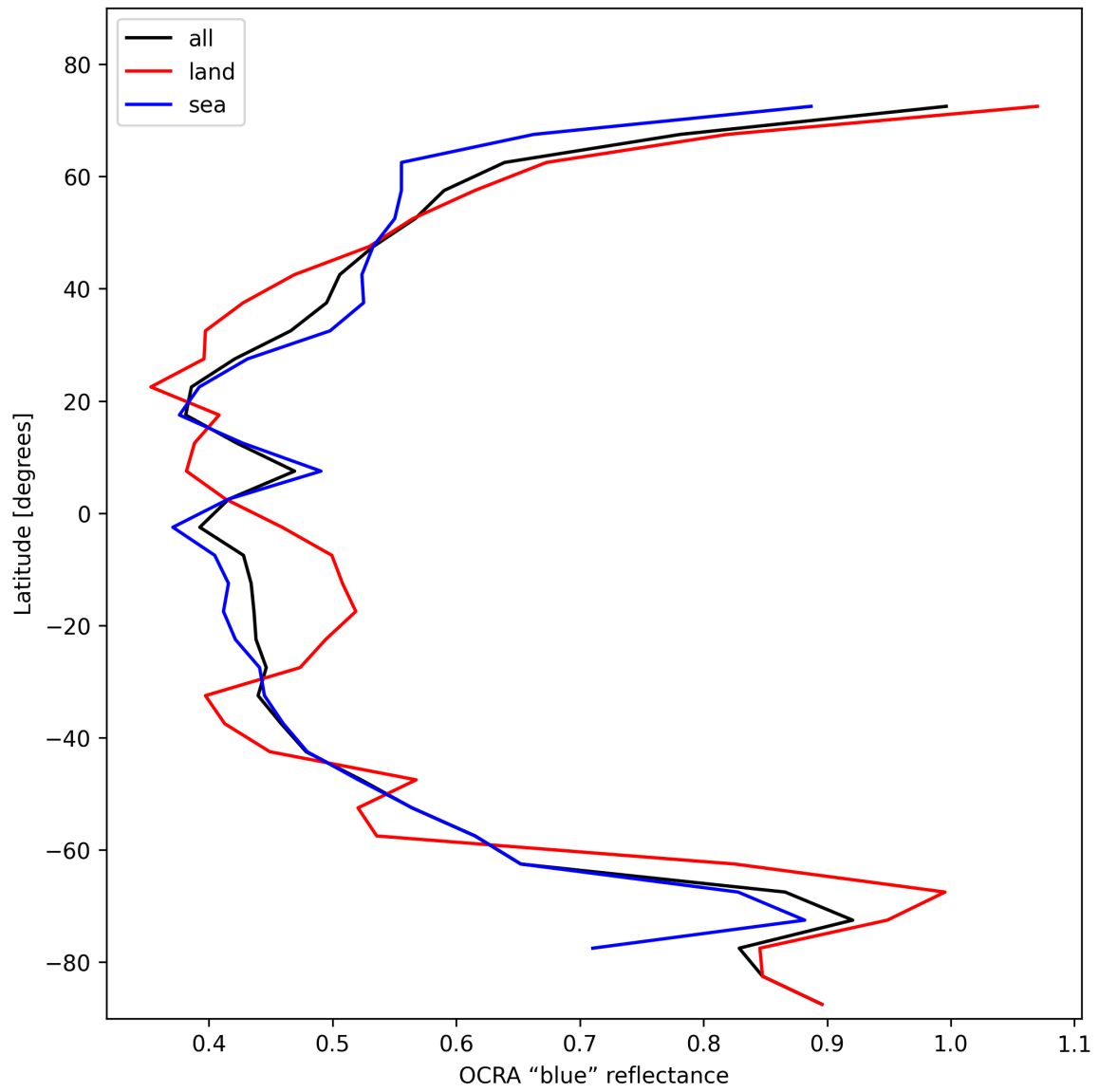
Figure 35: Zonal average of “OCRA “blue” reflectance” for 2025-11-13 to 2025-11-15.
