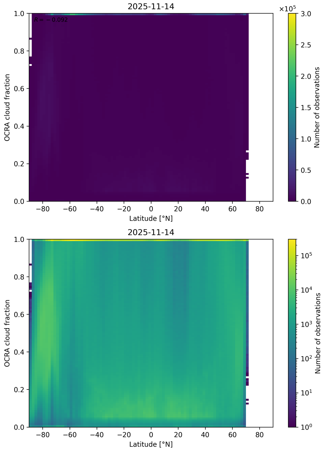
Figure 93: Scatter density plot of “Latitude” against “OCRA cloud fraction” for 2025-11-13 to 2025-11-15.
