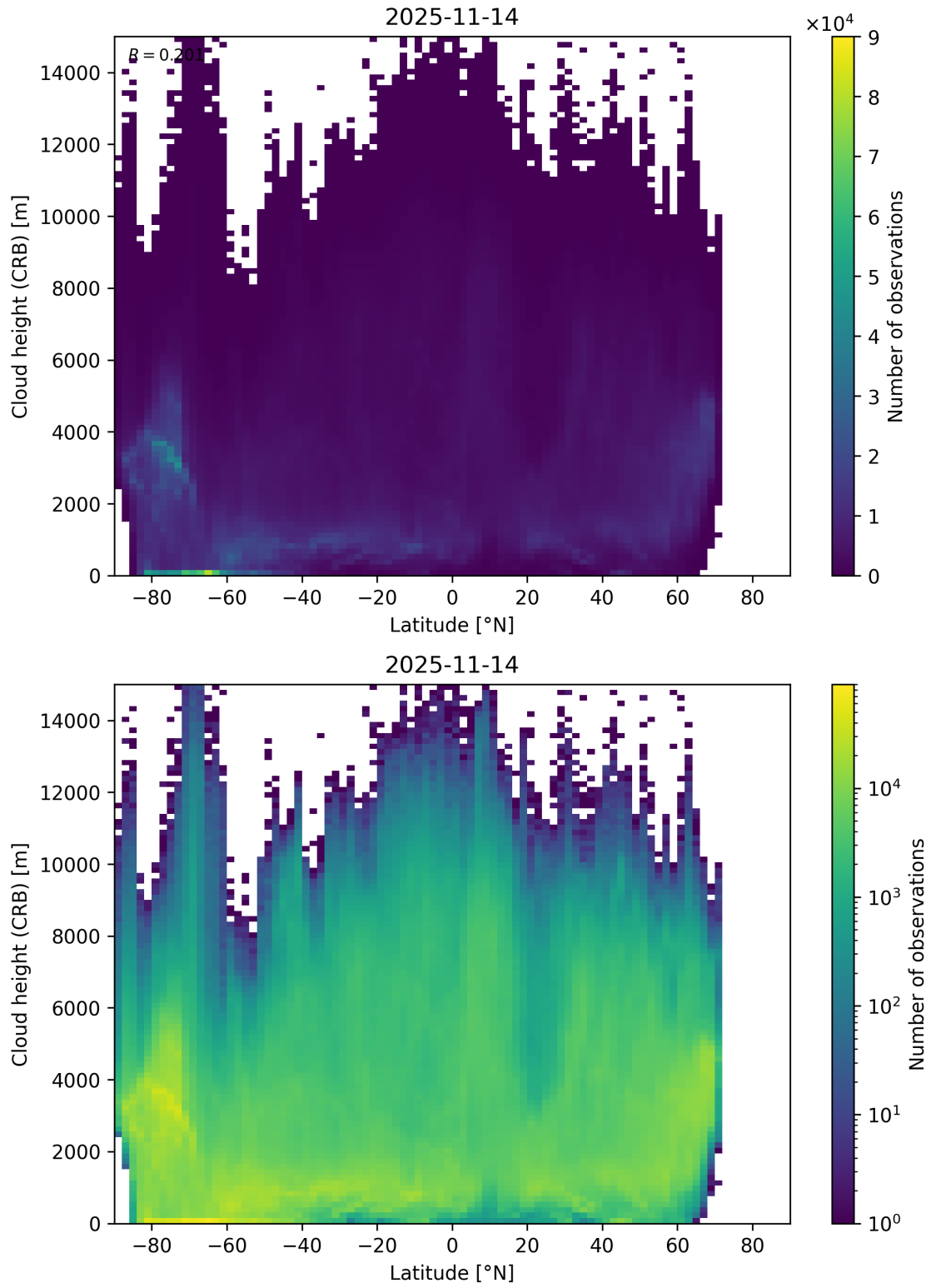
Figure 95: Scatter density plot of “Latitude” against “Cloud height (CRB)” for 2025-11-13 to 2025-11-15.
