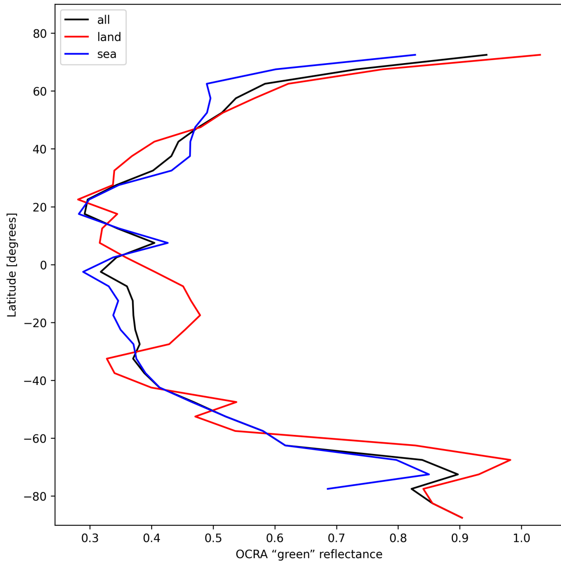
Figure 36: Zonal average of “OCRA “green” reflectance” for 2025-11-13 to 2025-11-15.
