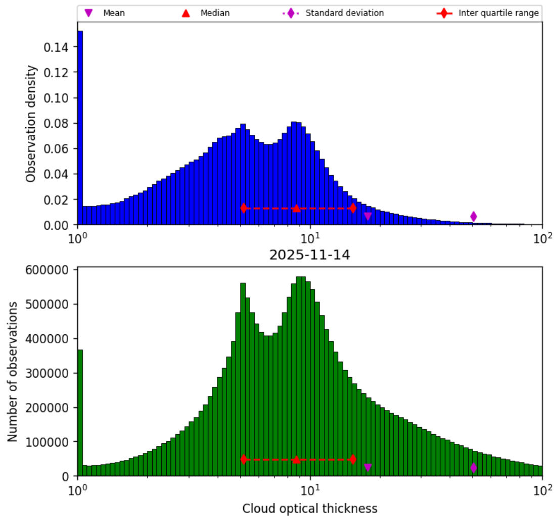
Figure 41: Histogram of “Cloud optical thickness” for 2025-11-13 to 2025-11-15
