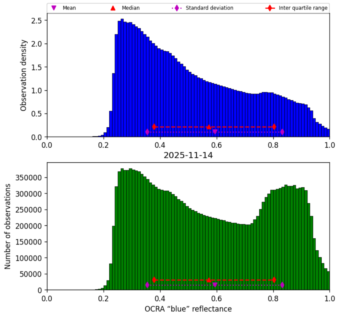
Figure 51: Histogram of “OCRA “blue” reflectance” for 2025-11-13 to 2025-11-15
