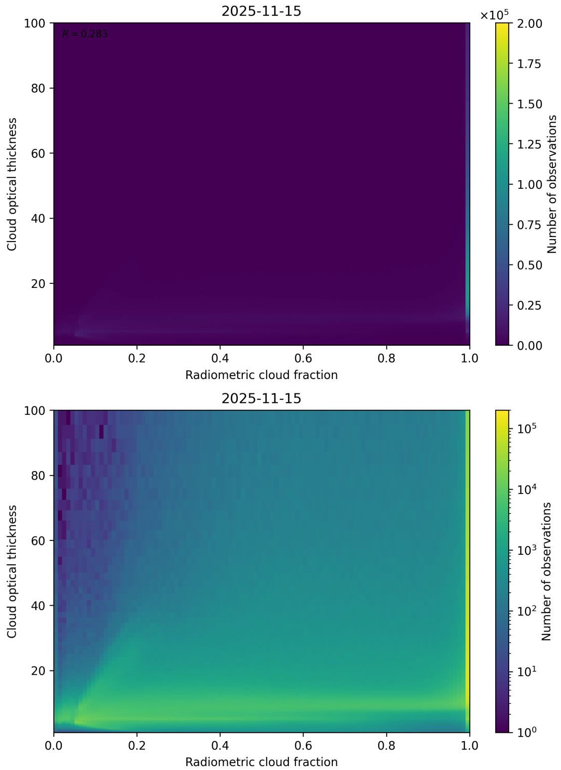
Figure 75: Scatter density plot of “Radiometric cloud fraction” against “Cloud optical thickness” for 2025-11-14 to 2025-11-16.
