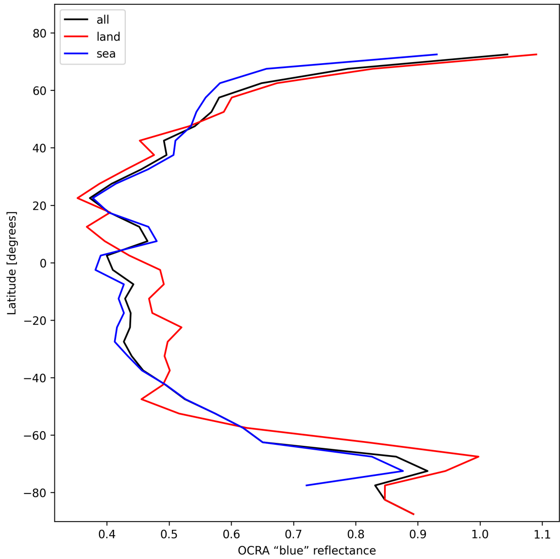
Figure 35: Zonal average of “OCRA “blue” reflectance” for 2025-11-14 to 2025-11-16.
