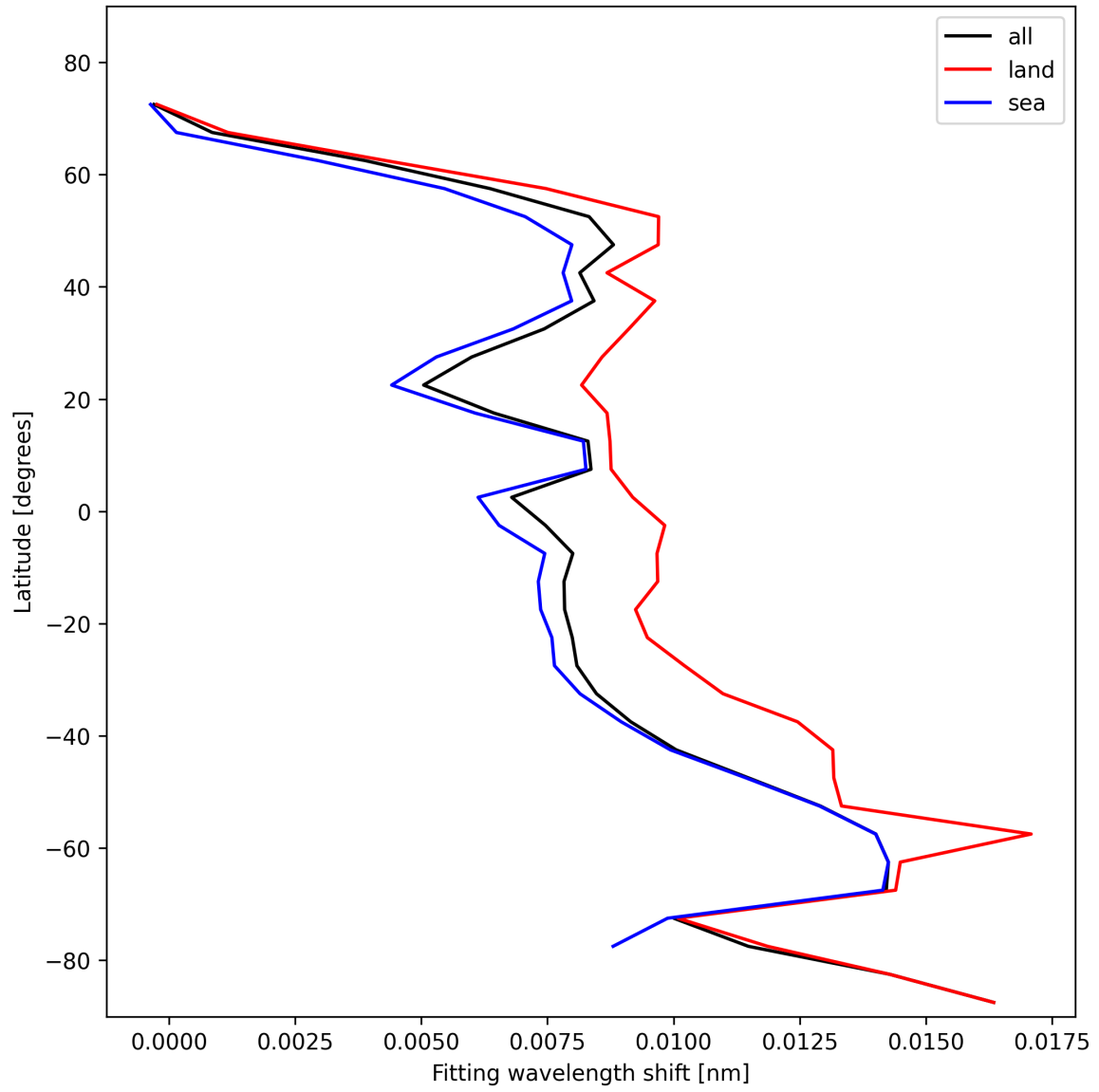
Figure 33: Zonal average of “Fitting wavelength shift” for 2025-11-14 to 2025-11-16.
