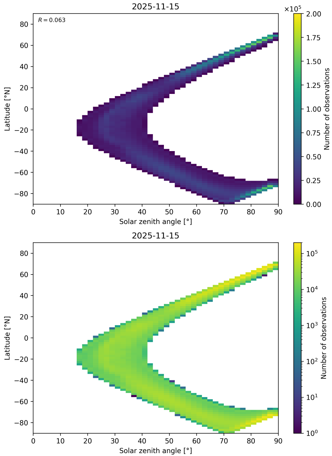
Figure 105: Scatter density plot of “Solar zenith angle” against “Latitude” for 2025-11-14 to 2025-11-16.
