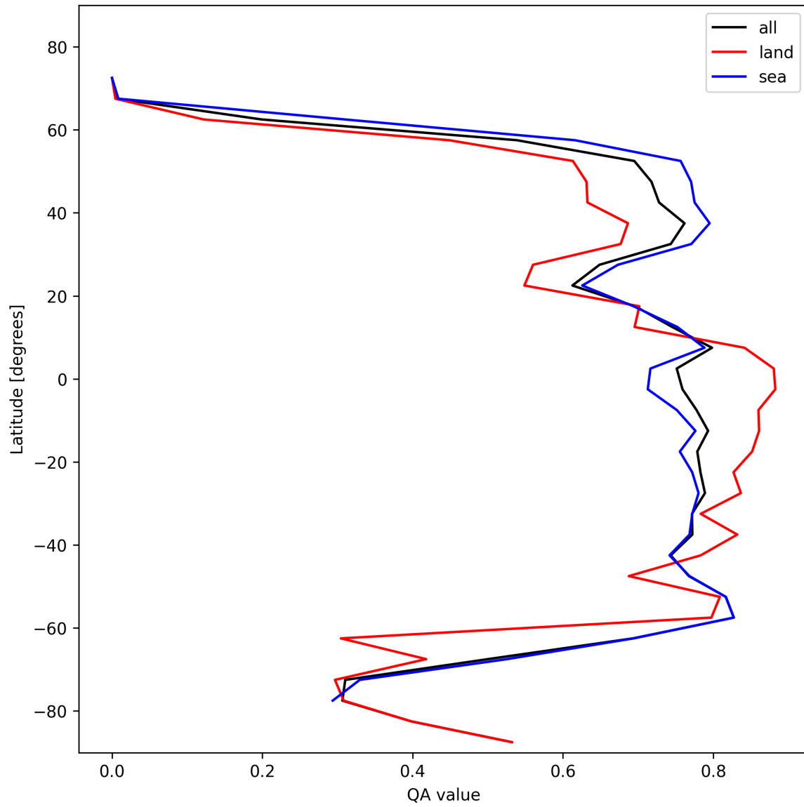
Figure 22: Zonal average of “QA value” for 2025-11-14 to 2025-11-16.
