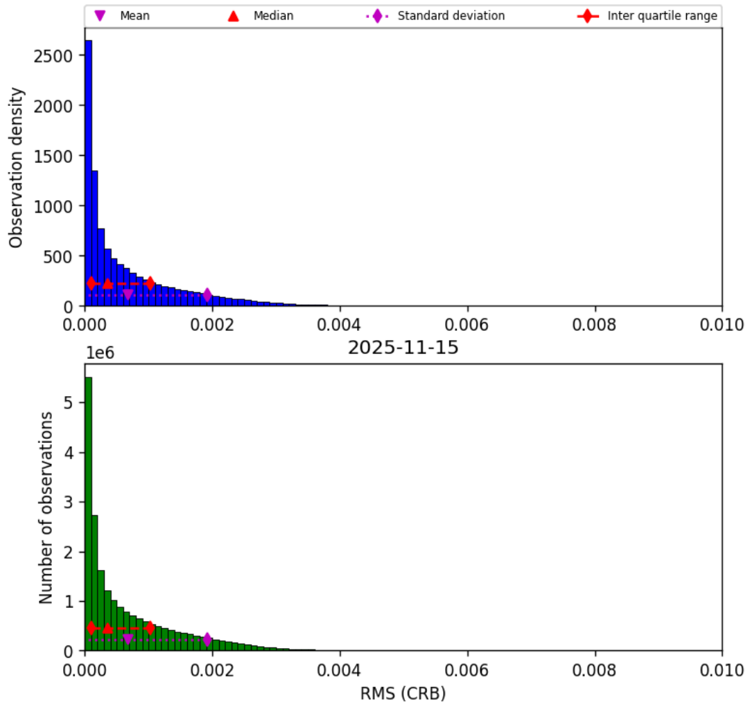
Figure 48: Histogram of “RMS (CRB)” for 2025-11-14 to 2025-11-16
