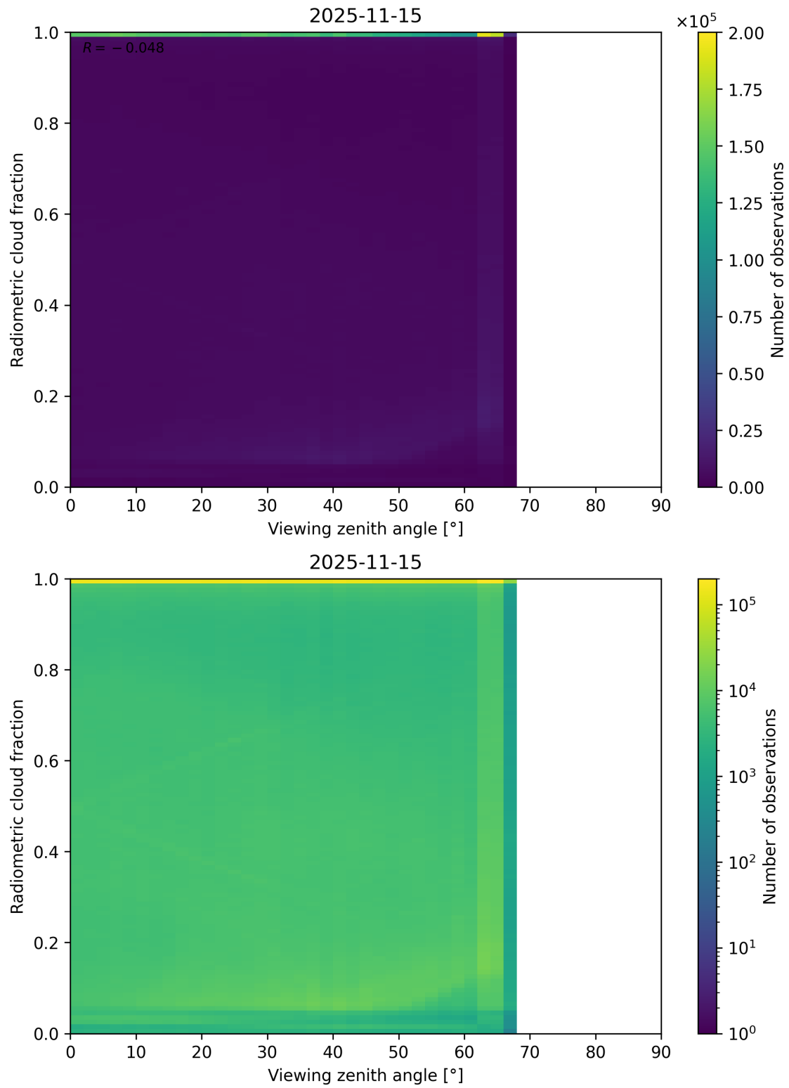
Figure 107: Scatter density plot of “Viewing zenith angle” against “Radiometric cloud fraction” for 2025-11-14 to 2025-11-16.
