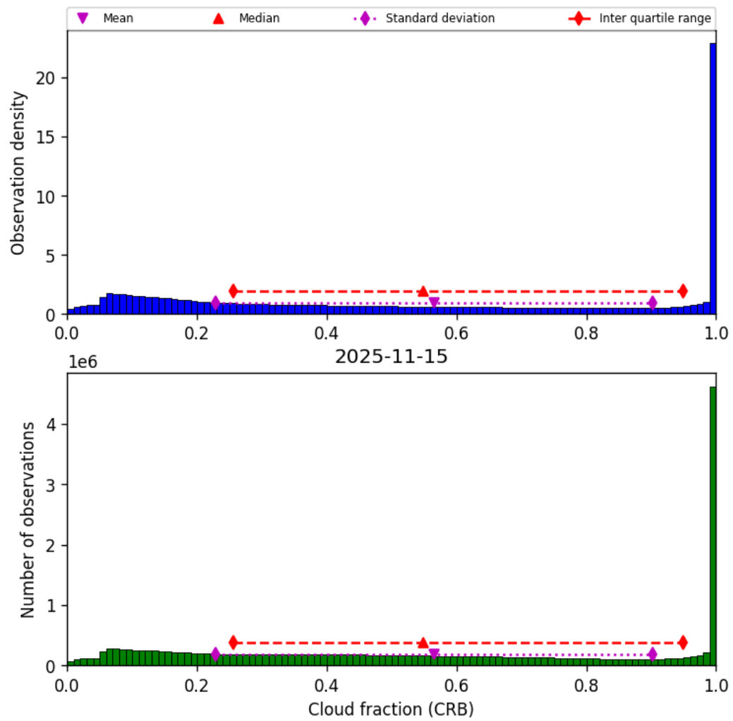
Figure 42: Histogram of “Cloud fraction (CRB)” for 2025-11-14 to 2025-11-16
