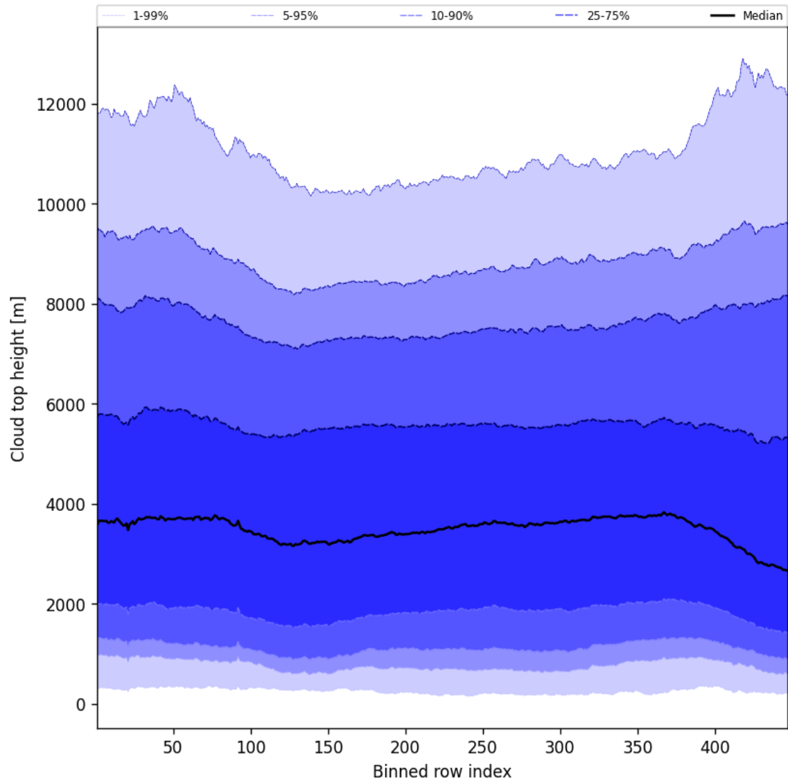
Figure 56: Along track statistics of “Cloud top height” for 2025-11-14 to 2025-11-16
