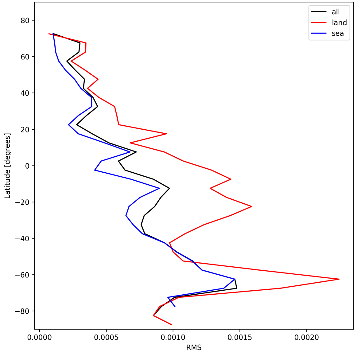
Figure 31: Zonal average of “RMS” for 2025-11-14 to 2025-11-16.
