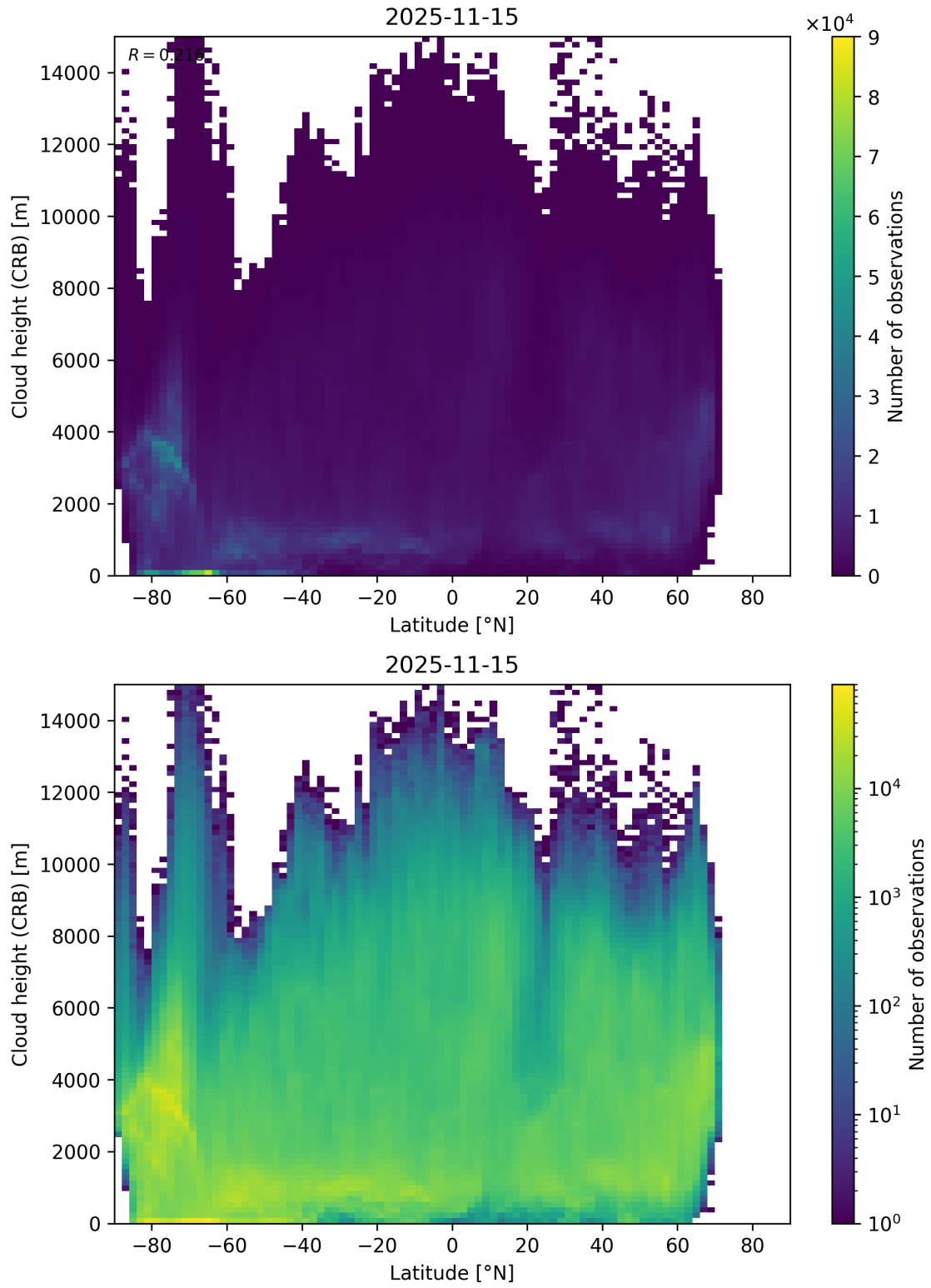
Figure 95: Scatter density plot of “Latitude” against “Cloud height (CRB)” for 2025-11-14 to 2025-11-16.
