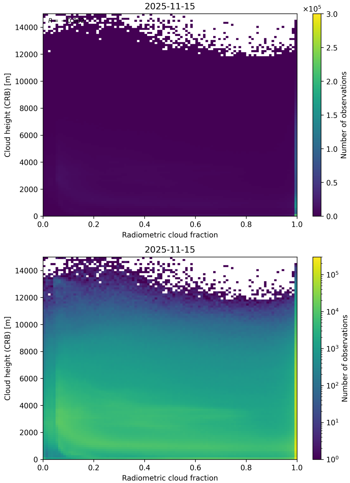
Figure 74: Scatter density plot of “Radiometric cloud fraction” against “Cloud height (CRB)” for 2025-11-14 to 2025-11-16.
