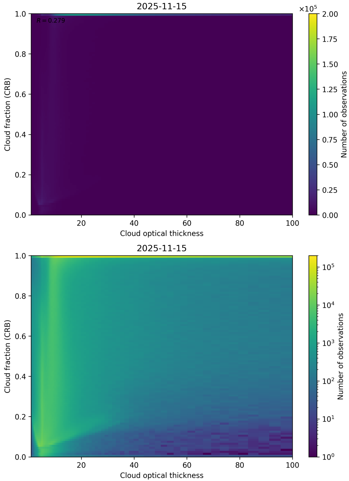
Figure 84: Scatter density plot of “Cloud optical thickness” against “Cloud fraction (CRB)” for 2025-11-14 to 2025-11-16.
