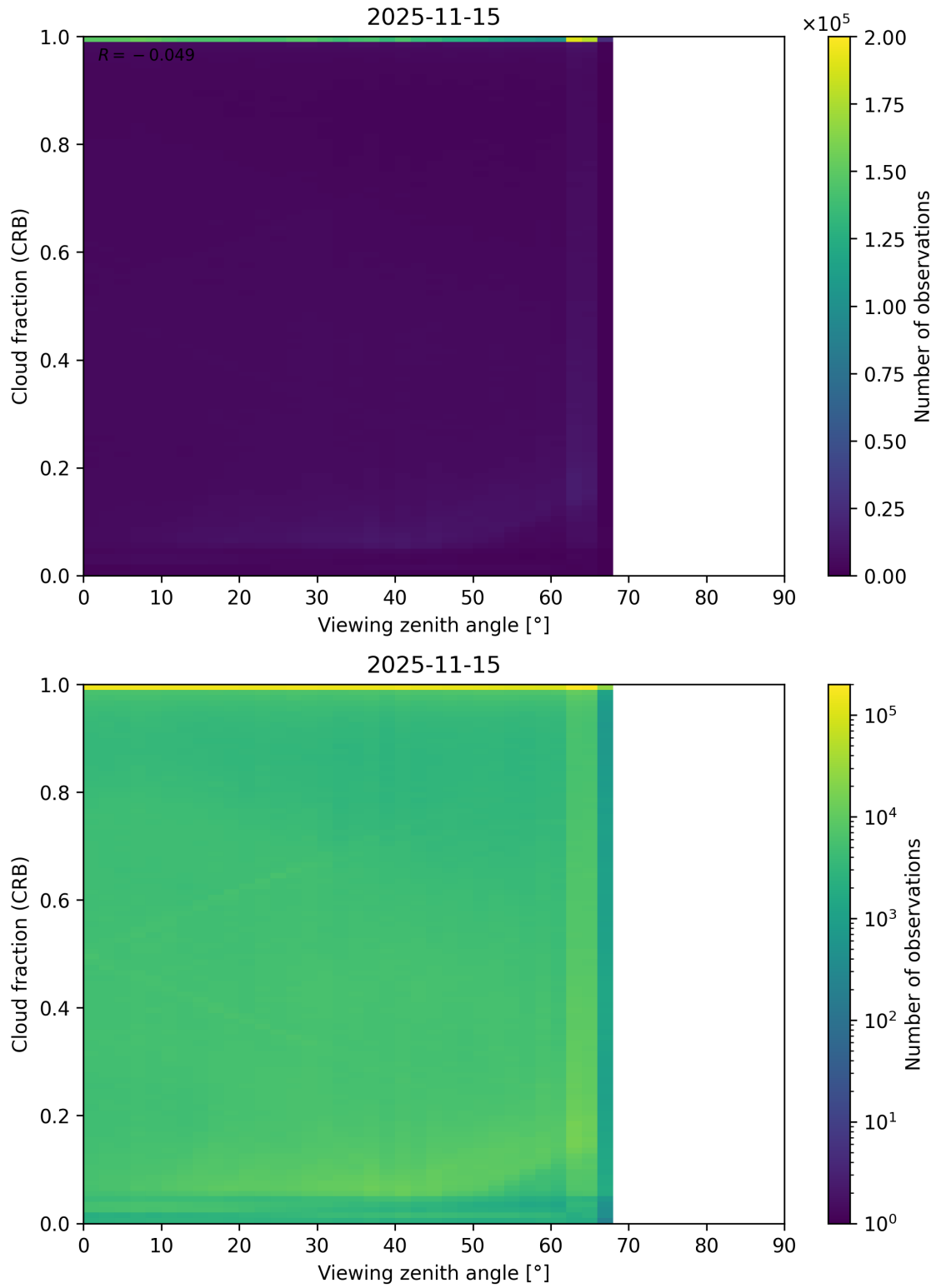
Figure 109: Scatter density plot of “Viewing zenith angle” against “Cloud fraction (CRB)” for 2025-11-14 to 2025-11-16.
