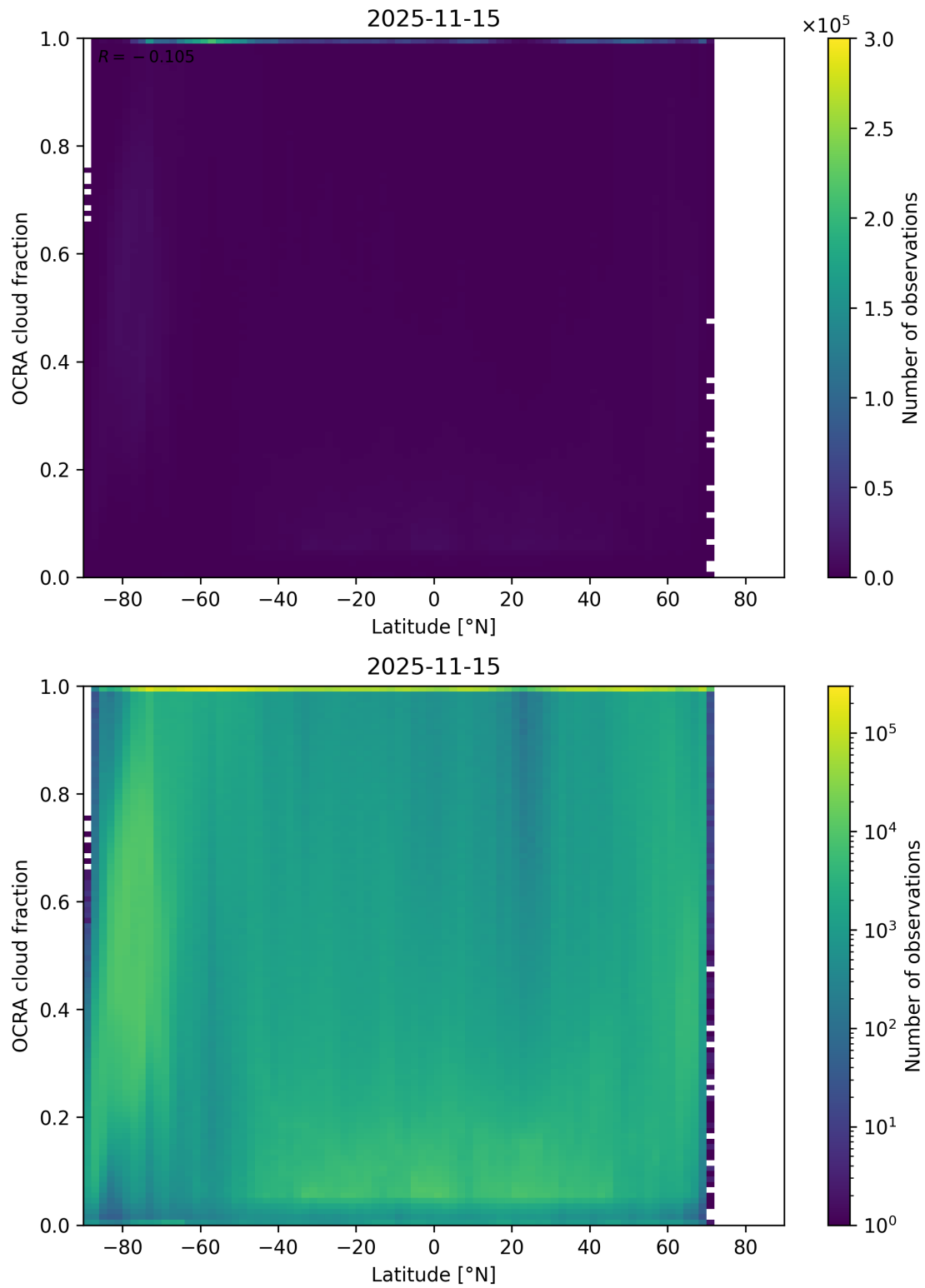
Figure 93: Scatter density plot of “Latitude” against “OCRA cloud fraction” for 2025-11-14 to 2025-11-16.
