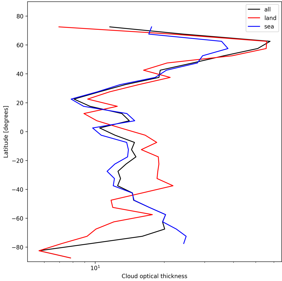
Figure 25: Zonal average of “Cloud optical thickness” for 2025-11-14 to 2025-11-16.
