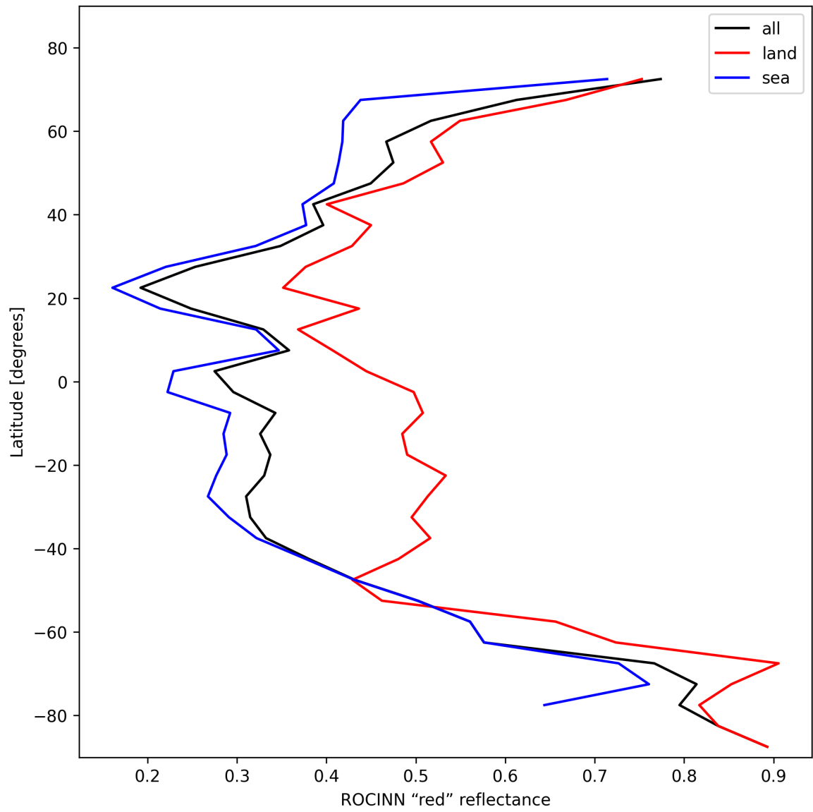
Figure 37: Zonal average of “ROCINN “red” reflectance” for 2025-11-14 to 2025-11-16.
