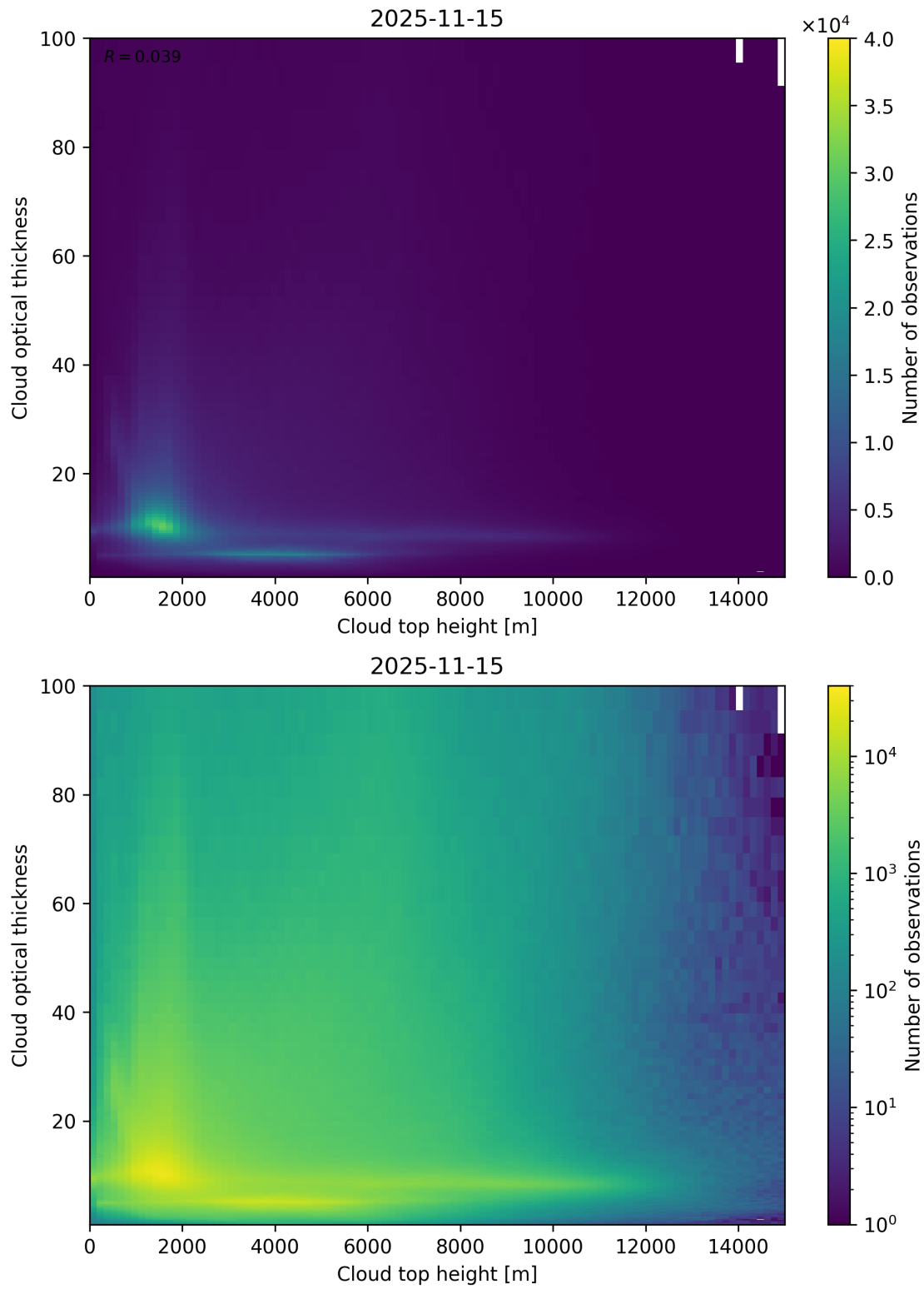
Figure 90: Scatter density plot of “Cloud top height” against “Cloud optical thickness” for 2025-11-14 to 2025-11-16.
