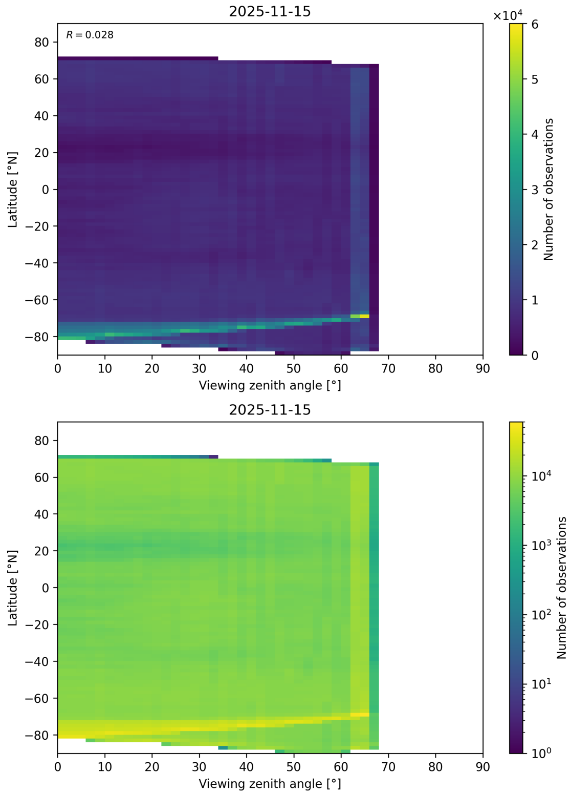
Figure 113: Scatter density plot of “Viewing zenith angle” against “Latitude” for 2025-11-14 to 2025-11-16.
