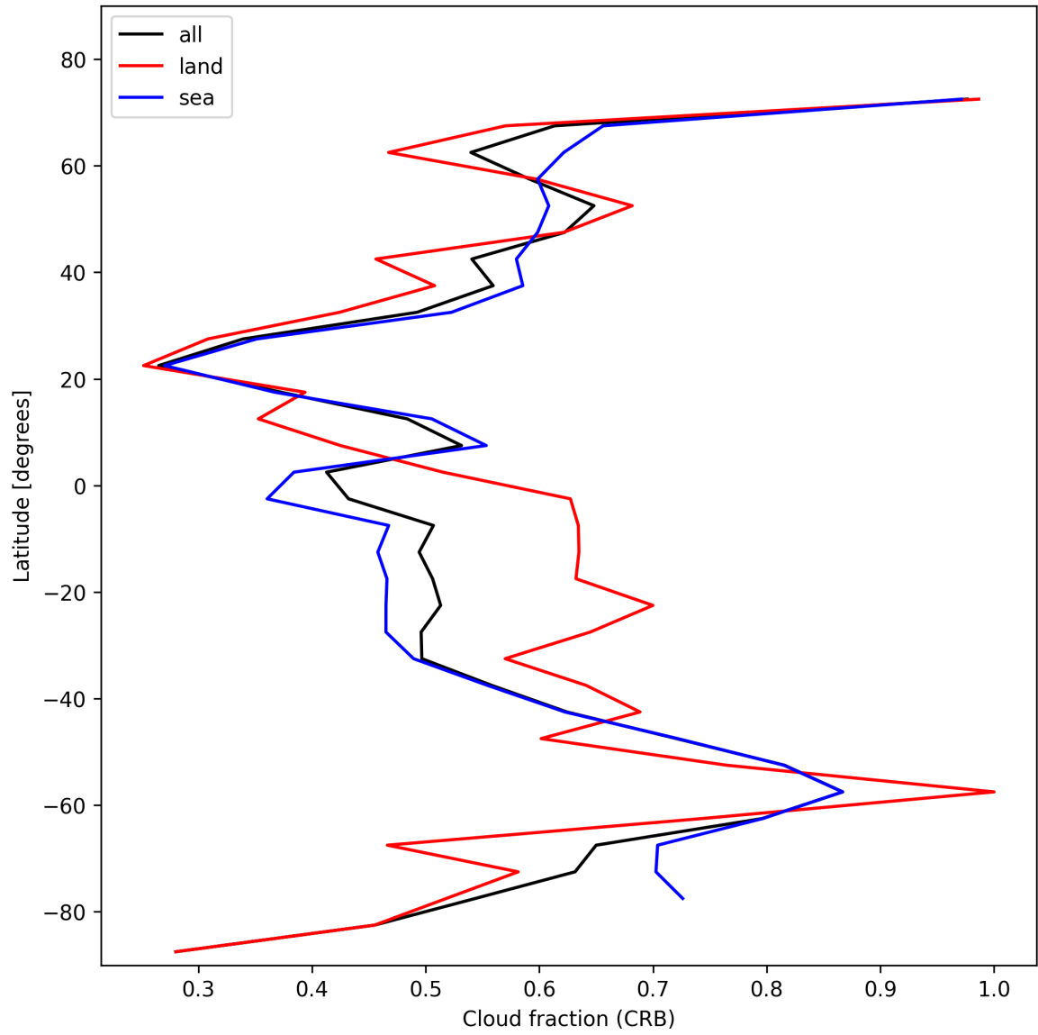
Figure 26: Zonal average of “Cloud fraction (CRB)” for 2025-11-14 to 2025-11-16.
