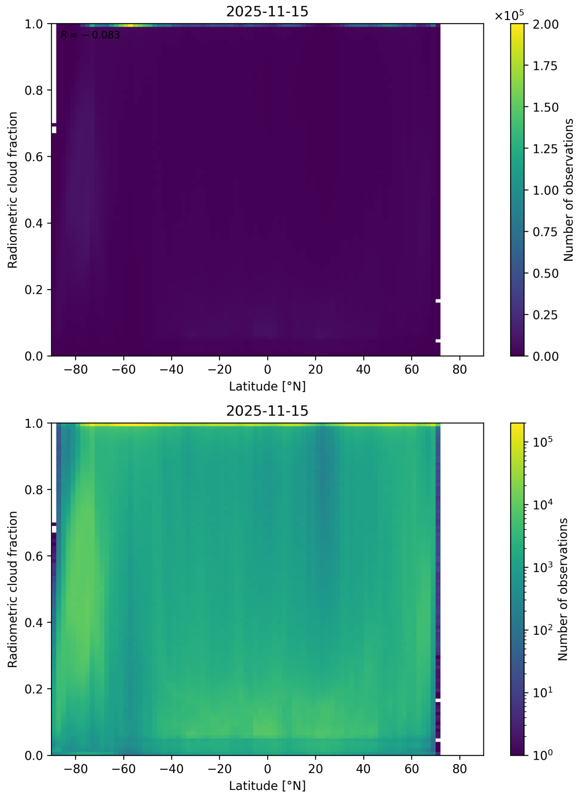
Figure 92: Scatter density plot of “Latitude” against “Radiometric cloud fraction” for 2025-11-14 to 2025-11-16.
