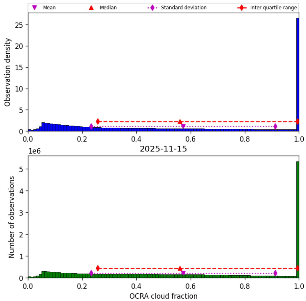
Figure 50: Histogram of “OCRA cloud fraction” for 2025-11-14 to 2025-11-16
