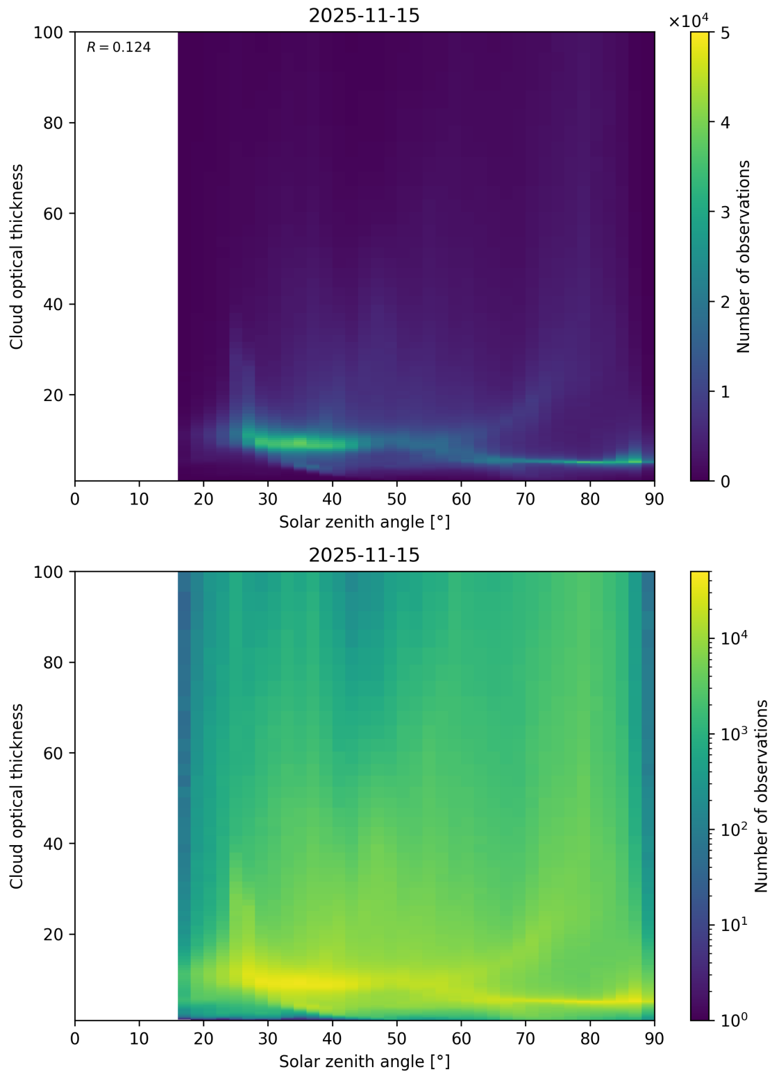
Figure 103: Scatter density plot of “Solar zenith angle” against “Cloud optical thickness” for 2025-11-14 to 2025-11-16.
