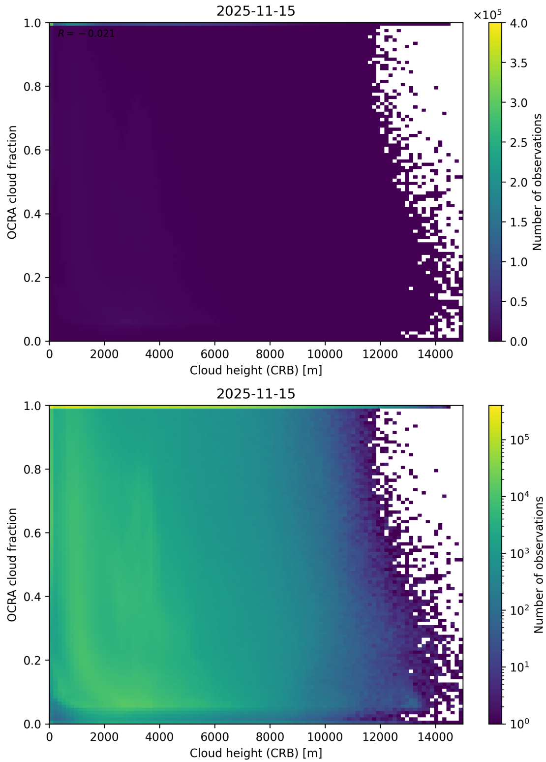
Figure 81: Scatter density plot of “Cloud height (CRB)” against “OCRA cloud fraction” for 2025-11-14 to 2025-11-16.
