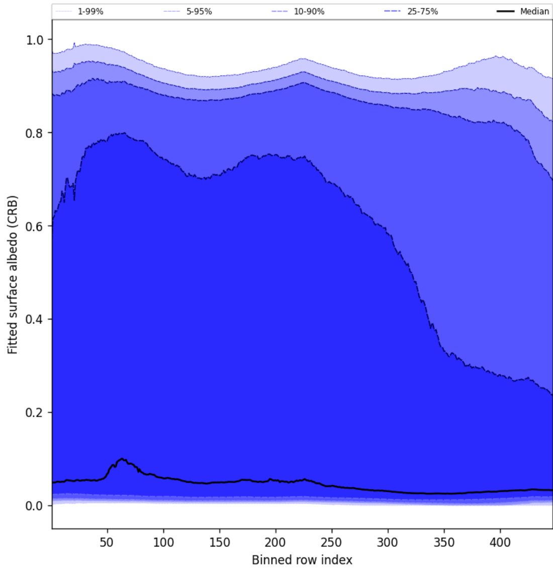
Figure 62: Along track statistics of “Fitted surface albedo (CRB)” for 2025-11-14 to 2025-11-16
