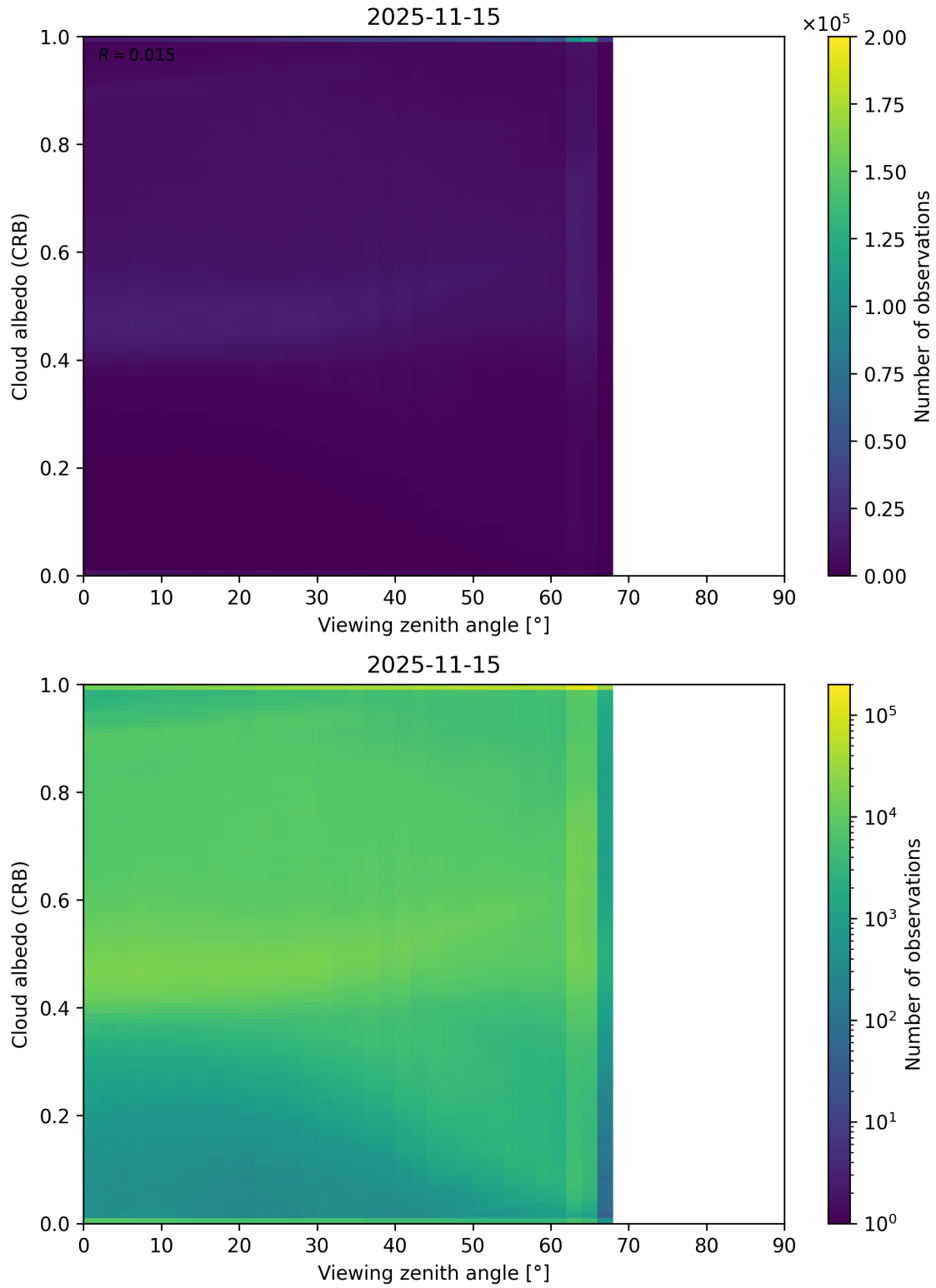
Figure 106: Scatter density plot of “Viewing zenith angle” against “Cloud albedo (CRB)” for 2025-11-14 to 2025-11-16.
