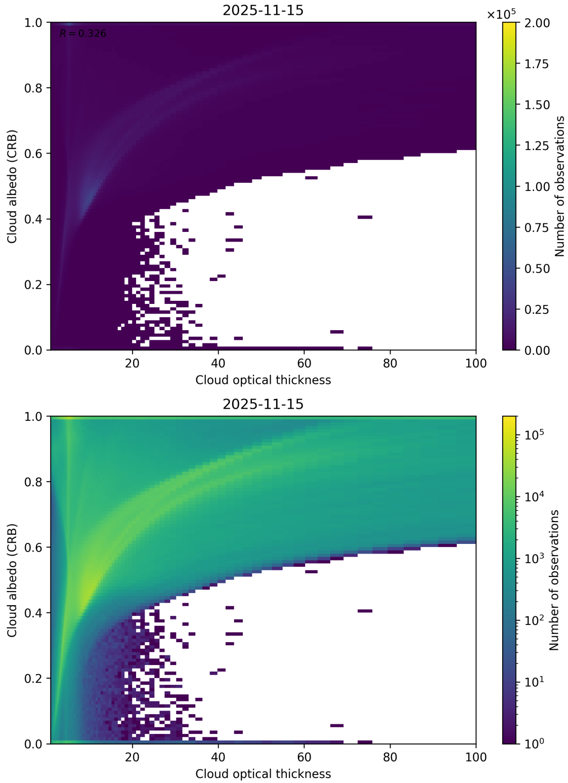
Figure 82: Scatter density plot of “Cloud optical thickness” against “Cloud albedo (CRB)” for 2025-11-14 to 2025-11-16.
