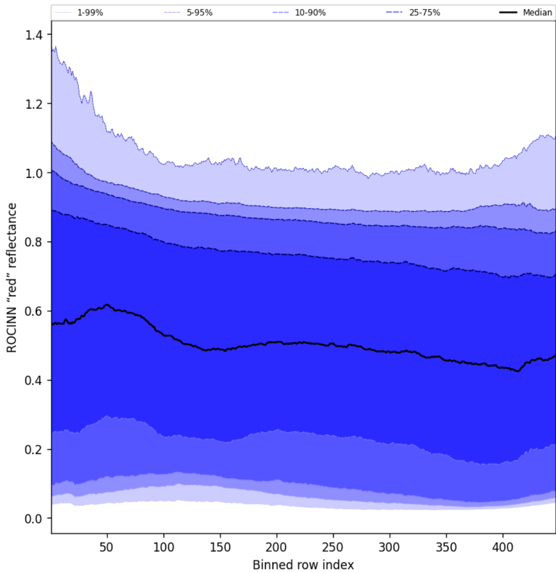
Figure 69: Along track statistics of “ROCINN “red” reflectance” for 2025-11-14 to 2025-11-16
