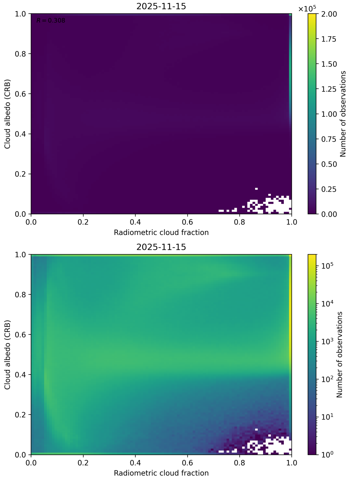
Figure 71: Scatter density plot of “Radiometric cloud fraction” against “Cloud albedo (CRB)” for 2025-11-14 to 2025-11-16.
