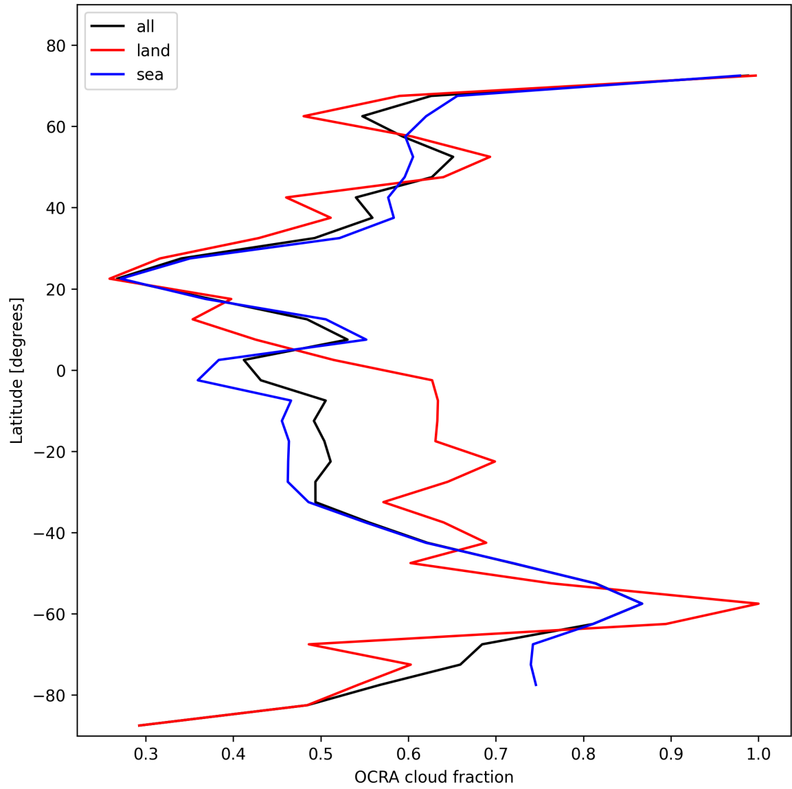
Figure 34: Zonal average of “OCRA cloud fraction” for 2025-11-14 to 2025-11-16.
