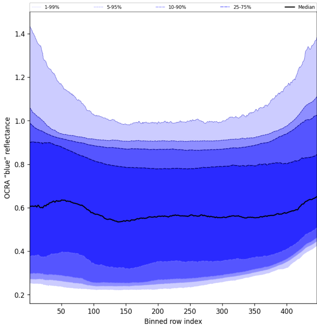
Figure 67: Along track statistics of “OCRA “blue” reflectance” for 2025-11-14 to 2025-11-16
