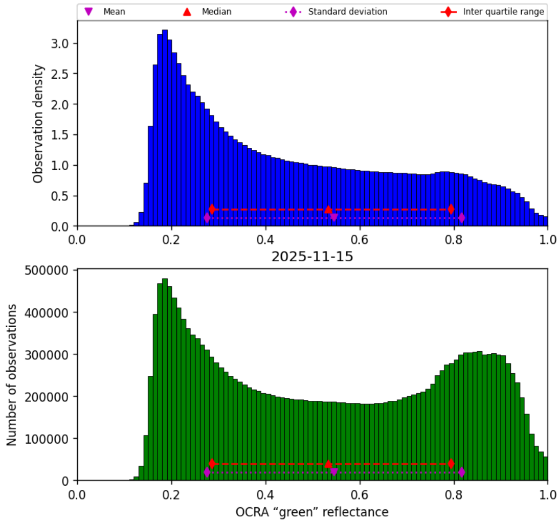
Figure 52: Histogram of “OCRA “green” reflectance” for 2025-11-14 to 2025-11-16
