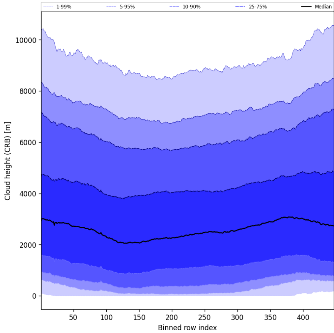
Figure 59: Along track statistics of “Cloud height (CRB)” for 2025-11-14 to 2025-11-16
