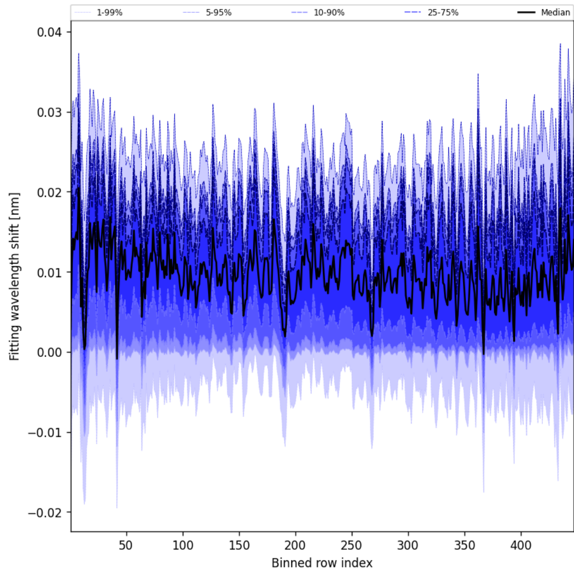
Figure 65: Along track statistics of “Fitting wavelength shift” for 2025-11-14 to 2025-11-16
