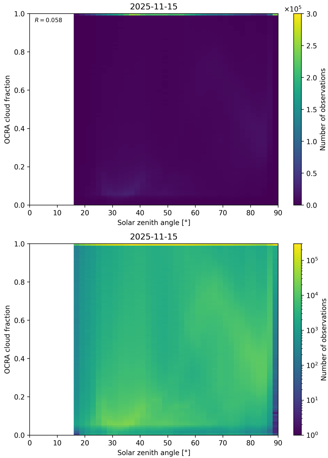
Figure 100: Scatter density plot of “Solar zenith angle” against “OCRA cloud fraction” for 2025-11-14 to 2025-11-16.
