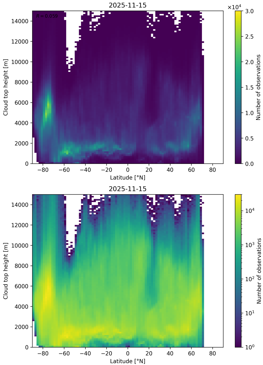
Figure 97: Scatter density plot of “Latitude” against “Cloud top height” for 2025-11-14 to 2025-11-16.
