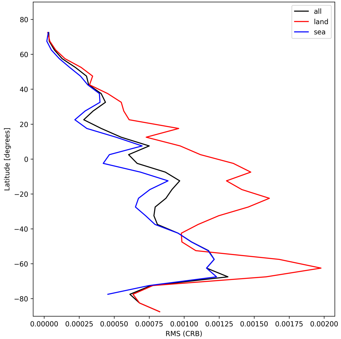
Figure 32: Zonal average of “RMS (CRB)” for 2025-11-14 to 2025-11-16.
