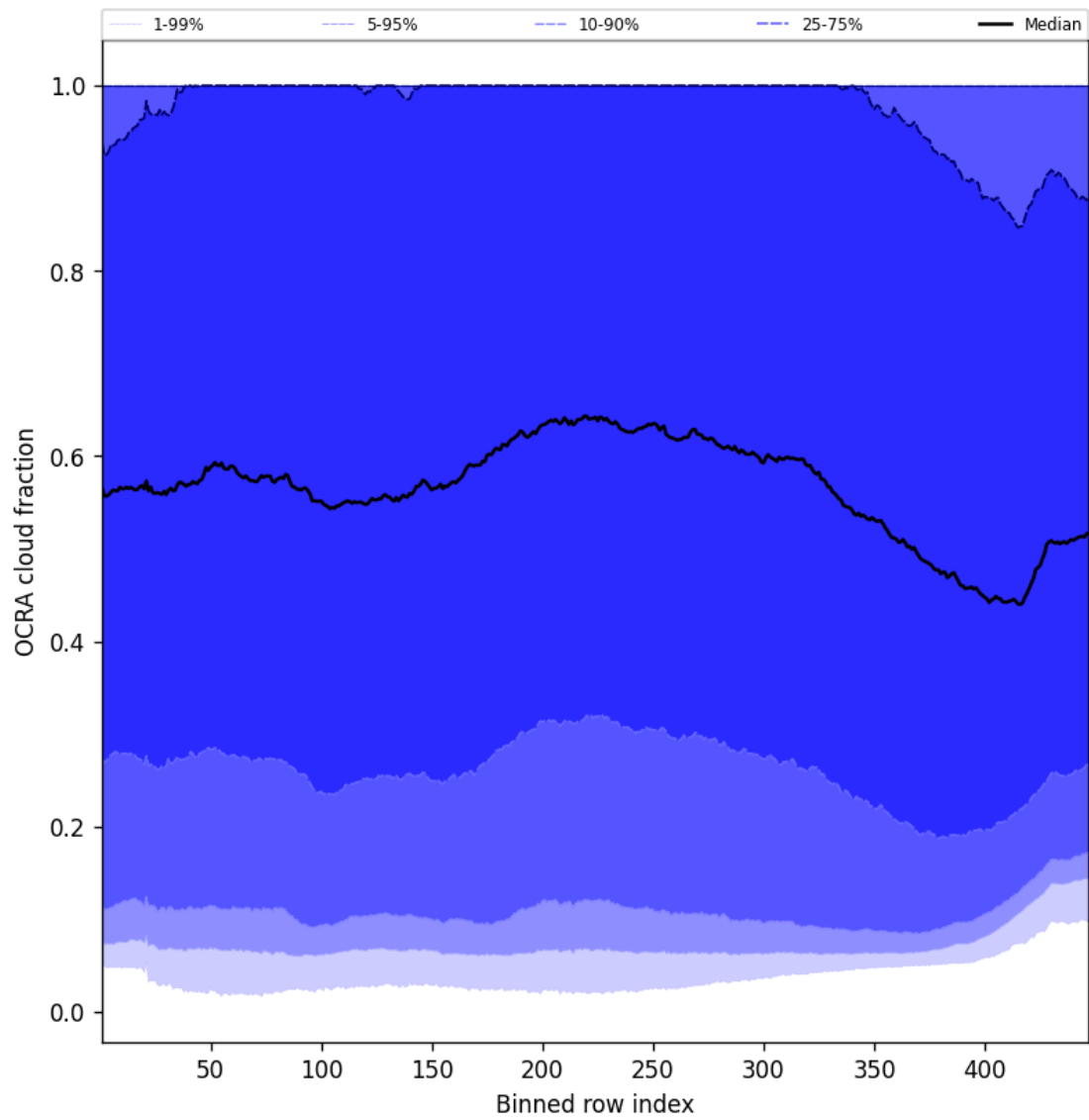
Figure 66: Along track statistics of “OCRA cloud fraction” for 2025-11-14 to 2025-11-16
