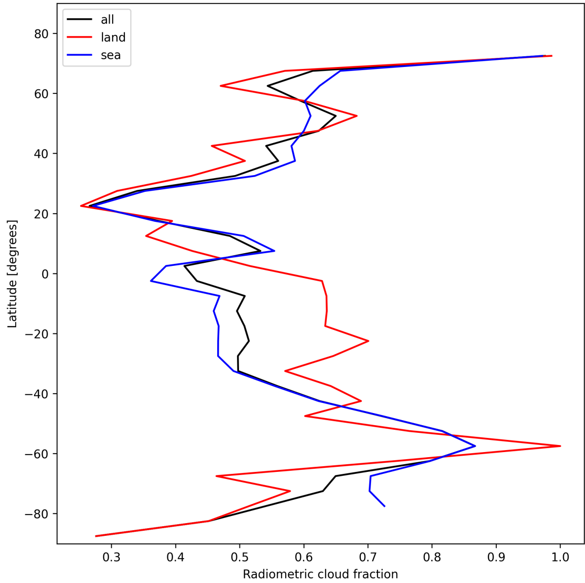
Figure 23: Zonal average of “Radiometric cloud fraction” for 2025-11-14 to 2025-11-16.
