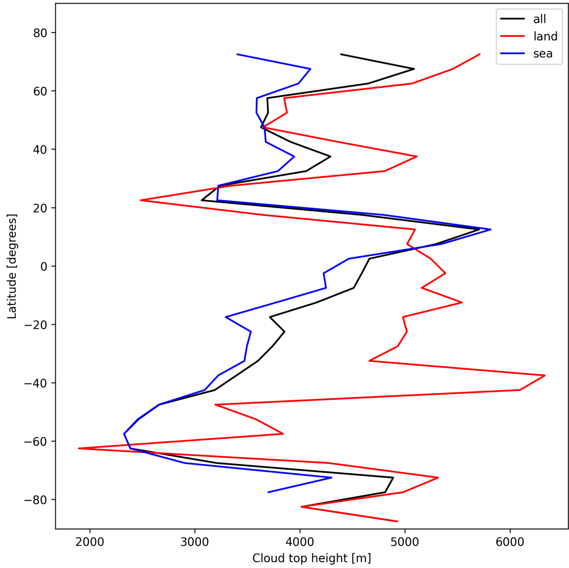
Figure 24: Zonal average of “Cloud top height” for 2025-11-14 to 2025-11-16.
