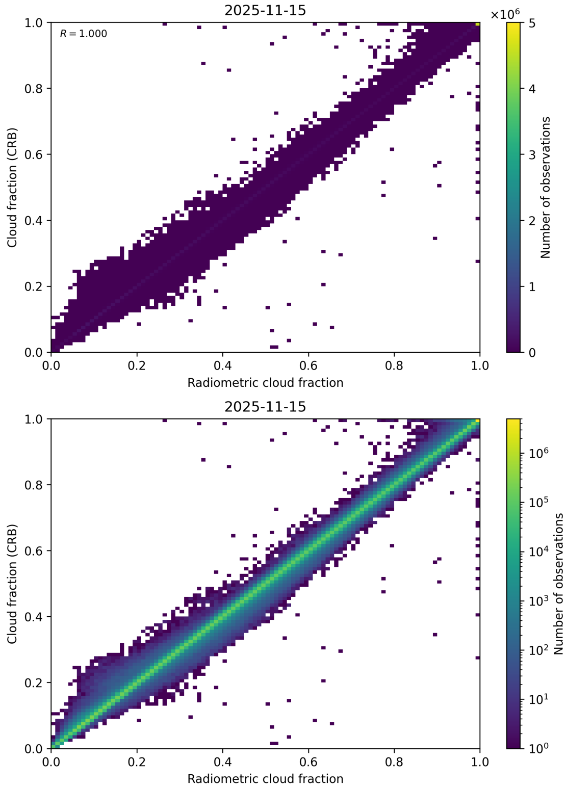
Figure 73: Scatter density plot of “Radiometric cloud fraction” against “Cloud fraction (CRB)” for 2025-11-14 to 2025-11-16.
