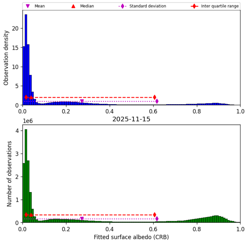
Figure 46: Histogram of “Fitted surface albedo (CRB)” for 2025-11-14 to 2025-11-16
