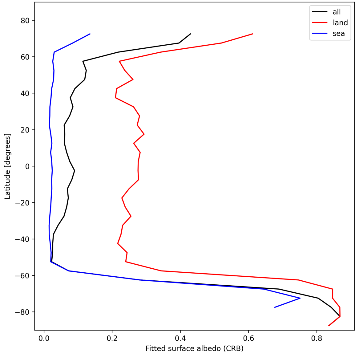
Figure 30: Zonal average of “Fitted surface albedo (CRB)” for 2025-11-14 to 2025-11-16.
