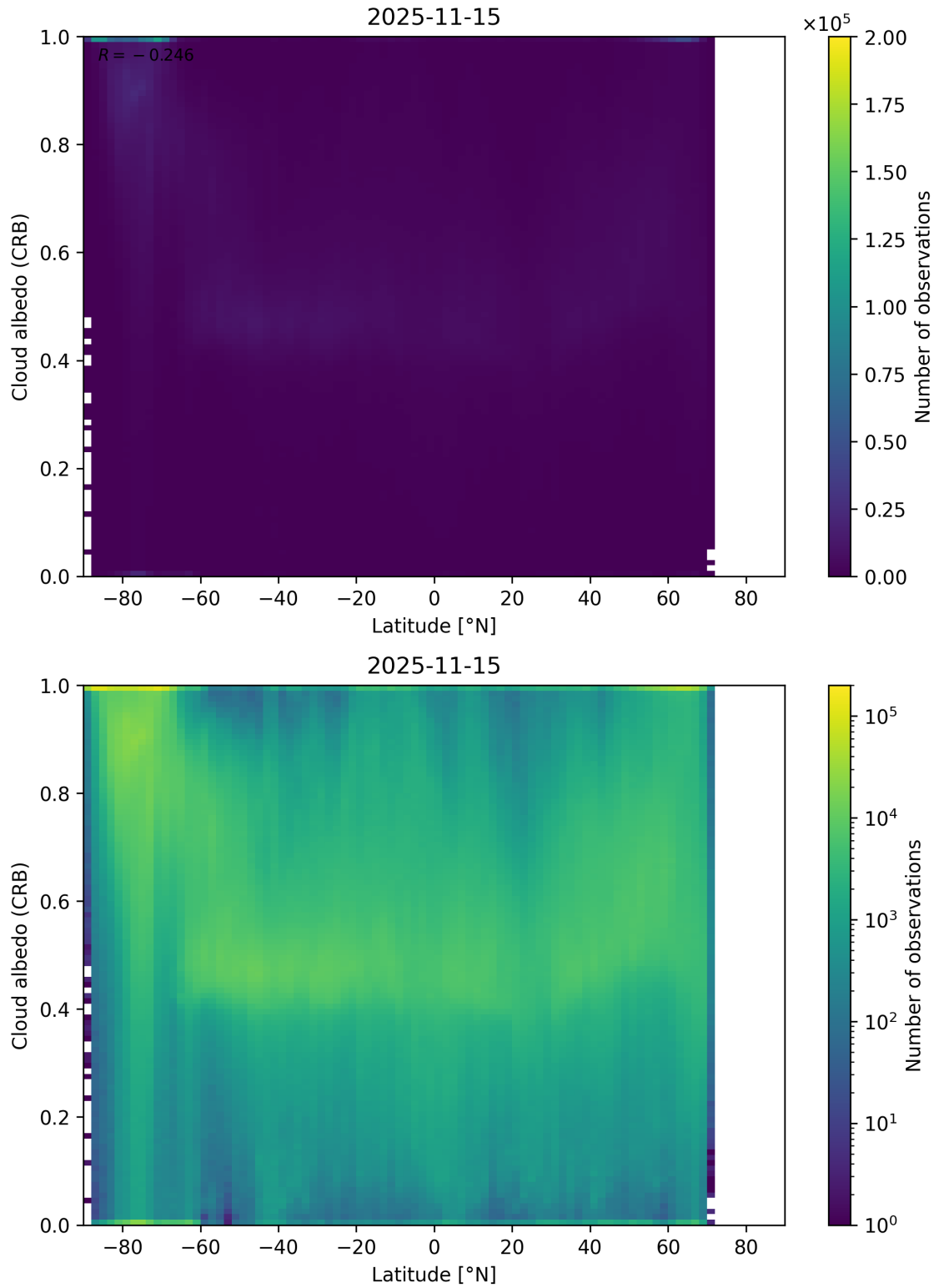
Figure 91: Scatter density plot of “Latitude” against “Cloud albedo (CRB)” for 2025-11-14 to 2025-11-16.
