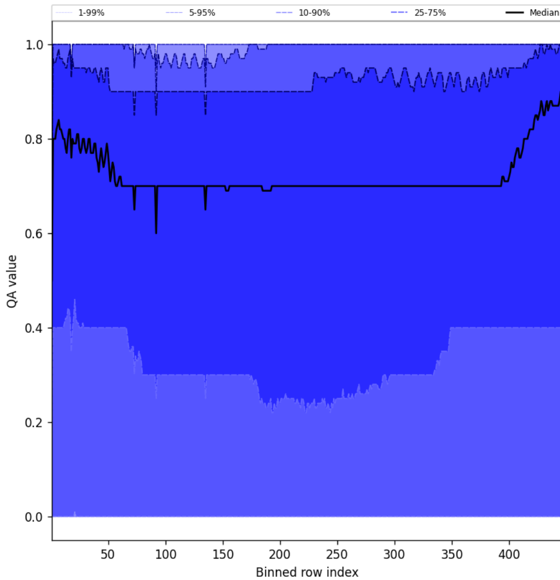
Figure 54: Along track statistics of “QA value” for 2025-11-14 to 2025-11-16
