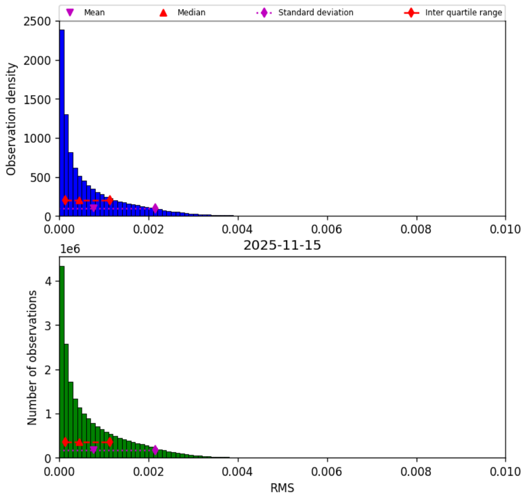
Figure 47: Histogram of “RMS” for 2025-11-14 to 2025-11-16
