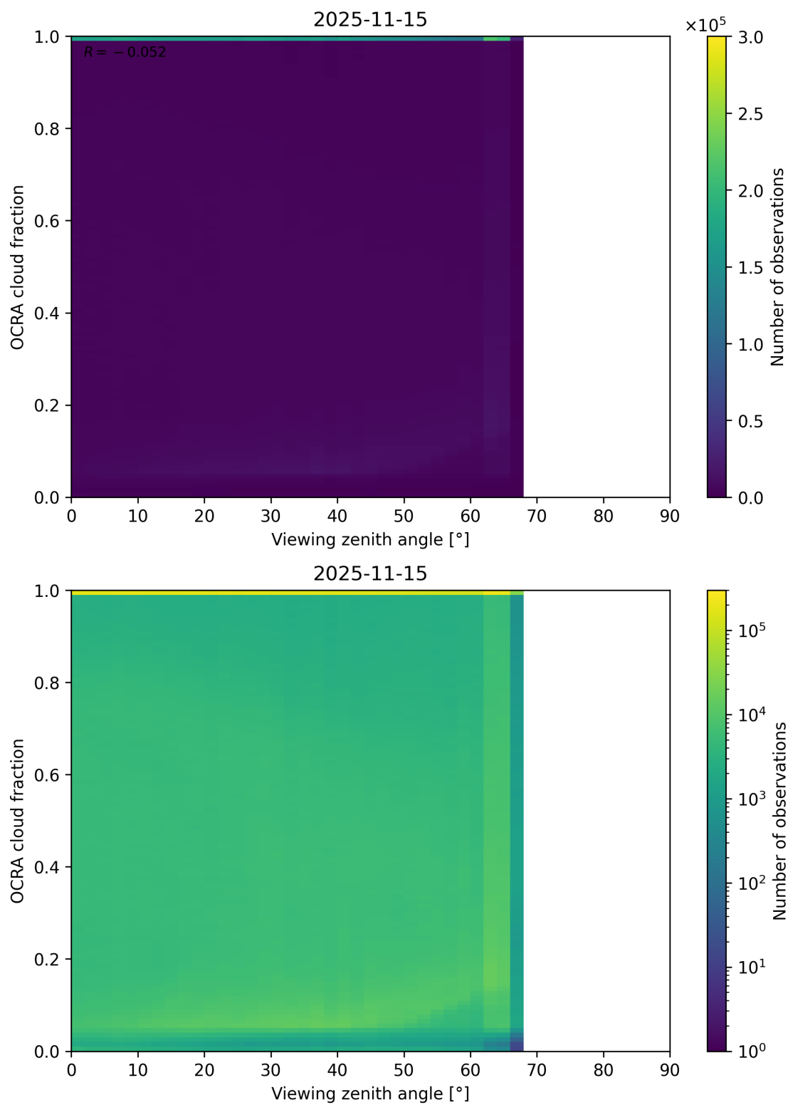
Figure 108: Scatter density plot of “Viewing zenith angle” against “OCRA cloud fraction” for 2025-11-14 to 2025-11-16.
