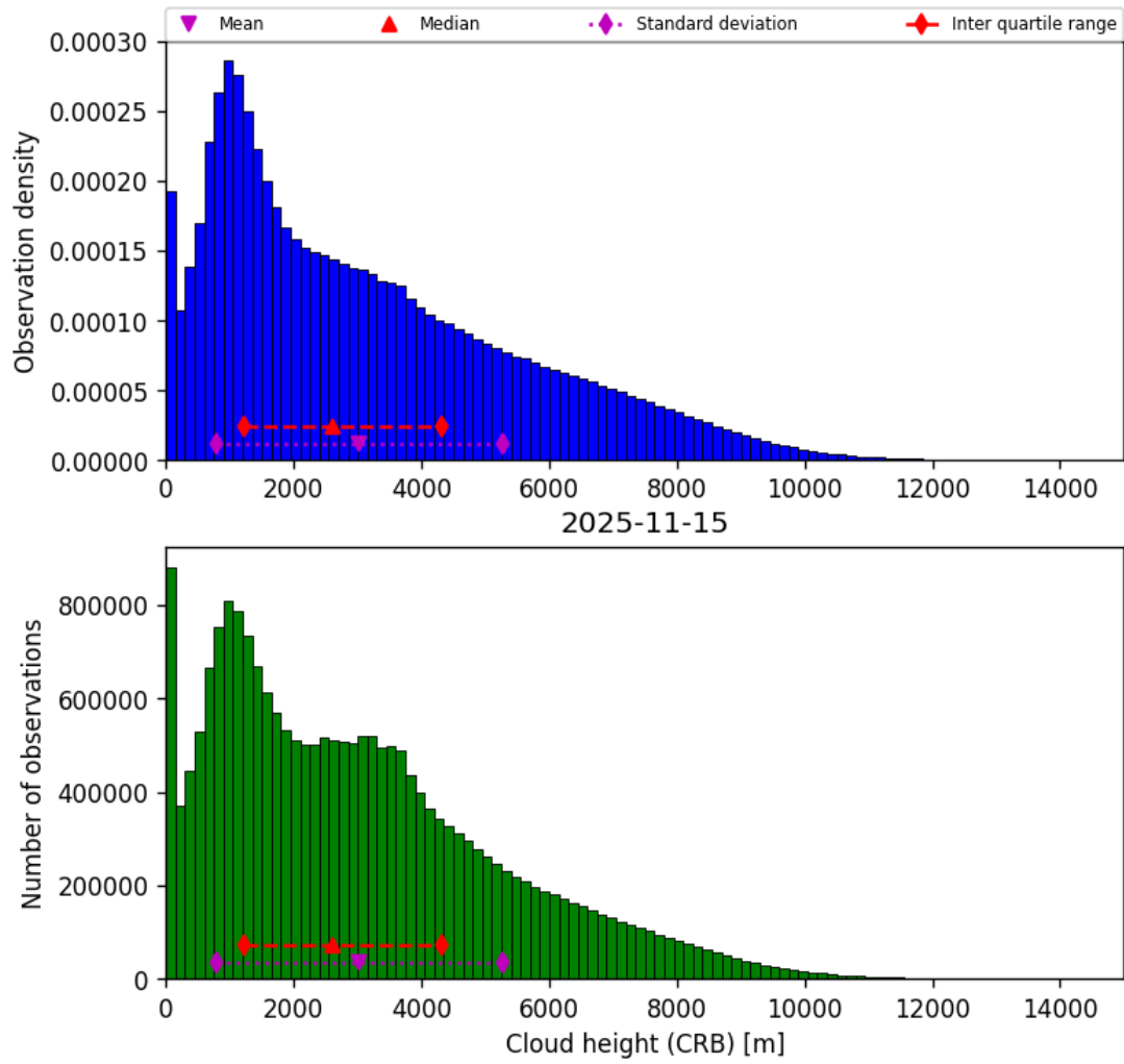
Figure 43: Histogram of “Cloud height (CRB)” for 2025-11-14 to 2025-11-16
