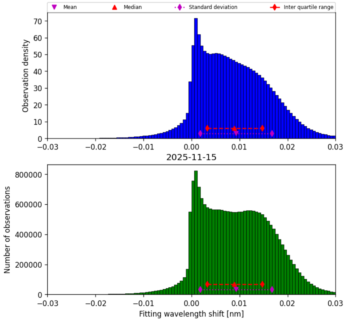
Figure 49: Histogram of “Fitting wavelength shift” for 2025-11-14 to 2025-11-16
