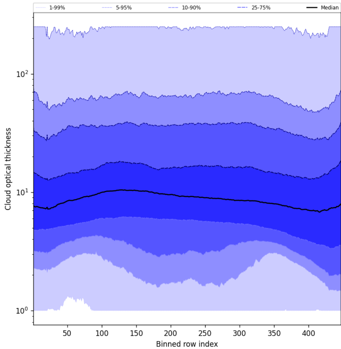
Figure 57: Along track statistics of “Cloud optical thickness” for 2025-11-14 to 2025-11-16
