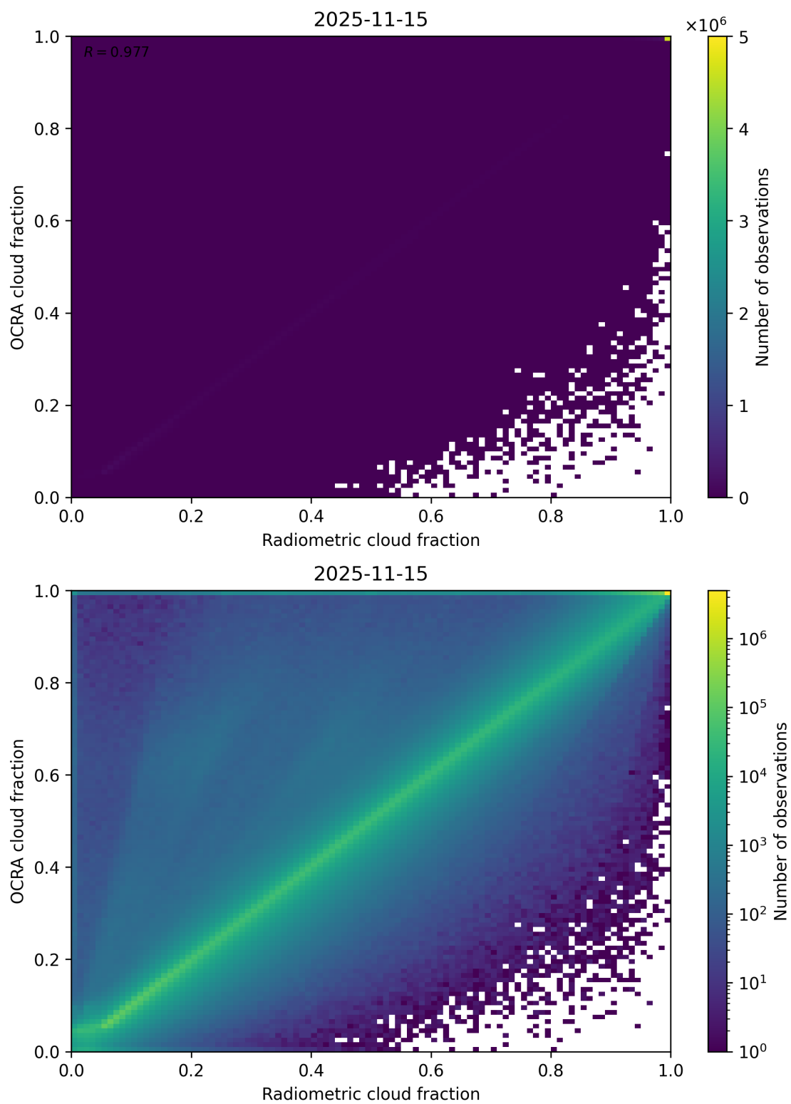
Figure 72: Scatter density plot of “Radiometric cloud fraction” against “OCRA cloud fraction” for 2025-11-14 to 2025-11-16.
