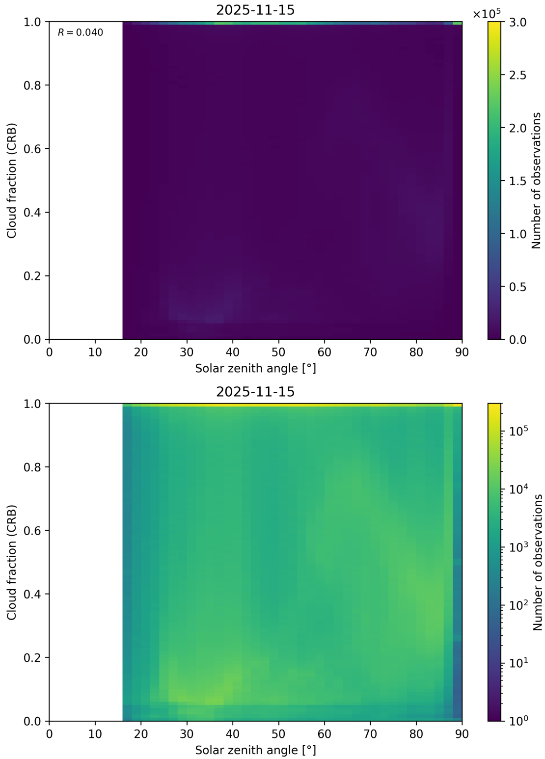
Figure 101: Scatter density plot of “Solar zenith angle” against “Cloud fraction (CRB)” for 2025-11-14 to 2025-11-16.
