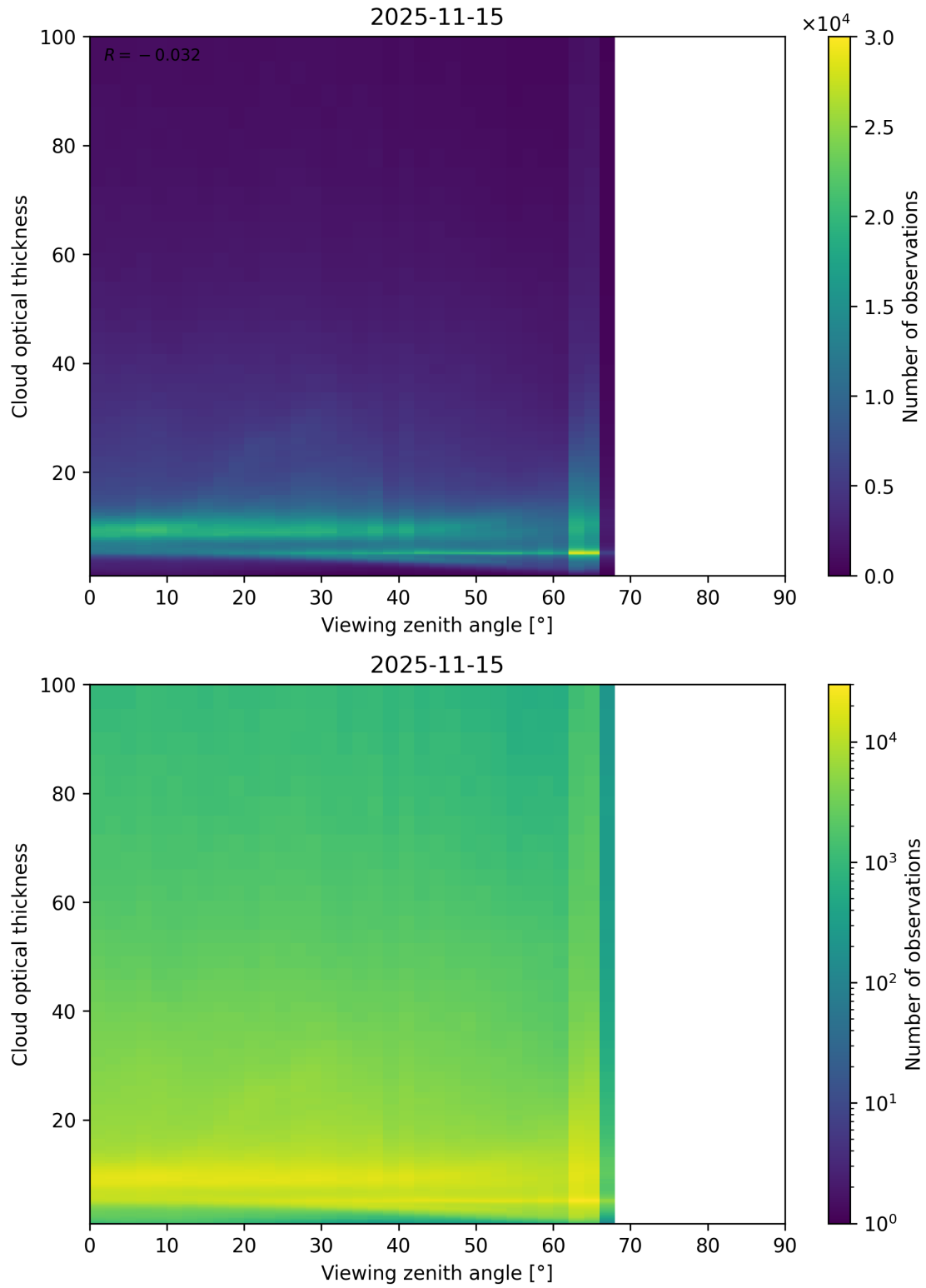
Figure 111: Scatter density plot of “Viewing zenith angle” against “Cloud optical thickness” for 2025-11-14 to 2025-11-16.
