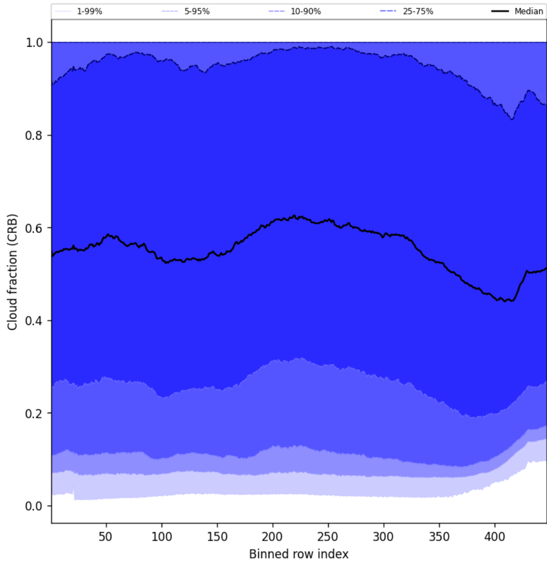
Figure 58: Along track statistics of “Cloud fraction (CRB)” for 2025-11-14 to 2025-11-16
