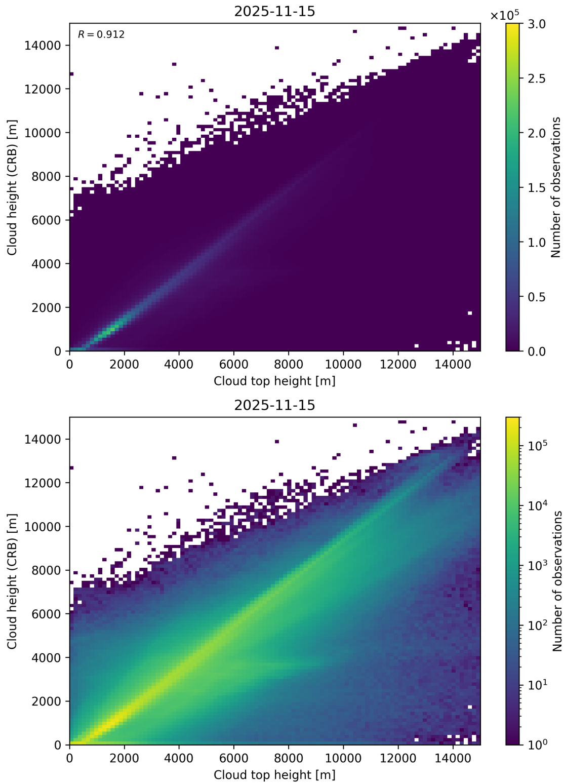
Figure 89: Scatter density plot of “Cloud top height” against “Cloud height (CRB)” for 2025-11-14 to 2025-11-16.
