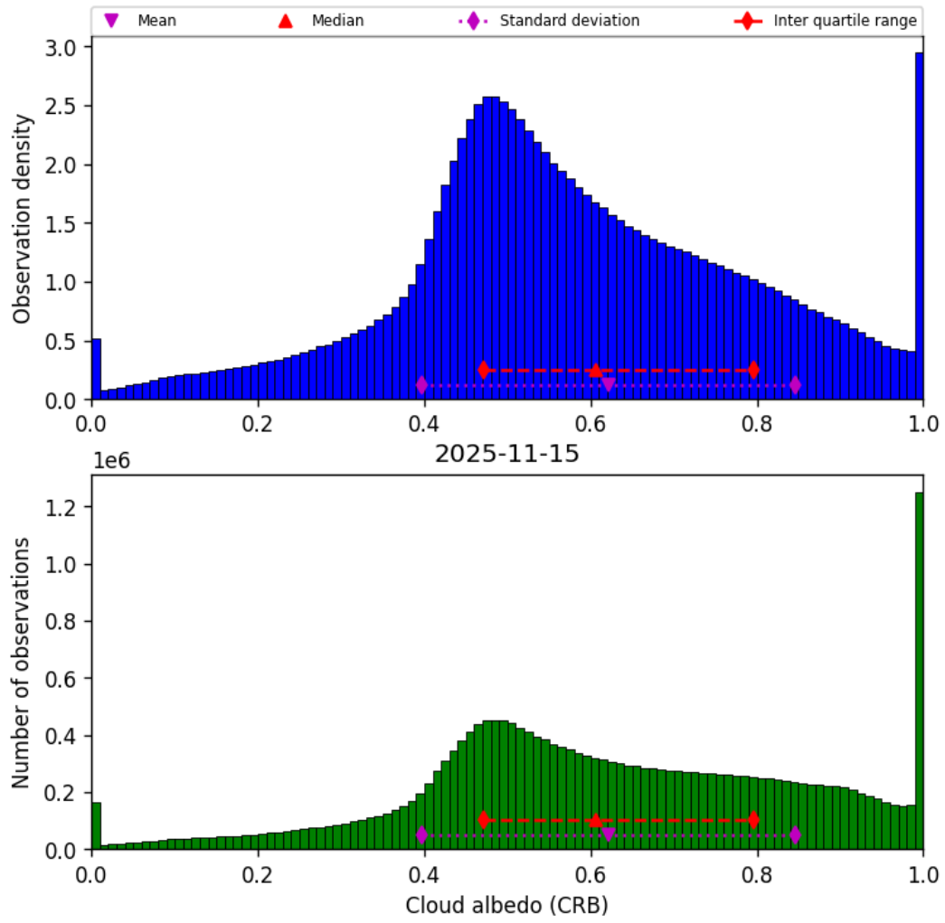
Figure 44: Histogram of “Cloud albedo (CRB)” for 2025-11-14 to 2025-11-16
