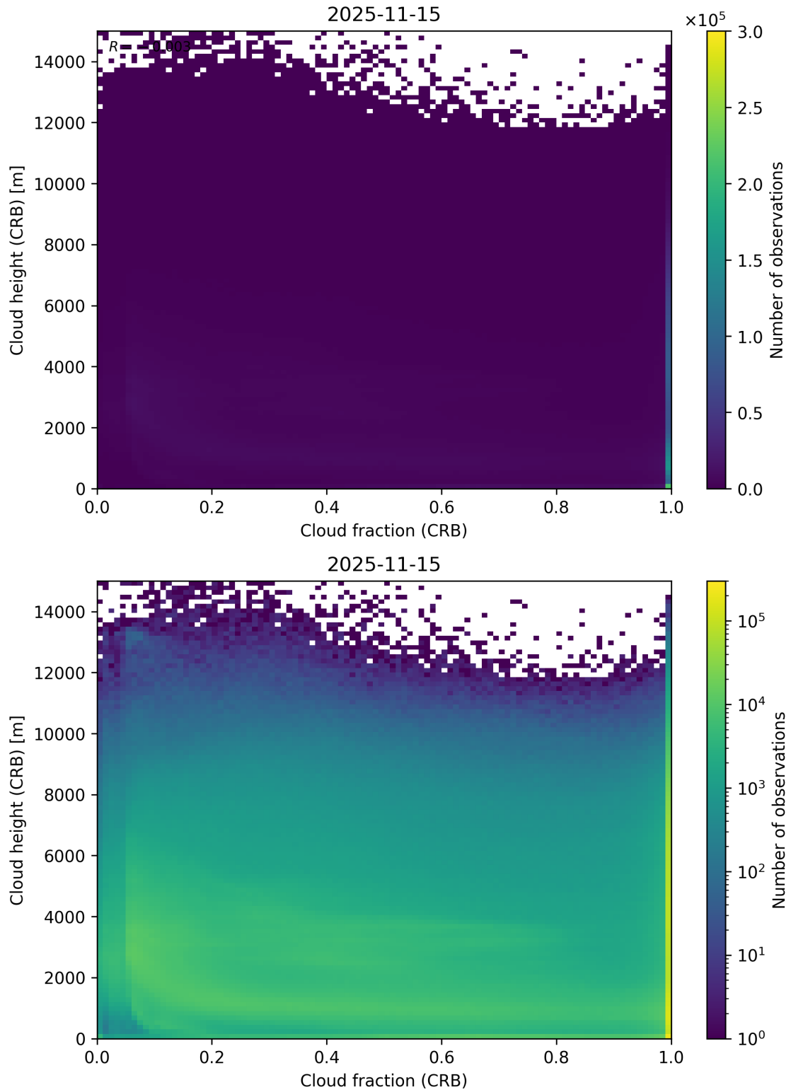
Figure 79: Scatter density plot of “Cloud fraction (CRB)” against “Cloud height (CRB)” for 2025-11-14 to 2025-11-16.
