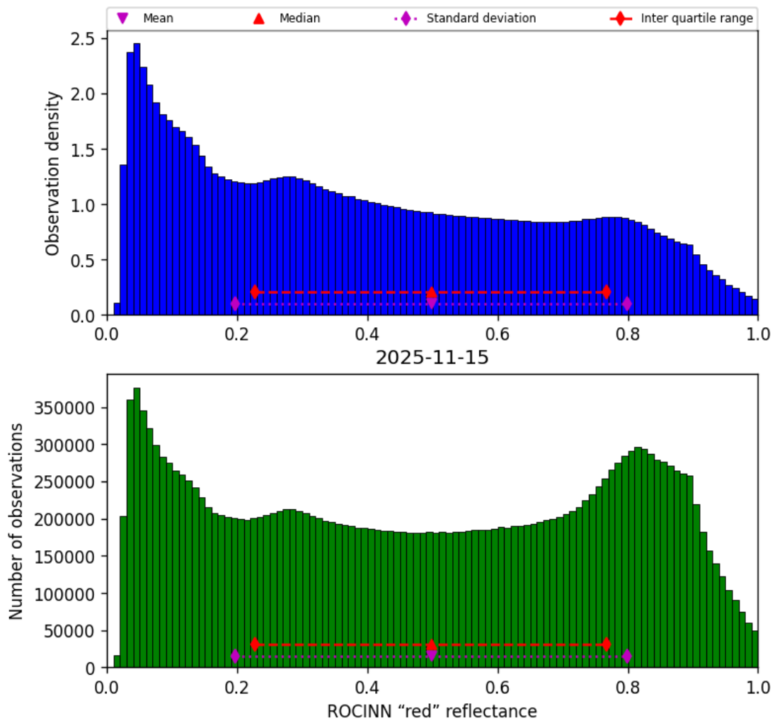
Figure 53: Histogram of “ROCINN “red” reflectance” for 2025-11-14 to 2025-11-16
