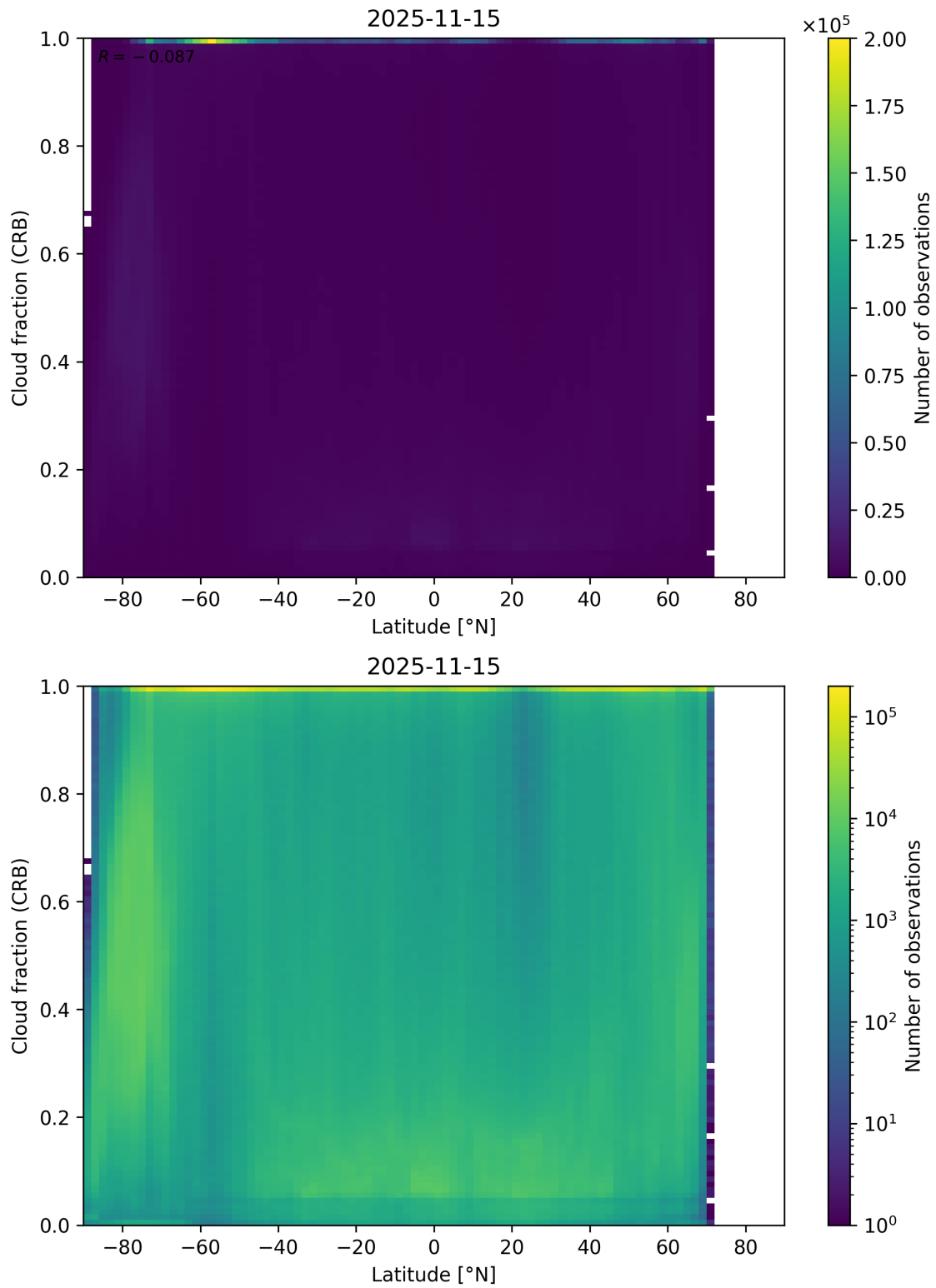
Figure 94: Scatter density plot of “Latitude” against “Cloud fraction (CRB)” for 2025-11-14 to 2025-11-16.
