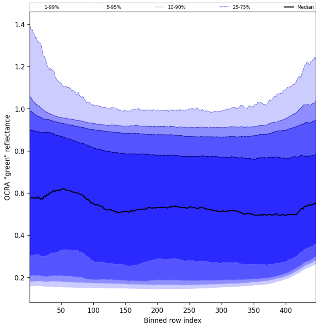
Figure 68: Along track statistics of “OCRA “green” reflectance” for 2025-11-14 to 2025-11-16
