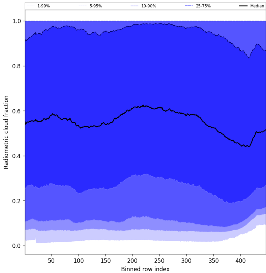
Figure 55: Along track statistics of “Radiometric cloud fraction” for 2025-11-14 to 2025-11-16
