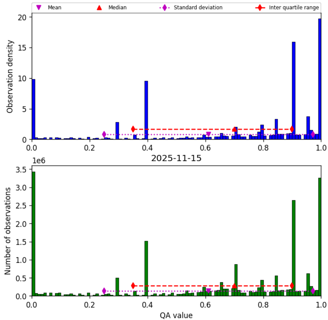
Figure 38: Histogram of “QA value” for 2025-11-14 to 2025-11-16
