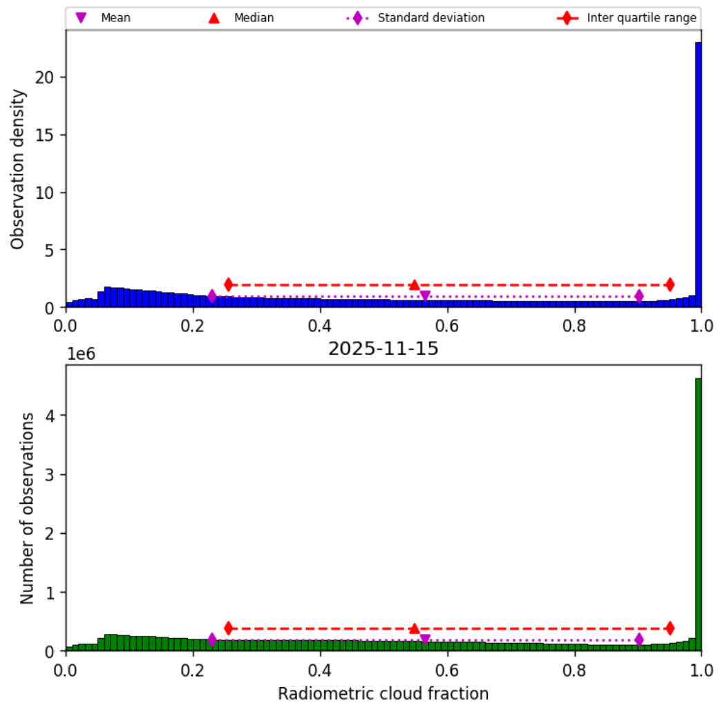
Figure 39: Histogram of “Radiometric cloud fraction” for 2025-11-14 to 2025-11-16
