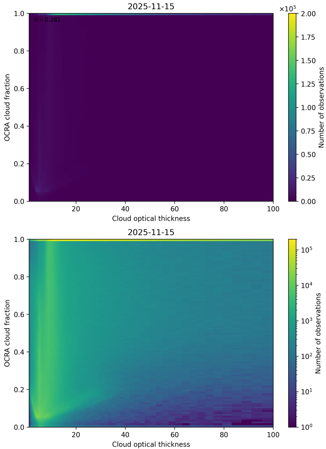
Figure 83: Scatter density plot of “Cloud optical thickness” against “OCRA cloud fraction” for 2025-11-14 to 2025-11-16.
