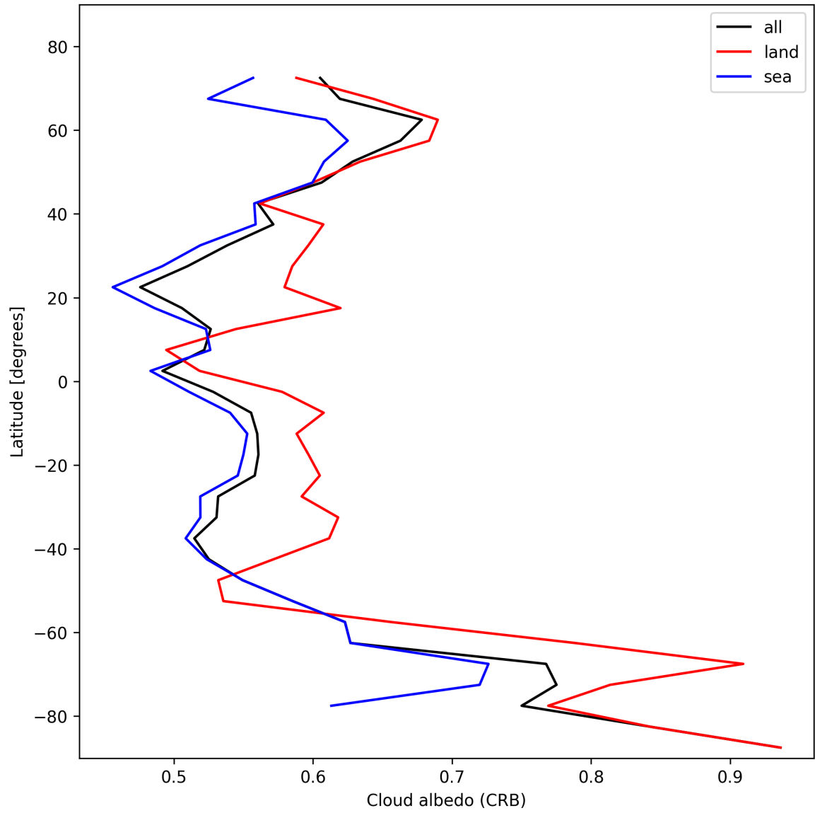
Figure 28: Zonal average of “Cloud albedo (CRB)” for 2025-11-14 to 2025-11-16.
