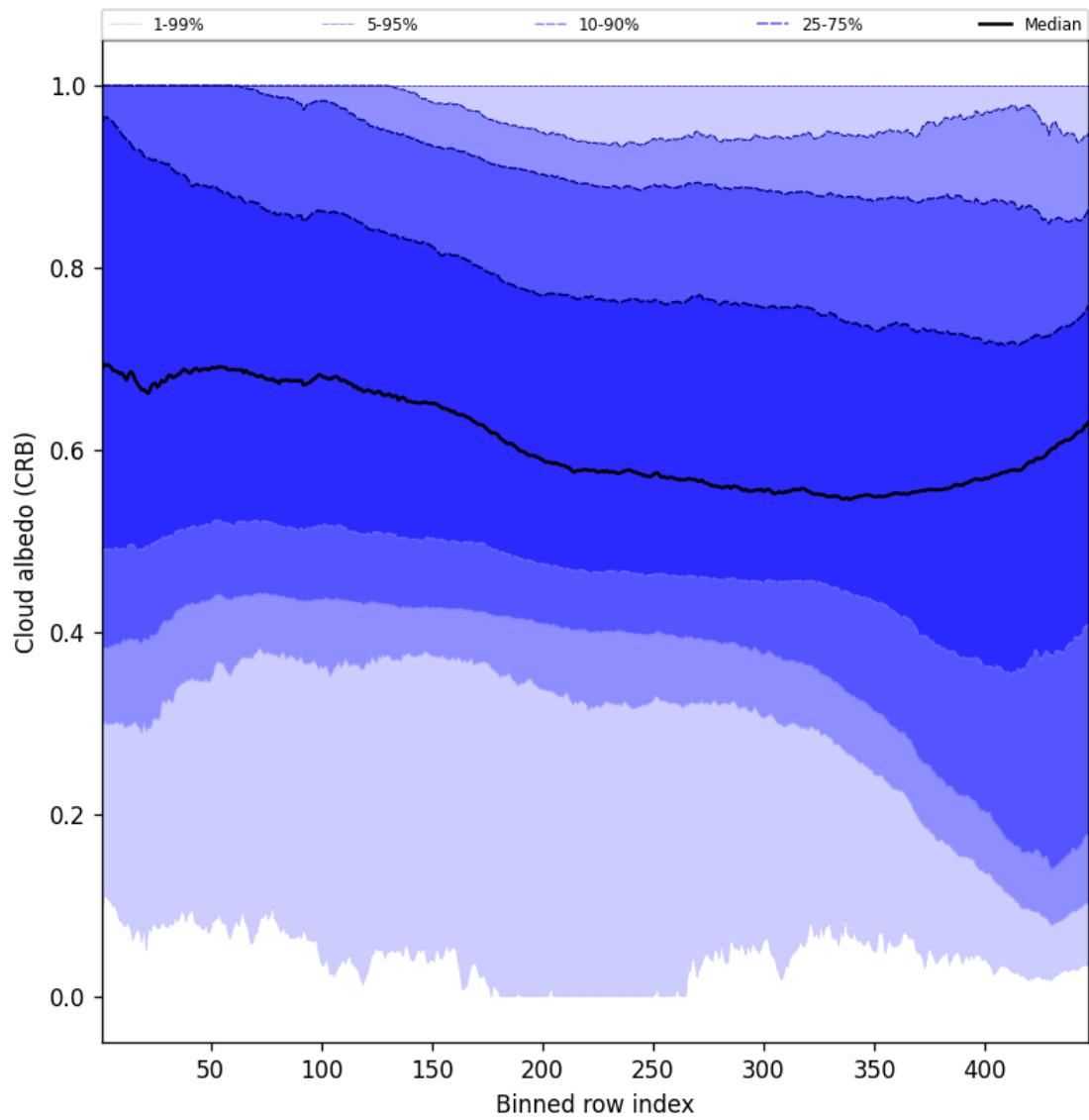
Figure 60: Along track statistics of “Cloud albedo (CRB)” for 2025-11-14 to 2025-11-16
