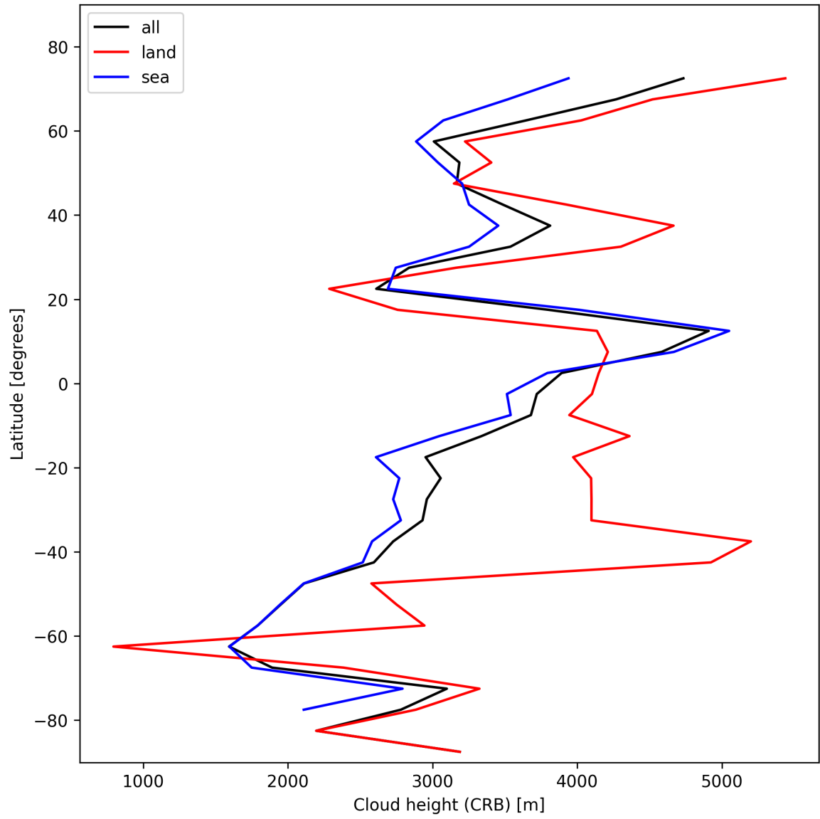
Figure 27: Zonal average of “Cloud height (CRB)” for 2025-11-14 to 2025-11-16.
