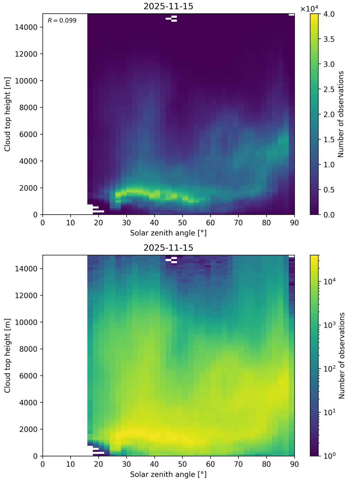
Figure 104: Scatter density plot of “Solar zenith angle” against “Cloud top height” for 2025-11-14 to 2025-11-16.
