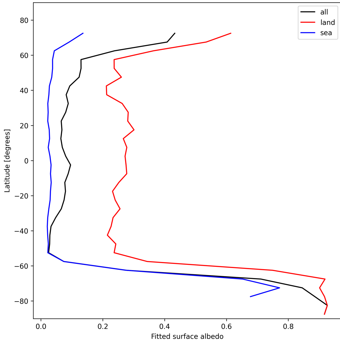
Figure 29: Zonal average of “Fitted surface albedo” for 2025-11-14 to 2025-11-16.
