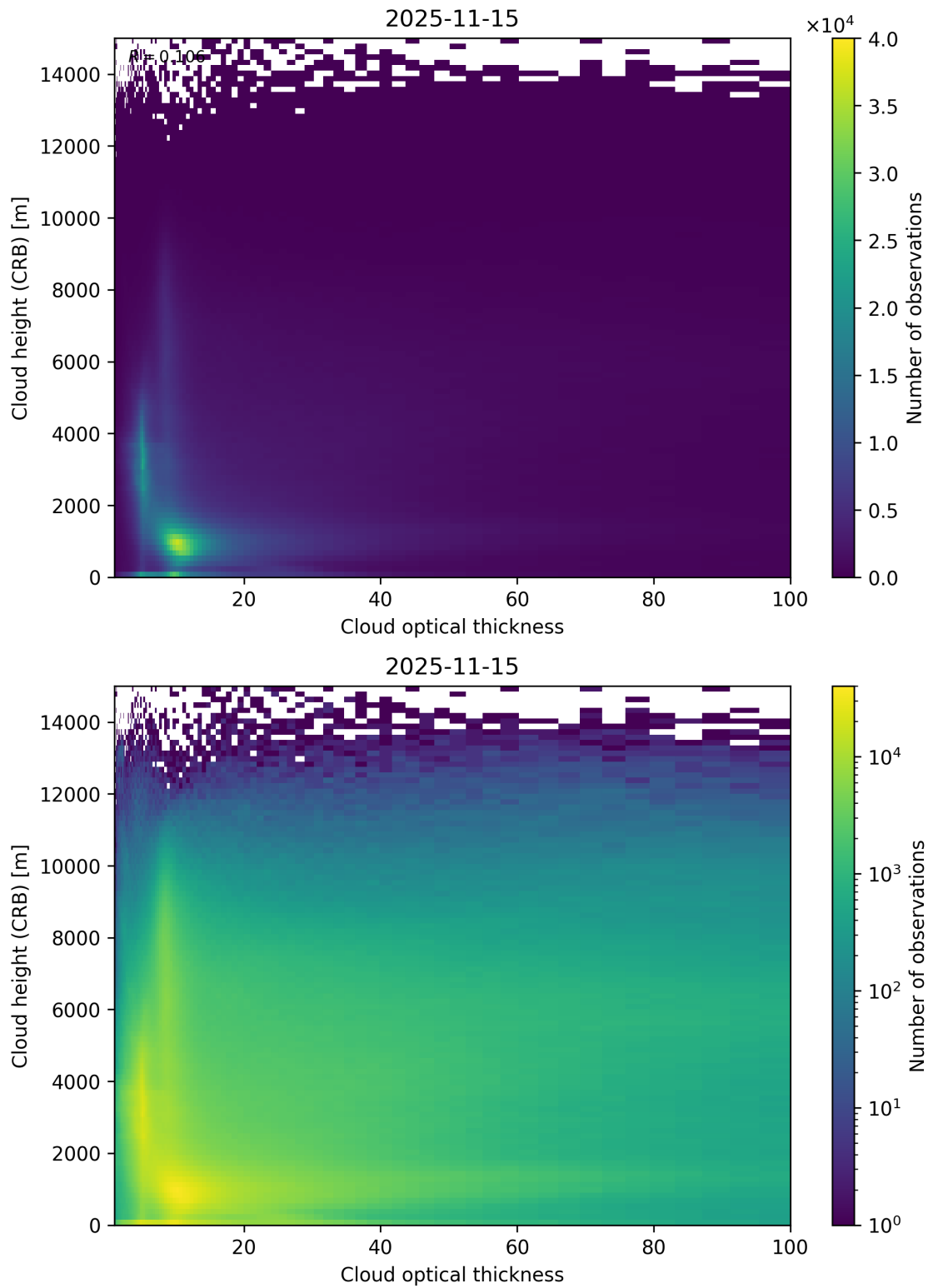
Figure 85: Scatter density plot of “Cloud optical thickness” against “Cloud height (CRB)” for 2025-11-14 to 2025-11-16.
