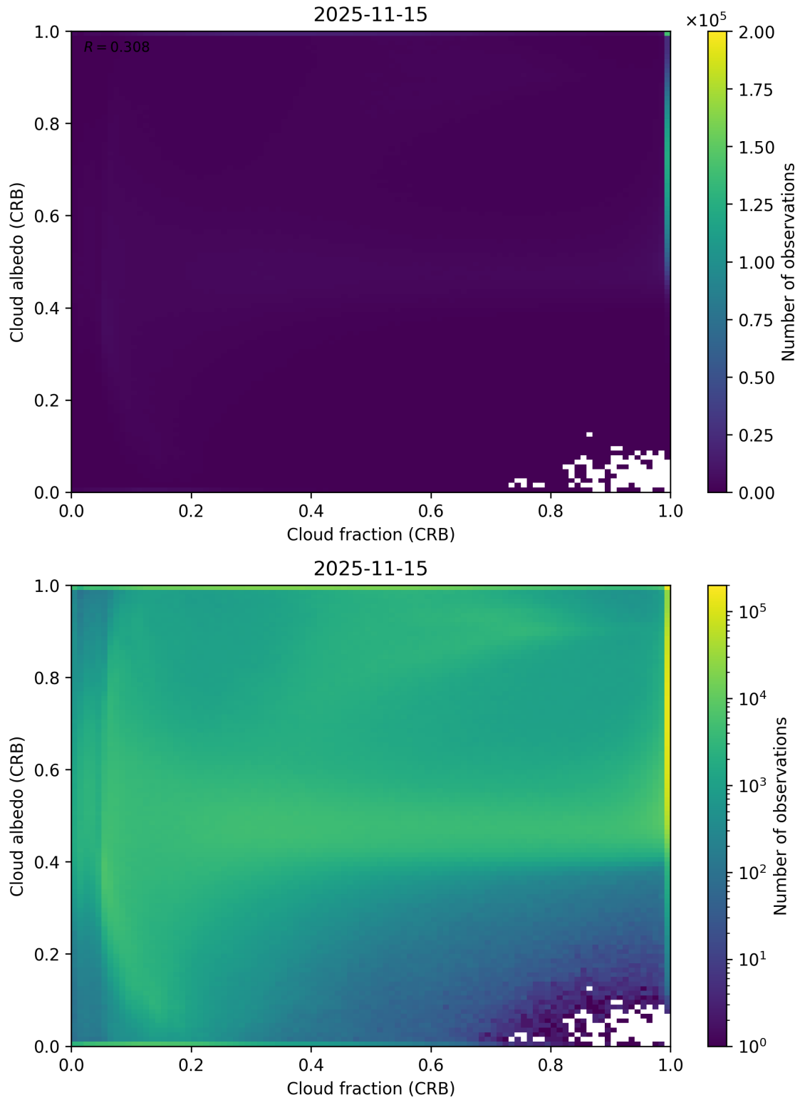
Figure 77: Scatter density plot of “Cloud fraction (CRB)” against “Cloud albedo (CRB)” for 2025-11-14 to 2025-11-16.
