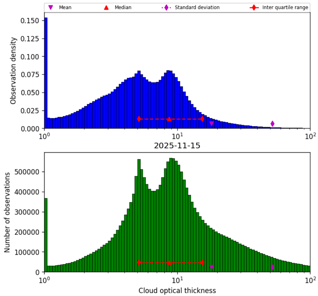
Figure 41: Histogram of “Cloud optical thickness” for 2025-11-14 to 2025-11-16
