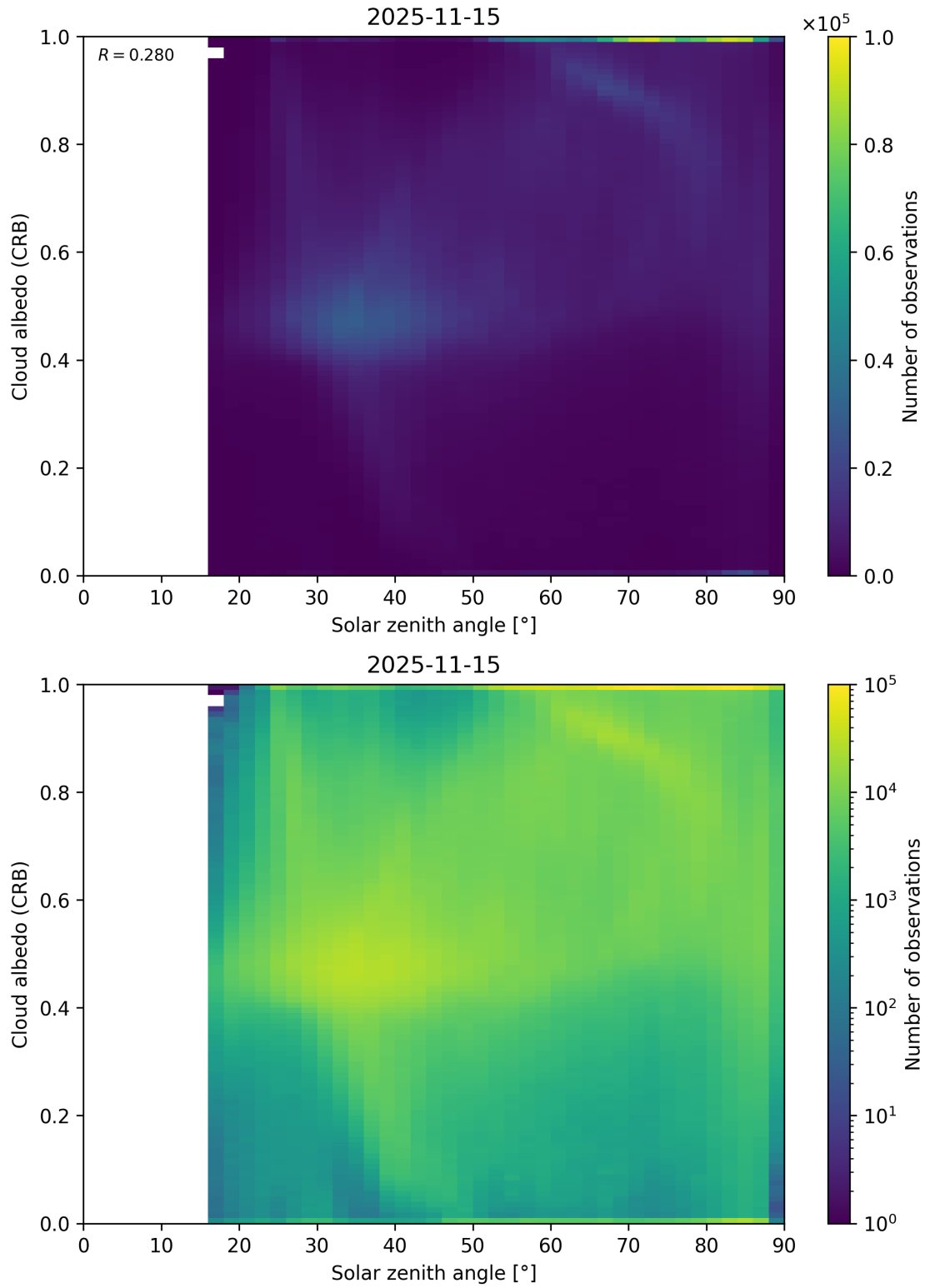
Figure 98: Scatter density plot of “Solar zenith angle” against “Cloud albedo (CRB)” for 2025-11-14 to 2025-11-16.
