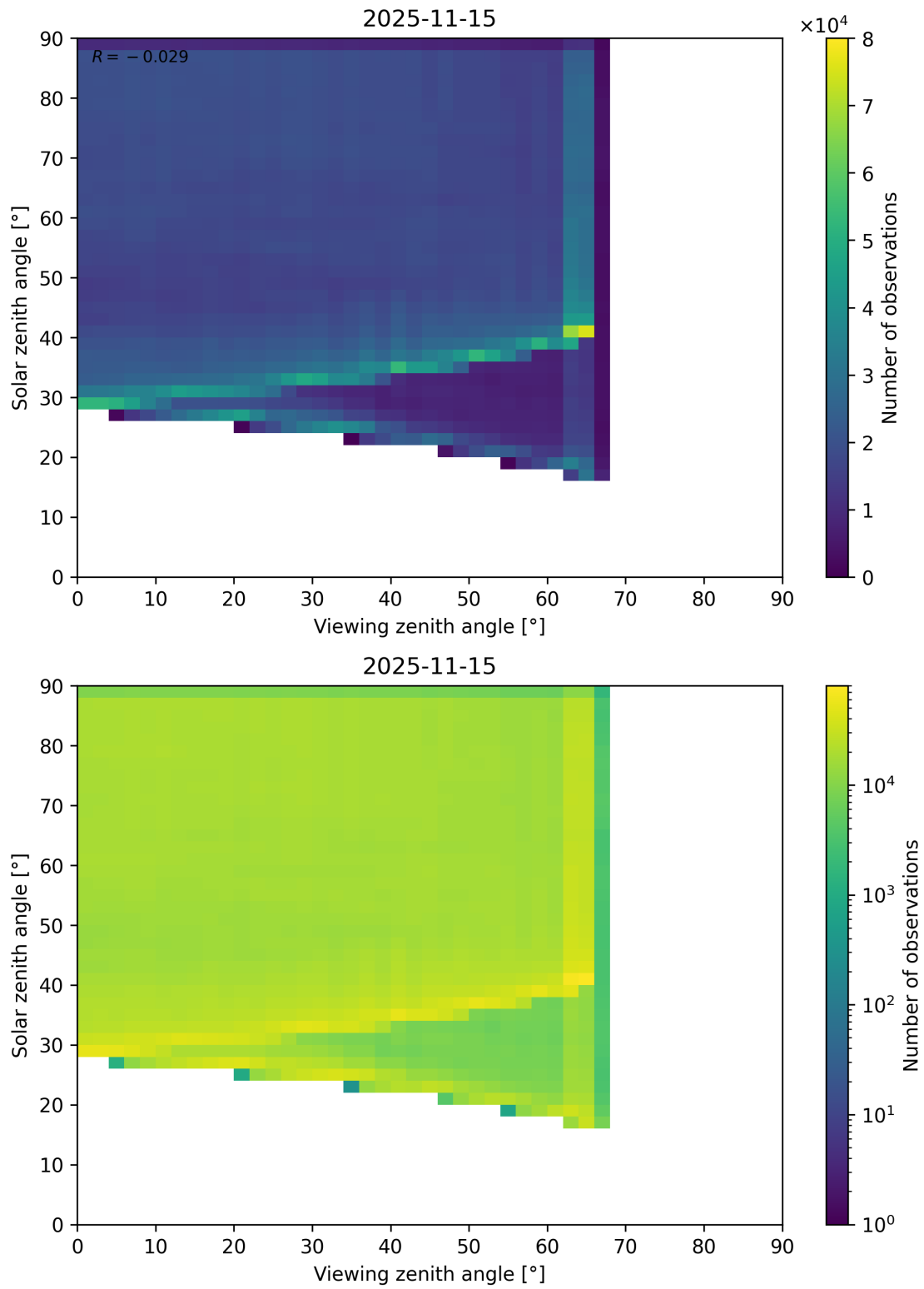
Figure 114: Scatter density plot of “Viewing zenith angle” against “Solar zenith angle” for 2025-11-14 to 2025-11-16.
