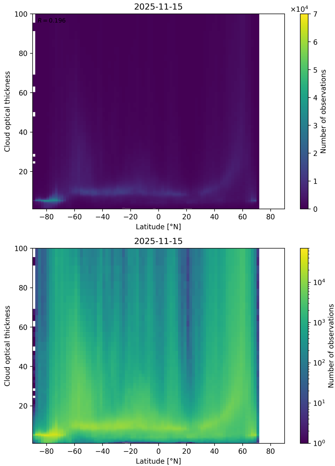
Figure 96: Scatter density plot of “Latitude” against “Cloud optical thickness” for 2025-11-14 to 2025-11-16.
