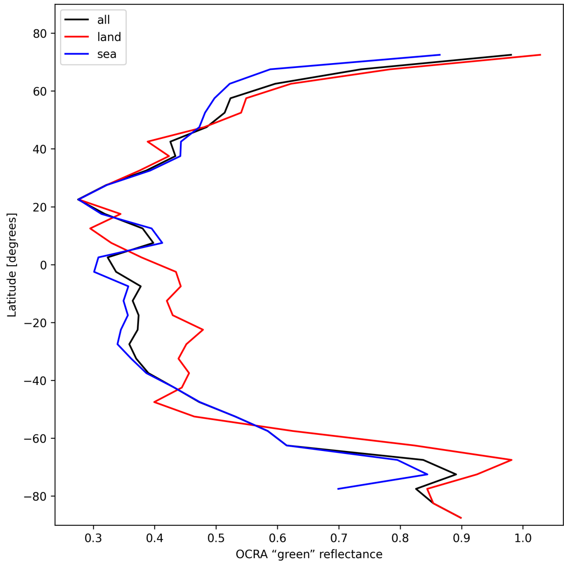
Figure 36: Zonal average of “OCRA “green” reflectance” for 2025-11-14 to 2025-11-16.
