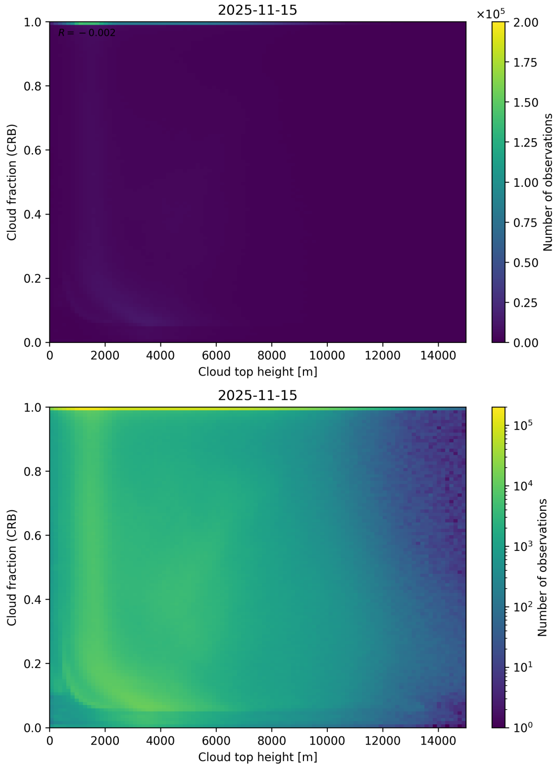
Figure 88: Scatter density plot of “Cloud top height” against “Cloud fraction (CRB)” for 2025-11-14 to 2025-11-16.
