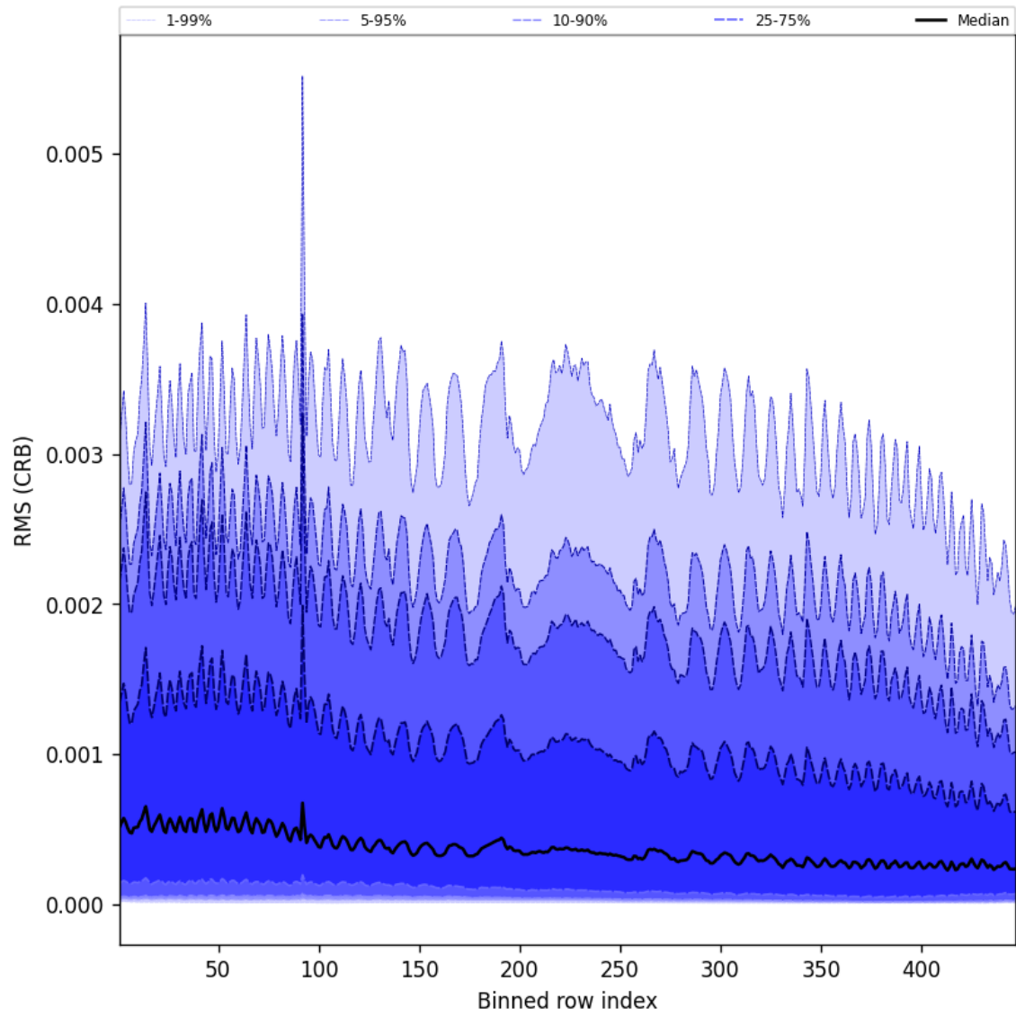
Figure 64: Along track statistics of “RMS (CRB)” for 2025-11-14 to 2025-11-16
