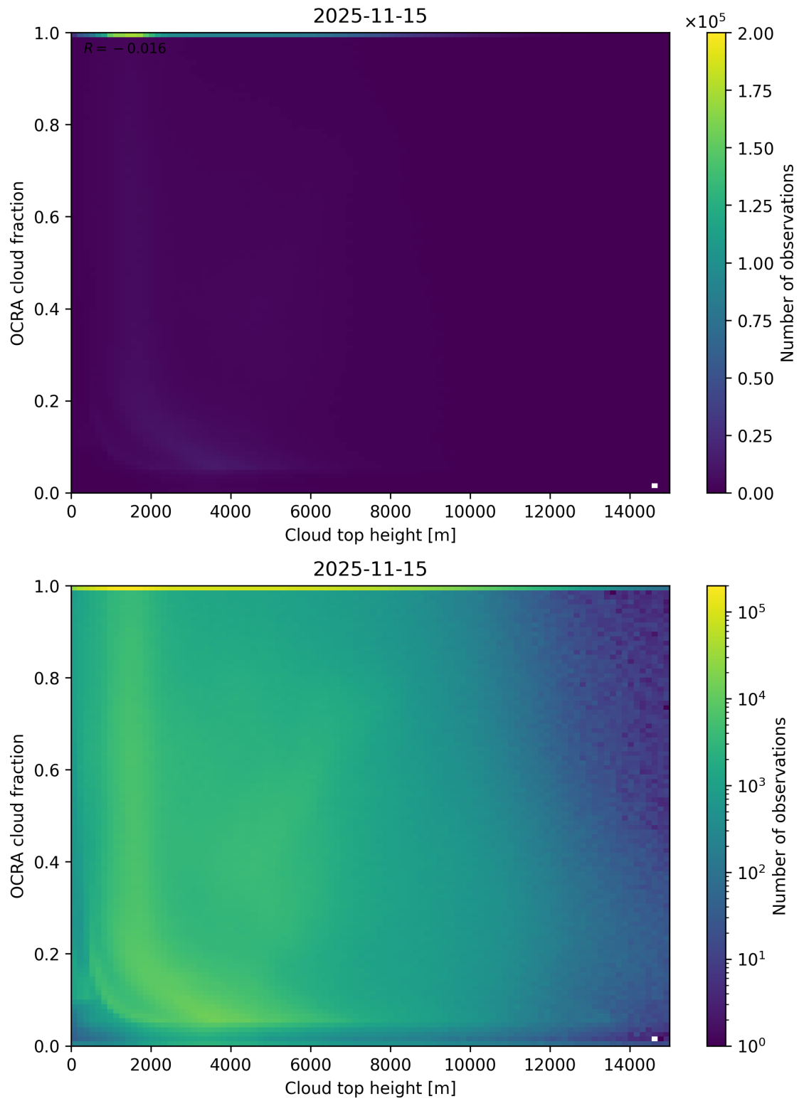
Figure 87: Scatter density plot of “Cloud top height” against “OCRA cloud fraction” for 2025-11-14 to 2025-11-16.
