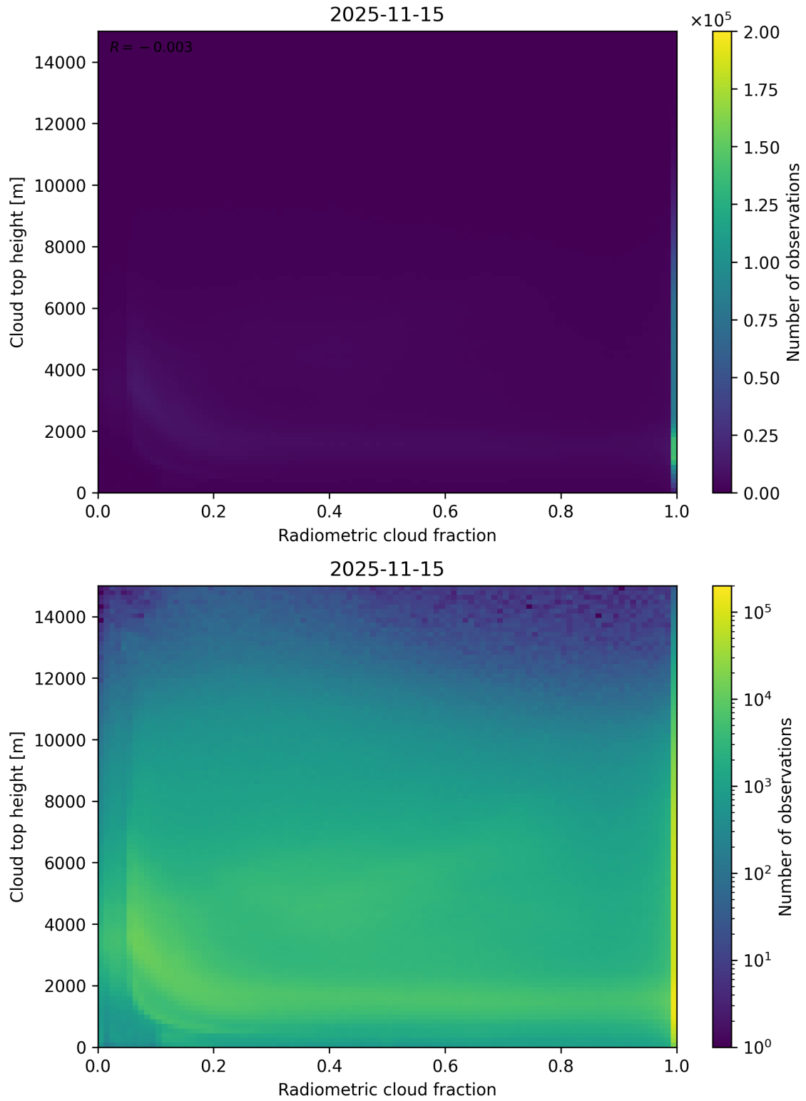
Figure 76: Scatter density plot of “Radiometric cloud fraction” against “Cloud top height” for 2025-11-14 to 2025-11-16.
