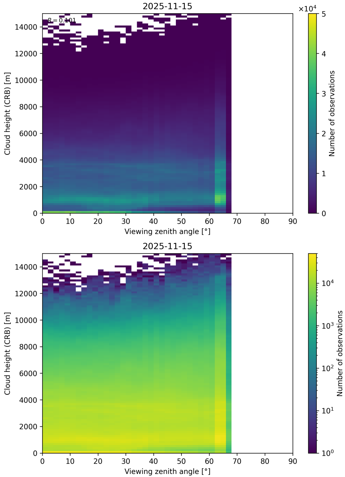
Figure 110: Scatter density plot of “Viewing zenith angle” against “Cloud height (CRB)” for 2025-11-14 to 2025-11-16.
