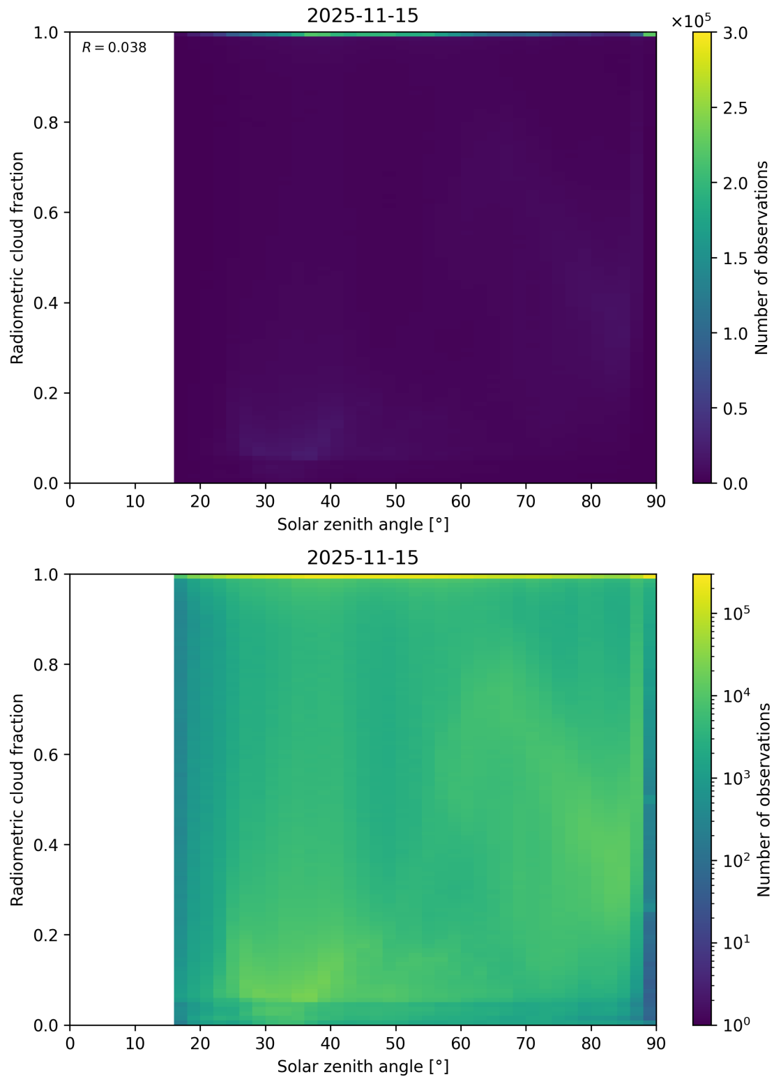
Figure 99: Scatter density plot of “Solar zenith angle” against “Radiometric cloud fraction” for 2025-11-14 to 2025-11-16.
