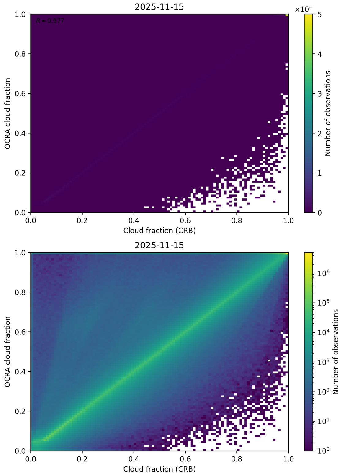
Figure 78: Scatter density plot of “Cloud fraction (CRB)” against “OCRA cloud fraction” for 2025-11-14 to 2025-11-16.
