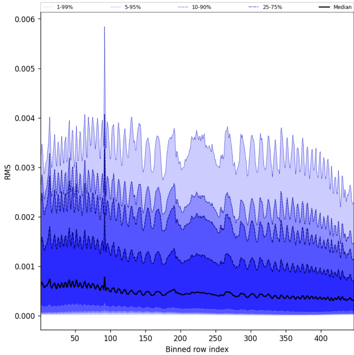
Figure 63: Along track statistics of “RMS” for 2025-11-14 to 2025-11-16
