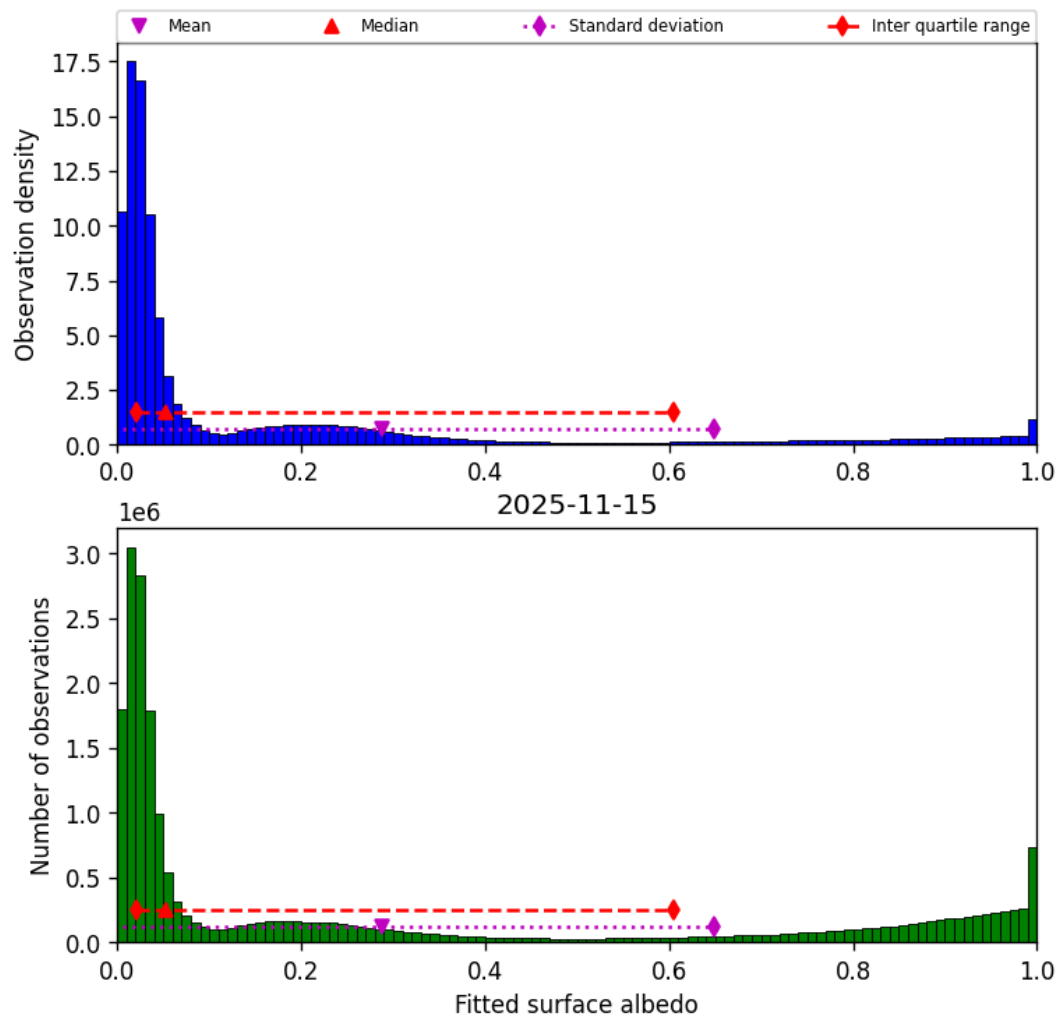
Figure 45: Histogram of “Fitted surface albedo” for 2025-11-14 to 2025-11-16
