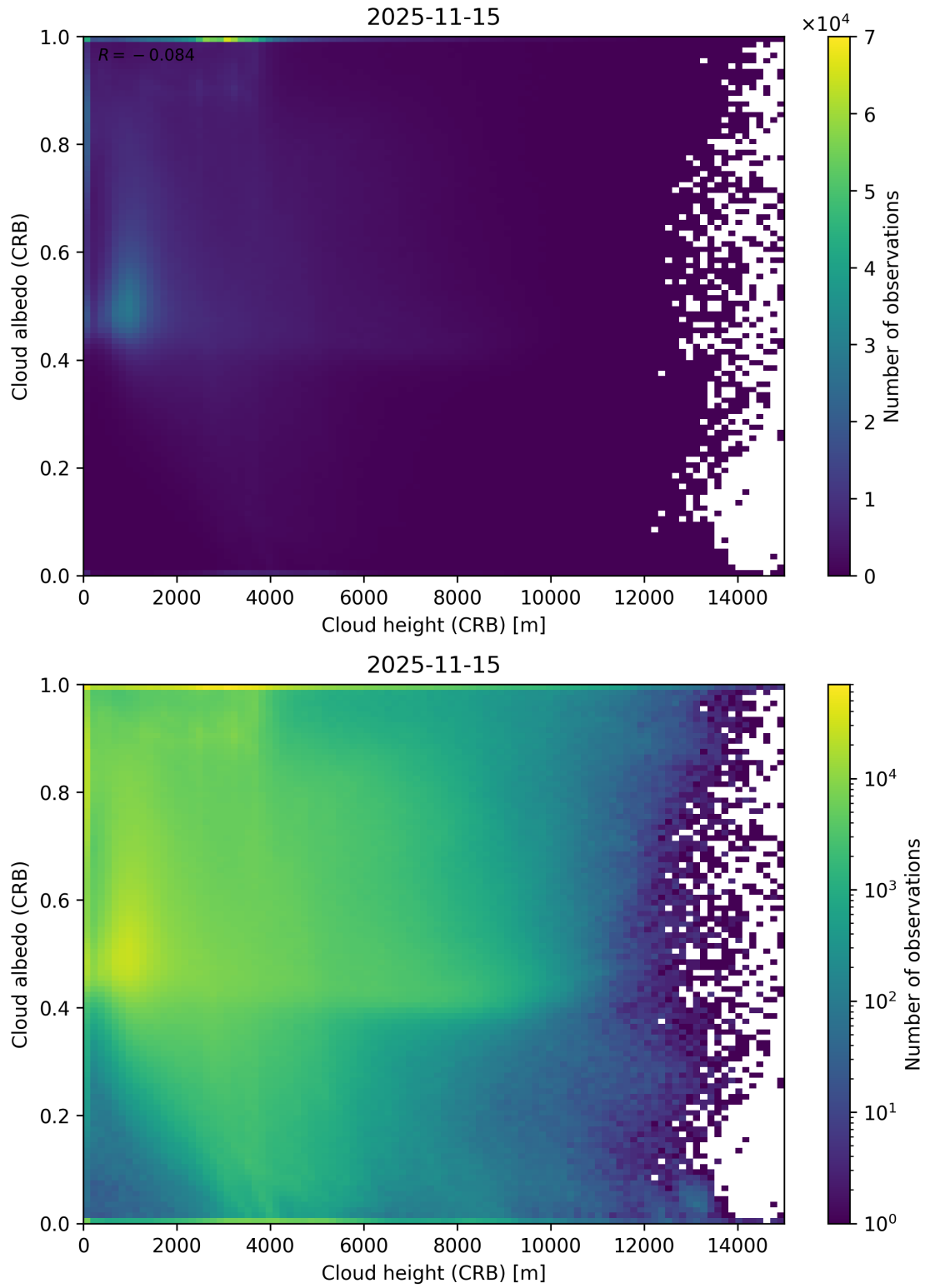
Figure 80: Scatter density plot of “Cloud height (CRB)” against “Cloud albedo (CRB)” for 2025-11-14 to 2025-11-16.
