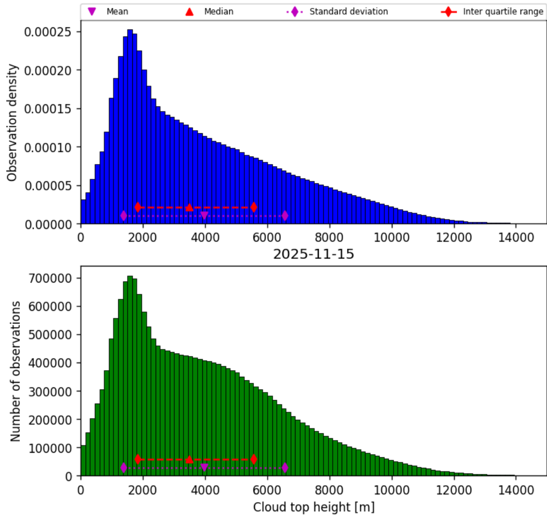
Figure 40: Histogram of “Cloud top height” for 2025-11-14 to 2025-11-16
