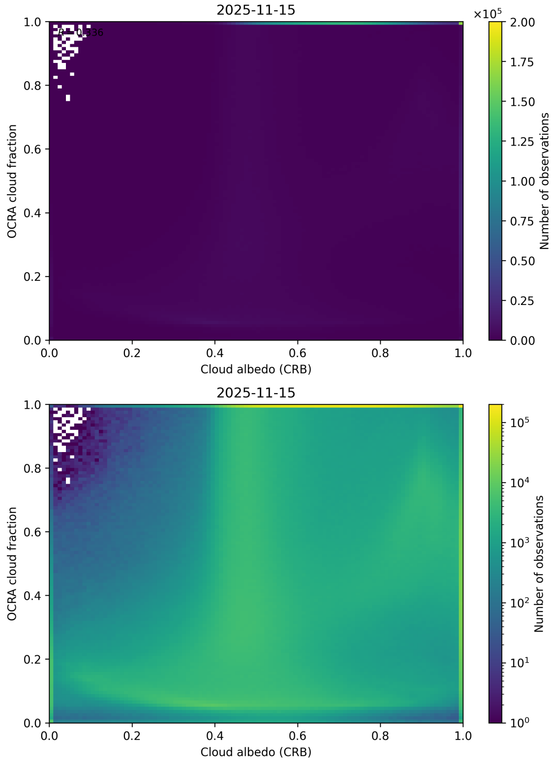
Figure 70: Scatter density plot of “Cloud albedo (CRB)” against “OCRA cloud fraction” for 2025-11-14 to 2025-11-16.
