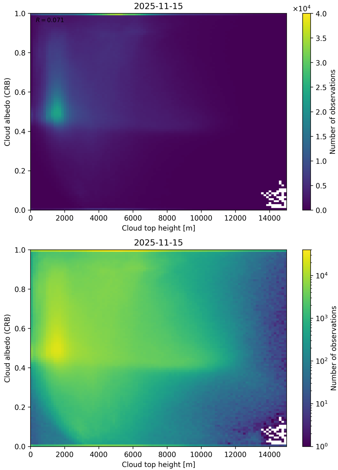
Figure 86: Scatter density plot of “Cloud top height” against “Cloud albedo (CRB)” for 2025-11-14 to 2025-11-16.
