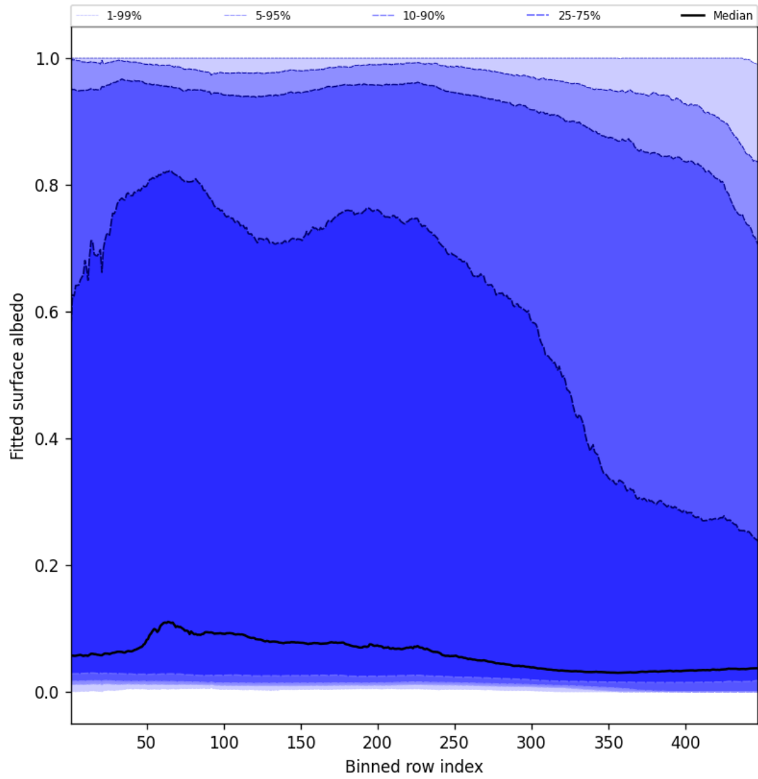
Figure 61: Along track statistics of “Fitted surface albedo” for 2025-11-14 to 2025-11-16
