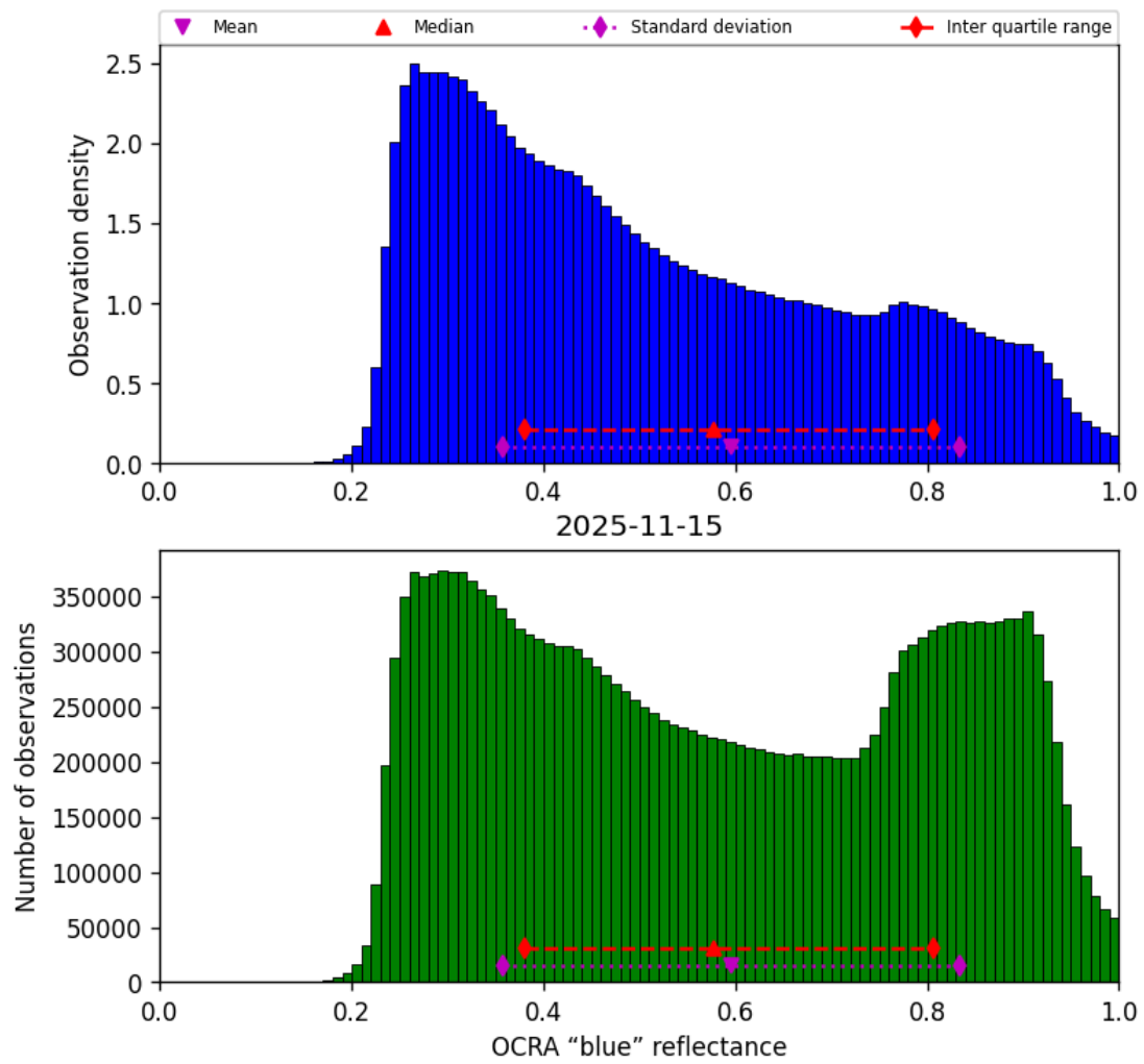
Figure 51: Histogram of “OCRA “blue” reflectance” for 2025-11-14 to 2025-11-16
