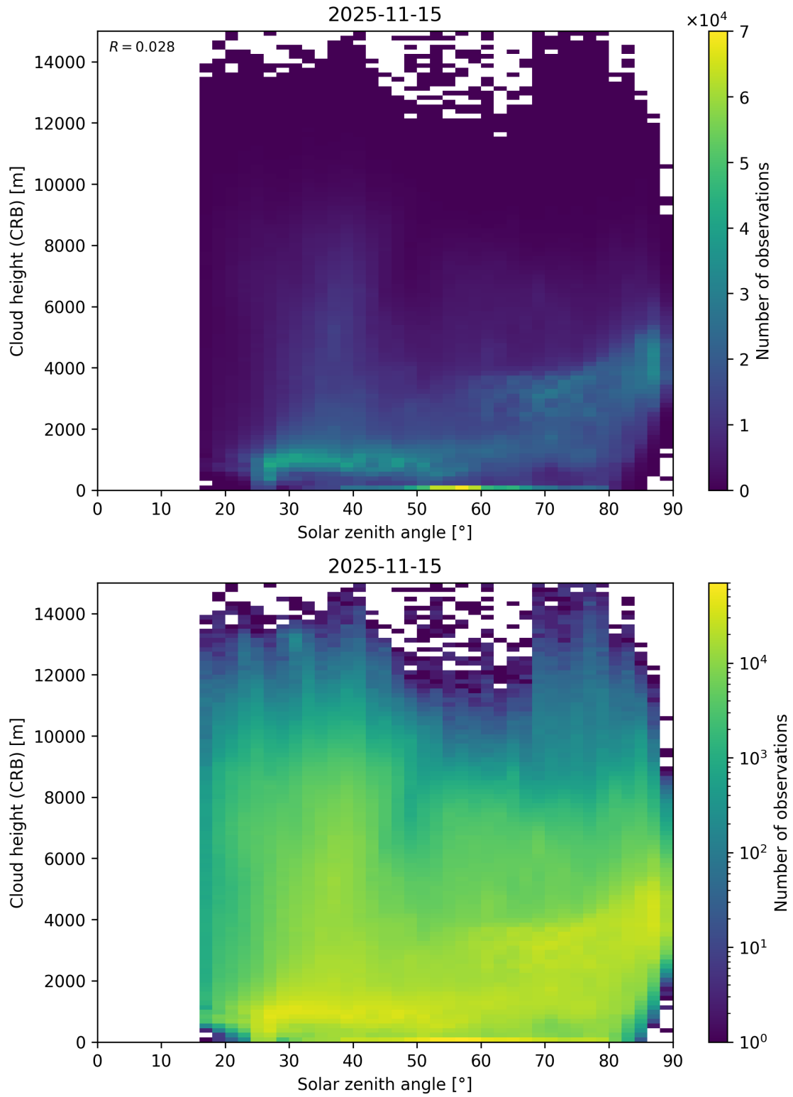
Figure 102: Scatter density plot of “Solar zenith angle” against “Cloud height (CRB)” for 2025-11-14 to 2025-11-16.
