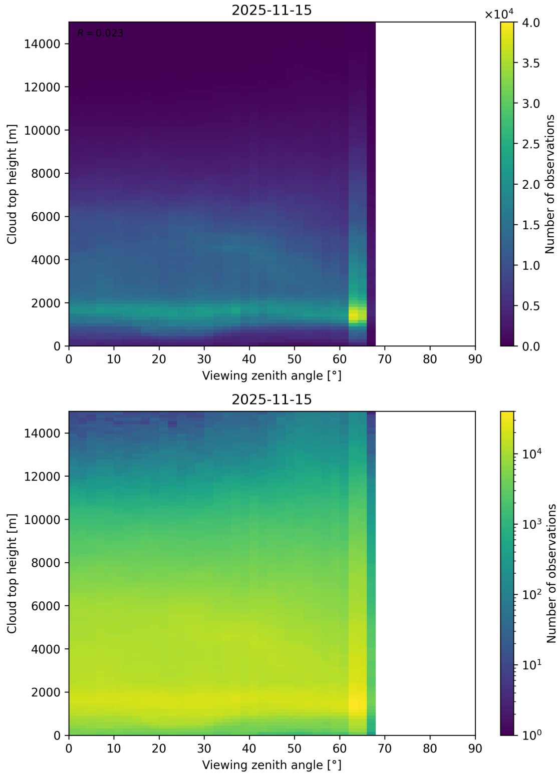
Figure 112: Scatter density plot of “Viewing zenith angle” against “Cloud top height” for 2025-11-14 to 2025-11-16.
