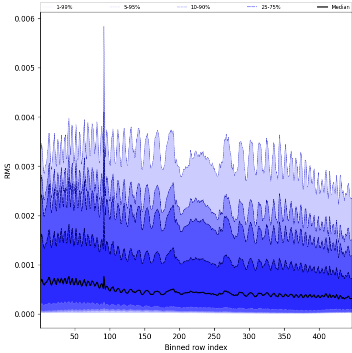
Figure 63: Along track statistics of “RMS” for 2025-11-15 to 2025-11-17
