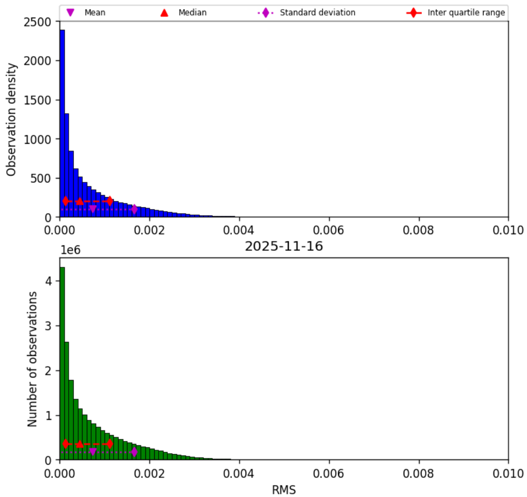
Figure 47: Histogram of “RMS” for 2025-11-15 to 2025-11-17
