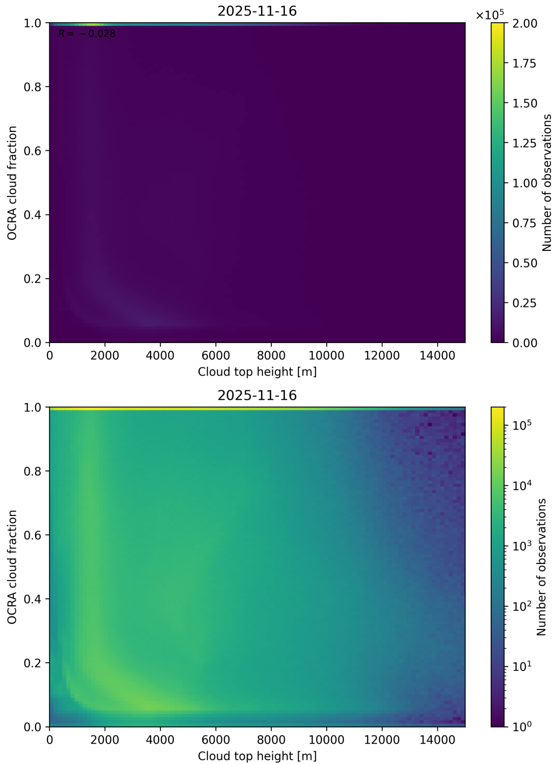
Figure 87: Scatter density plot of “Cloud top height” against “OCRA cloud fraction” for 2025-11-15 to 2025-11-17.
