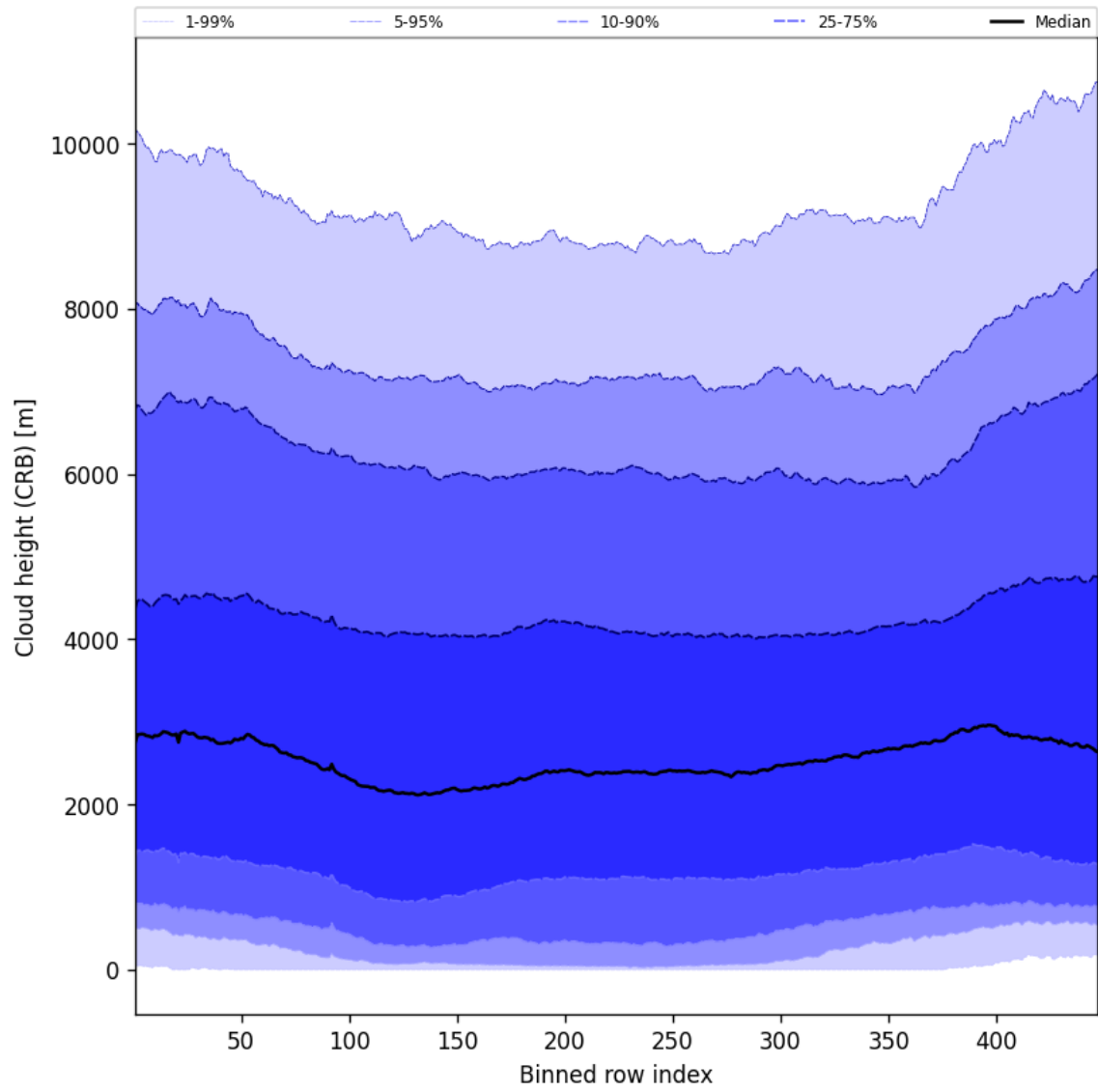
Figure 59: Along track statistics of “Cloud height (CRB)” for 2025-11-15 to 2025-11-17
