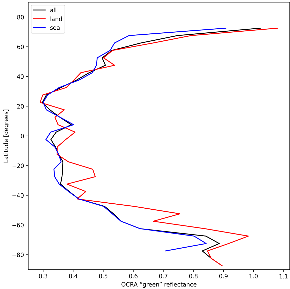
Figure 36: Zonal average of “OCRA “green” reflectance” for 2025-11-15 to 2025-11-17.
