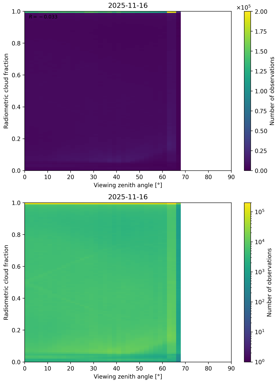
Figure 107: Scatter density plot of “Viewing zenith angle” against “Radiometric cloud fraction” for 2025-11-15 to 2025-11-17.
