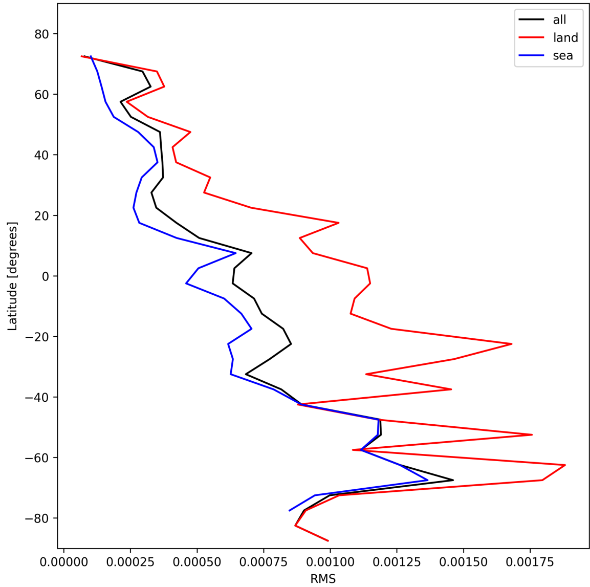
Figure 31: Zonal average of “RMS” for 2025-11-15 to 2025-11-17.
