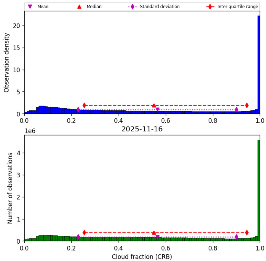
Figure 42: Histogram of “Cloud fraction (CRB)” for 2025-11-15 to 2025-11-17
