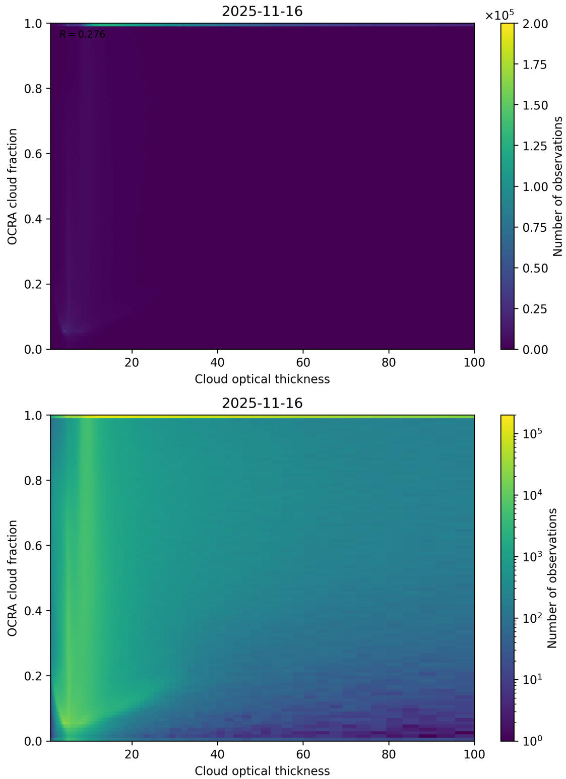
Figure 83: Scatter density plot of “Cloud optical thickness” against “OCRA cloud fraction” for 2025-11-15 to 2025-11-17.
