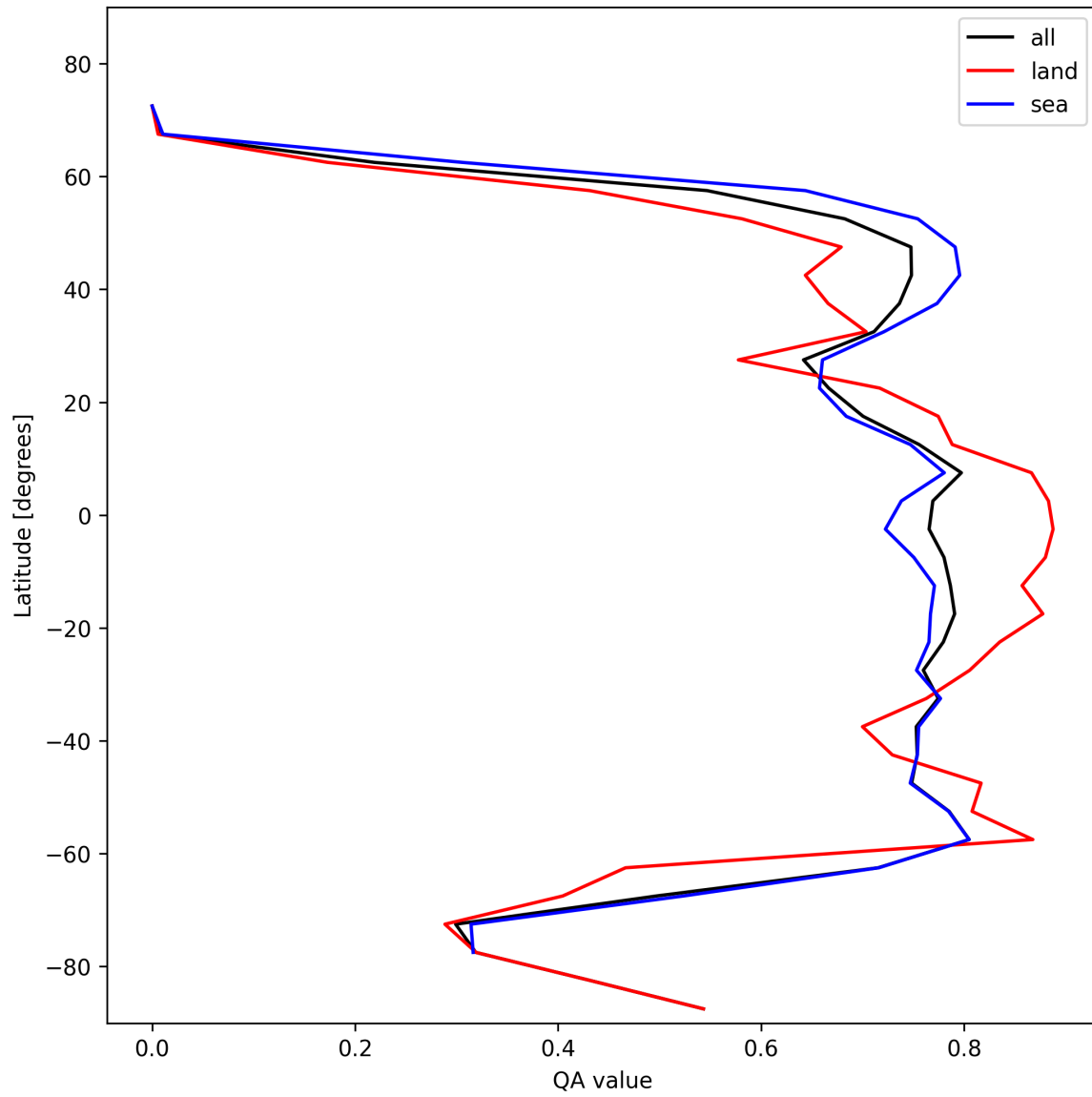
Figure 22: Zonal average of “QA value” for 2025-11-15 to 2025-11-17.
