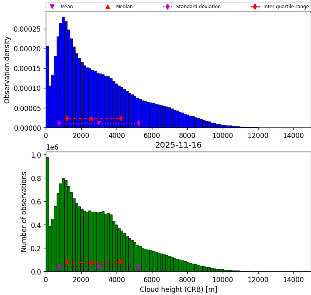
Figure 43: Histogram of “Cloud height (CRB)” for 2025-11-15 to 2025-11-17
