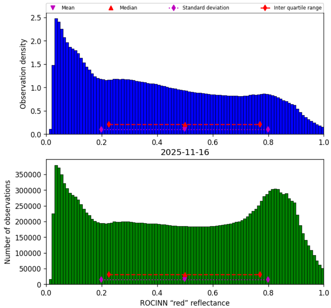
Figure 53: Histogram of “ROCINN “red” reflectance” for 2025-11-15 to 2025-11-17
