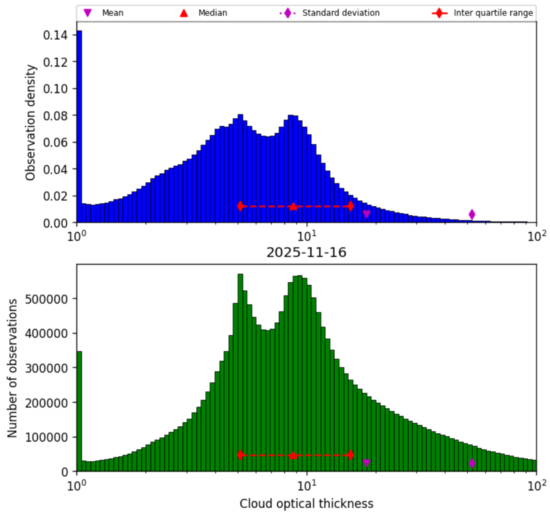
Figure 41: Histogram of “Cloud optical thickness” for 2025-11-15 to 2025-11-17
