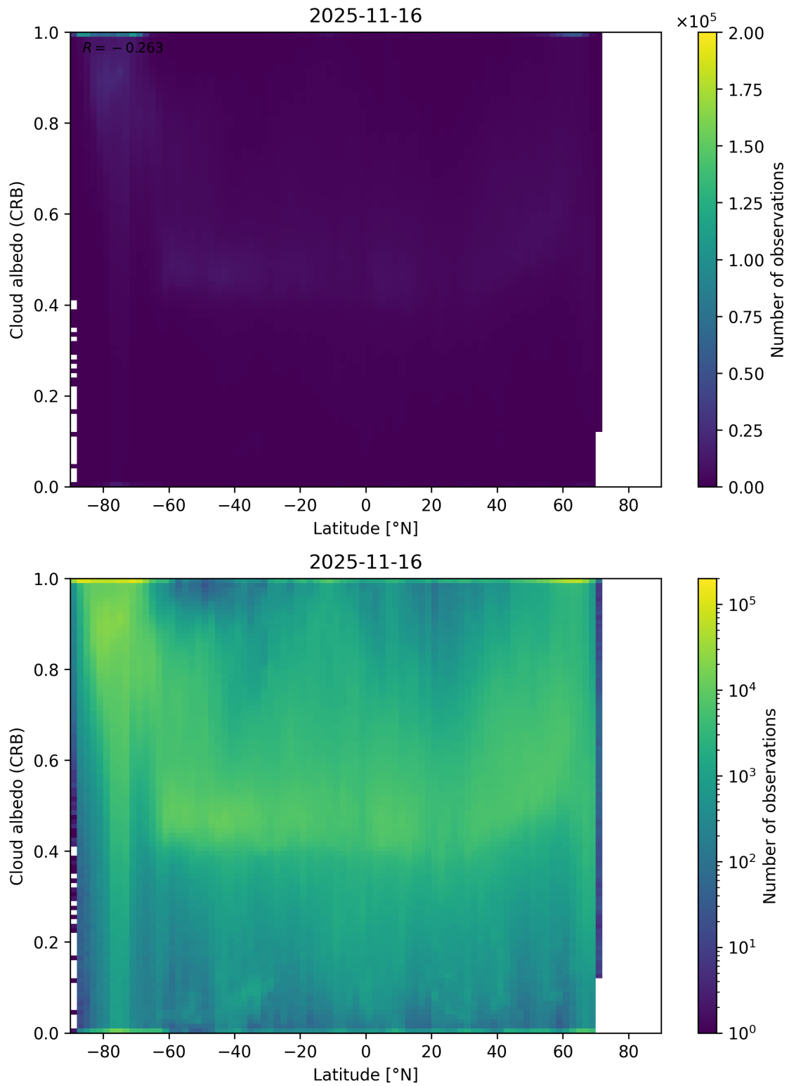
Figure 91: Scatter density plot of “Latitude” against “Cloud albedo (CRB)” for 2025-11-15 to 2025-11-17.
