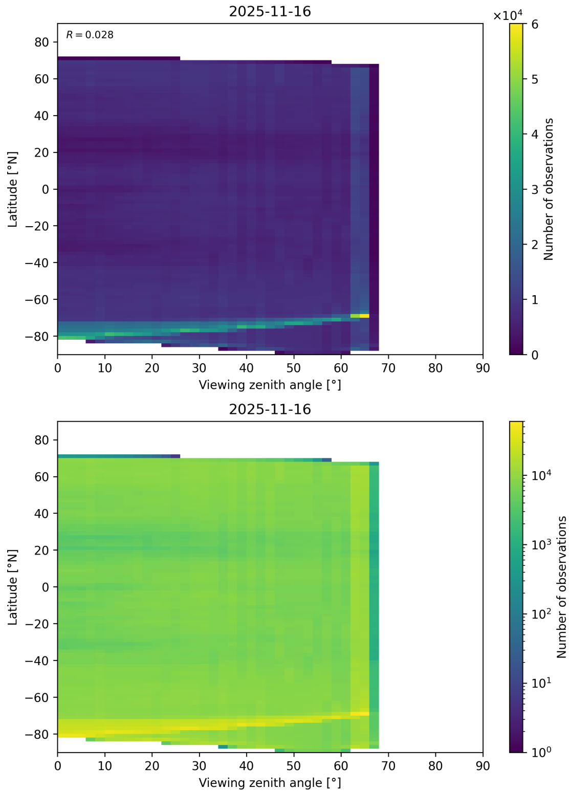
Figure 113: Scatter density plot of “Viewing zenith angle” against “Latitude” for 2025-11-15 to 2025-11-17.
