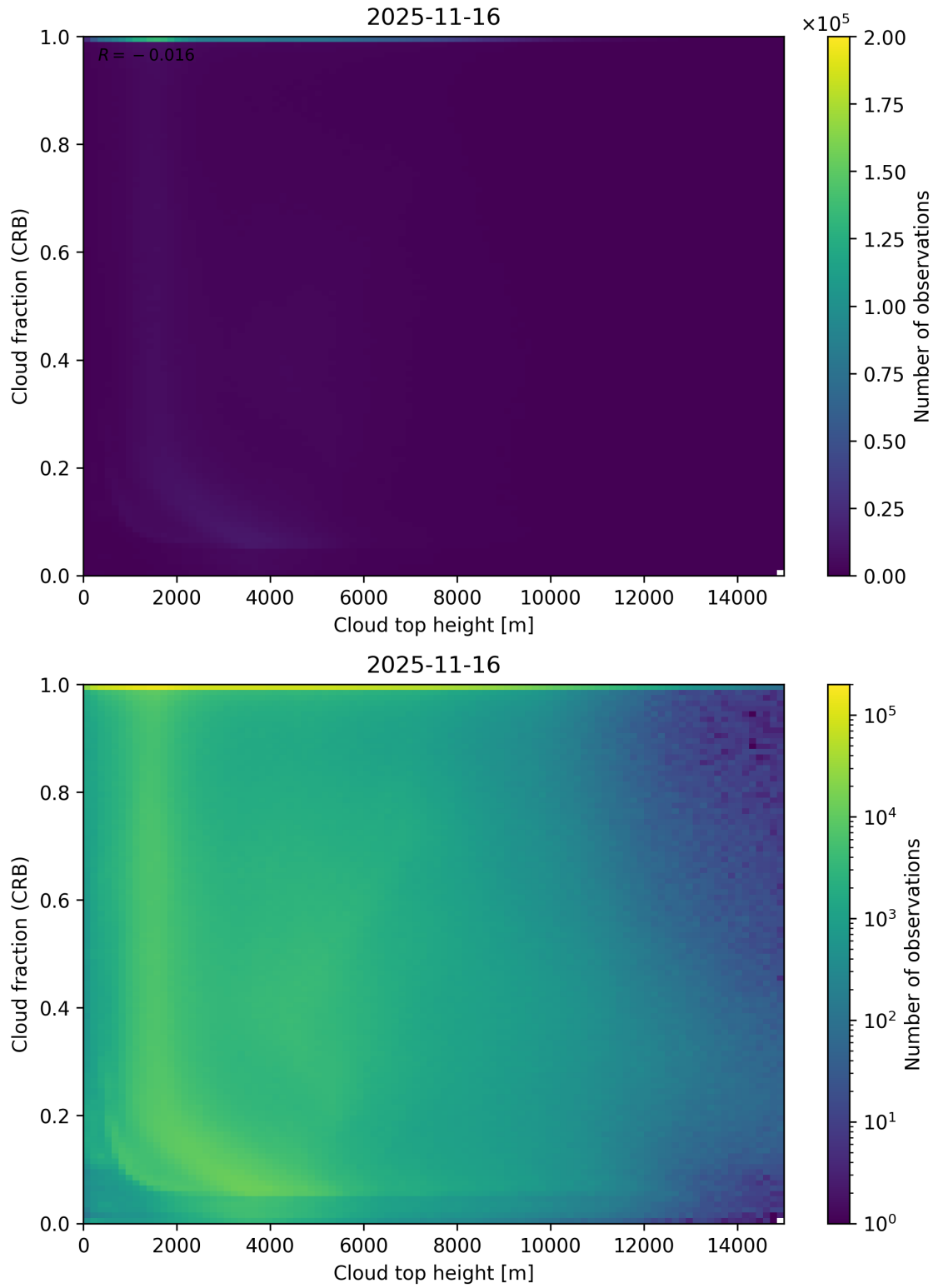
Figure 88: Scatter density plot of “Cloud top height” against “Cloud fraction (CRB)” for 2025-11-15 to 2025-11-17.
