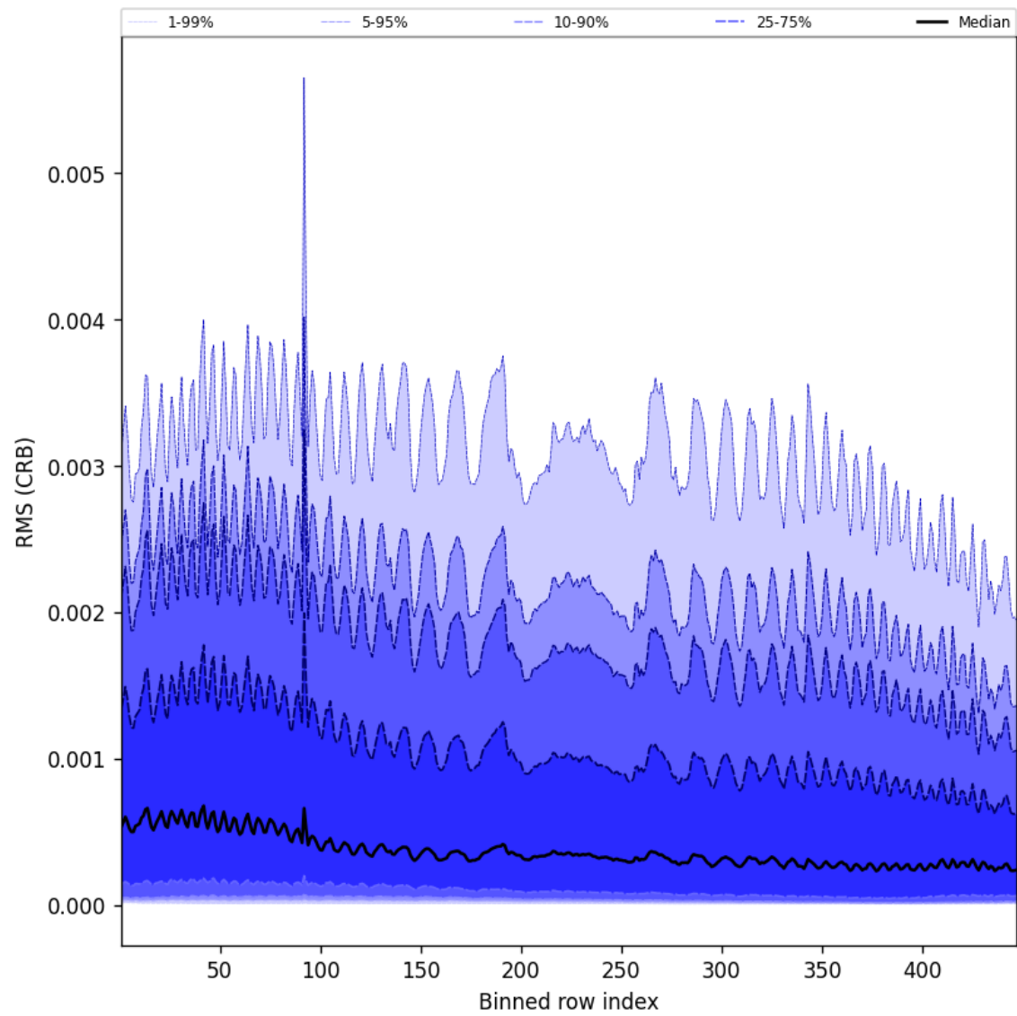
Figure 64: Along track statistics of “RMS (CRB)” for 2025-11-15 to 2025-11-17
