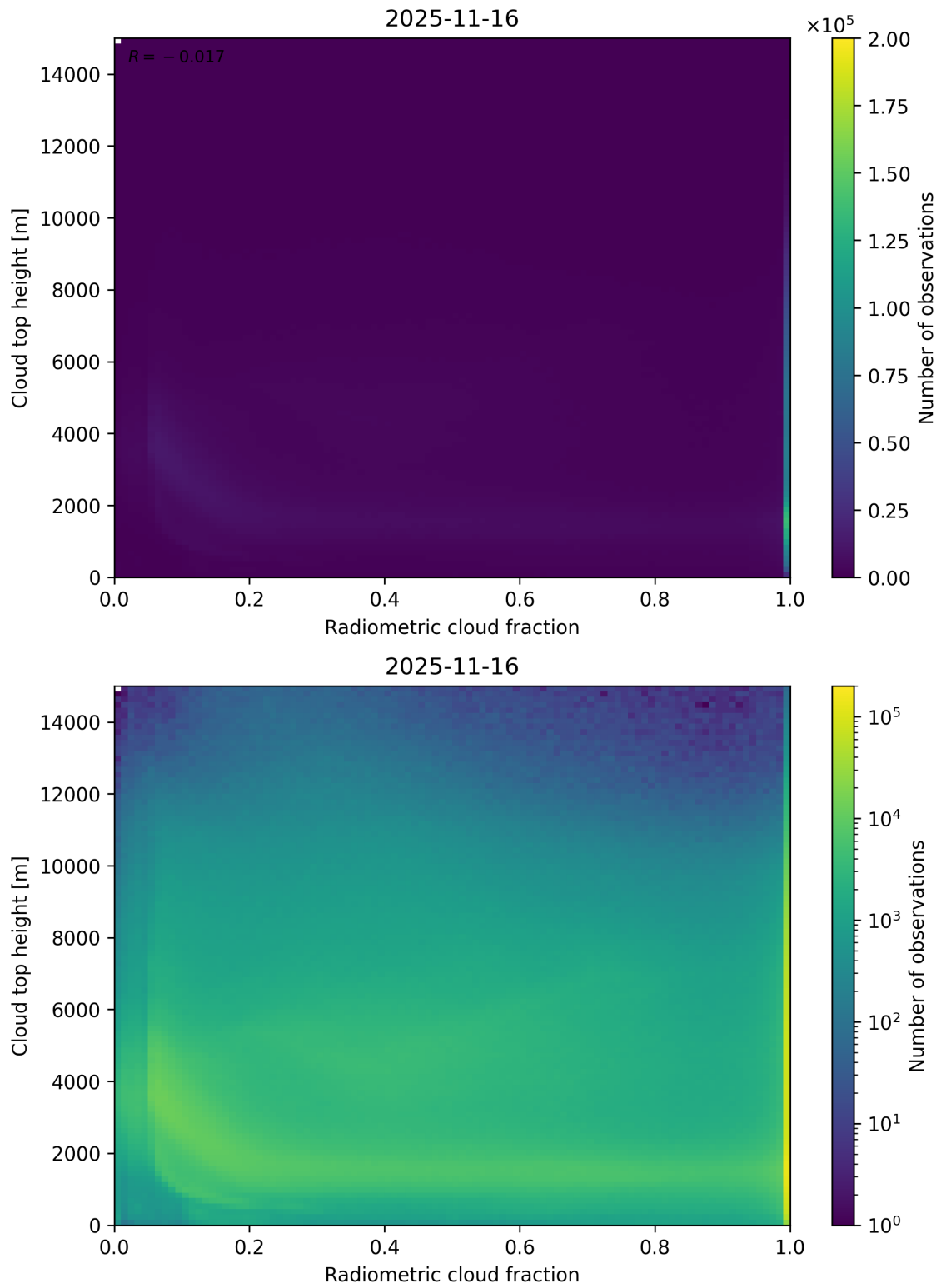
Figure 76: Scatter density plot of “Radiometric cloud fraction” against “Cloud top height” for 2025-11-15 to 2025-11-17.
