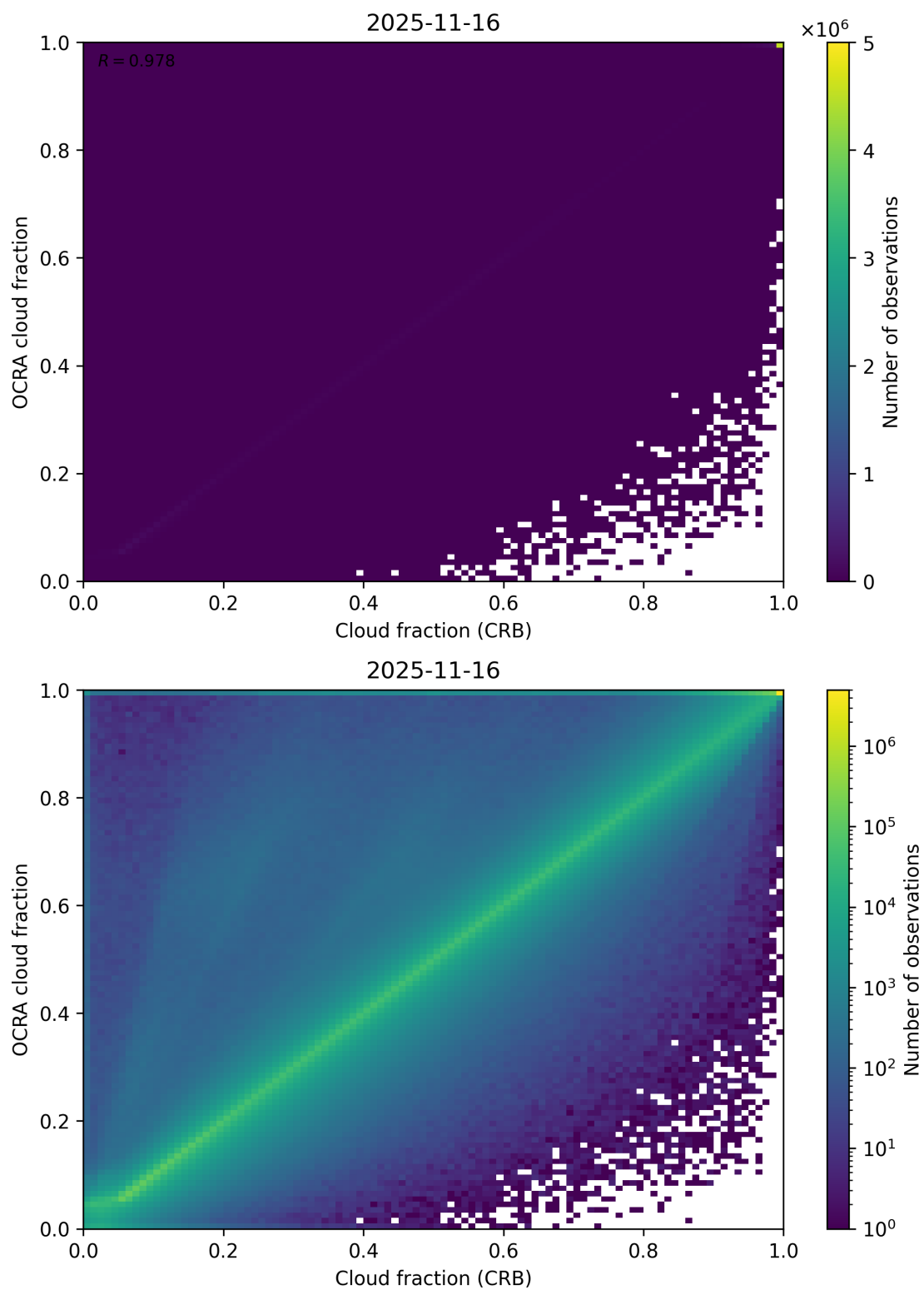
Figure 78: Scatter density plot of “Cloud fraction (CRB)” against “OCRA cloud fraction” for 2025-11-15 to 2025-11-17.
