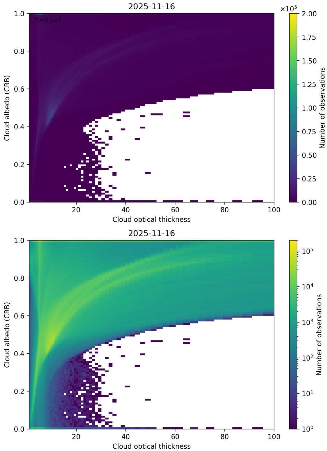
Figure 82: Scatter density plot of “Cloud optical thickness” against “Cloud albedo (CRB)” for 2025-11-15 to 2025-11-17.
