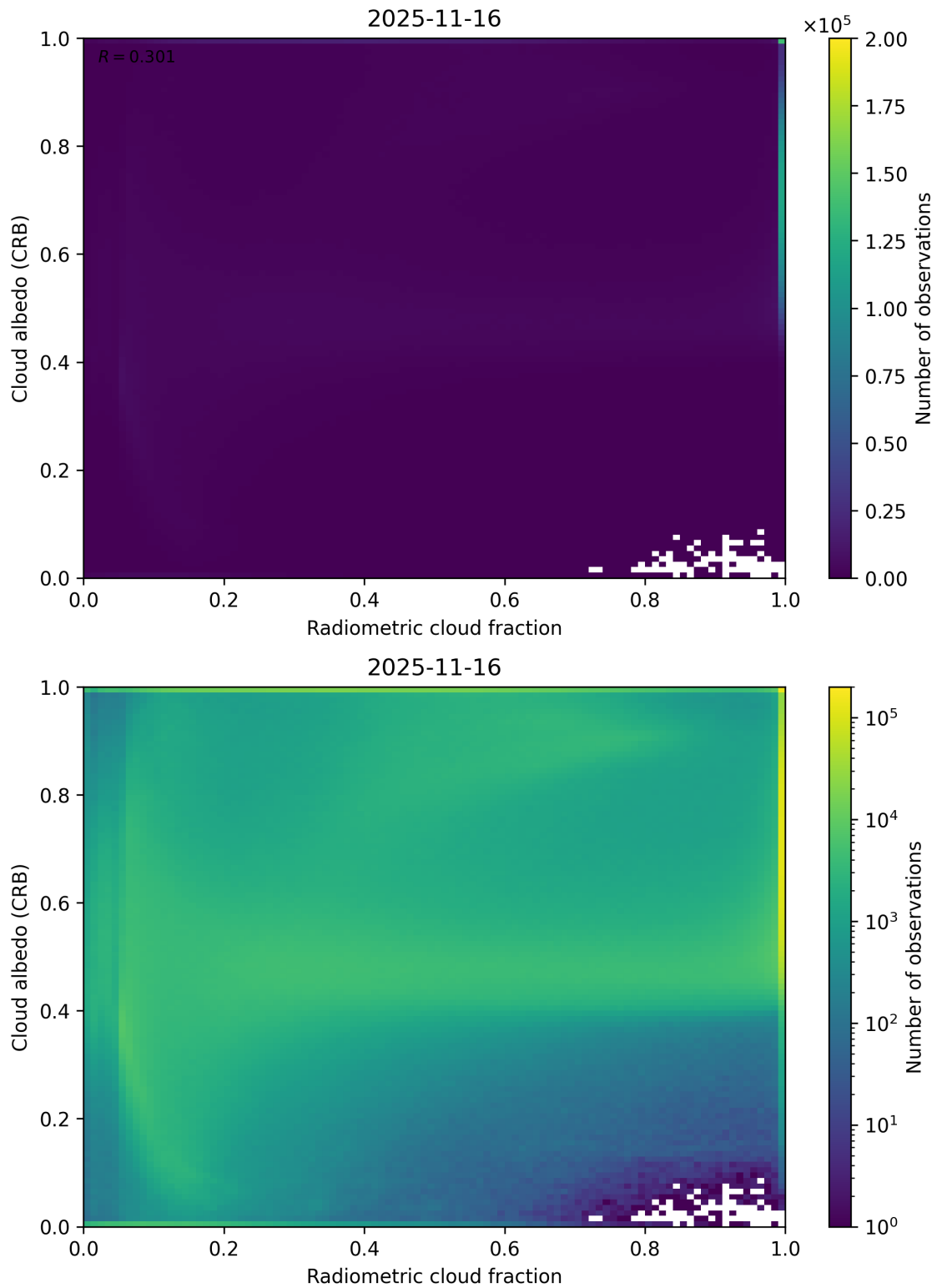
Figure 71: Scatter density plot of “Radiometric cloud fraction” against “Cloud albedo (CRB)” for 2025-11-15 to 2025-11-17.
