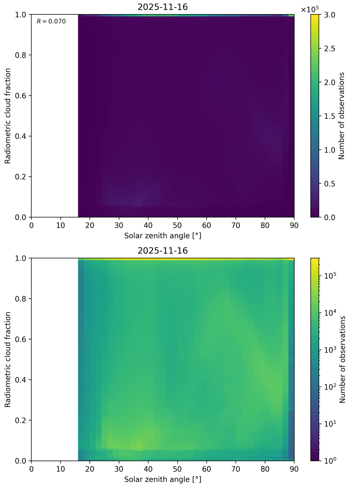
Figure 99: Scatter density plot of “Solar zenith angle” against “Radiometric cloud fraction” for 2025-11-15 to 2025-11-17.
