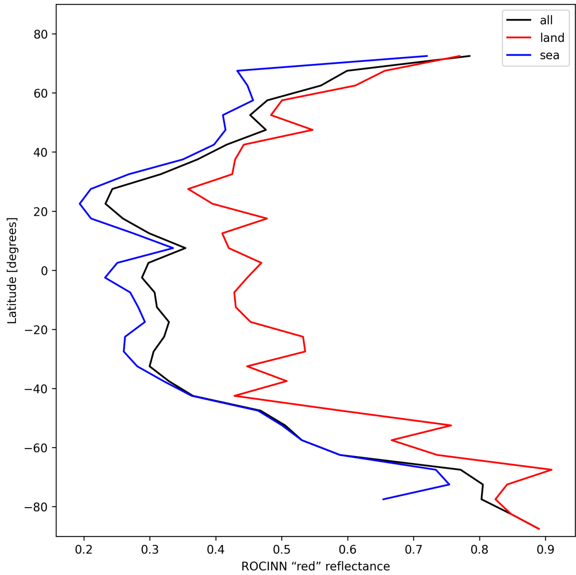
Figure 37: Zonal average of "ROCINN "red" reflectance" for 2025-11-15 to 2025-11-17.
