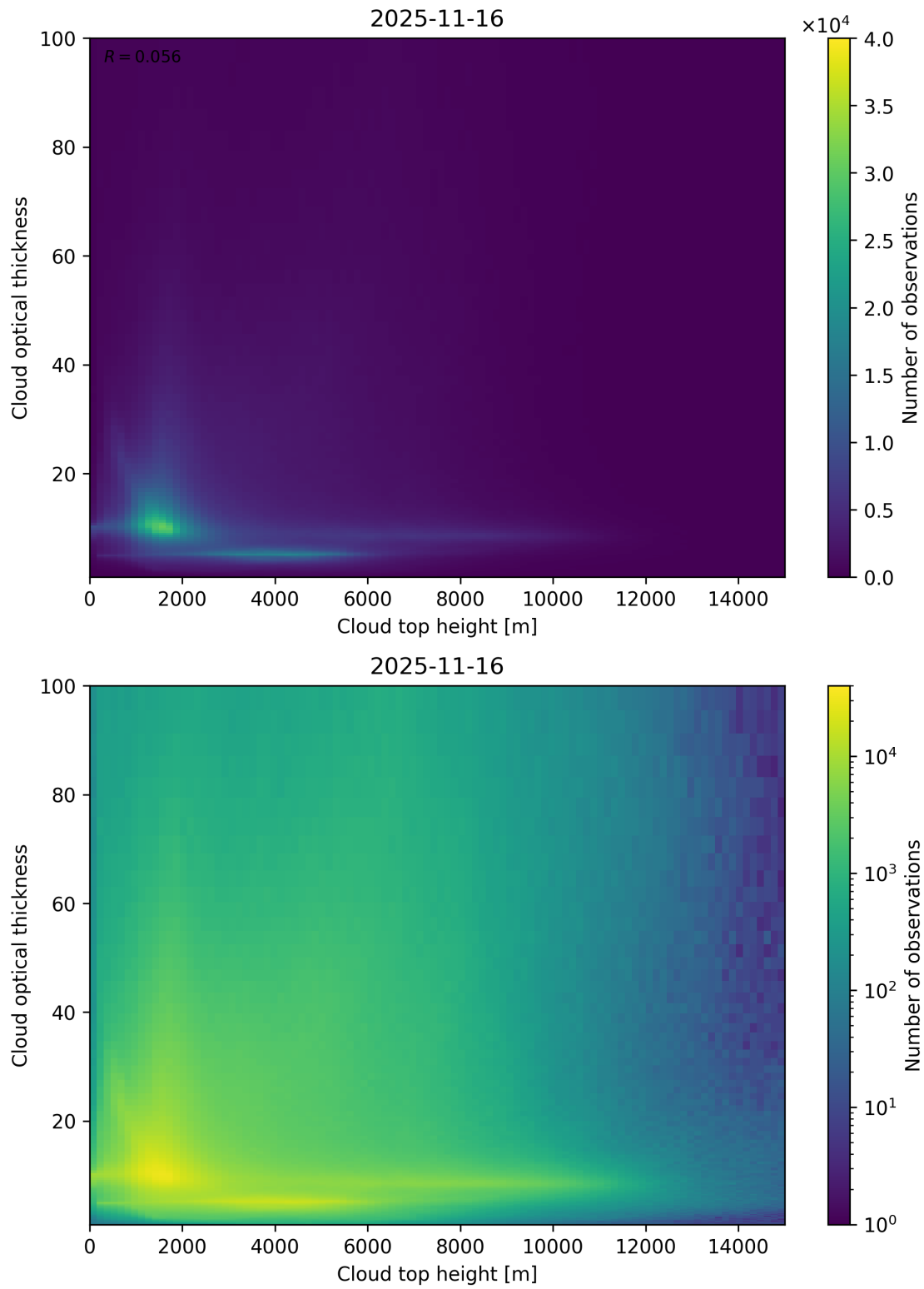
Figure 90: Scatter density plot of “Cloud top height” against “Cloud optical thickness” for 2025-11-15 to 2025-11-17.
