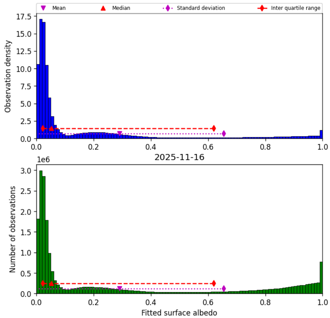
Figure 45: Histogram of “Fitted surface albedo” for 2025-11-15 to 2025-11-17
