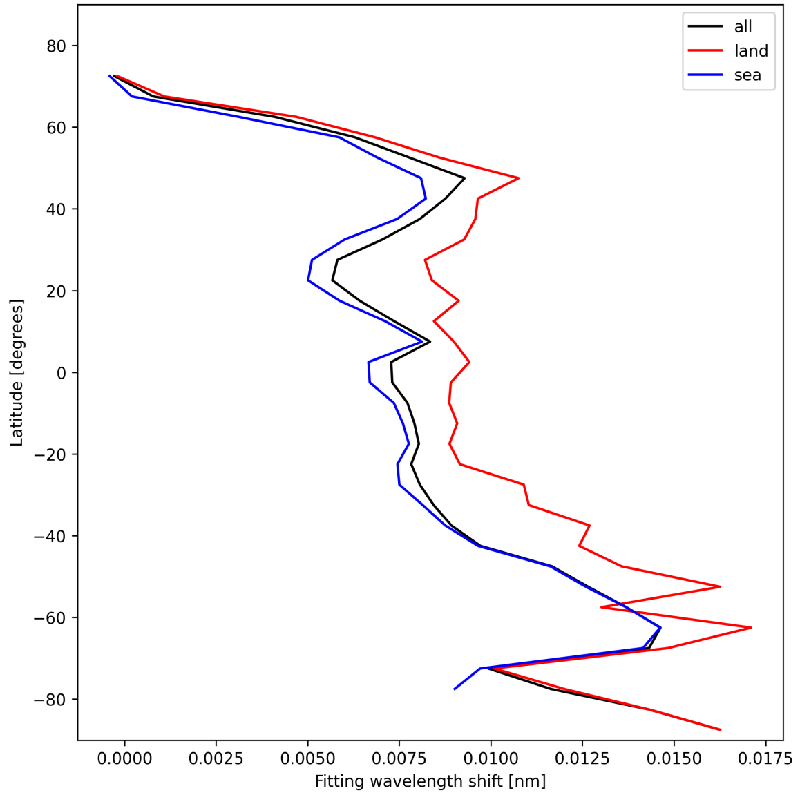
Figure 33: Zonal average of “Fitting wavelength shift” for 2025-11-15 to 2025-11-17.
