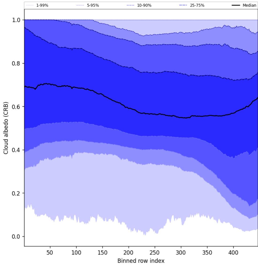
Figure 60: Along track statistics of “Cloud albedo (CRB)” for 2025-11-15 to 2025-11-17
