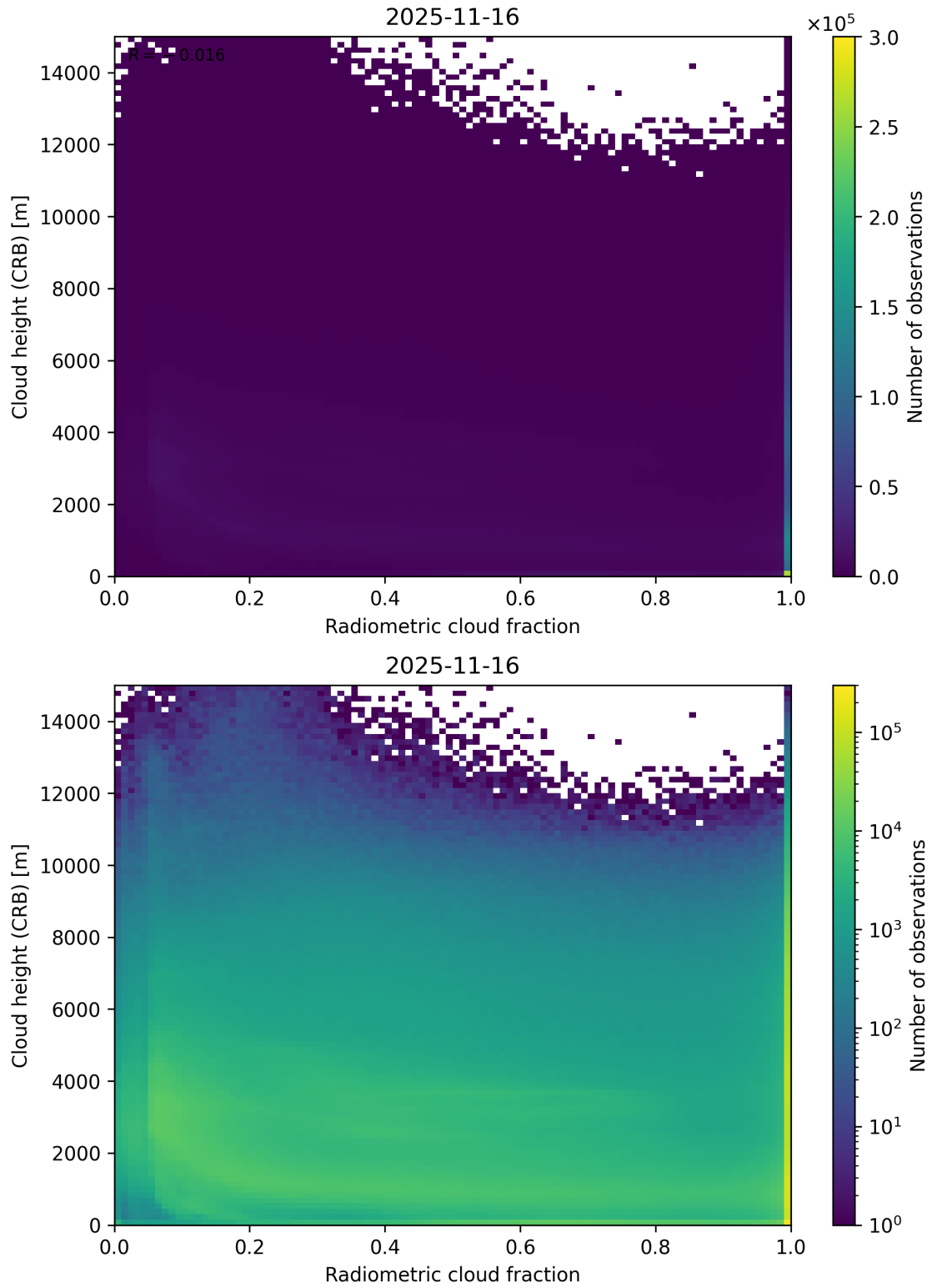
Figure 74: Scatter density plot of “Radiometric cloud fraction” against “Cloud height (CRB)” for 2025-11-15 to 2025-11-17.
