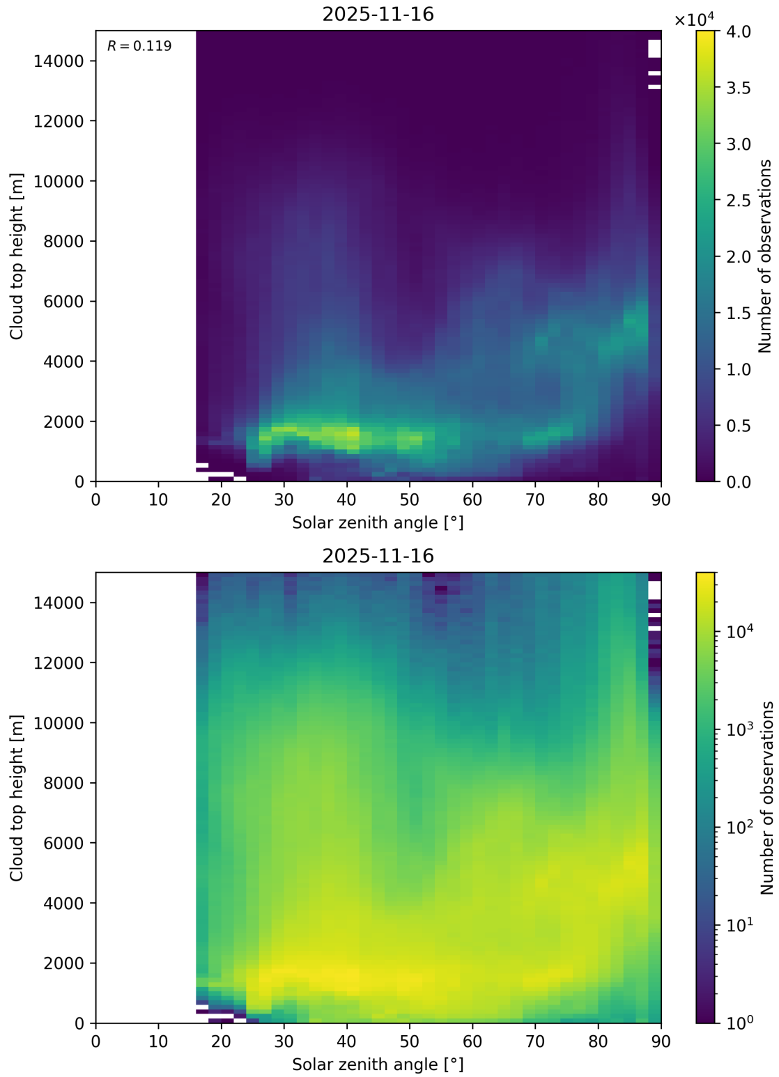
Figure 104: Scatter density plot of “Solar zenith angle” against “Cloud top height” for 2025-11-15 to 2025-11-17.
