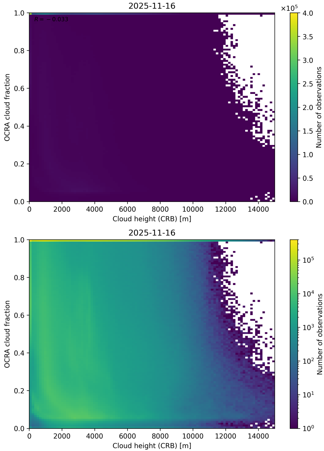
Figure 81: Scatter density plot of “Cloud height (CRB)” against “OCRA cloud fraction” for 2025-11-15 to 2025-11-17.
