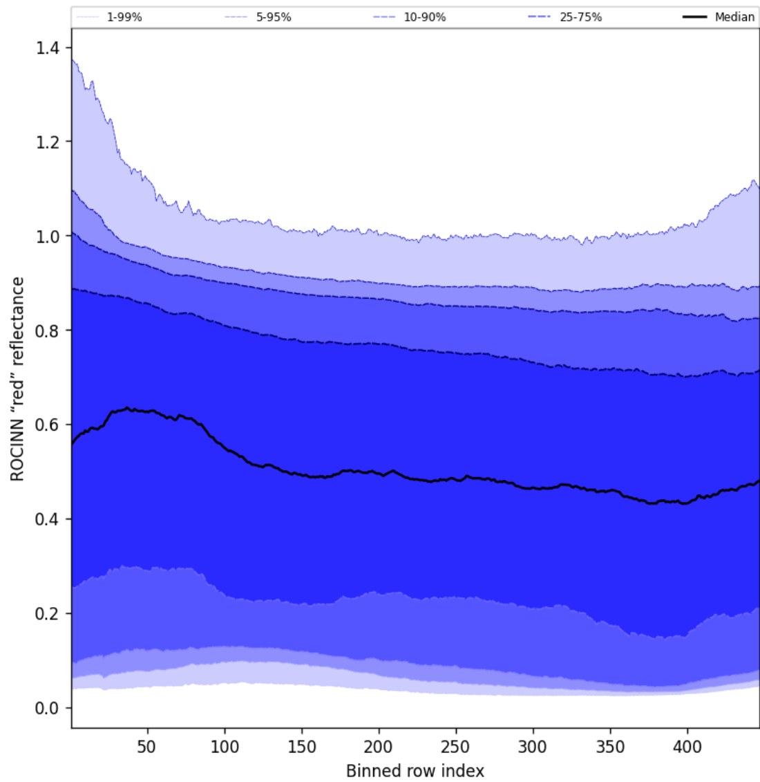
Figure 69: Along track statistics of “ROCINN “red” reflectance” for 2025-11-15 to 2025-11-17
