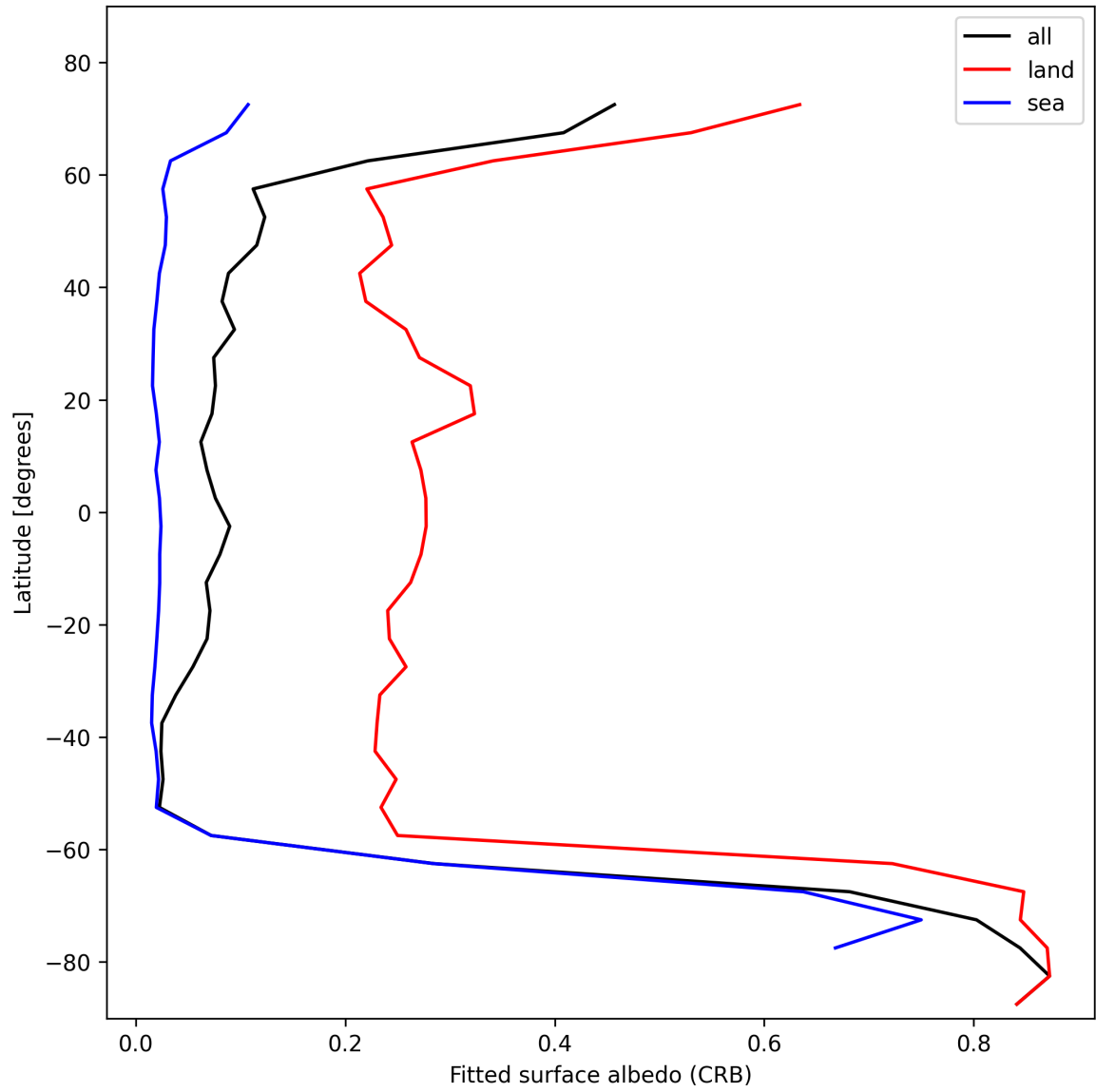
Figure 30: Zonal average of “Fitted surface albedo (CRB)” for 2025-11-15 to 2025-11-17.
