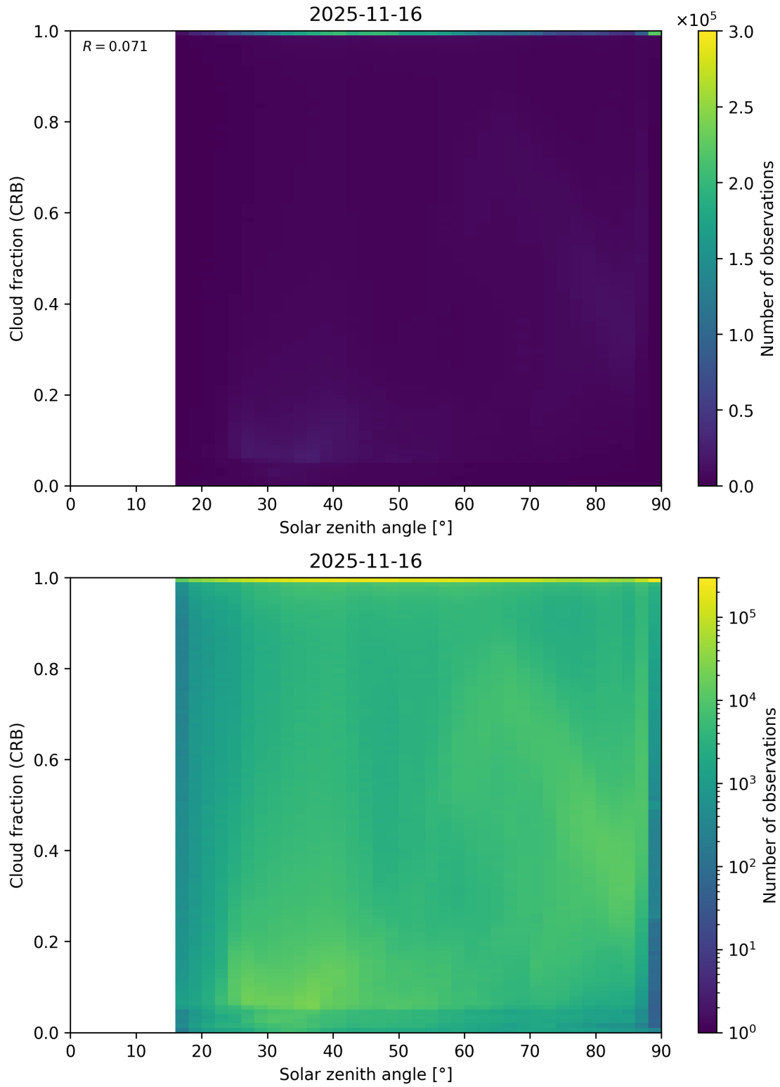
Figure 101: Scatter density plot of “Solar zenith angle” against “Cloud fraction (CRB)” for 2025-11-15 to 2025-11-17.
