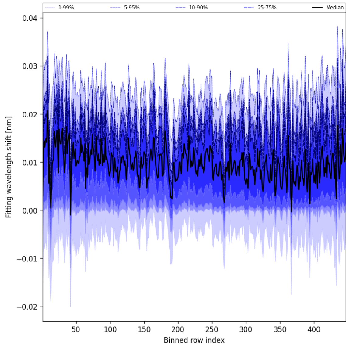
Figure 65: Along track statistics of “Fitting wavelength shift” for 2025-11-15 to 2025-11-17
