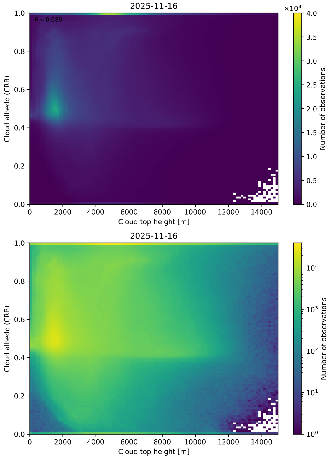
Figure 86: Scatter density plot of “Cloud top height” against “Cloud albedo (CRB)” for 2025-11-15 to 2025-11-17.
