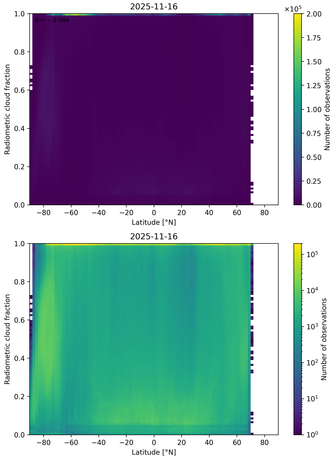
Figure 92: Scatter density plot of “Latitude” against “Radiometric cloud fraction” for 2025-11-15 to 2025-11-17.
