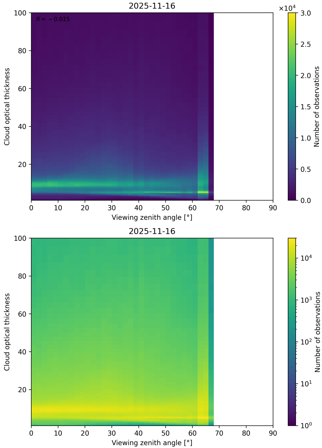
Figure 111: Scatter density plot of “Viewing zenith angle” against “Cloud optical thickness” for 2025-11-15 to 2025-11-17.
