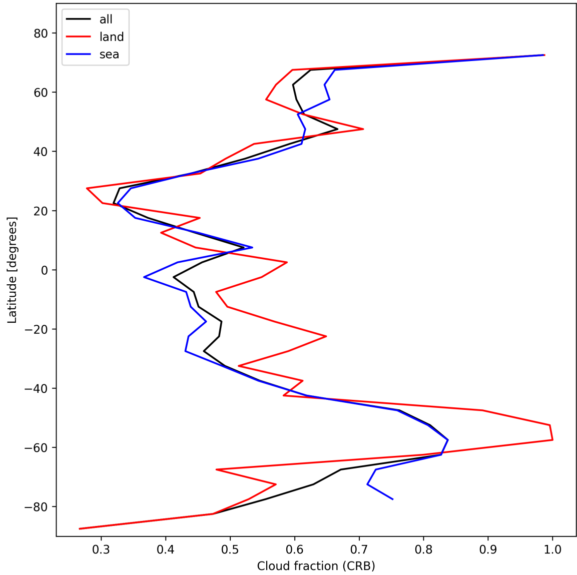
Figure 26: Zonal average of “Cloud fraction (CRB)” for 2025-11-15 to 2025-11-17.
