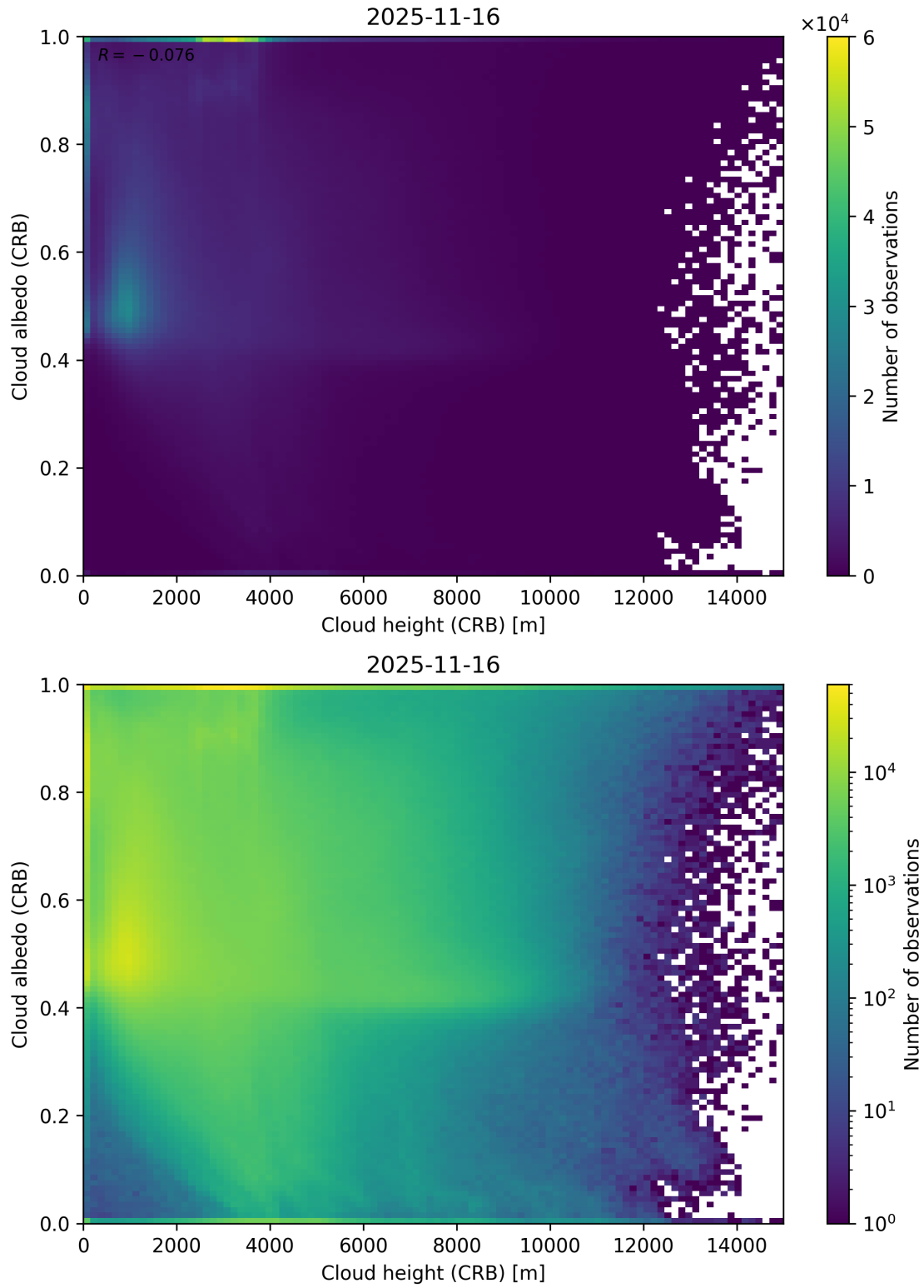
Figure 80: Scatter density plot of “Cloud height (CRB)” against “Cloud albedo (CRB)” for 2025-11-15 to 2025-11-17.
