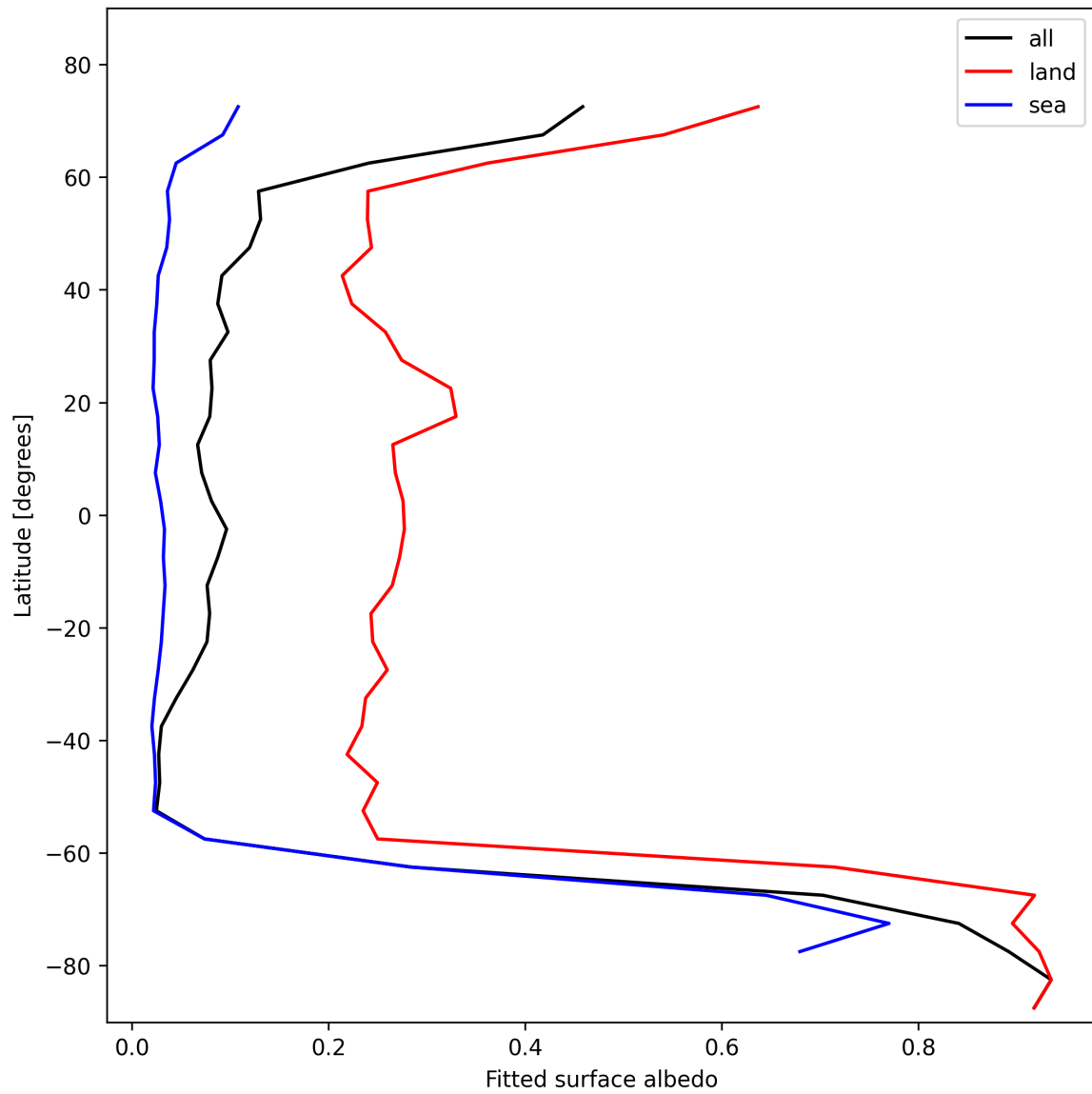
Figure 29: Zonal average of “Fitted surface albedo” for 2025-11-15 to 2025-11-17.
