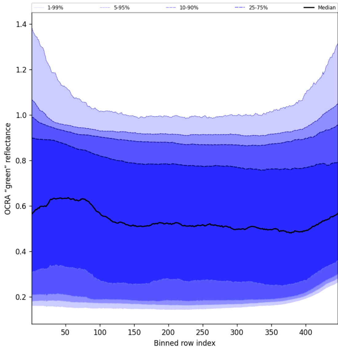
Figure 68: Along track statistics of "OCRA "green" reflectance" for 2025-11-15 to 2025-11-17
