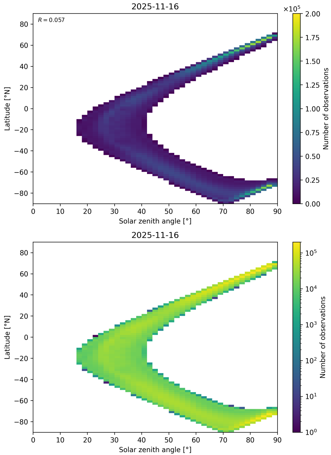
Figure 105: Scatter density plot of “Solar zenith angle” against “Latitude” for 2025-11-15 to 2025-11-17.
