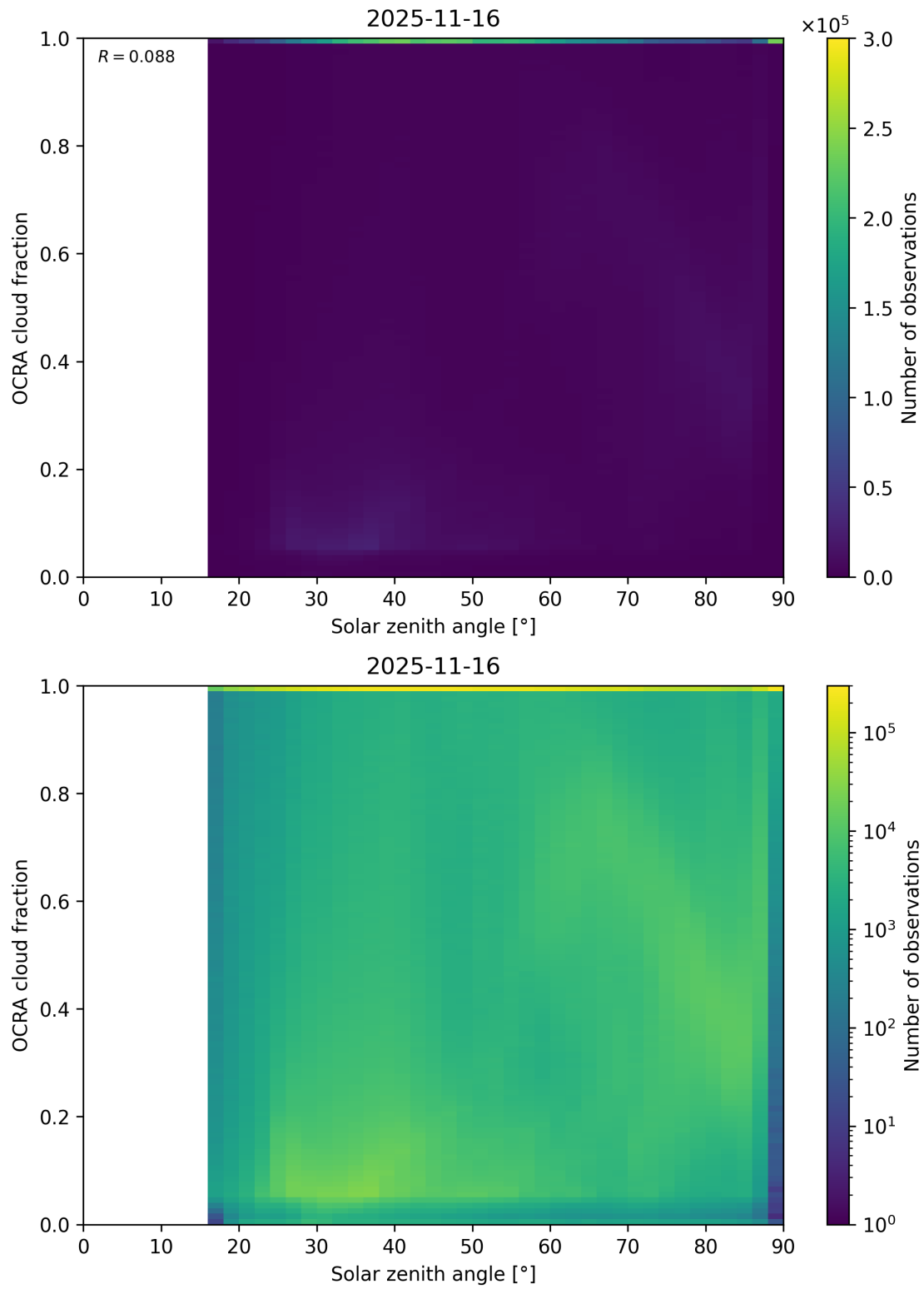
Figure 100: Scatter density plot of “Solar zenith angle” against “OCRA cloud fraction” for 2025-11-15 to 2025-11-17.
