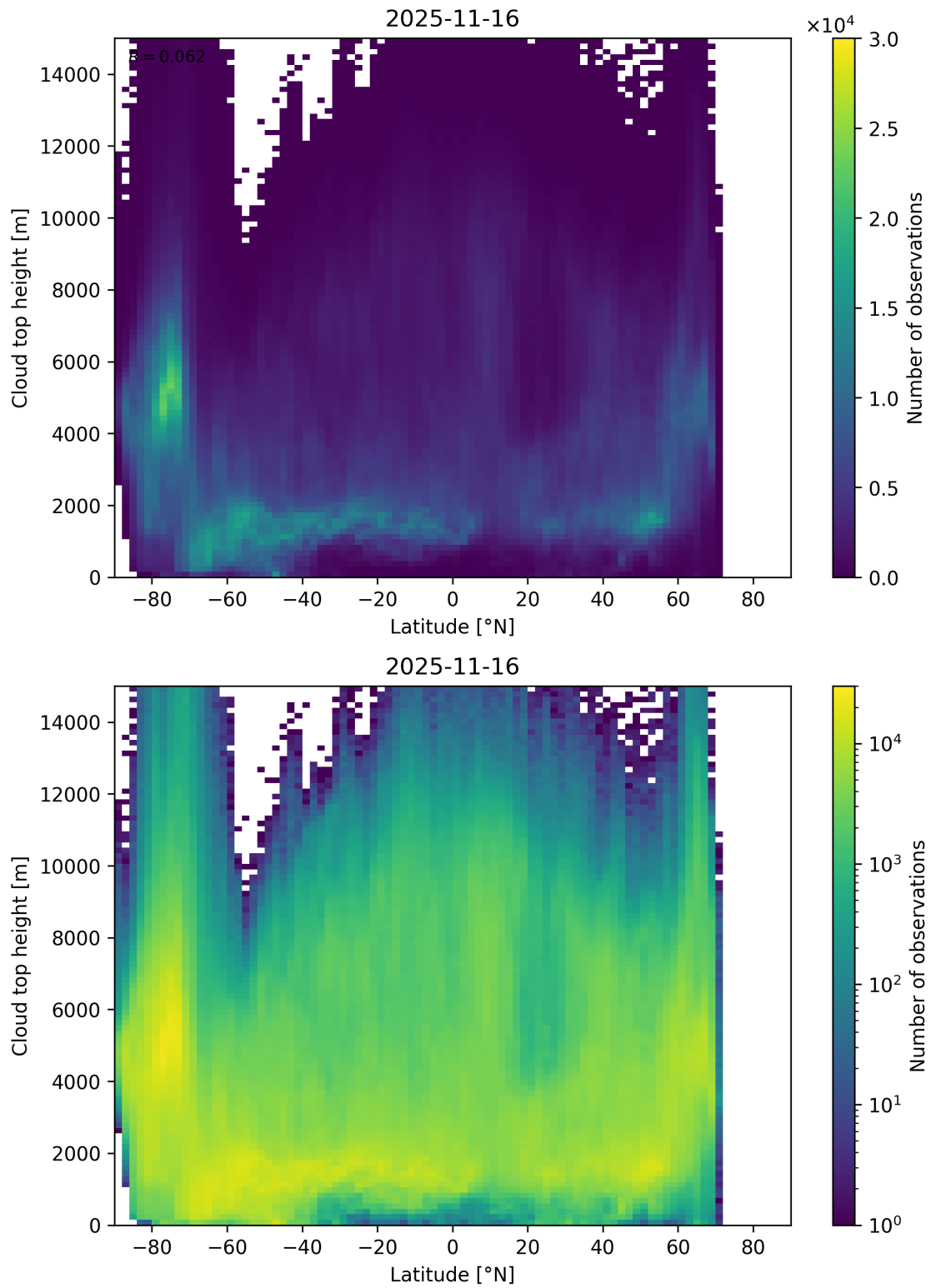
Figure 97: Scatter density plot of “Latitude” against “Cloud top height” for 2025-11-15 to 2025-11-17.
