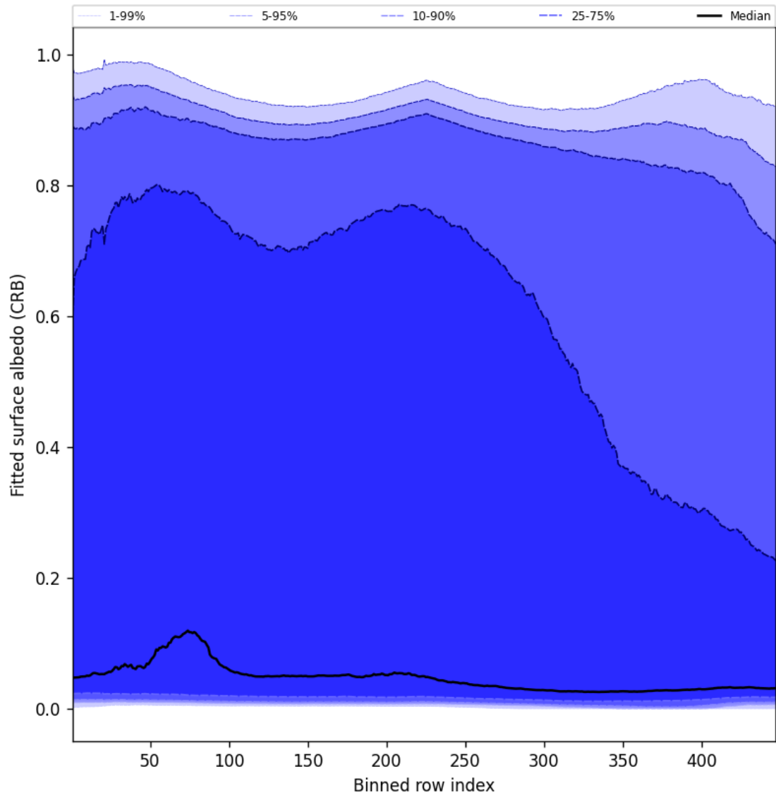
Figure 62: Along track statistics of “Fitted surface albedo (CRB)” for 2025-11-15 to 2025-11-17
