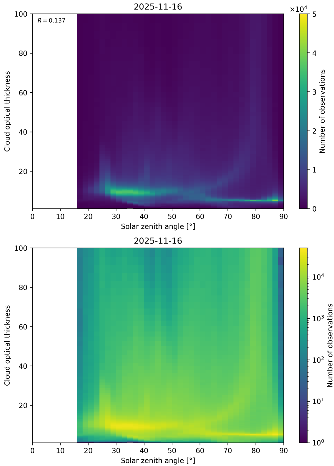
Figure 103: Scatter density plot of “Solar zenith angle” against “Cloud optical thickness” for 2025-11-15 to 2025-11-17.
