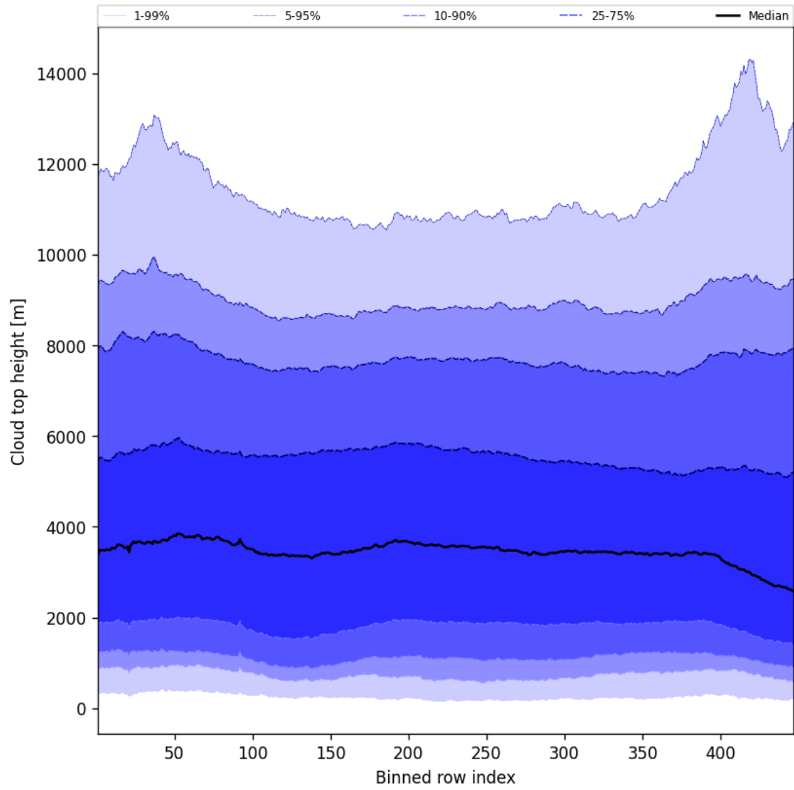
Figure 56: Along track statistics of “Cloud top height” for 2025-11-15 to 2025-11-17
