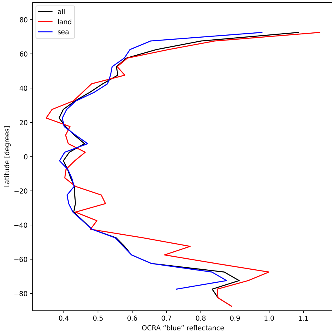
Figure 35: Zonal average of “OCRA “blue” reflectance” for 2025-11-15 to 2025-11-17.
