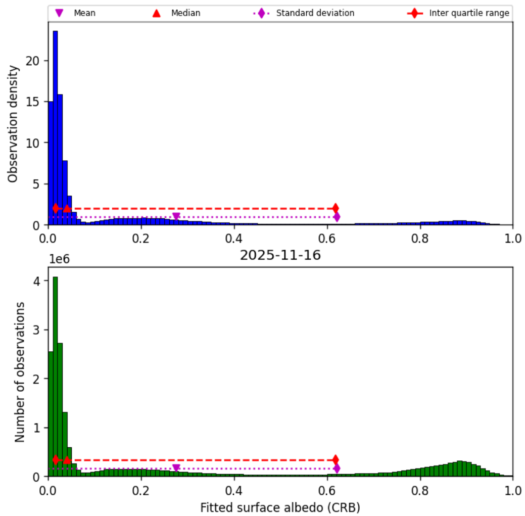
Figure 46: Histogram of “Fitted surface albedo (CRB)” for 2025-11-15 to 2025-11-17
