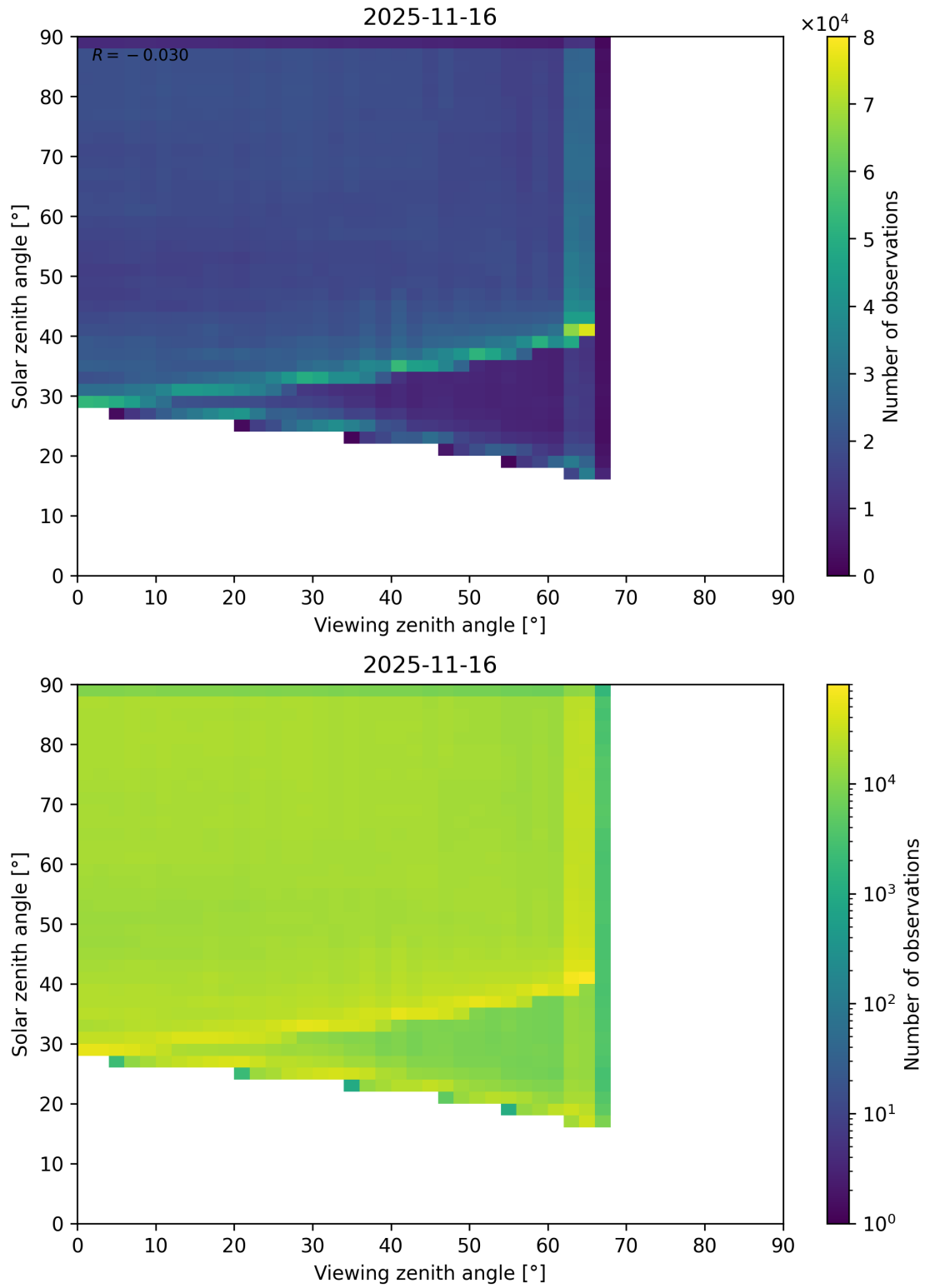
Figure 114: Scatter density plot of “Viewing zenith angle” against “Solar zenith angle” for 2025-11-15 to 2025-11-17.
