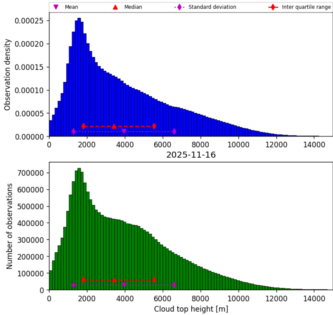
Figure 40: Histogram of “Cloud top height” for 2025-11-15 to 2025-11-17
