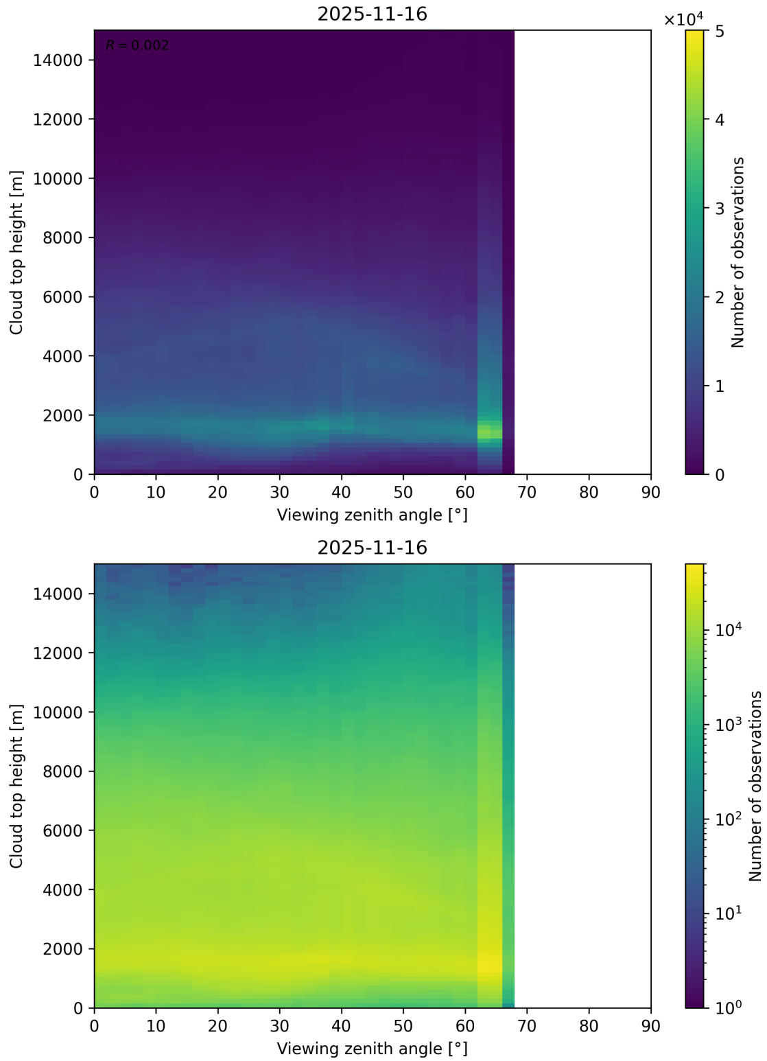
Figure 112: Scatter density plot of “Viewing zenith angle” against “Cloud top height” for 2025-11-15 to 2025-11-17.
