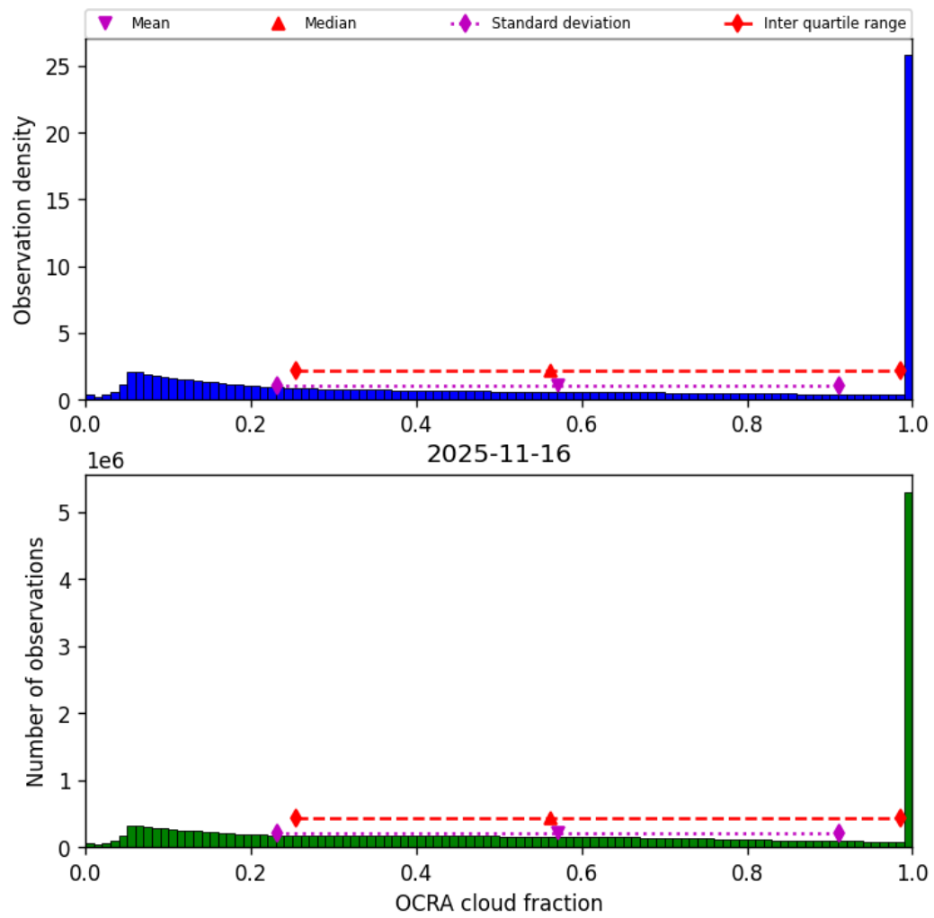
Figure 50: Histogram of “OCRA cloud fraction” for 2025-11-15 to 2025-11-17
