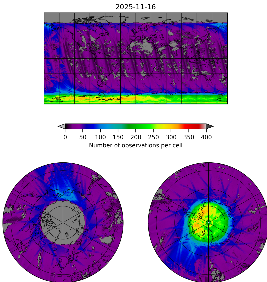
Figure 21: Map of the number of observations for 2025-11-15 to 2025-11-17
