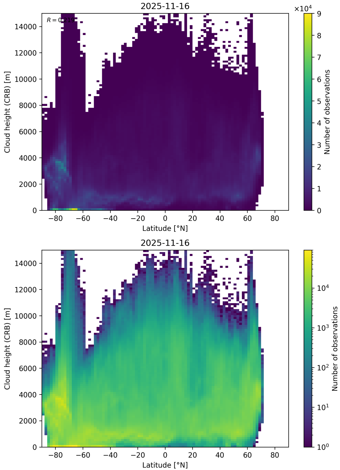
Figure 95: Scatter density plot of “Latitude” against “Cloud height (CRB)” for 2025-11-15 to 2025-11-17.
