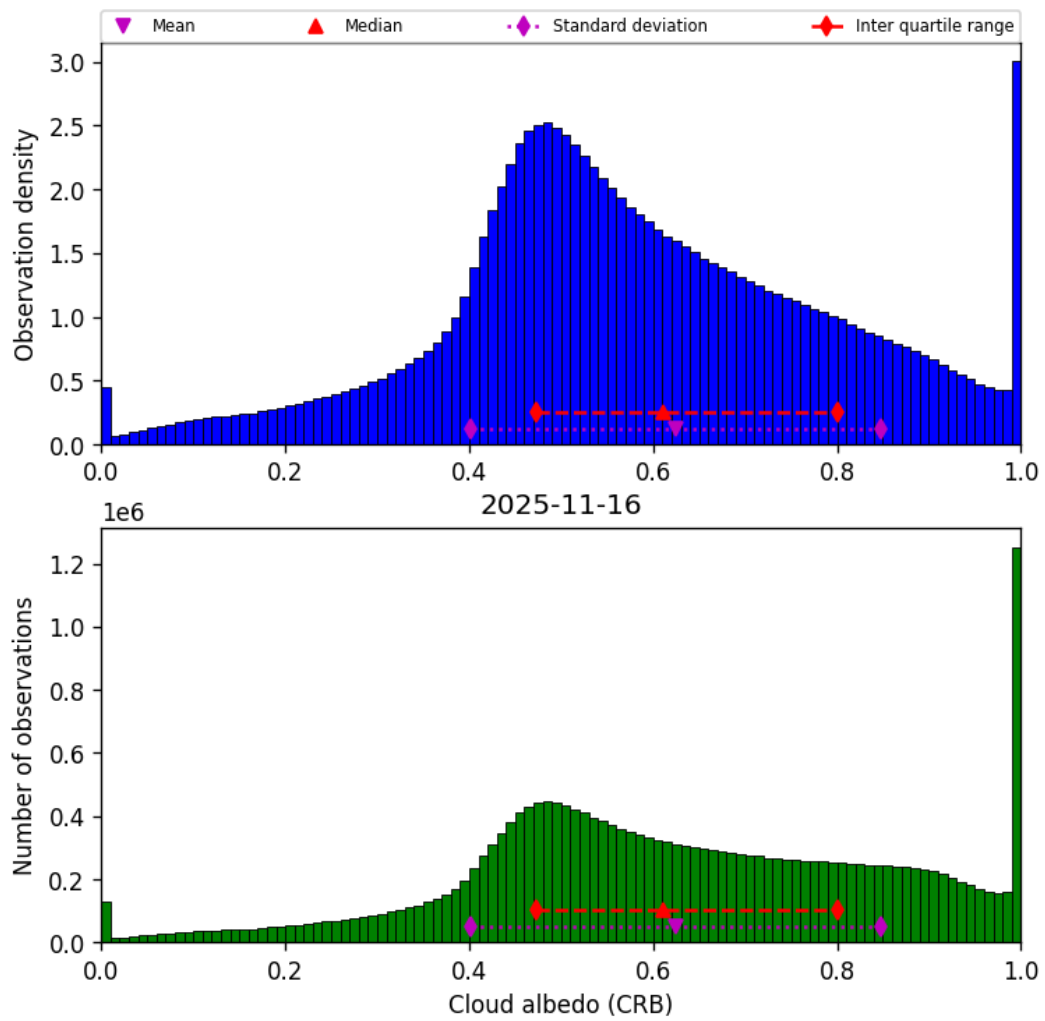
Figure 44: Histogram of “Cloud albedo (CRB)” for 2025-11-15 to 2025-11-17
