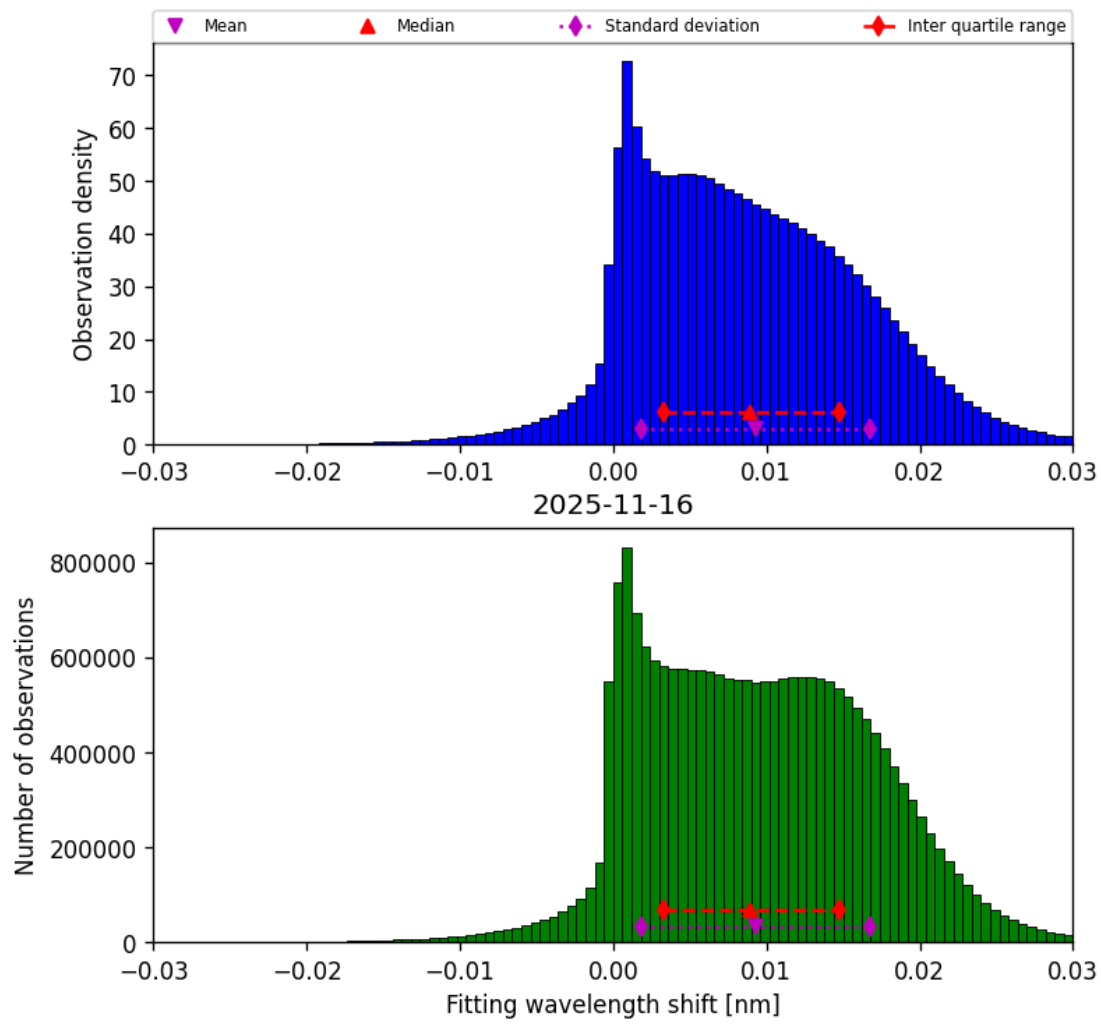
Figure 49: Histogram of “Fitting wavelength shift” for 2025-11-15 to 2025-11-17
