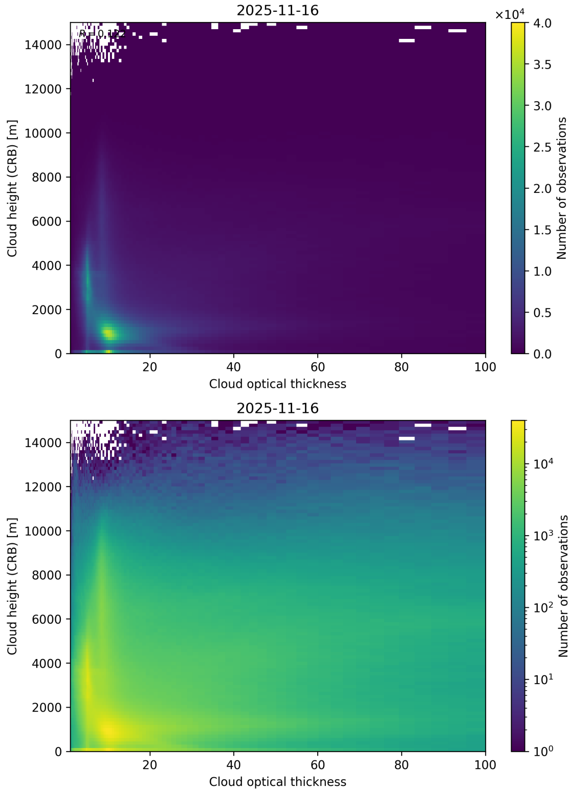
Figure 85: Scatter density plot of “Cloud optical thickness” against “Cloud height (CRB)” for 2025-11-15 to 2025-11-17.
