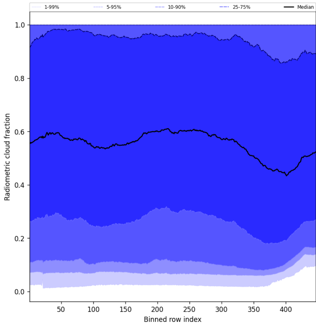
Figure 55: Along track statistics of “Radiometric cloud fraction” for 2025-11-15 to 2025-11-17
