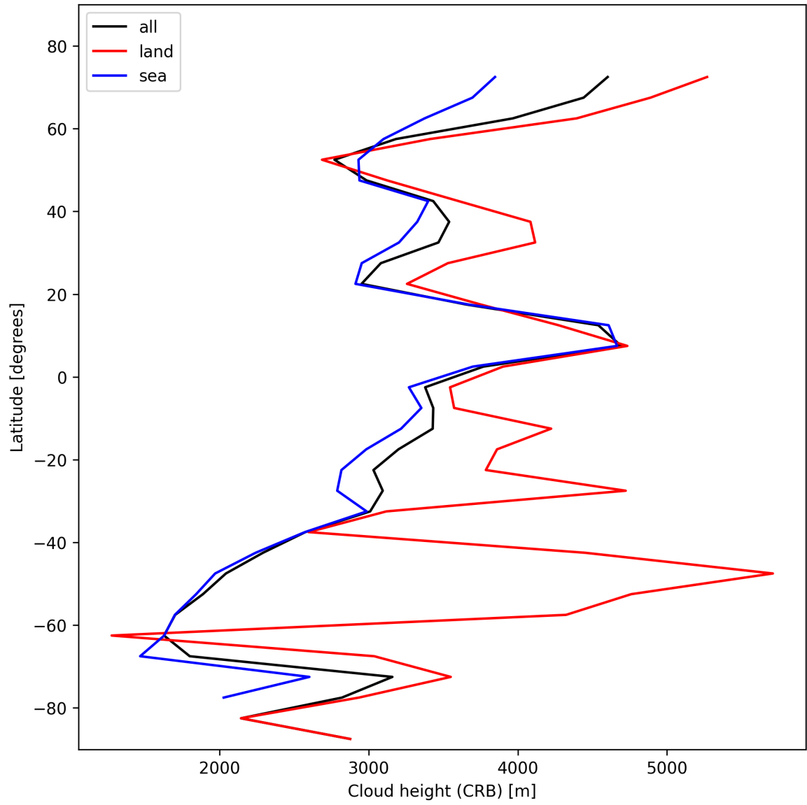
Figure 27: Zonal average of “Cloud height (CRB)” for 2025-11-15 to 2025-11-17.
