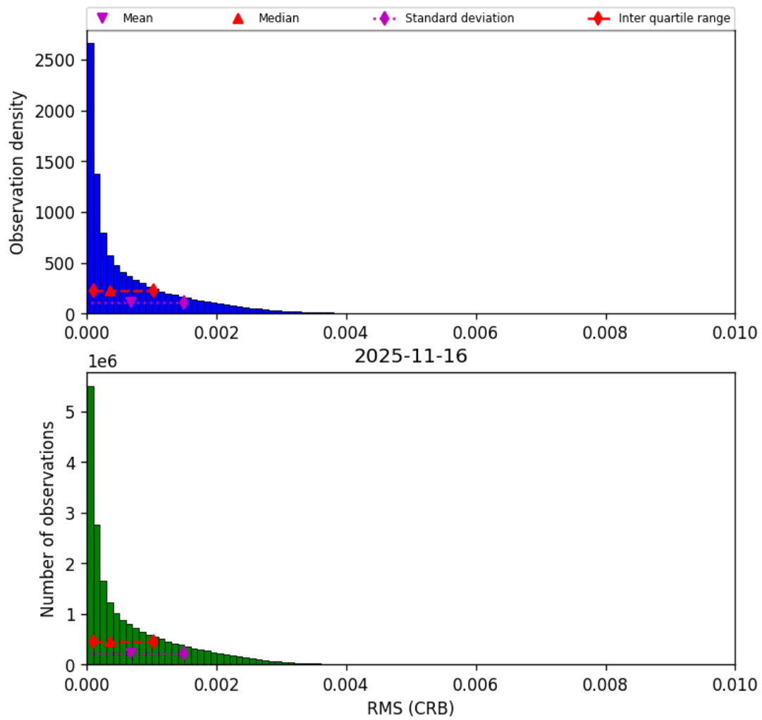
Figure 48: Histogram of “RMS (CRB)” for 2025-11-15 to 2025-11-17
