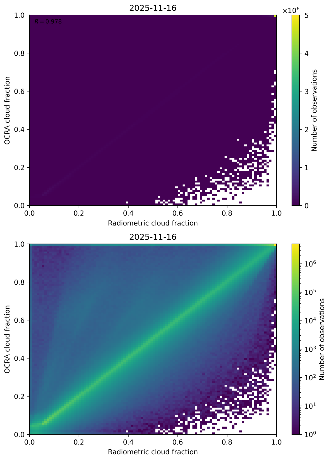
Figure 72: Scatter density plot of “Radiometric cloud fraction” against “OCRA cloud fraction” for 2025-11-15 to 2025-11-17.
