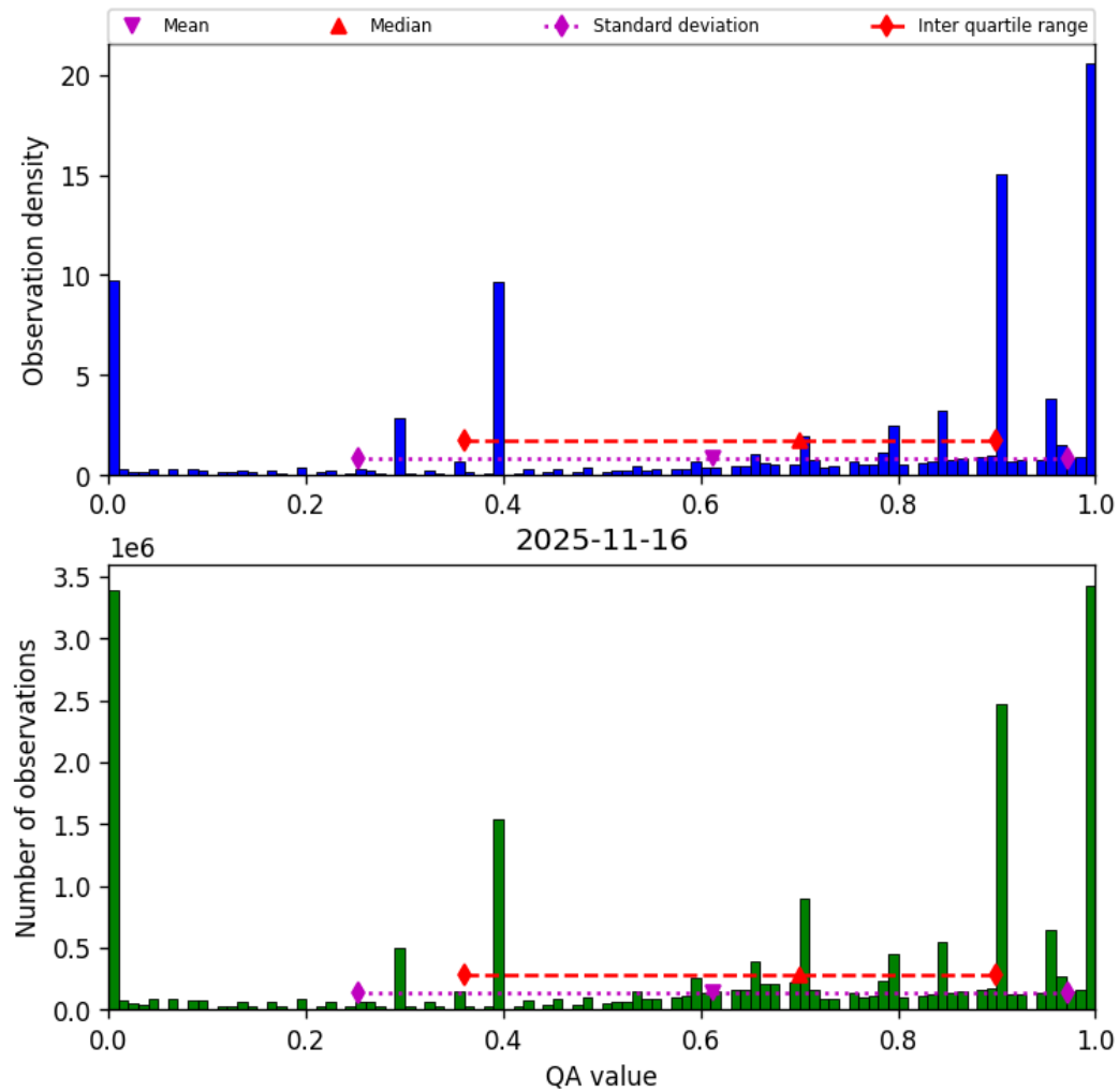
Figure 38: Histogram of “QA value” for 2025-11-15 to 2025-11-17
