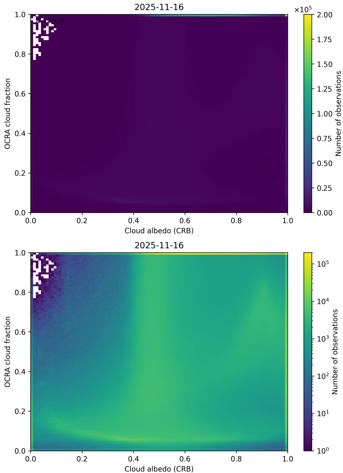
Figure 70: Scatter density plot of “Cloud albedo (CRB)” against “OCRA cloud fraction” for 2025-11-15 to 2025-11-17.
