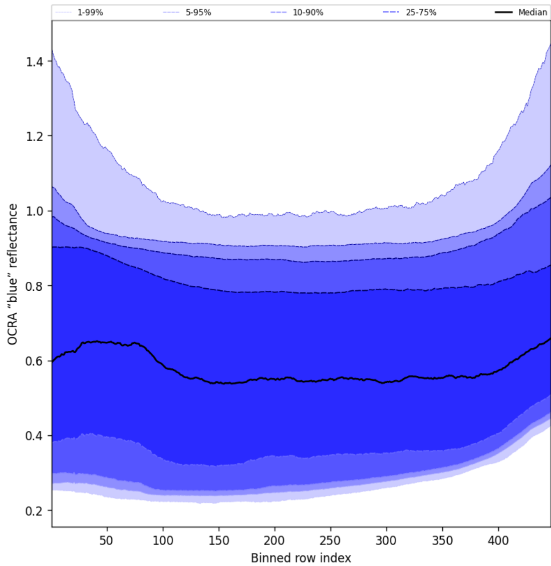
Figure 67: Along track statistics of “OCRA “blue” reflectance” for 2025-11-15 to 2025-11-17
