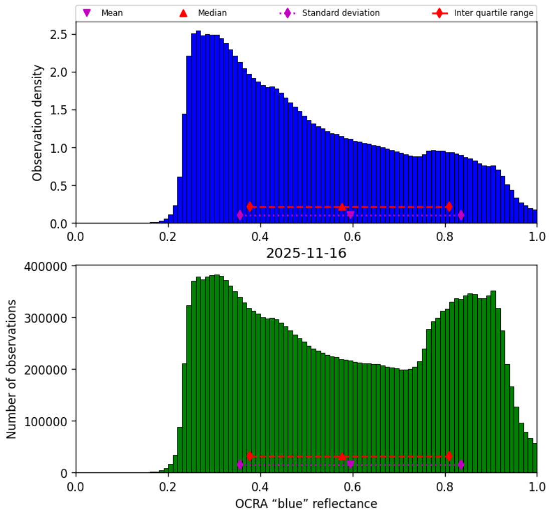
Figure 51: Histogram of “OCRA “blue” reflectance” for 2025-11-15 to 2025-11-17
