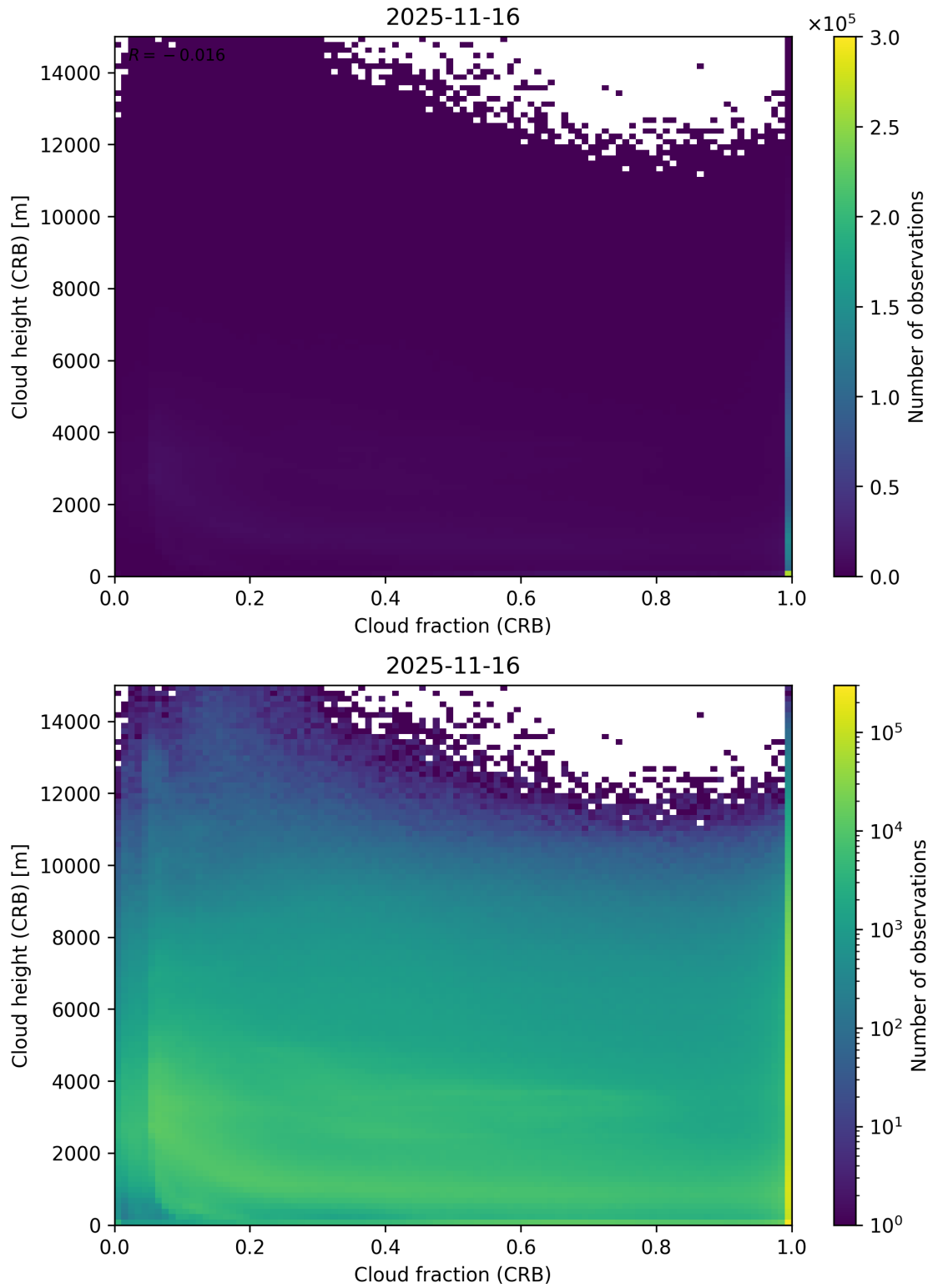
Figure 79: Scatter density plot of “Cloud fraction (CRB)” against “Cloud height (CRB)” for 2025-11-15 to 2025-11-17.
