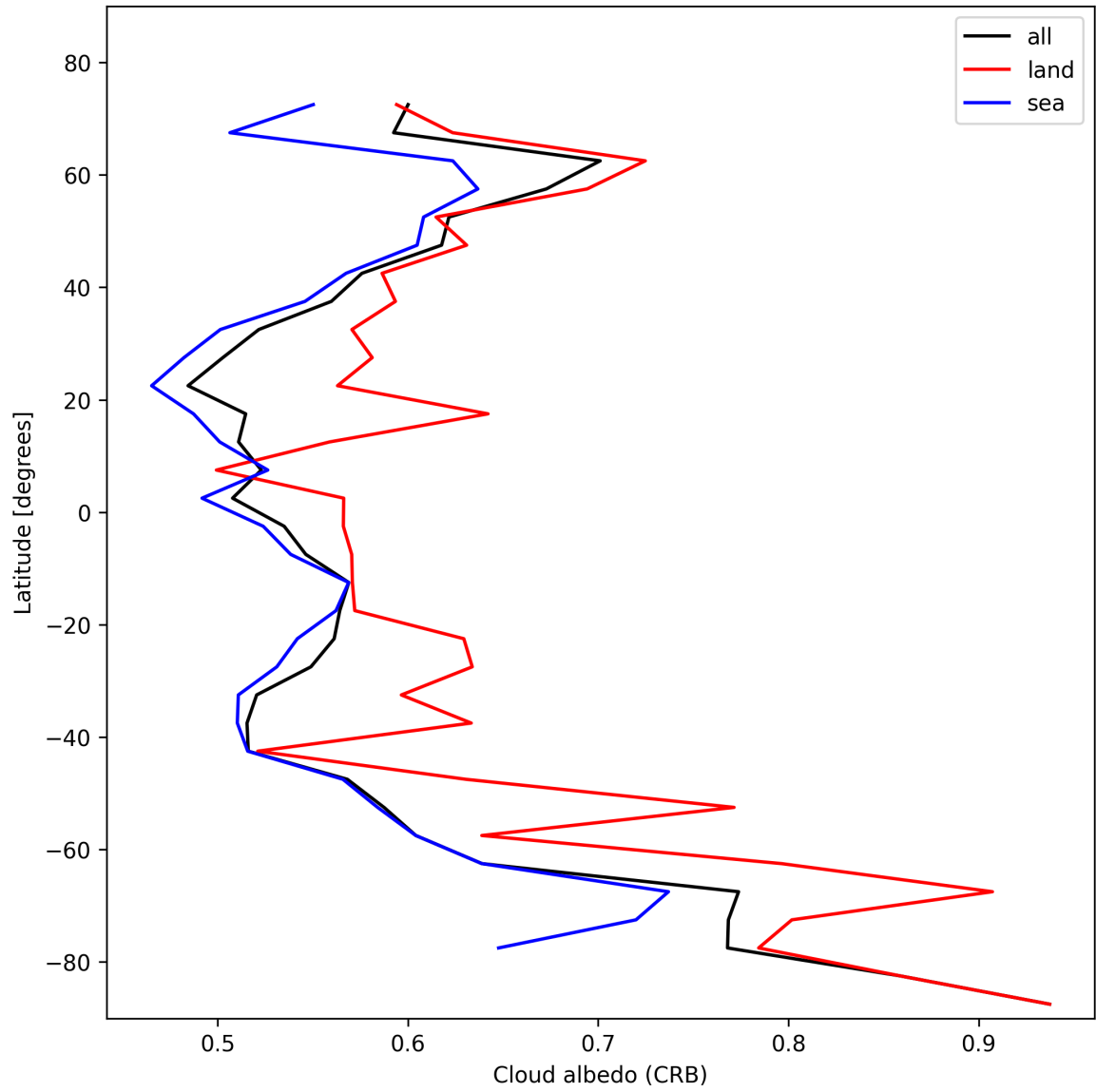
Figure 28: Zonal average of “Cloud albedo (CRB)” for 2025-11-15 to 2025-11-17.
