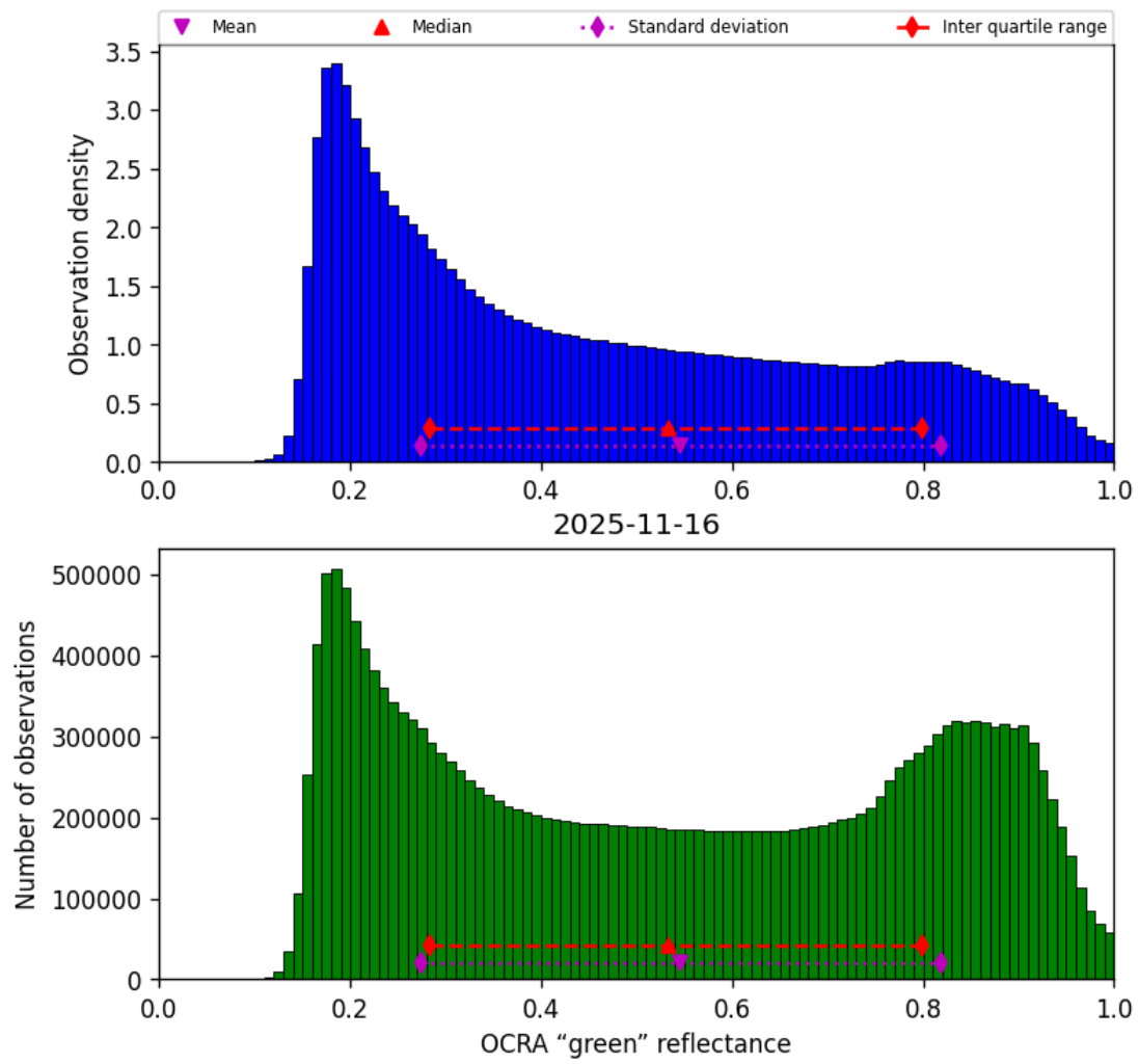
Figure 52: Histogram of “OCRA “green” reflectance” for 2025-11-15 to 2025-11-17
