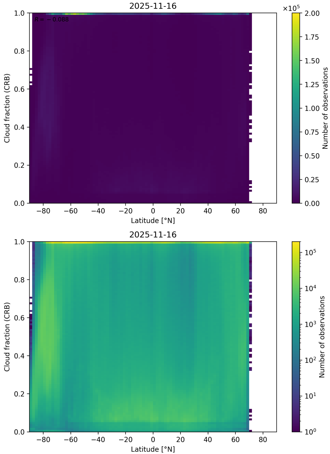
Figure 94: Scatter density plot of “Latitude” against “Cloud fraction (CRB)” for 2025-11-15 to 2025-11-17.
