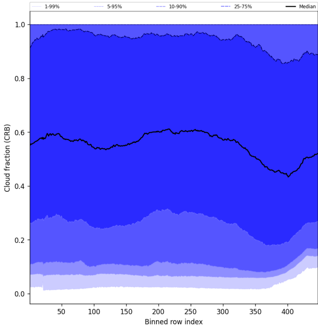
Figure 58: Along track statistics of “Cloud fraction (CRB)” for 2025-11-15 to 2025-11-17
