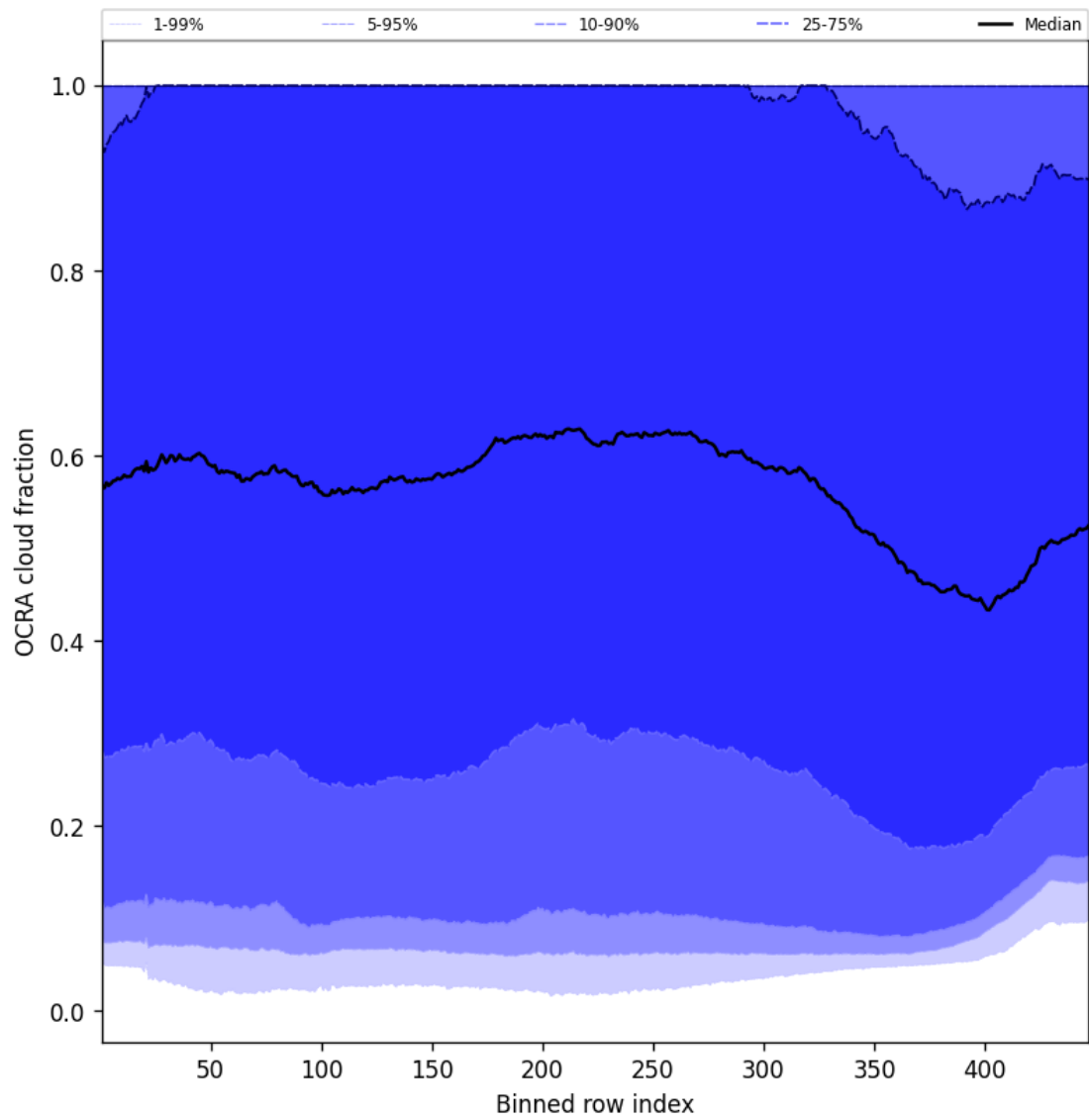
Figure 66: Along track statistics of “OCRA cloud fraction” for 2025-11-15 to 2025-11-17
