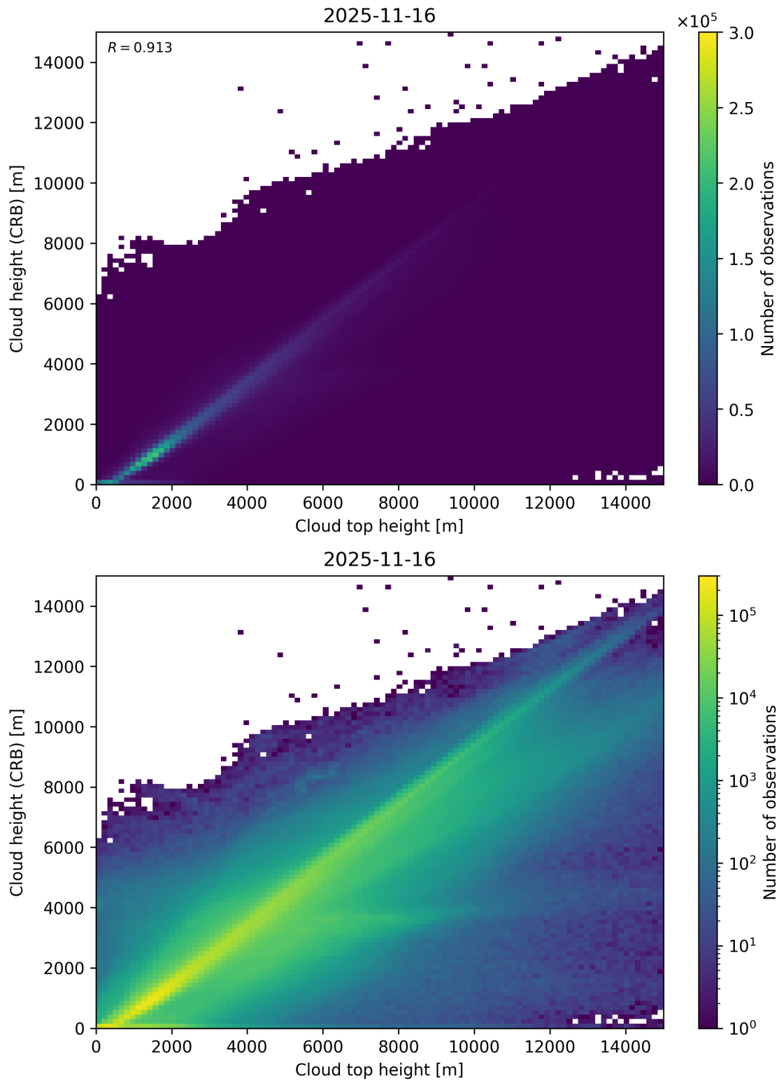
Figure 89: Scatter density plot of “Cloud top height” against “Cloud height (CRB)” for 2025-11-15 to 2025-11-17.
