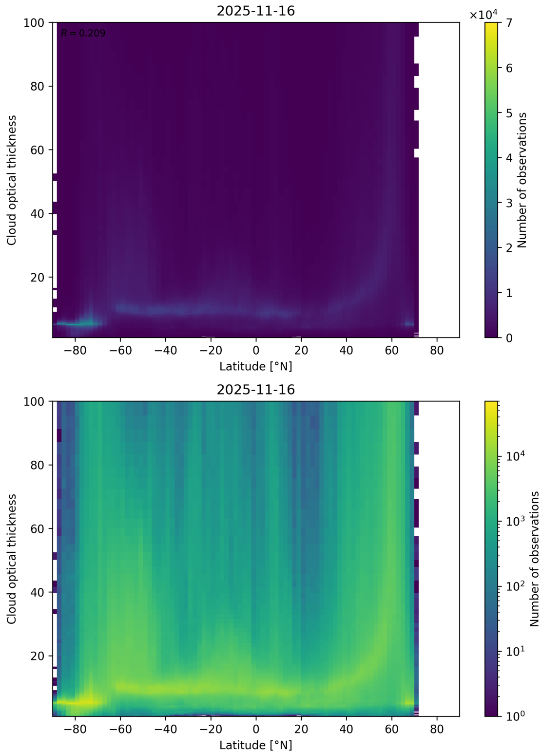
Figure 96: Scatter density plot of “Latitude” against “Cloud optical thickness” for 2025-11-15 to 2025-11-17.
