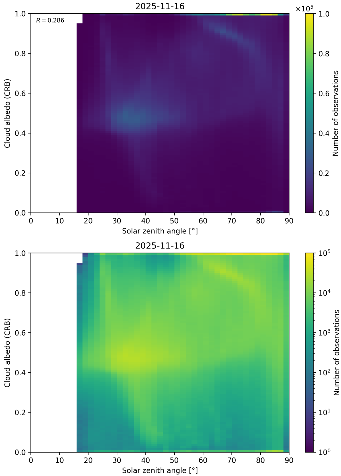
Figure 98: Scatter density plot of “Solar zenith angle” against “Cloud albedo (CRB)” for 2025-11-15 to 2025-11-17.
