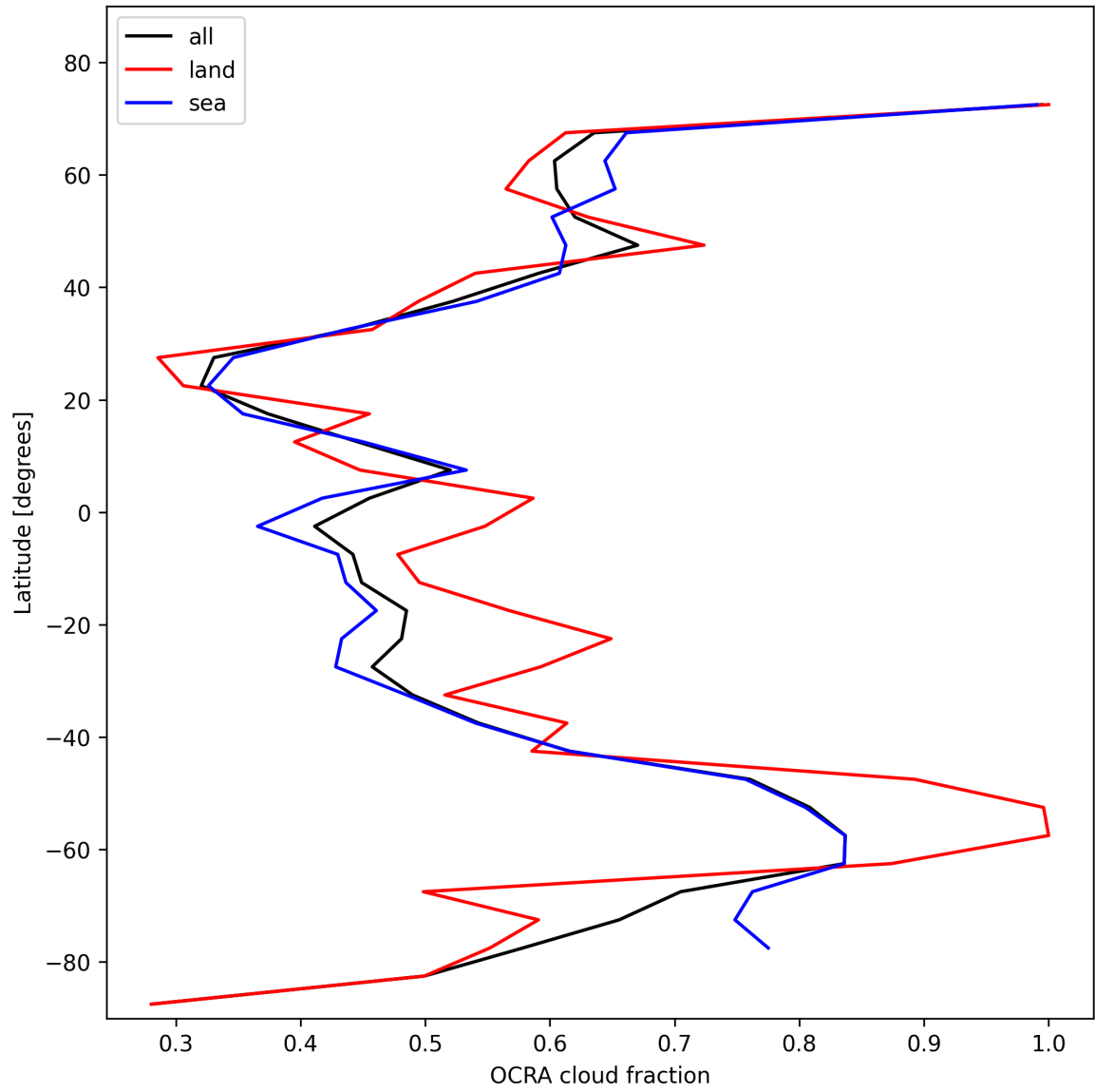
Figure 34: Zonal average of “OCRA cloud fraction” for 2025-11-15 to 2025-11-17.
