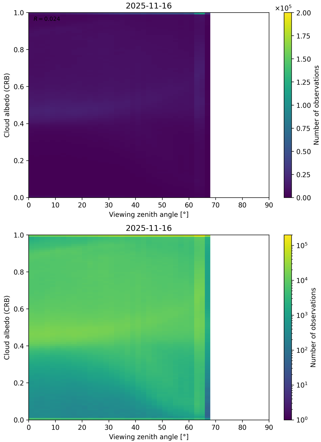
Figure 106: Scatter density plot of “Viewing zenith angle” against “Cloud albedo (CRB)” for 2025-11-15 to 2025-11-17.
