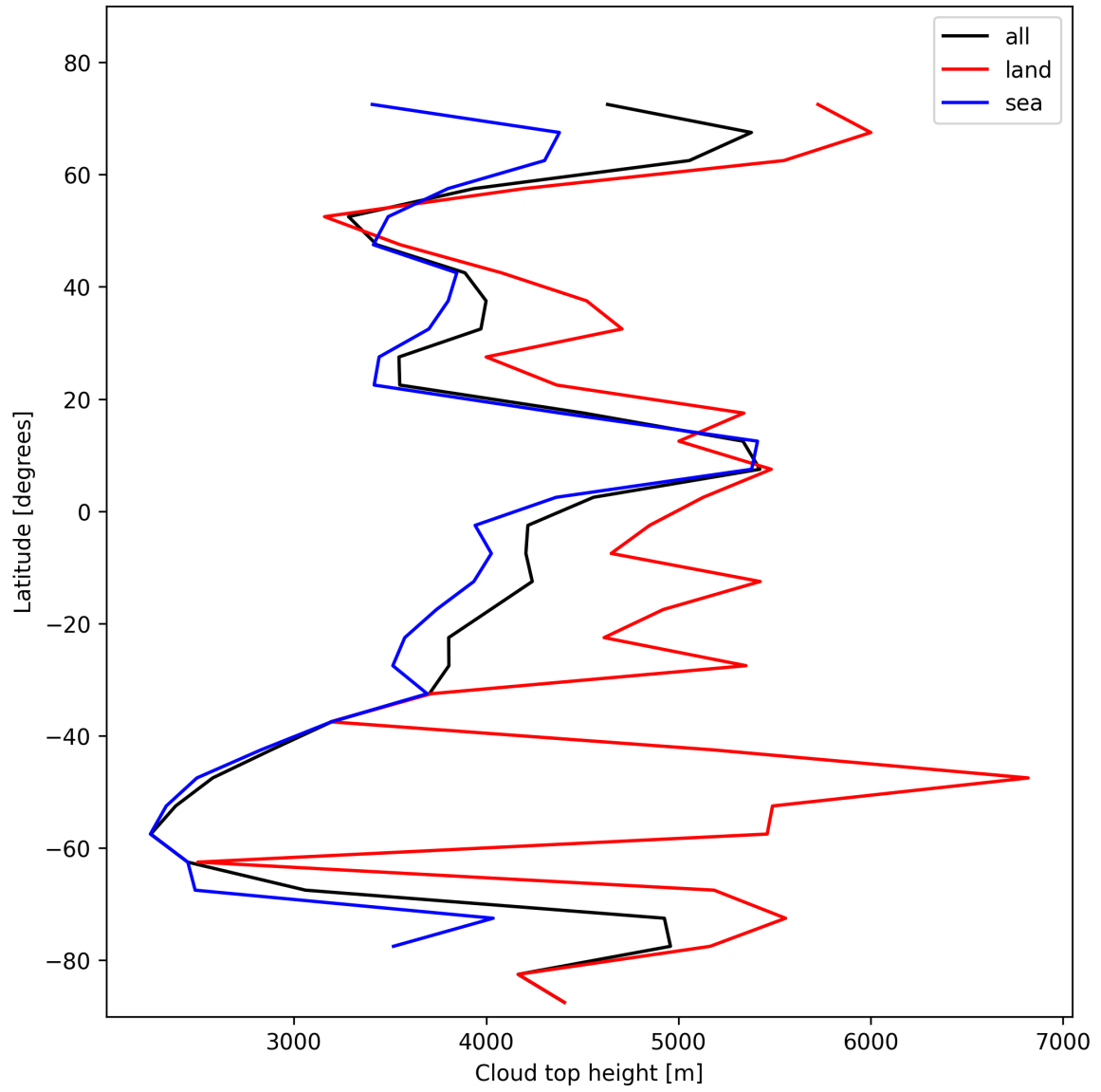
Figure 24: Zonal average of “Cloud top height” for 2025-11-15 to 2025-11-17.
