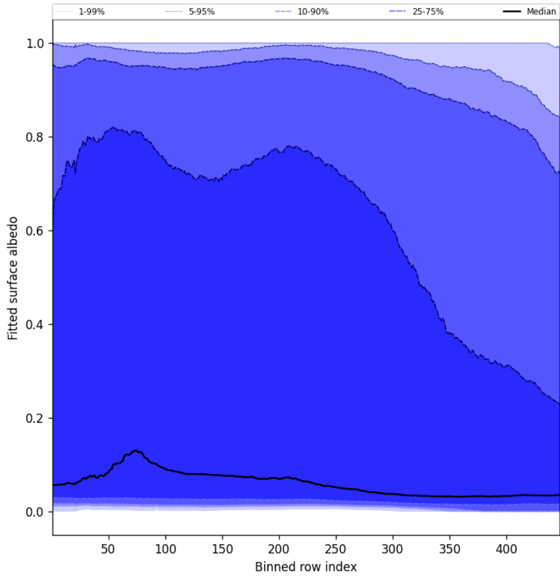
Figure 61: Along track statistics of “Fitted surface albedo” for 2025-11-15 to 2025-11-17
