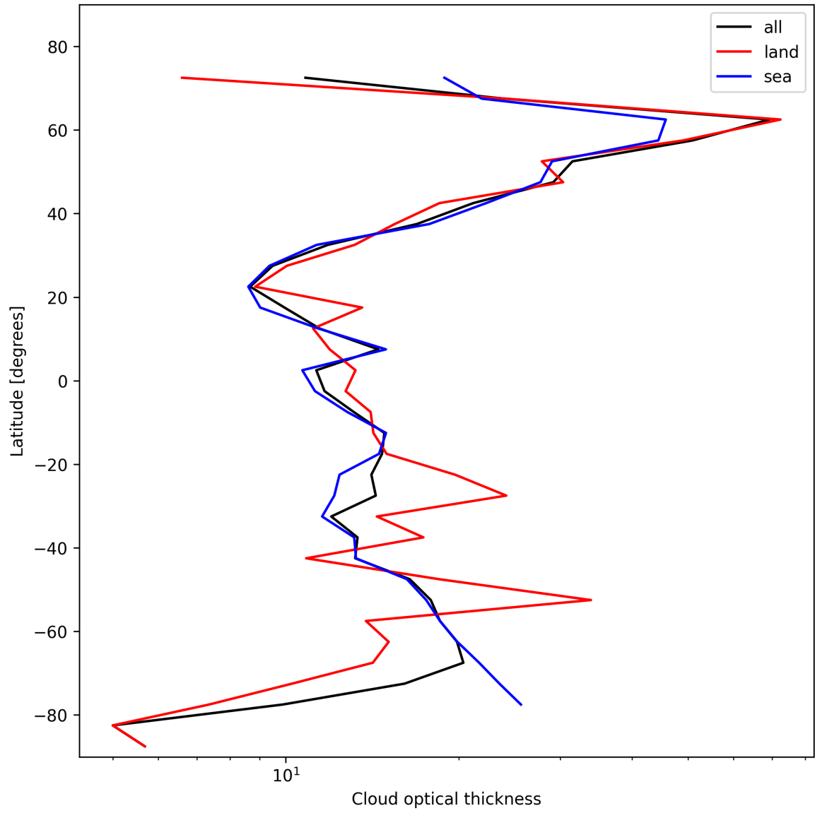
Figure 25: Zonal average of “Cloud optical thickness” for 2025-11-15 to 2025-11-17.
