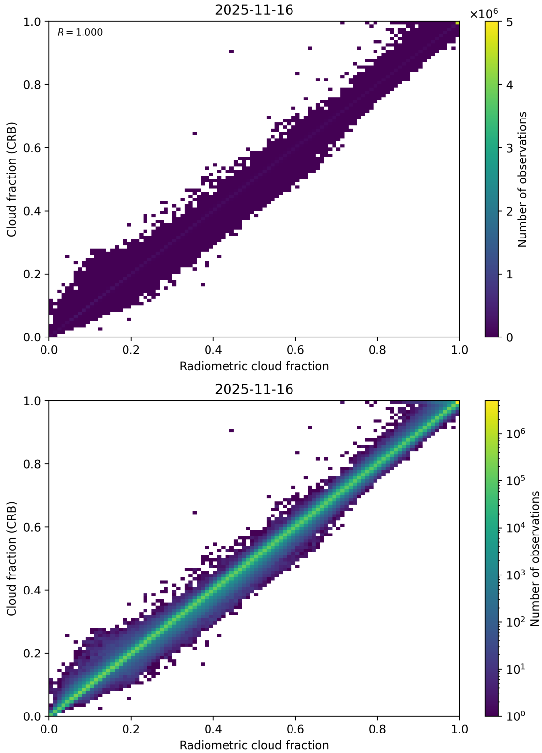
Figure 73: Scatter density plot of “Radiometric cloud fraction” against “Cloud fraction (CRB)” for 2025-11-15 to 2025-11-17.
