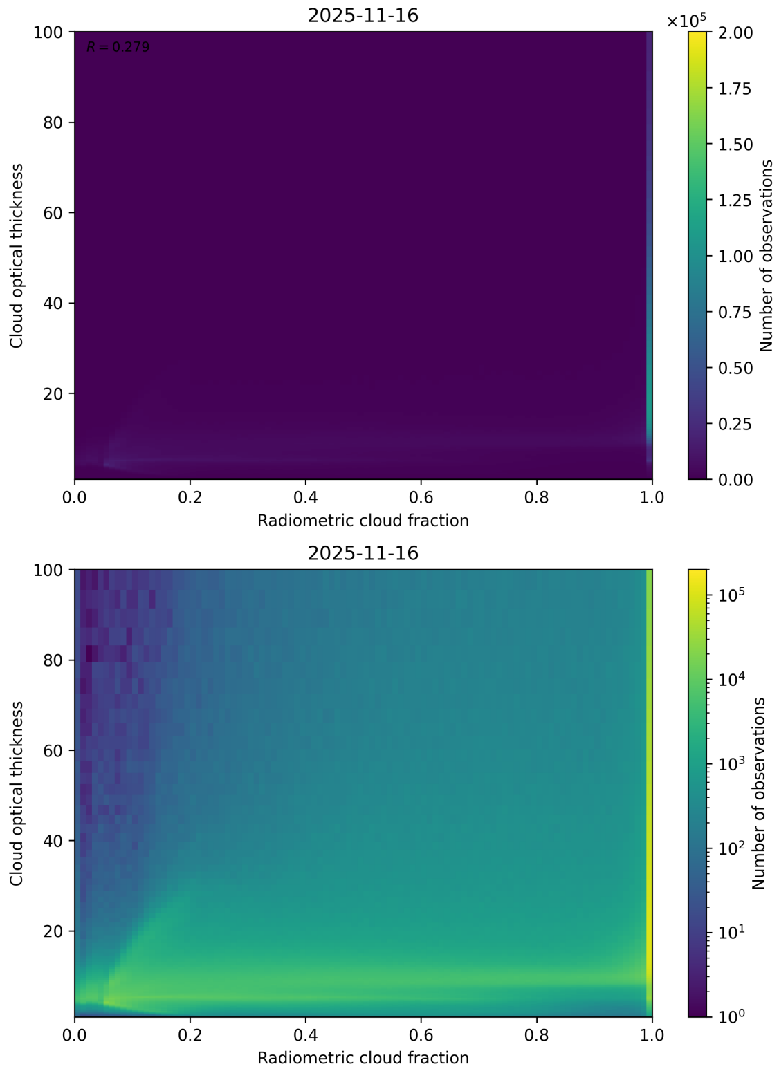
Figure 75: Scatter density plot of “Radiometric cloud fraction” against “Cloud optical thickness” for 2025-11-15 to 2025-11-17.
