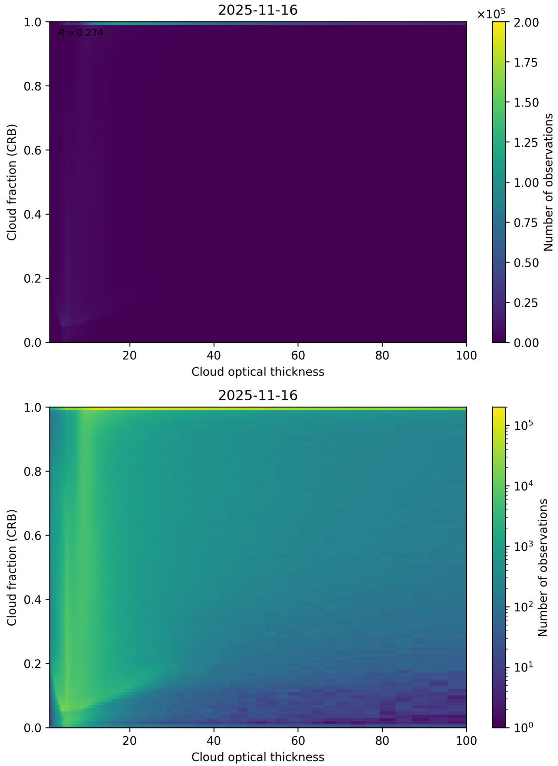
Figure 84: Scatter density plot of “Cloud optical thickness” against “Cloud fraction (CRB)” for 2025-11-15 to 2025-11-17.
