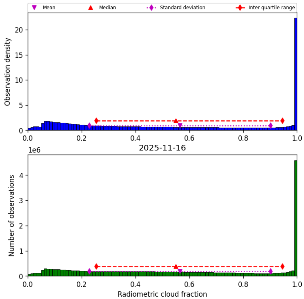
Figure 39: Histogram of “Radiometric cloud fraction” for 2025-11-15 to 2025-11-17
