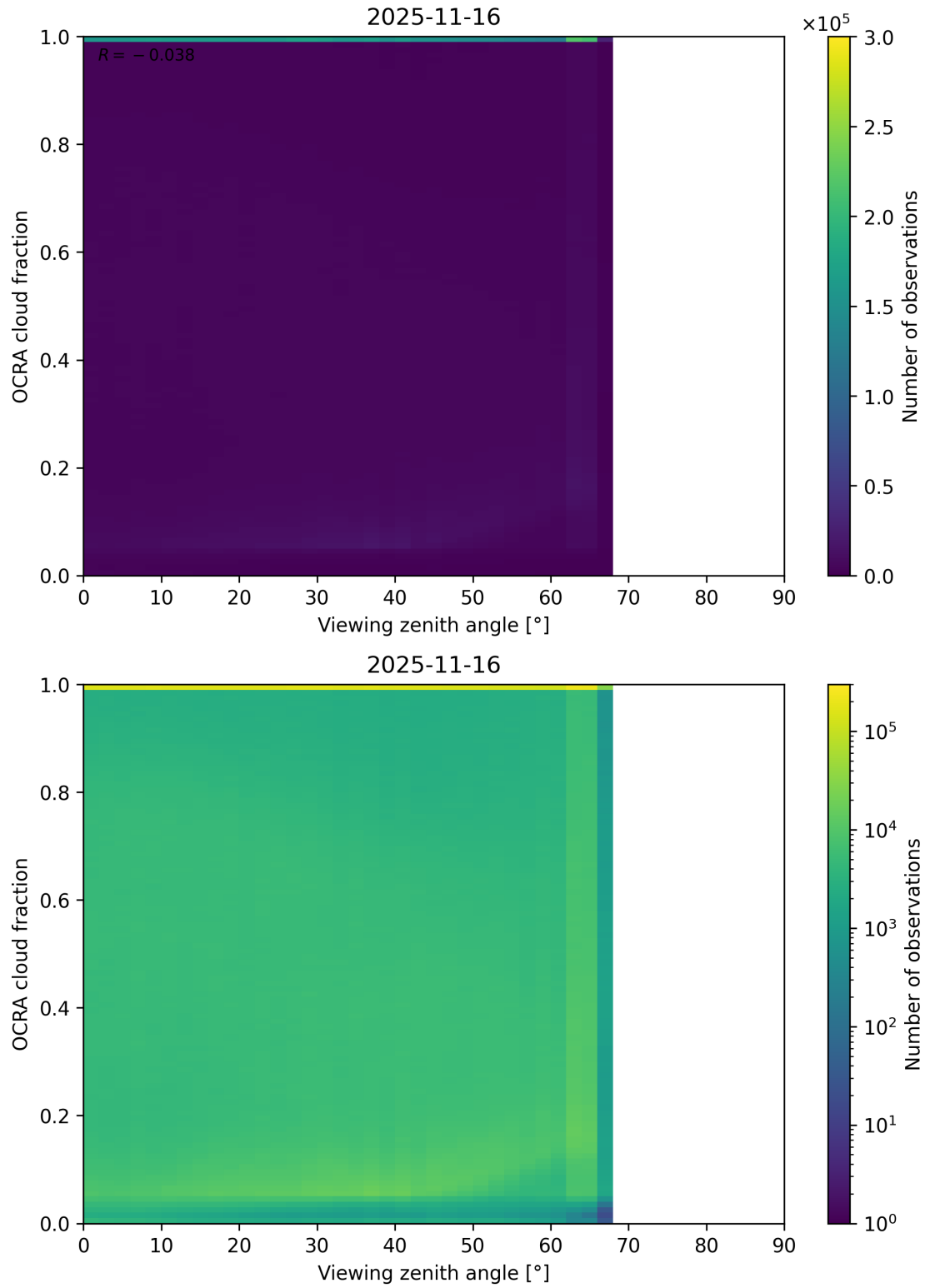
Figure 108: Scatter density plot of “Viewing zenith angle” against “OCRA cloud fraction” for 2025-11-15 to 2025-11-17.
