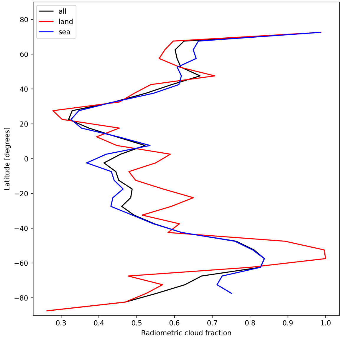
Figure 23: Zonal average of “Radiometric cloud fraction” for 2025-11-15 to 2025-11-17.
