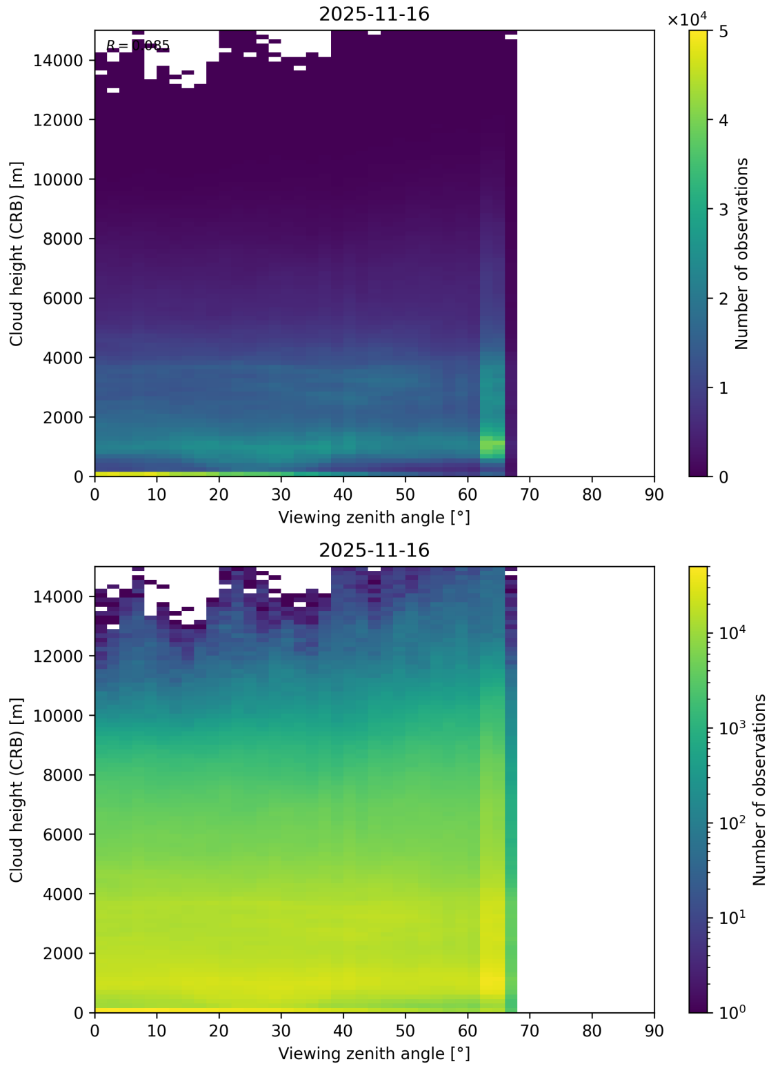
Figure 110: Scatter density plot of “Viewing zenith angle” against “Cloud height (CRB)” for 2025-11-15 to 2025-11-17.
