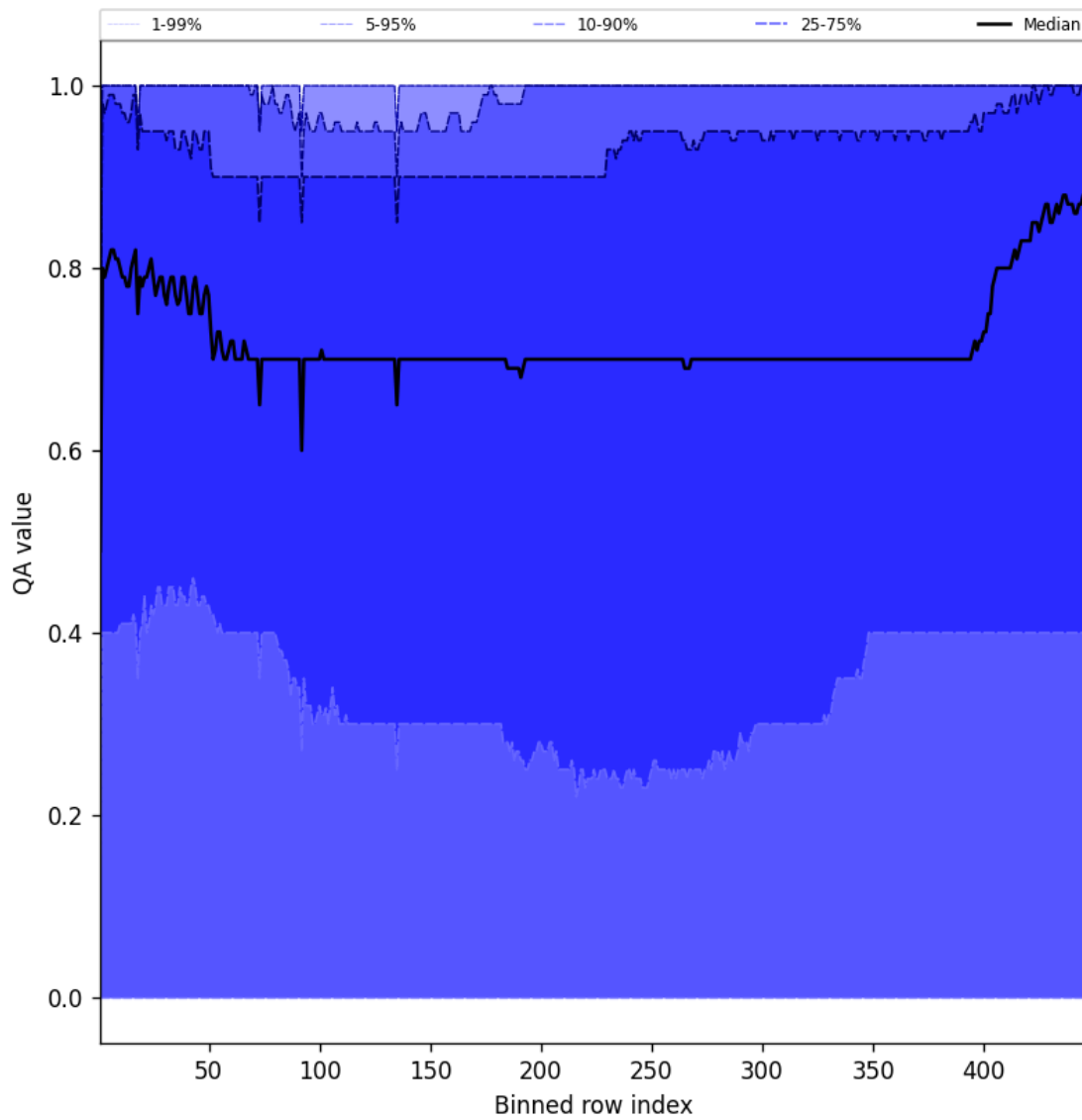
Figure 54: Along track statistics of “QA value” for 2025-11-15 to 2025-11-17
