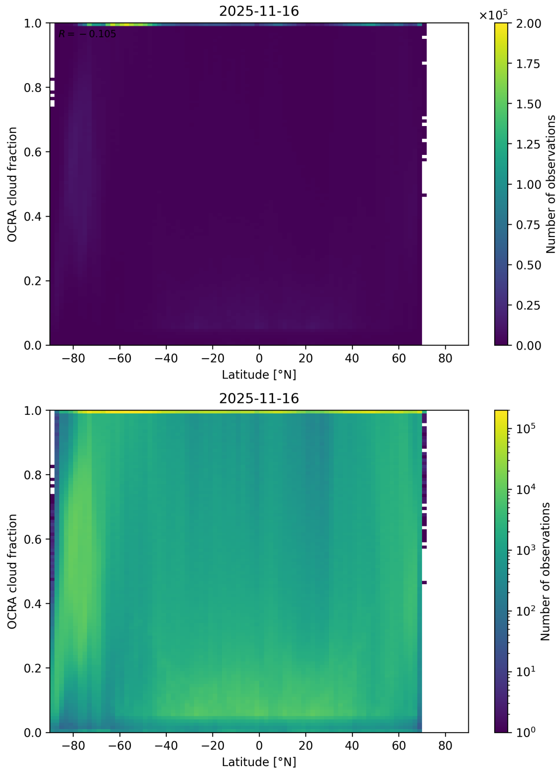
Figure 93: Scatter density plot of “Latitude” against “OCRA cloud fraction” for 2025-11-15 to 2025-11-17.
