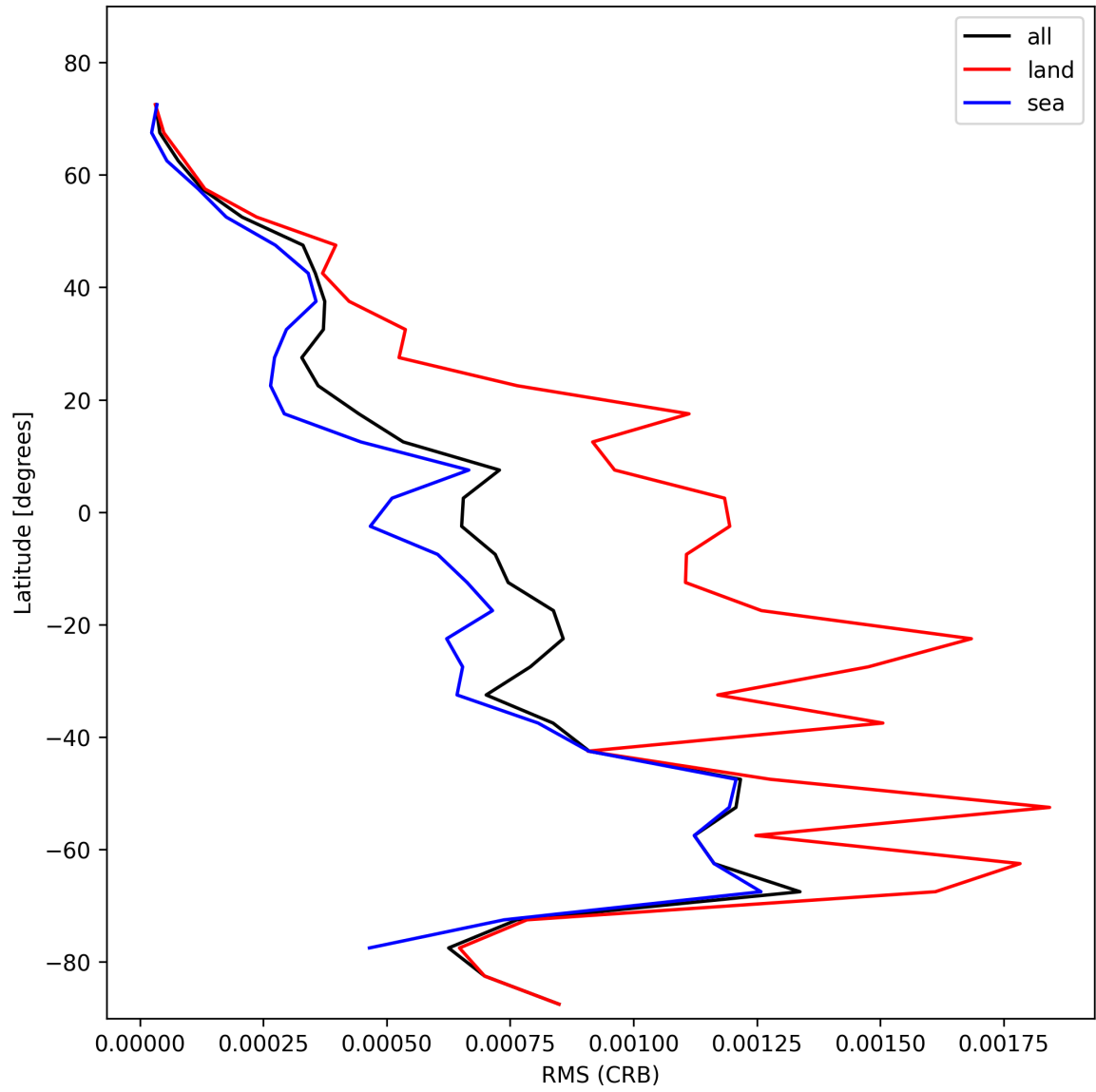
Figure 32: Zonal average of “RMS (CRB)” for 2025-11-15 to 2025-11-17.
