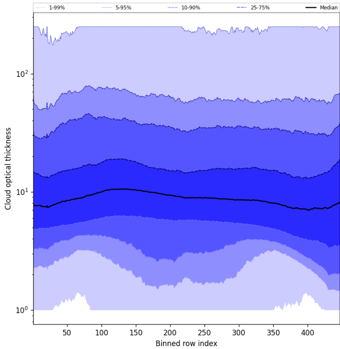
Figure 57: Along track statistics of “Cloud optical thickness” for 2025-11-15 to 2025-11-17
