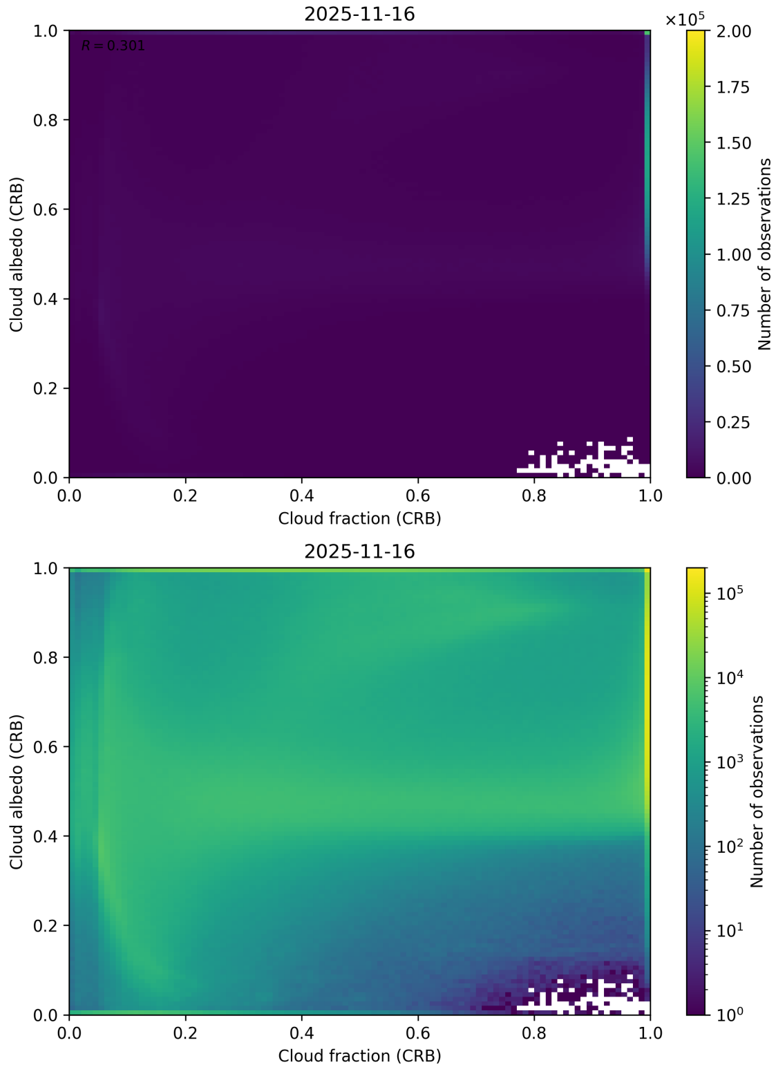
Figure 77: Scatter density plot of “Cloud fraction (CRB)” against “Cloud albedo (CRB)” for 2025-11-15 to 2025-11-17.
