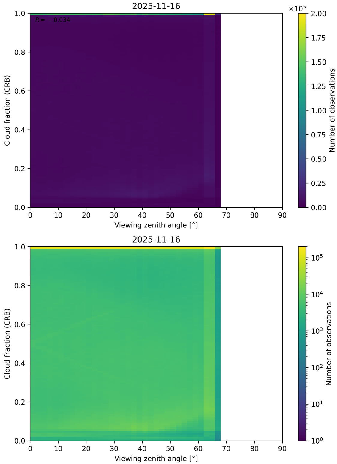
Figure 109: Scatter density plot of “Viewing zenith angle” against “Cloud fraction (CRB)” for 2025-11-15 to 2025-11-17.
