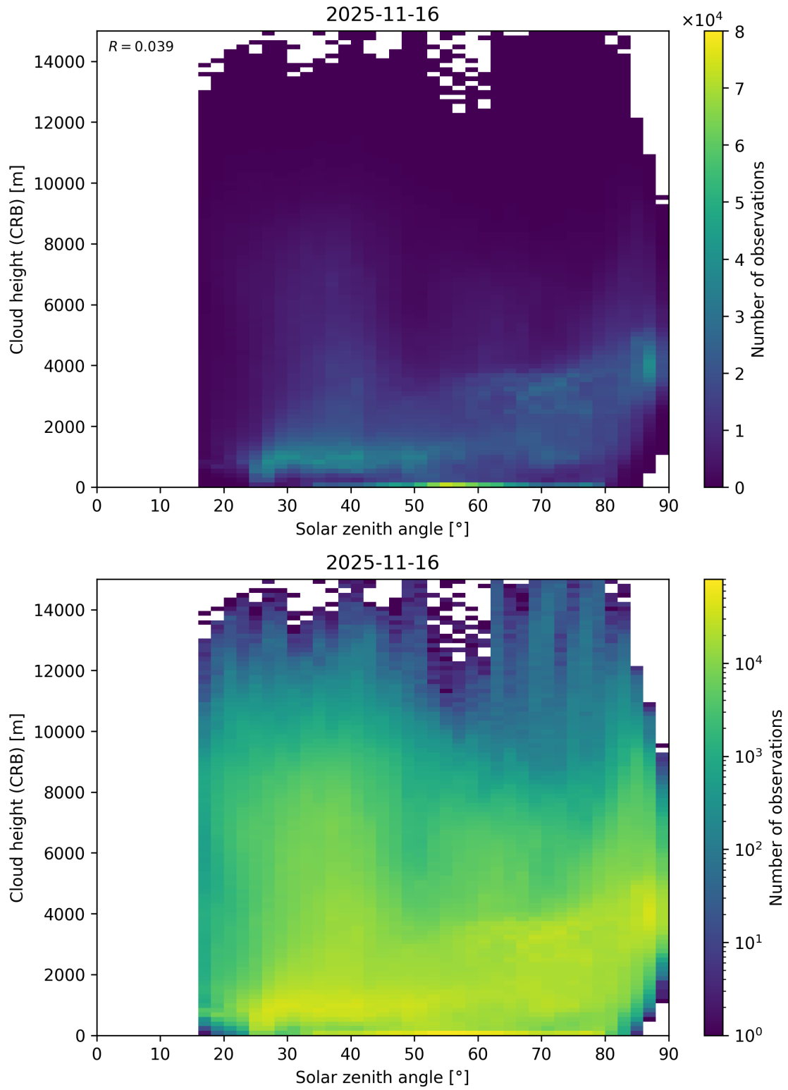
Figure 102: Scatter density plot of “Solar zenith angle” against “Cloud height (CRB)” for 2025-11-15 to 2025-11-17.
