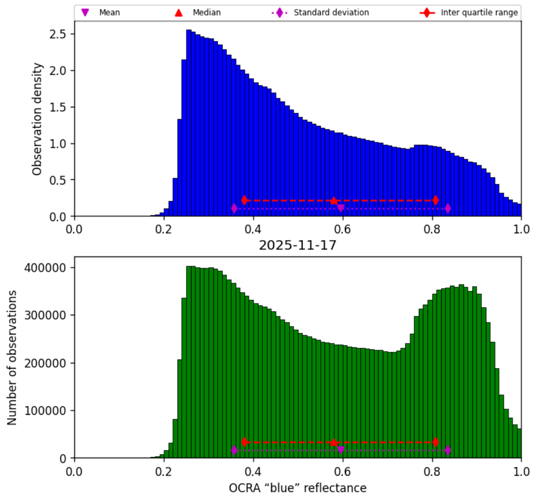
Figure 51: Histogram of “OCRA “blue” reflectance” for 2025-11-16 to 2025-11-18
