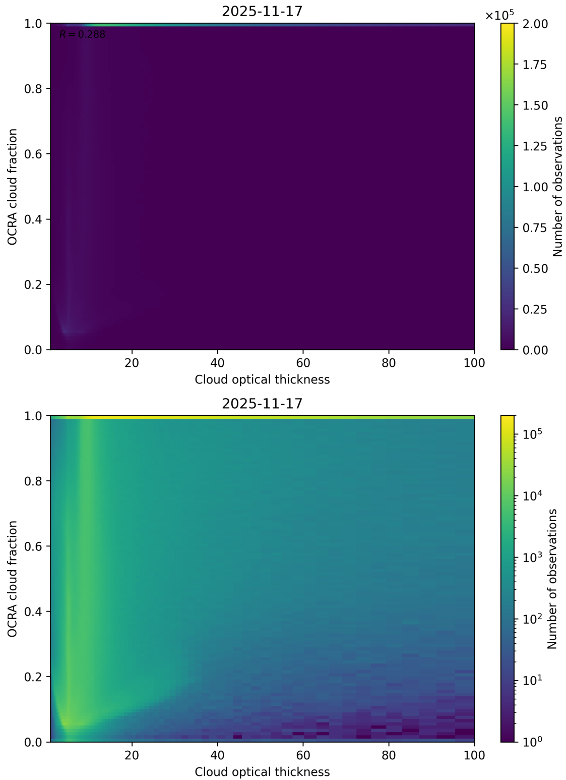
Figure 83: Scatter density plot of “Cloud optical thickness” against “OCRA cloud fraction” for 2025-11-16 to 2025-11-18.
