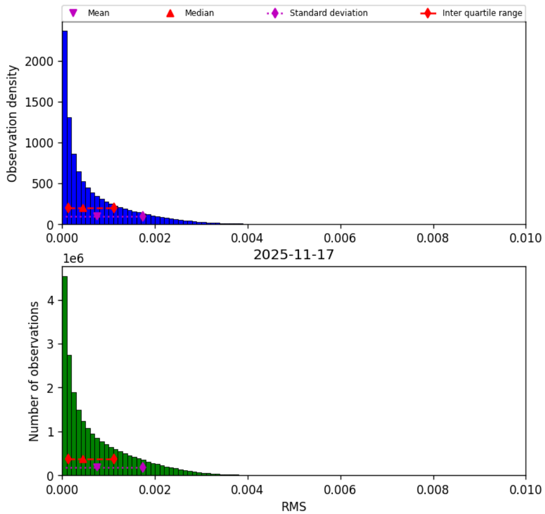
Figure 47: Histogram of “RMS” for 2025-11-16 to 2025-11-18
