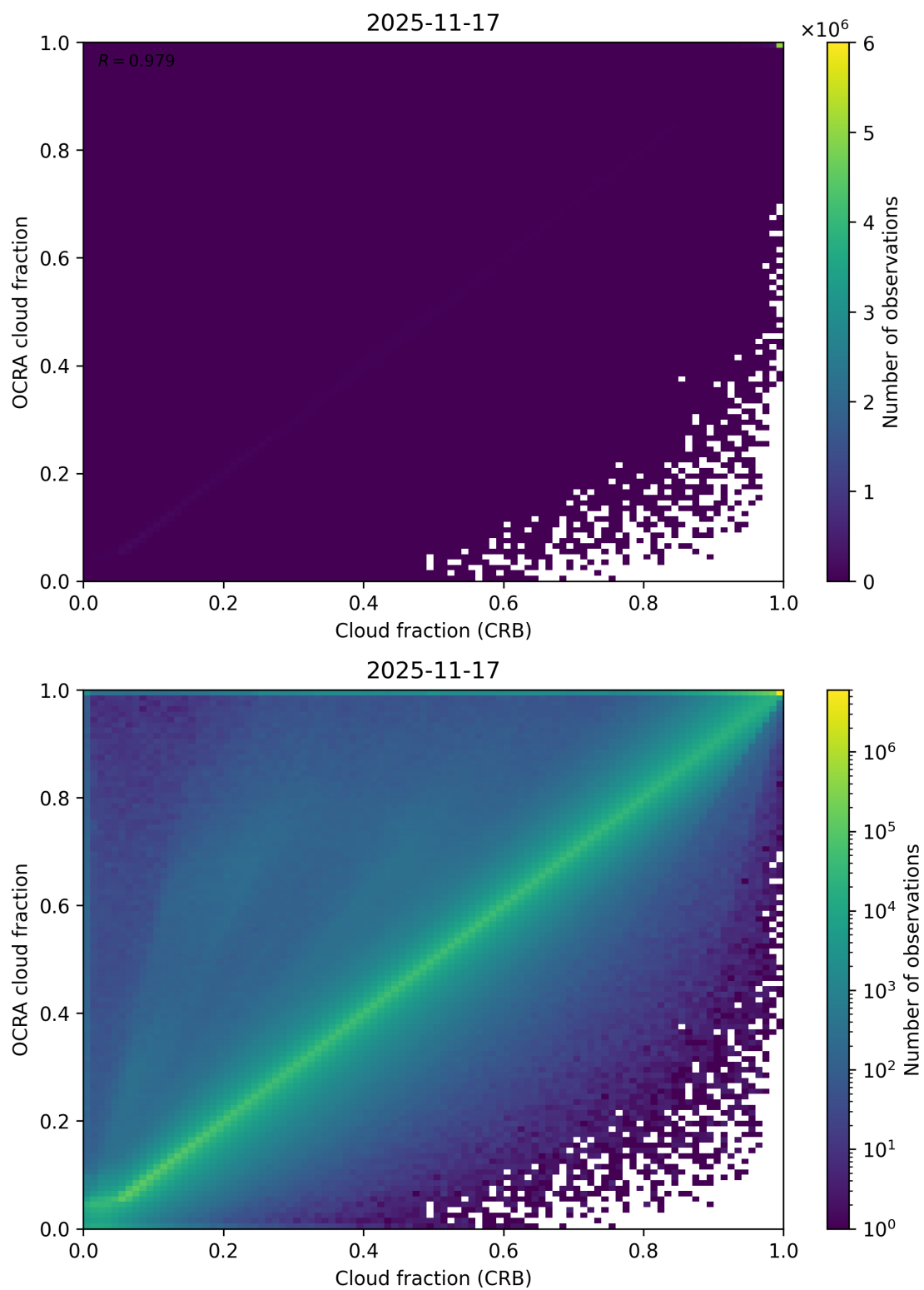
Figure 78: Scatter density plot of “Cloud fraction (CRB)” against “OCRA cloud fraction” for 2025-11-16 to 2025-11-18.
