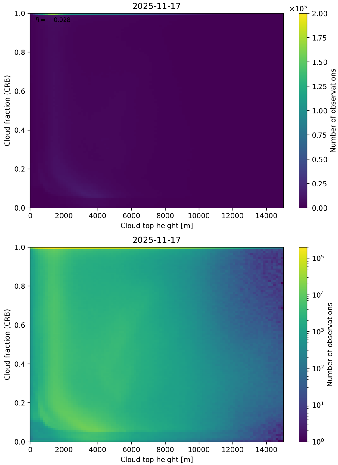
Figure 88: Scatter density plot of “Cloud top height” against “Cloud fraction (CRB)” for 2025-11-16 to 2025-11-18.
