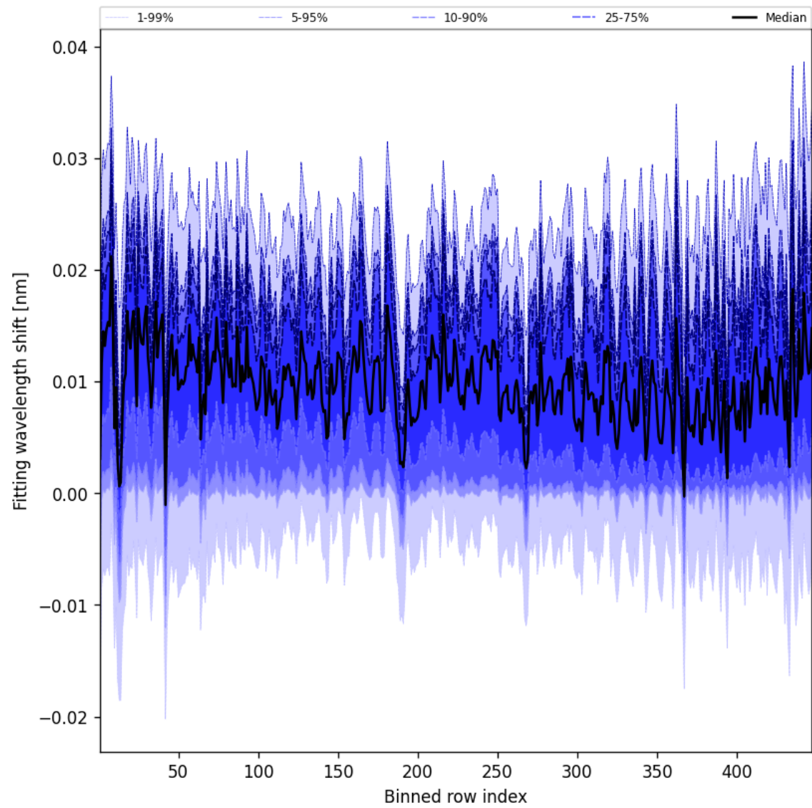
Figure 65: Along track statistics of “Fitting wavelength shift” for 2025-11-16 to 2025-11-18
