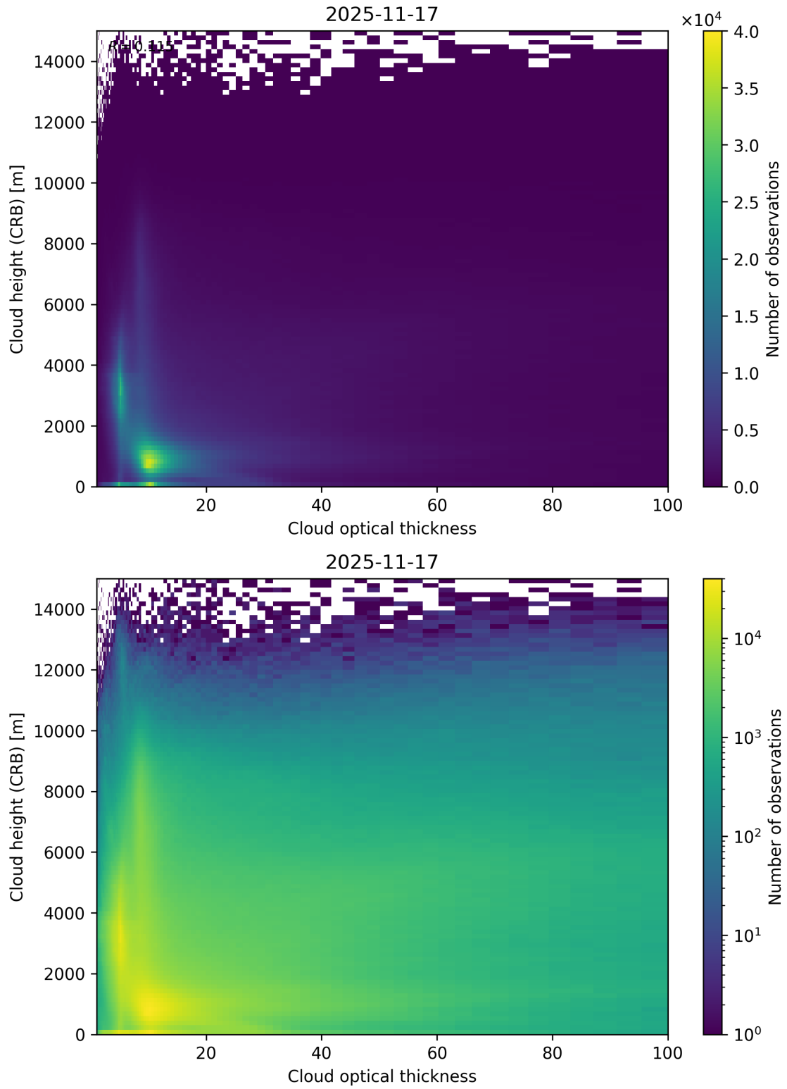
Figure 85: Scatter density plot of “Cloud optical thickness” against “Cloud height (CRB)” for 2025-11-16 to 2025-11-18.
