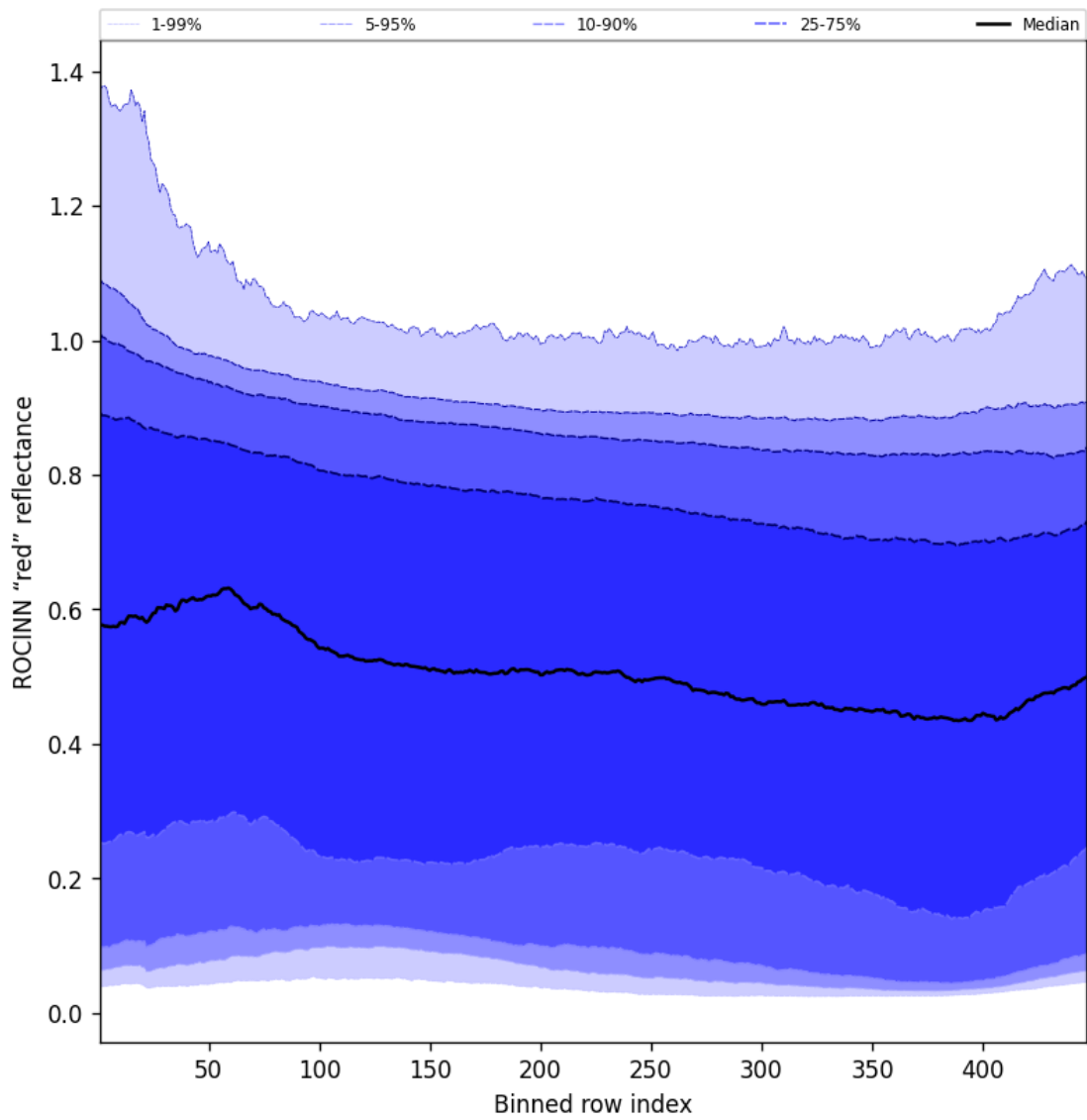
Figure 69: Along track statistics of “ROCINN “red” reflectance” for 2025-11-16 to 2025-11-18
