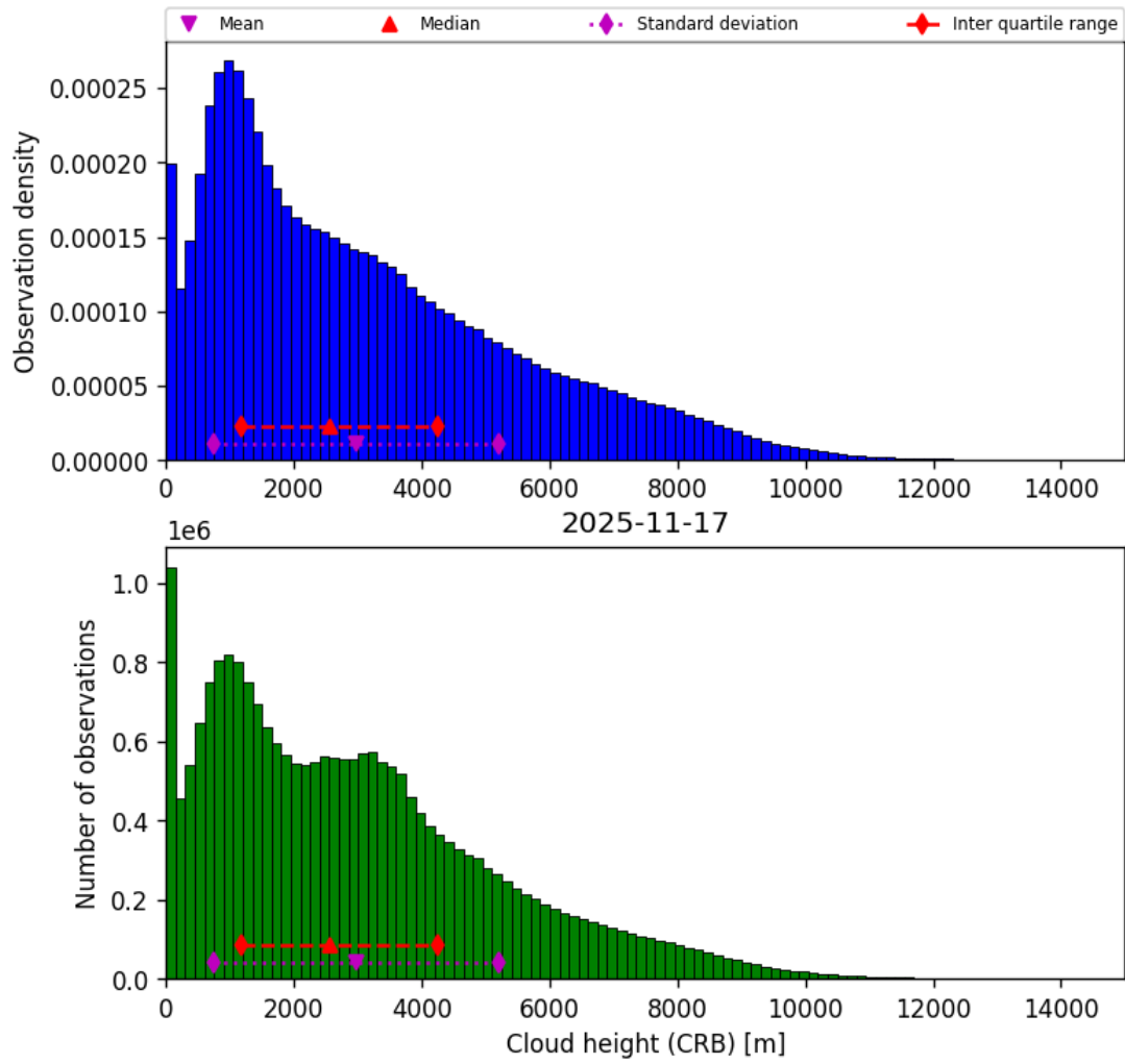
Figure 43: Histogram of “Cloud height (CRB)” for 2025-11-16 to 2025-11-18
