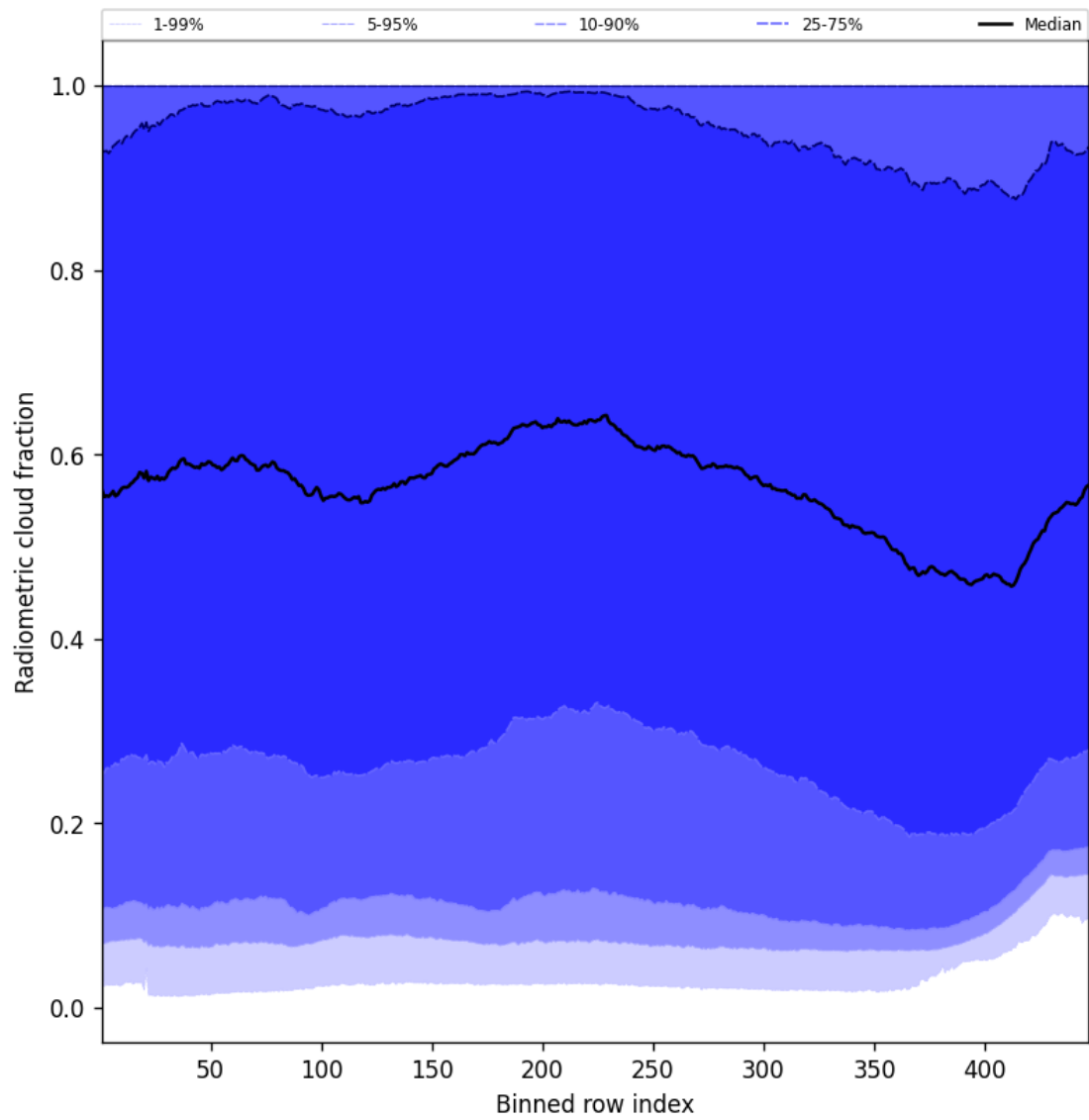
Figure 55: Along track statistics of “Radiometric cloud fraction” for 2025-11-16 to 2025-11-18
