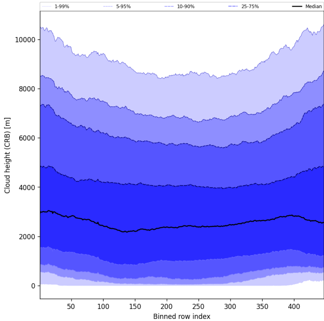
Figure 59: Along track statistics of “Cloud height (CRB)” for 2025-11-16 to 2025-11-18
