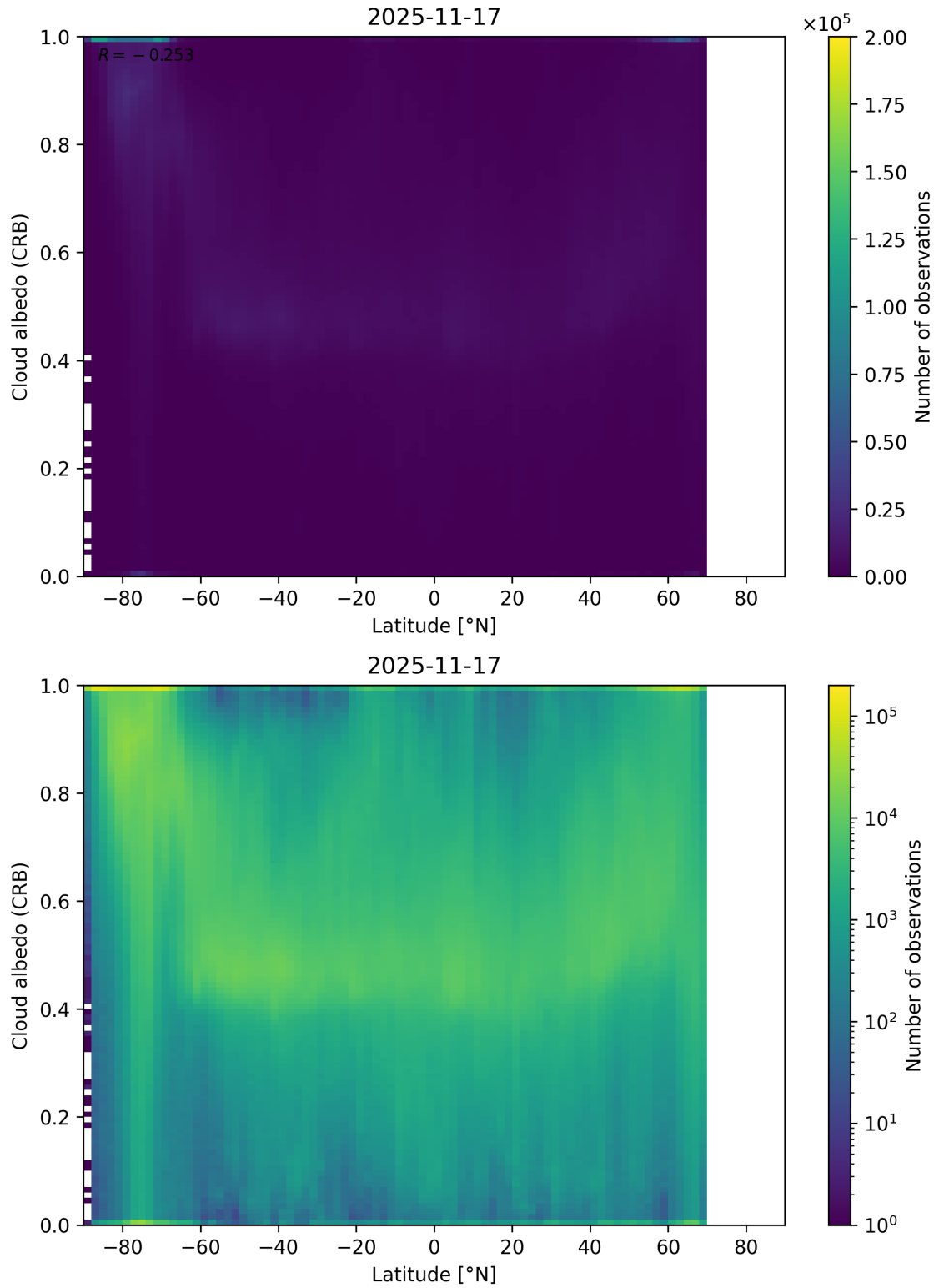
Figure 91: Scatter density plot of “Latitude” against “Cloud albedo (CRB)” for 2025-11-16 to 2025-11-18.
