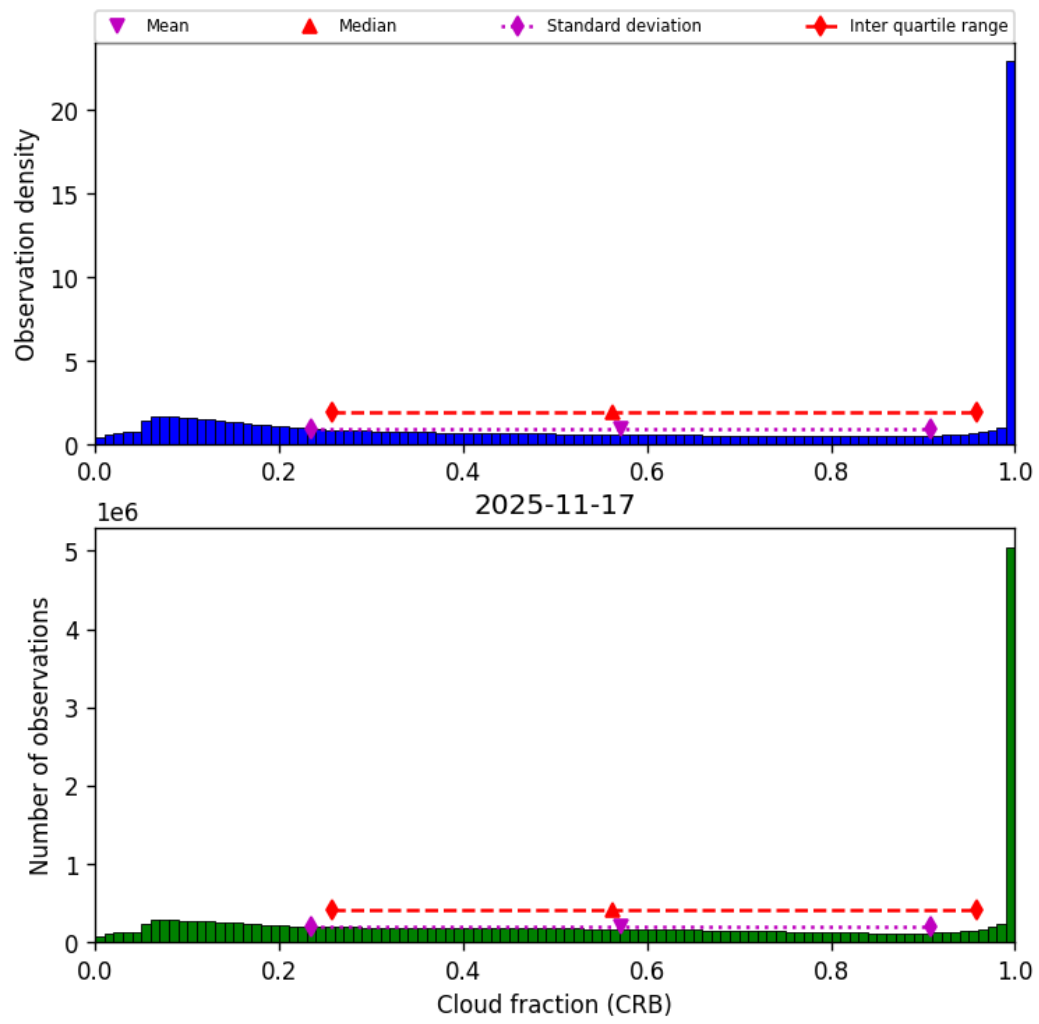
Figure 42: Histogram of “Cloud fraction (CRB)” for 2025-11-16 to 2025-11-18
