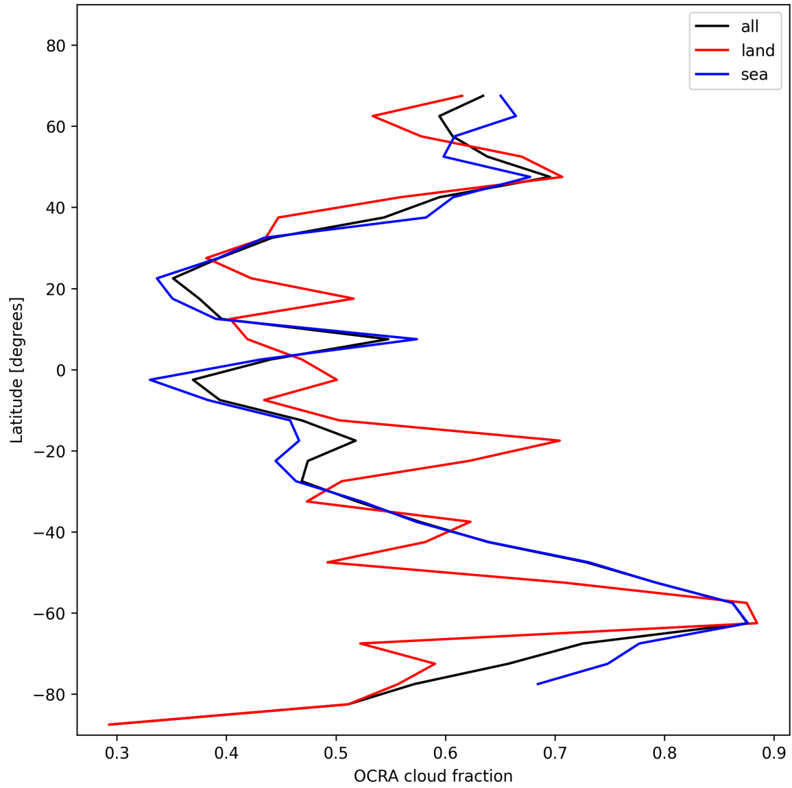
Figure 34: Zonal average of “OCRA cloud fraction” for 2025-11-16 to 2025-11-18.
