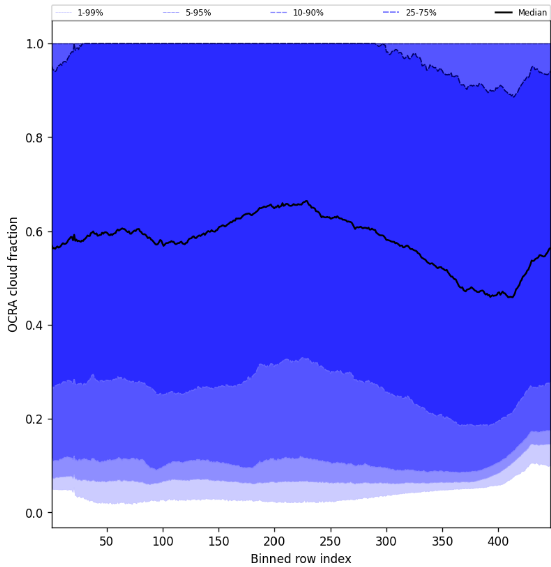
Figure 66: Along track statistics of “OCRA cloud fraction” for 2025-11-16 to 2025-11-18
