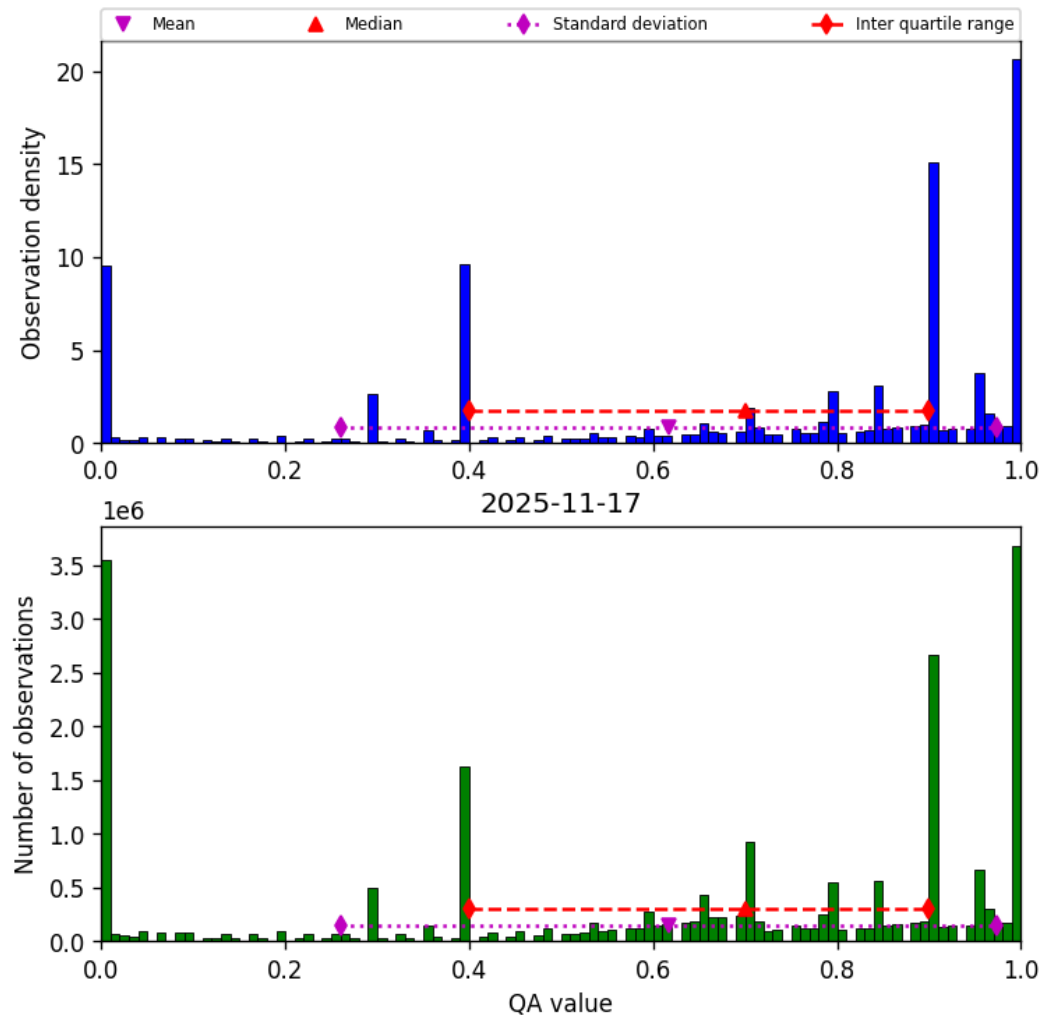
Figure 38: Histogram of “QA value” for 2025-11-16 to 2025-11-18
