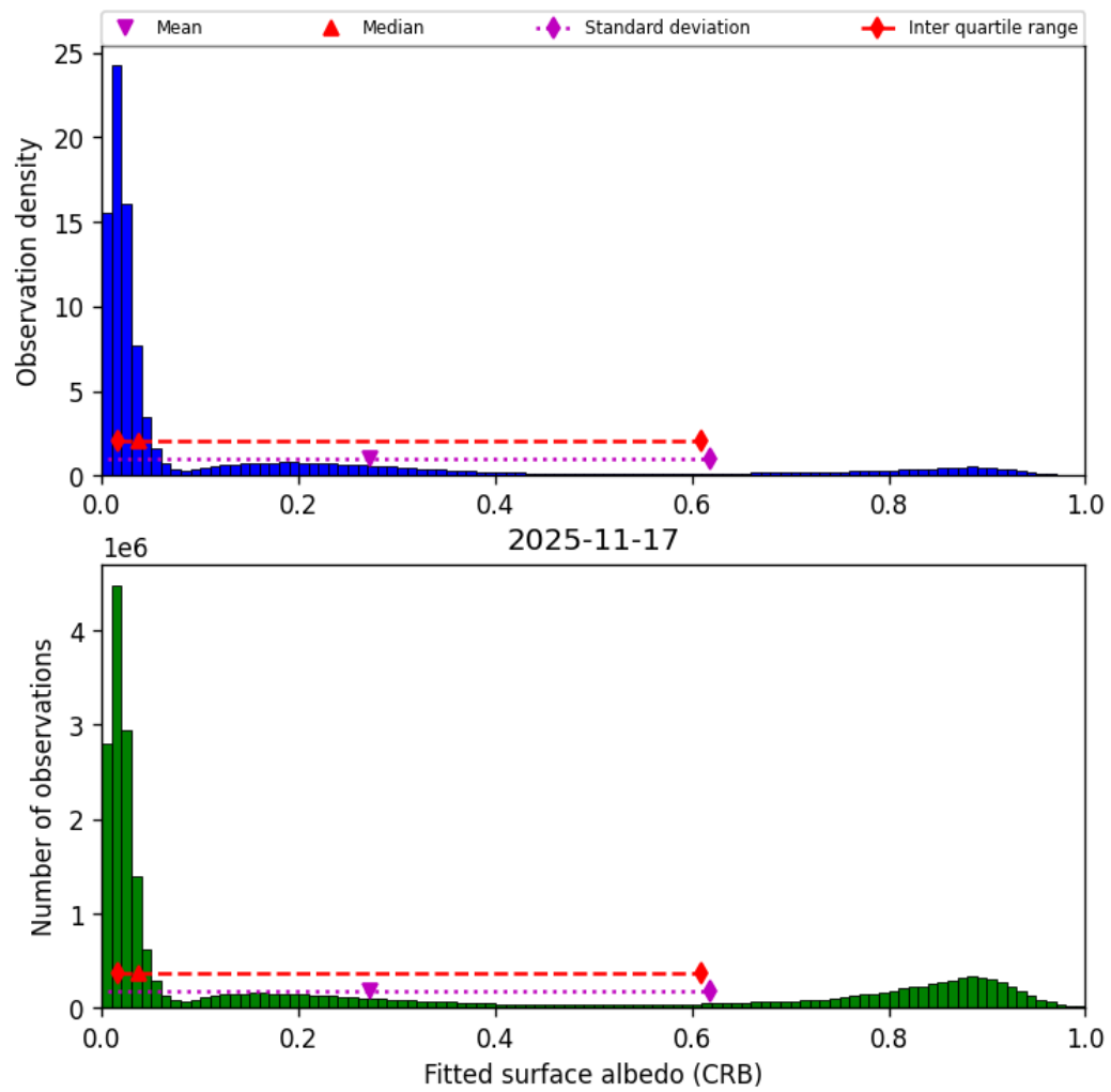
Figure 46: Histogram of “Fitted surface albedo (CRB)” for 2025-11-16 to 2025-11-18
