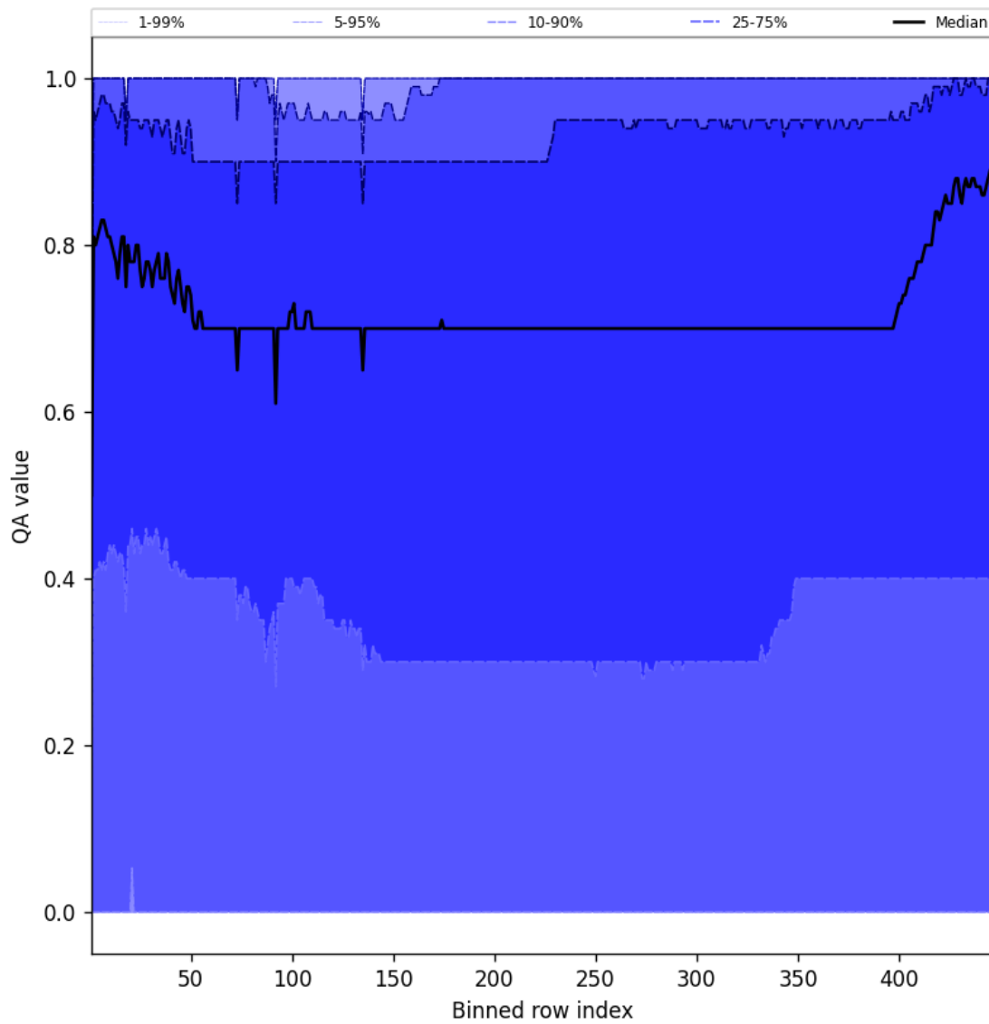
Figure 54: Along track statistics of “QA value” for 2025-11-16 to 2025-11-18
