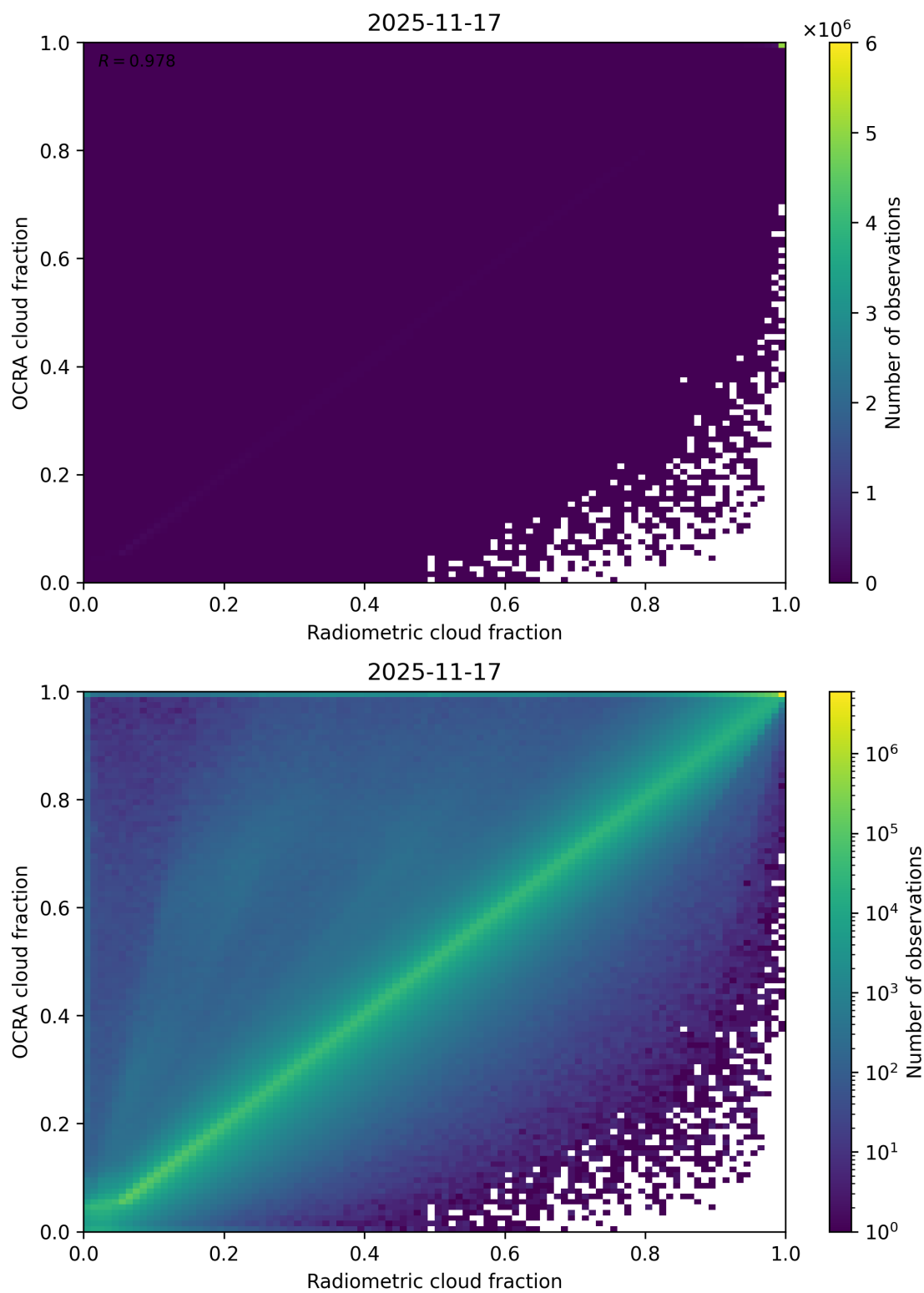
Figure 72: Scatter density plot of “Radiometric cloud fraction” against “OCRA cloud fraction” for 2025-11-16 to 2025-11-18.
