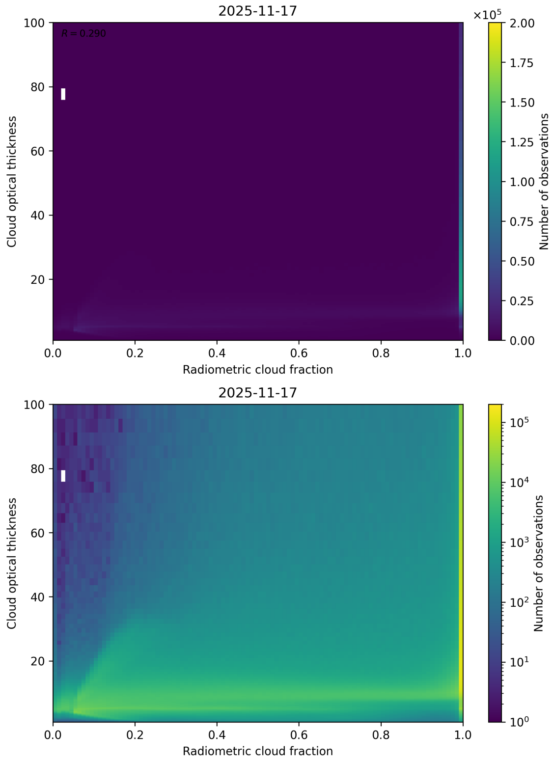
Figure 75: Scatter density plot of “Radiometric cloud fraction” against “Cloud optical thickness” for 2025-11-16 to 2025-11-18.
