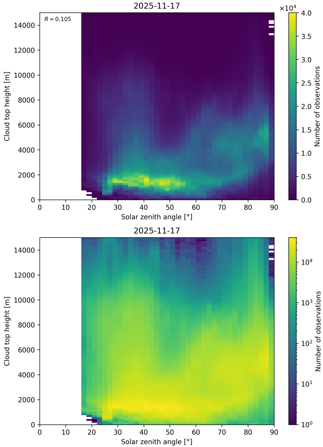
Figure 104: Scatter density plot of “Solar zenith angle” against “Cloud top height” for 2025-11-16 to 2025-11-18.
