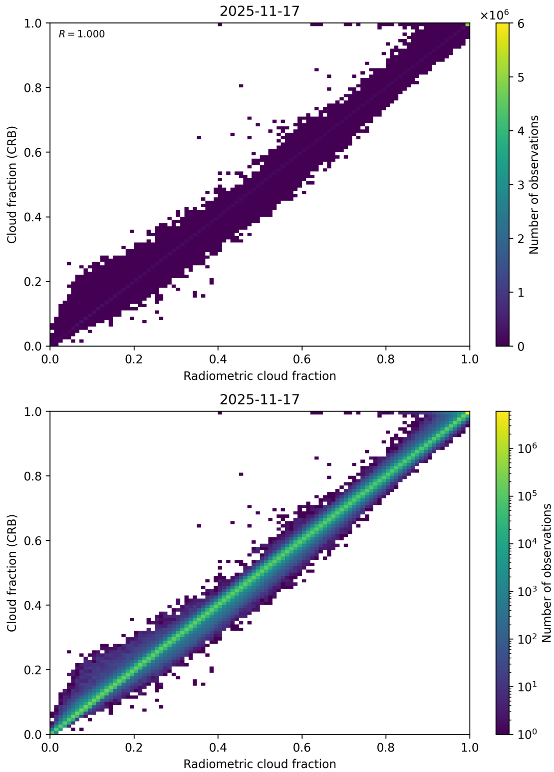
Figure 73: Scatter density plot of “Radiometric cloud fraction” against “Cloud fraction (CRB)” for 2025-11-16 to 2025-11-18.
