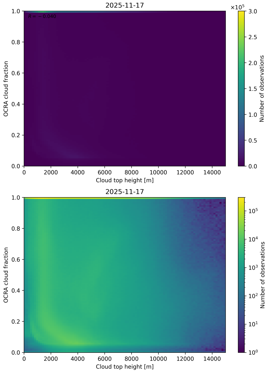
Figure 87: Scatter density plot of “Cloud top height” against “OCRA cloud fraction” for 2025-11-16 to 2025-11-18.
