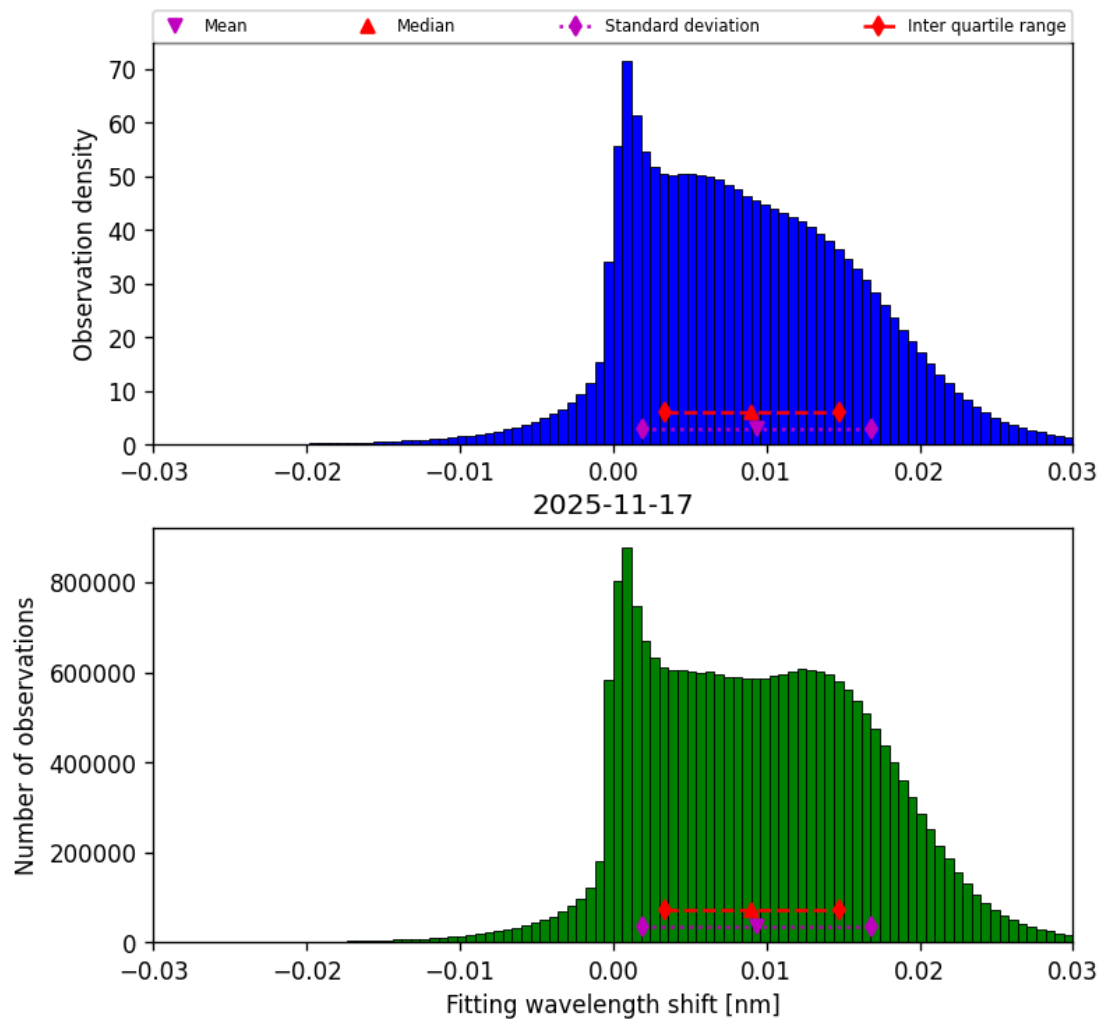
Figure 49: Histogram of “Fitting wavelength shift” for 2025-11-16 to 2025-11-18
