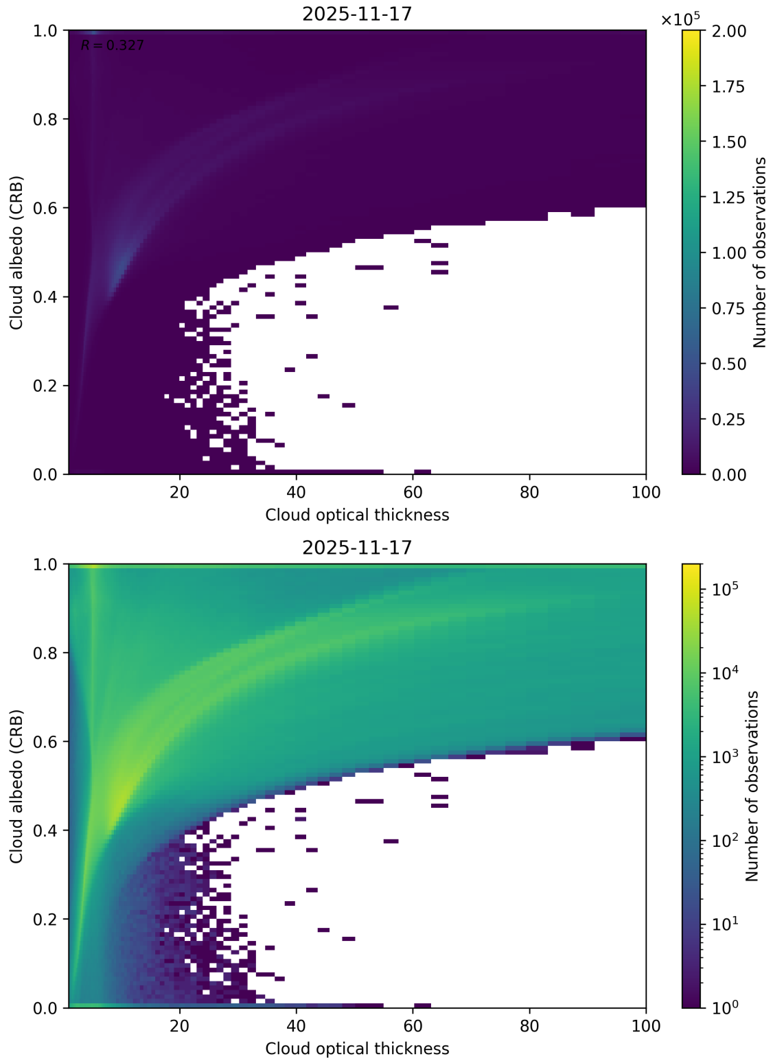
Figure 82: Scatter density plot of “Cloud optical thickness” against “Cloud albedo (CRB)” for 2025-11-16 to 2025-11-18.
