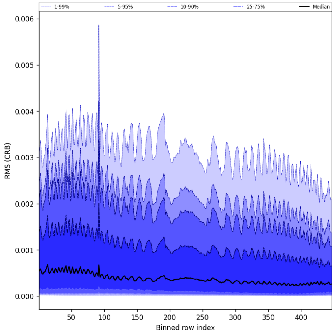
Figure 64: Along track statistics of “RMS (CRB)” for 2025-11-16 to 2025-11-18
