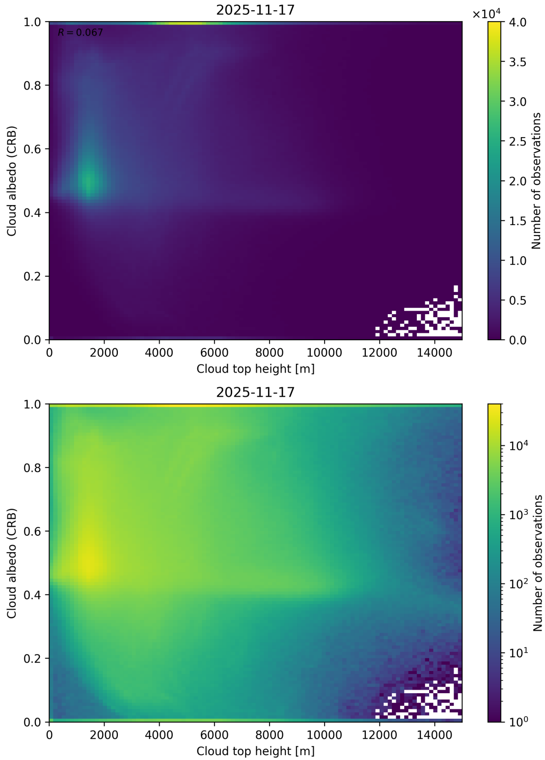
Figure 86: Scatter density plot of “Cloud top height” against “Cloud albedo (CRB)” for 2025-11-16 to 2025-11-18.
