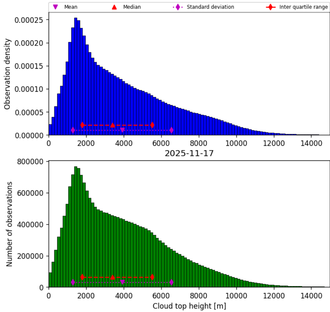
Figure 40: Histogram of “Cloud top height” for 2025-11-16 to 2025-11-18
