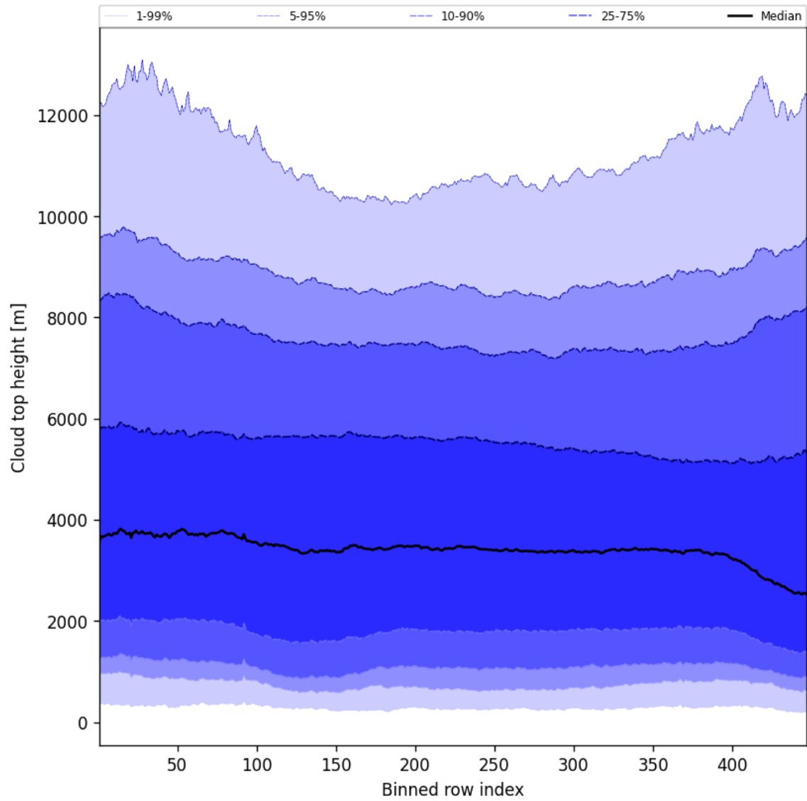
Figure 56: Along track statistics of “Cloud top height” for 2025-11-16 to 2025-11-18
