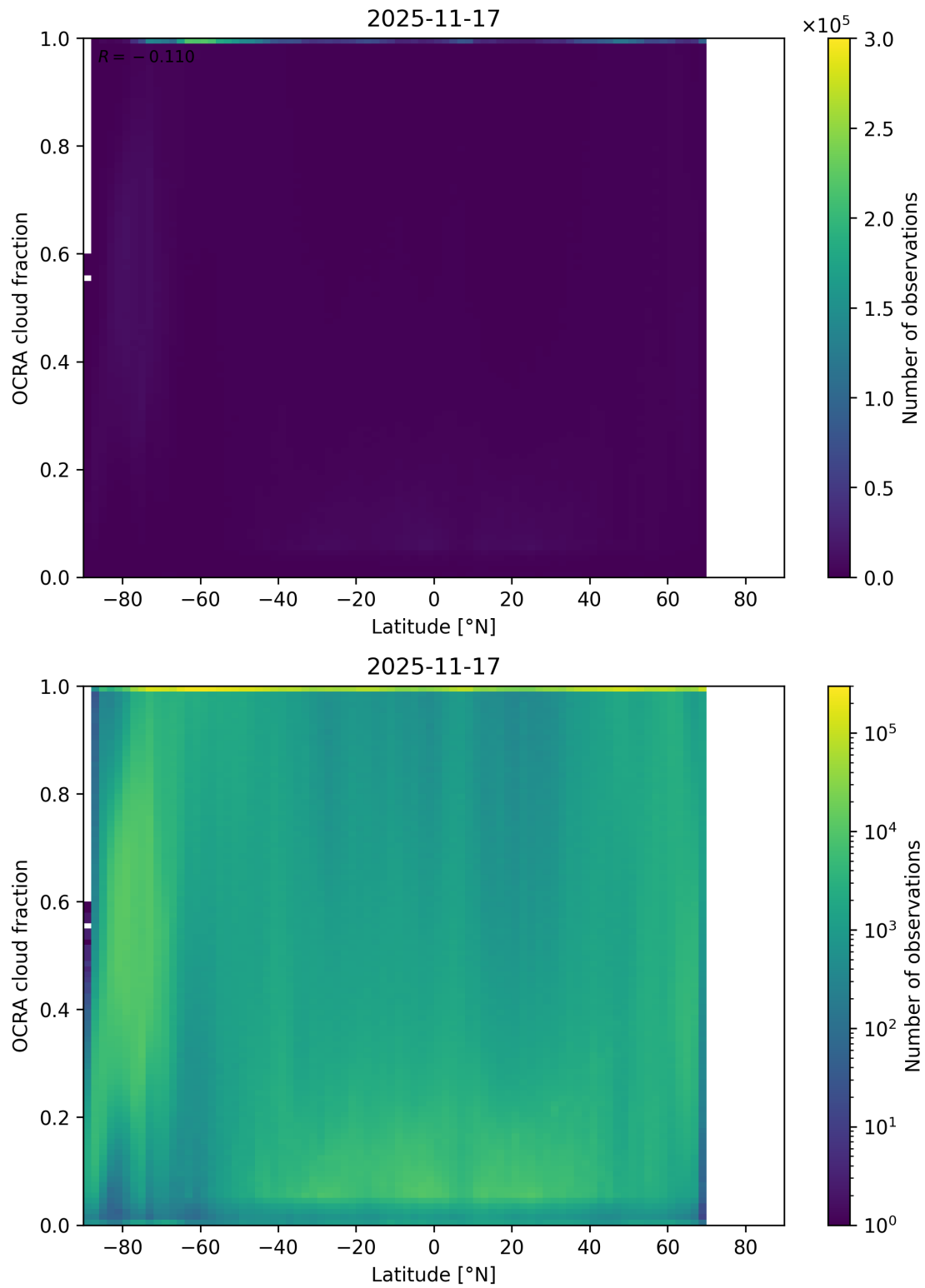
Figure 93: Scatter density plot of “Latitude” against “OCRA cloud fraction” for 2025-11-16 to 2025-11-18.
