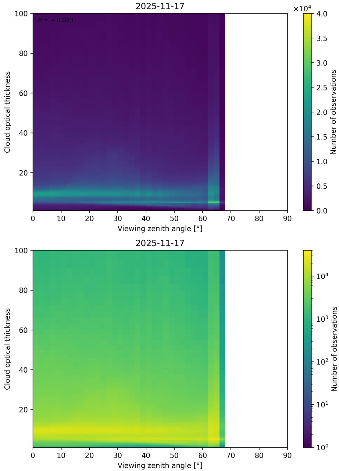
Figure 111: Scatter density plot of “Viewing zenith angle” against “Cloud optical thickness” for 2025-11-16 to 2025-11-18.
