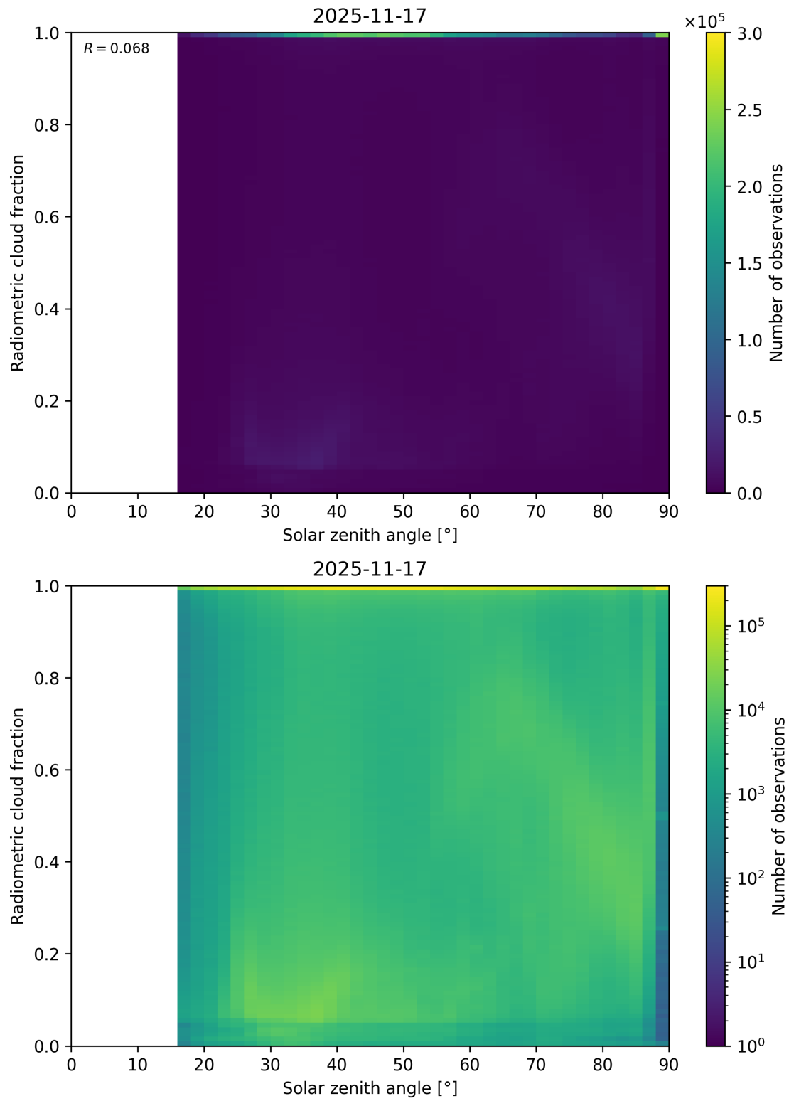
Figure 99: Scatter density plot of “Solar zenith angle” against “Radiometric cloud fraction” for 2025-11-16 to 2025-11-18.
