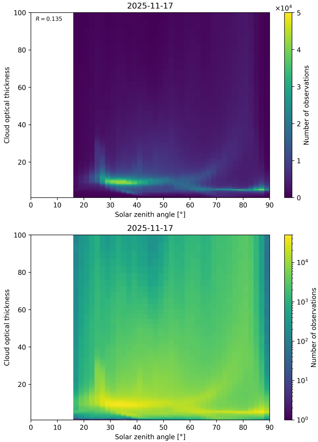
Figure 103: Scatter density plot of “Solar zenith angle” against “Cloud optical thickness” for 2025-11-16 to 2025-11-18.
