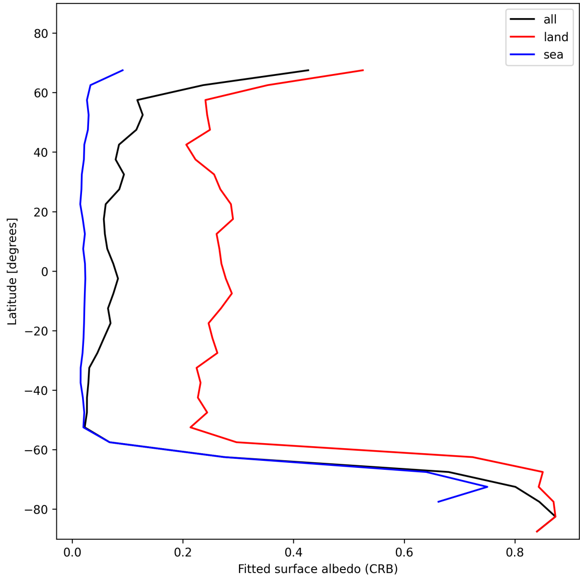
Figure 30: Zonal average of “Fitted surface albedo (CRB)” for 2025-11-16 to 2025-11-18.
