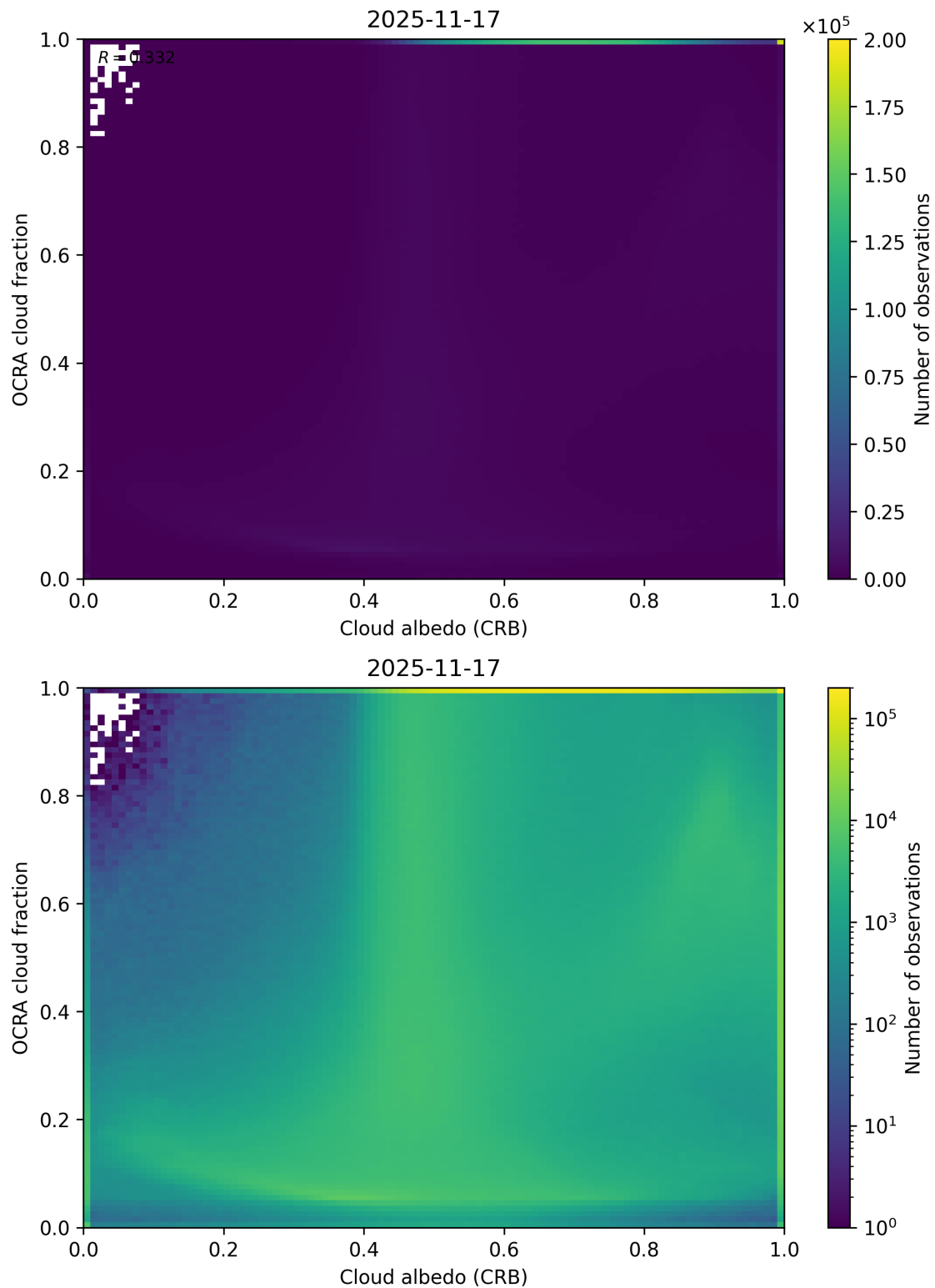
Figure 70: Scatter density plot of “Cloud albedo (CRB)” against “OCRA cloud fraction” for 2025-11-16 to 2025-11-18.
