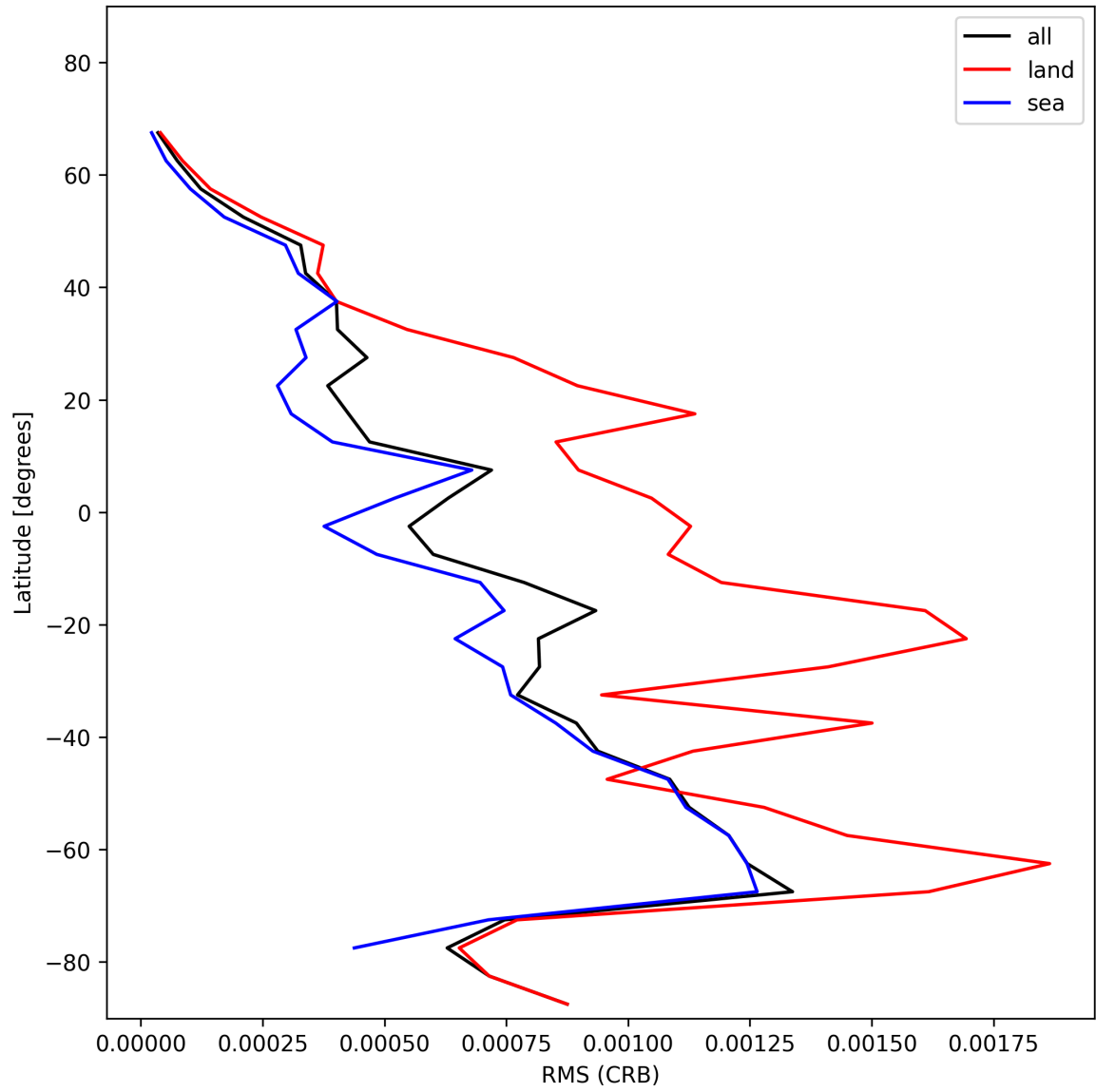
Figure 32: Zonal average of “RMS (CRB)” for 2025-11-16 to 2025-11-18.
