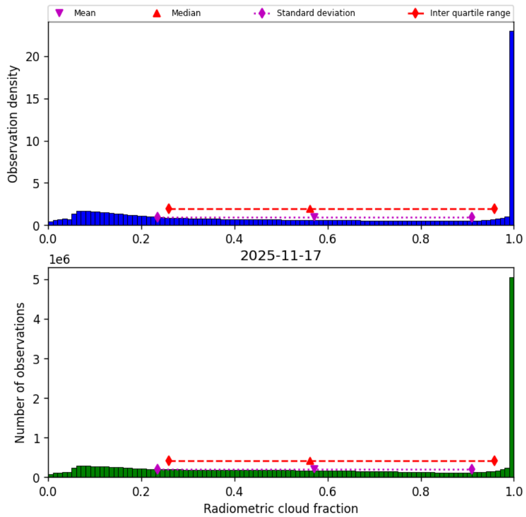
Figure 39: Histogram of “Radiometric cloud fraction” for 2025-11-16 to 2025-11-18
