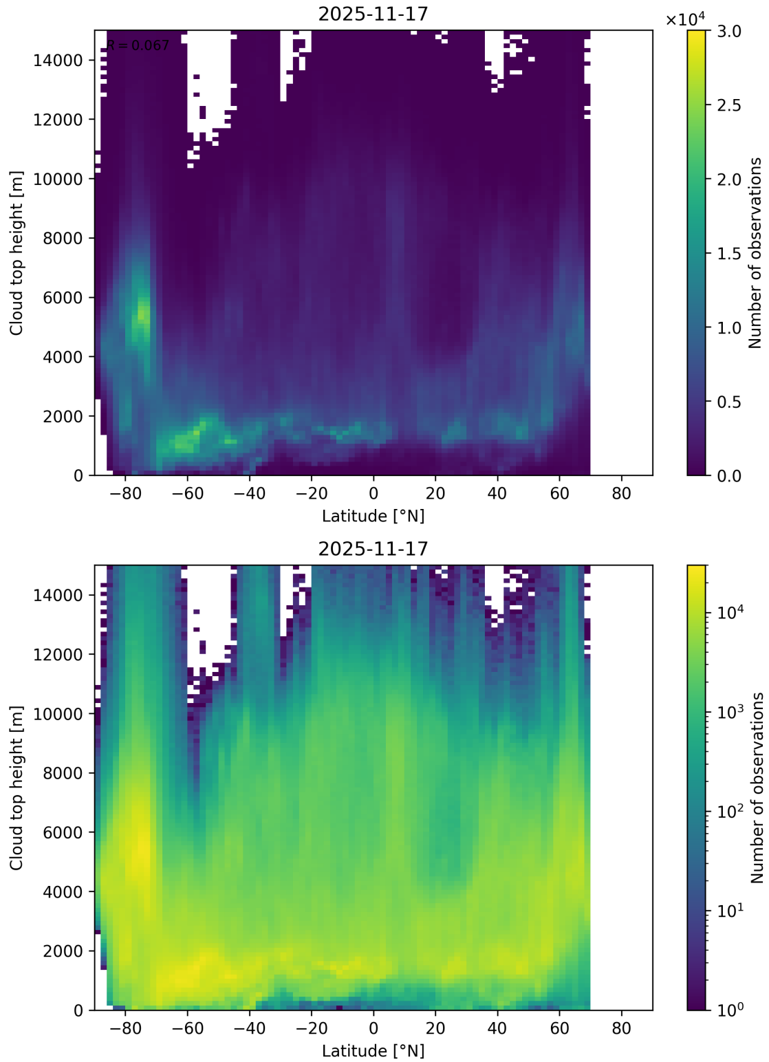
Figure 97: Scatter density plot of “Latitude” against “Cloud top height” for 2025-11-16 to 2025-11-18.
