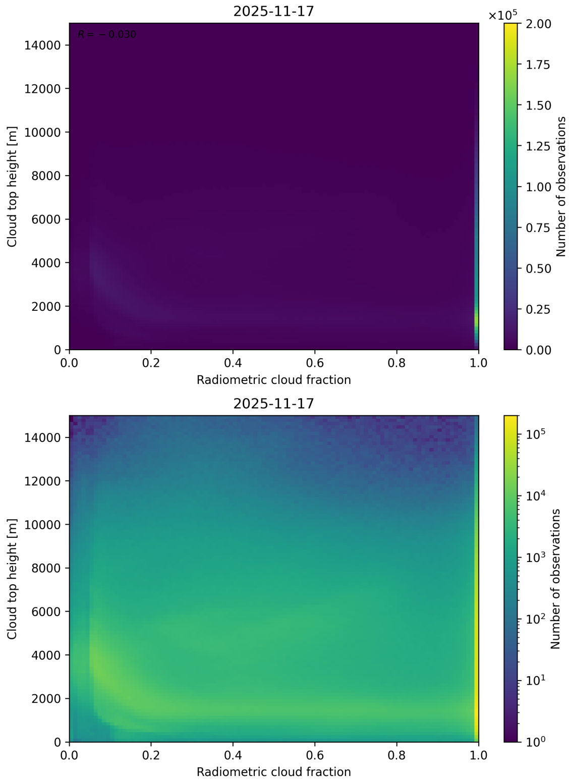
Figure 76: Scatter density plot of “Radiometric cloud fraction” against “Cloud top height” for 2025-11-16 to 2025-11-18.
