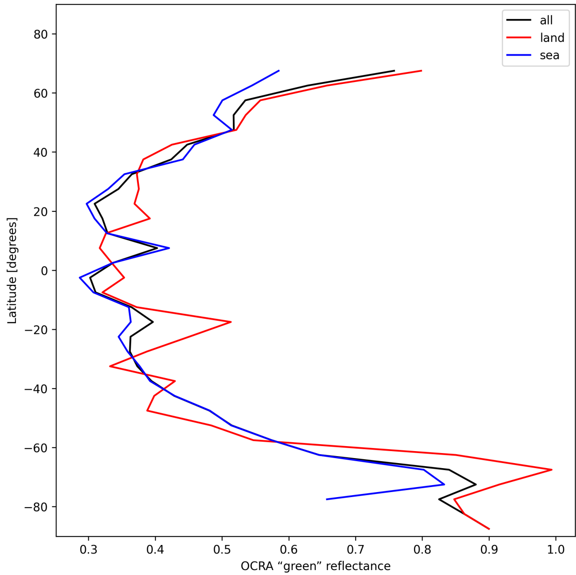
Figure 36: Zonal average of “OCRA “green” reflectance” for 2025-11-16 to 2025-11-18.
