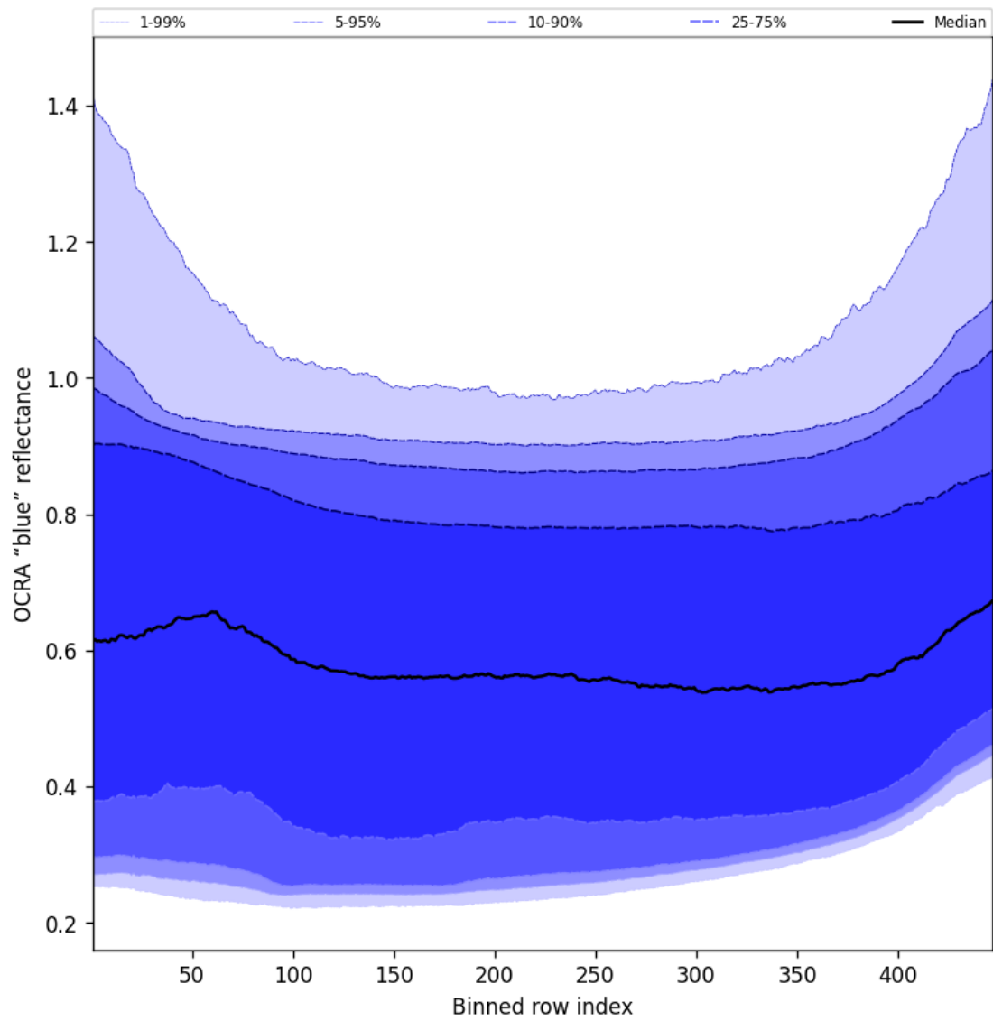
Figure 67: Along track statistics of “OCRA “blue” reflectance” for 2025-11-16 to 2025-11-18
