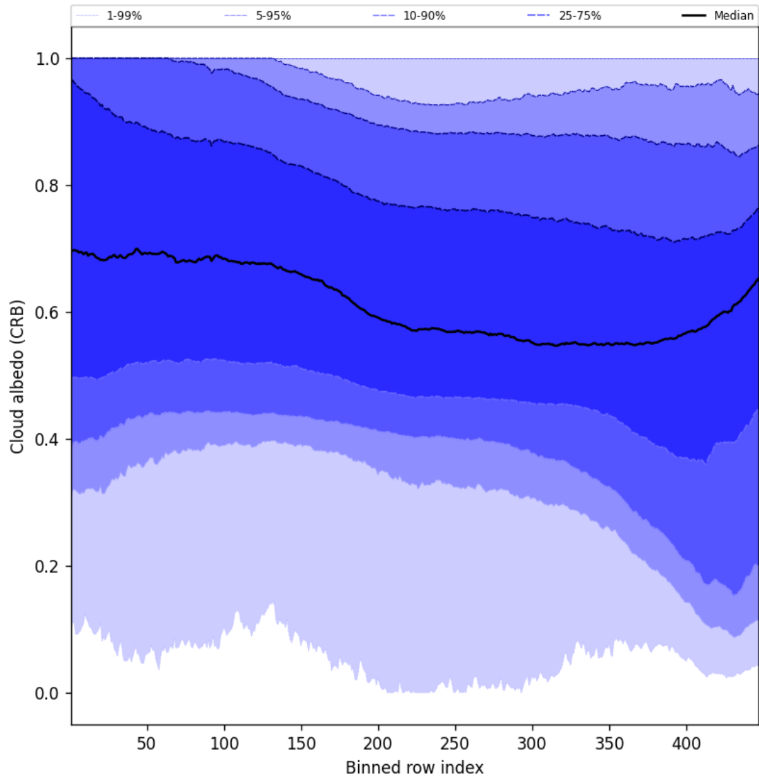
Figure 60: Along track statistics of “Cloud albedo (CRB)” for 2025-11-16 to 2025-11-18
