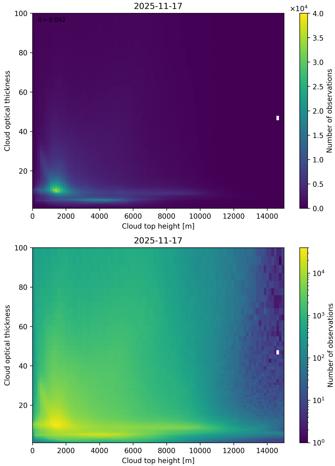
Figure 90: Scatter density plot of “Cloud top height” against “Cloud optical thickness” for 2025-11-16 to 2025-11-18.
