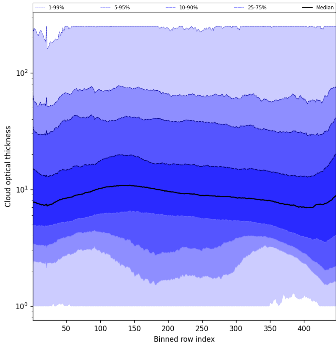
Figure 57: Along track statistics of “Cloud optical thickness” for 2025-11-16 to 2025-11-18
