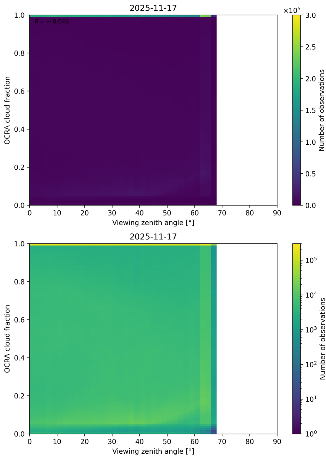
Figure 108: Scatter density plot of “Viewing zenith angle” against “OCRA cloud fraction” for 2025-11-16 to 2025-11-18.
