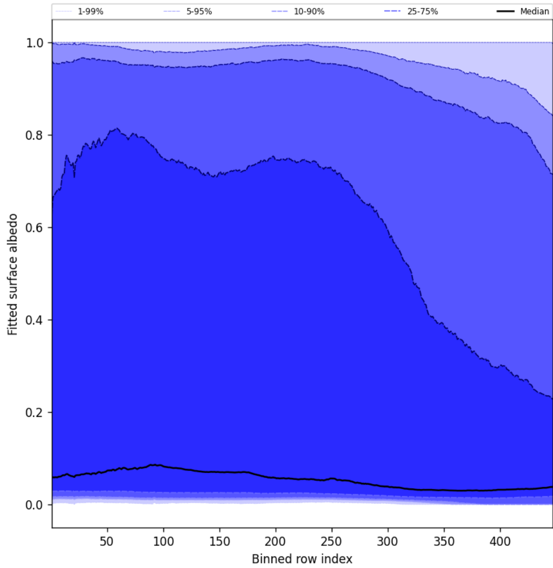
Figure 61: Along track statistics of “Fitted surface albedo” for 2025-11-16 to 2025-11-18
