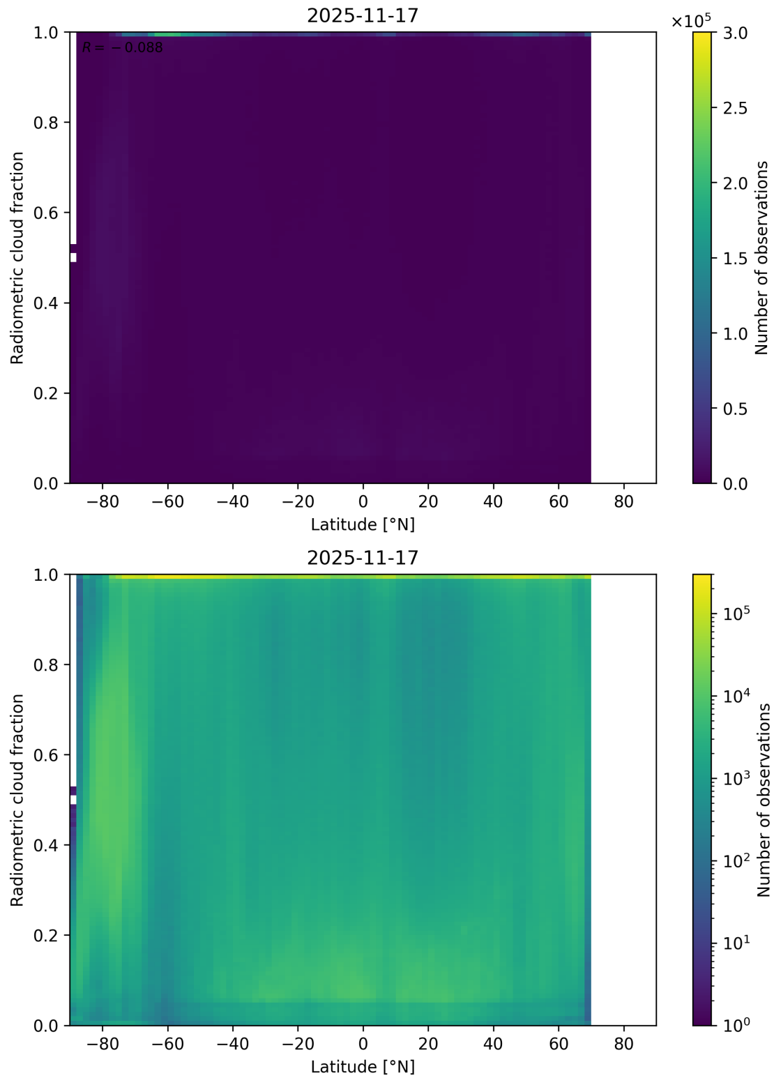
Figure 92: Scatter density plot of “Latitude” against “Radiometric cloud fraction” for 2025-11-16 to 2025-11-18.
