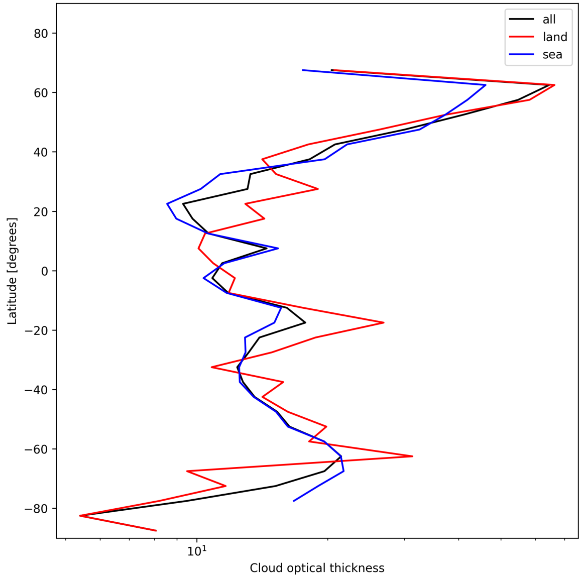
Figure 25: Zonal average of “Cloud optical thickness” for 2025-11-16 to 2025-11-18.
