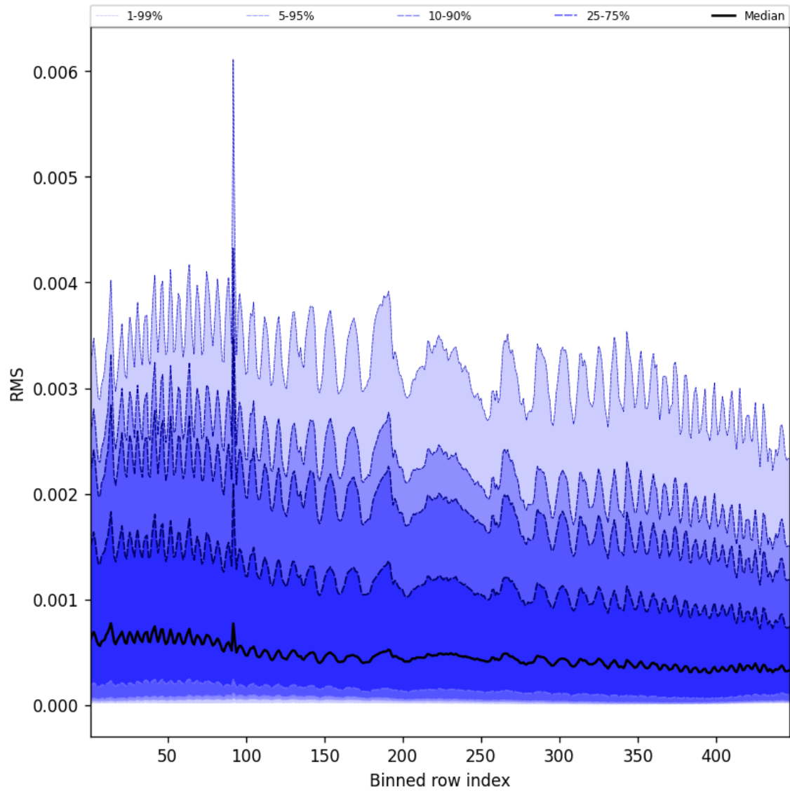
Figure 63: Along track statistics of “RMS” for 2025-11-16 to 2025-11-18
