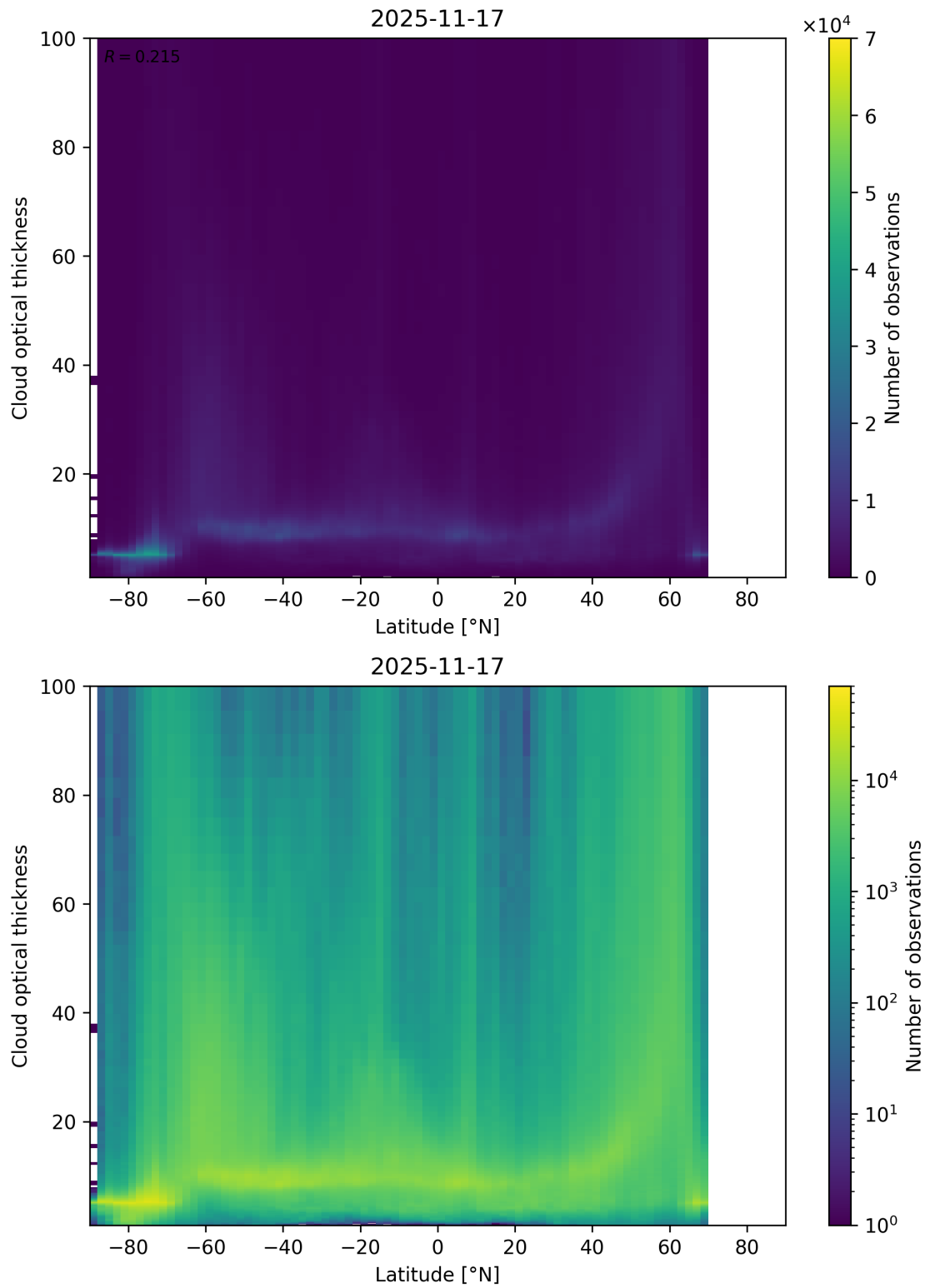
Figure 96: Scatter density plot of “Latitude” against “Cloud optical thickness” for 2025-11-16 to 2025-11-18.
