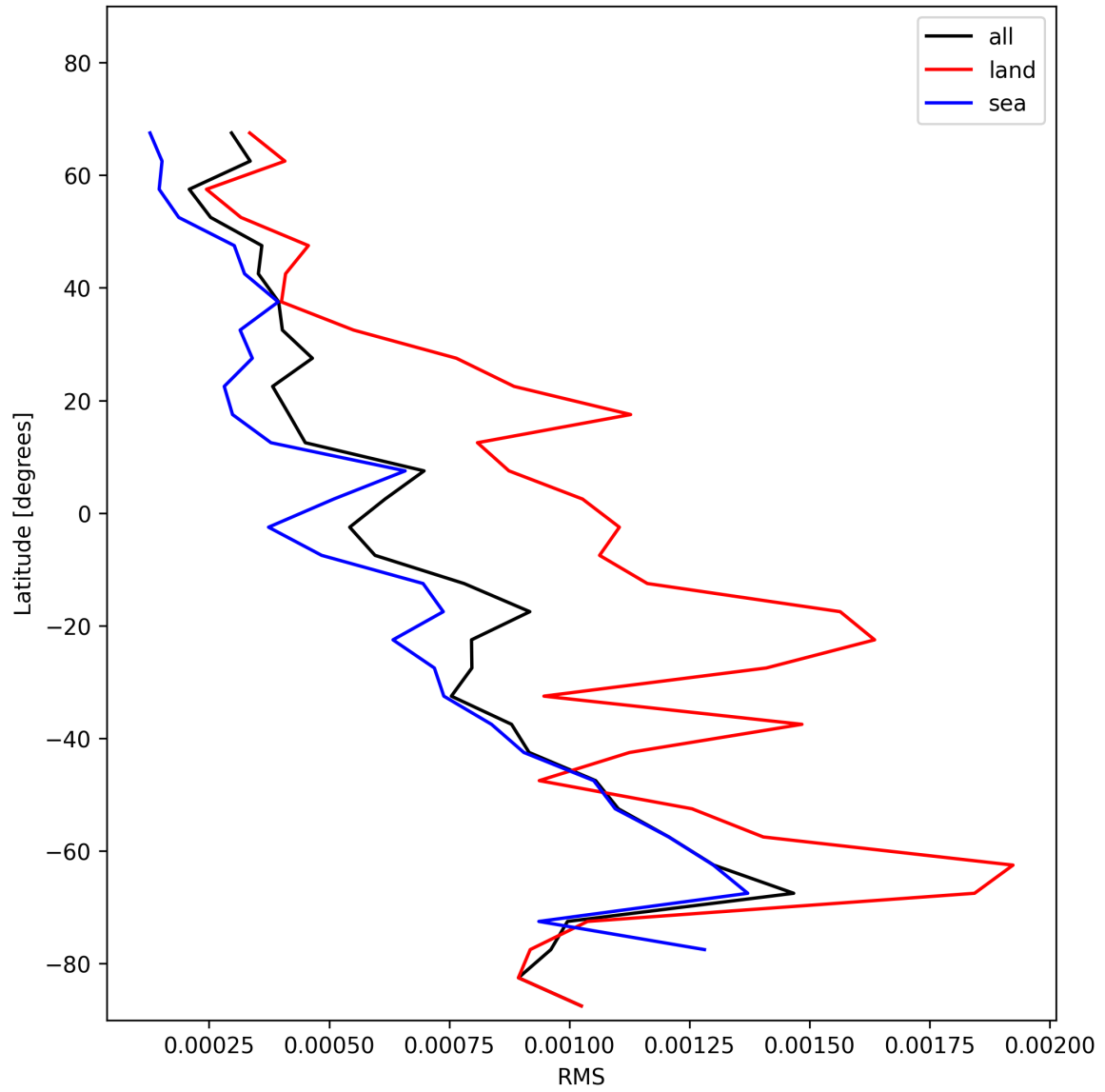
Figure 31: Zonal average of “RMS” for 2025-11-16 to 2025-11-18.
