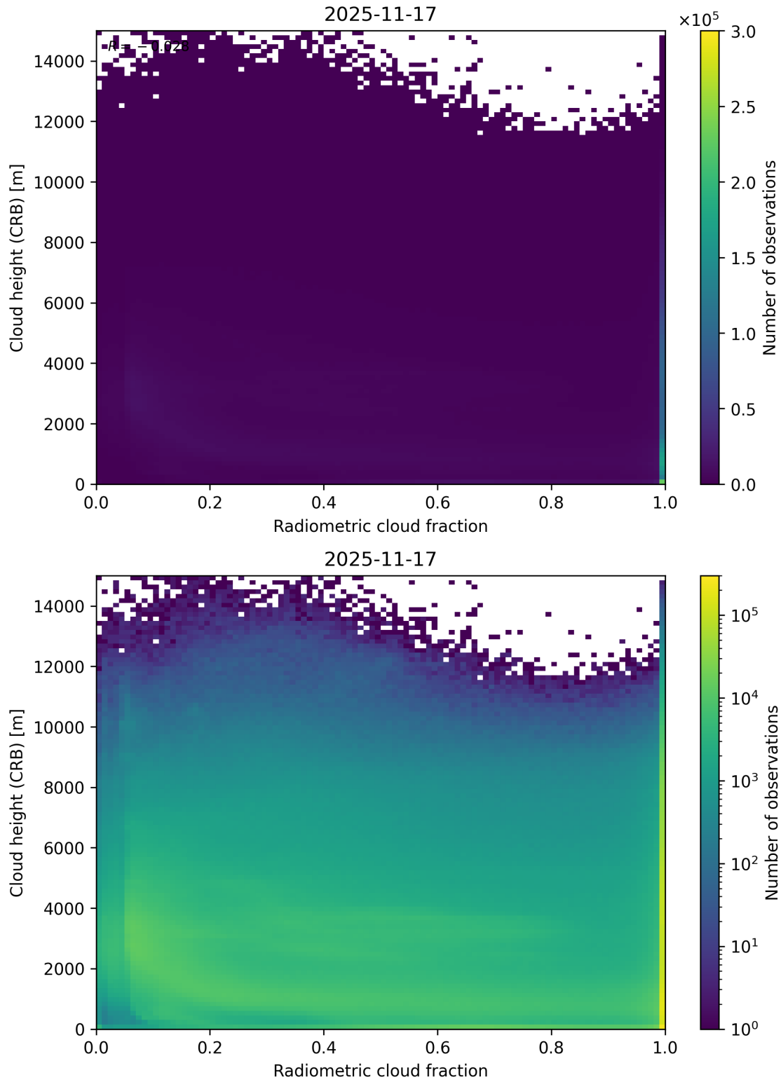
Figure 74: Scatter density plot of “Radiometric cloud fraction” against “Cloud height (CRB)” for 2025-11-16 to 2025-11-18.
