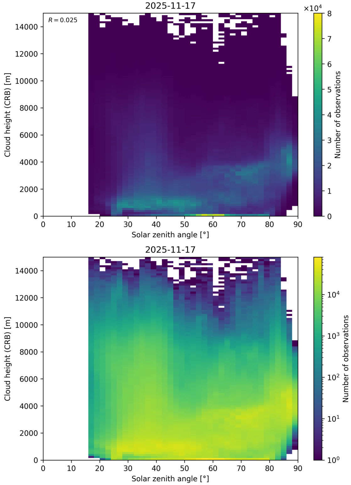
Figure 102: Scatter density plot of “Solar zenith angle” against “Cloud height (CRB)” for 2025-11-16 to 2025-11-18.
