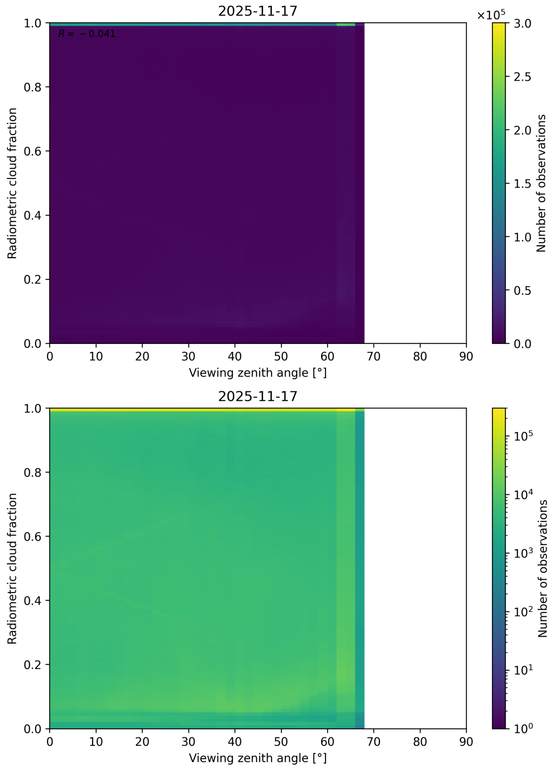
Figure 107: Scatter density plot of “Viewing zenith angle” against “Radiometric cloud fraction” for 2025-11-16 to 2025-11-18.
