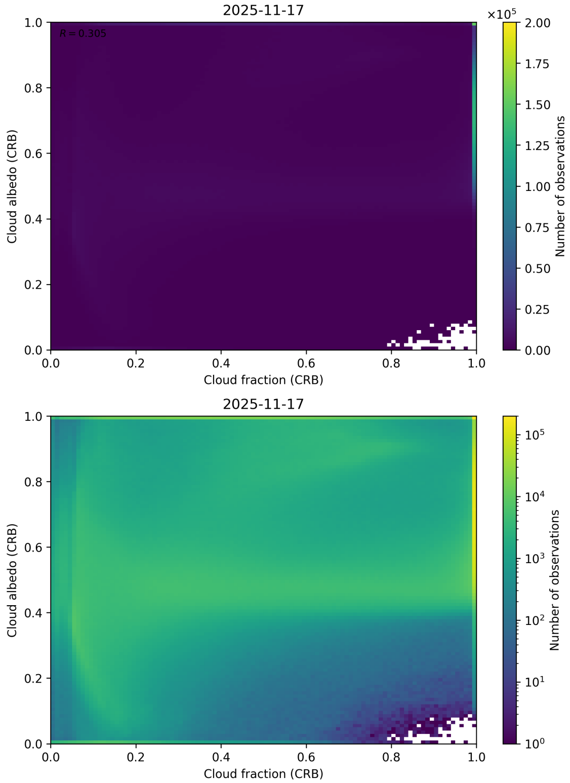
Figure 77: Scatter density plot of “Cloud fraction (CRB)” against “Cloud albedo (CRB)” for 2025-11-16 to 2025-11-18.
