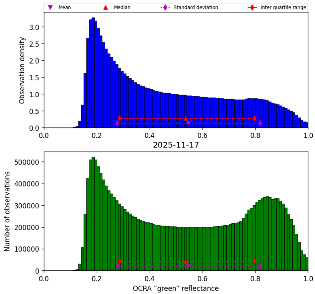
Figure 52: Histogram of “OCRA “green” reflectance” for 2025-11-16 to 2025-11-18
