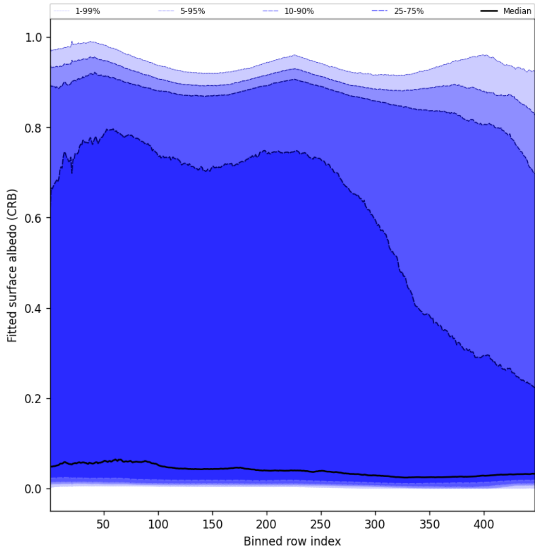
Figure 62: Along track statistics of “Fitted surface albedo (CRB)” for 2025-11-16 to 2025-11-18
