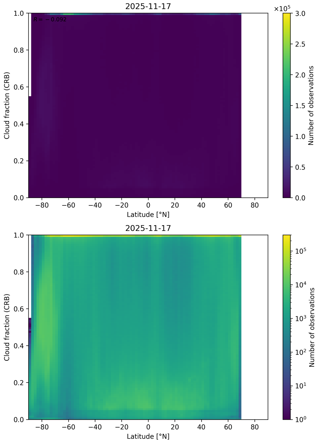
Figure 94: Scatter density plot of “Latitude” against “Cloud fraction (CRB)” for 2025-11-16 to 2025-11-18.
