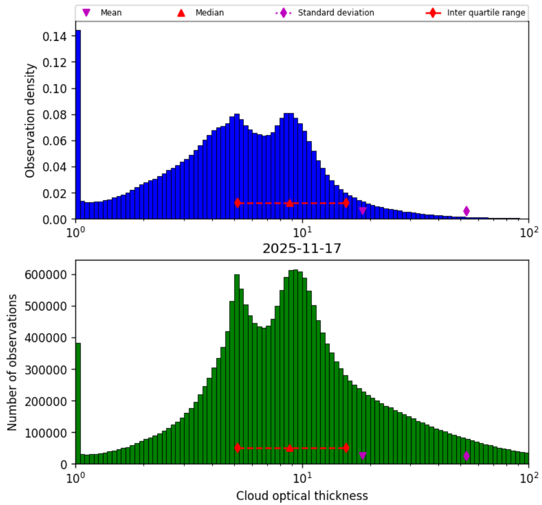
Figure 41: Histogram of “Cloud optical thickness” for 2025-11-16 to 2025-11-18
