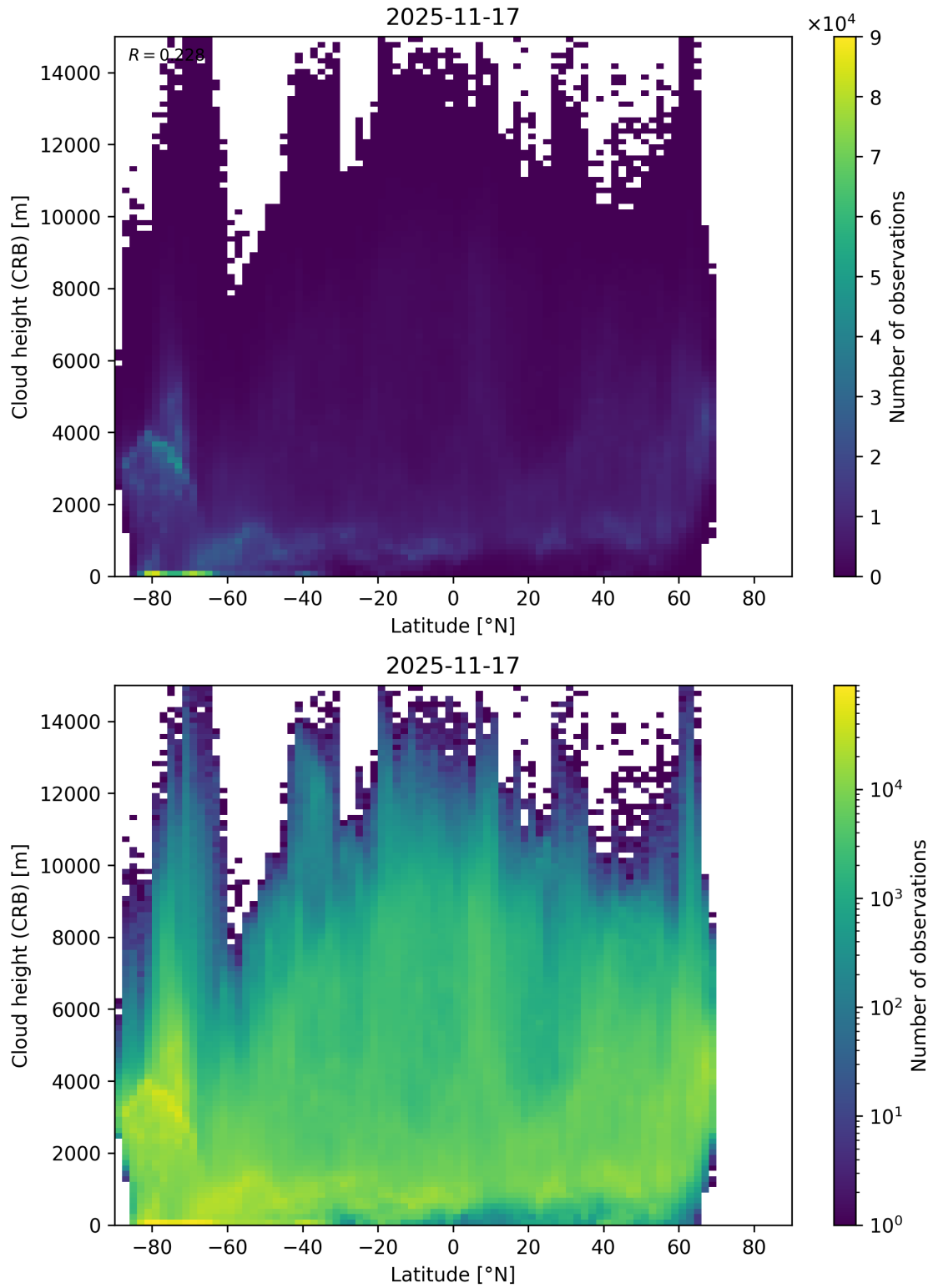
Figure 95: Scatter density plot of “Latitude” against “Cloud height (CRB)” for 2025-11-16 to 2025-11-18.
