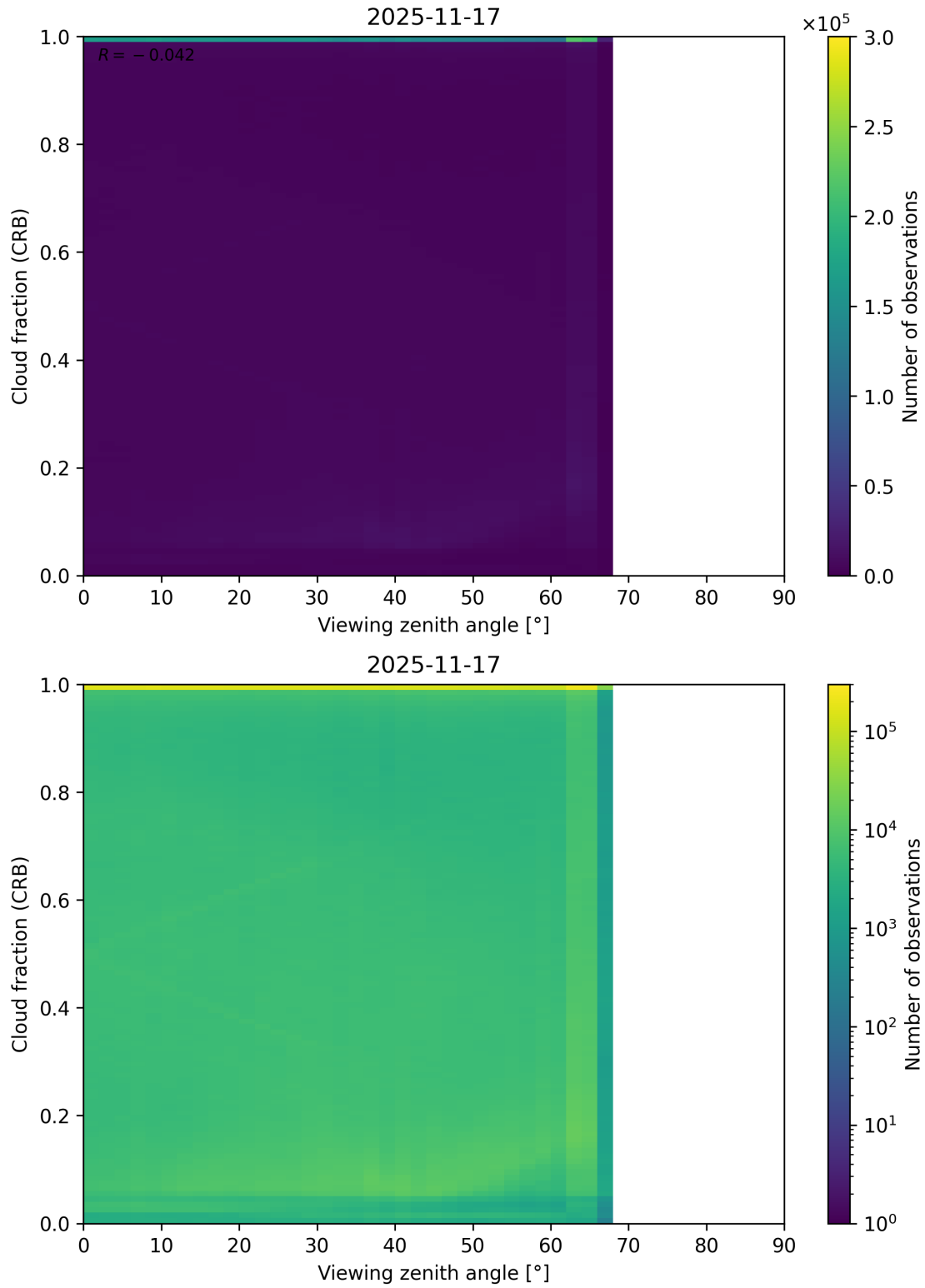
Figure 109: Scatter density plot of “Viewing zenith angle” against “Cloud fraction (CRB)” for 2025-11-16 to 2025-11-18.
