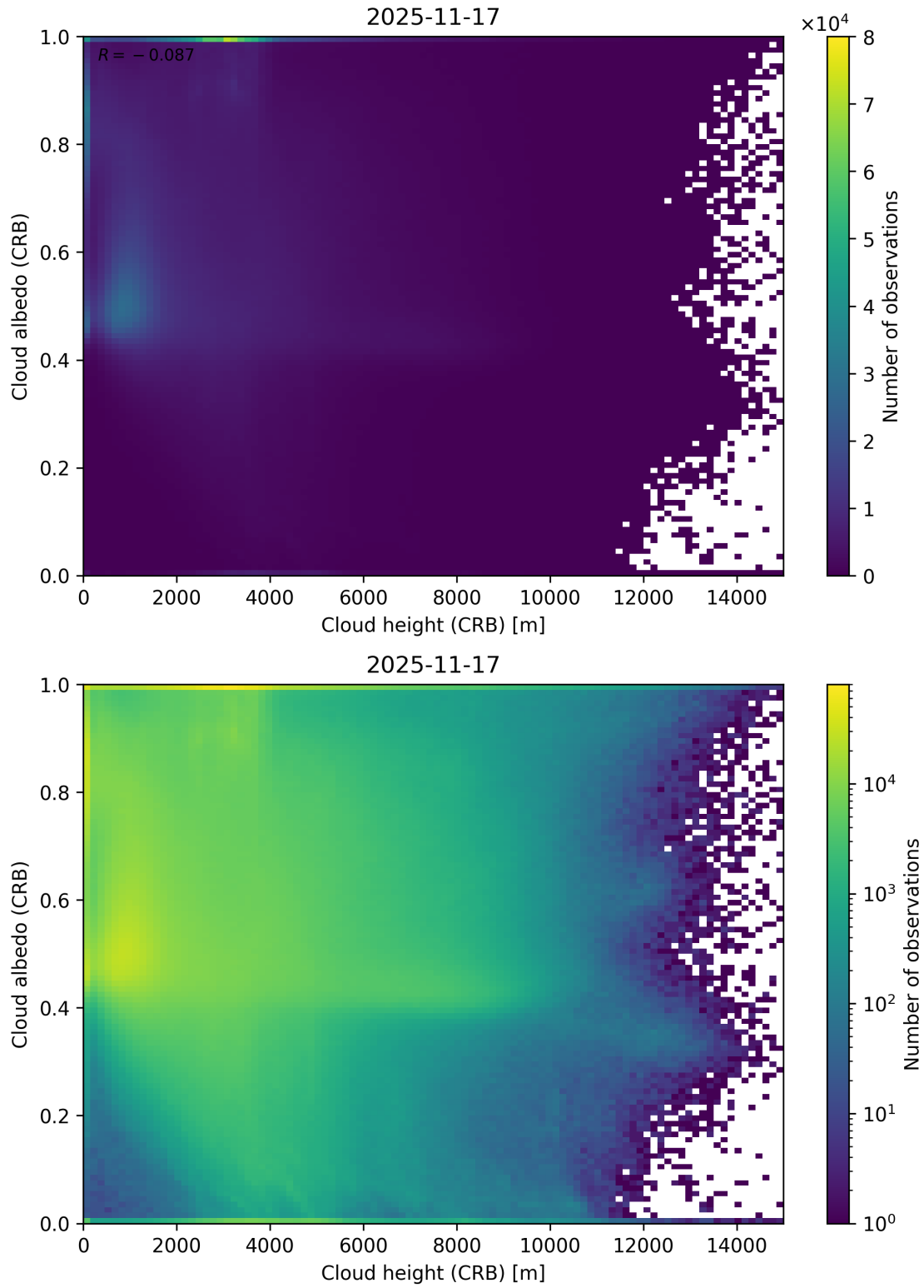
Figure 80: Scatter density plot of “Cloud height (CRB)” against “Cloud albedo (CRB)” for 2025-11-16 to 2025-11-18.
