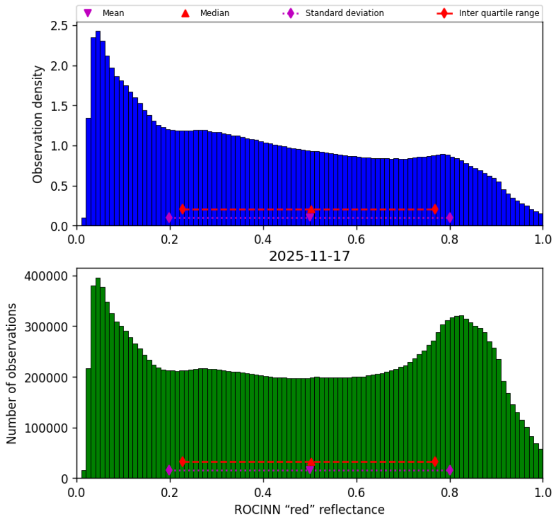
Figure 53: Histogram of “ROCINN “red” reflectance” for 2025-11-16 to 2025-11-18
