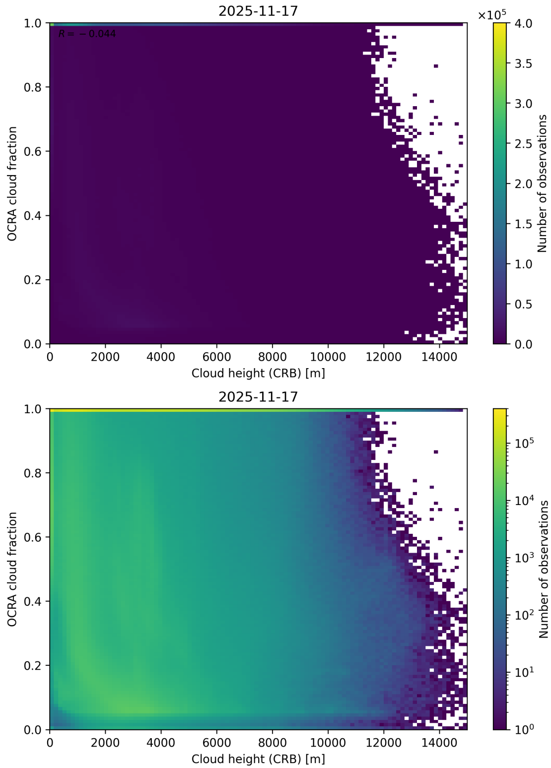
Figure 81: Scatter density plot of “Cloud height (CRB)” against “OCRA cloud fraction” for 2025-11-16 to 2025-11-18.
