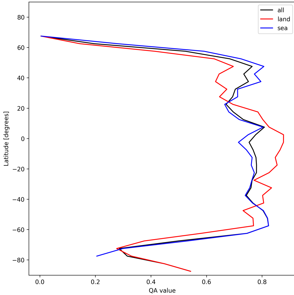
Figure 22: Zonal average of “QA value” for 2025-11-16 to 2025-11-18.
