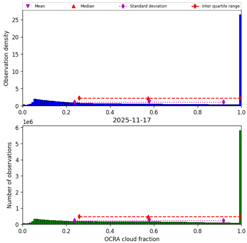
Figure 50: Histogram of “OCRA cloud fraction” for 2025-11-16 to 2025-11-18
