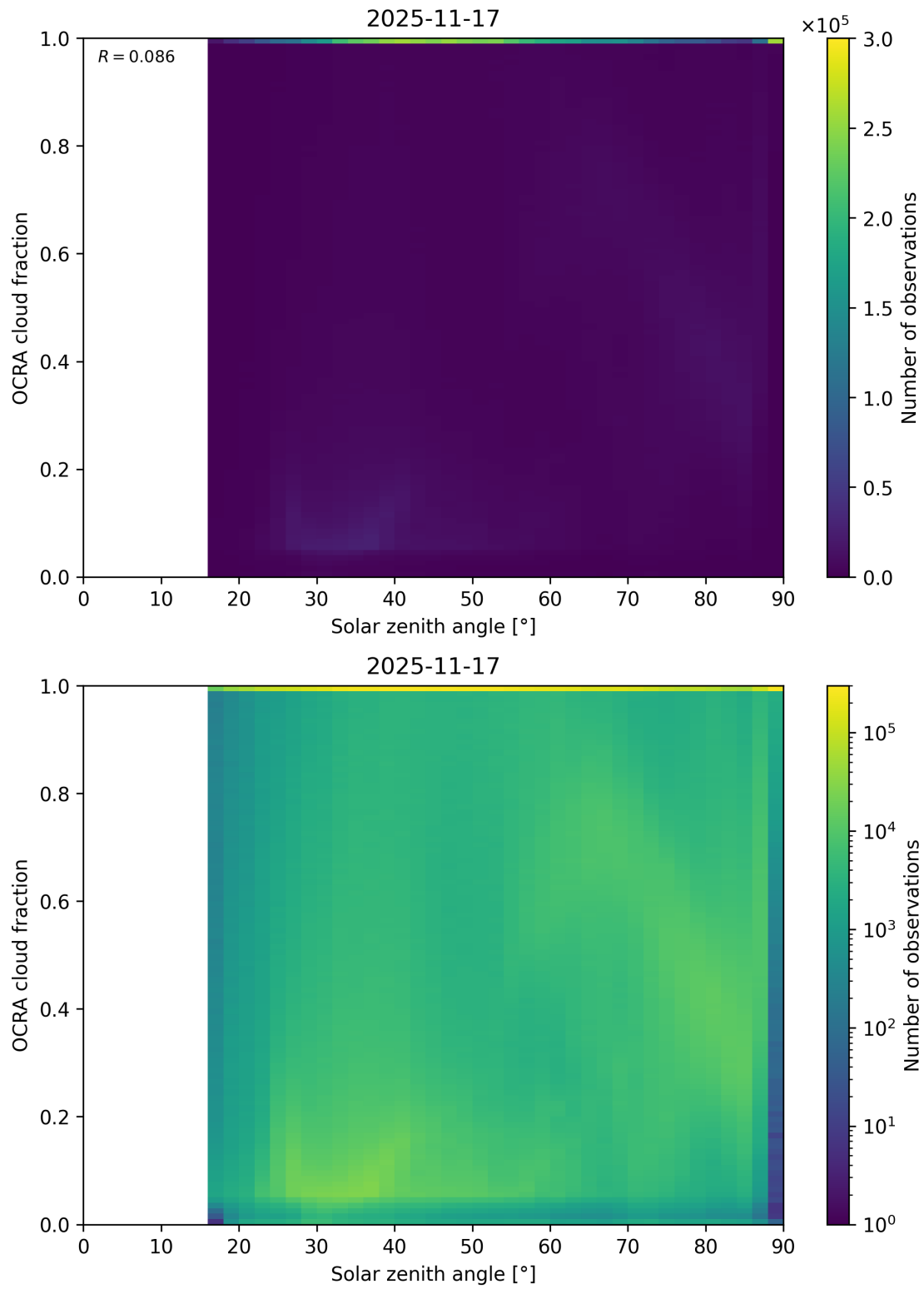
Figure 100: Scatter density plot of “Solar zenith angle” against “OCRA cloud fraction” for 2025-11-16 to 2025-11-18.
