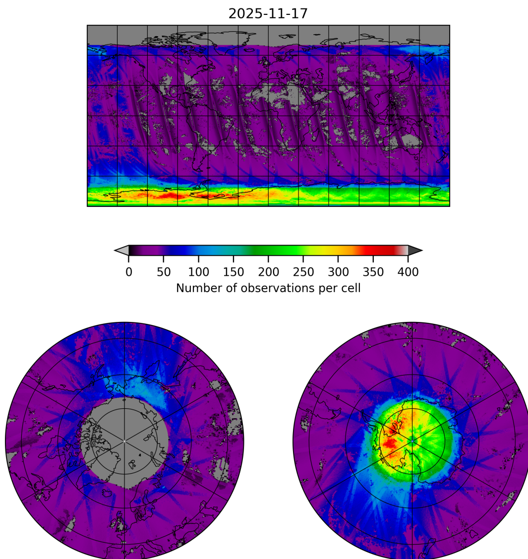
Figure 21: Map of the number of observations for 2025-11-16 to 2025-11-18
