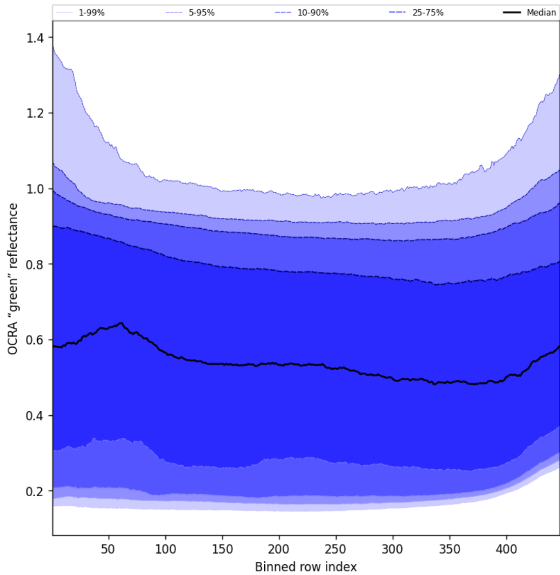
Figure 68: Along track statistics of “OCRA “green” reflectance” for 2025-11-16 to 2025-11-18
