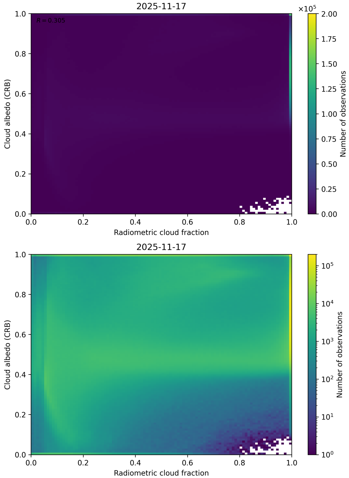
Figure 71: Scatter density plot of “Radiometric cloud fraction” against “Cloud albedo (CRB)” for 2025-11-16 to 2025-11-18.
