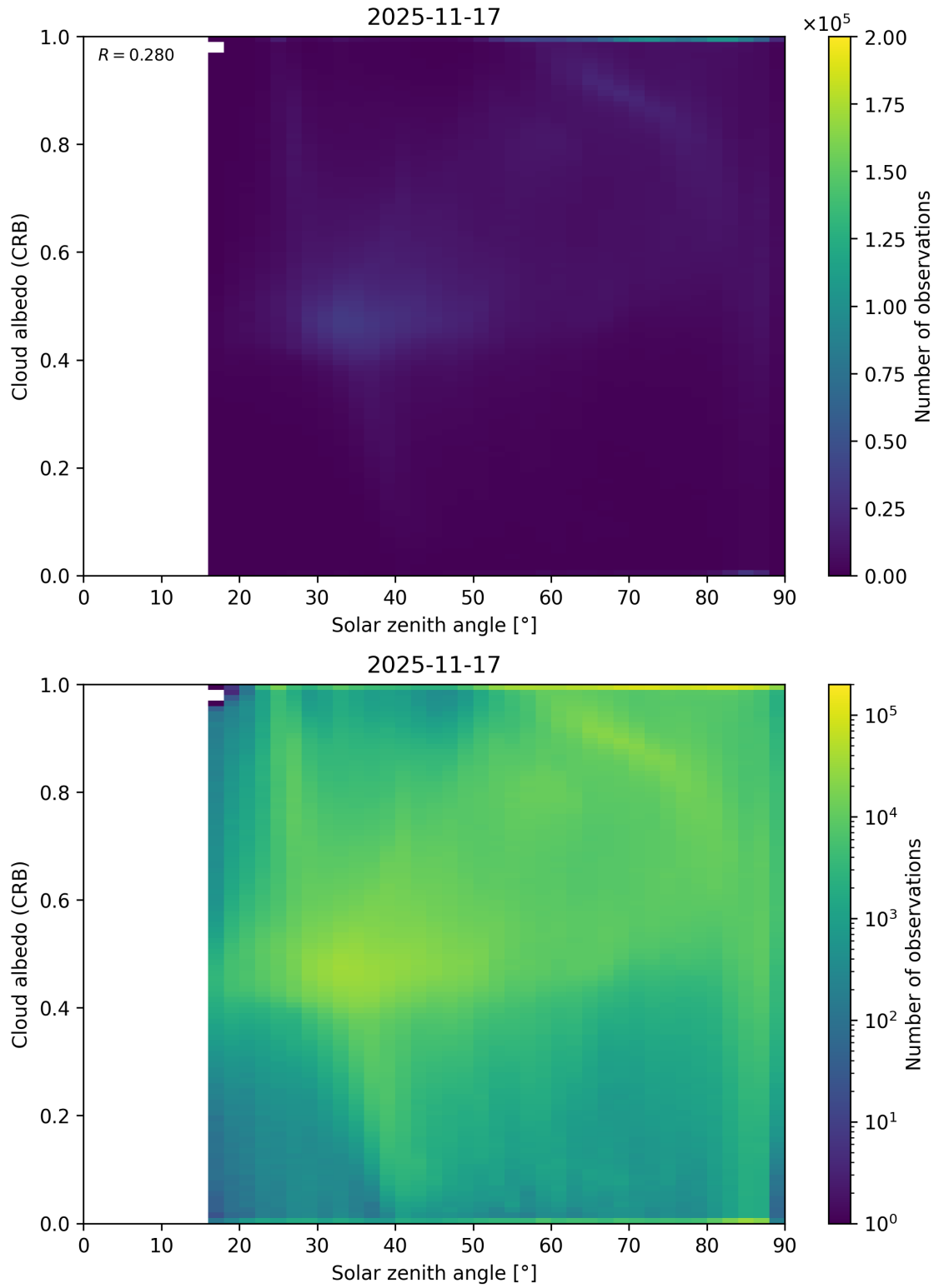
Figure 98: Scatter density plot of “Solar zenith angle” against “Cloud albedo (CRB)” for 2025-11-16 to 2025-11-18.
