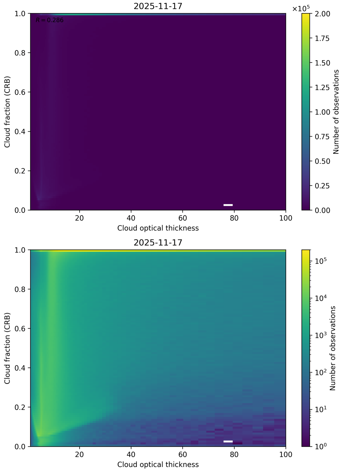
Figure 84: Scatter density plot of “Cloud optical thickness” against “Cloud fraction (CRB)” for 2025-11-16 to 2025-11-18.
