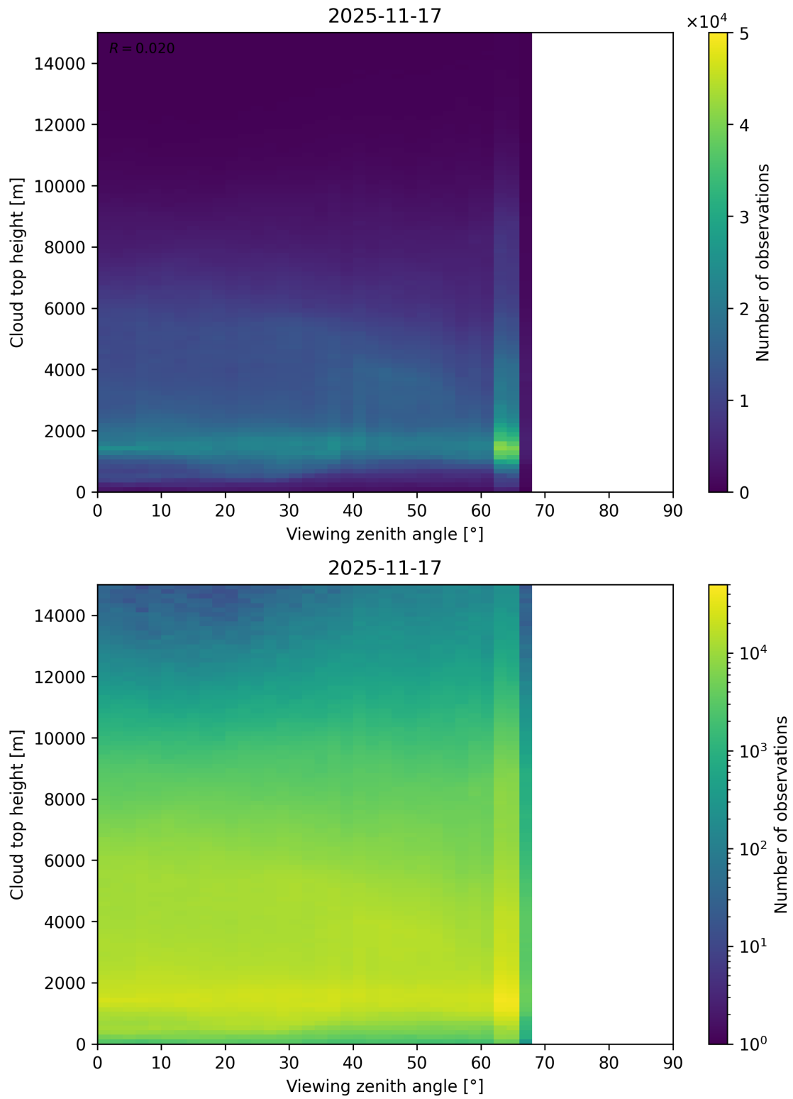
Figure 112: Scatter density plot of “Viewing zenith angle” against “Cloud top height” for 2025-11-16 to 2025-11-18.
