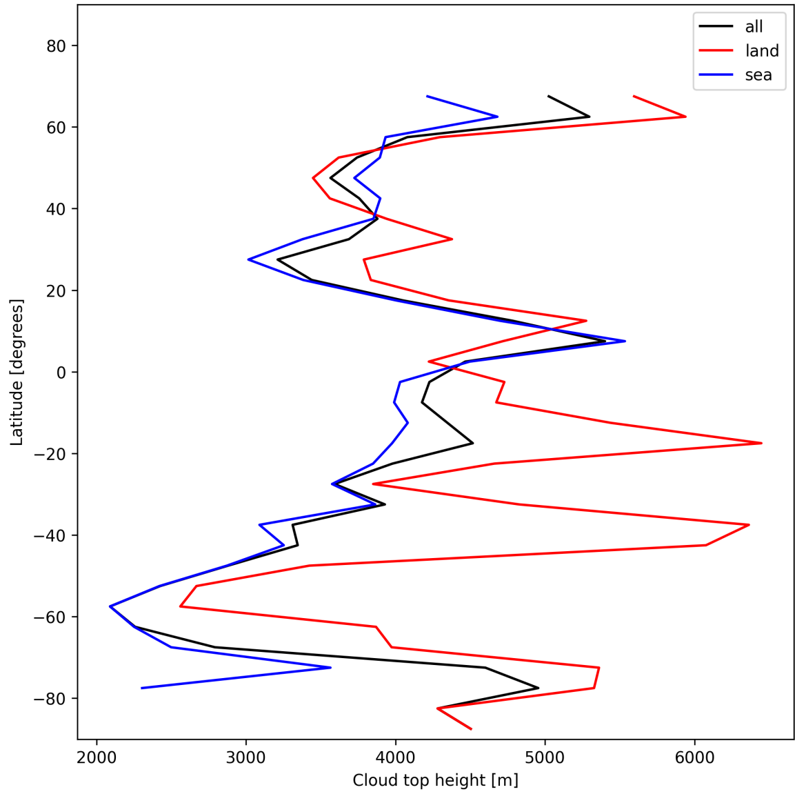
Figure 24: Zonal average of “Cloud top height” for 2025-11-16 to 2025-11-18.
