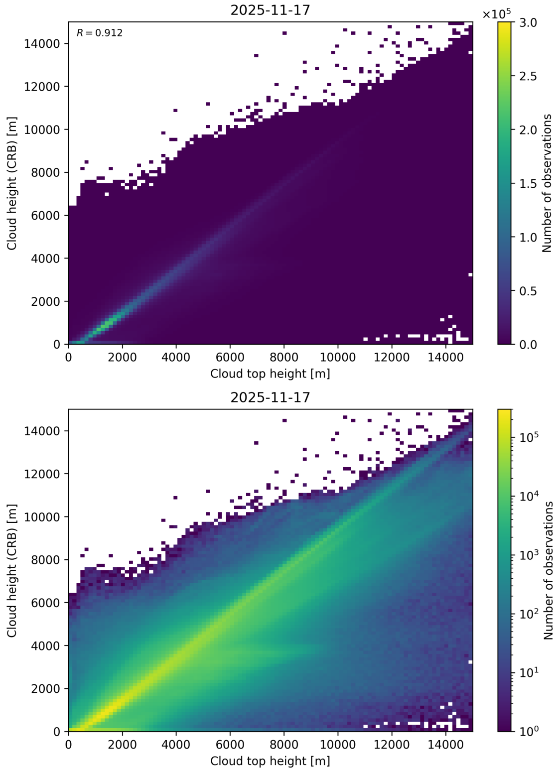
Figure 89: Scatter density plot of “Cloud top height” against “Cloud height (CRB)” for 2025-11-16 to 2025-11-18.
