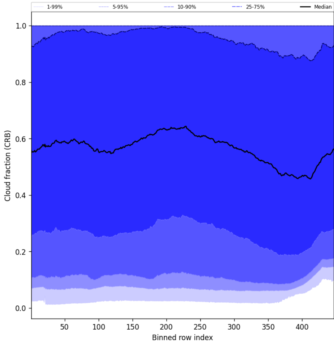
Figure 58: Along track statistics of “Cloud fraction (CRB)” for 2025-11-16 to 2025-11-18
