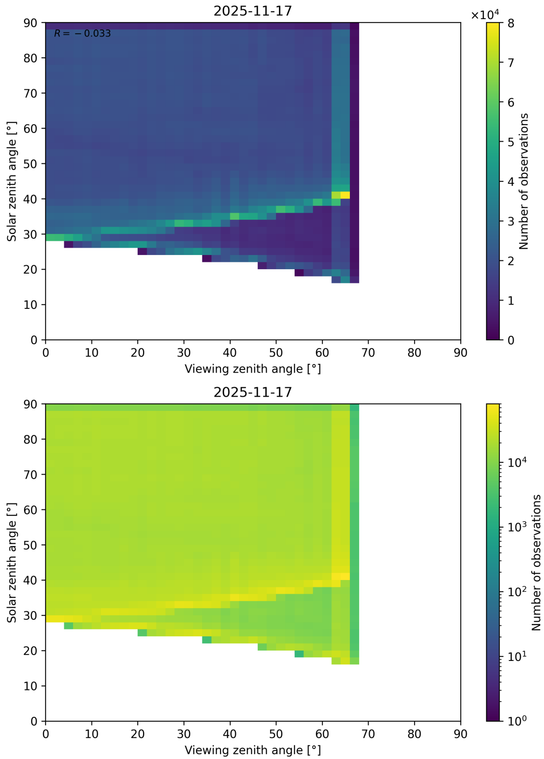
Figure 114: Scatter density plot of “Viewing zenith angle” against “Solar zenith angle” for 2025-11-16 to 2025-11-18.
