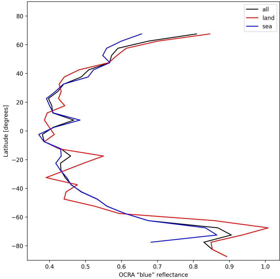
Figure 35: Zonal average of “OCRA “blue” reflectance” for 2025-11-16 to 2025-11-18.
