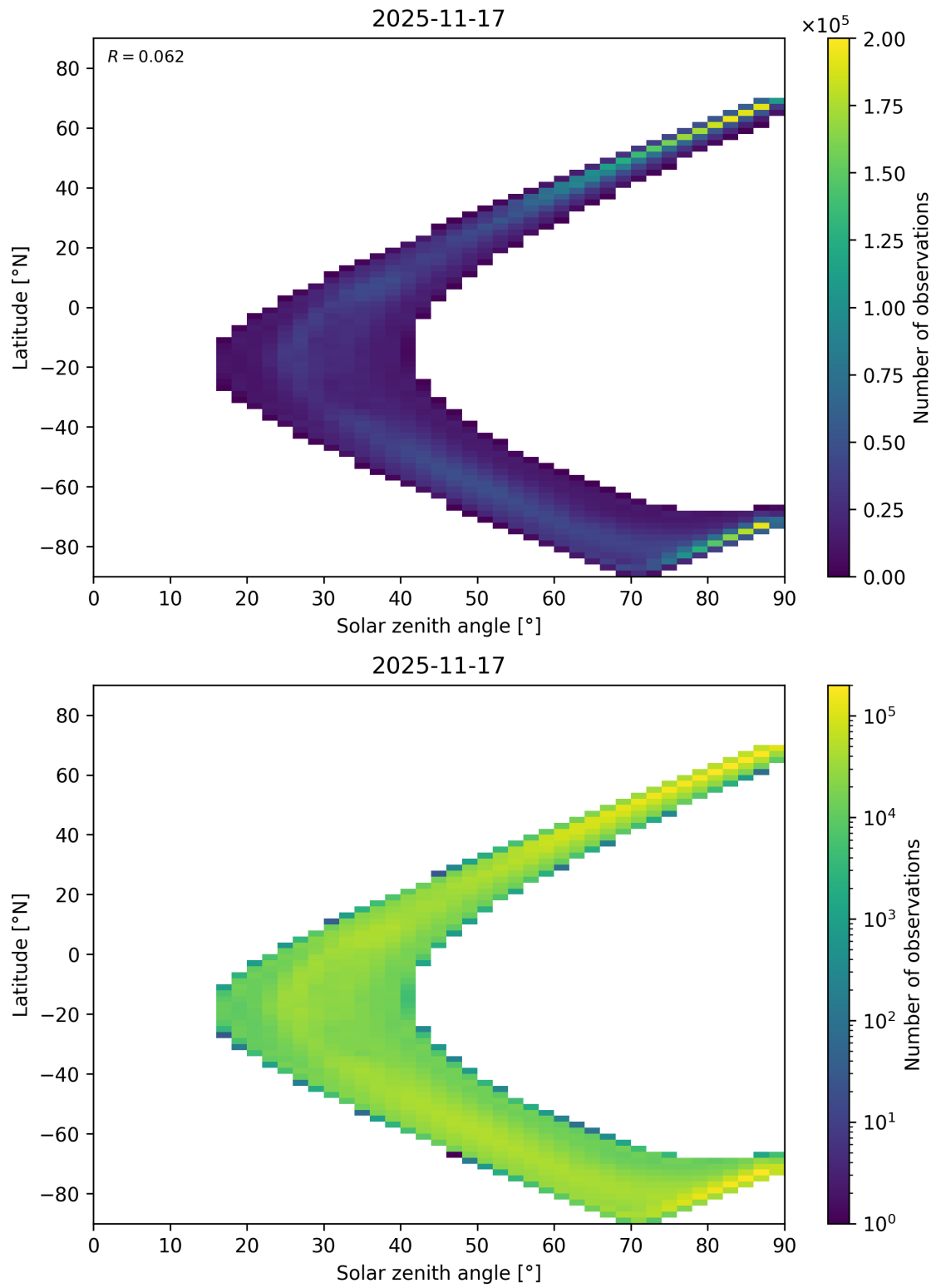
Figure 105: Scatter density plot of “Solar zenith angle” against “Latitude” for 2025-11-16 to 2025-11-18.
