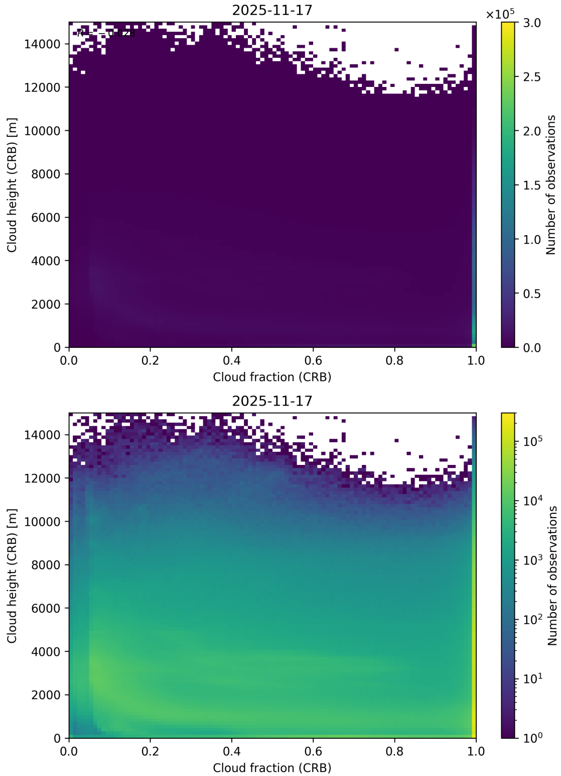
Figure 79: Scatter density plot of “Cloud fraction (CRB)” against “Cloud height (CRB)” for 2025-11-16 to 2025-11-18.
