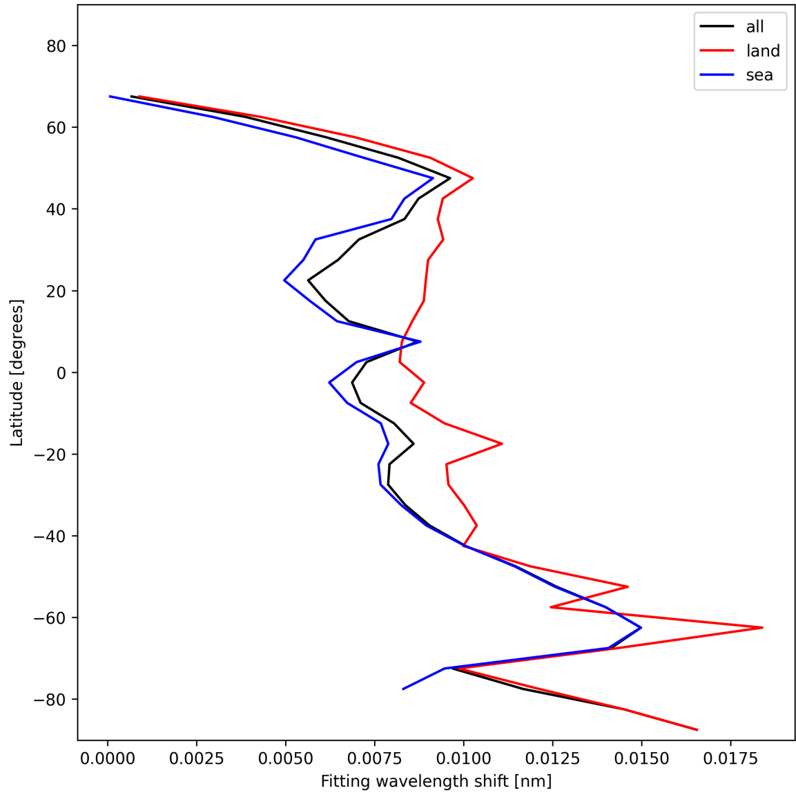
Figure 33: Zonal average of “Fitting wavelength shift” for 2025-11-16 to 2025-11-18.
