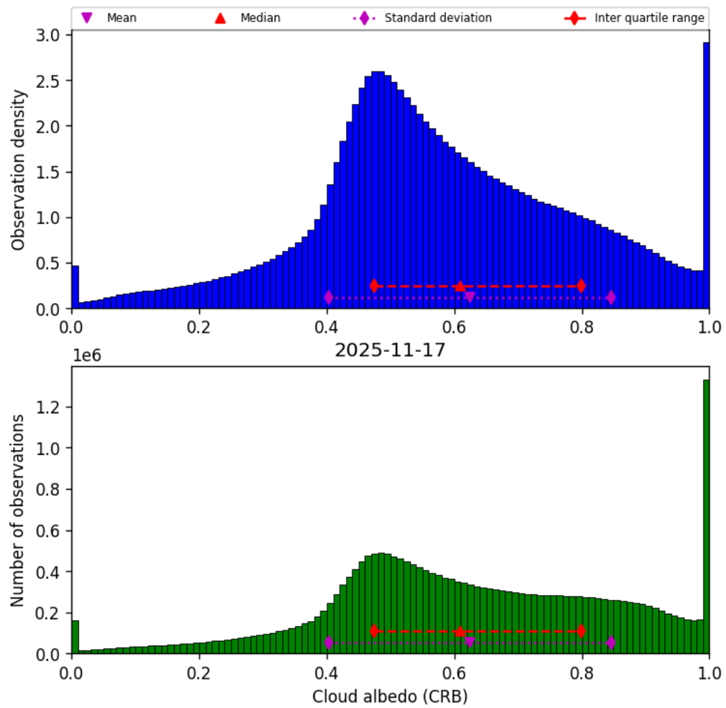
Figure 44: Histogram of “Cloud albedo (CRB)” for 2025-11-16 to 2025-11-18
