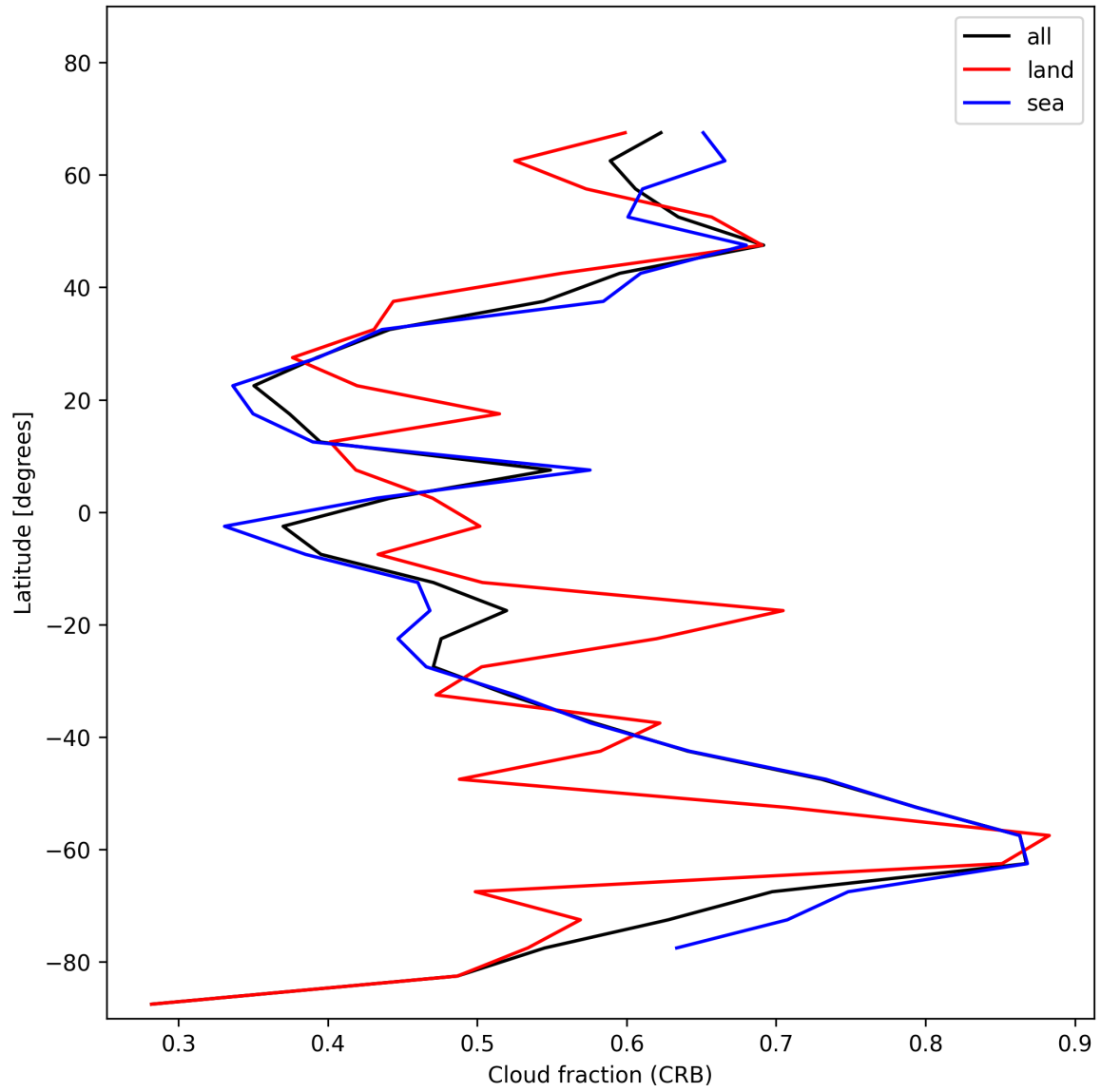
Figure 26: Zonal average of “Cloud fraction (CRB)” for 2025-11-16 to 2025-11-18.
