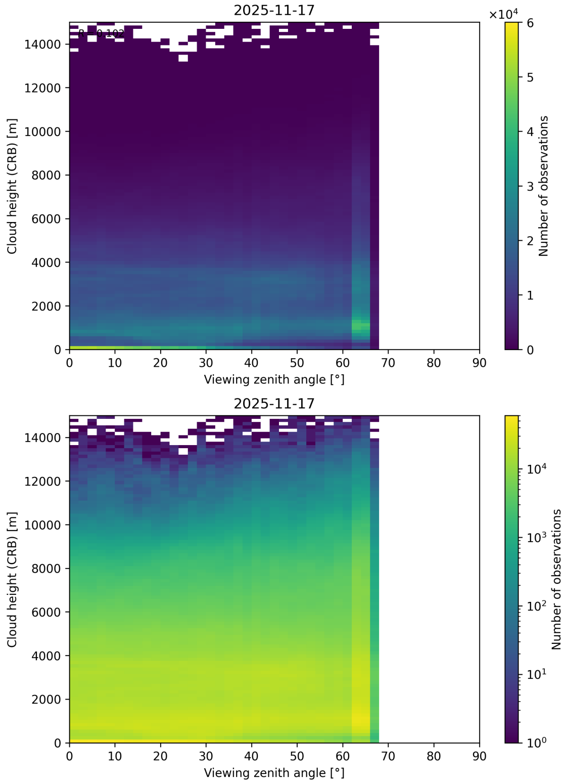
Figure 110: Scatter density plot of “Viewing zenith angle” against “Cloud height (CRB)” for 2025-11-16 to 2025-11-18.
