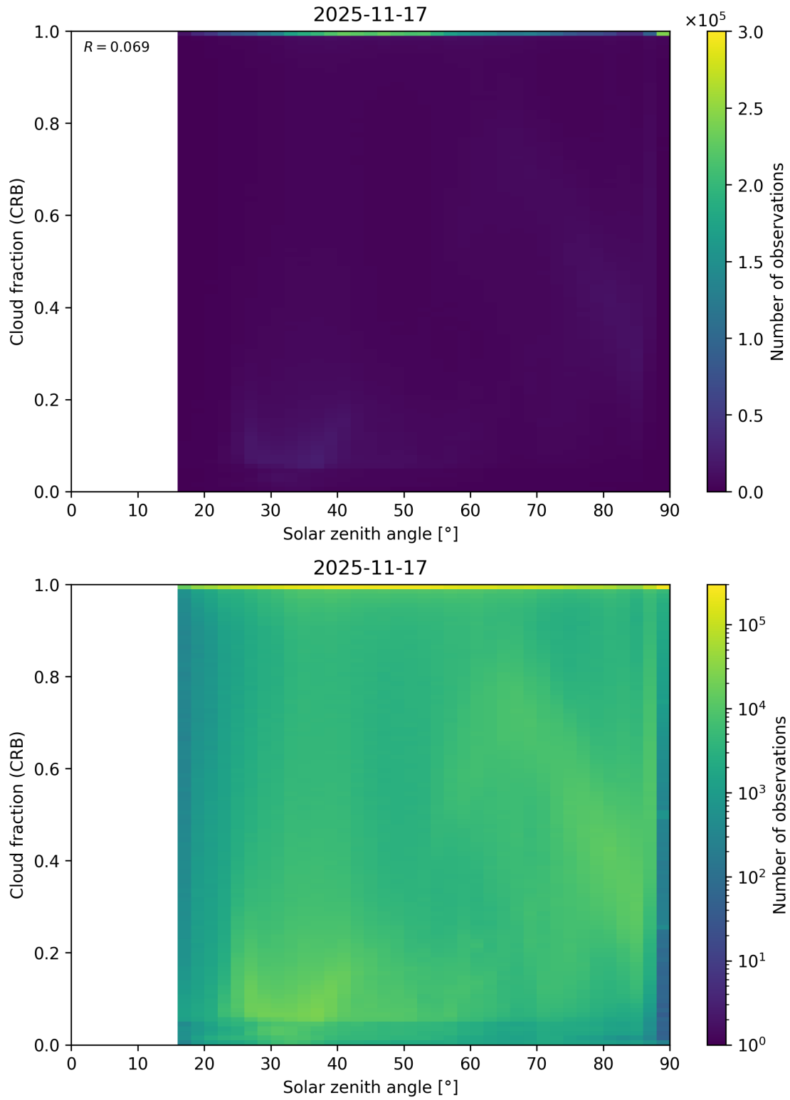
Figure 101: Scatter density plot of “Solar zenith angle” against “Cloud fraction (CRB)” for 2025-11-16 to 2025-11-18.
