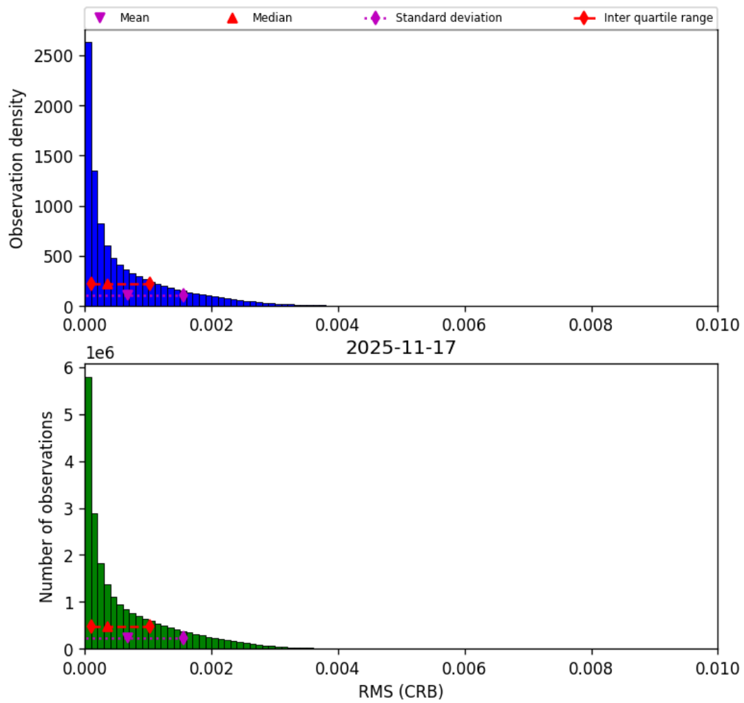
Figure 48: Histogram of “RMS (CRB)” for 2025-11-16 to 2025-11-18
