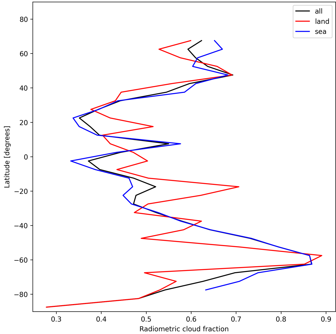
Figure 23: Zonal average of “Radiometric cloud fraction” for 2025-11-16 to 2025-11-18.
