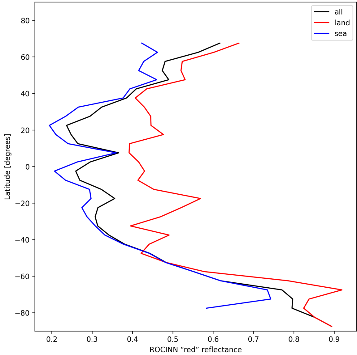
Figure 37: Zonal average of “ROCINN “red” reflectance” for 2025-11-16 to 2025-11-18.
