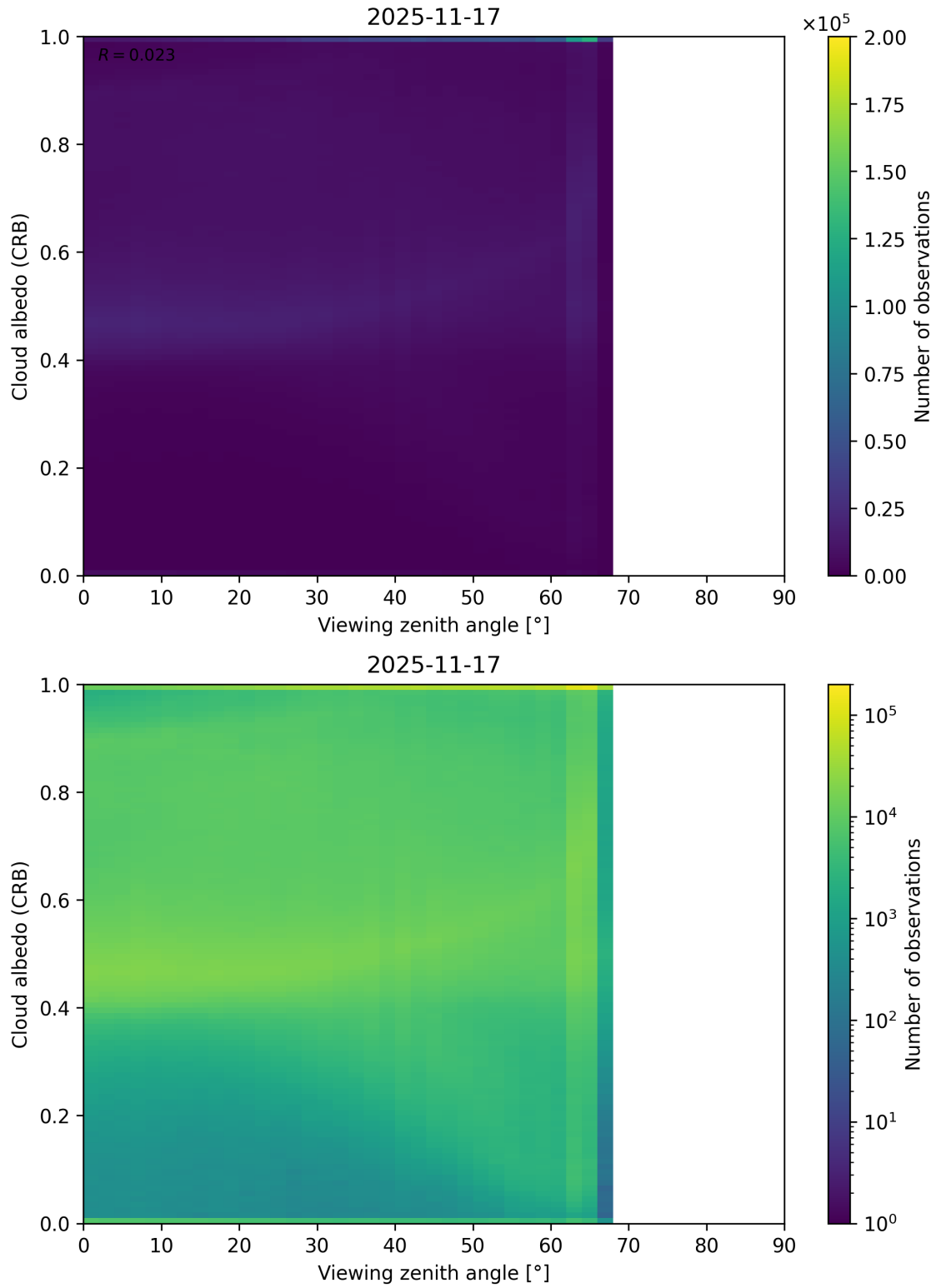
Figure 106: Scatter density plot of “Viewing zenith angle” against “Cloud albedo (CRB)” for 2025-11-16 to 2025-11-18.
