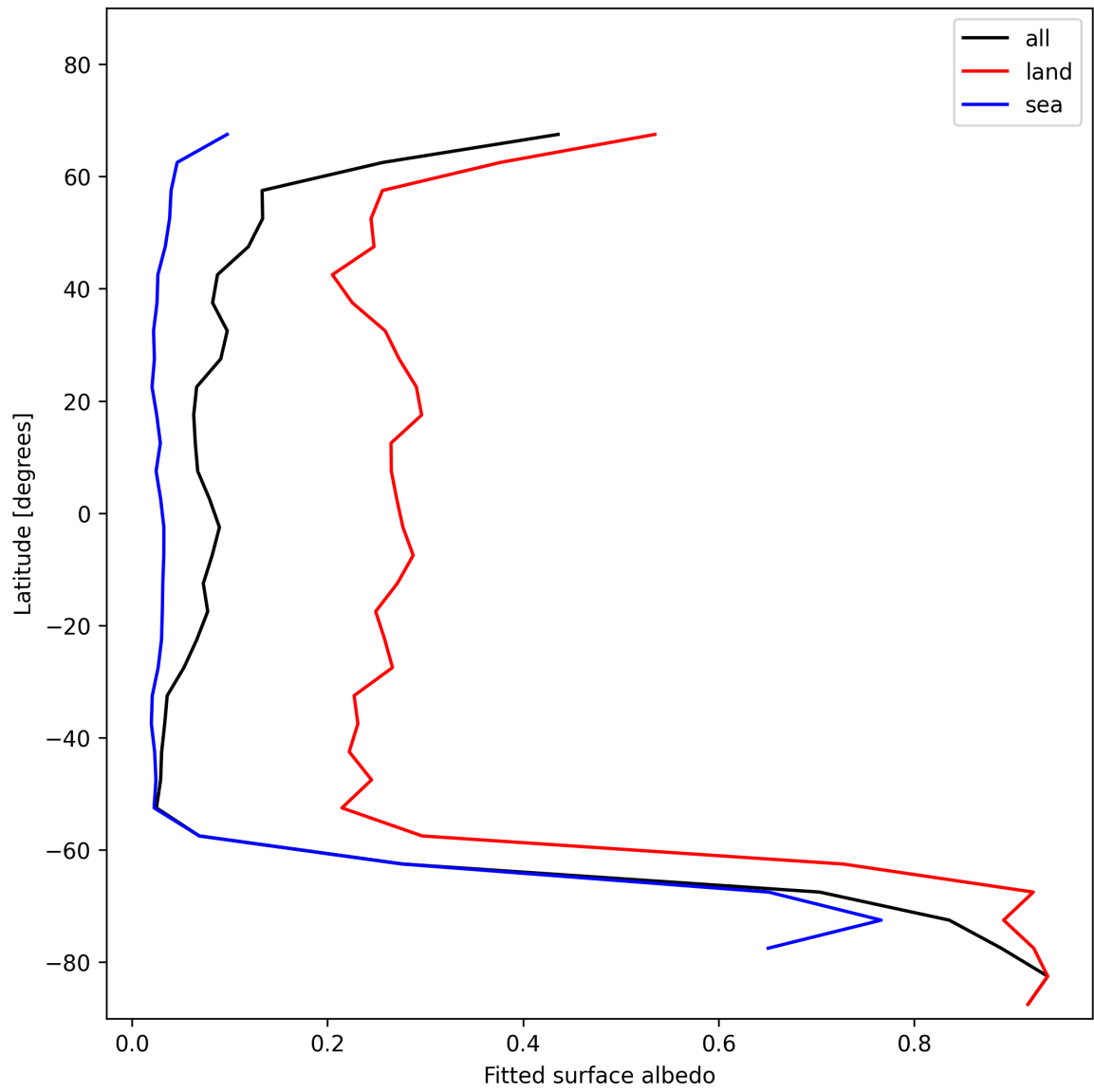
Figure 29: Zonal average of “Fitted surface albedo” for 2025-11-16 to 2025-11-18.
