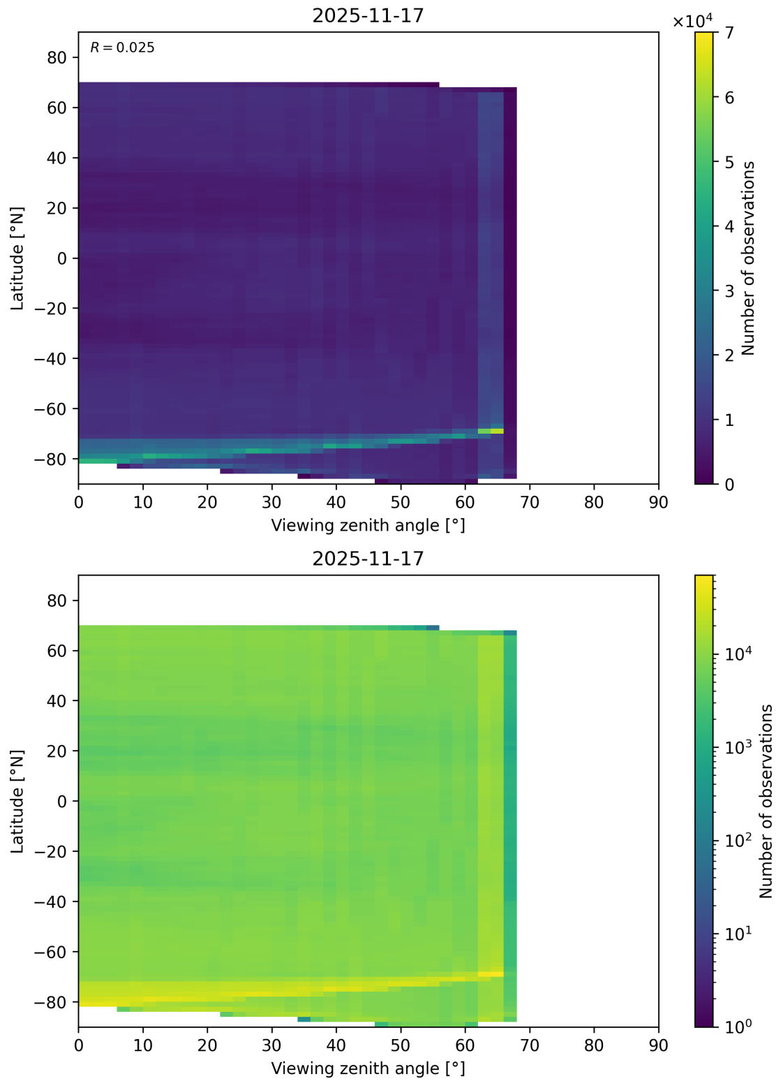
Figure 113: Scatter density plot of “Viewing zenith angle” against “Latitude” for 2025-11-16 to 2025-11-18.
