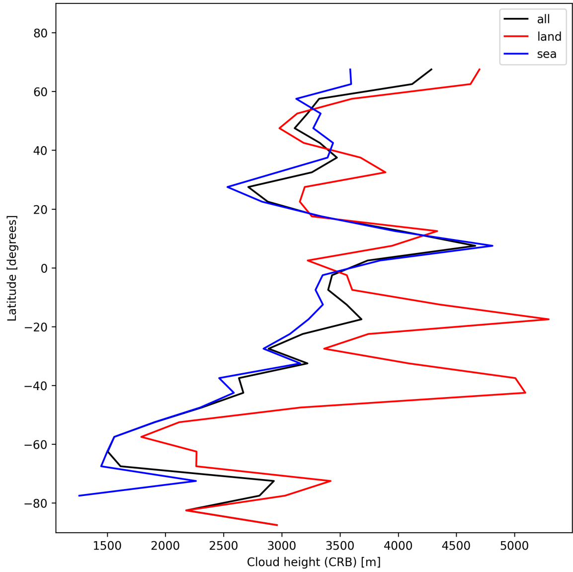
Figure 27: Zonal average of “Cloud height (CRB)” for 2025-11-16 to 2025-11-18.
