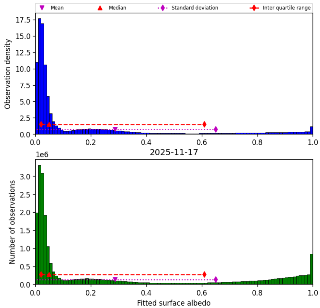
Figure 45: Histogram of “Fitted surface albedo” for 2025-11-16 to 2025-11-18
