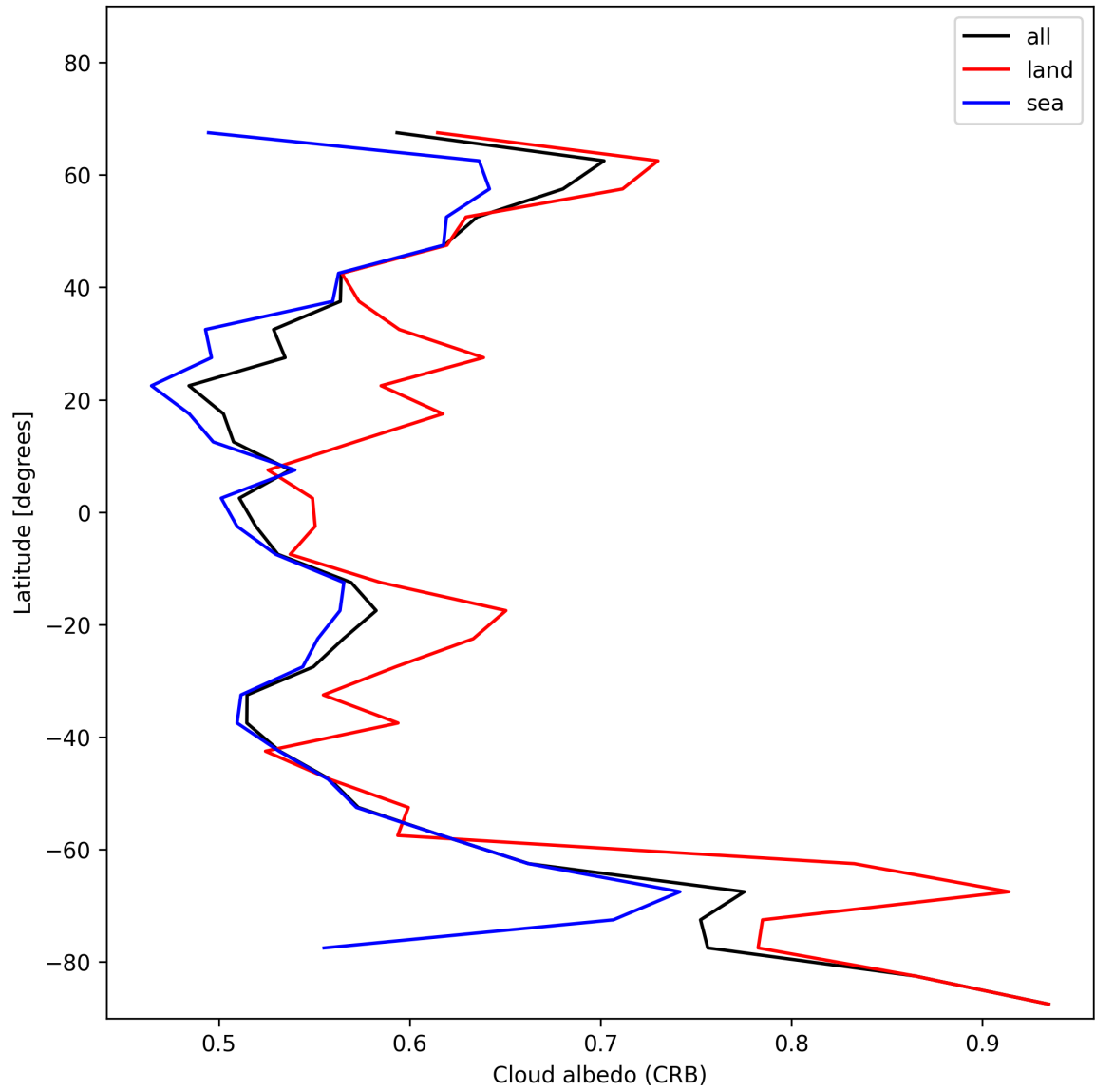
Figure 28: Zonal average of “Cloud albedo (CRB)” for 2025-11-16 to 2025-11-18.
