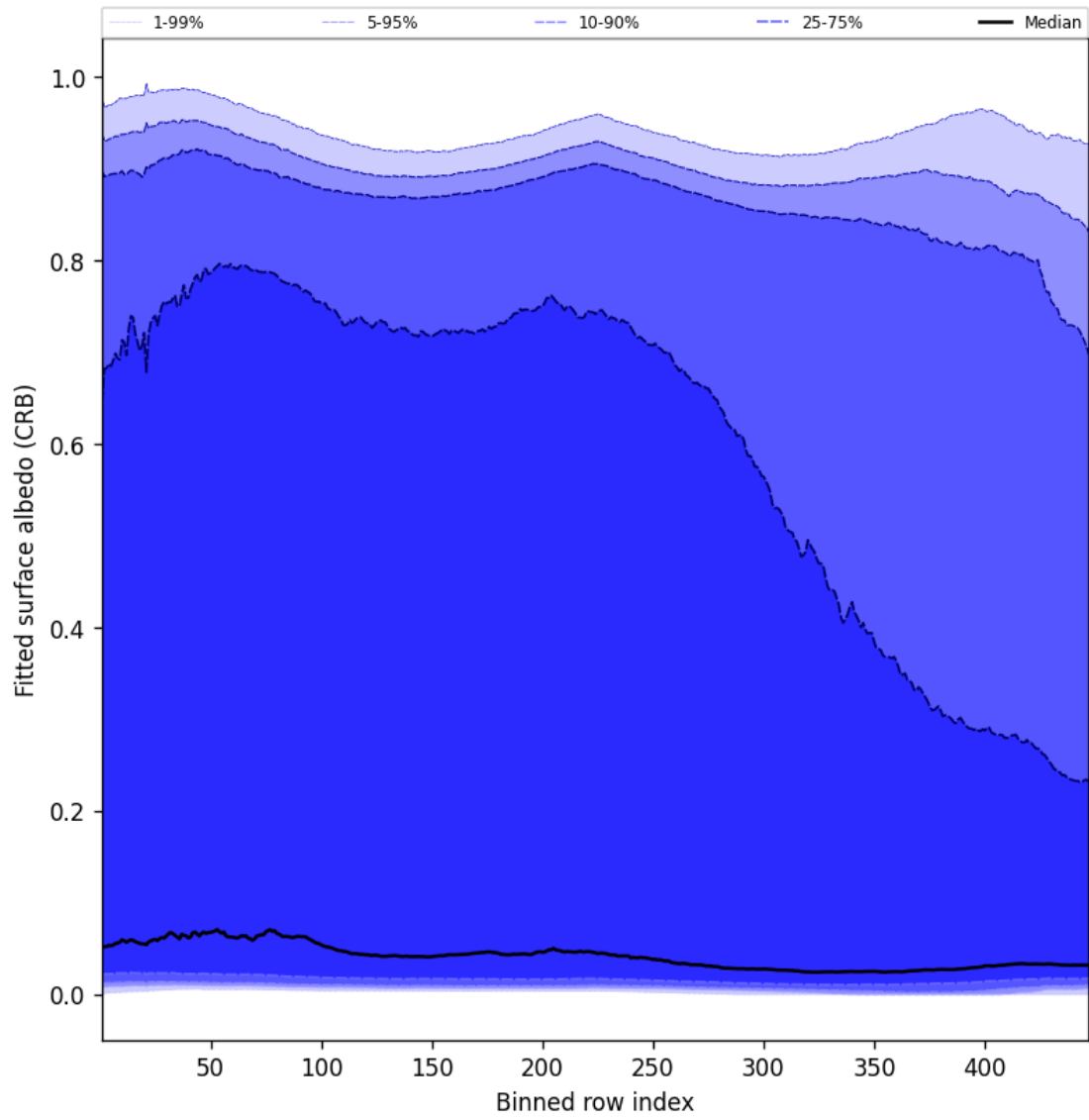
Figure 62: Along track statistics of “Fitted surface albedo (CRB)” for 2025-11-18 to 2025-11-19
