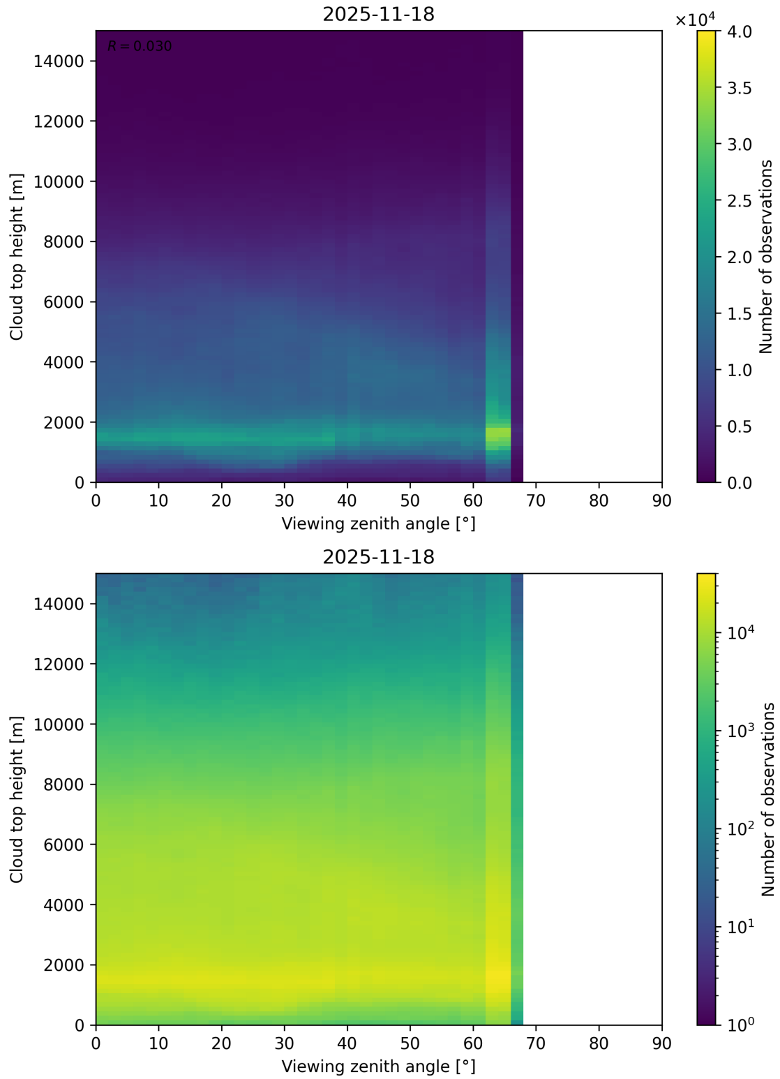
Figure 112: Scatter density plot of “Viewing zenith angle” against “Cloud top height” for 2025-11-18 to 2025-11-19.
