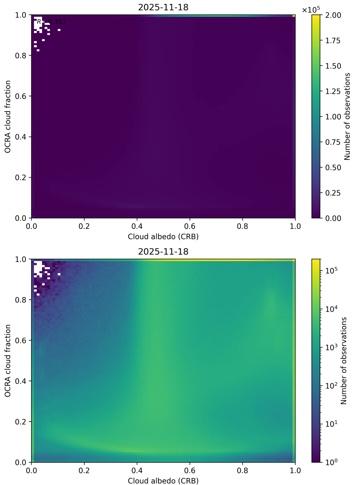
Figure 70: Scatter density plot of “Cloud albedo (CRB)” against “OCRA cloud fraction” for 2025-11-18 to 2025-11-19.
