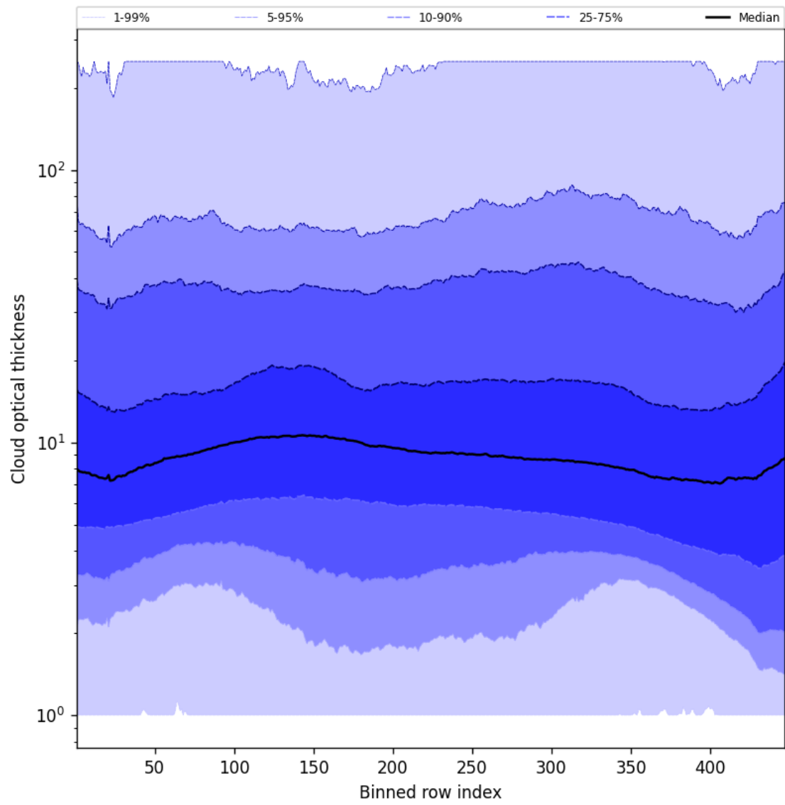
Figure 57: Along track statistics of “Cloud optical thickness” for 2025-11-18 to 2025-11-19
