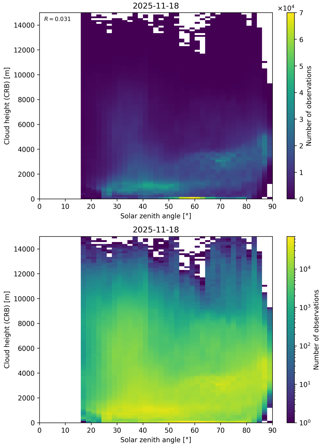
Figure 102: Scatter density plot of “Solar zenith angle” against “Cloud height (CRB)” for 2025-11-18 to 2025-11-19.
