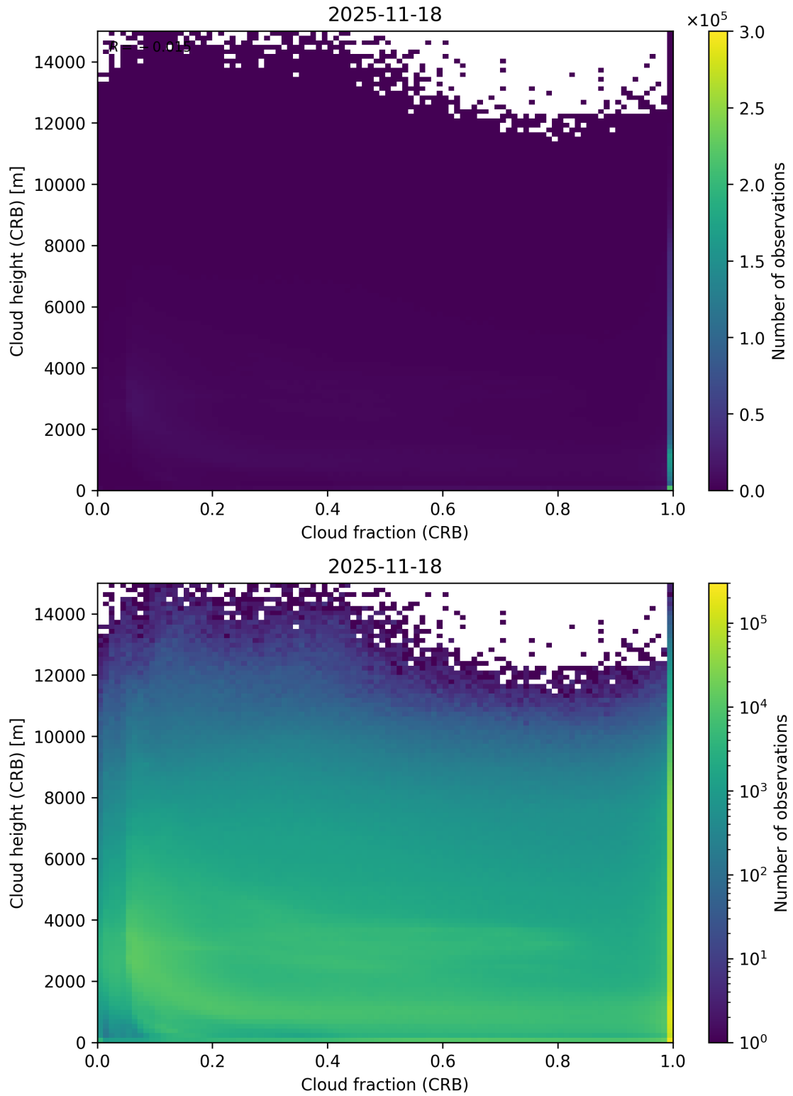
Figure 79: Scatter density plot of “Cloud fraction (CRB)” against “Cloud height (CRB)” for 2025-11-18 to 2025-11-19.
