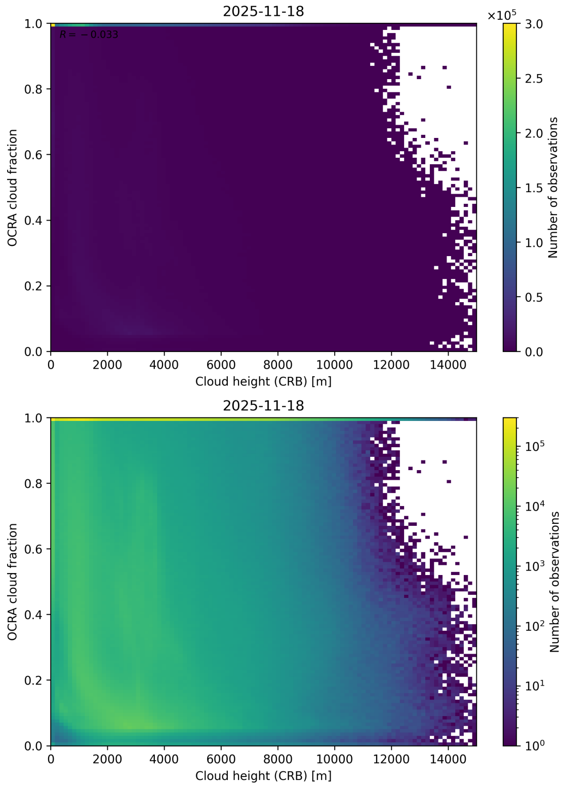
Figure 81: Scatter density plot of “Cloud height (CRB)” against “OCRA cloud fraction” for 2025-11-18 to 2025-11-19.
