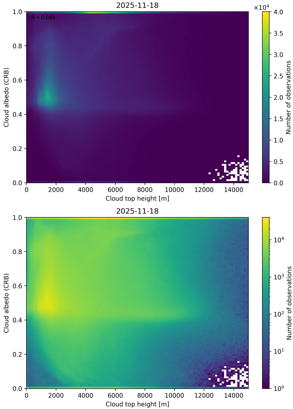
Figure 86: Scatter density plot of “Cloud top height” against “Cloud albedo (CRB)” for 2025-11-18 to 2025-11-19.
