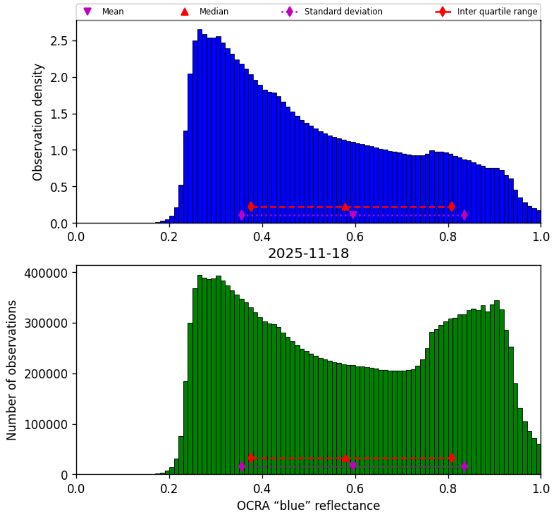
Figure 51: Histogram of "OCRA "blue" reflectance" for 2025-11-18 to 2025-11-19
