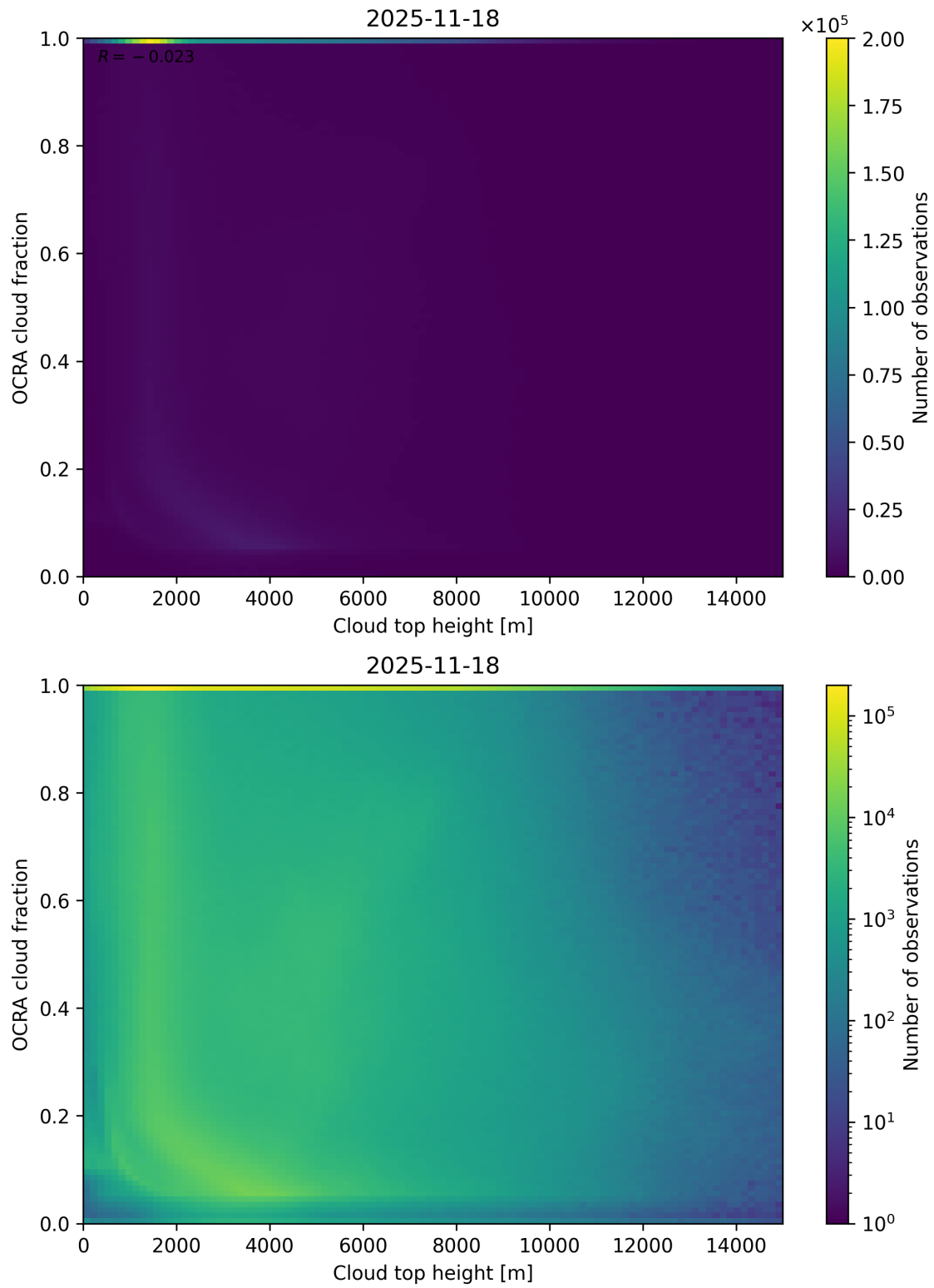
Figure 87: Scatter density plot of “Cloud top height” against “OCRA cloud fraction” for 2025-11-18 to 2025-11-19.
