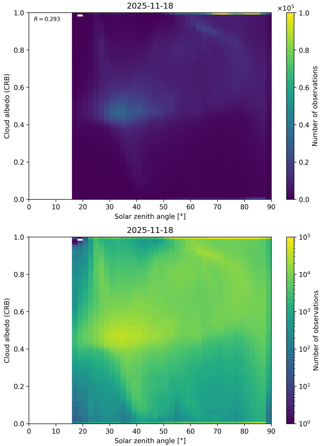
Figure 98: Scatter density plot of “Solar zenith angle” against “Cloud albedo (CRB)” for 2025-11-18 to 2025-11-19.
