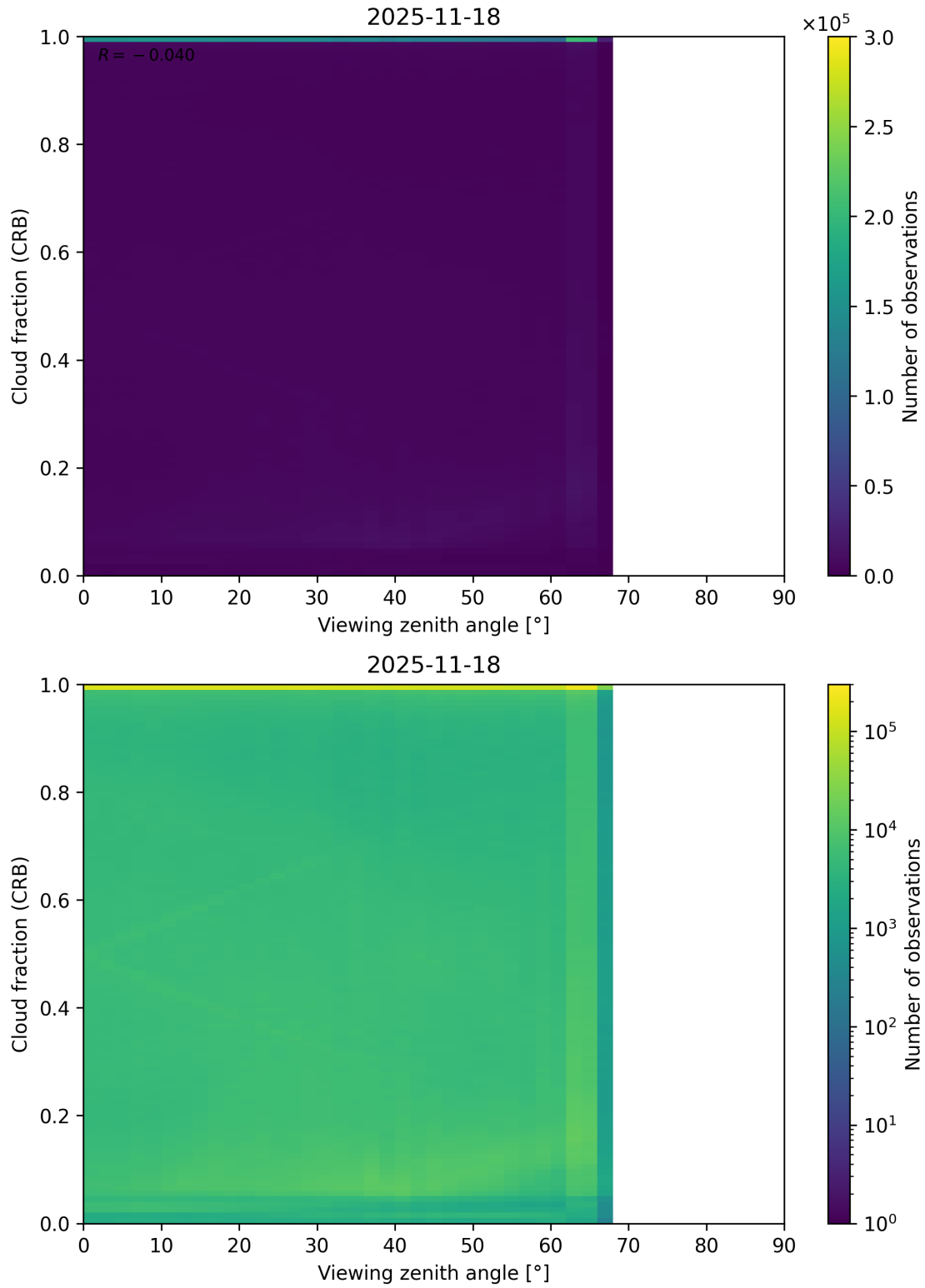
Figure 109: Scatter density plot of “Viewing zenith angle” against “Cloud fraction (CRB)” for 2025-11-18 to 2025-11-19.
