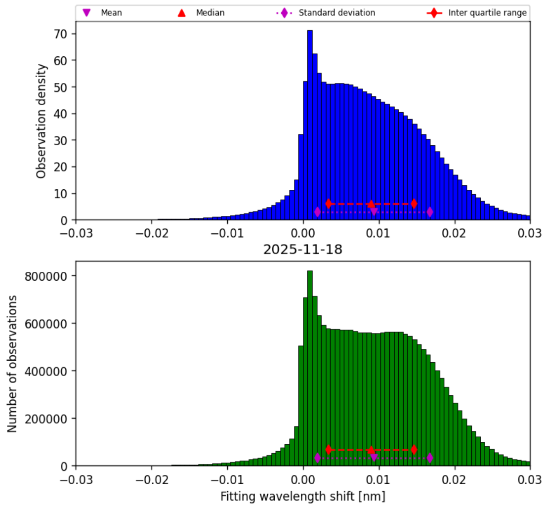
Figure 49: Histogram of “Fitting wavelength shift” for 2025-11-18 to 2025-11-19
