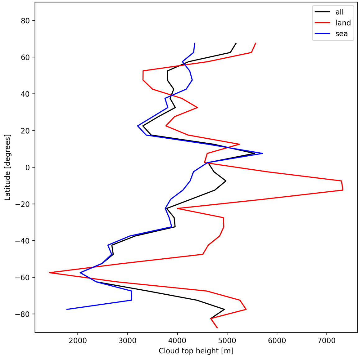
Figure 24: Zonal average of “Cloud top height” for 2025-11-18 to 2025-11-19.
