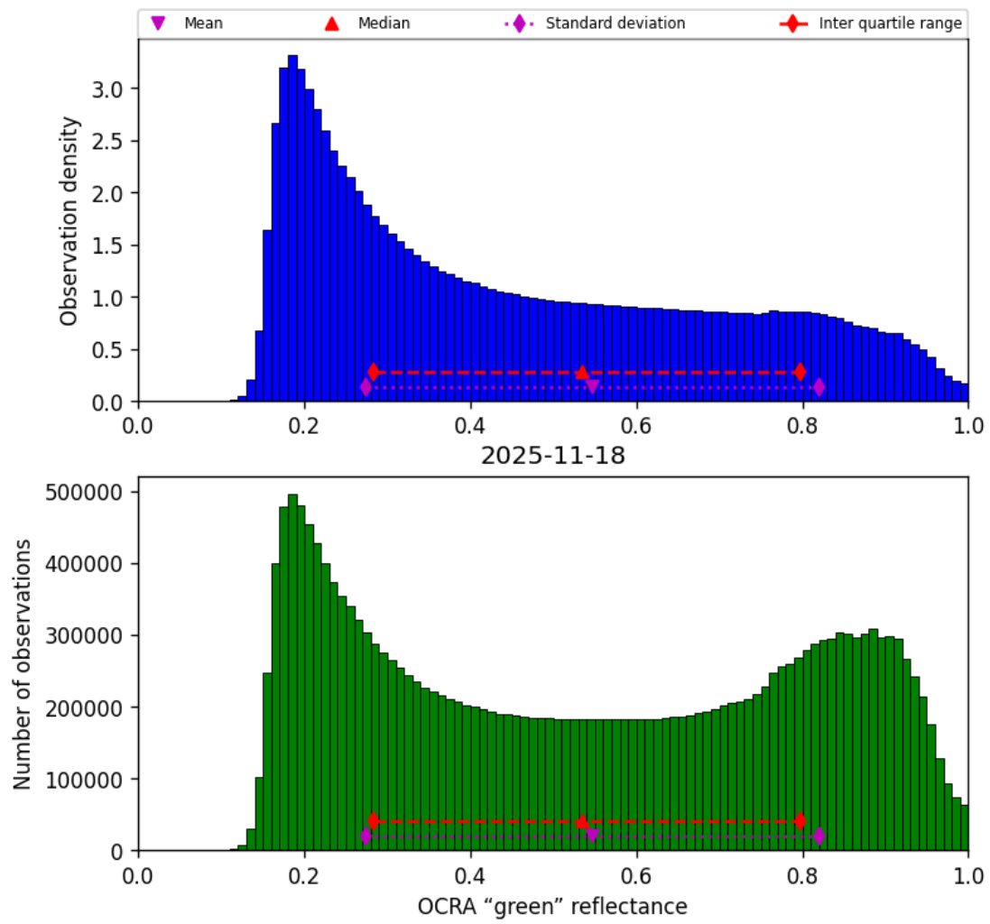
Figure 52: Histogram of “OCRA “green” reflectance” for 2025-11-18 to 2025-11-19
