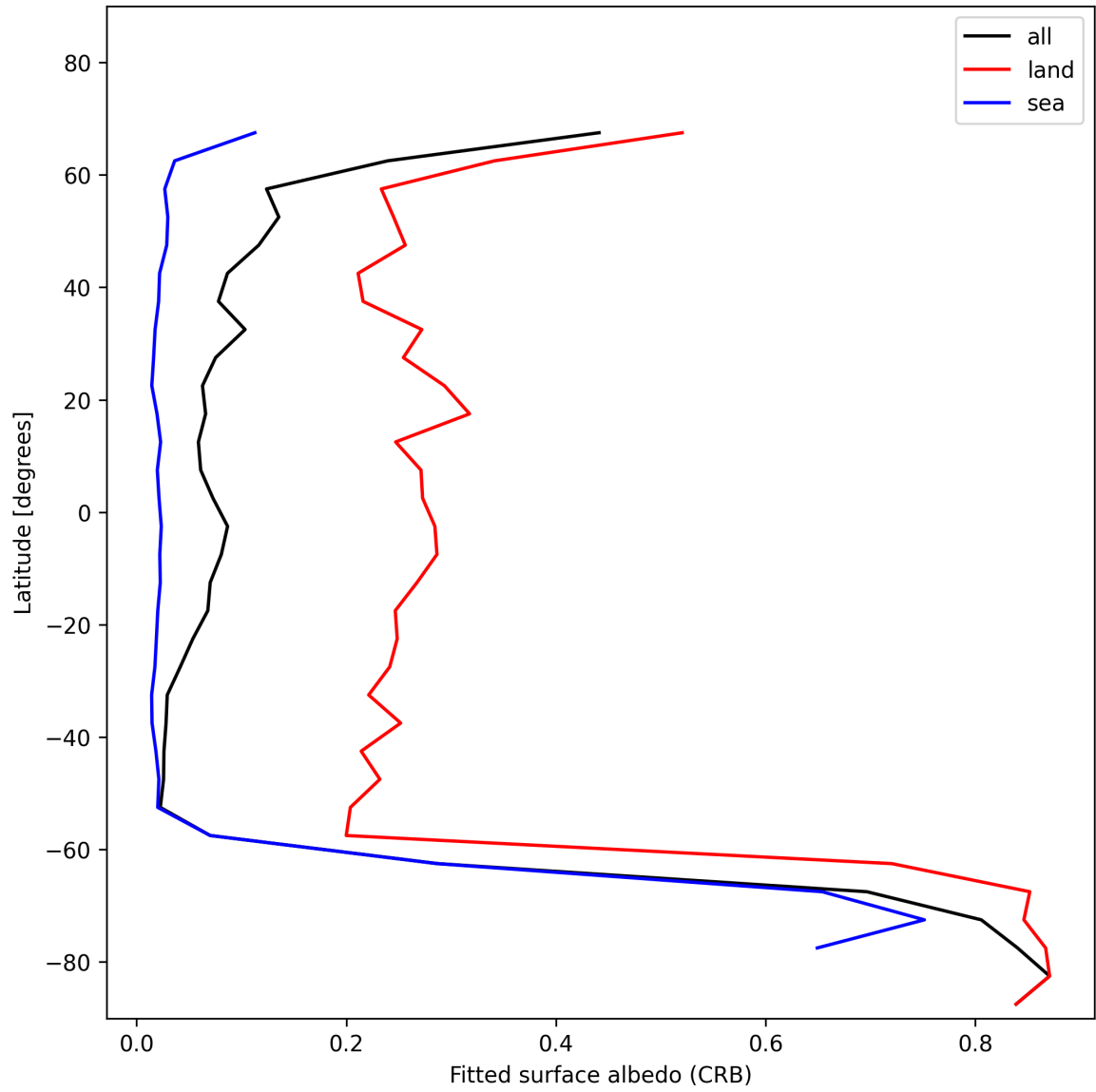
Figure 30: Zonal average of “Fitted surface albedo (CRB)” for 2025-11-18 to 2025-11-19.
