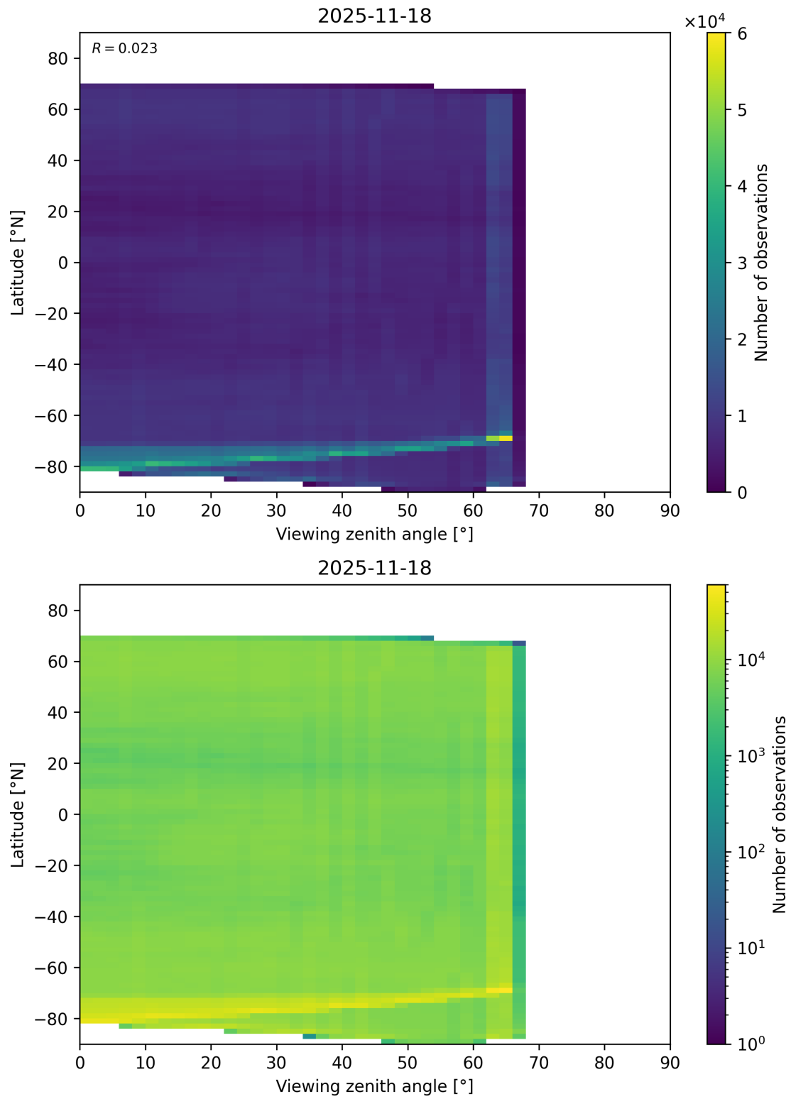
Figure 113: Scatter density plot of “Viewing zenith angle” against “Latitude” for 2025-11-18 to 2025-11-19.
