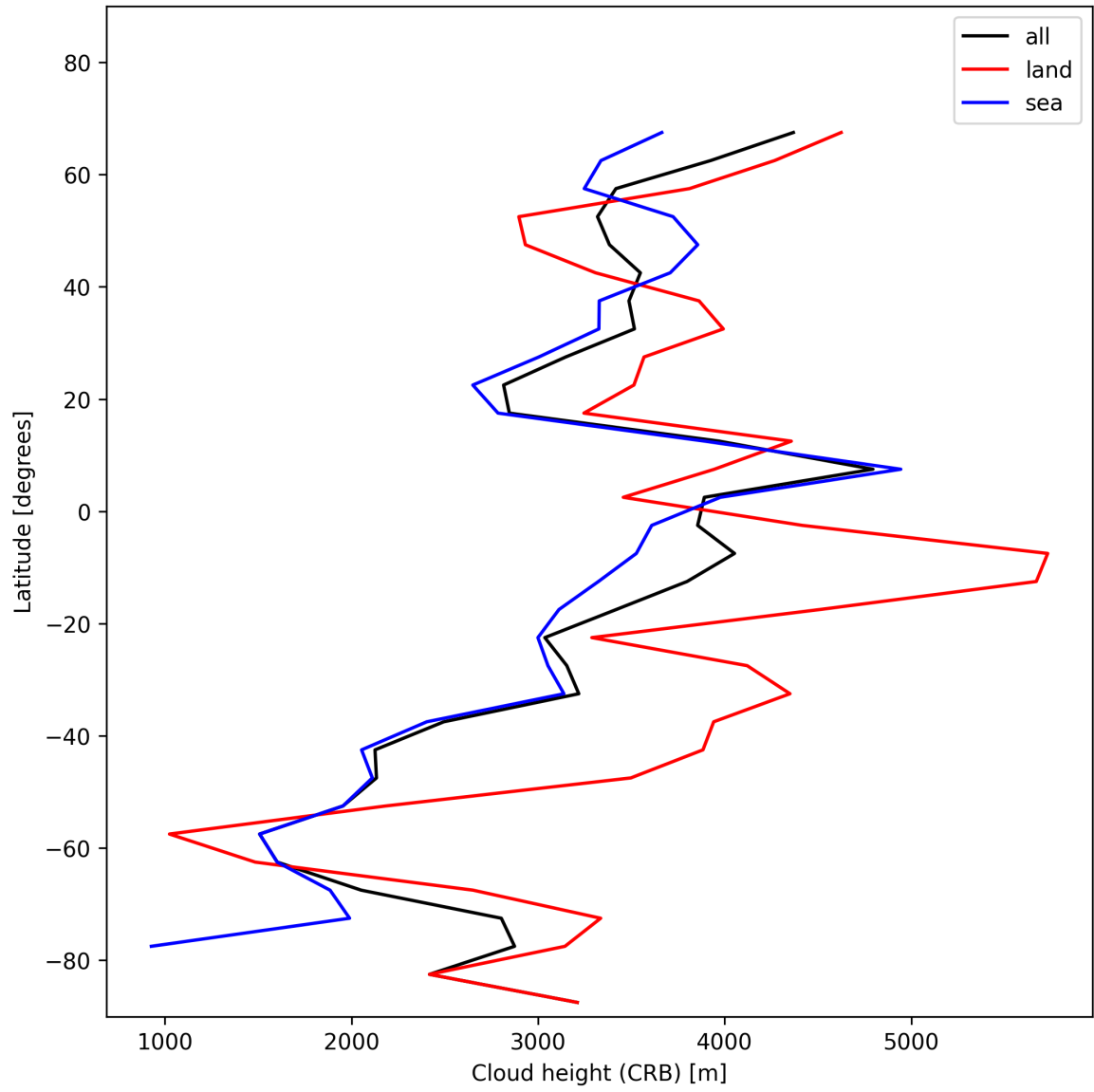
Figure 27: Zonal average of “Cloud height (CRB)” for 2025-11-18 to 2025-11-19.
