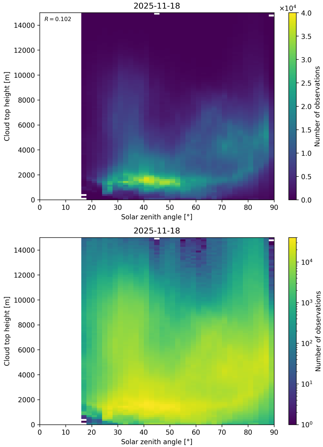
Figure 104: Scatter density plot of “Solar zenith angle” against “Cloud top height” for 2025-11-18 to 2025-11-19.
