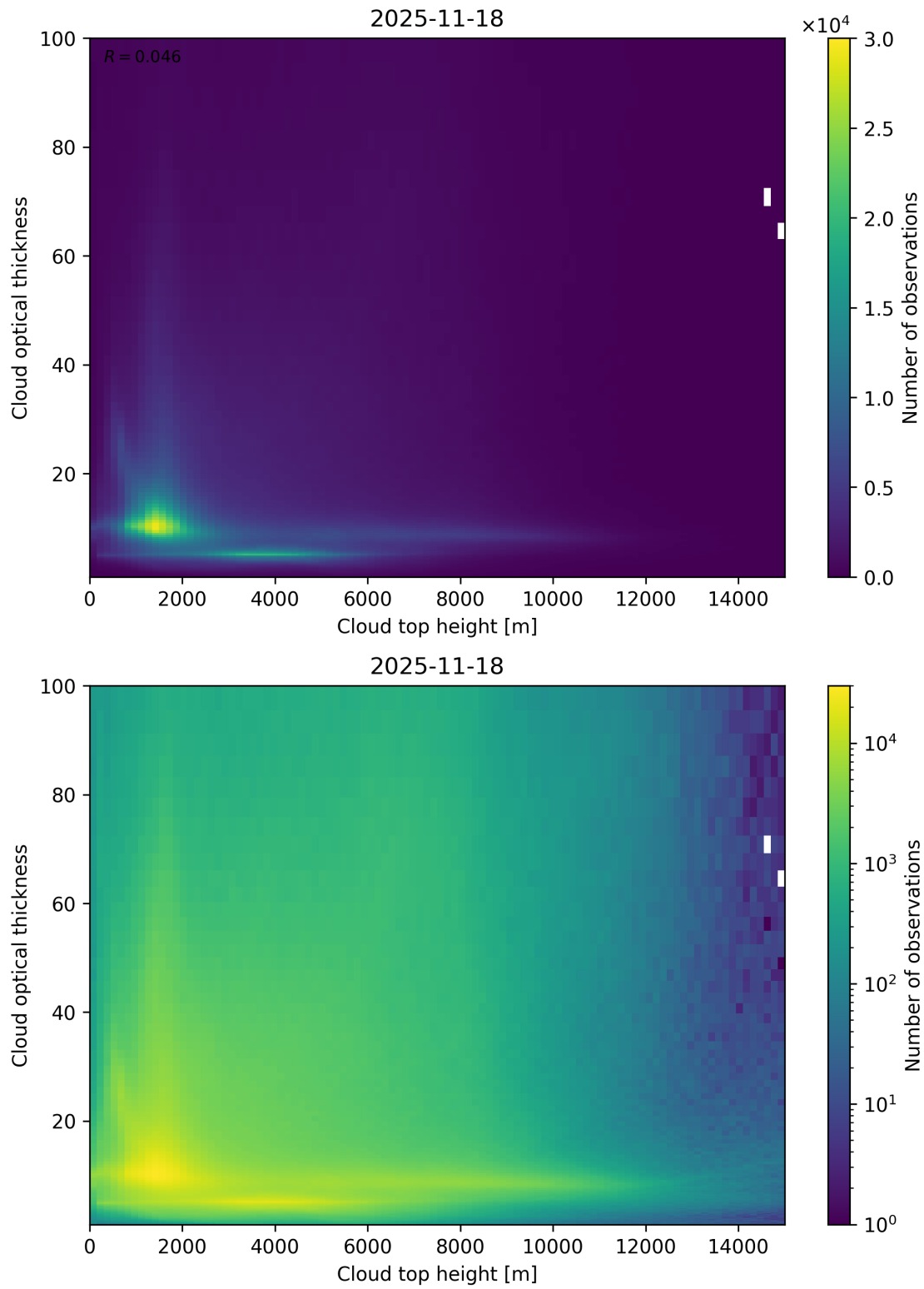
Figure 90: Scatter density plot of “Cloud top height” against “Cloud optical thickness” for 2025-11-18 to 2025-11-19.
