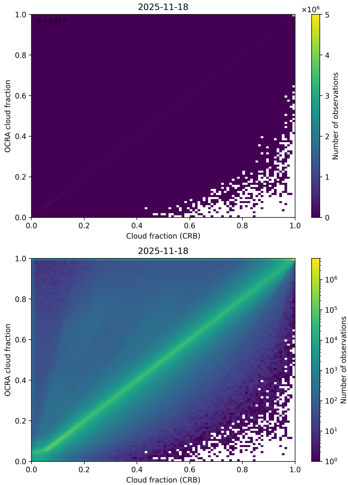
Figure 78: Scatter density plot of “Cloud fraction (CRB)” against “OCRA cloud fraction” for 2025-11-18 to 2025-11-19.
