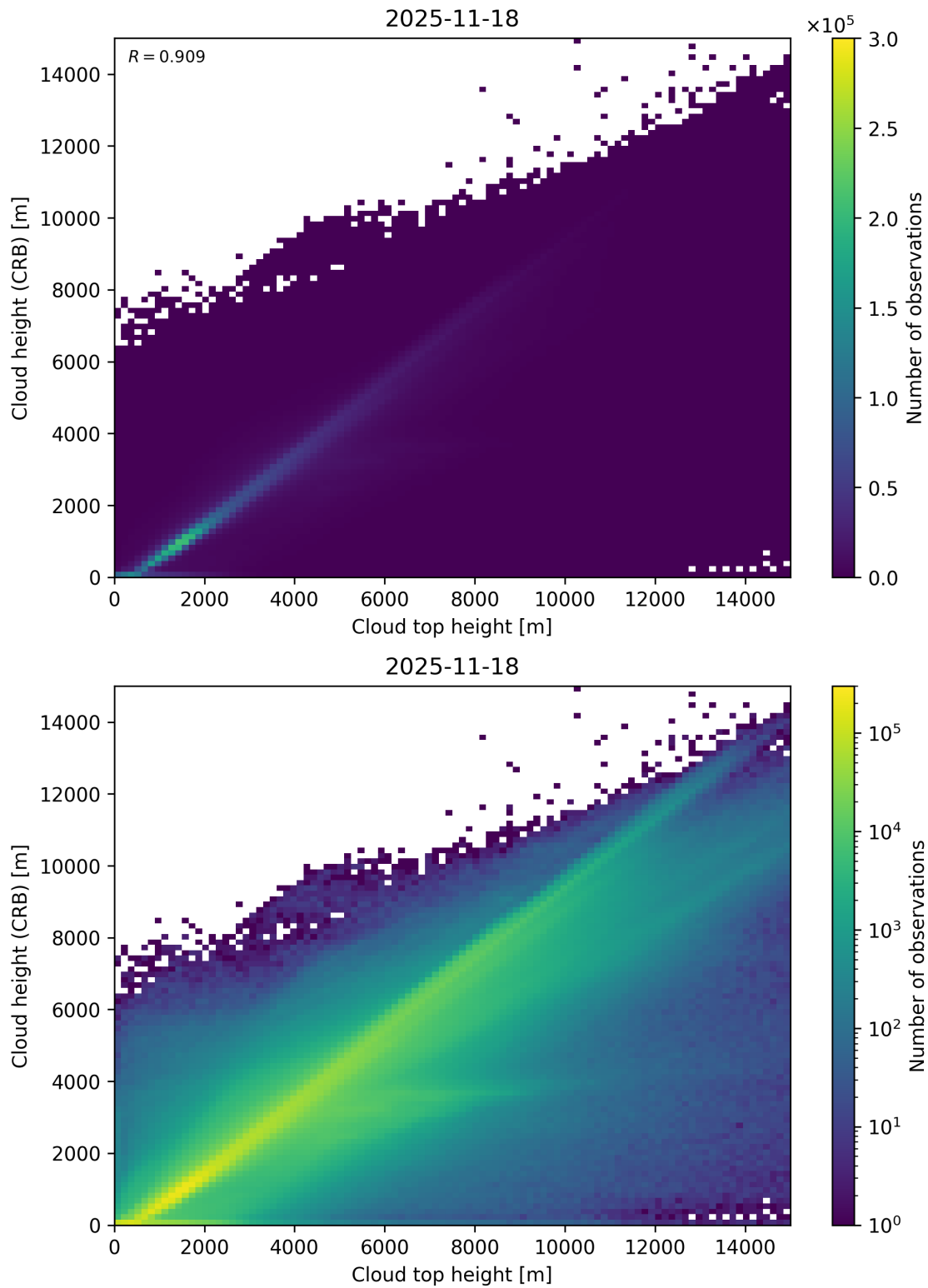
Figure 89: Scatter density plot of “Cloud top height” against “Cloud height (CRB)” for 2025-11-18 to 2025-11-19.
