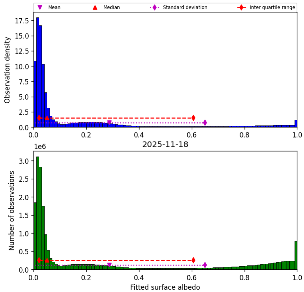
Figure 45: Histogram of “Fitted surface albedo” for 2025-11-18 to 2025-11-19
