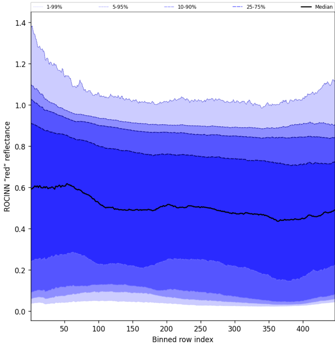
Figure 69: Along track statistics of "ROCINN "red" reflectance" for 2025-11-18 to 2025-11-19
