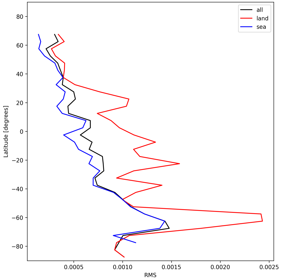
Figure 31: Zonal average of “RMS” for 2025-11-18 to 2025-11-19.
