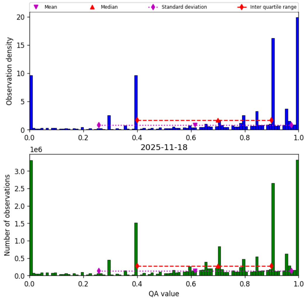
Figure 38: Histogram of “QA value” for 2025-11-18 to 2025-11-19
