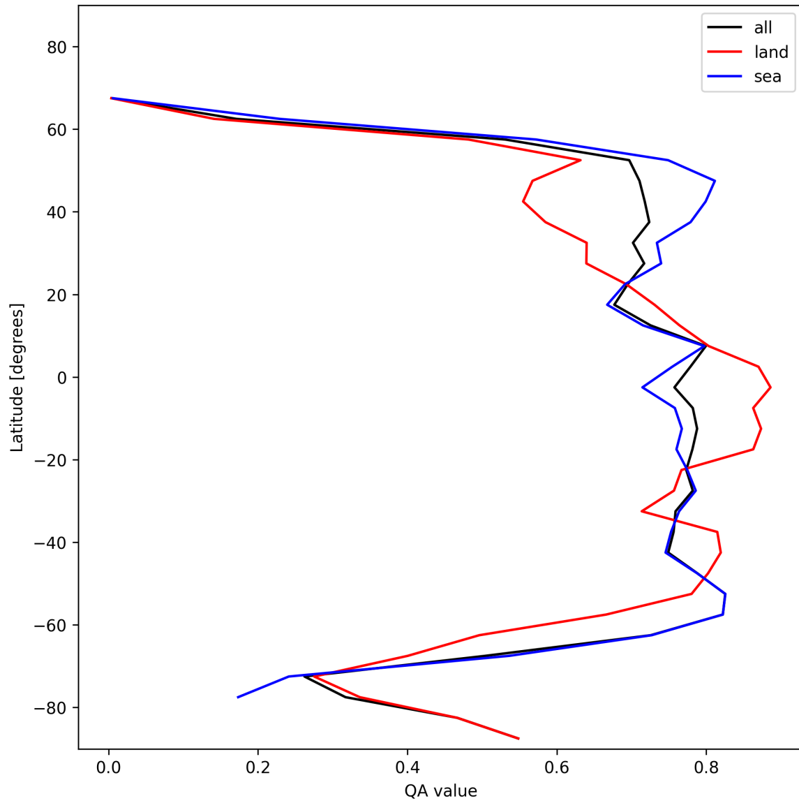
Figure 22: Zonal average of “QA value” for 2025-11-18 to 2025-11-19.
