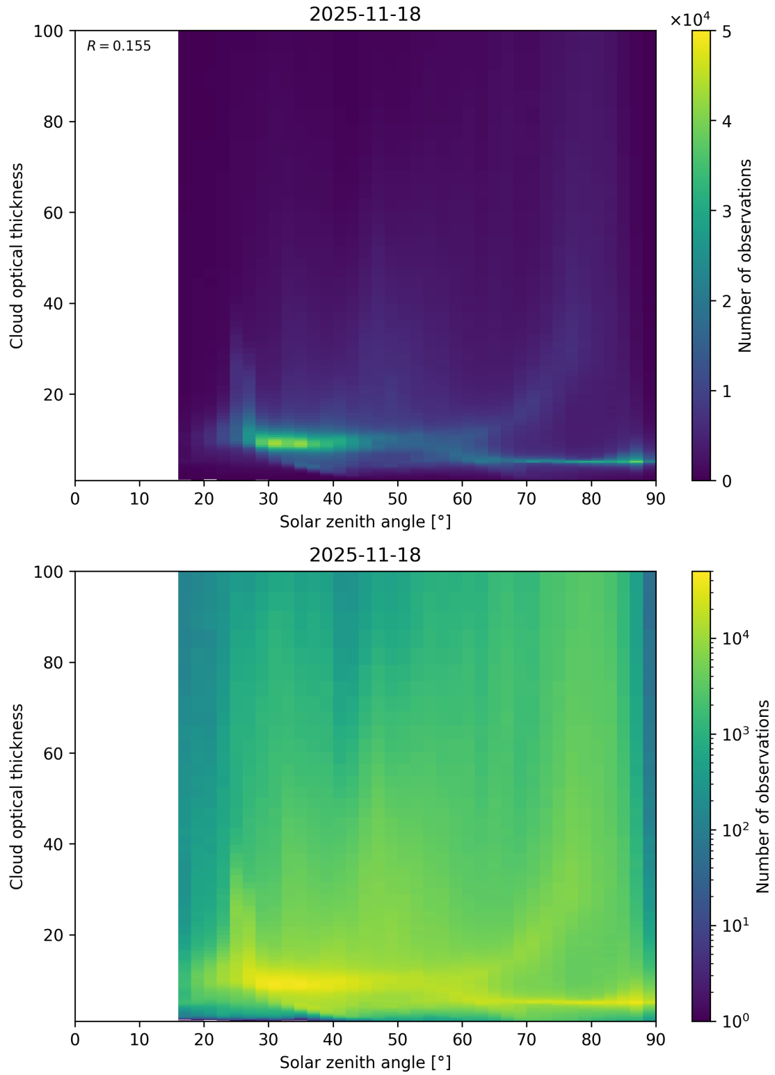
Figure 103: Scatter density plot of “Solar zenith angle” against “Cloud optical thickness” for 2025-11-18 to 2025-11-19.
