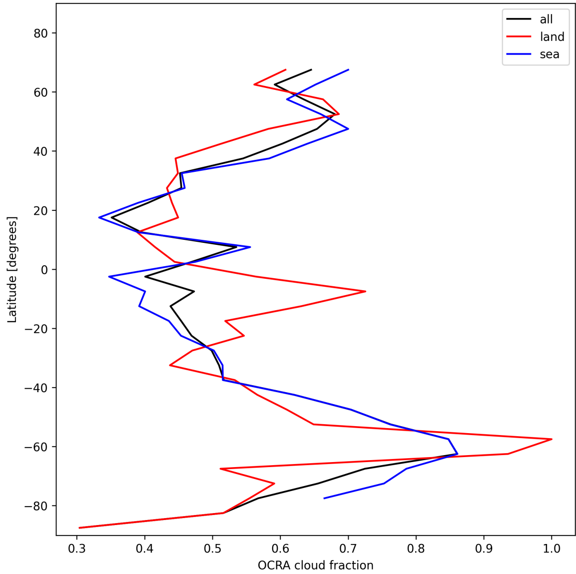
Figure 34: Zonal average of “OCRA cloud fraction” for 2025-11-18 to 2025-11-19.
