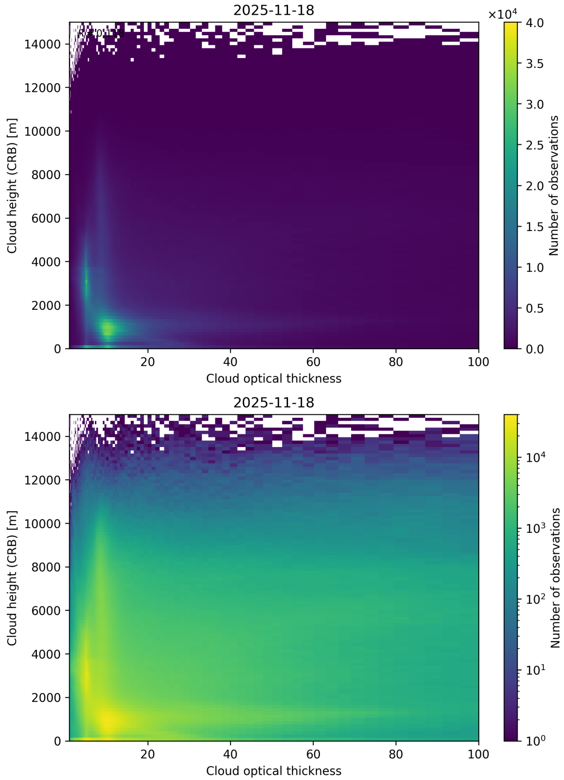
Figure 85: Scatter density plot of “Cloud optical thickness” against “Cloud height (CRB)” for 2025-11-18 to 2025-11-19.
