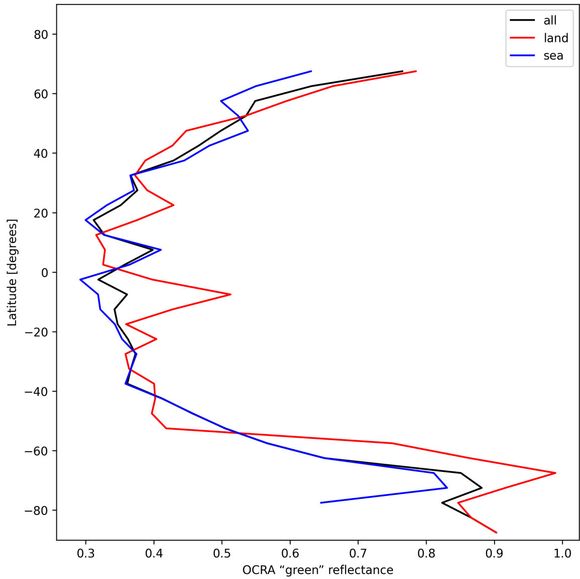
Figure 36: Zonal average of “OCRA “green” reflectance” for 2025-11-18 to 2025-11-19.
