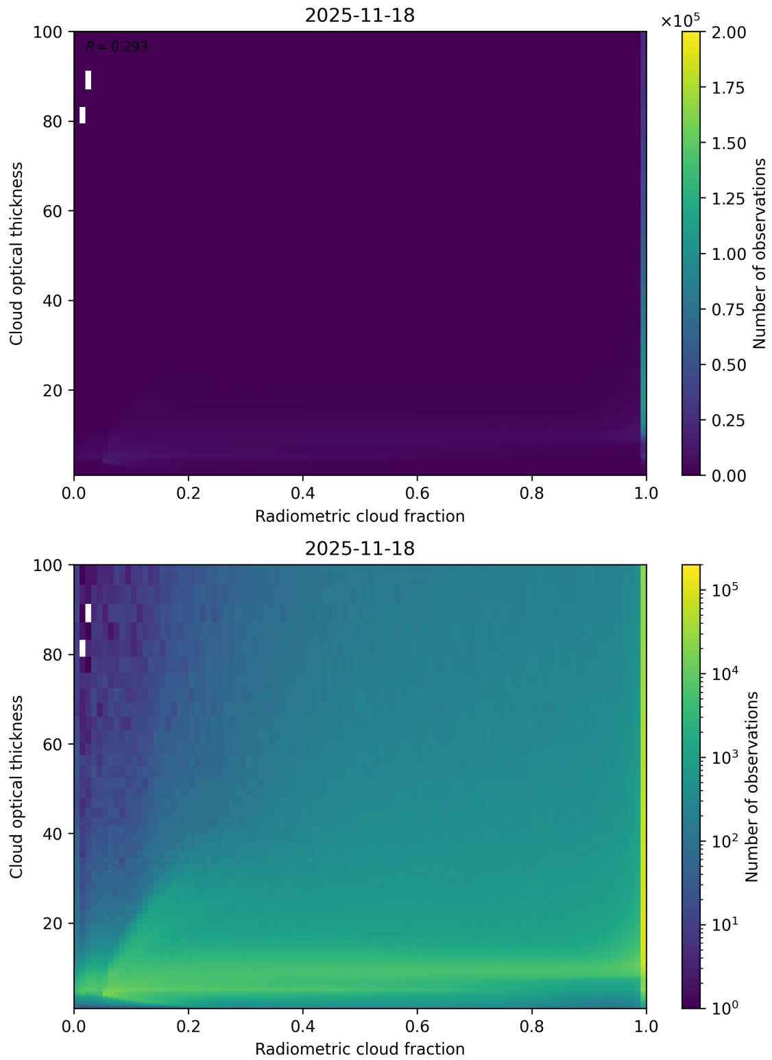
Figure 75: Scatter density plot of “Radiometric cloud fraction” against “Cloud optical thickness” for 2025-11-18 to 2025-11-19.
