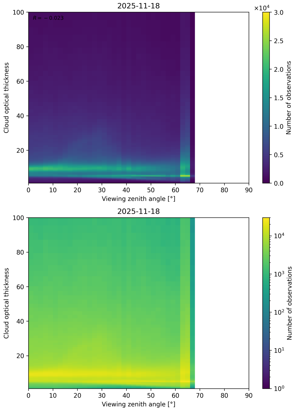
Figure 111: Scatter density plot of “Viewing zenith angle” against “Cloud optical thickness” for 2025-11-18 to 2025-11-19.
