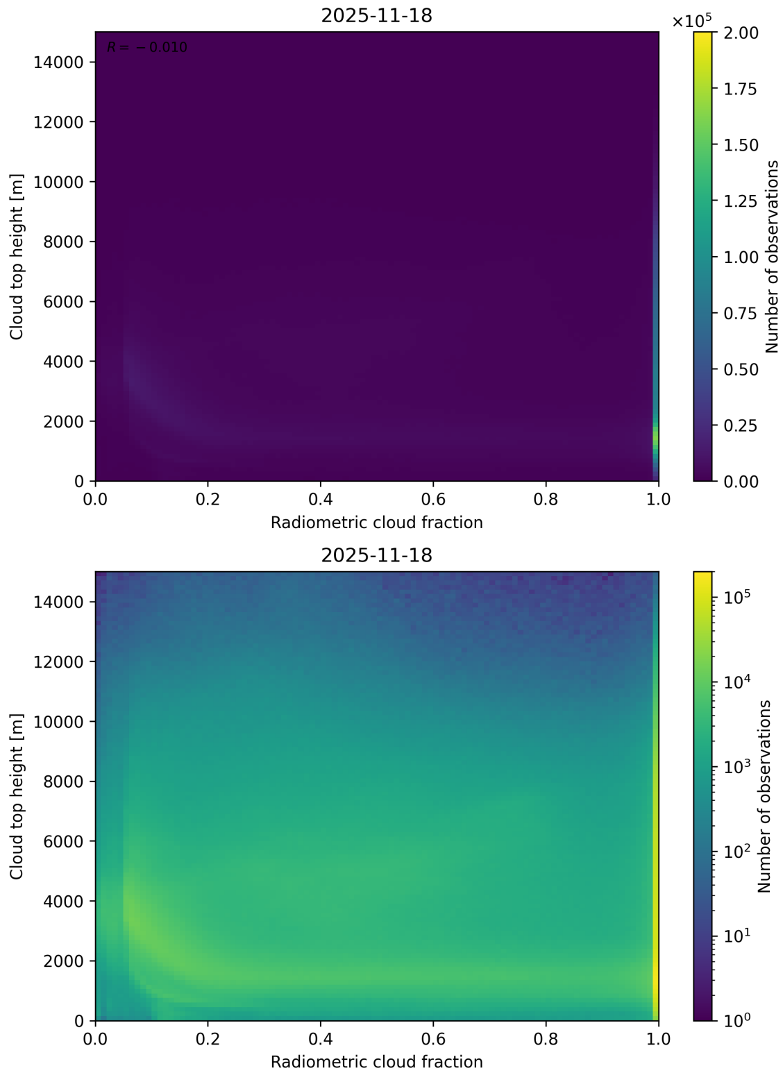
Figure 76: Scatter density plot of “Radiometric cloud fraction” against “Cloud top height” for 2025-11-18 to 2025-11-19.
