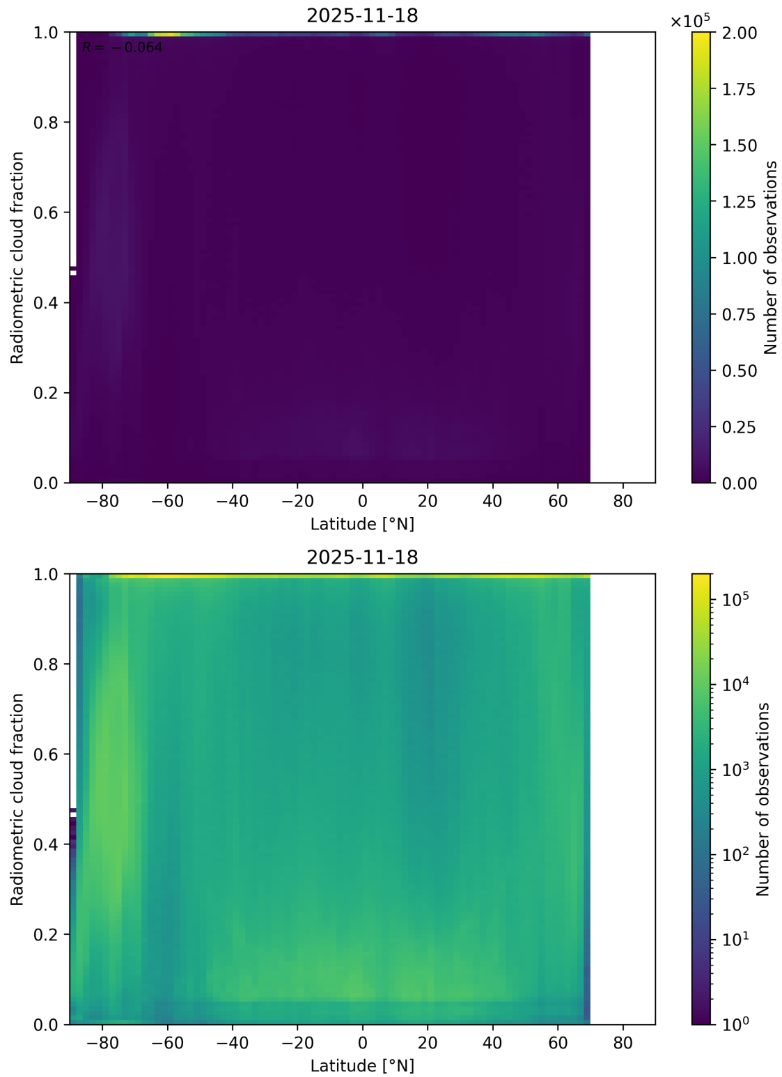
Figure 92: Scatter density plot of “Latitude” against “Radiometric cloud fraction” for 2025-11-18 to 2025-11-19.
