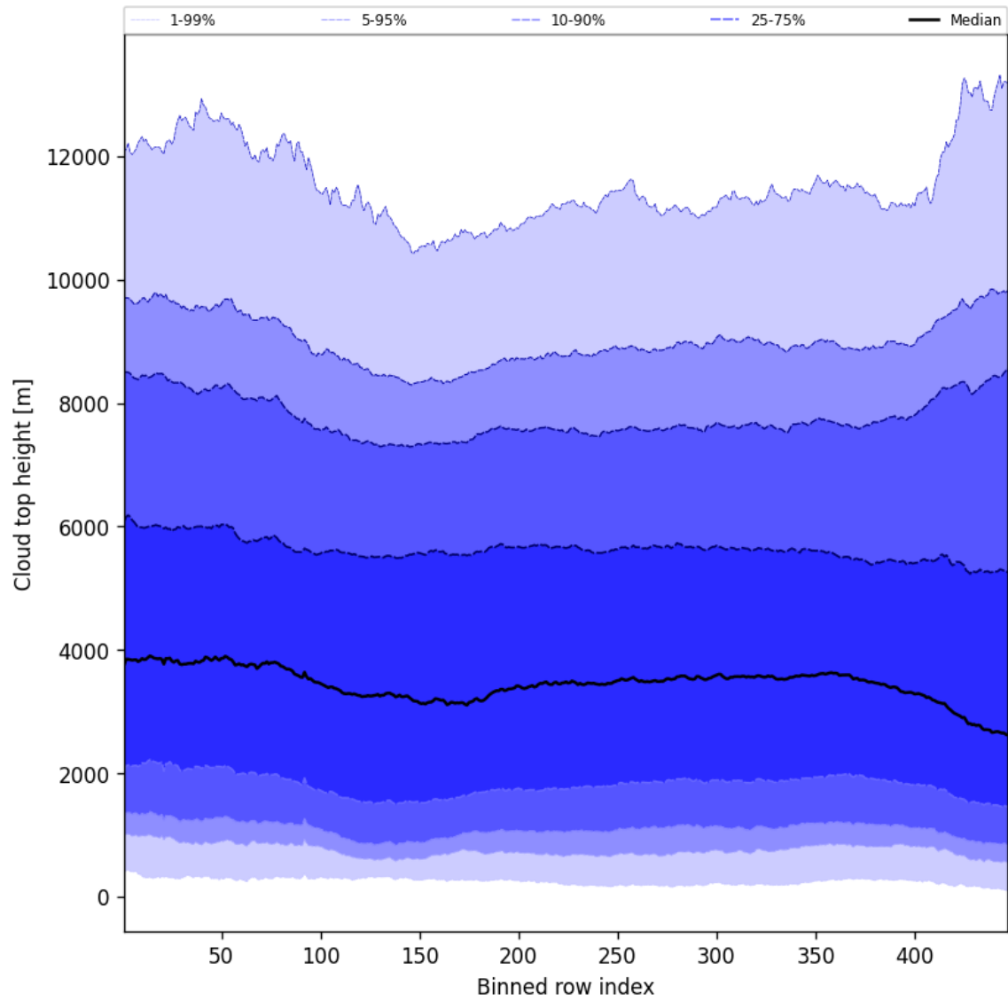
Figure 56: Along track statistics of “Cloud top height” for 2025-11-18 to 2025-11-19
