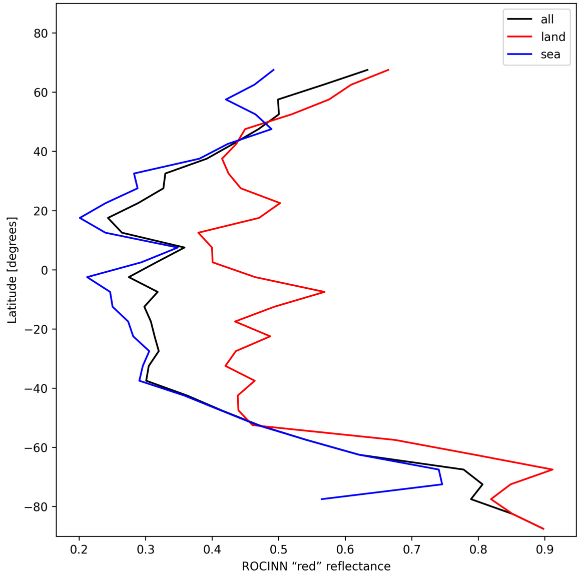
Figure 37: Zonal average of "ROCINN "red" reflectance" for 2025-11-18 to 2025-11-19.
