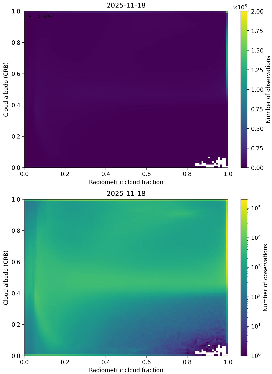
Figure 71: Scatter density plot of “Radiometric cloud fraction” against “Cloud albedo (CRB)” for 2025-11-18 to 2025-11-19.
