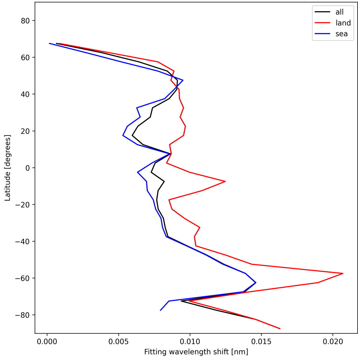
Figure 33: Zonal average of “Fitting wavelength shift” for 2025-11-18 to 2025-11-19.
