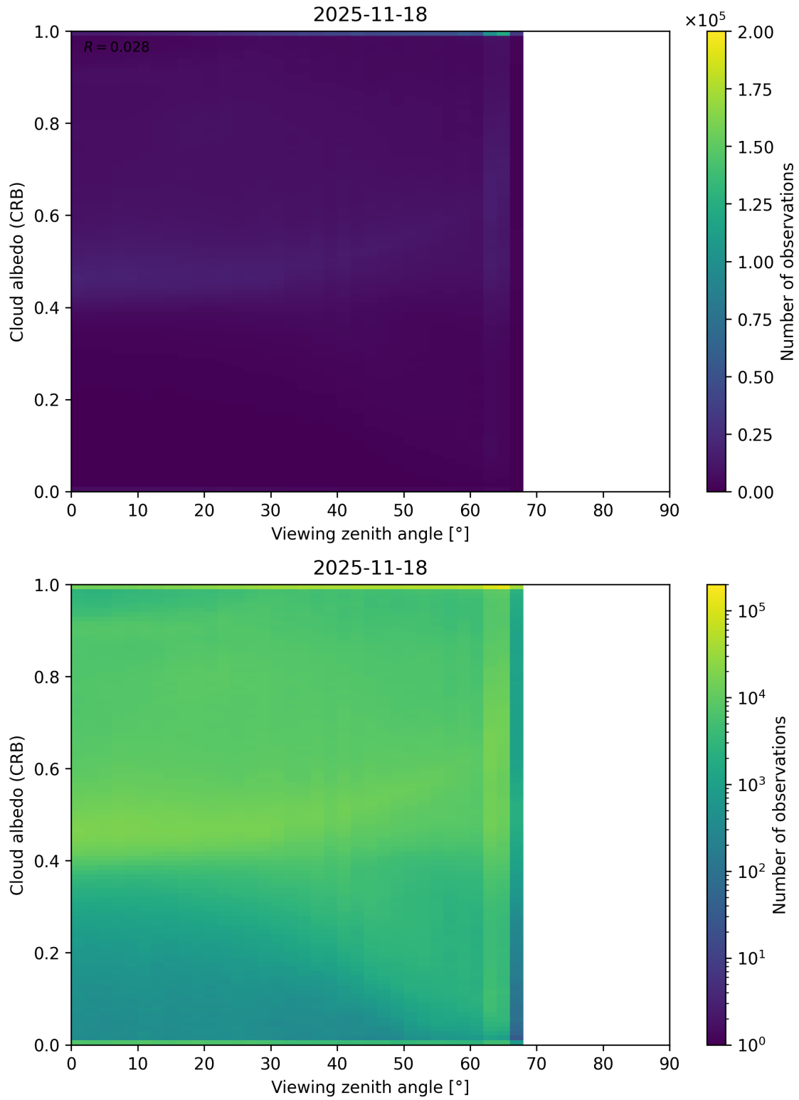
Figure 106: Scatter density plot of “Viewing zenith angle” against “Cloud albedo (CRB)” for 2025-11-18 to 2025-11-19.
