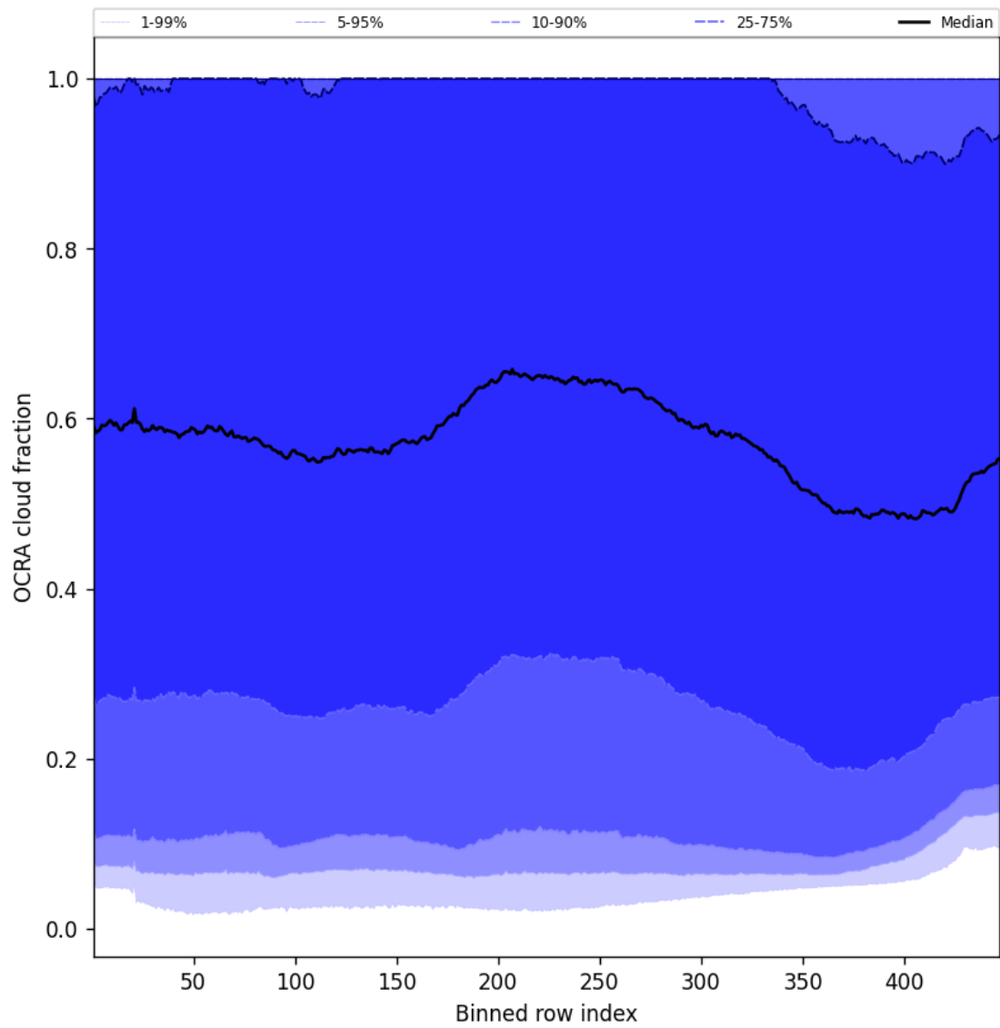
Figure 66: Along track statistics of “OCRA cloud fraction” for 2025-11-18 to 2025-11-19
