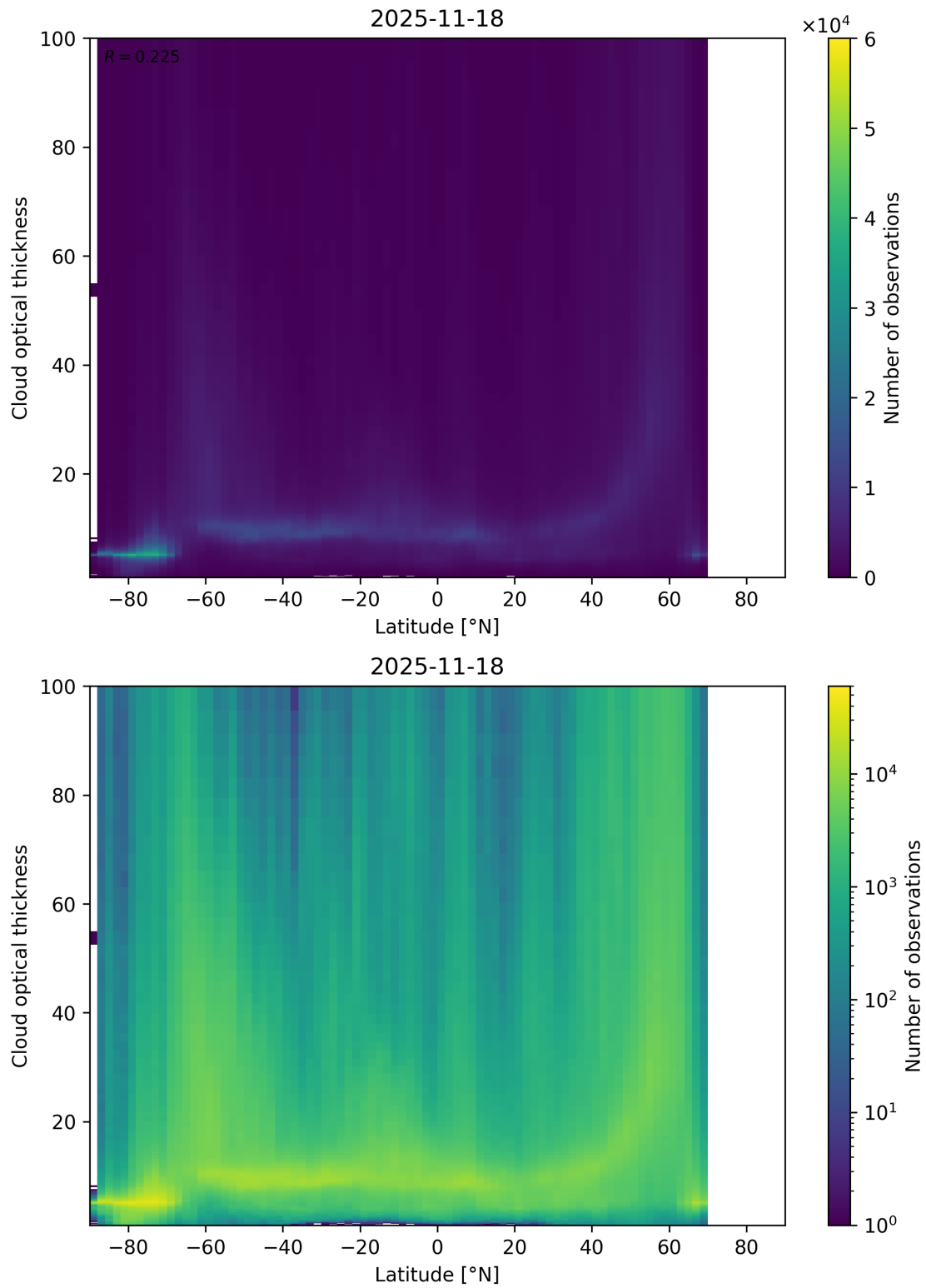
Figure 96: Scatter density plot of “Latitude” against “Cloud optical thickness” for 2025-11-18 to 2025-11-19.
