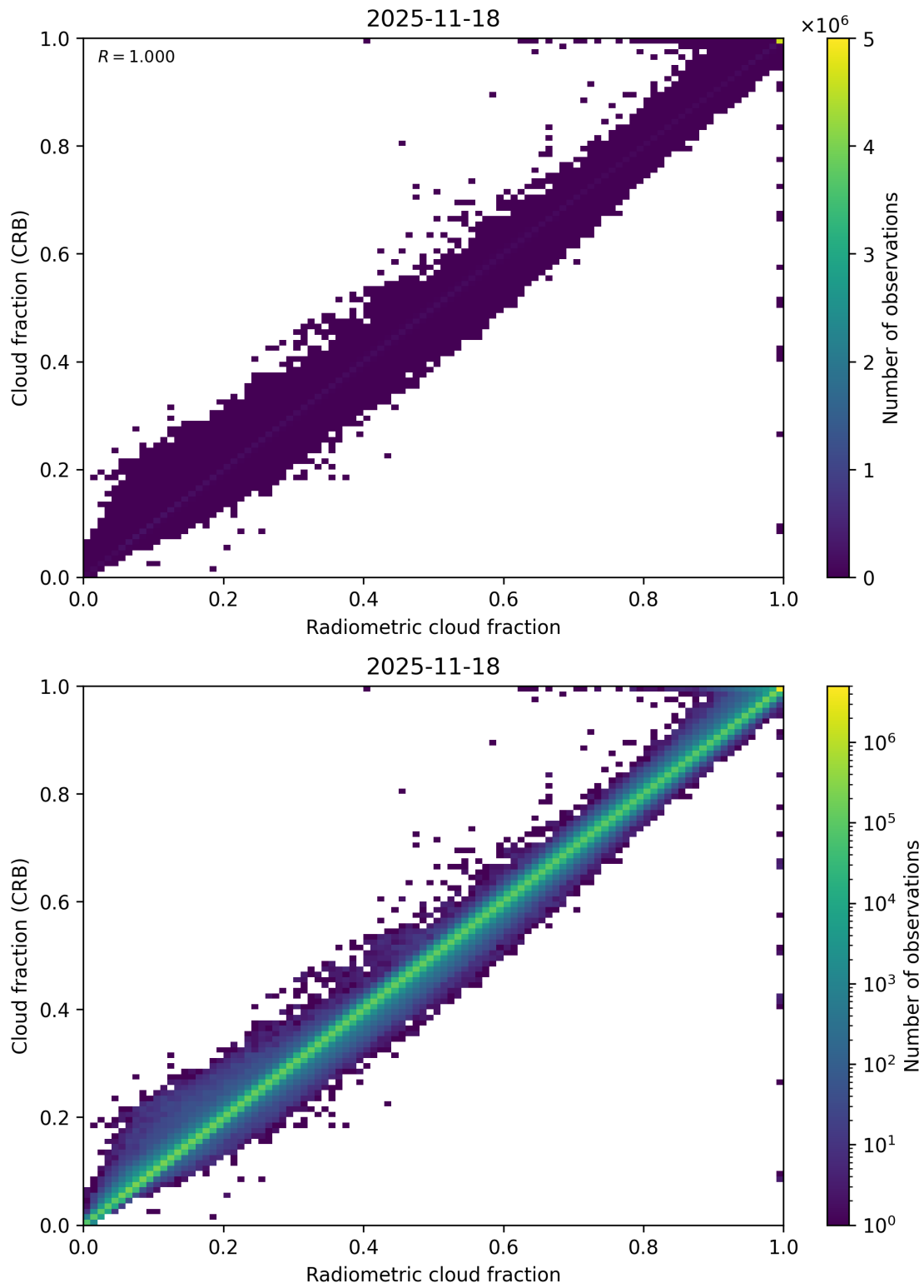
Figure 73: Scatter density plot of “Radiometric cloud fraction” against “Cloud fraction (CRB)” for 2025-11-18 to 2025-11-19.
