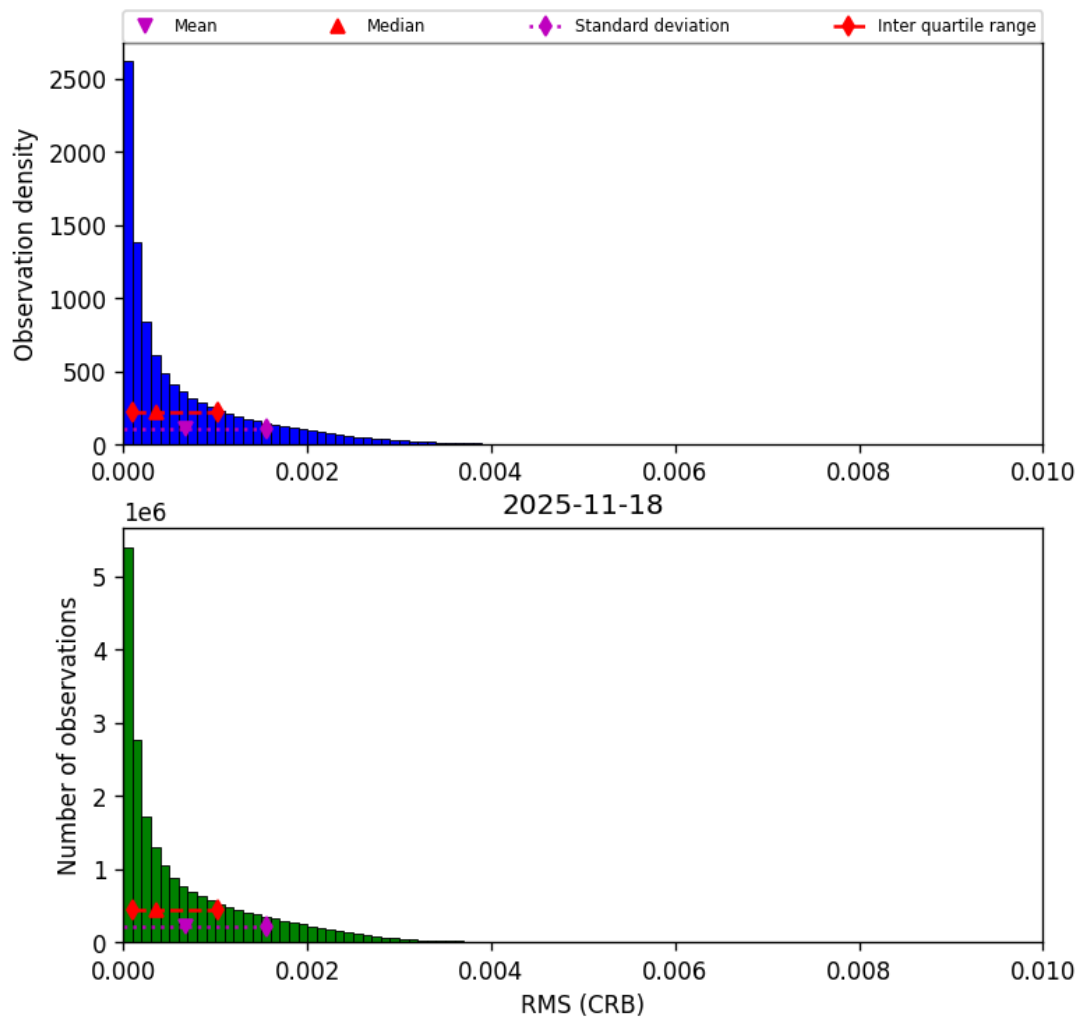
Figure 48: Histogram of “RMS (CRB)” for 2025-11-18 to 2025-11-19
