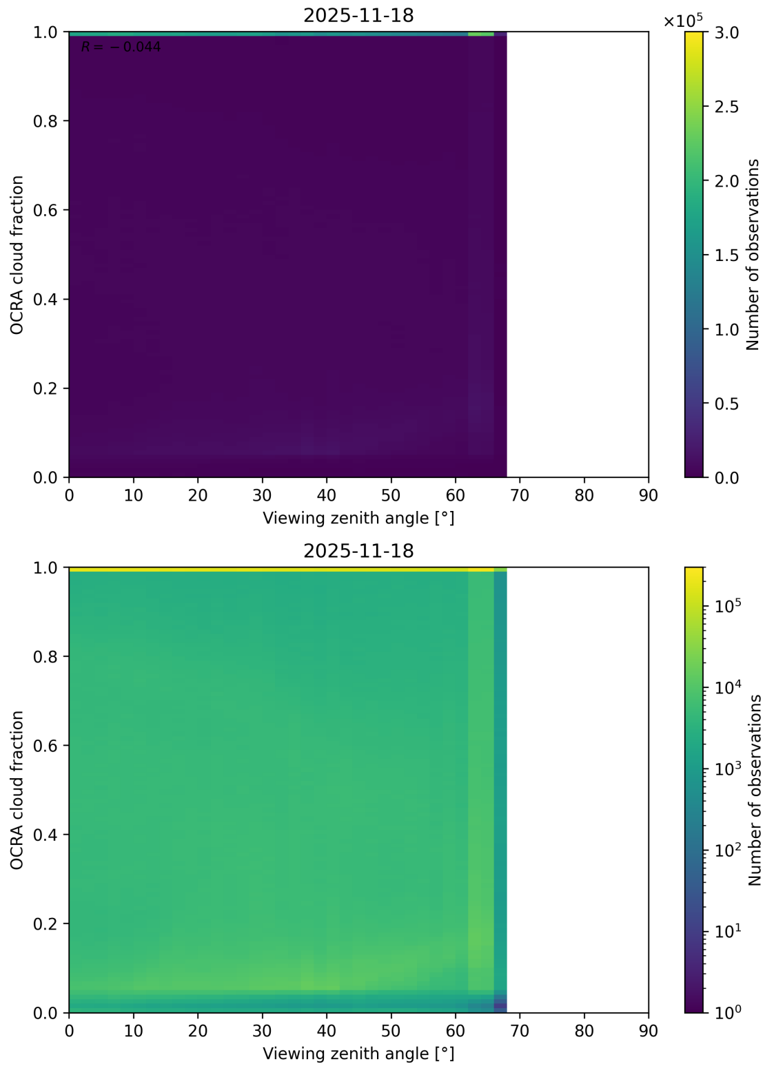
Figure 108: Scatter density plot of “Viewing zenith angle” against “OCRA cloud fraction” for 2025-11-18 to 2025-11-19.
