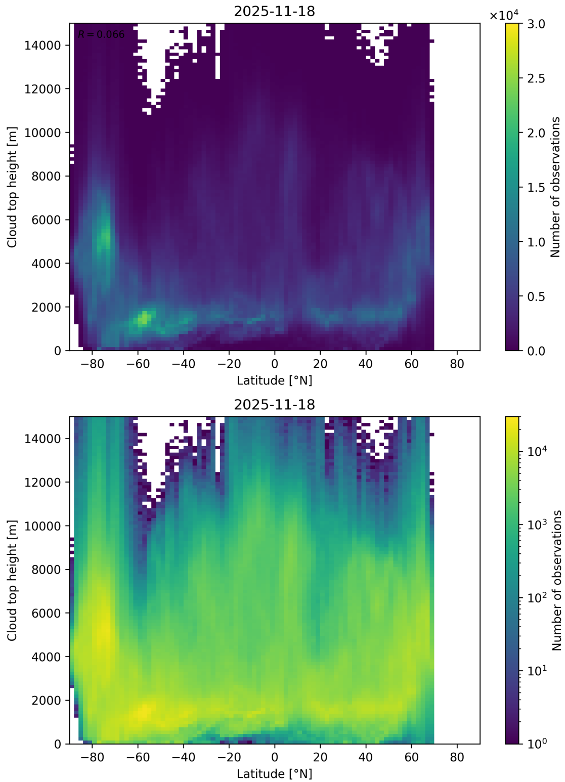
Figure 97: Scatter density plot of “Latitude” against “Cloud top height” for 2025-11-18 to 2025-11-19.
