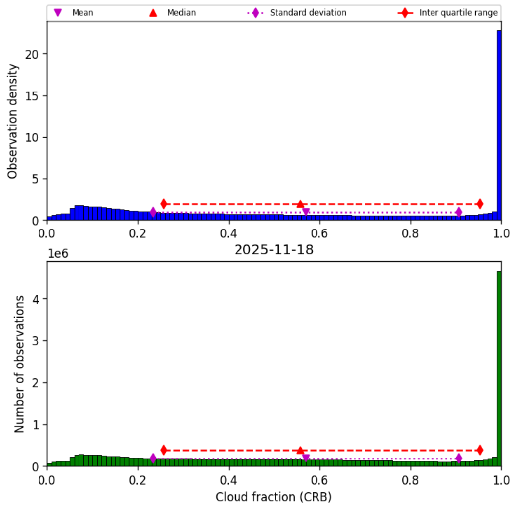
Figure 42: Histogram of “Cloud fraction (CRB)” for 2025-11-18 to 2025-11-19
