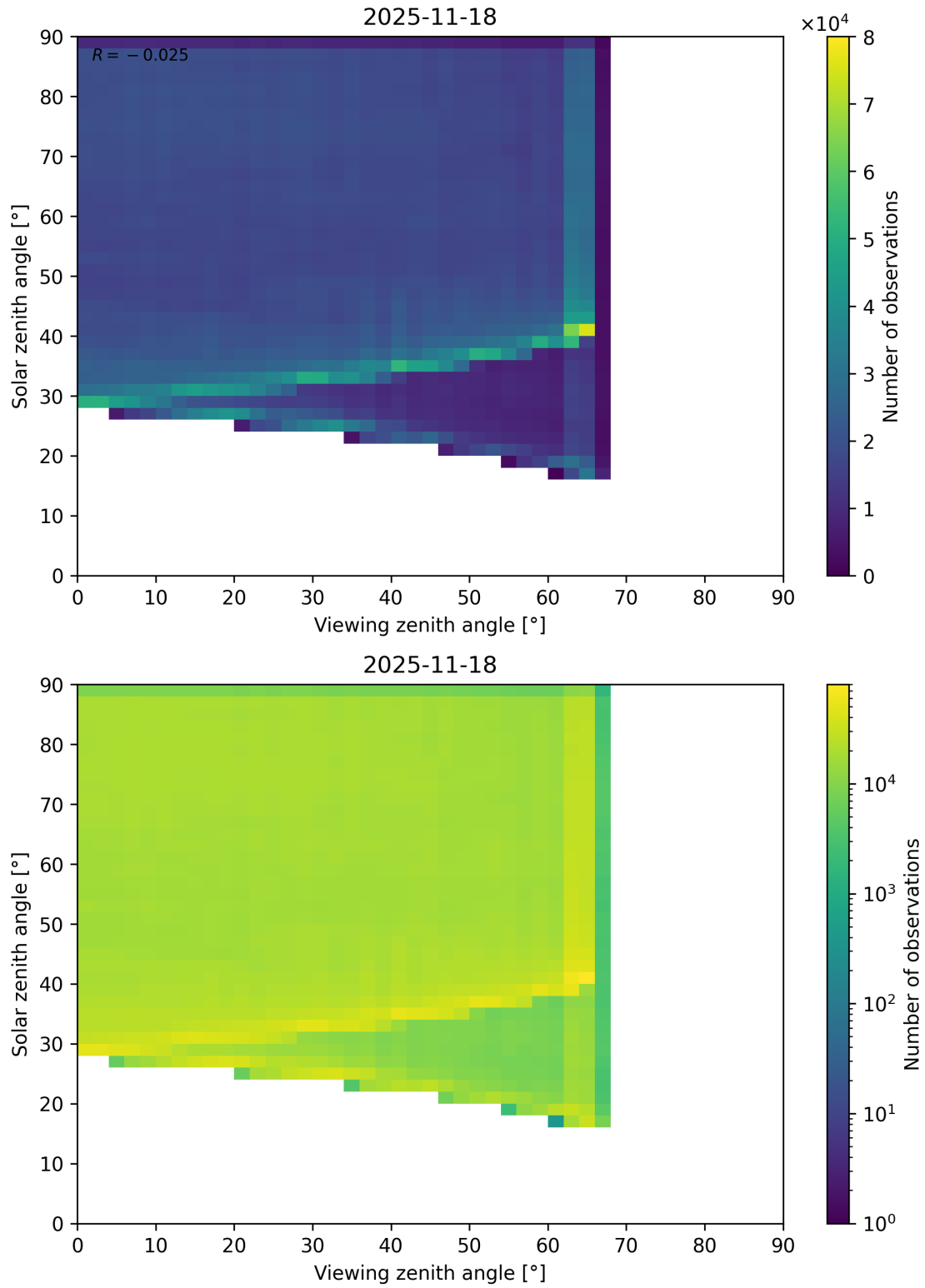
Figure 114: Scatter density plot of “Viewing zenith angle” against “Solar zenith angle” for 2025-11-18 to 2025-11-19.
