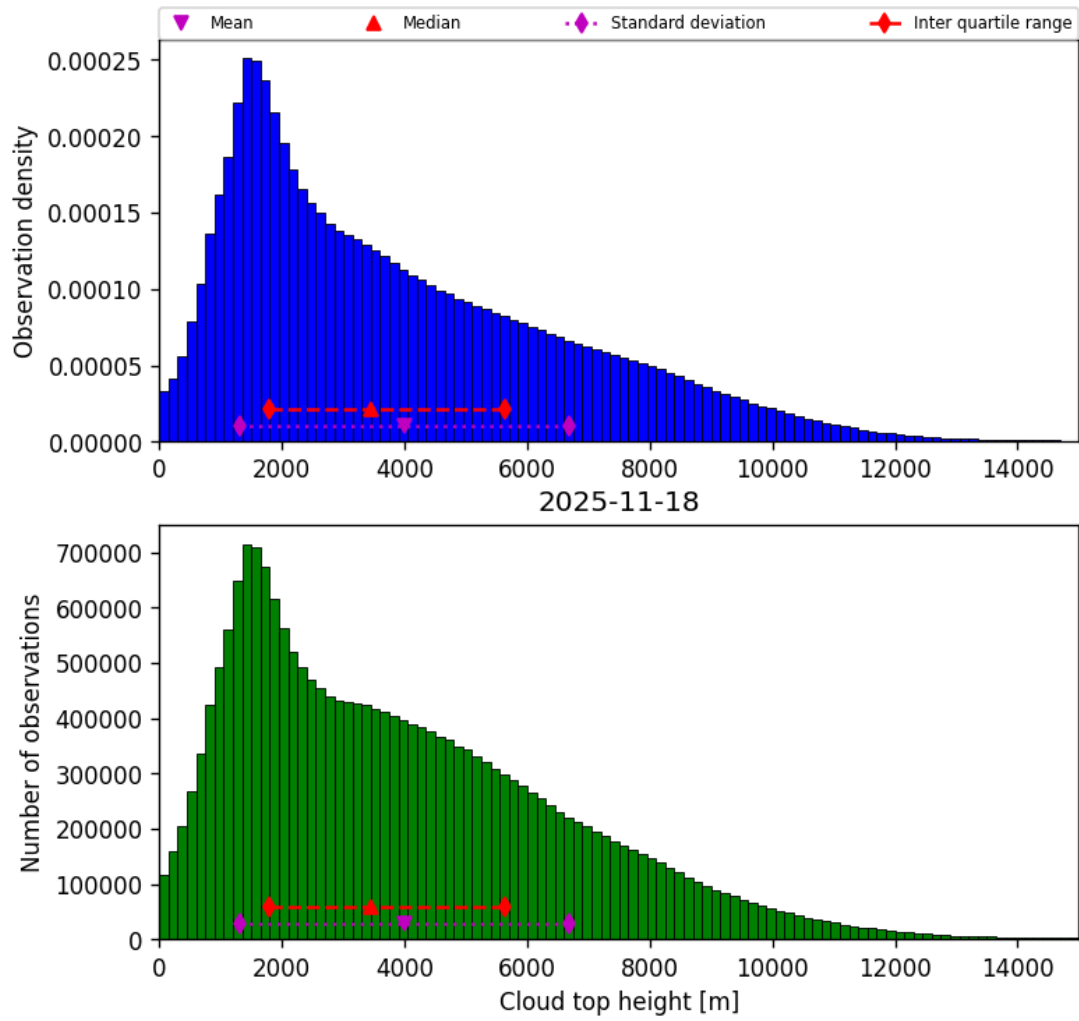
Figure 40: Histogram of “Cloud top height” for 2025-11-18 to 2025-11-19
