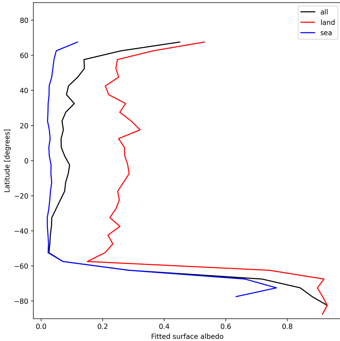
Figure 29: Zonal average of “Fitted surface albedo” for 2025-11-18 to 2025-11-19.
