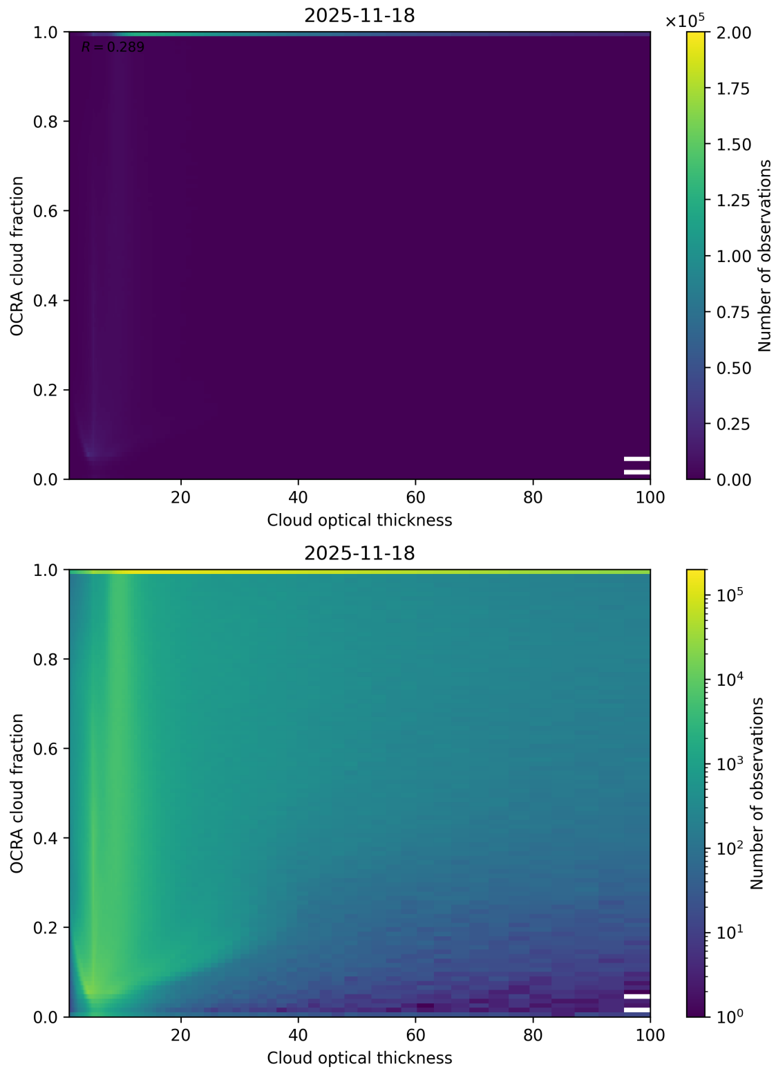
Figure 83: Scatter density plot of “Cloud optical thickness” against “OCRA cloud fraction” for 2025-11-18 to 2025-11-19.
