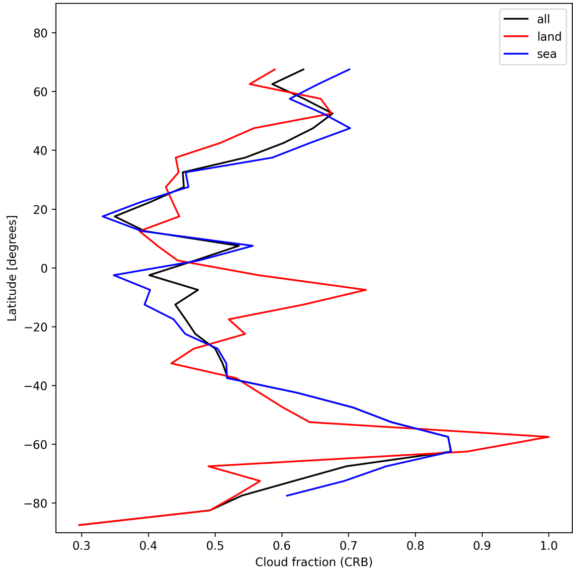
Figure 26: Zonal average of “Cloud fraction (CRB)” for 2025-11-18 to 2025-11-19.
