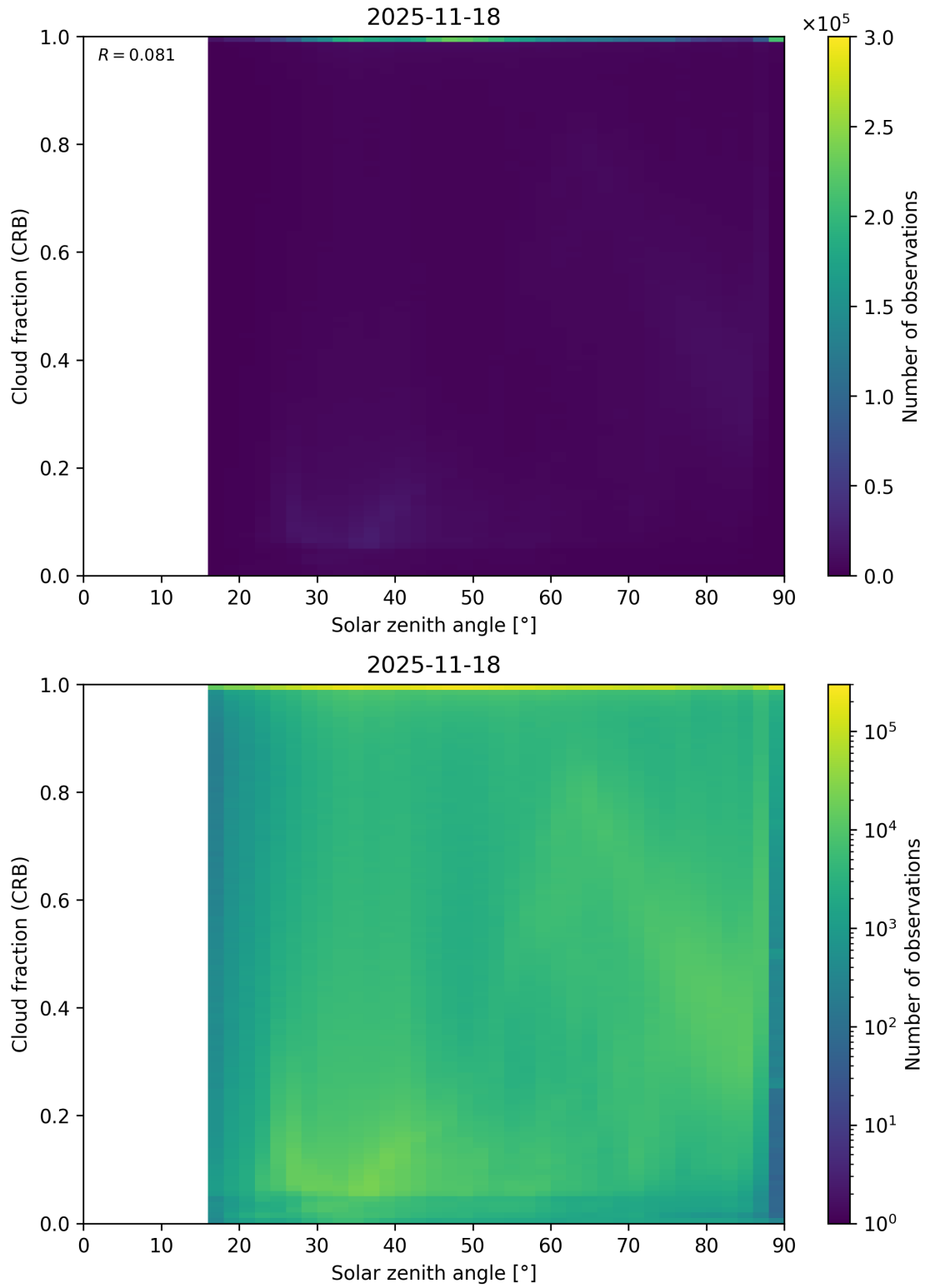
Figure 101: Scatter density plot of “Solar zenith angle” against “Cloud fraction (CRB)” for 2025-11-18 to 2025-11-19.
