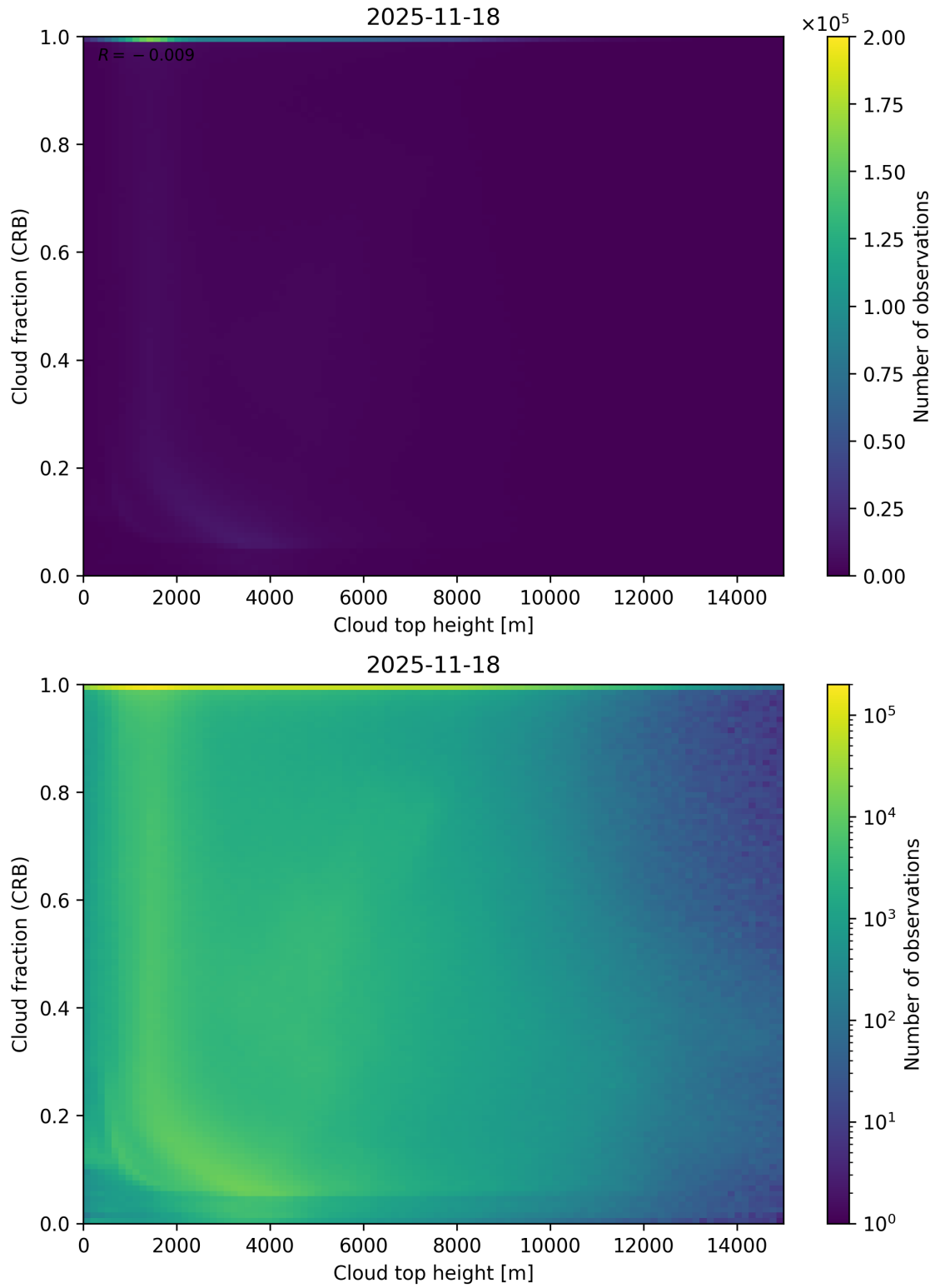
Figure 88: Scatter density plot of “Cloud top height” against “Cloud fraction (CRB)” for 2025-11-18 to 2025-11-19.
