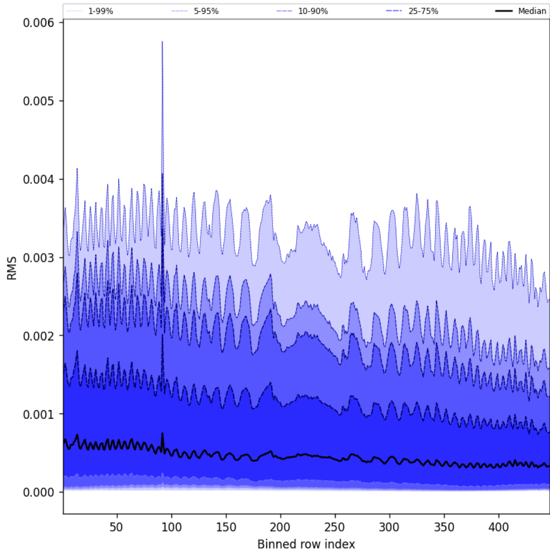
Figure 63: Along track statistics of “RMS” for 2025-11-18 to 2025-11-19
