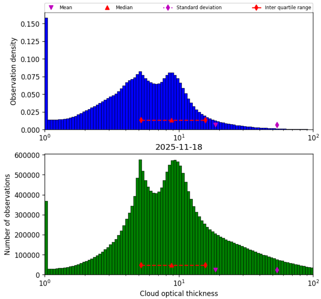
Figure 41: Histogram of “Cloud optical thickness” for 2025-11-18 to 2025-11-19
