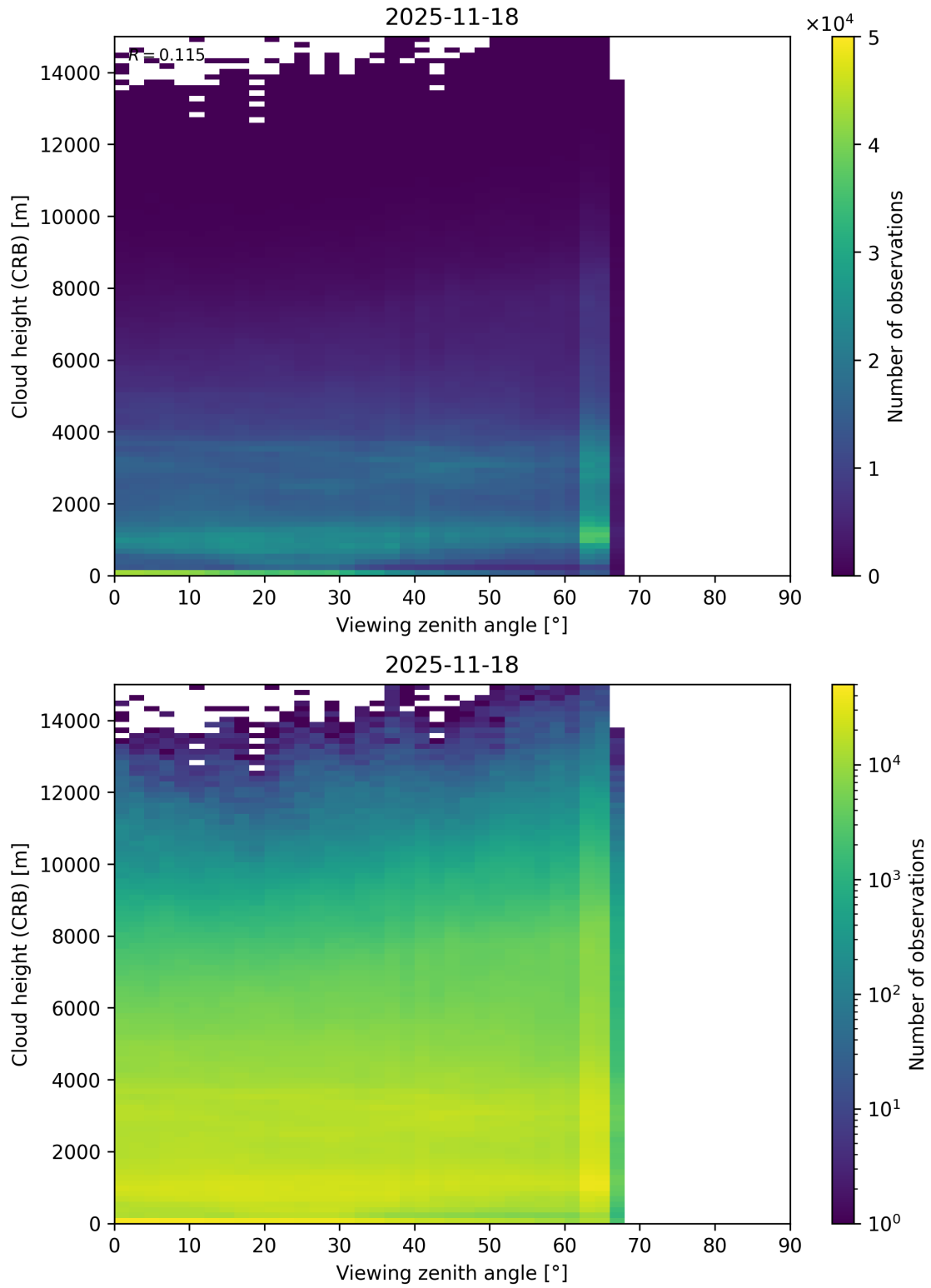
Figure 110: Scatter density plot of “Viewing zenith angle” against “Cloud height (CRB)” for 2025-11-18 to 2025-11-19.
