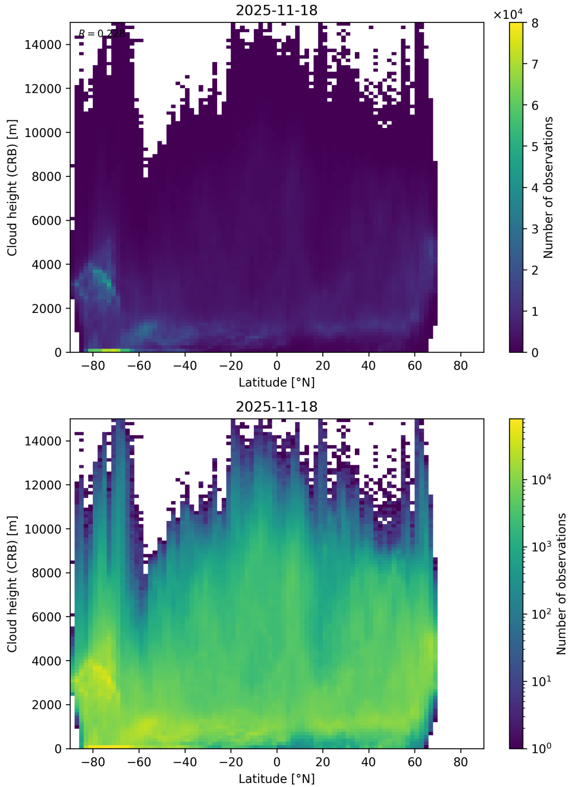
Figure 95: Scatter density plot of “Latitude” against “Cloud height (CRB)” for 2025-11-18 to 2025-11-19.
