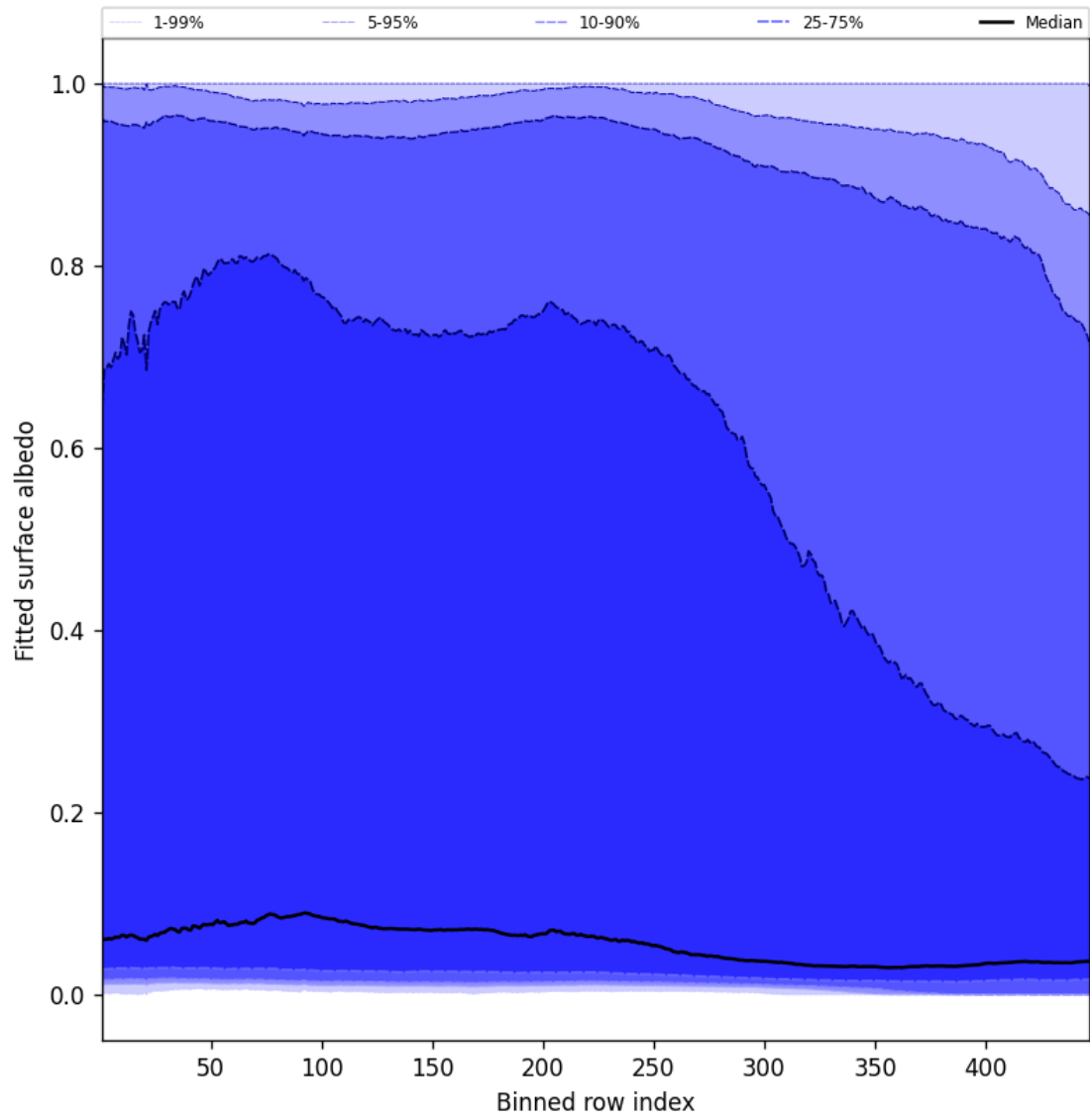
Figure 61: Along track statistics of “Fitted surface albedo” for 2025-11-18 to 2025-11-19
