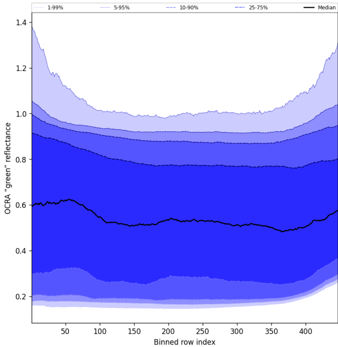
Figure 68: Along track statistics of "OCRA "green" reflectance" for 2025-11-18 to 2025-11-19
