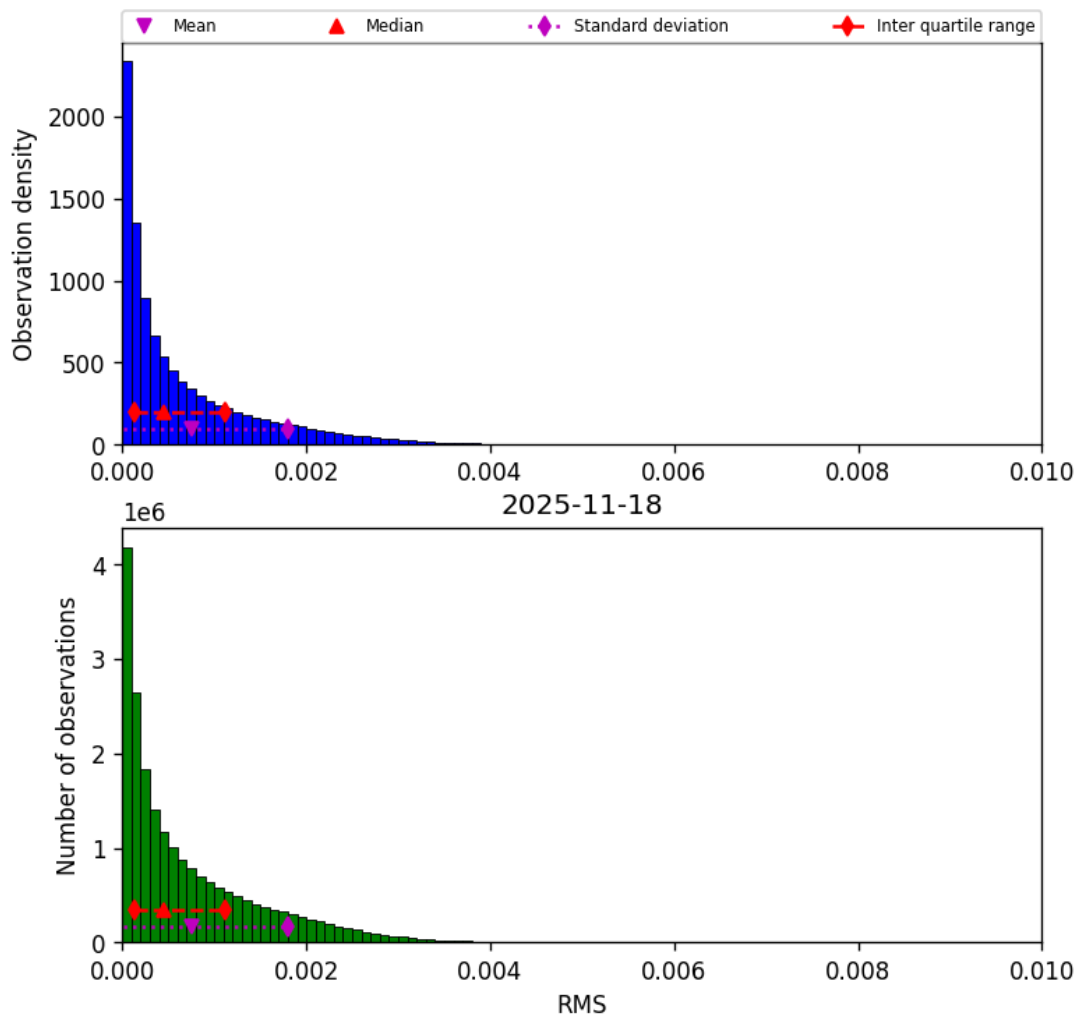
Figure 47: Histogram of “RMS” for 2025-11-18 to 2025-11-19
