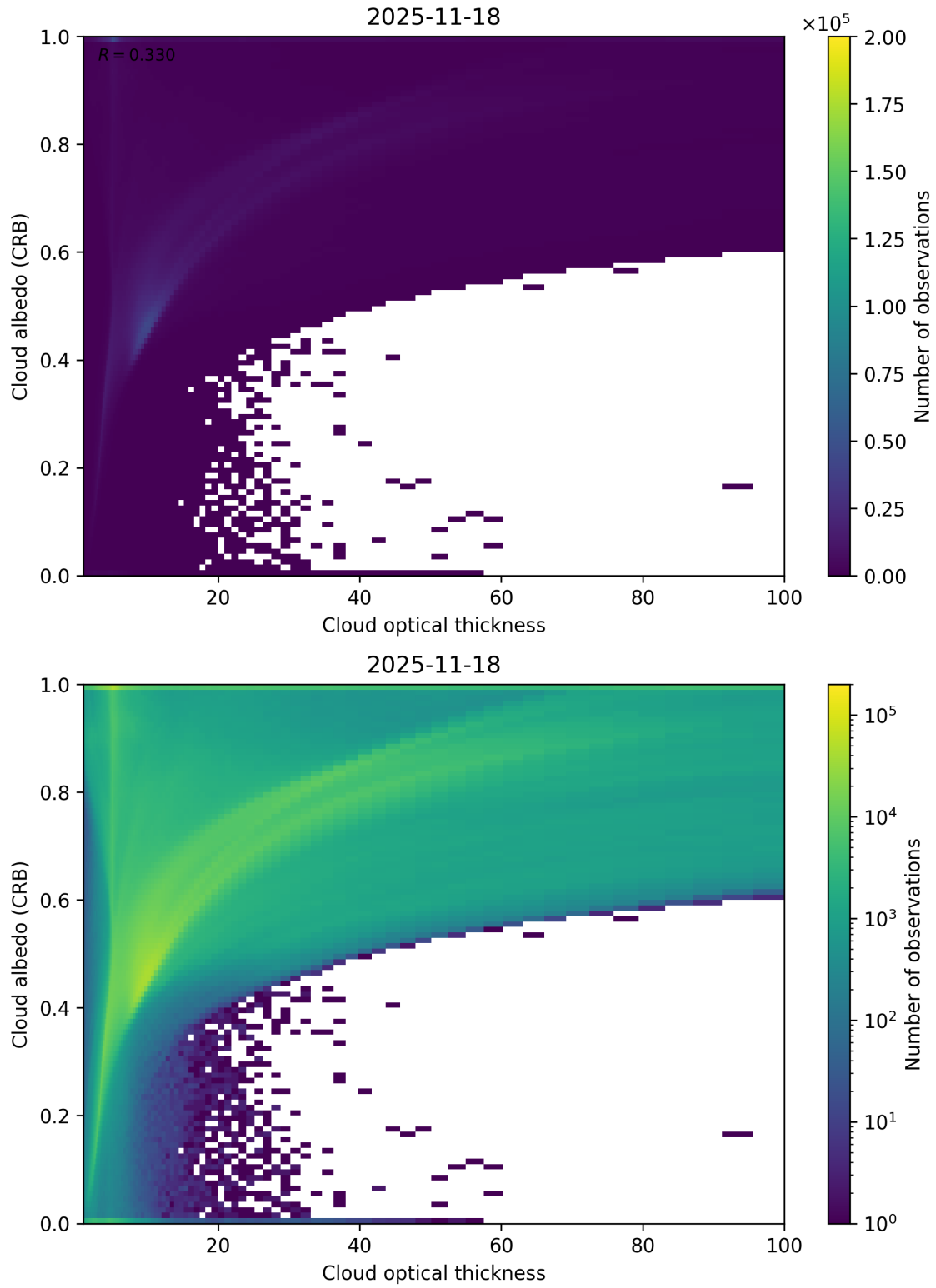
Figure 82: Scatter density plot of “Cloud optical thickness” against “Cloud albedo (CRB)” for 2025-11-18 to 2025-11-19.
