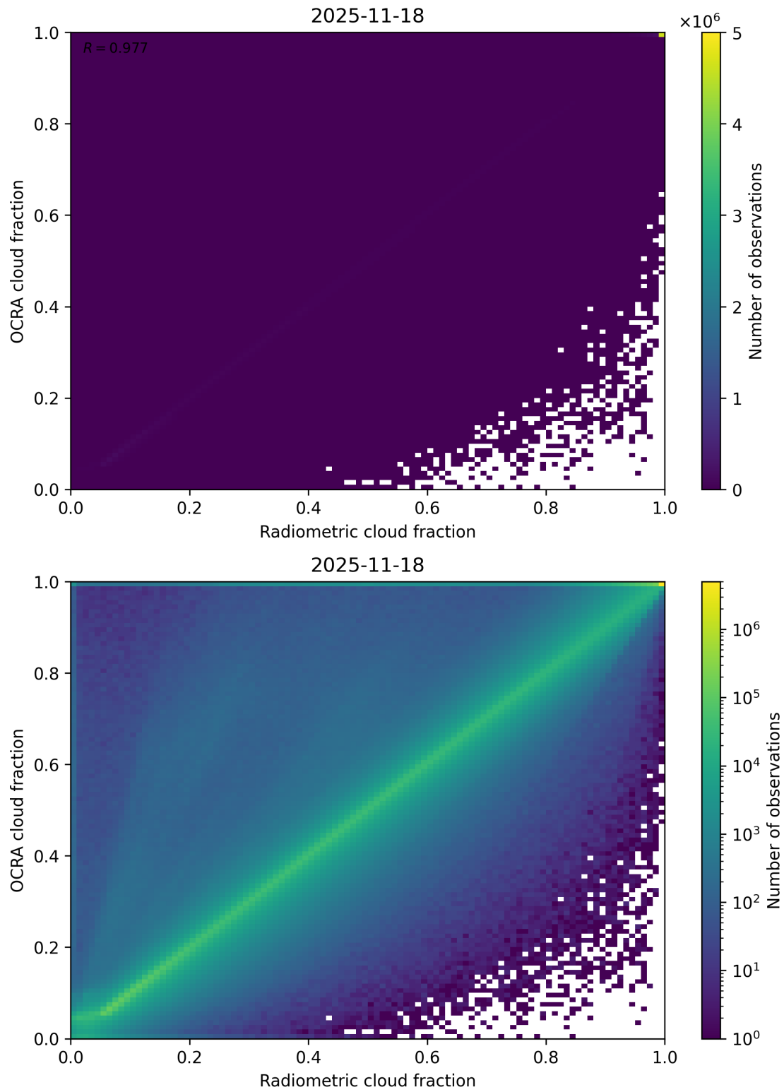
Figure 72: Scatter density plot of “Radiometric cloud fraction” against “OCRA cloud fraction” for 2025-11-18 to 2025-11-19.
