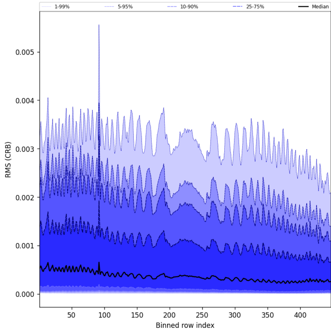
Figure 64: Along track statistics of “RMS (CRB)” for 2025-11-18 to 2025-11-19
