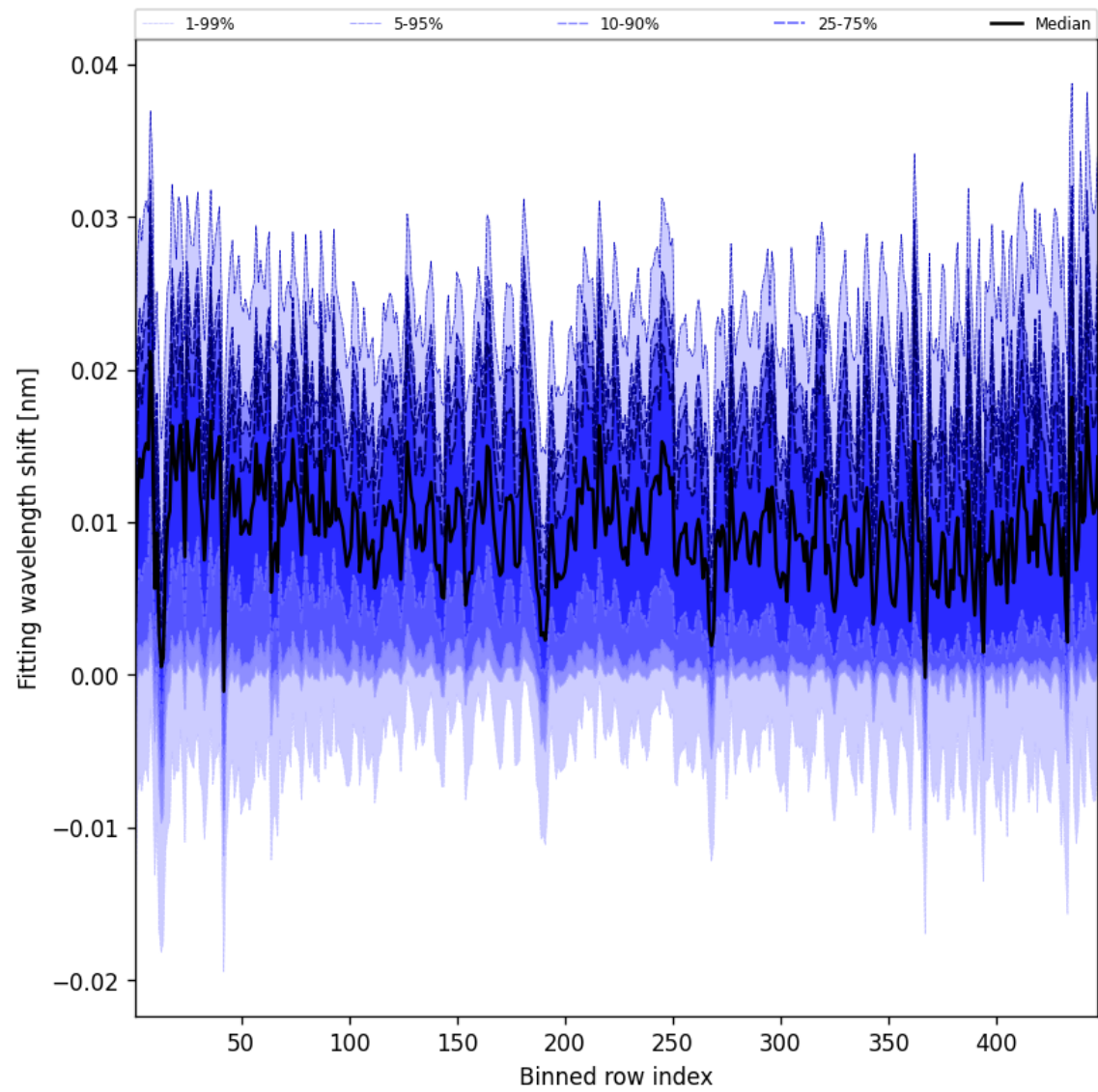
Figure 65: Along track statistics of “Fitting wavelength shift” for 2025-11-18 to 2025-11-19
