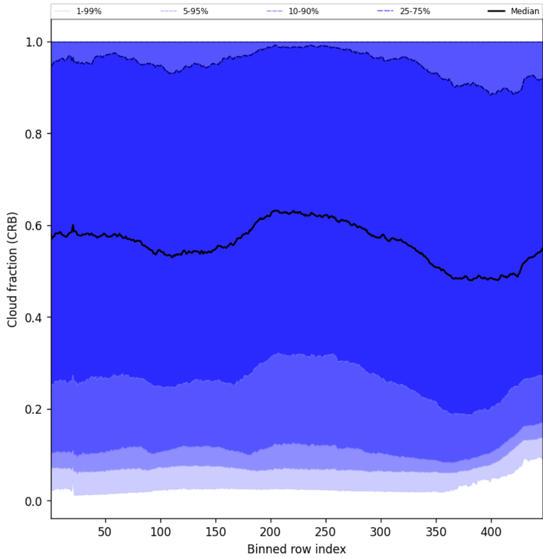
Figure 58: Along track statistics of “Cloud fraction (CRB)” for 2025-11-18 to 2025-11-19
