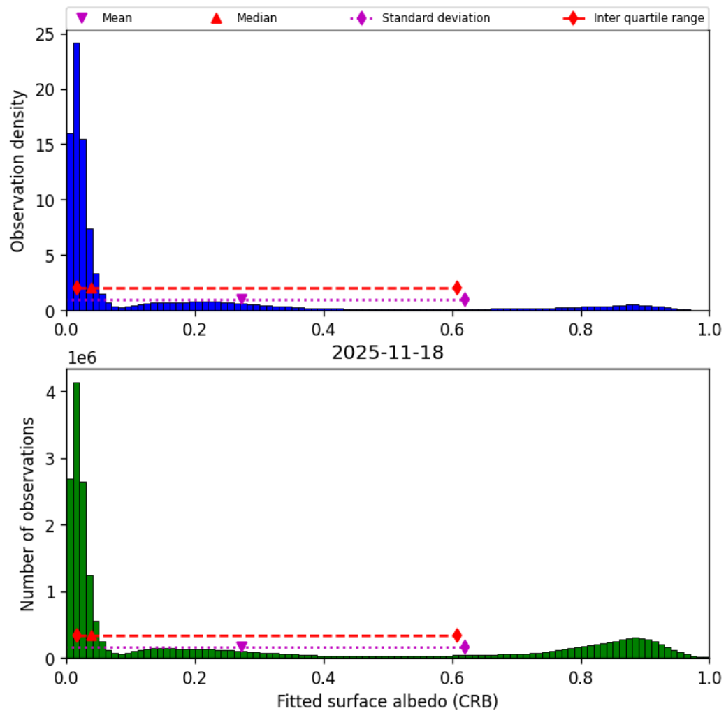
Figure 46: Histogram of “Fitted surface albedo (CRB)” for 2025-11-18 to 2025-11-19
