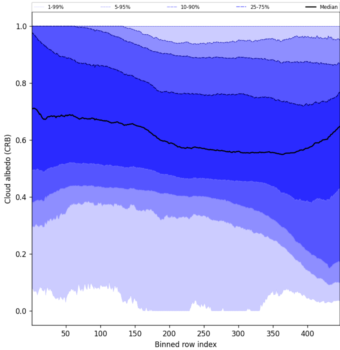
Figure 60: Along track statistics of “Cloud albedo (CRB)” for 2025-11-18 to 2025-11-19
