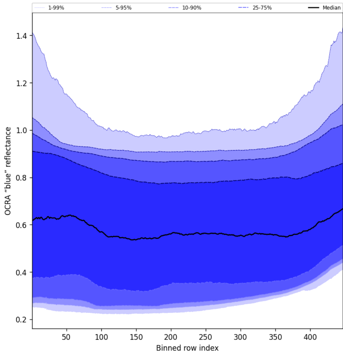
Figure 67: Along track statistics of “OCRA “blue” reflectance” for 2025-11-18 to 2025-11-19
