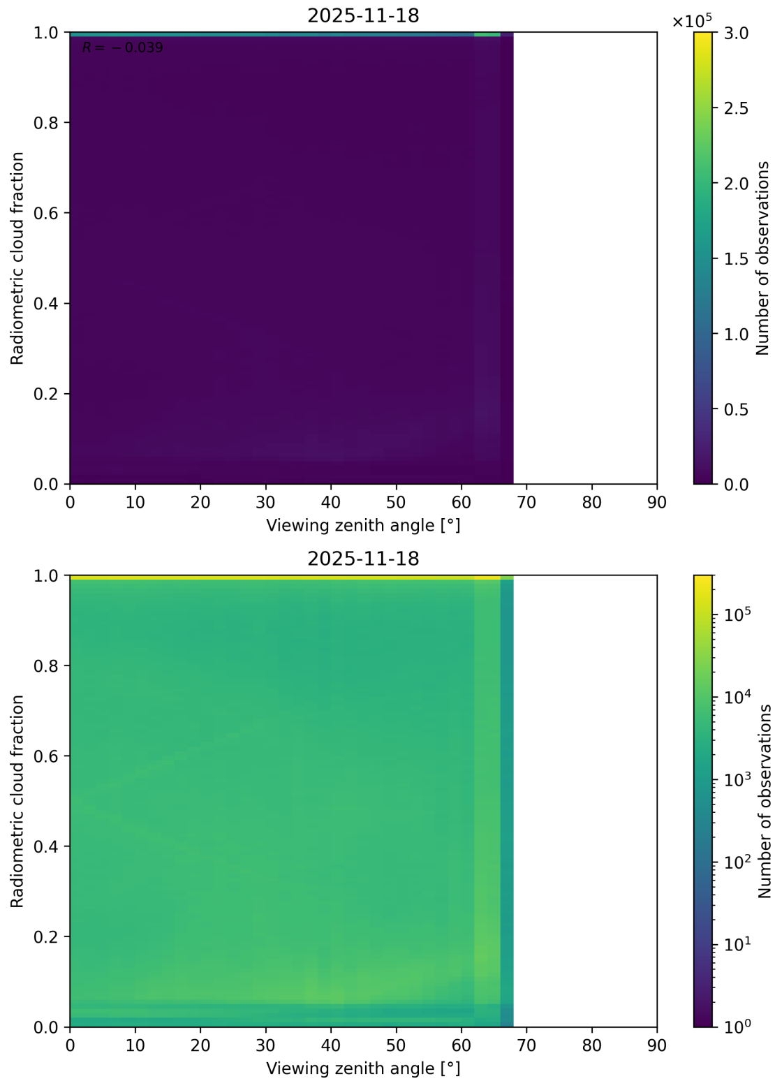
Figure 107: Scatter density plot of “Viewing zenith angle” against “Radiometric cloud fraction” for 2025-11-18 to 2025-11-19.
