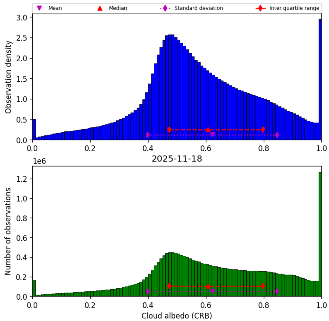
Figure 44: Histogram of “Cloud albedo (CRB)” for 2025-11-18 to 2025-11-19
