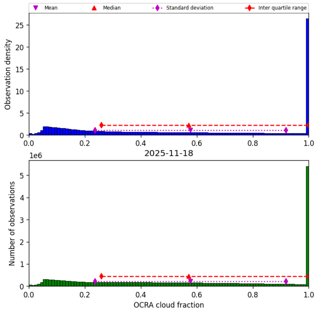
Figure 50: Histogram of “OCRA cloud fraction” for 2025-11-18 to 2025-11-19
