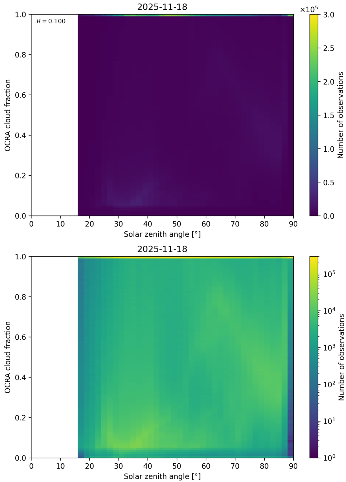
Figure 100: Scatter density plot of “Solar zenith angle” against “OCRA cloud fraction” for 2025-11-18 to 2025-11-19.
