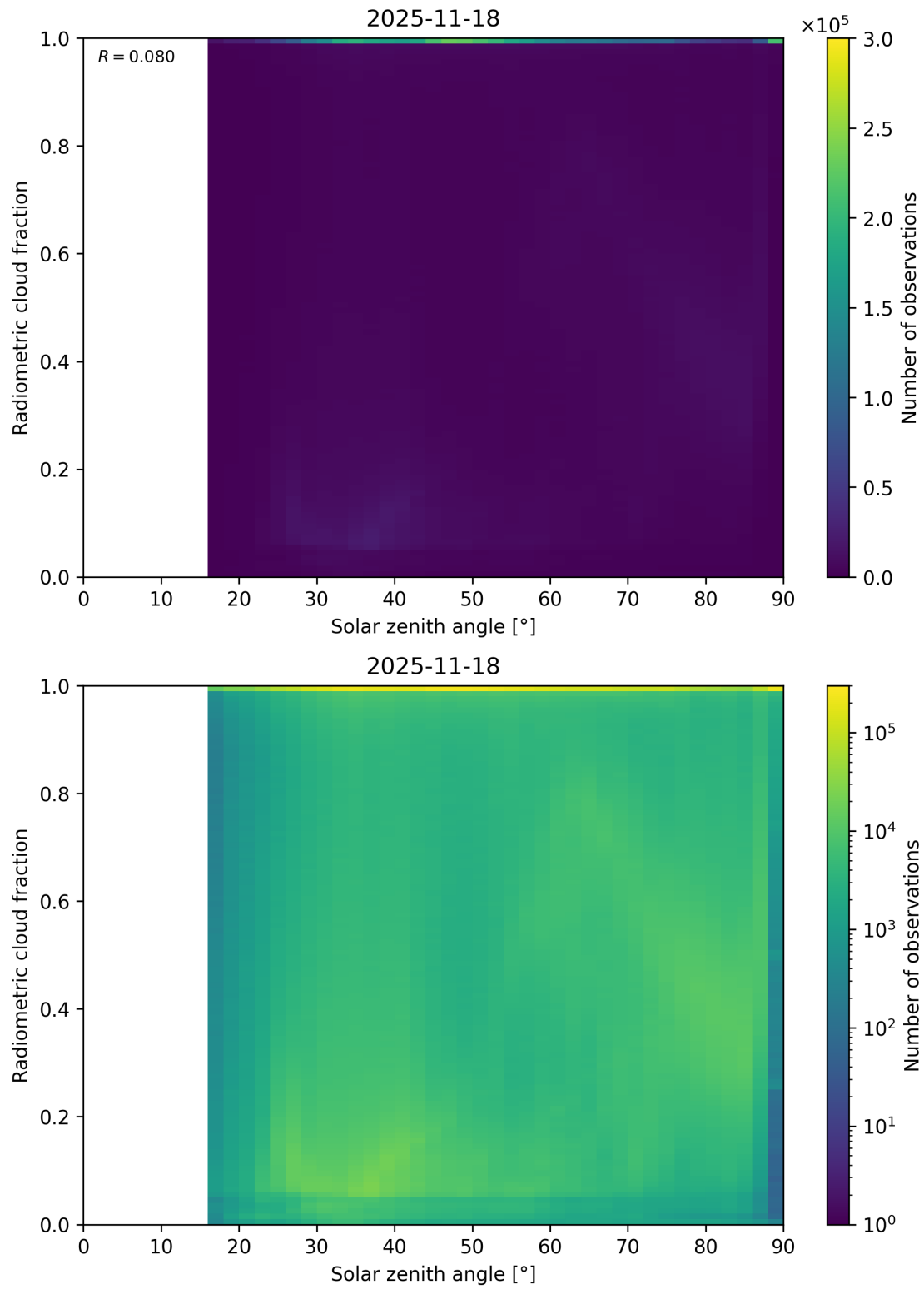
Figure 99: Scatter density plot of “Solar zenith angle” against “Radiometric cloud fraction” for 2025-11-18 to 2025-11-19.
