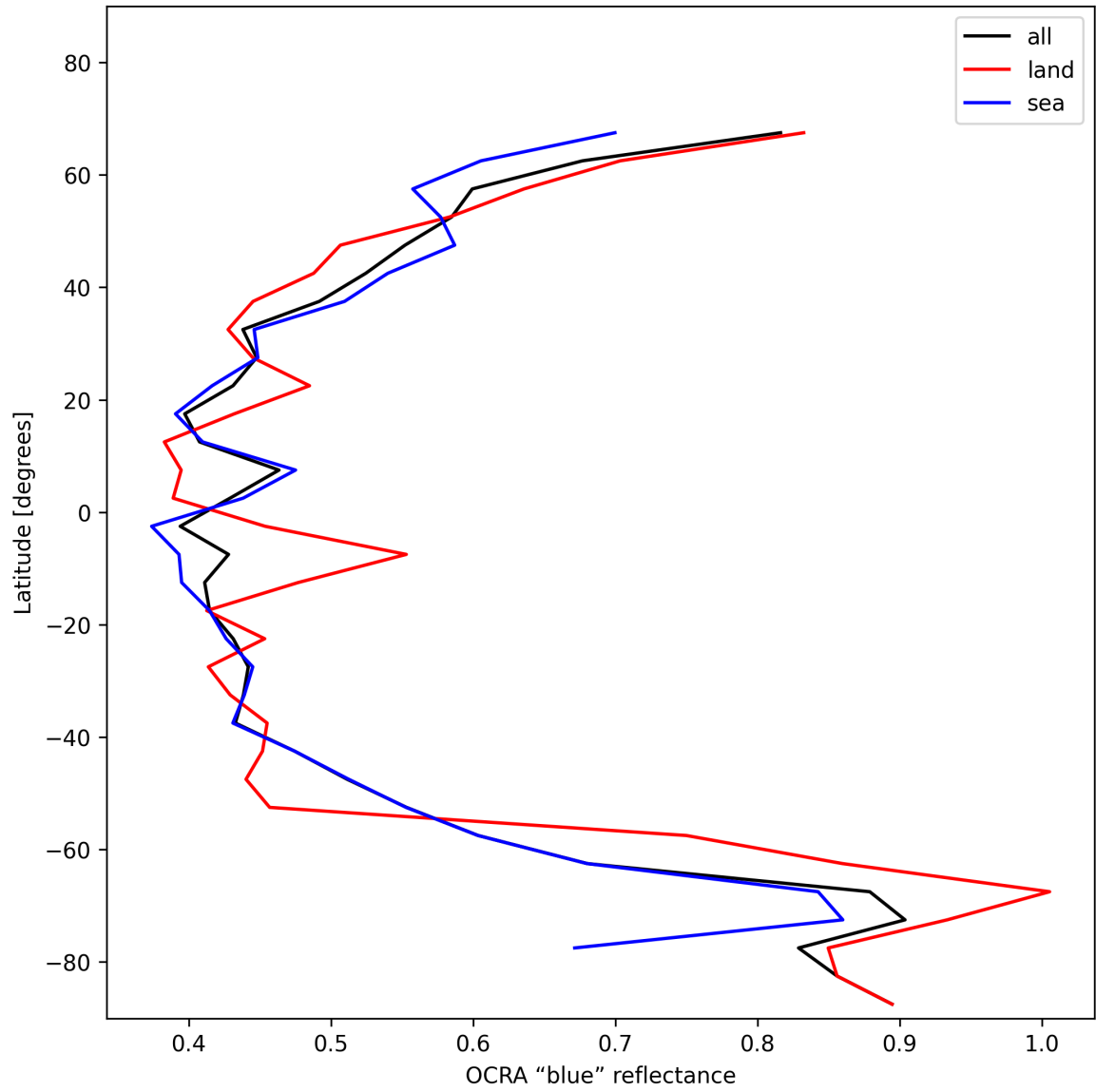
Figure 35: Zonal average of “OCRA “blue” reflectance” for 2025-11-18 to 2025-11-19.
