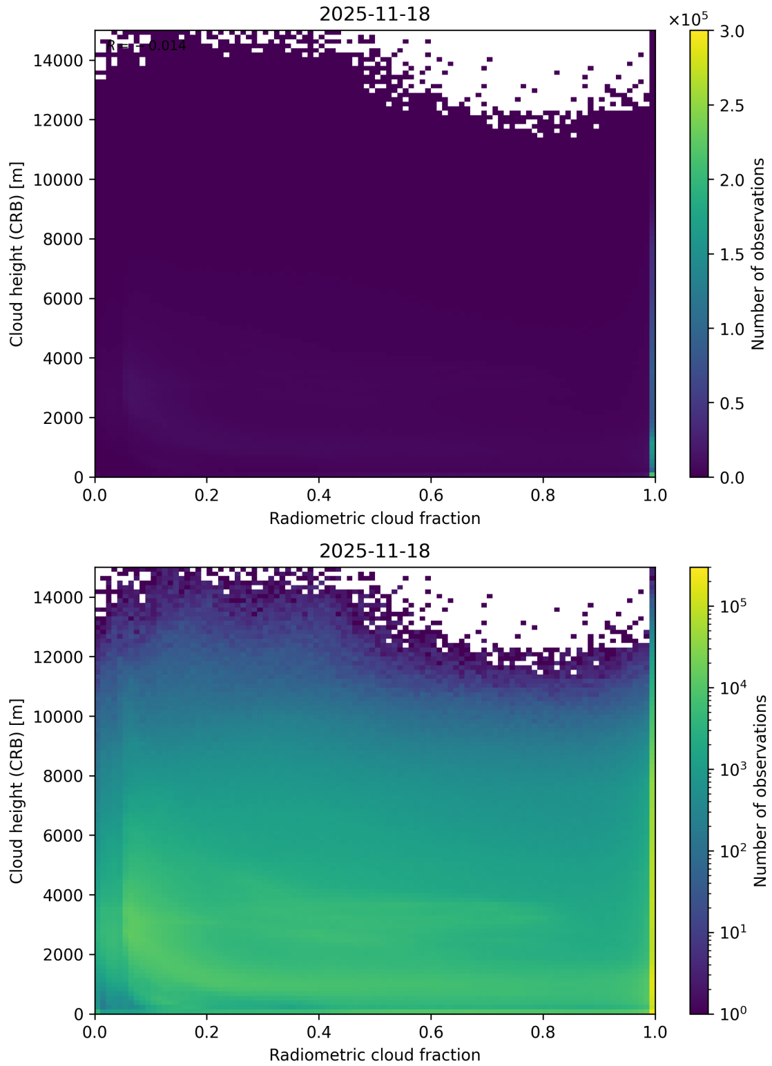
Figure 74: Scatter density plot of “Radiometric cloud fraction” against “Cloud height (CRB)” for 2025-11-18 to 2025-11-19.
