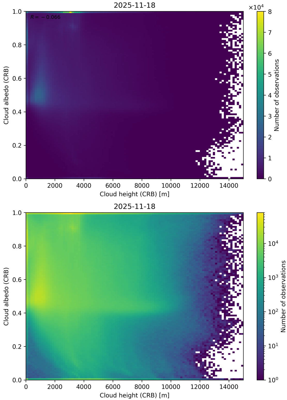
Figure 80: Scatter density plot of “Cloud height (CRB)” against “Cloud albedo (CRB)” for 2025-11-18 to 2025-11-19.
