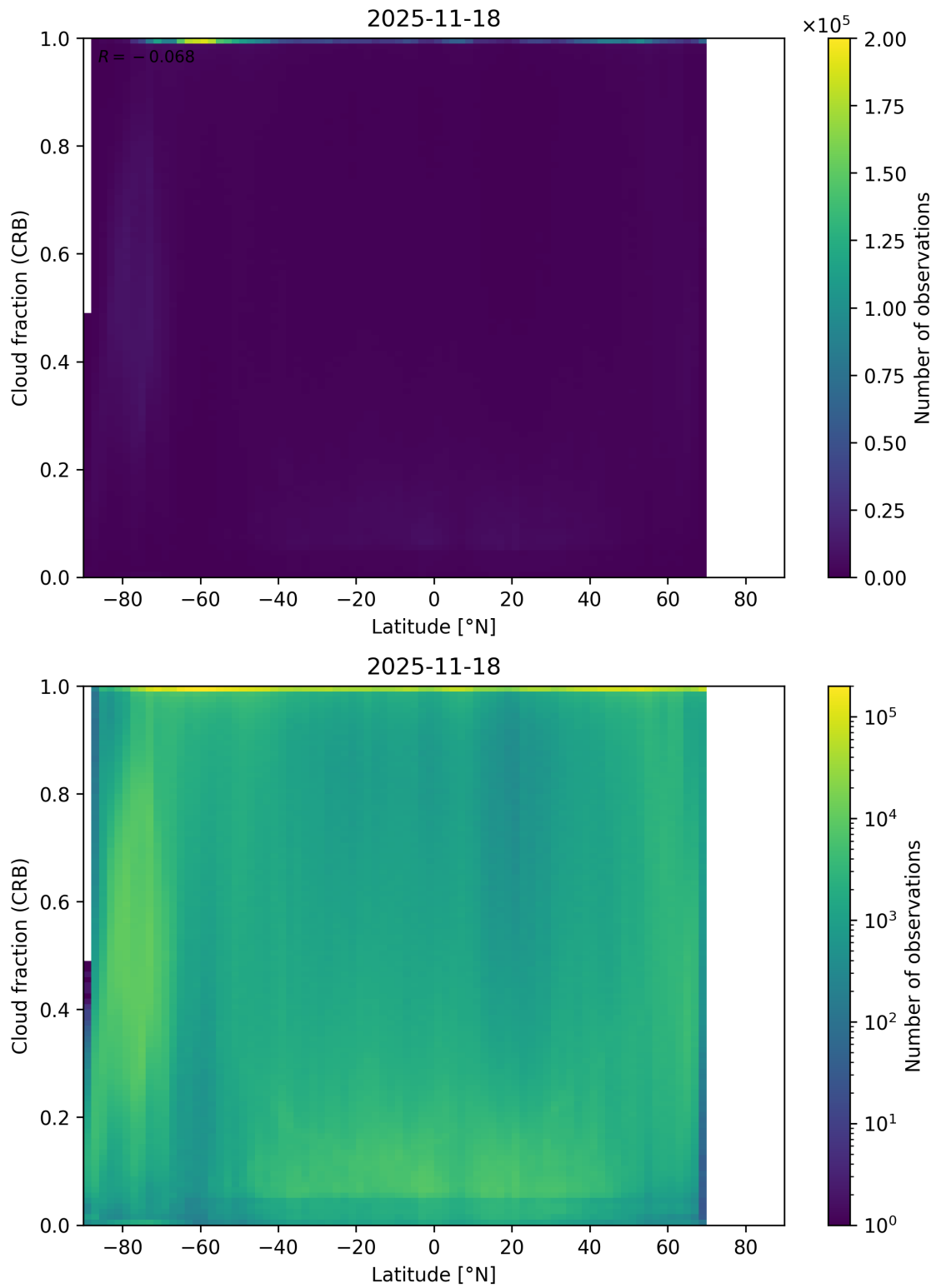
Figure 94: Scatter density plot of “Latitude” against “Cloud fraction (CRB)” for 2025-11-18 to 2025-11-19.
