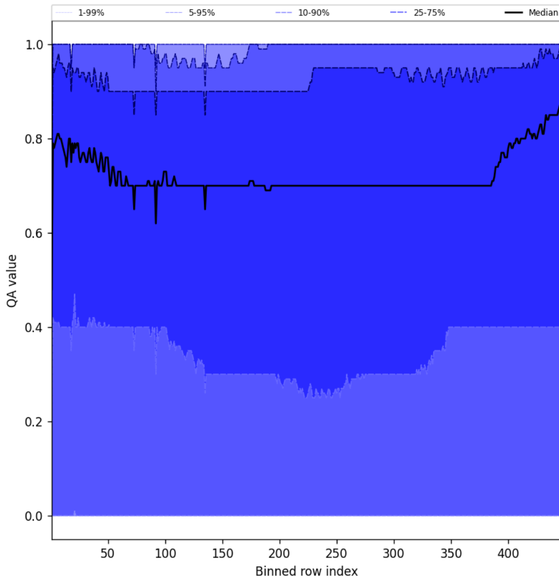
Figure 54: Along track statistics of “QA value” for 2025-11-18 to 2025-11-19
