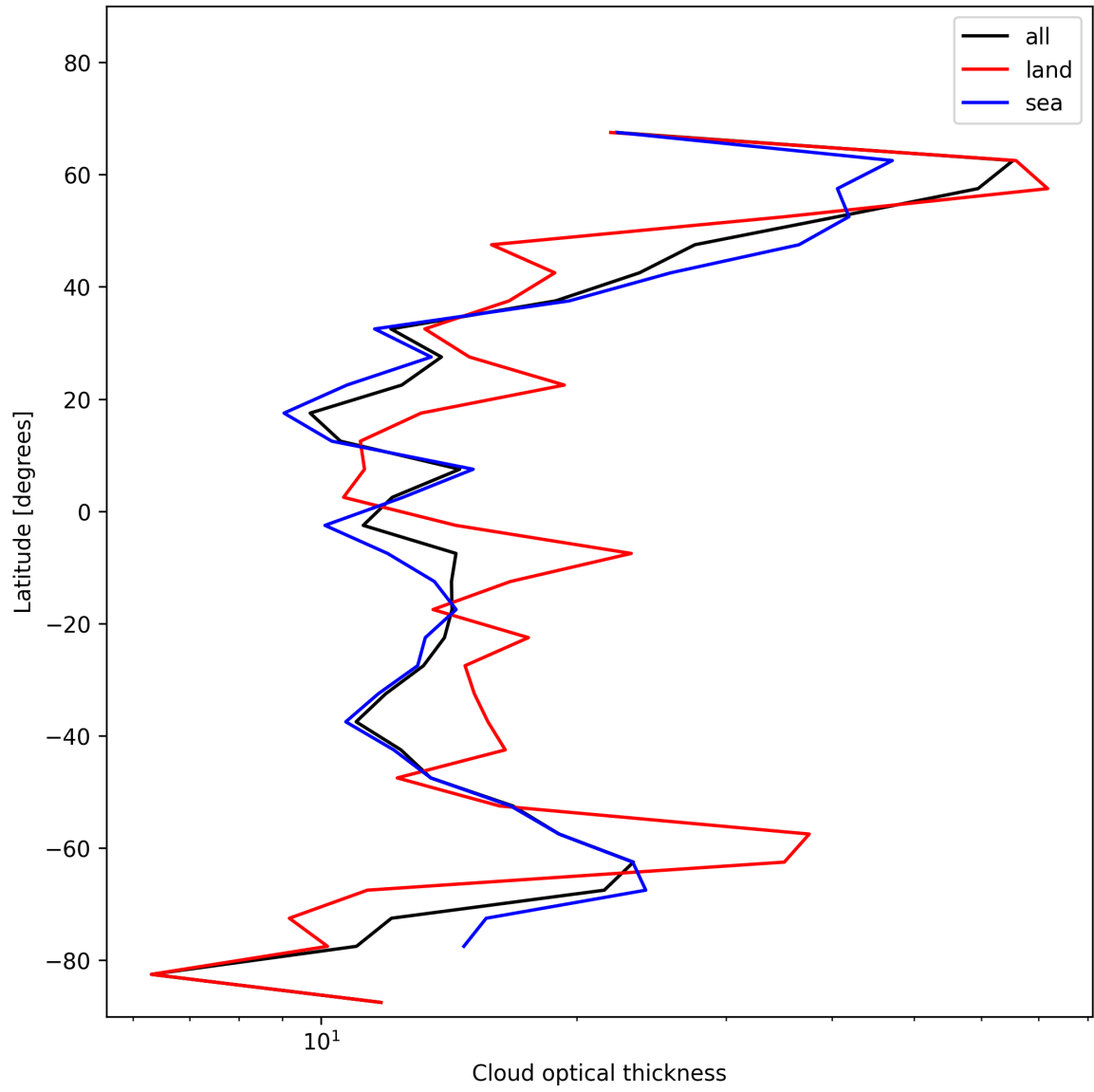
Figure 25: Zonal average of “Cloud optical thickness” for 2025-11-18 to 2025-11-19.
