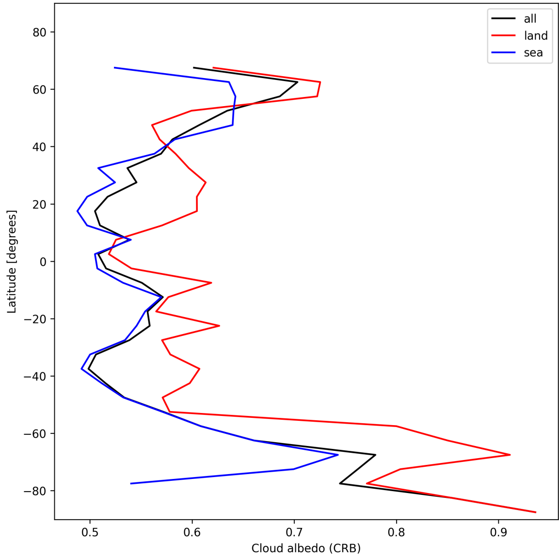
Figure 28: Zonal average of “Cloud albedo (CRB)” for 2025-11-18 to 2025-11-19.
