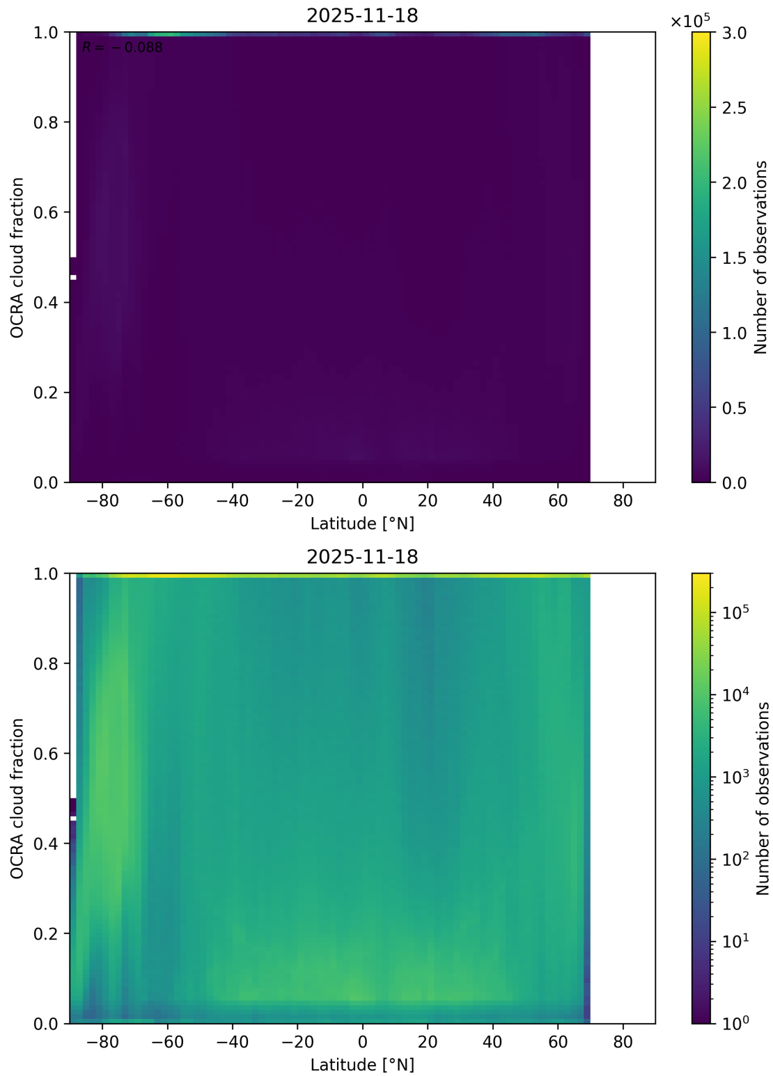
Figure 93: Scatter density plot of “Latitude” against “OCRA cloud fraction” for 2025-11-18 to 2025-11-19.
