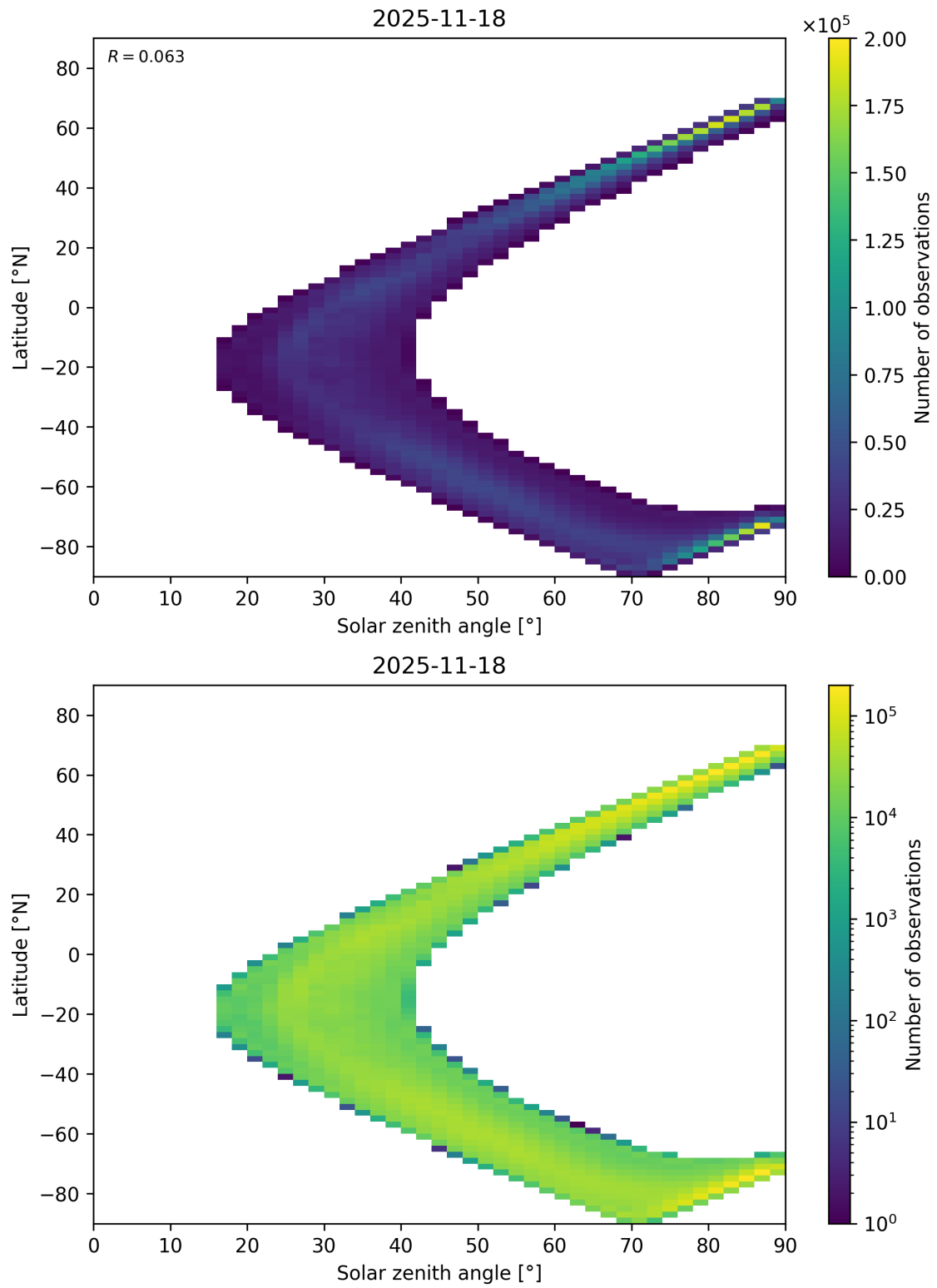
Figure 105: Scatter density plot of “Solar zenith angle” against “Latitude” for 2025-11-18 to 2025-11-19.
