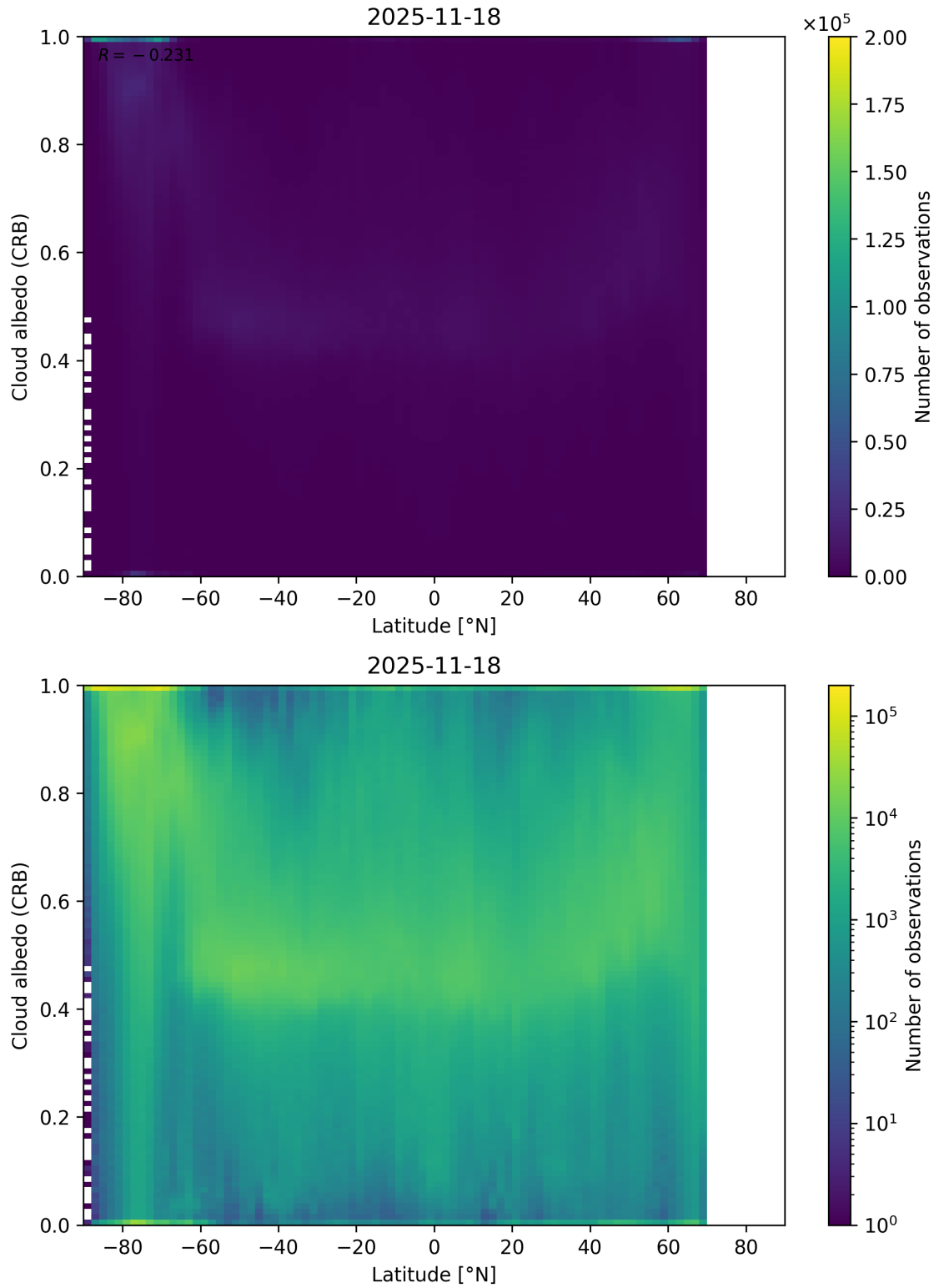
Figure 91: Scatter density plot of “Latitude” against “Cloud albedo (CRB)” for 2025-11-18 to 2025-11-19.
