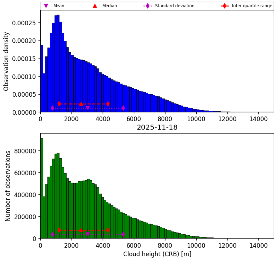
Figure 43: Histogram of “Cloud height (CRB)” for 2025-11-18 to 2025-11-19
