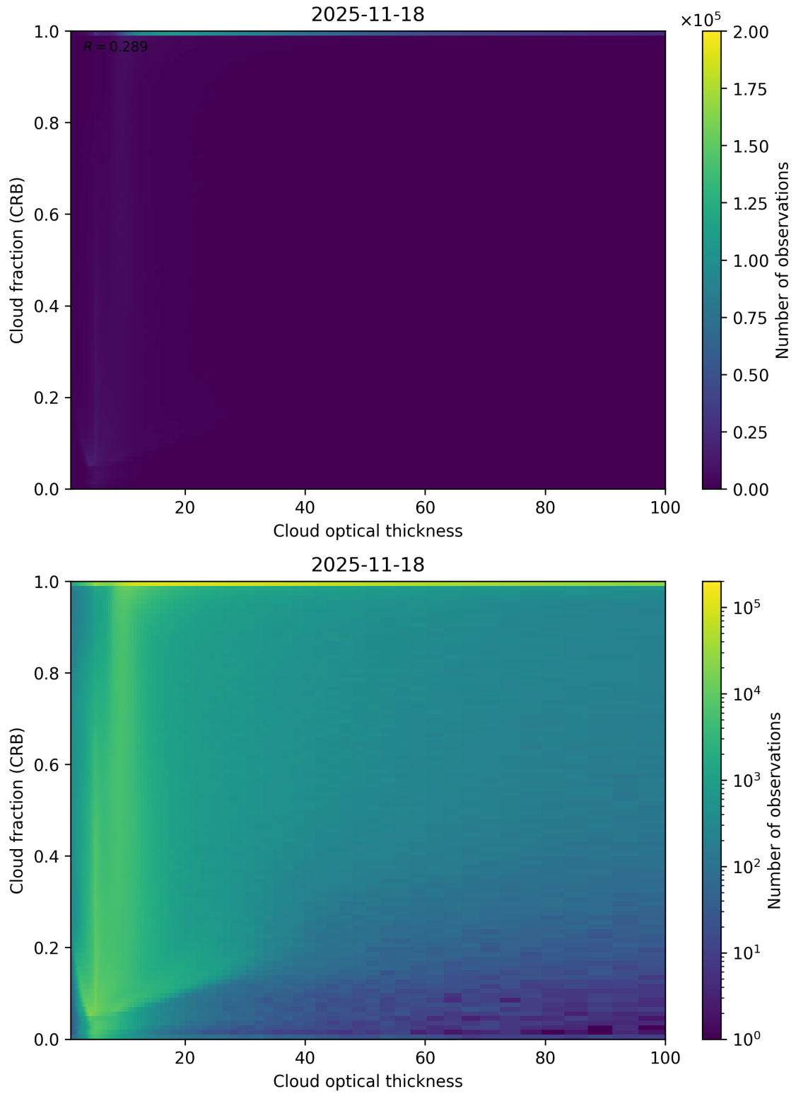
Figure 84: Scatter density plot of “Cloud optical thickness” against “Cloud fraction (CRB)” for 2025-11-18 to 2025-11-19.
