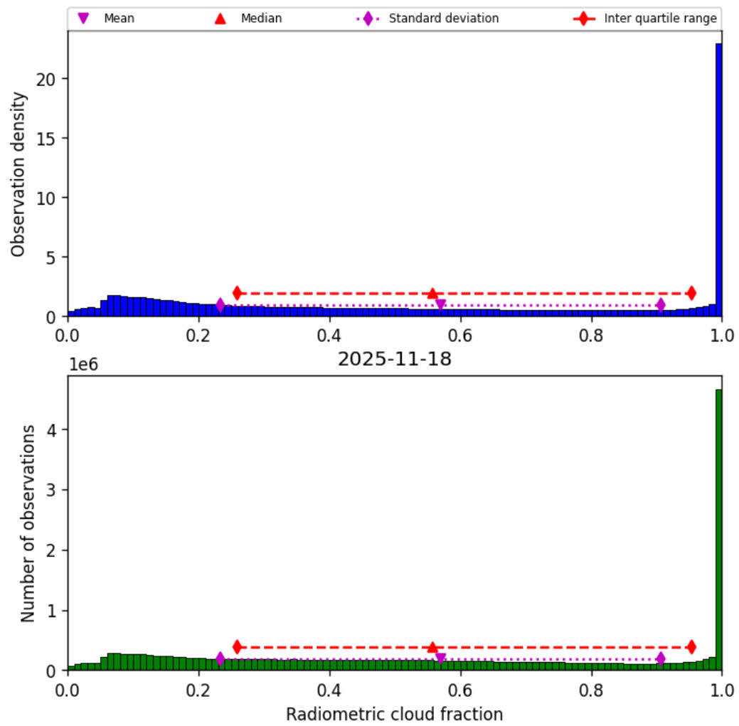
Figure 39: Histogram of “Radiometric cloud fraction” for 2025-11-18 to 2025-11-19
