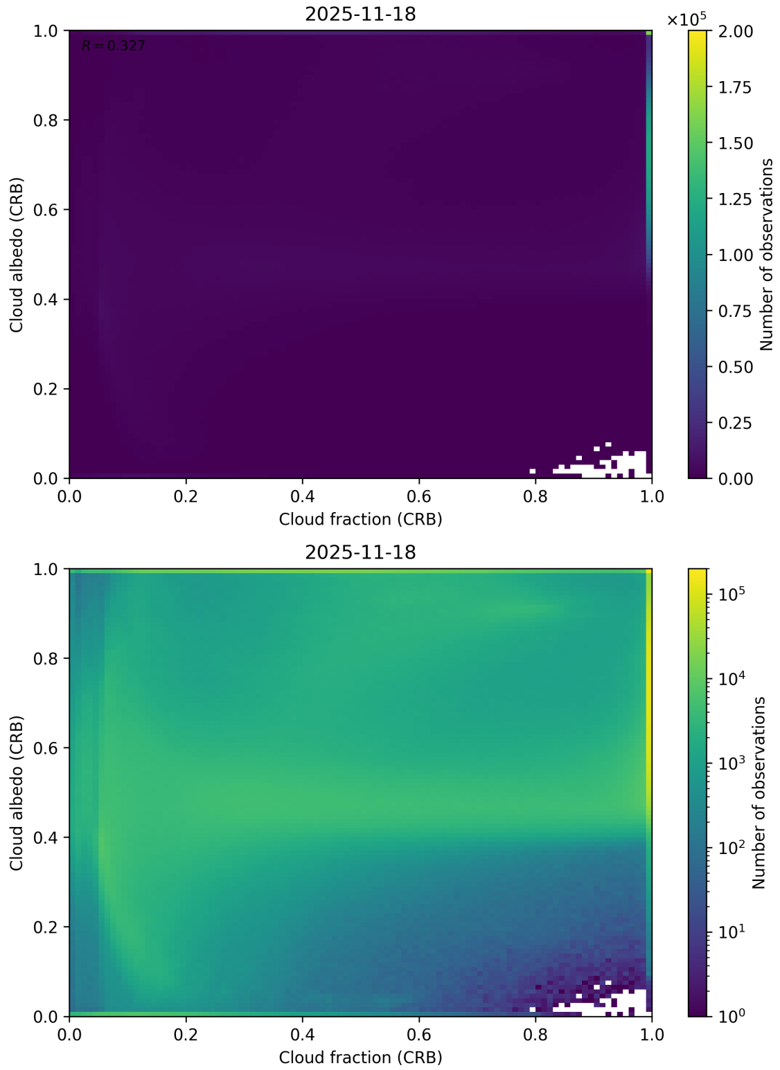
Figure 77: Scatter density plot of “Cloud fraction (CRB)” against “Cloud albedo (CRB)” for 2025-11-18 to 2025-11-19.
