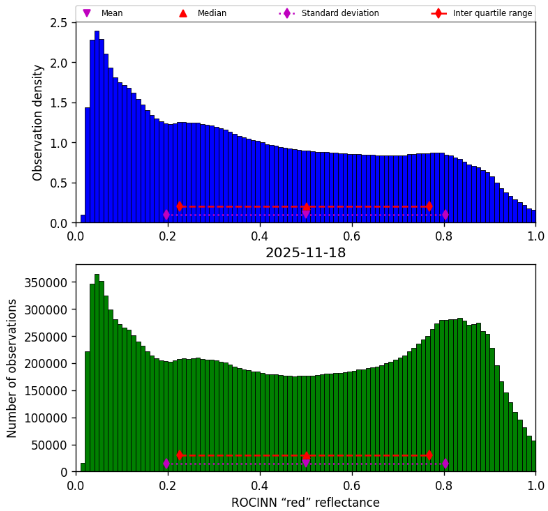
Figure 53: Histogram of “ROCINN “red” reflectance” for 2025-11-18 to 2025-11-19
