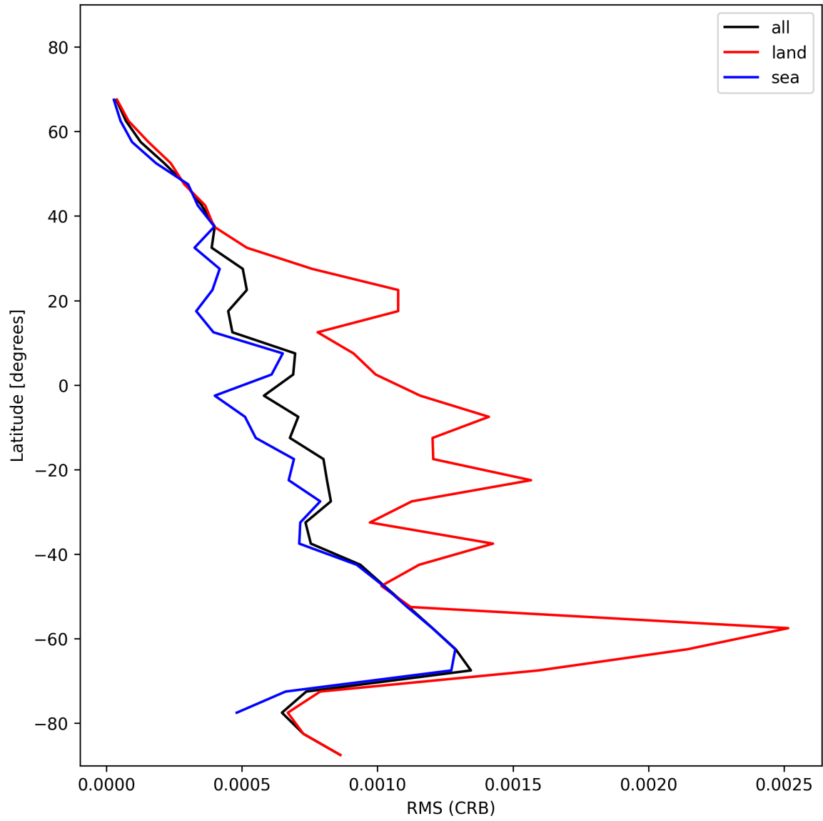
Figure 32: Zonal average of “RMS (CRB)” for 2025-11-18 to 2025-11-19.
