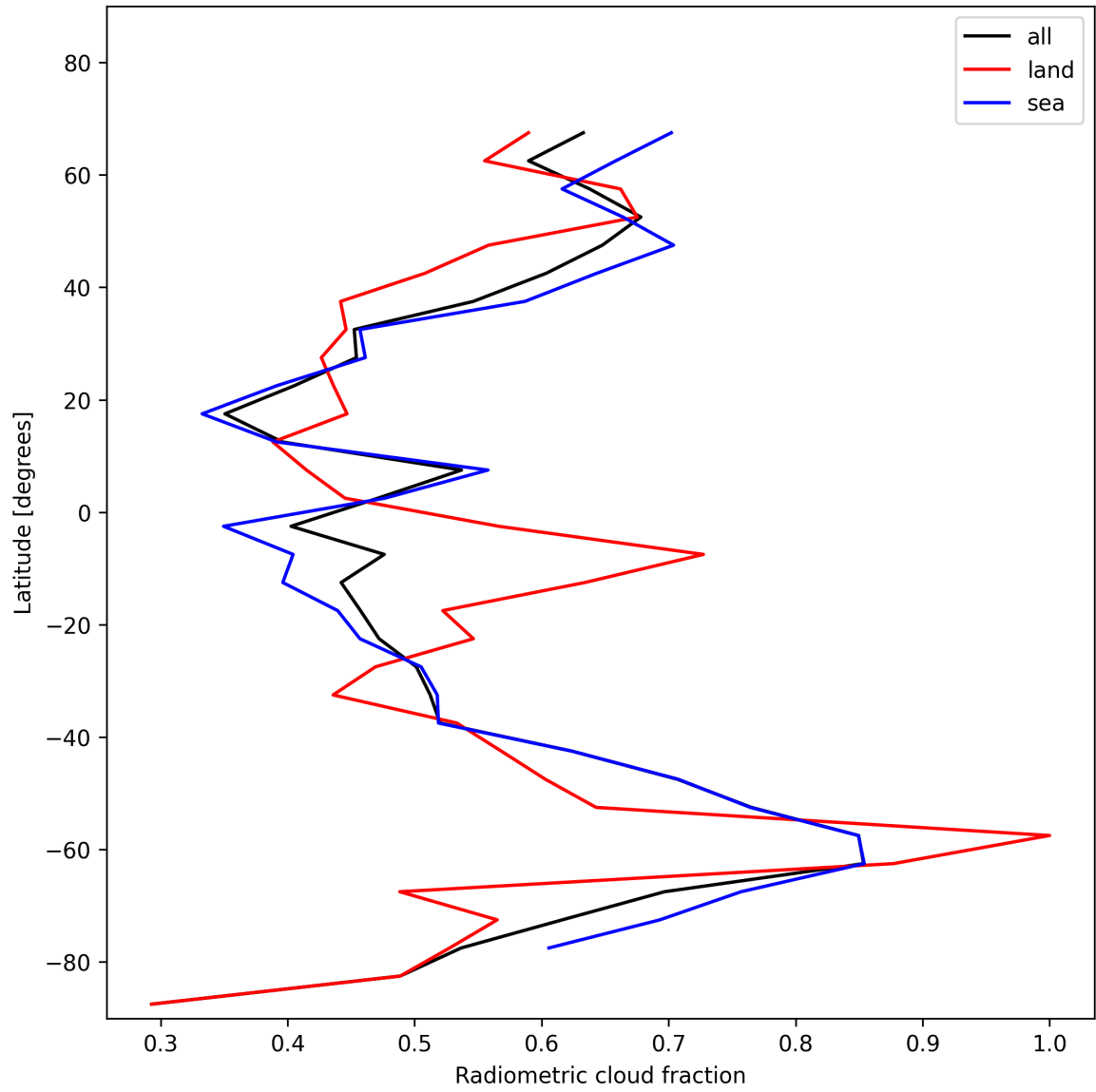
Figure 23: Zonal average of “Radiometric cloud fraction” for 2025-11-18 to 2025-11-19.
