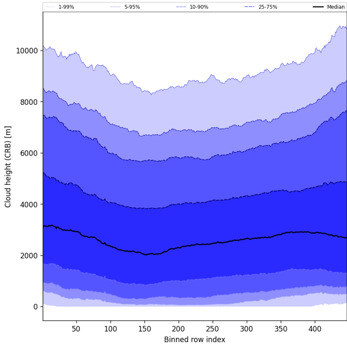
Figure 59: Along track statistics of “Cloud height (CRB)” for 2025-11-18 to 2025-11-19
