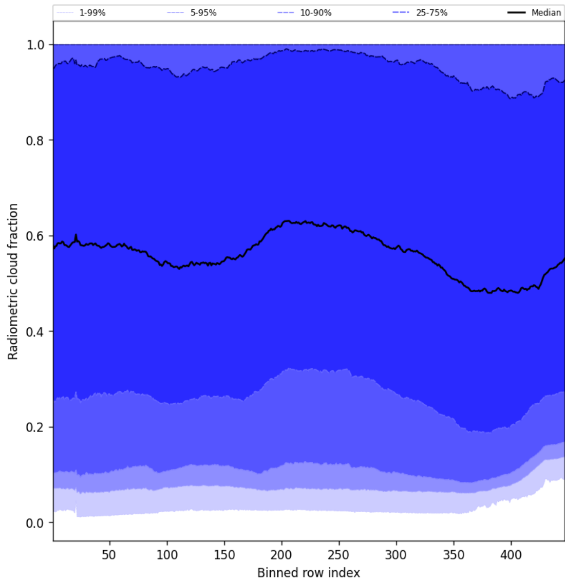
Figure 55: Along track statistics of “Radiometric cloud fraction” for 2025-11-18 to 2025-11-19
