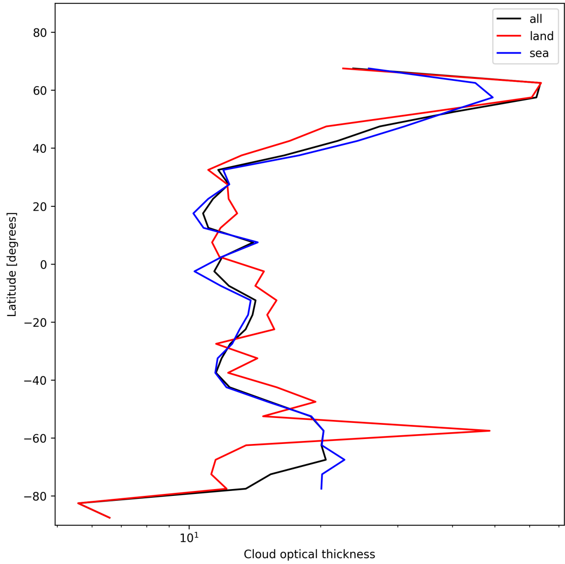
Figure 25: Zonal average of “Cloud optical thickness” for 2025-11-18 to 2025-11-20.
