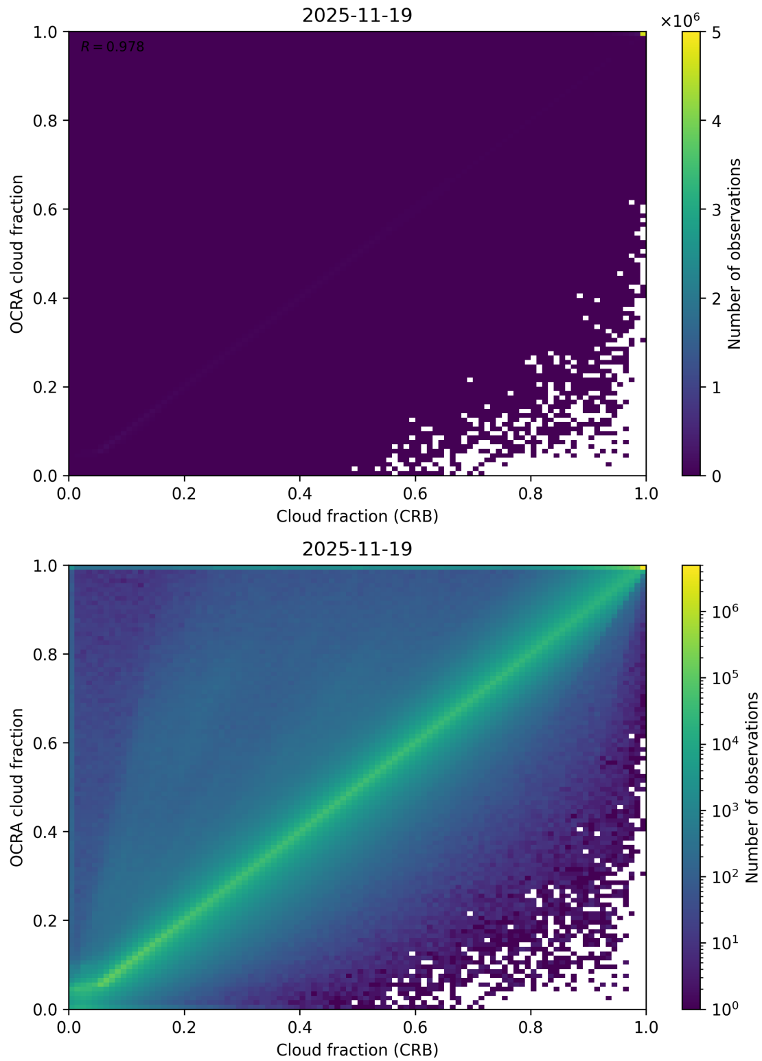
Figure 78: Scatter density plot of “Cloud fraction (CRB)” against “OCRA cloud fraction” for 2025-11-18 to 2025-11-20.
