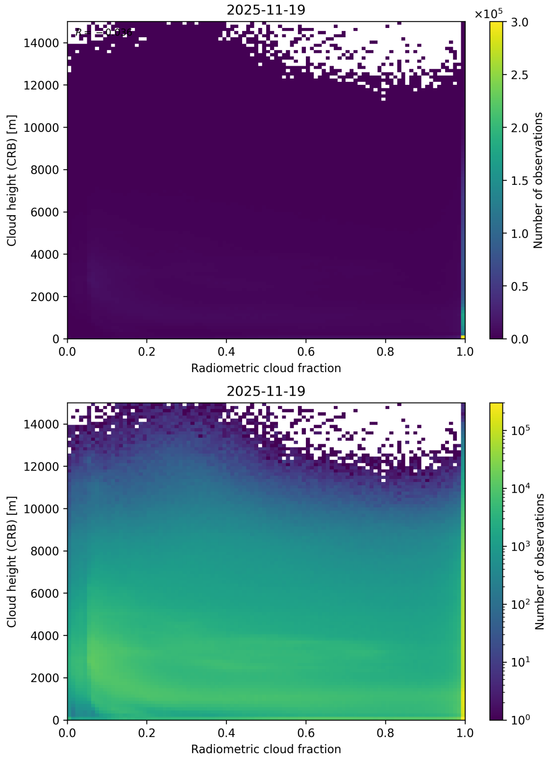
Figure 74: Scatter density plot of “Radiometric cloud fraction” against “Cloud height (CRB)” for 2025-11-18 to 2025-11-20.
