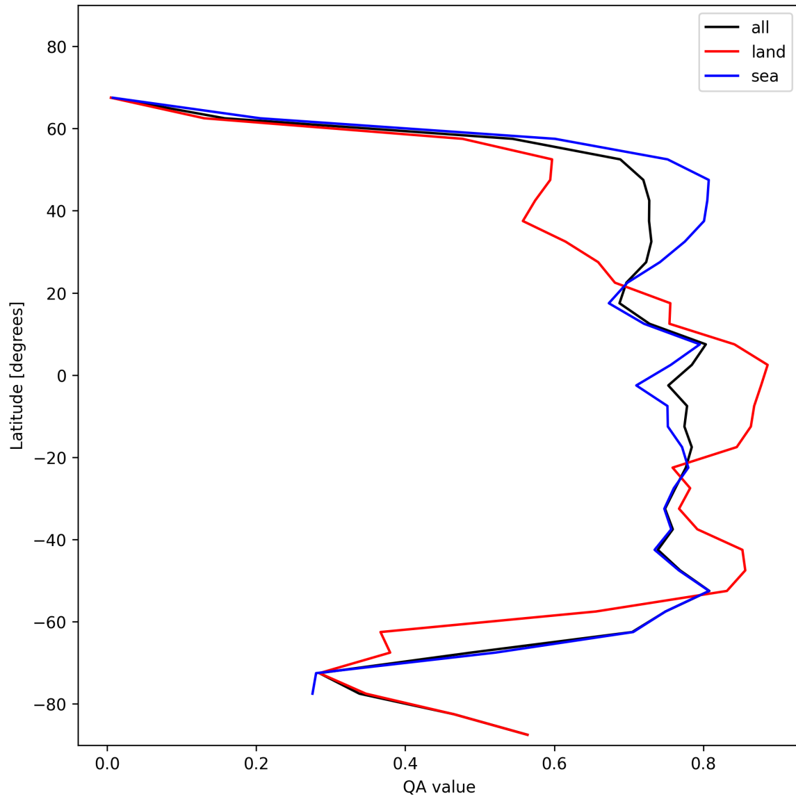
Figure 22: Zonal average of “QA value” for 2025-11-18 to 2025-11-20.
