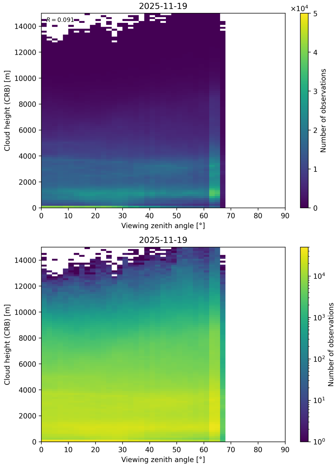
Figure 110: Scatter density plot of “Viewing zenith angle” against “Cloud height (CRB)” for 2025-11-18 to 2025-11-20.
