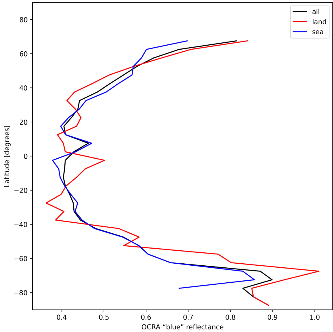
Figure 35: Zonal average of “OCRA “blue” reflectance” for 2025-11-18 to 2025-11-20.
