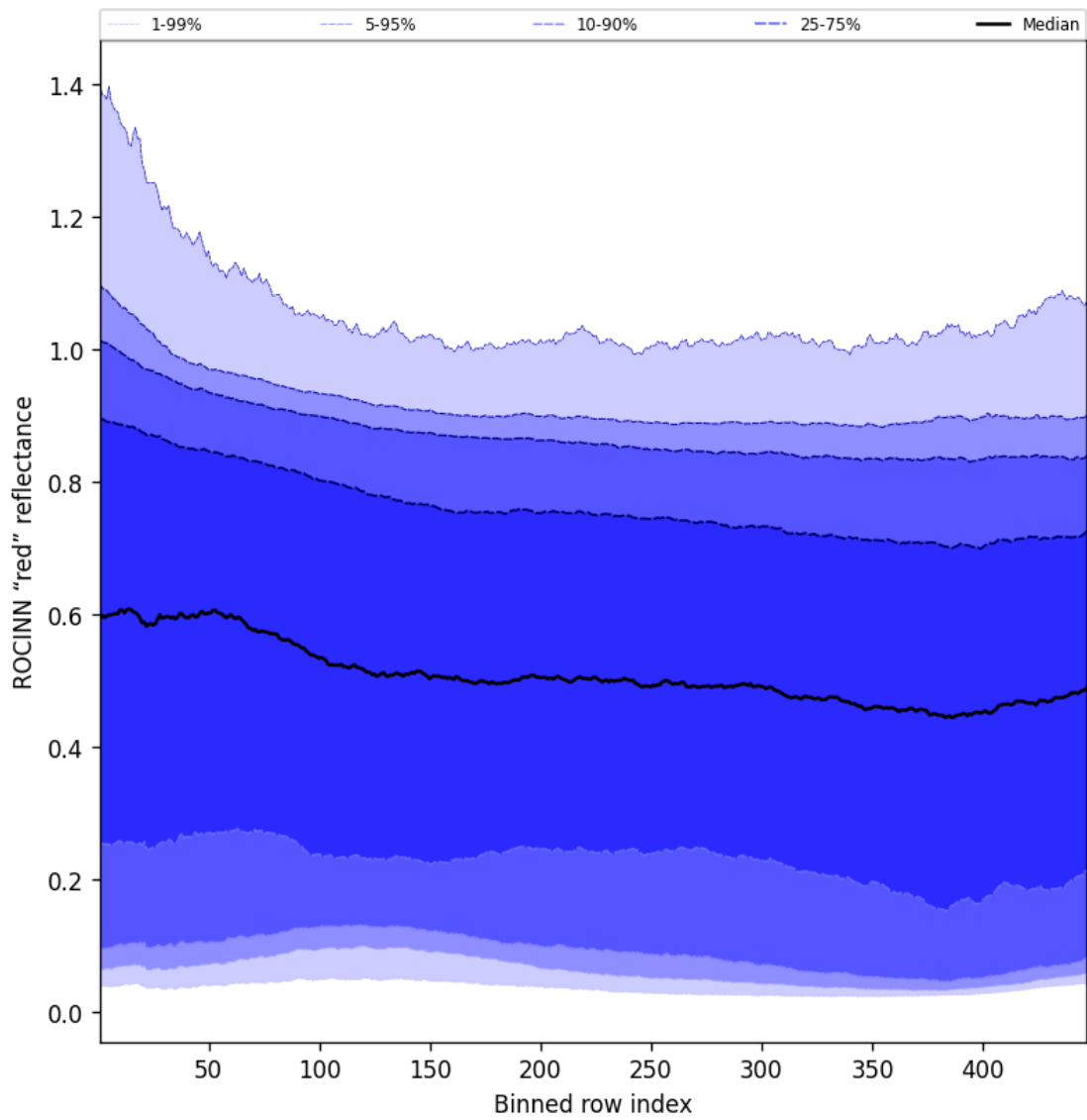
Figure 69: Along track statistics of "ROCINN "red" reflectance" for 2025-11-18 to 2025-11-20
