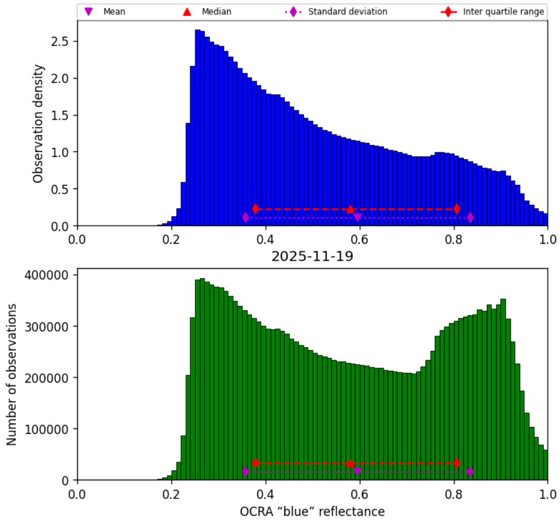
Figure 51: Histogram of “OCRA “blue” reflectance” for 2025-11-18 to 2025-11-20
