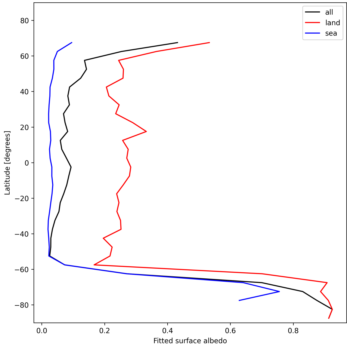
Figure 29: Zonal average of “Fitted surface albedo” for 2025-11-18 to 2025-11-20.
