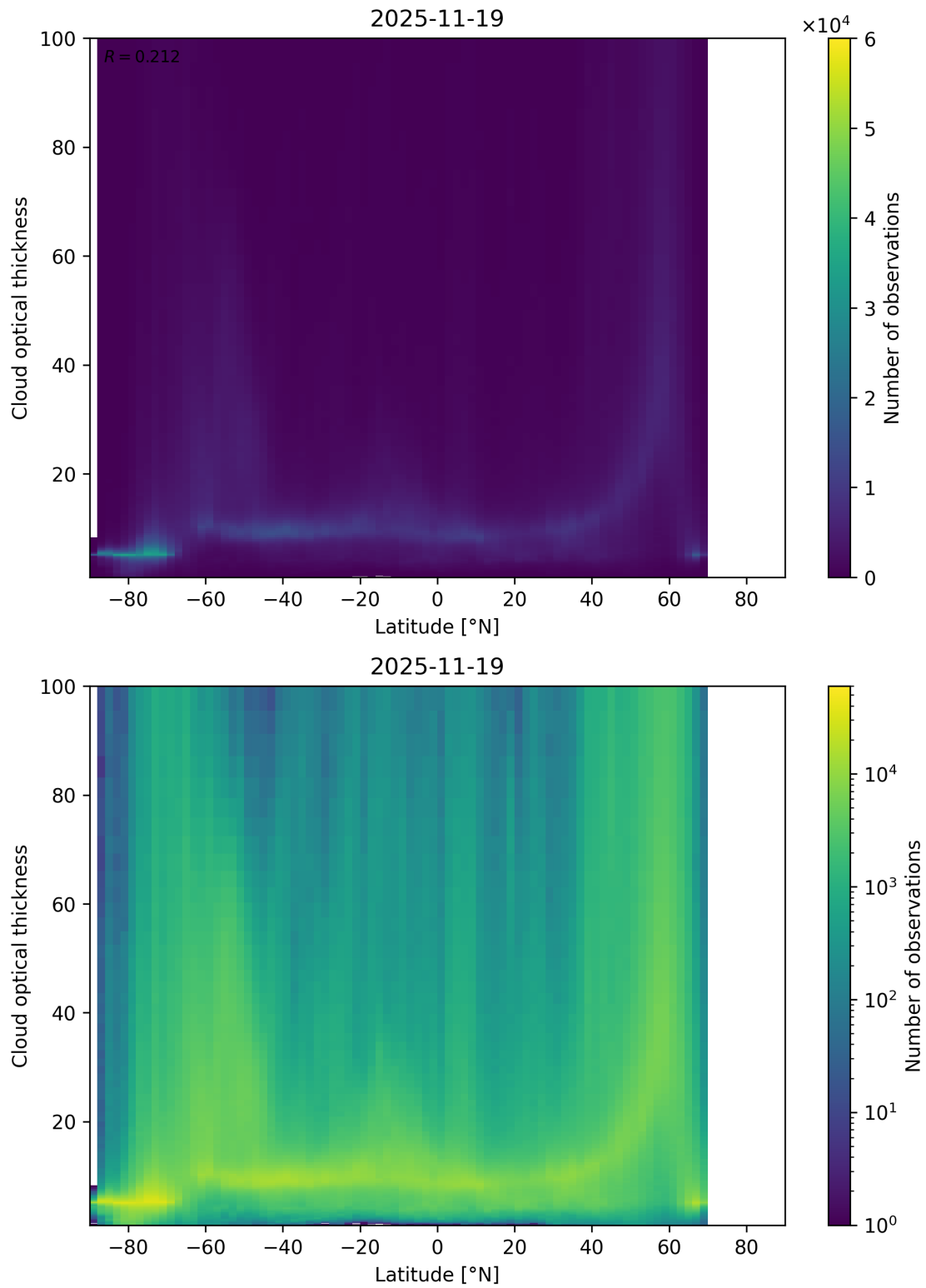
Figure 96: Scatter density plot of “Latitude” against “Cloud optical thickness” for 2025-11-18 to 2025-11-20.
