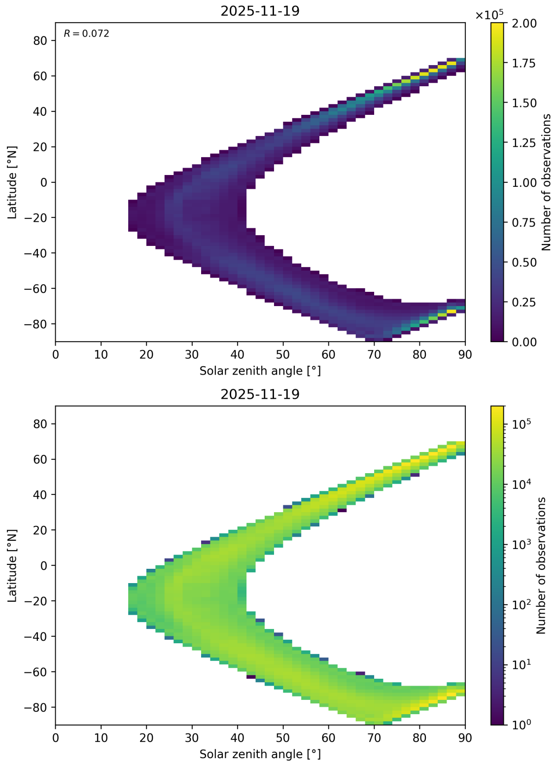
Figure 105: Scatter density plot of “Solar zenith angle” against “Latitude” for 2025-11-18 to 2025-11-20.
