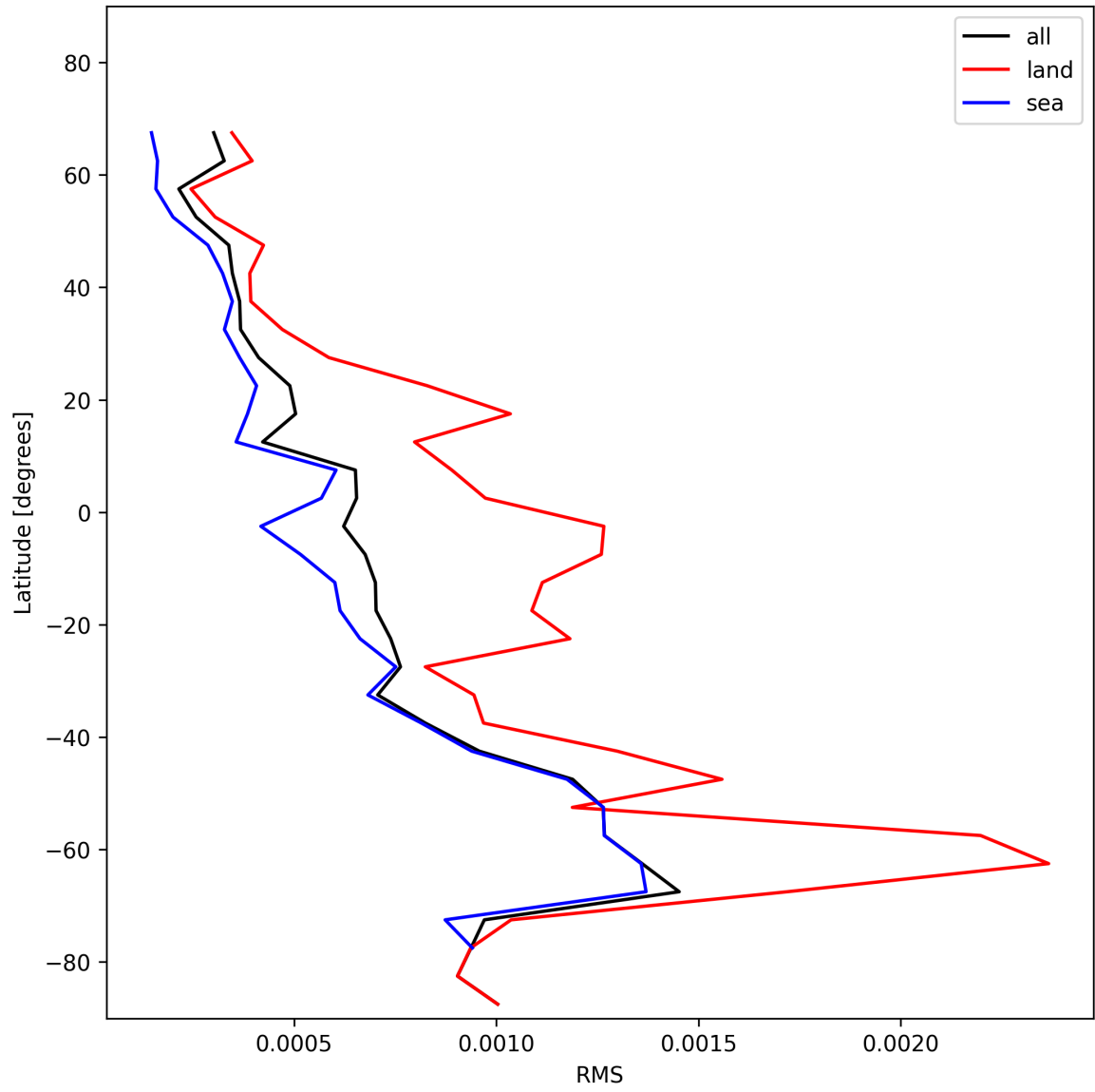
Figure 31: Zonal average of “RMS” for 2025-11-18 to 2025-11-20.
