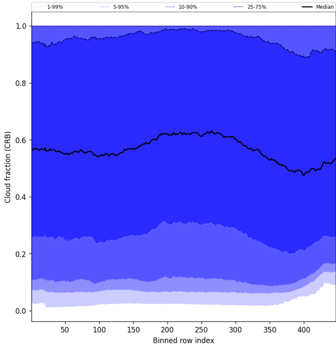
Figure 58: Along track statistics of “Cloud fraction (CRB)” for 2025-11-18 to 2025-11-20
