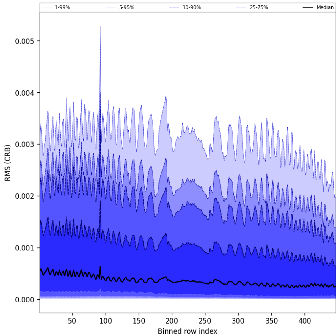
Figure 64: Along track statistics of “RMS (CRB)” for 2025-11-18 to 2025-11-20
