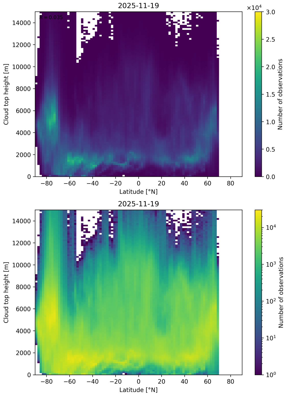
Figure 97: Scatter density plot of “Latitude” against “Cloud top height” for 2025-11-18 to 2025-11-20.
