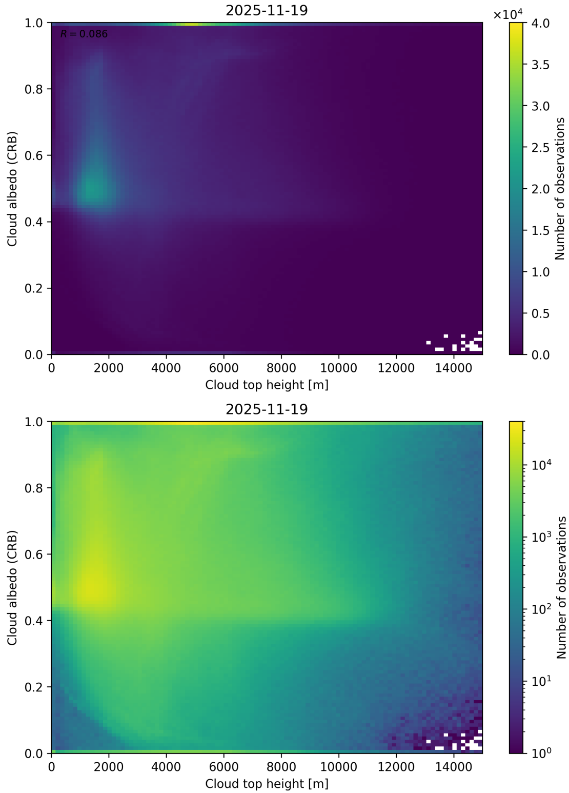
Figure 86: Scatter density plot of “Cloud top height” against “Cloud albedo (CRB)” for 2025-11-18 to 2025-11-20.
