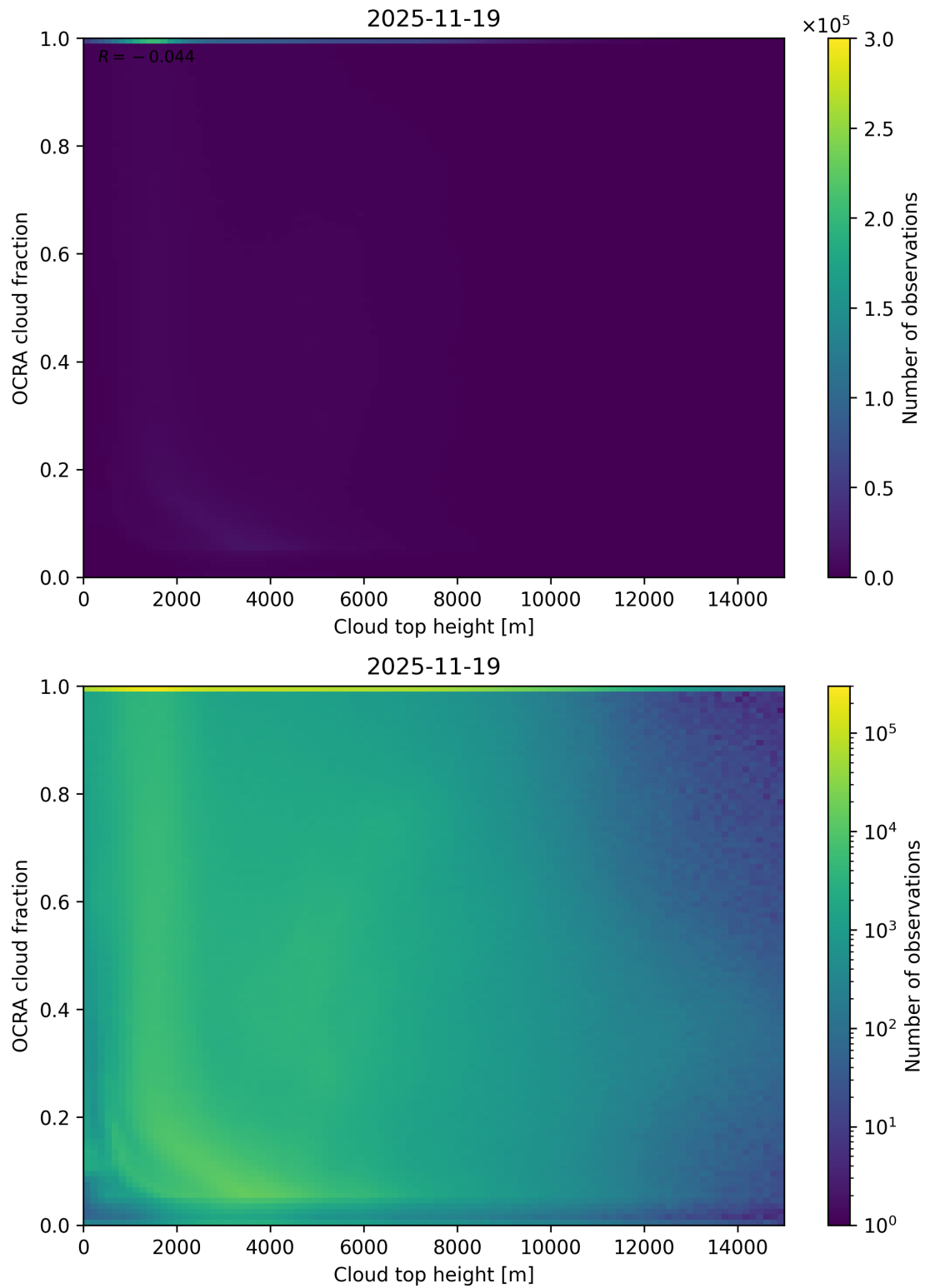
Figure 87: Scatter density plot of “Cloud top height” against “OCRA cloud fraction” for 2025-11-18 to 2025-11-20.
