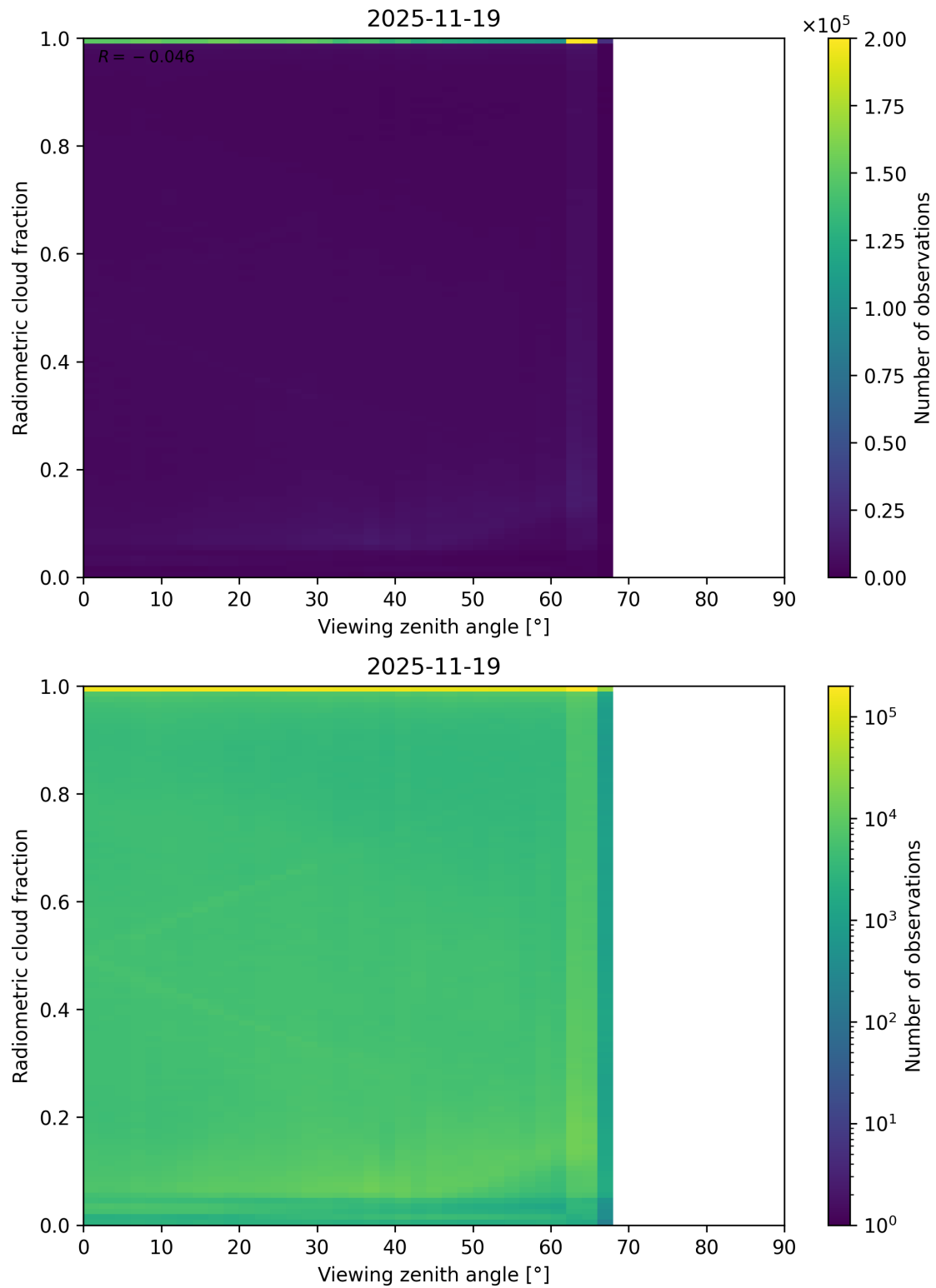
Figure 107: Scatter density plot of “Viewing zenith angle” against “Radiometric cloud fraction” for 2025-11-18 to 2025-11-20.
