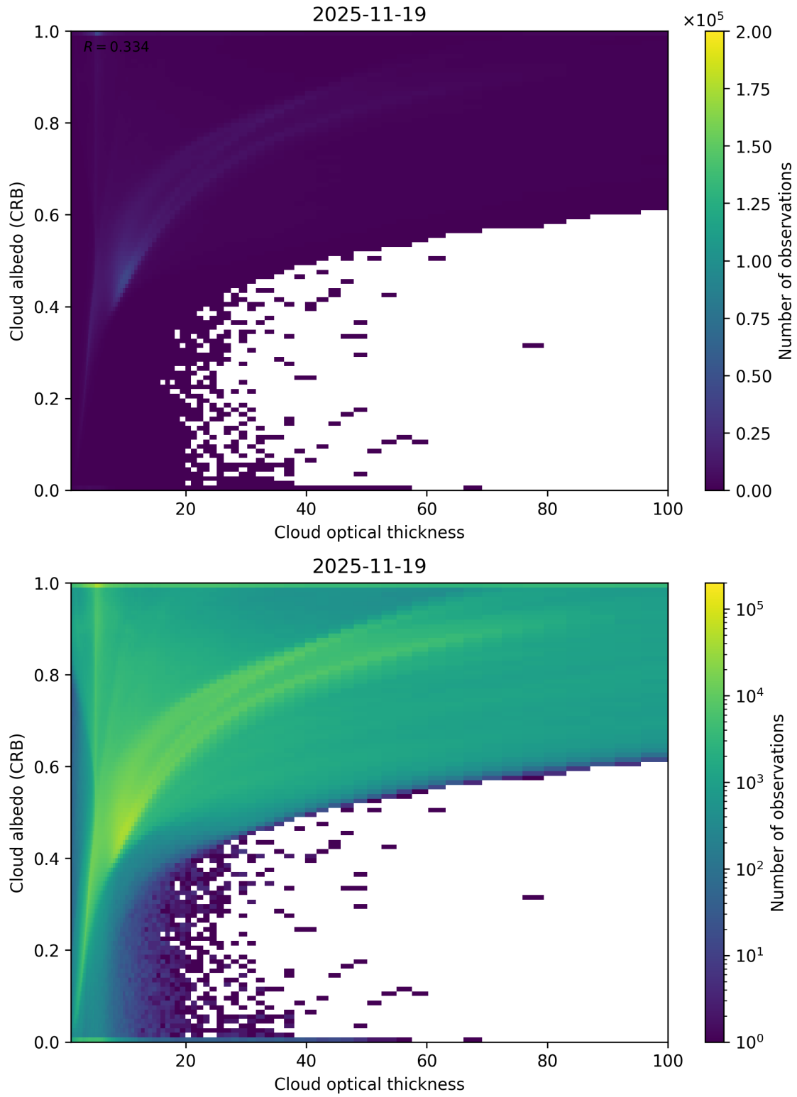
Figure 82: Scatter density plot of “Cloud optical thickness” against “Cloud albedo (CRB)” for 2025-11-18 to 2025-11-20.
