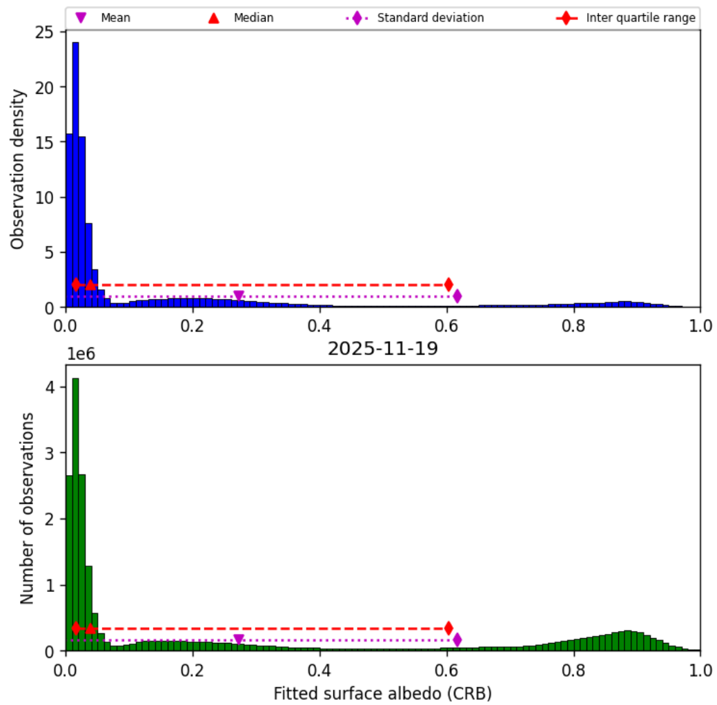
Figure 46: Histogram of “Fitted surface albedo (CRB)” for 2025-11-18 to 2025-11-20
