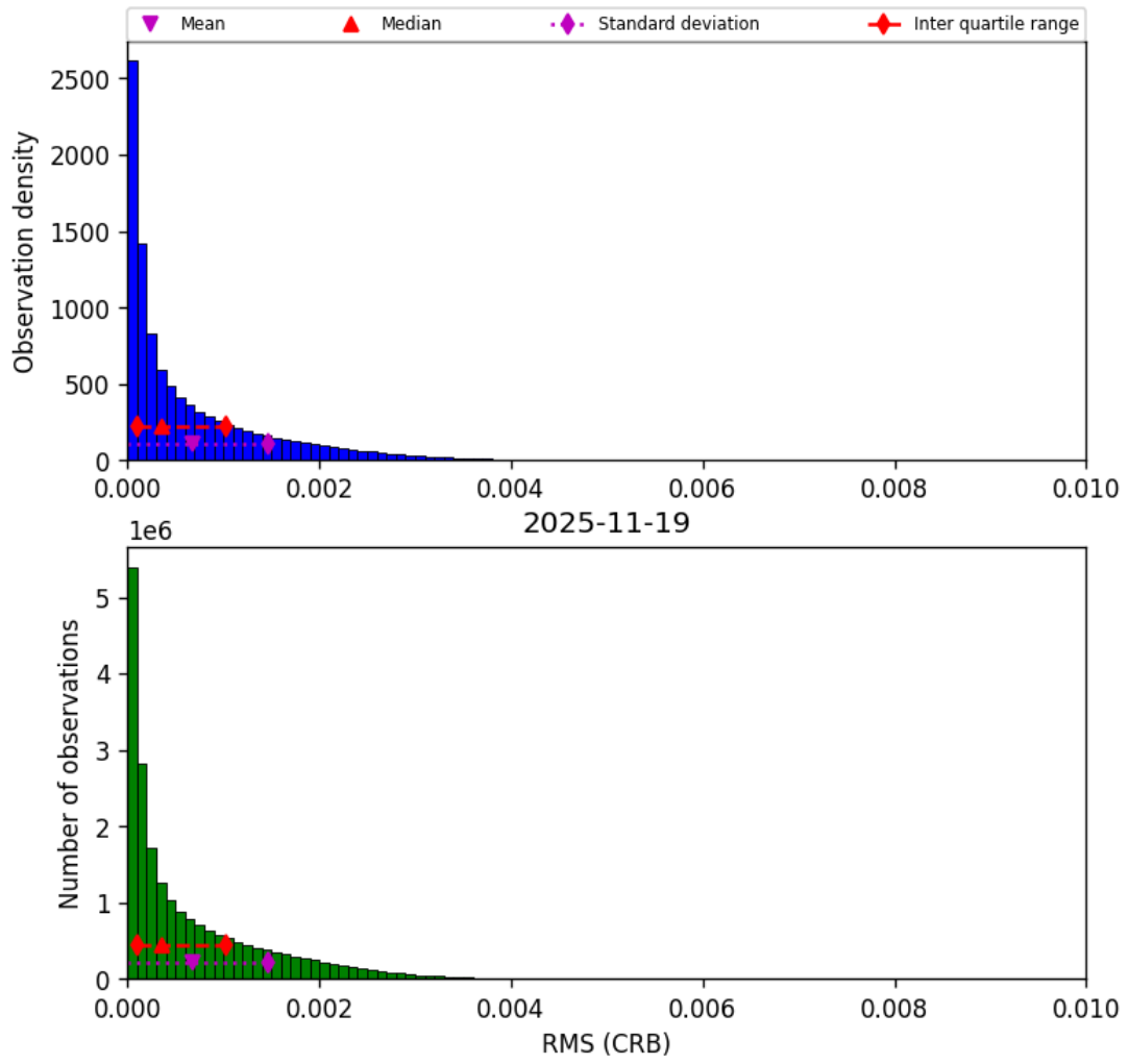
Figure 48: Histogram of “RMS (CRB)” for 2025-11-18 to 2025-11-20
