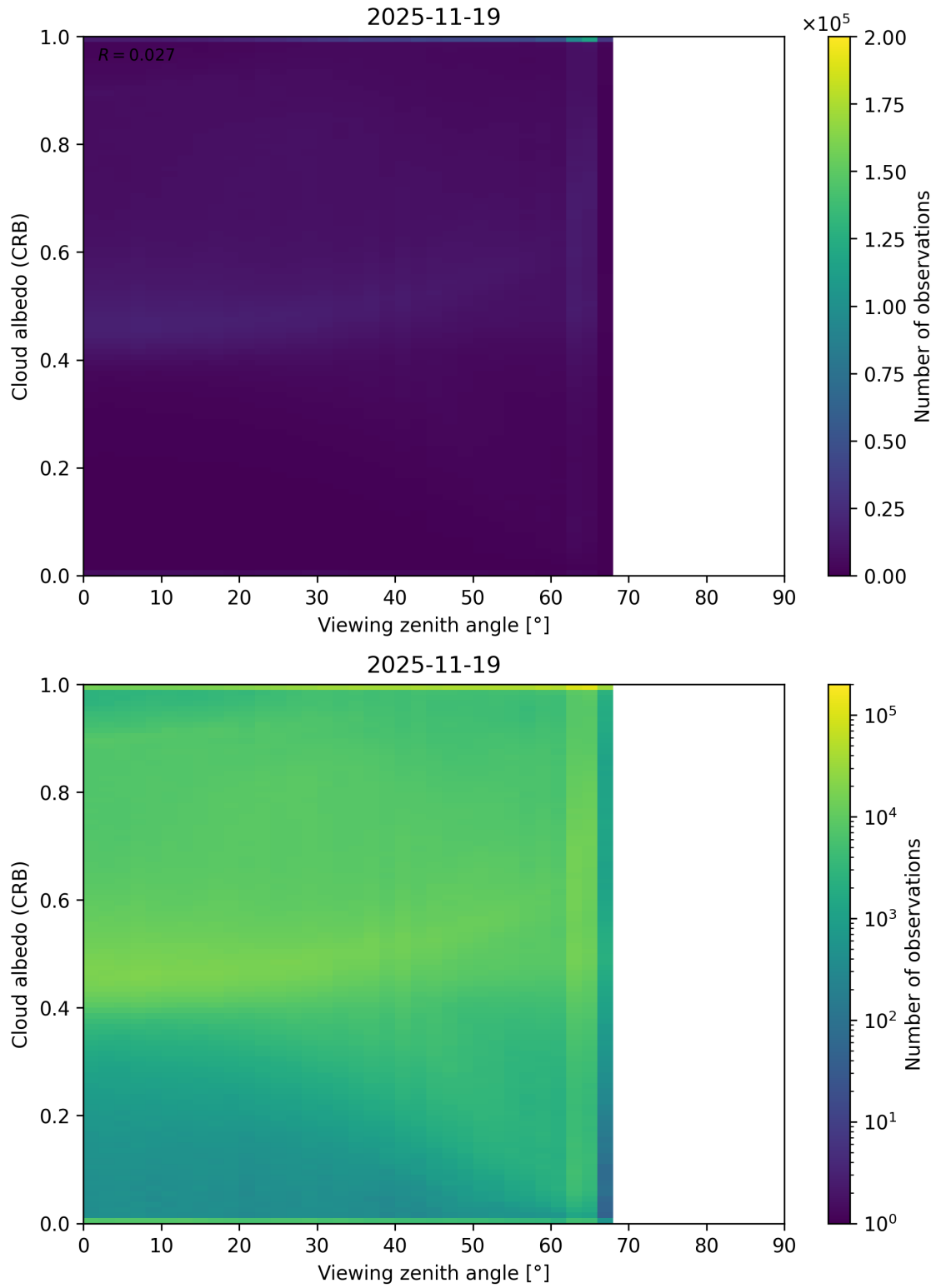
Figure 106: Scatter density plot of “Viewing zenith angle” against “Cloud albedo (CRB)” for 2025-11-18 to 2025-11-20.
