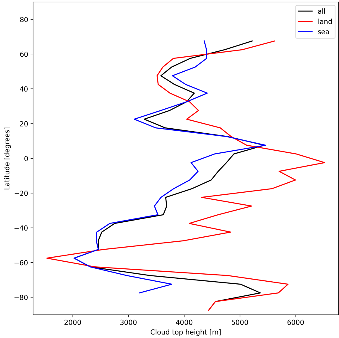
Figure 24: Zonal average of “Cloud top height” for 2025-11-18 to 2025-11-20.
