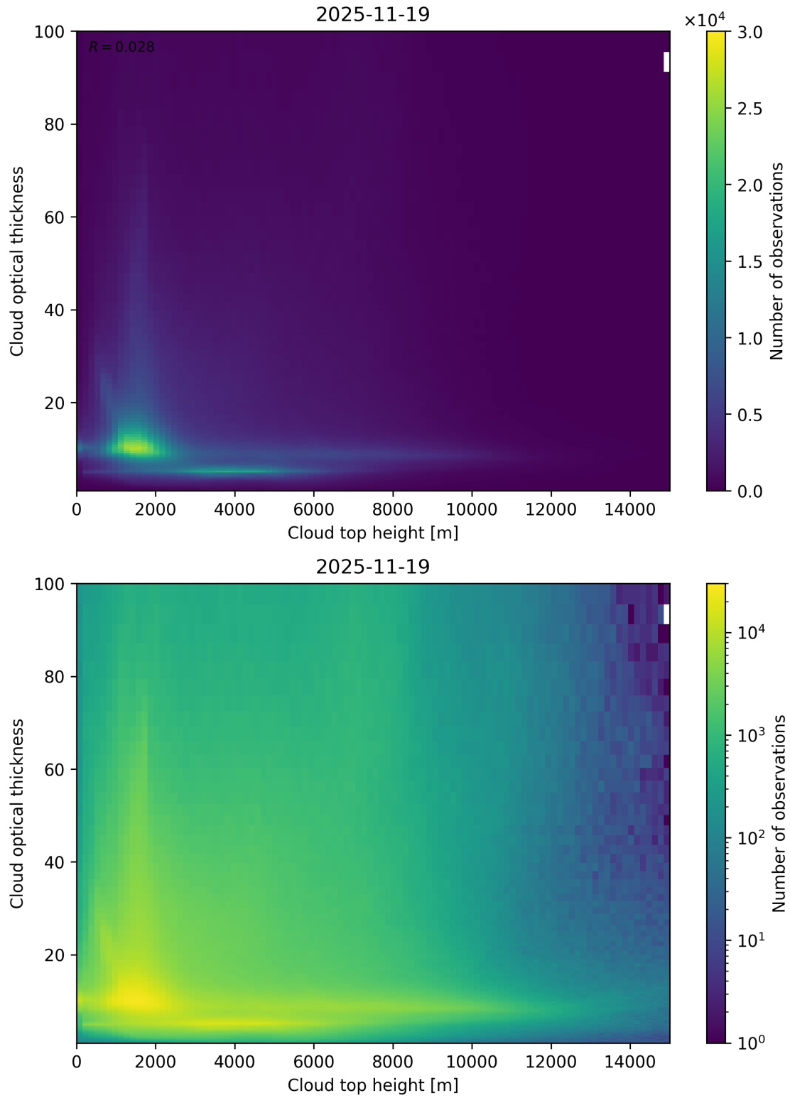
Figure 90: Scatter density plot of “Cloud top height” against “Cloud optical thickness” for 2025-11-18 to 2025-11-20.
