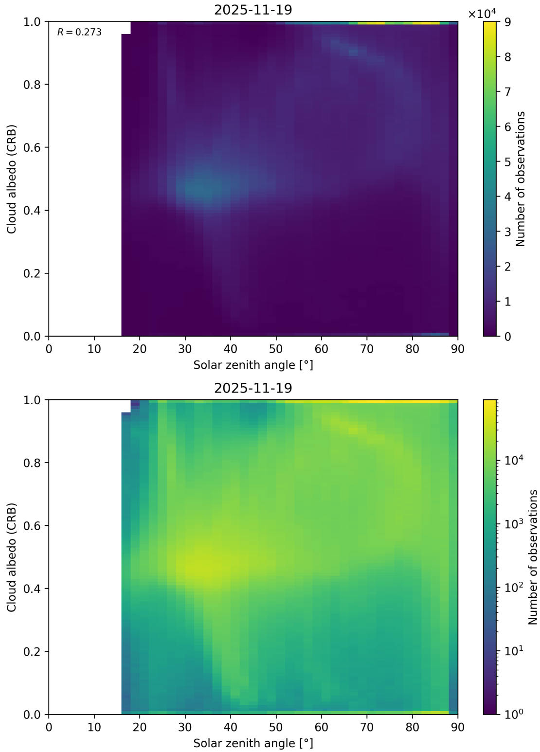
Figure 98: Scatter density plot of “Solar zenith angle” against “Cloud albedo (CRB)” for 2025-11-18 to 2025-11-20.
