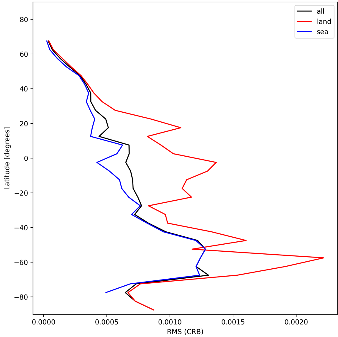
Figure 32: Zonal average of “RMS (CRB)” for 2025-11-18 to 2025-11-20.
