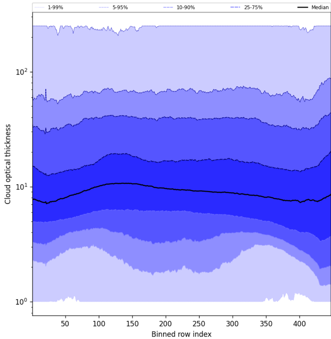
Figure 57: Along track statistics of “Cloud optical thickness” for 2025-11-18 to 2025-11-20
