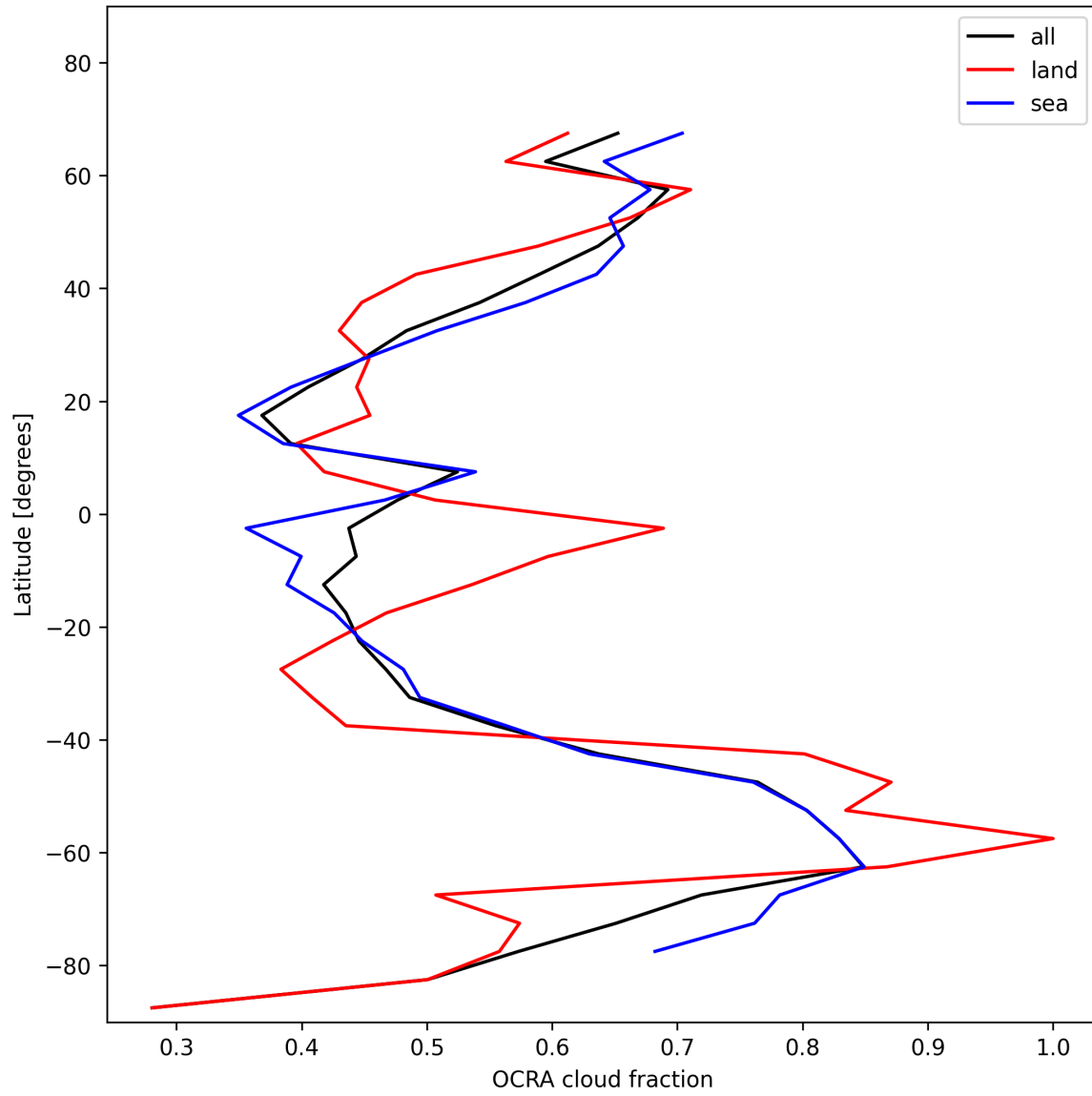
Figure 34: Zonal average of “OCRA cloud fraction” for 2025-11-18 to 2025-11-20.
