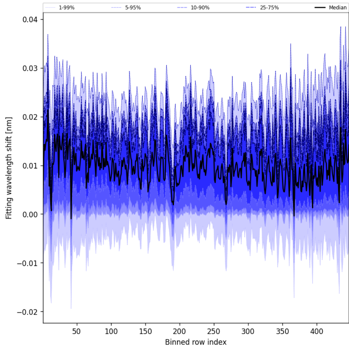
Figure 65: Along track statistics of “Fitting wavelength shift” for 2025-11-18 to 2025-11-20
