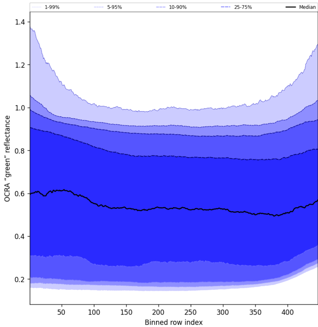
Figure 68: Along track statistics of “OCRA “green” reflectance” for 2025-11-18 to 2025-11-20
