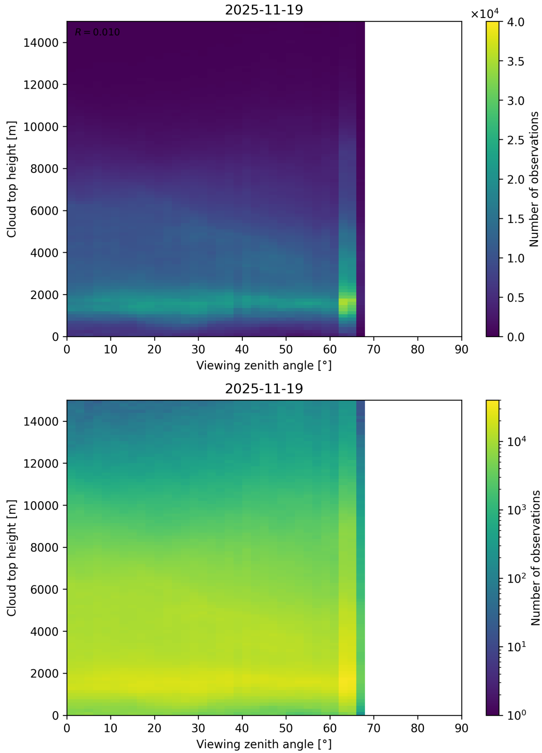
Figure 112: Scatter density plot of “Viewing zenith angle” against “Cloud top height” for 2025-11-18 to 2025-11-20.
