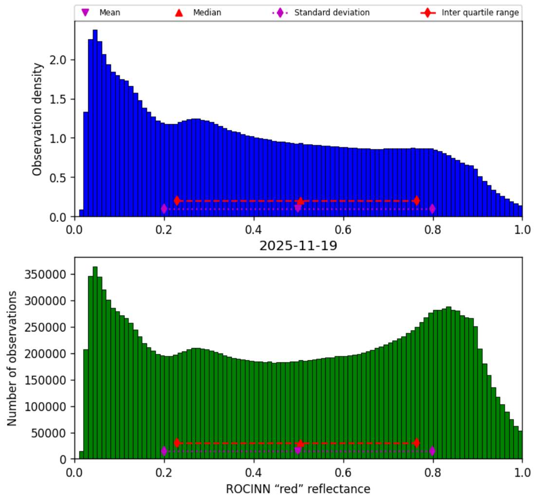
Figure 53: Histogram of “ROCINN “red” reflectance” for 2025-11-18 to 2025-11-20
