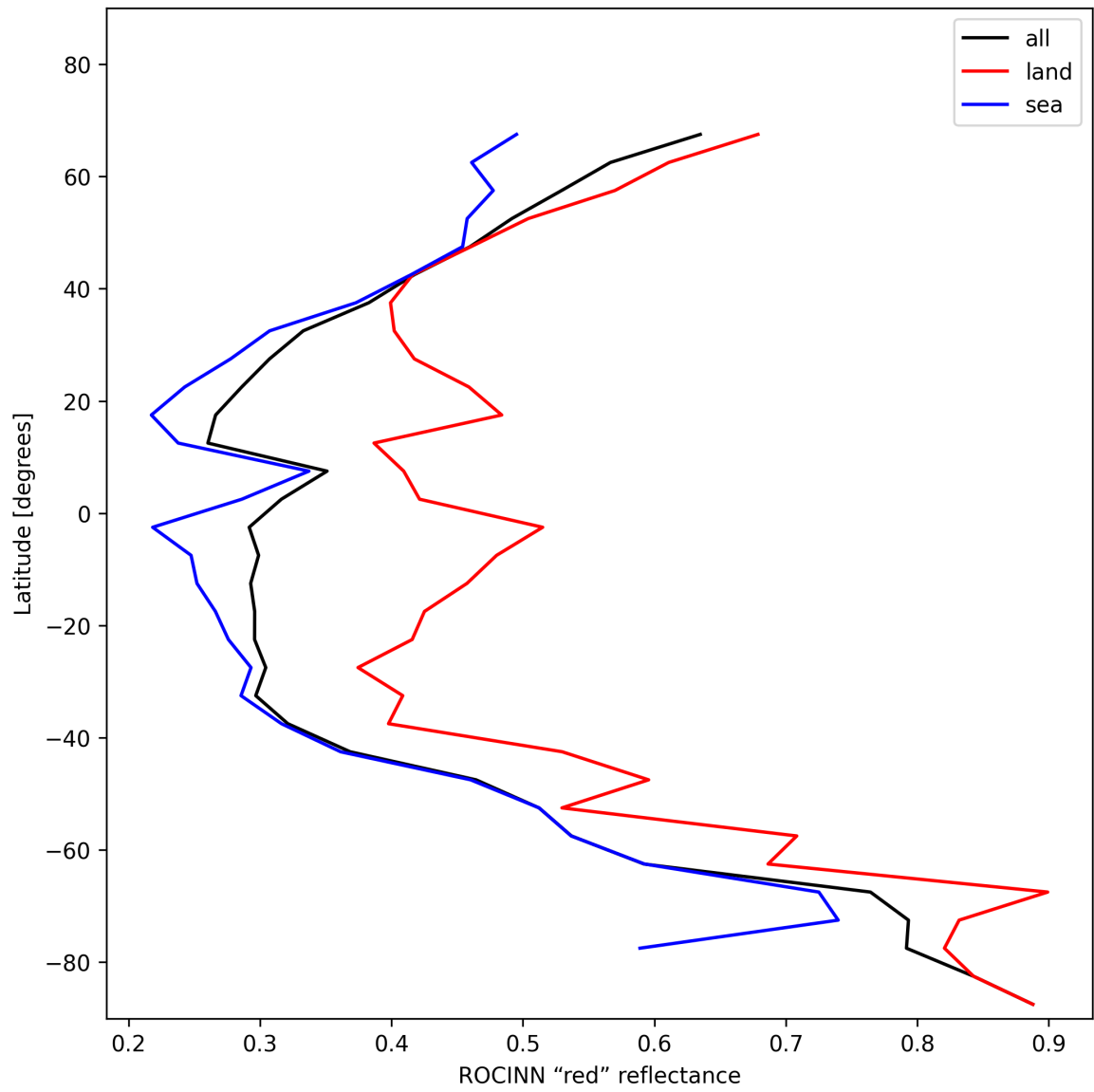
Figure 37: Zonal average of “ROCINN “red” reflectance” for 2025-11-18 to 2025-11-20.
