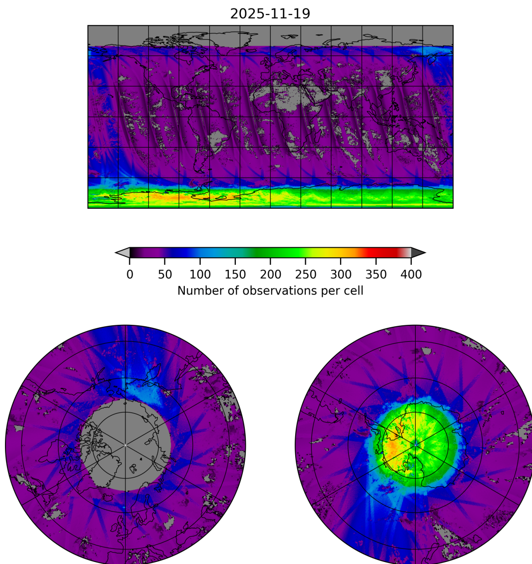
Figure 21: Map of the number of observations for 2025-11-18 to 2025-11-20
