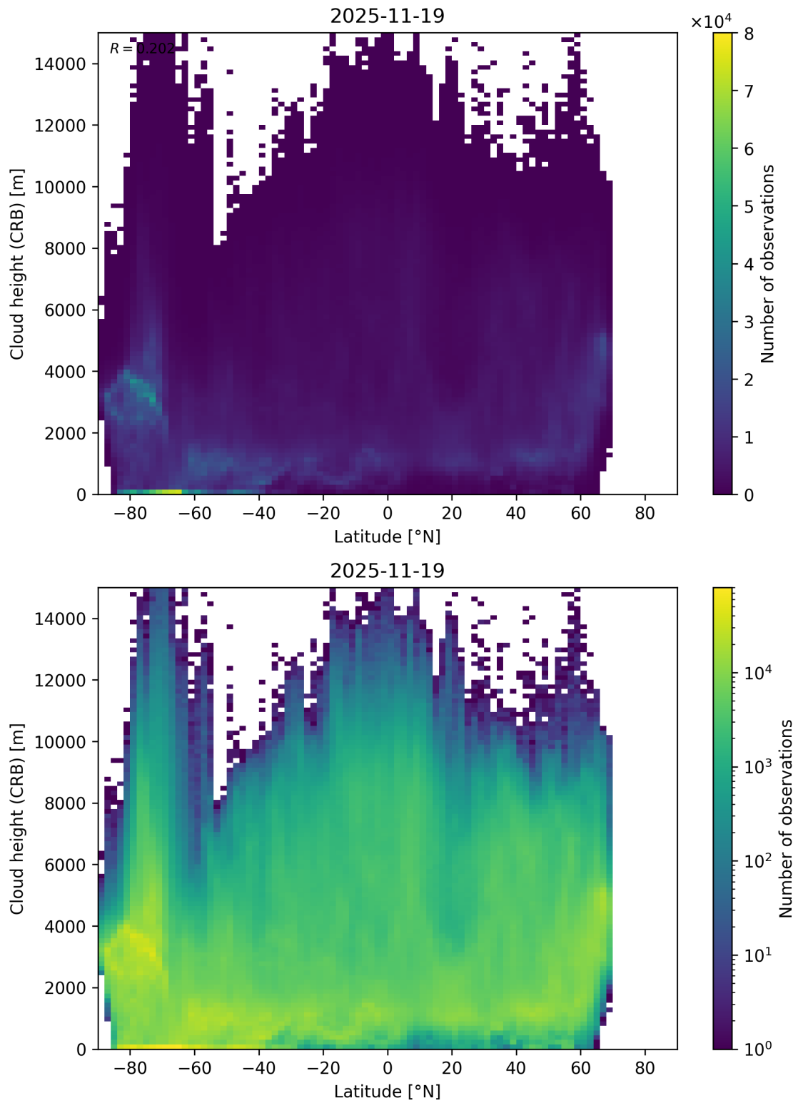
Figure 95: Scatter density plot of “Latitude” against “Cloud height (CRB)” for 2025-11-18 to 2025-11-20.
