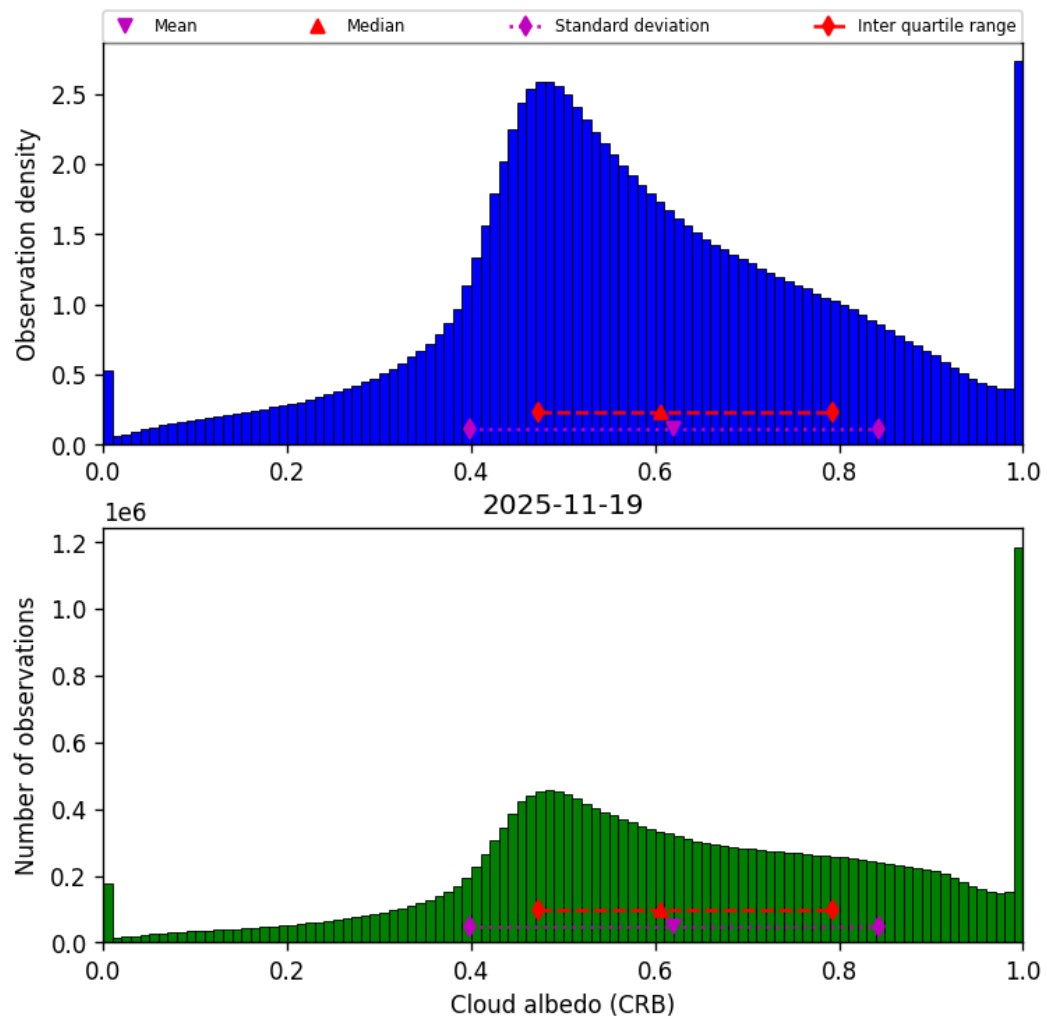
Figure 44: Histogram of “Cloud albedo (CRB)” for 2025-11-18 to 2025-11-20
