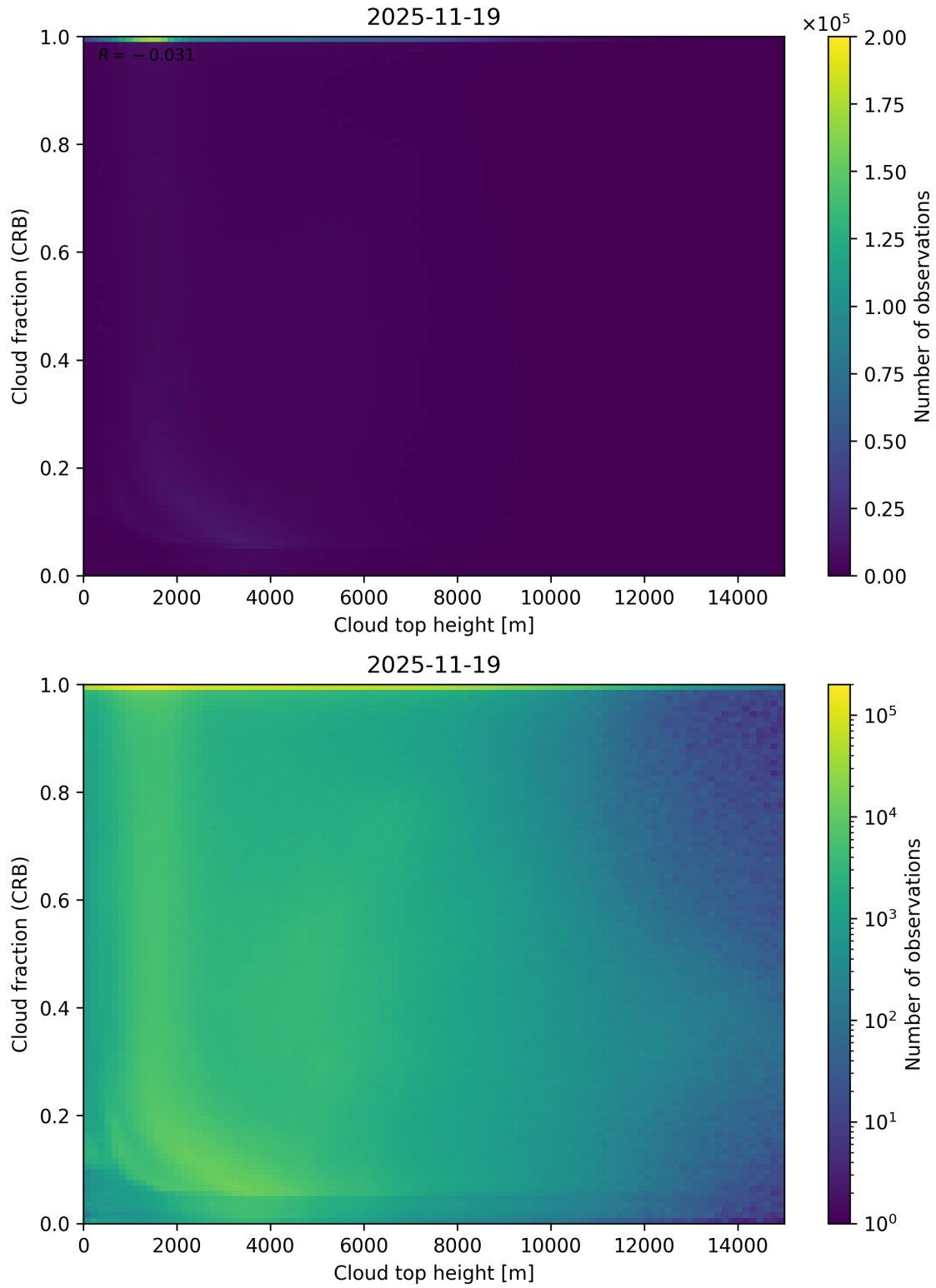
Figure 88: Scatter density plot of “Cloud top height” against “Cloud fraction (CRB)” for 2025-11-18 to 2025-11-20.
