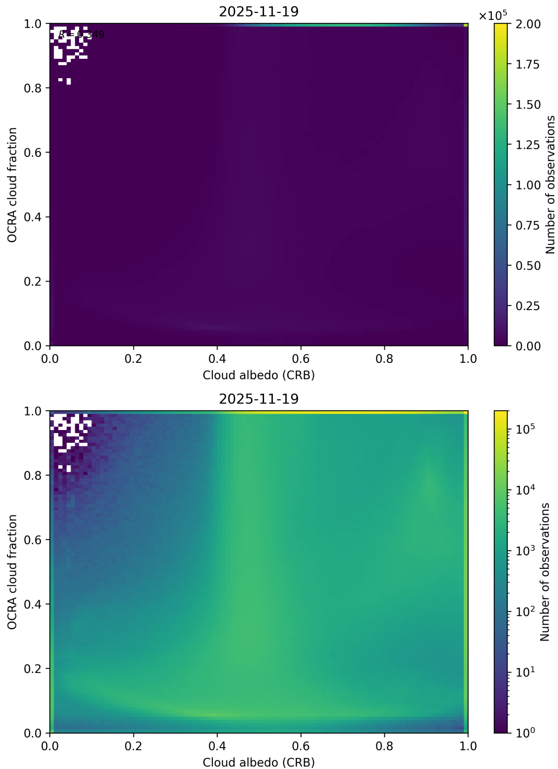
Figure 70: Scatter density plot of “Cloud albedo (CRB)” against “OCRA cloud fraction” for 2025-11-18 to 2025-11-20.
