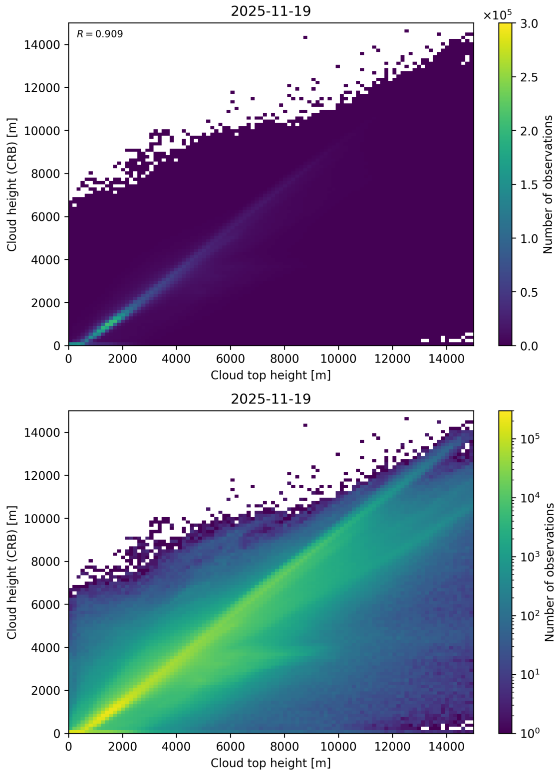
Figure 89: Scatter density plot of “Cloud top height” against “Cloud height (CRB)” for 2025-11-18 to 2025-11-20.
