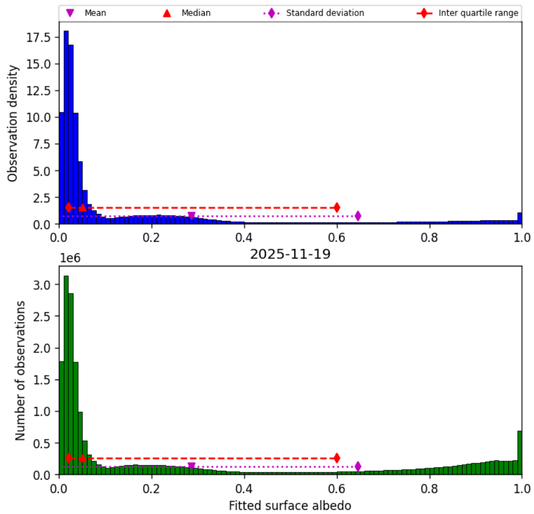
Figure 45: Histogram of “Fitted surface albedo” for 2025-11-18 to 2025-11-20
