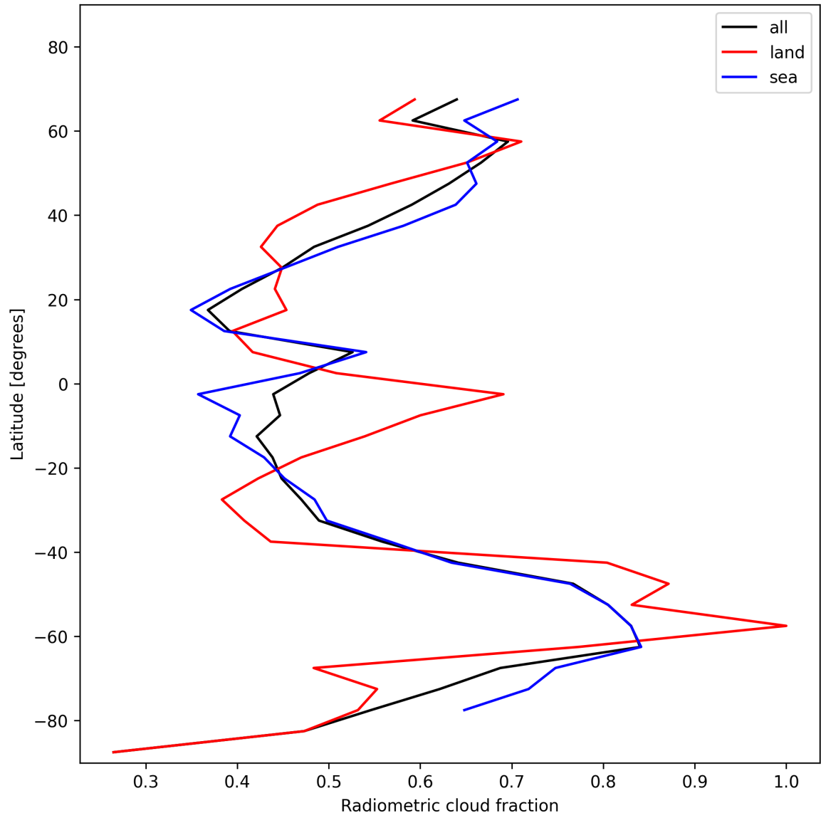
Figure 23: Zonal average of “Radiometric cloud fraction” for 2025-11-18 to 2025-11-20.
