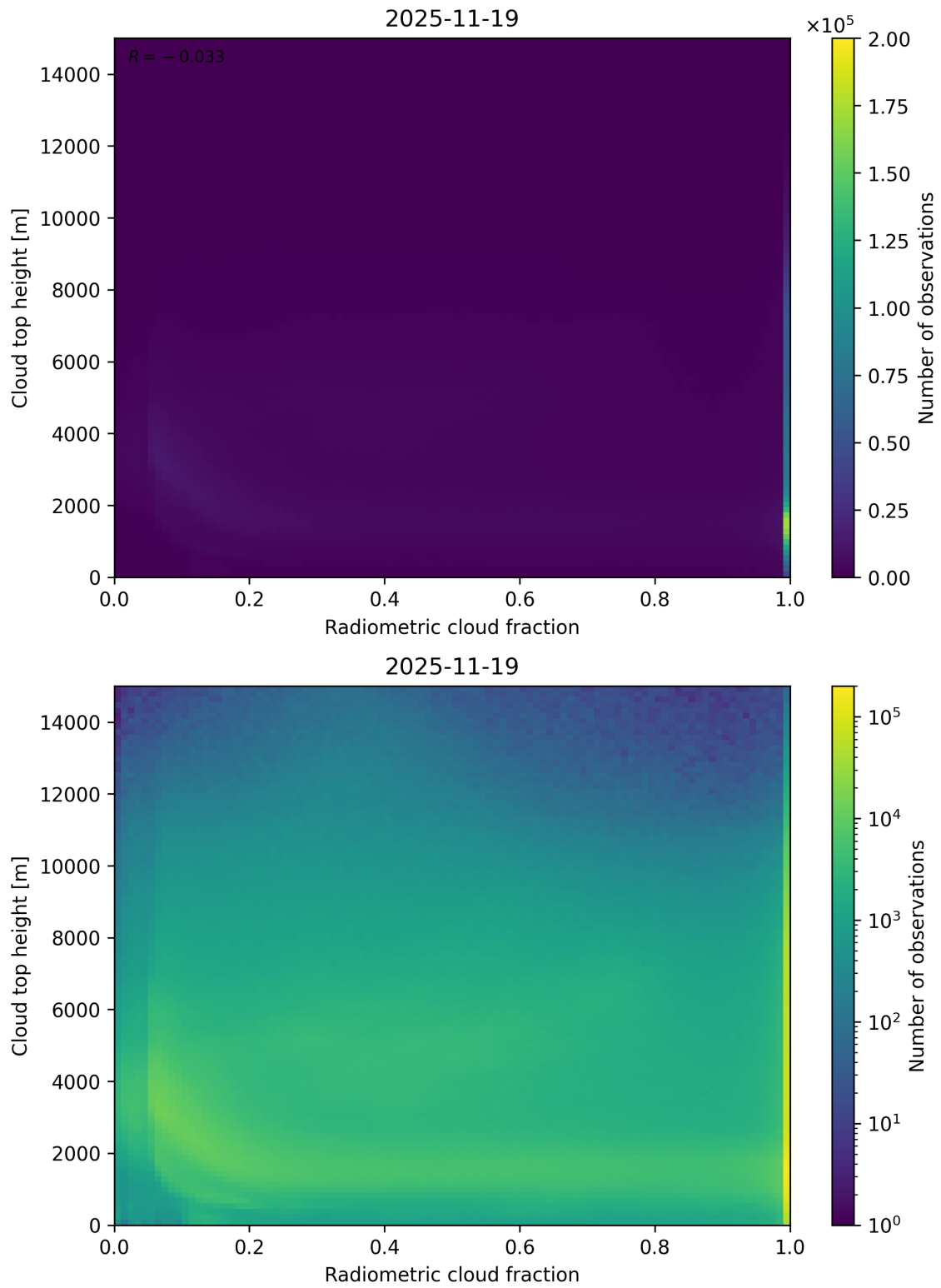
Figure 76: Scatter density plot of “Radiometric cloud fraction” against “Cloud top height” for 2025-11-18 to 2025-11-20.
