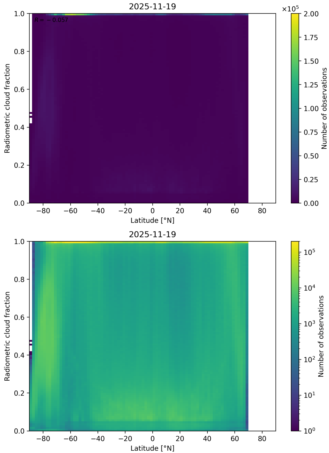
Figure 92: Scatter density plot of “Latitude” against “Radiometric cloud fraction” for 2025-11-18 to 2025-11-20.
