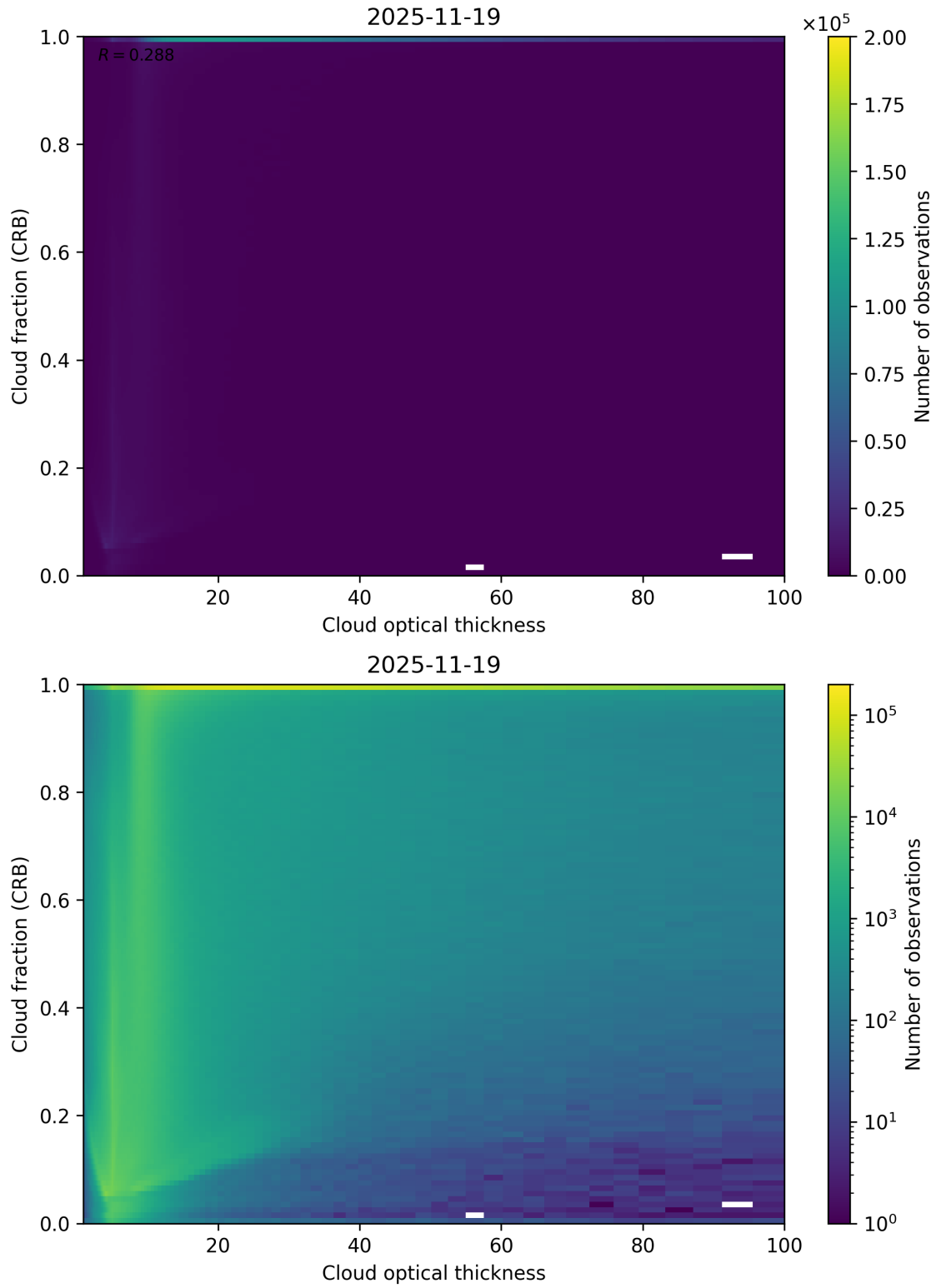
Figure 84: Scatter density plot of “Cloud optical thickness” against “Cloud fraction (CRB)” for 2025-11-18 to 2025-11-20.
