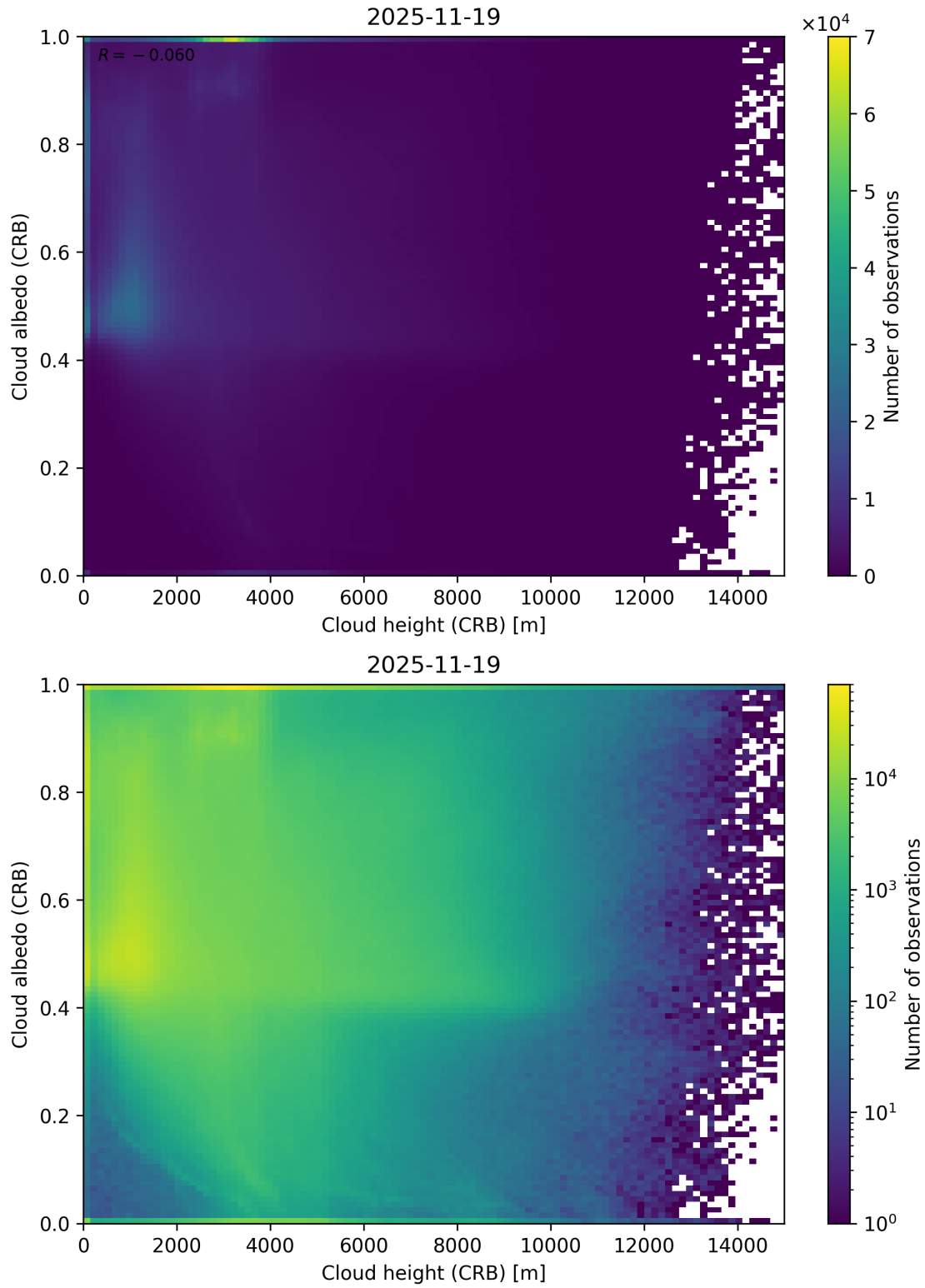
Figure 80: Scatter density plot of “Cloud height (CRB)” against “Cloud albedo (CRB)” for 2025-11-18 to 2025-11-20.
