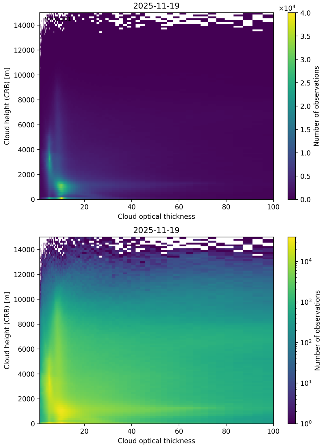
Figure 85: Scatter density plot of “Cloud optical thickness” against “Cloud height (CRB)” for 2025-11-18 to 2025-11-20.
