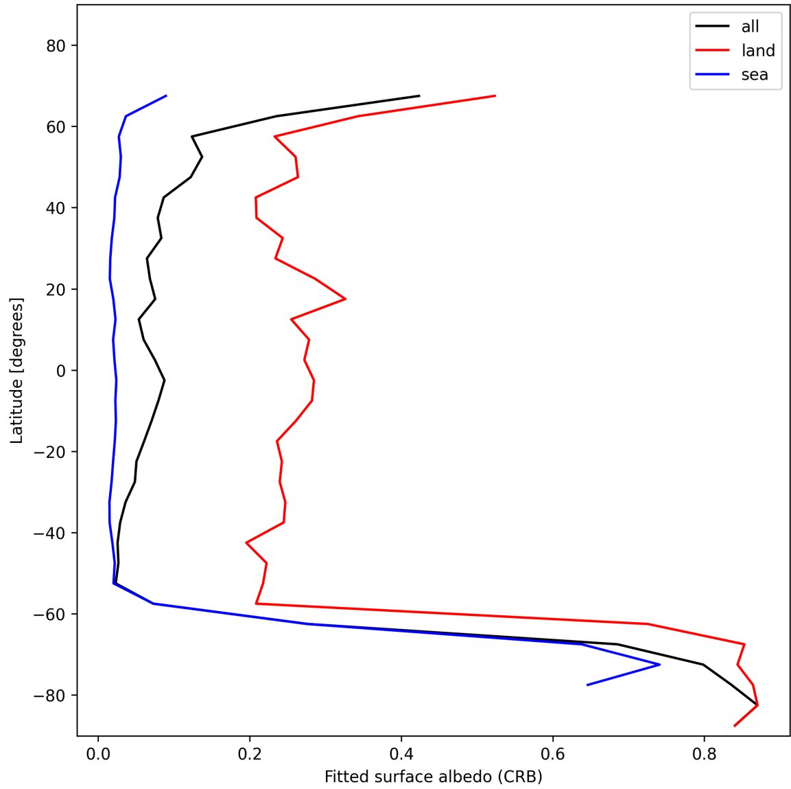
Figure 30: Zonal average of “Fitted surface albedo (CRB)” for 2025-11-18 to 2025-11-20.
