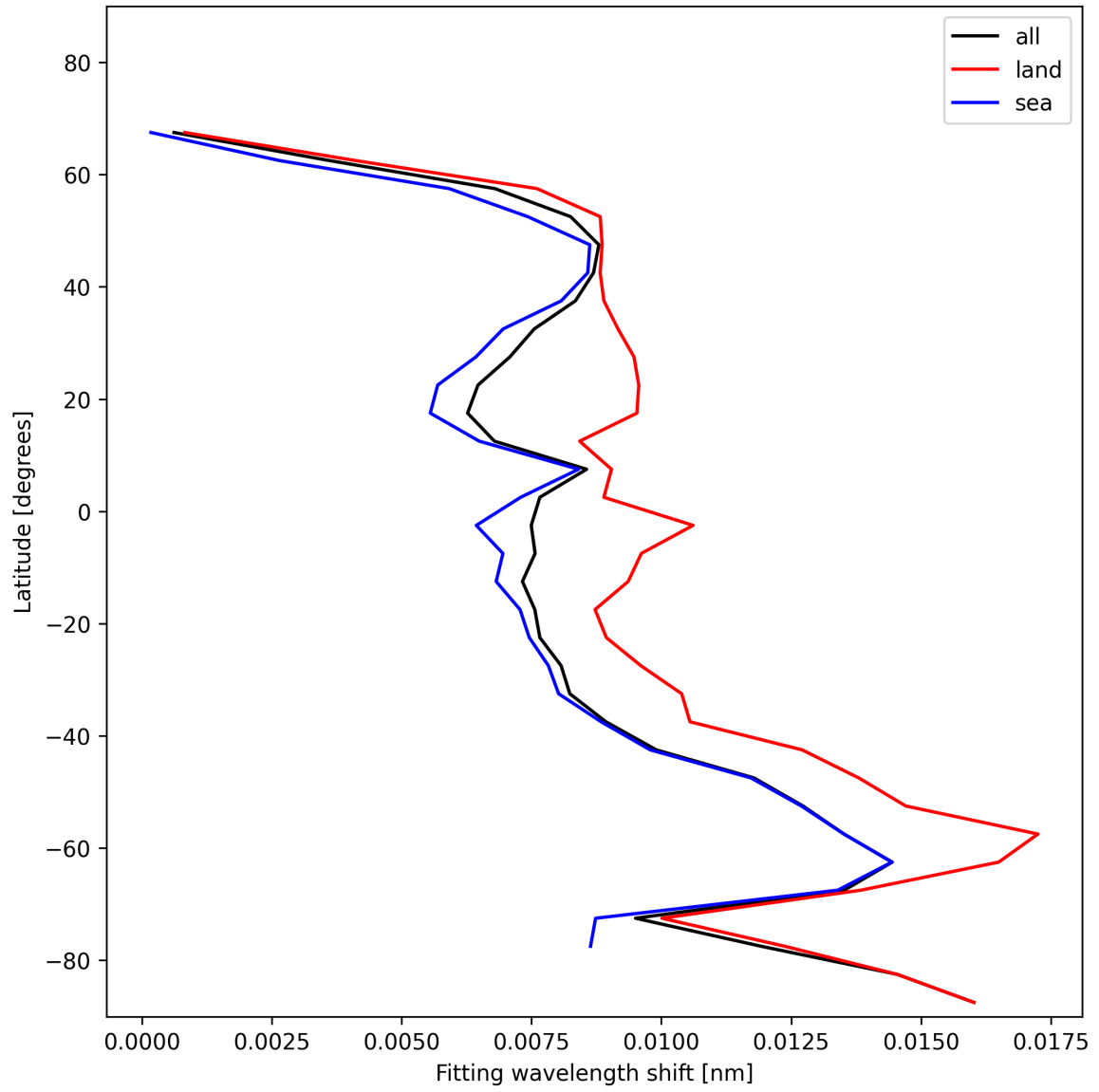
Figure 33: Zonal average of “Fitting wavelength shift” for 2025-11-18 to 2025-11-20.
