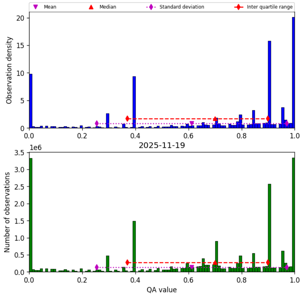
Figure 38: Histogram of “QA value” for 2025-11-18 to 2025-11-20
