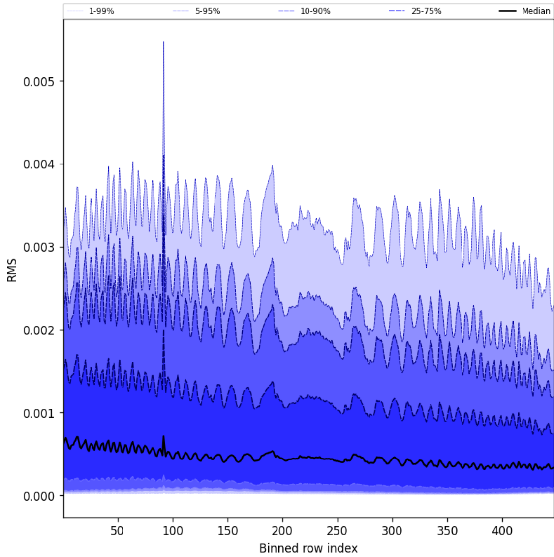
Figure 63: Along track statistics of “RMS” for 2025-11-18 to 2025-11-20
