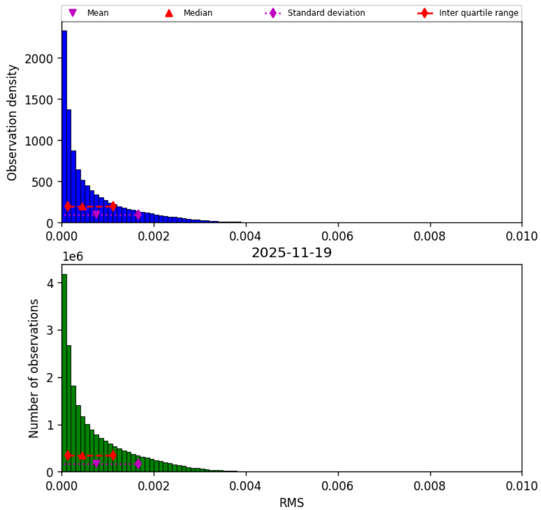
Figure 47: Histogram of “RMS” for 2025-11-18 to 2025-11-20
