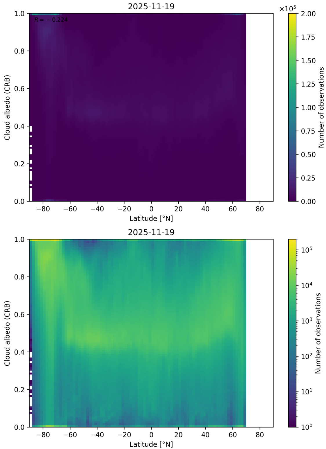
Figure 91: Scatter density plot of “Latitude” against “Cloud albedo (CRB)” for 2025-11-18 to 2025-11-20.
