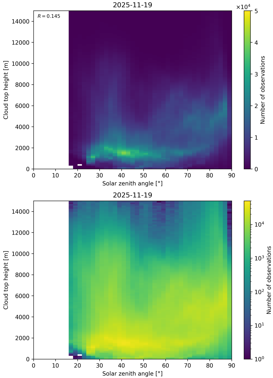
Figure 104: Scatter density plot of “Solar zenith angle” against “Cloud top height” for 2025-11-18 to 2025-11-20.
