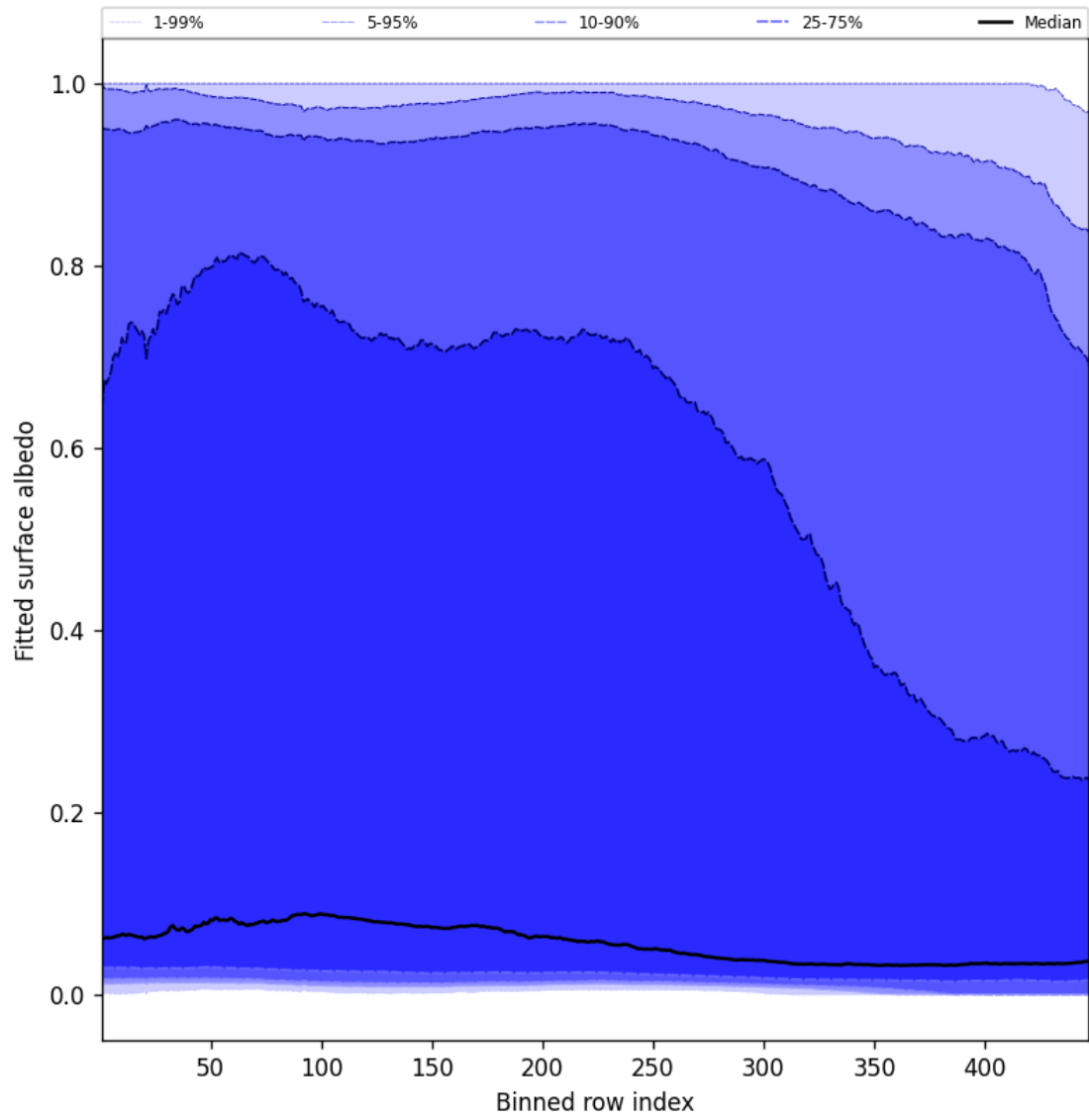
Figure 61: Along track statistics of “Fitted surface albedo” for 2025-11-18 to 2025-11-20
