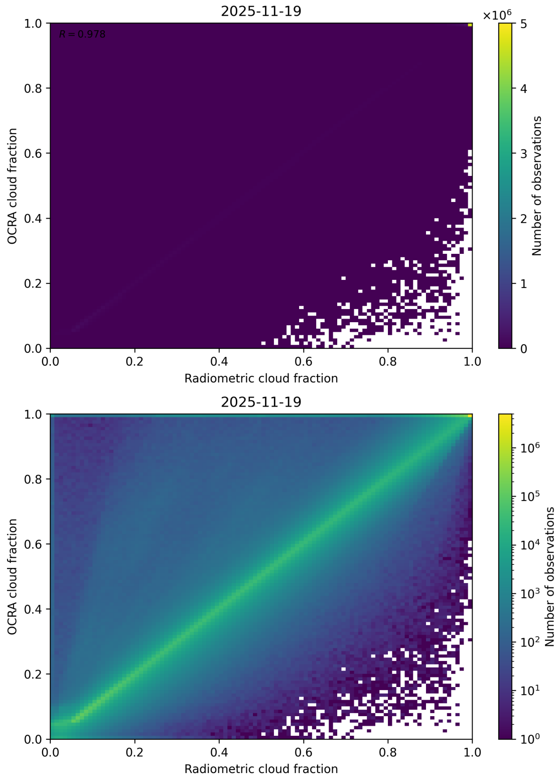
Figure 72: Scatter density plot of “Radiometric cloud fraction” against “OCRA cloud fraction” for 2025-11-18 to 2025-11-20.
