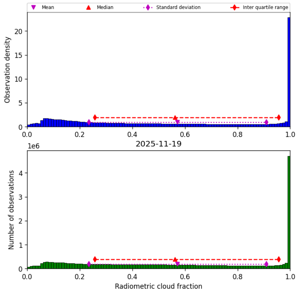
Figure 39: Histogram of “Radiometric cloud fraction” for 2025-11-18 to 2025-11-20
