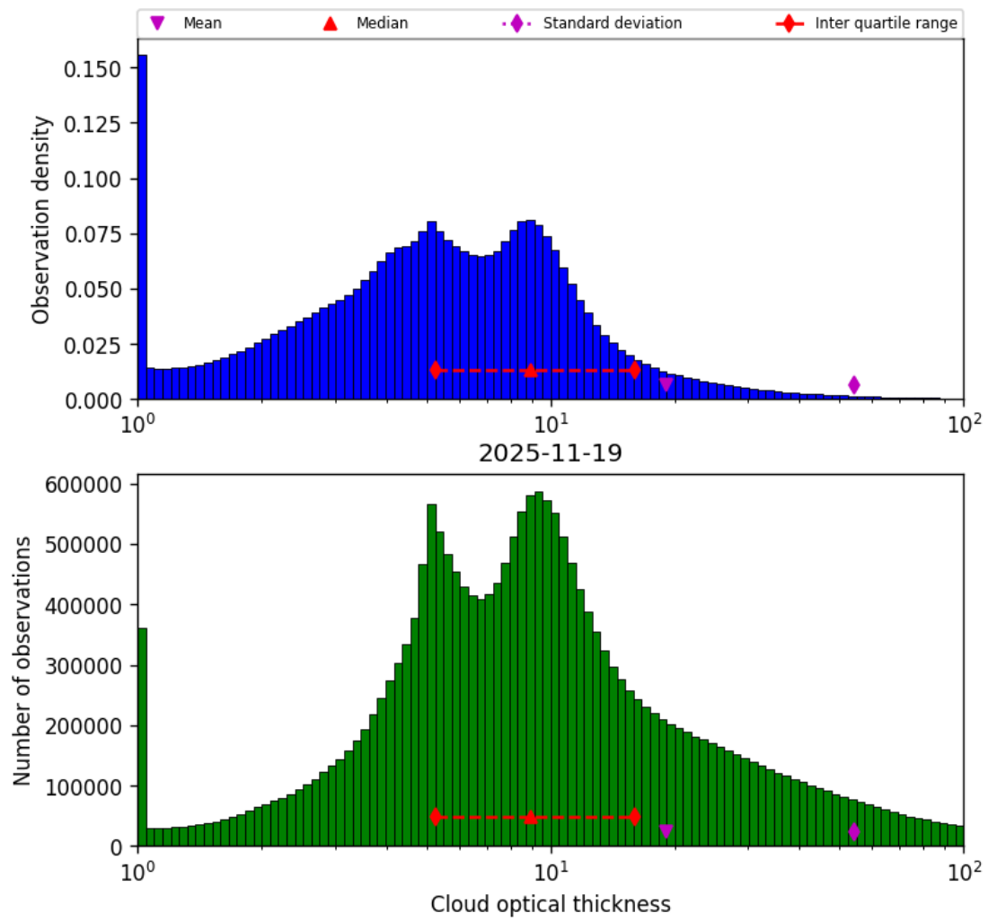
Figure 41: Histogram of “Cloud optical thickness” for 2025-11-18 to 2025-11-20
