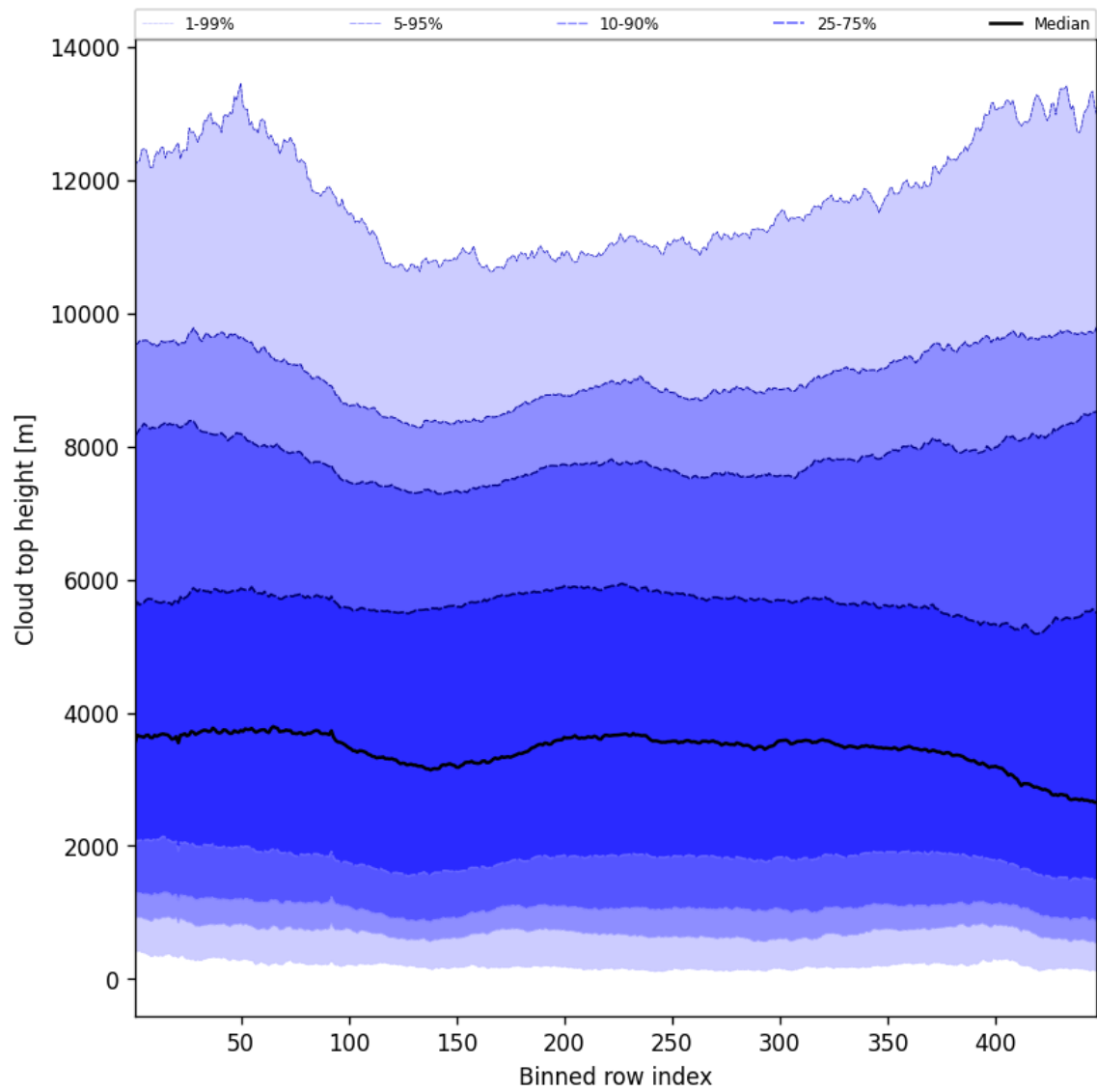
Figure 56: Along track statistics of “Cloud top height” for 2025-11-18 to 2025-11-20
