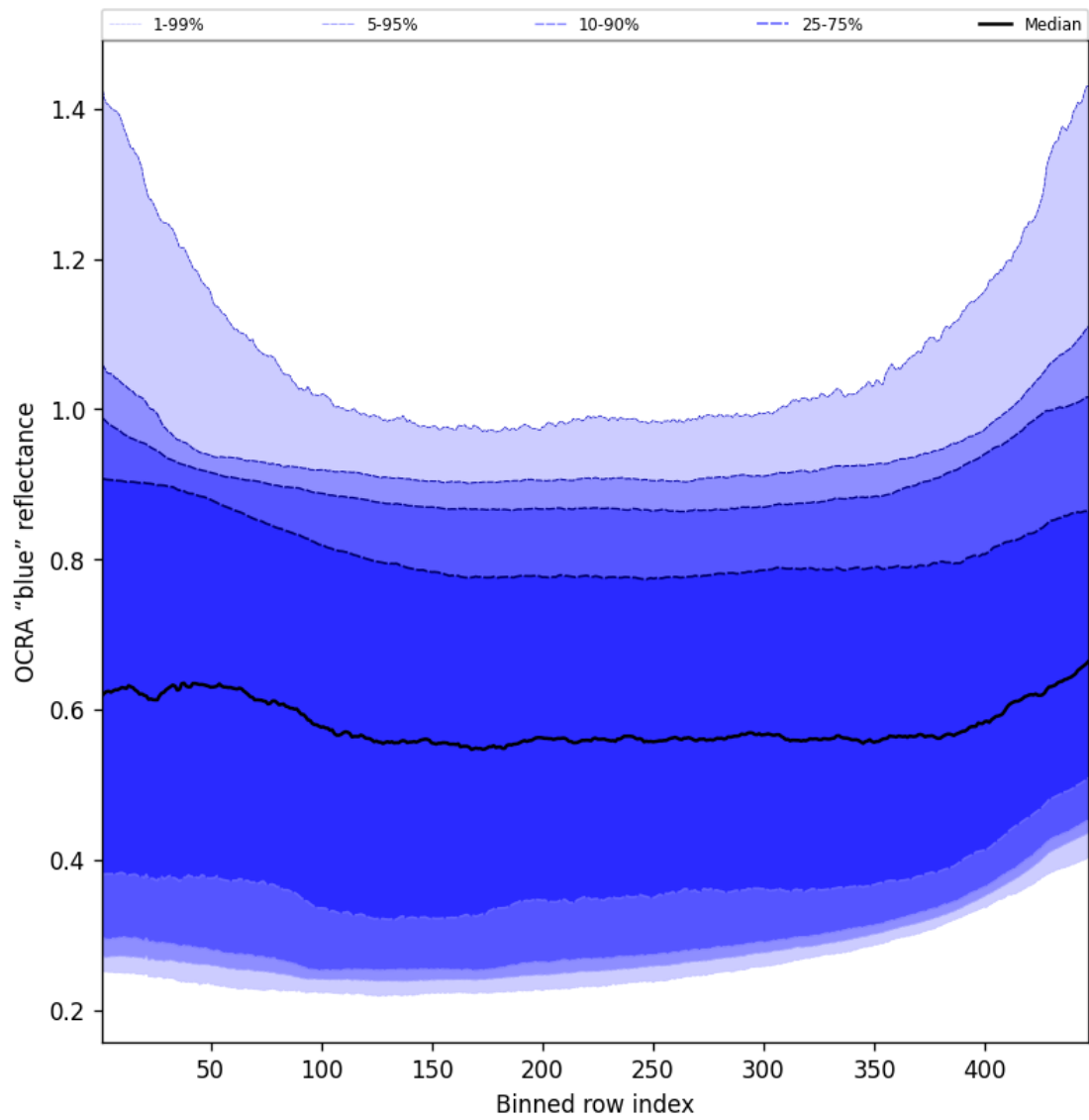
Figure 67: Along track statistics of "OCRA "blue" reflectance" for 2025-11-18 to 2025-11-20
