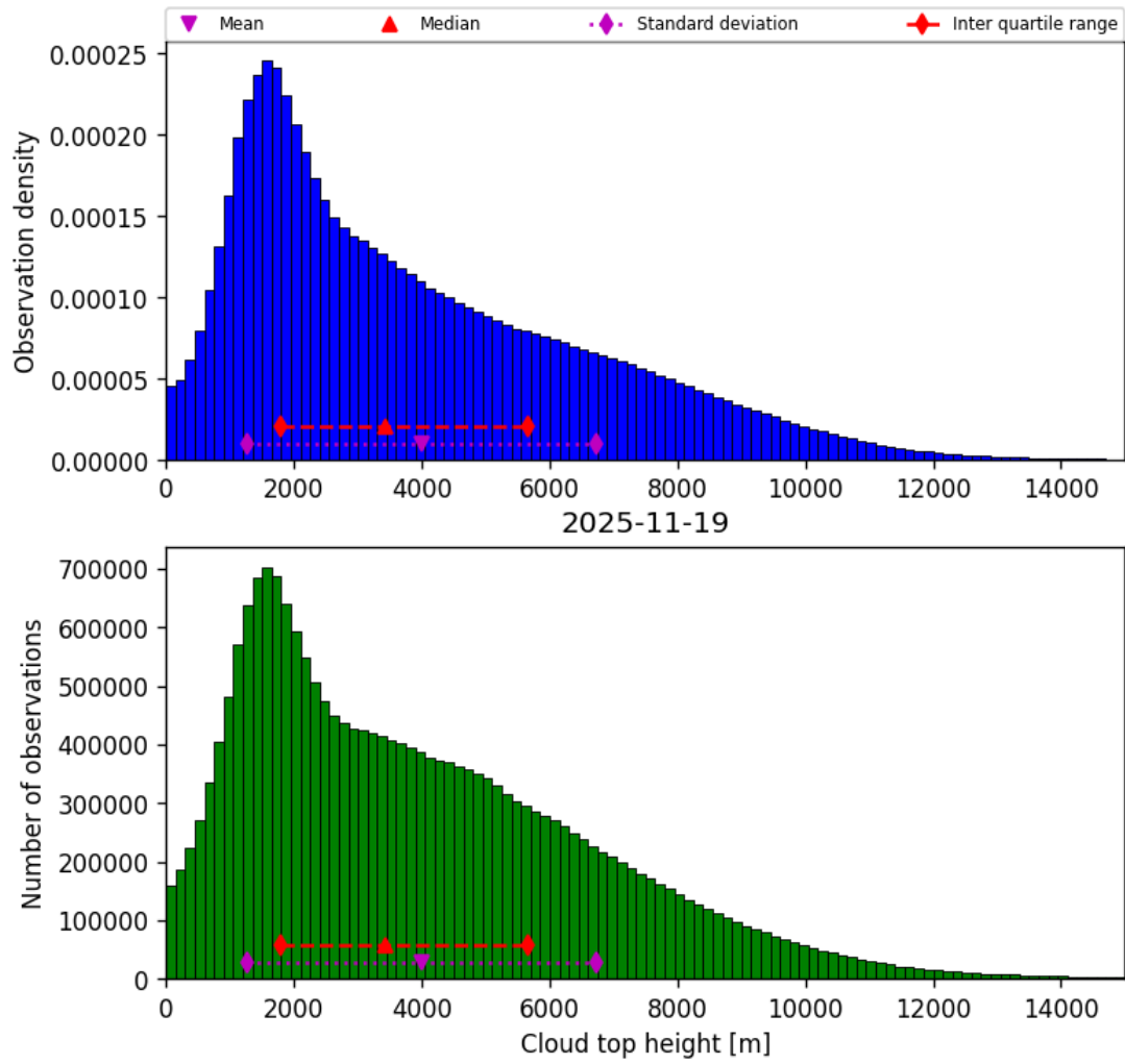
Figure 40: Histogram of “Cloud top height” for 2025-11-18 to 2025-11-20
