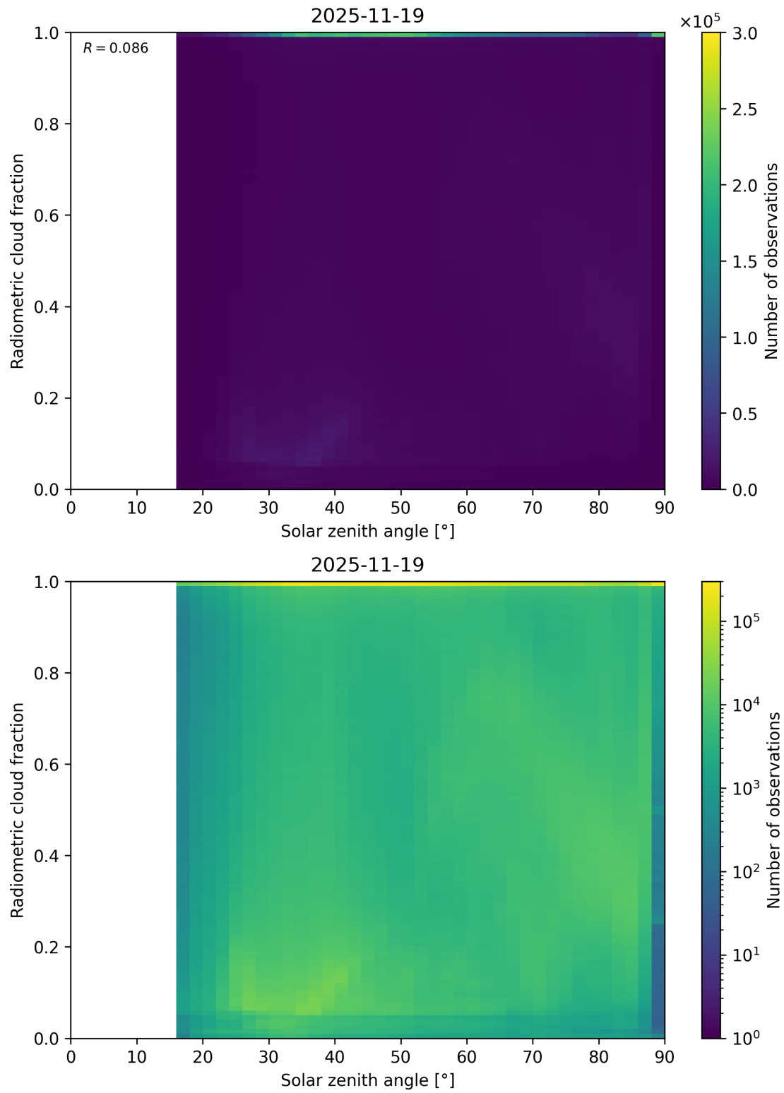
Figure 99: Scatter density plot of “Solar zenith angle” against “Radiometric cloud fraction” for 2025-11-18 to 2025-11-20.
