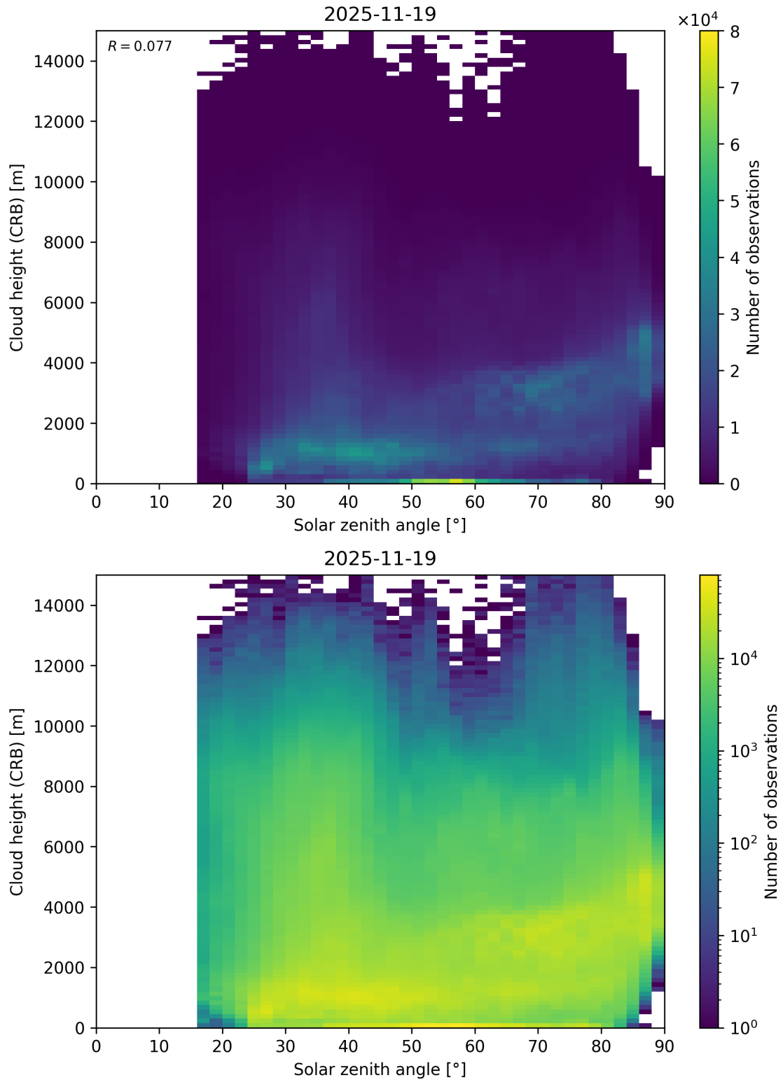
Figure 102: Scatter density plot of “Solar zenith angle” against “Cloud height (CRB)” for 2025-11-18 to 2025-11-20.
