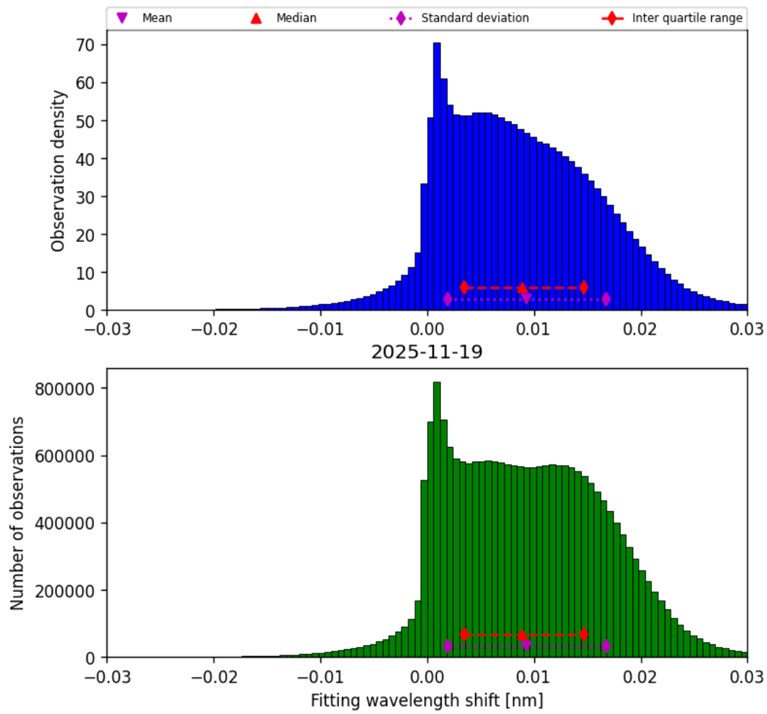
Figure 49: Histogram of “Fitting wavelength shift” for 2025-11-18 to 2025-11-20
