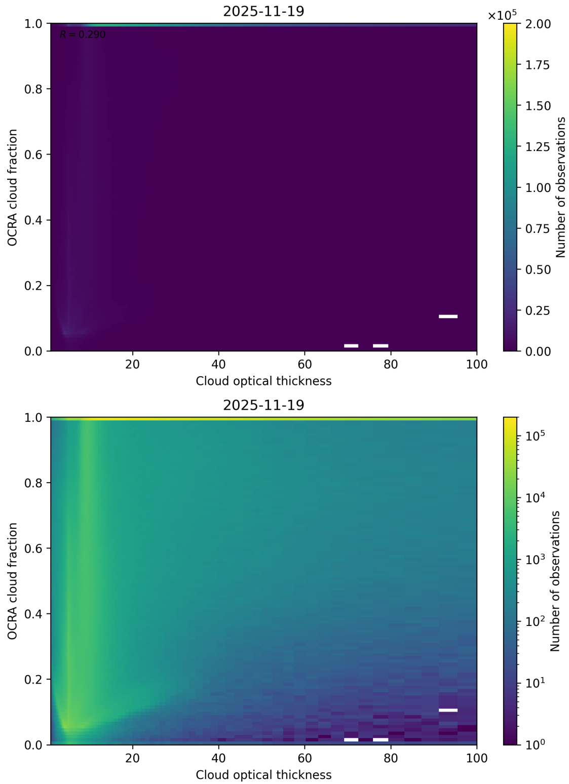
Figure 83: Scatter density plot of “Cloud optical thickness” against “OCRA cloud fraction” for 2025-11-18 to 2025-11-20.
