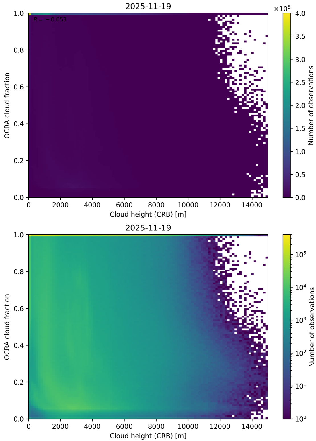
Figure 81: Scatter density plot of “Cloud height (CRB)” against “OCRA cloud fraction” for 2025-11-18 to 2025-11-20.
