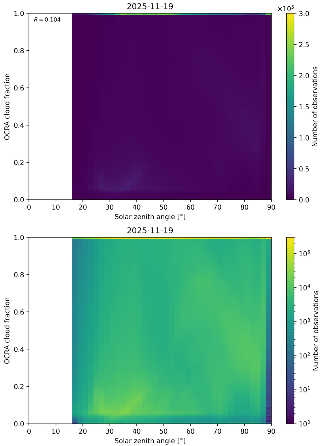
Figure 100: Scatter density plot of “Solar zenith angle” against “OCRA cloud fraction” for 2025-11-18 to 2025-11-20.
