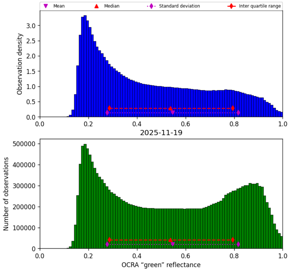
Figure 52: Histogram of “OCRA “green” reflectance” for 2025-11-18 to 2025-11-20
