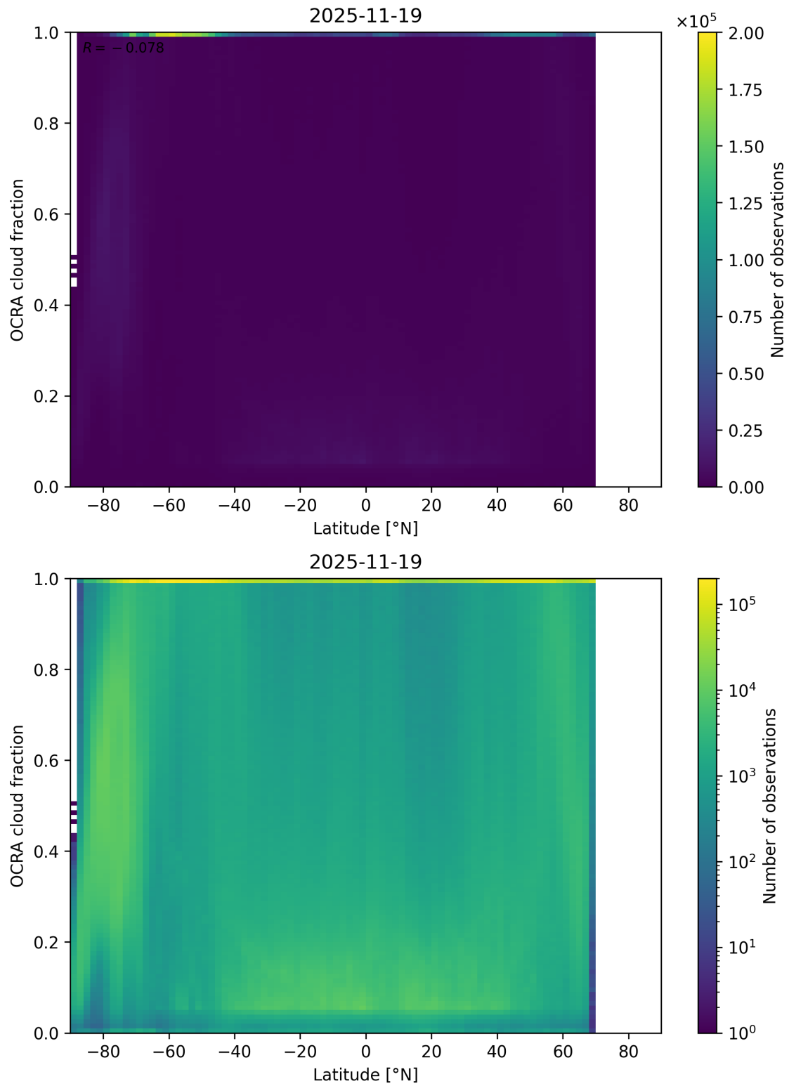
Figure 93: Scatter density plot of “Latitude” against “OCRA cloud fraction” for 2025-11-18 to 2025-11-20.
