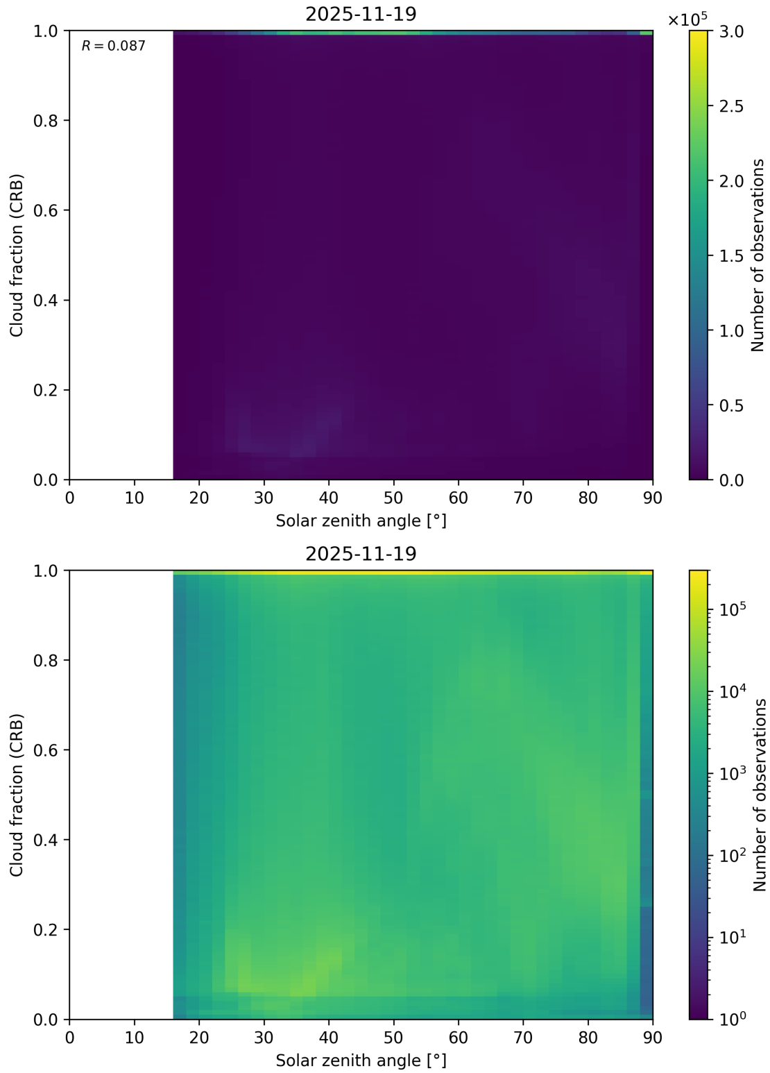
Figure 101: Scatter density plot of “Solar zenith angle” against “Cloud fraction (CRB)” for 2025-11-18 to 2025-11-20.
