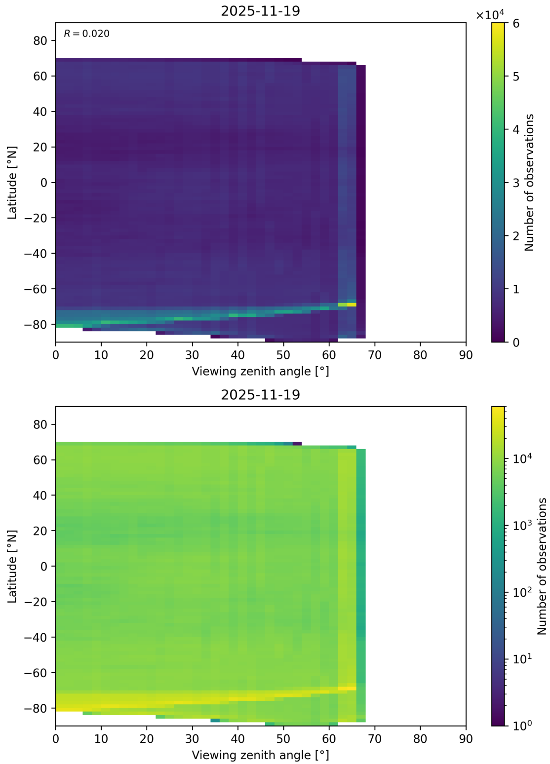
Figure 113: Scatter density plot of “Viewing zenith angle” against “Latitude” for 2025-11-18 to 2025-11-20.
