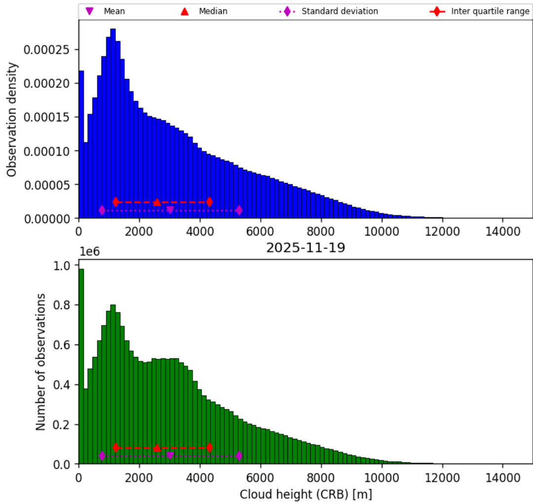
Figure 43: Histogram of “Cloud height (CRB)” for 2025-11-18 to 2025-11-20
