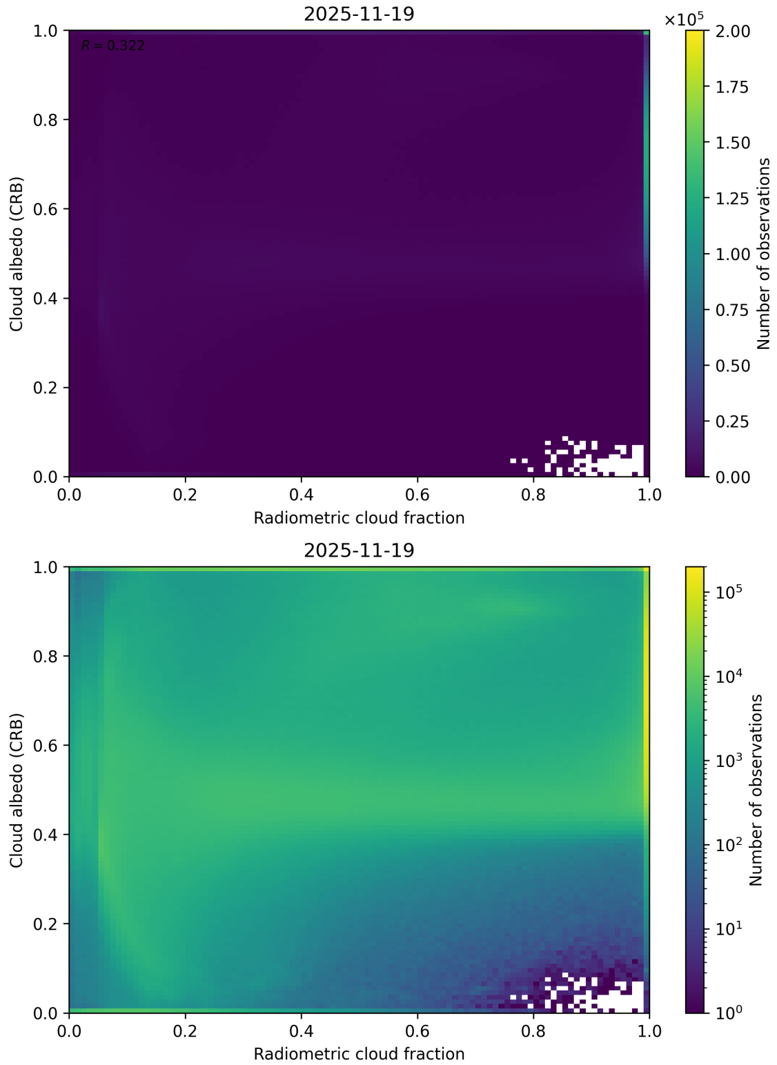
Figure 71: Scatter density plot of “Radiometric cloud fraction” against “Cloud albedo (CRB)” for 2025-11-18 to 2025-11-20.
