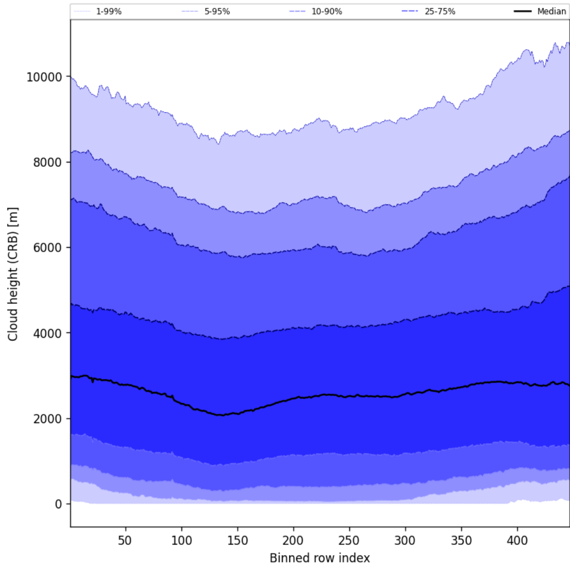
Figure 59: Along track statistics of “Cloud height (CRB)” for 2025-11-18 to 2025-11-20
