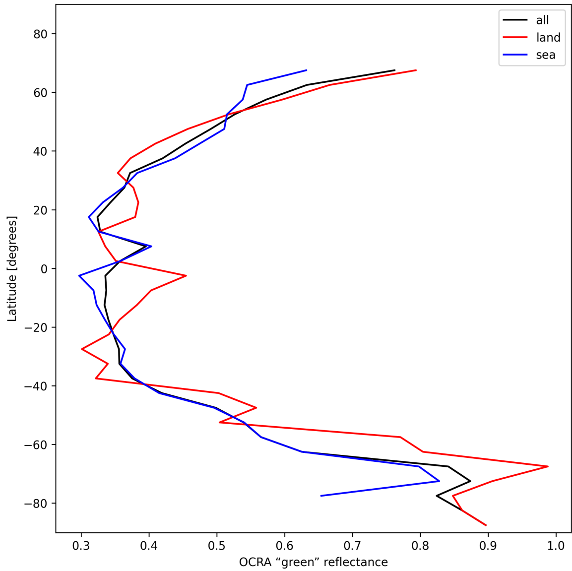
Figure 36: Zonal average of “OCRA “green” reflectance” for 2025-11-18 to 2025-11-20.
