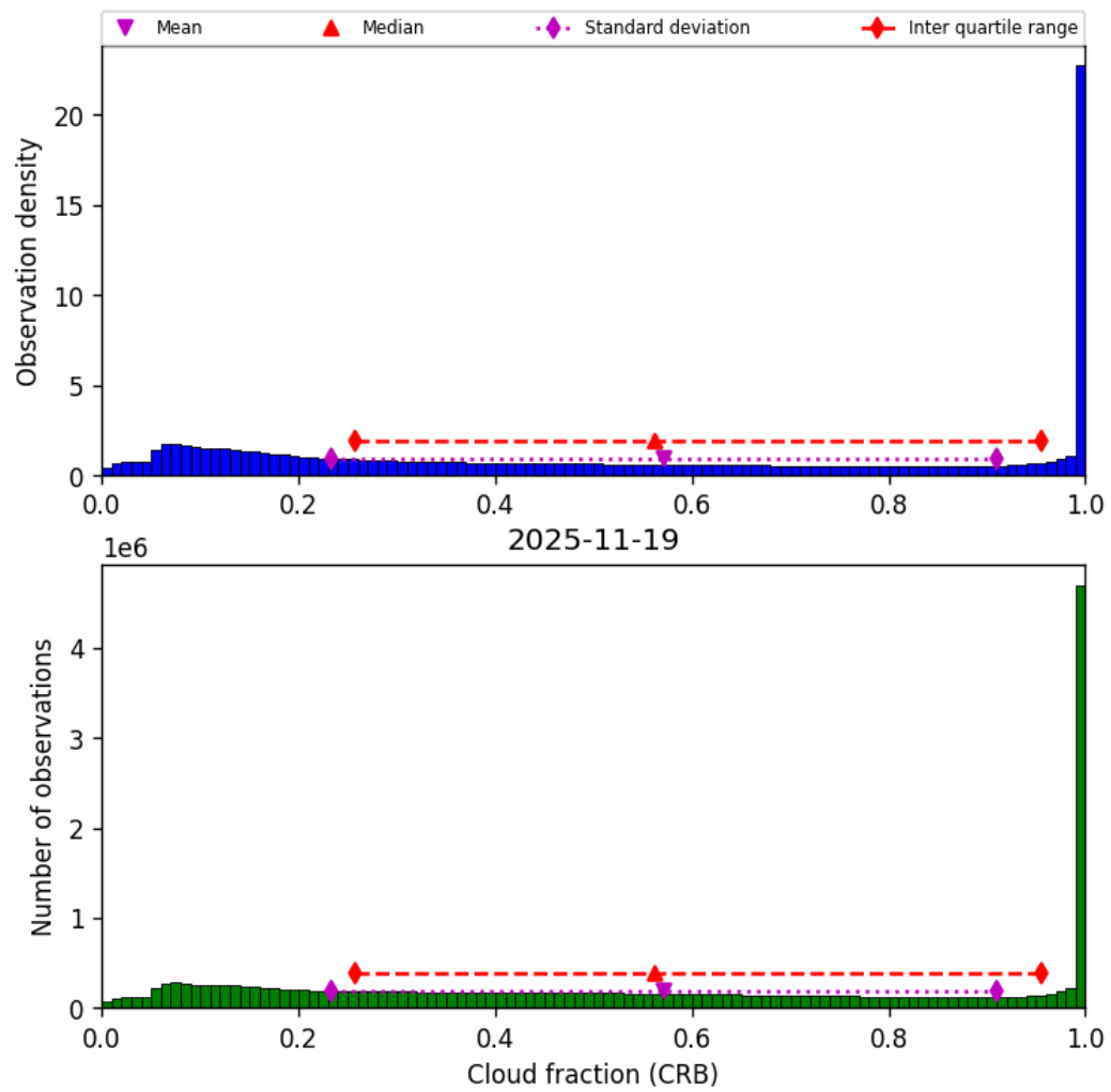
Figure 42: Histogram of “Cloud fraction (CRB)” for 2025-11-18 to 2025-11-20
