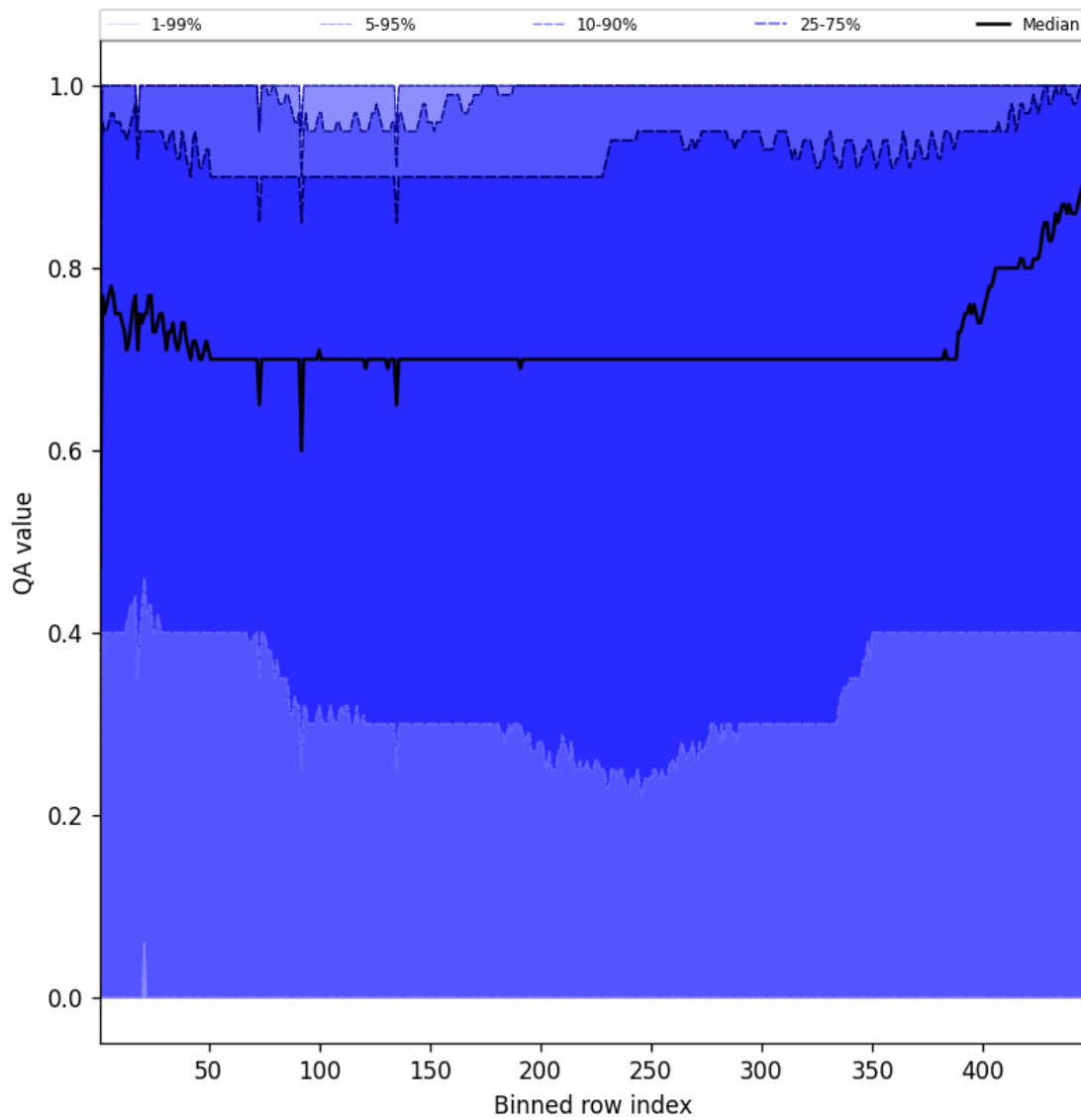
Figure 54: Along track statistics of “QA value” for 2025-11-18 to 2025-11-20
