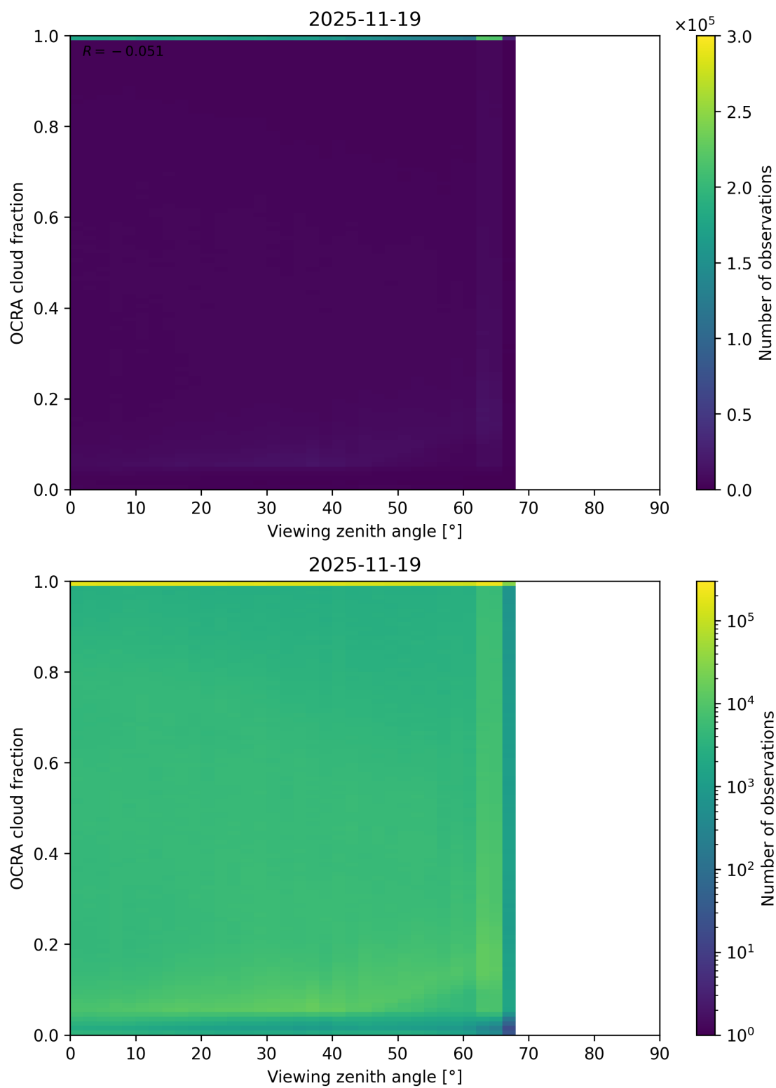
Figure 108: Scatter density plot of “Viewing zenith angle” against “OCRA cloud fraction” for 2025-11-18 to 2025-11-20.
