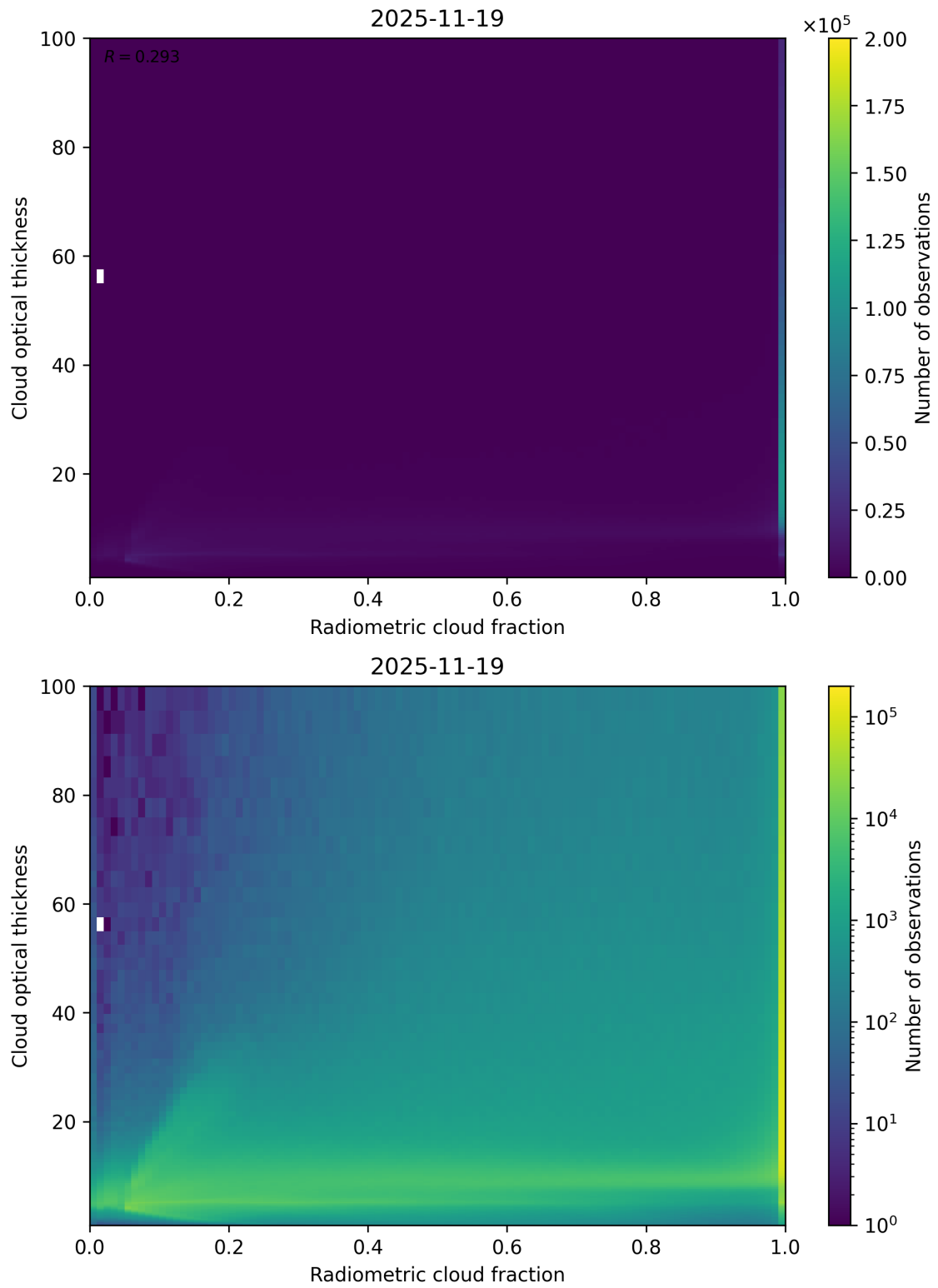
Figure 75: Scatter density plot of “Radiometric cloud fraction” against “Cloud optical thickness” for 2025-11-18 to 2025-11-20.
