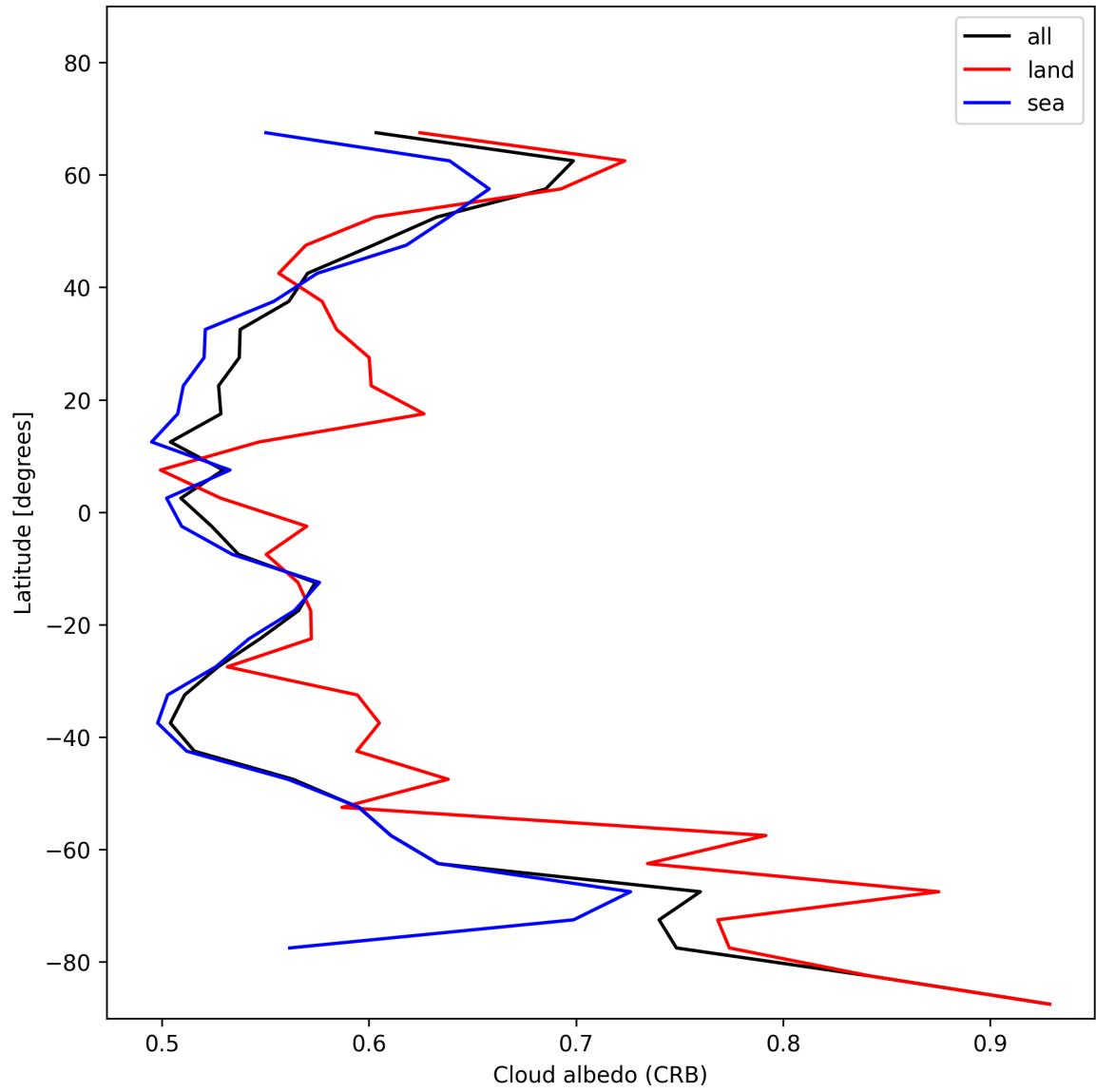
Figure 28: Zonal average of “Cloud albedo (CRB)” for 2025-11-18 to 2025-11-20.
