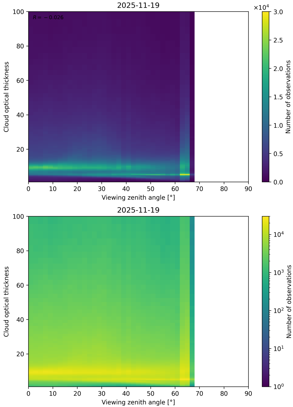
Figure 111: Scatter density plot of “Viewing zenith angle” against “Cloud optical thickness” for 2025-11-18 to 2025-11-20.
