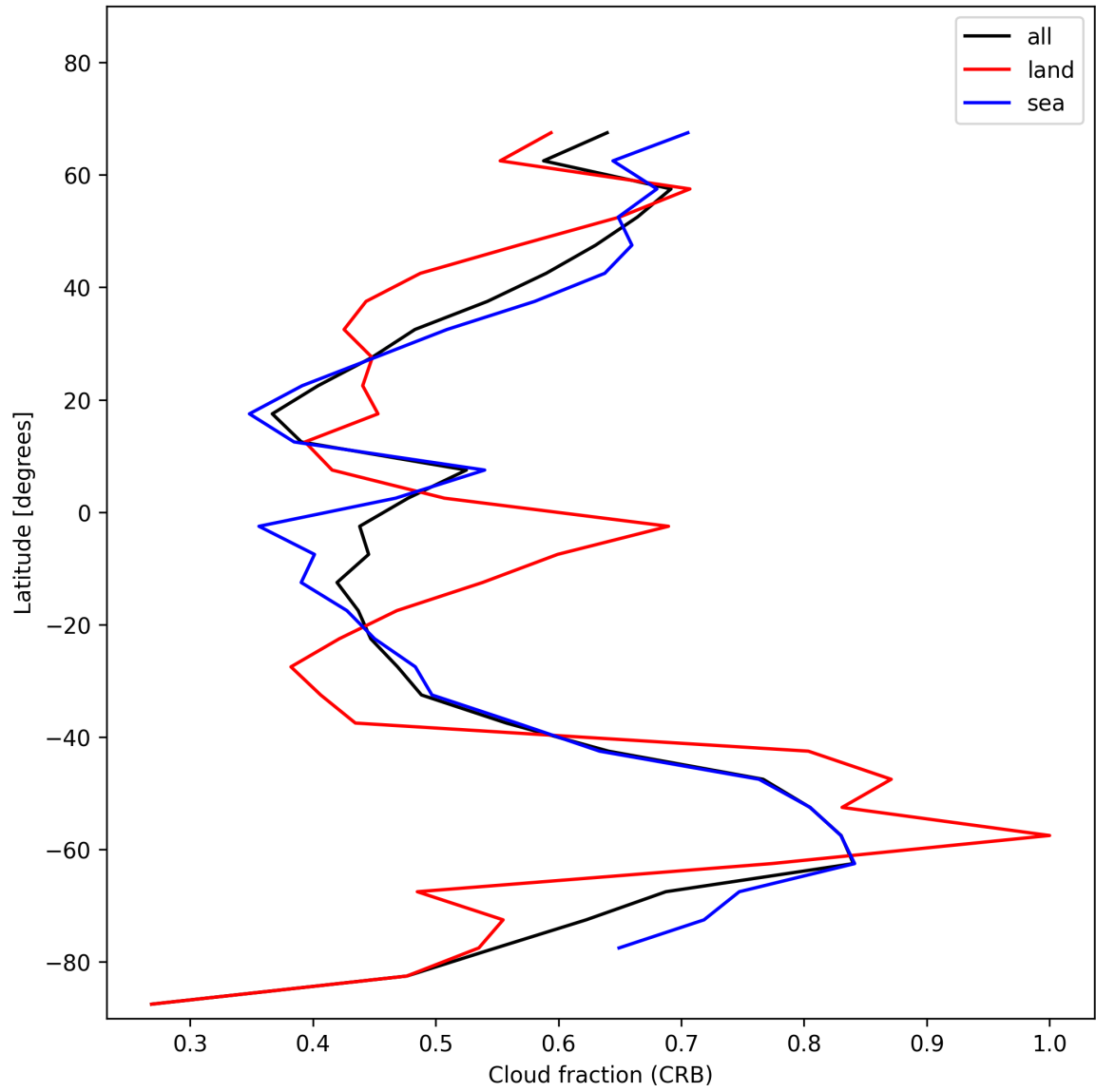
Figure 26: Zonal average of “Cloud fraction (CRB)” for 2025-11-18 to 2025-11-20.
