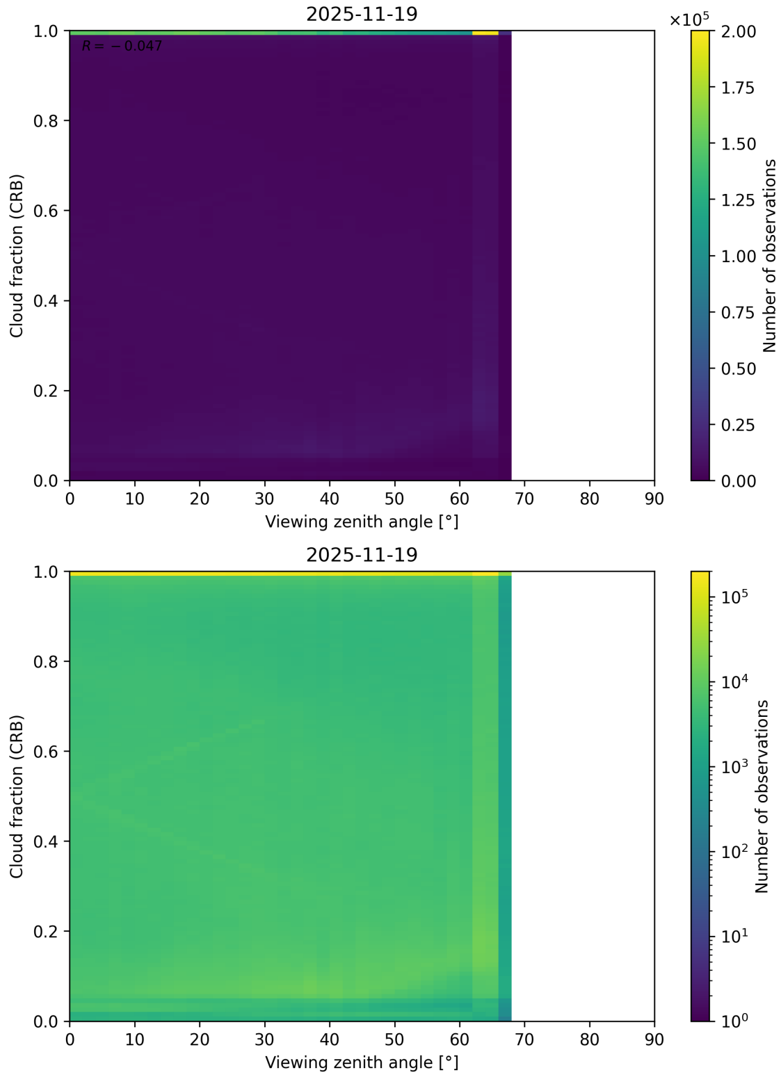
Figure 109: Scatter density plot of “Viewing zenith angle” against “Cloud fraction (CRB)” for 2025-11-18 to 2025-11-20.
