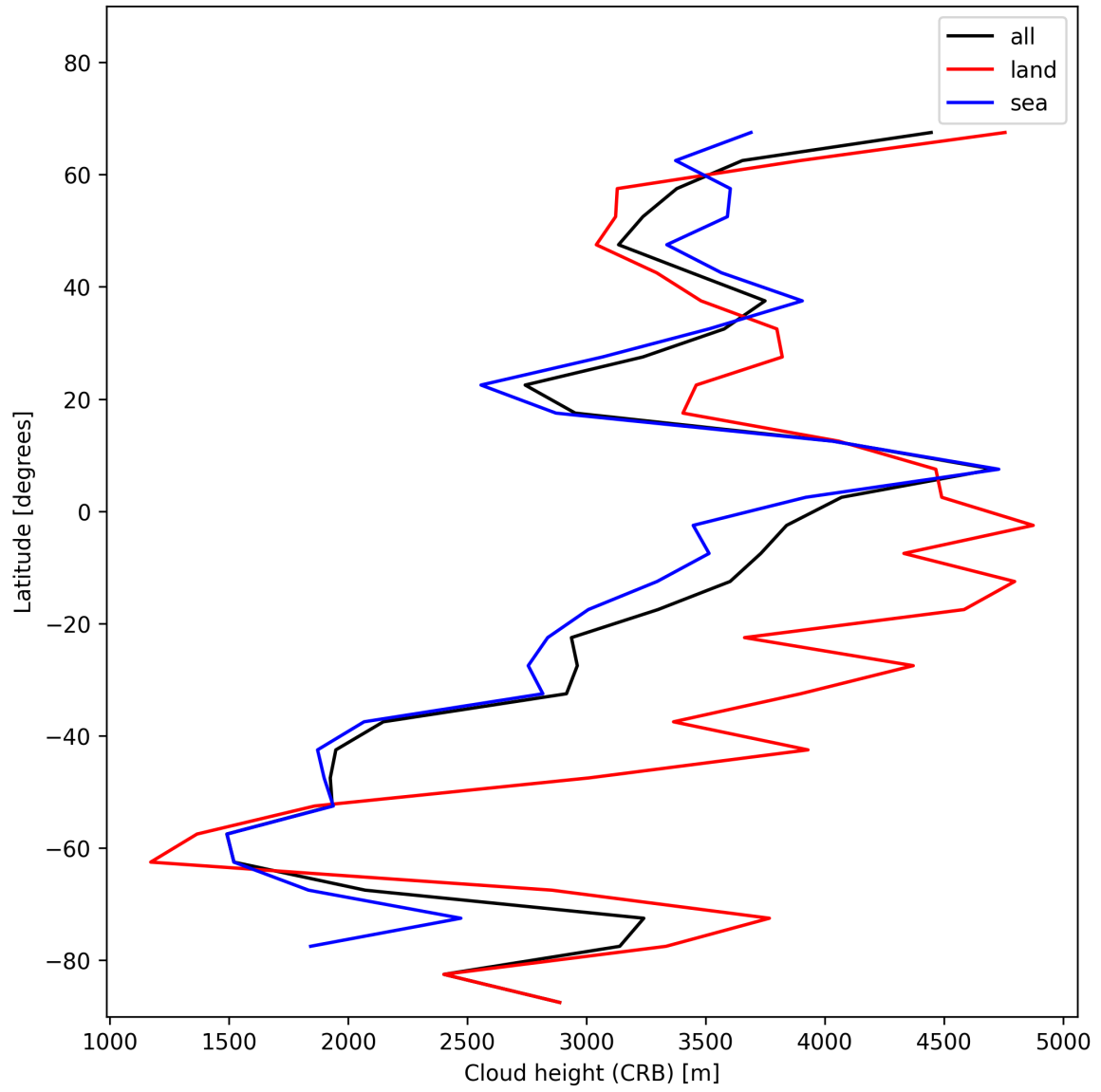
Figure 27: Zonal average of “Cloud height (CRB)” for 2025-11-18 to 2025-11-20.
