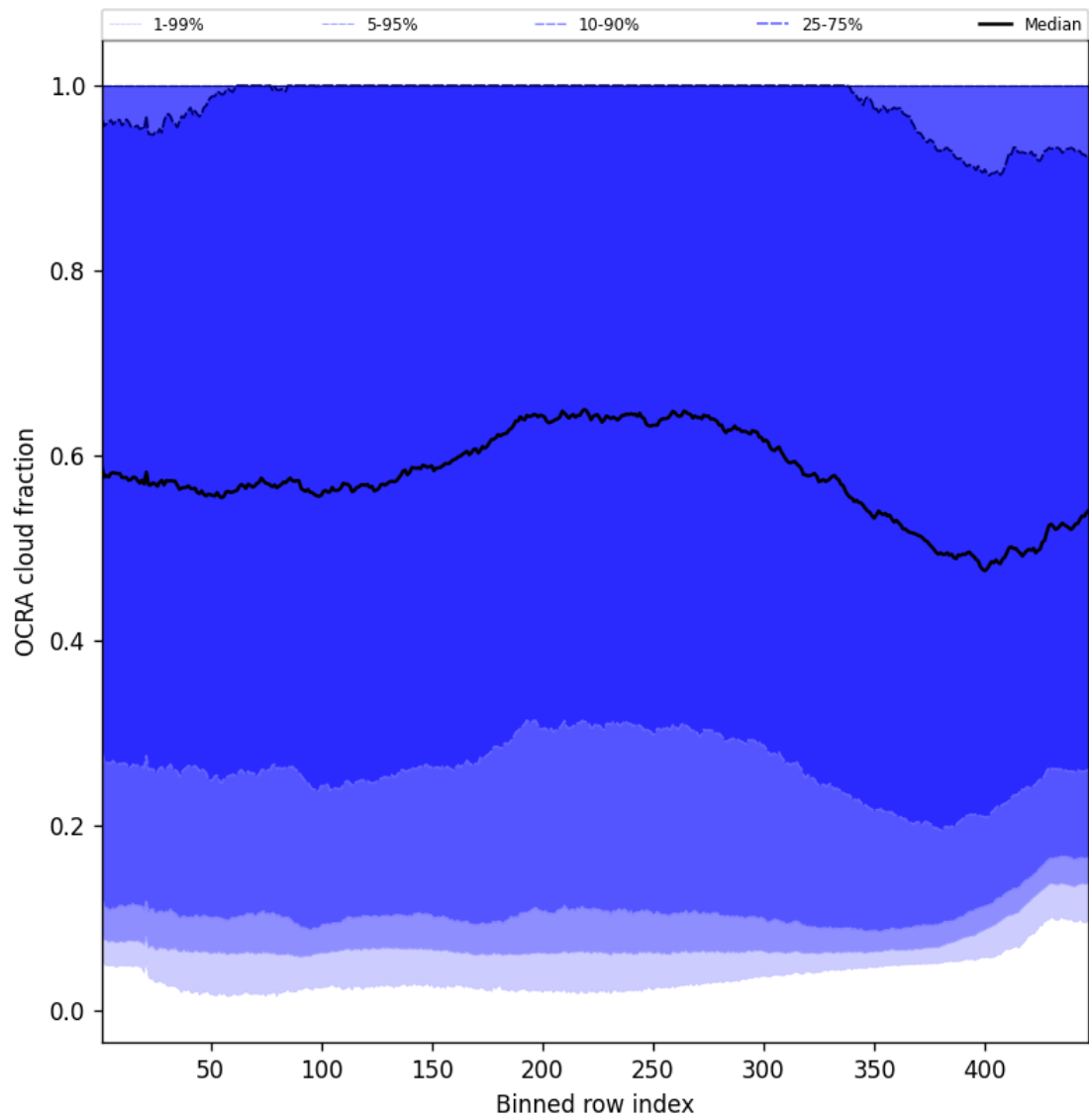
Figure 66: Along track statistics of “OCRA cloud fraction” for 2025-11-18 to 2025-11-20
