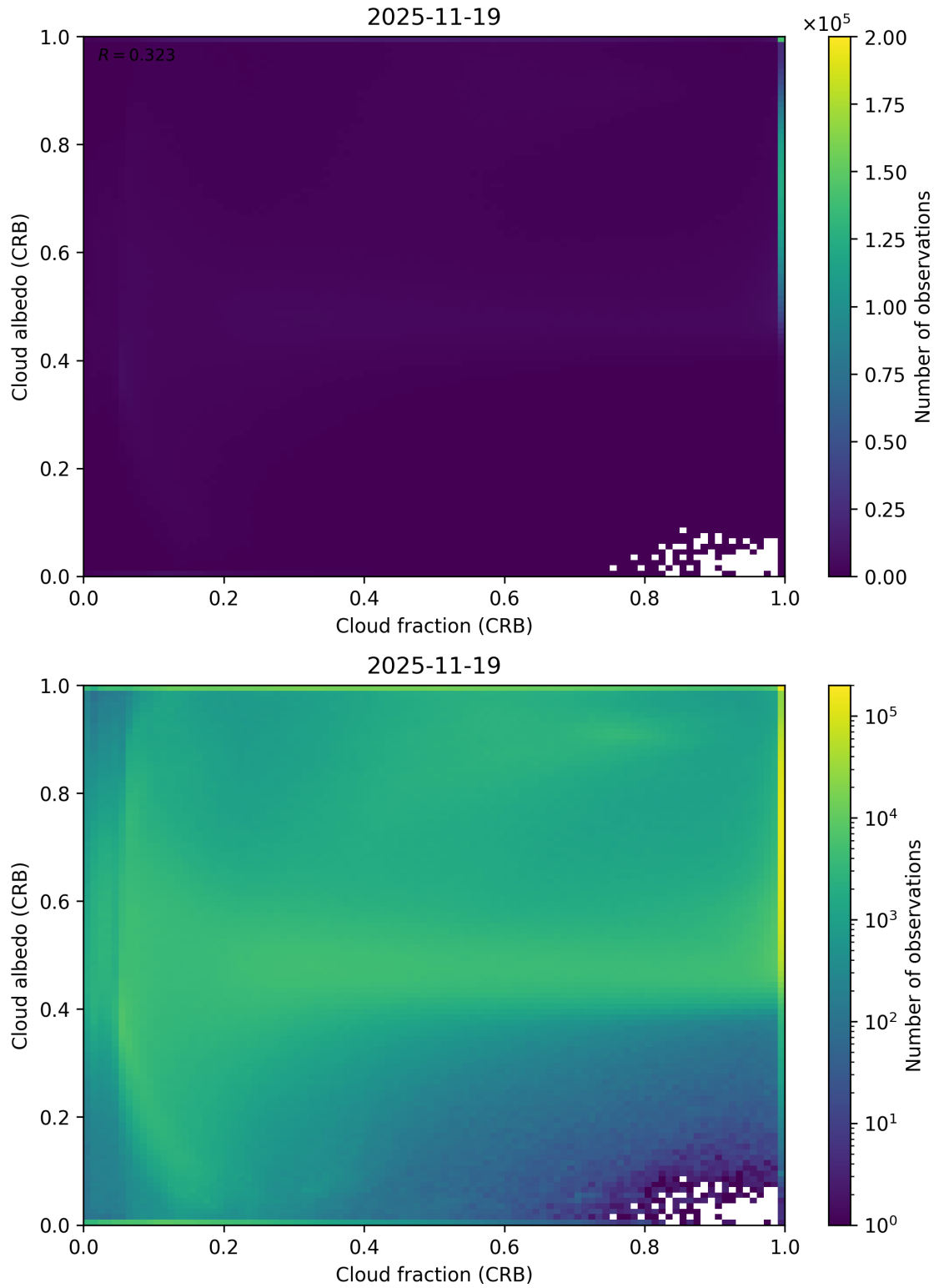
Figure 77: Scatter density plot of “Cloud fraction (CRB)” against “Cloud albedo (CRB)” for 2025-11-18 to 2025-11-20.
