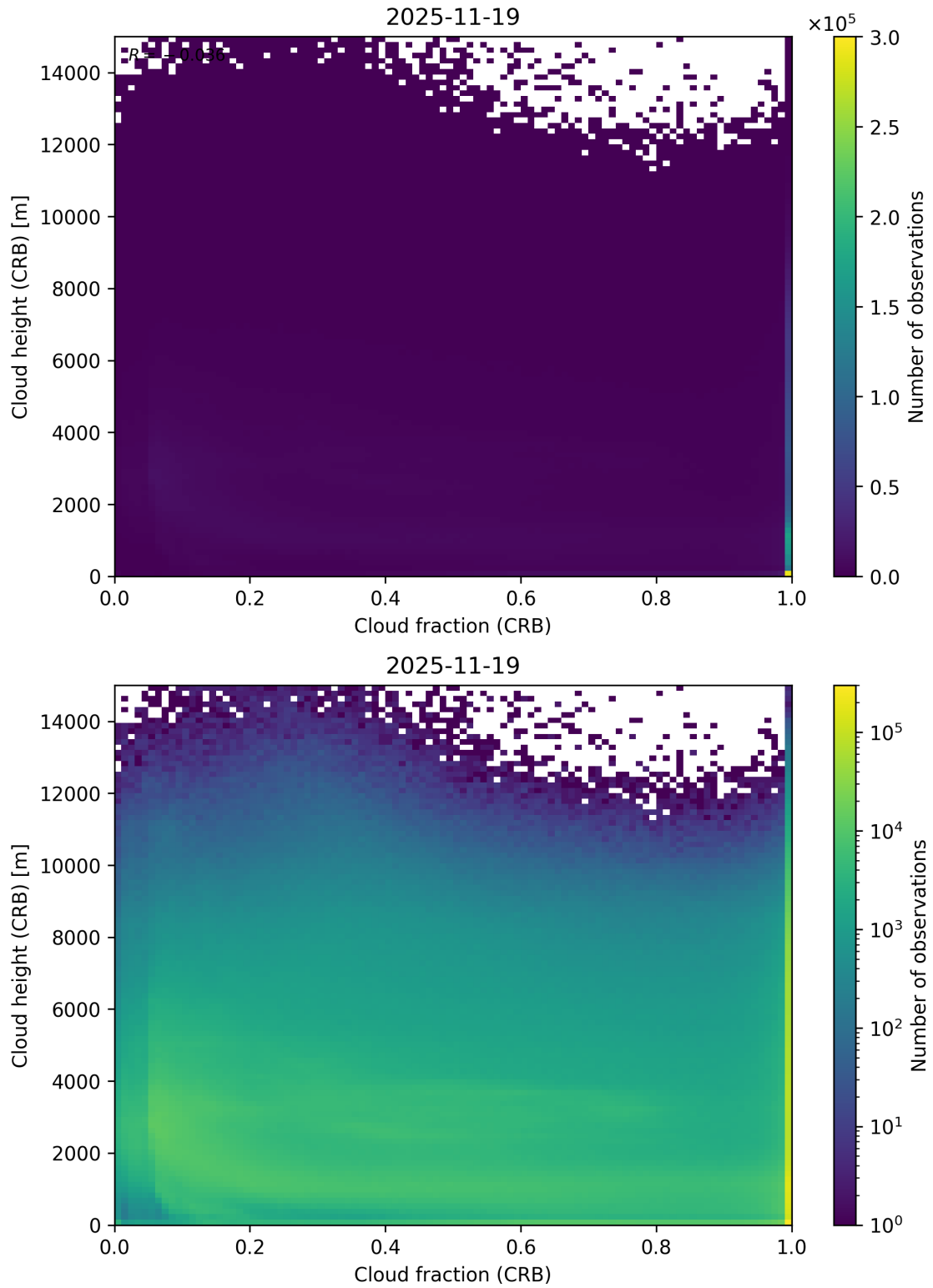
Figure 79: Scatter density plot of “Cloud fraction (CRB)” against “Cloud height (CRB)” for 2025-11-18 to 2025-11-20.
