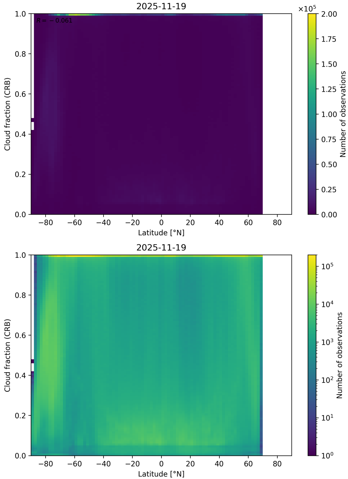
Figure 94: Scatter density plot of “Latitude” against “Cloud fraction (CRB)” for 2025-11-18 to 2025-11-20.
