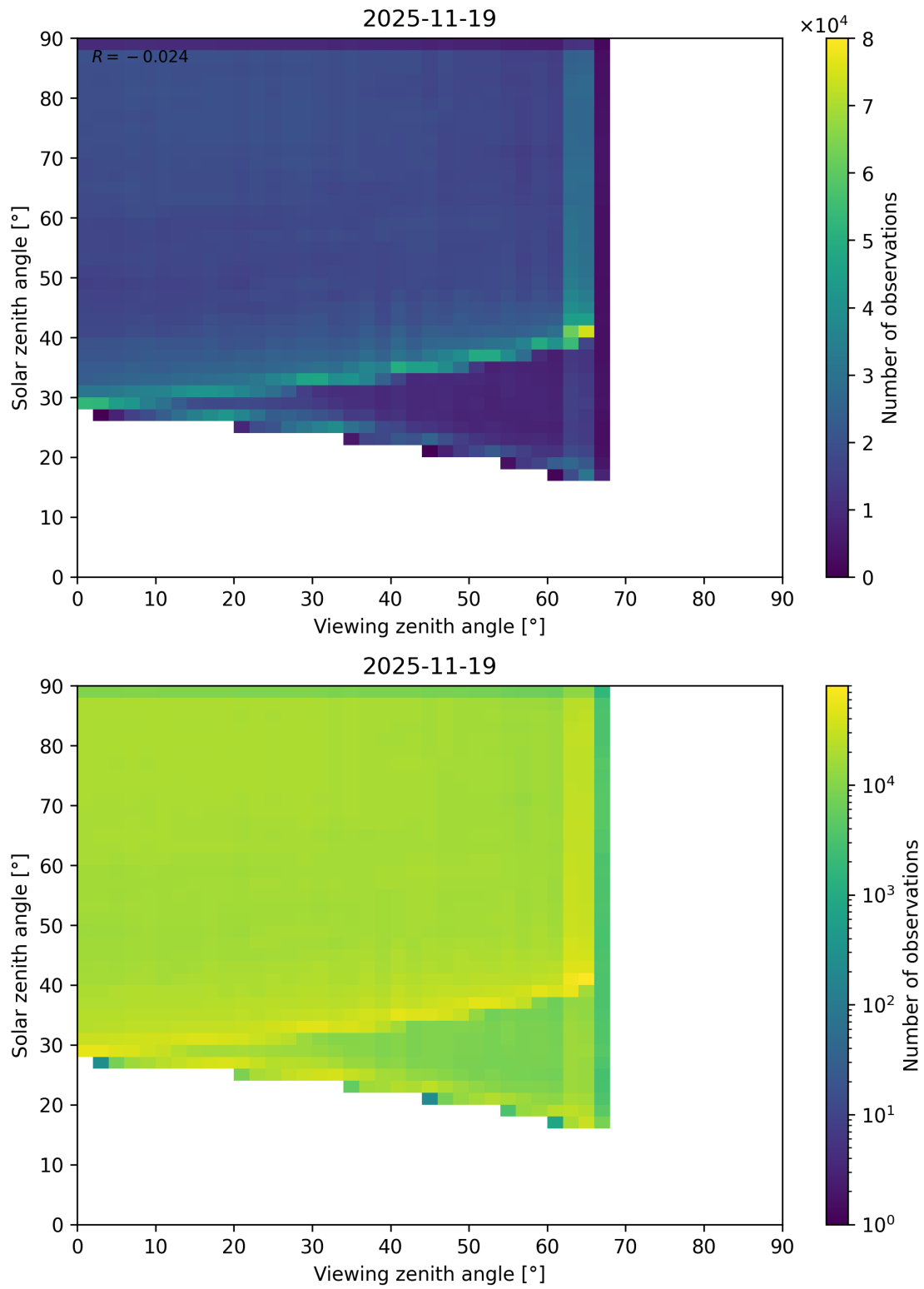
Figure 114: Scatter density plot of “Viewing zenith angle” against “Solar zenith angle” for 2025-11-18 to 2025-11-20.
