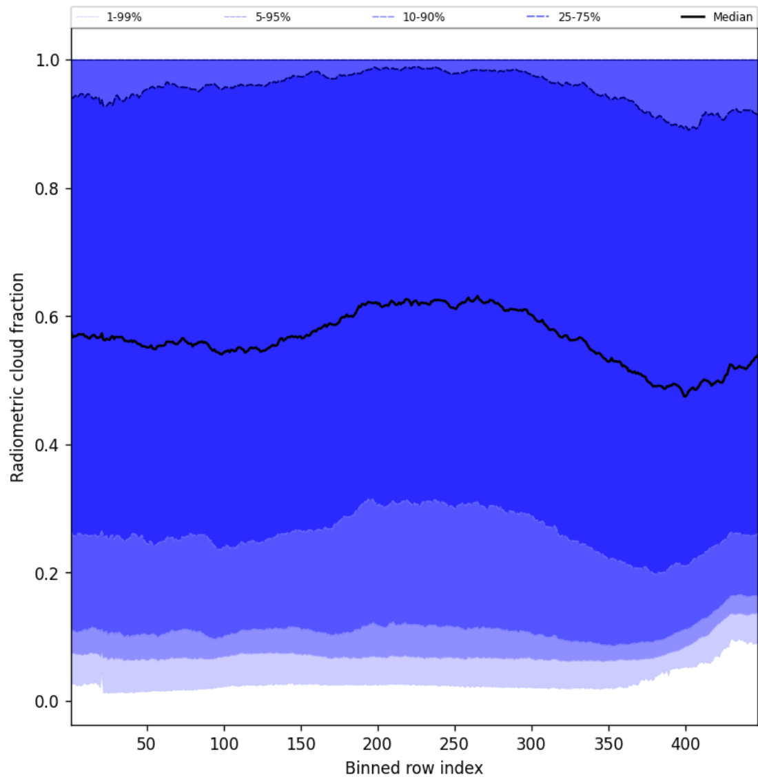
Figure 55: Along track statistics of “Radiometric cloud fraction” for 2025-11-18 to 2025-11-20
