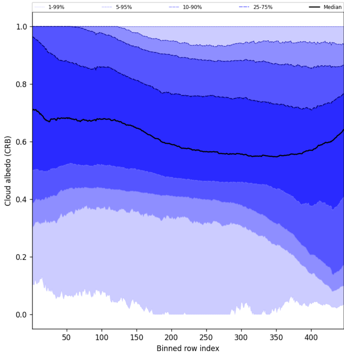
Figure 60: Along track statistics of “Cloud albedo (CRB)” for 2025-11-18 to 2025-11-20
