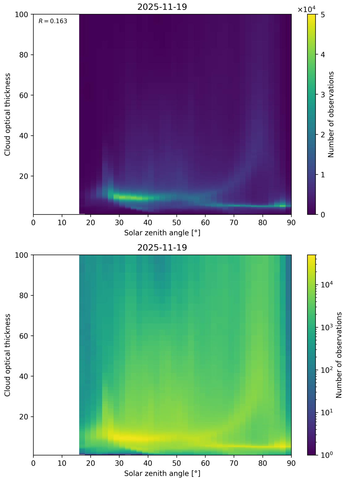
Figure 103: Scatter density plot of “Solar zenith angle” against “Cloud optical thickness” for 2025-11-18 to 2025-11-20.
