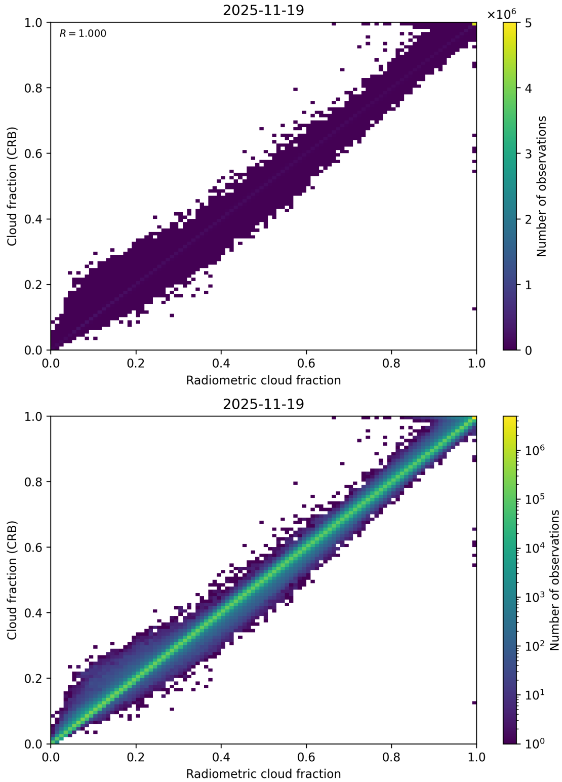
Figure 73: Scatter density plot of “Radiometric cloud fraction” against “Cloud fraction (CRB)” for 2025-11-18 to 2025-11-20.
