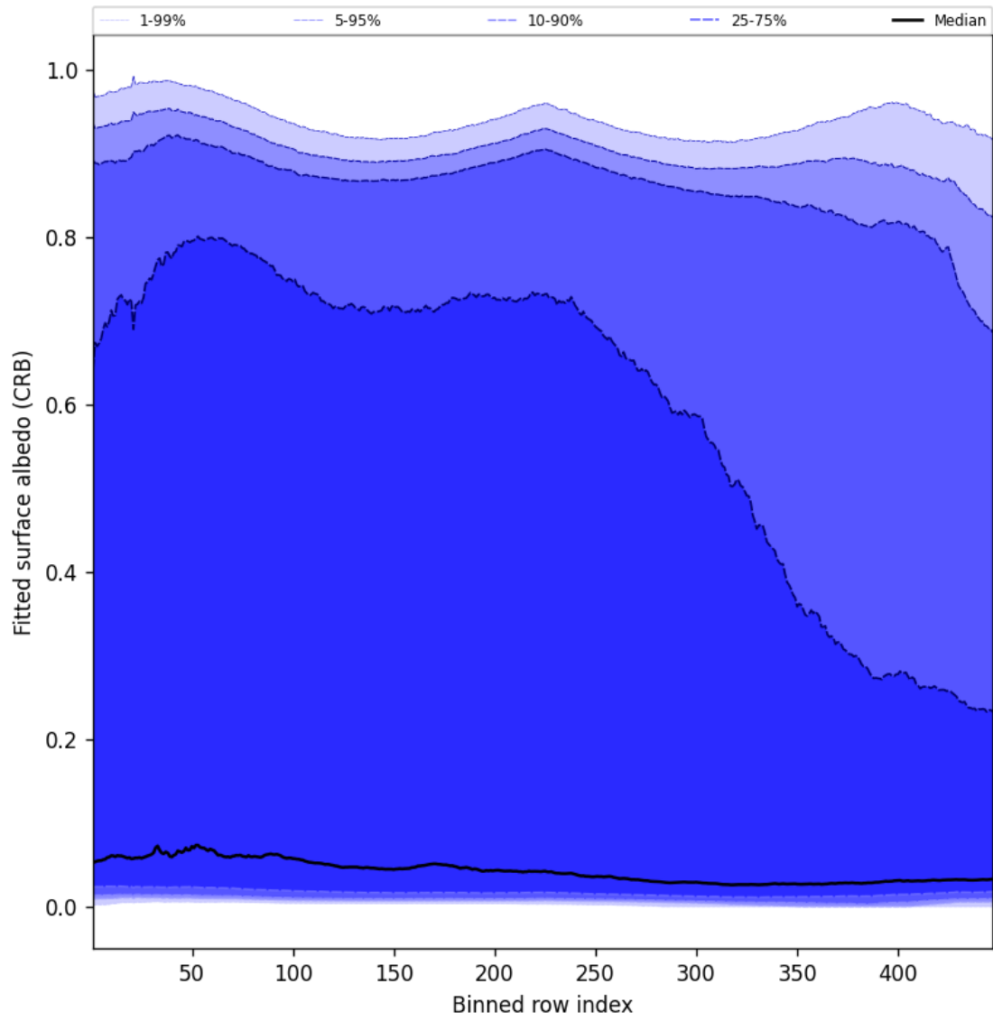
Figure 62: Along track statistics of “Fitted surface albedo (CRB)” for 2025-11-18 to 2025-11-20
