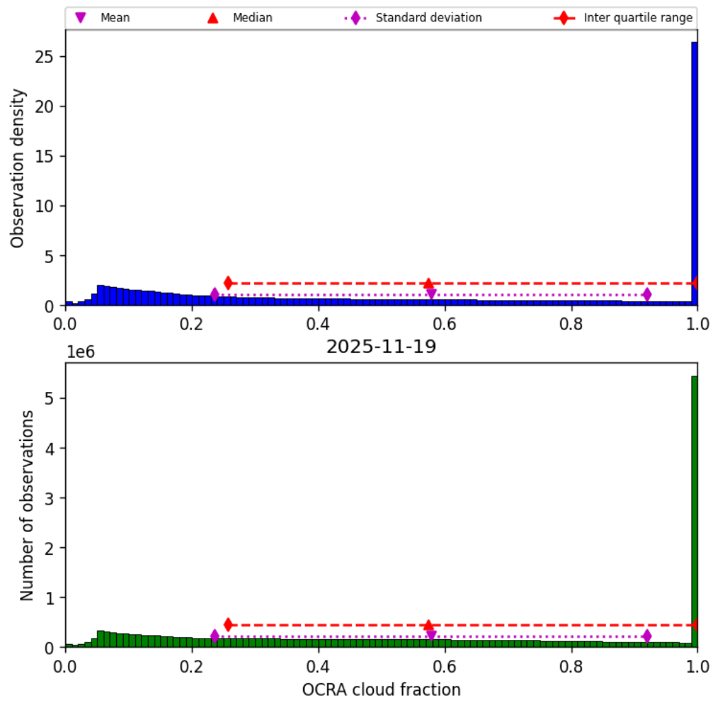
Figure 50: Histogram of “OCRA cloud fraction” for 2025-11-18 to 2025-11-20
