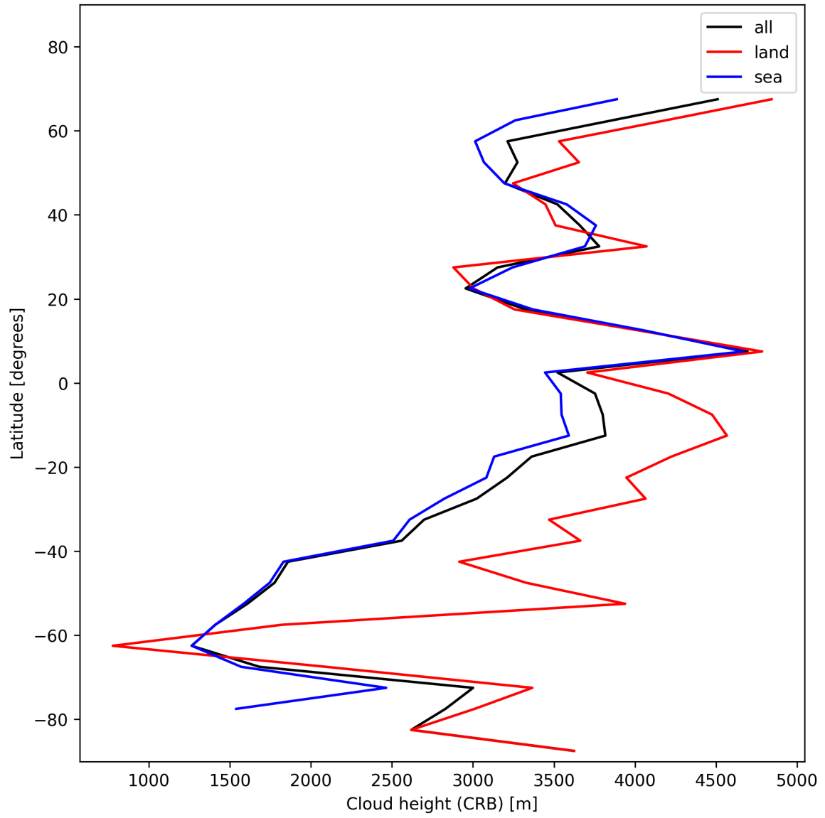
Figure 27: Zonal average of “Cloud height (CRB)” for 2025-11-20 to 2025-11-22.
