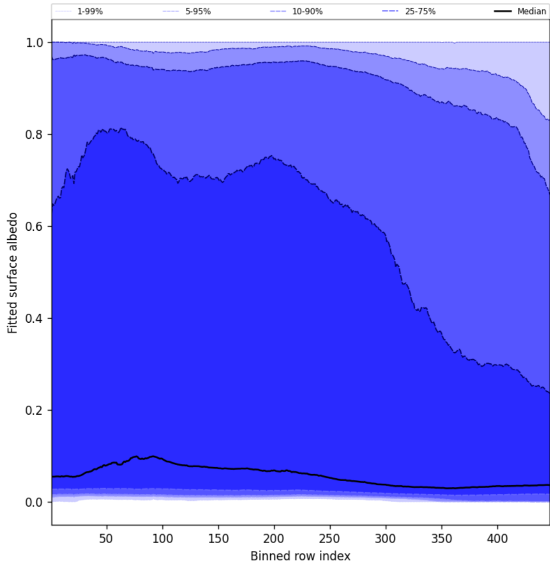
Figure 61: Along track statistics of “Fitted surface albedo” for 2025-11-20 to 2025-11-22
