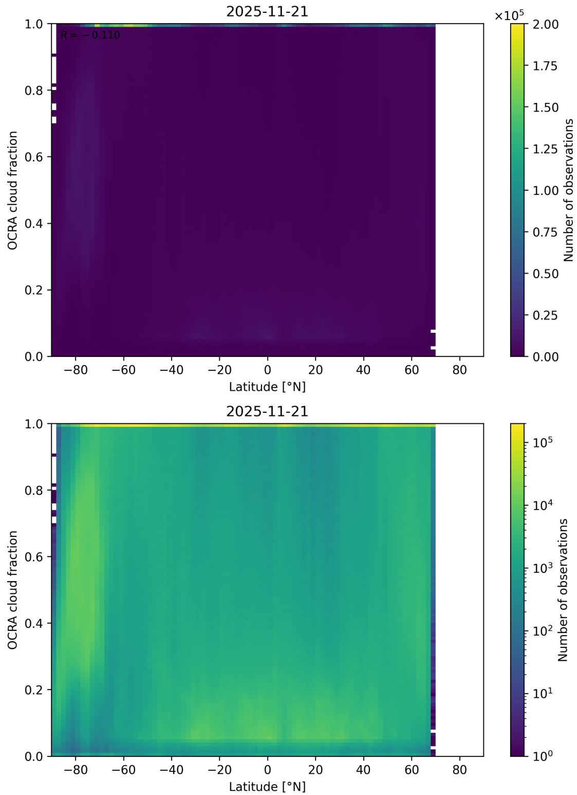
Figure 93: Scatter density plot of “Latitude” against “OCRA cloud fraction” for 2025-11-20 to 2025-11-22.
