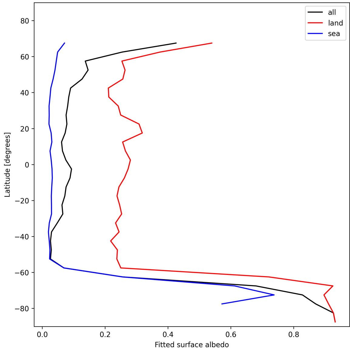
Figure 29: Zonal average of “Fitted surface albedo” for 2025-11-20 to 2025-11-22.
