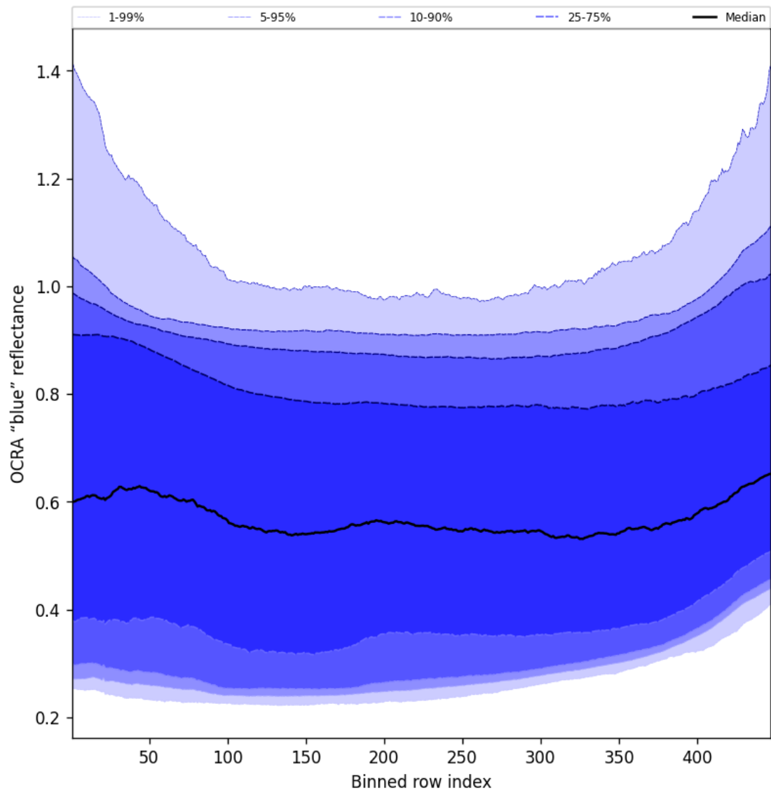
Figure 67: Along track statistics of "OCRA "blue" reflectance" for 2025-11-20 to 2025-11-22
