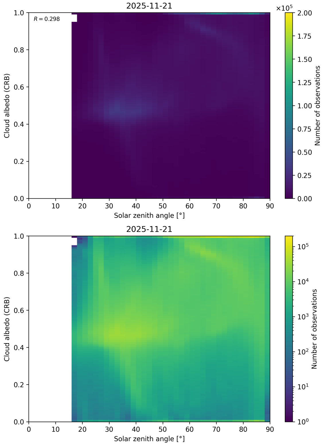
Figure 98: Scatter density plot of “Solar zenith angle” against “Cloud albedo (CRB)” for 2025-11-20 to 2025-11-22.
