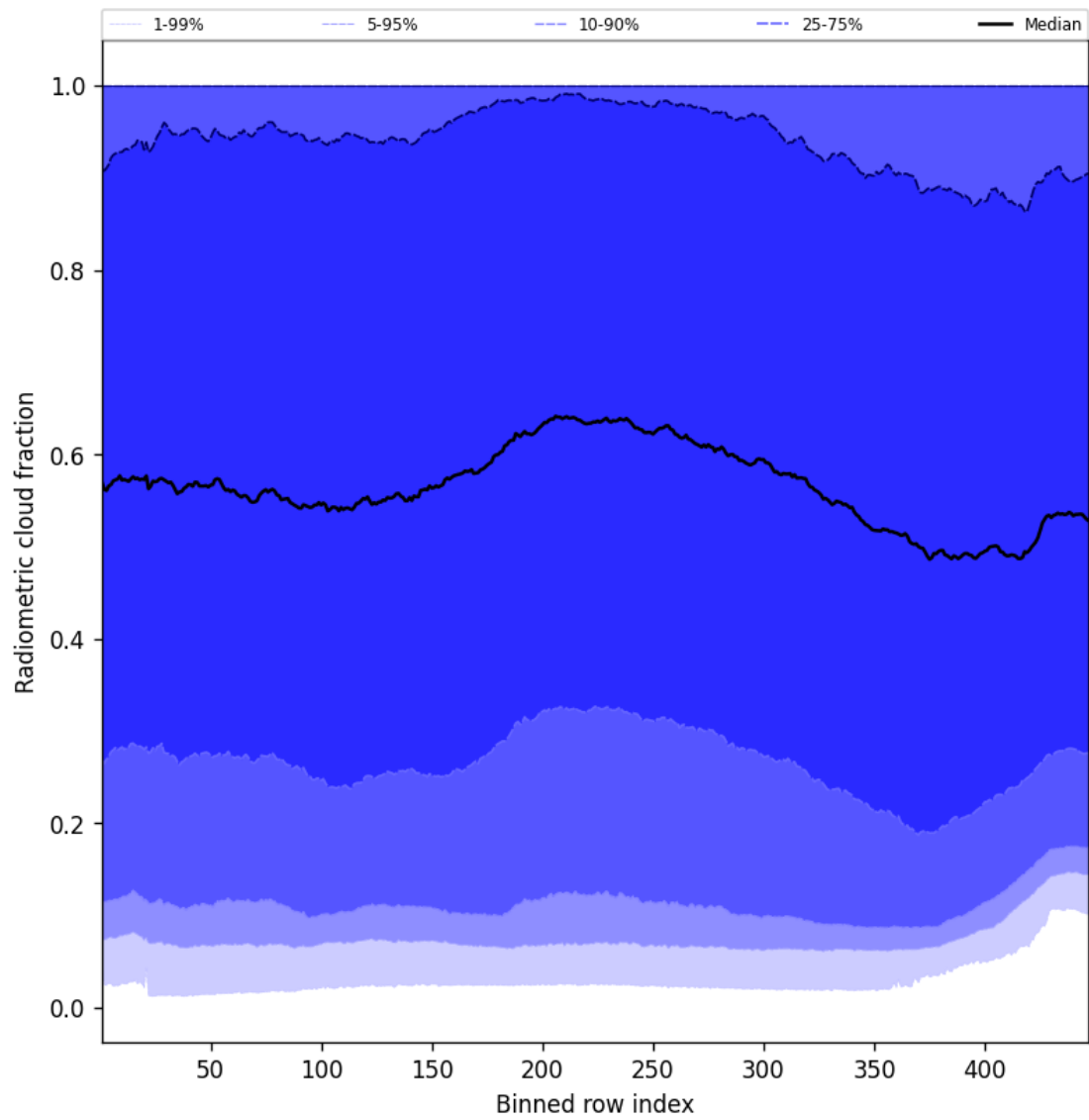
Figure 55: Along track statistics of “Radiometric cloud fraction” for 2025-11-20 to 2025-11-22
