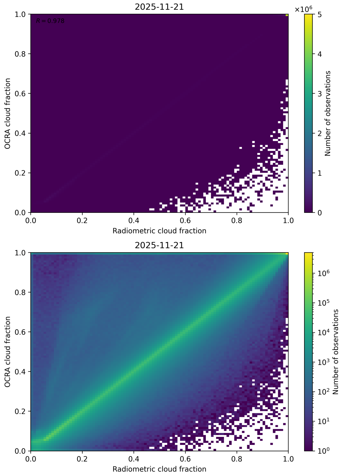
Figure 72: Scatter density plot of “Radiometric cloud fraction” against “OCRA cloud fraction” for 2025-11-20 to 2025-11-22.
