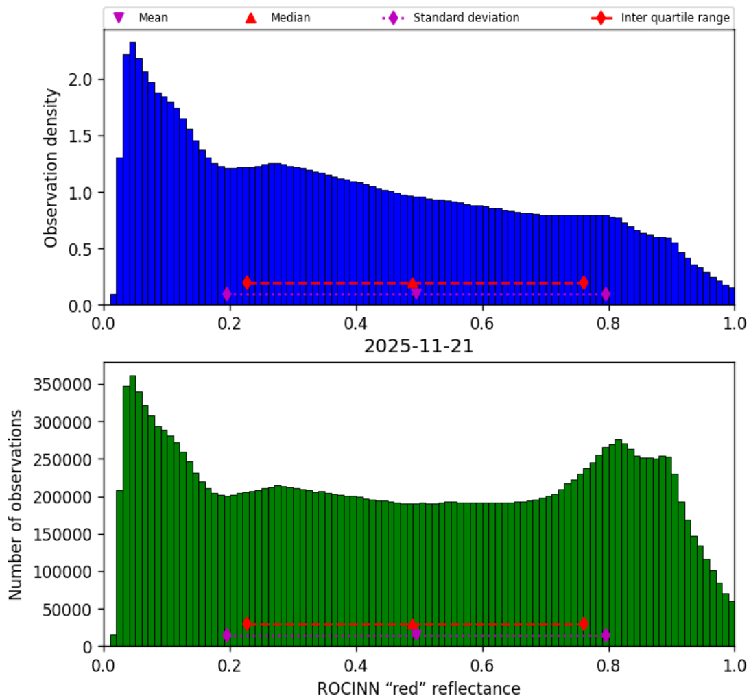
Figure 53: Histogram of “ROCINN “red” reflectance” for 2025-11-20 to 2025-11-22
