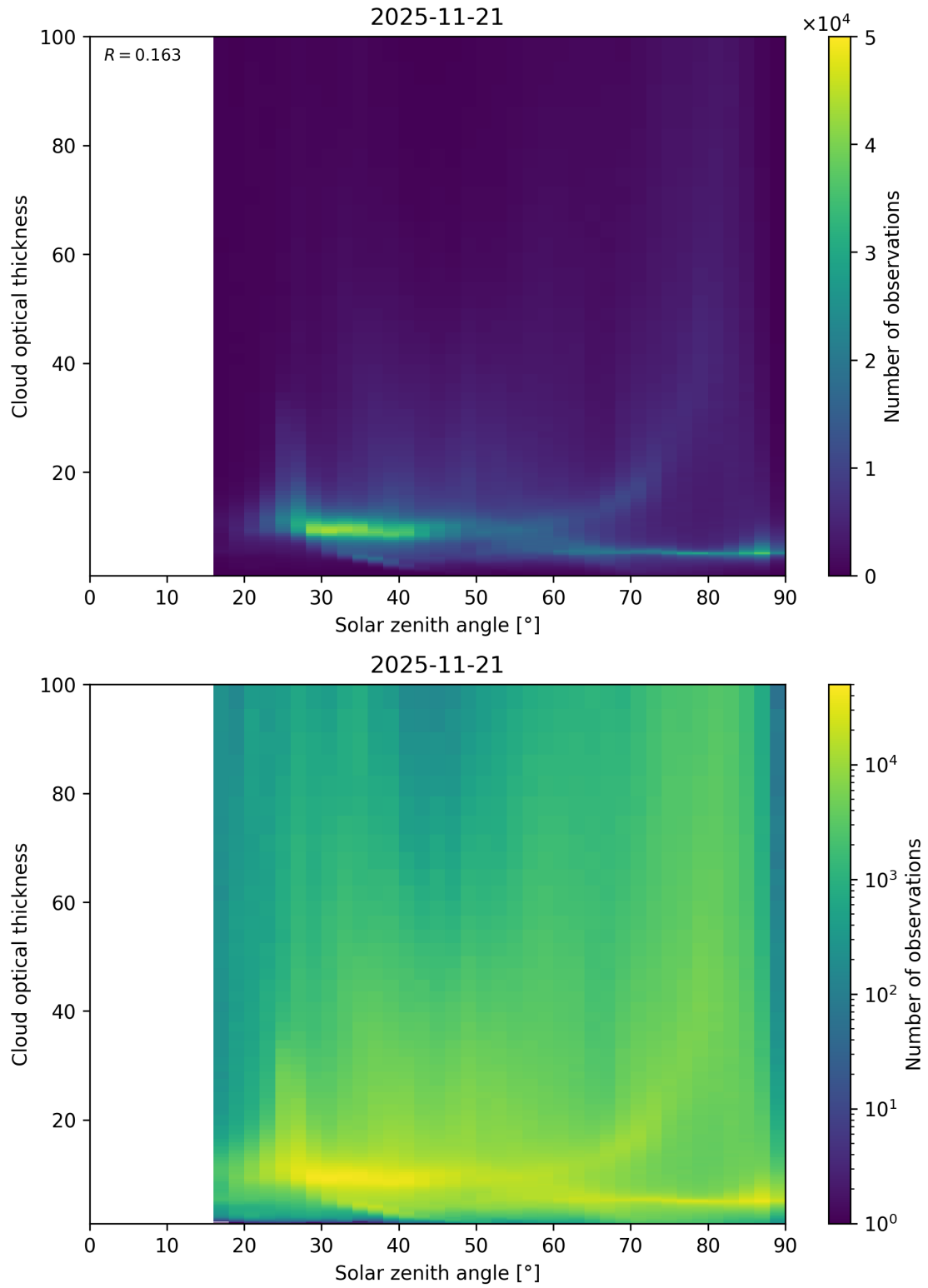
Figure 103: Scatter density plot of “Solar zenith angle” against “Cloud optical thickness” for 2025-11-20 to 2025-11-22.
