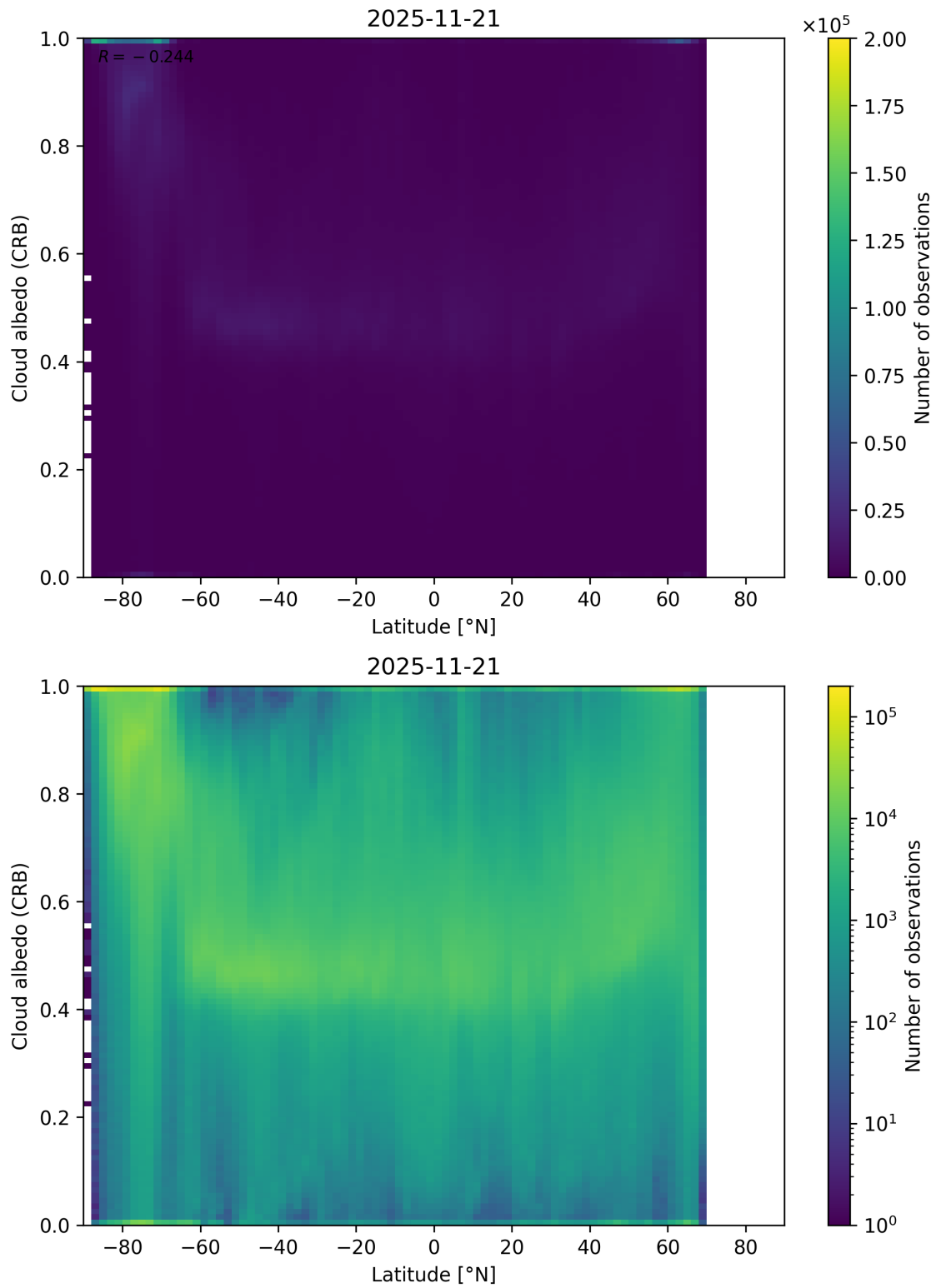
Figure 91: Scatter density plot of “Latitude” against “Cloud albedo (CRB)” for 2025-11-20 to 2025-11-22.
