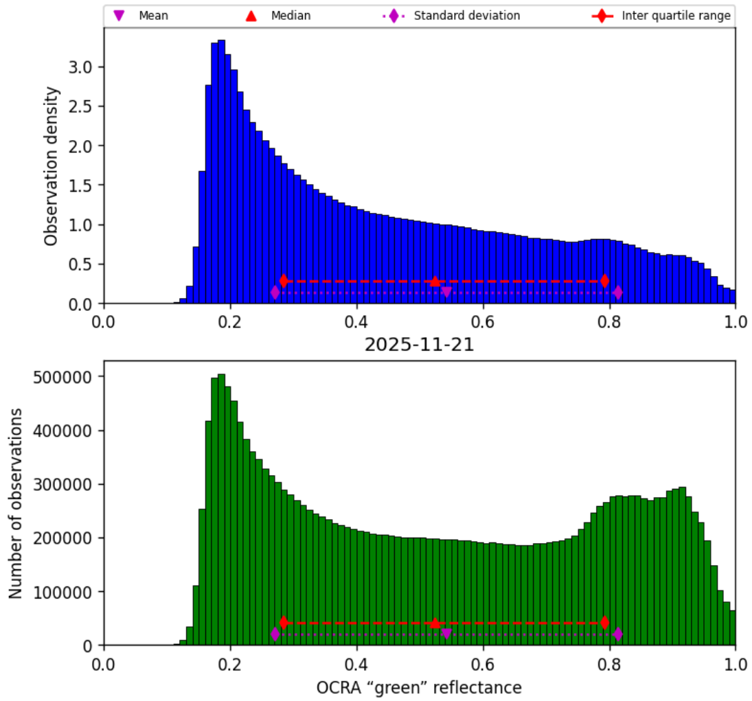
Figure 52: Histogram of “OCRA “green” reflectance” for 2025-11-20 to 2025-11-22
