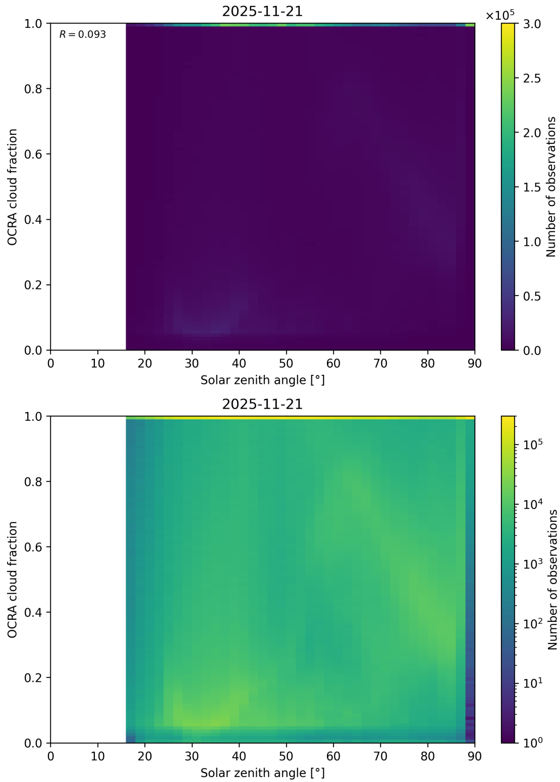
Figure 100: Scatter density plot of “Solar zenith angle” against “OCRA cloud fraction” for 2025-11-20 to 2025-11-22.
