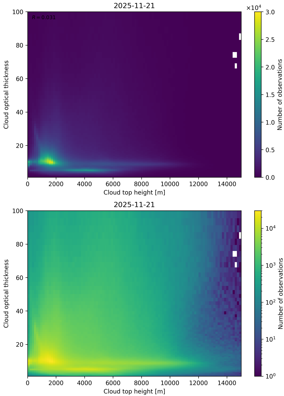
Figure 90: Scatter density plot of “Cloud top height” against “Cloud optical thickness” for 2025-11-20 to 2025-11-22.
