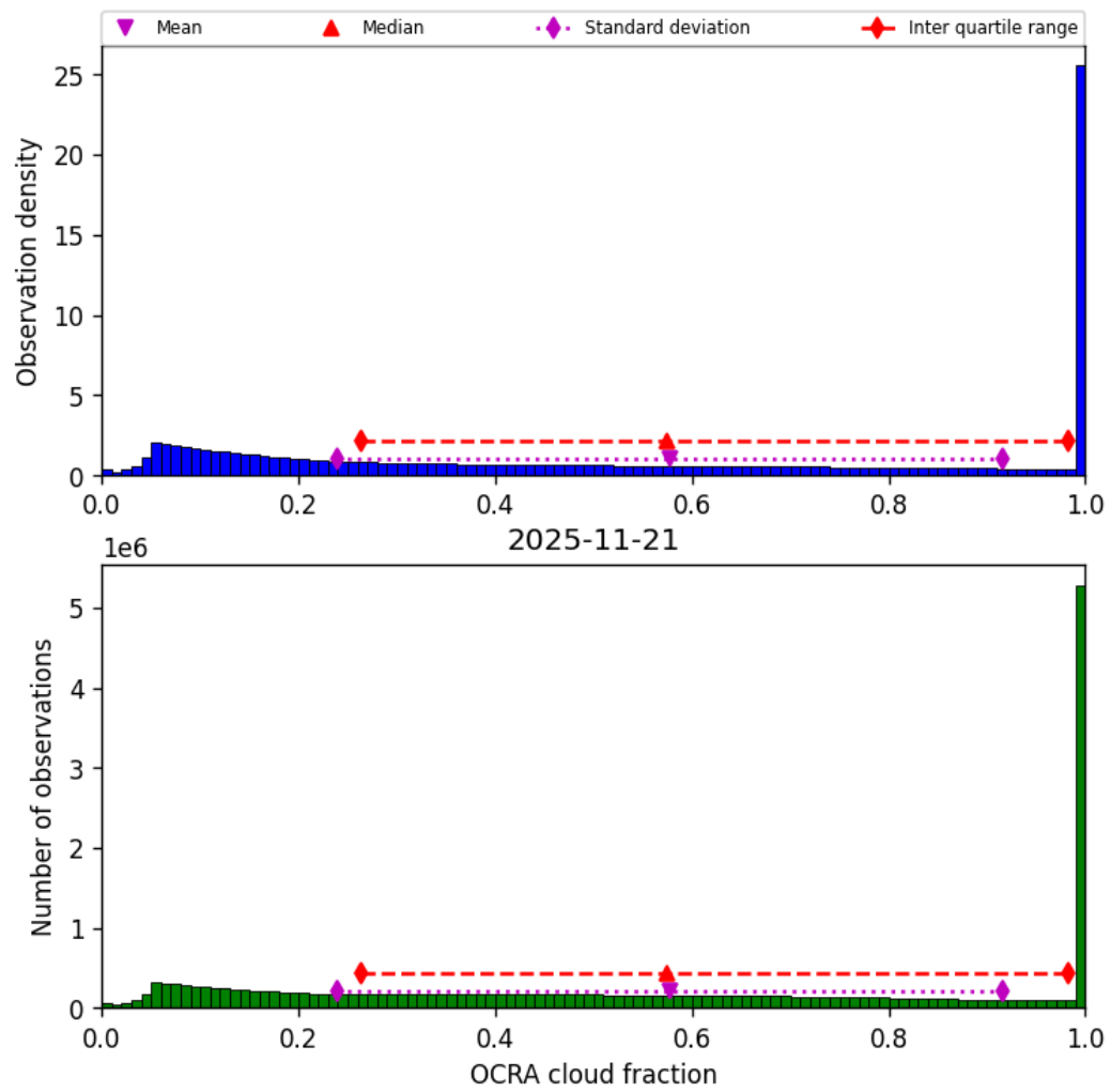
Figure 50: Histogram of “OCRA cloud fraction” for 2025-11-20 to 2025-11-22
