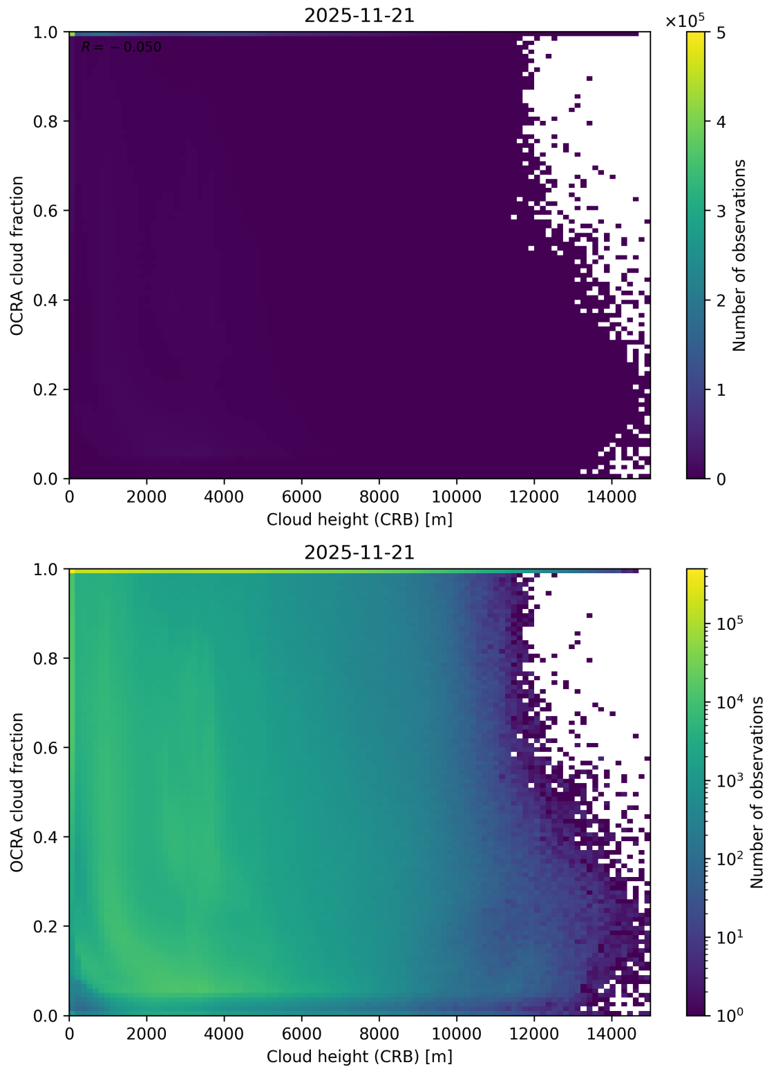
Figure 81: Scatter density plot of “Cloud height (CRB)” against “OCRA cloud fraction” for 2025-11-20 to 2025-11-22.
