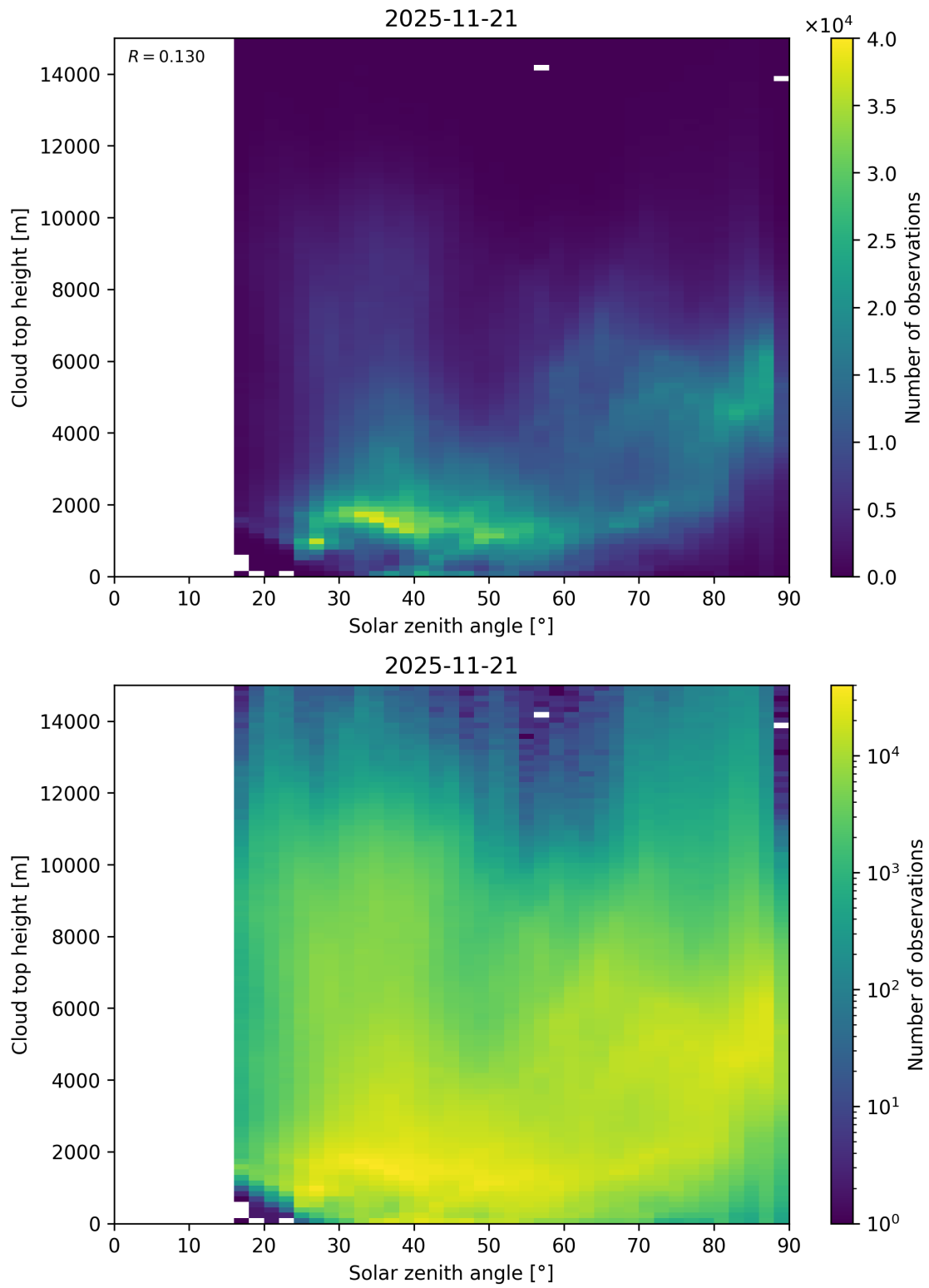
Figure 104: Scatter density plot of “Solar zenith angle” against “Cloud top height” for 2025-11-20 to 2025-11-22.
