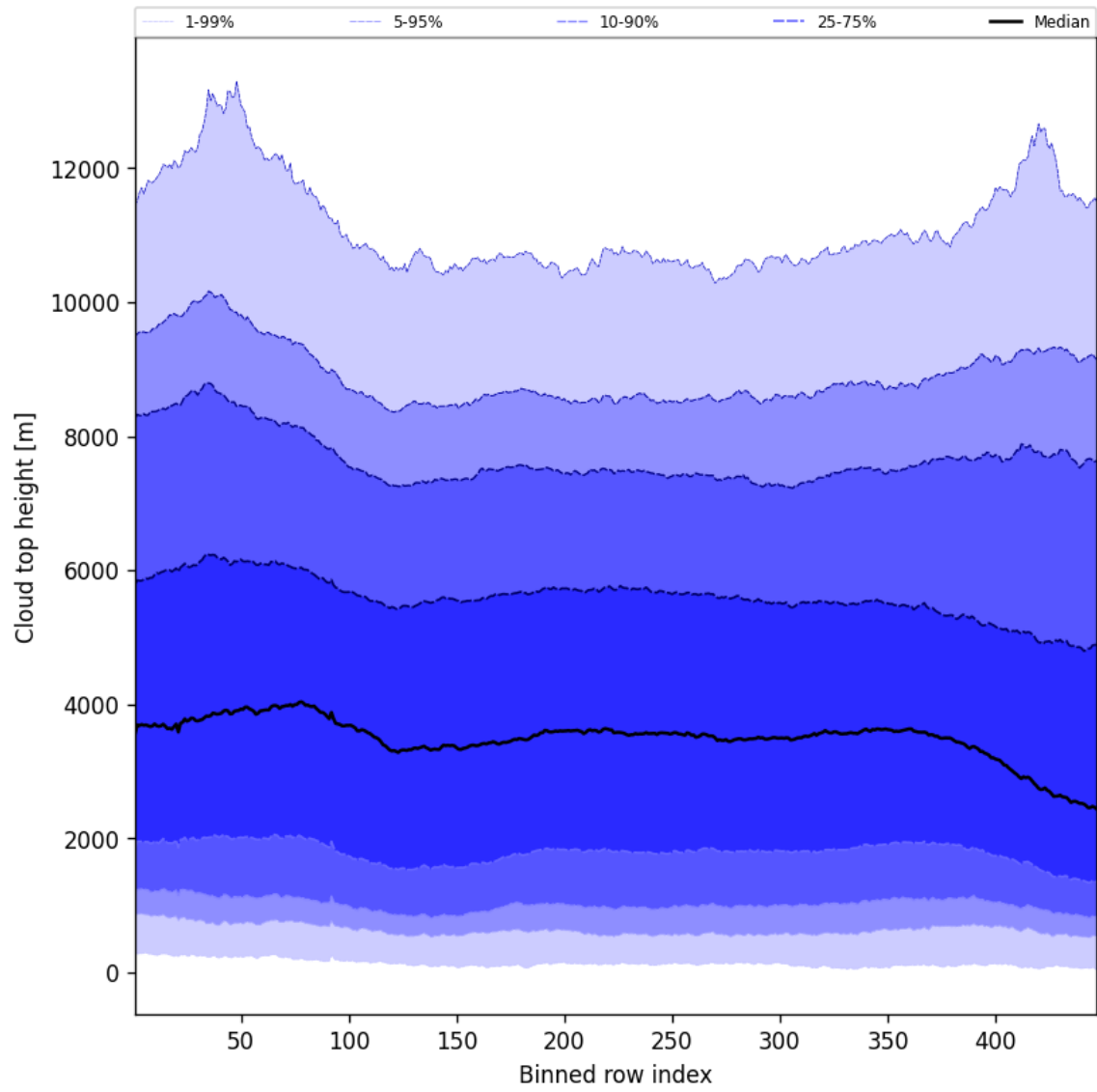
Figure 56: Along track statistics of “Cloud top height” for 2025-11-20 to 2025-11-22
