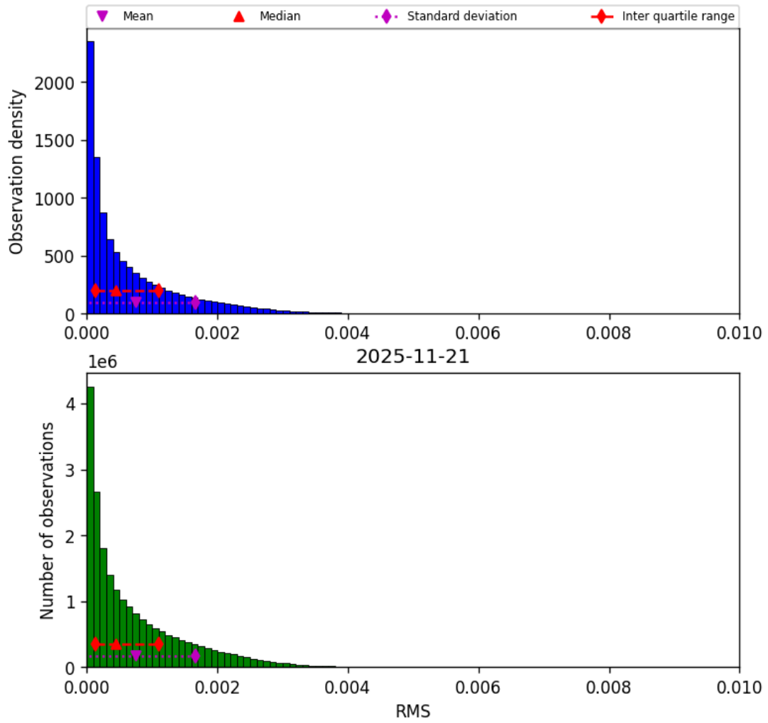
Figure 47: Histogram of “RMS” for 2025-11-20 to 2025-11-22
