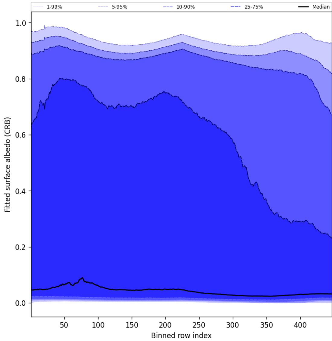
Figure 62: Along track statistics of “Fitted surface albedo (CRB)” for 2025-11-20 to 2025-11-22
