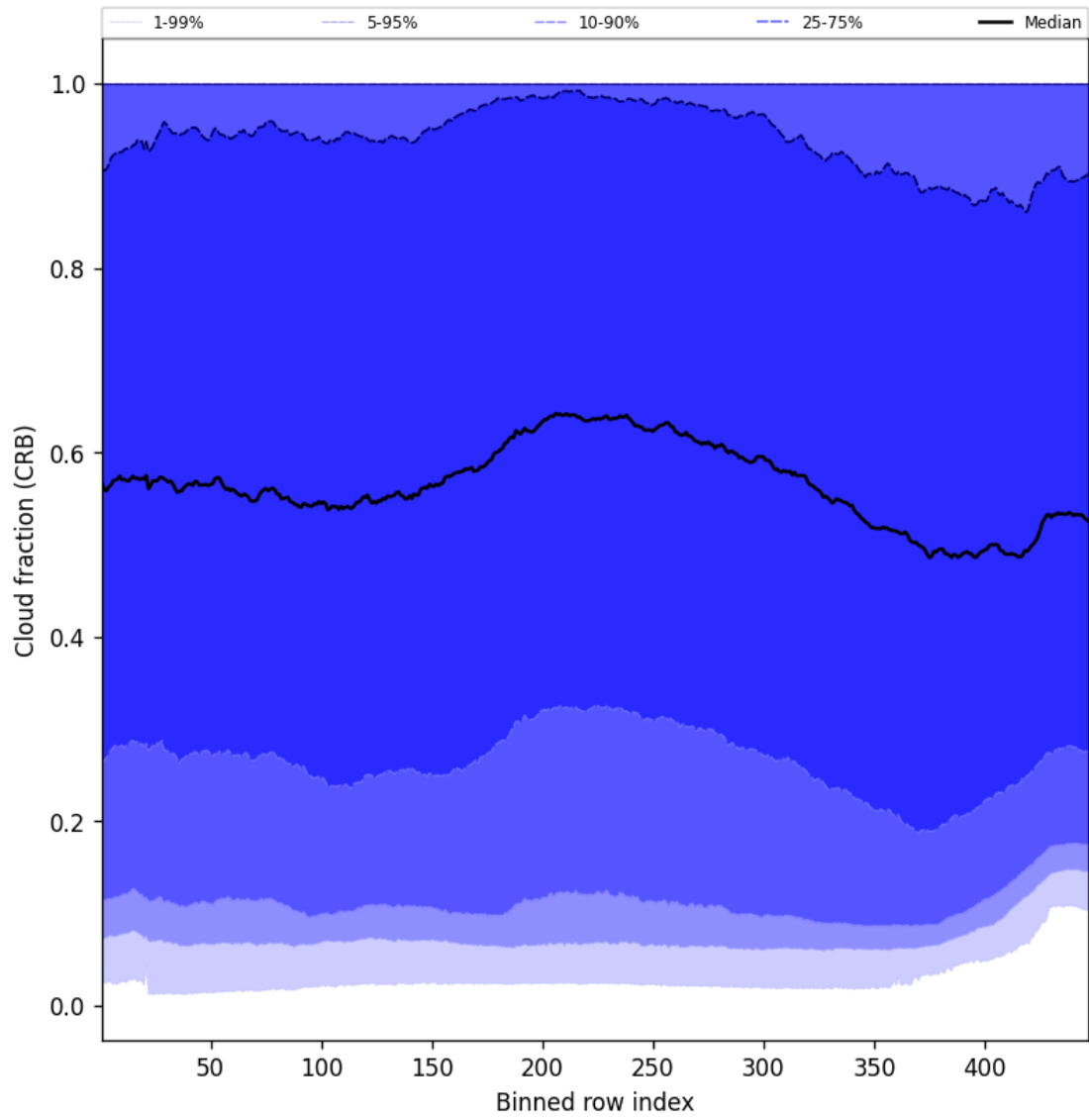
Figure 58: Along track statistics of “Cloud fraction (CRB)” for 2025-11-20 to 2025-11-22
