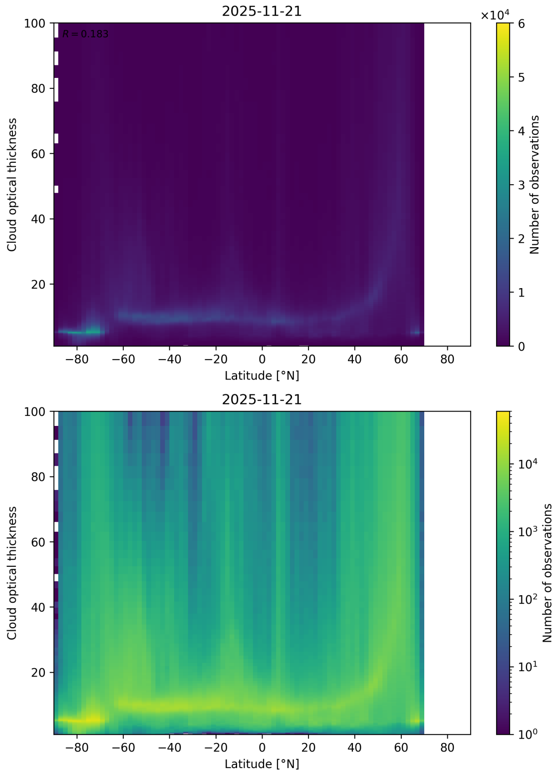
Figure 96: Scatter density plot of “Latitude” against “Cloud optical thickness” for 2025-11-20 to 2025-11-22.
