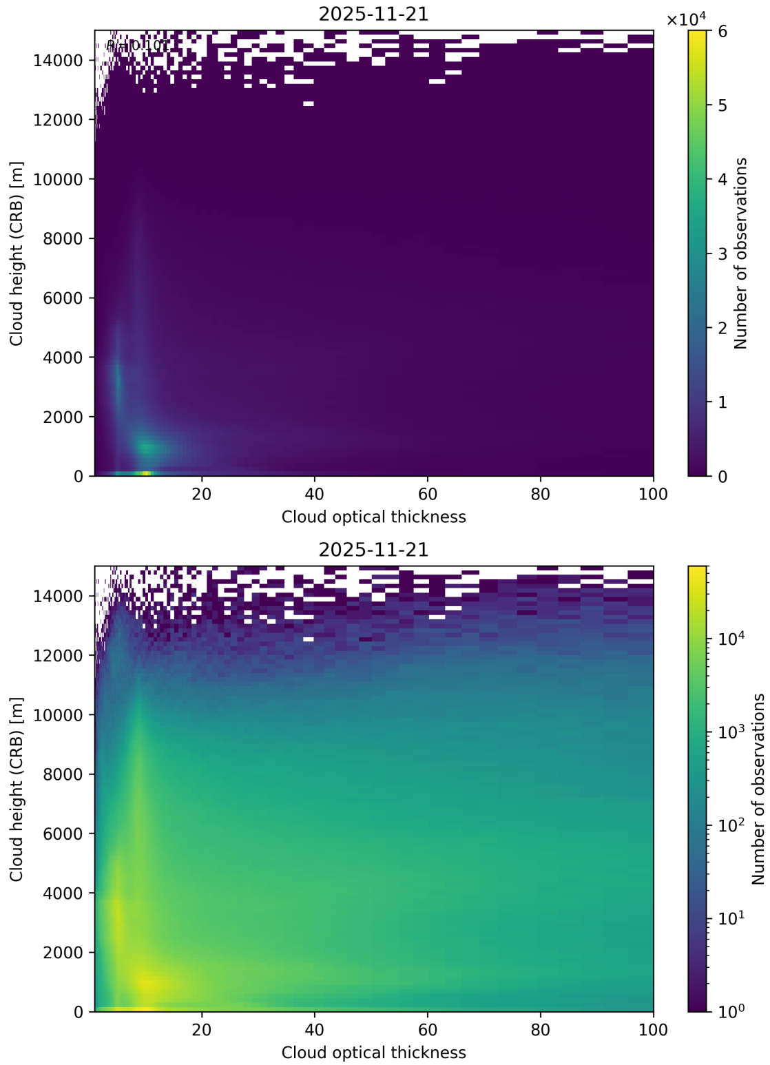
Figure 85: Scatter density plot of “Cloud optical thickness” against “Cloud height (CRB)” for 2025-11-20 to 2025-11-22.
