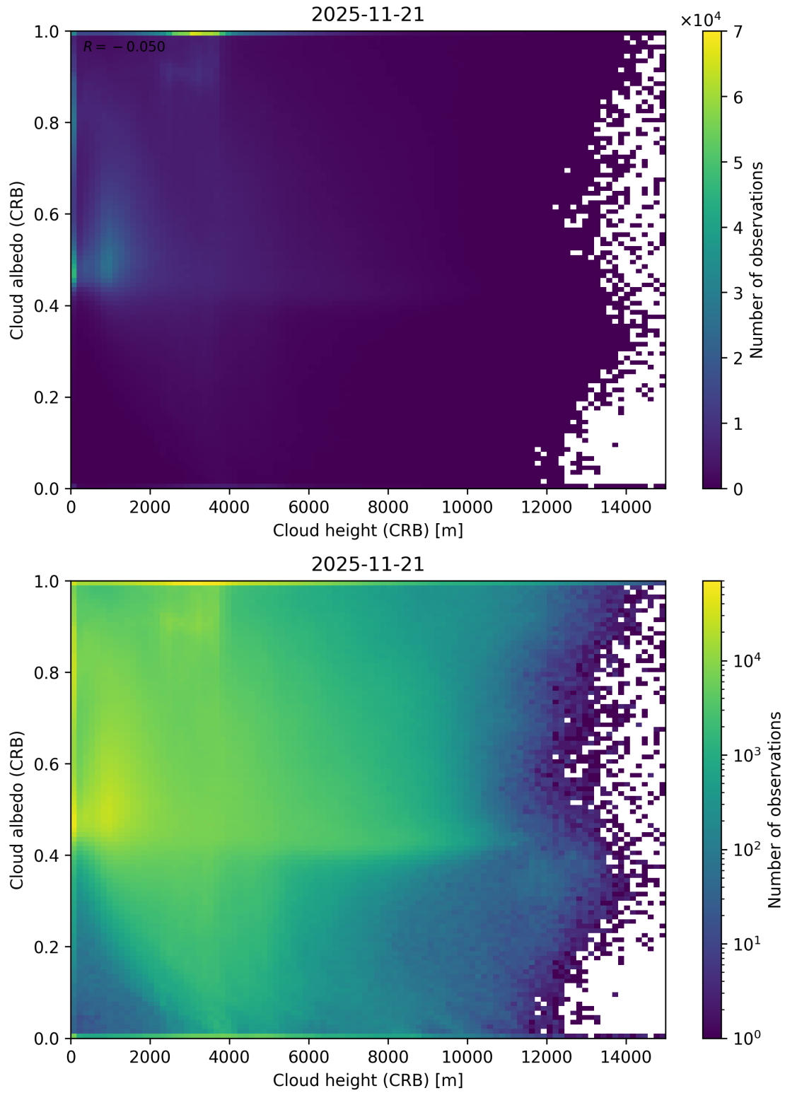
Figure 80: Scatter density plot of “Cloud height (CRB)” against “Cloud albedo (CRB)” for 2025-11-20 to 2025-11-22.
