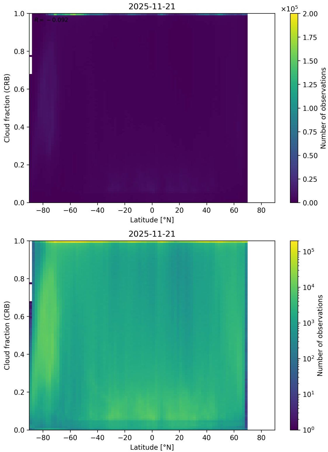
Figure 94: Scatter density plot of “Latitude” against “Cloud fraction (CRB)” for 2025-11-20 to 2025-11-22.
