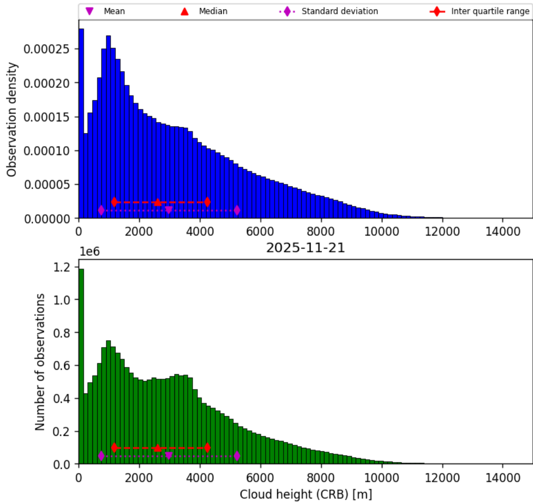
Figure 43: Histogram of “Cloud height (CRB)” for 2025-11-20 to 2025-11-22
