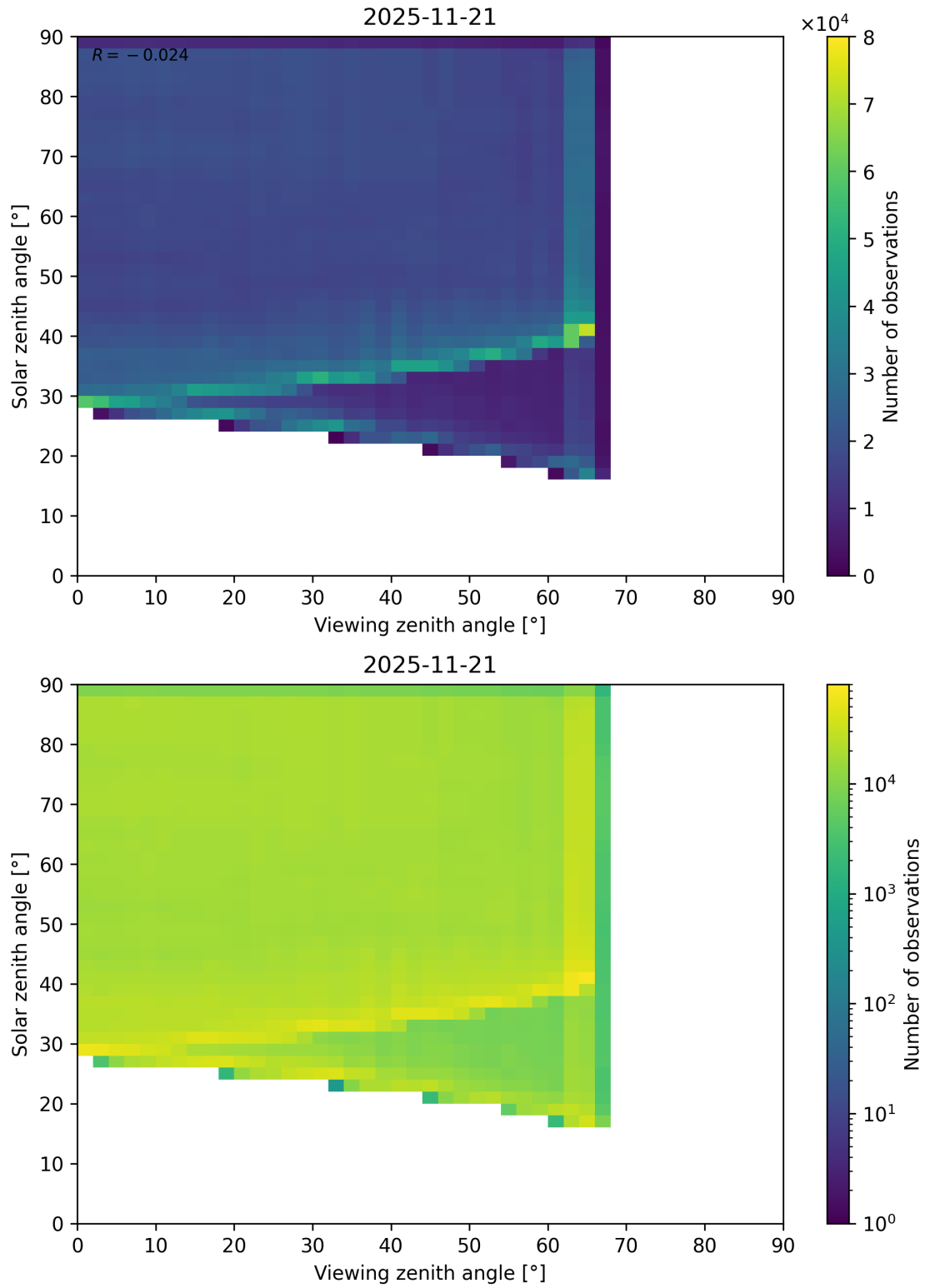
Figure 114: Scatter density plot of “Viewing zenith angle” against “Solar zenith angle” for 2025-11-20 to 2025-11-22.
