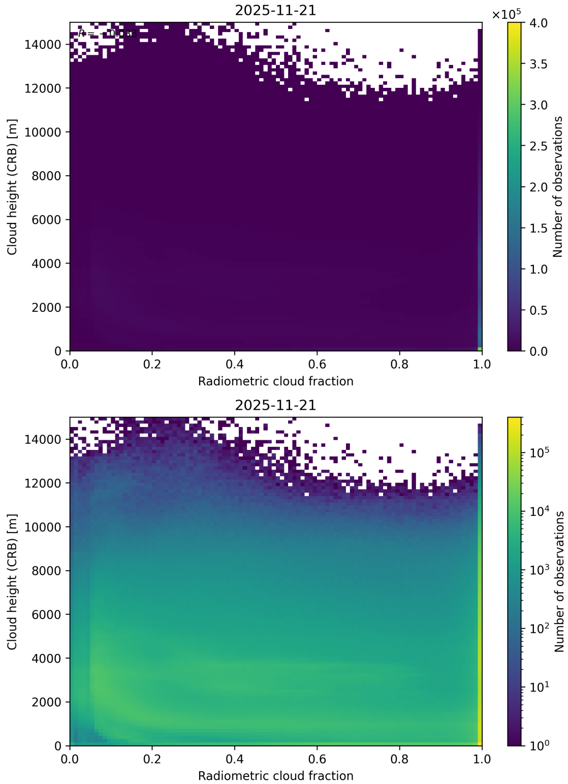
Figure 74: Scatter density plot of “Radiometric cloud fraction” against “Cloud height (CRB)” for 2025-11-20 to 2025-11-22.
