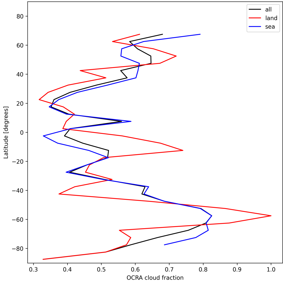
Figure 34: Zonal average of “OCRA cloud fraction” for 2025-11-20 to 2025-11-22.
