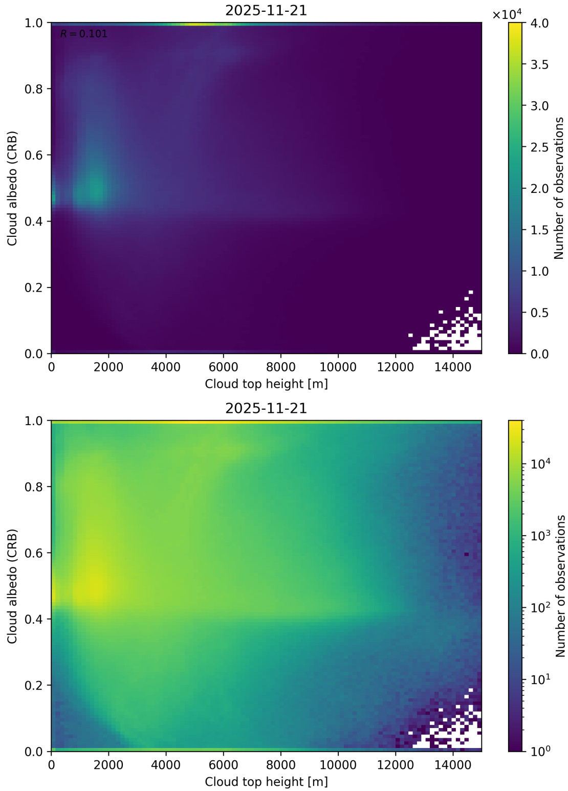
Figure 86: Scatter density plot of “Cloud top height” against “Cloud albedo (CRB)” for 2025-11-20 to 2025-11-22.
