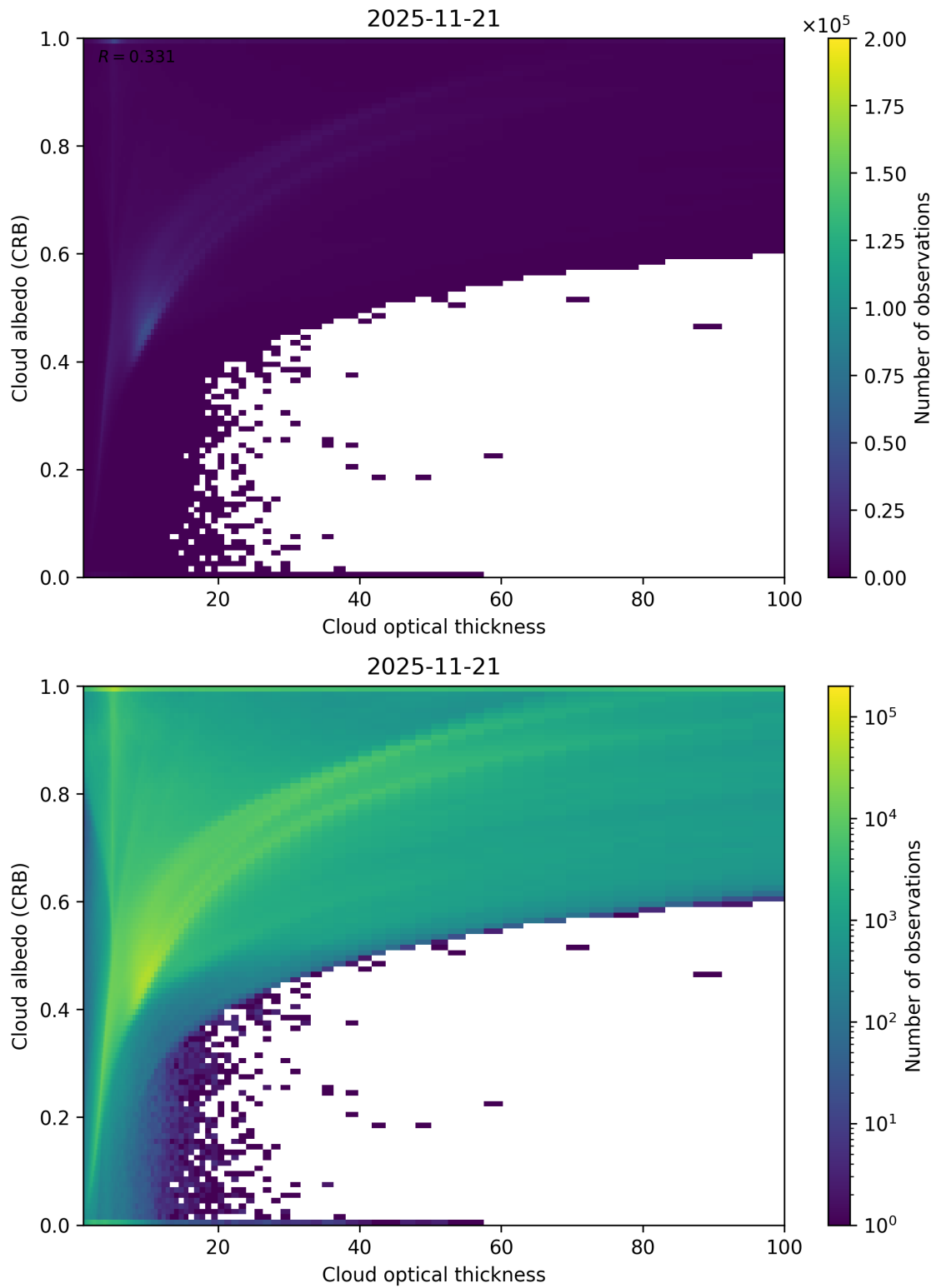
Figure 82: Scatter density plot of “Cloud optical thickness” against “Cloud albedo (CRB)” for 2025-11-20 to 2025-11-22.
