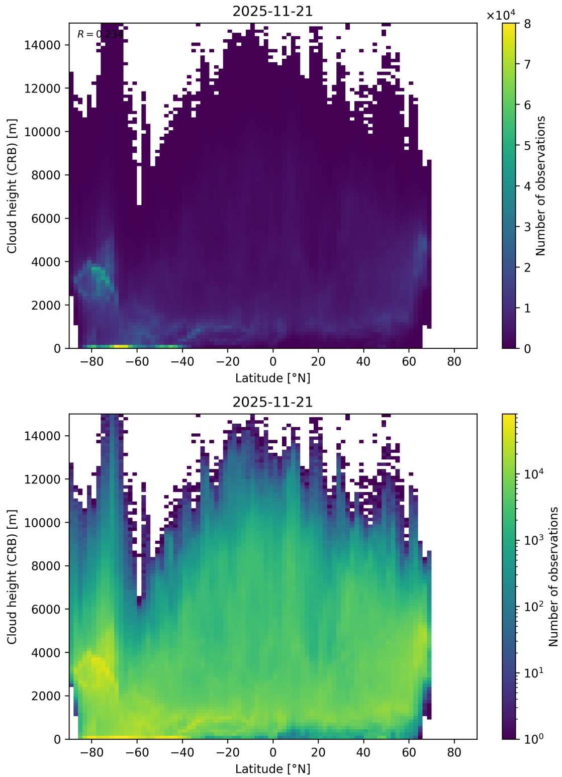
Figure 95: Scatter density plot of “Latitude” against “Cloud height (CRB)” for 2025-11-20 to 2025-11-22.
