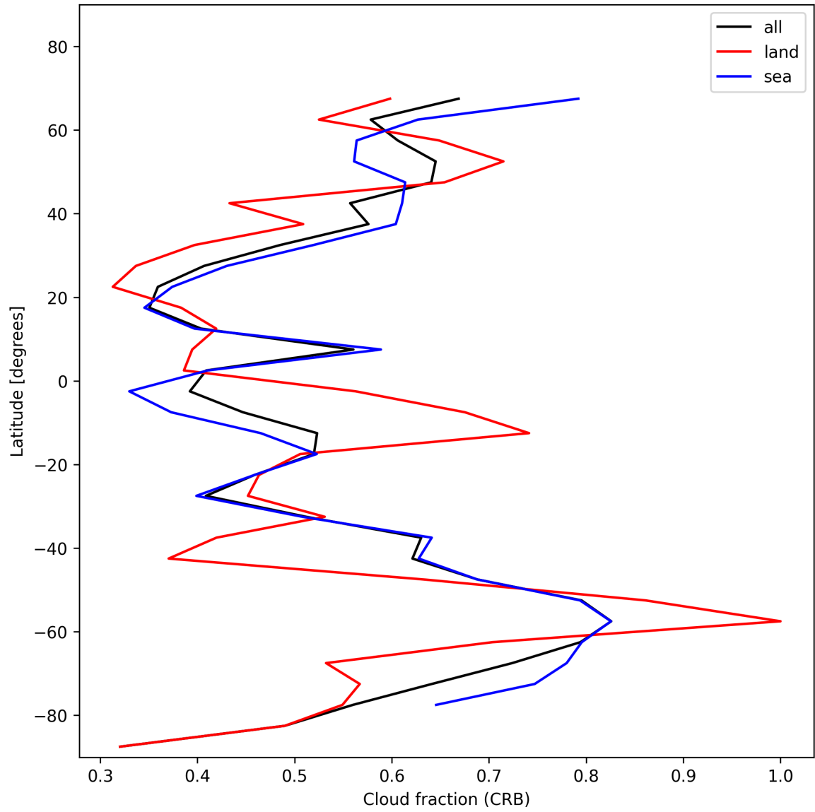
Figure 26: Zonal average of “Cloud fraction (CRB)” for 2025-11-20 to 2025-11-22.
