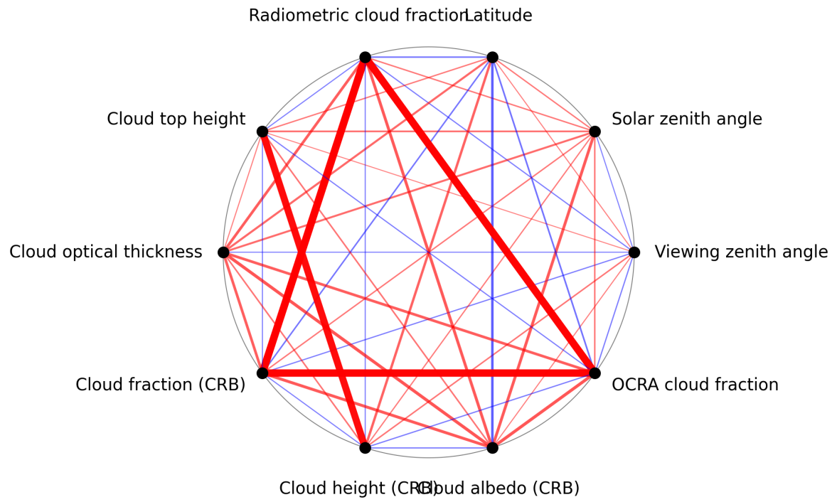
Figure 1: Map of correlation graph for 2025-11-20 to 2025-11-22.
