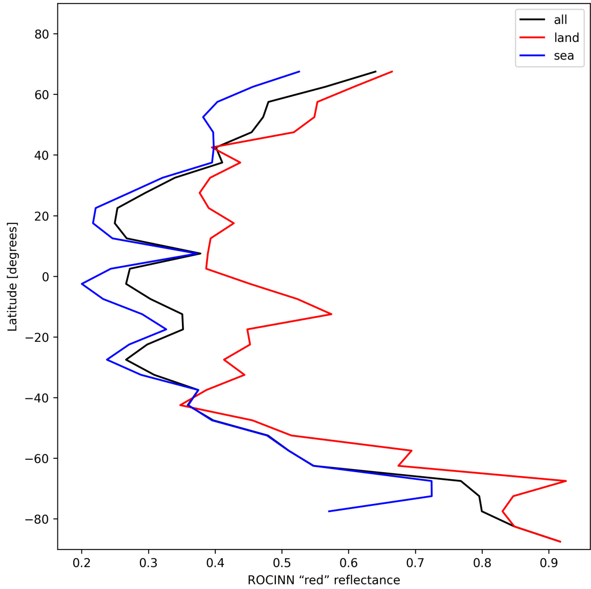
Figure 37: Zonal average of “ROCINN “red” reflectance” for 2025-11-20 to 2025-11-22.
