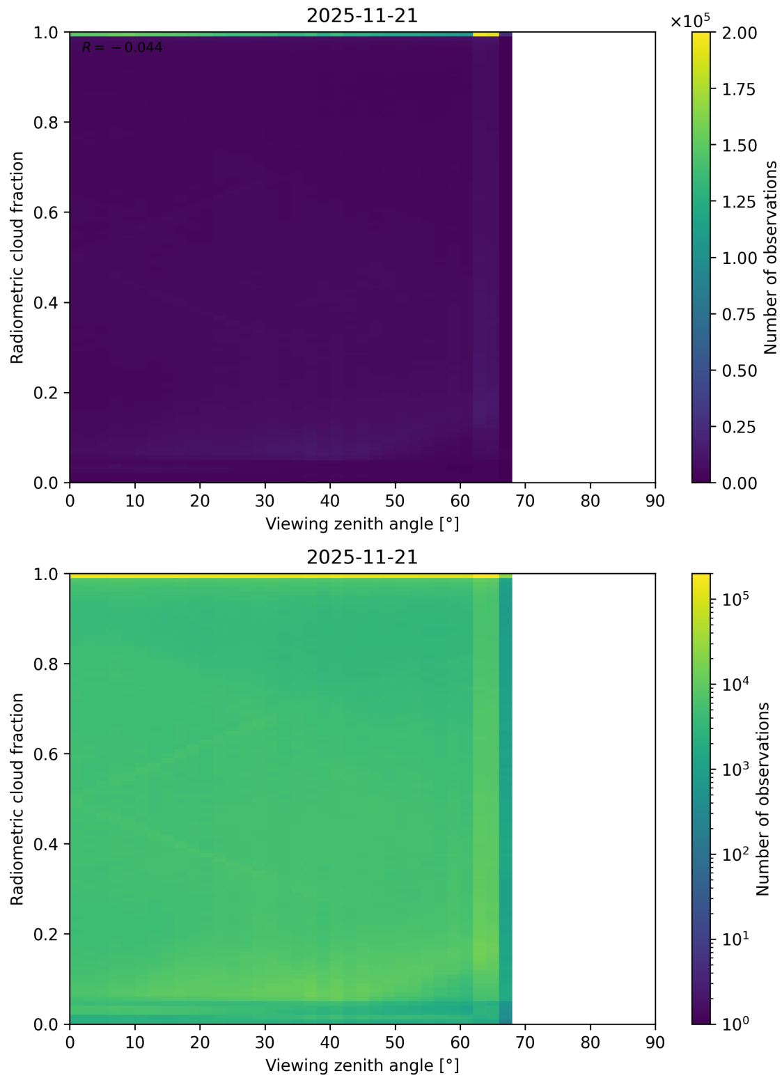
Figure 107: Scatter density plot of “Viewing zenith angle” against “Radiometric cloud fraction” for 2025-11-20 to 2025-11-22.
