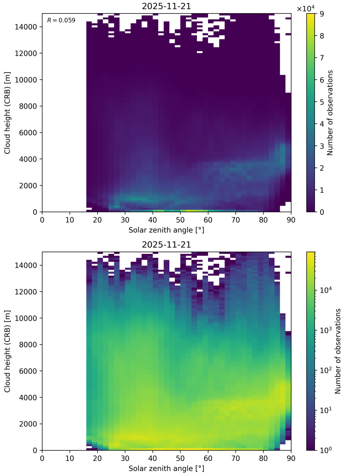
Figure 102: Scatter density plot of “Solar zenith angle” against “Cloud height (CRB)” for 2025-11-20 to 2025-11-22.
