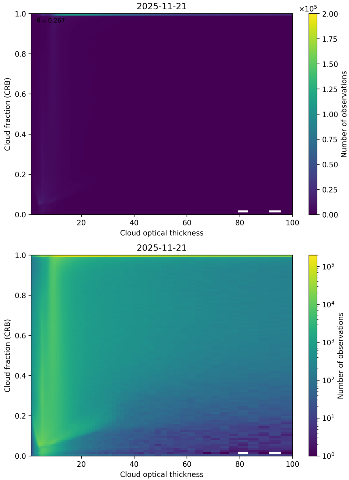
Figure 84: Scatter density plot of “Cloud optical thickness” against “Cloud fraction (CRB)” for 2025-11-20 to 2025-11-22.
