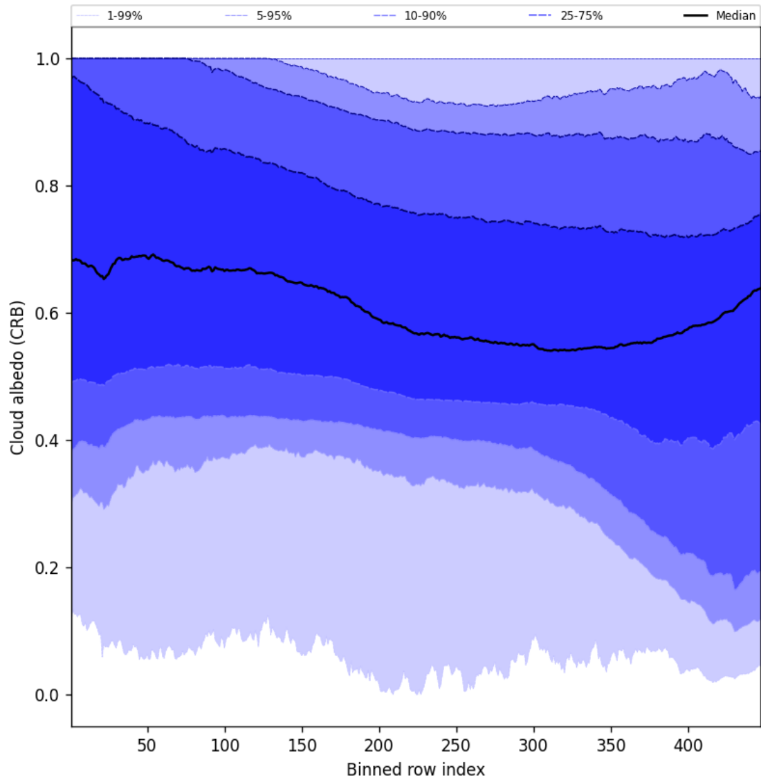
Figure 60: Along track statistics of “Cloud albedo (CRB)” for 2025-11-20 to 2025-11-22
