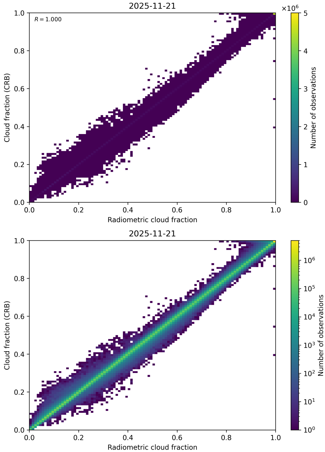
Figure 73: Scatter density plot of “Radiometric cloud fraction” against “Cloud fraction (CRB)” for 2025-11-20 to 2025-11-22.
