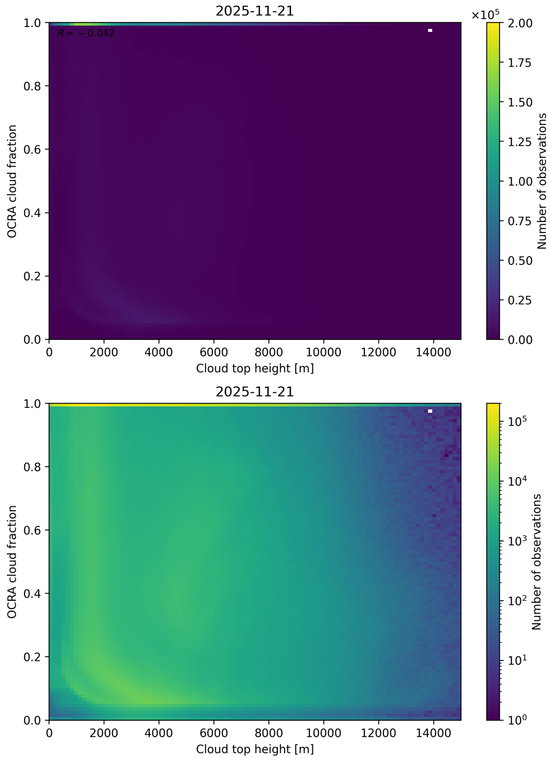
Figure 87: Scatter density plot of “Cloud top height” against “OCRA cloud fraction” for 2025-11-20 to 2025-11-22.
