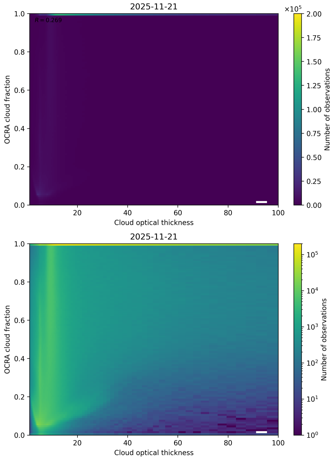
Figure 83: Scatter density plot of “Cloud optical thickness” against “OCRA cloud fraction” for 2025-11-20 to 2025-11-22.
