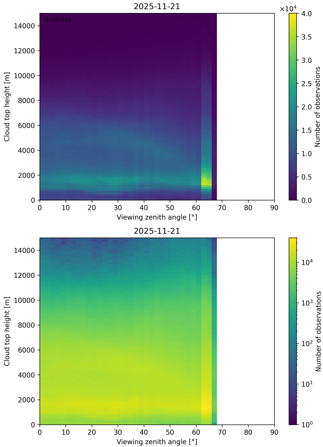
Figure 112: Scatter density plot of “Viewing zenith angle” against “Cloud top height” for 2025-11-20 to 2025-11-22.
