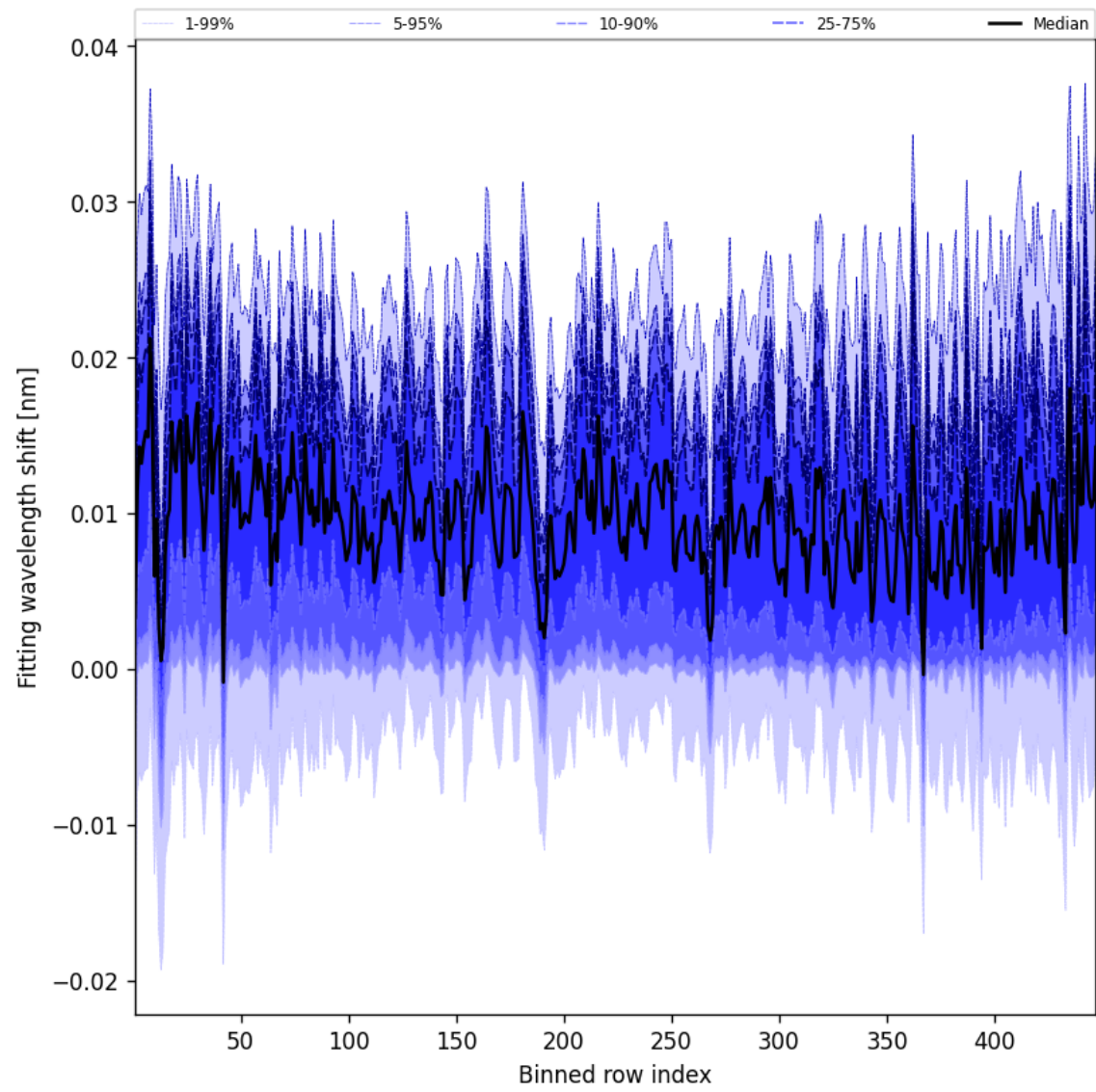
Figure 65: Along track statistics of “Fitting wavelength shift” for 2025-11-20 to 2025-11-22
