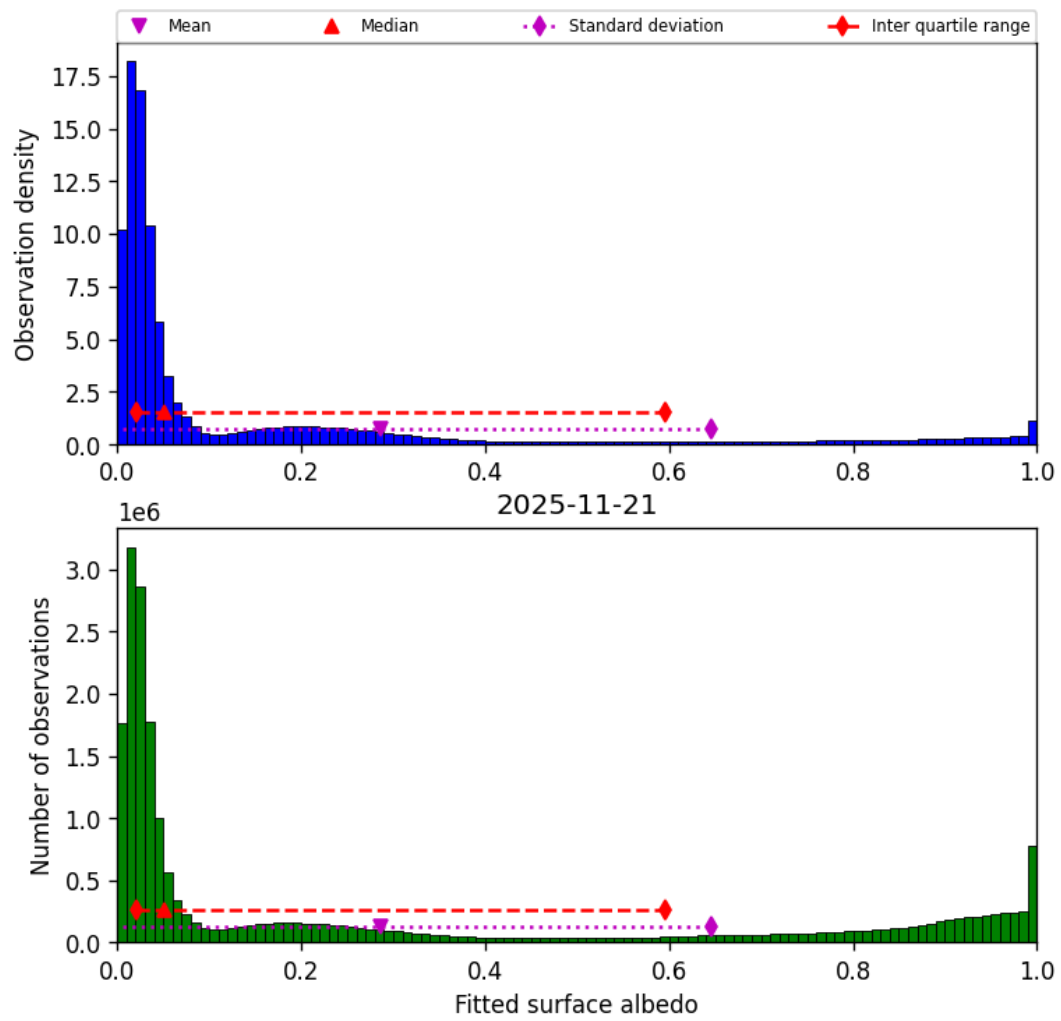
Figure 45: Histogram of “Fitted surface albedo” for 2025-11-20 to 2025-11-22
