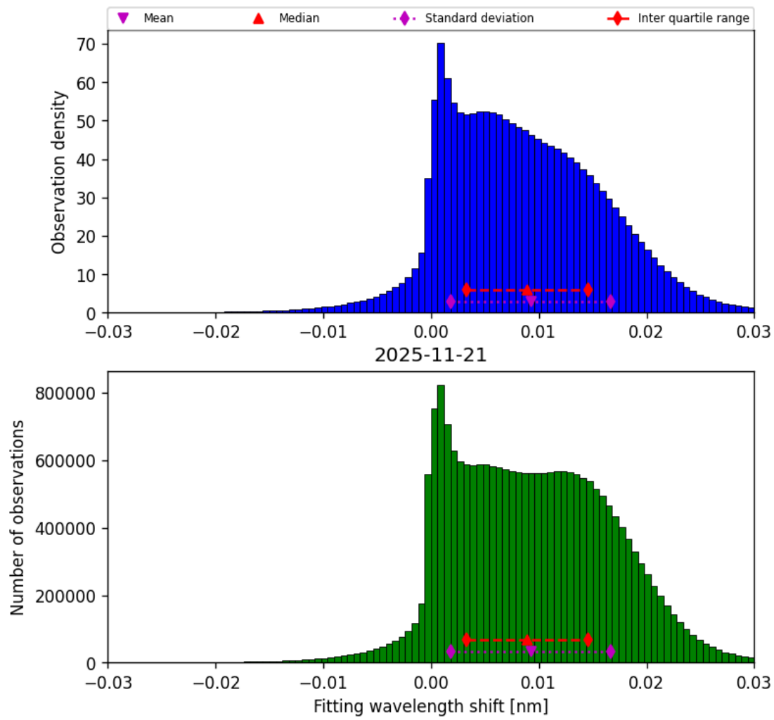
Figure 49: Histogram of “Fitting wavelength shift” for 2025-11-20 to 2025-11-22
