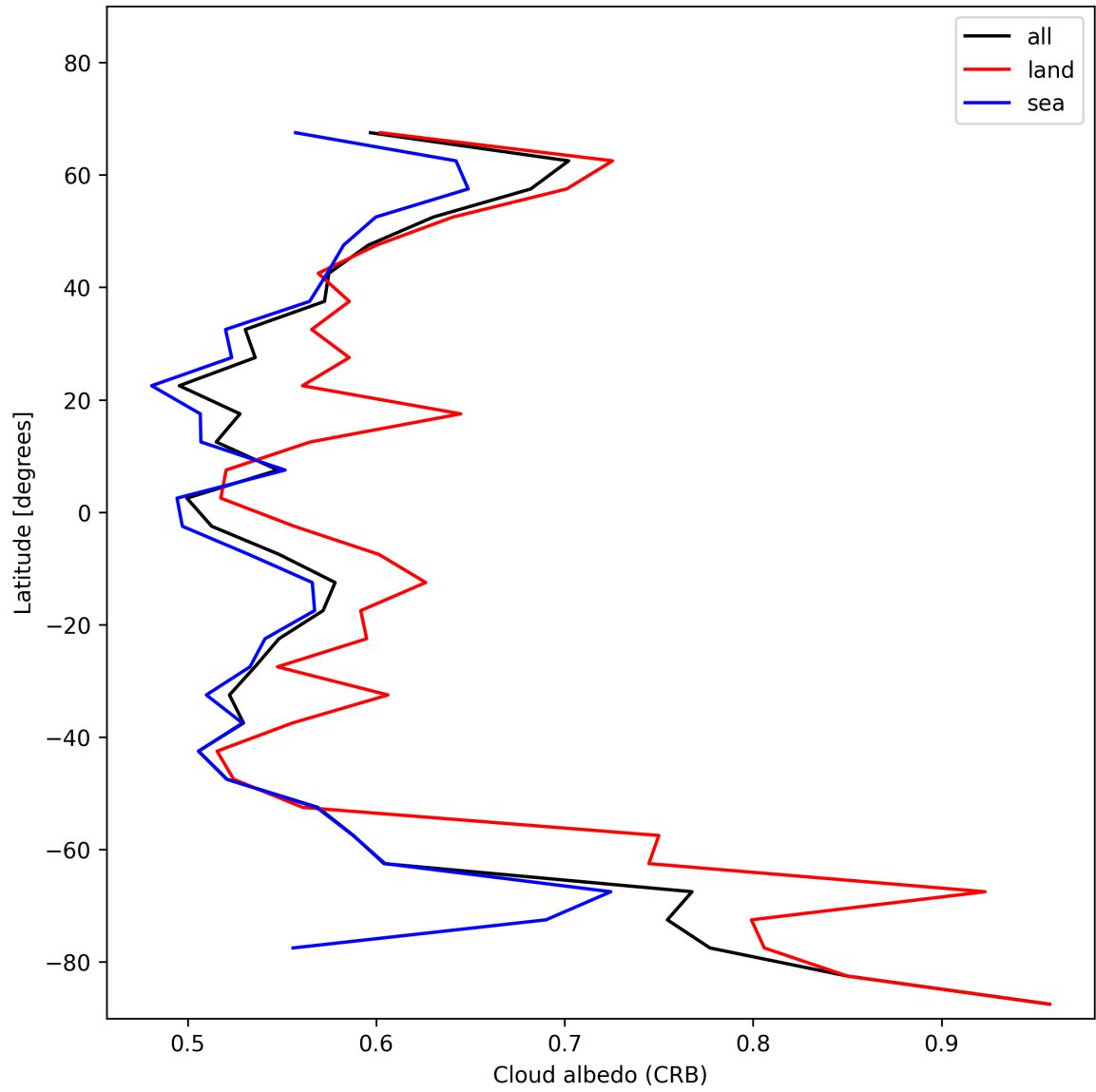
Figure 28: Zonal average of “Cloud albedo (CRB)” for 2025-11-20 to 2025-11-22.
