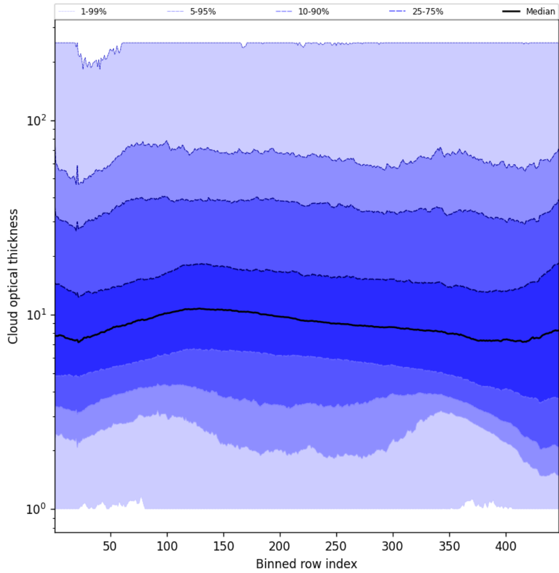
Figure 57: Along track statistics of “Cloud optical thickness” for 2025-11-20 to 2025-11-22
