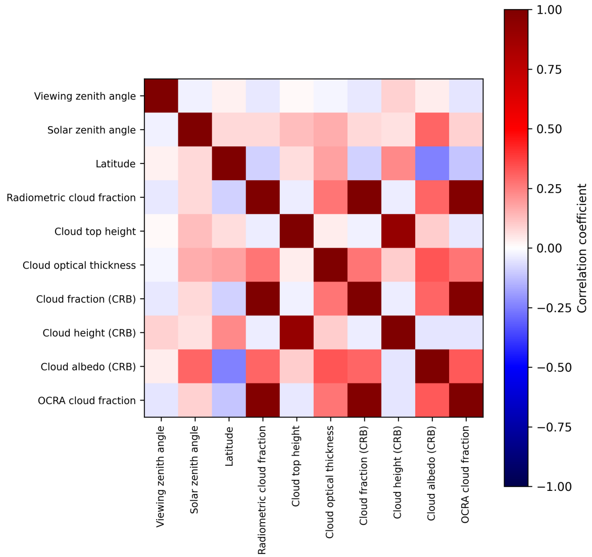
Figure 2: Map of correlation matrix for 2025-11-20 to 2025-11-22.
