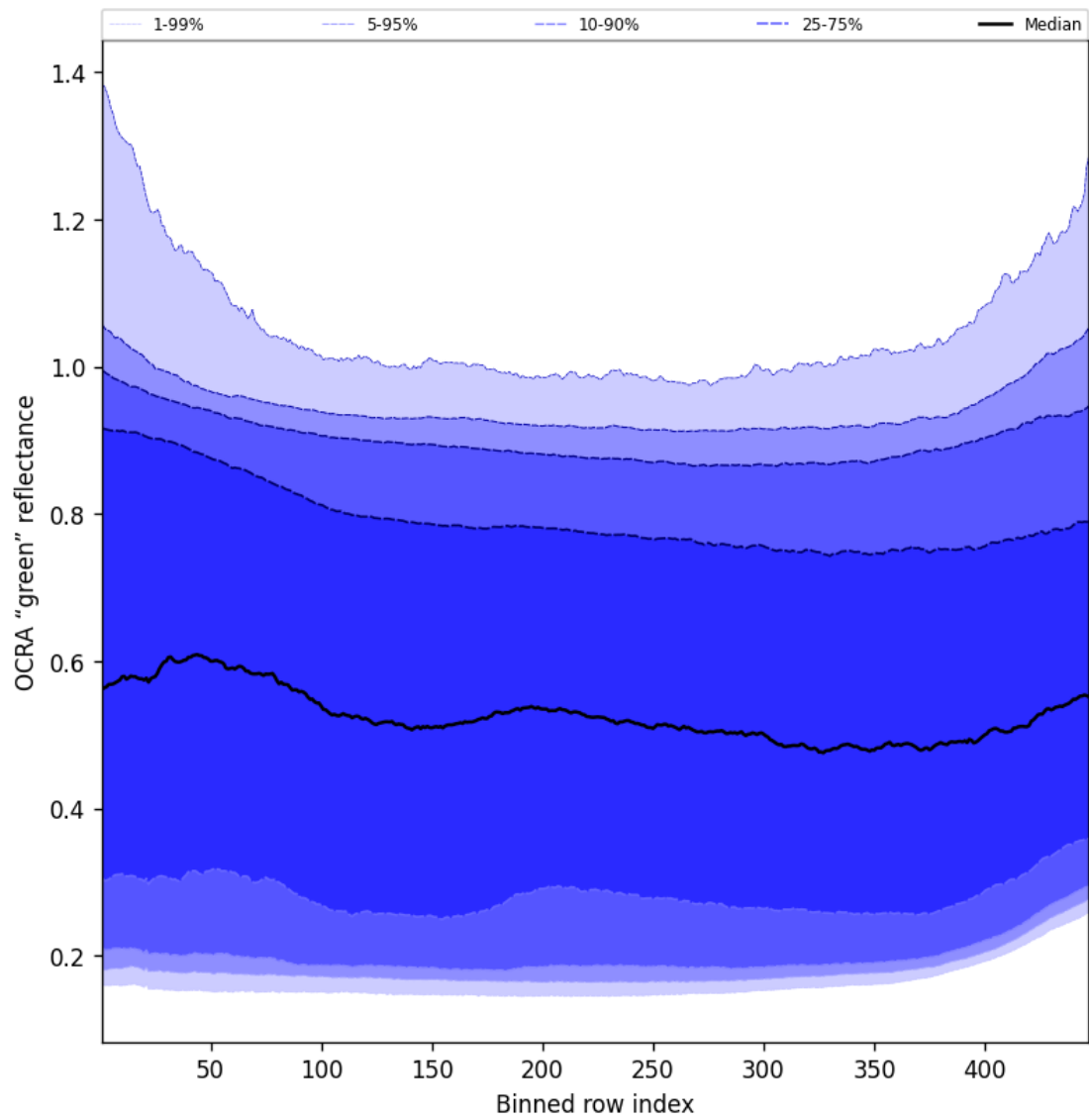
Figure 68: Along track statistics of “OCRA “green” reflectance” for 2025-11-20 to 2025-11-22
