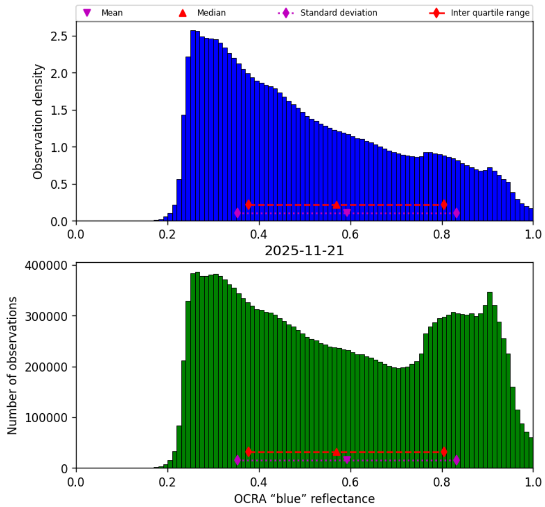
Figure 51: Histogram of “OCRA “blue” reflectance” for 2025-11-20 to 2025-11-22
