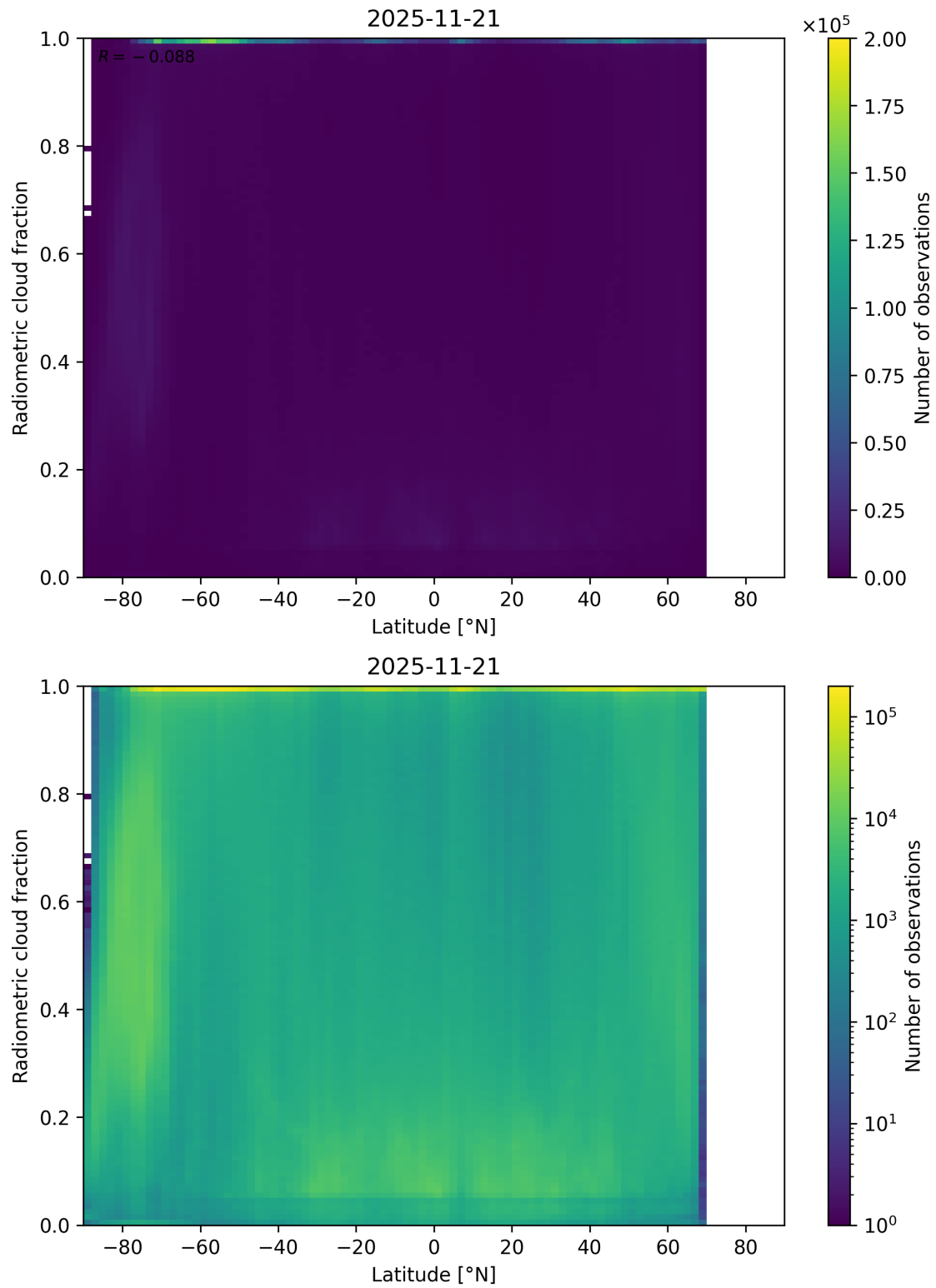
Figure 92: Scatter density plot of “Latitude” against “Radiometric cloud fraction” for 2025-11-20 to 2025-11-22.
