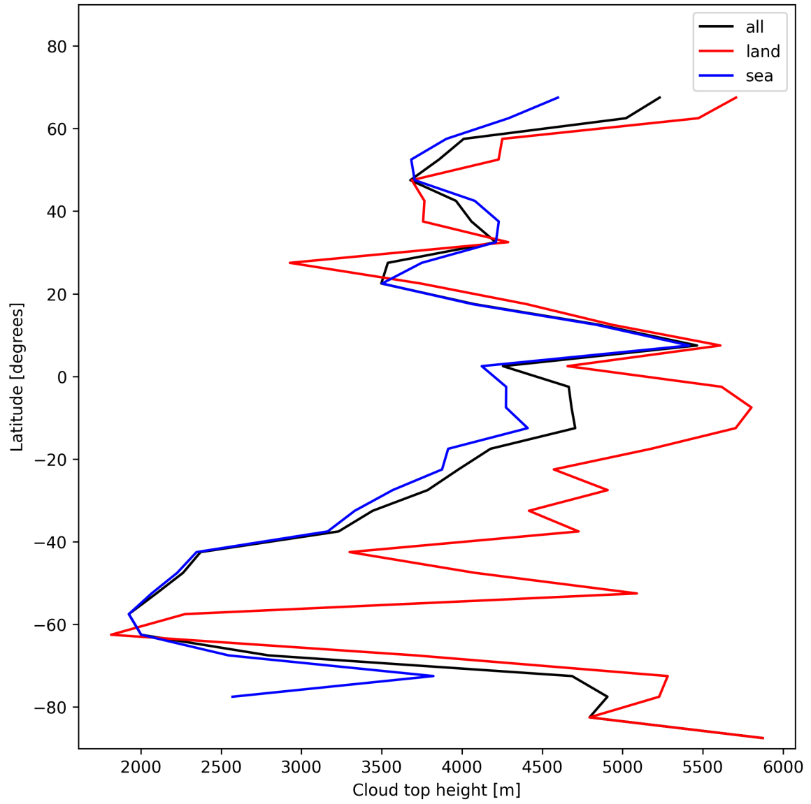
Figure 24: Zonal average of “Cloud top height” for 2025-11-20 to 2025-11-22.
