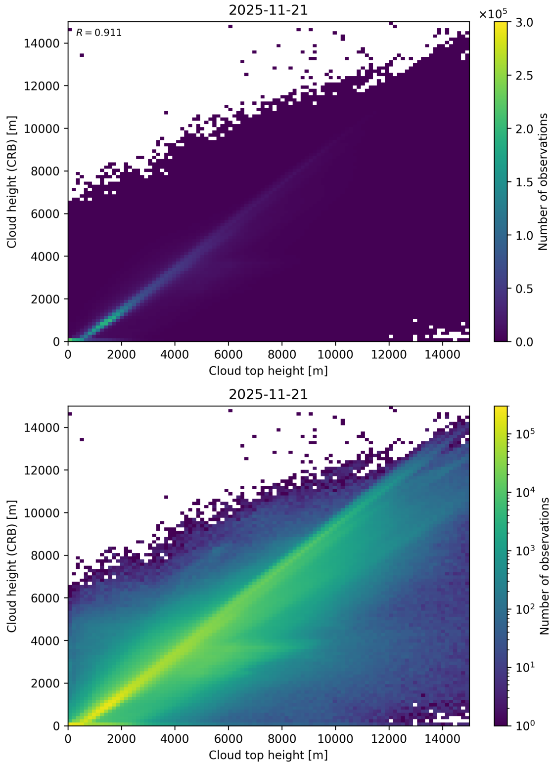
Figure 89: Scatter density plot of “Cloud top height” against “Cloud height (CRB)” for 2025-11-20 to 2025-11-22.
