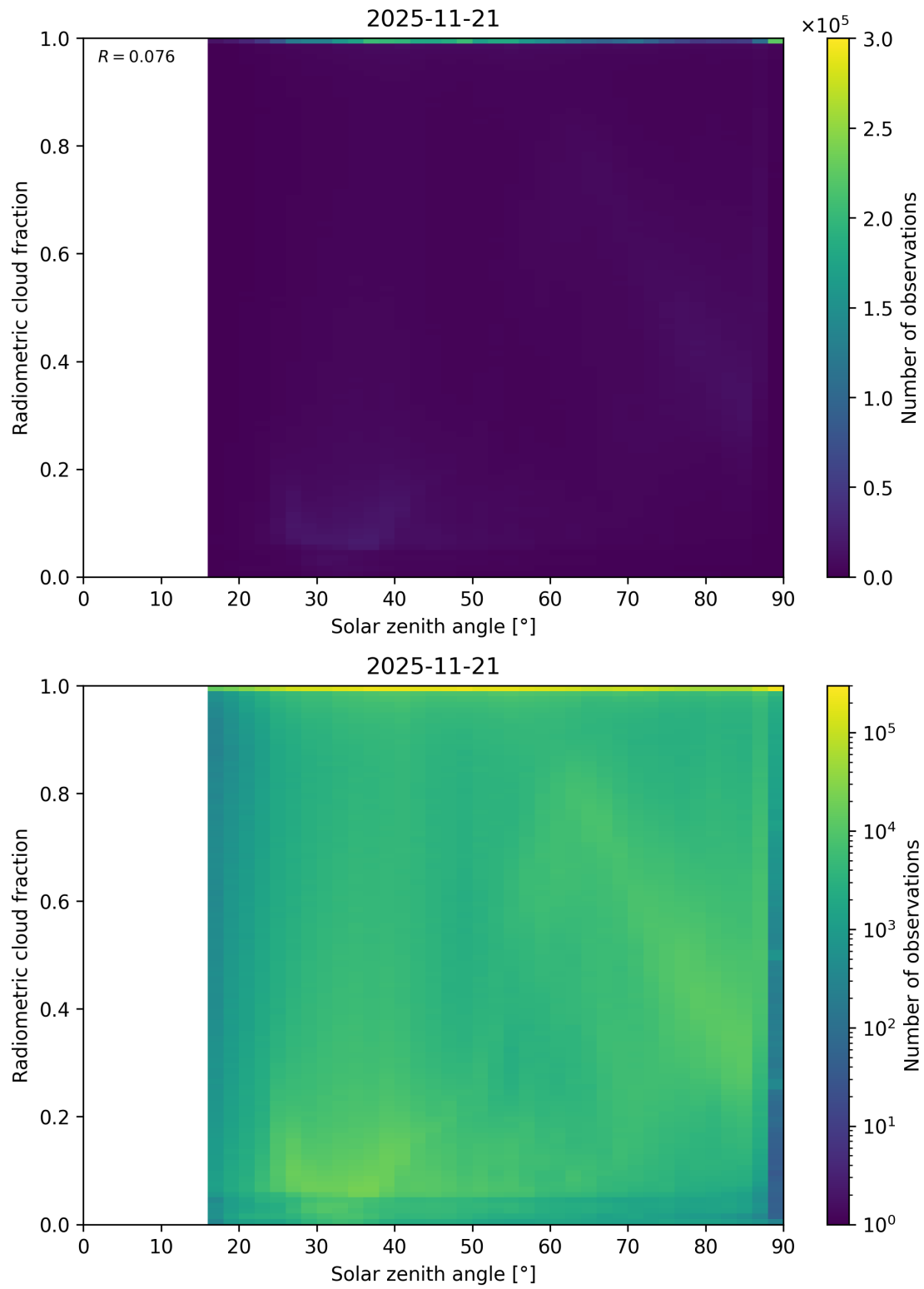
Figure 99: Scatter density plot of “Solar zenith angle” against “Radiometric cloud fraction” for 2025-11-20 to 2025-11-22.
