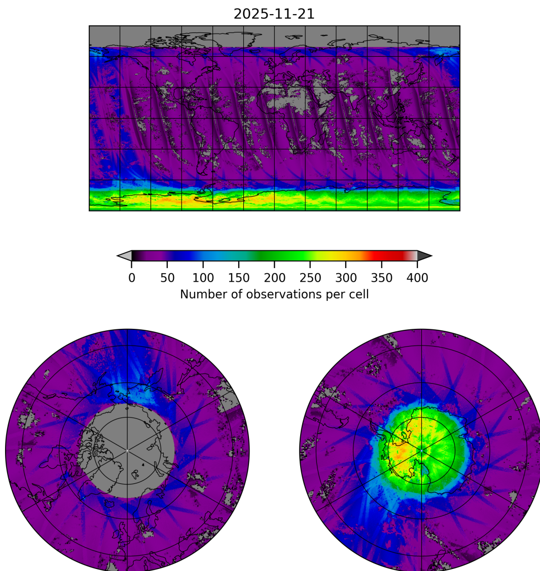
Figure 21: Map of the number of observations for 2025-11-20 to 2025-11-22
