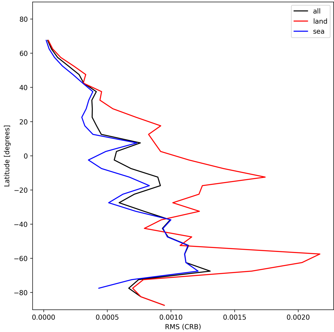
Figure 32: Zonal average of “RMS (CRB)” for 2025-11-20 to 2025-11-22.
