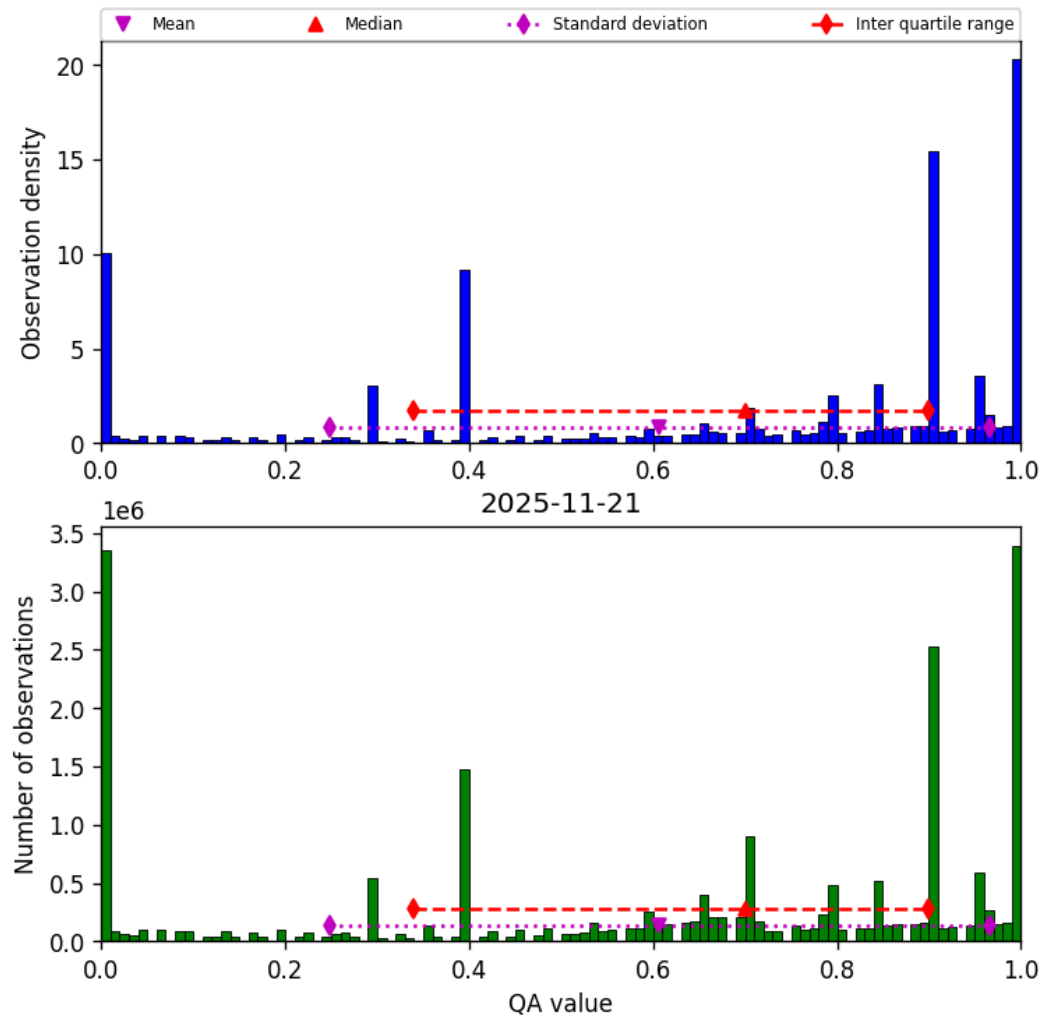
Figure 38: Histogram of “QA value” for 2025-11-20 to 2025-11-22
