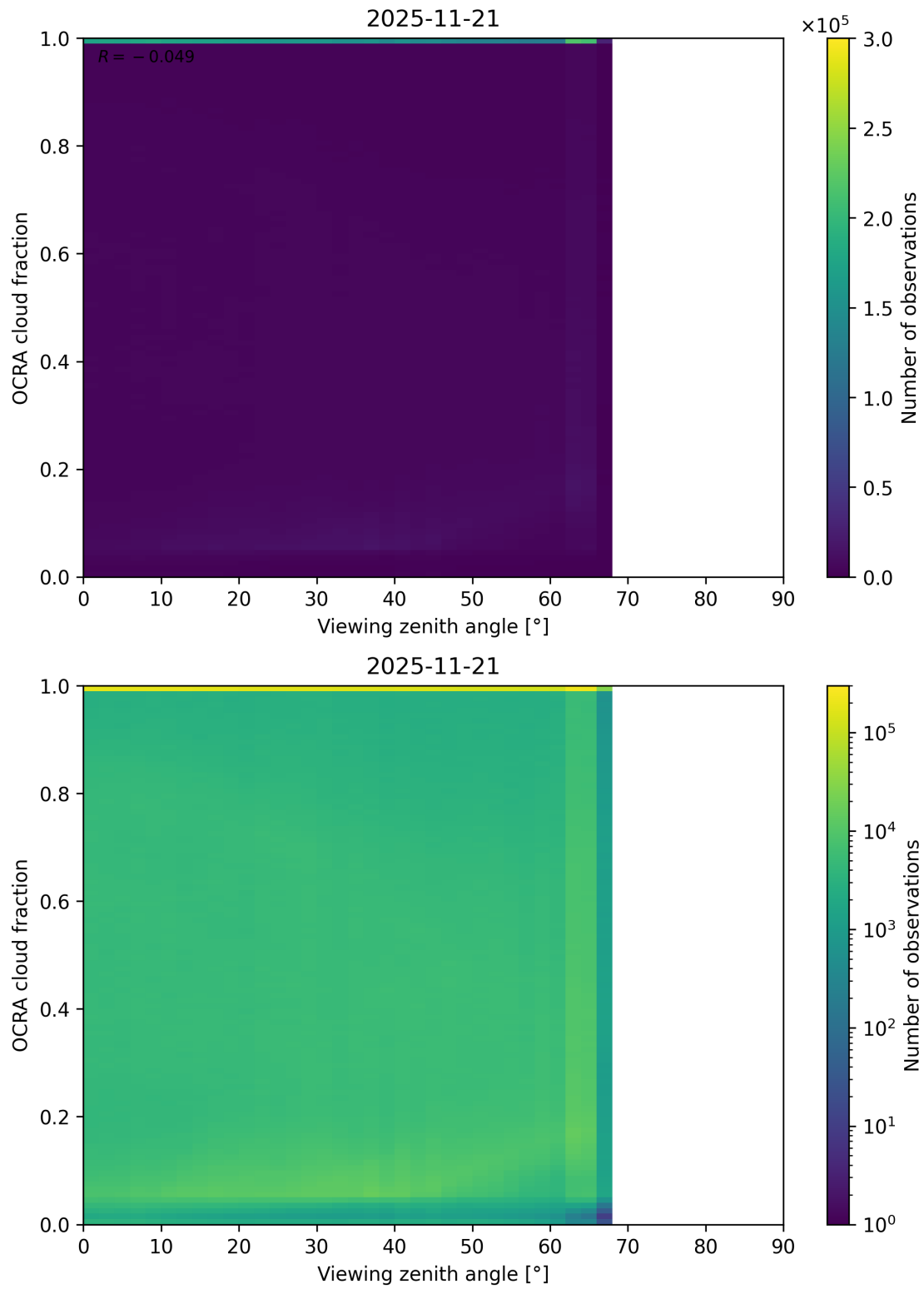
Figure 108: Scatter density plot of “Viewing zenith angle” against “OCRA cloud fraction” for 2025-11-20 to 2025-11-22.
