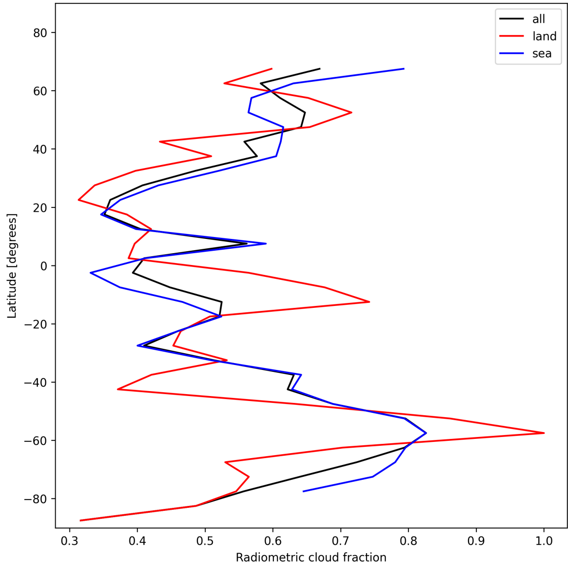
Figure 23: Zonal average of “Radiometric cloud fraction” for 2025-11-20 to 2025-11-22.
