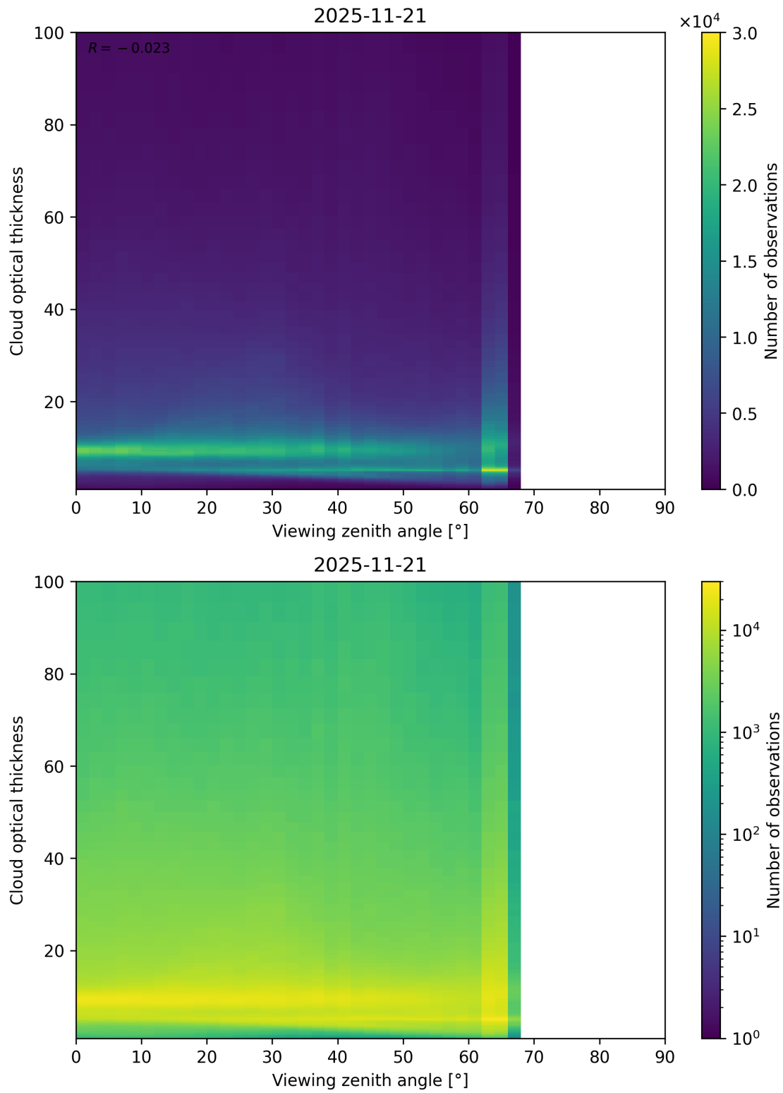
Figure 111: Scatter density plot of “Viewing zenith angle” against “Cloud optical thickness” for 2025-11-20 to 2025-11-22.
