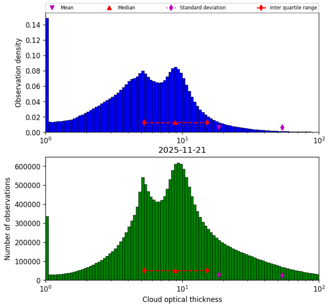
Figure 41: Histogram of “Cloud optical thickness” for 2025-11-20 to 2025-11-22
