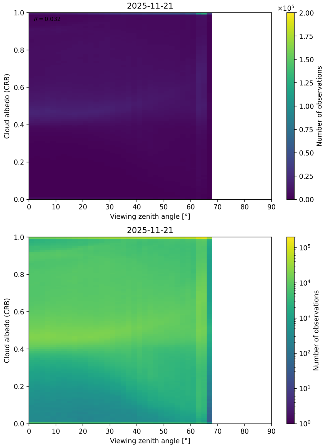
Figure 106: Scatter density plot of “Viewing zenith angle” against “Cloud albedo (CRB)” for 2025-11-20 to 2025-11-22.
