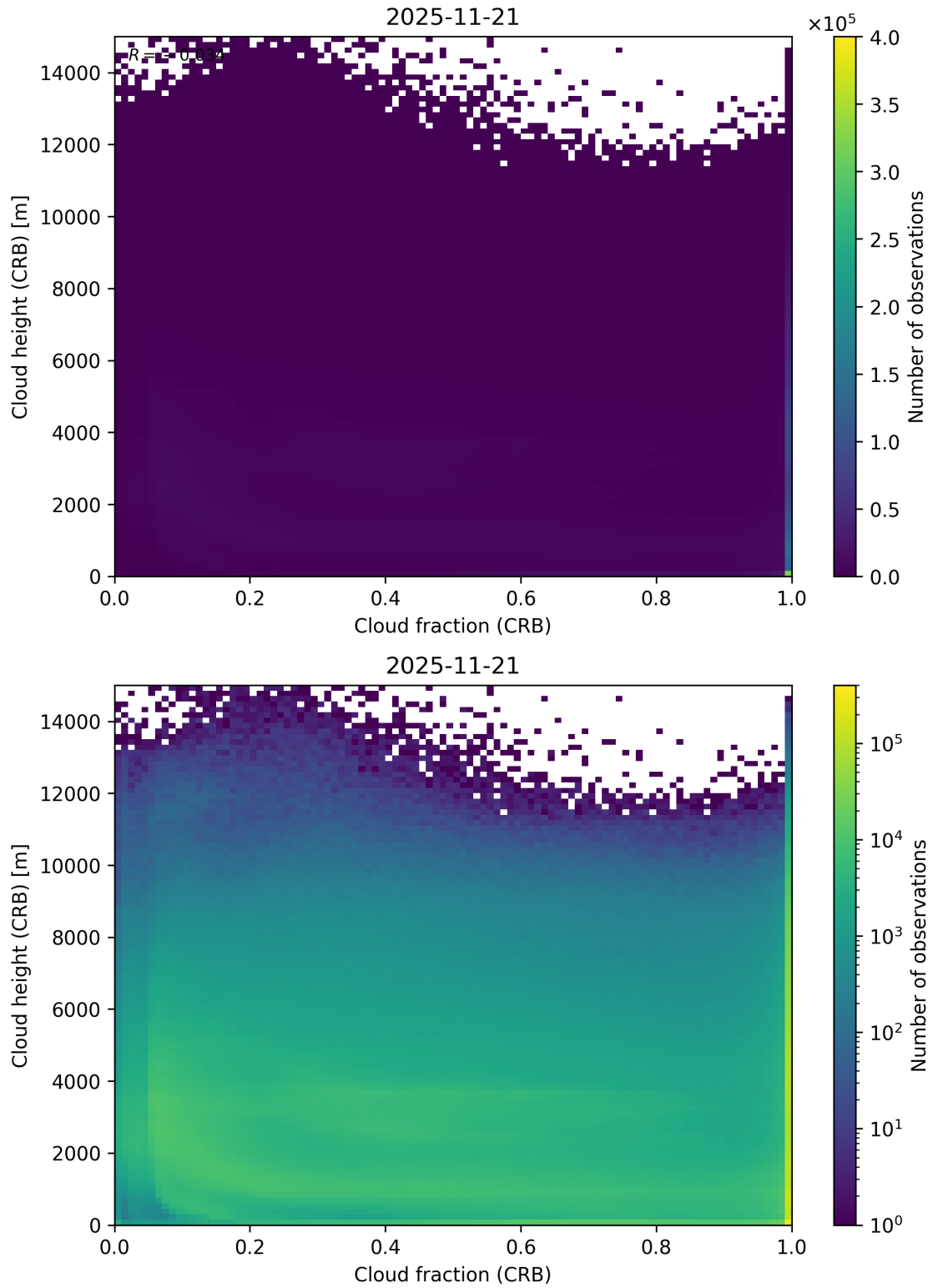
Figure 79: Scatter density plot of “Cloud fraction (CRB)” against “Cloud height (CRB)” for 2025-11-20 to 2025-11-22.
