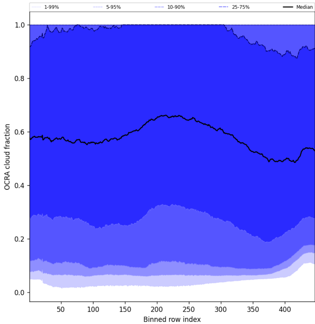
Figure 66: Along track statistics of “OCRA cloud fraction” for 2025-11-20 to 2025-11-22
