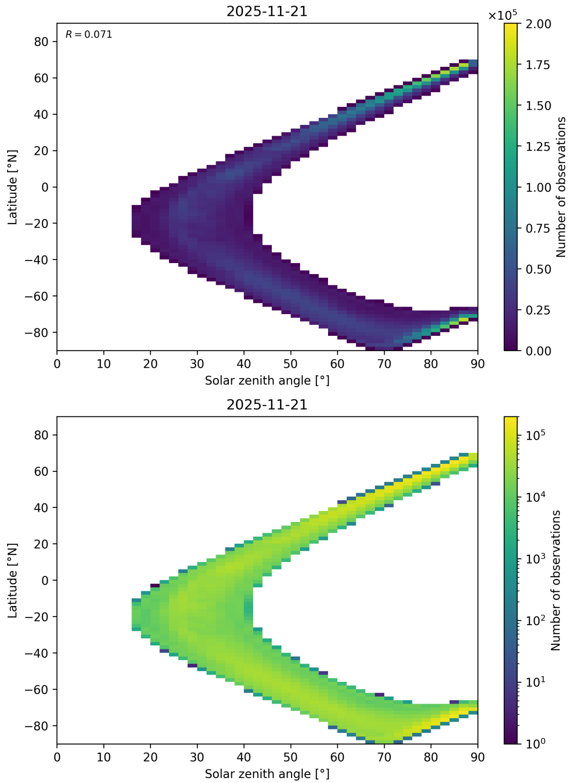
Figure 105: Scatter density plot of “Solar zenith angle” against “Latitude” for 2025-11-20 to 2025-11-22.
