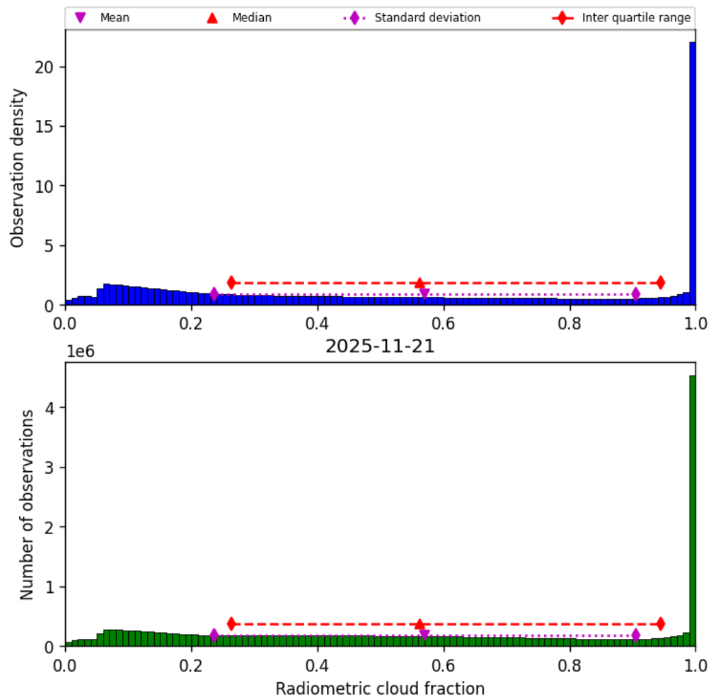
Figure 39: Histogram of “Radiometric cloud fraction” for 2025-11-20 to 2025-11-22
