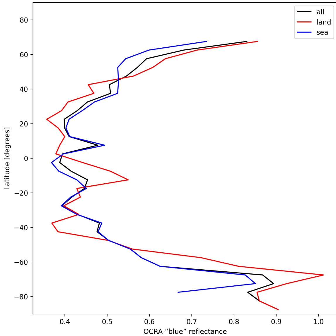
Figure 35: Zonal average of “OCRA “blue” reflectance” for 2025-11-20 to 2025-11-22.
