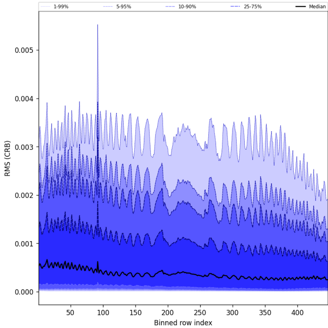
Figure 64: Along track statistics of “RMS (CRB)” for 2025-11-20 to 2025-11-22
