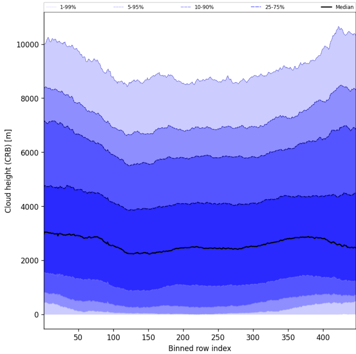
Figure 59: Along track statistics of “Cloud height (CRB)” for 2025-11-20 to 2025-11-22
