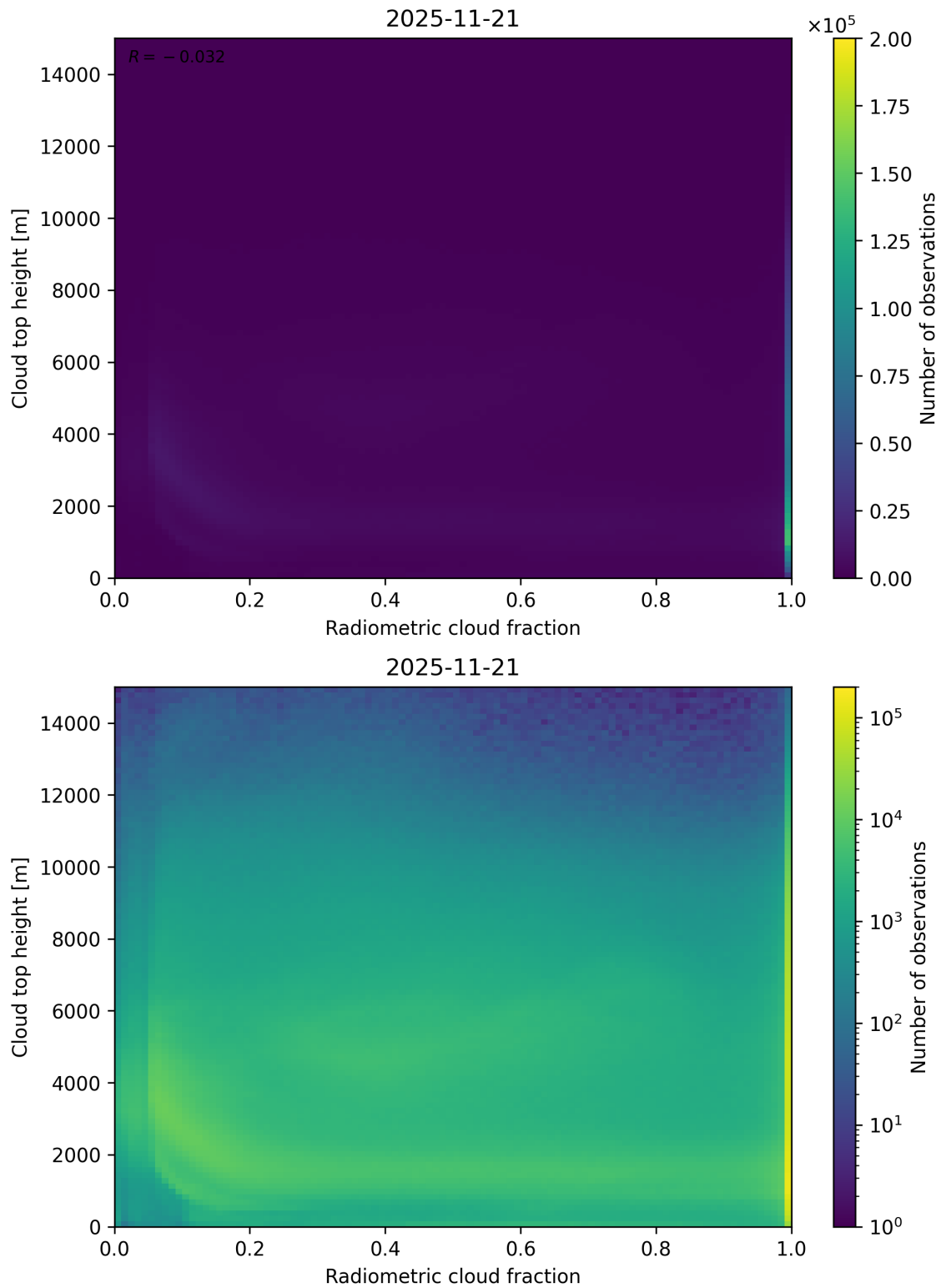
Figure 76: Scatter density plot of “Radiometric cloud fraction” against “Cloud top height” for 2025-11-20 to 2025-11-22.
