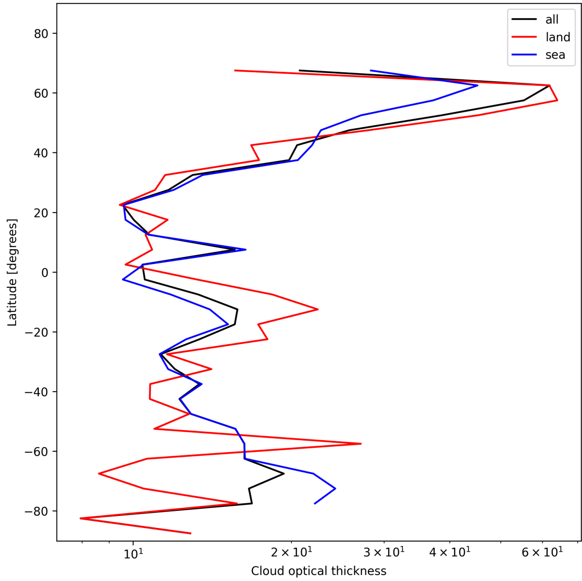
Figure 25: Zonal average of “Cloud optical thickness” for 2025-11-20 to 2025-11-22.
