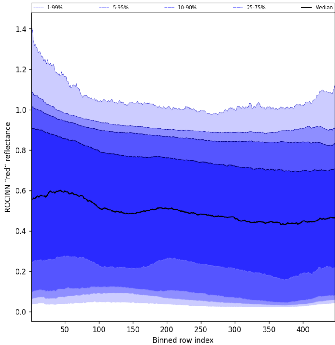
Figure 69: Along track statistics of "ROCINN "red" reflectance" for 2025-11-20 to 2025-11-22
