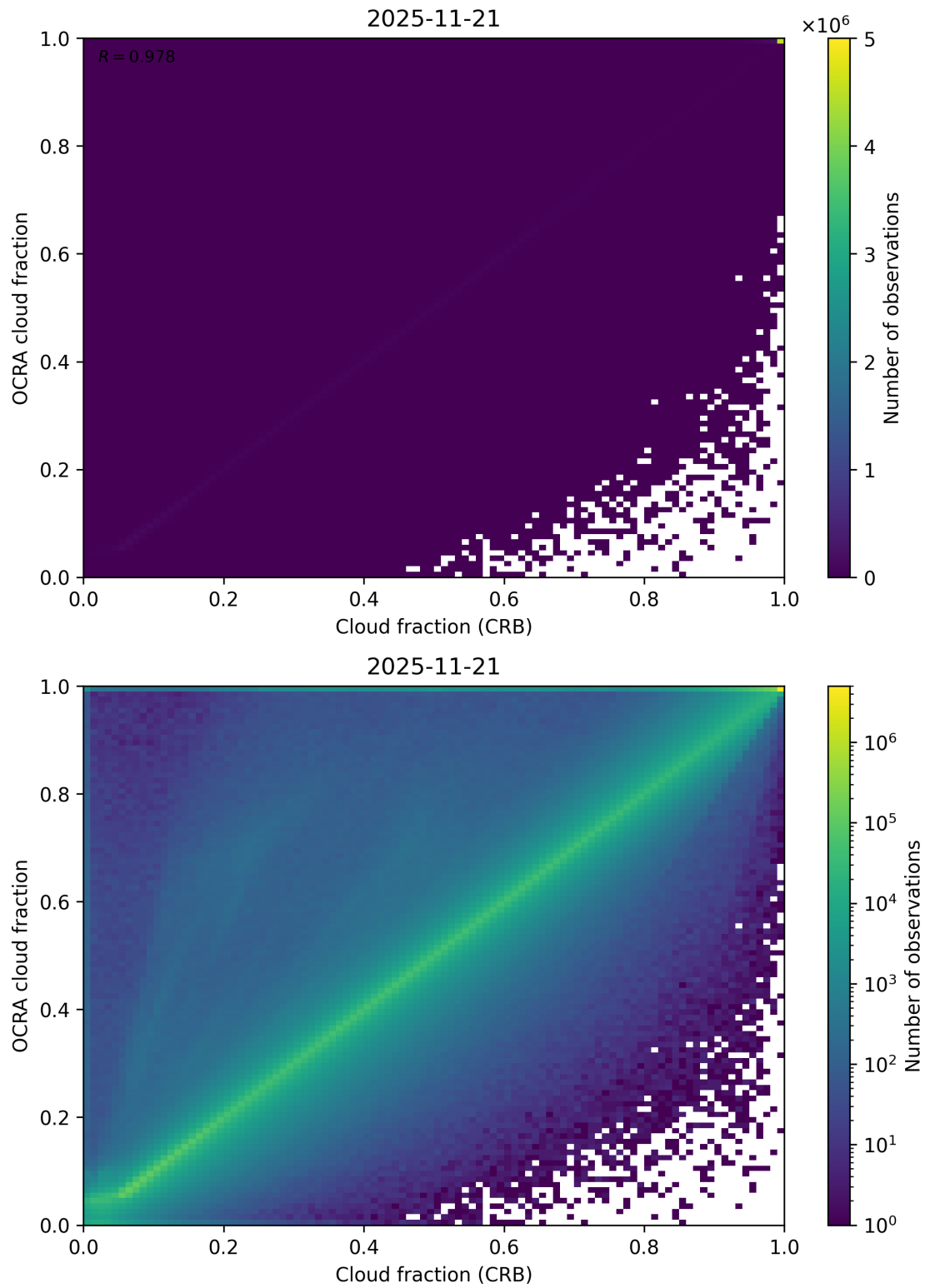
Figure 78: Scatter density plot of “Cloud fraction (CRB)” against “OCRA cloud fraction” for 2025-11-20 to 2025-11-22.
