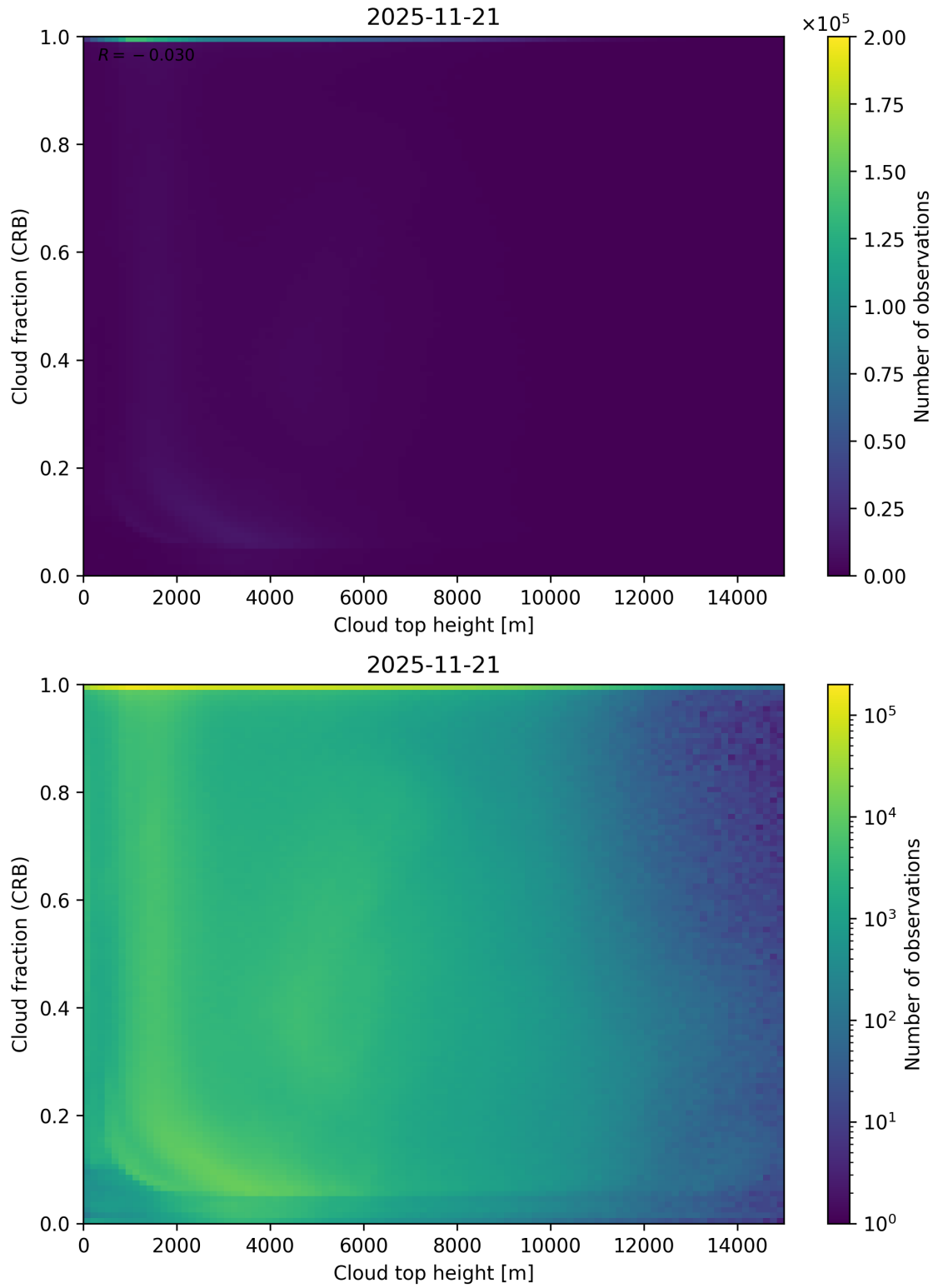
Figure 88: Scatter density plot of “Cloud top height” against “Cloud fraction (CRB)” for 2025-11-20 to 2025-11-22.
