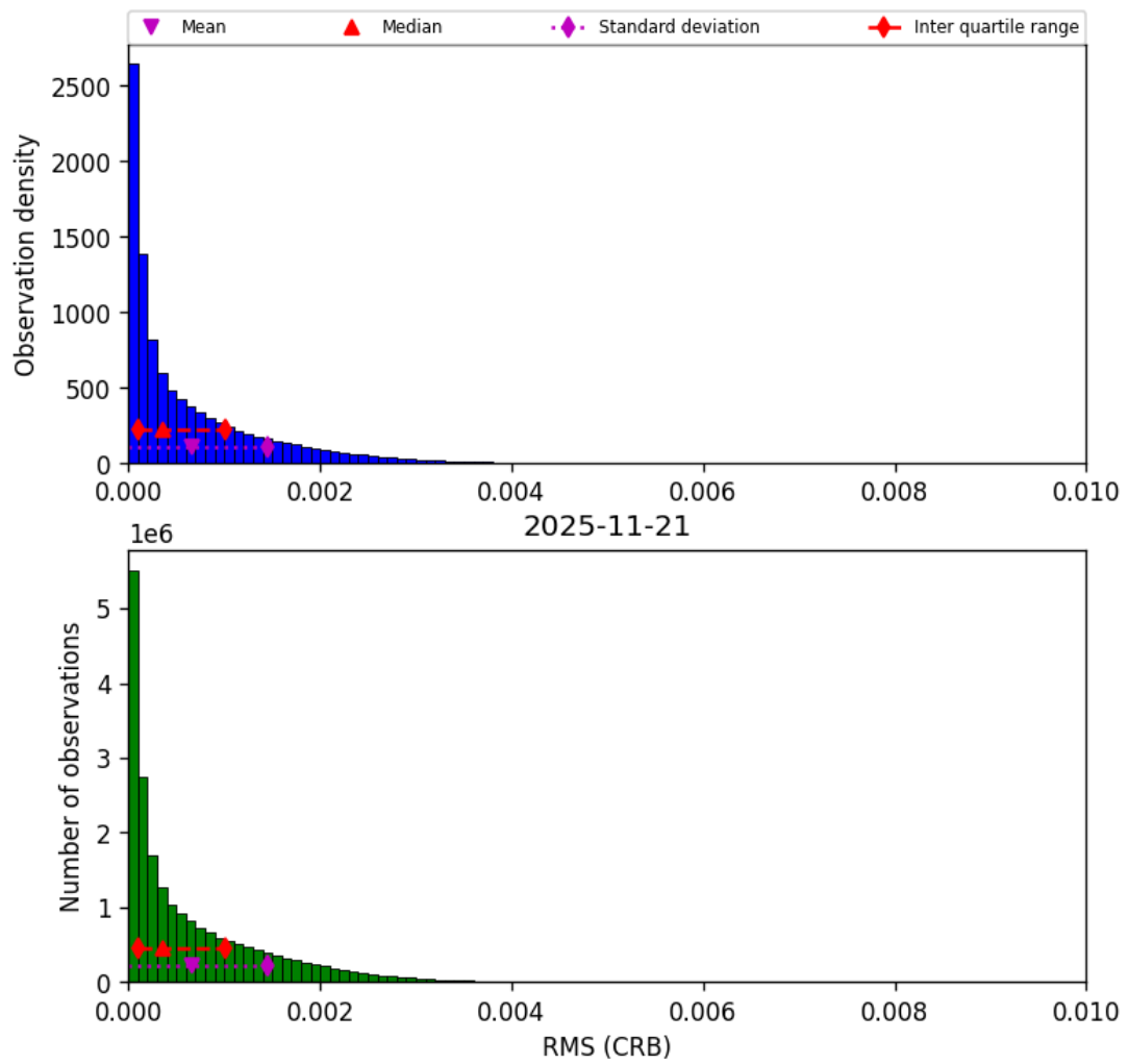
Figure 48: Histogram of “RMS (CRB)” for 2025-11-20 to 2025-11-22
