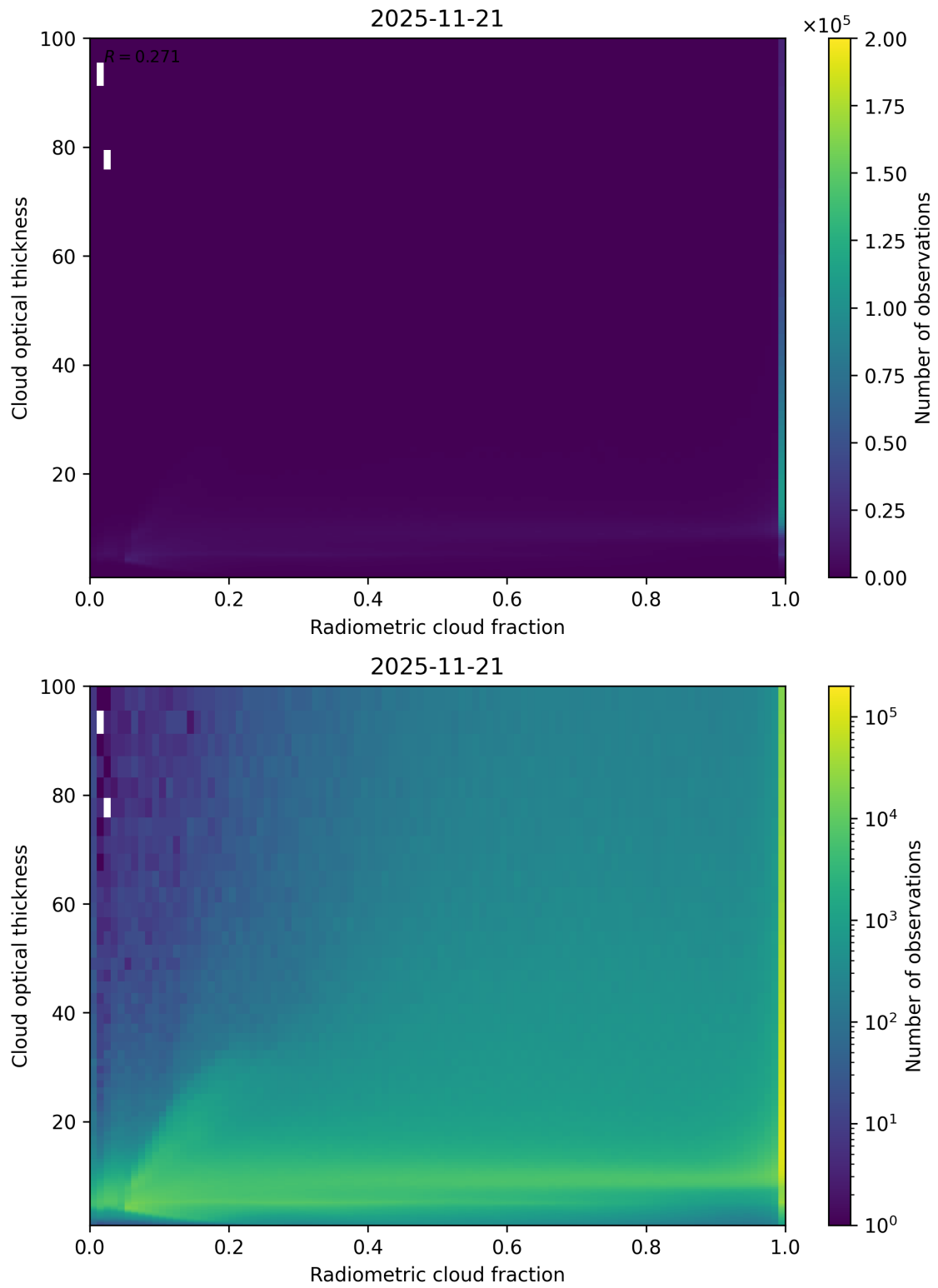
Figure 75: Scatter density plot of “Radiometric cloud fraction” against “Cloud optical thickness” for 2025-11-20 to 2025-11-22.
