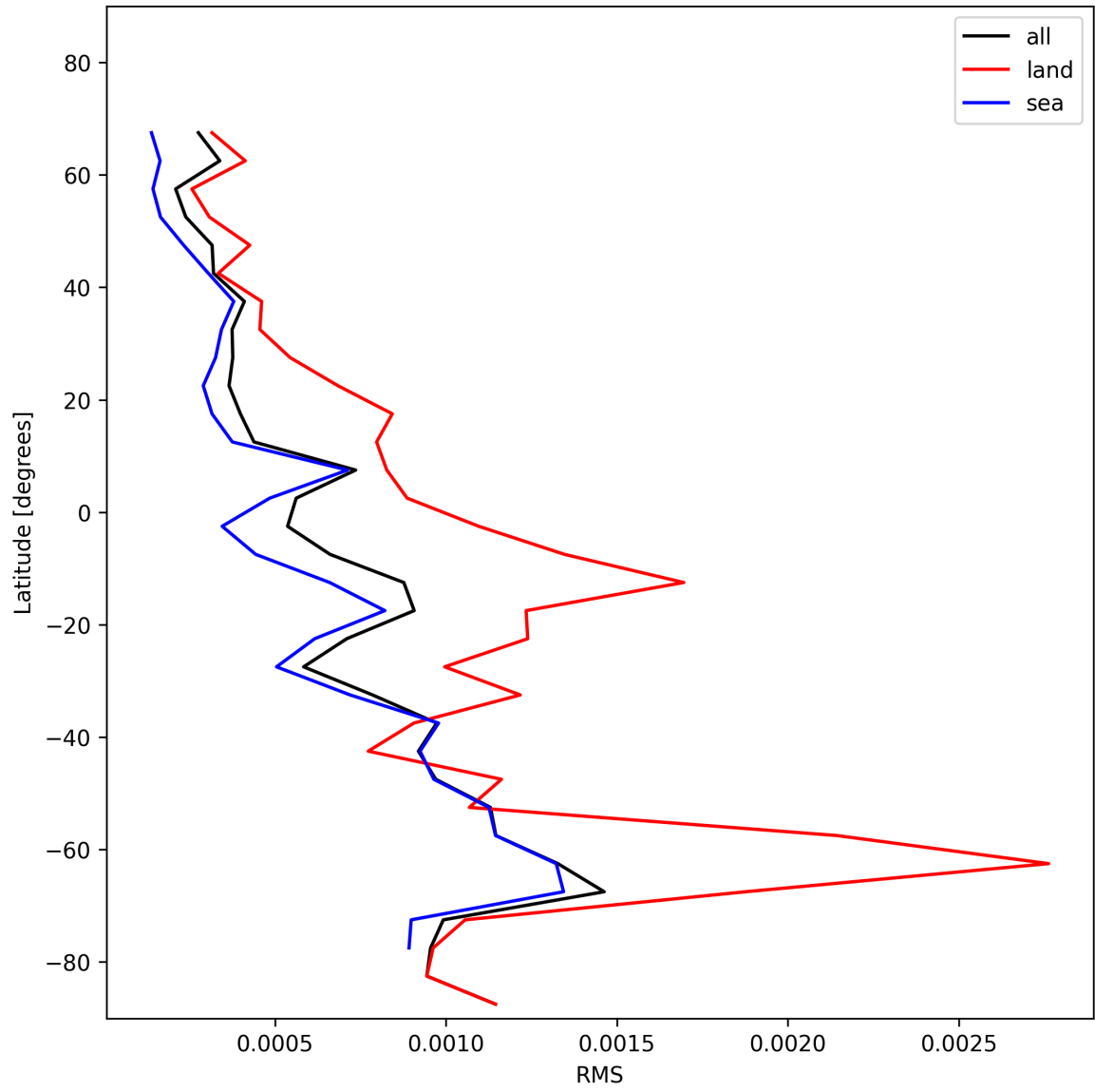
Figure 31: Zonal average of “RMS” for 2025-11-20 to 2025-11-22.
