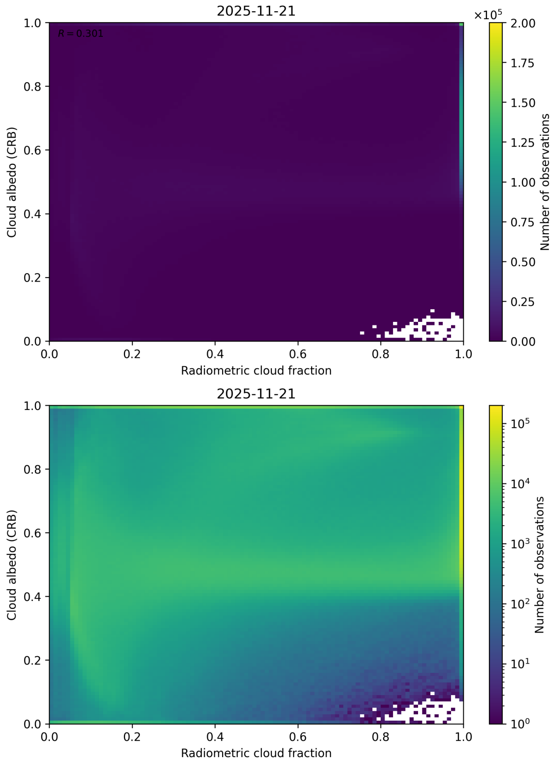
Figure 71: Scatter density plot of “Radiometric cloud fraction” against “Cloud albedo (CRB)” for 2025-11-20 to 2025-11-22.
