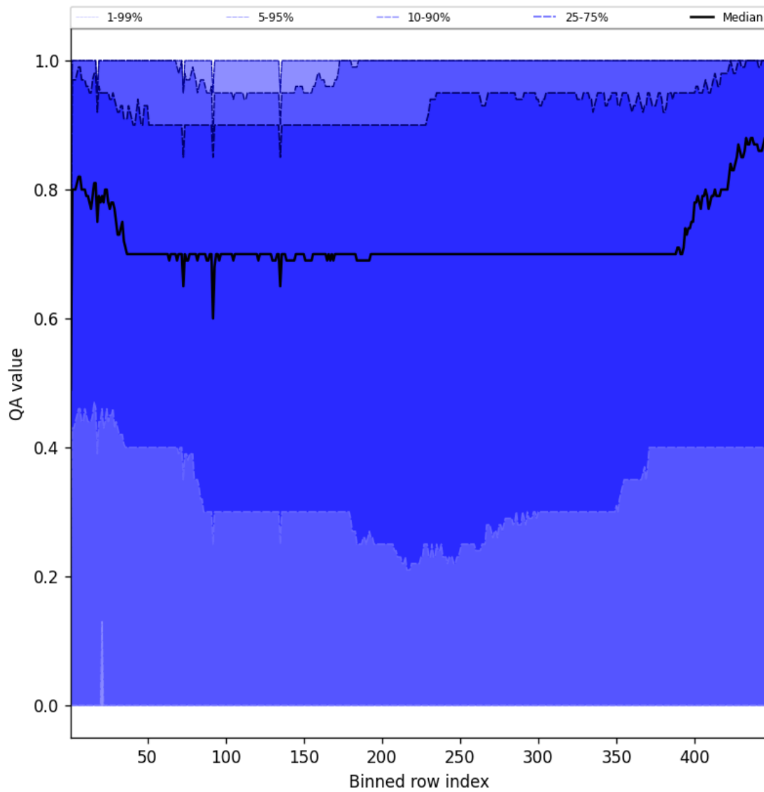
Figure 54: Along track statistics of “QA value” for 2025-11-20 to 2025-11-22
