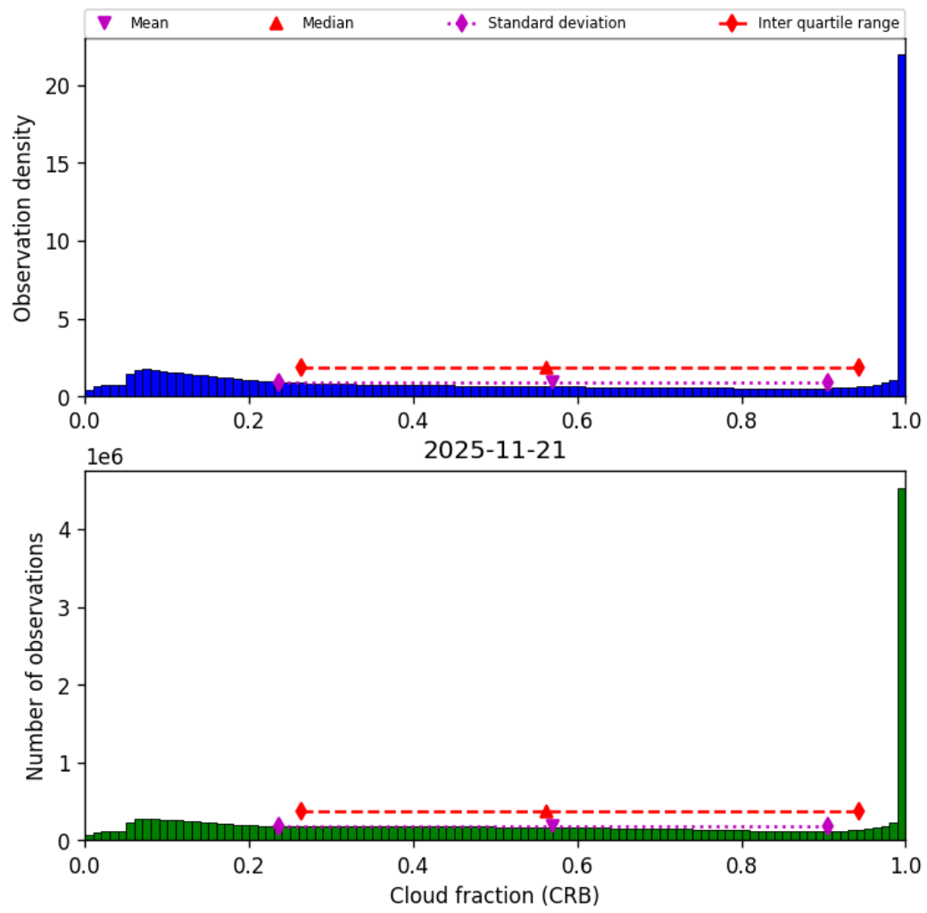
Figure 42: Histogram of “Cloud fraction (CRB)” for 2025-11-20 to 2025-11-22
