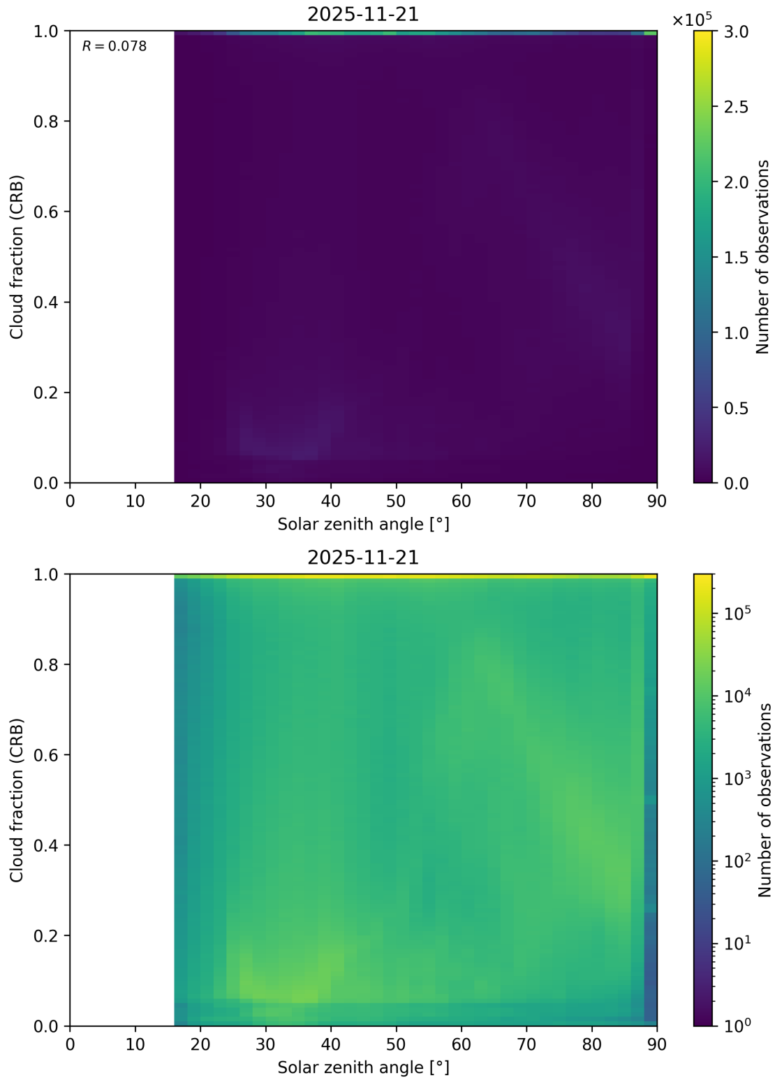
Figure 101: Scatter density plot of “Solar zenith angle” against “Cloud fraction (CRB)” for 2025-11-20 to 2025-11-22.
