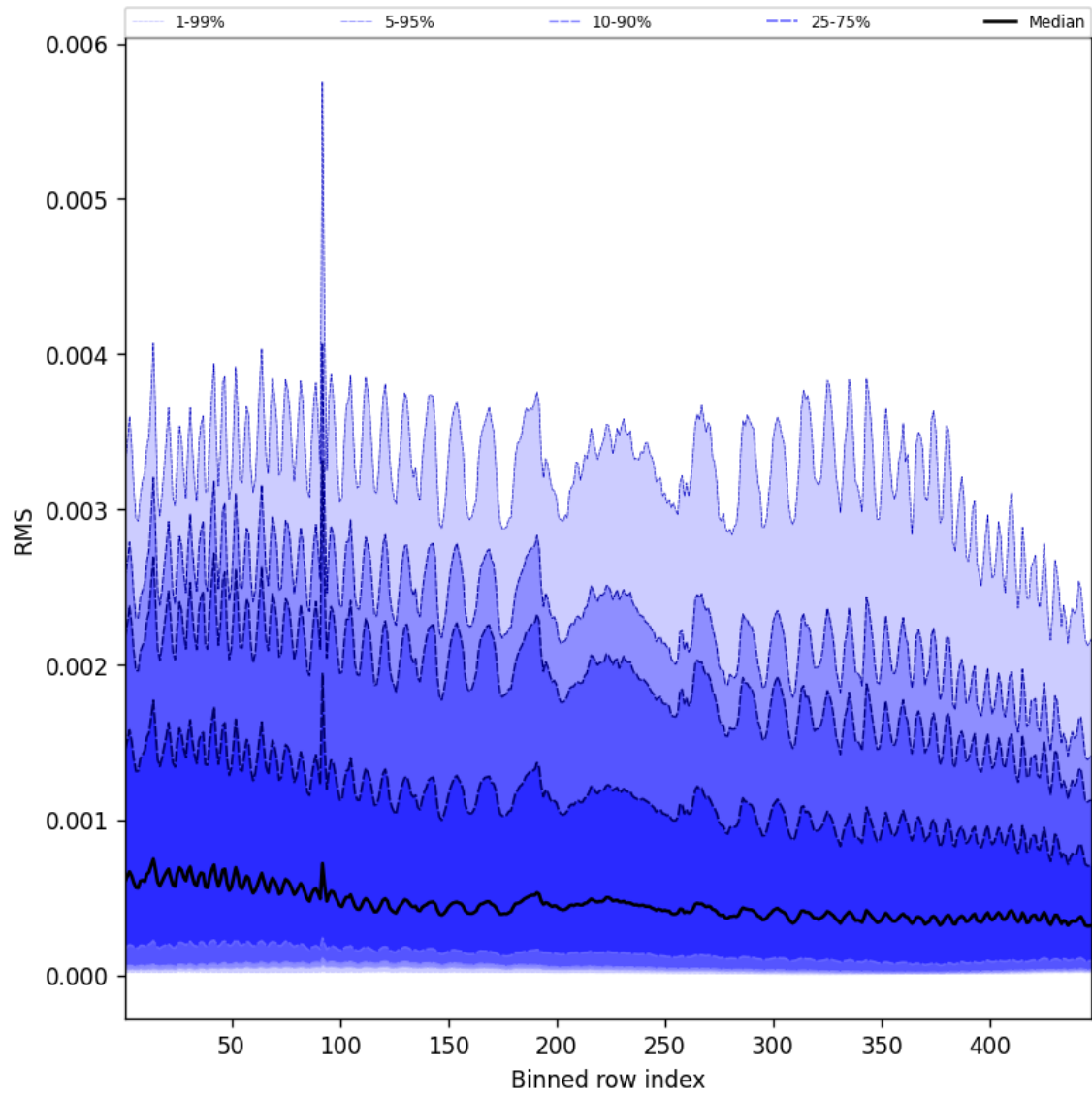
Figure 63: Along track statistics of “RMS” for 2025-11-20 to 2025-11-22
