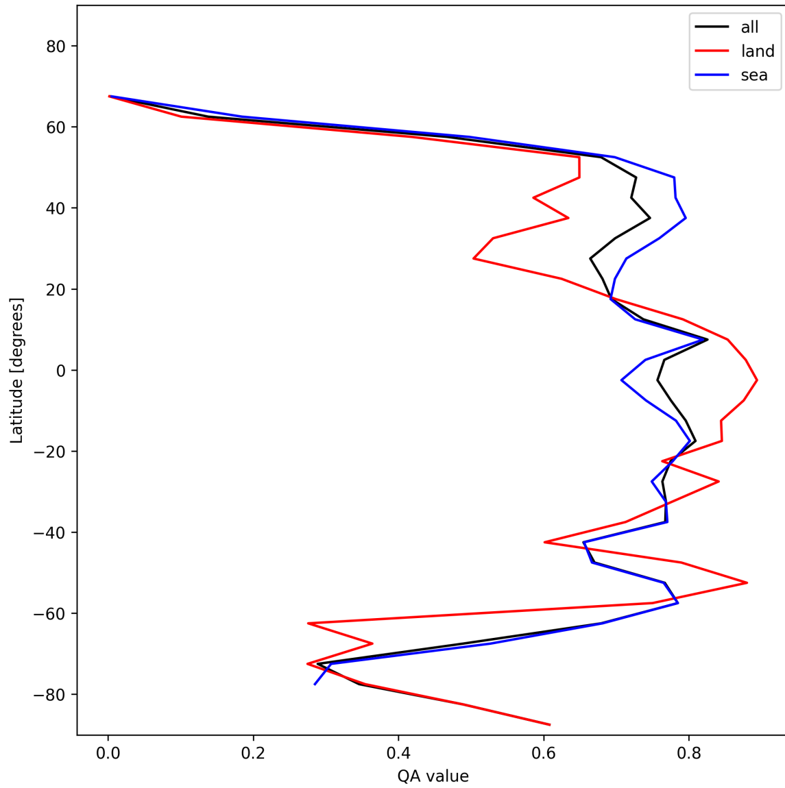
Figure 22: Zonal average of “QA value” for 2025-11-20 to 2025-11-22.
