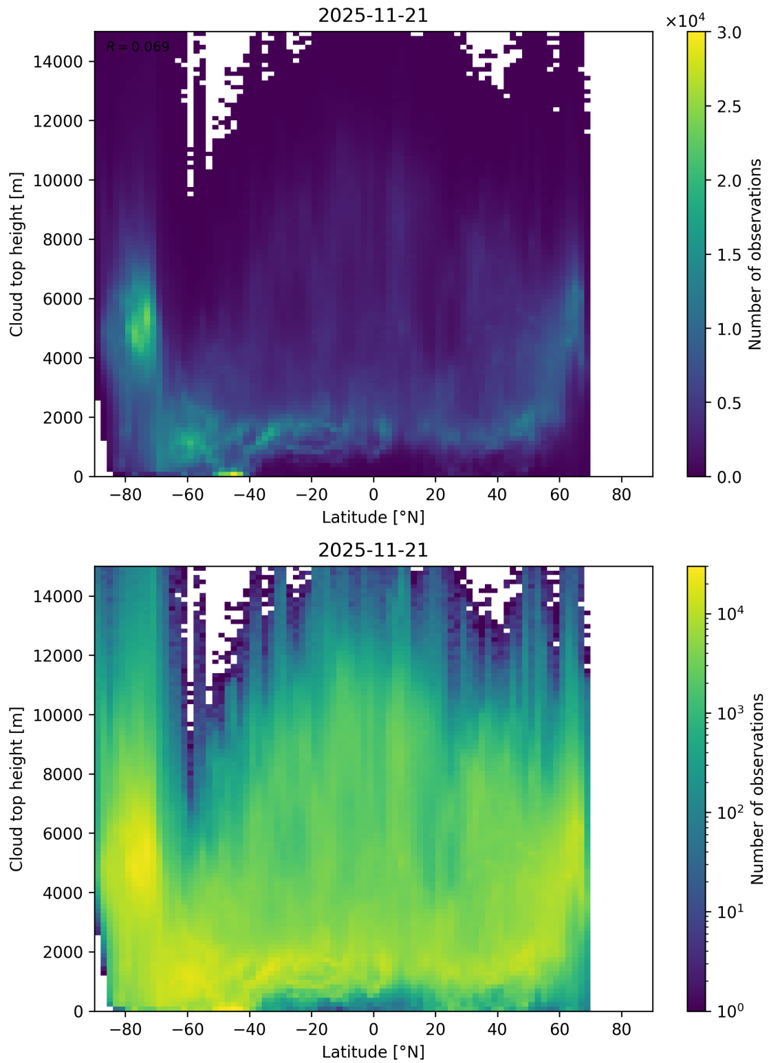
Figure 97: Scatter density plot of “Latitude” against “Cloud top height” for 2025-11-20 to 2025-11-22.
