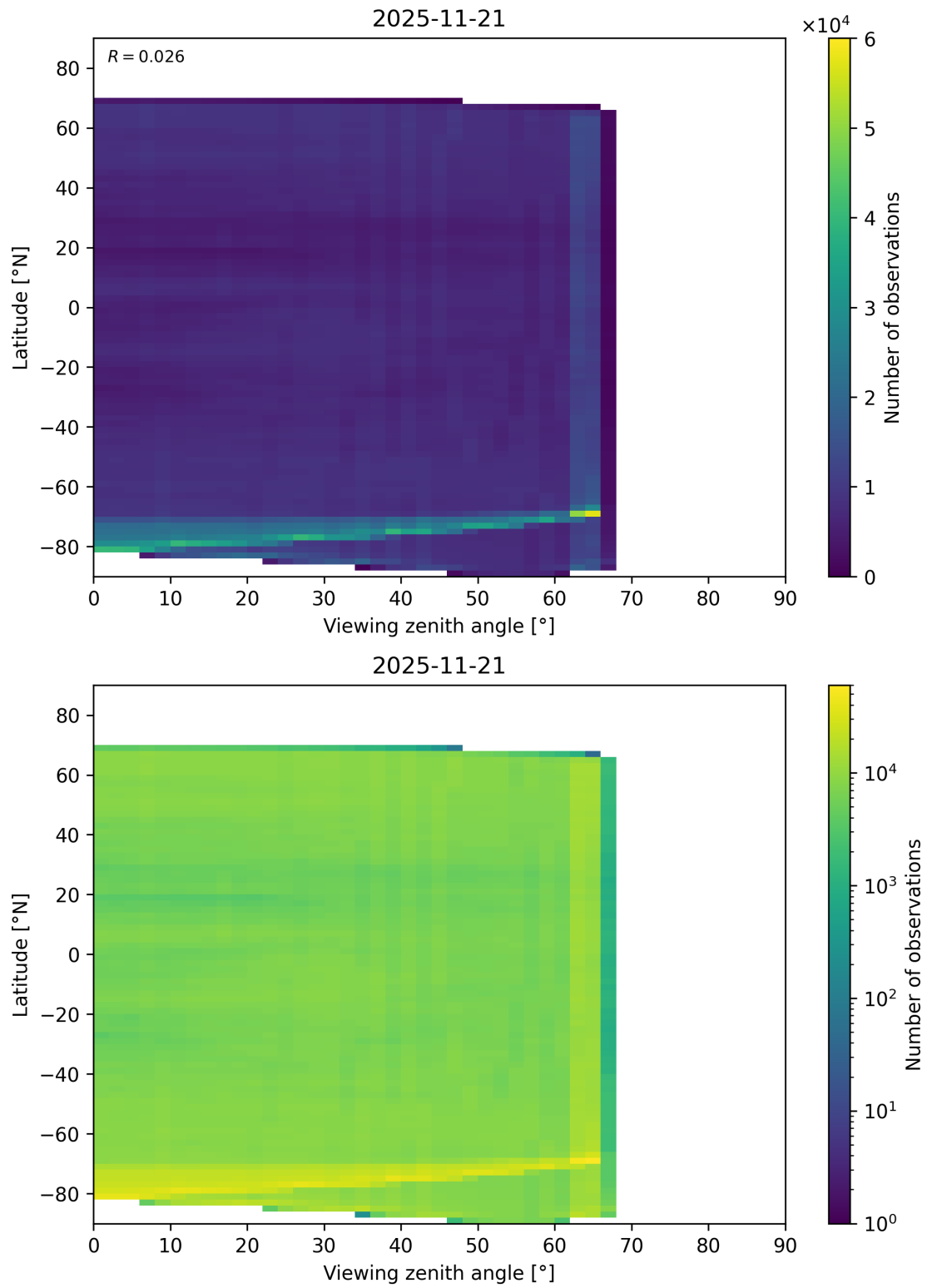
Figure 113: Scatter density plot of “Viewing zenith angle” against “Latitude” for 2025-11-20 to 2025-11-22.
