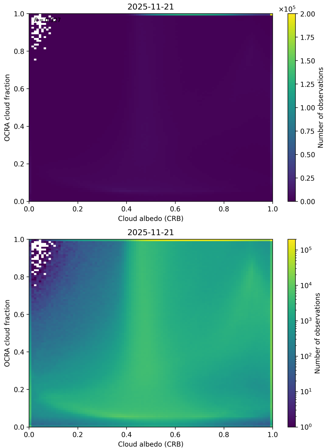
Figure 70: Scatter density plot of “Cloud albedo (CRB)” against “OCRA cloud fraction” for 2025-11-20 to 2025-11-22.
