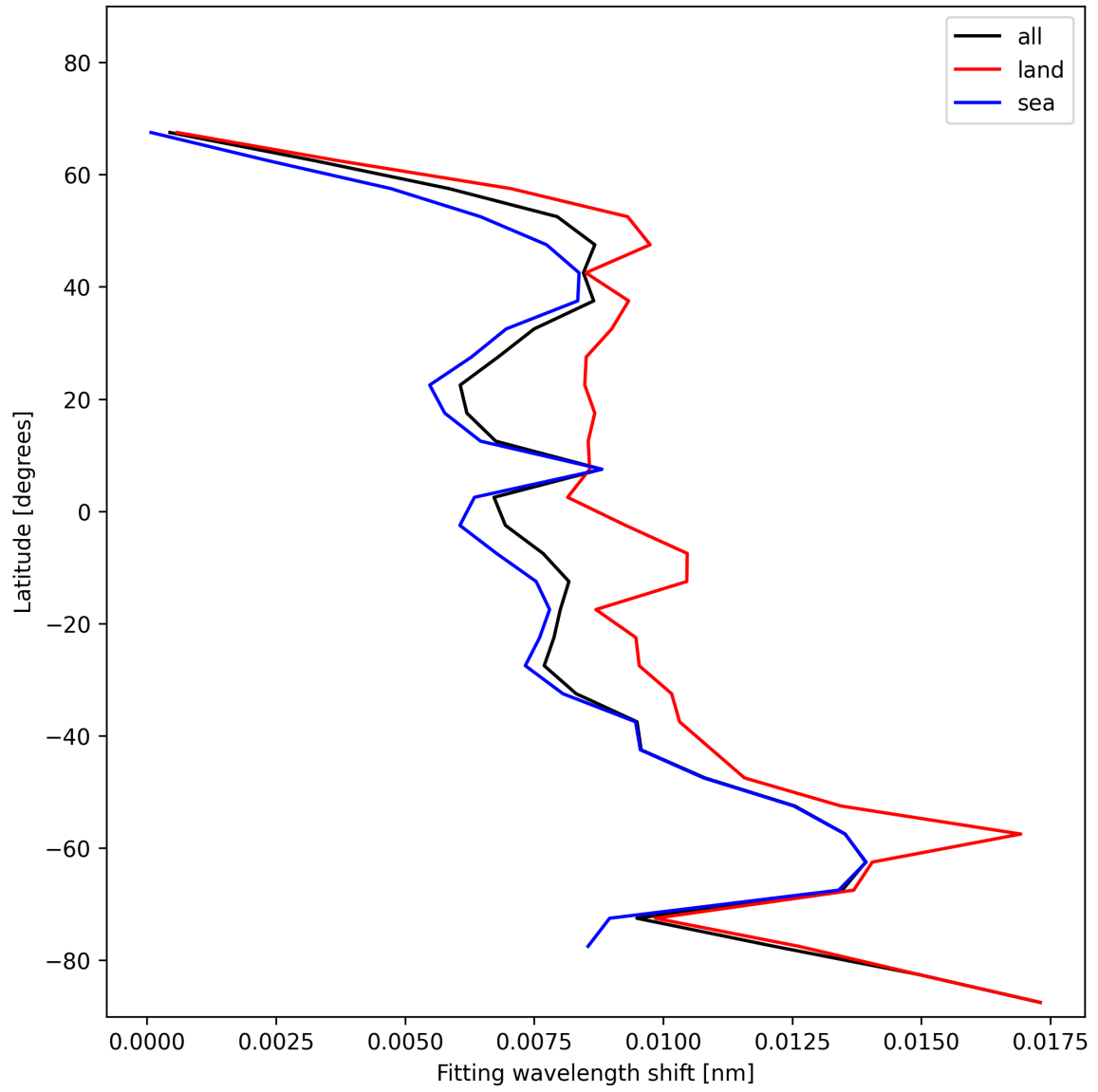
Figure 33: Zonal average of “Fitting wavelength shift” for 2025-11-20 to 2025-11-22.
