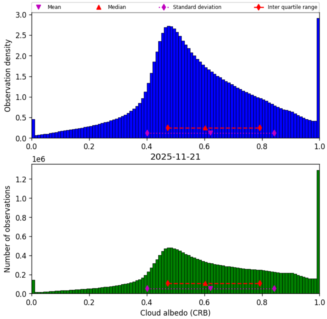
Figure 44: Histogram of “Cloud albedo (CRB)” for 2025-11-20 to 2025-11-22
