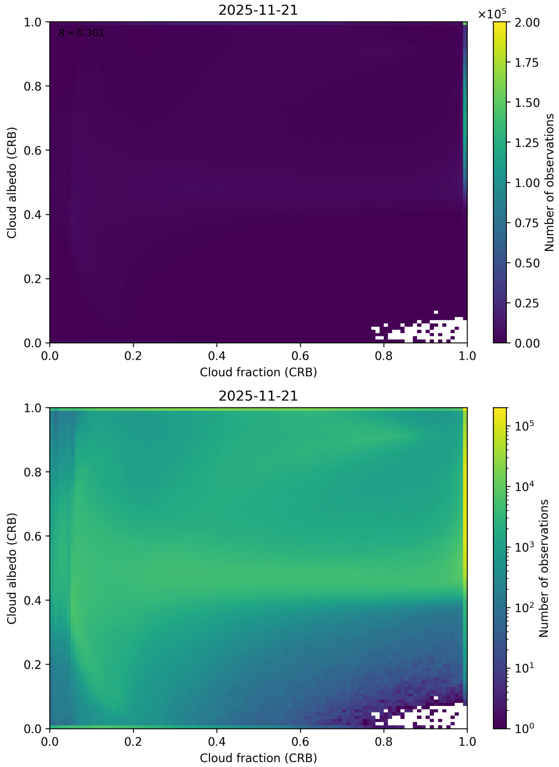
Figure 77: Scatter density plot of “Cloud fraction (CRB)” against “Cloud albedo (CRB)” for 2025-11-20 to 2025-11-22.
