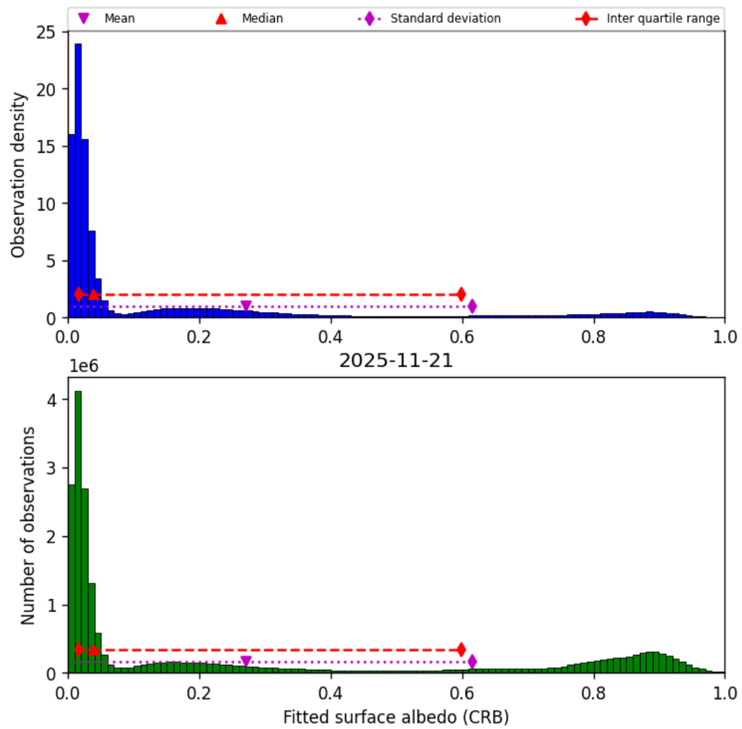
Figure 46: Histogram of “Fitted surface albedo (CRB)” for 2025-11-20 to 2025-11-22
