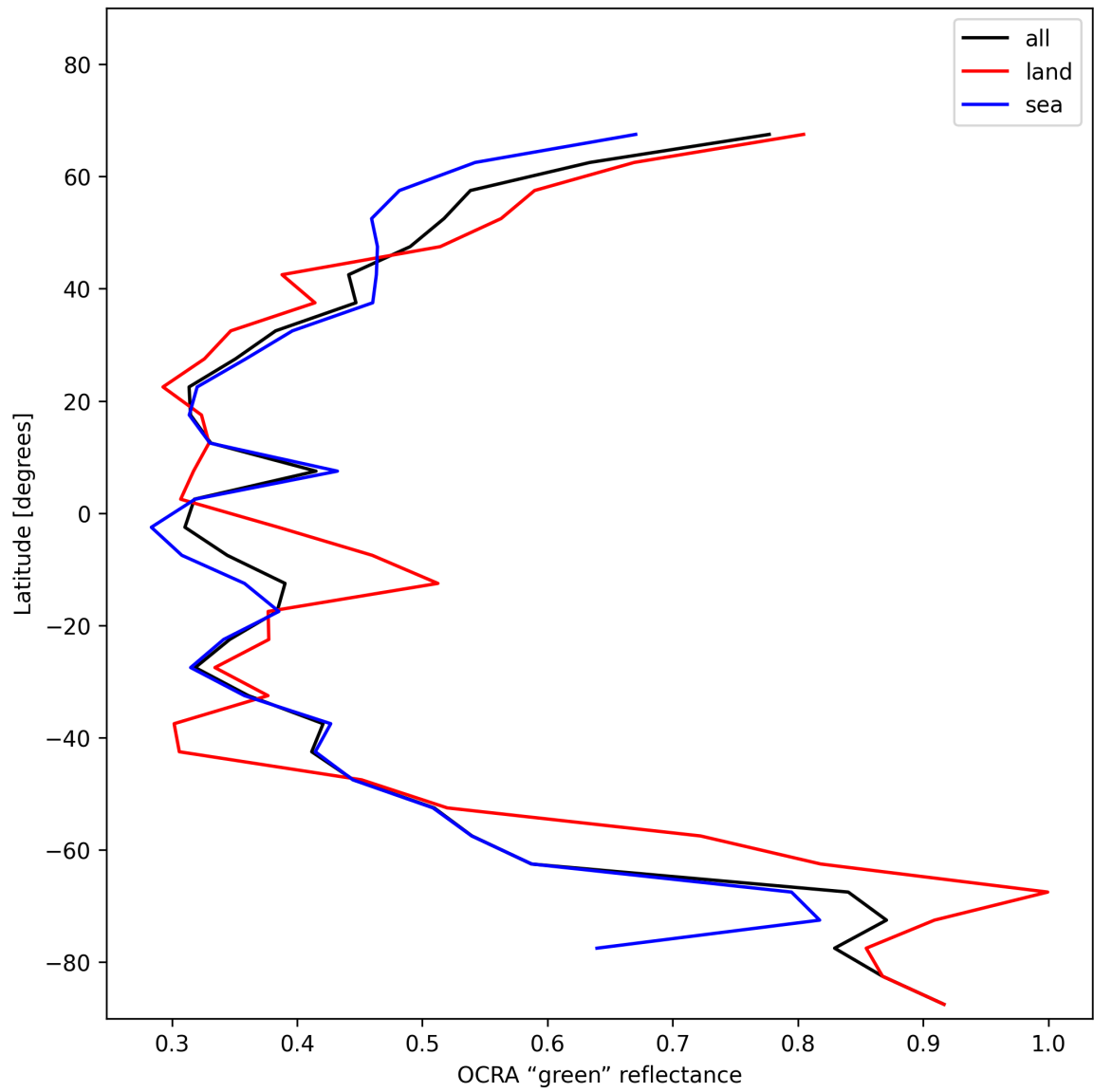
Figure 36: Zonal average of "OCRA "green" reflectance" for 2025-11-20 to 2025-11-22.
