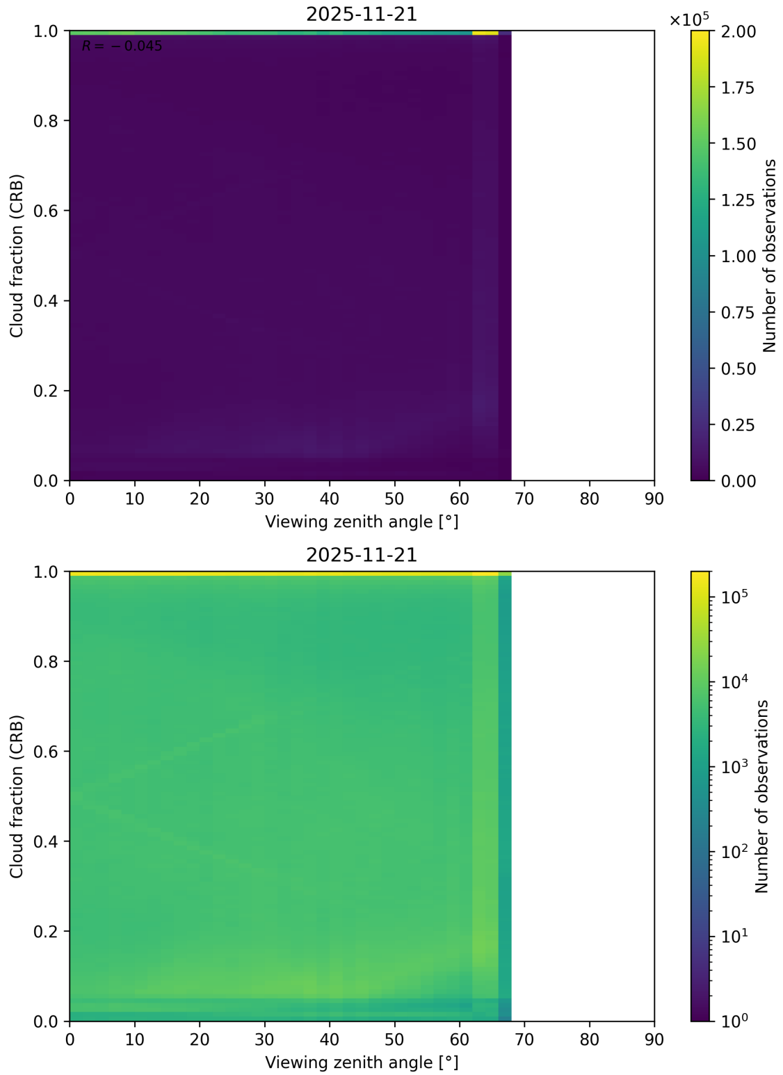
Figure 109: Scatter density plot of “Viewing zenith angle” against “Cloud fraction (CRB)” for 2025-11-20 to 2025-11-22.
