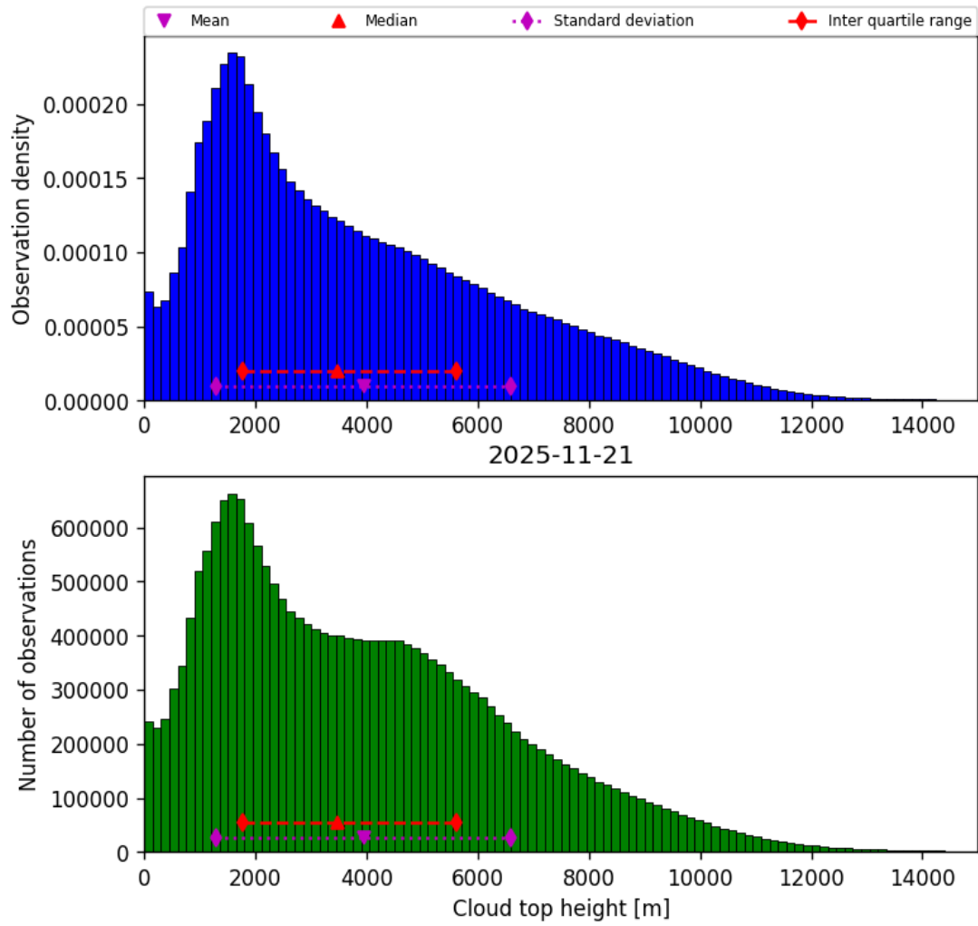
Figure 40: Histogram of “Cloud top height” for 2025-11-20 to 2025-11-22
