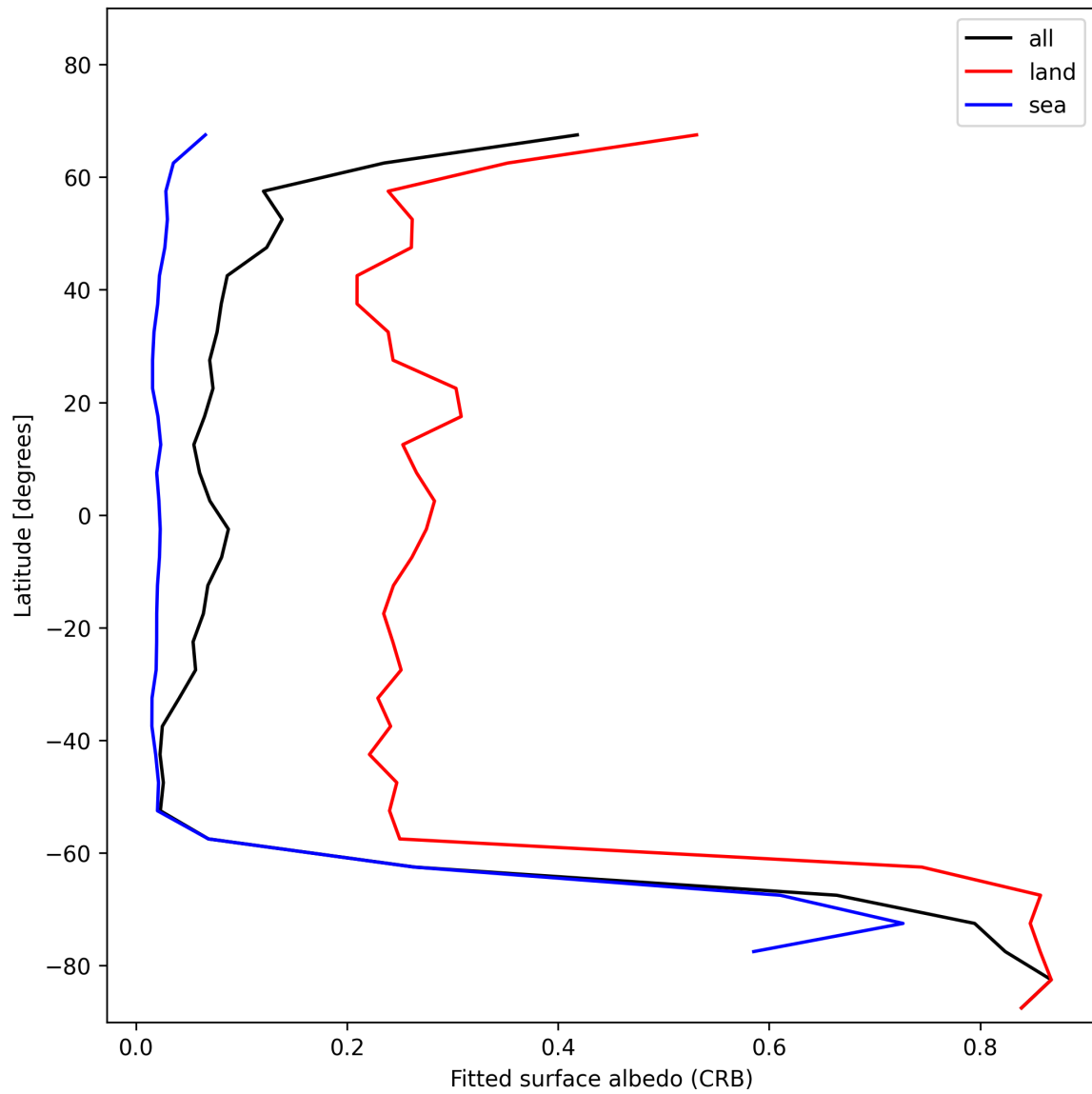
Figure 30: Zonal average of “Fitted surface albedo (CRB)” for 2025-11-20 to 2025-11-22.
