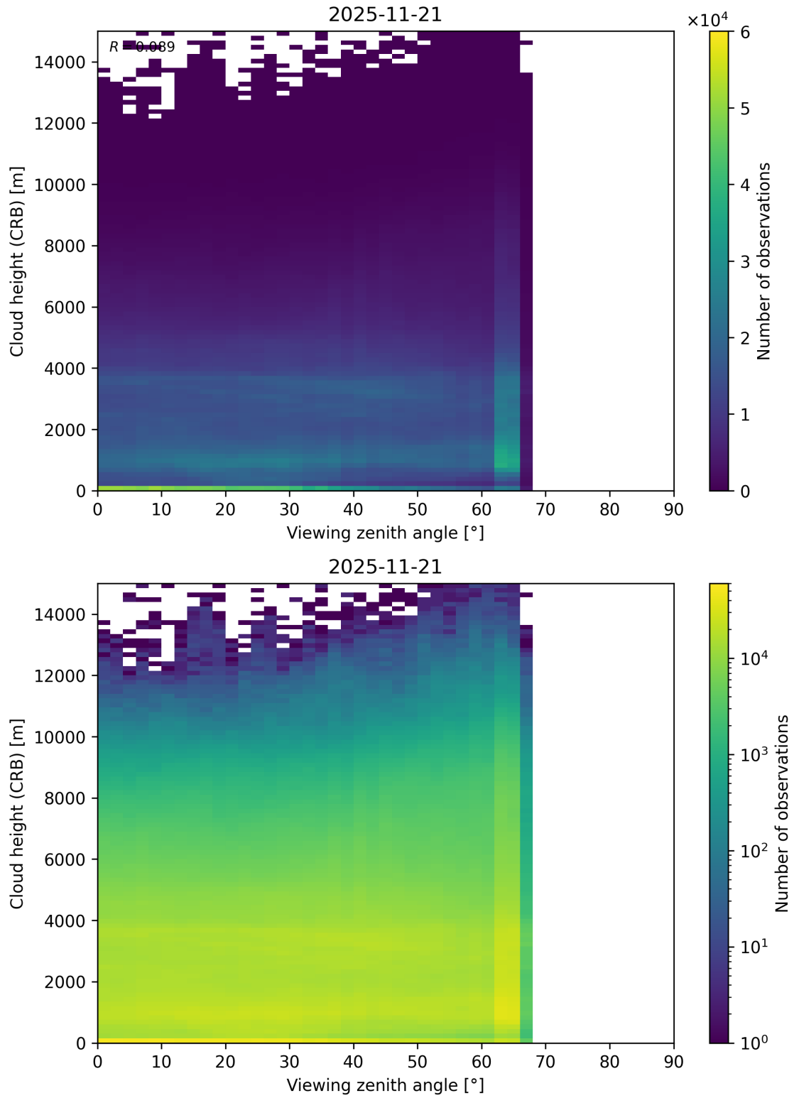
Figure 110: Scatter density plot of “Viewing zenith angle” against “Cloud height (CRB)” for 2025-11-20 to 2025-11-22.
