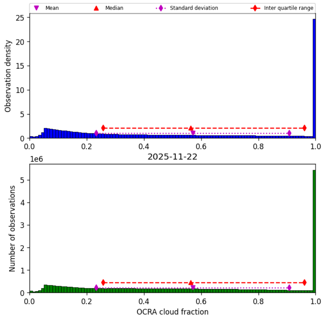
Figure 50: Histogram of “OCRA cloud fraction” for 2025-11-21 to 2025-11-23
