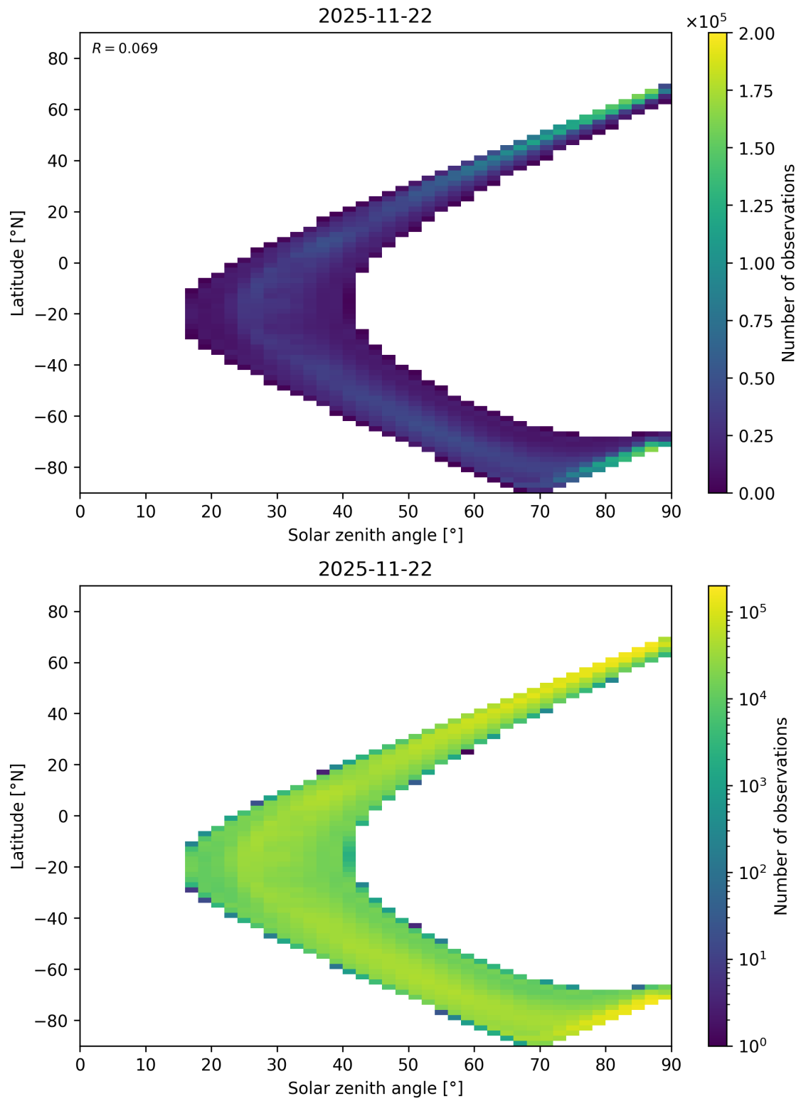
Figure 105: Scatter density plot of “Solar zenith angle” against “Latitude” for 2025-11-21 to 2025-11-23.
