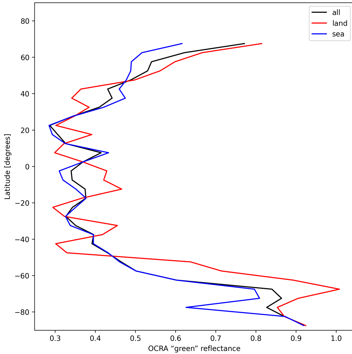
Figure 36: Zonal average of “OCRA “green” reflectance” for 2025-11-21 to 2025-11-23.
