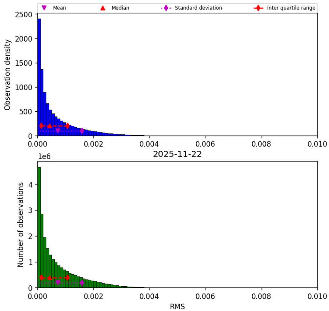
Figure 47: Histogram of “RMS” for 2025-11-21 to 2025-11-23
