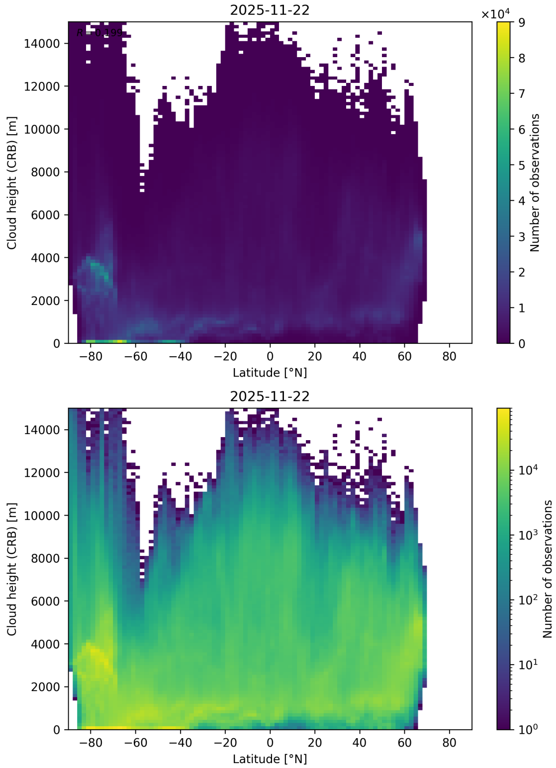
Figure 95: Scatter density plot of “Latitude” against “Cloud height (CRB)” for 2025-11-21 to 2025-11-23.
