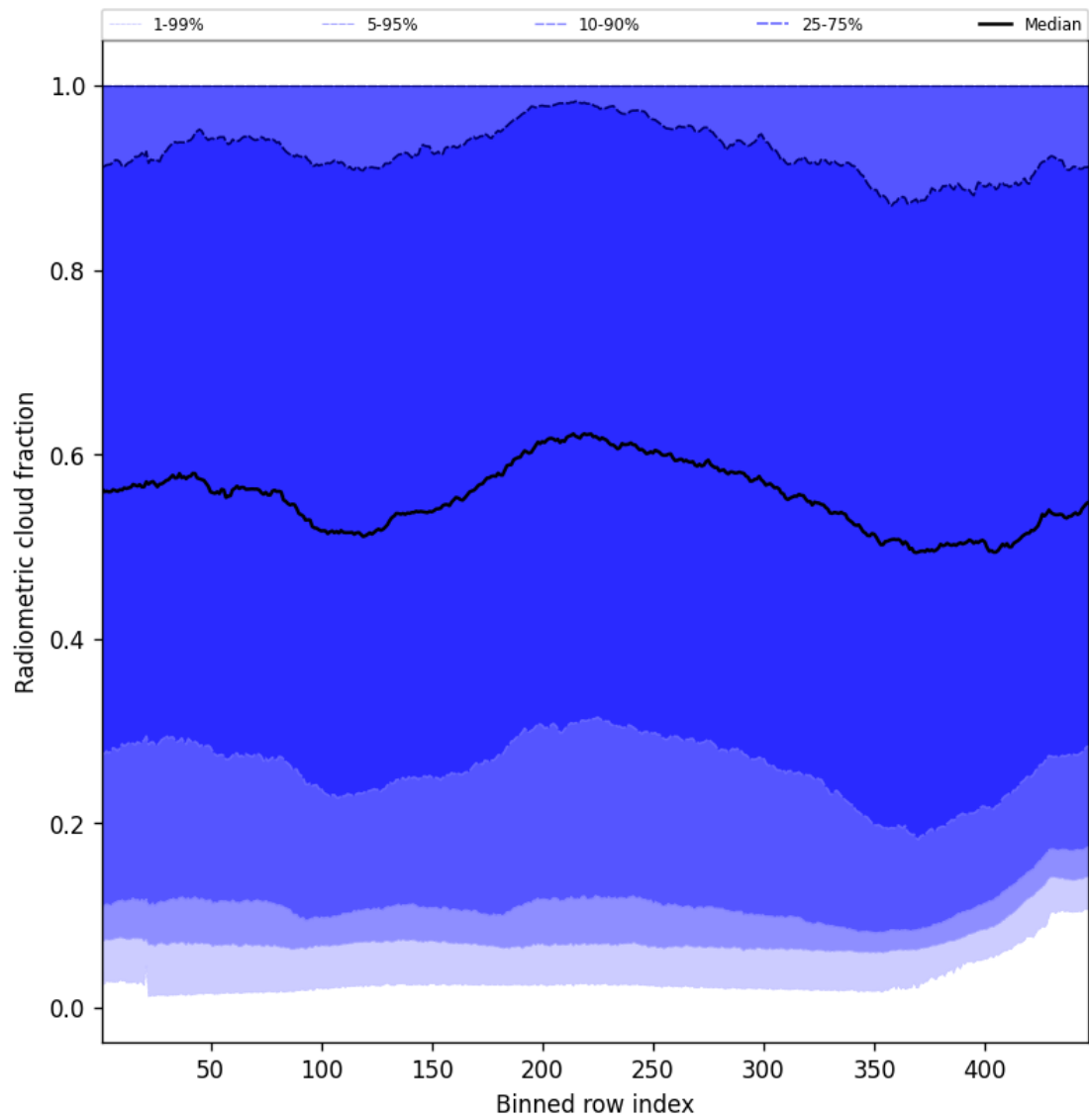
Figure 55: Along track statistics of “Radiometric cloud fraction” for 2025-11-21 to 2025-11-23
