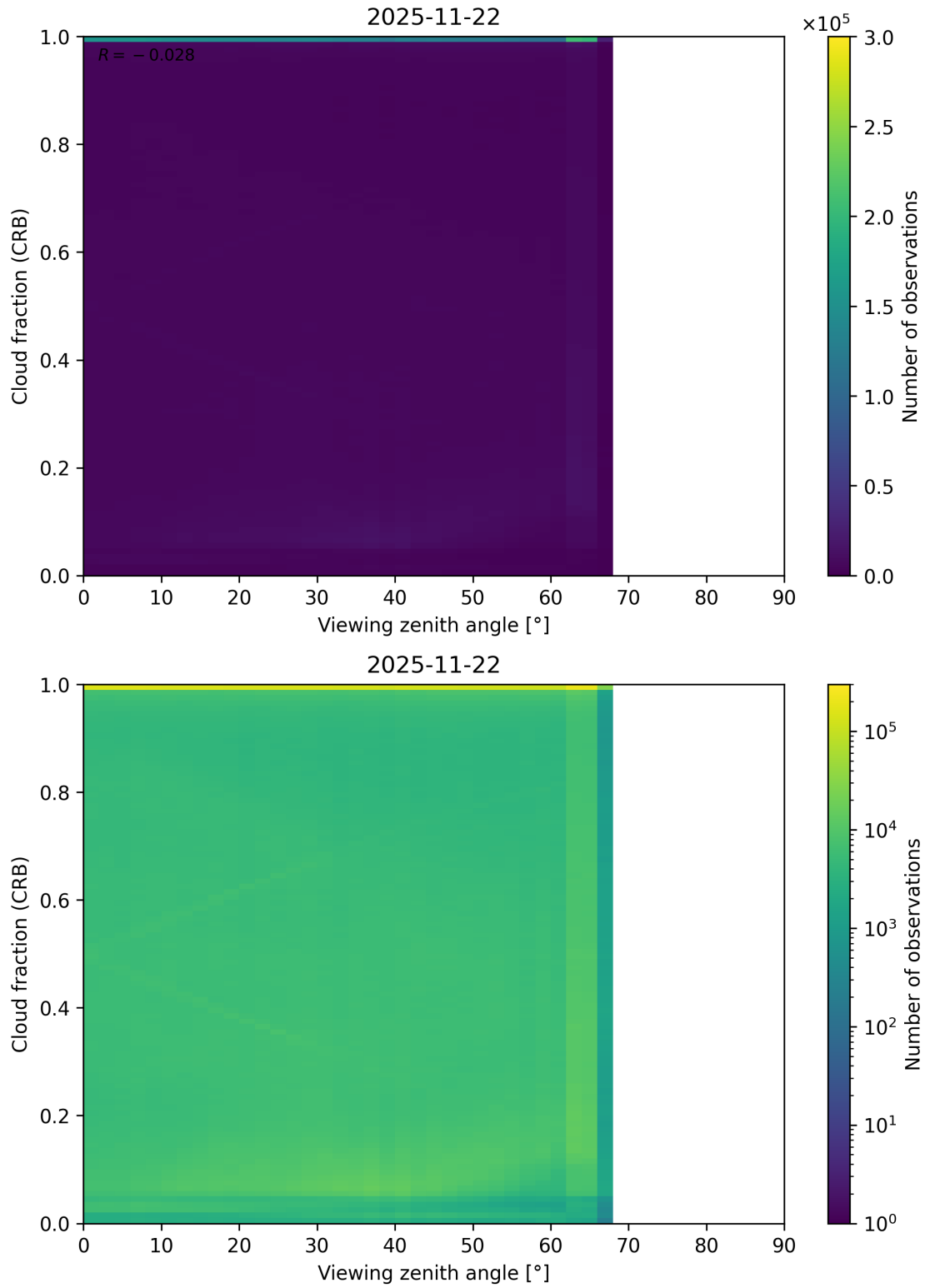
Figure 109: Scatter density plot of “Viewing zenith angle” against “Cloud fraction (CRB)” for 2025-11-21 to 2025-11-23.
