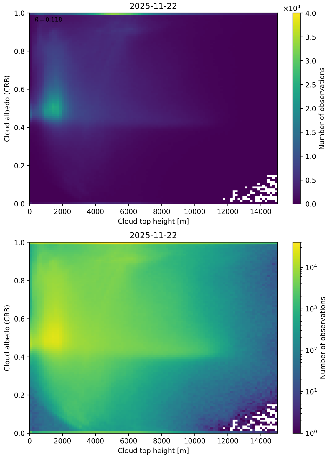
Figure 86: Scatter density plot of “Cloud top height” against “Cloud albedo (CRB)” for 2025-11-21 to 2025-11-23.
