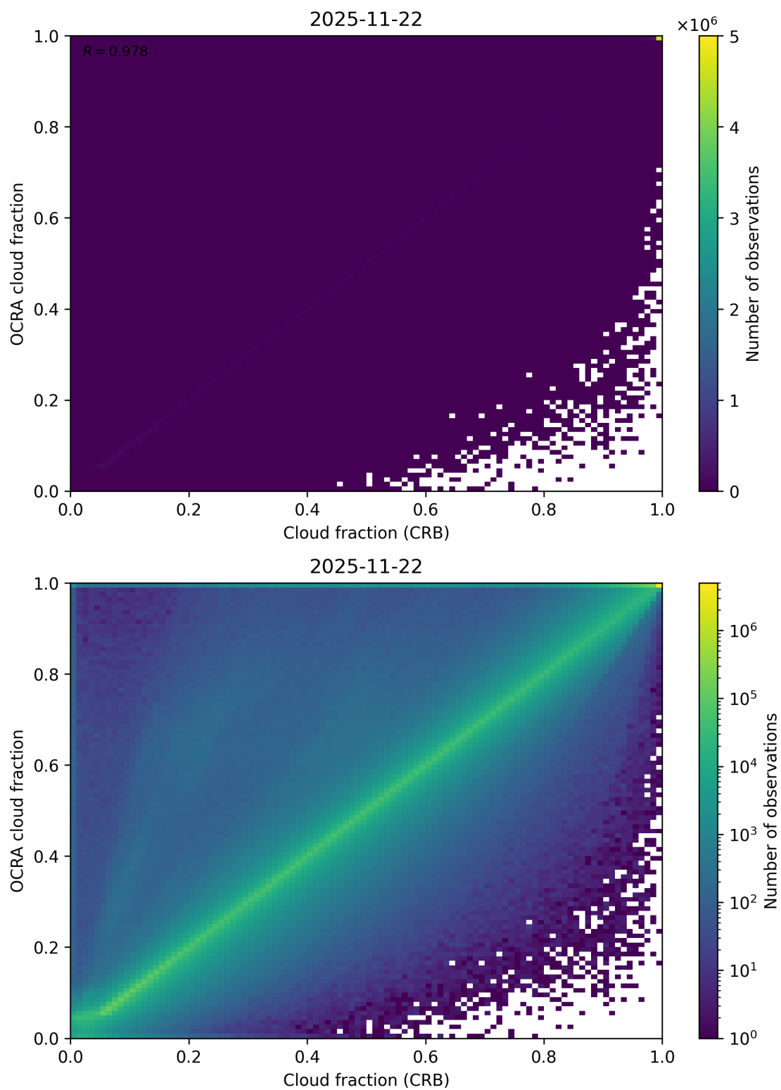
Figure 78: Scatter density plot of “Cloud fraction (CRB)” against “OCRA cloud fraction” for 2025-11-21 to 2025-11-23.
