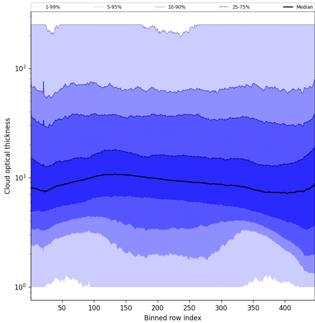
Figure 57: Along track statistics of “Cloud optical thickness” for 2025-11-21 to 2025-11-23
