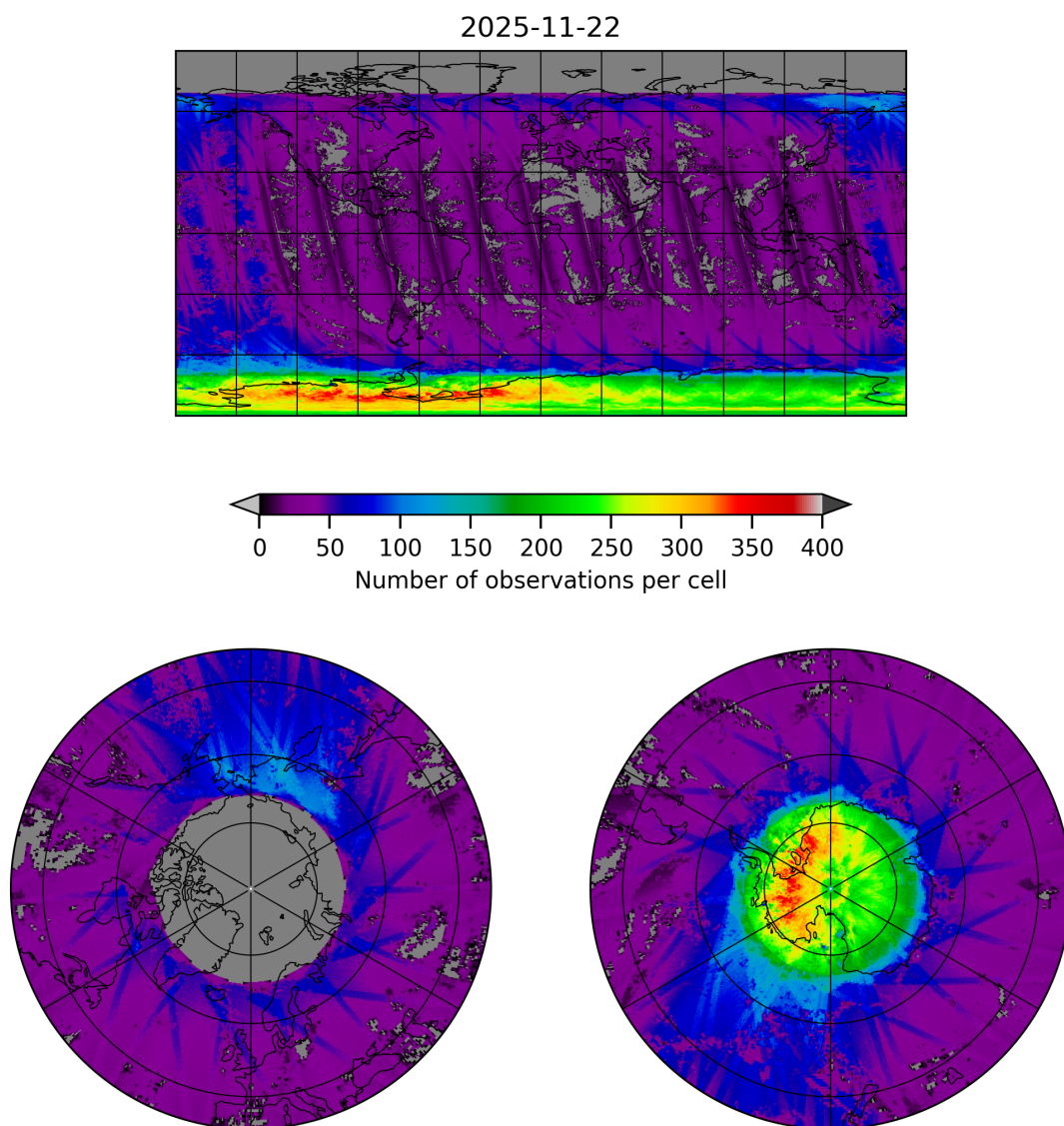
Figure 21: Map of the number of observations for 2025-11-21 to 2025-11-23
