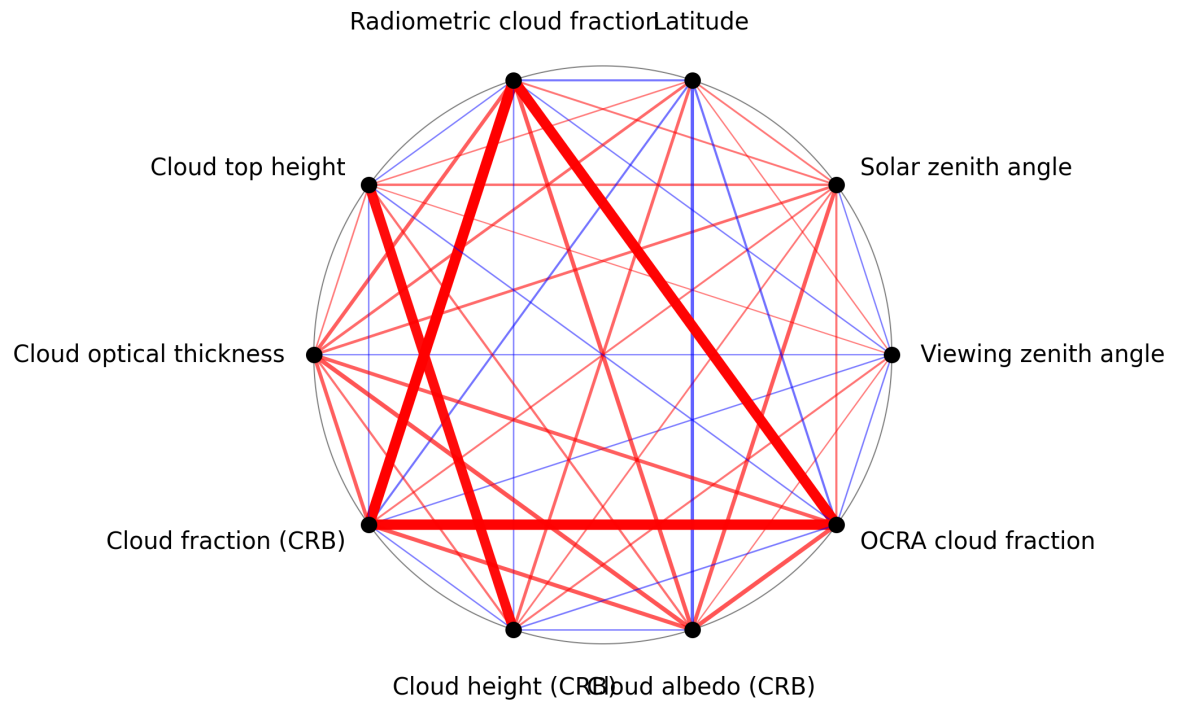
Figure 1: Map of correlation graph for 2025-11-21 to 2025-11-23.
