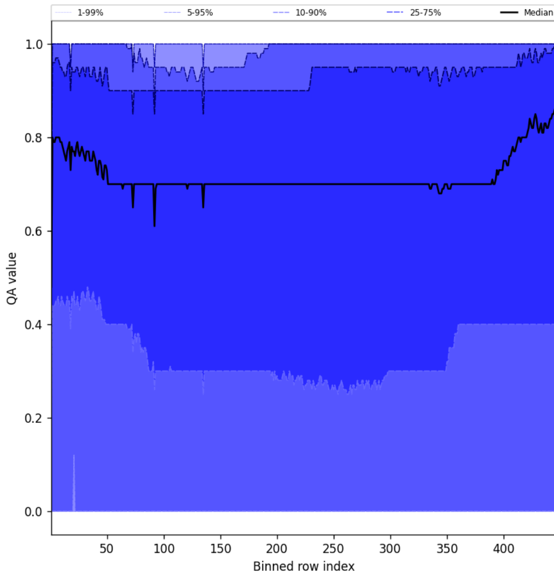
Figure 54: Along track statistics of “QA value” for 2025-11-21 to 2025-11-23
