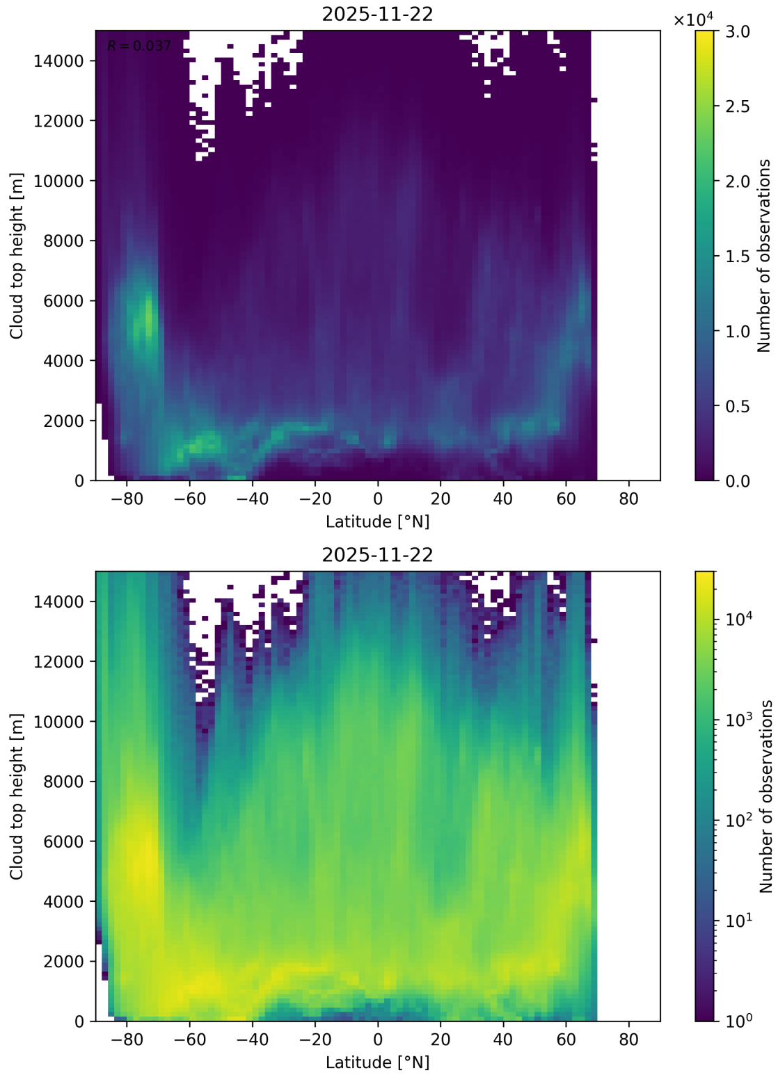
Figure 97: Scatter density plot of “Latitude” against “Cloud top height” for 2025-11-21 to 2025-11-23.
