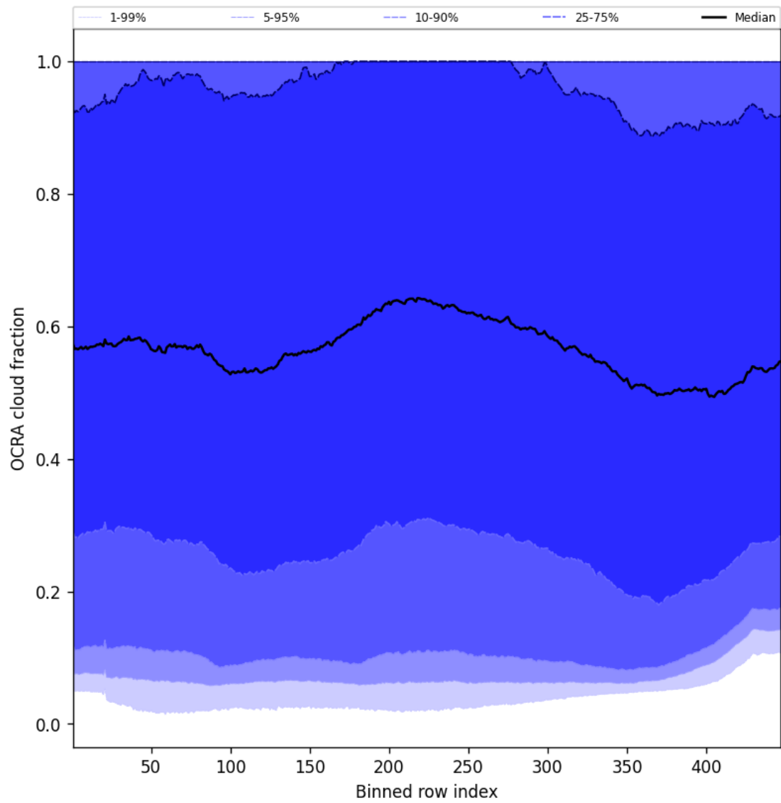
Figure 66: Along track statistics of “OCRA cloud fraction” for 2025-11-21 to 2025-11-23
