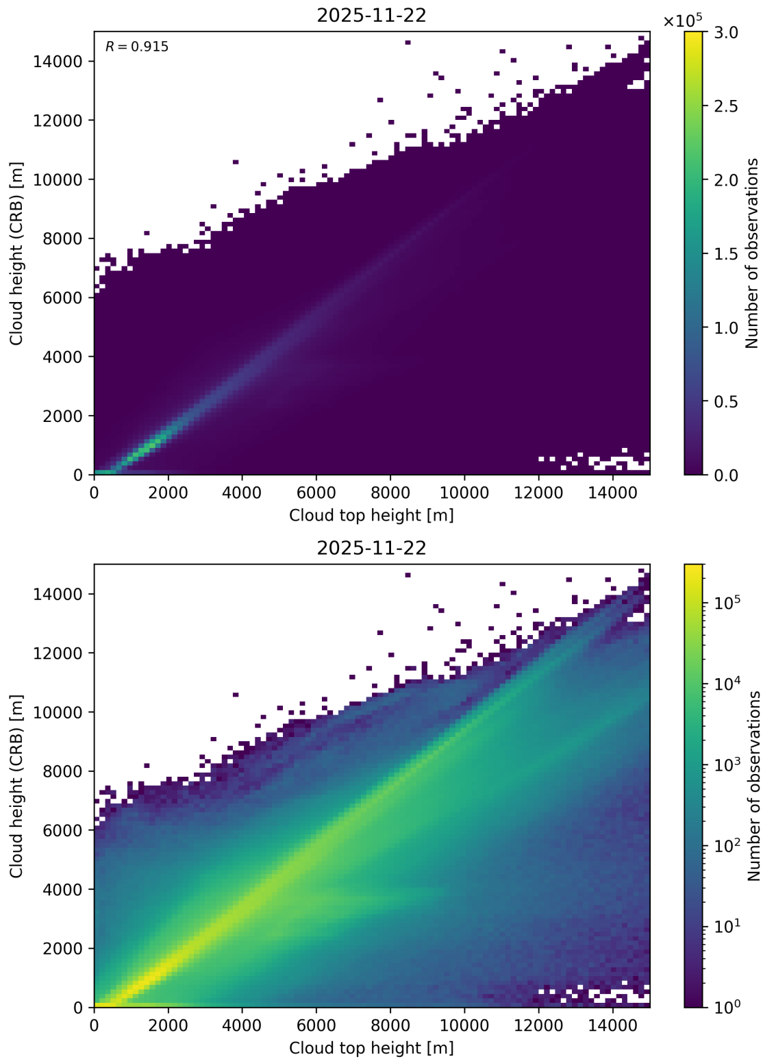
Figure 89: Scatter density plot of “Cloud top height” against “Cloud height (CRB)” for 2025-11-21 to 2025-11-23.
