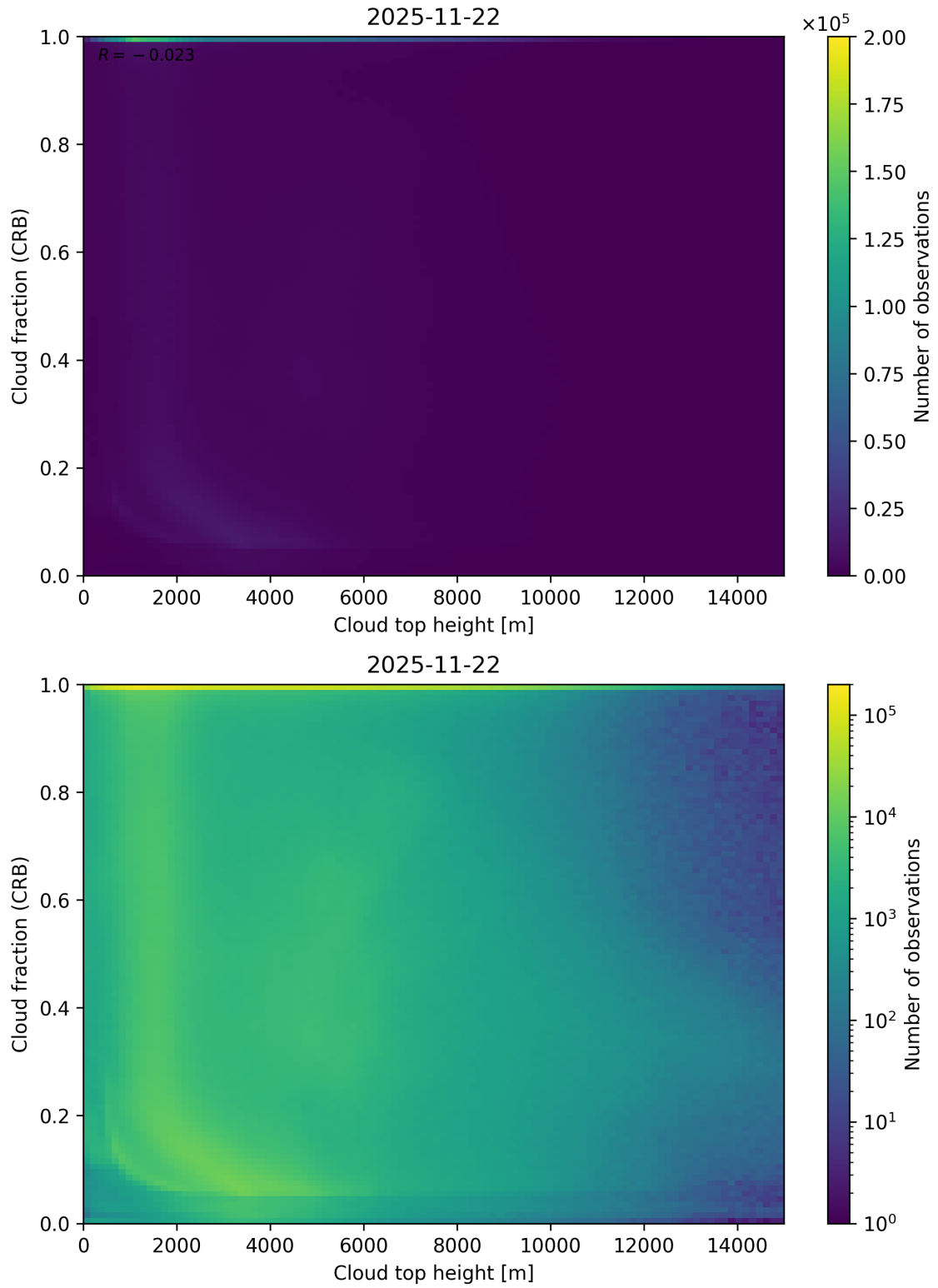
Figure 88: Scatter density plot of “Cloud top height” against “Cloud fraction (CRB)” for 2025-11-21 to 2025-11-23.
