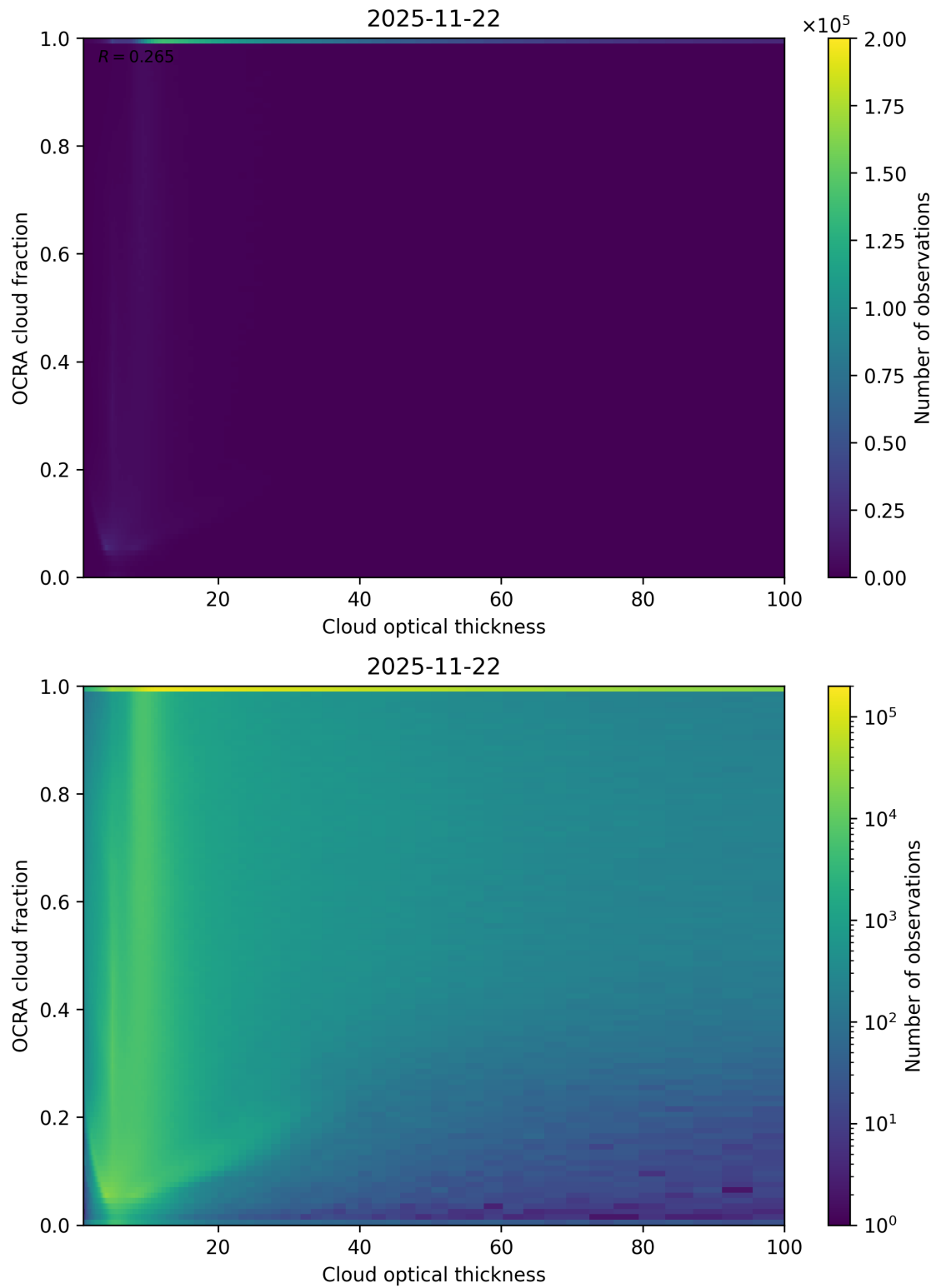
Figure 83: Scatter density plot of “Cloud optical thickness” against “OCRA cloud fraction” for 2025-11-21 to 2025-11-23.
