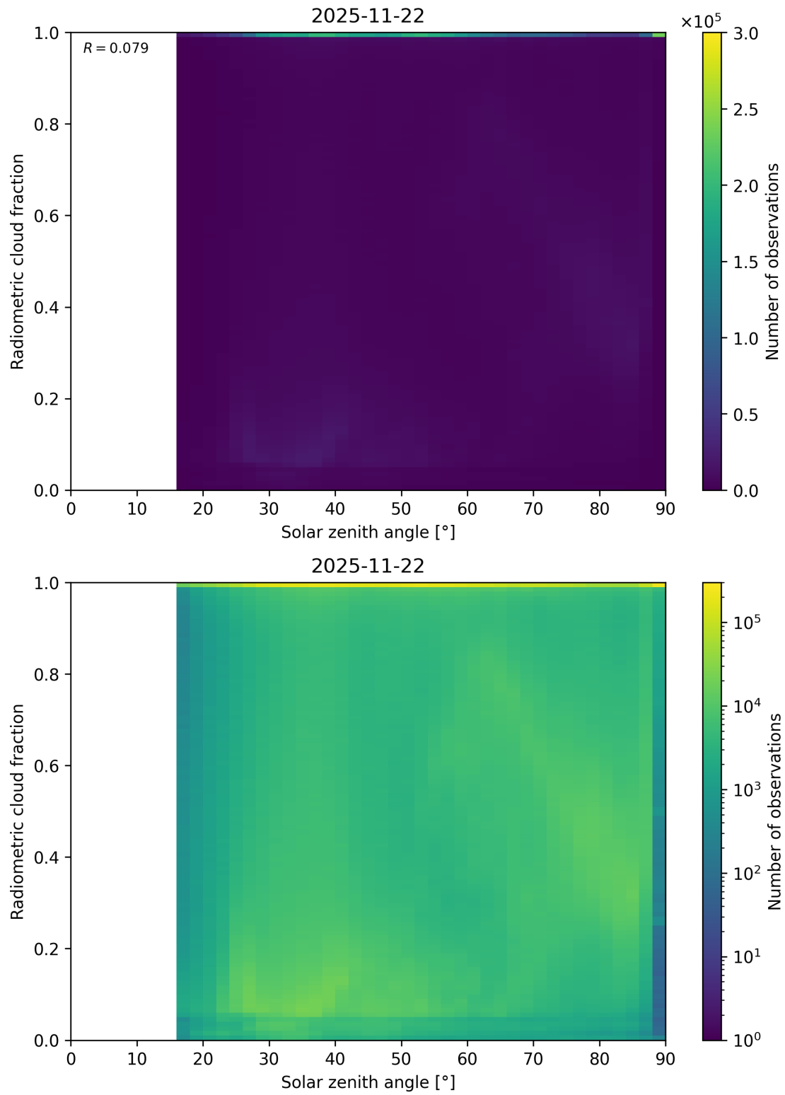
Figure 99: Scatter density plot of “Solar zenith angle” against “Radiometric cloud fraction” for 2025-11-21 to 2025-11-23.
