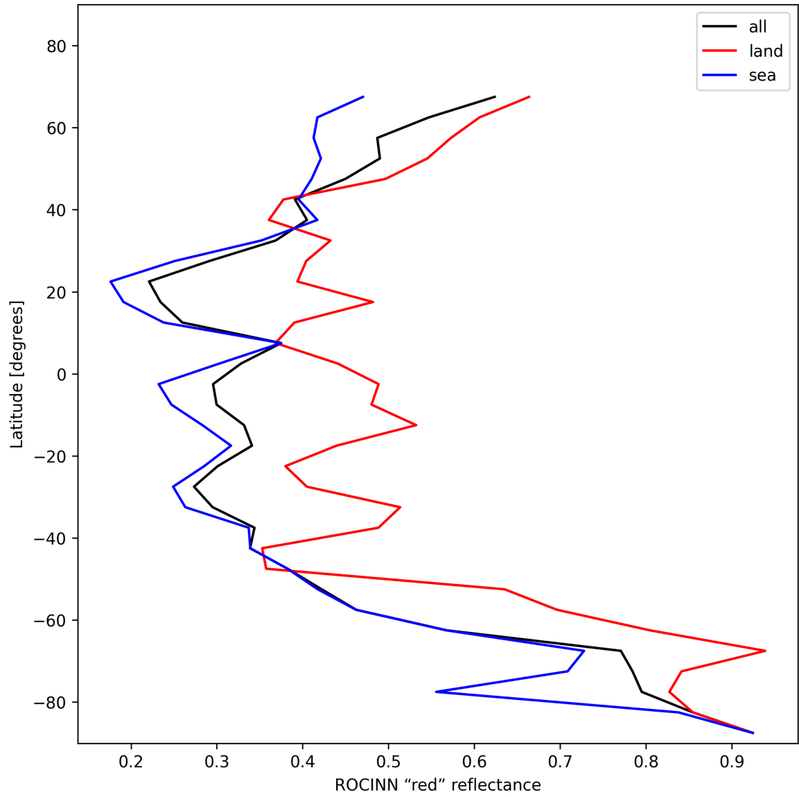
Figure 37: Zonal average of “ROCINN “red” reflectance” for 2025-11-21 to 2025-11-23.
