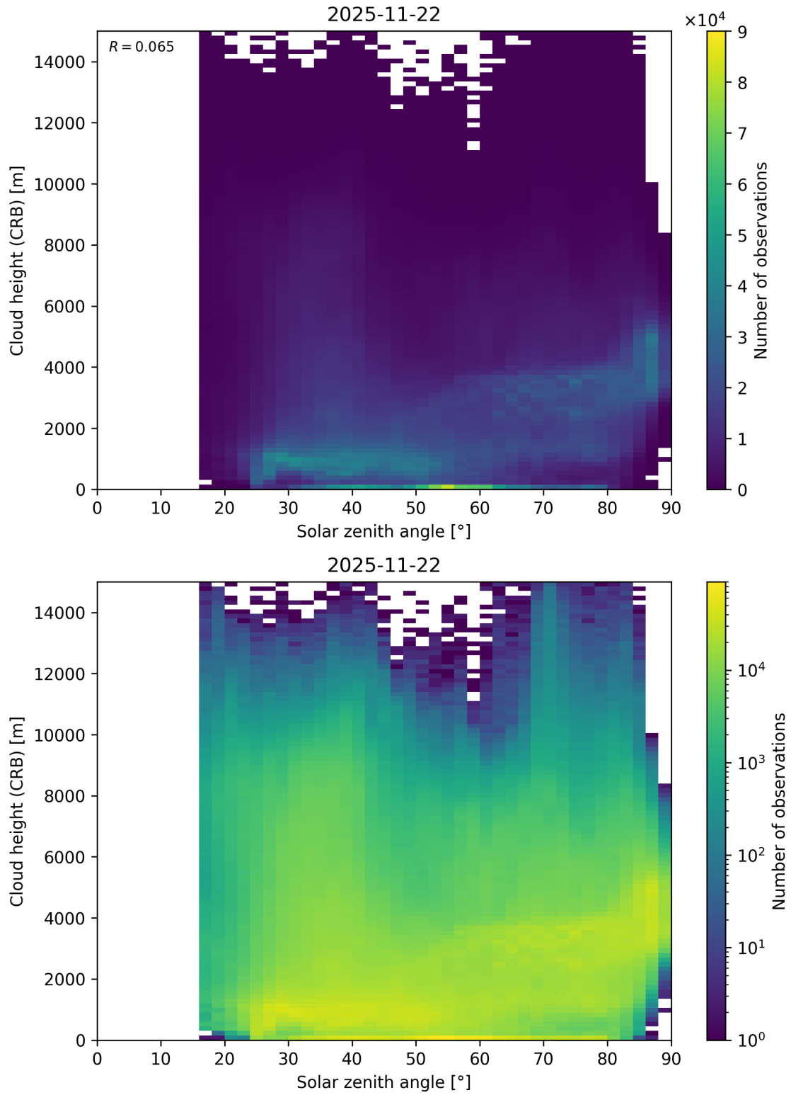
Figure 102: Scatter density plot of “Solar zenith angle” against “Cloud height (CRB)” for 2025-11-21 to 2025-11-23.
