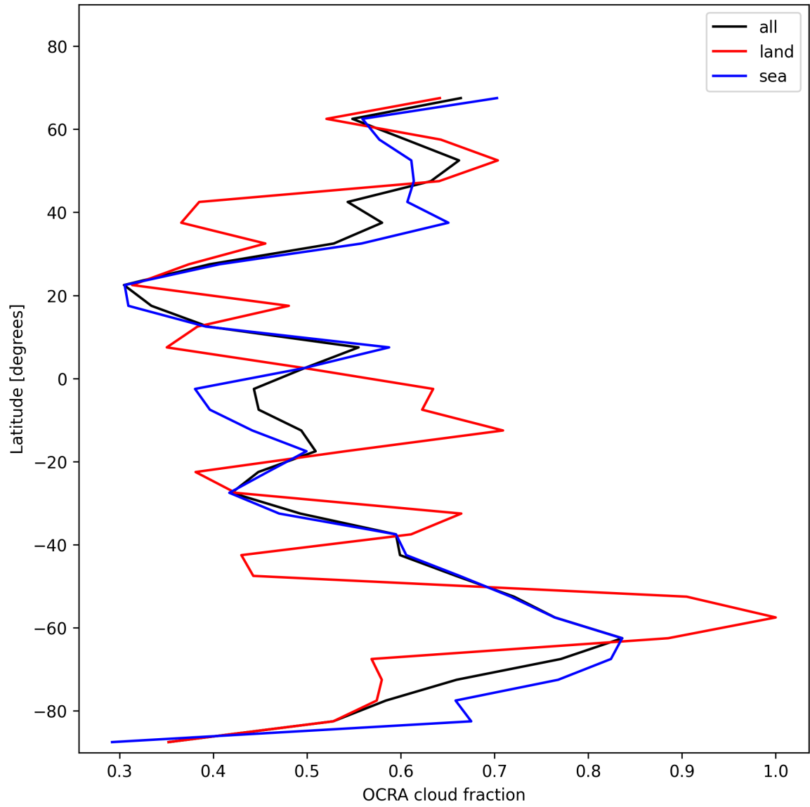
Figure 34: Zonal average of “OCRA cloud fraction” for 2025-11-21 to 2025-11-23.
