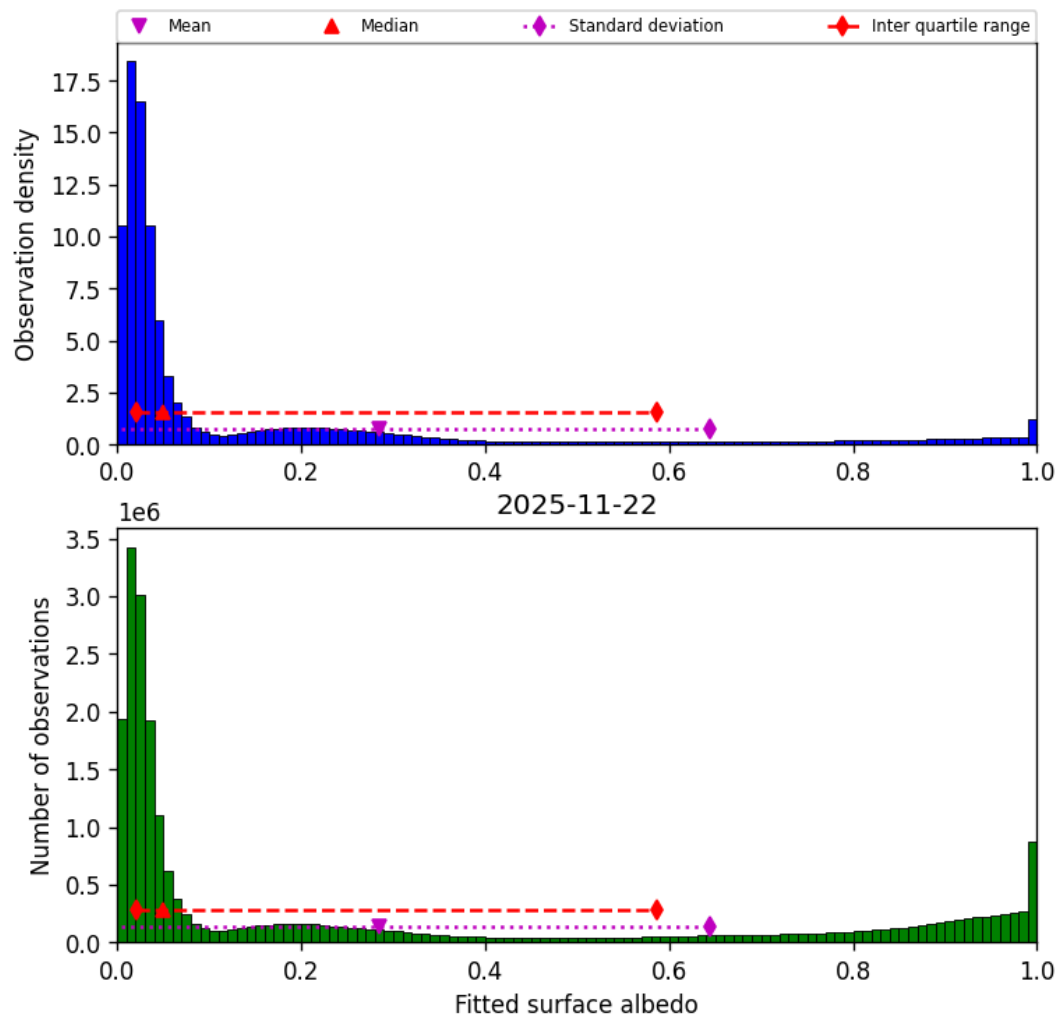
Figure 45: Histogram of “Fitted surface albedo” for 2025-11-21 to 2025-11-23
