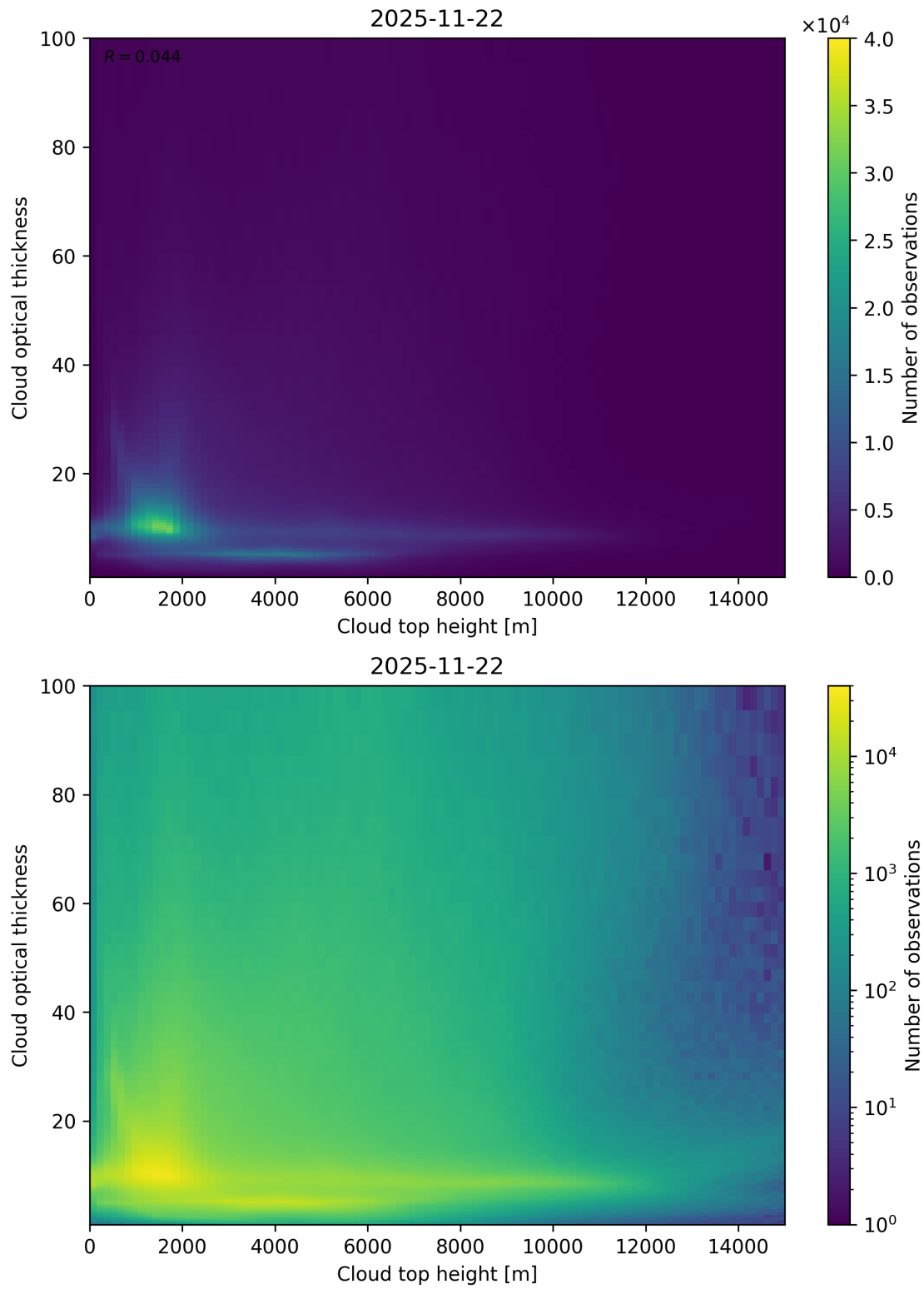
Figure 90: Scatter density plot of “Cloud top height” against “Cloud optical thickness” for 2025-11-21 to 2025-11-23.
