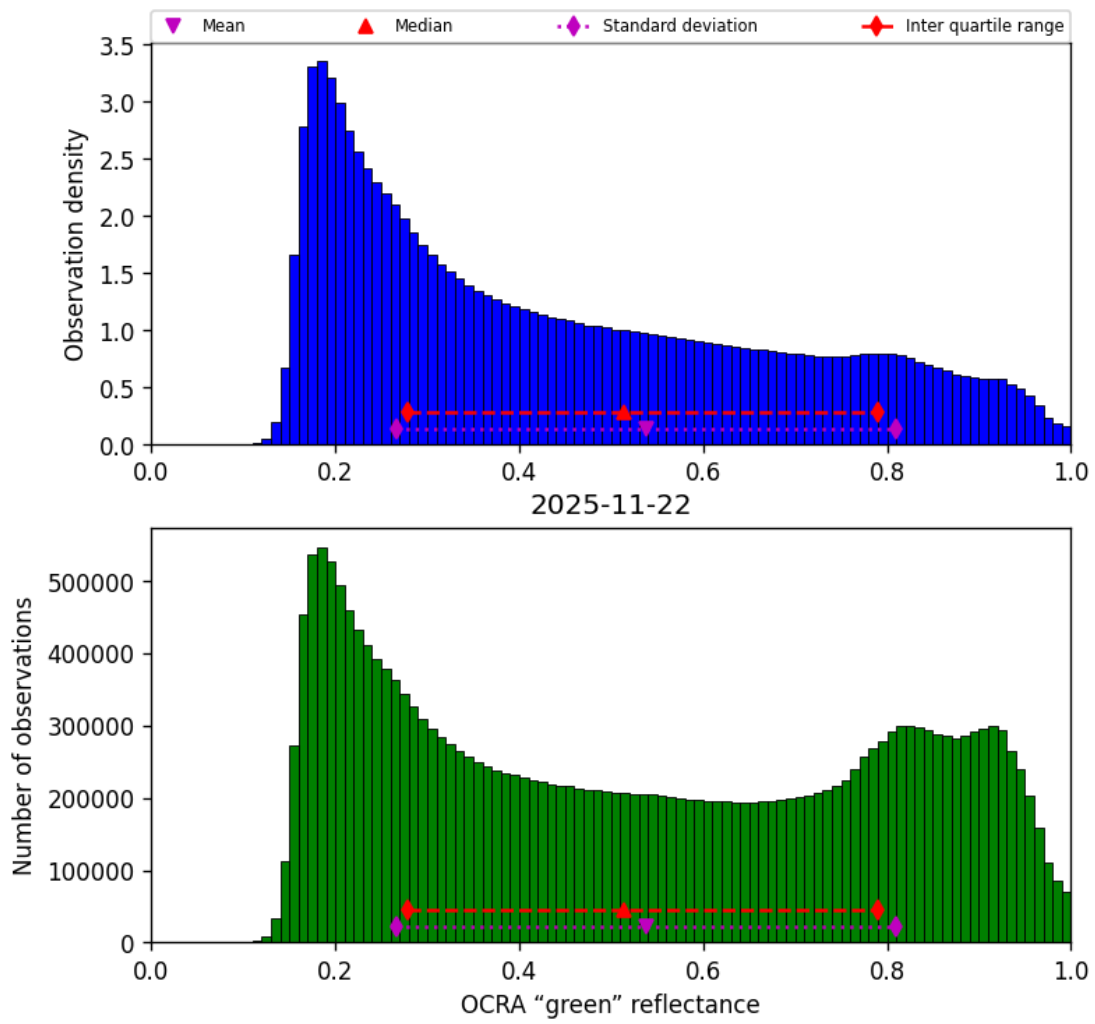
Figure 52: Histogram of “OCRA “green” reflectance” for 2025-11-21 to 2025-11-23
