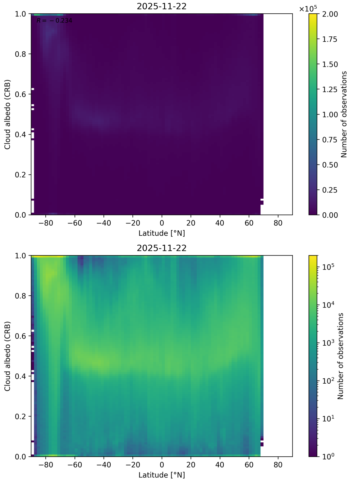
Figure 91: Scatter density plot of “Latitude” against “Cloud albedo (CRB)” for 2025-11-21 to 2025-11-23.
