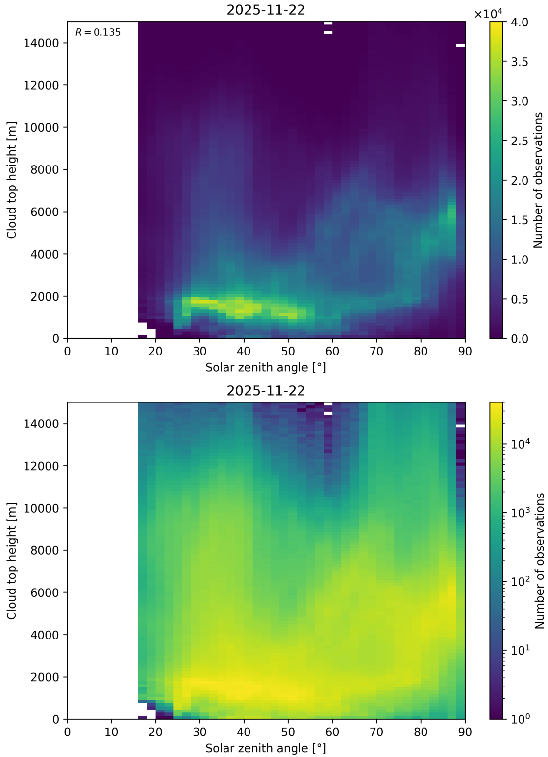
Figure 104: Scatter density plot of “Solar zenith angle” against “Cloud top height” for 2025-11-21 to 2025-11-23.
