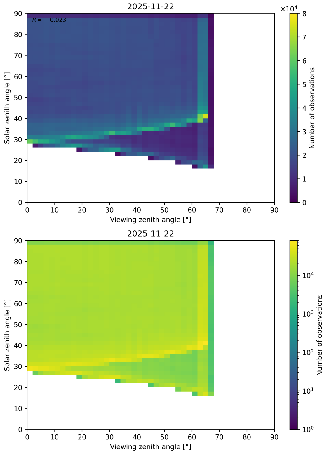
Figure 114: Scatter density plot of “Viewing zenith angle” against “Solar zenith angle” for 2025-11-21 to 2025-11-23.
