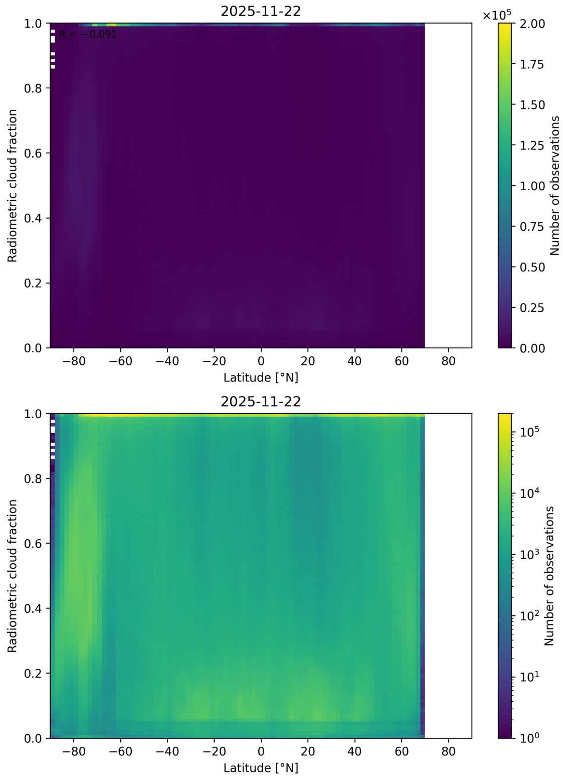
Figure 92: Scatter density plot of “Latitude” against “Radiometric cloud fraction” for 2025-11-21 to 2025-11-23.
