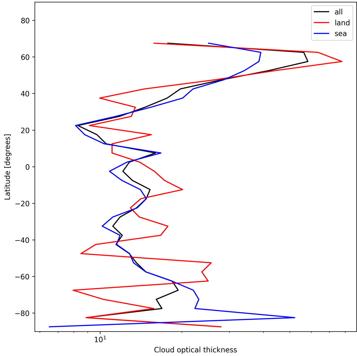
Figure 25: Zonal average of “Cloud optical thickness” for 2025-11-21 to 2025-11-23.
