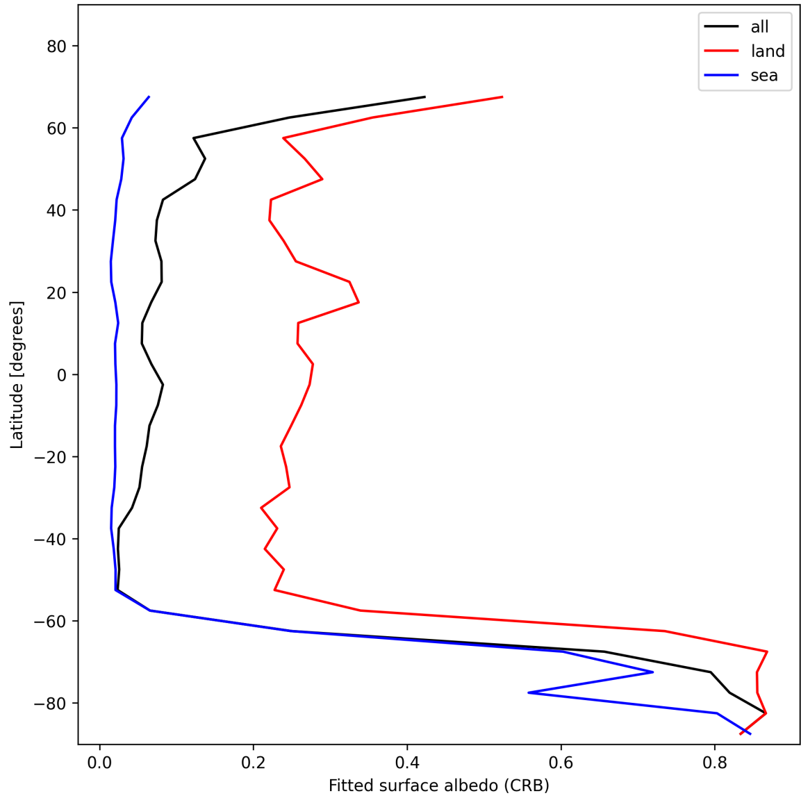
Figure 30: Zonal average of “Fitted surface albedo (CRB)” for 2025-11-21 to 2025-11-23.
