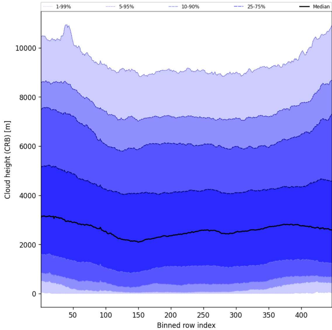
Figure 59: Along track statistics of “Cloud height (CRB)” for 2025-11-21 to 2025-11-23
