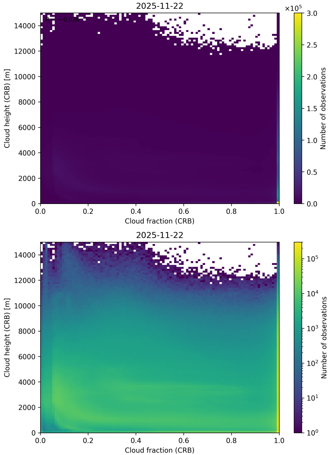
Figure 79: Scatter density plot of “Cloud fraction (CRB)” against “Cloud height (CRB)” for 2025-11-21 to 2025-11-23.
