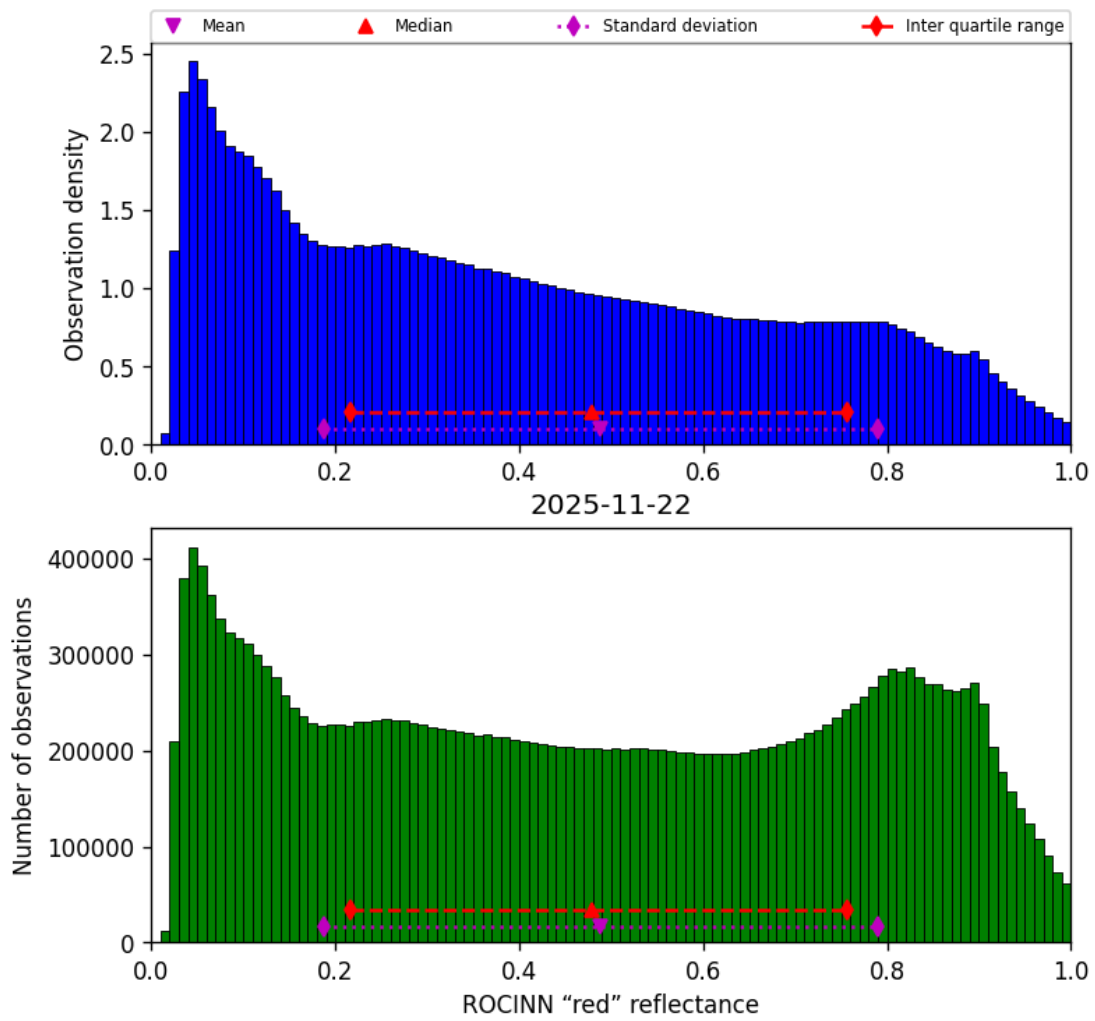
Figure 53: Histogram of “ROCINN “red” reflectance” for 2025-11-21 to 2025-11-23
