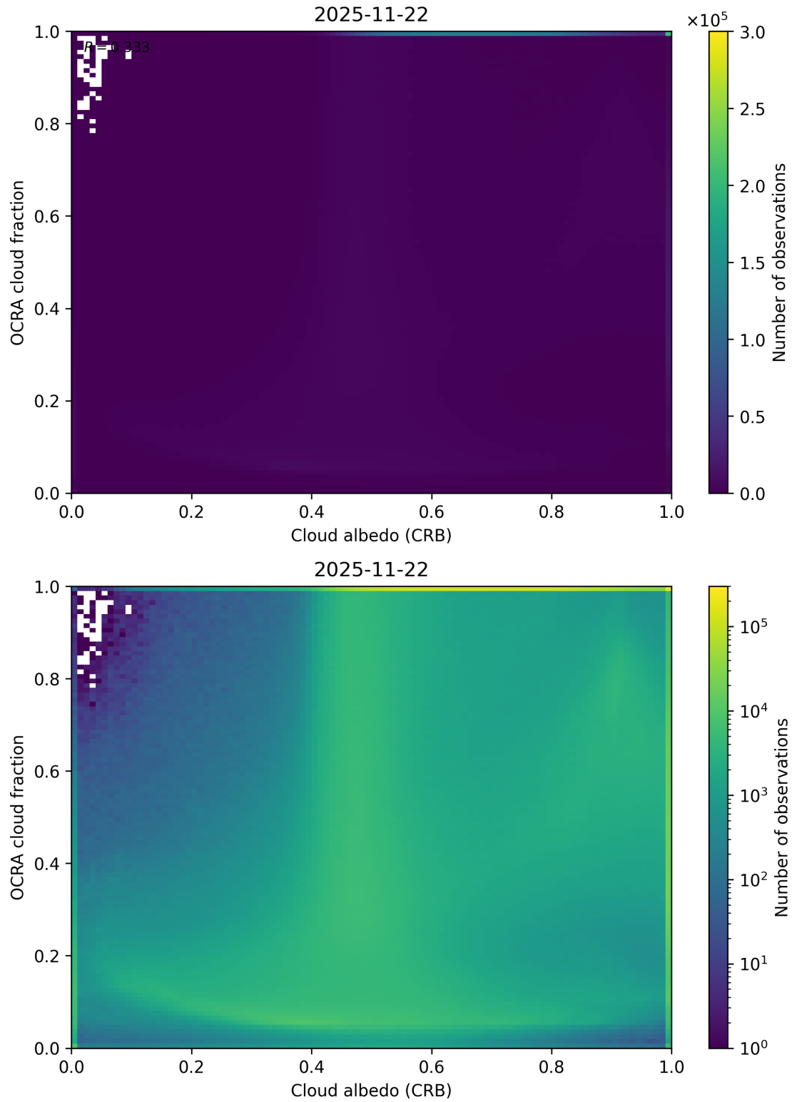
Figure 70: Scatter density plot of “Cloud albedo (CRB)” against “OCRA cloud fraction” for 2025-11-21 to 2025-11-23.
