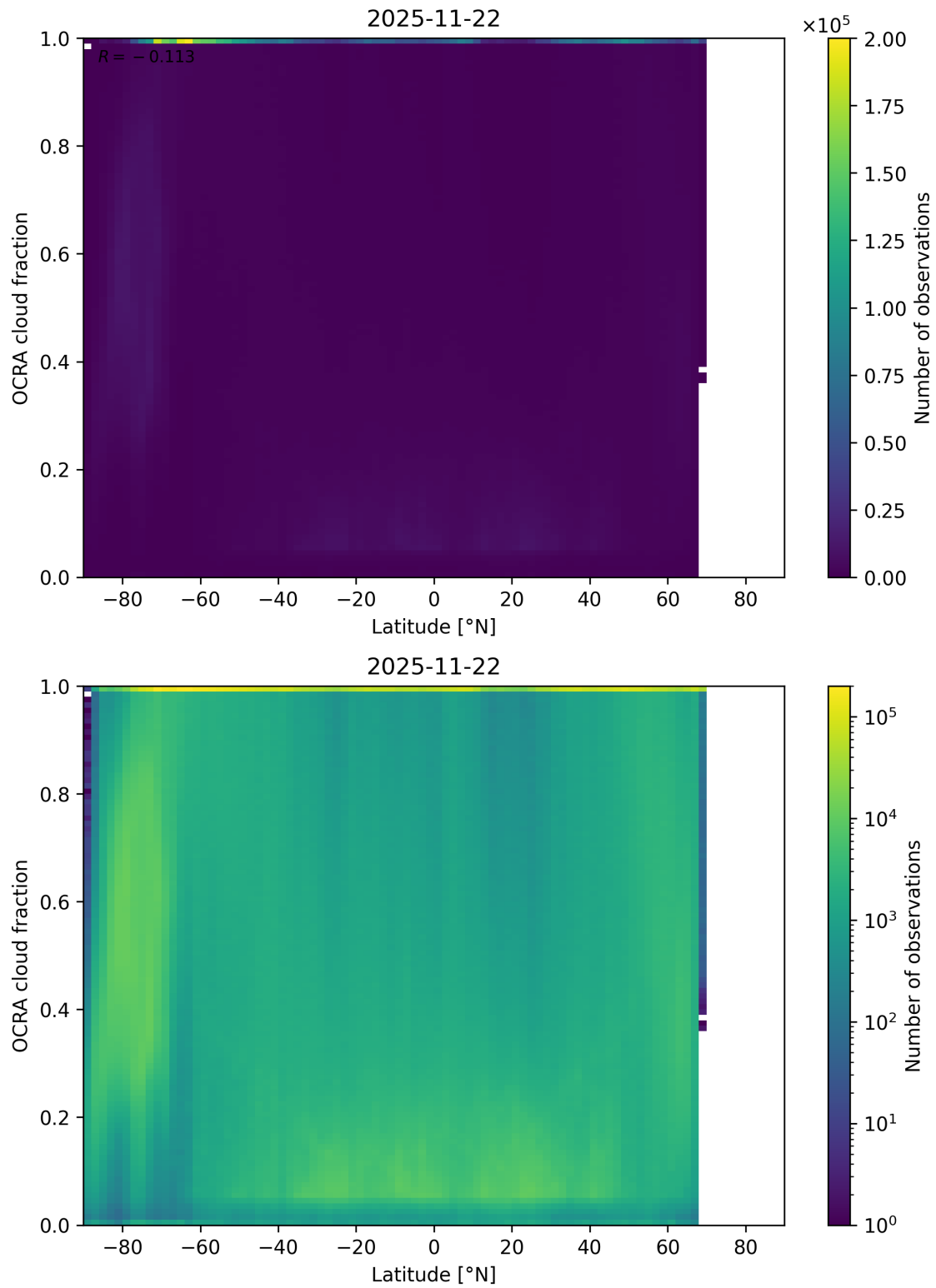
Figure 93: Scatter density plot of “Latitude” against “OCRA cloud fraction” for 2025-11-21 to 2025-11-23.
