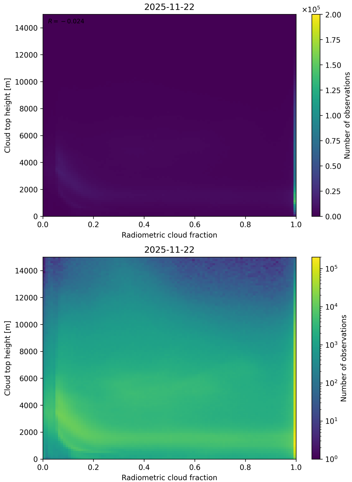
Figure 76: Scatter density plot of “Radiometric cloud fraction” against “Cloud top height” for 2025-11-21 to 2025-11-23.
