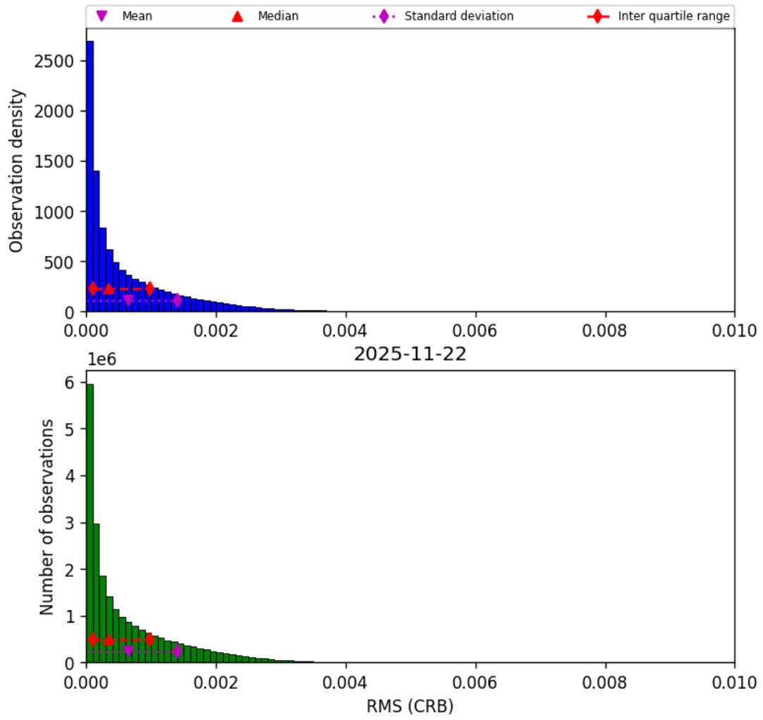
Figure 48: Histogram of “RMS (CRB)” for 2025-11-21 to 2025-11-23
