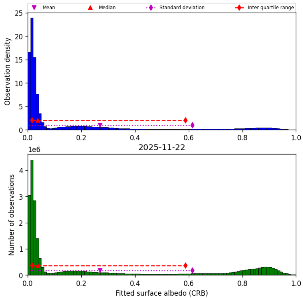
Figure 46: Histogram of “Fitted surface albedo (CRB)” for 2025-11-21 to 2025-11-23
