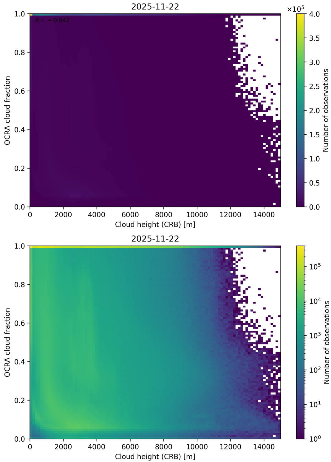
Figure 81: Scatter density plot of “Cloud height (CRB)” against “OCRA cloud fraction” for 2025-11-21 to 2025-11-23.
