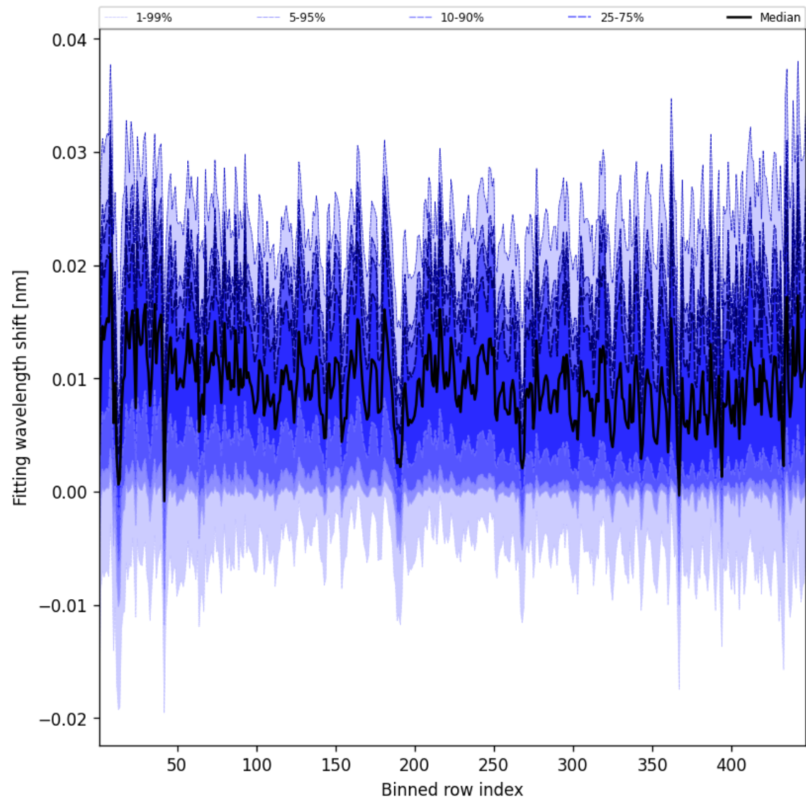
Figure 65: Along track statistics of “Fitting wavelength shift” for 2025-11-21 to 2025-11-23
