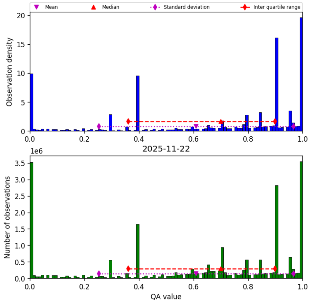
Figure 38: Histogram of “QA value” for 2025-11-21 to 2025-11-23
