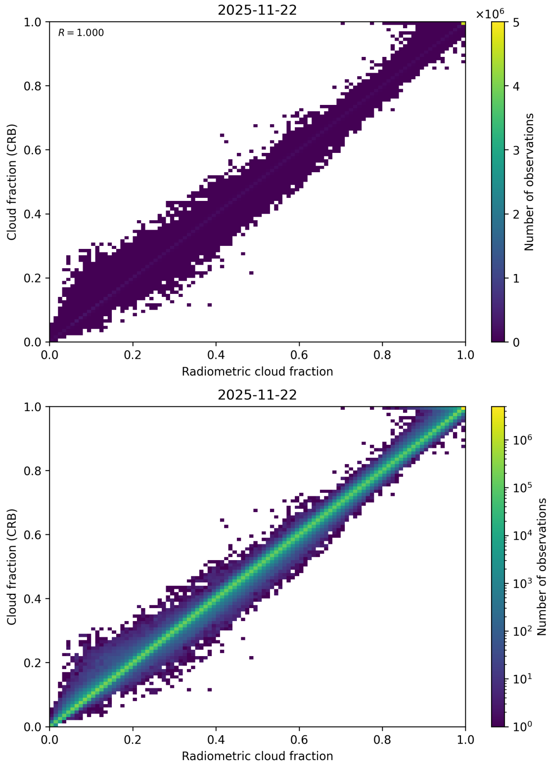
Figure 73: Scatter density plot of “Radiometric cloud fraction” against “Cloud fraction (CRB)” for 2025-11-21 to 2025-11-23.
