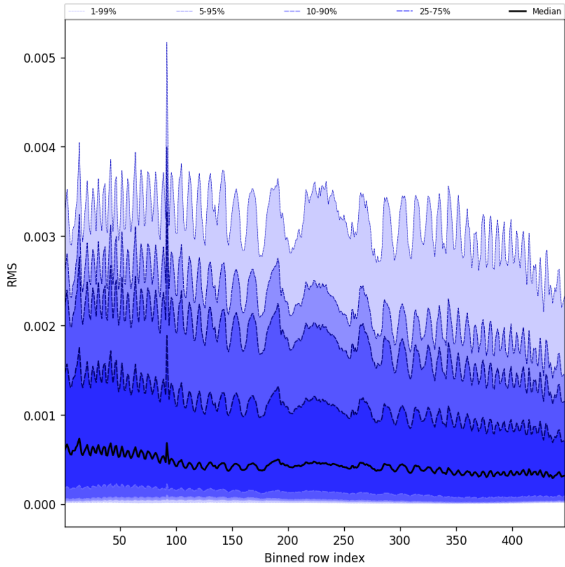
Figure 63: Along track statistics of “RMS” for 2025-11-21 to 2025-11-23
