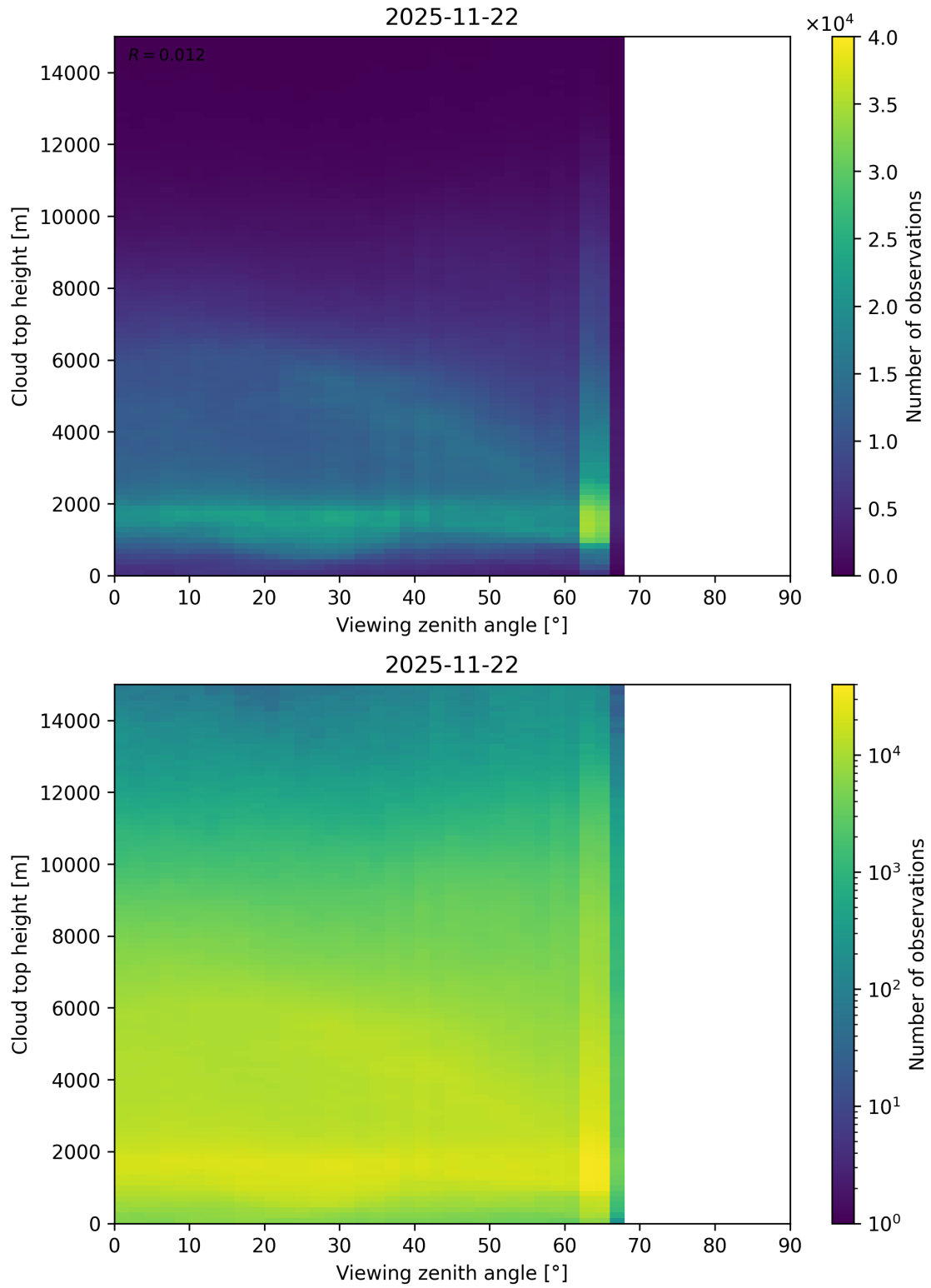
Figure 112: Scatter density plot of “Viewing zenith angle” against “Cloud top height” for 2025-11-21 to 2025-11-23.
