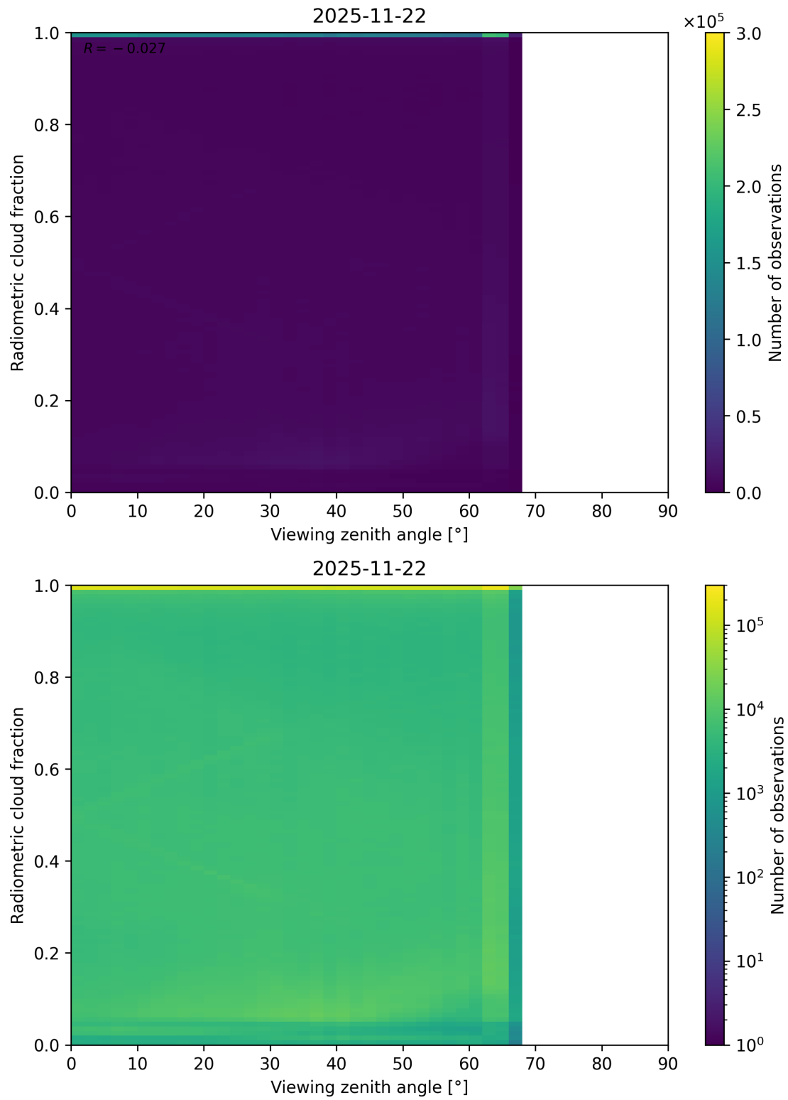
Figure 107: Scatter density plot of “Viewing zenith angle” against “Radiometric cloud fraction” for 2025-11-21 to 2025-11-23.
