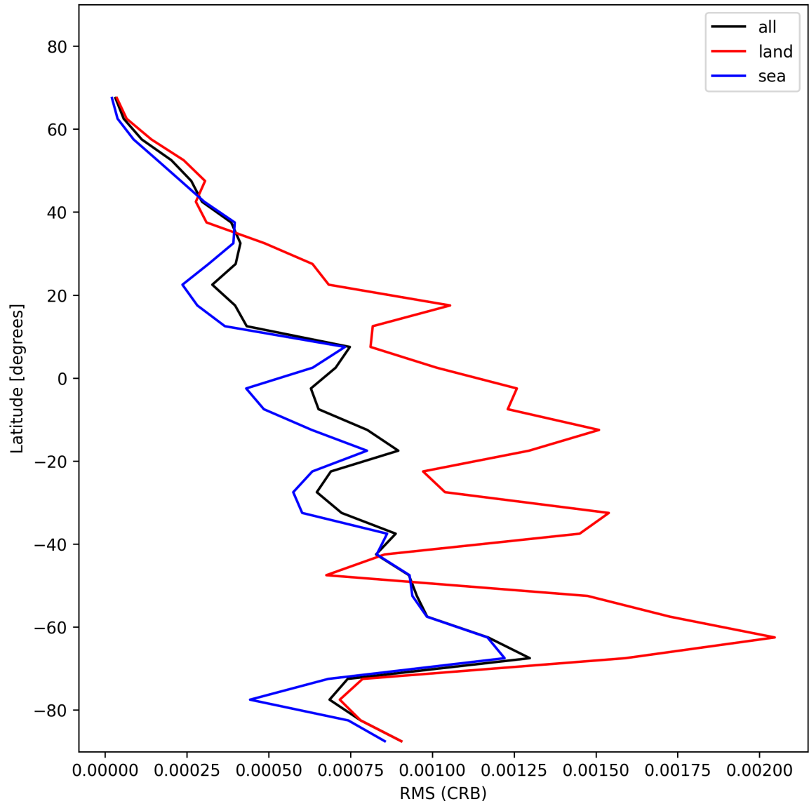
Figure 32: Zonal average of “RMS (CRB)” for 2025-11-21 to 2025-11-23.
