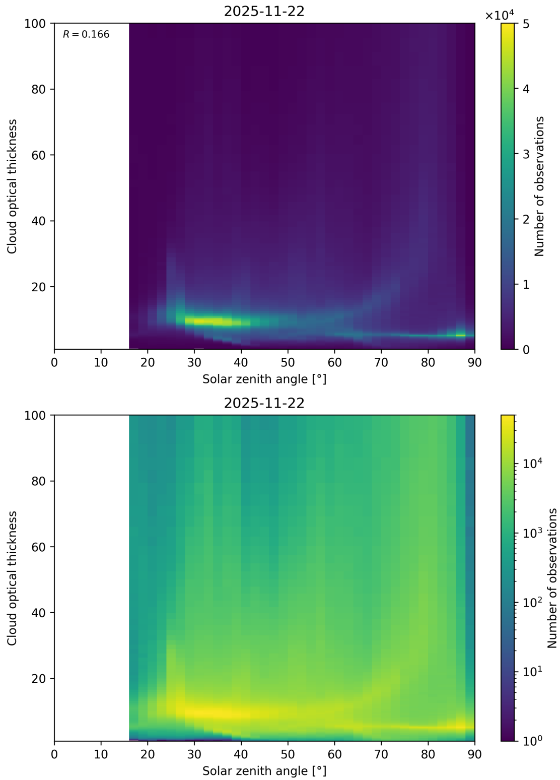
Figure 103: Scatter density plot of “Solar zenith angle” against “Cloud optical thickness” for 2025-11-21 to 2025-11-23.
