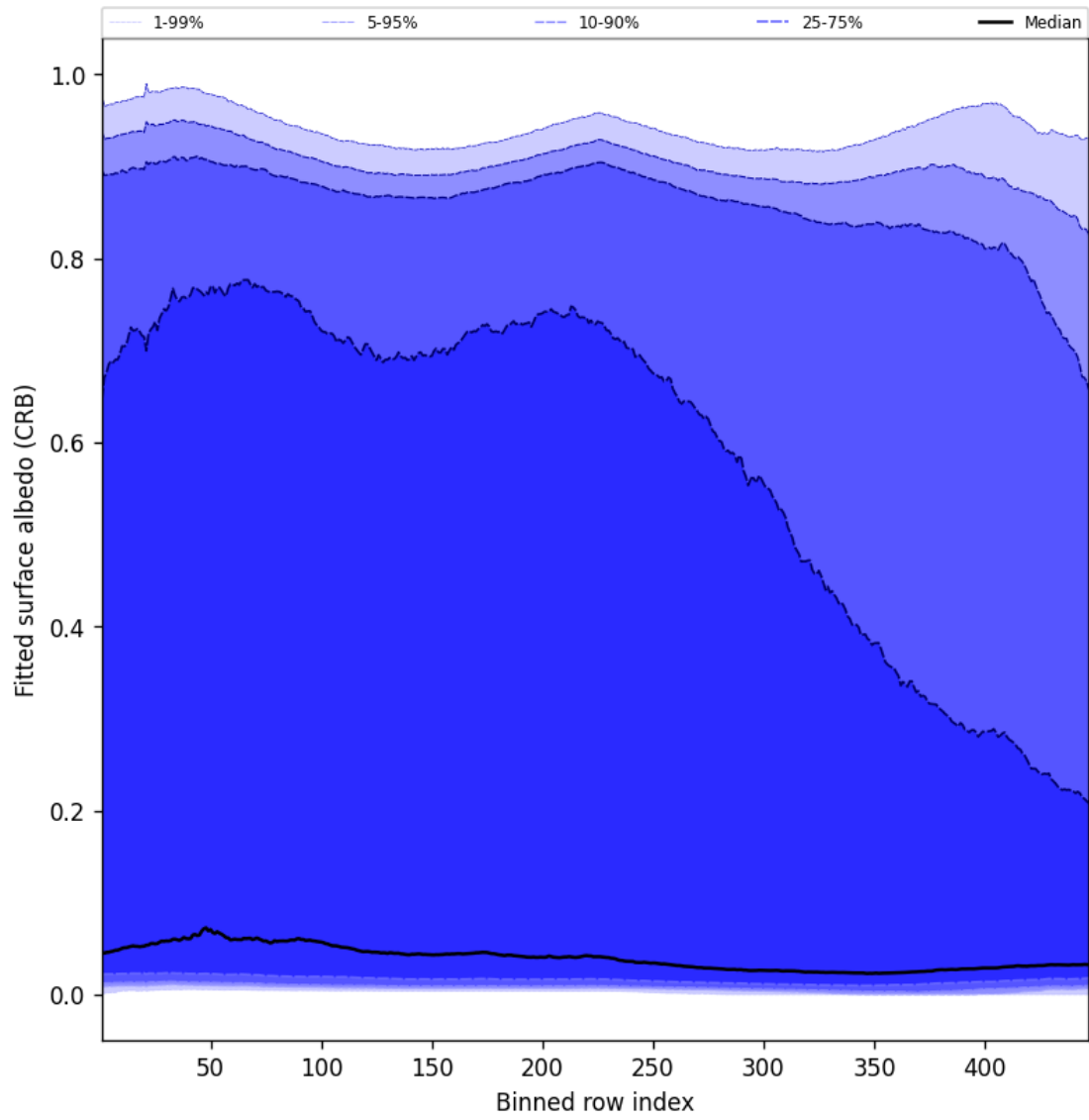
Figure 62: Along track statistics of “Fitted surface albedo (CRB)” for 2025-11-21 to 2025-11-23
