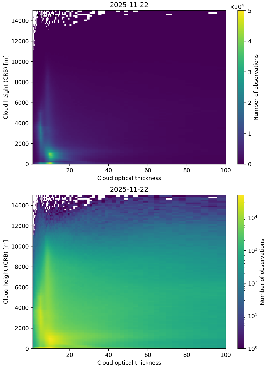
Figure 85: Scatter density plot of “Cloud optical thickness” against “Cloud height (CRB)” for 2025-11-21 to 2025-11-23.
