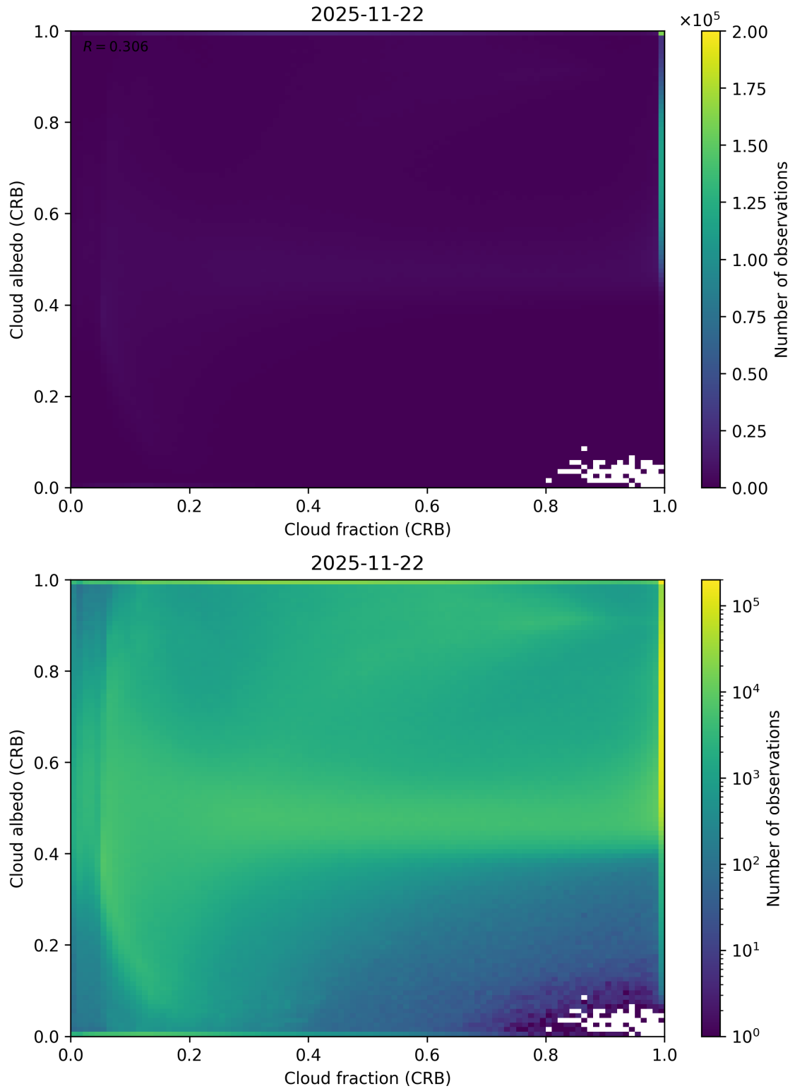
Figure 77: Scatter density plot of “Cloud fraction (CRB)” against “Cloud albedo (CRB)” for 2025-11-21 to 2025-11-23.
