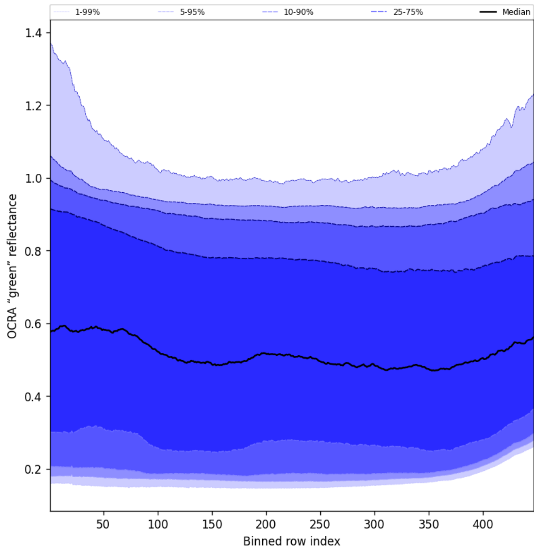
Figure 68: Along track statistics of “OCRA “green” reflectance” for 2025-11-21 to 2025-11-23
