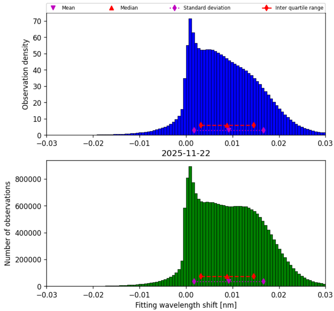
Figure 49: Histogram of “Fitting wavelength shift” for 2025-11-21 to 2025-11-23
