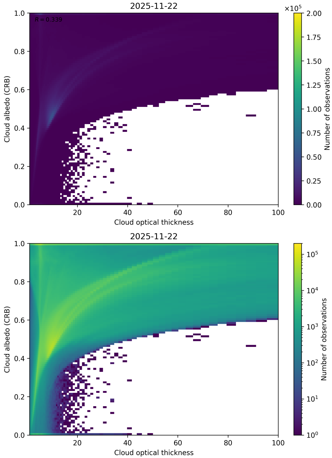
Figure 82: Scatter density plot of “Cloud optical thickness” against “Cloud albedo (CRB)” for 2025-11-21 to 2025-11-23.
