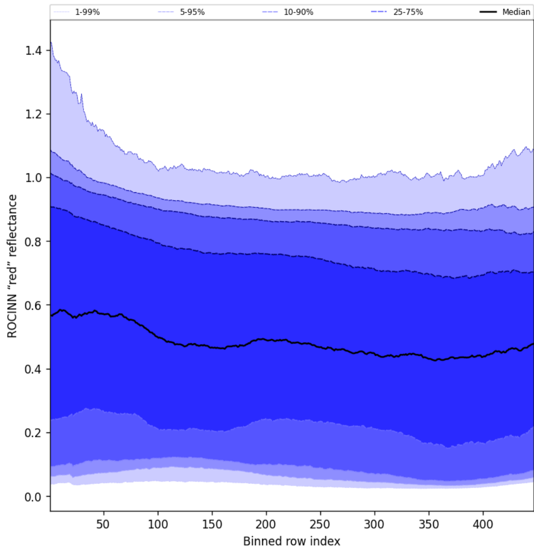
Figure 69: Along track statistics of “ROCINN “red” reflectance” for 2025-11-21 to 2025-11-23
