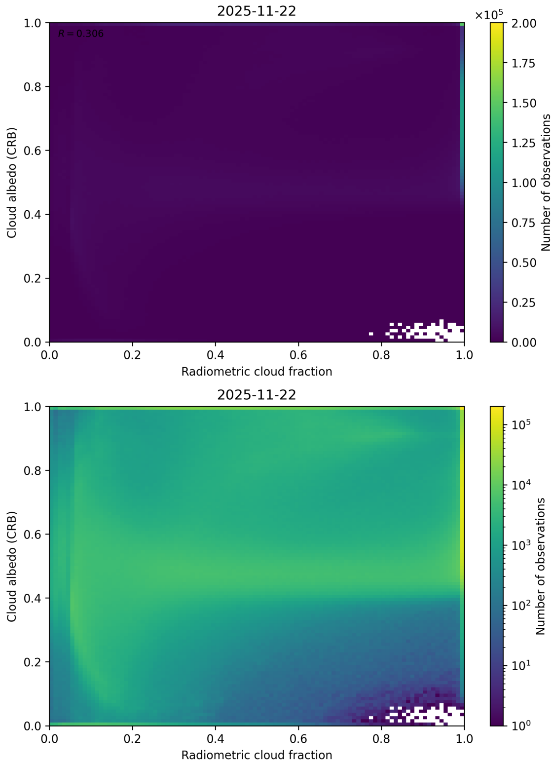
Figure 71: Scatter density plot of “Radiometric cloud fraction” against “Cloud albedo (CRB)” for 2025-11-21 to 2025-11-23.
