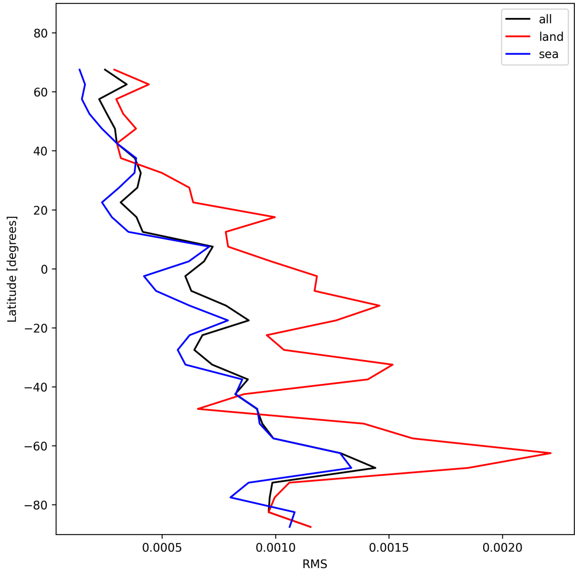
Figure 31: Zonal average of “RMS” for 2025-11-21 to 2025-11-23.
