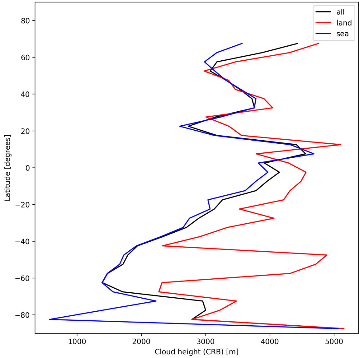
Figure 27: Zonal average of “Cloud height (CRB)” for 2025-11-21 to 2025-11-23.
