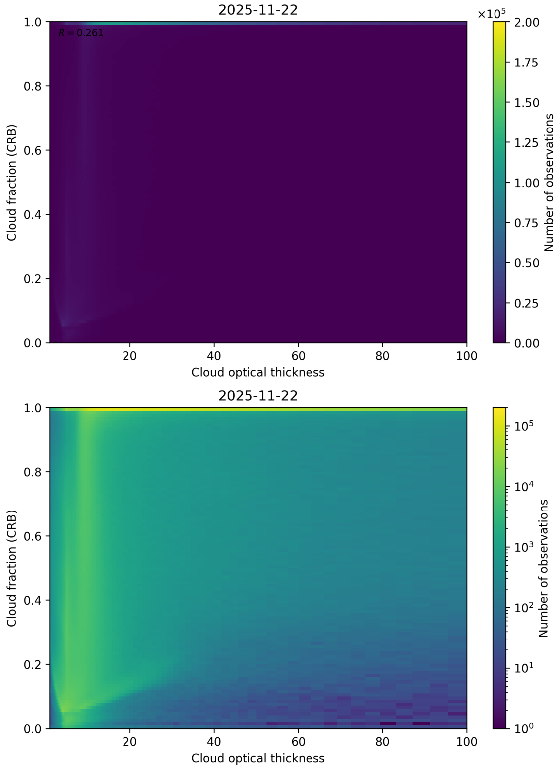
Figure 84: Scatter density plot of “Cloud optical thickness” against “Cloud fraction (CRB)” for 2025-11-21 to 2025-11-23.
