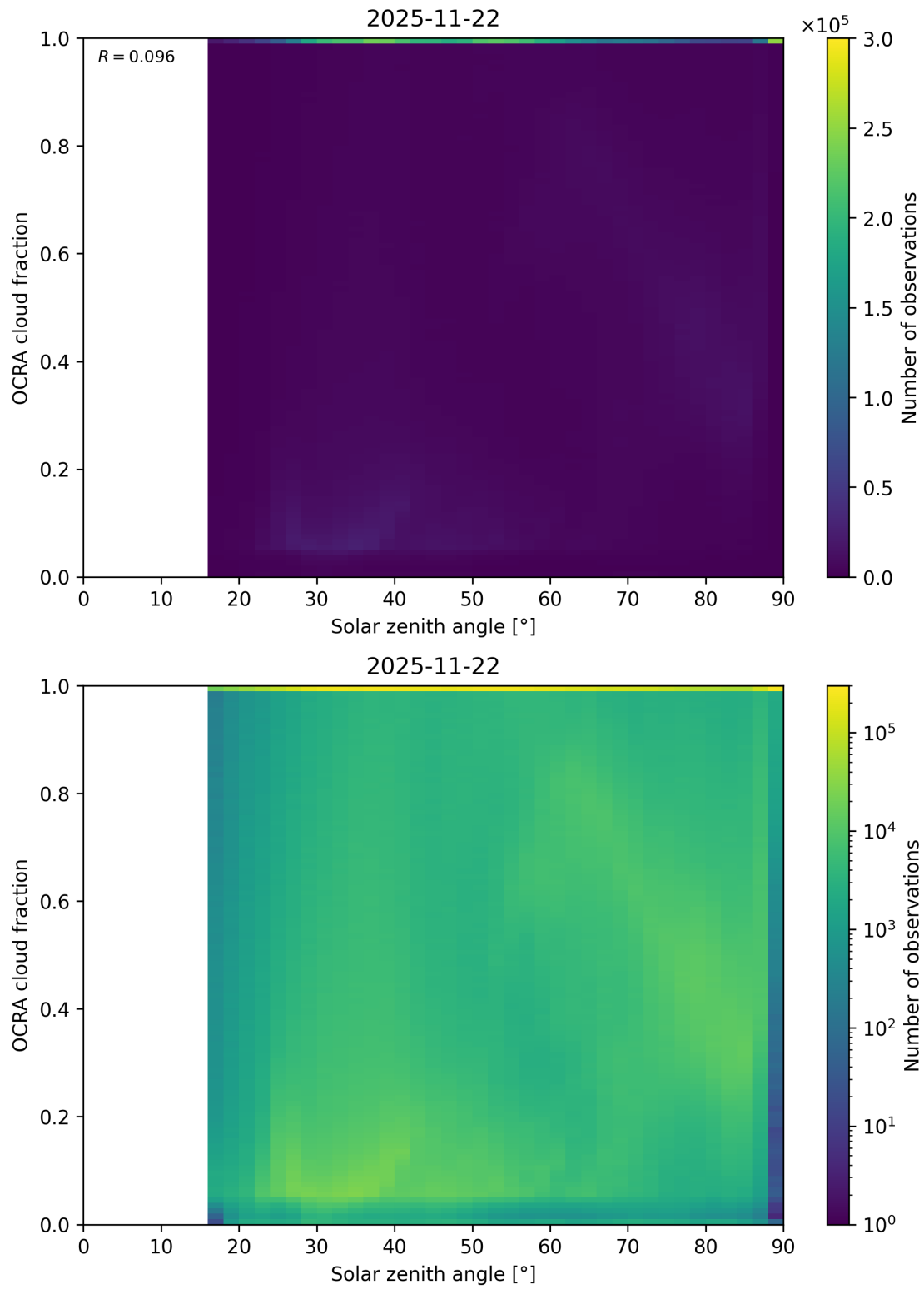
Figure 100: Scatter density plot of “Solar zenith angle” against “OCRA cloud fraction” for 2025-11-21 to 2025-11-23.
