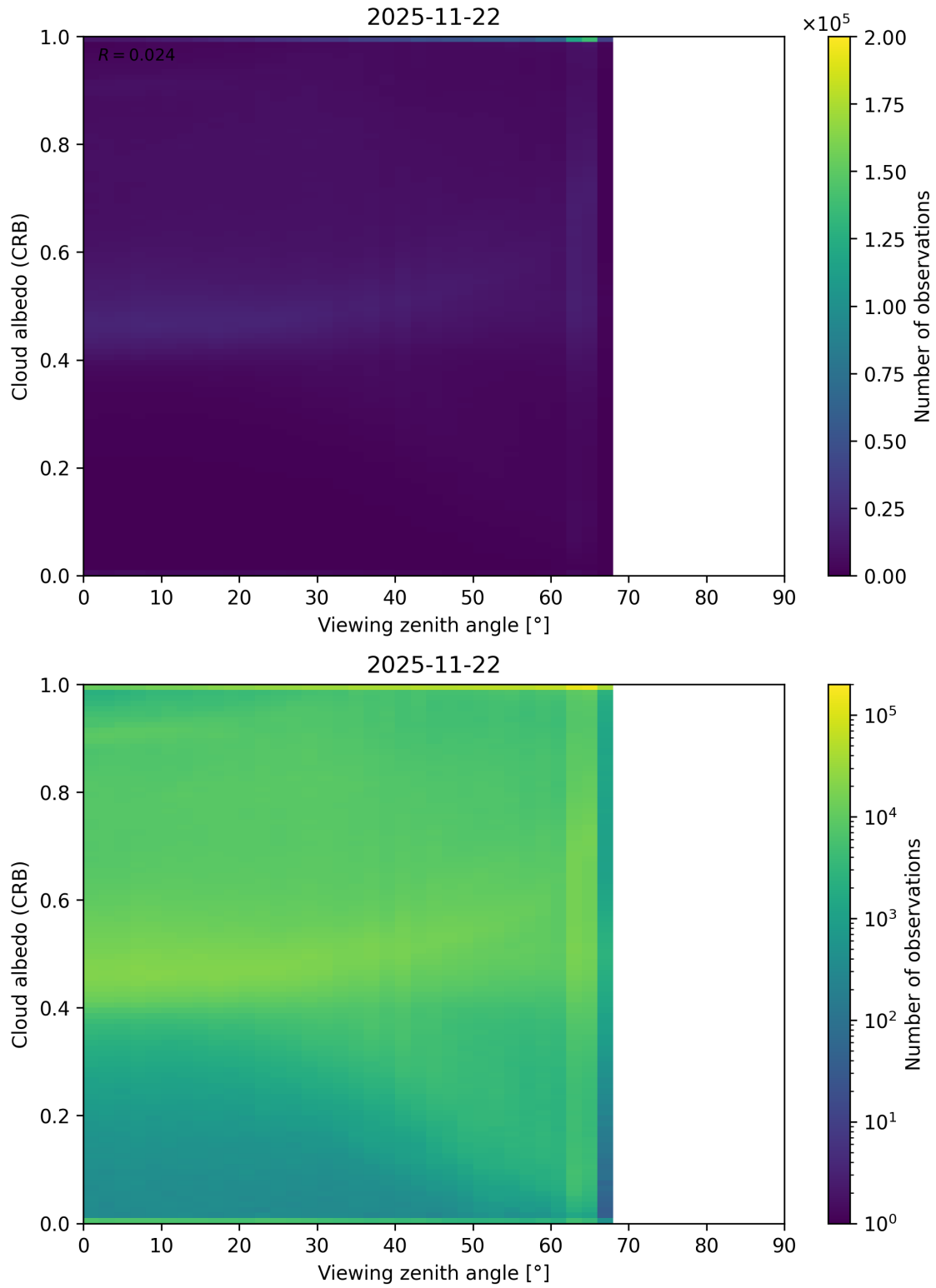
Figure 106: Scatter density plot of “Viewing zenith angle” against “Cloud albedo (CRB)” for 2025-11-21 to 2025-11-23.
