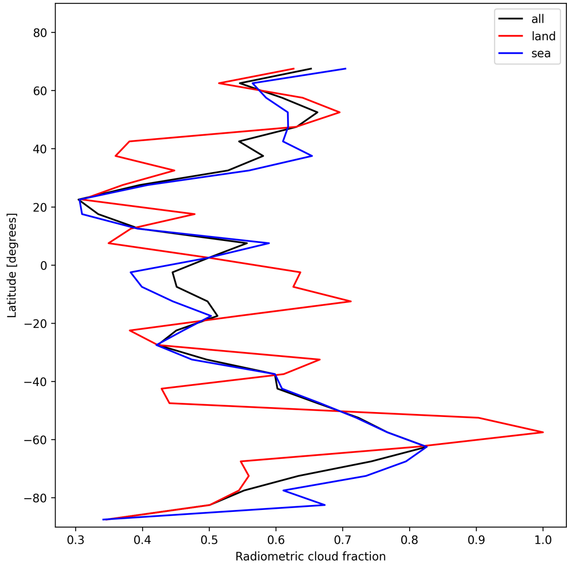
Figure 23: Zonal average of “Radiometric cloud fraction” for 2025-11-21 to 2025-11-23.
