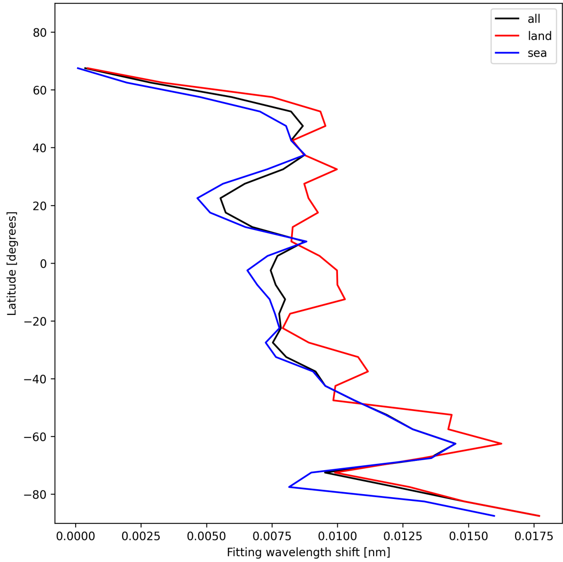
Figure 33: Zonal average of “Fitting wavelength shift” for 2025-11-21 to 2025-11-23.
