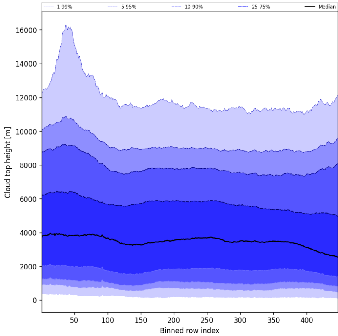
Figure 56: Along track statistics of “Cloud top height” for 2025-11-21 to 2025-11-23
