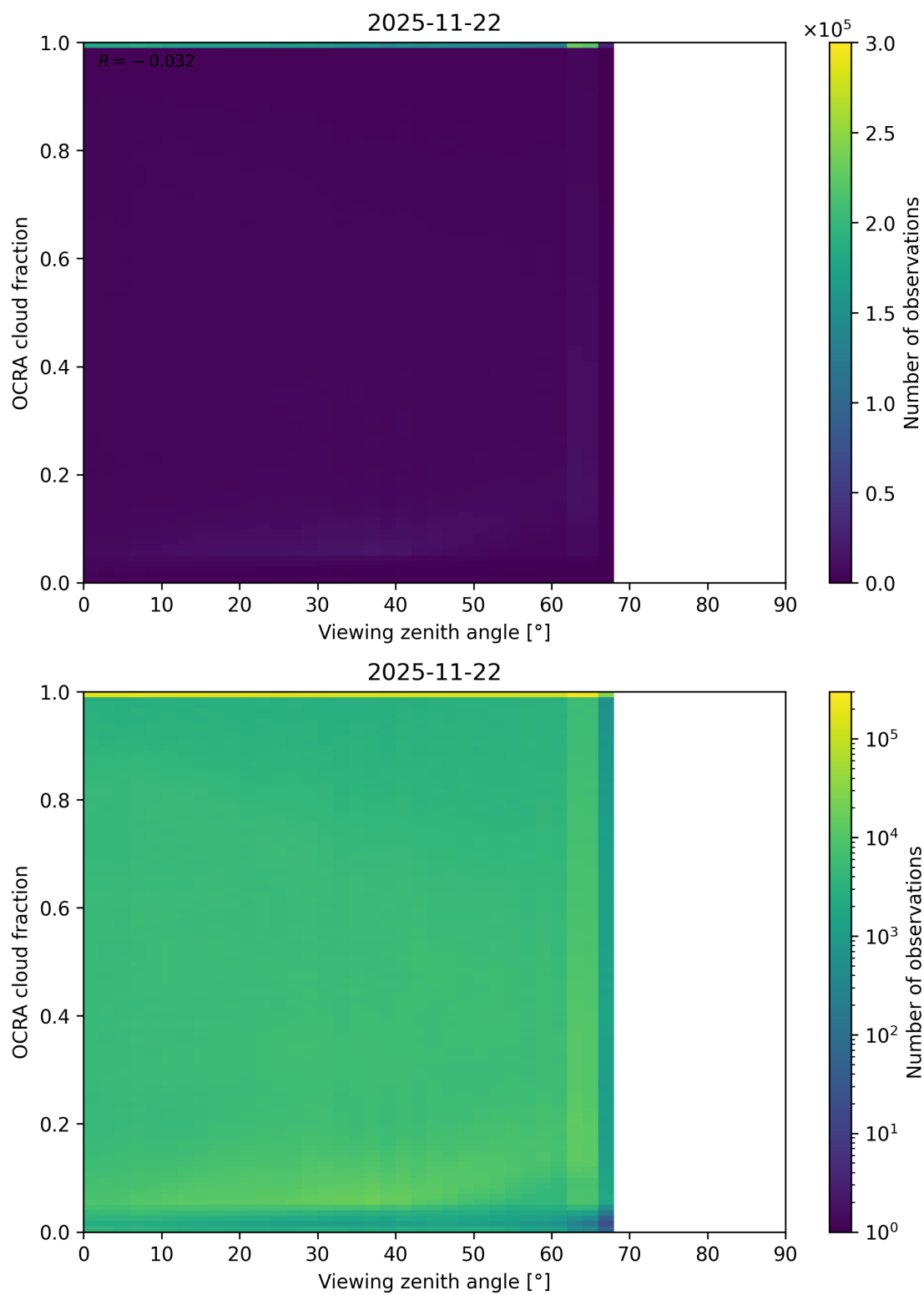
Figure 108: Scatter density plot of “Viewing zenith angle” against “OCRA cloud fraction” for 2025-11-21 to 2025-11-23.
