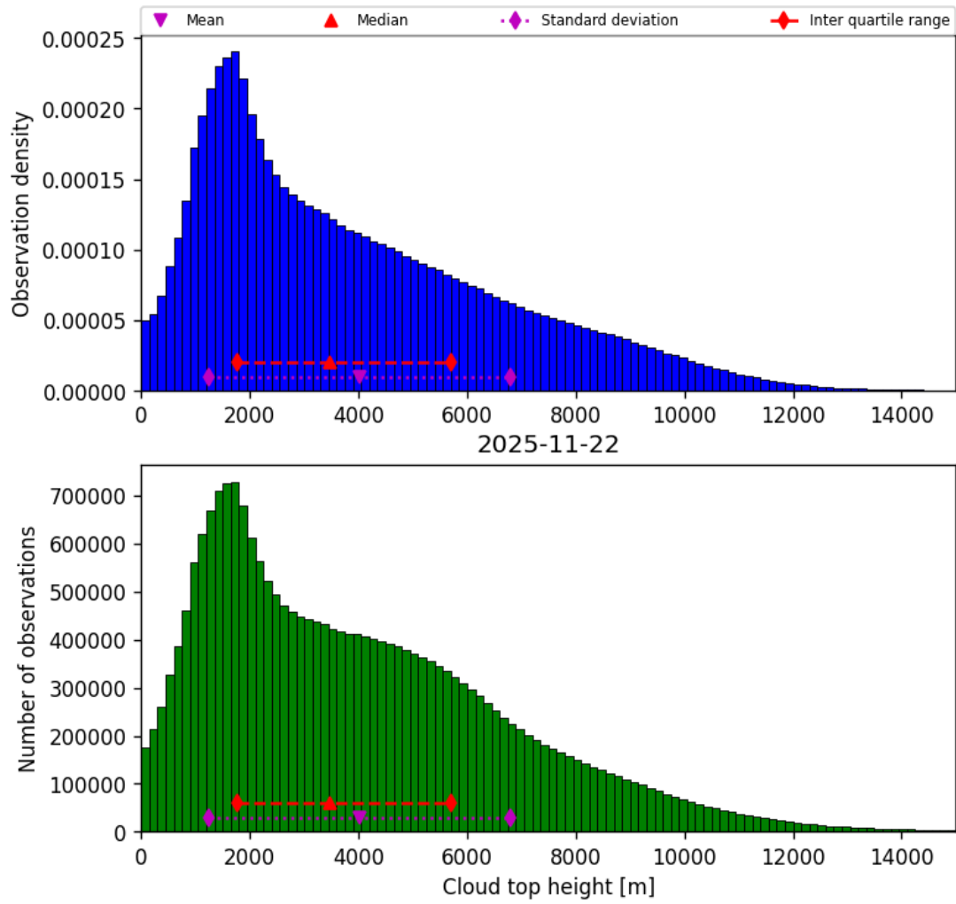
Figure 40: Histogram of “Cloud top height” for 2025-11-21 to 2025-11-23
