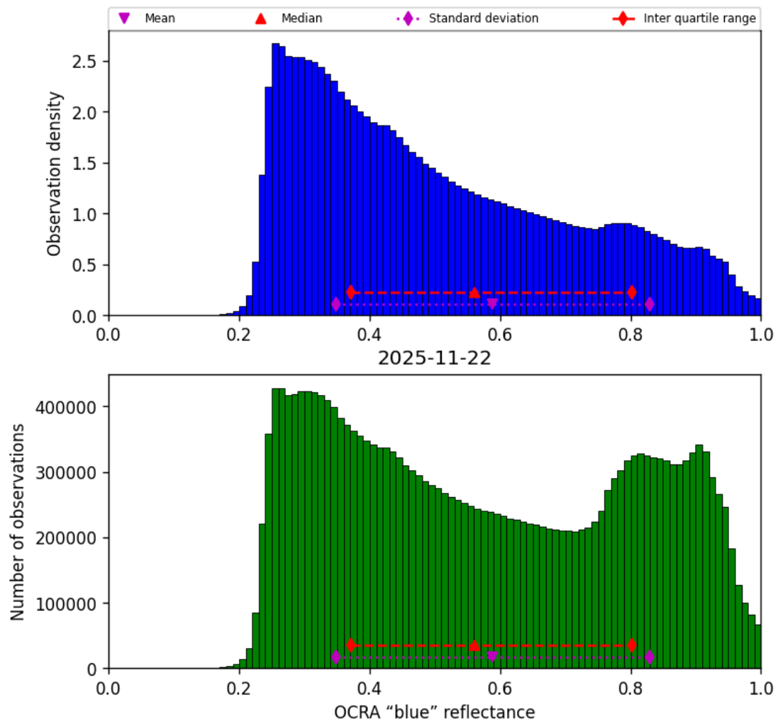
Figure 51: Histogram of “OCRA “blue” reflectance” for 2025-11-21 to 2025-11-23
