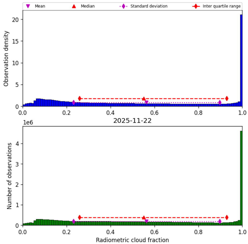
Figure 39: Histogram of “Radiometric cloud fraction” for 2025-11-21 to 2025-11-23
