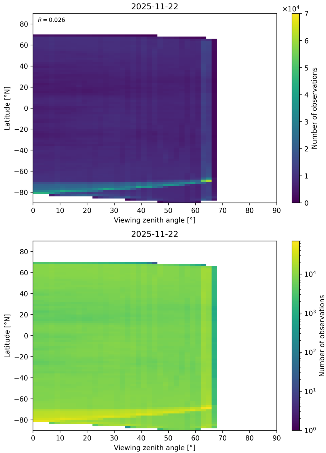
Figure 113: Scatter density plot of “Viewing zenith angle” against “Latitude” for 2025-11-21 to 2025-11-23.
