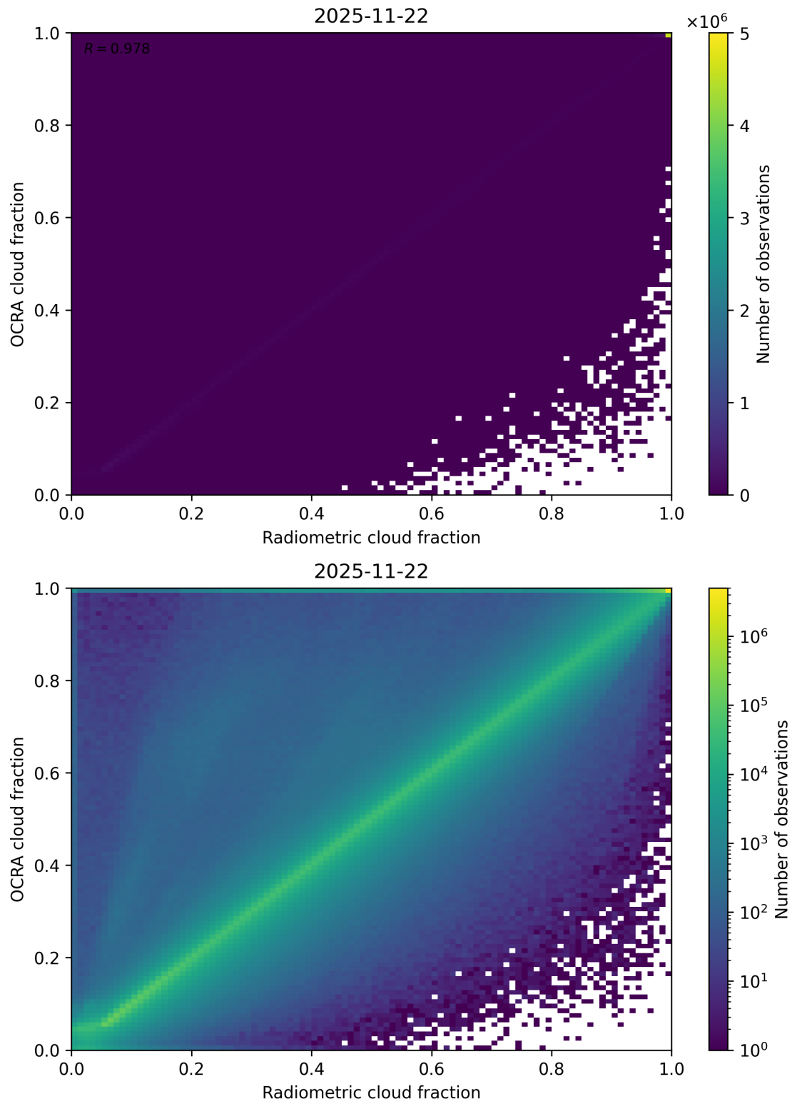
Figure 72: Scatter density plot of “Radiometric cloud fraction” against “OCRA cloud fraction” for 2025-11-21 to 2025-11-23.
