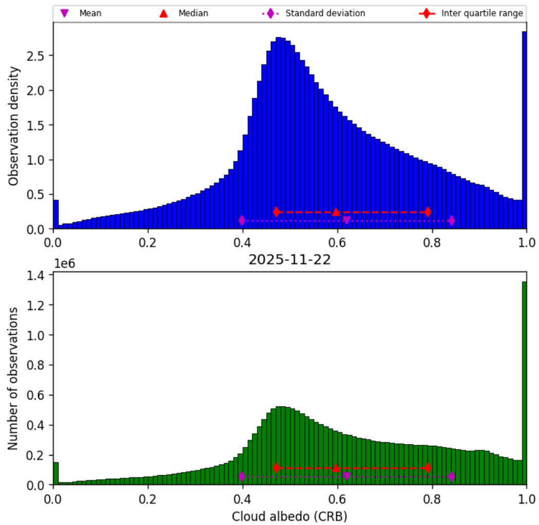
Figure 44: Histogram of “Cloud albedo (CRB)” for 2025-11-21 to 2025-11-23
