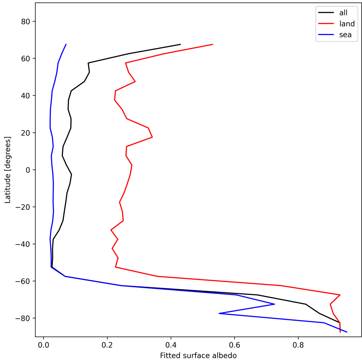
Figure 29: Zonal average of “Fitted surface albedo” for 2025-11-21 to 2025-11-23.
