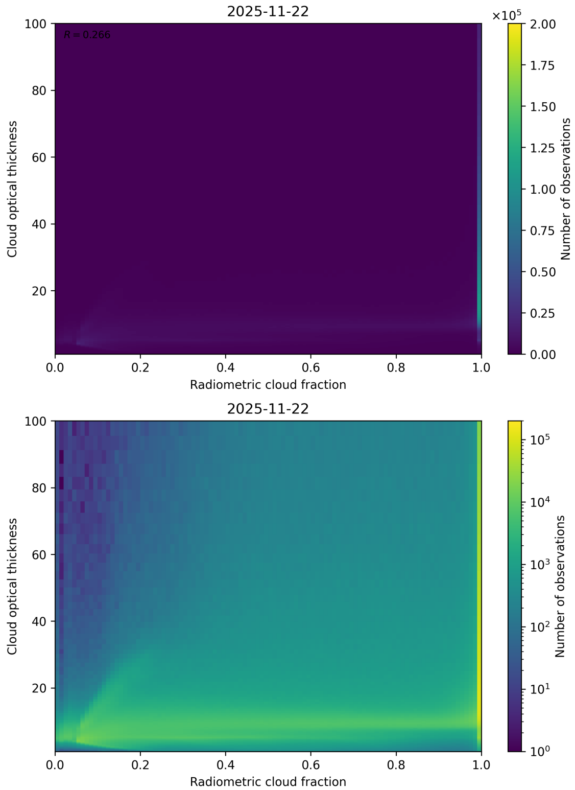
Figure 75: Scatter density plot of “Radiometric cloud fraction” against “Cloud optical thickness” for 2025-11-21 to 2025-11-23.
