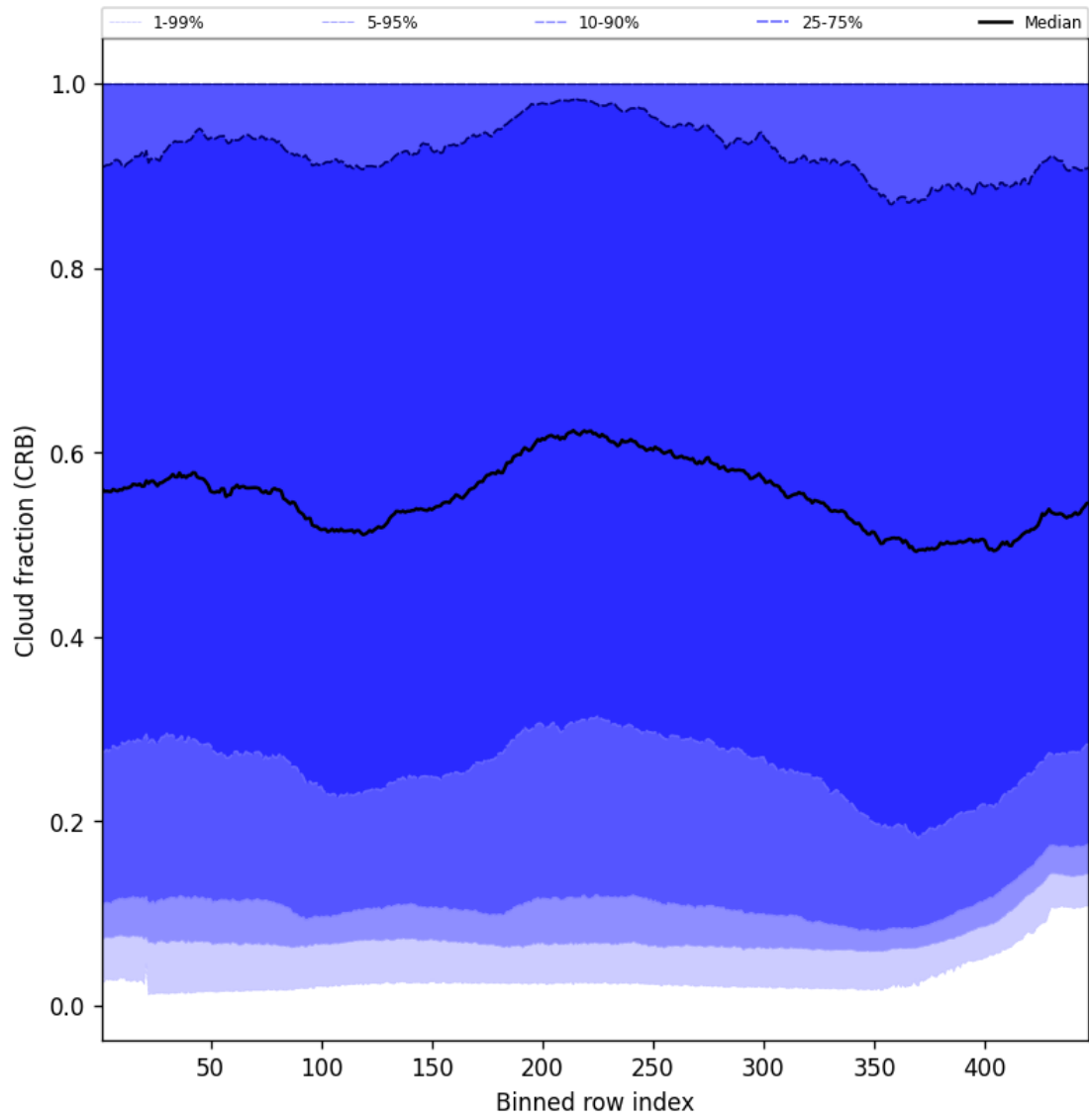
Figure 58: Along track statistics of “Cloud fraction (CRB)” for 2025-11-21 to 2025-11-23
