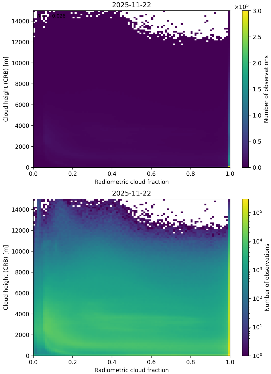
Figure 74: Scatter density plot of “Radiometric cloud fraction” against “Cloud height (CRB)” for 2025-11-21 to 2025-11-23.
