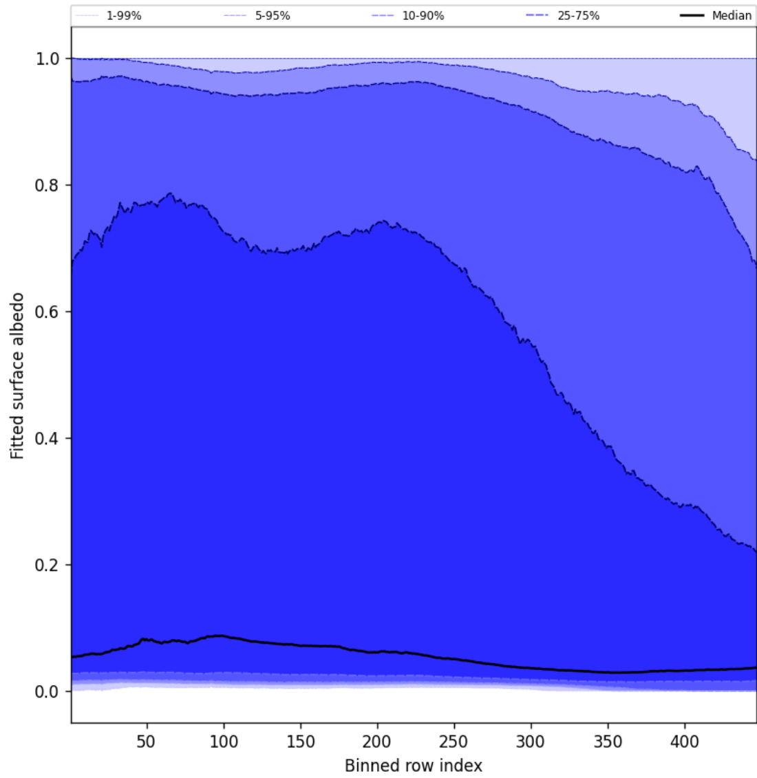
Figure 61: Along track statistics of “Fitted surface albedo” for 2025-11-21 to 2025-11-23
