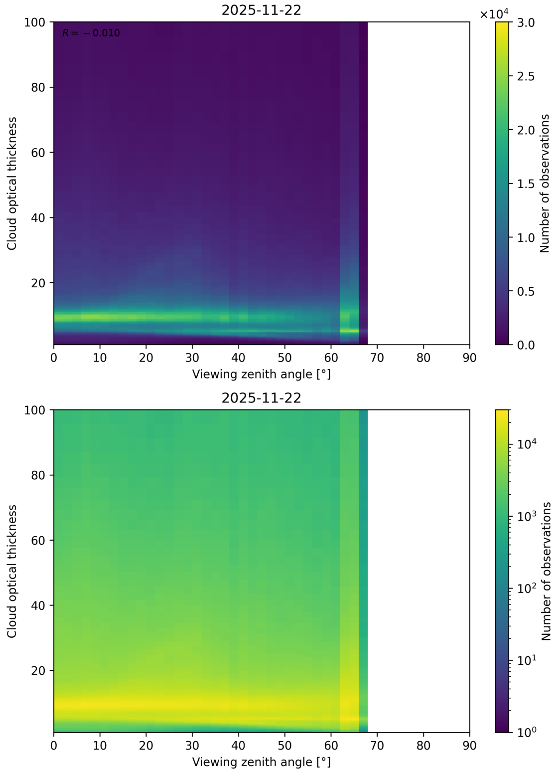
Figure 111: Scatter density plot of “Viewing zenith angle” against “Cloud optical thickness” for 2025-11-21 to 2025-11-23.
