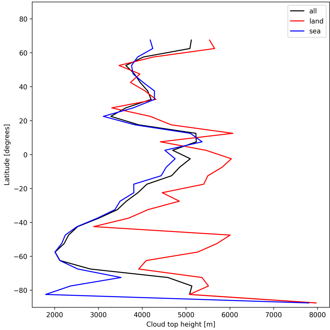
Figure 24: Zonal average of “Cloud top height” for 2025-11-21 to 2025-11-23.
