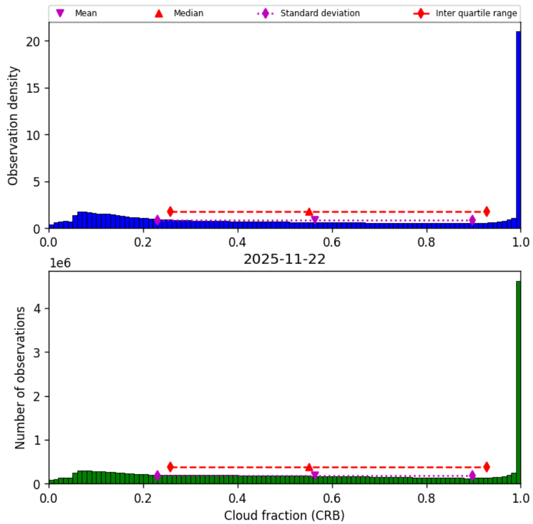
Figure 42: Histogram of “Cloud fraction (CRB)” for 2025-11-21 to 2025-11-23
