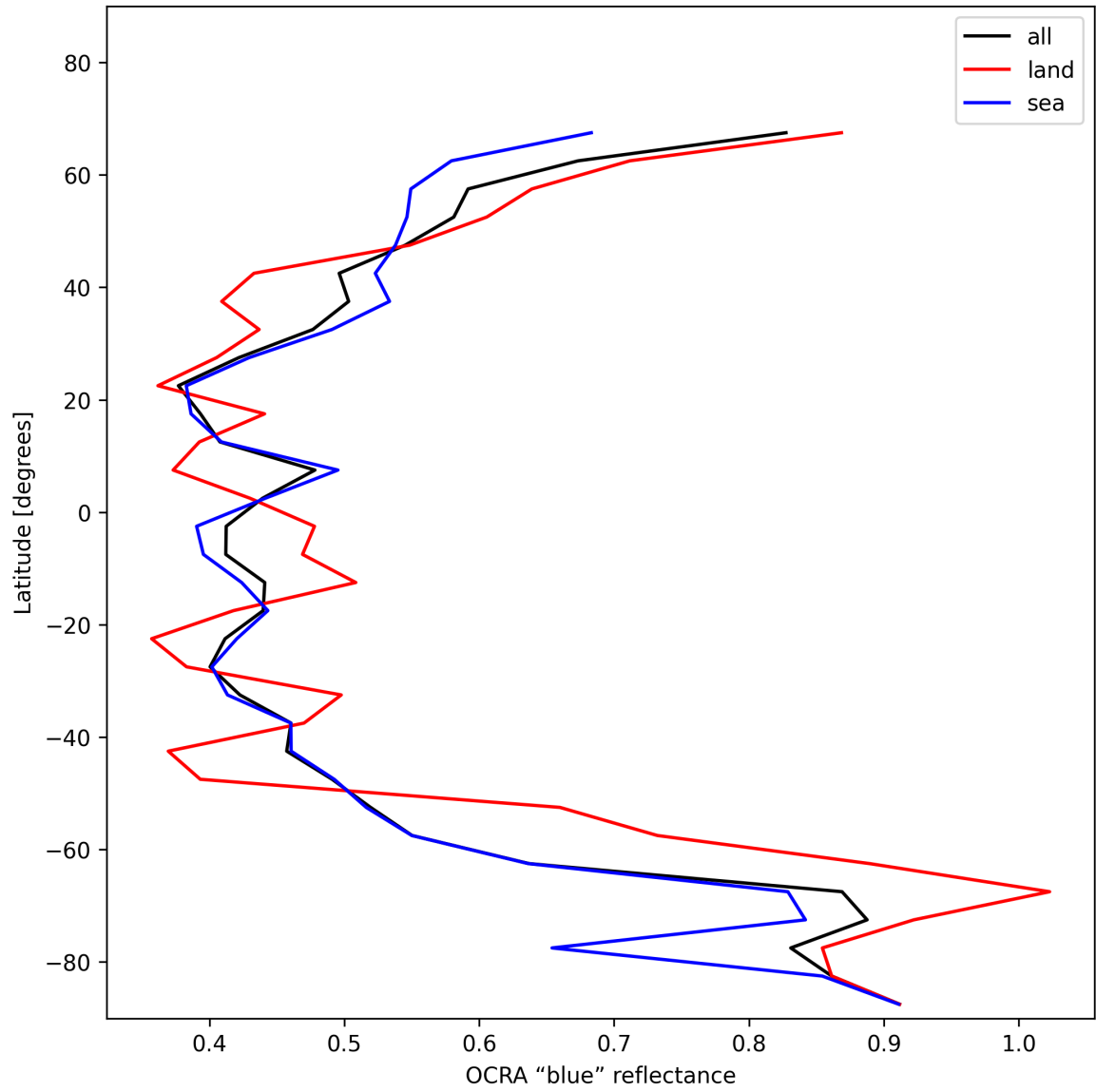
Figure 35: Zonal average of “OCRA “blue” reflectance” for 2025-11-21 to 2025-11-23.
