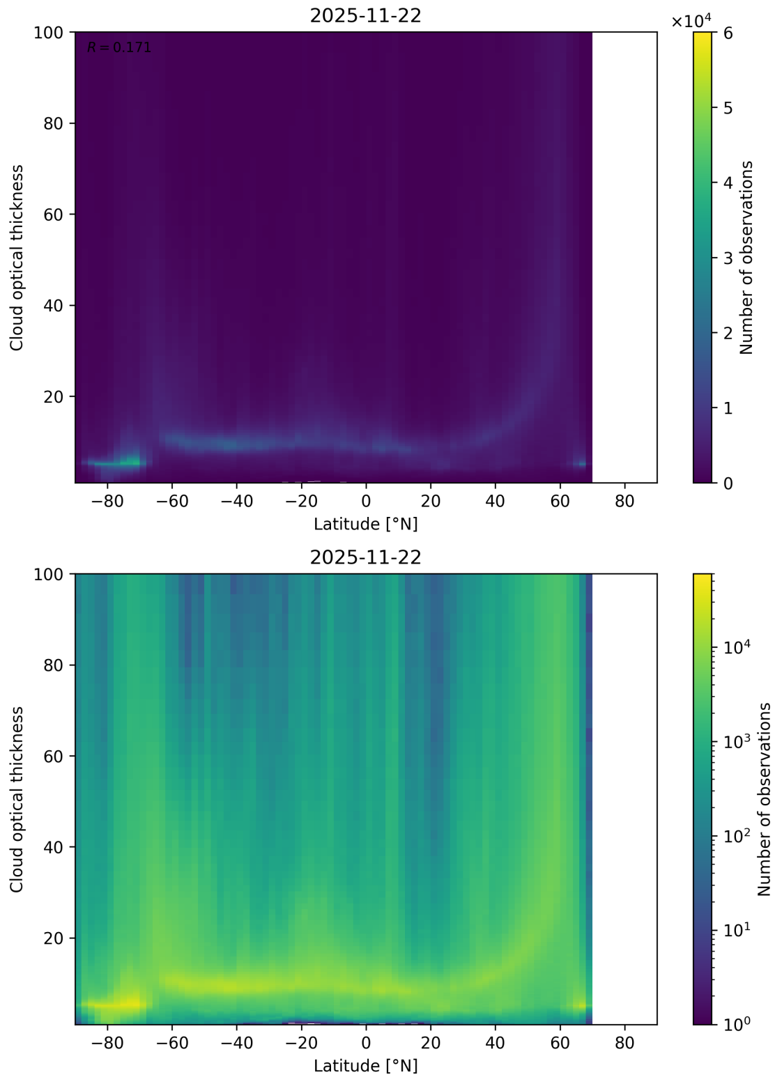
Figure 96: Scatter density plot of “Latitude” against “Cloud optical thickness” for 2025-11-21 to 2025-11-23.
