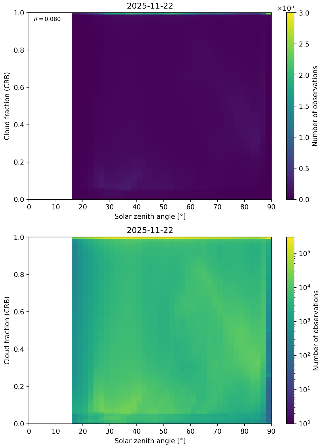
Figure 101: Scatter density plot of “Solar zenith angle” against “Cloud fraction (CRB)” for 2025-11-21 to 2025-11-23.
