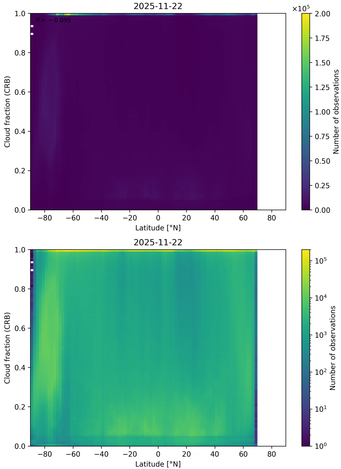
Figure 94: Scatter density plot of “Latitude” against “Cloud fraction (CRB)” for 2025-11-21 to 2025-11-23.
