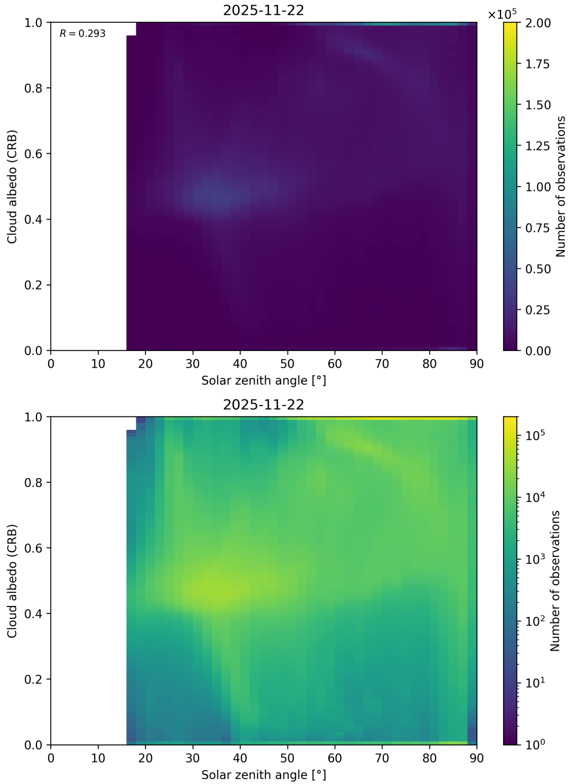
Figure 98: Scatter density plot of “Solar zenith angle” against “Cloud albedo (CRB)” for 2025-11-21 to 2025-11-23.
