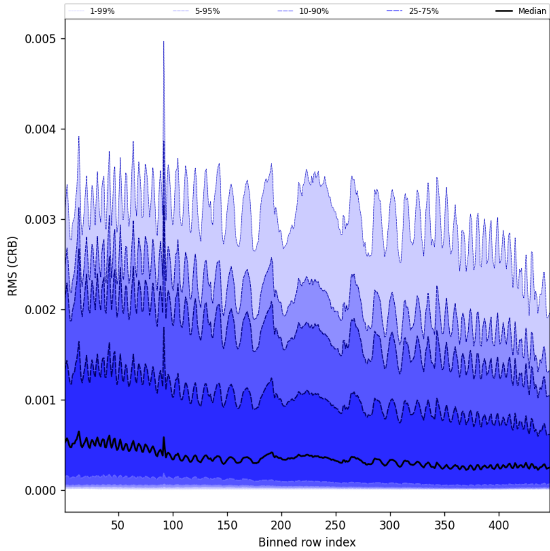
Figure 64: Along track statistics of “RMS (CRB)” for 2025-11-21 to 2025-11-23
