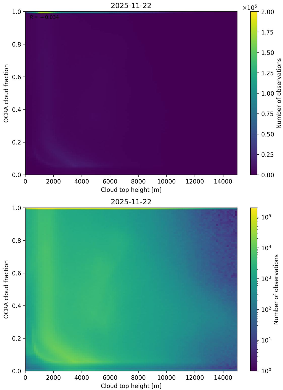
Figure 87: Scatter density plot of “Cloud top height” against “OCRA cloud fraction” for 2025-11-21 to 2025-11-23.
