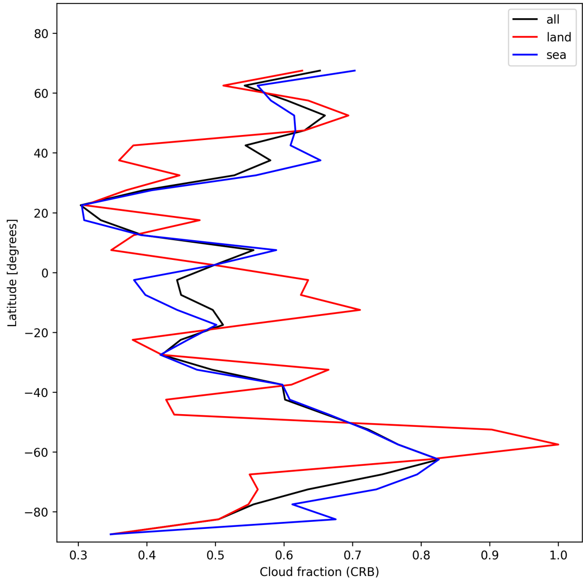
Figure 26: Zonal average of “Cloud fraction (CRB)” for 2025-11-21 to 2025-11-23.
