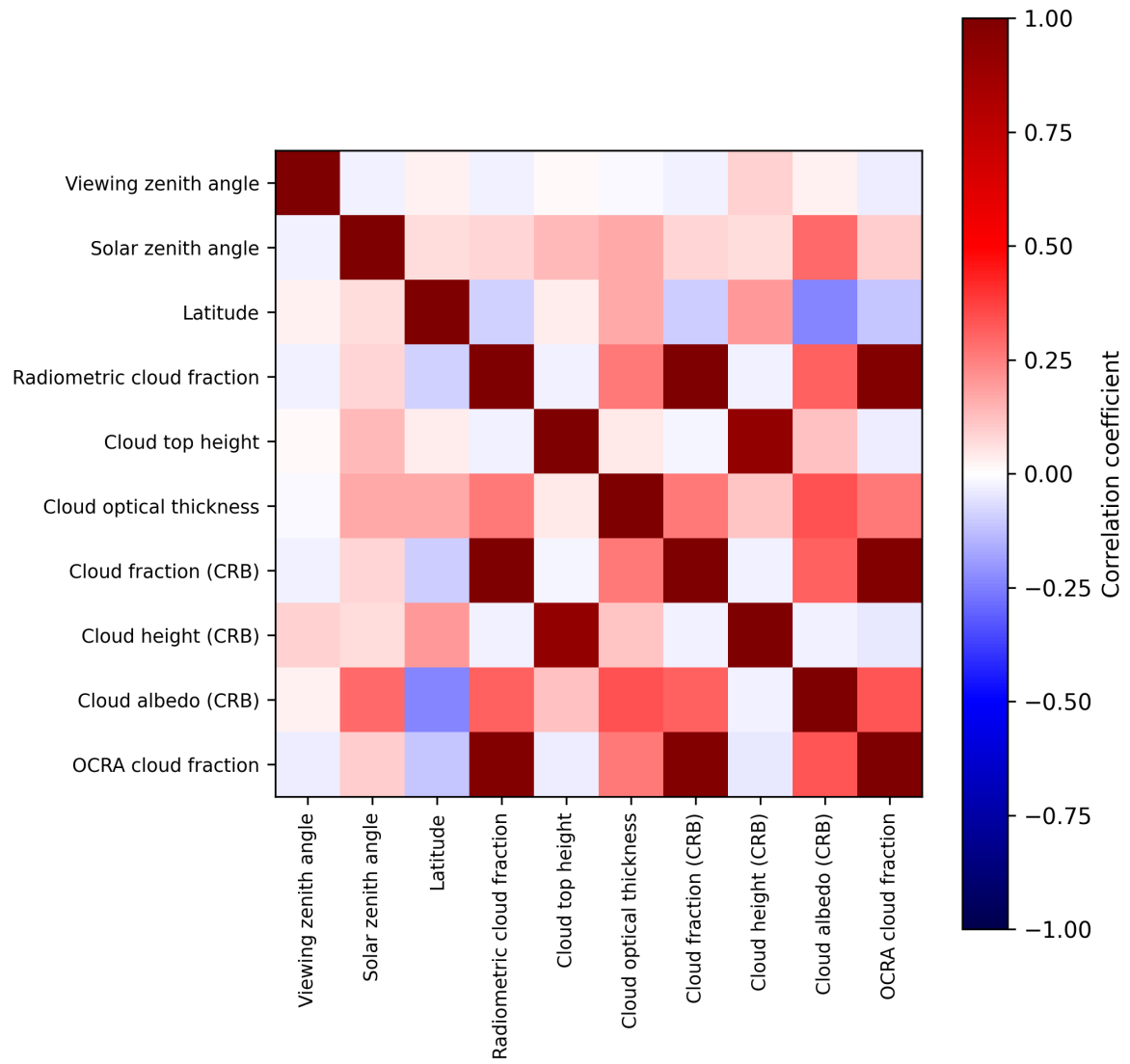
Figure 2: Map of correlation matrix for 2025-11-21 to 2025-11-23.
