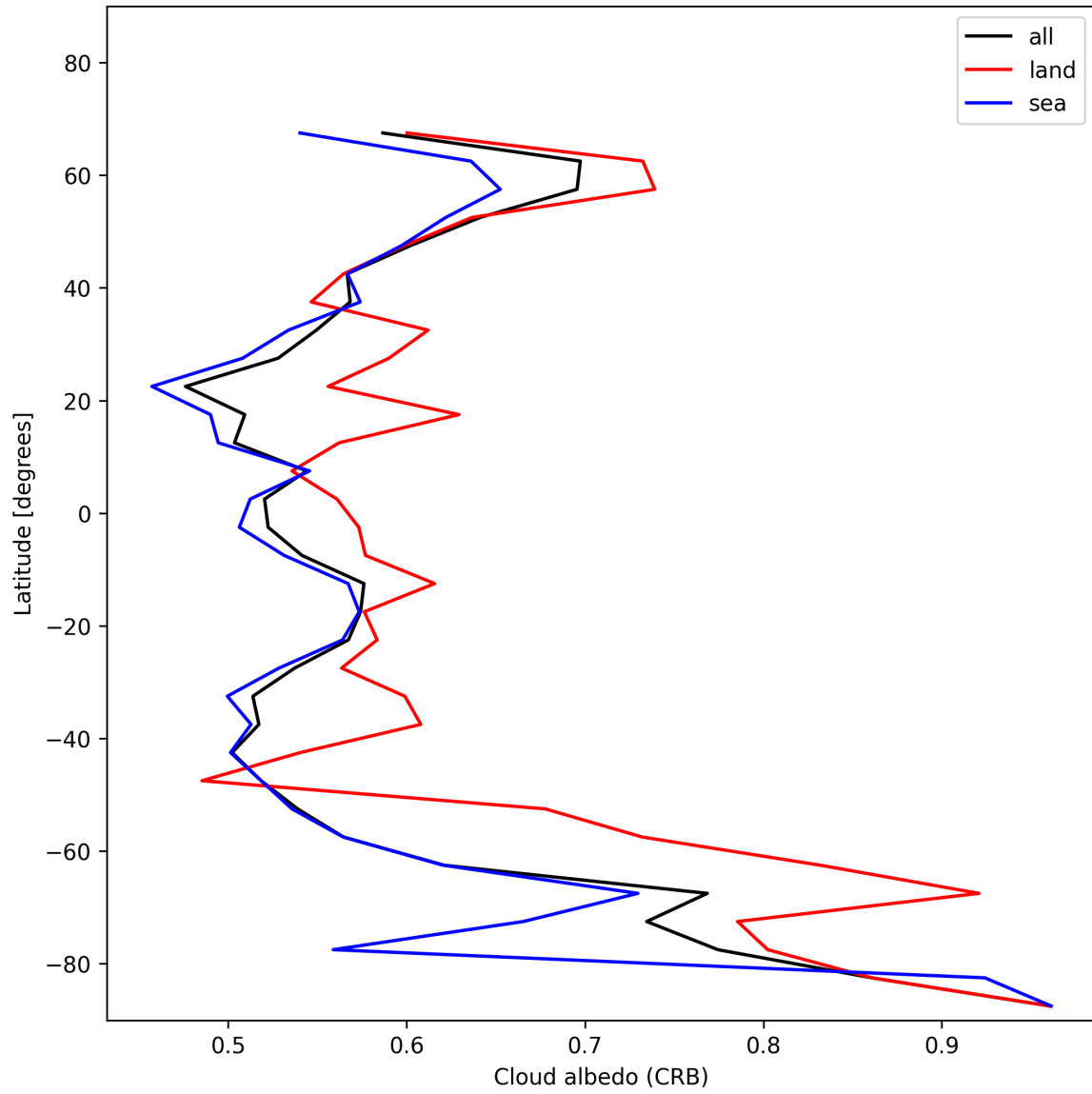
Figure 28: Zonal average of “Cloud albedo (CRB)” for 2025-11-21 to 2025-11-23.
