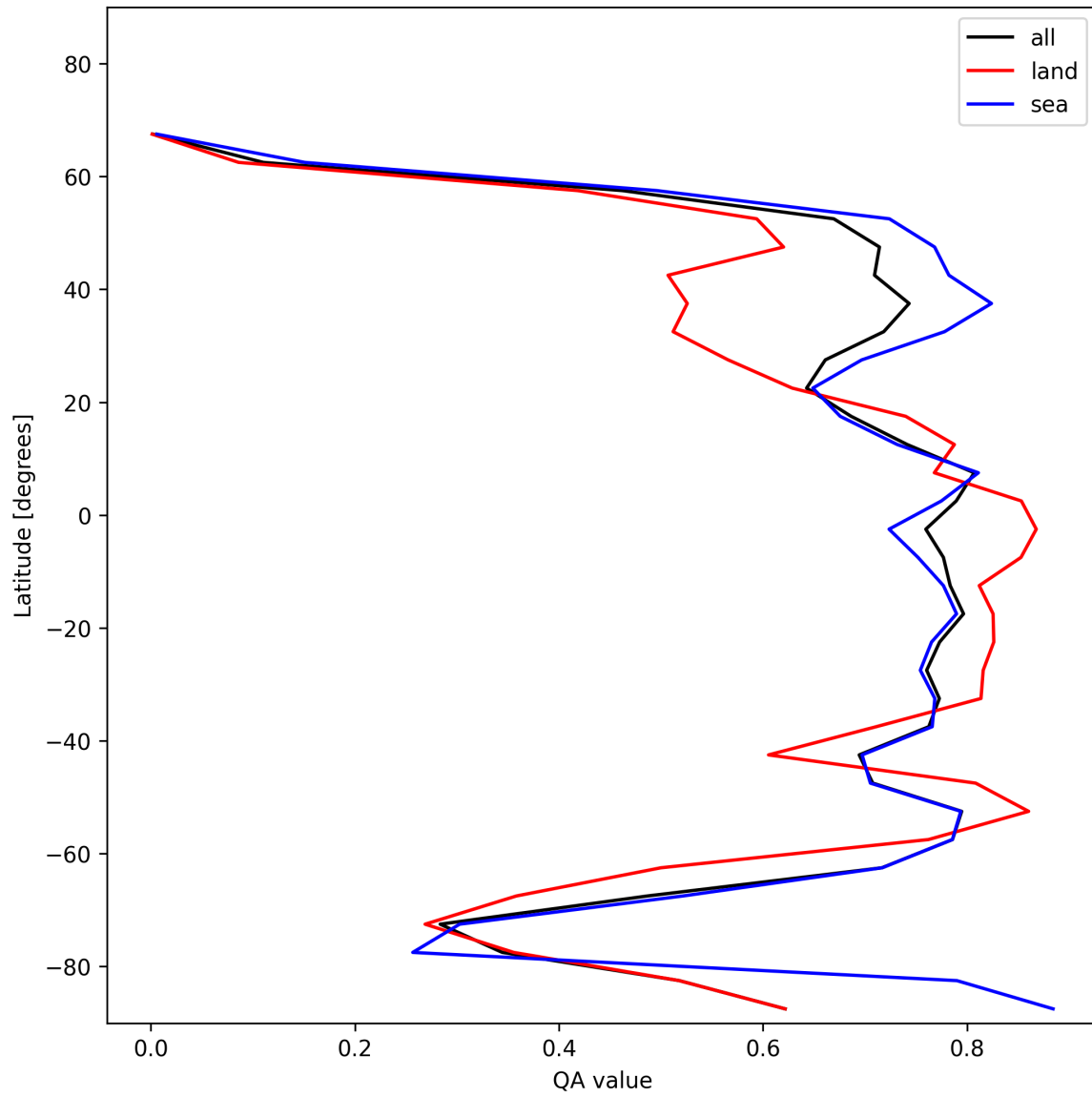
Figure 22: Zonal average of “QA value” for 2025-11-21 to 2025-11-23.
