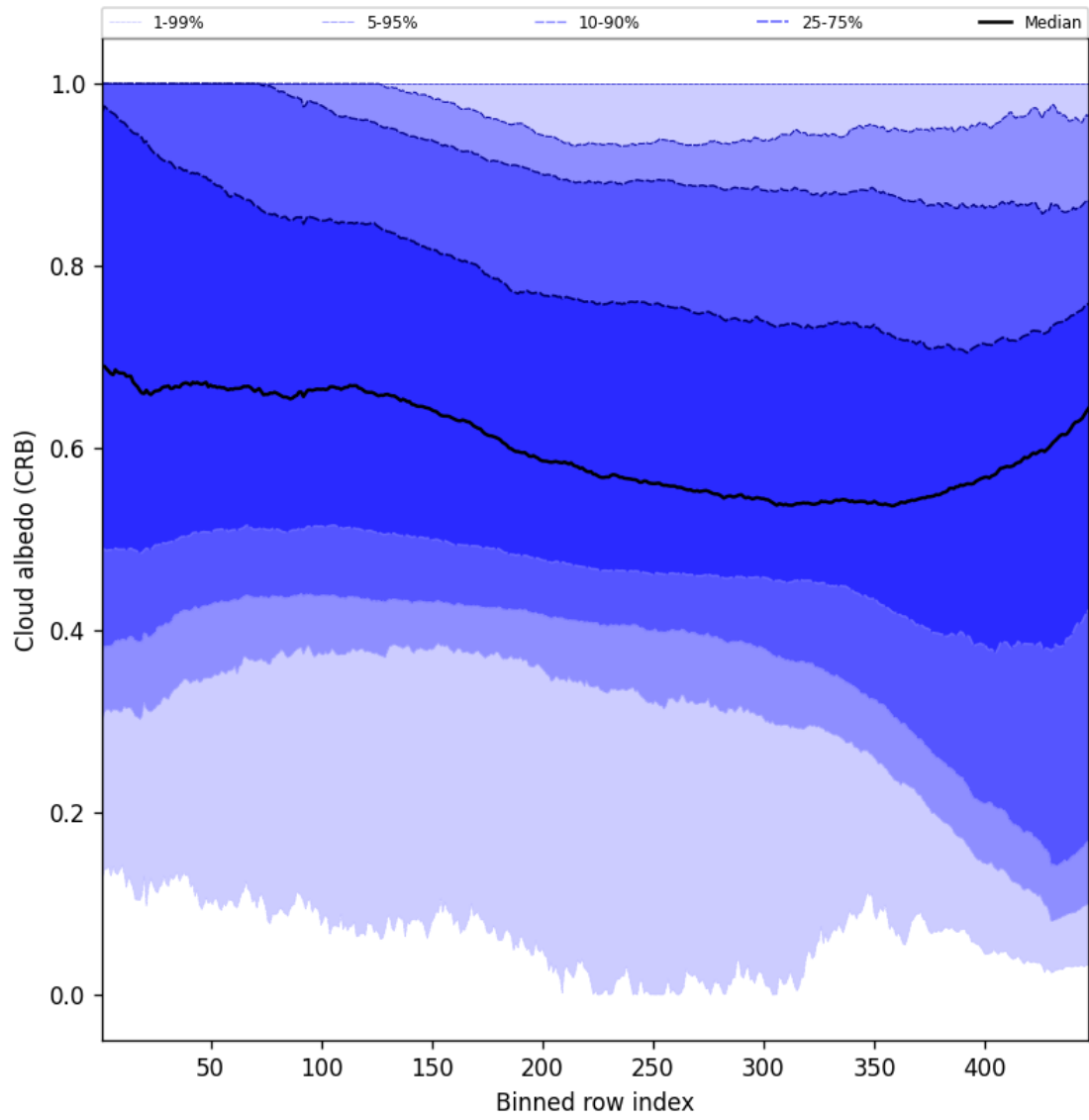
Figure 60: Along track statistics of “Cloud albedo (CRB)” for 2025-11-21 to 2025-11-23
