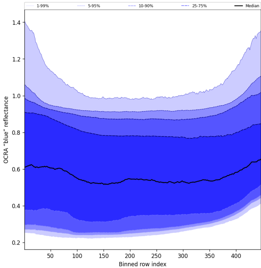
Figure 67: Along track statistics of “OCRA “blue” reflectance” for 2025-11-21 to 2025-11-23
