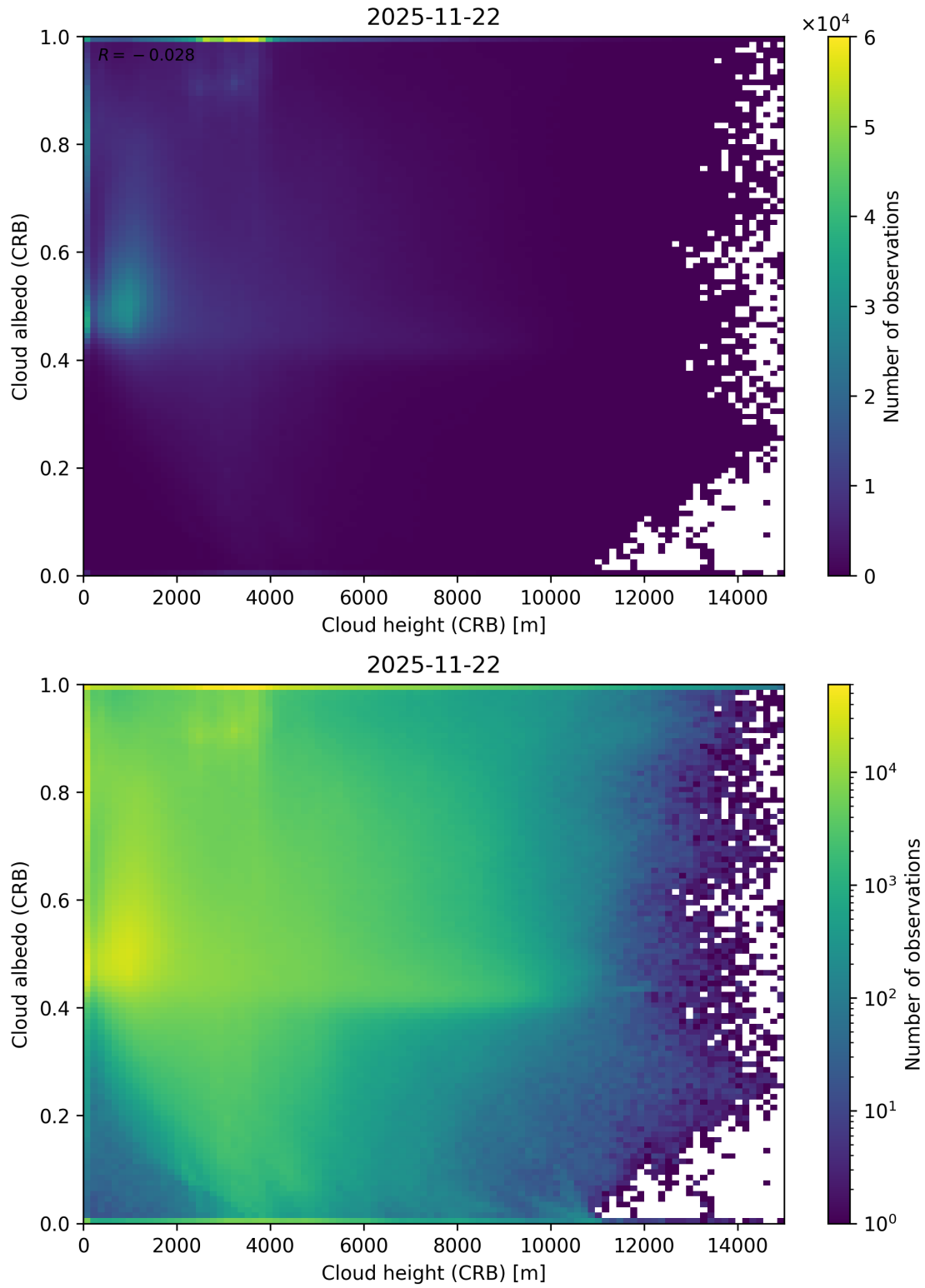
Figure 80: Scatter density plot of “Cloud height (CRB)” against “Cloud albedo (CRB)” for 2025-11-21 to 2025-11-23.
