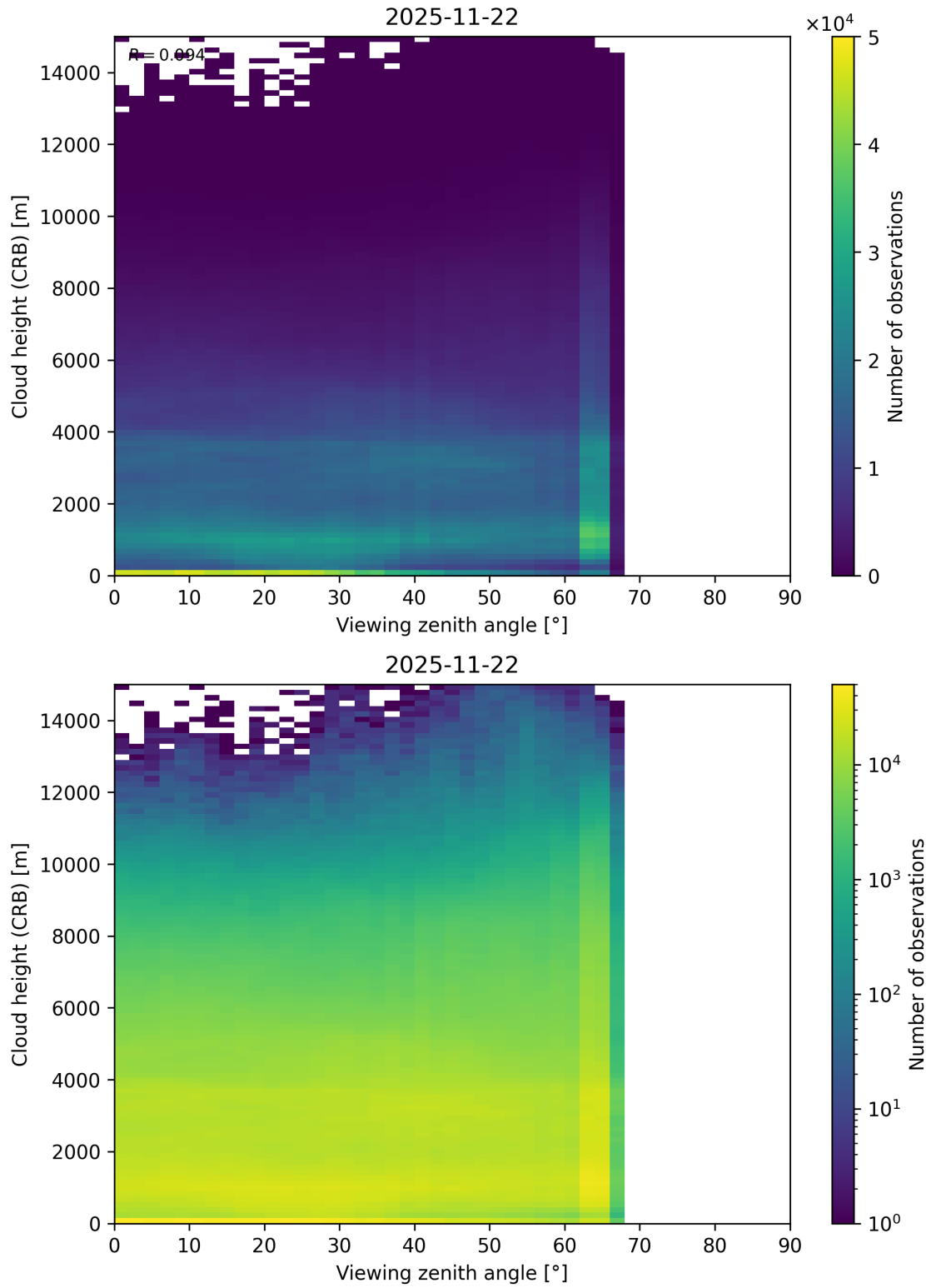
Figure 110: Scatter density plot of “Viewing zenith angle” against “Cloud height (CRB)” for 2025-11-21 to 2025-11-23.
