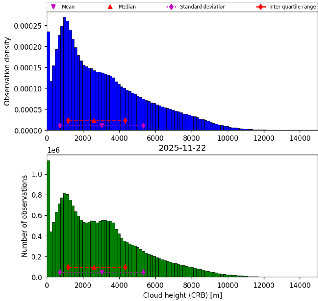
Figure 43: Histogram of “Cloud height (CRB)” for 2025-11-21 to 2025-11-23
