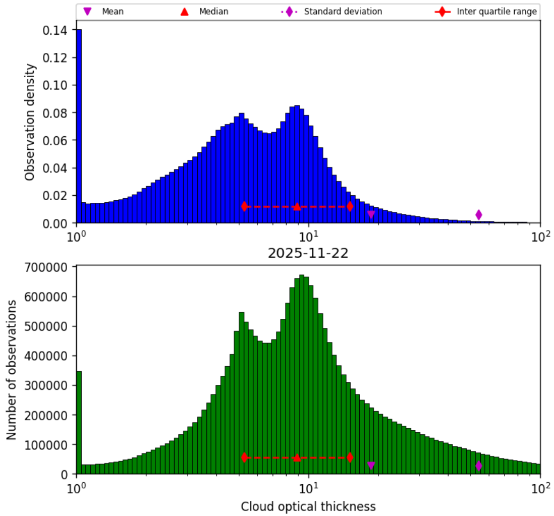
Figure 41: Histogram of “Cloud optical thickness” for 2025-11-21 to 2025-11-23
