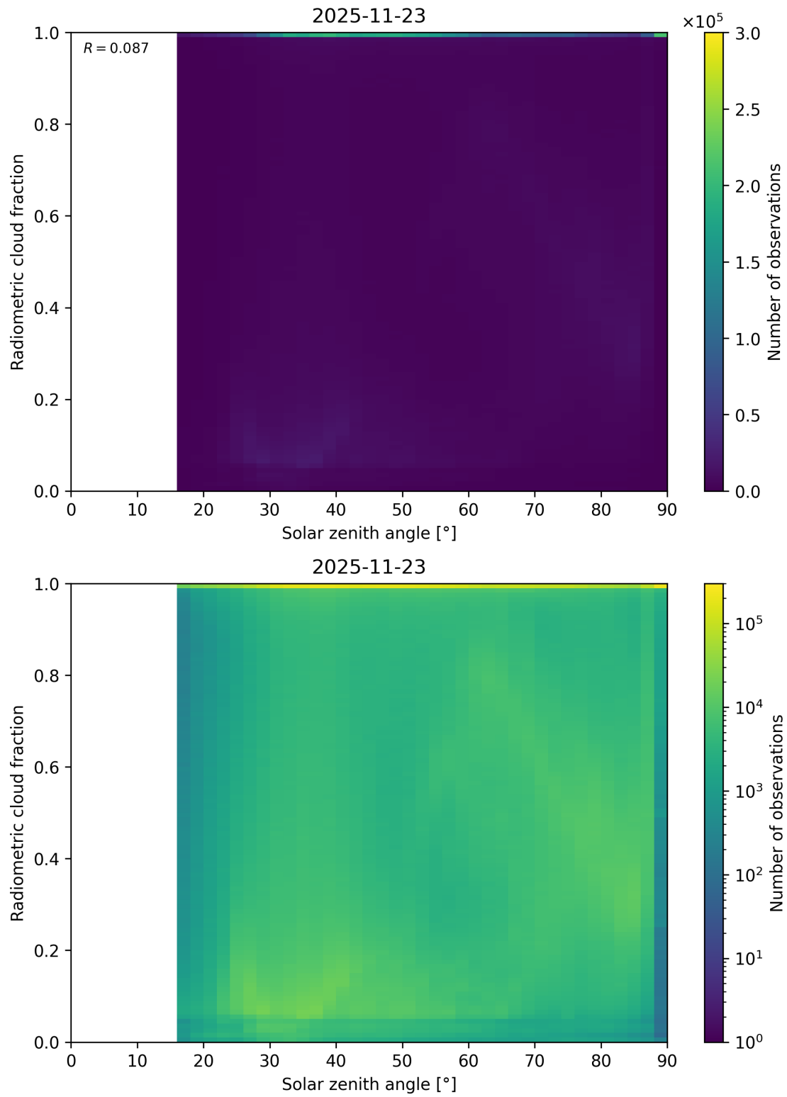
Figure 99: Scatter density plot of “Solar zenith angle” against “Radiometric cloud fraction” for 2025-11-23 to 2025-11-24.
