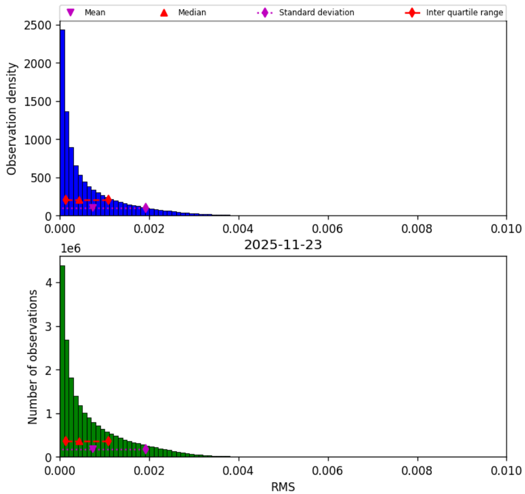
Figure 47: Histogram of “RMS” for 2025-11-23 to 2025-11-24
