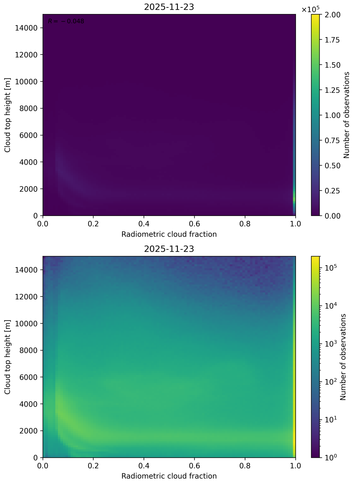
Figure 76: Scatter density plot of “Radiometric cloud fraction” against “Cloud top height” for 2025-11-23 to 2025-11-24.
