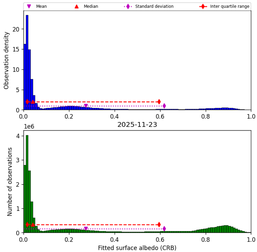
Figure 46: Histogram of “Fitted surface albedo (CRB)” for 2025-11-23 to 2025-11-24
