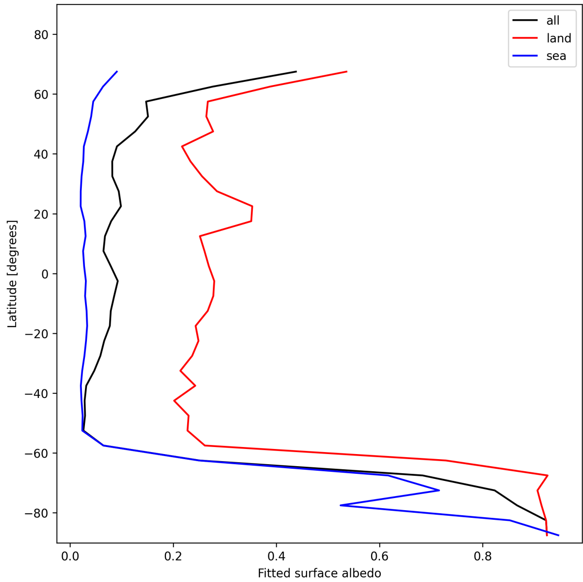
Figure 29: Zonal average of “Fitted surface albedo” for 2025-11-23 to 2025-11-24.
