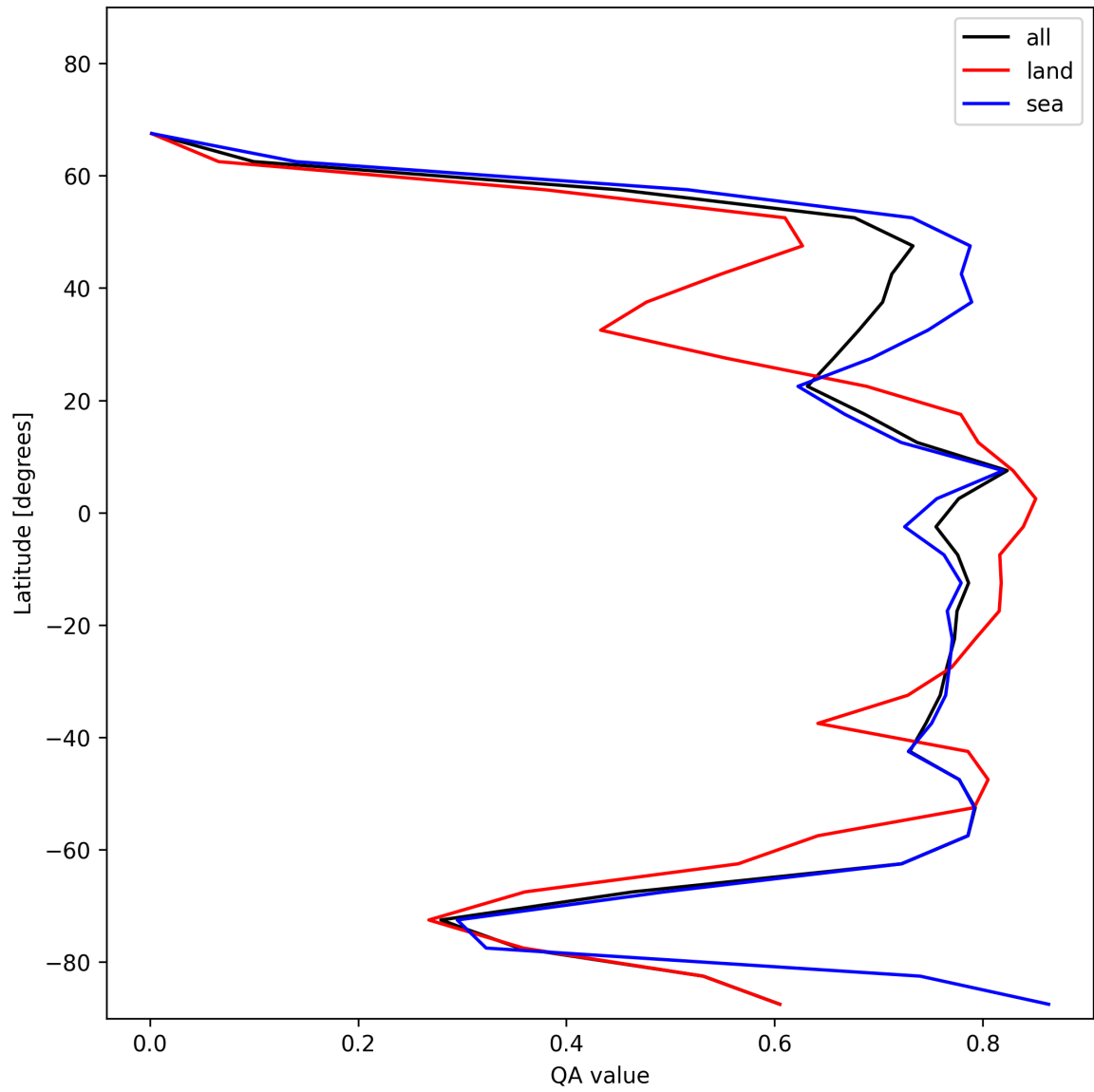
Figure 22: Zonal average of “QA value” for 2025-11-23 to 2025-11-24.
