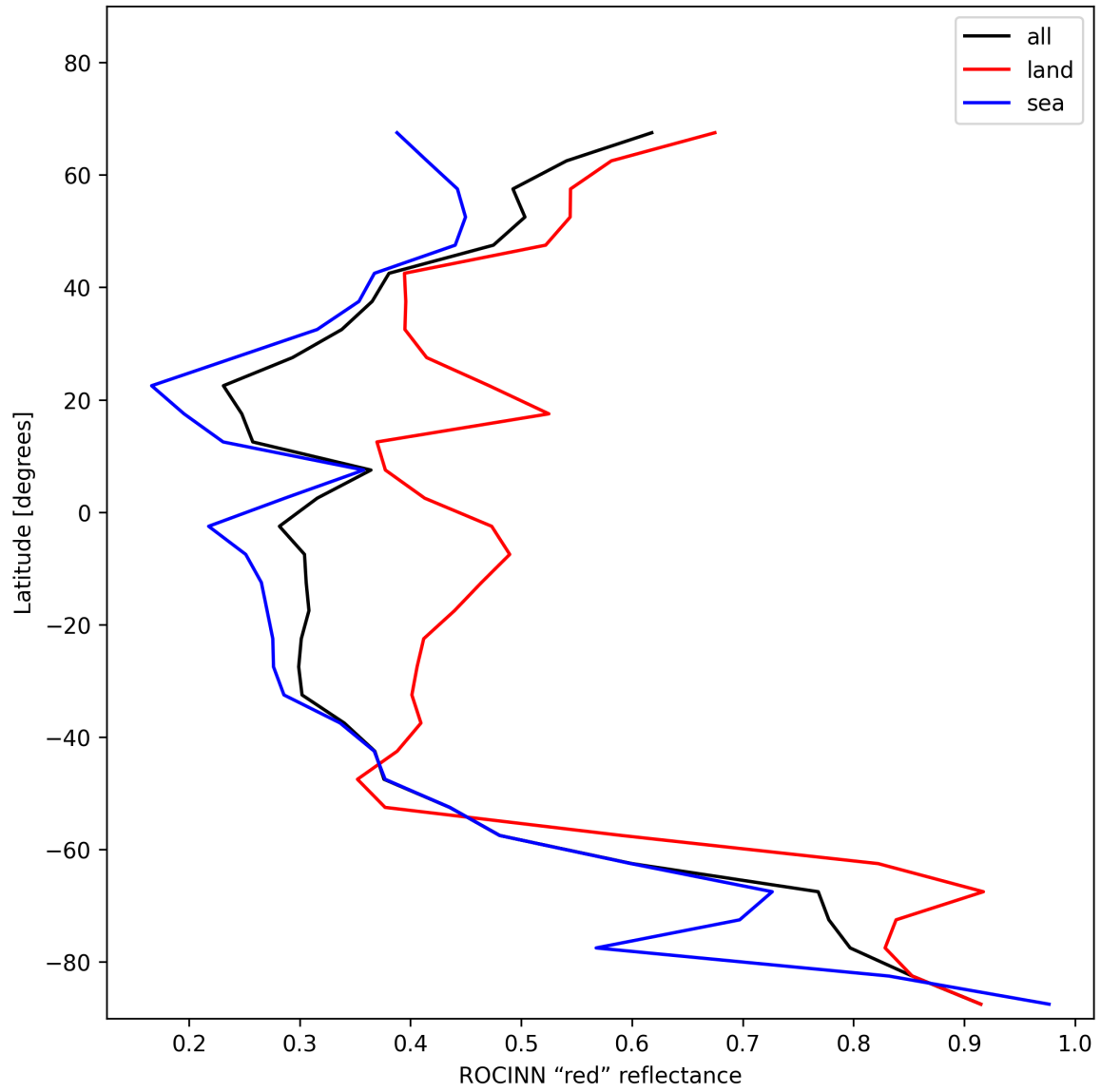
Figure 37: Zonal average of “ROCINN “red” reflectance” for 2025-11-23 to 2025-11-24.
