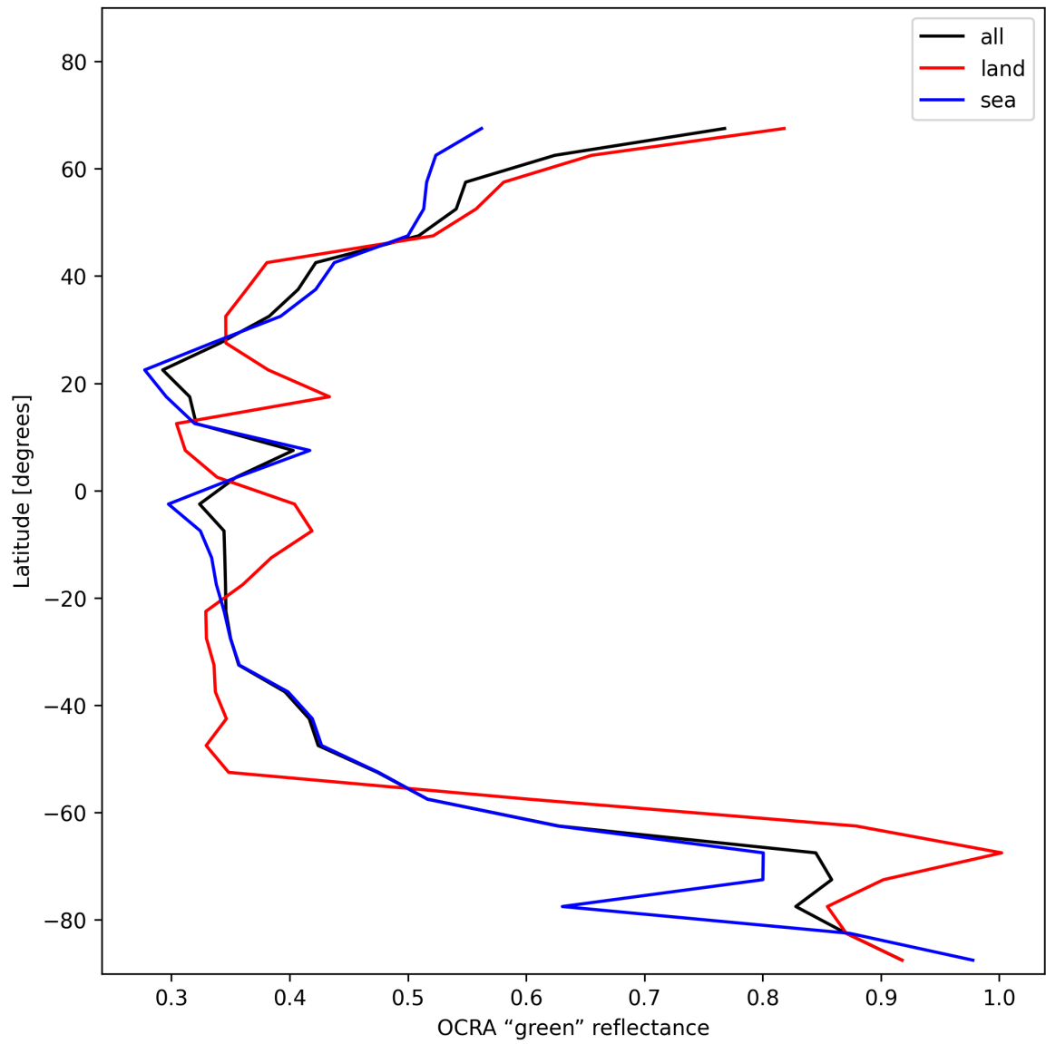
Figure 36: Zonal average of “OCRA “green” reflectance” for 2025-11-23 to 2025-11-24.
