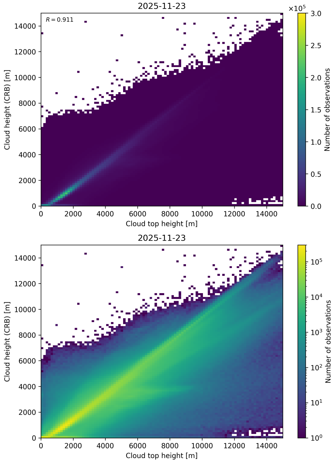
Figure 89: Scatter density plot of “Cloud top height” against “Cloud height (CRB)” for 2025-11-23 to 2025-11-24.
