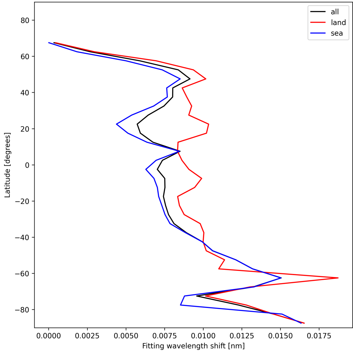
Figure 33: Zonal average of “Fitting wavelength shift” for 2025-11-23 to 2025-11-24.
