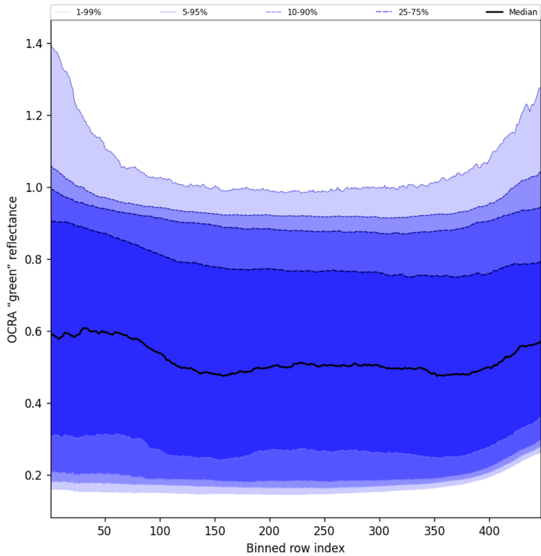
Figure 68: Along track statistics of “OCRA “green” reflectance” for 2025-11-23 to 2025-11-24
