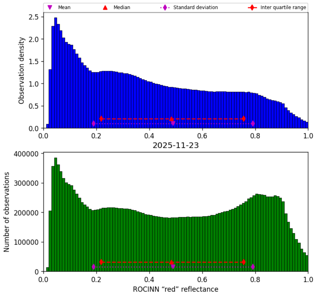
Figure 53: Histogram of “ROCINN “red” reflectance” for 2025-11-23 to 2025-11-24
