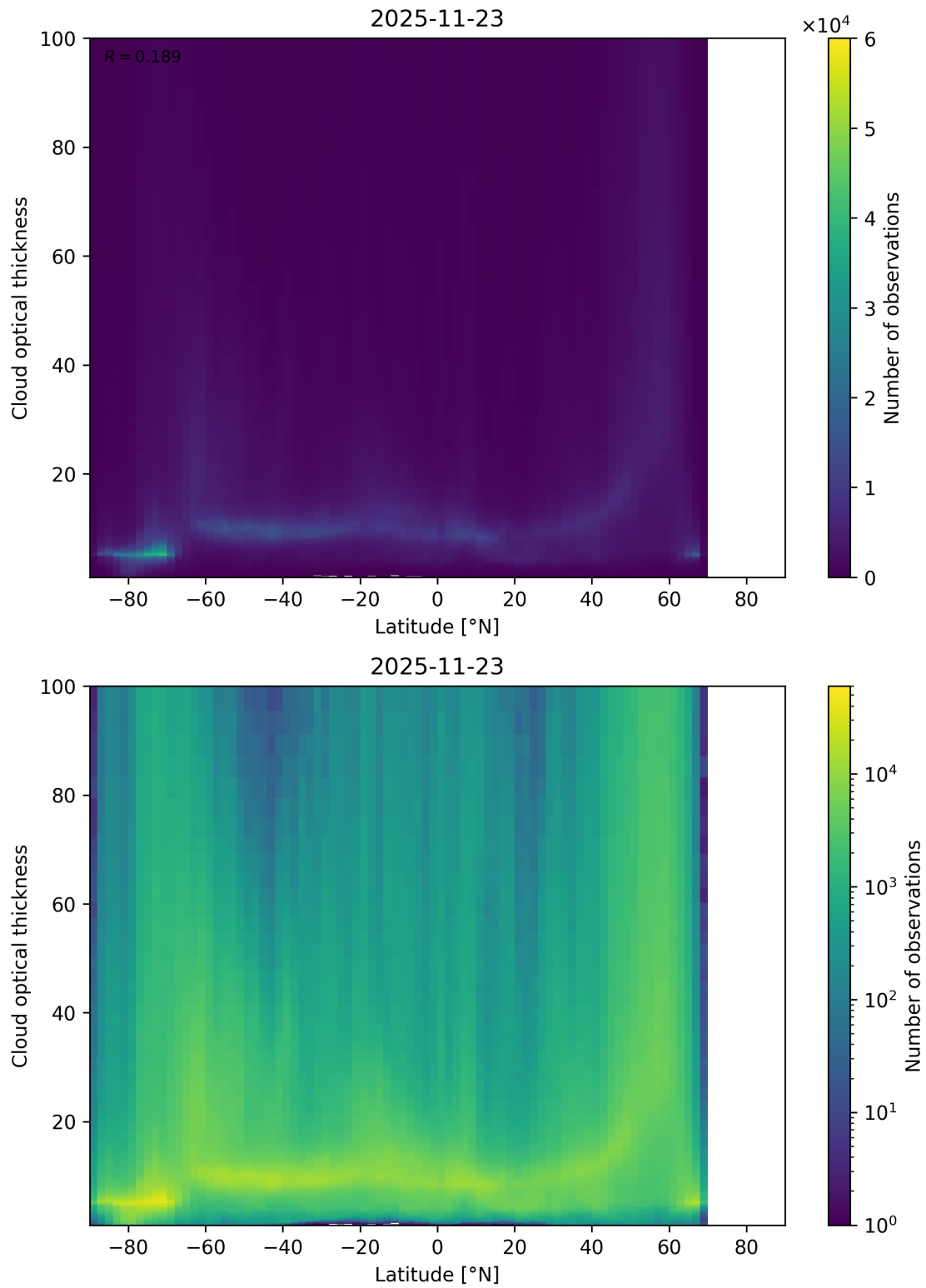
Figure 96: Scatter density plot of “Latitude” against “Cloud optical thickness” for 2025-11-23 to 2025-11-24.
