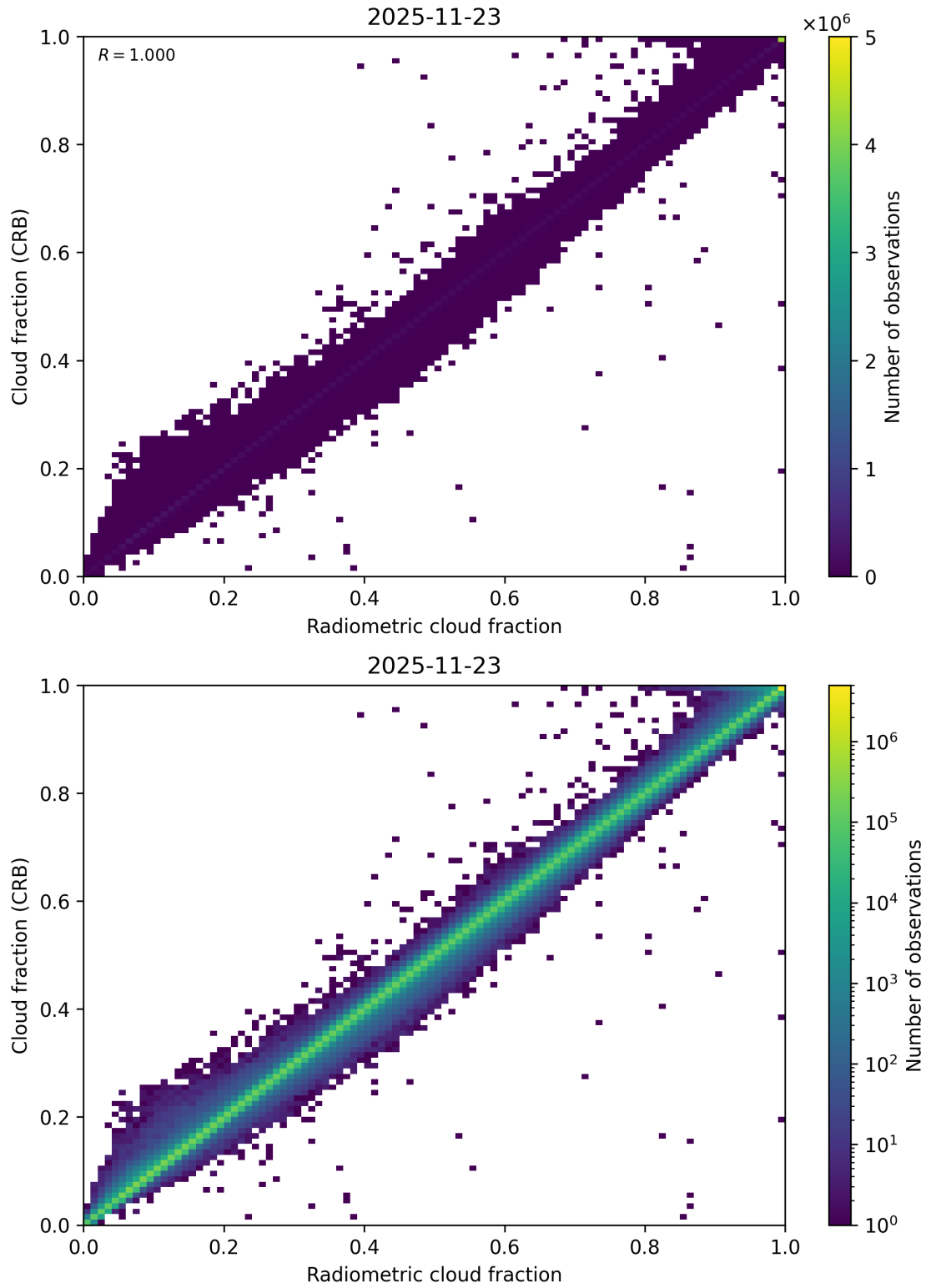
Figure 73: Scatter density plot of “Radiometric cloud fraction” against “Cloud fraction (CRB)” for 2025-11-23 to 2025-11-24.
