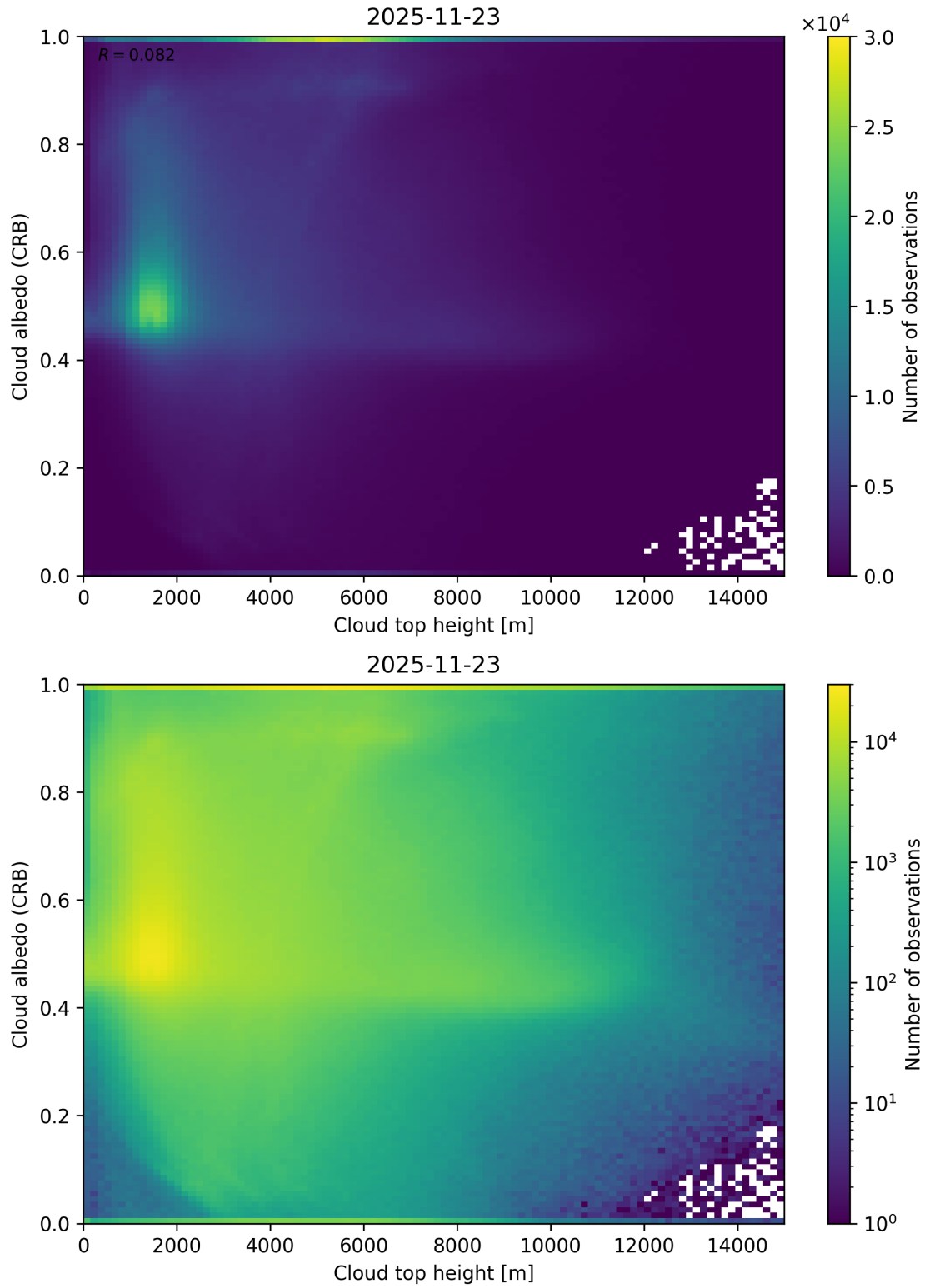
Figure 86: Scatter density plot of “Cloud top height” against “Cloud albedo (CRB)” for 2025-11-23 to 2025-11-24.
