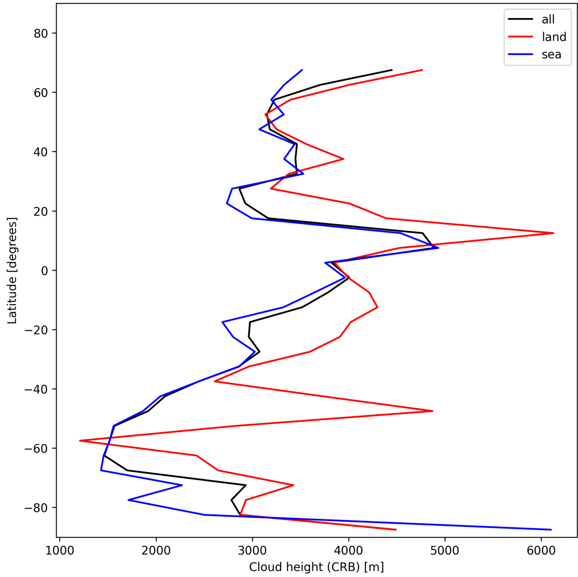
Figure 27: Zonal average of “Cloud height (CRB)” for 2025-11-23 to 2025-11-24.
