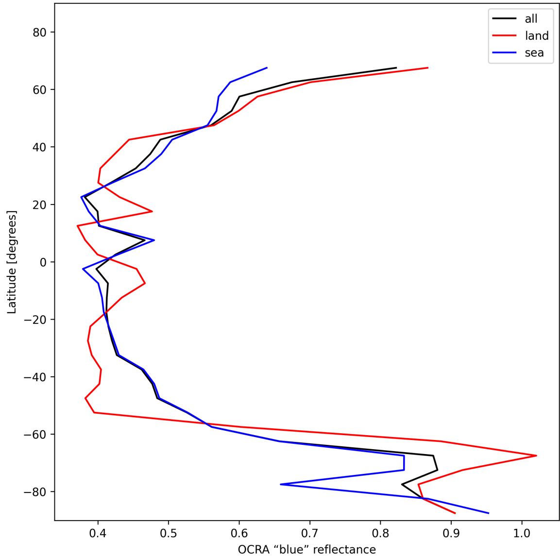
Figure 35: Zonal average of “OCRA “blue” reflectance” for 2025-11-23 to 2025-11-24.
