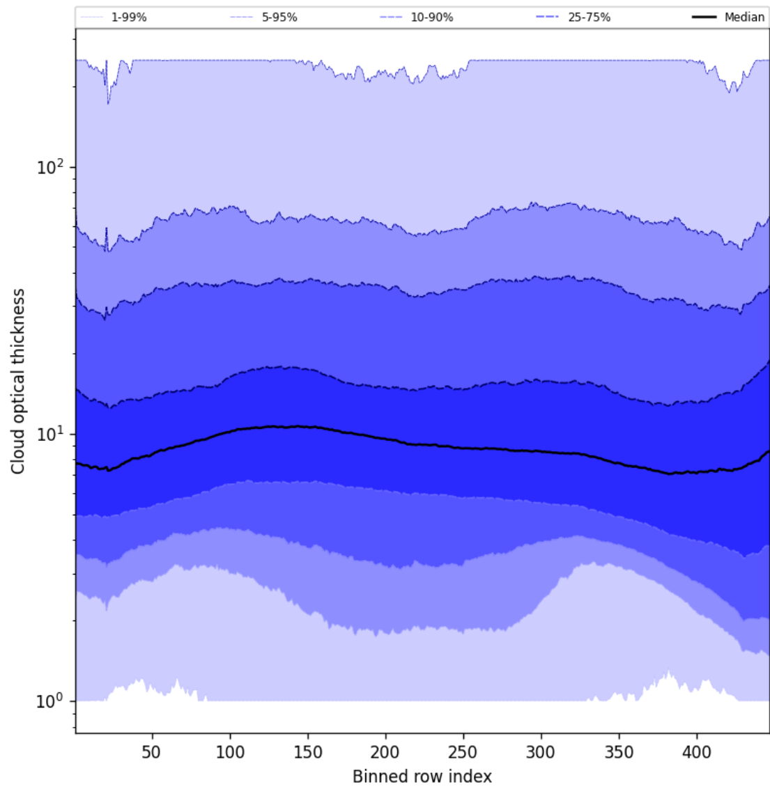
Figure 57: Along track statistics of “Cloud optical thickness” for 2025-11-23 to 2025-11-24
