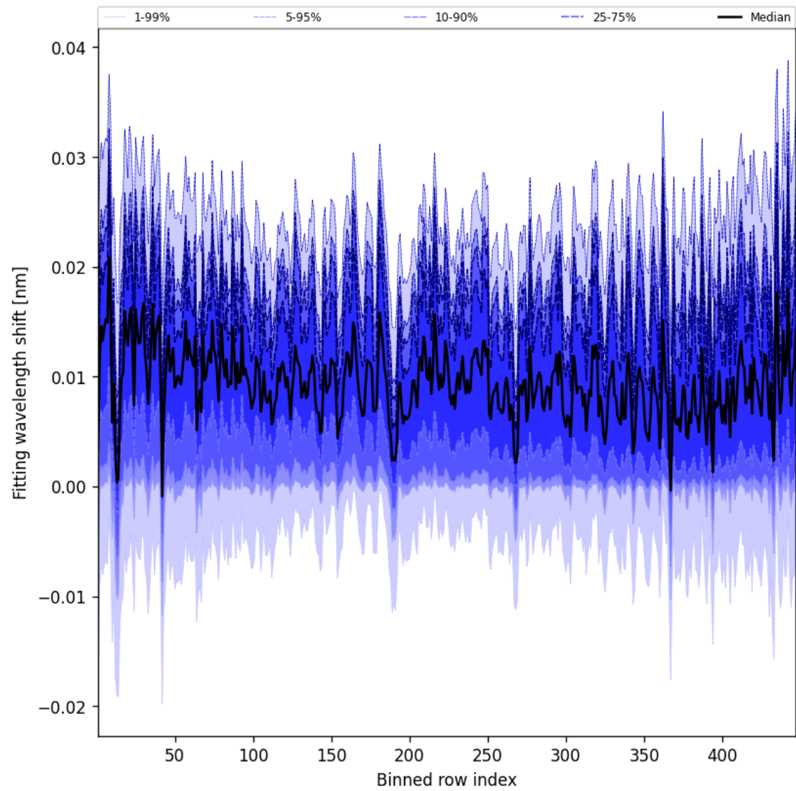
Figure 65: Along track statistics of “Fitting wavelength shift” for 2025-11-23 to 2025-11-24
