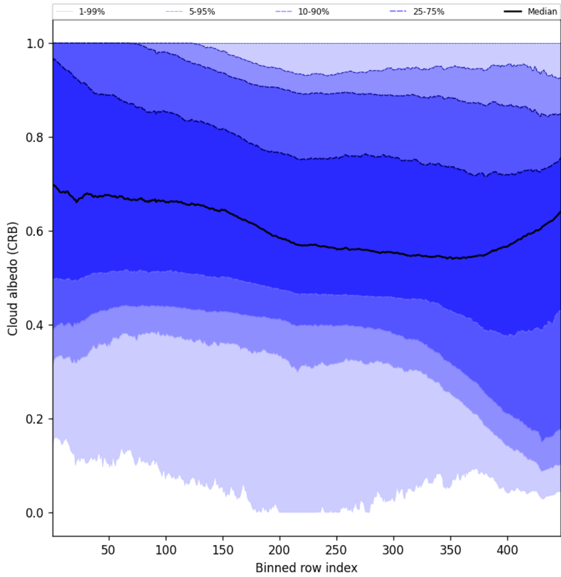
Figure 60: Along track statistics of “Cloud albedo (CRB)” for 2025-11-23 to 2025-11-24
