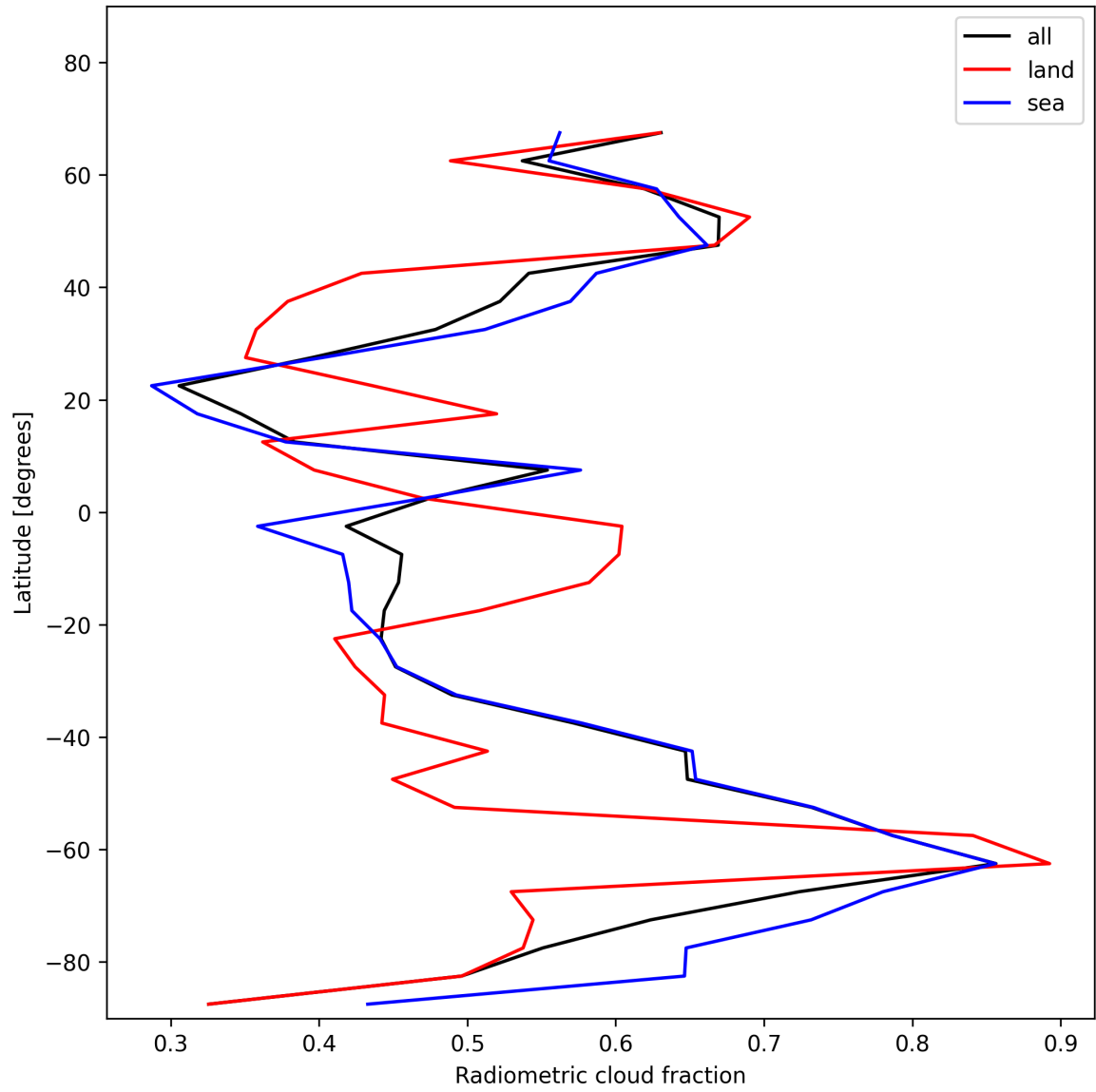
Figure 23: Zonal average of “Radiometric cloud fraction” for 2025-11-23 to 2025-11-24.
