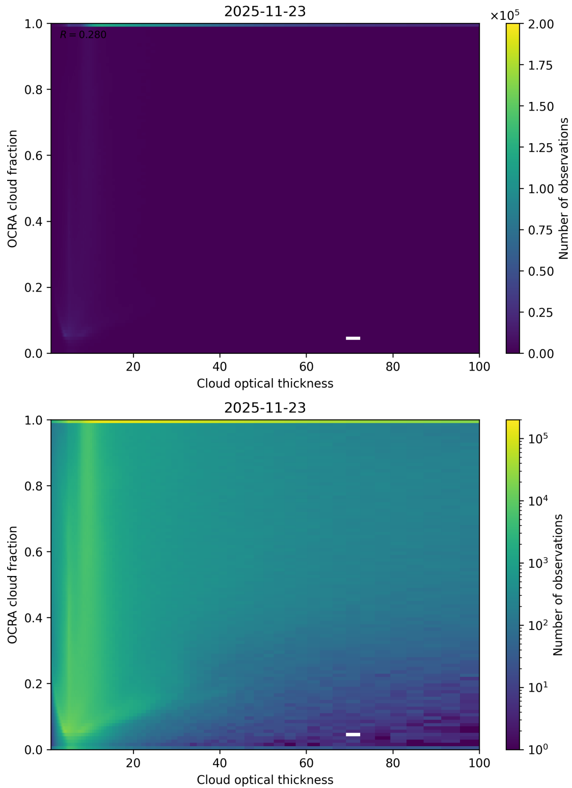
Figure 83: Scatter density plot of “Cloud optical thickness” against “OCRA cloud fraction” for 2025-11-23 to 2025-11-24.
