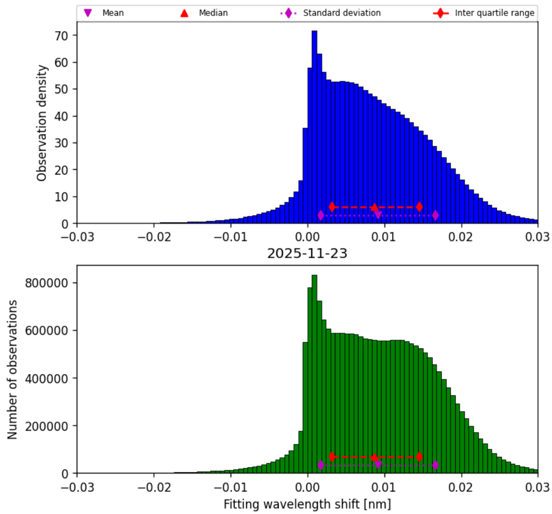
Figure 49: Histogram of “Fitting wavelength shift” for 2025-11-23 to 2025-11-24
