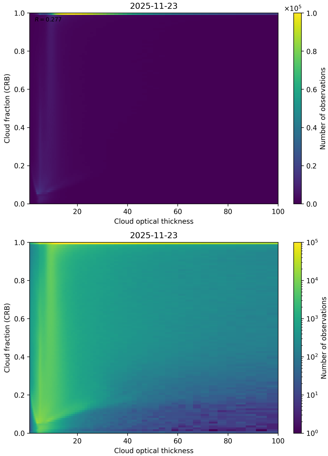
Figure 84: Scatter density plot of “Cloud optical thickness” against “Cloud fraction (CRB)” for 2025-11-23 to 2025-11-24.
