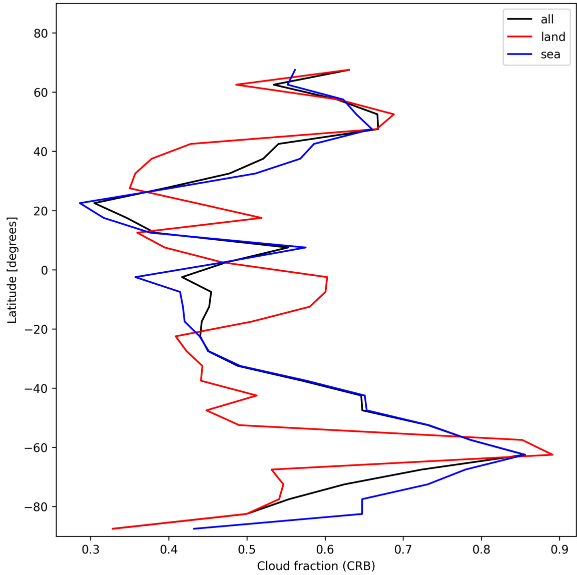
Figure 26: Zonal average of “Cloud fraction (CRB)” for 2025-11-23 to 2025-11-24.
