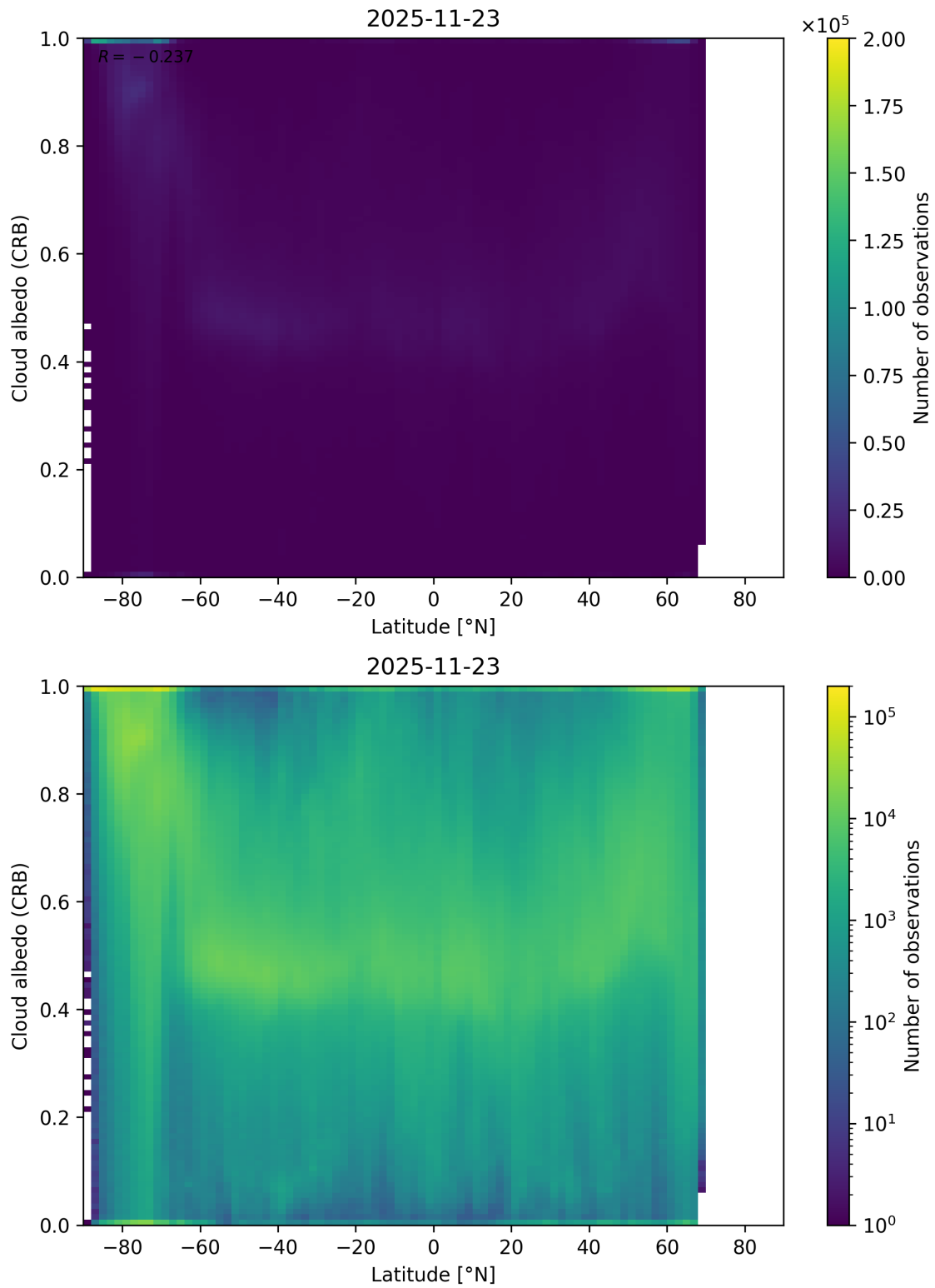
Figure 91: Scatter density plot of “Latitude” against “Cloud albedo (CRB)” for 2025-11-23 to 2025-11-24.
