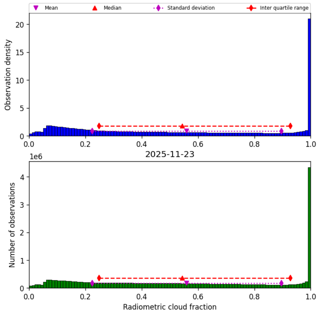
Figure 39: Histogram of “Radiometric cloud fraction” for 2025-11-23 to 2025-11-24
