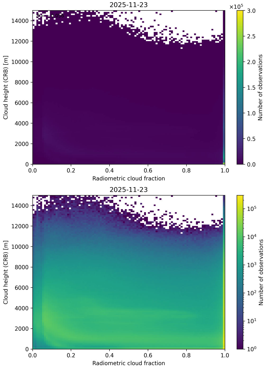
Figure 74: Scatter density plot of “Radiometric cloud fraction” against “Cloud height (CRB)” for 2025-11-23 to 2025-11-24.
