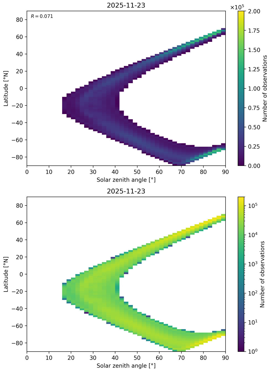
Figure 105: Scatter density plot of “Solar zenith angle” against “Latitude” for 2025-11-23 to 2025-11-24.
