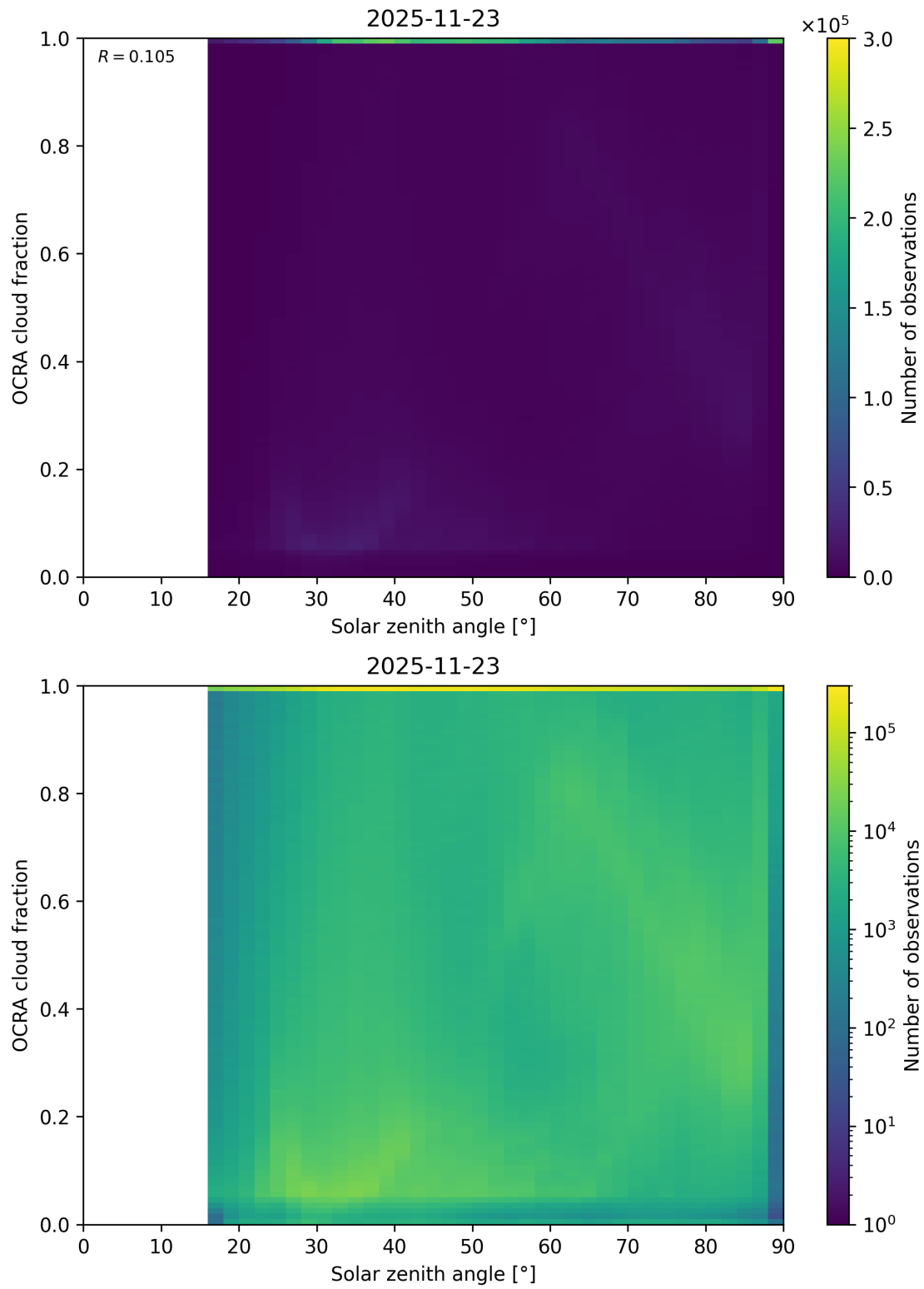
Figure 100: Scatter density plot of “Solar zenith angle” against “OCRA cloud fraction” for 2025-11-23 to 2025-11-24.
