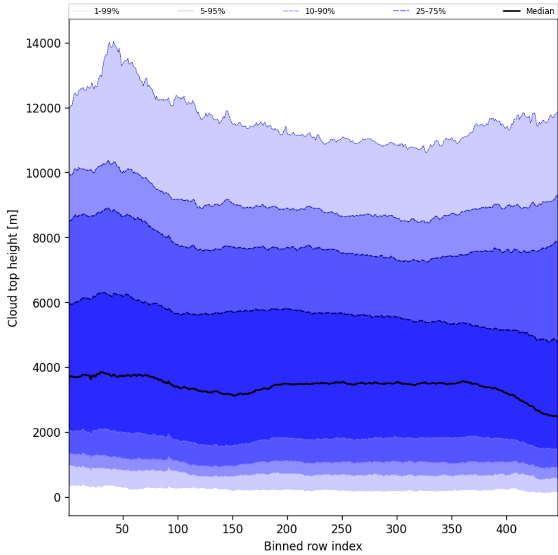
Figure 56: Along track statistics of “Cloud top height” for 2025-11-23 to 2025-11-24
