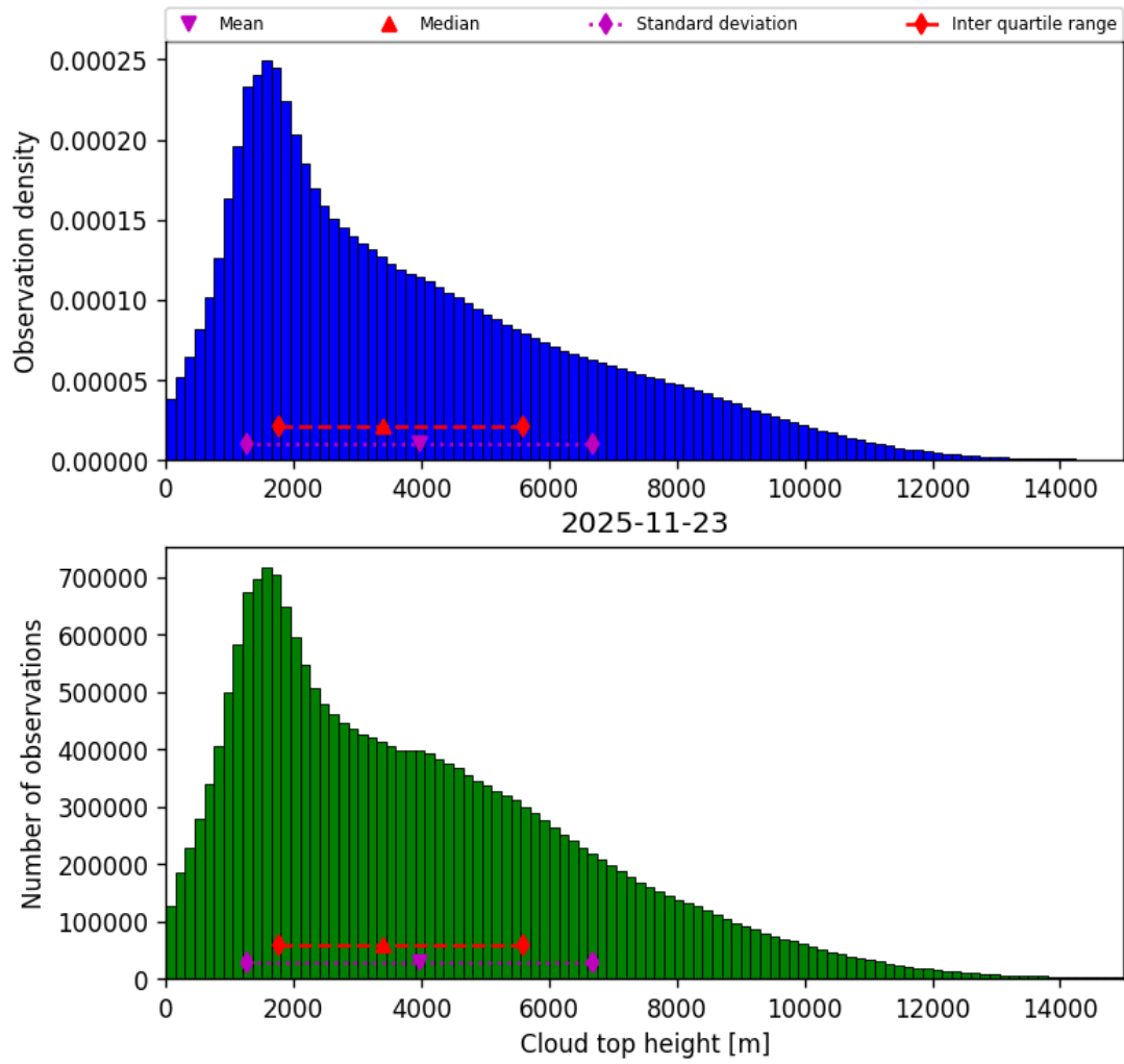
Figure 40: Histogram of “Cloud top height” for 2025-11-23 to 2025-11-24
