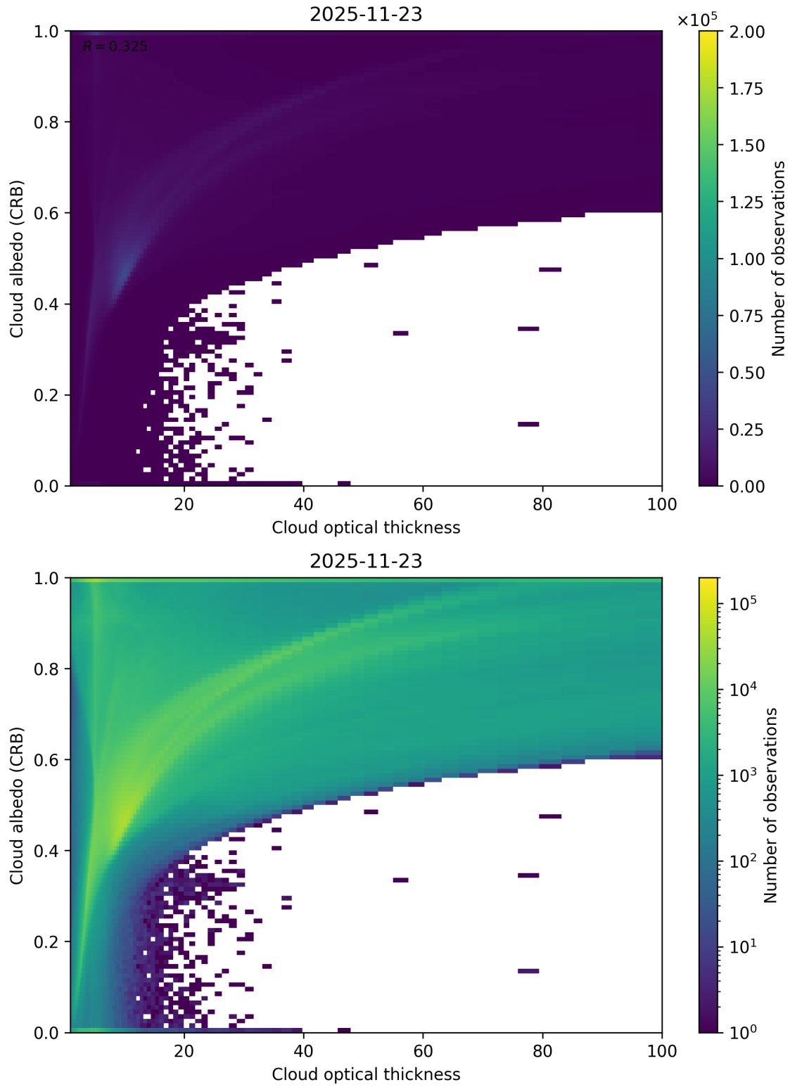
Figure 82: Scatter density plot of “Cloud optical thickness” against “Cloud albedo (CRB)” for 2025-11-23 to 2025-11-24.
