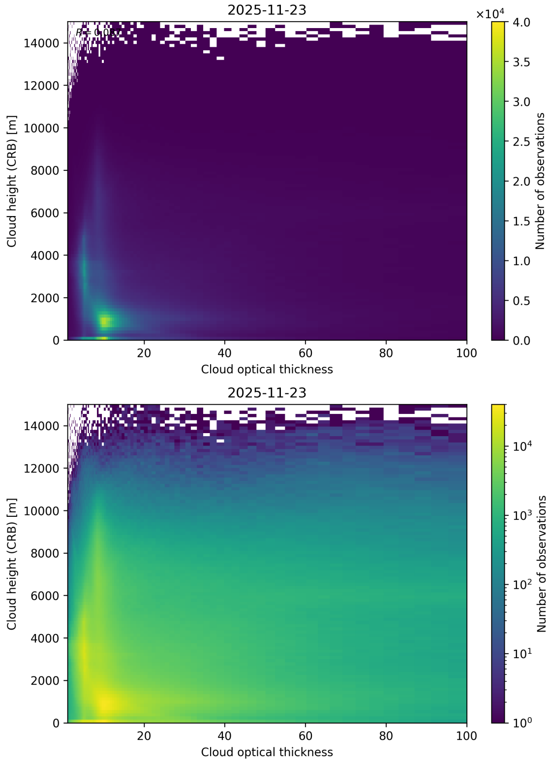
Figure 85: Scatter density plot of “Cloud optical thickness” against “Cloud height (CRB)” for 2025-11-23 to 2025-11-24.
