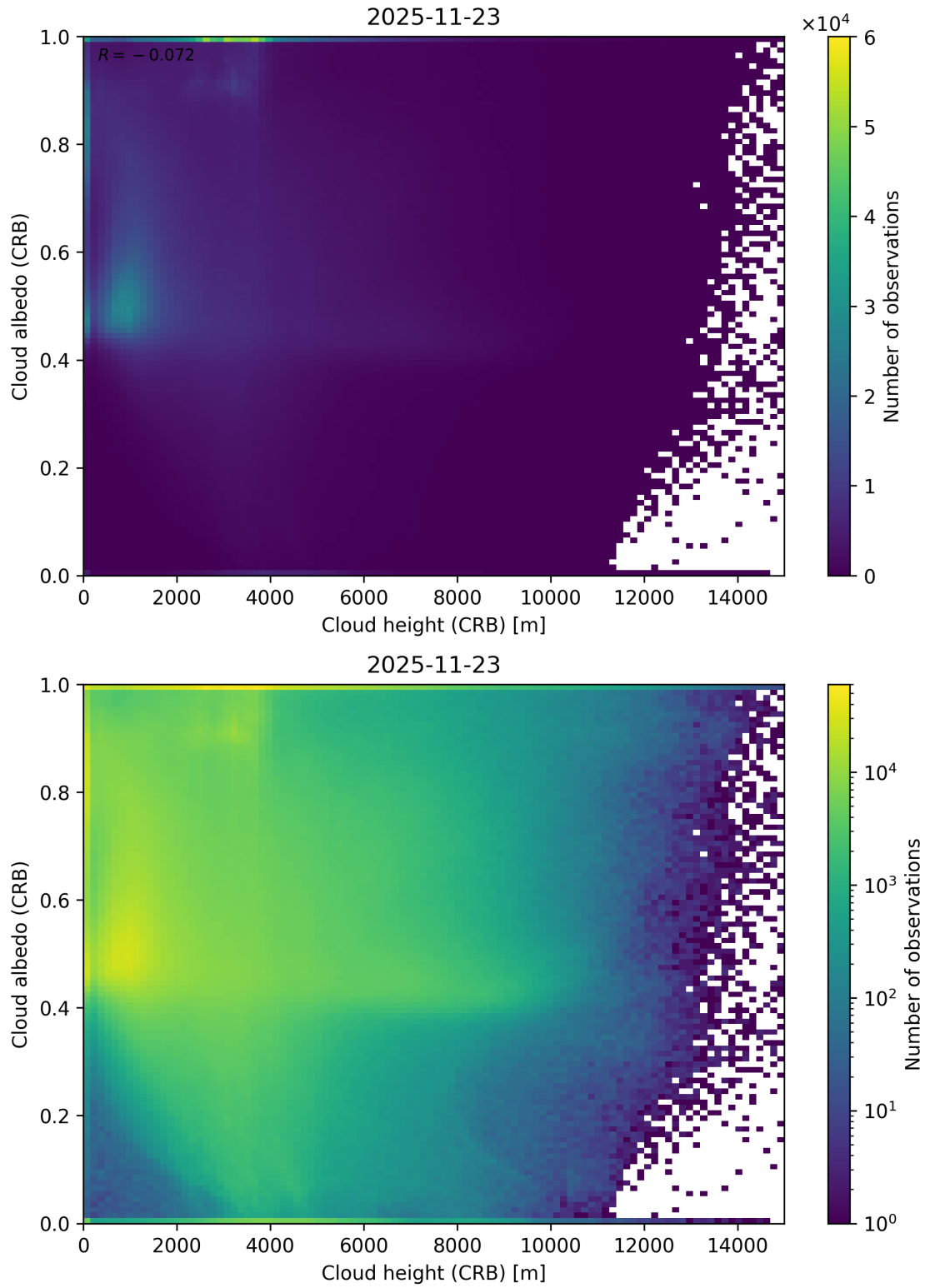
Figure 80: Scatter density plot of “Cloud height (CRB)” against “Cloud albedo (CRB)” for 2025-11-23 to 2025-11-24.
