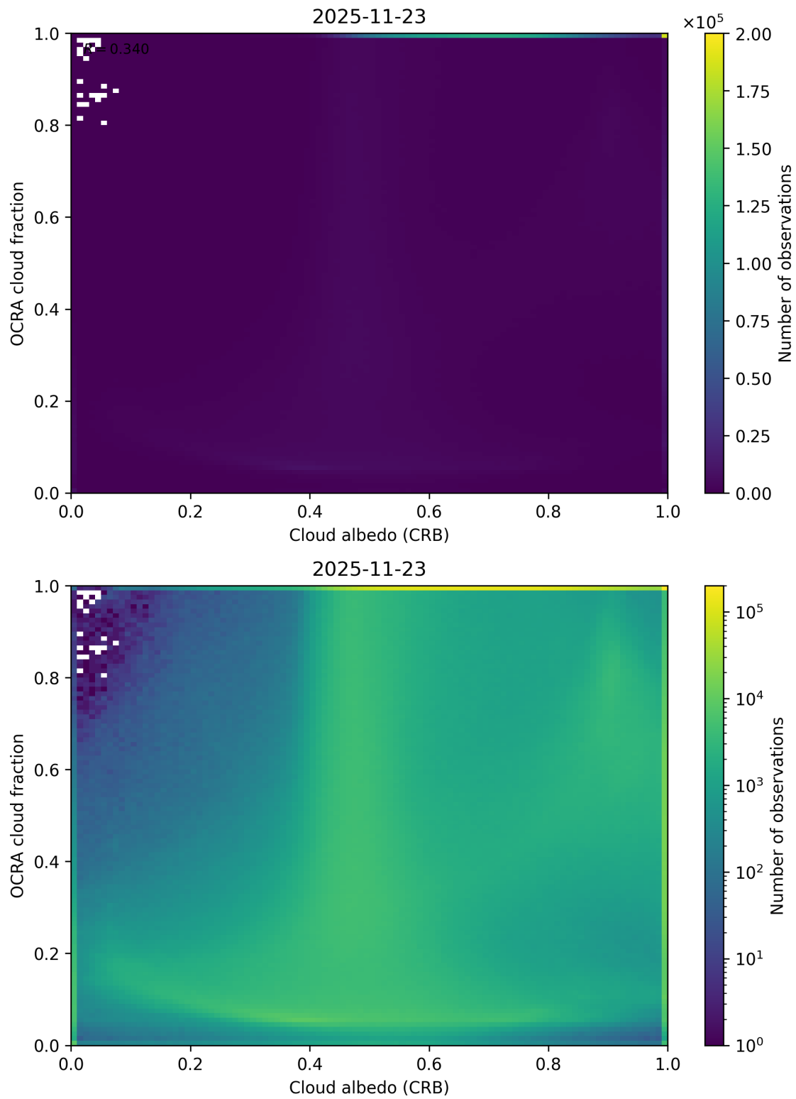
Figure 70: Scatter density plot of “Cloud albedo (CRB)” against “OCRA cloud fraction” for 2025-11-23 to 2025-11-24.
