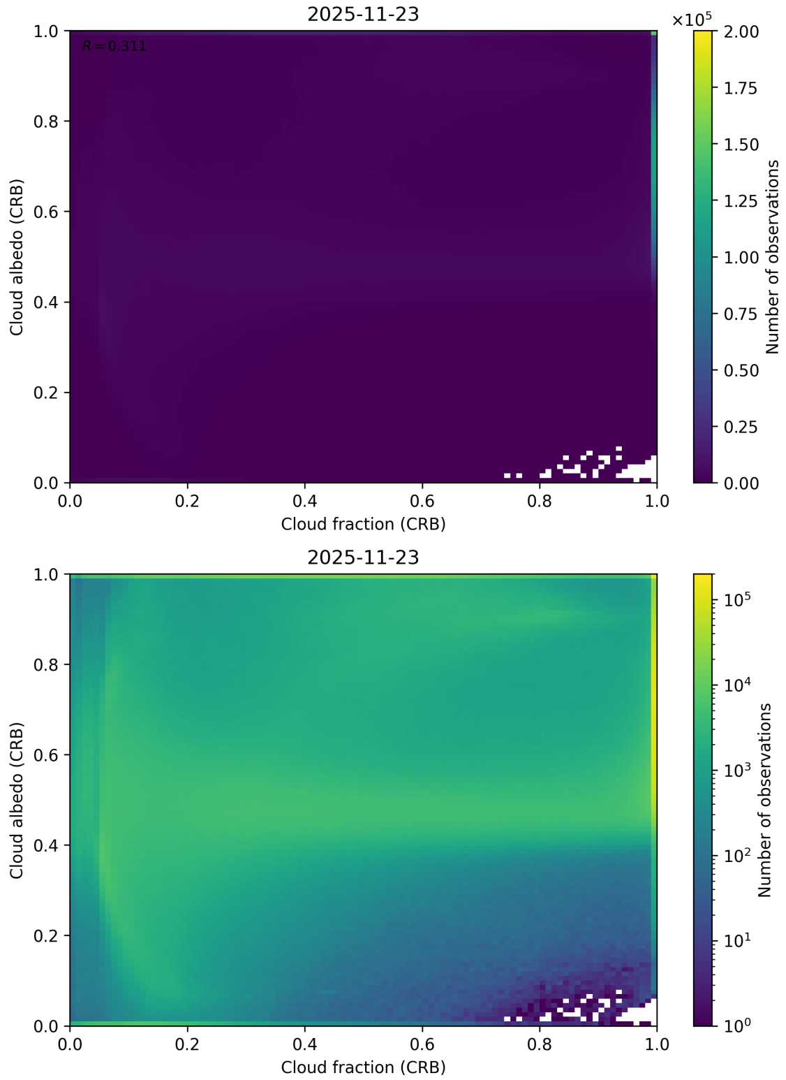
Figure 77: Scatter density plot of “Cloud fraction (CRB)” against “Cloud albedo (CRB)” for 2025-11-23 to 2025-11-24.
