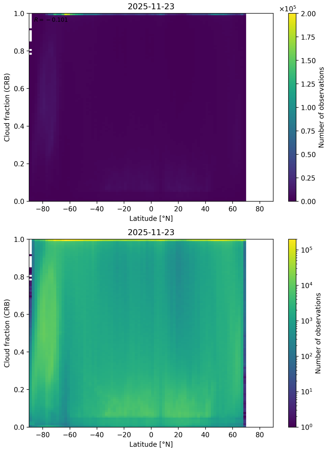
Figure 94: Scatter density plot of “Latitude” against “Cloud fraction (CRB)” for 2025-11-23 to 2025-11-24.
