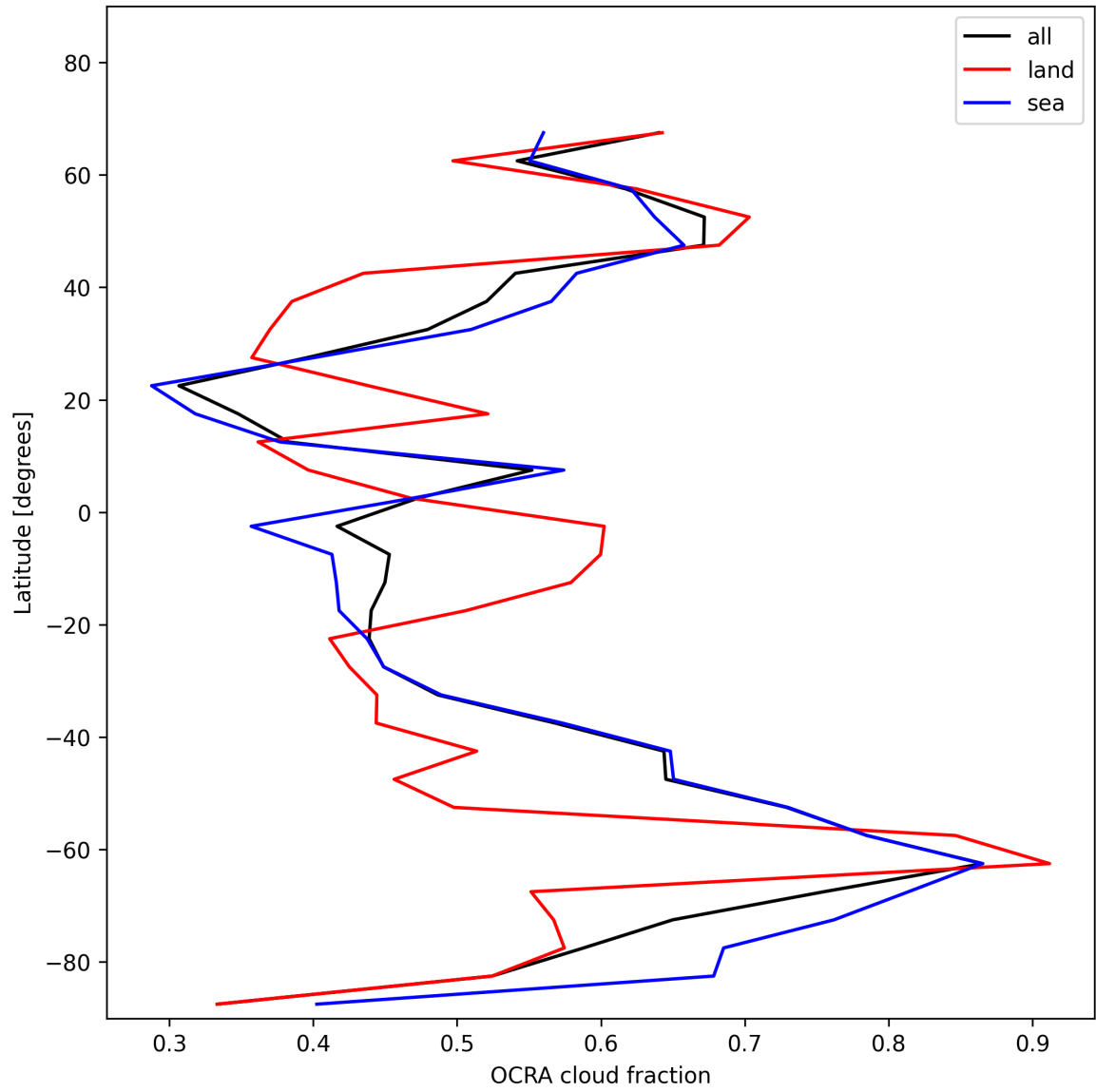
Figure 34: Zonal average of “OCRA cloud fraction” for 2025-11-23 to 2025-11-24.
