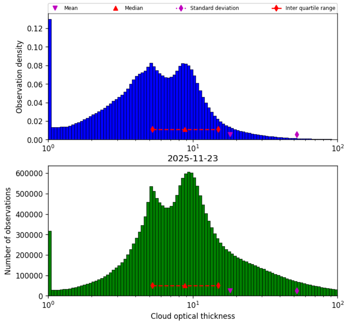
Figure 41: Histogram of “Cloud optical thickness” for 2025-11-23 to 2025-11-24
