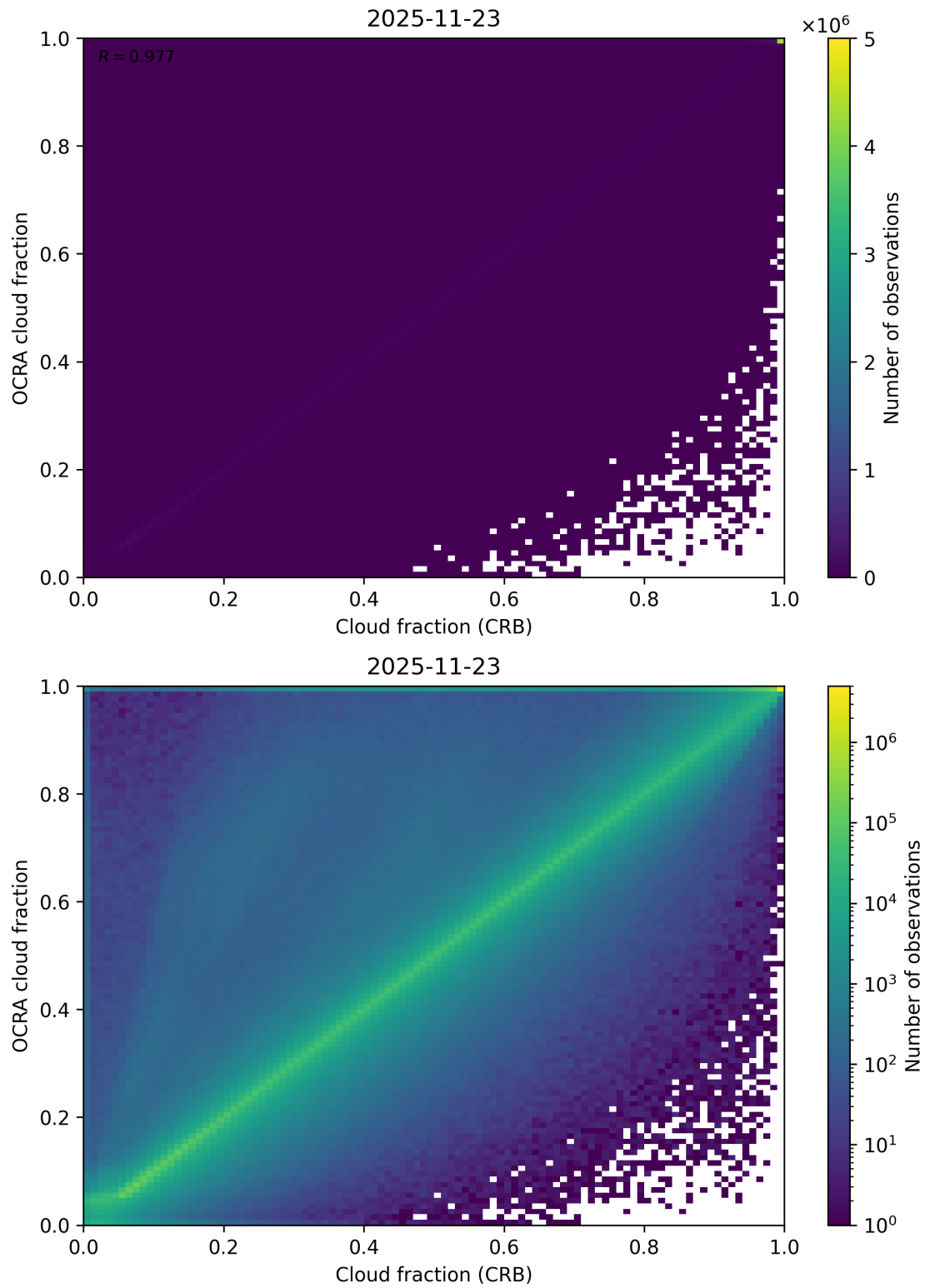
Figure 78: Scatter density plot of “Cloud fraction (CRB)” against “OCRA cloud fraction” for 2025-11-23 to 2025-11-24.
