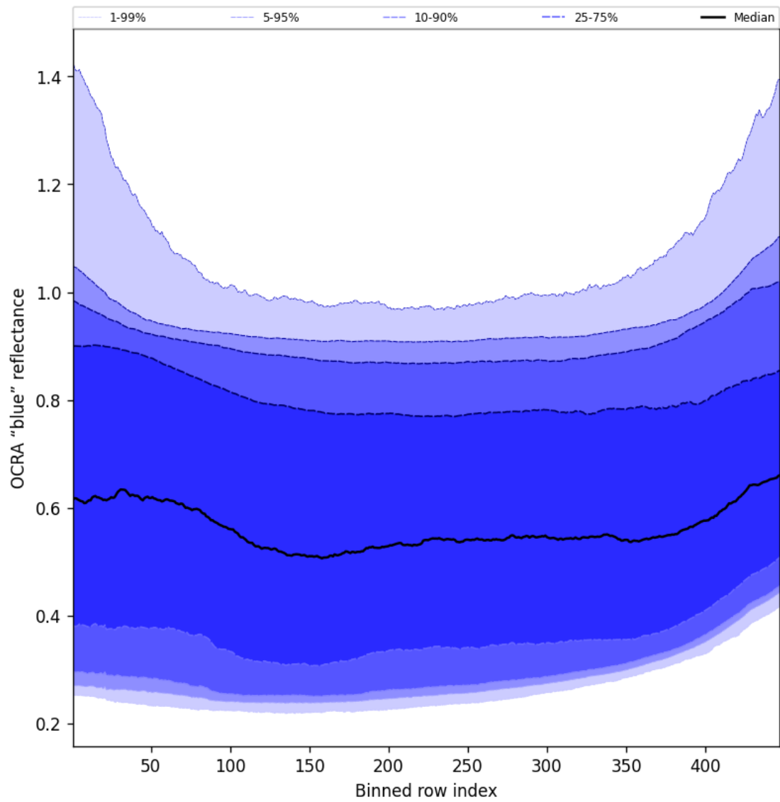
Figure 67: Along track statistics of “OCRA “blue” reflectance” for 2025-11-23 to 2025-11-24
