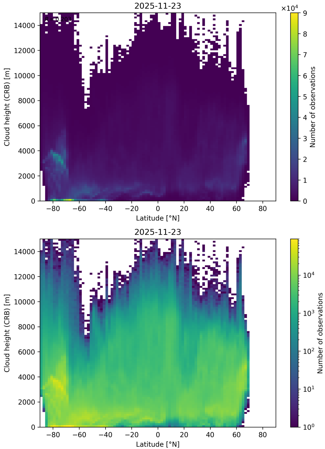
Figure 95: Scatter density plot of “Latitude” against “Cloud height (CRB)” for 2025-11-23 to 2025-11-24.
