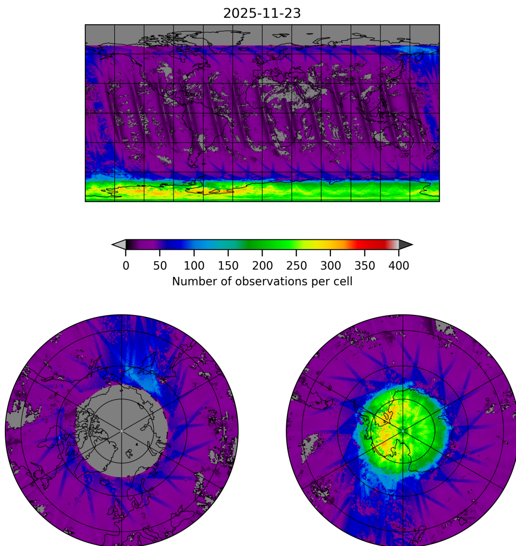
Figure 21: Map of the number of observations for 2025-11-23 to 2025-11-24
