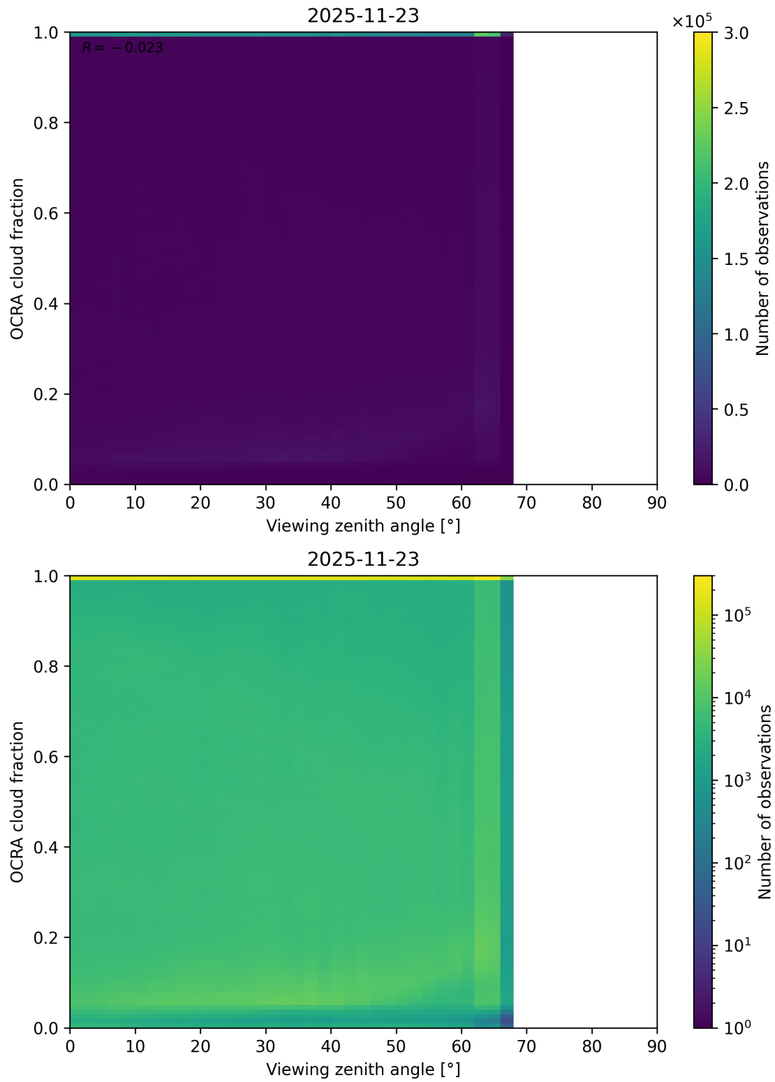
Figure 108: Scatter density plot of “Viewing zenith angle” against “OCRA cloud fraction” for 2025-11-23 to 2025-11-24.
