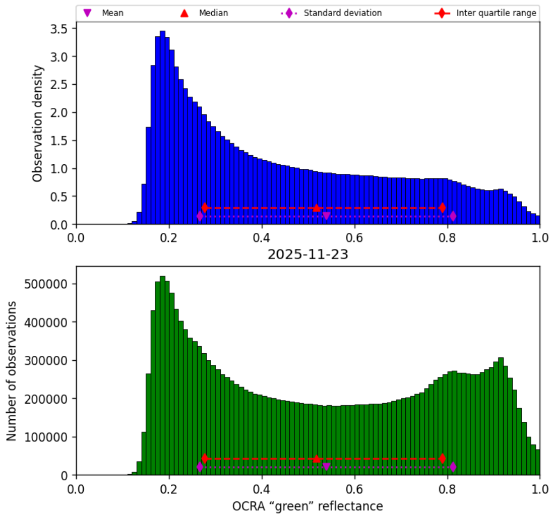
Figure 52: Histogram of “OCRA “green” reflectance” for 2025-11-23 to 2025-11-24
