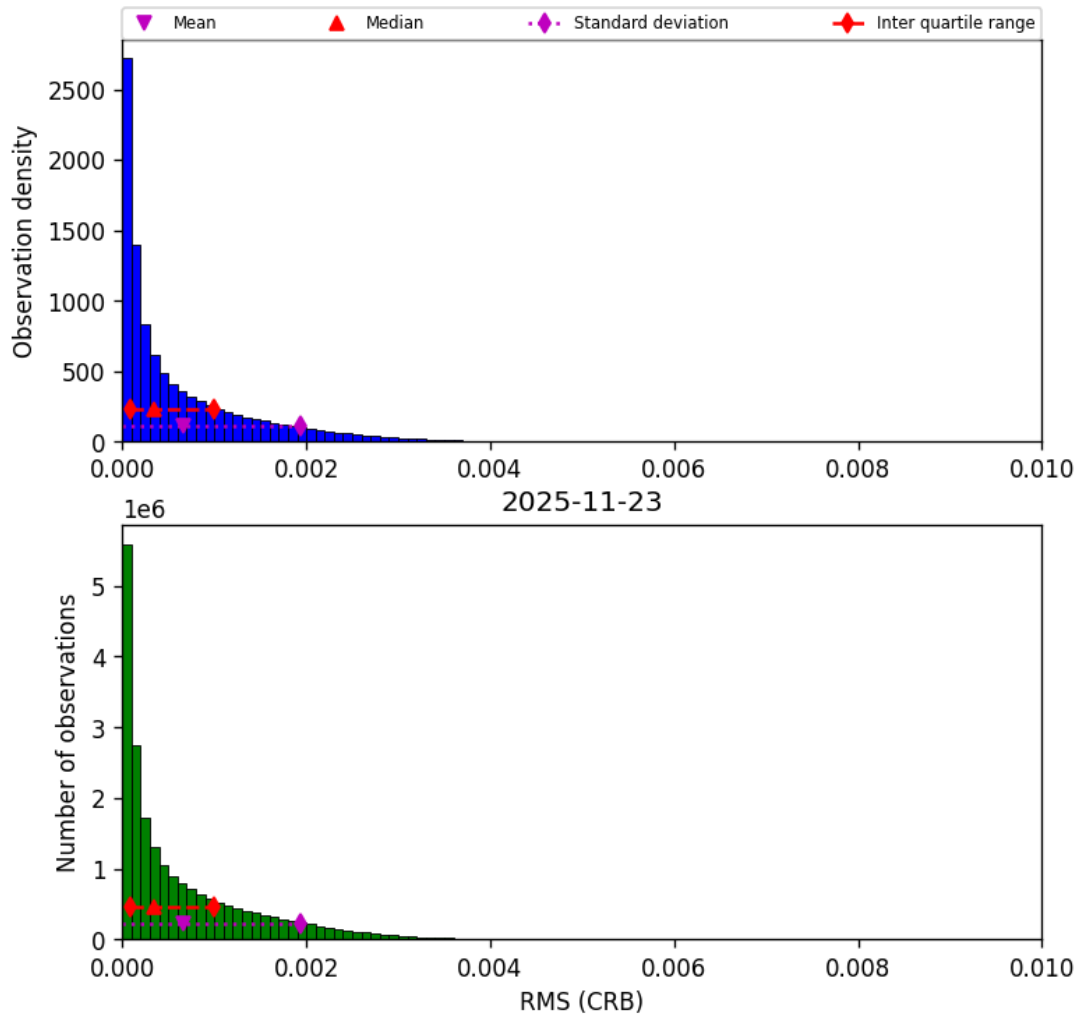
Figure 48: Histogram of “RMS (CRB)” for 2025-11-23 to 2025-11-24
