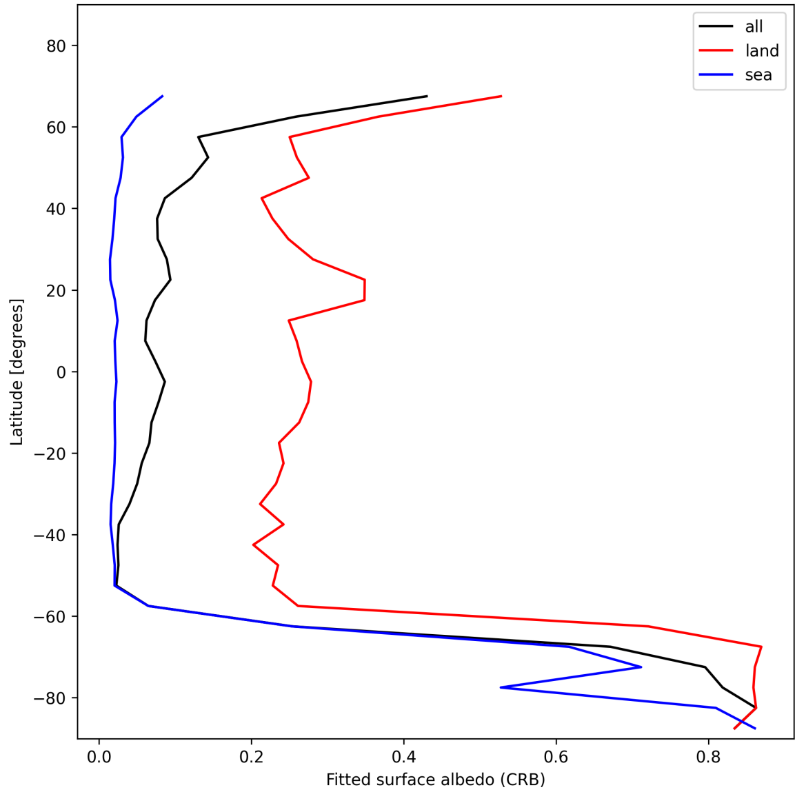
Figure 30: Zonal average of “Fitted surface albedo (CRB)” for 2025-11-23 to 2025-11-24.
