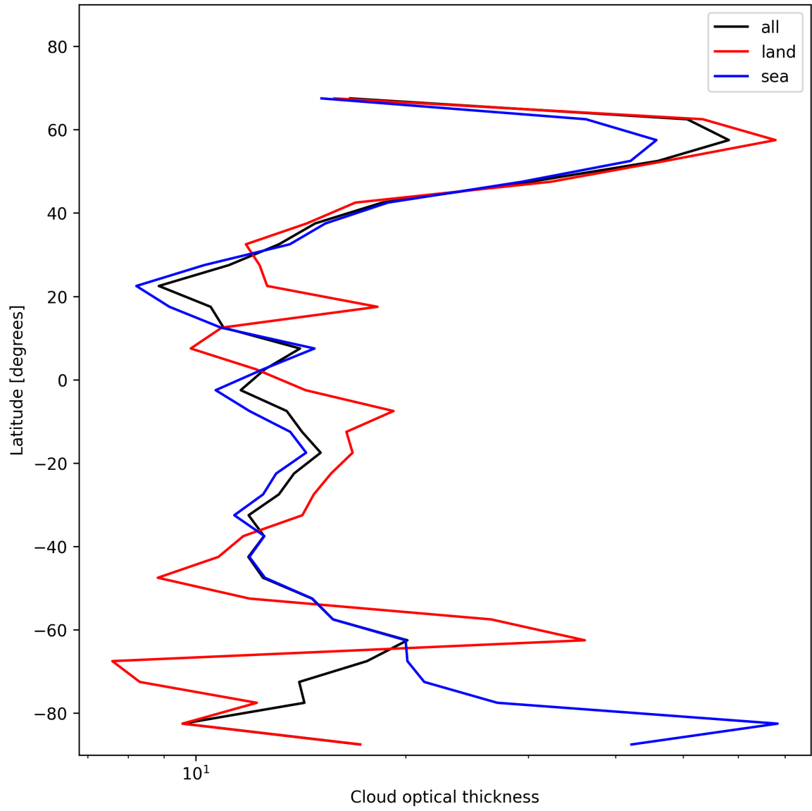
Figure 25: Zonal average of “Cloud optical thickness” for 2025-11-23 to 2025-11-24.
