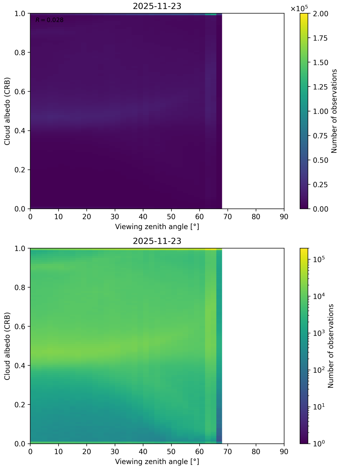
Figure 106: Scatter density plot of “Viewing zenith angle” against “Cloud albedo (CRB)” for 2025-11-23 to 2025-11-24.
