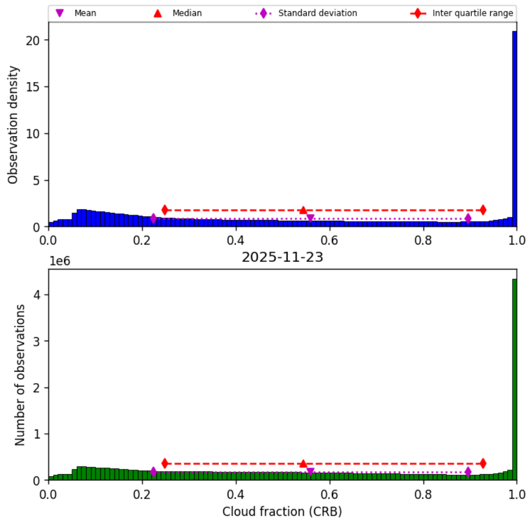
Figure 42: Histogram of “Cloud fraction (CRB)” for 2025-11-23 to 2025-11-24
