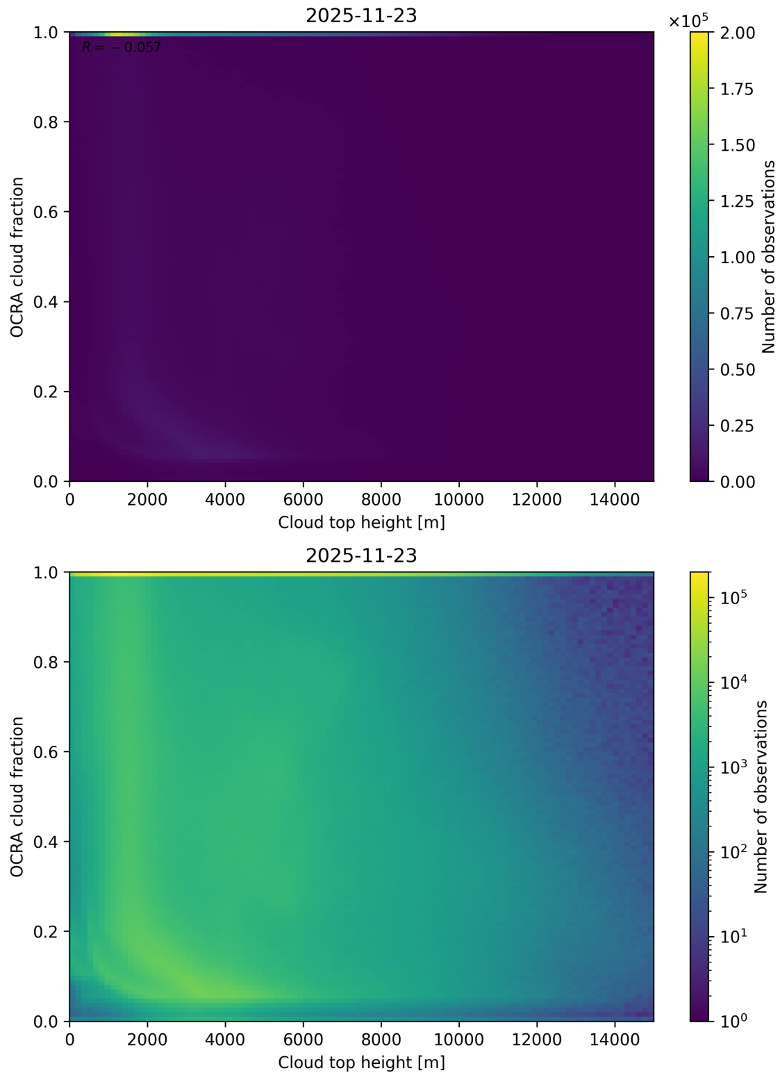
Figure 87: Scatter density plot of “Cloud top height” against “OCRA cloud fraction” for 2025-11-23 to 2025-11-24.
