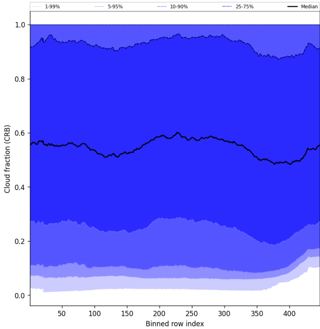
Figure 58: Along track statistics of “Cloud fraction (CRB)” for 2025-11-23 to 2025-11-24
