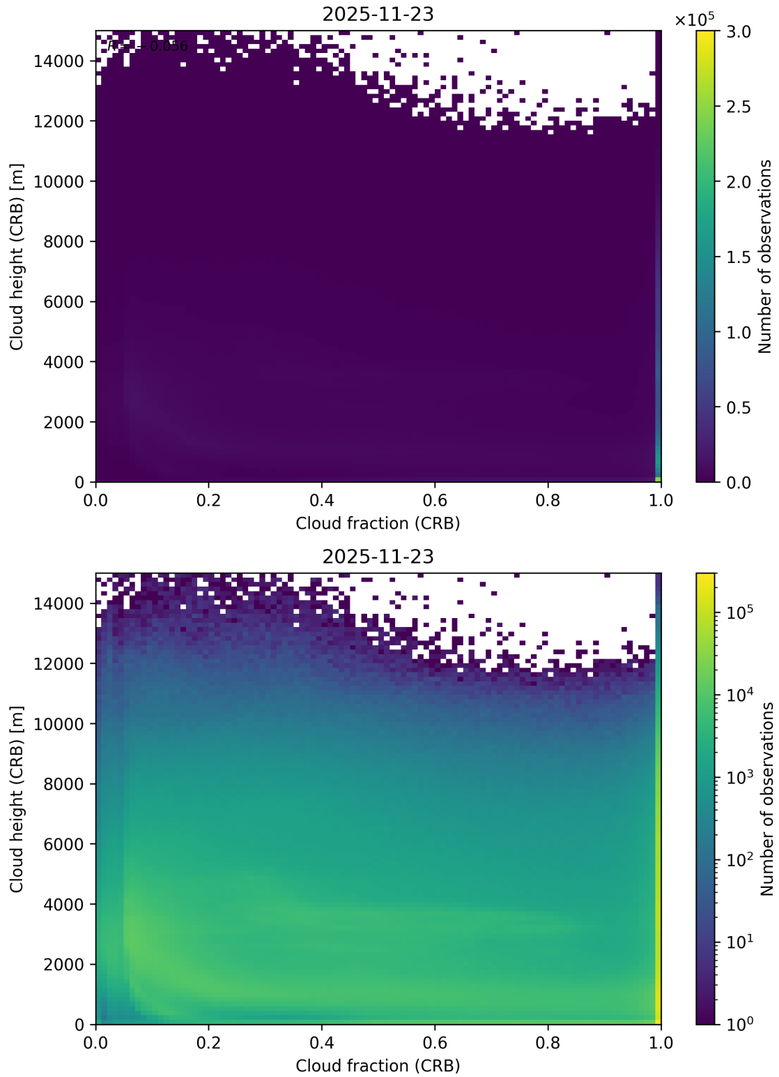
Figure 79: Scatter density plot of “Cloud fraction (CRB)” against “Cloud height (CRB)” for 2025-11-23 to 2025-11-24.
