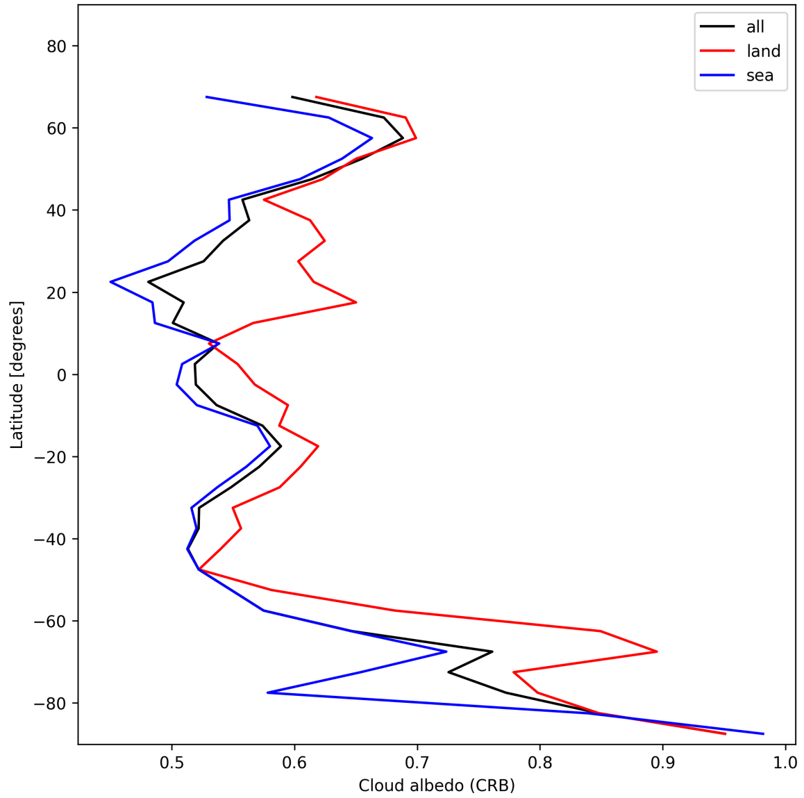
Figure 28: Zonal average of “Cloud albedo (CRB)” for 2025-11-23 to 2025-11-24.
