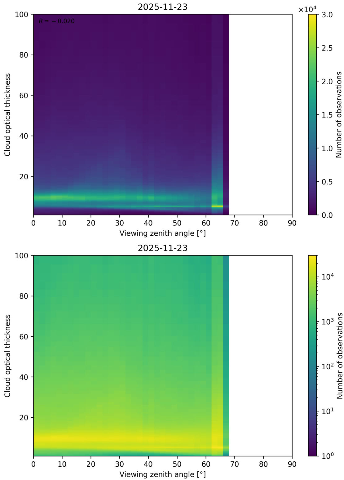
Figure 111: Scatter density plot of “Viewing zenith angle” against “Cloud optical thickness” for 2025-11-23 to 2025-11-24.
