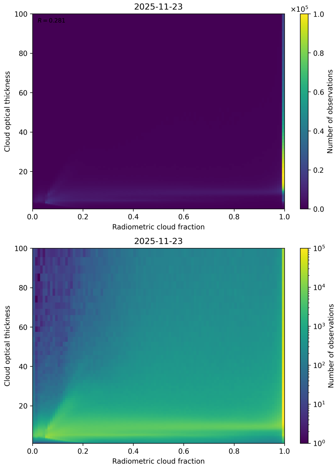
Figure 75: Scatter density plot of “Radiometric cloud fraction” against “Cloud optical thickness” for 2025-11-23 to 2025-11-24.
