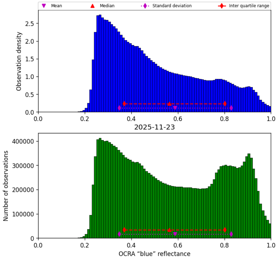
Figure 51: Histogram of “OCRA “blue” reflectance” for 2025-11-23 to 2025-11-24
