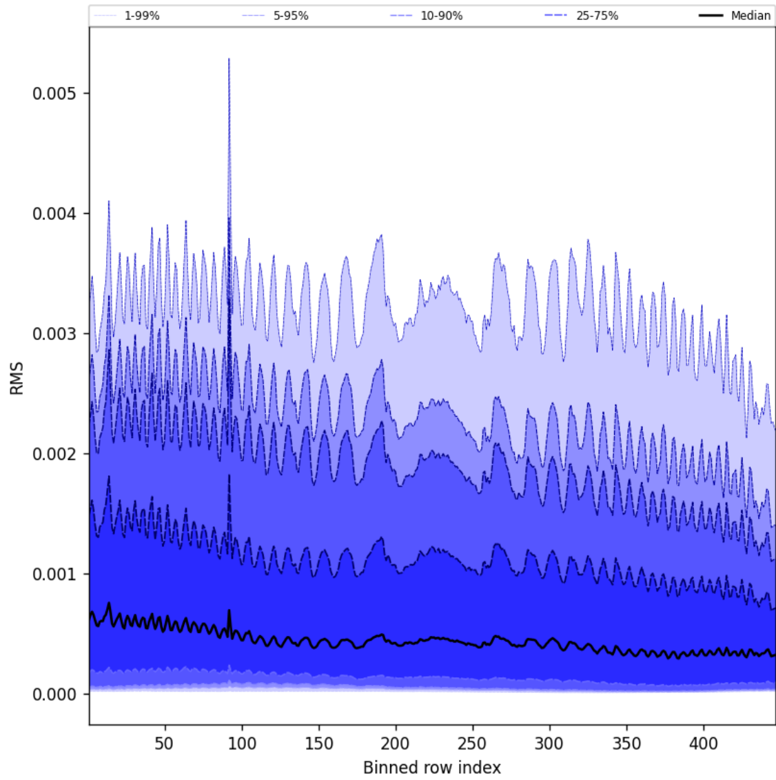
Figure 63: Along track statistics of “RMS” for 2025-11-23 to 2025-11-24
