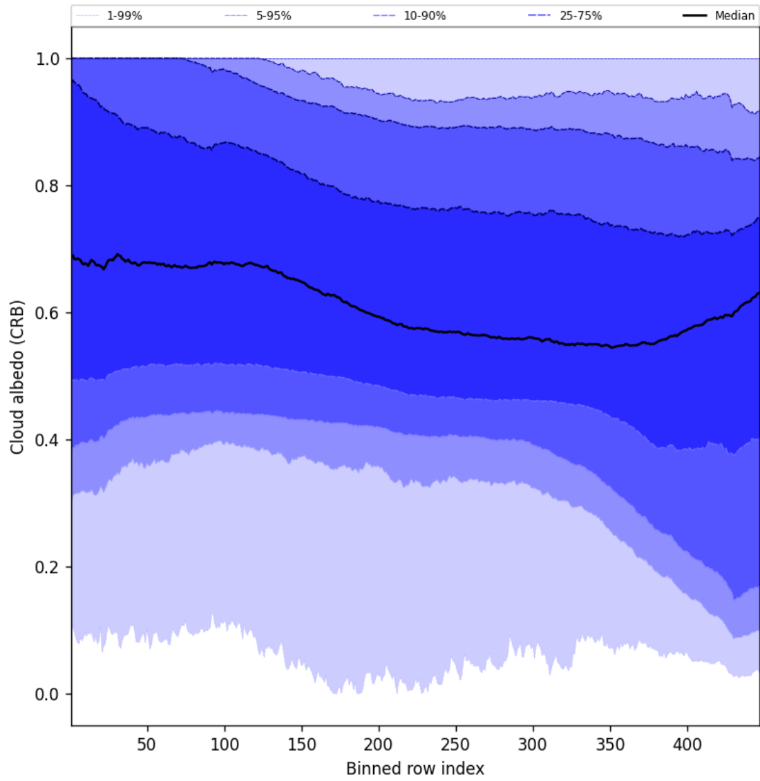
Figure 60: Along track statistics of “Cloud albedo (CRB)” for 2025-11-23 to 2025-11-25
