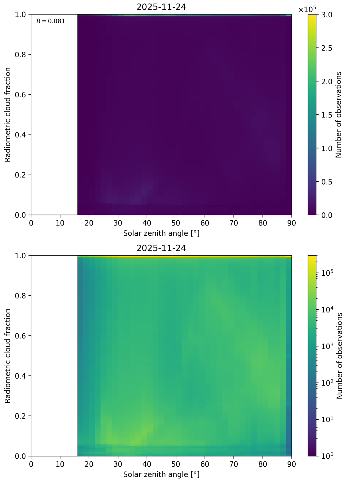
Figure 99: Scatter density plot of “Solar zenith angle” against “Radiometric cloud fraction” for 2025-11-23 to 2025-11-25.
