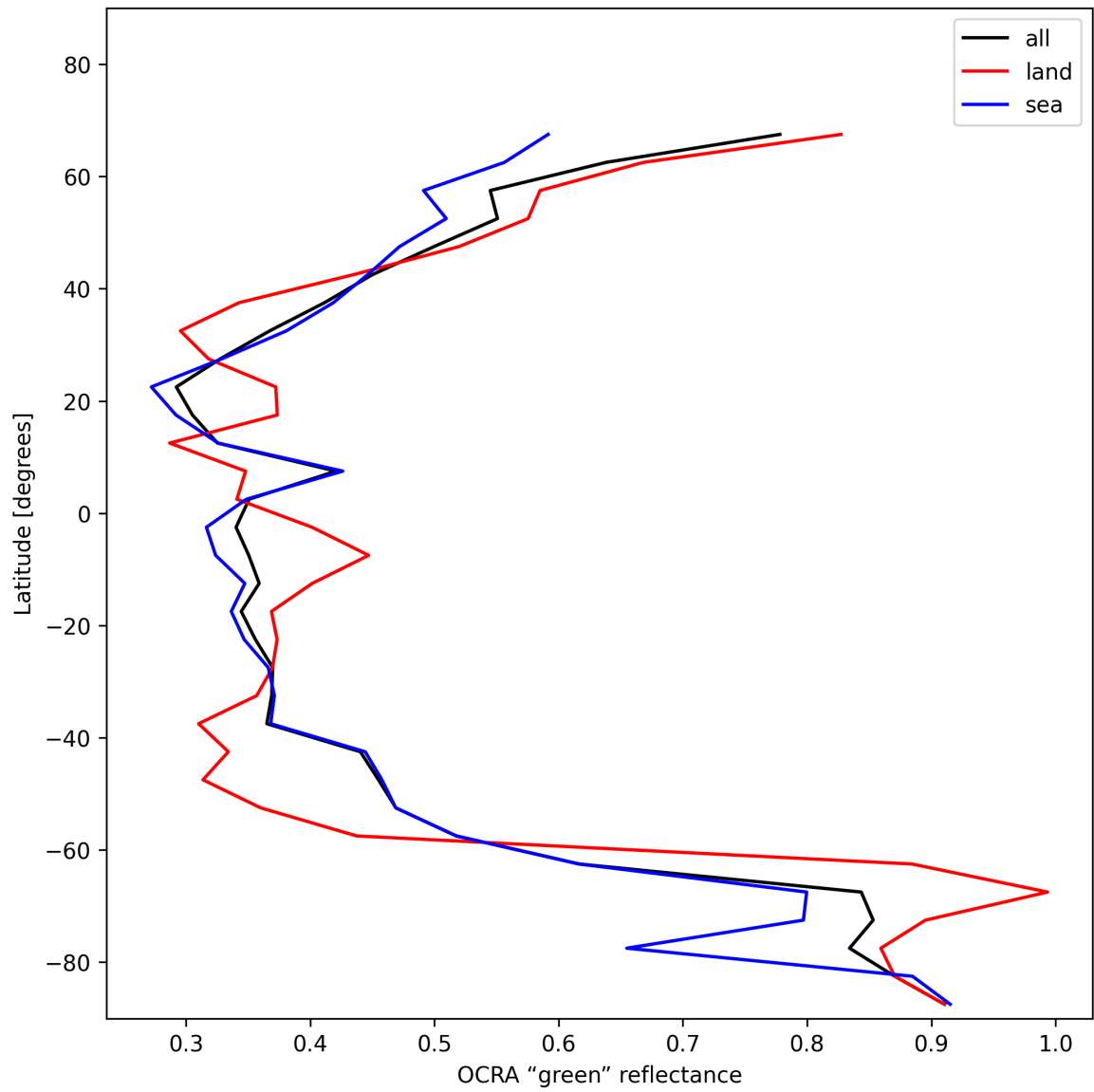
Figure 36: Zonal average of “OCRA “green” reflectance” for 2025-11-23 to 2025-11-25.
