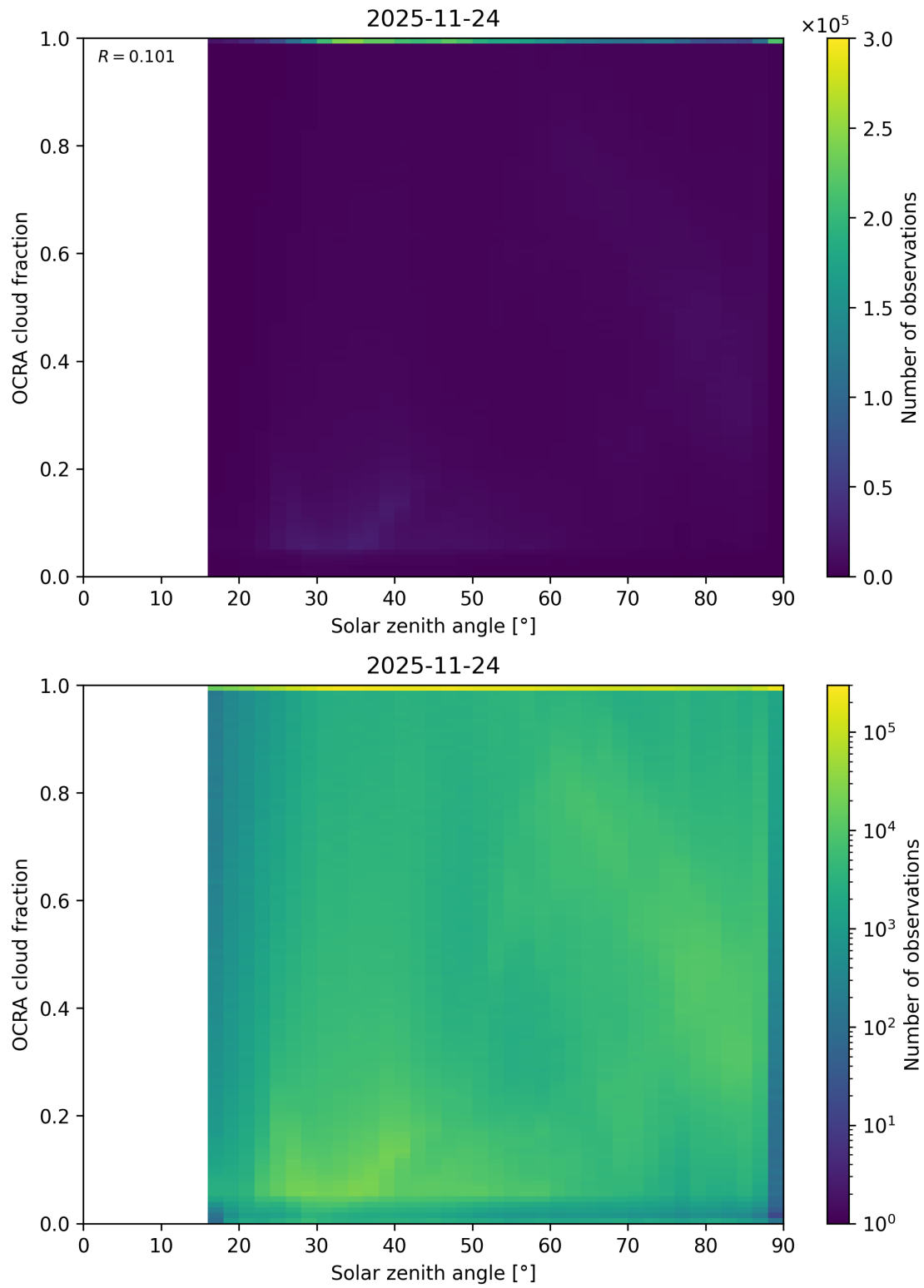
Figure 100: Scatter density plot of “Solar zenith angle” against “OCRA cloud fraction” for 2025-11-23 to 2025-11-25.
