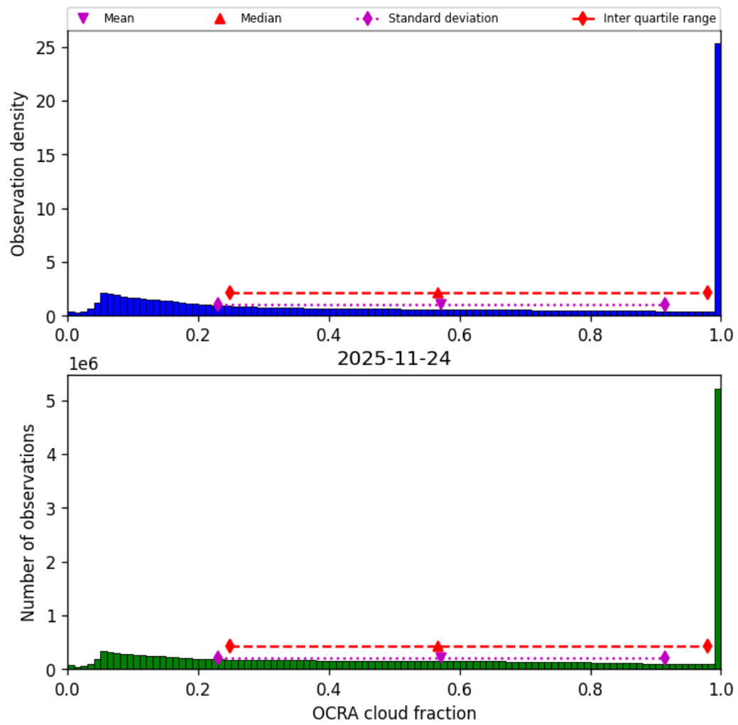
Figure 50: Histogram of “OCRA cloud fraction” for 2025-11-23 to 2025-11-25
