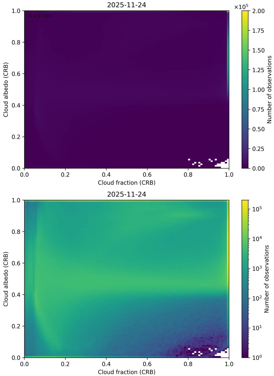
Figure 77: Scatter density plot of “Cloud fraction (CRB)” against “Cloud albedo (CRB)” for 2025-11-23 to 2025-11-25.
