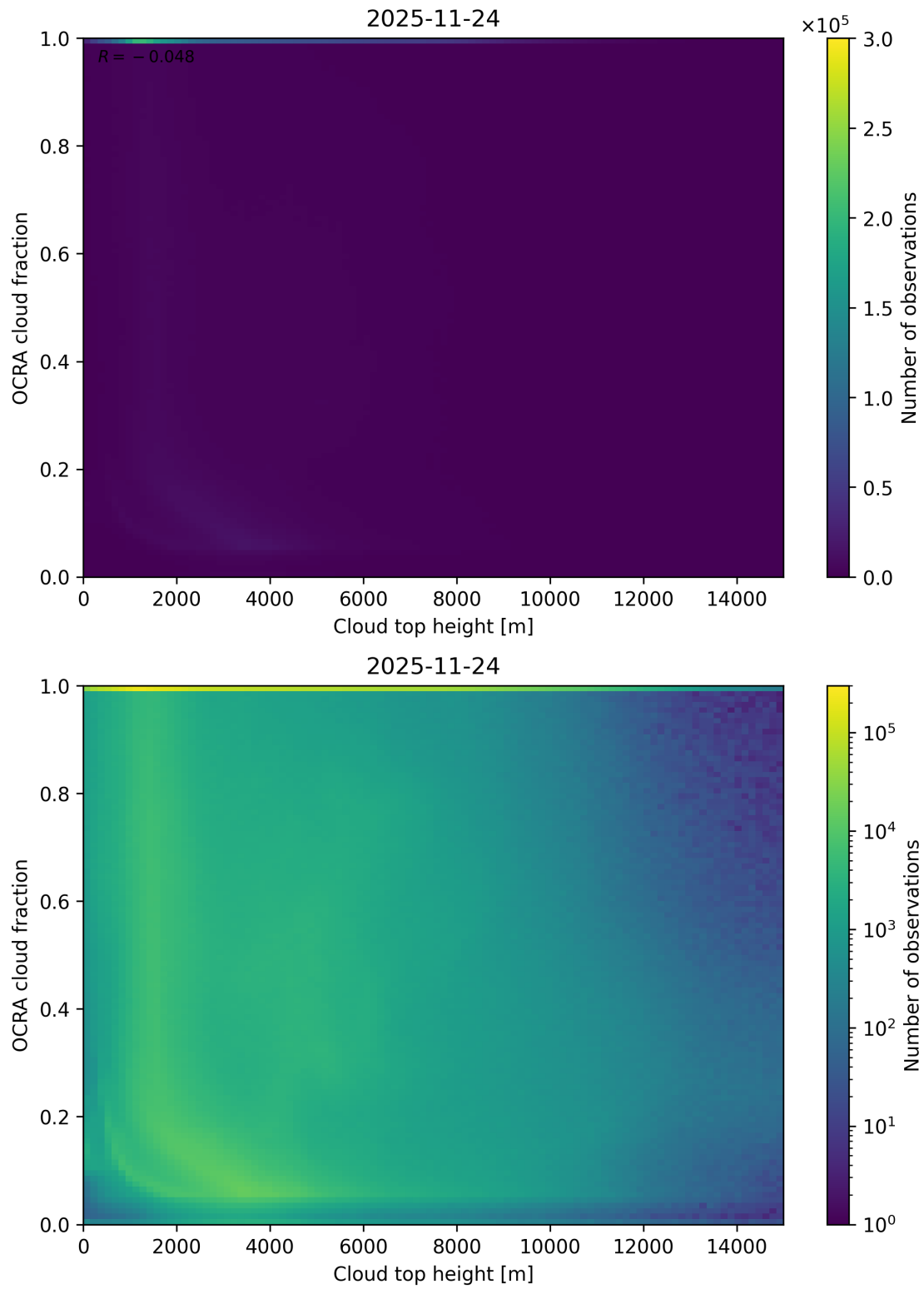
Figure 87: Scatter density plot of “Cloud top height” against “OCRA cloud fraction” for 2025-11-23 to 2025-11-25.
