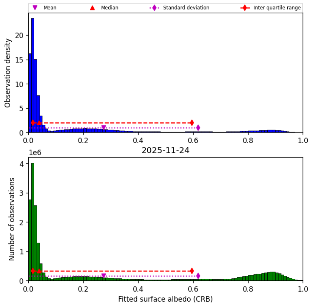
Figure 46: Histogram of “Fitted surface albedo (CRB)” for 2025-11-23 to 2025-11-25
