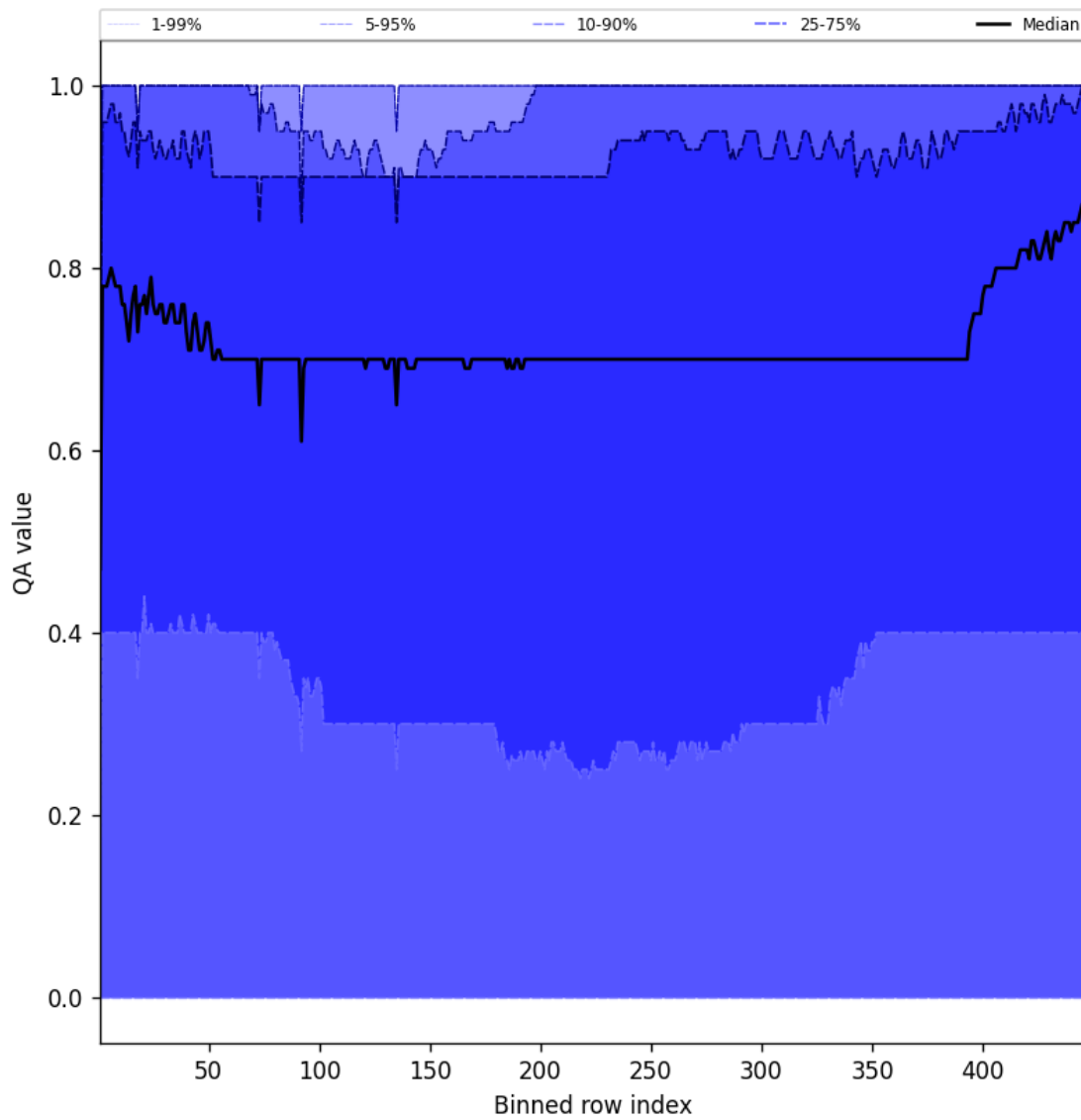
Figure 54: Along track statistics of “QA value” for 2025-11-23 to 2025-11-25
