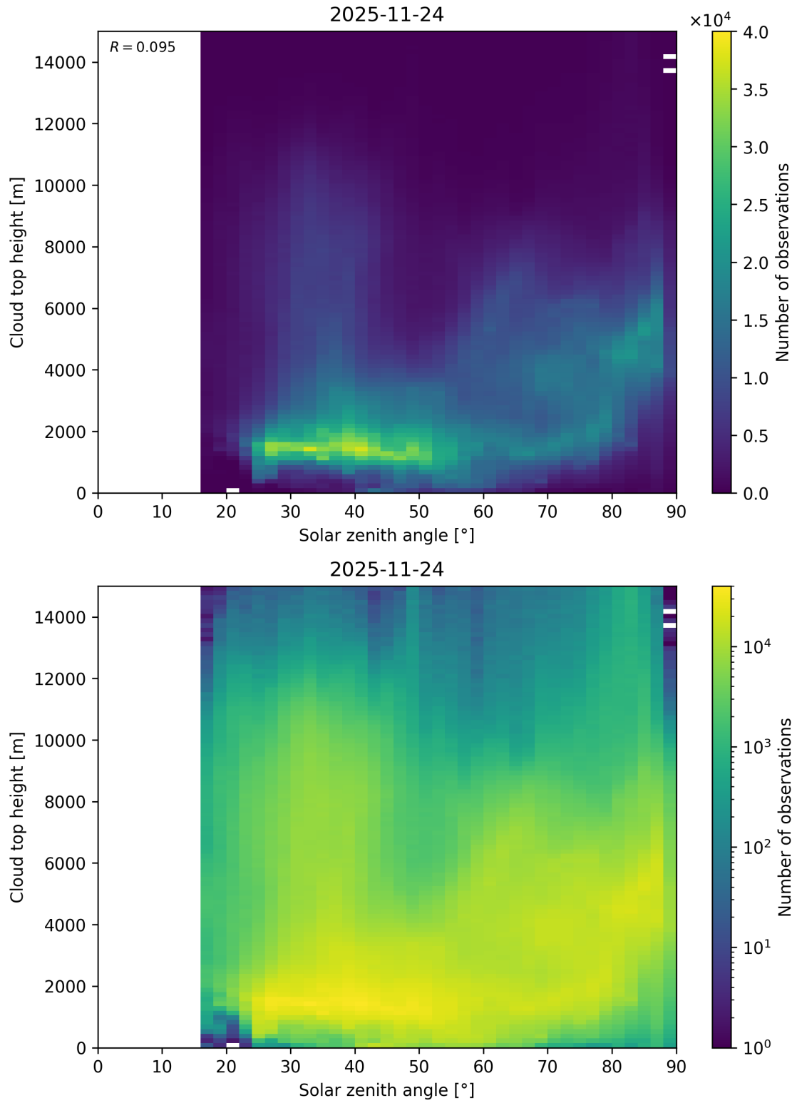
Figure 104: Scatter density plot of “Solar zenith angle” against “Cloud top height” for 2025-11-23 to 2025-11-25.
