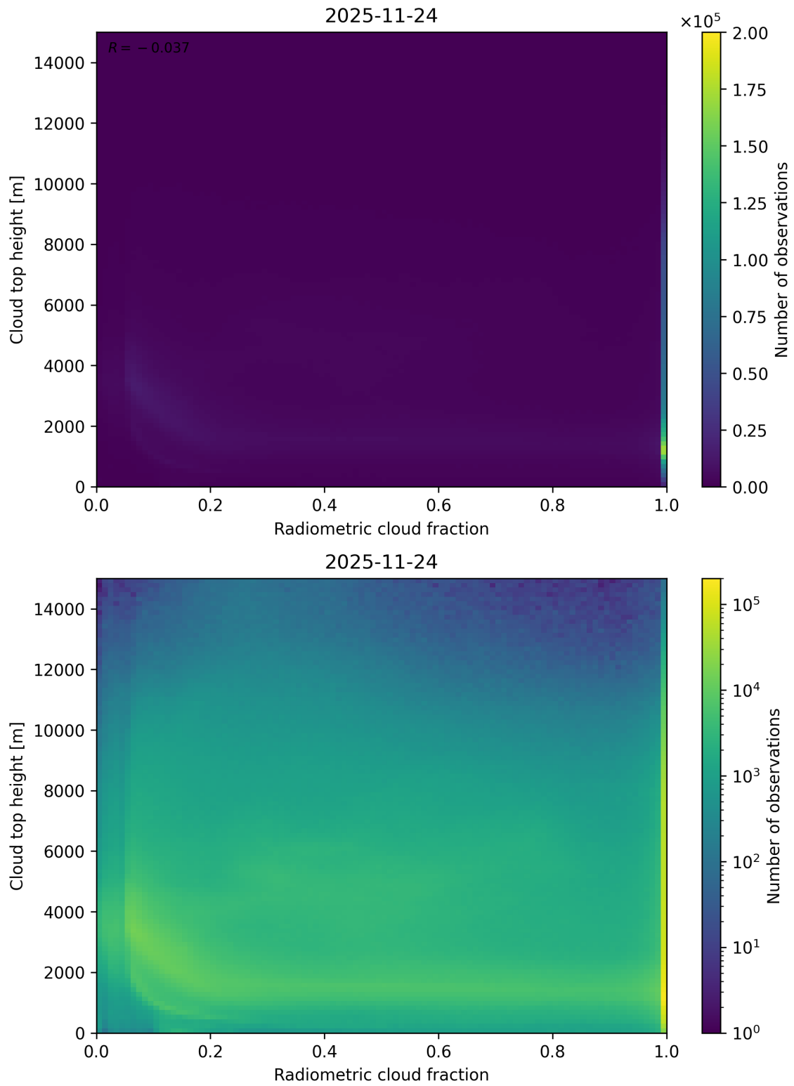
Figure 76: Scatter density plot of “Radiometric cloud fraction” against “Cloud top height” for 2025-11-23 to 2025-11-25.
