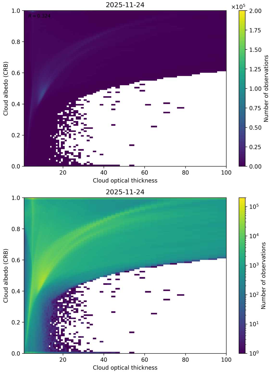
Figure 82: Scatter density plot of “Cloud optical thickness” against “Cloud albedo (CRB)” for 2025-11-23 to 2025-11-25.
