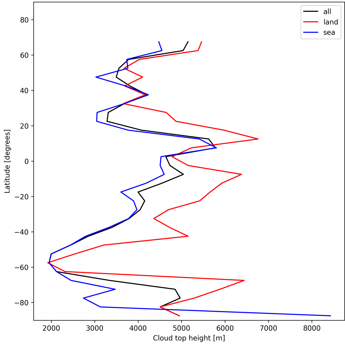
Figure 24: Zonal average of “Cloud top height” for 2025-11-23 to 2025-11-25.
