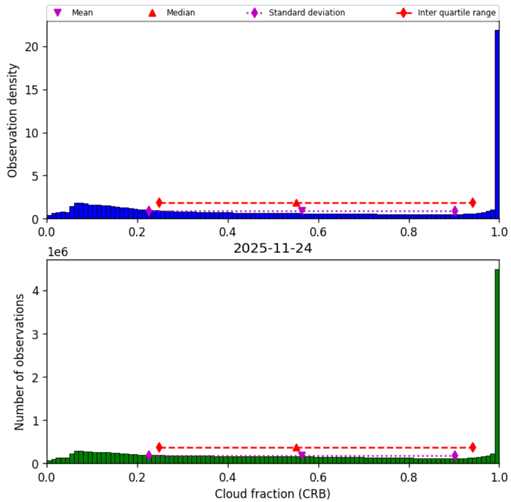
Figure 42: Histogram of “Cloud fraction (CRB)” for 2025-11-23 to 2025-11-25
