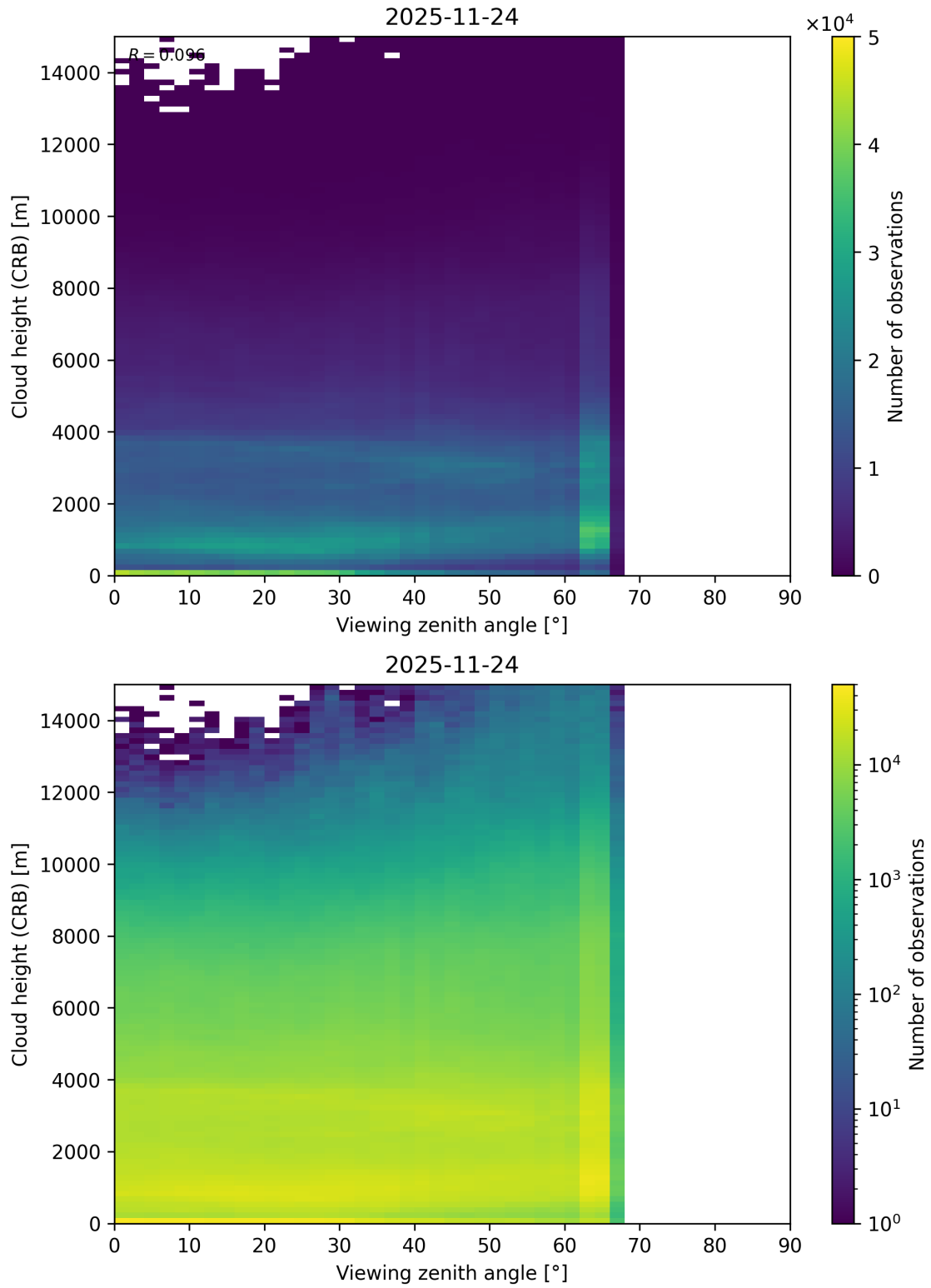
Figure 110: Scatter density plot of “Viewing zenith angle” against “Cloud height (CRB)” for 2025-11-23 to 2025-11-25.
