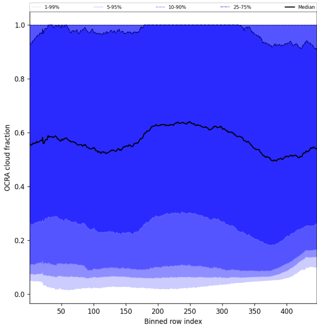
Figure 66: Along track statistics of “OCRA cloud fraction” for 2025-11-23 to 2025-11-25
