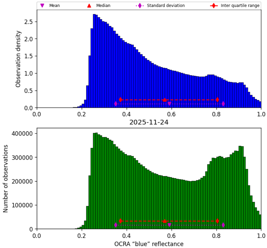
Figure 51: Histogram of “OCRA “blue” reflectance” for 2025-11-23 to 2025-11-25
