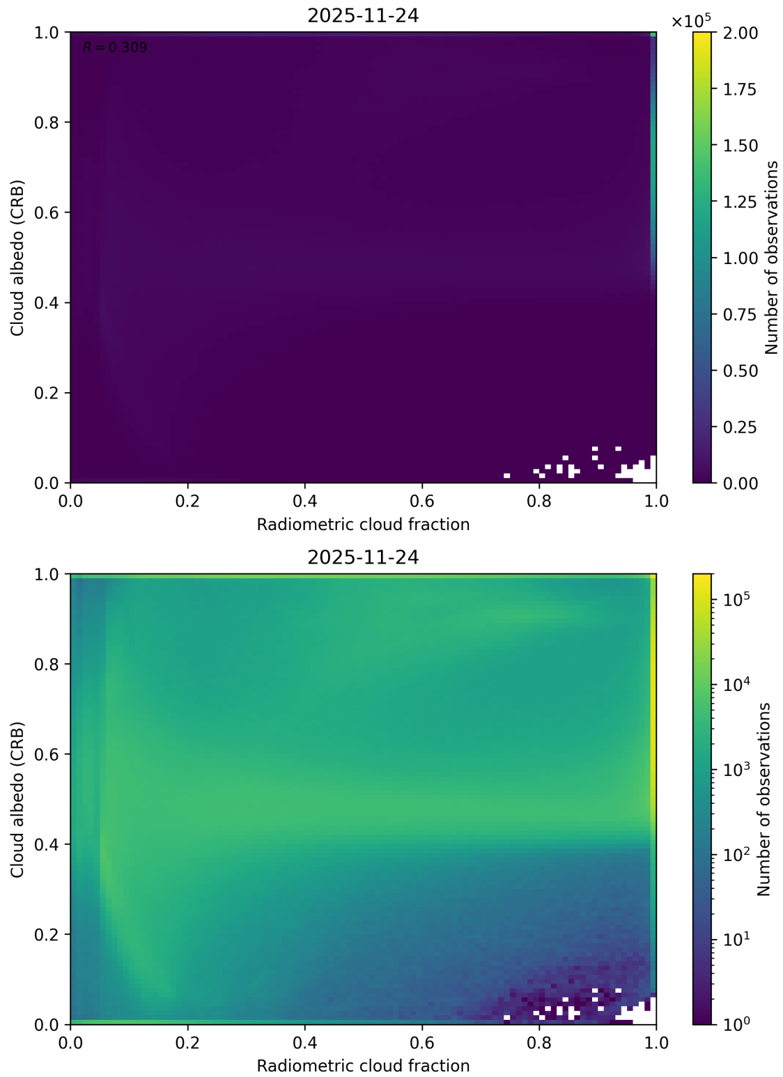
Figure 71: Scatter density plot of “Radiometric cloud fraction” against “Cloud albedo (CRB)” for 2025-11-23 to 2025-11-25.
