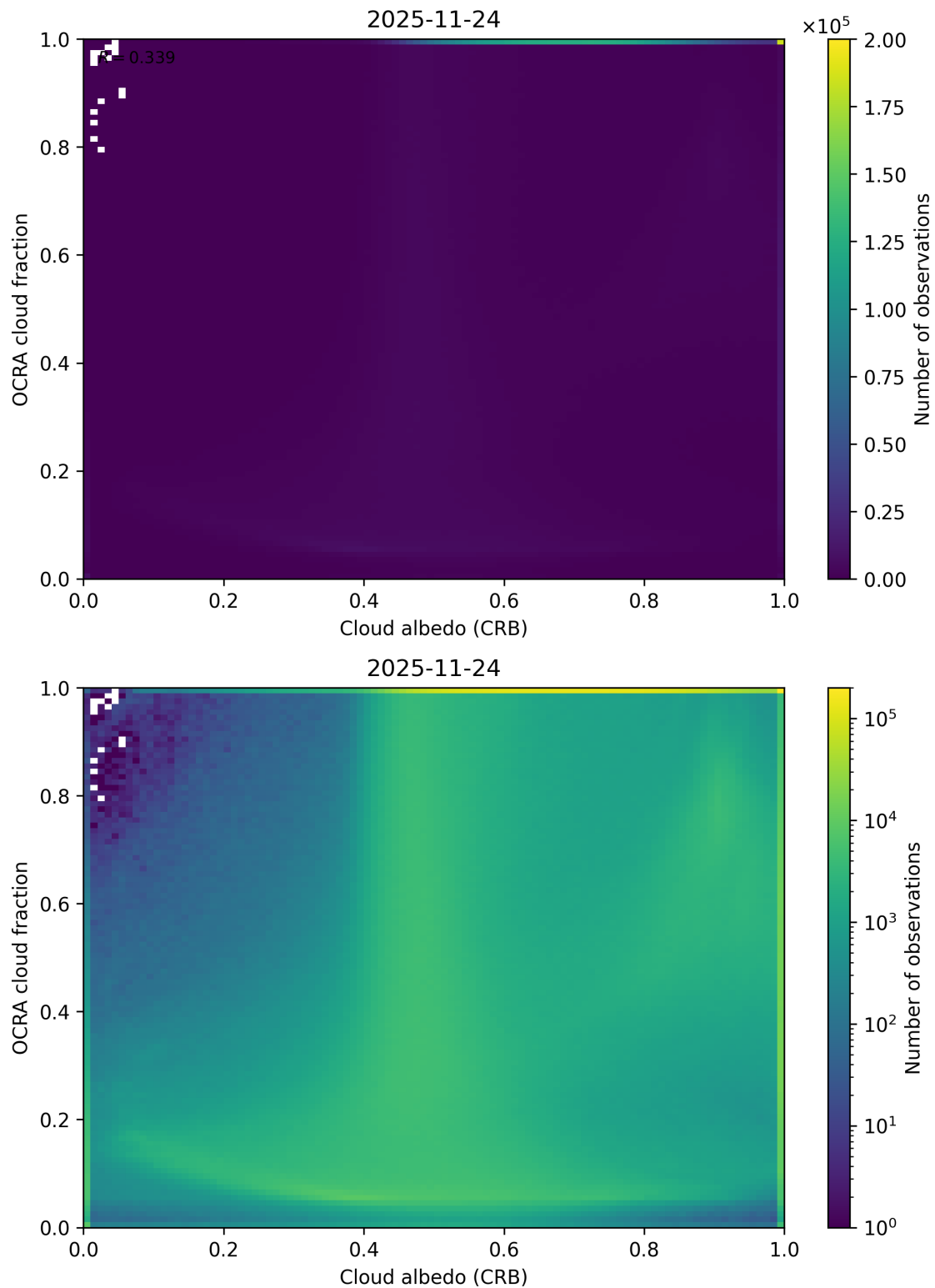
Figure 70: Scatter density plot of “Cloud albedo (CRB)” against “OCRA cloud fraction” for 2025-11-23 to 2025-11-25.
