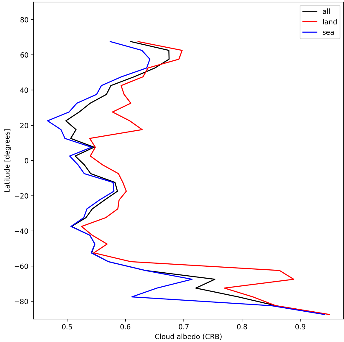
Figure 28: Zonal average of “Cloud albedo (CRB)” for 2025-11-23 to 2025-11-25.
