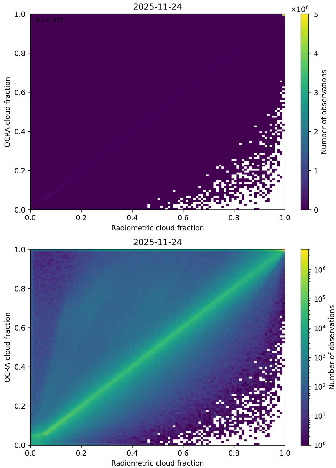
Figure 72: Scatter density plot of “Radiometric cloud fraction” against “OCRA cloud fraction” for 2025-11-23 to 2025-11-25.
