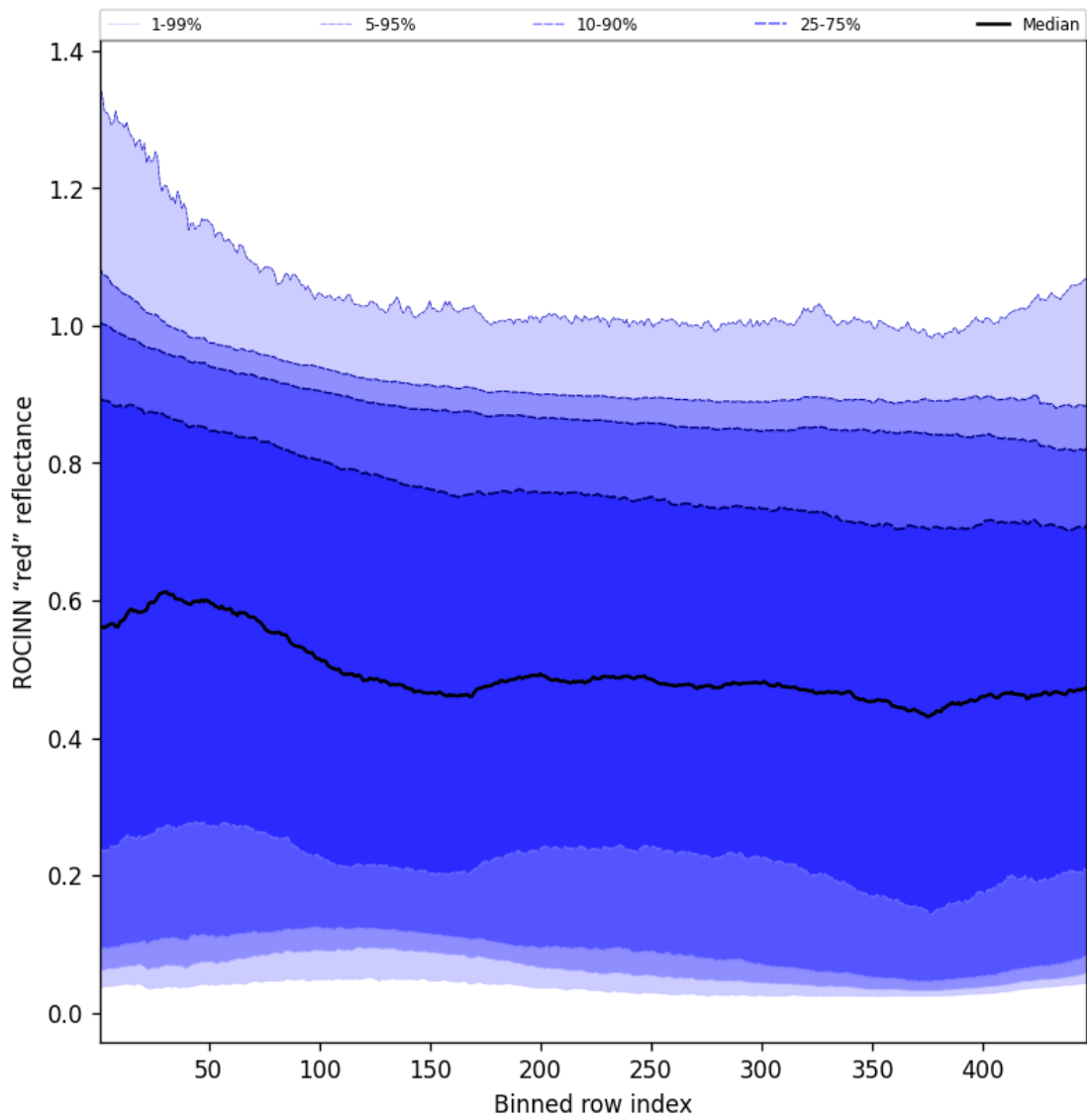
Figure 69: Along track statistics of “ROCINN “red” reflectance” for 2025-11-23 to 2025-11-25
