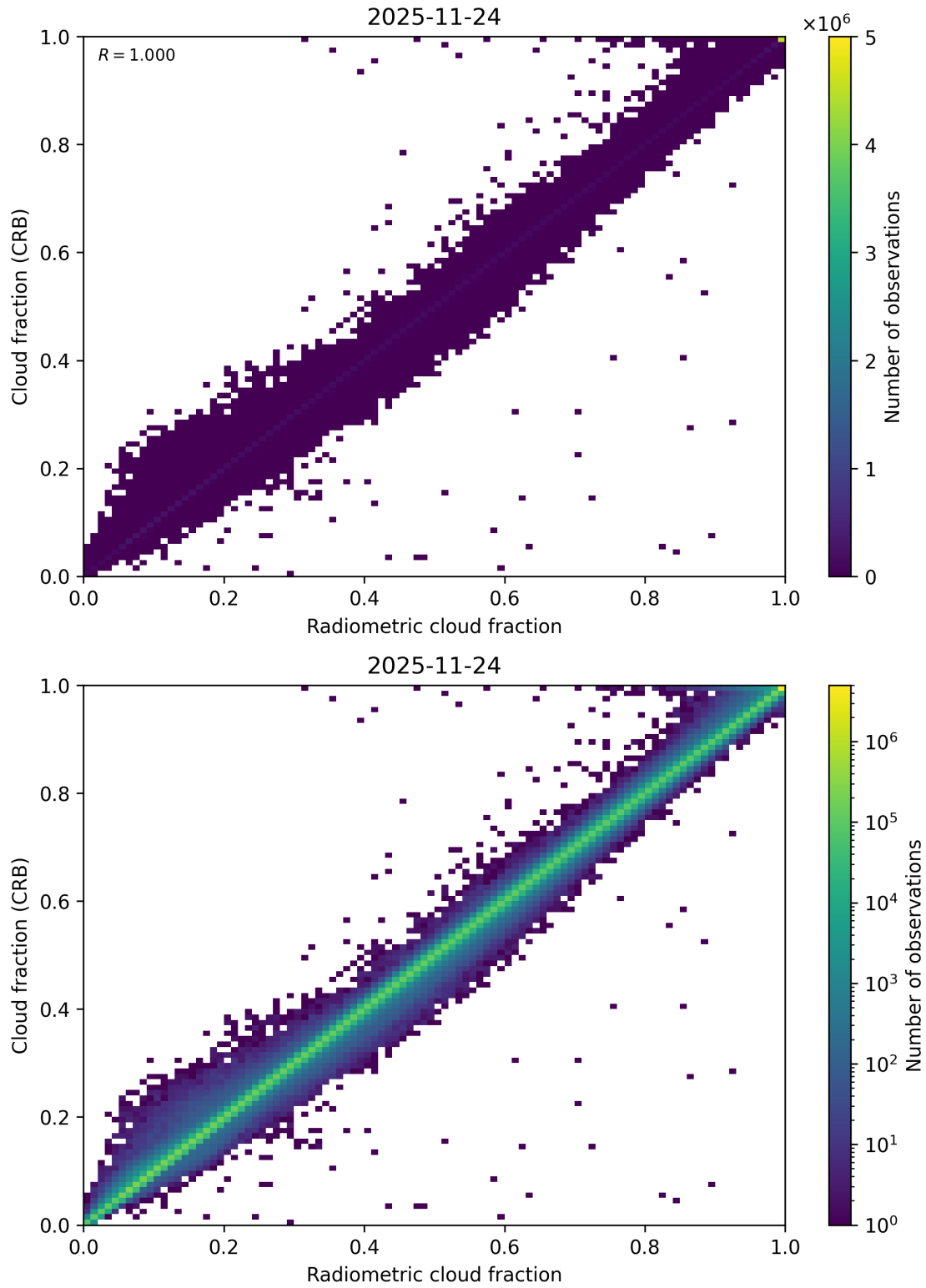
Figure 73: Scatter density plot of “Radiometric cloud fraction” against “Cloud fraction (CRB)” for 2025-11-23 to 2025-11-25.
