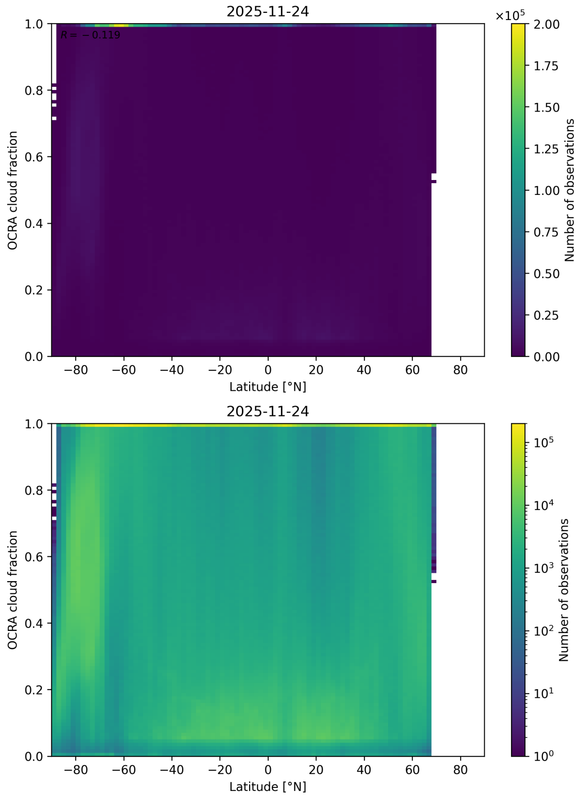
Figure 93: Scatter density plot of “Latitude” against “OCRA cloud fraction” for 2025-11-23 to 2025-11-25.
