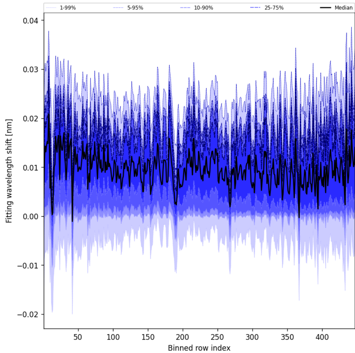
Figure 65: Along track statistics of “Fitting wavelength shift” for 2025-11-23 to 2025-11-25
