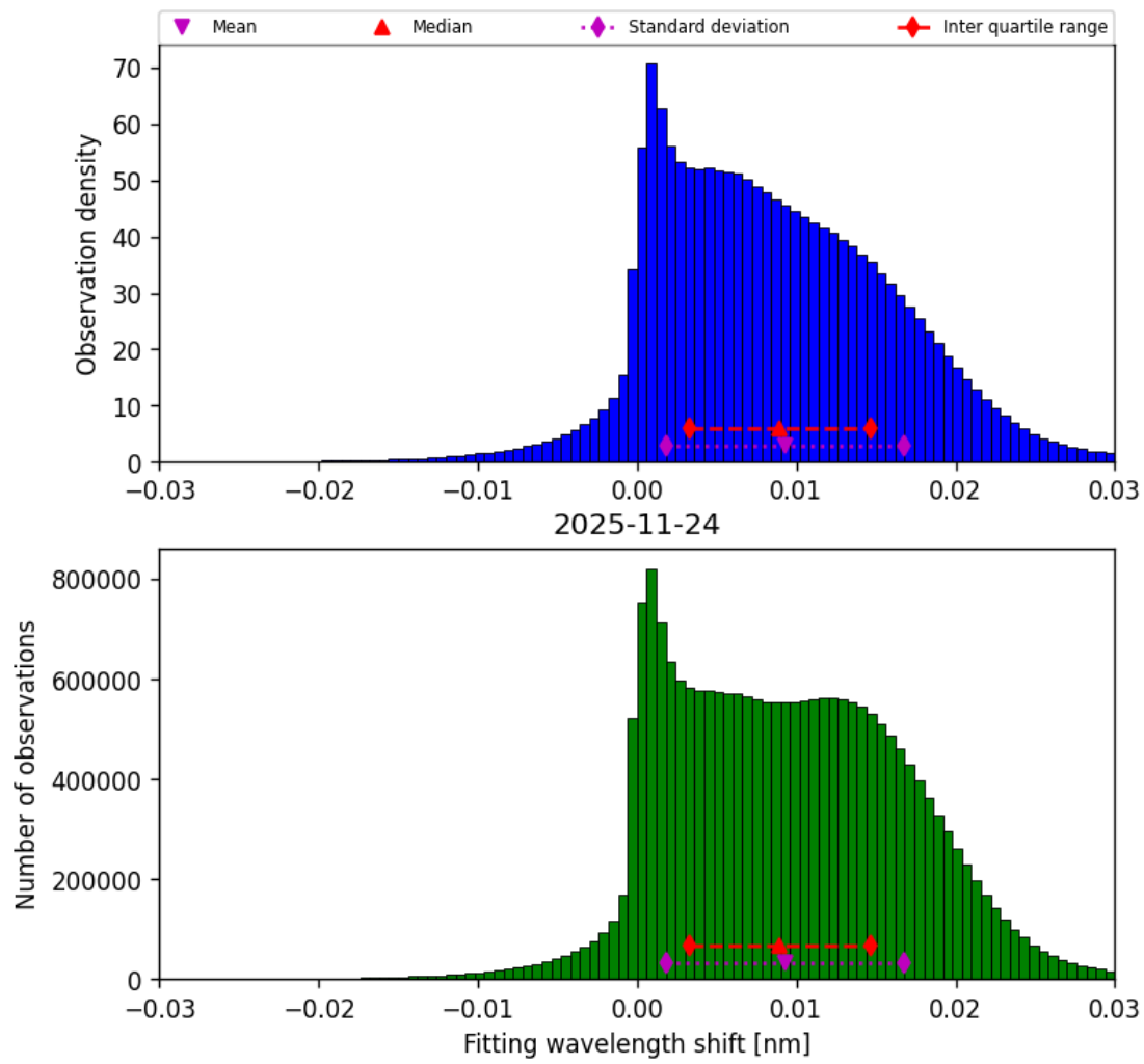
Figure 49: Histogram of “Fitting wavelength shift” for 2025-11-23 to 2025-11-25
