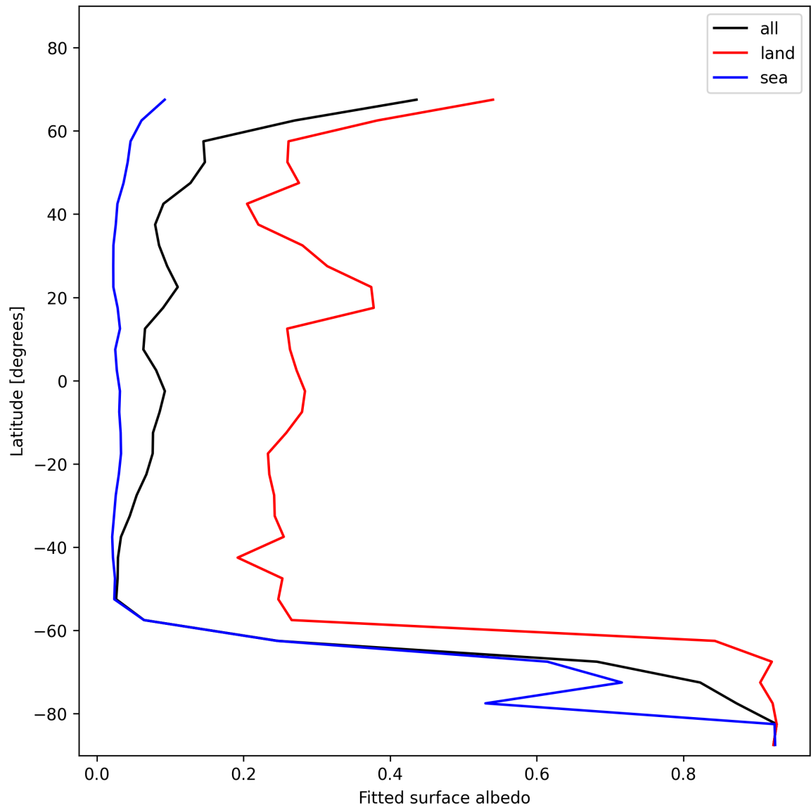
Figure 29: Zonal average of “Fitted surface albedo” for 2025-11-23 to 2025-11-25.
