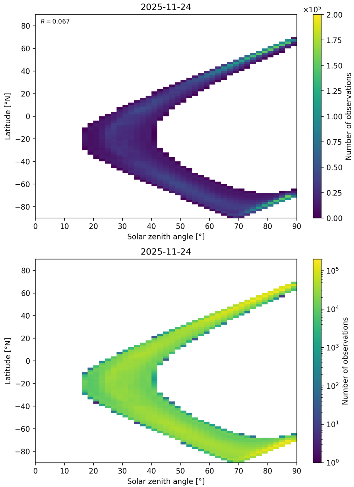
Figure 105: Scatter density plot of “Solar zenith angle” against “Latitude” for 2025-11-23 to 2025-11-25.
