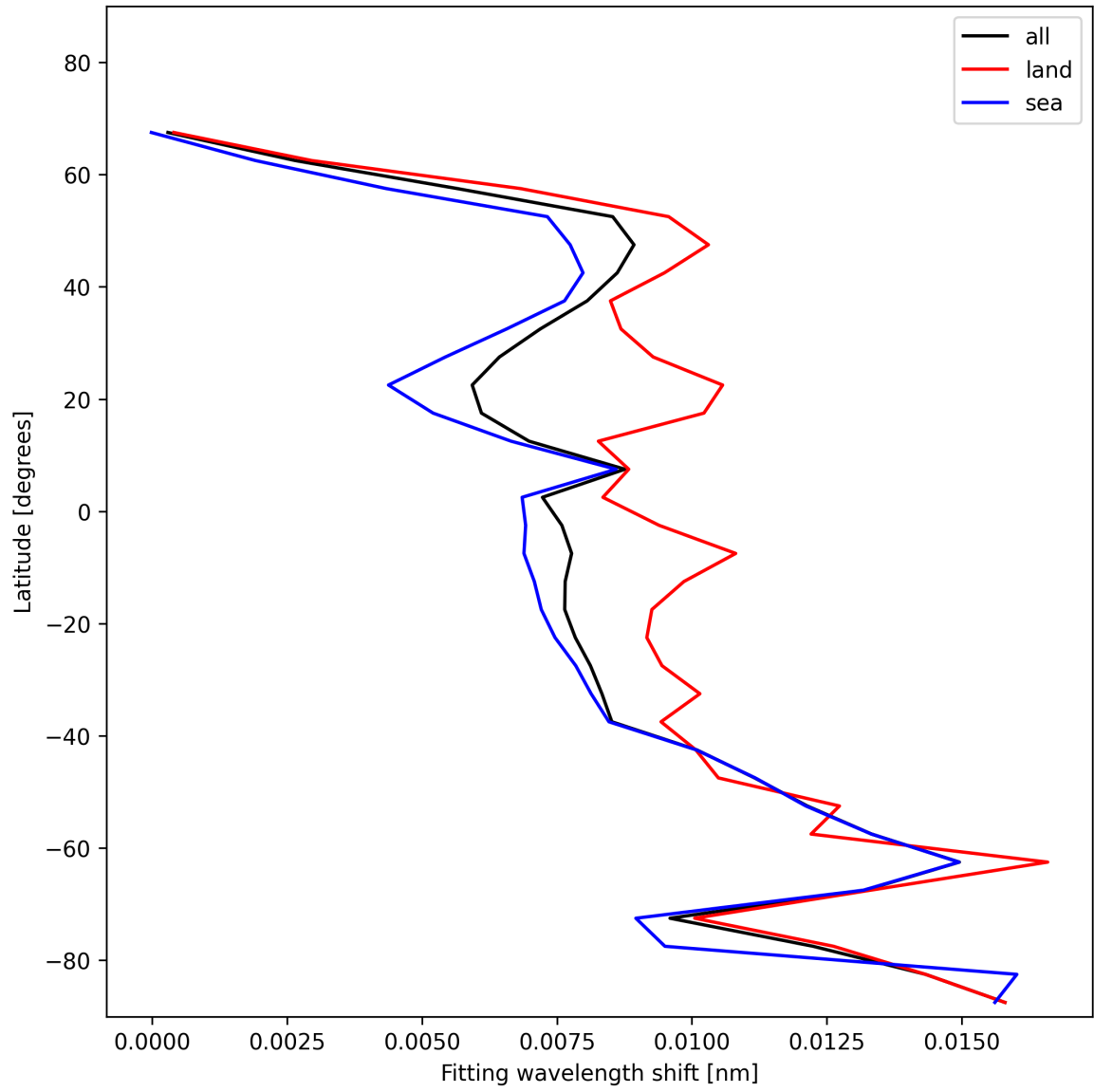
Figure 33: Zonal average of “Fitting wavelength shift” for 2025-11-23 to 2025-11-25.
