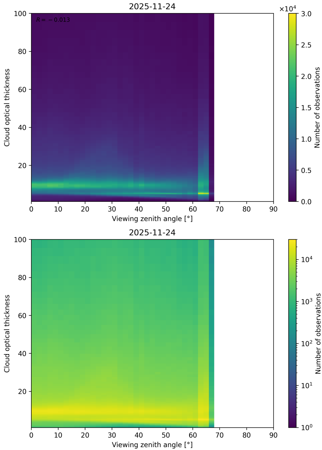
Figure 111: Scatter density plot of “Viewing zenith angle” against “Cloud optical thickness” for 2025-11-23 to 2025-11-25.
