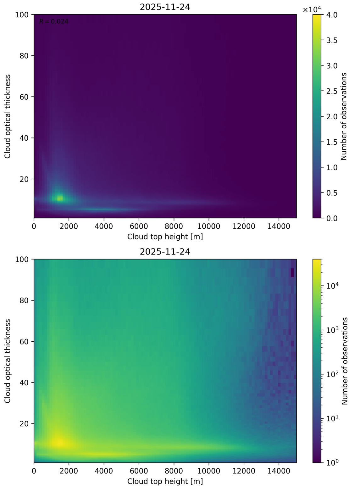
Figure 90: Scatter density plot of “Cloud top height” against “Cloud optical thickness” for 2025-11-23 to 2025-11-25.
