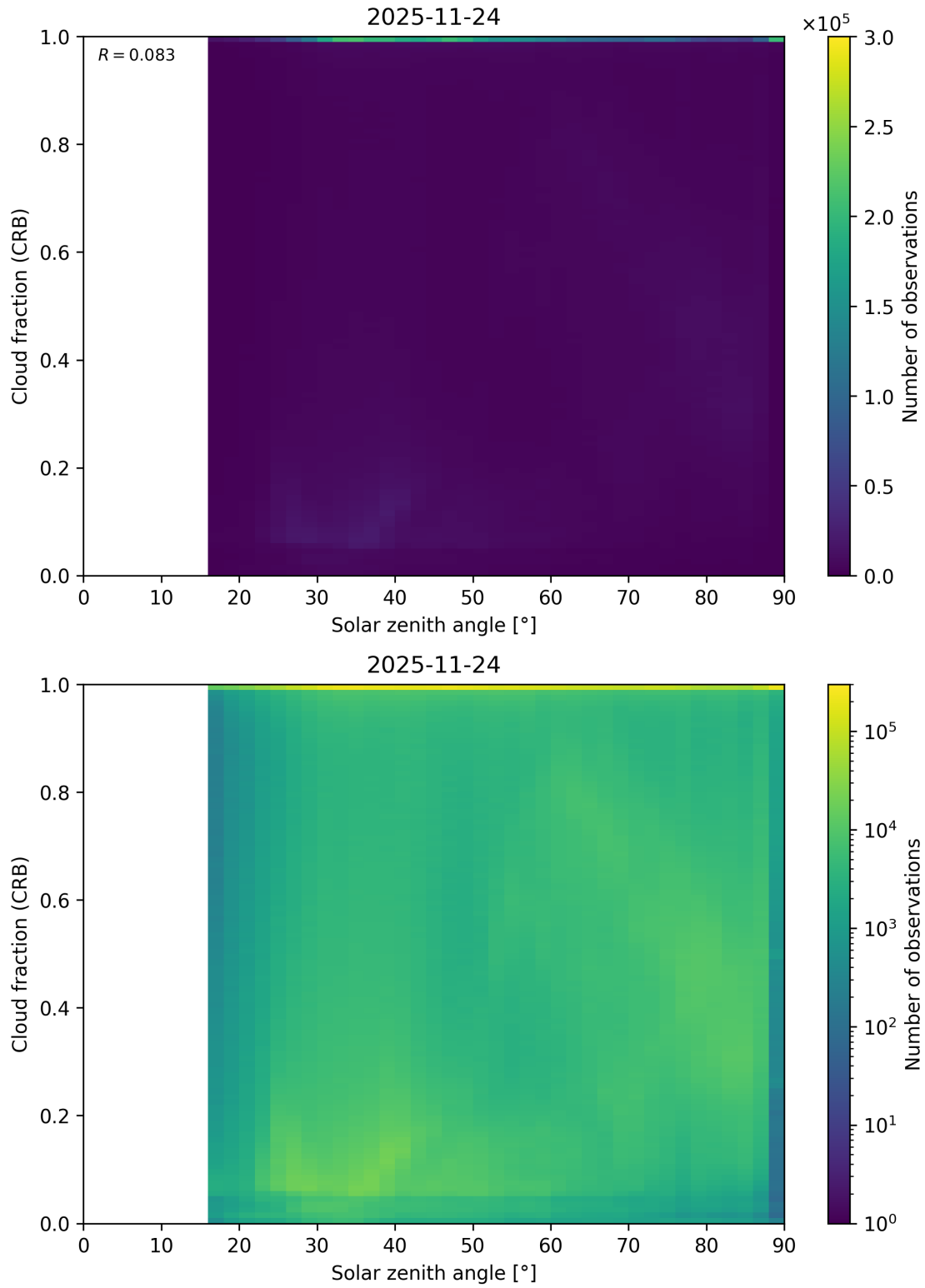
Figure 101: Scatter density plot of “Solar zenith angle” against “Cloud fraction (CRB)” for 2025-11-23 to 2025-11-25.
