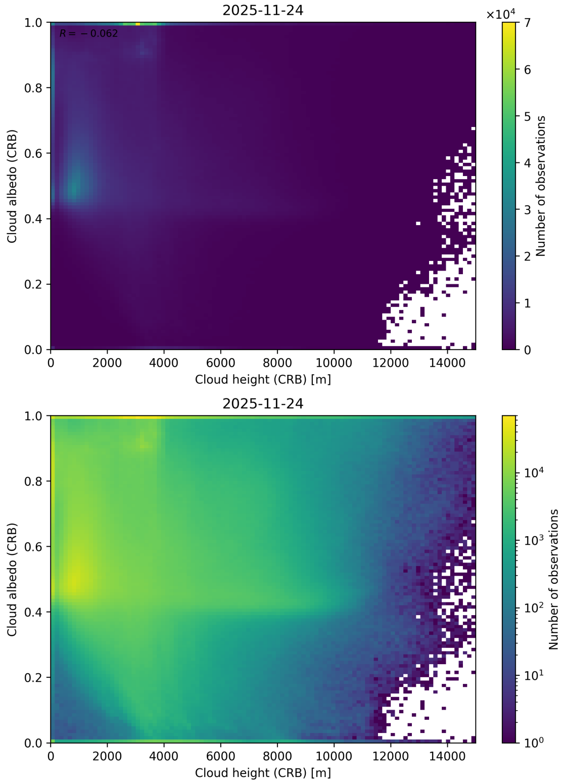
Figure 80: Scatter density plot of “Cloud height (CRB)” against “Cloud albedo (CRB)” for 2025-11-23 to 2025-11-25.
