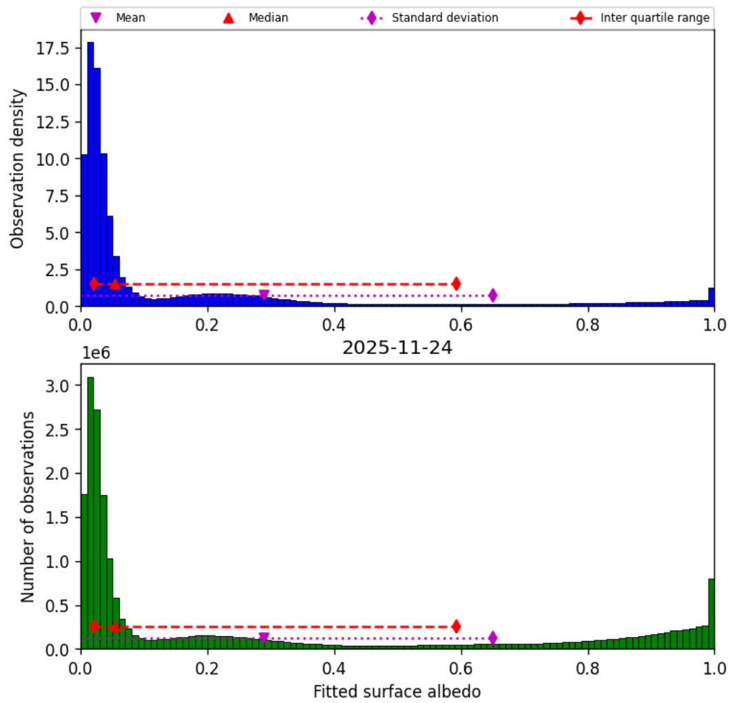
Figure 45: Histogram of “Fitted surface albedo” for 2025-11-23 to 2025-11-25
