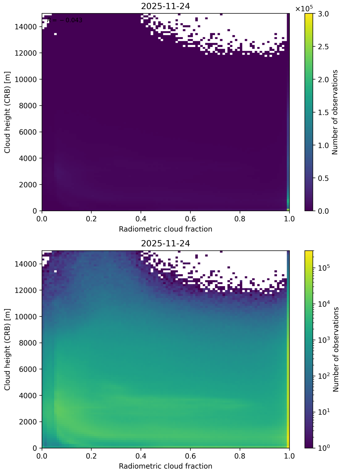
Figure 74: Scatter density plot of “Radiometric cloud fraction” against “Cloud height (CRB)” for 2025-11-23 to 2025-11-25.
