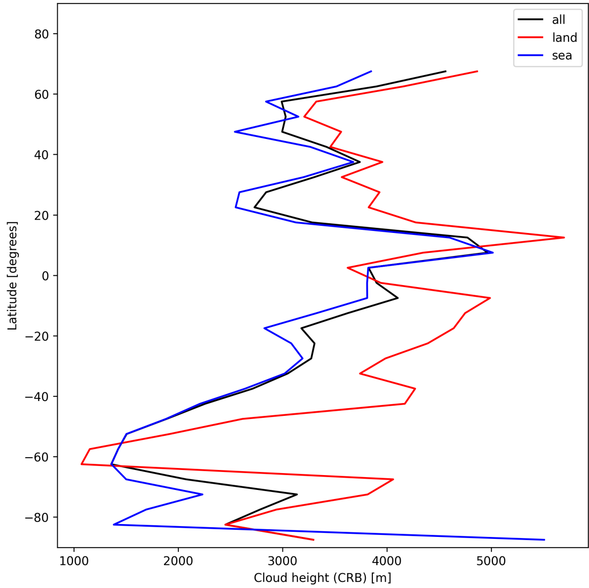
Figure 27: Zonal average of “Cloud height (CRB)” for 2025-11-23 to 2025-11-25.
