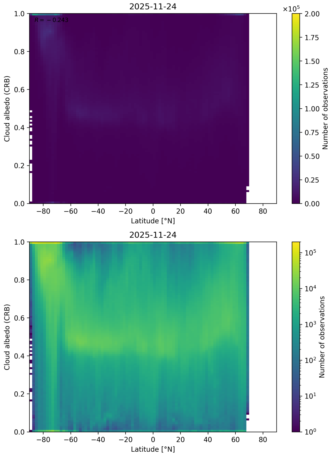
Figure 91: Scatter density plot of “Latitude” against “Cloud albedo (CRB)” for 2025-11-23 to 2025-11-25.
