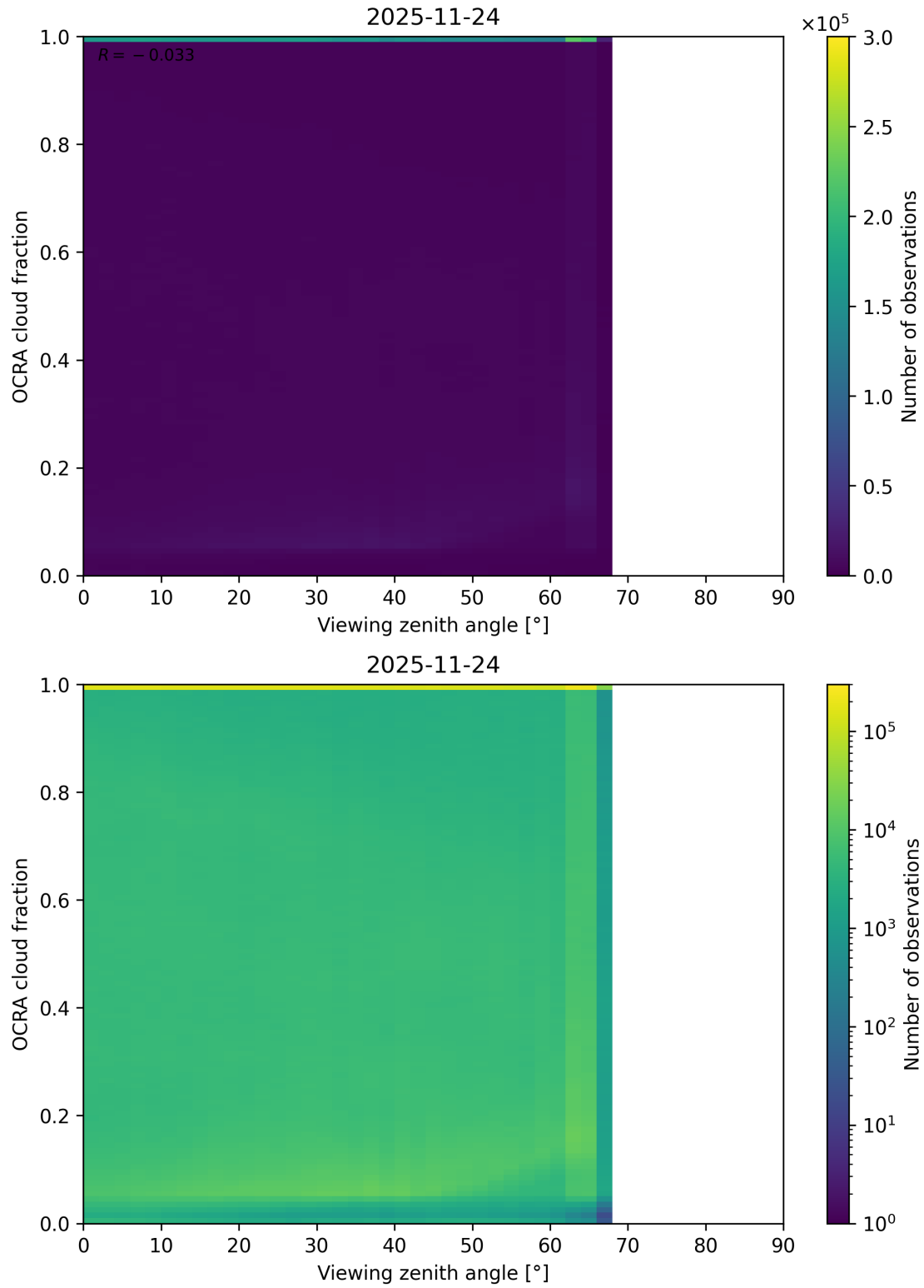
Figure 108: Scatter density plot of “Viewing zenith angle” against “OCRA cloud fraction” for 2025-11-23 to 2025-11-25.
