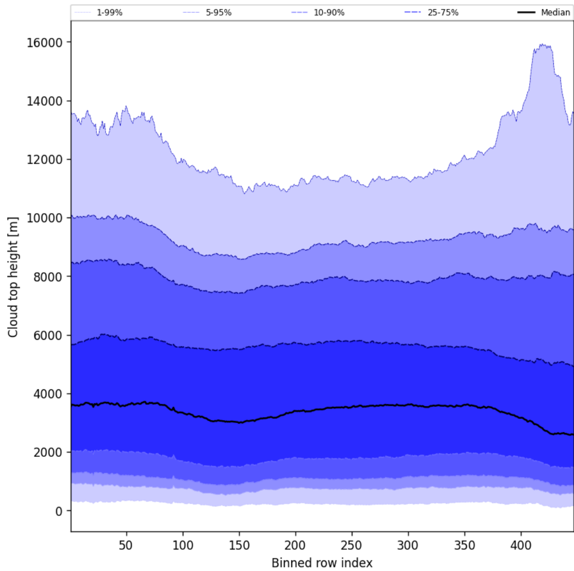
Figure 56: Along track statistics of “Cloud top height” for 2025-11-23 to 2025-11-25
