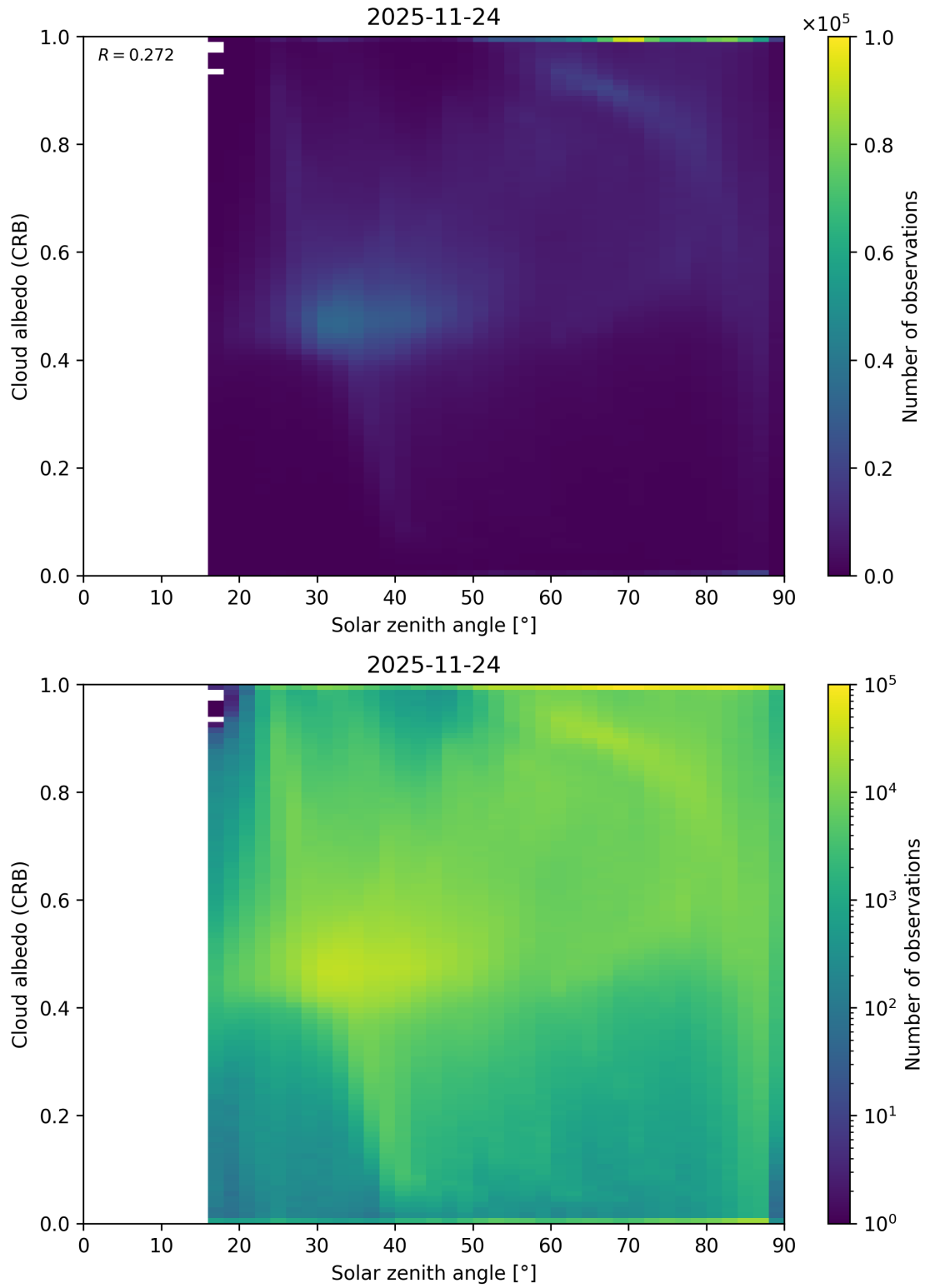
Figure 98: Scatter density plot of “Solar zenith angle” against “Cloud albedo (CRB)” for 2025-11-23 to 2025-11-25.
