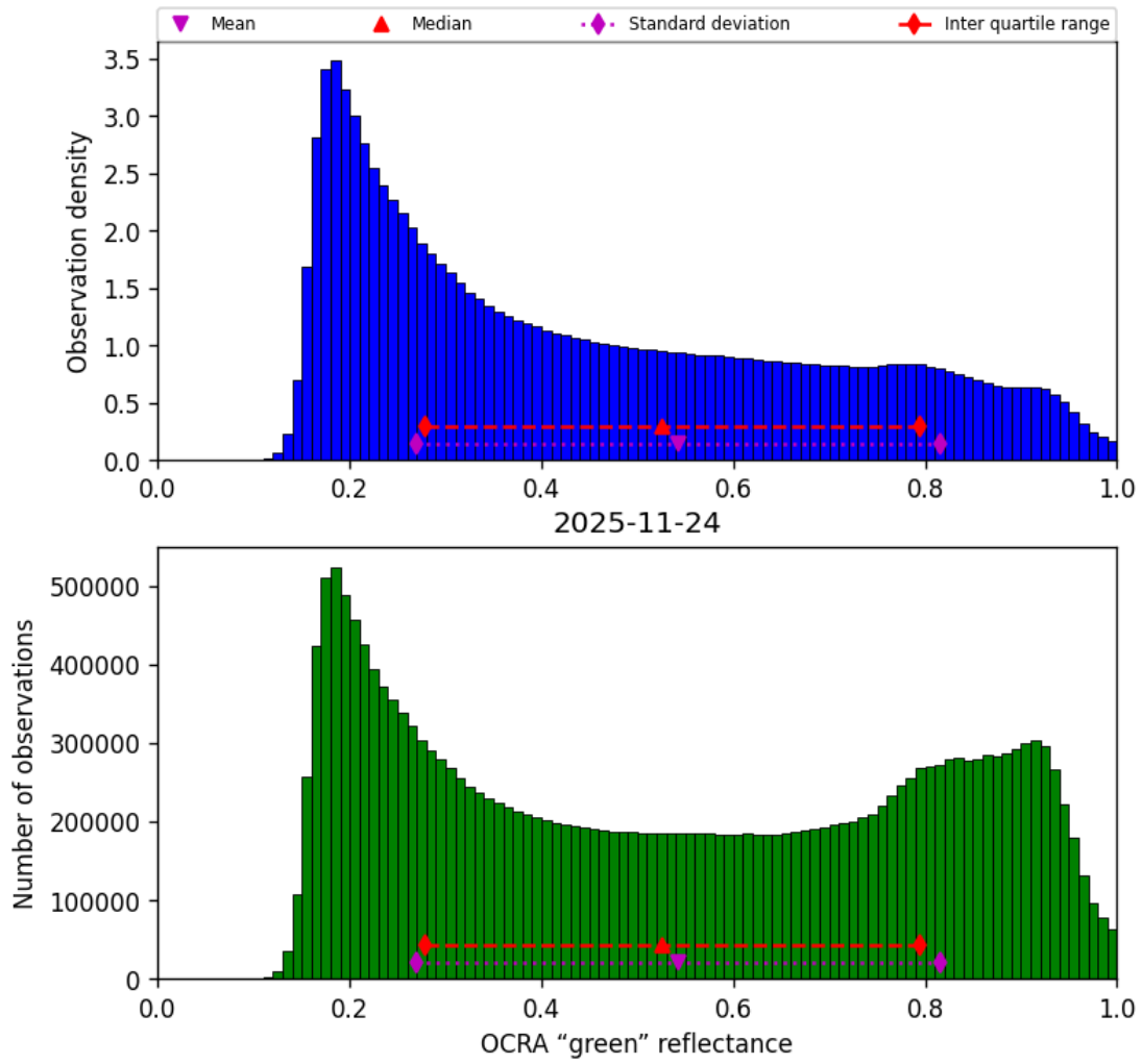
Figure 52: Histogram of “OCRA “green” reflectance” for 2025-11-23 to 2025-11-25
