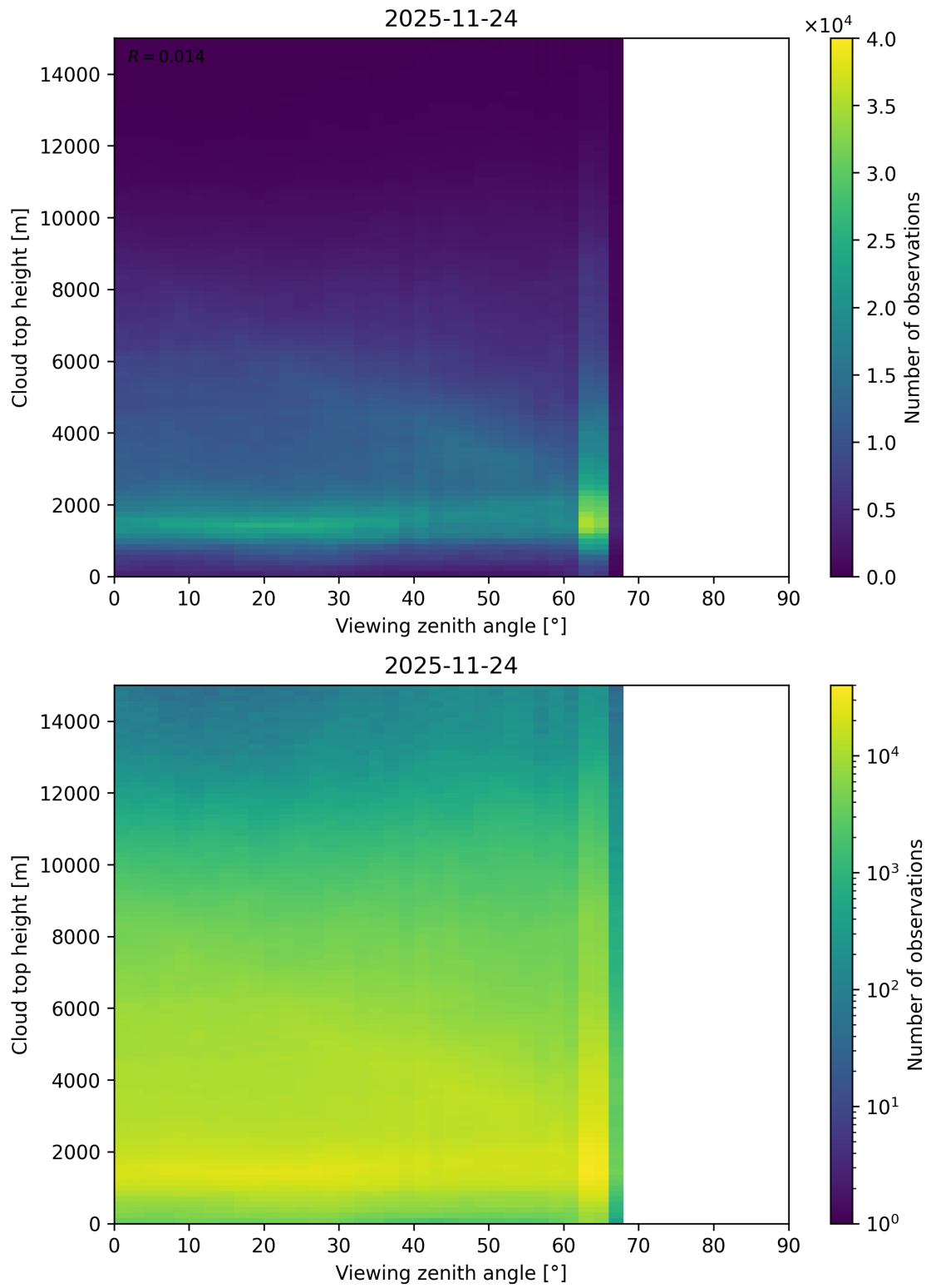
Figure 112: Scatter density plot of “Viewing zenith angle” against “Cloud top height” for 2025-11-23 to 2025-11-25.
