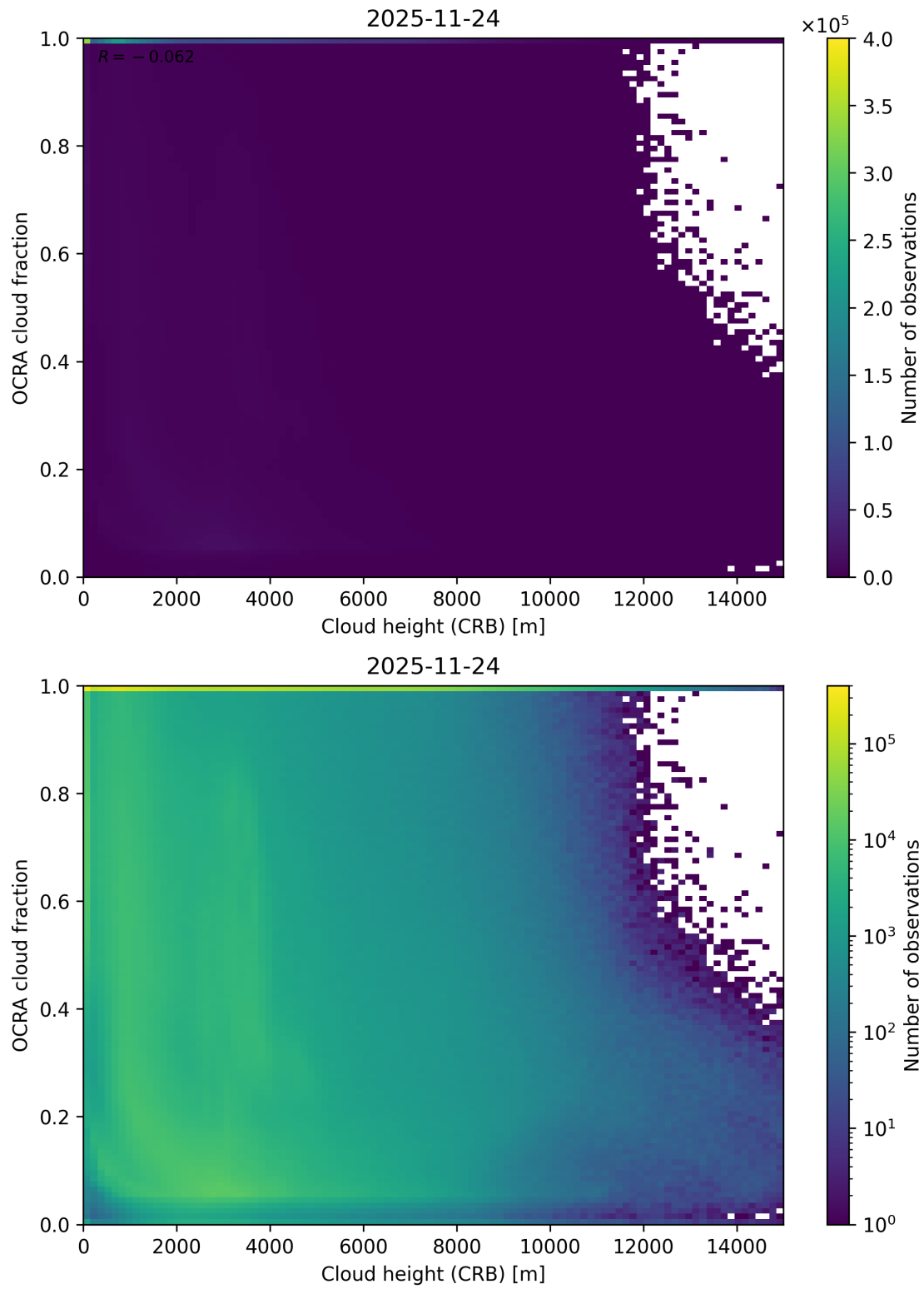
Figure 81: Scatter density plot of “Cloud height (CRB)” against “OCRA cloud fraction” for 2025-11-23 to 2025-11-25.
