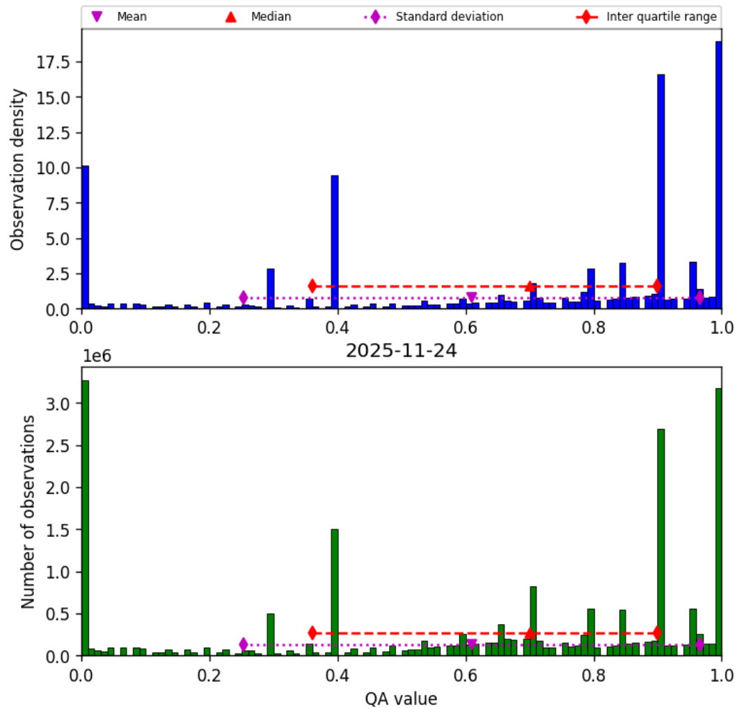
Figure 38: Histogram of “QA value” for 2025-11-23 to 2025-11-25
