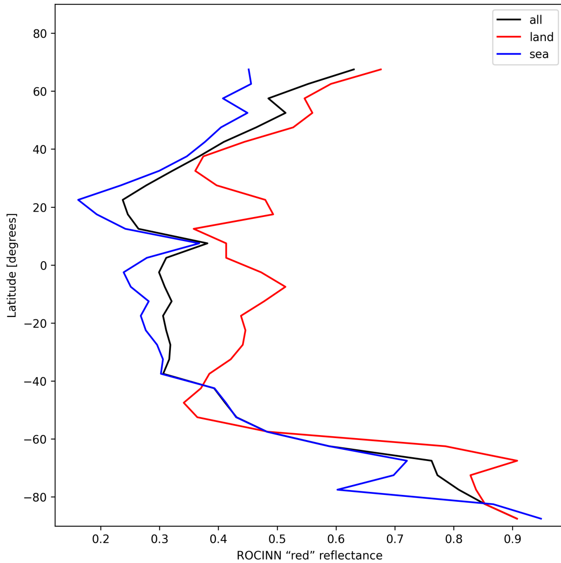
Figure 37: Zonal average of “ROCINN “red” reflectance” for 2025-11-23 to 2025-11-25.
