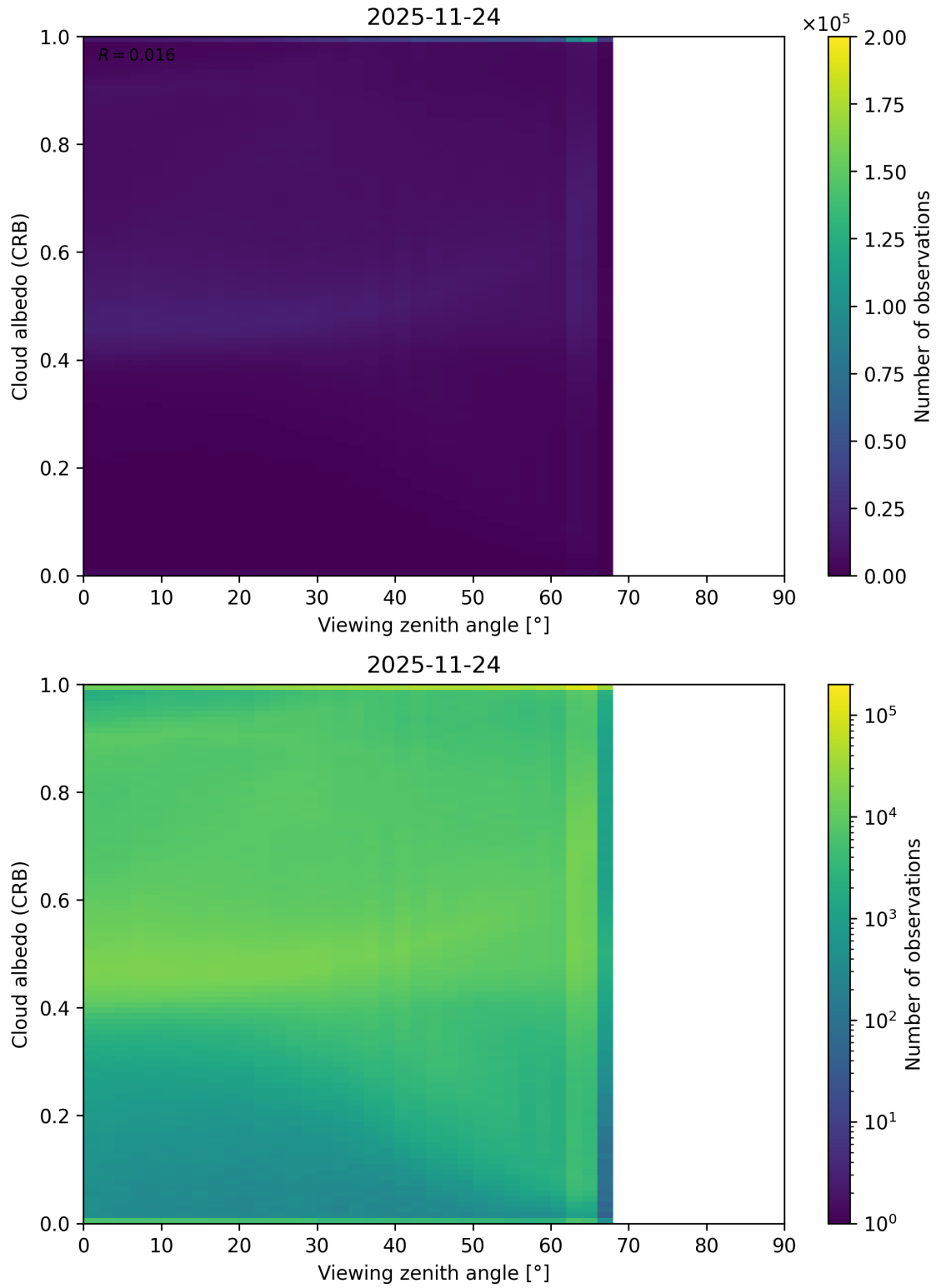
Figure 106: Scatter density plot of “Viewing zenith angle” against “Cloud albedo (CRB)” for 2025-11-23 to 2025-11-25.
