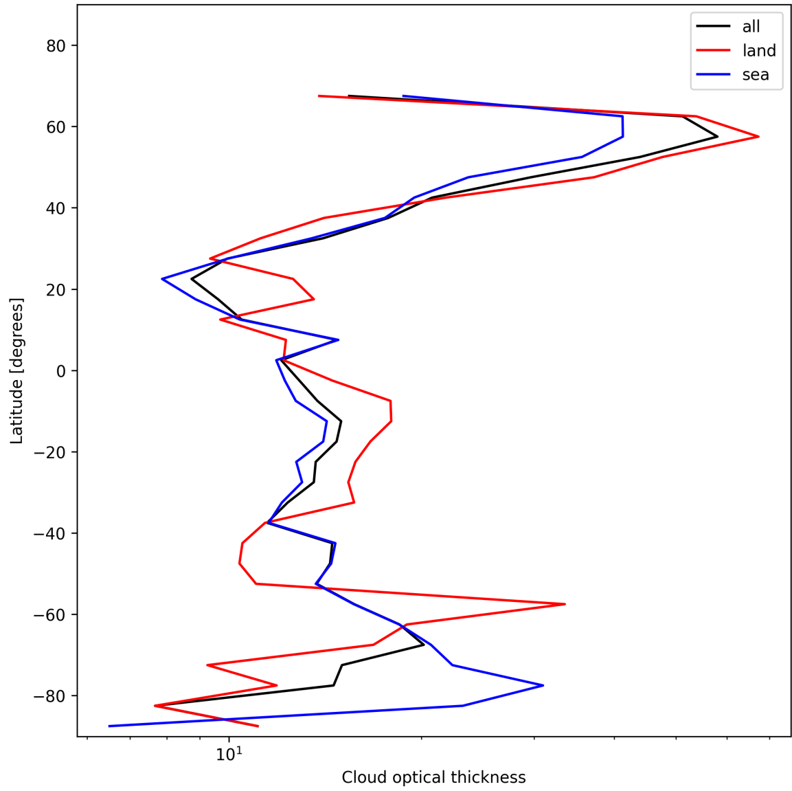
Figure 25: Zonal average of “Cloud optical thickness” for 2025-11-23 to 2025-11-25.
