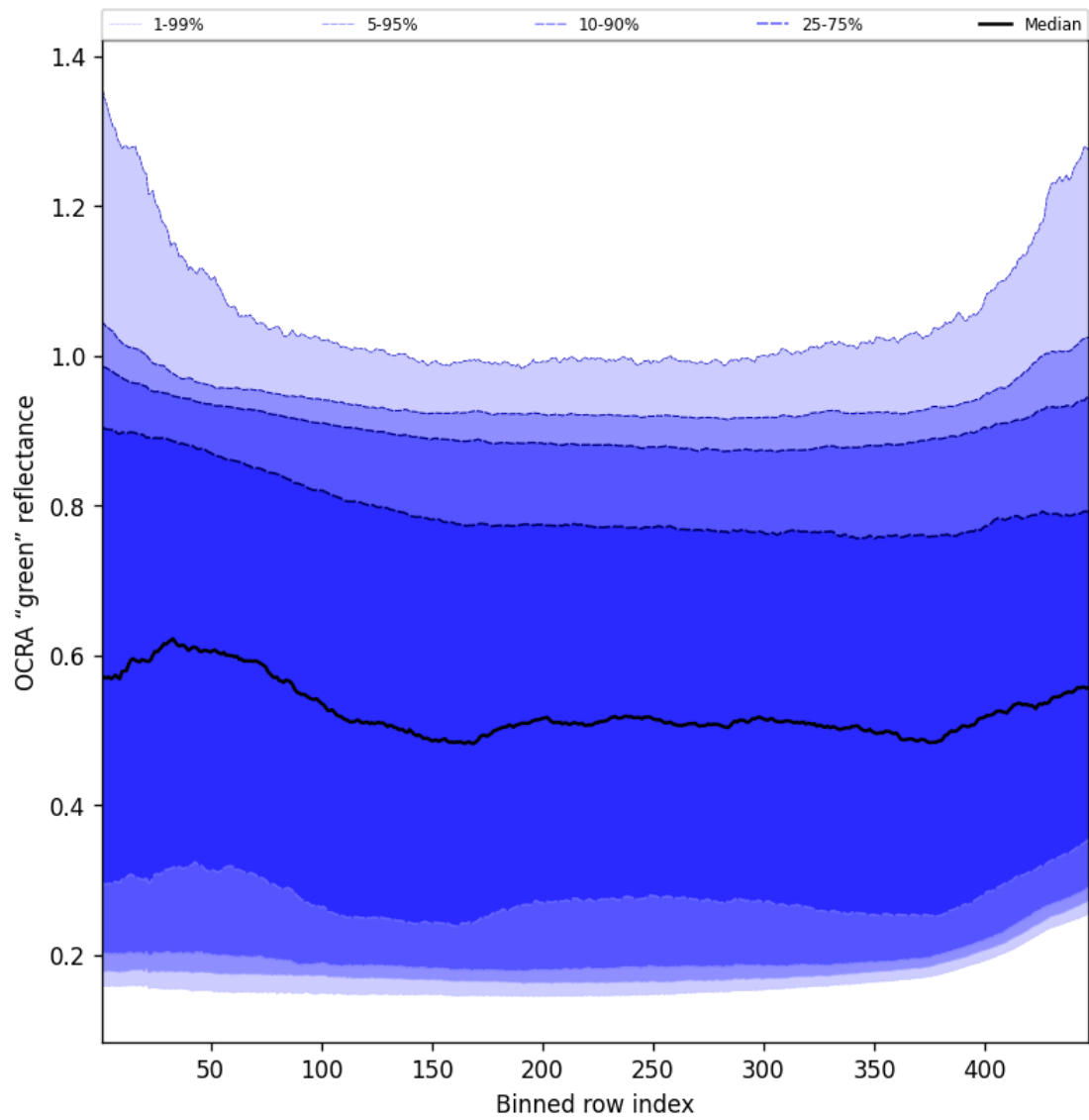
Figure 68: Along track statistics of “OCRA “green” reflectance” for 2025-11-23 to 2025-11-25
