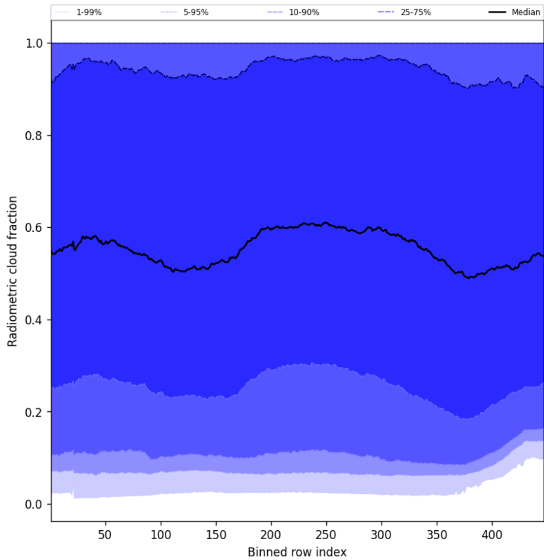
Figure 55: Along track statistics of “Radiometric cloud fraction” for 2025-11-23 to 2025-11-25
