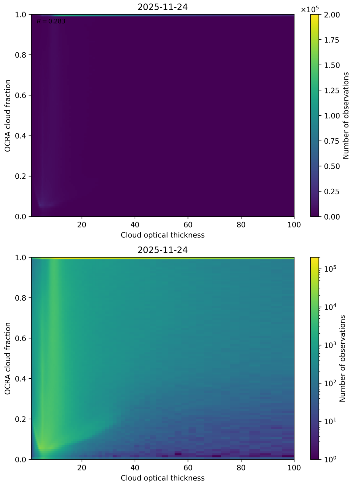
Figure 83: Scatter density plot of “Cloud optical thickness” against “OCRA cloud fraction” for 2025-11-23 to 2025-11-25.
