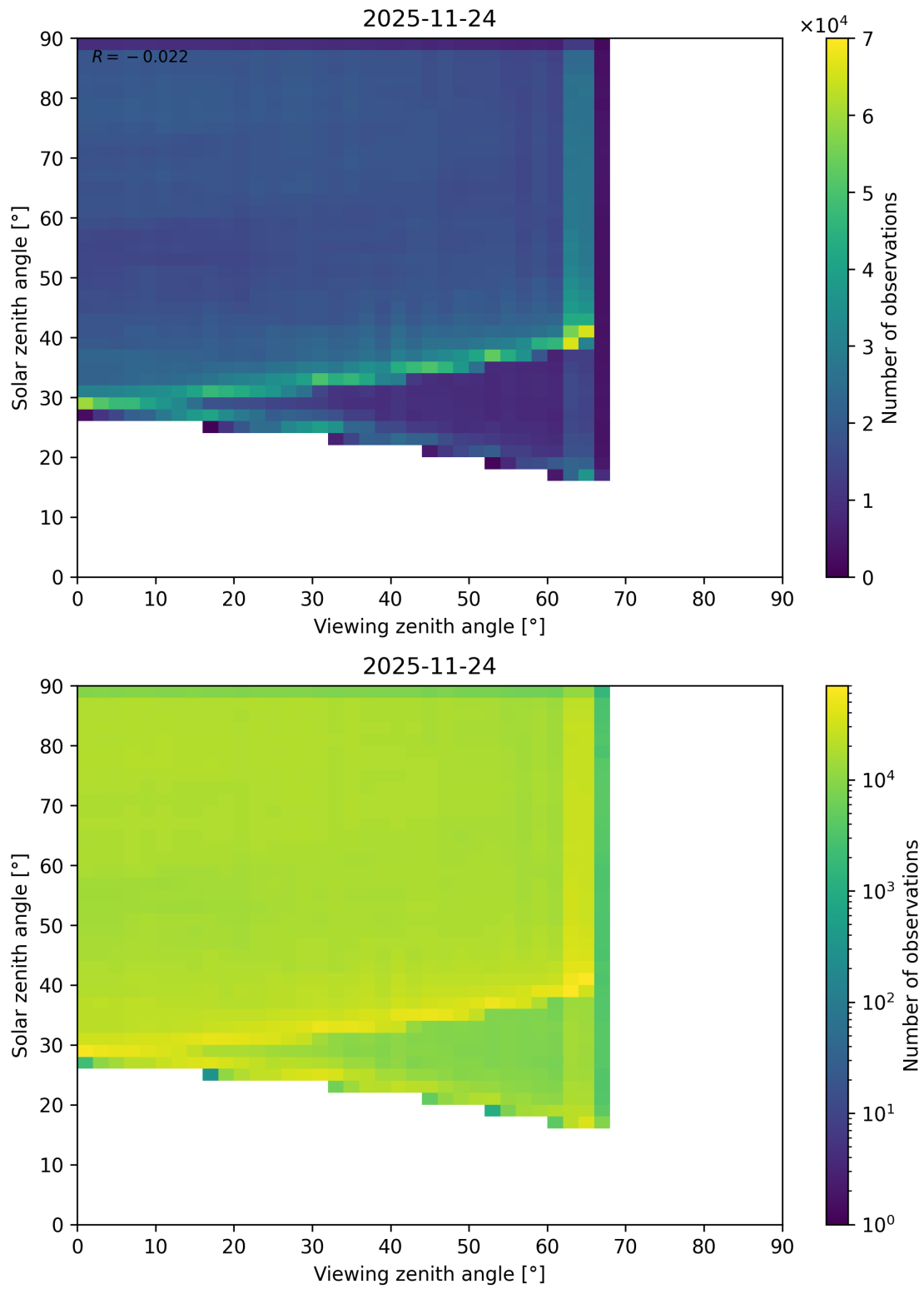
Figure 114: Scatter density plot of “Viewing zenith angle” against “Solar zenith angle” for 2025-11-23 to 2025-11-25.
