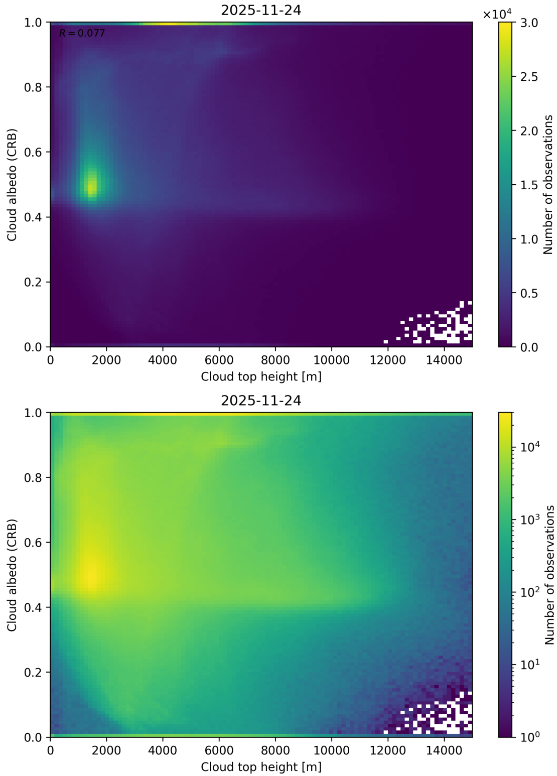
Figure 86: Scatter density plot of “Cloud top height” against “Cloud albedo (CRB)” for 2025-11-23 to 2025-11-25.
