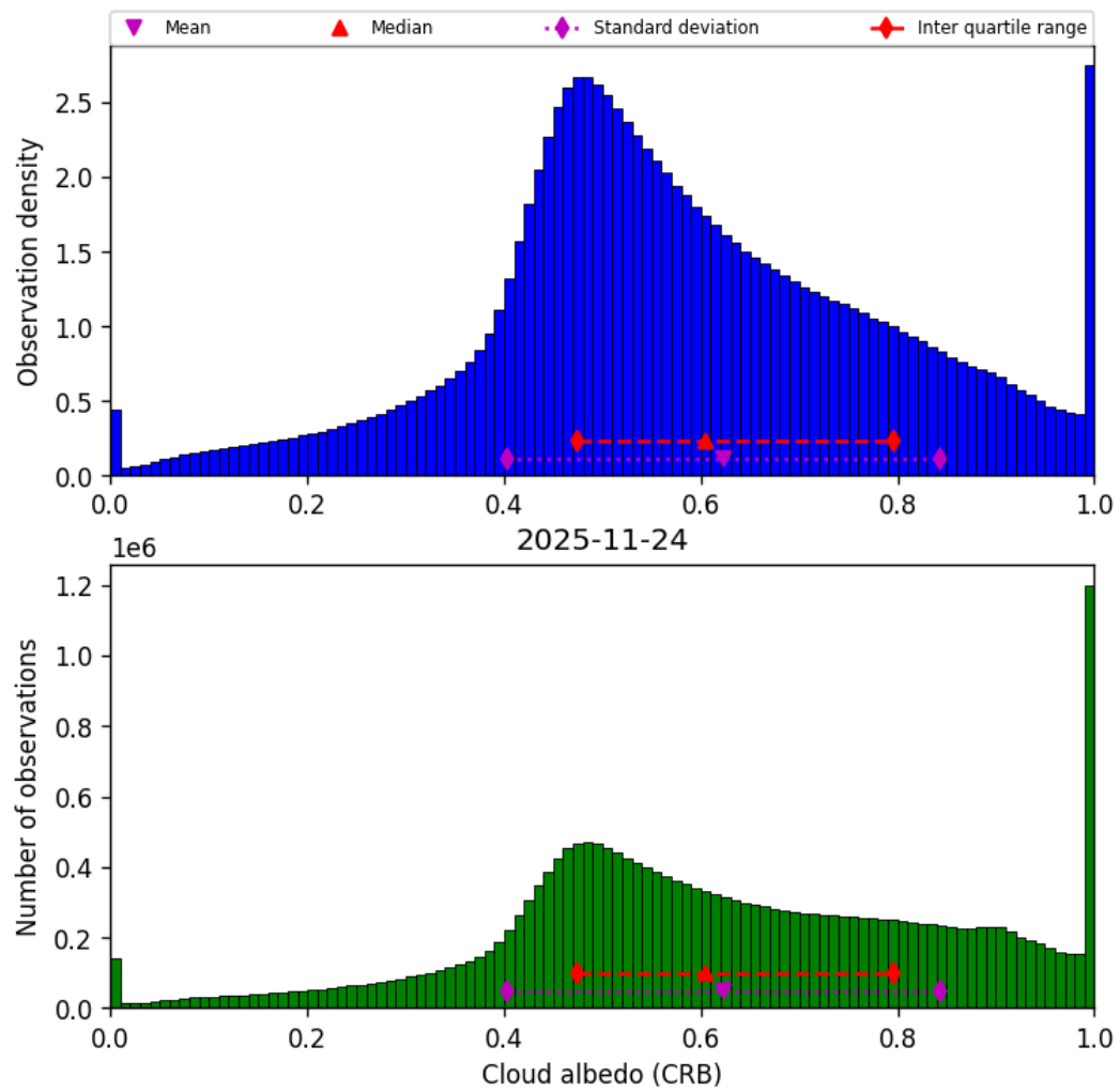
Figure 44: Histogram of “Cloud albedo (CRB)” for 2025-11-23 to 2025-11-25
