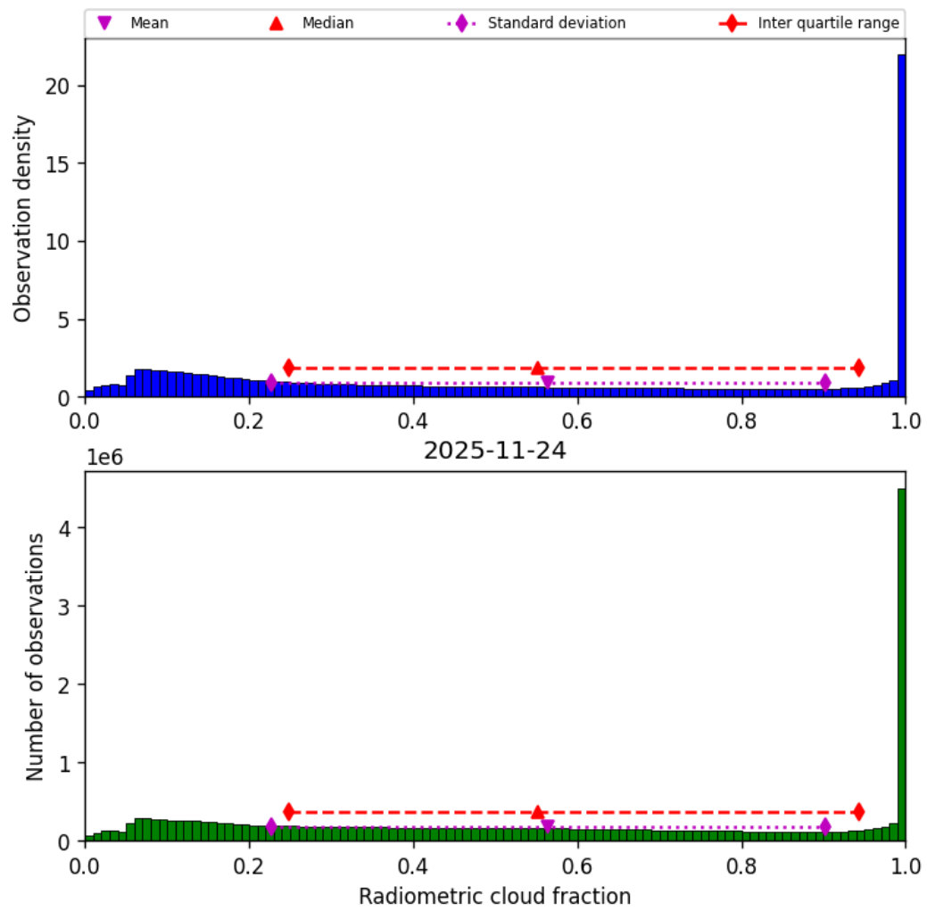
Figure 39: Histogram of “Radiometric cloud fraction” for 2025-11-23 to 2025-11-25
