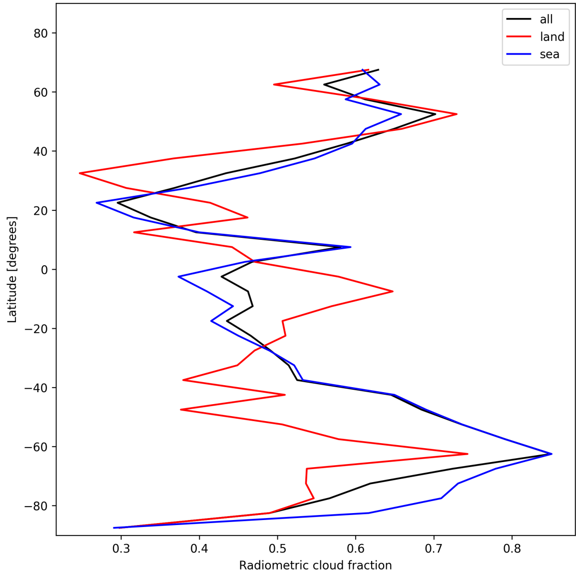
Figure 23: Zonal average of “Radiometric cloud fraction” for 2025-11-23 to 2025-11-25.
