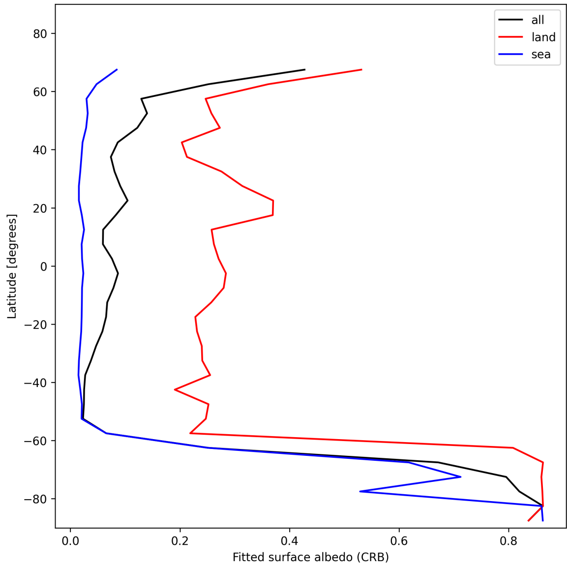
Figure 30: Zonal average of “Fitted surface albedo (CRB)” for 2025-11-23 to 2025-11-25.
