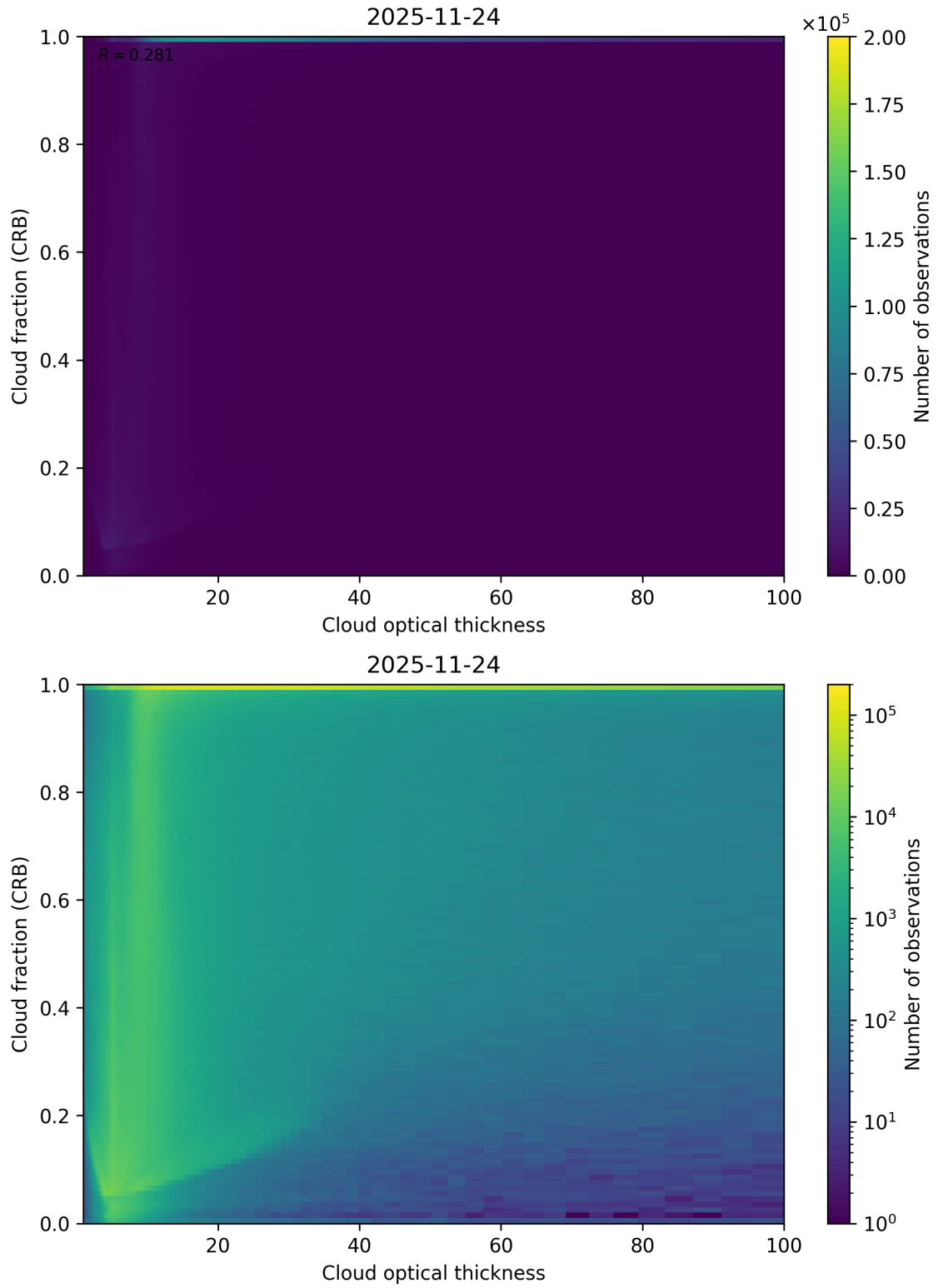
Figure 84: Scatter density plot of “Cloud optical thickness” against “Cloud fraction (CRB)” for 2025-11-23 to 2025-11-25.
