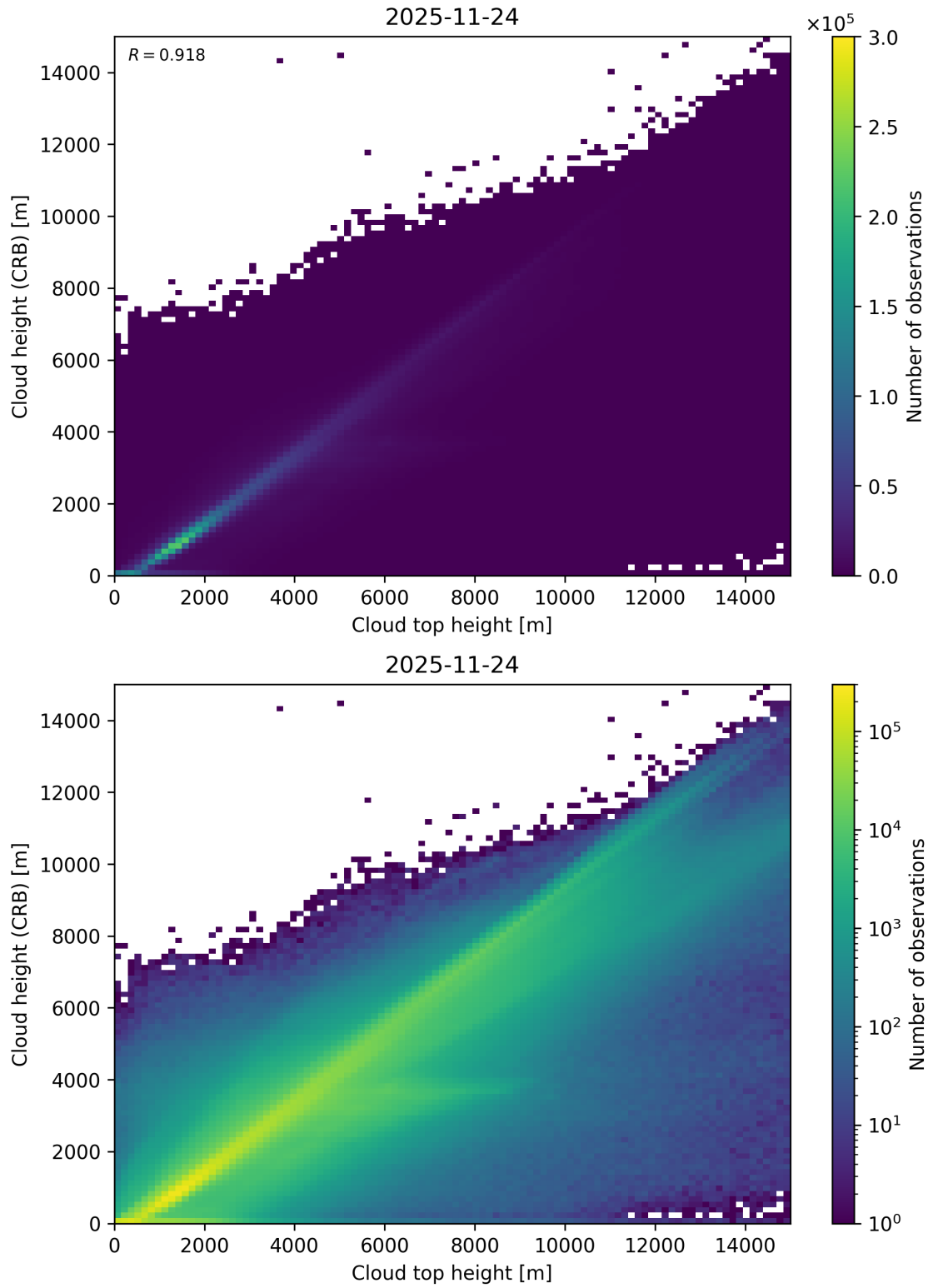
Figure 89: Scatter density plot of “Cloud top height” against “Cloud height (CRB)” for 2025-11-23 to 2025-11-25.
