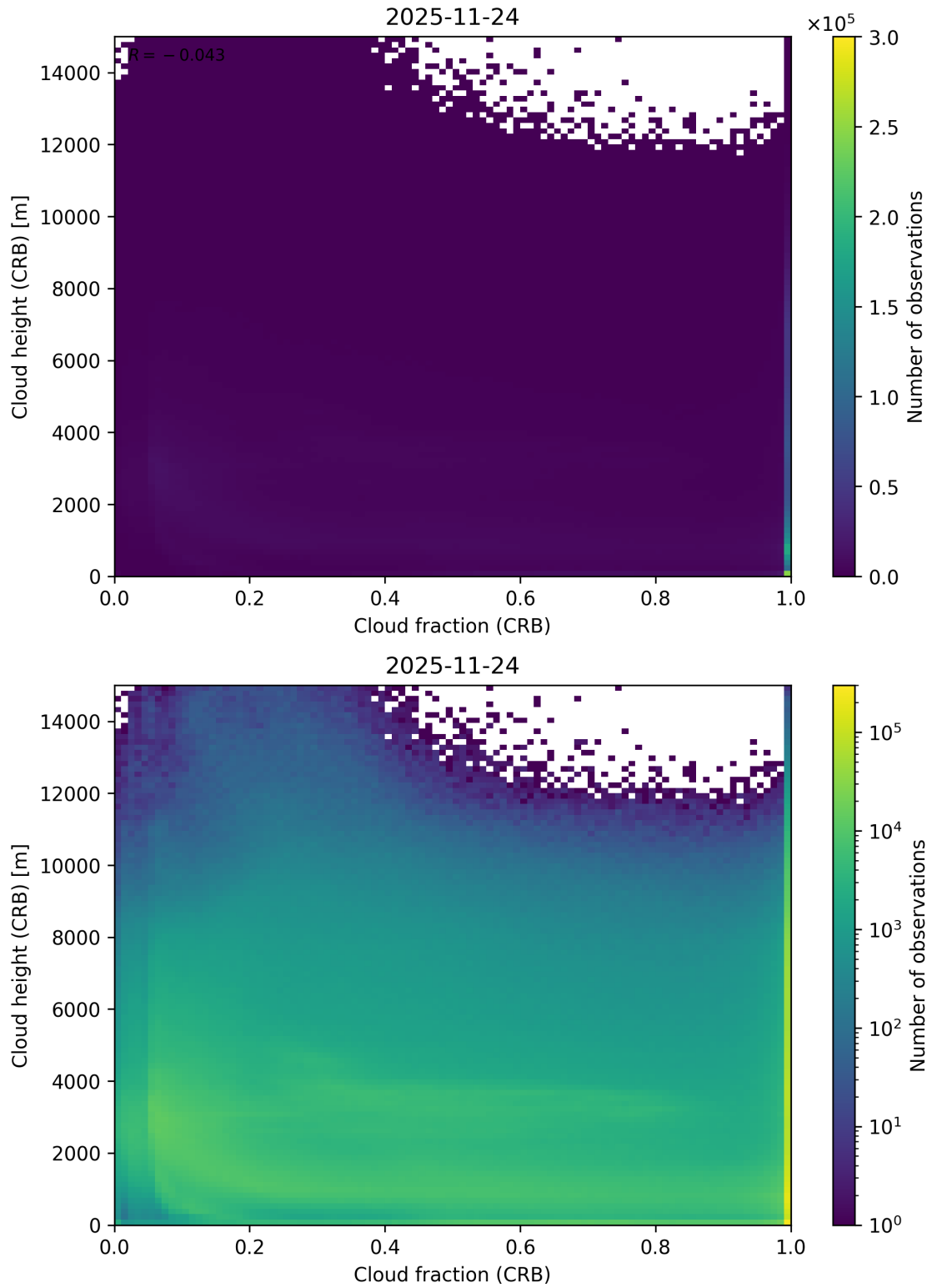
Figure 79: Scatter density plot of “Cloud fraction (CRB)” against “Cloud height (CRB)” for 2025-11-23 to 2025-11-25.
