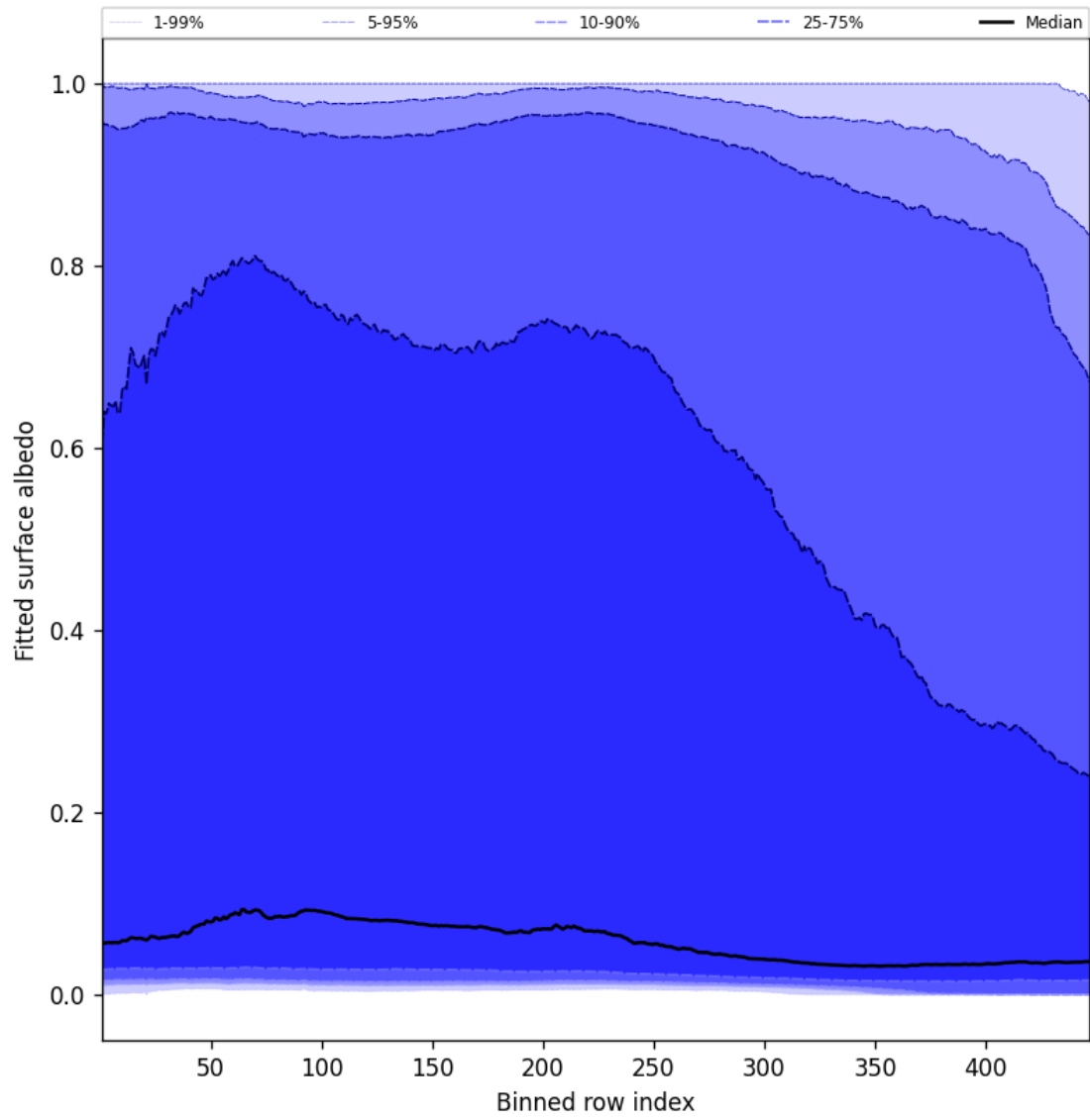
Figure 61: Along track statistics of “Fitted surface albedo” for 2025-11-23 to 2025-11-25
