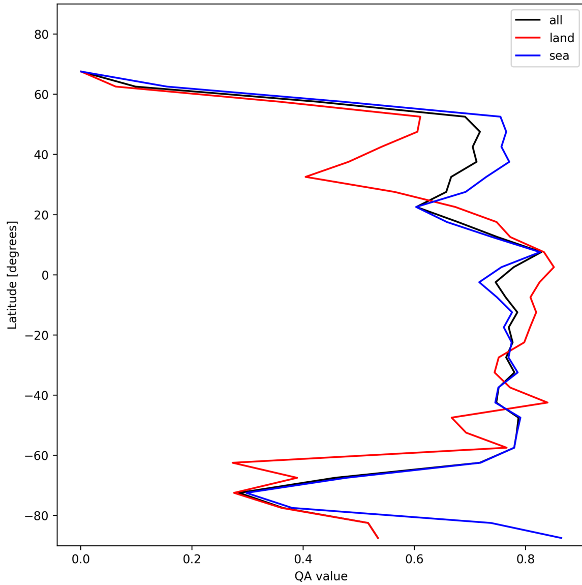
Figure 22: Zonal average of “QA value” for 2025-11-23 to 2025-11-25.
