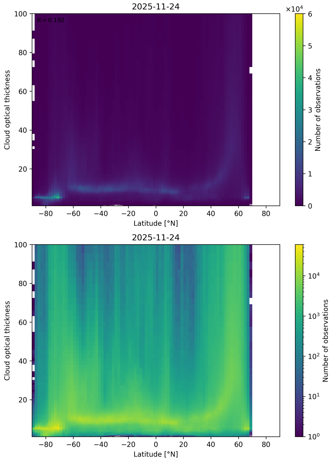
Figure 96: Scatter density plot of “Latitude” against “Cloud optical thickness” for 2025-11-23 to 2025-11-25.
