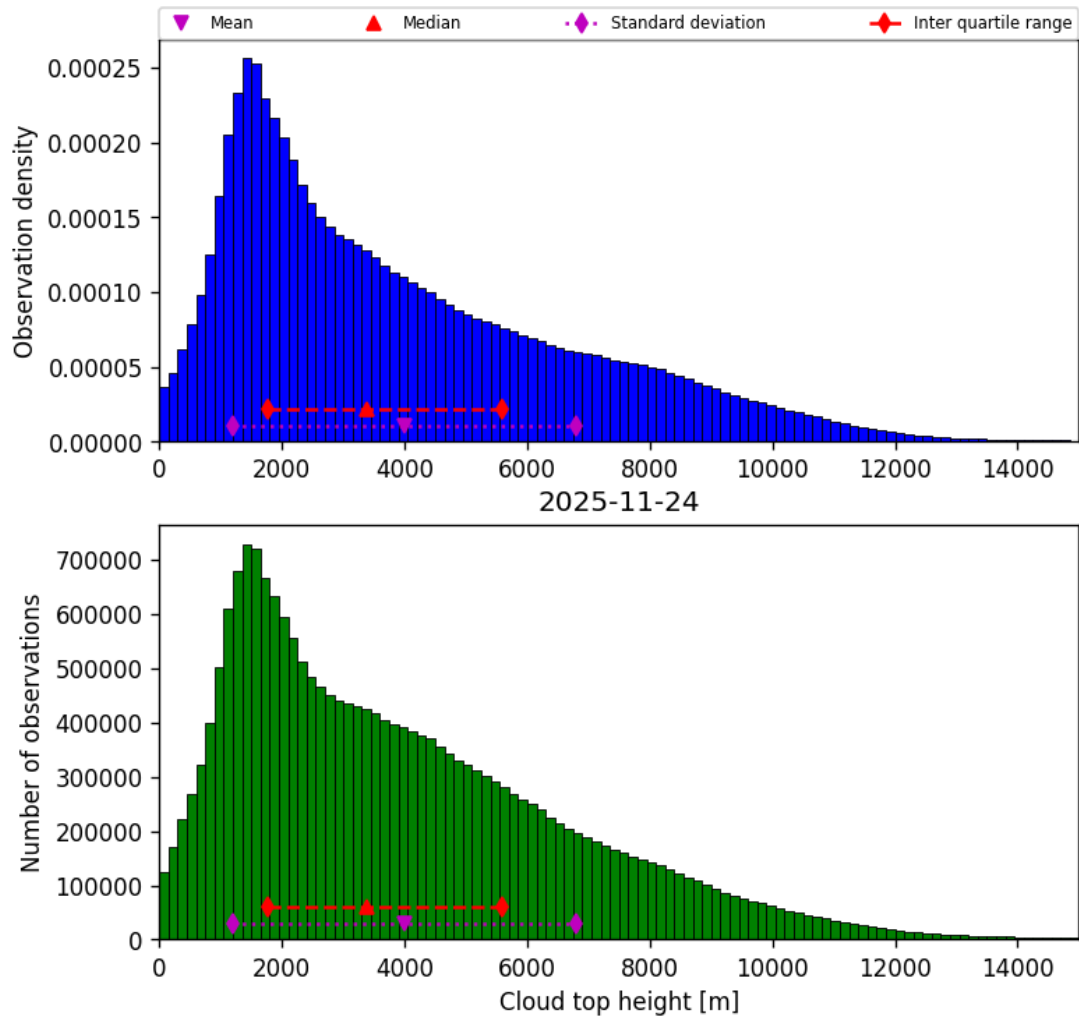
Figure 40: Histogram of “Cloud top height” for 2025-11-23 to 2025-11-25
