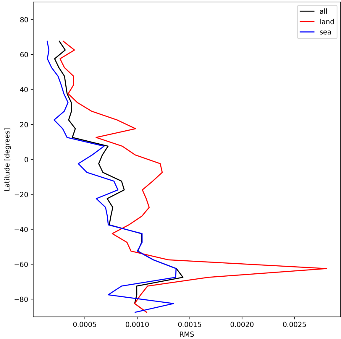
Figure 31: Zonal average of “RMS” for 2025-11-23 to 2025-11-25.
