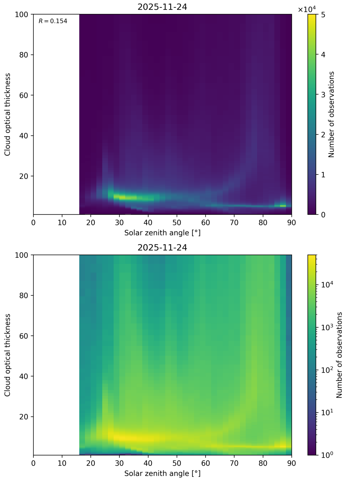
Figure 103: Scatter density plot of “Solar zenith angle” against “Cloud optical thickness” for 2025-11-23 to 2025-11-25.
