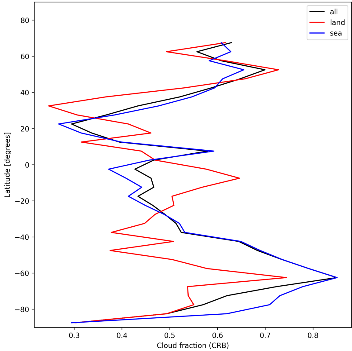
Figure 26: Zonal average of “Cloud fraction (CRB)” for 2025-11-23 to 2025-11-25.
