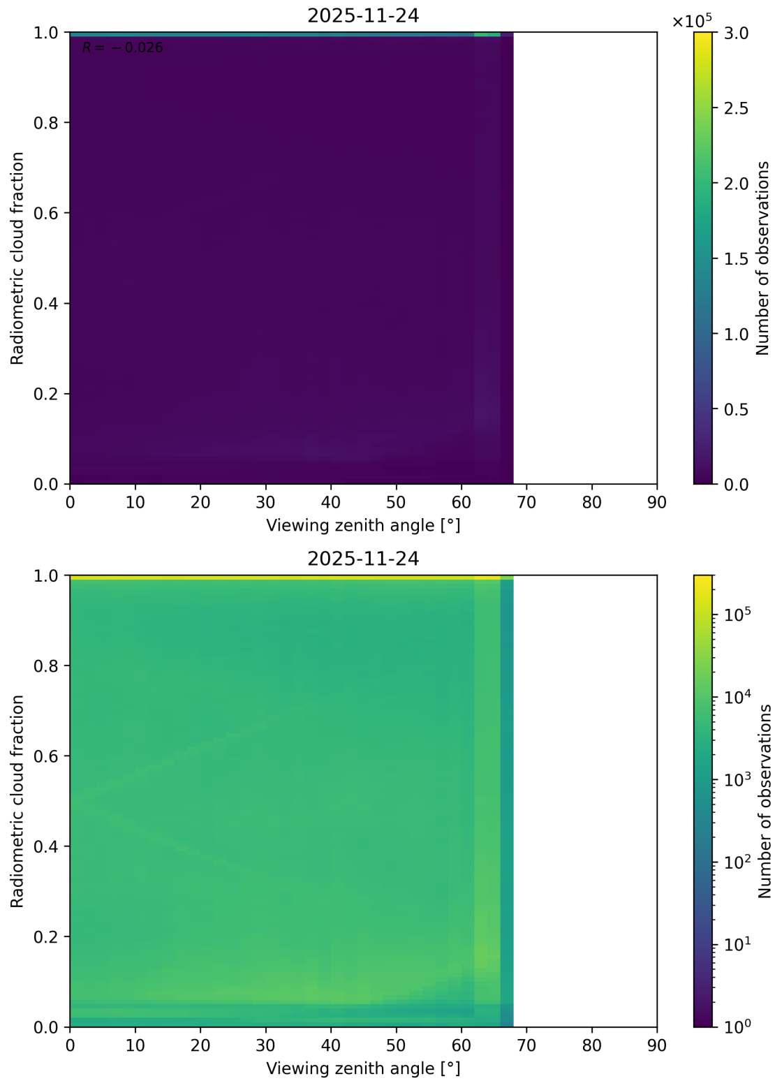
Figure 107: Scatter density plot of “Viewing zenith angle” against “Radiometric cloud fraction” for 2025-11-23 to 2025-11-25.
