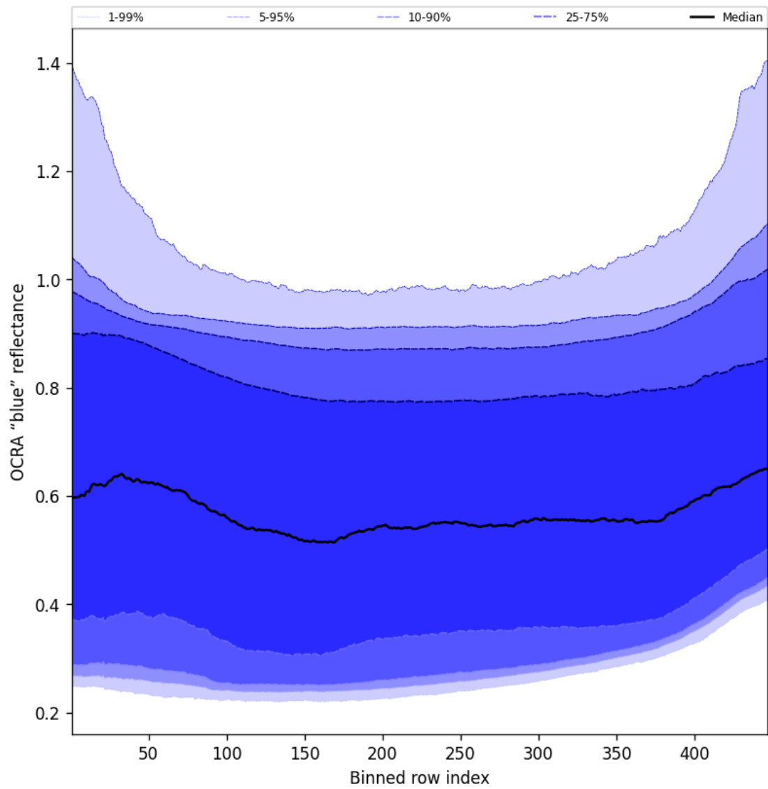
Figure 67: Along track statistics of “OCRA “blue” reflectance” for 2025-11-23 to 2025-11-25
