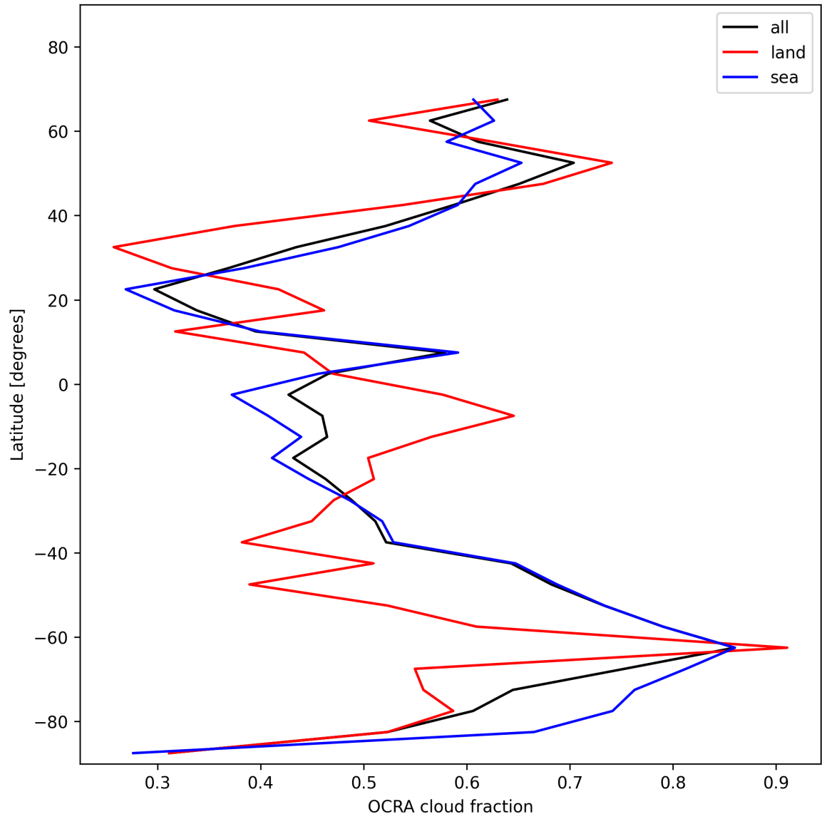
Figure 34: Zonal average of “OCRA cloud fraction” for 2025-11-23 to 2025-11-25.
