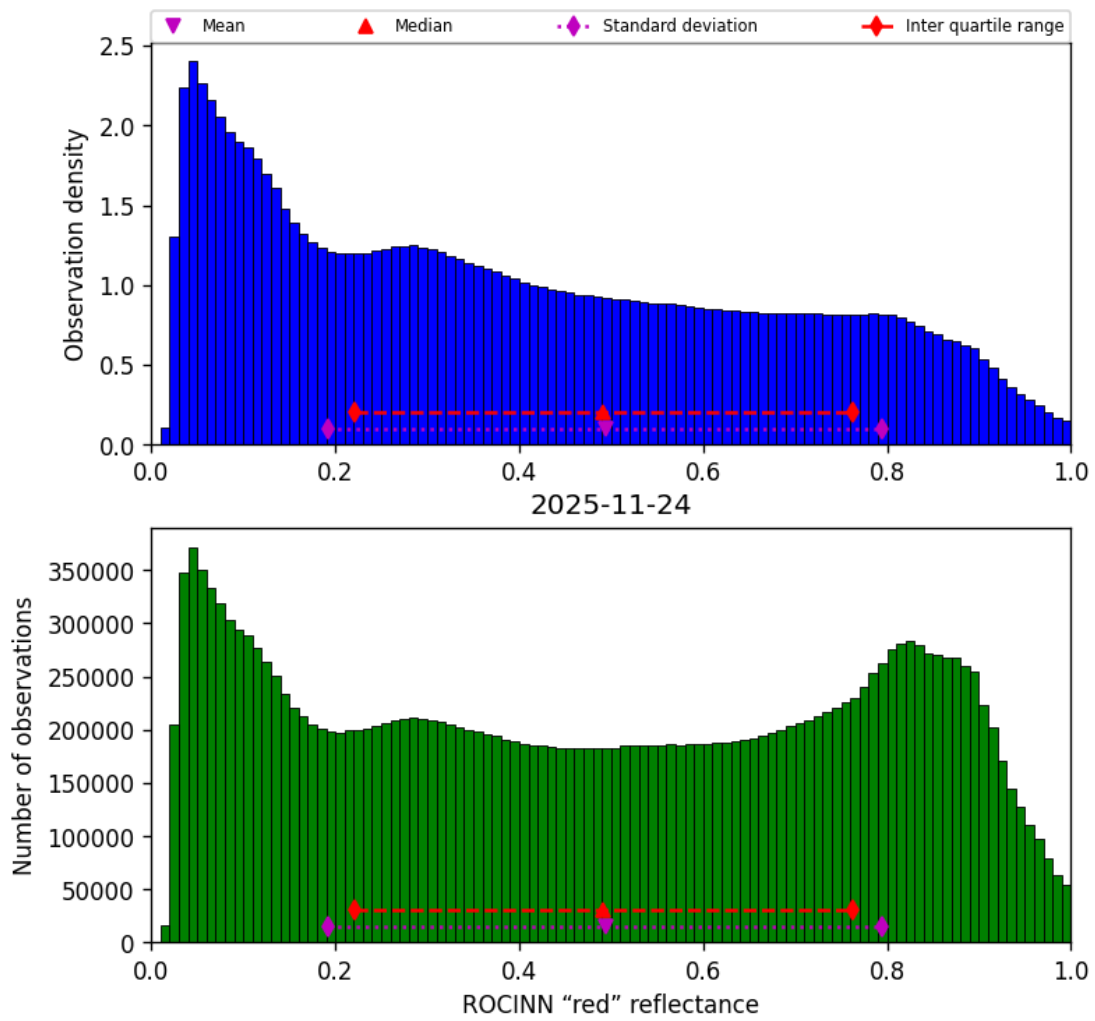
Figure 53: Histogram of “ROCINN “red” reflectance” for 2025-11-23 to 2025-11-25
