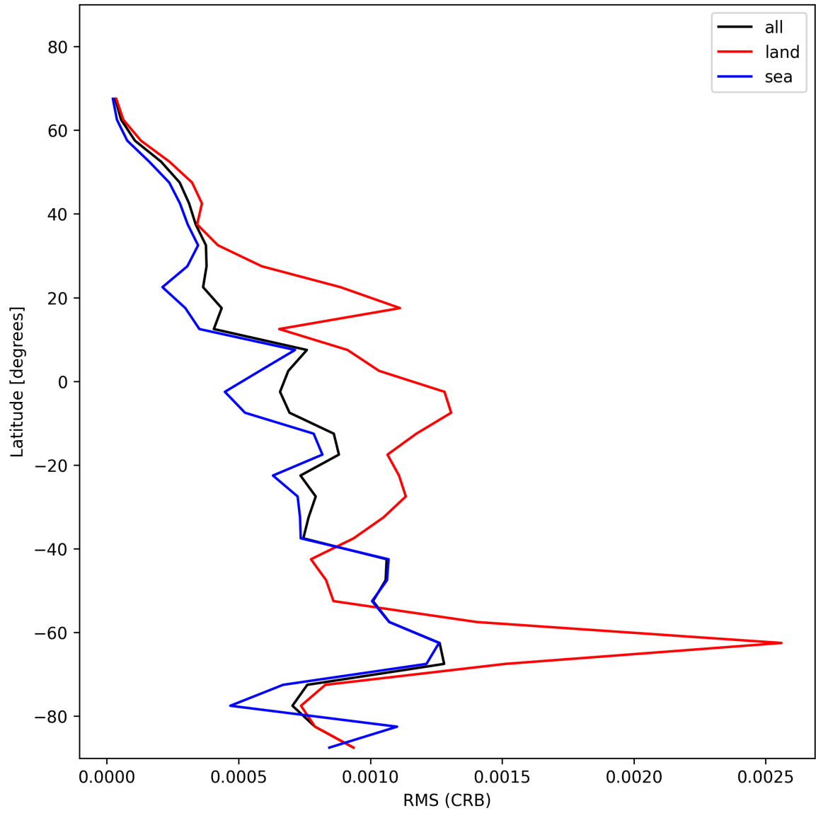
Figure 32: Zonal average of “RMS (CRB)” for 2025-11-23 to 2025-11-25.
