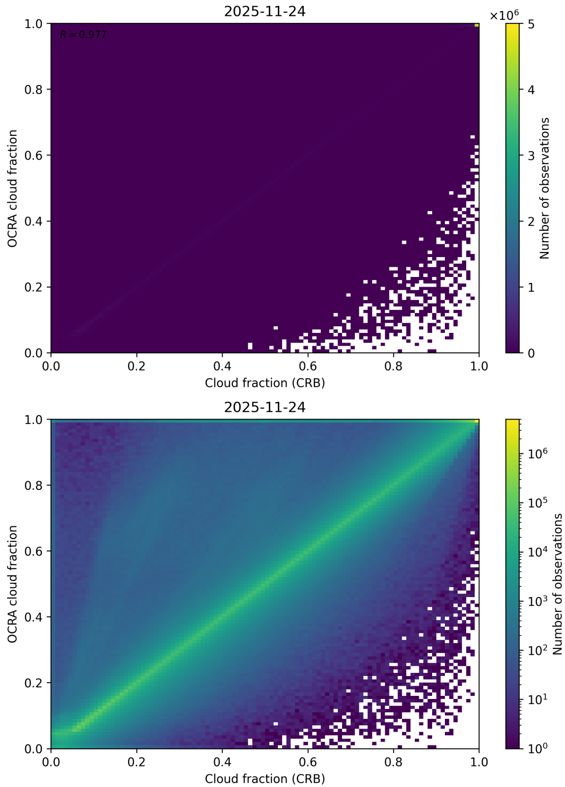
Figure 78: Scatter density plot of “Cloud fraction (CRB)” against “OCRA cloud fraction” for 2025-11-23 to 2025-11-25.
