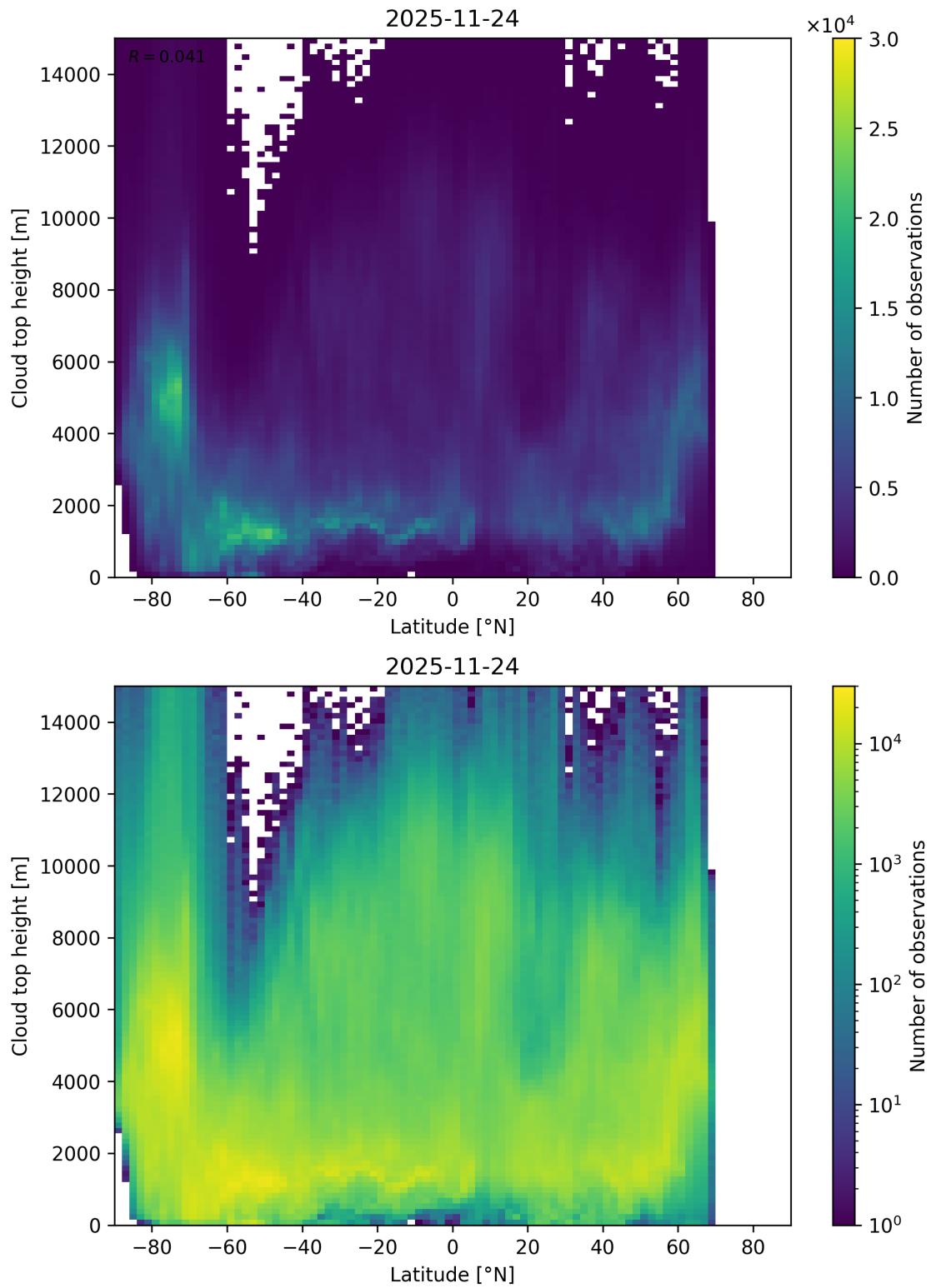
Figure 97: Scatter density plot of “Latitude” against “Cloud top height” for 2025-11-23 to 2025-11-25.
