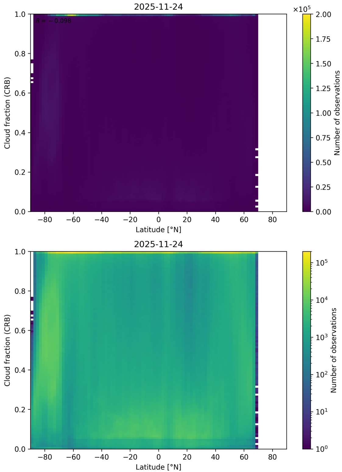
Figure 94: Scatter density plot of “Latitude” against “Cloud fraction (CRB)” for 2025-11-23 to 2025-11-25.
