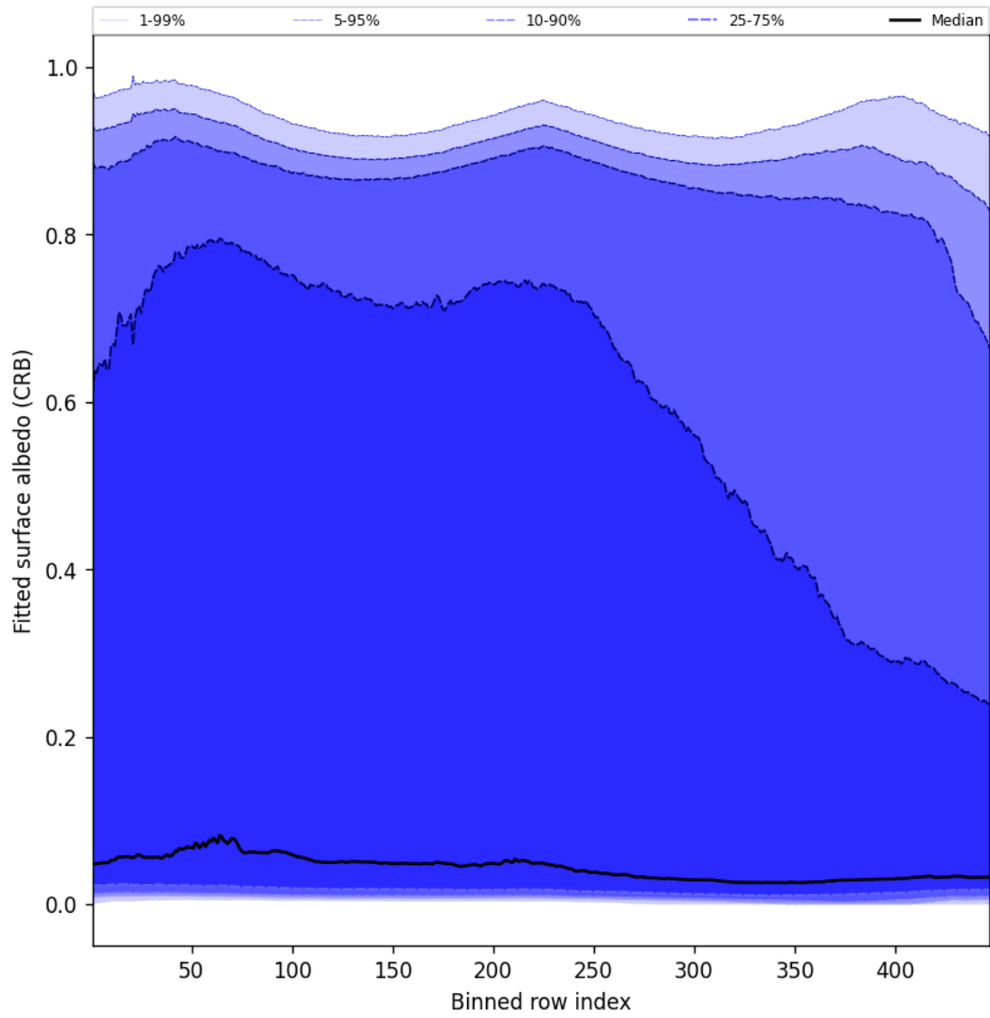
Figure 62: Along track statistics of “Fitted surface albedo (CRB)” for 2025-11-23 to 2025-11-25
