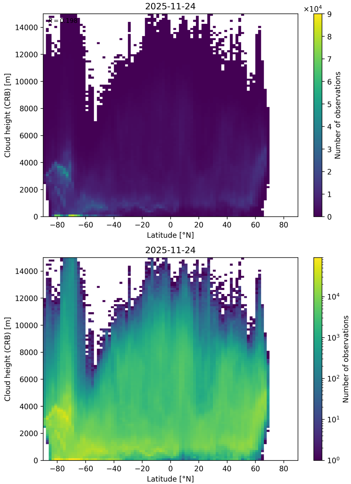
Figure 95: Scatter density plot of “Latitude” against “Cloud height (CRB)” for 2025-11-23 to 2025-11-25.
