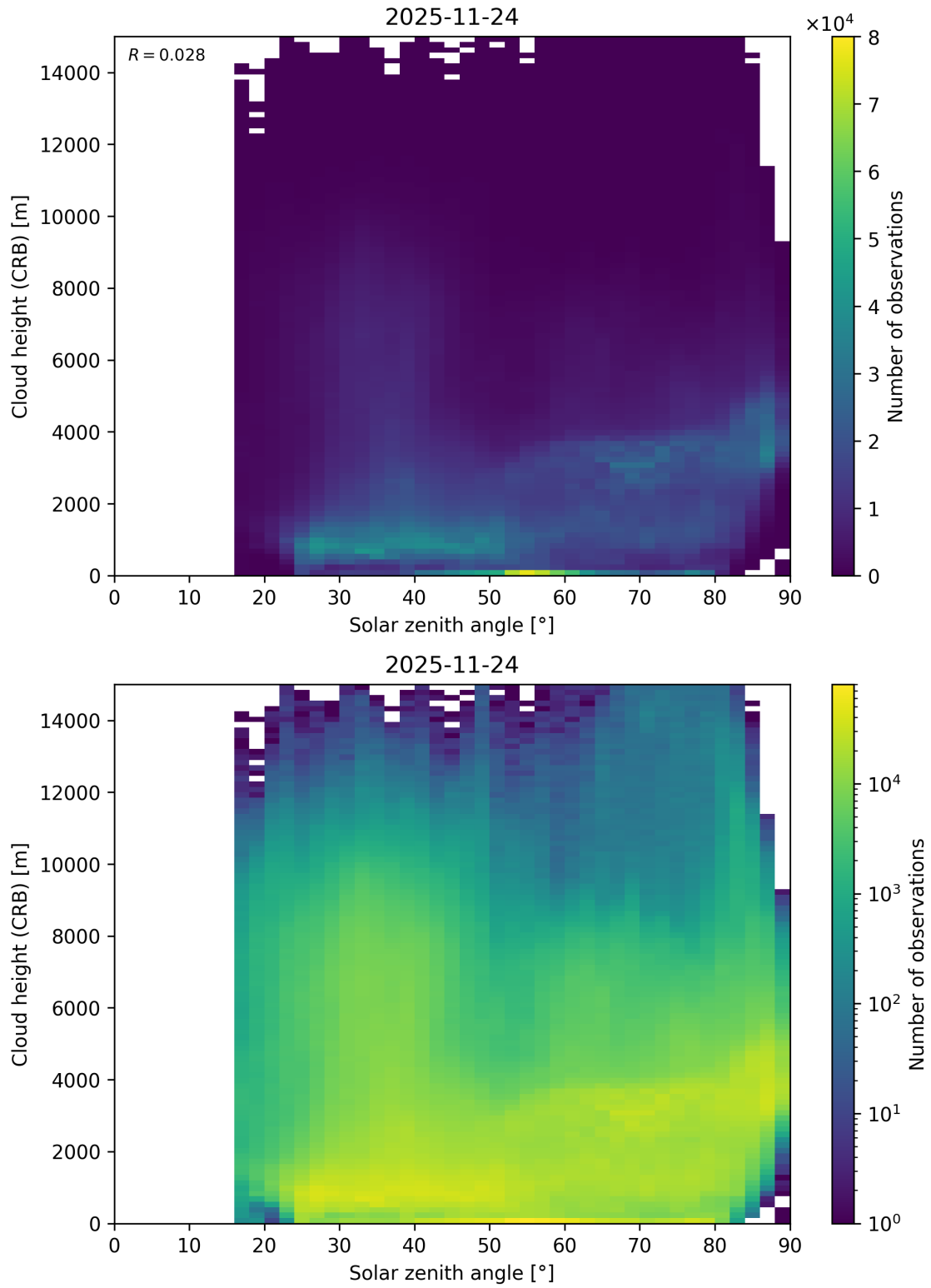
Figure 102: Scatter density plot of “Solar zenith angle” against “Cloud height (CRB)” for 2025-11-23 to 2025-11-25.
