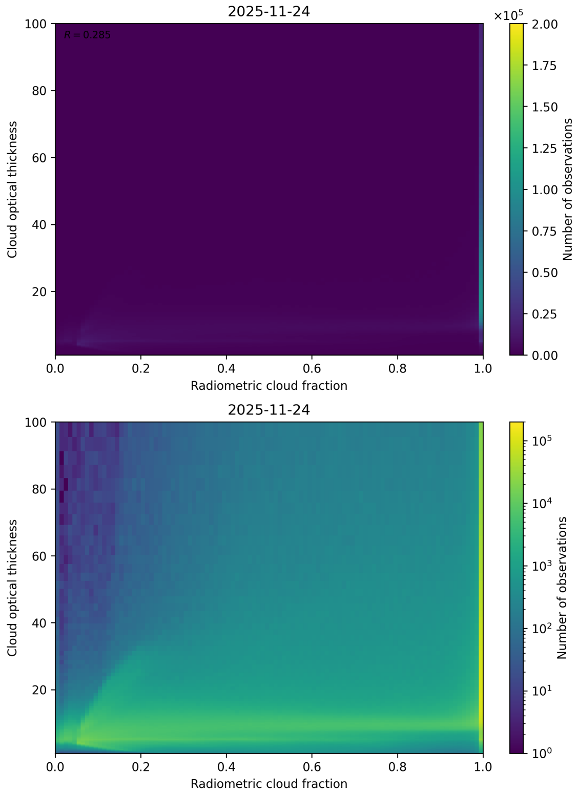
Figure 75: Scatter density plot of “Radiometric cloud fraction” against “Cloud optical thickness” for 2025-11-23 to 2025-11-25.
