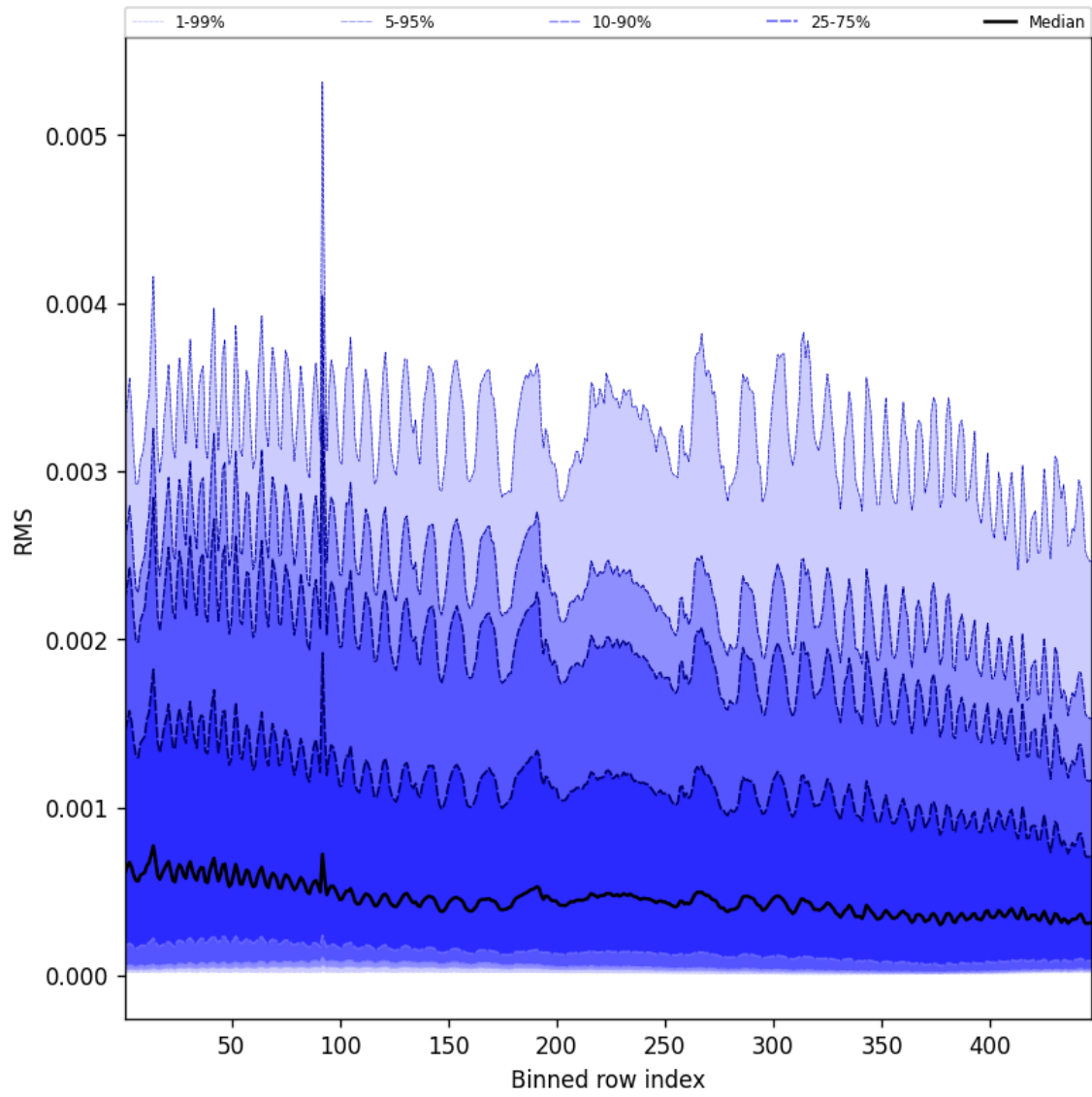
Figure 63: Along track statistics of “RMS” for 2025-11-23 to 2025-11-25
