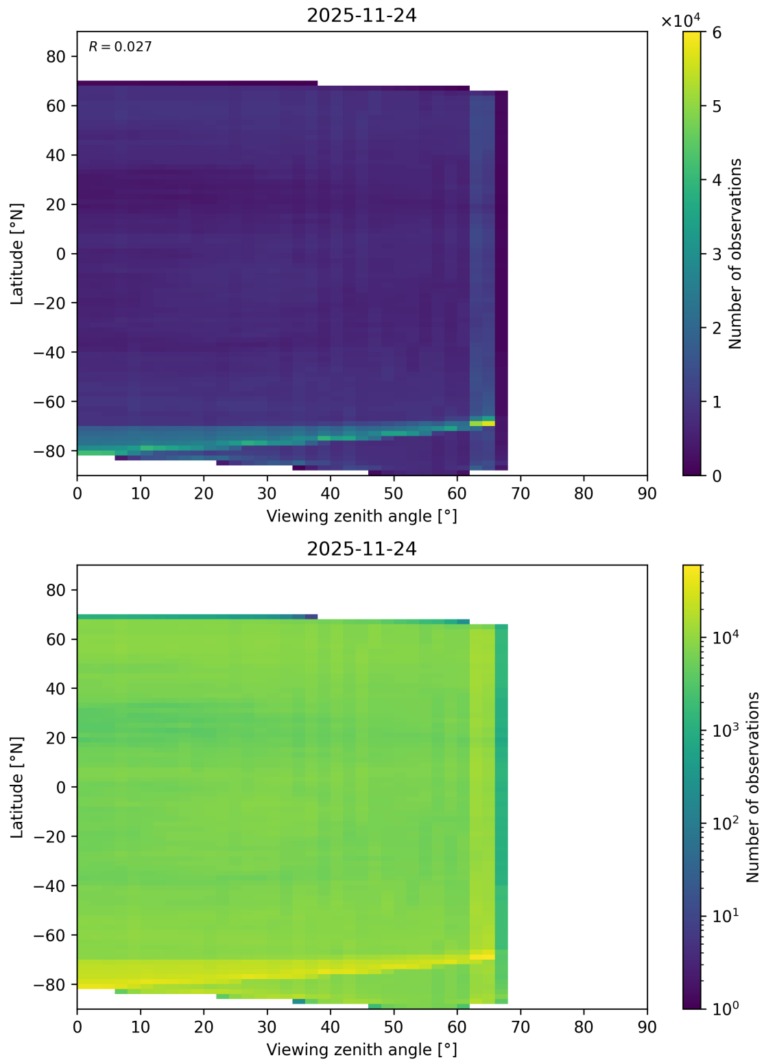
Figure 113: Scatter density plot of “Viewing zenith angle” against “Latitude” for 2025-11-23 to 2025-11-25.
