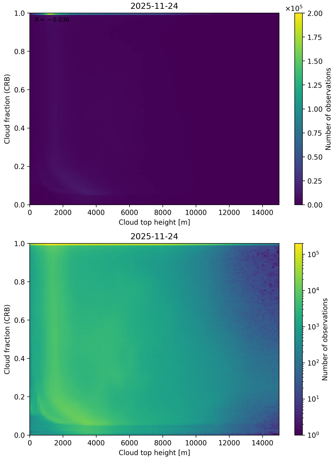
Figure 88: Scatter density plot of “Cloud top height” against “Cloud fraction (CRB)” for 2025-11-23 to 2025-11-25.
