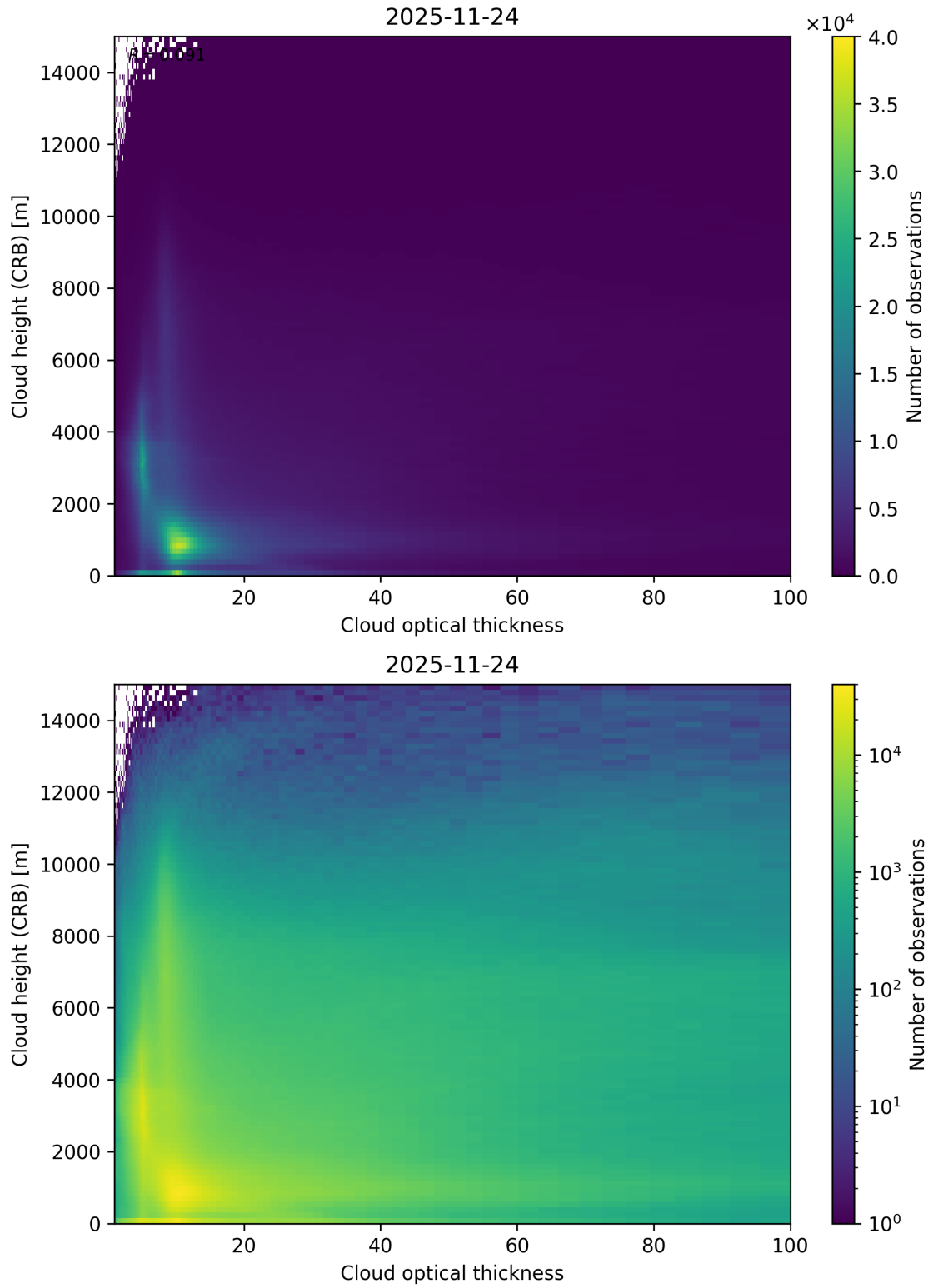
Figure 85: Scatter density plot of “Cloud optical thickness” against “Cloud height (CRB)” for 2025-11-23 to 2025-11-25.
