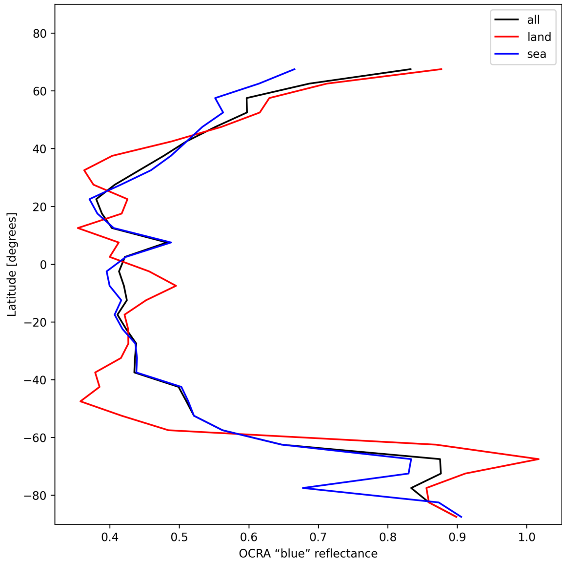
Figure 35: Zonal average of “OCRA “blue” reflectance” for 2025-11-23 to 2025-11-25.
