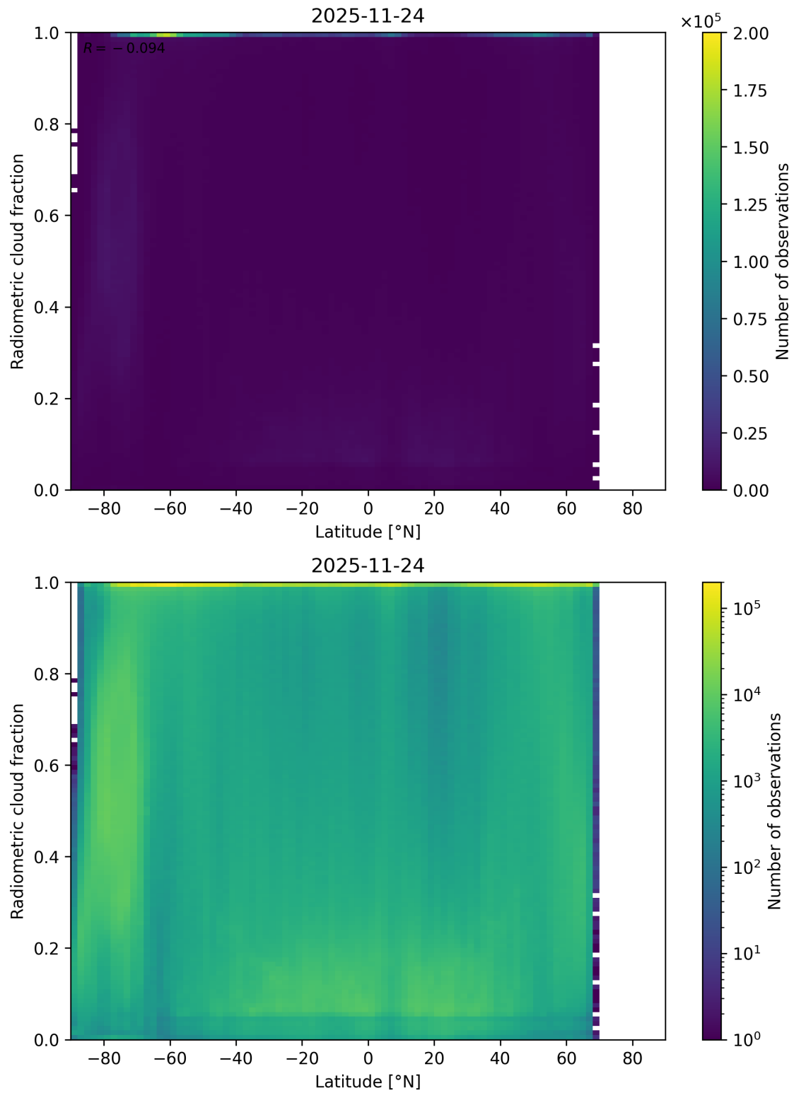
Figure 92: Scatter density plot of “Latitude” against “Radiometric cloud fraction” for 2025-11-23 to 2025-11-25.
