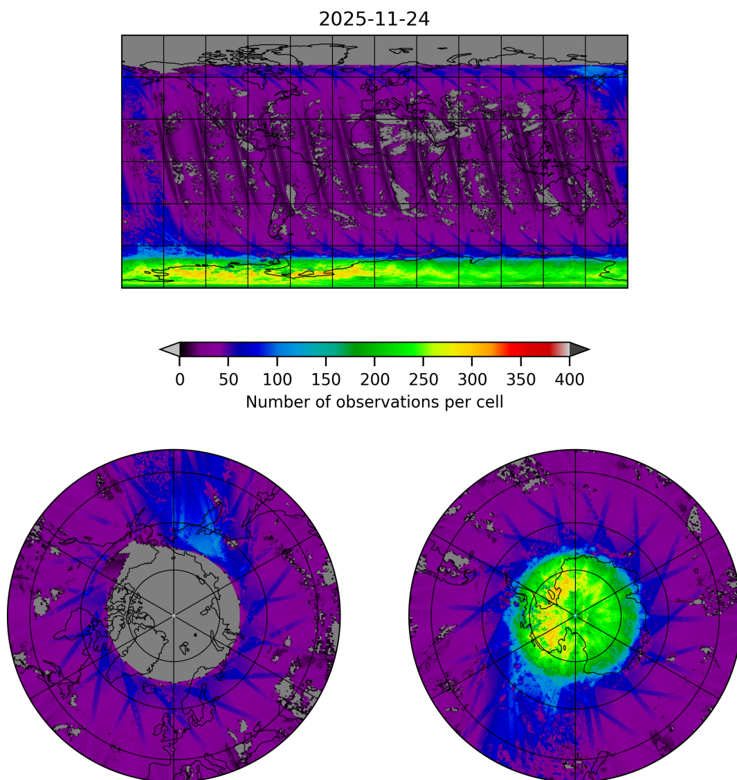
Figure 21: Map of the number of observations for 2025-11-23 to 2025-11-25
