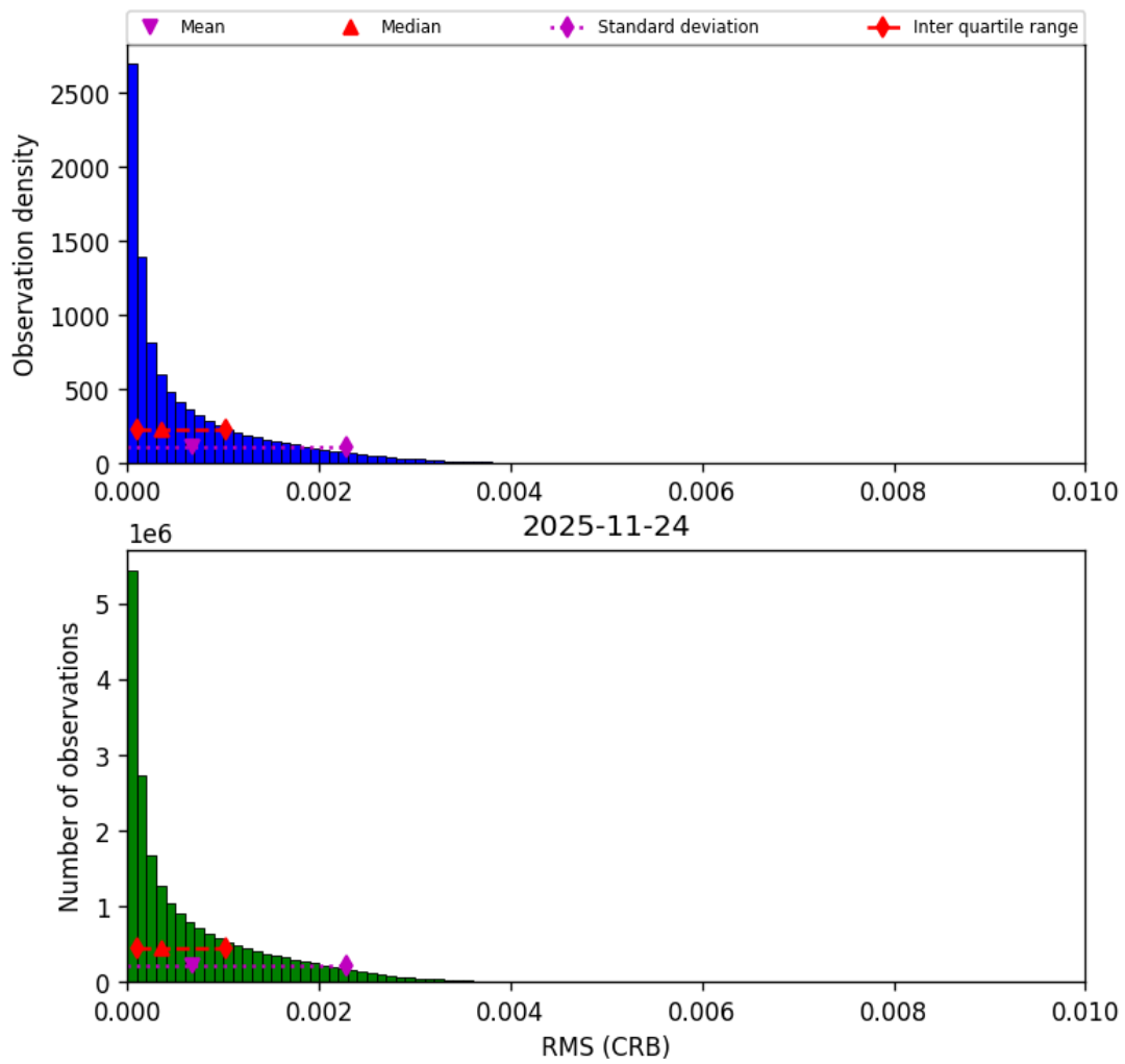
Figure 48: Histogram of “RMS (CRB)” for 2025-11-23 to 2025-11-25
