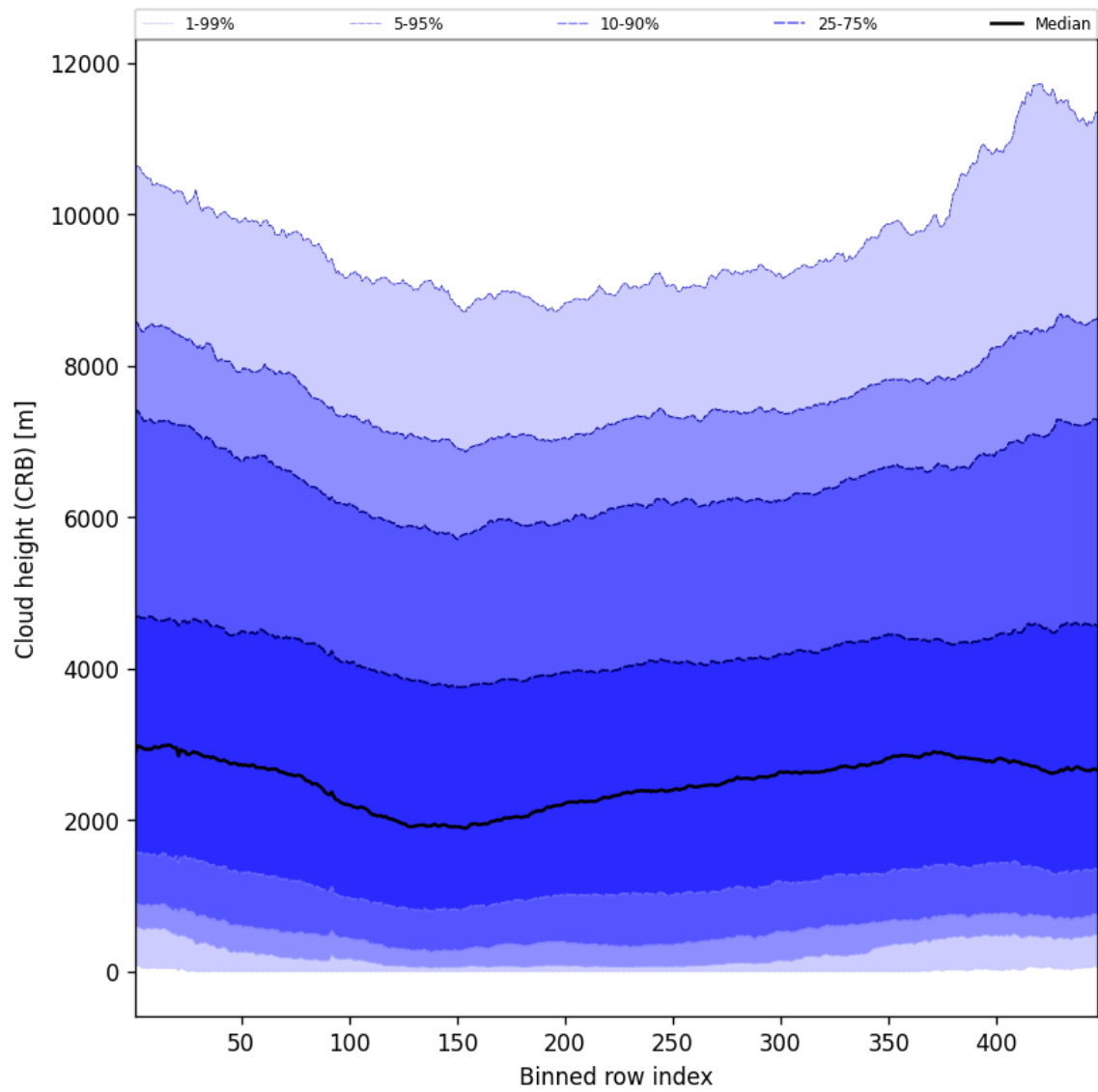
Figure 59: Along track statistics of “Cloud height (CRB)” for 2025-11-23 to 2025-11-25
