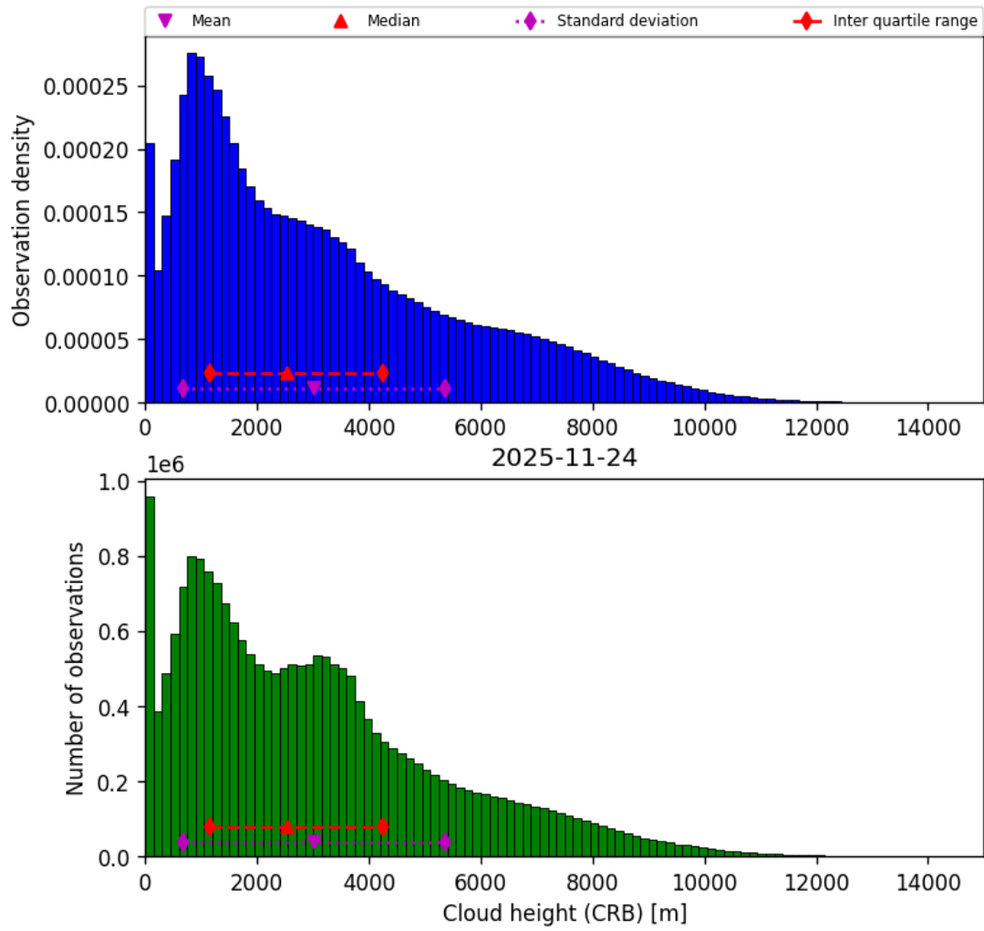
Figure 43: Histogram of “Cloud height (CRB)” for 2025-11-23 to 2025-11-25
