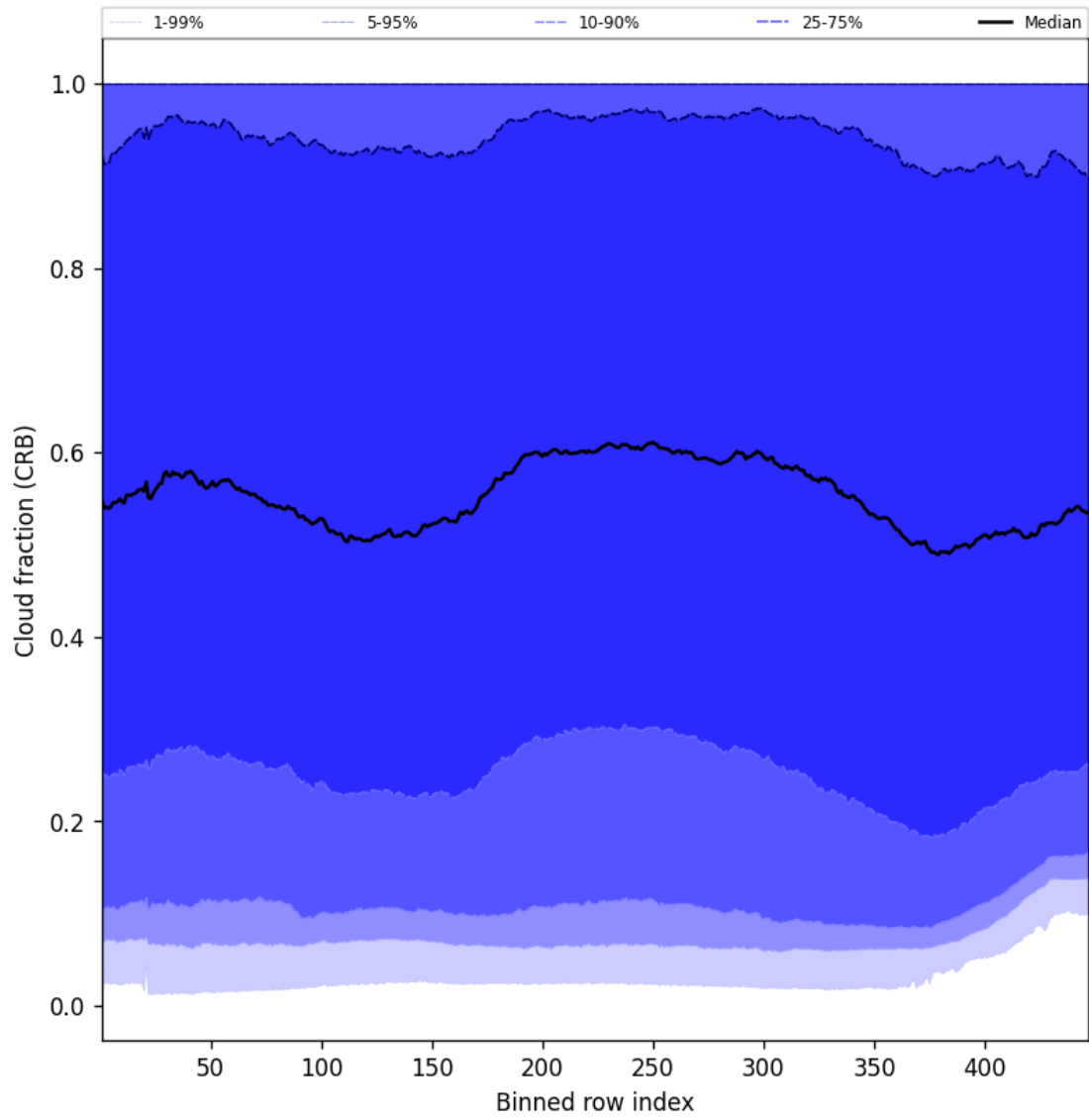
Figure 58: Along track statistics of “Cloud fraction (CRB)” for 2025-11-23 to 2025-11-25
