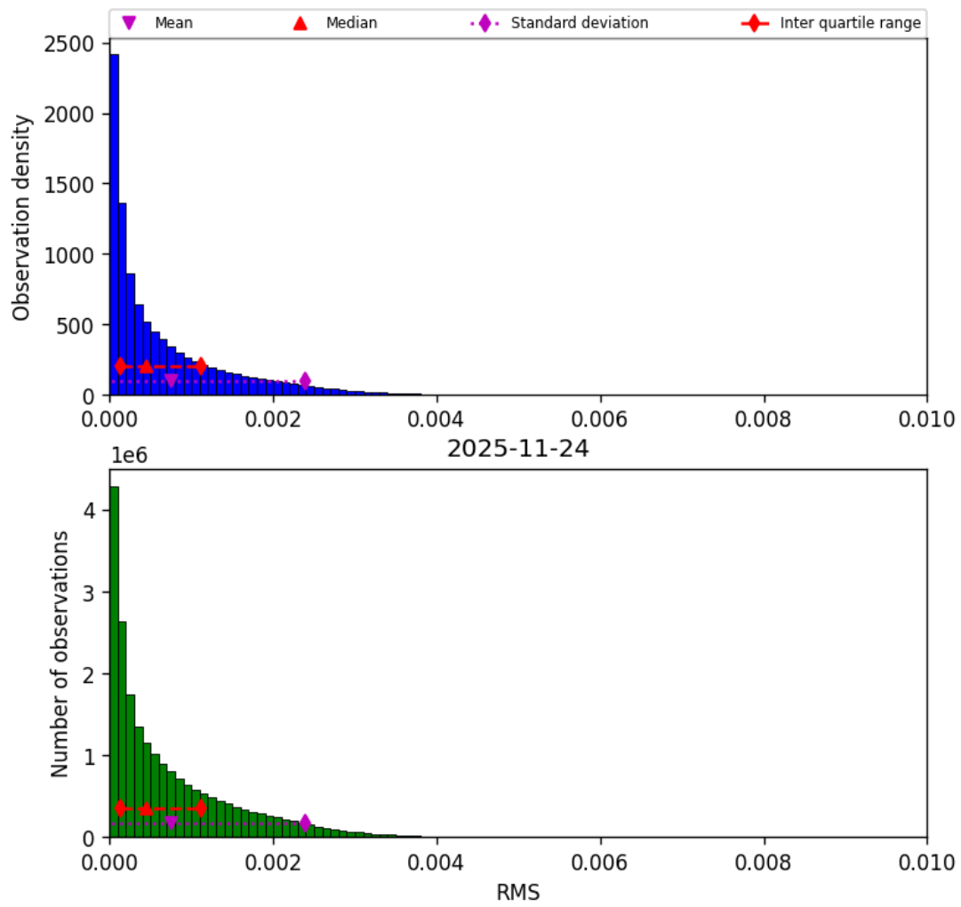
Figure 47: Histogram of “RMS” for 2025-11-23 to 2025-11-25
