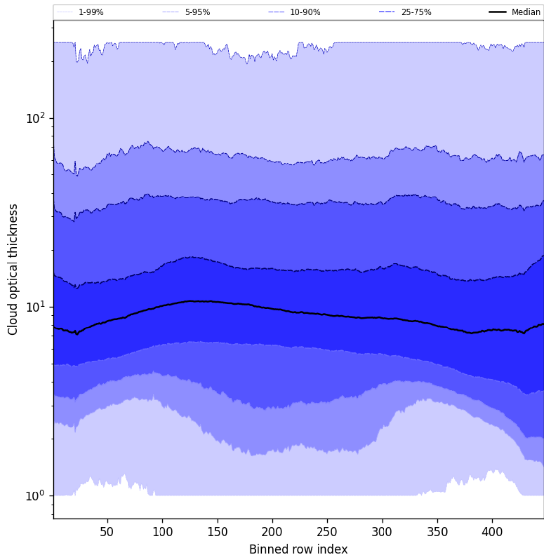
Figure 57: Along track statistics of “Cloud optical thickness” for 2025-11-23 to 2025-11-25
