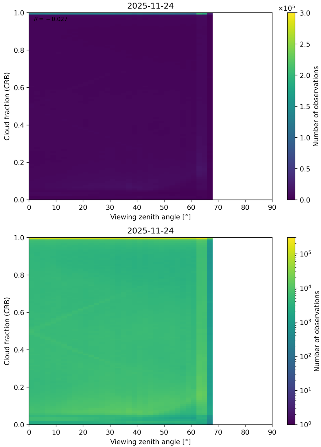
Figure 109: Scatter density plot of “Viewing zenith angle” against “Cloud fraction (CRB)” for 2025-11-23 to 2025-11-25.
