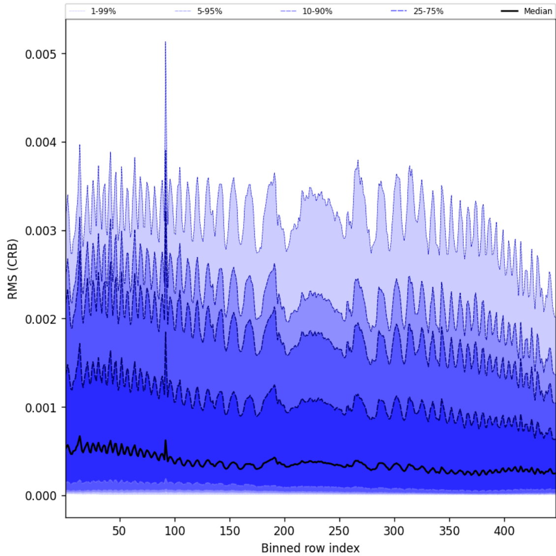
Figure 64: Along track statistics of “RMS (CRB)” for 2025-11-23 to 2025-11-25
