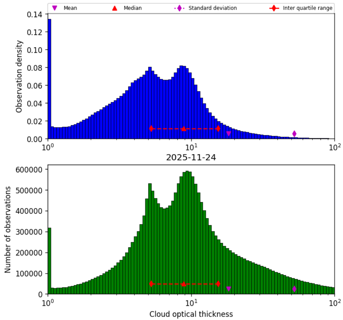
Figure 41: Histogram of “Cloud optical thickness” for 2025-11-23 to 2025-11-25
