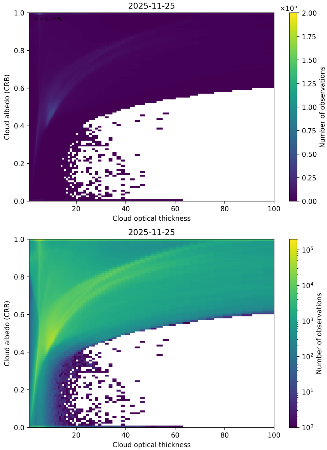
Figure 82: Scatter density plot of “Cloud optical thickness” against “Cloud albedo (CRB)” for 2025-11-24 to 2025-11-26.
