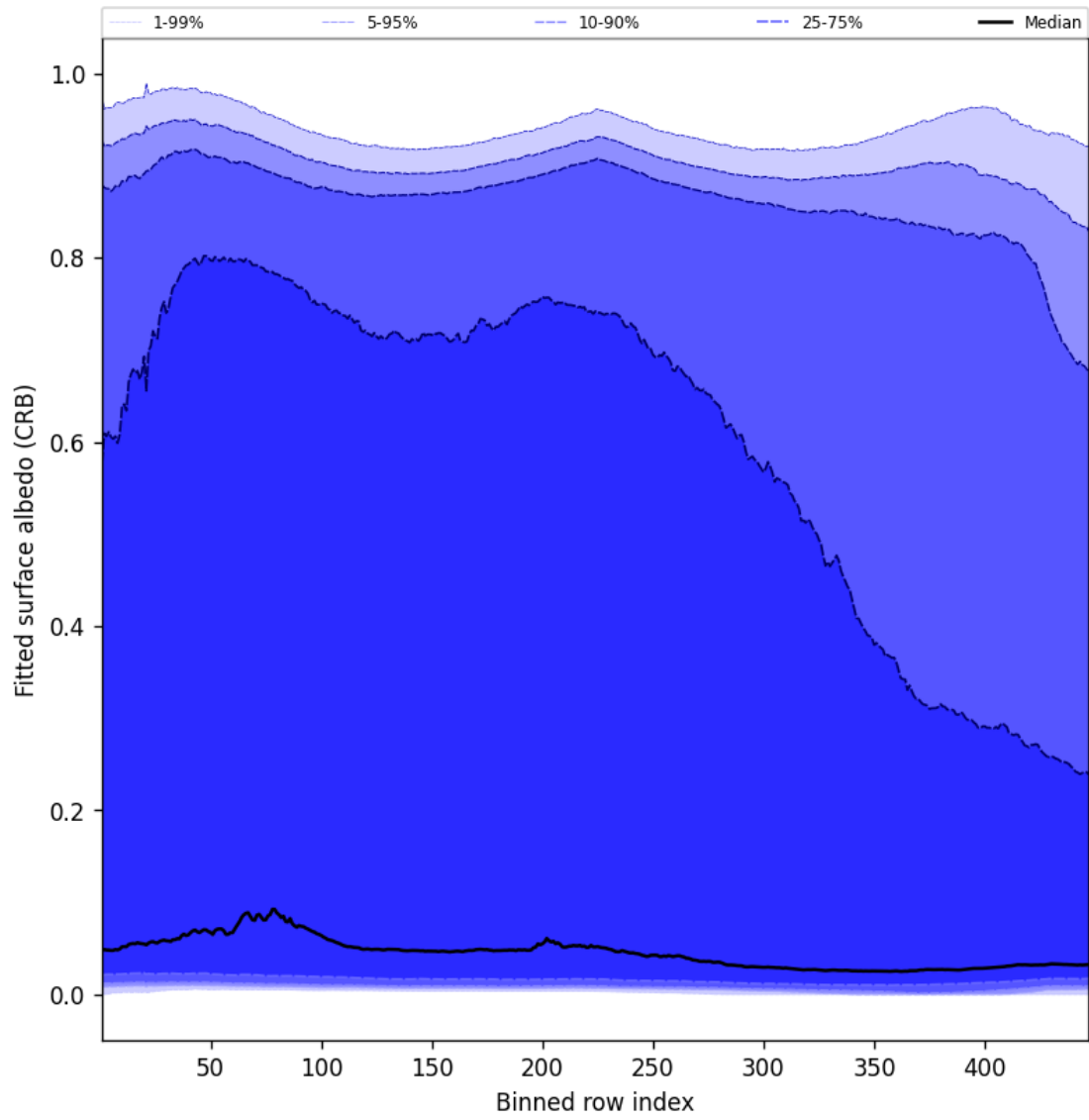
Figure 62: Along track statistics of “Fitted surface albedo (CRB)” for 2025-11-24 to 2025-11-26
