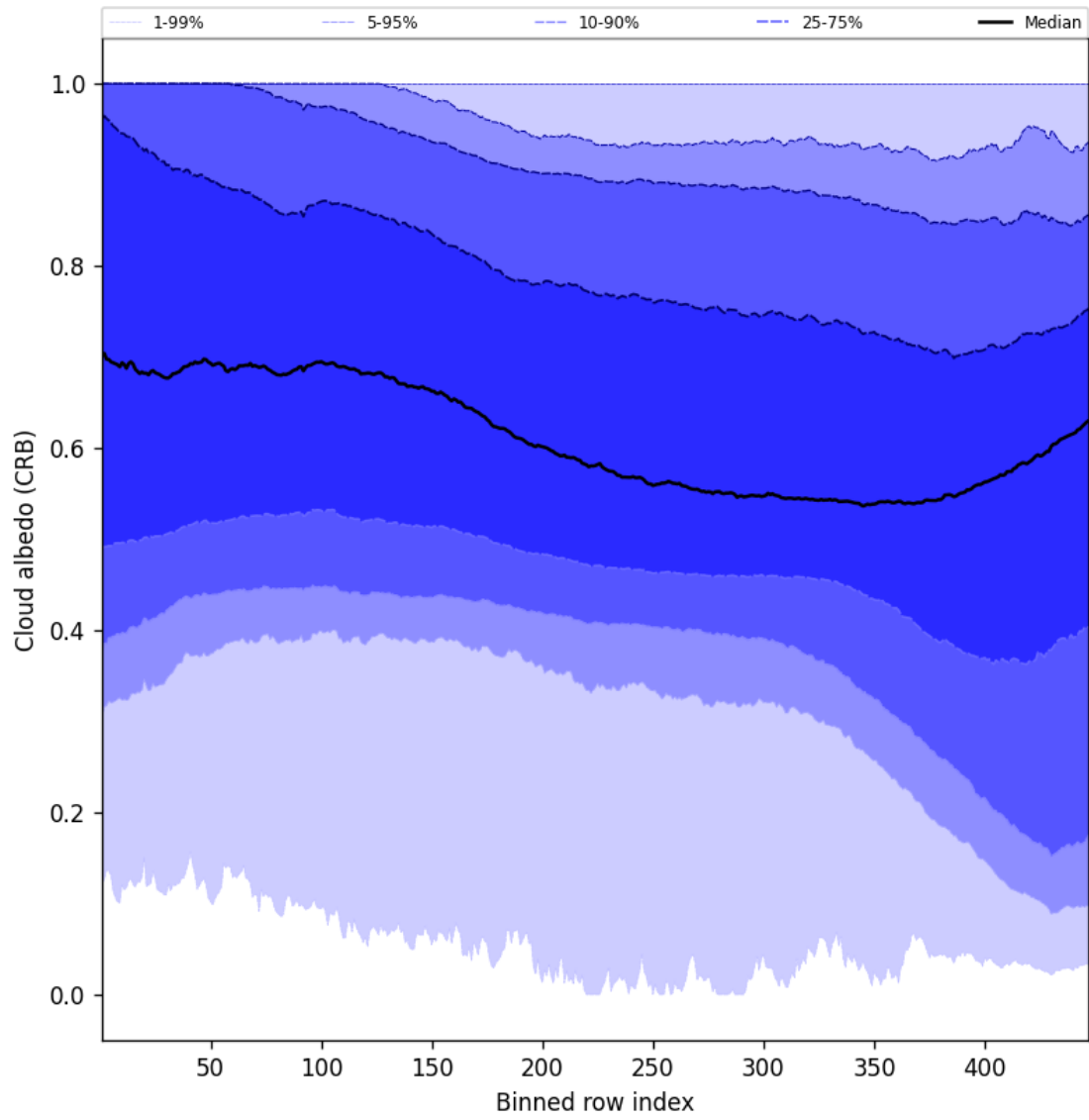
Figure 60: Along track statistics of “Cloud albedo (CRB)” for 2025-11-24 to 2025-11-26
