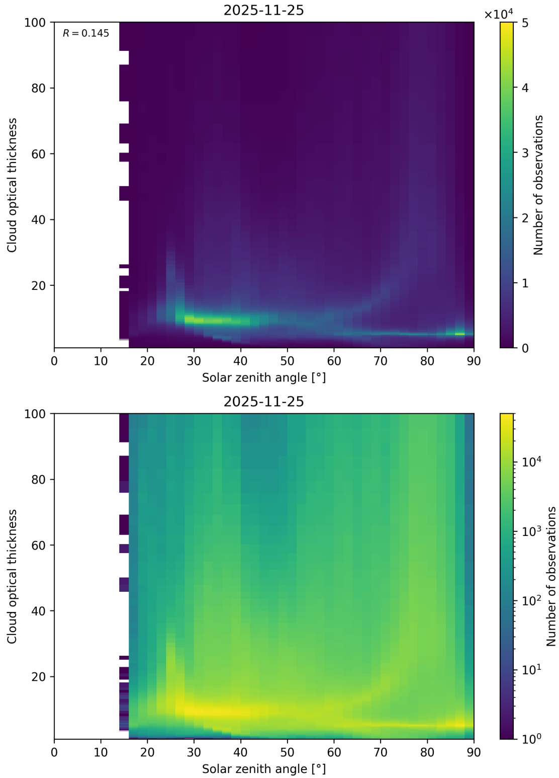
Figure 103: Scatter density plot of “Solar zenith angle” against “Cloud optical thickness” for 2025-11-24 to 2025-11-26.
