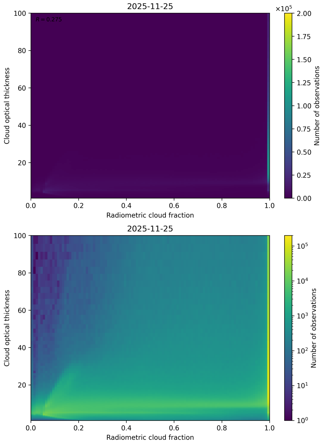
Figure 75: Scatter density plot of “Radiometric cloud fraction” against “Cloud optical thickness” for 2025-11-24 to 2025-11-26.
