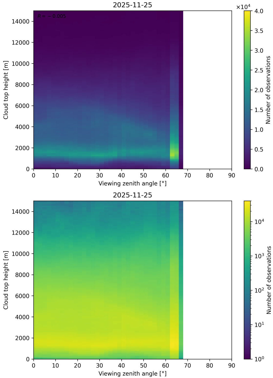
Figure 112: Scatter density plot of “Viewing zenith angle” against “Cloud top height” for 2025-11-24 to 2025-11-26.
