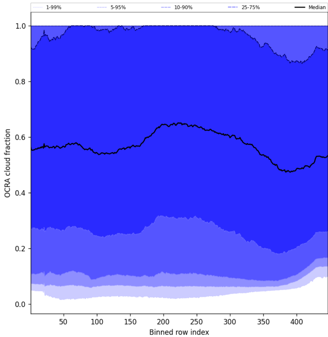
Figure 66: Along track statistics of “OCRA cloud fraction” for 2025-11-24 to 2025-11-26
