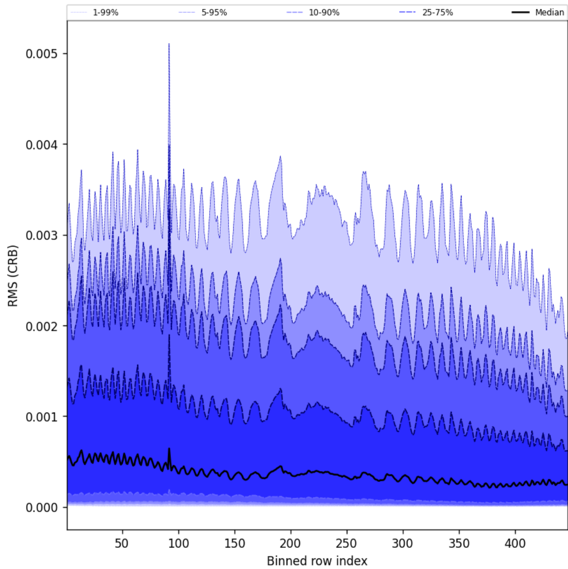
Figure 64: Along track statistics of “RMS (CRB)” for 2025-11-24 to 2025-11-26
