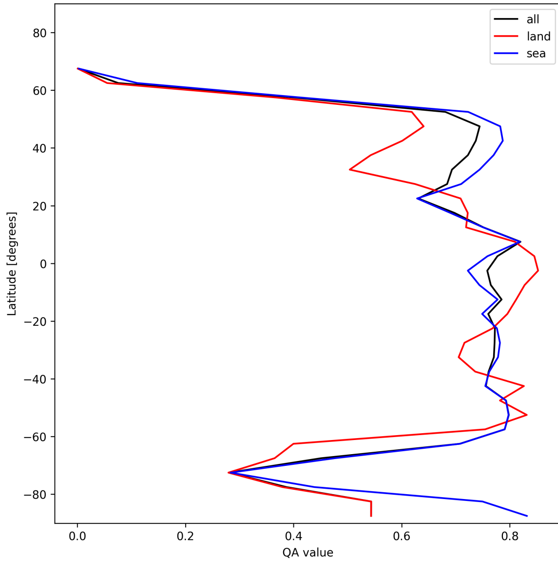
Figure 22: Zonal average of “QA value” for 2025-11-24 to 2025-11-26.
