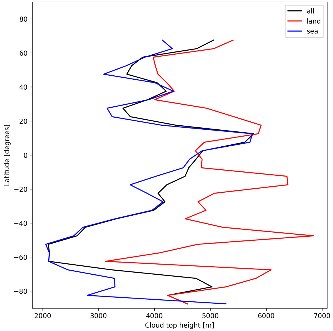
Figure 24: Zonal average of “Cloud top height” for 2025-11-24 to 2025-11-26.
