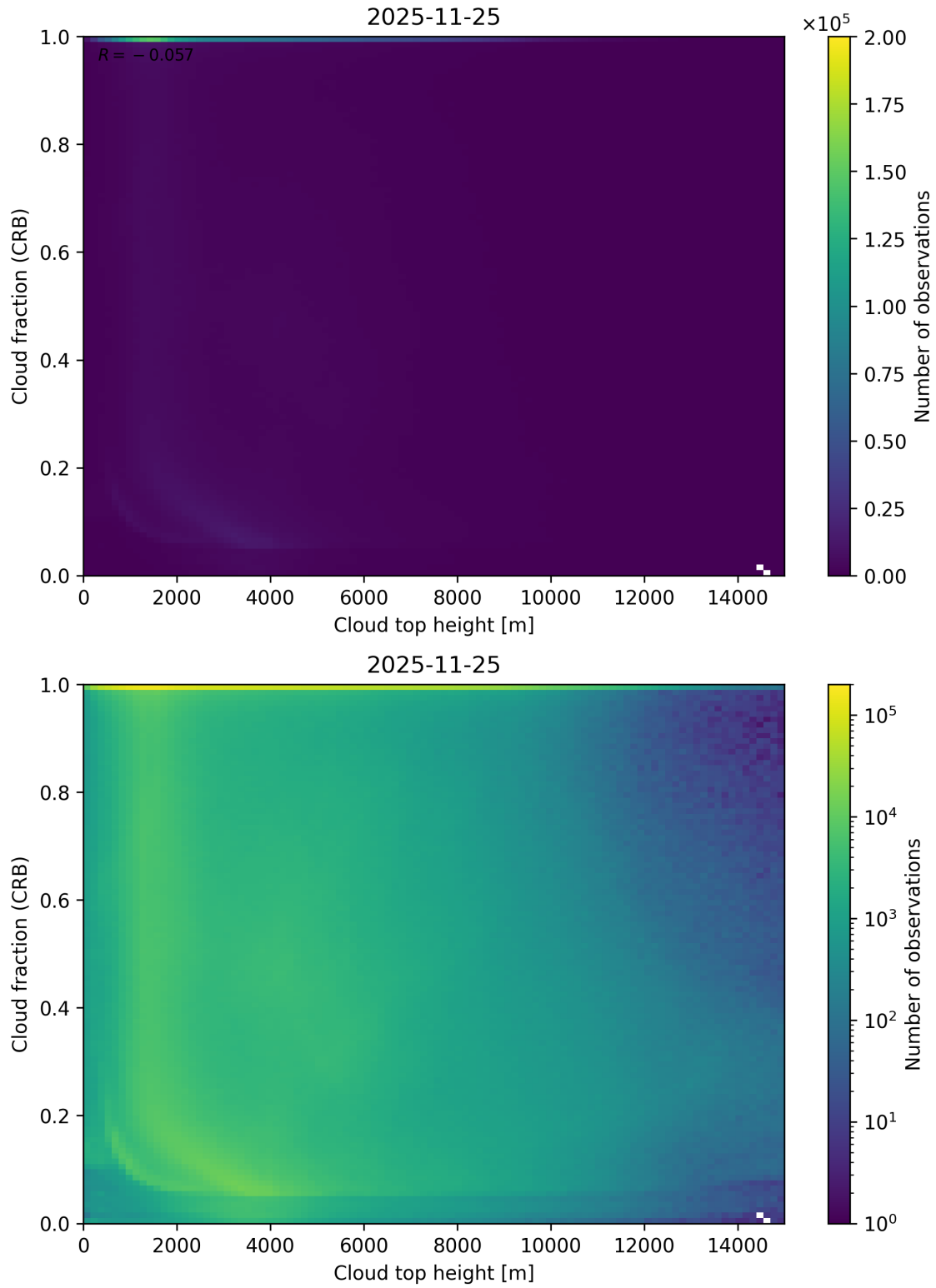
Figure 88: Scatter density plot of “Cloud top height” against “Cloud fraction (CRB)” for 2025-11-24 to 2025-11-26.
