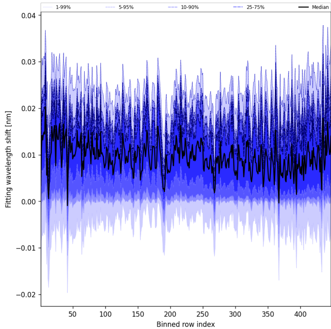
Figure 65: Along track statistics of “Fitting wavelength shift” for 2025-11-24 to 2025-11-26
