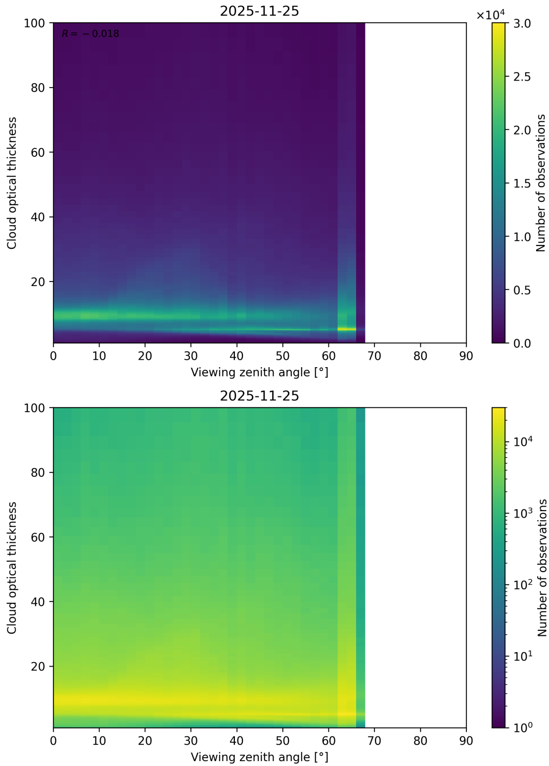
Figure 111: Scatter density plot of “Viewing zenith angle” against “Cloud optical thickness” for 2025-11-24 to 2025-11-26.
