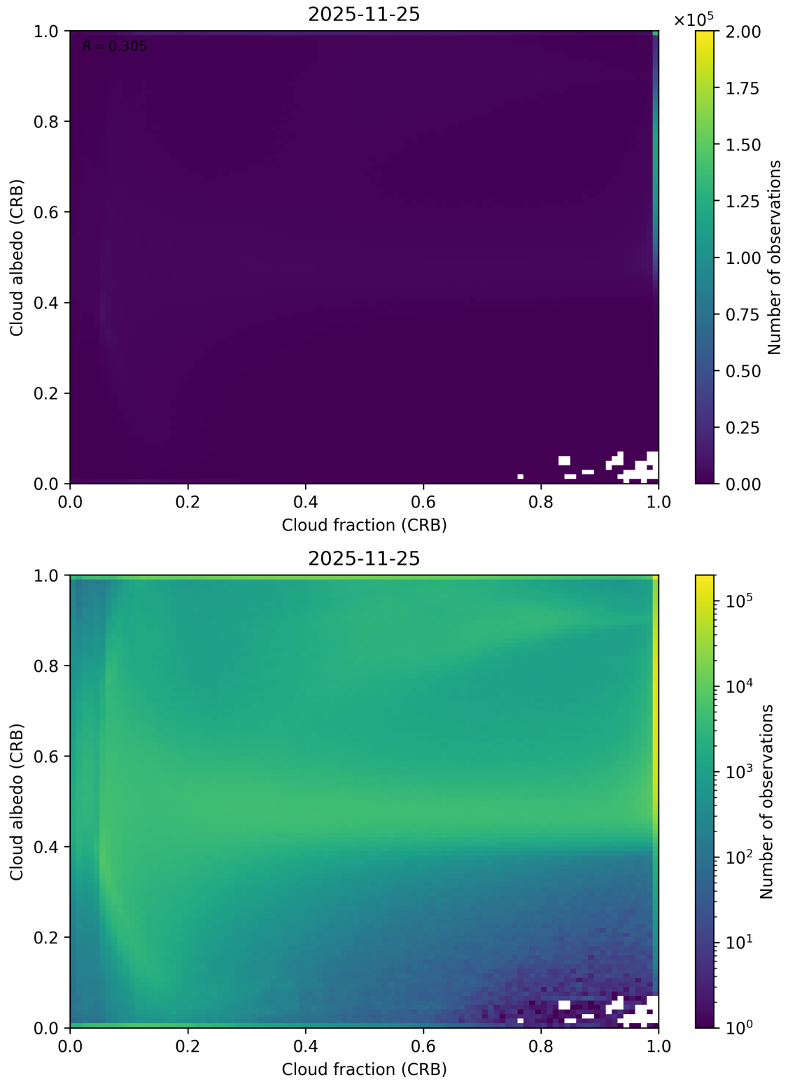
Figure 77: Scatter density plot of “Cloud fraction (CRB)” against “Cloud albedo (CRB)” for 2025-11-24 to 2025-11-26.
