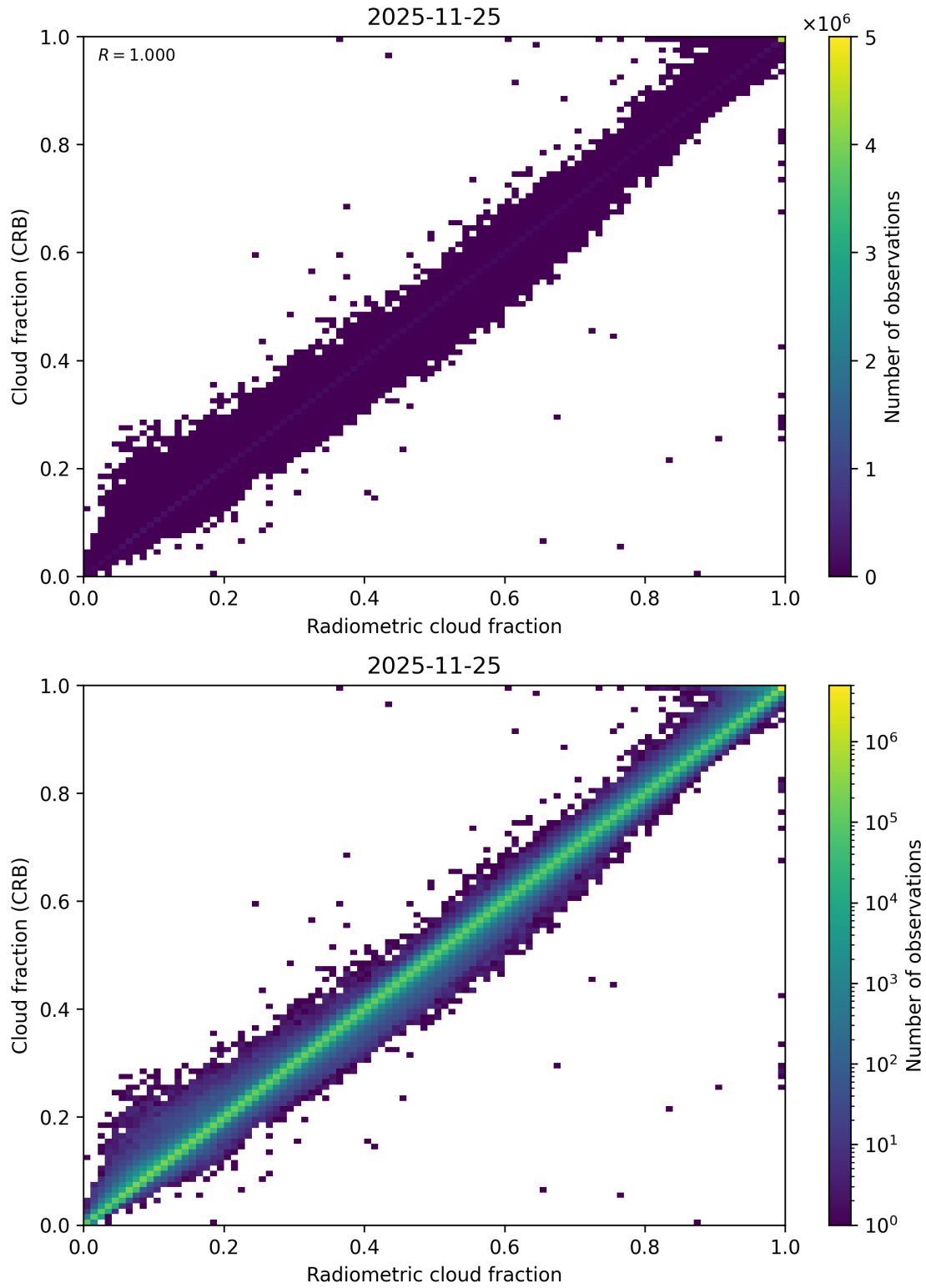
Figure 73: Scatter density plot of “Radiometric cloud fraction” against “Cloud fraction (CRB)” for 2025-11-24 to 2025-11-26.
