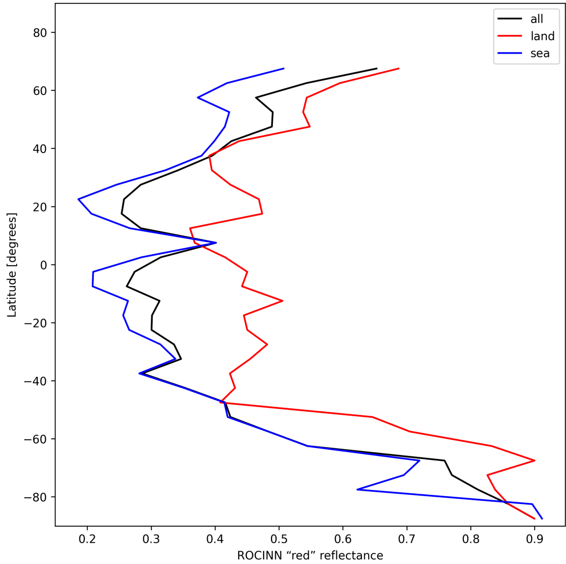
Figure 37: Zonal average of “ROCINN “red” reflectance” for 2025-11-24 to 2025-11-26.
