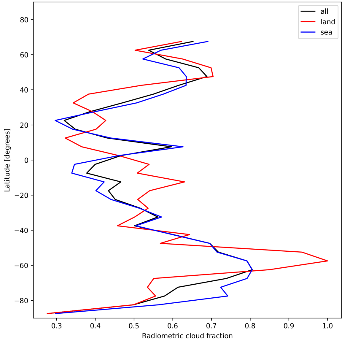
Figure 23: Zonal average of “Radiometric cloud fraction” for 2025-11-24 to 2025-11-26.
