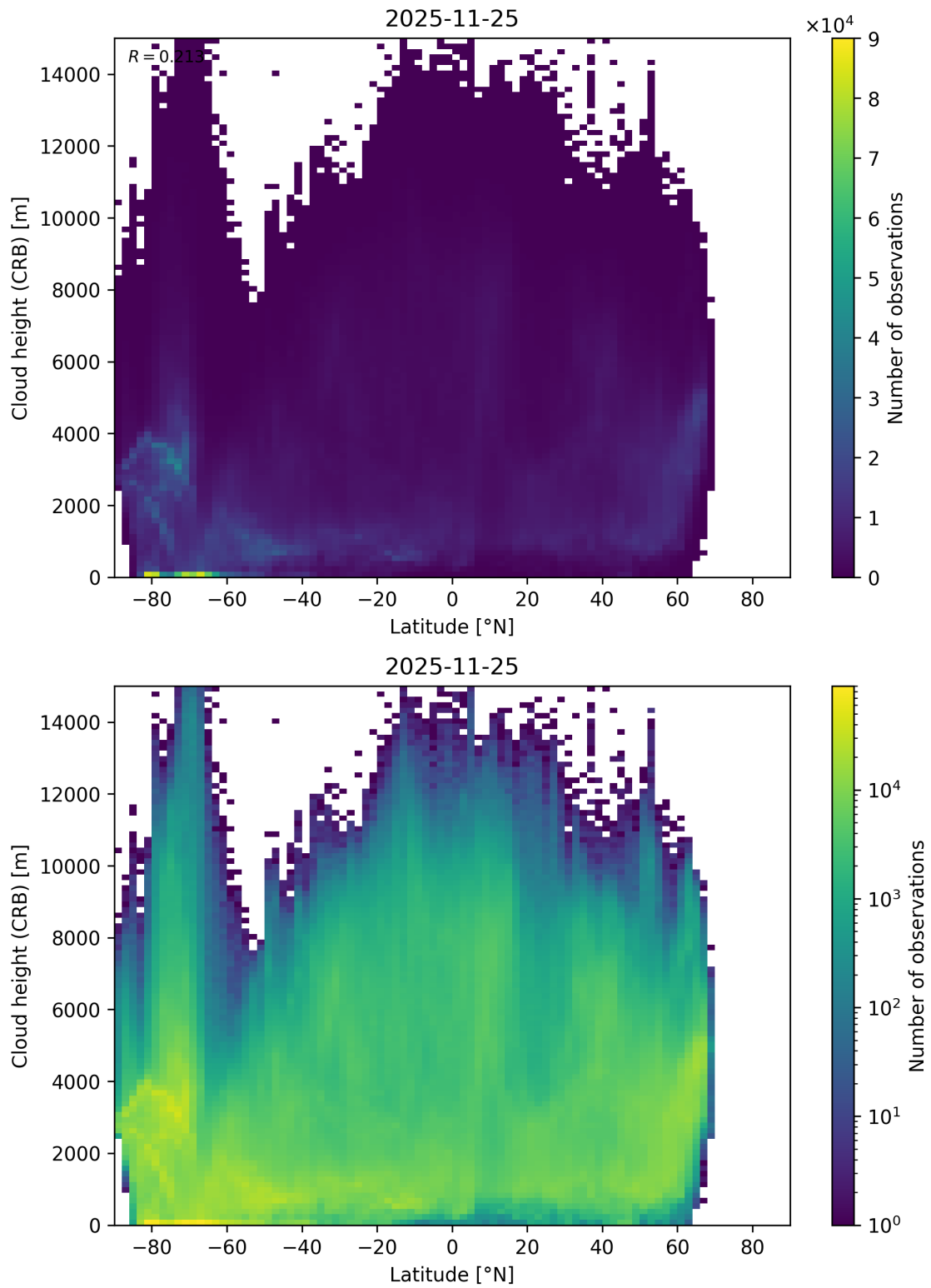
Figure 95: Scatter density plot of “Latitude” against “Cloud height (CRB)” for 2025-11-24 to 2025-11-26.
