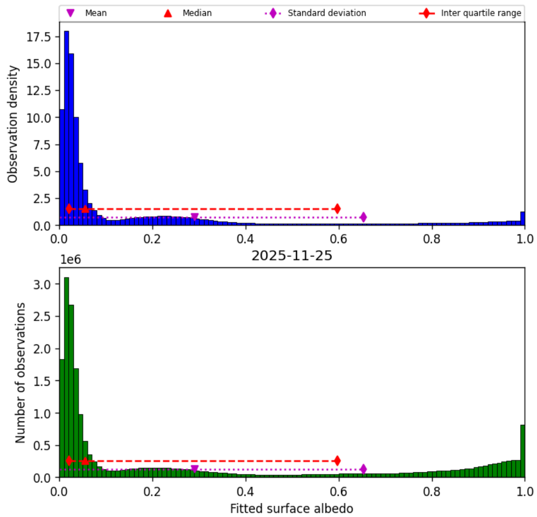
Figure 45: Histogram of “Fitted surface albedo” for 2025-11-24 to 2025-11-26
