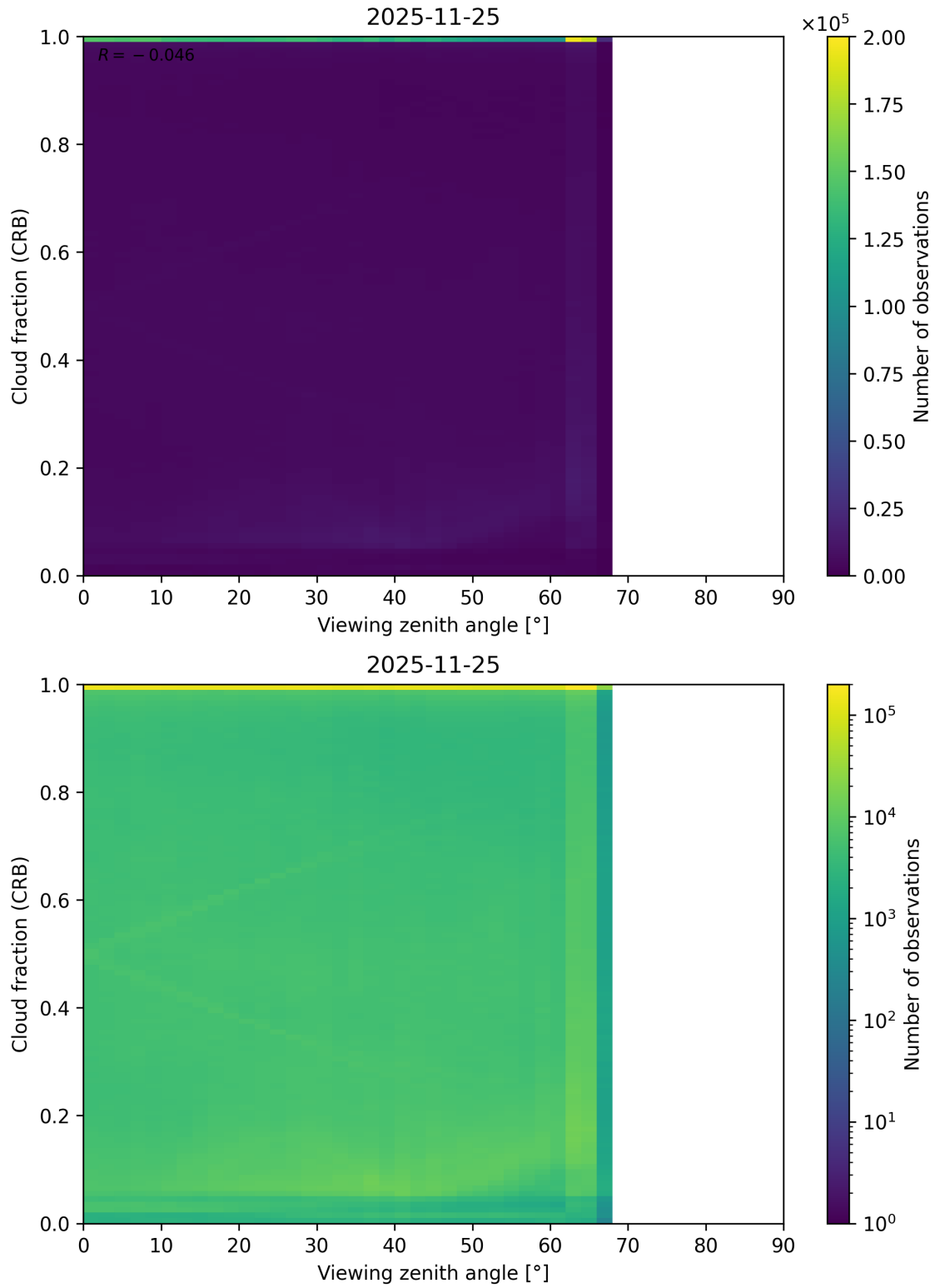
Figure 109: Scatter density plot of “Viewing zenith angle” against “Cloud fraction (CRB)” for 2025-11-24 to 2025-11-26.
