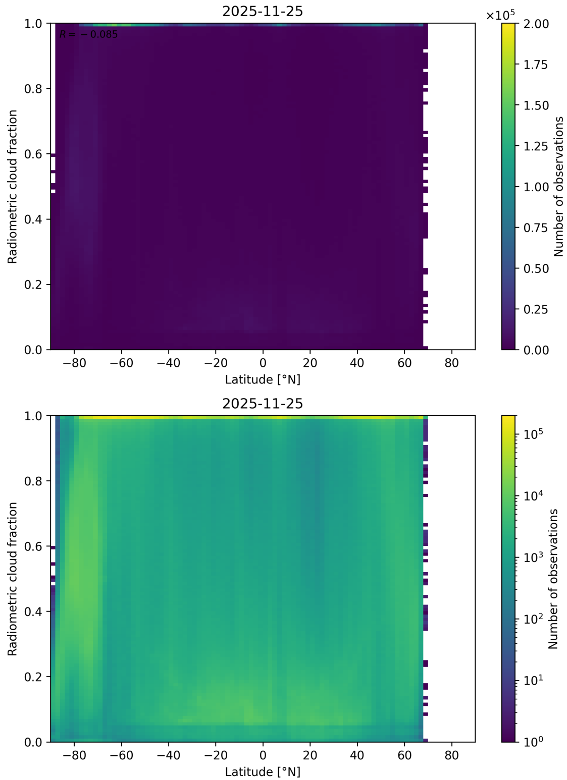
Figure 92: Scatter density plot of “Latitude” against “Radiometric cloud fraction” for 2025-11-24 to 2025-11-26.
