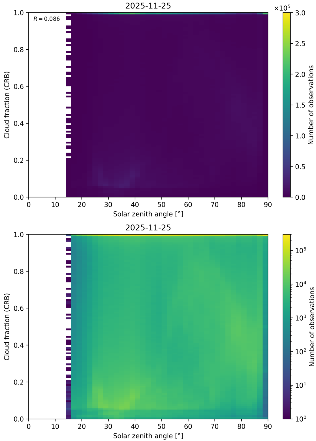
Figure 101: Scatter density plot of “Solar zenith angle” against “Cloud fraction (CRB)” for 2025-11-24 to 2025-11-26.
