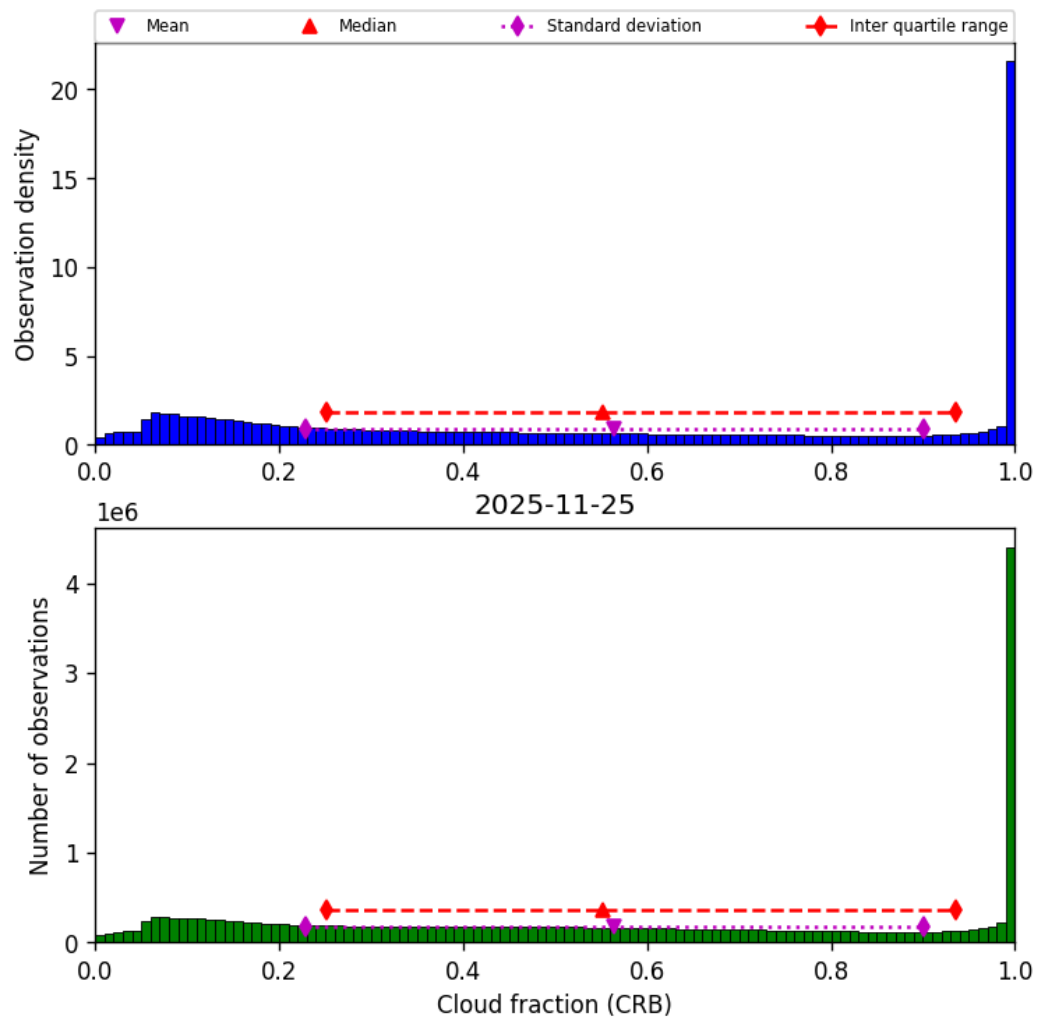
Figure 42: Histogram of “Cloud fraction (CRB)” for 2025-11-24 to 2025-11-26
