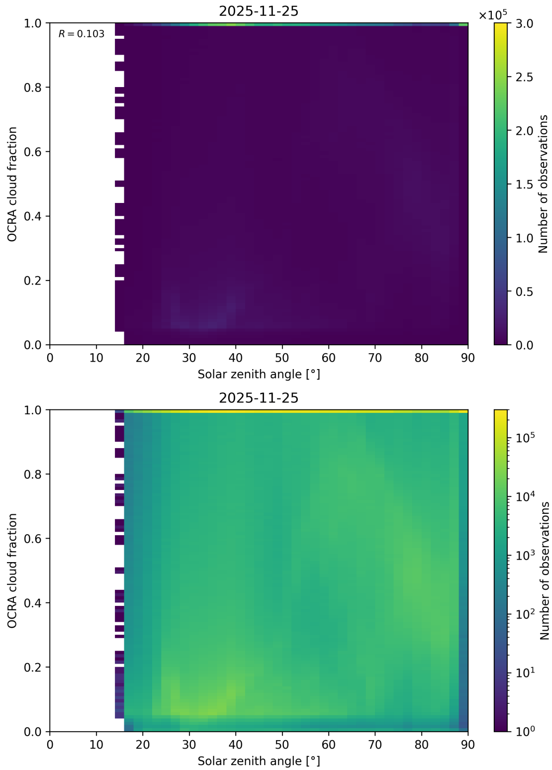
Figure 100: Scatter density plot of “Solar zenith angle” against “OCRA cloud fraction” for 2025-11-24 to 2025-11-26.
