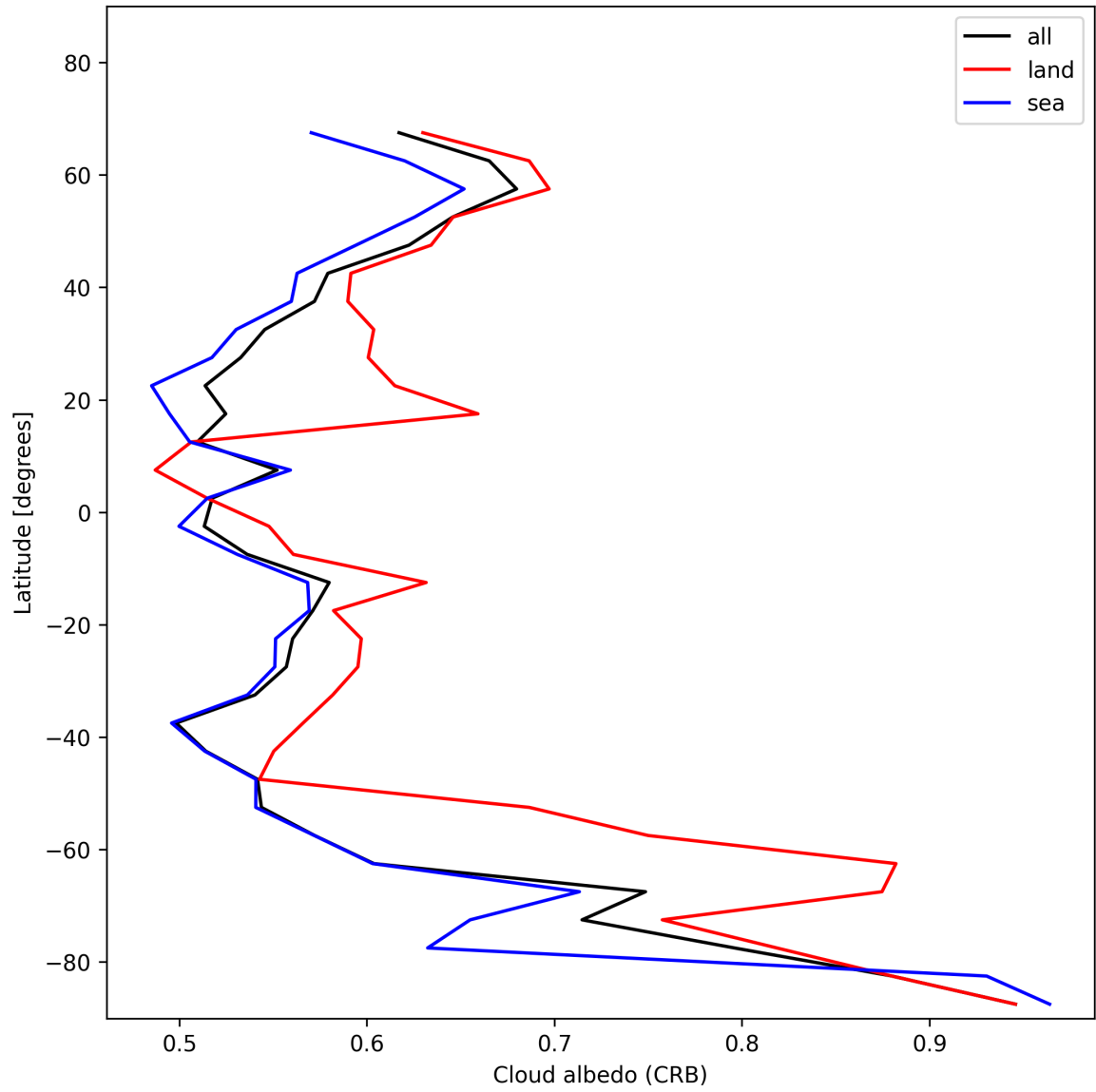
Figure 28: Zonal average of “Cloud albedo (CRB)” for 2025-11-24 to 2025-11-26.
