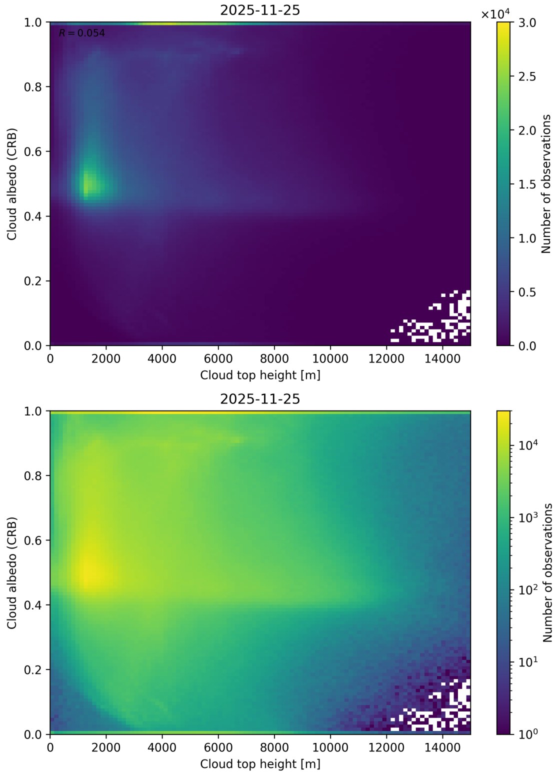
Figure 86: Scatter density plot of “Cloud top height” against “Cloud albedo (CRB)” for 2025-11-24 to 2025-11-26.
