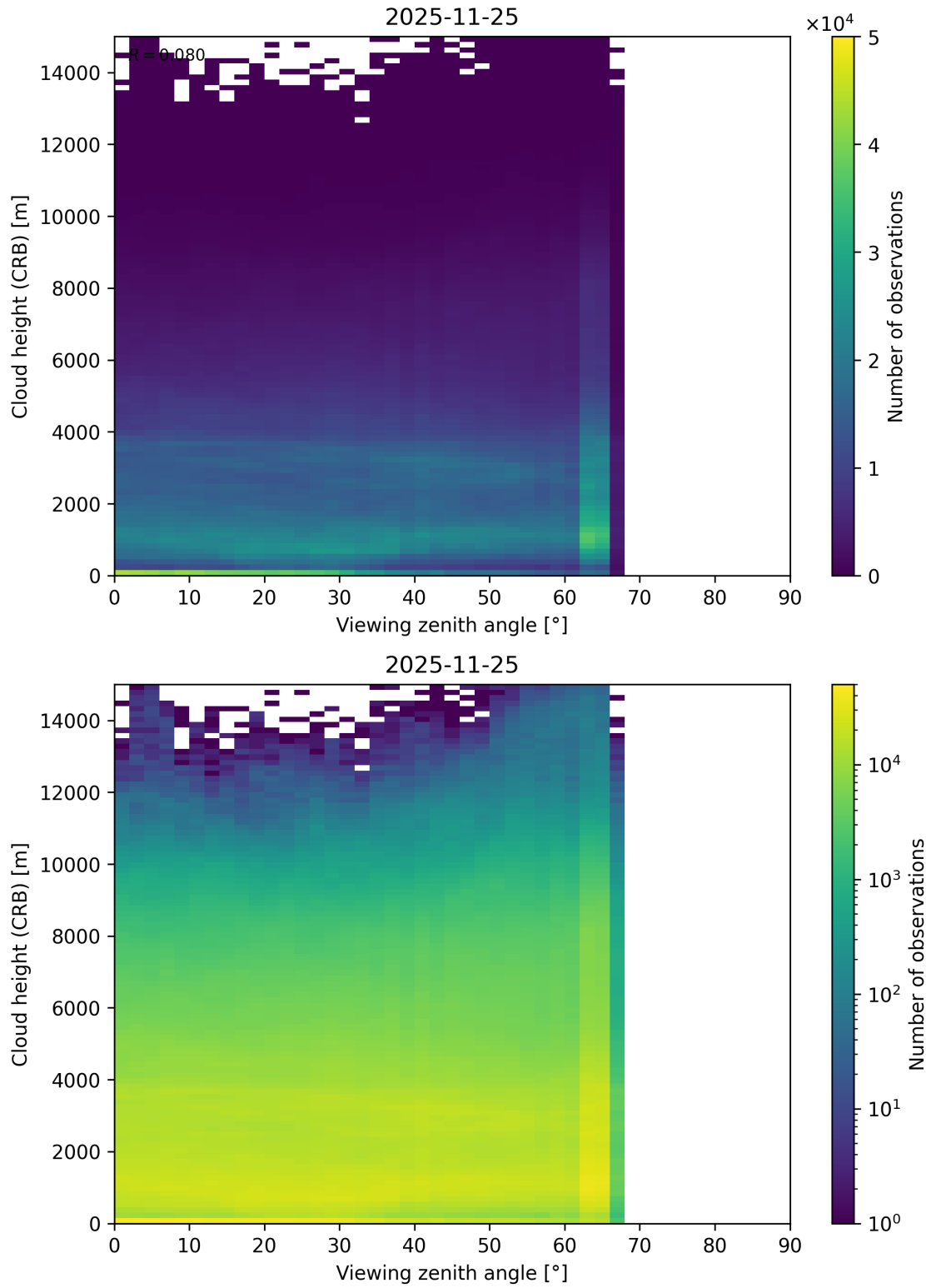
Figure 110: Scatter density plot of “Viewing zenith angle” against “Cloud height (CRB)” for 2025-11-24 to 2025-11-26.
