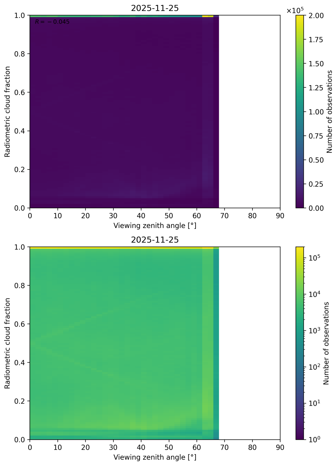
Figure 107: Scatter density plot of “Viewing zenith angle” against “Radiometric cloud fraction” for 2025-11-24 to 2025-11-26.
