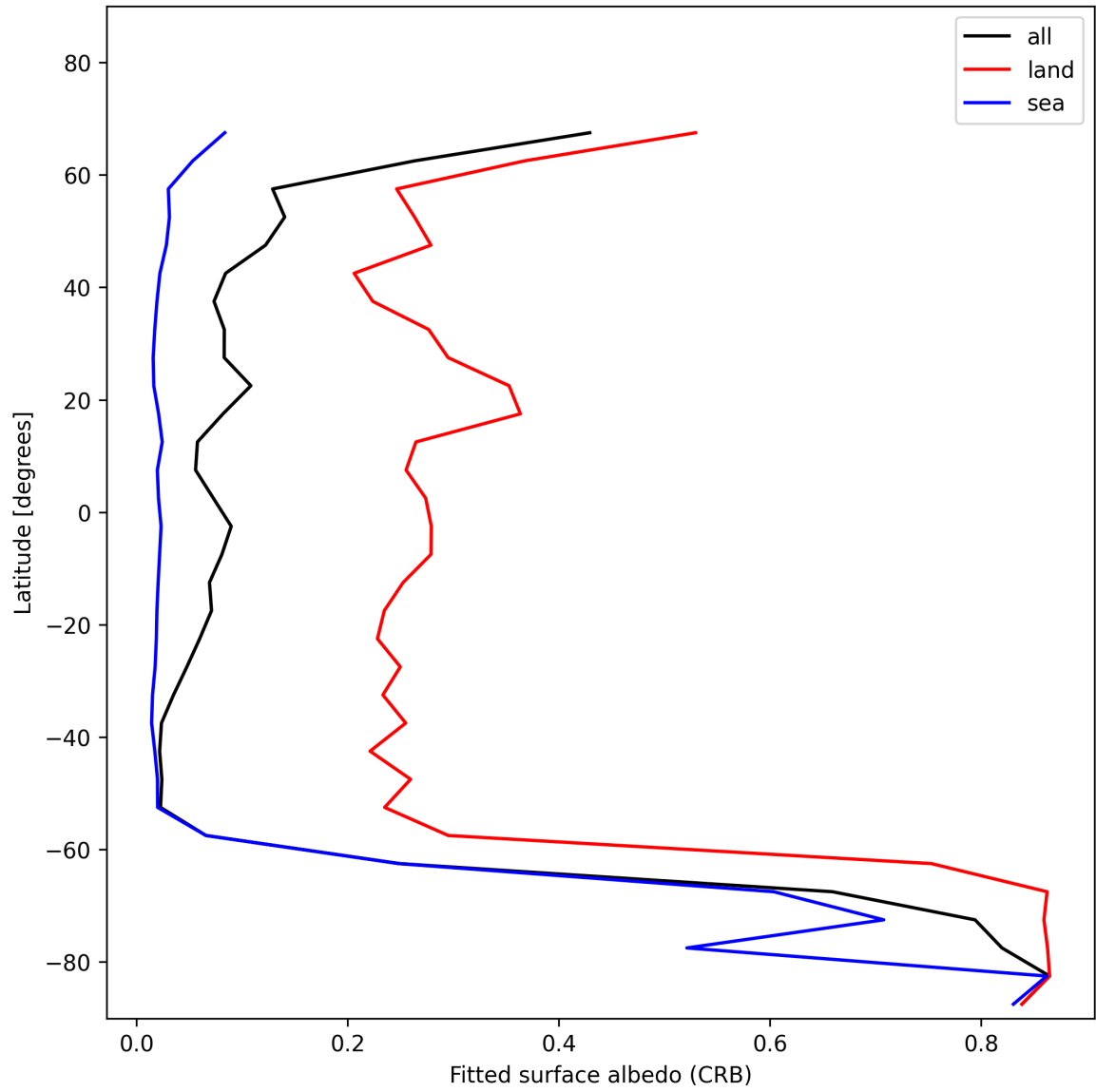
Figure 30: Zonal average of “Fitted surface albedo (CRB)” for 2025-11-24 to 2025-11-26.
