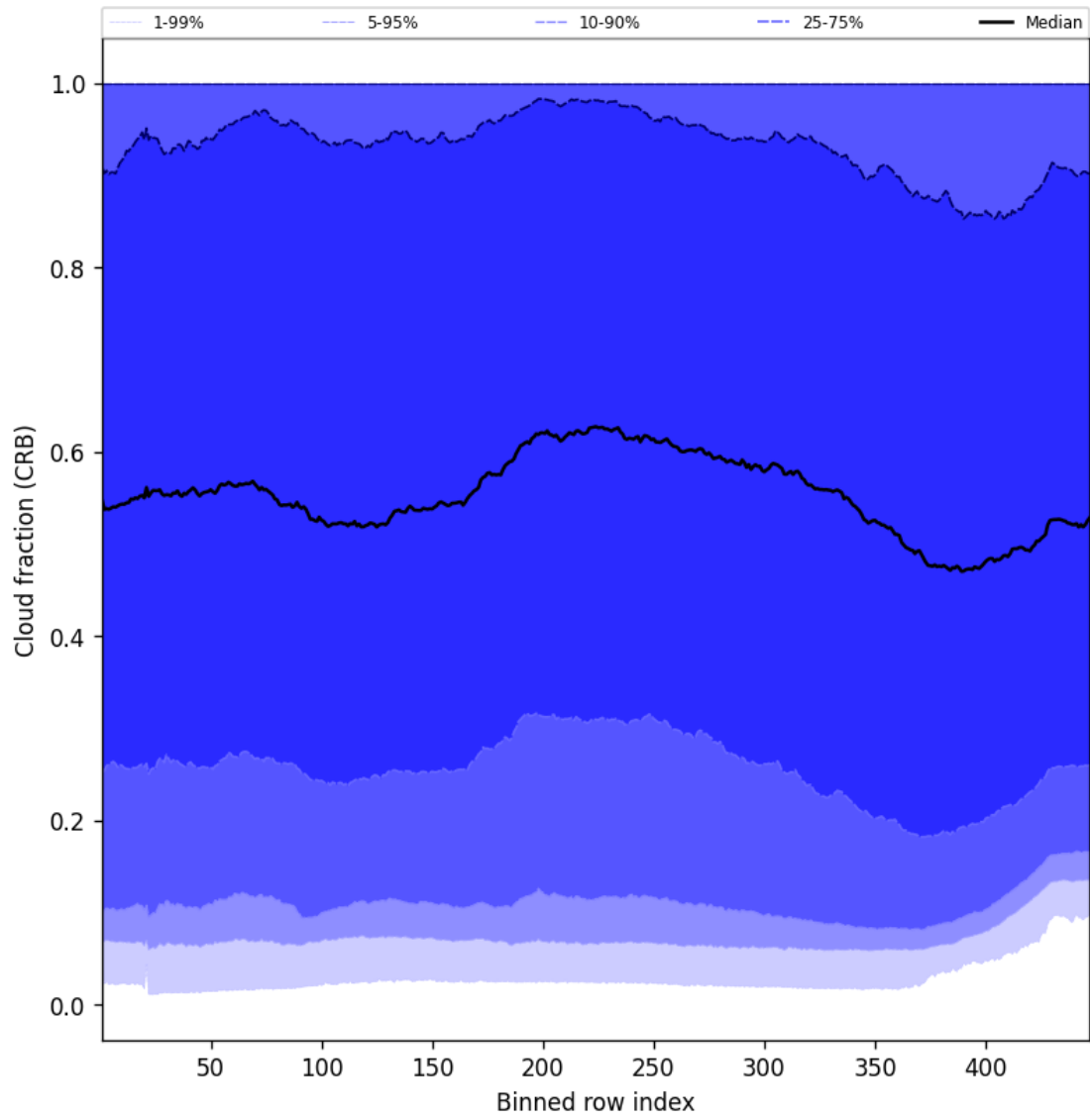
Figure 58: Along track statistics of “Cloud fraction (CRB)” for 2025-11-24 to 2025-11-26
