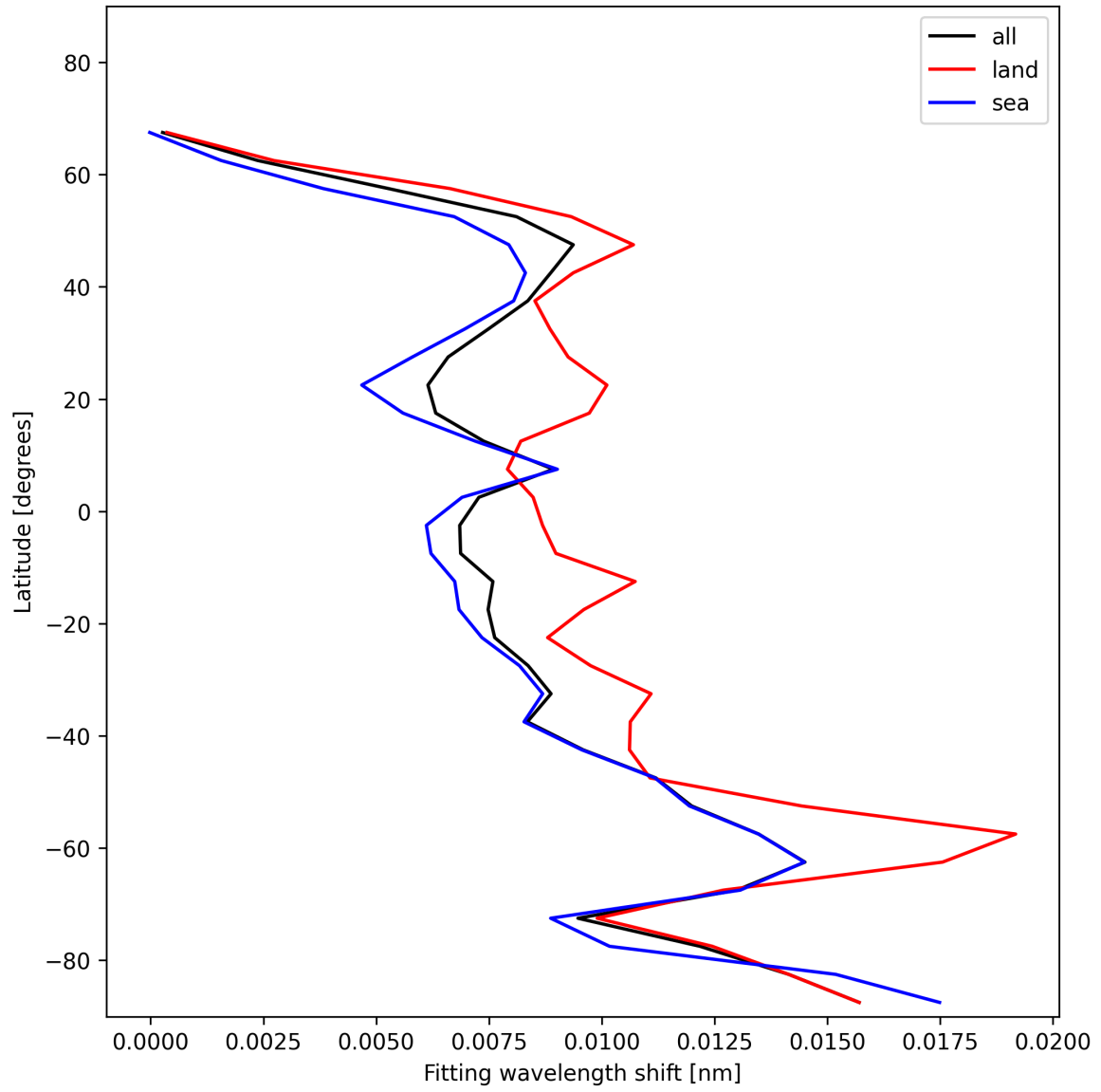
Figure 33: Zonal average of “Fitting wavelength shift” for 2025-11-24 to 2025-11-26.
