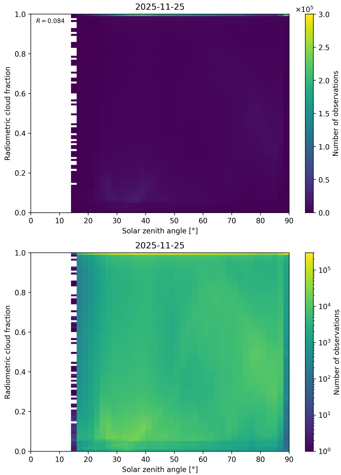
Figure 99: Scatter density plot of “Solar zenith angle” against “Radiometric cloud fraction” for 2025-11-24 to 2025-11-26.
