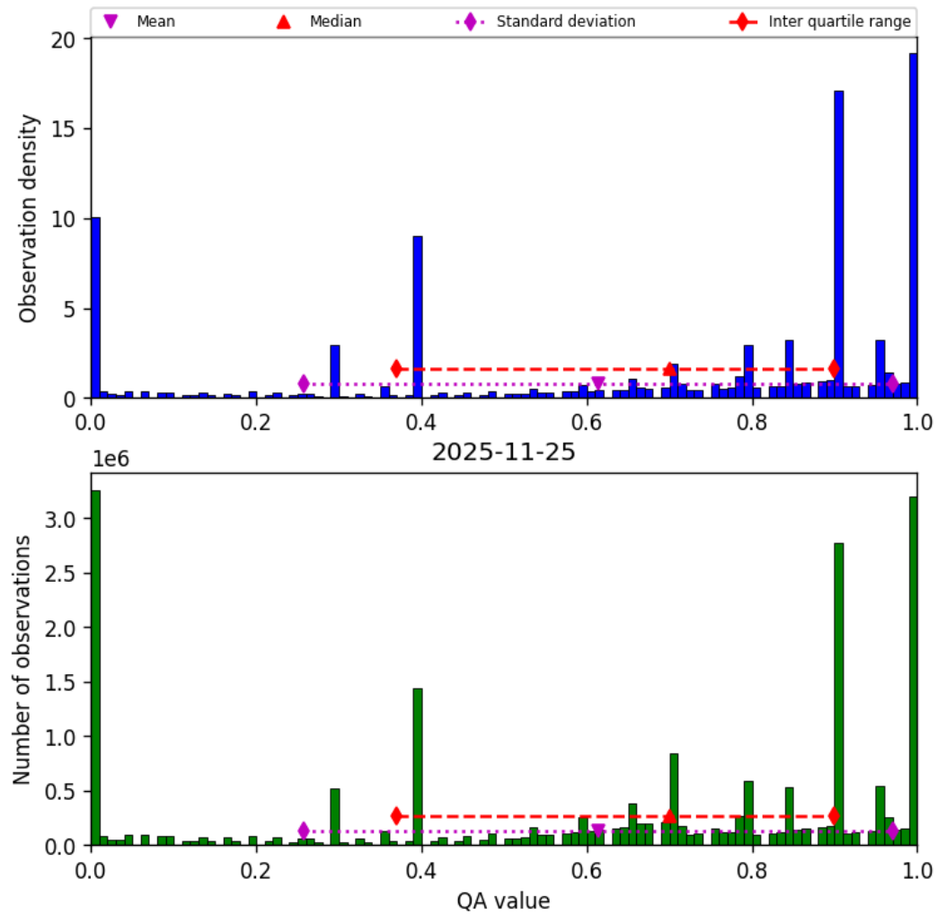
Figure 38: Histogram of “QA value” for 2025-11-24 to 2025-11-26
