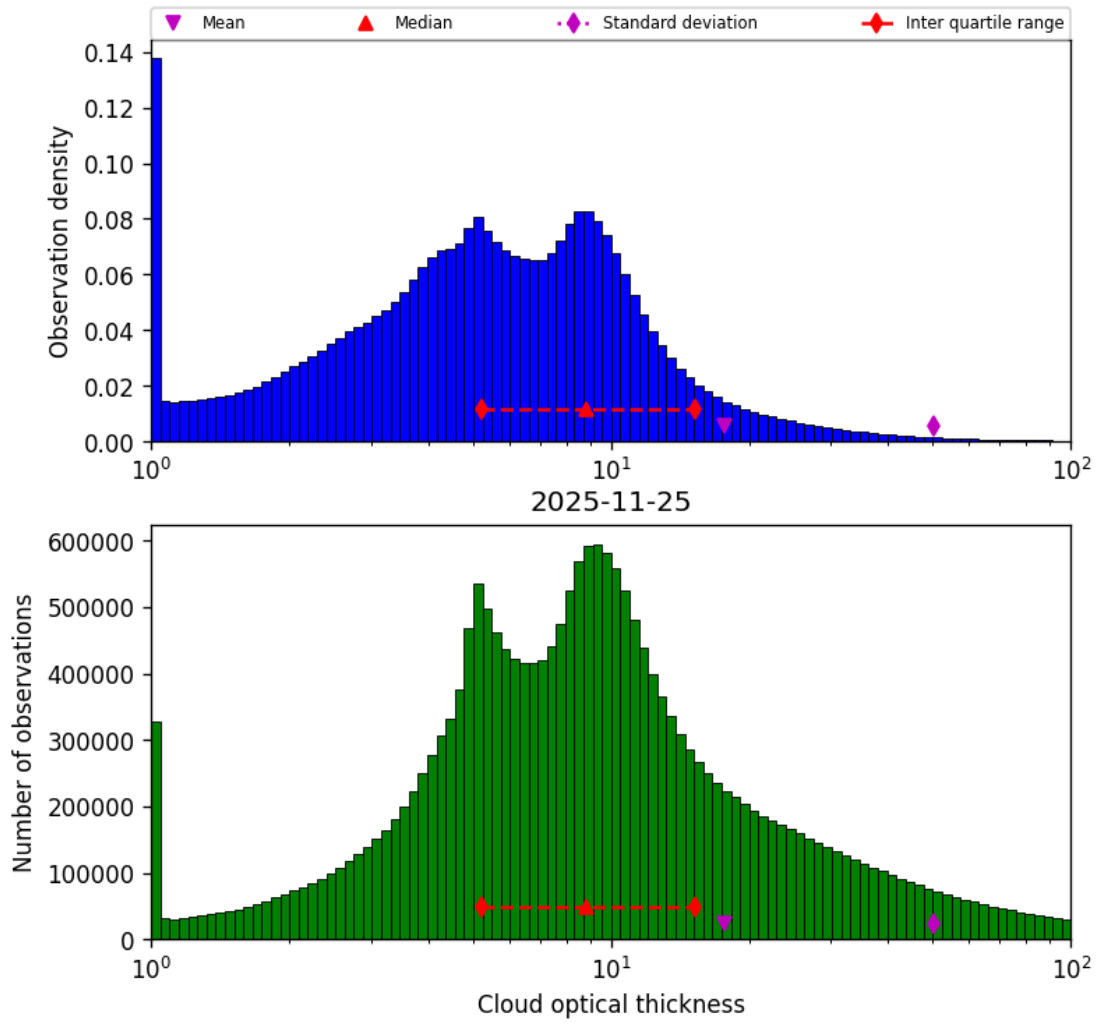
Figure 41: Histogram of “Cloud optical thickness” for 2025-11-24 to 2025-11-26
