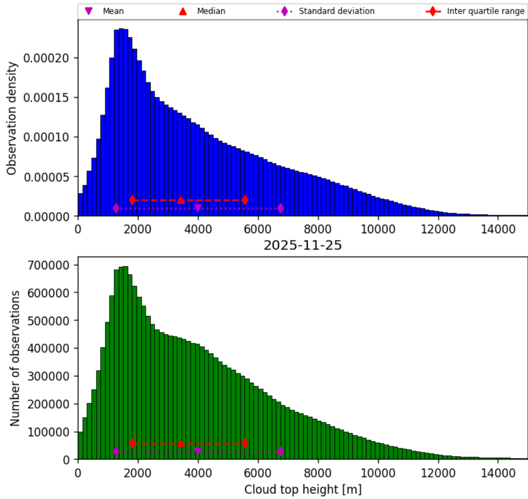
Figure 40: Histogram of “Cloud top height” for 2025-11-24 to 2025-11-26
