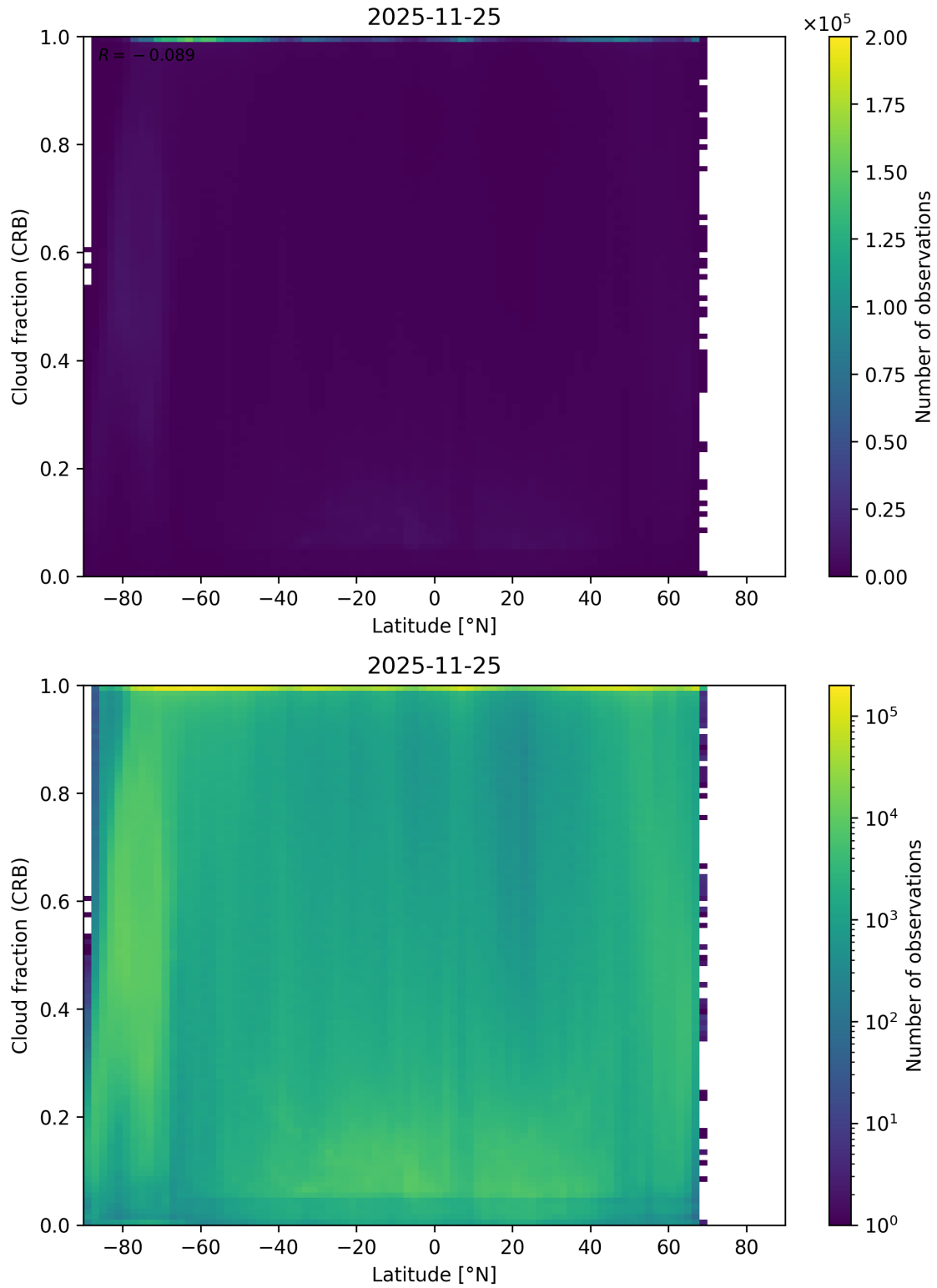
Figure 94: Scatter density plot of “Latitude” against “Cloud fraction (CRB)” for 2025-11-24 to 2025-11-26.
