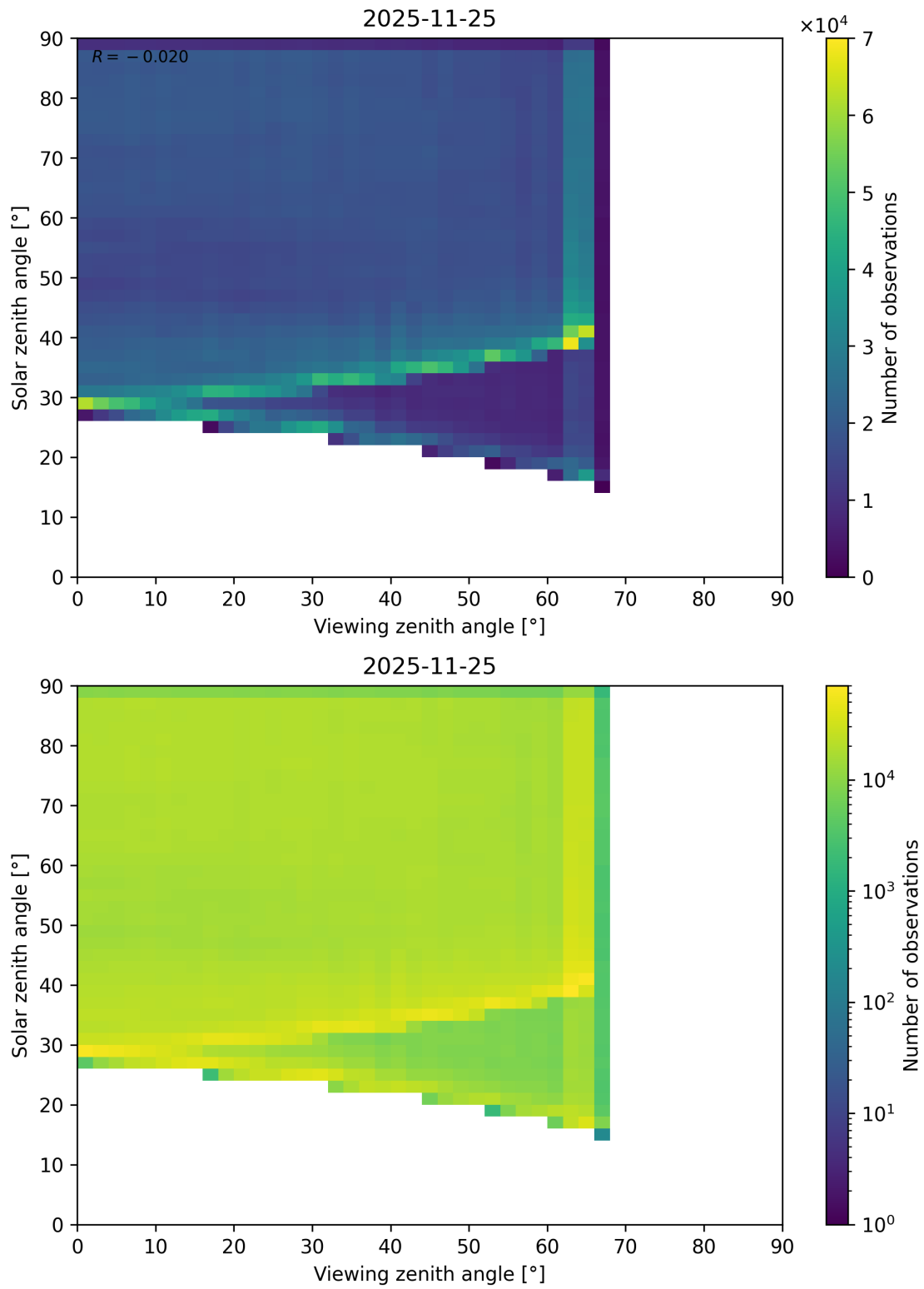
Figure 114: Scatter density plot of “Viewing zenith angle” against “Solar zenith angle” for 2025-11-24 to 2025-11-26.
