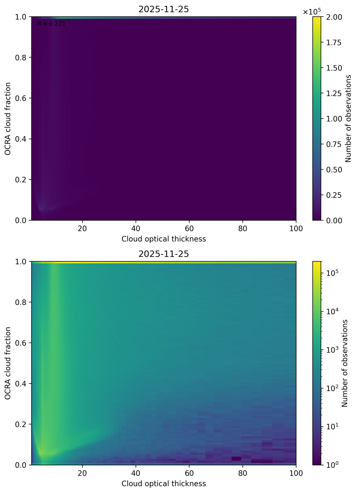
Figure 83: Scatter density plot of “Cloud optical thickness” against “OCRA cloud fraction” for 2025-11-24 to 2025-11-26.
