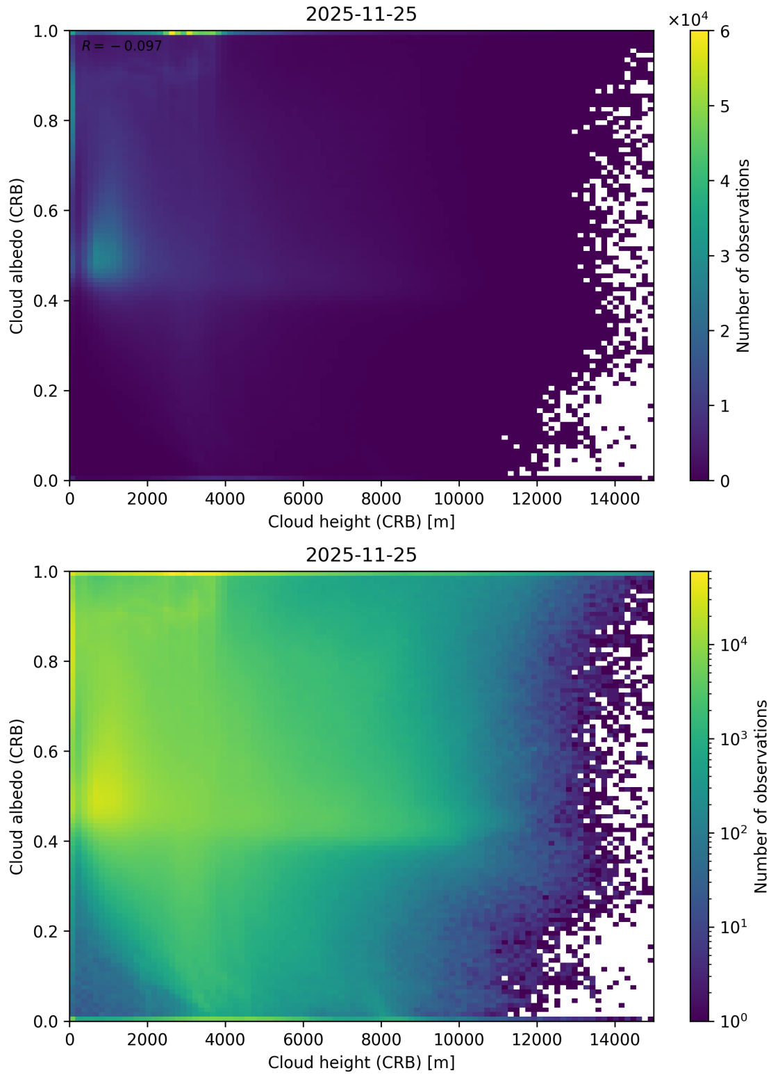
Figure 80: Scatter density plot of “Cloud height (CRB)” against “Cloud albedo (CRB)” for 2025-11-24 to 2025-11-26.
