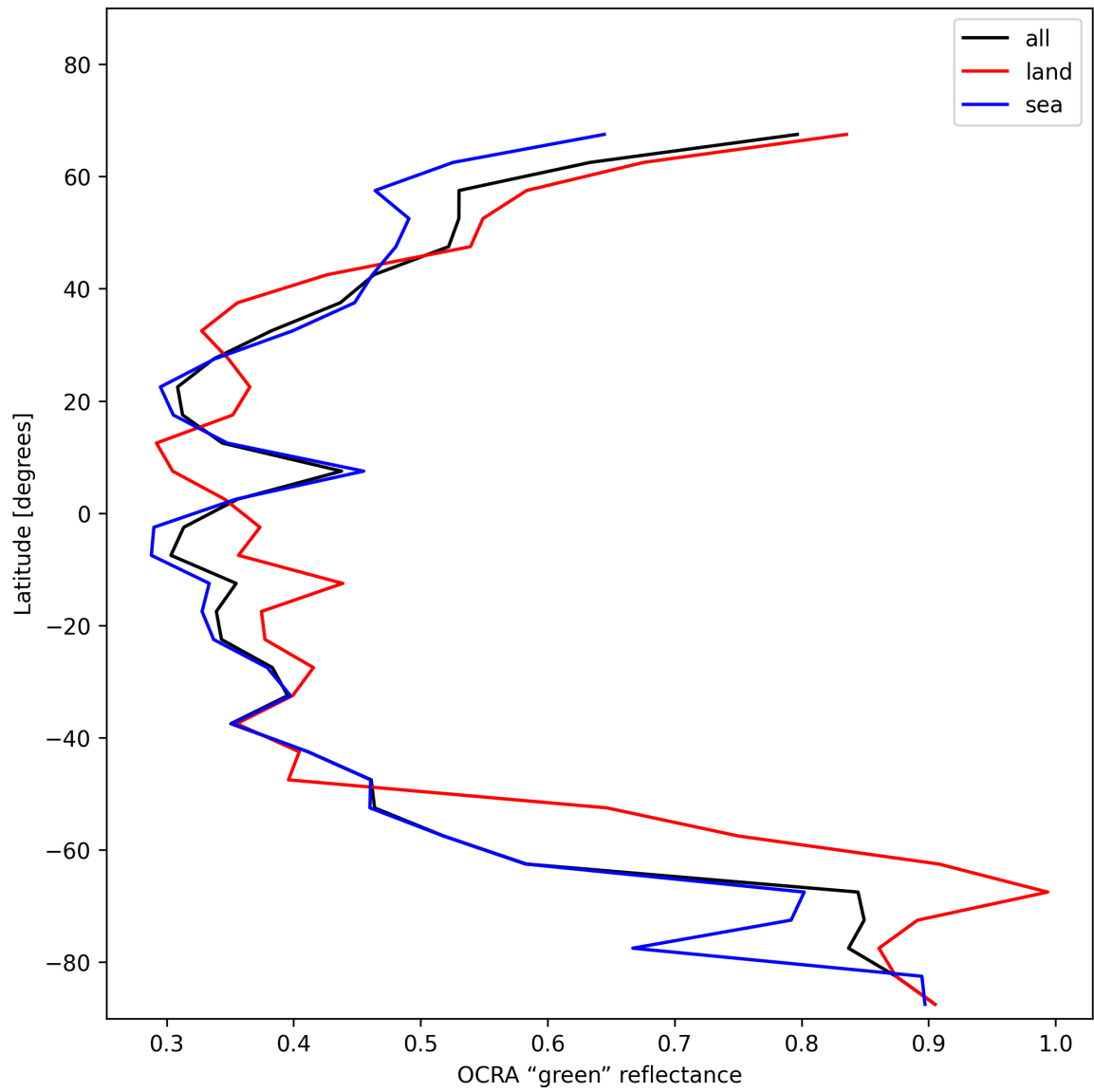
Figure 36: Zonal average of “OCRA “green” reflectance” for 2025-11-24 to 2025-11-26.
