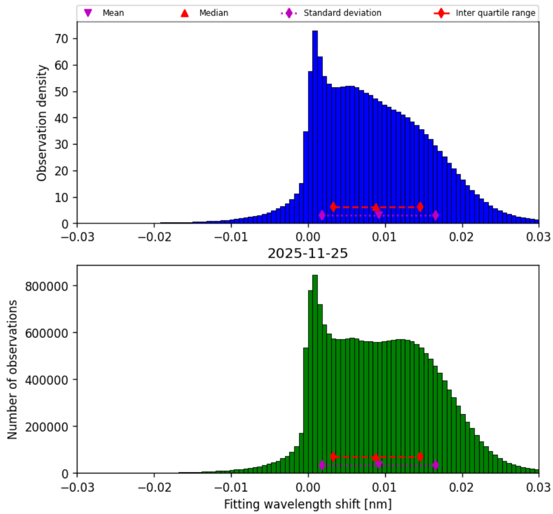
Figure 49: Histogram of “Fitting wavelength shift” for 2025-11-24 to 2025-11-26
