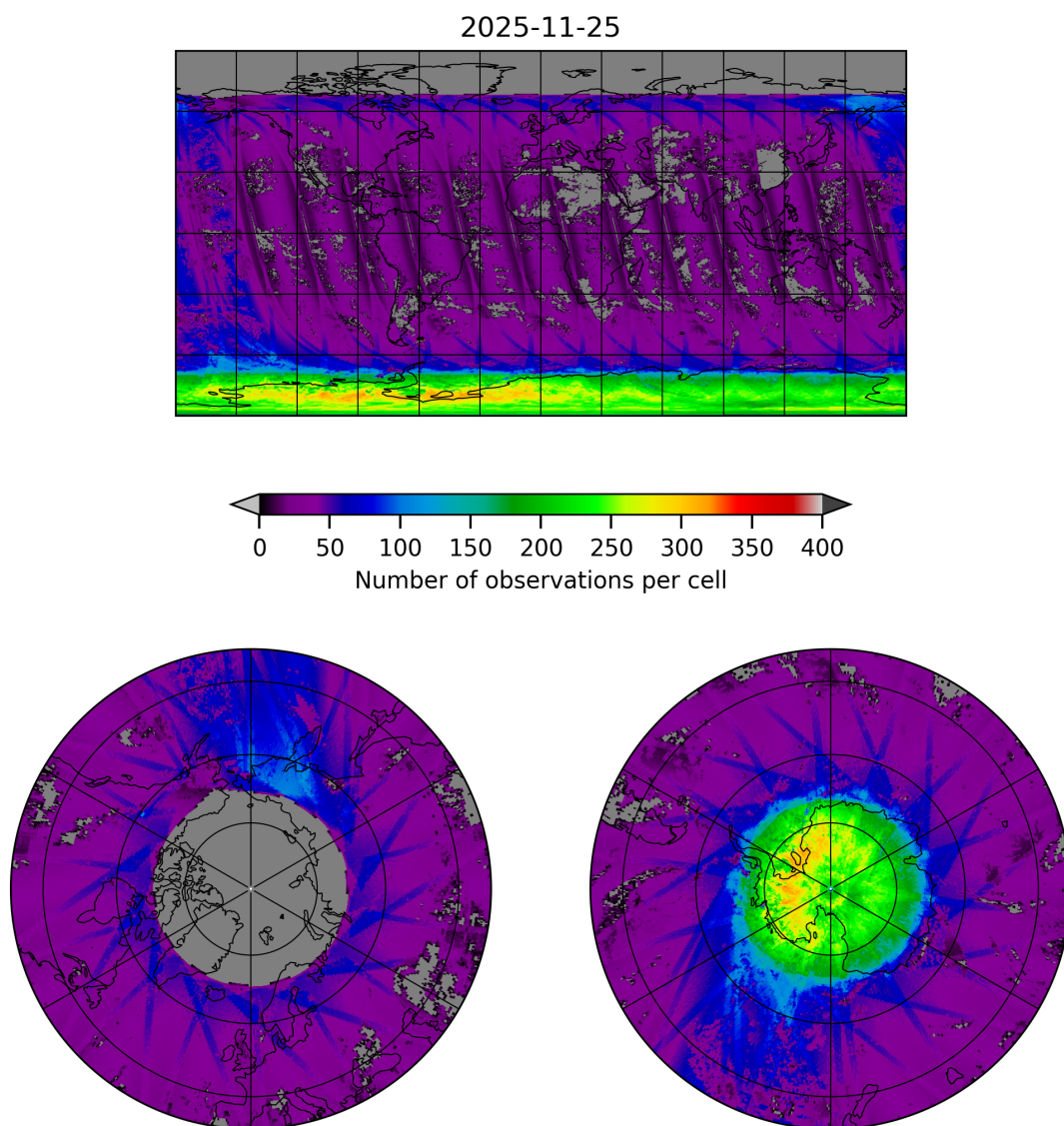
Figure 21: Map of the number of observations for 2025-11-24 to 2025-11-26
