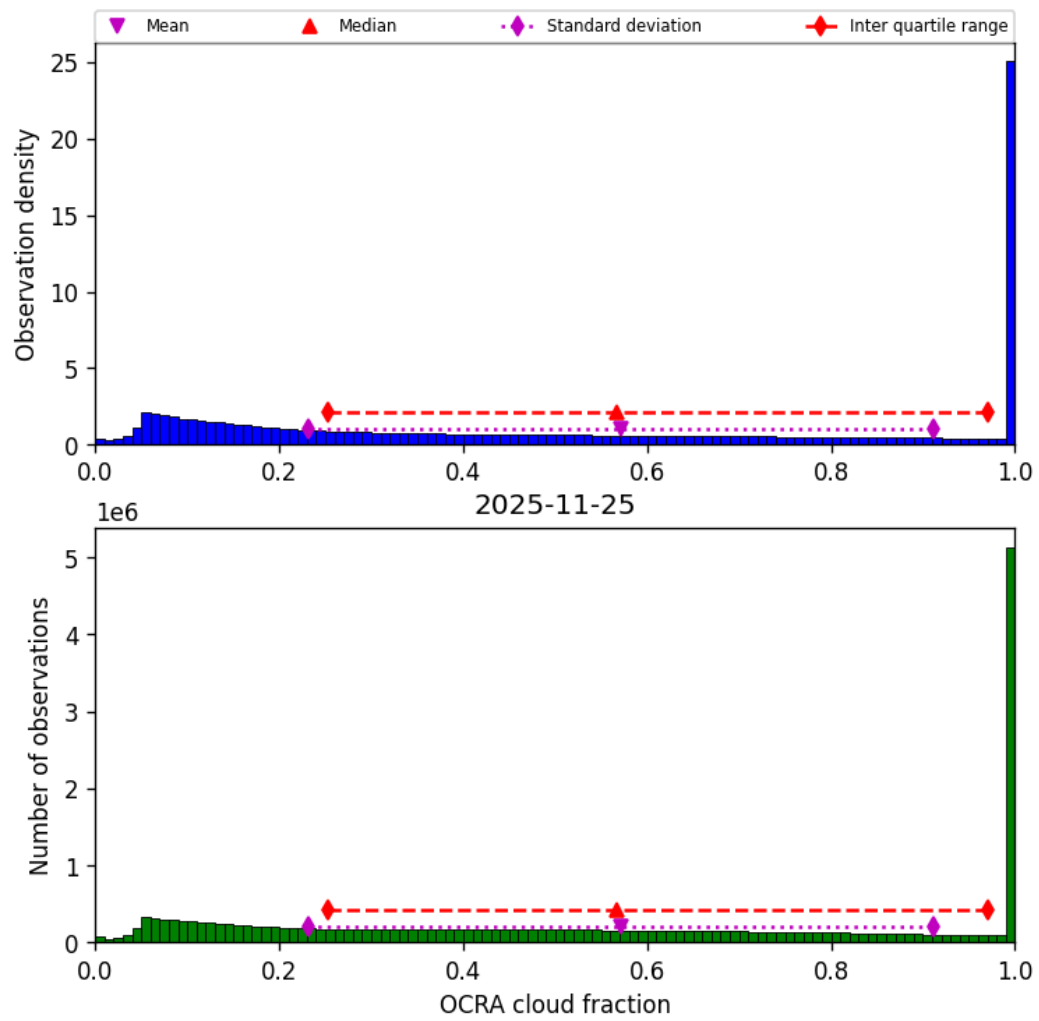
Figure 50: Histogram of “OCRA cloud fraction” for 2025-11-24 to 2025-11-26
