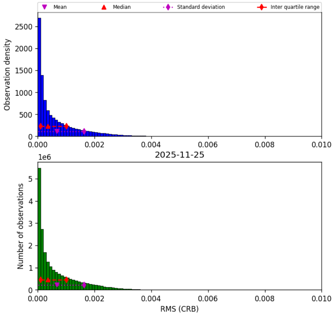
Figure 48: Histogram of “RMS (CRB)” for 2025-11-24 to 2025-11-26
