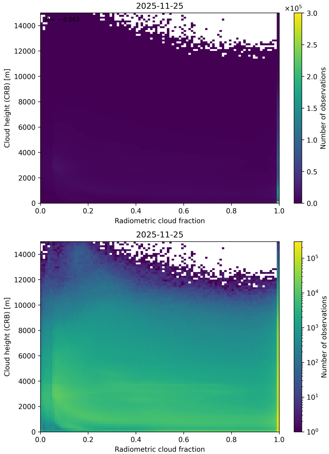
Figure 74: Scatter density plot of “Radiometric cloud fraction” against “Cloud height (CRB)” for 2025-11-24 to 2025-11-26.
