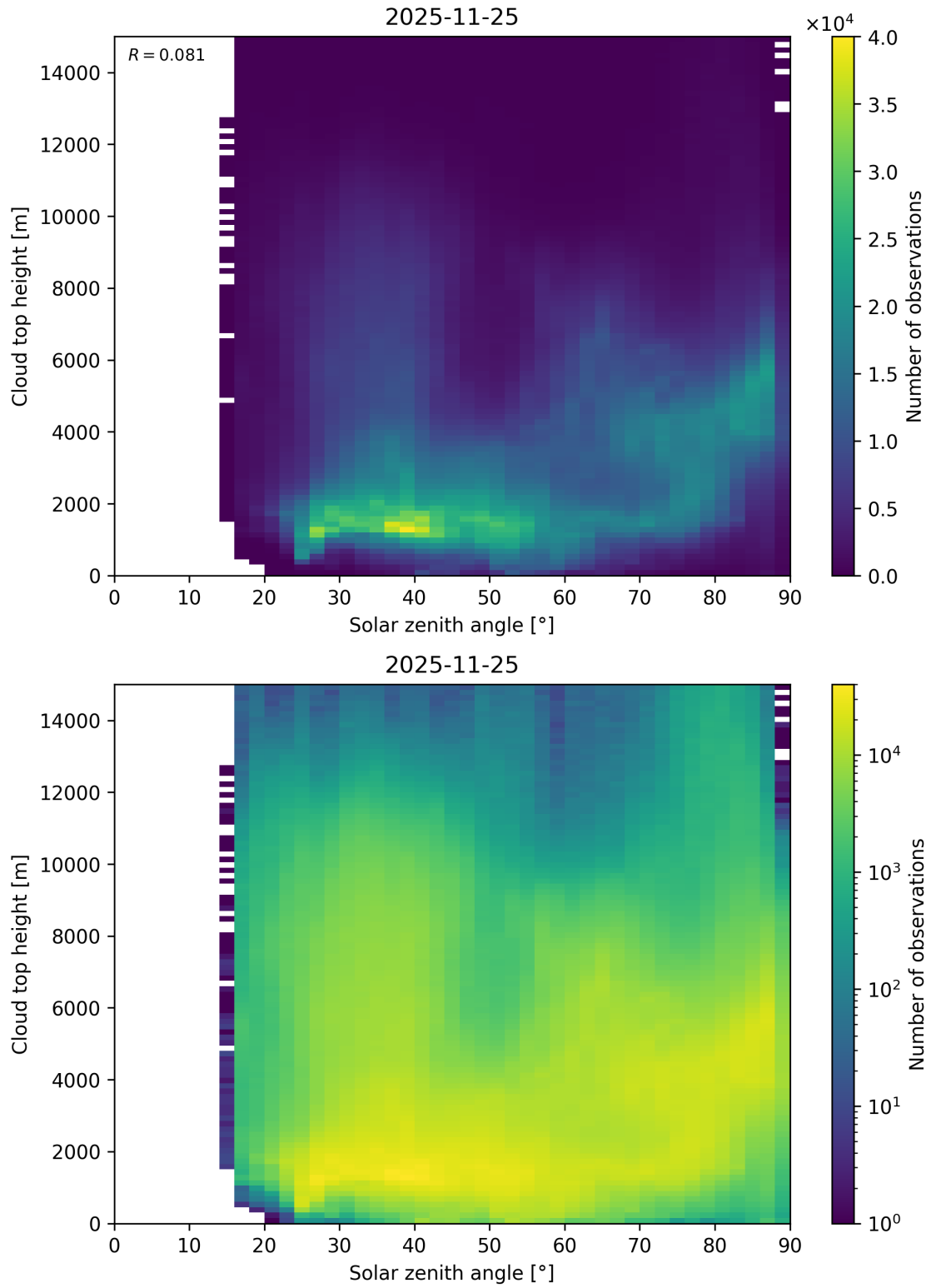
Figure 104: Scatter density plot of “Solar zenith angle” against “Cloud top height” for 2025-11-24 to 2025-11-26.
