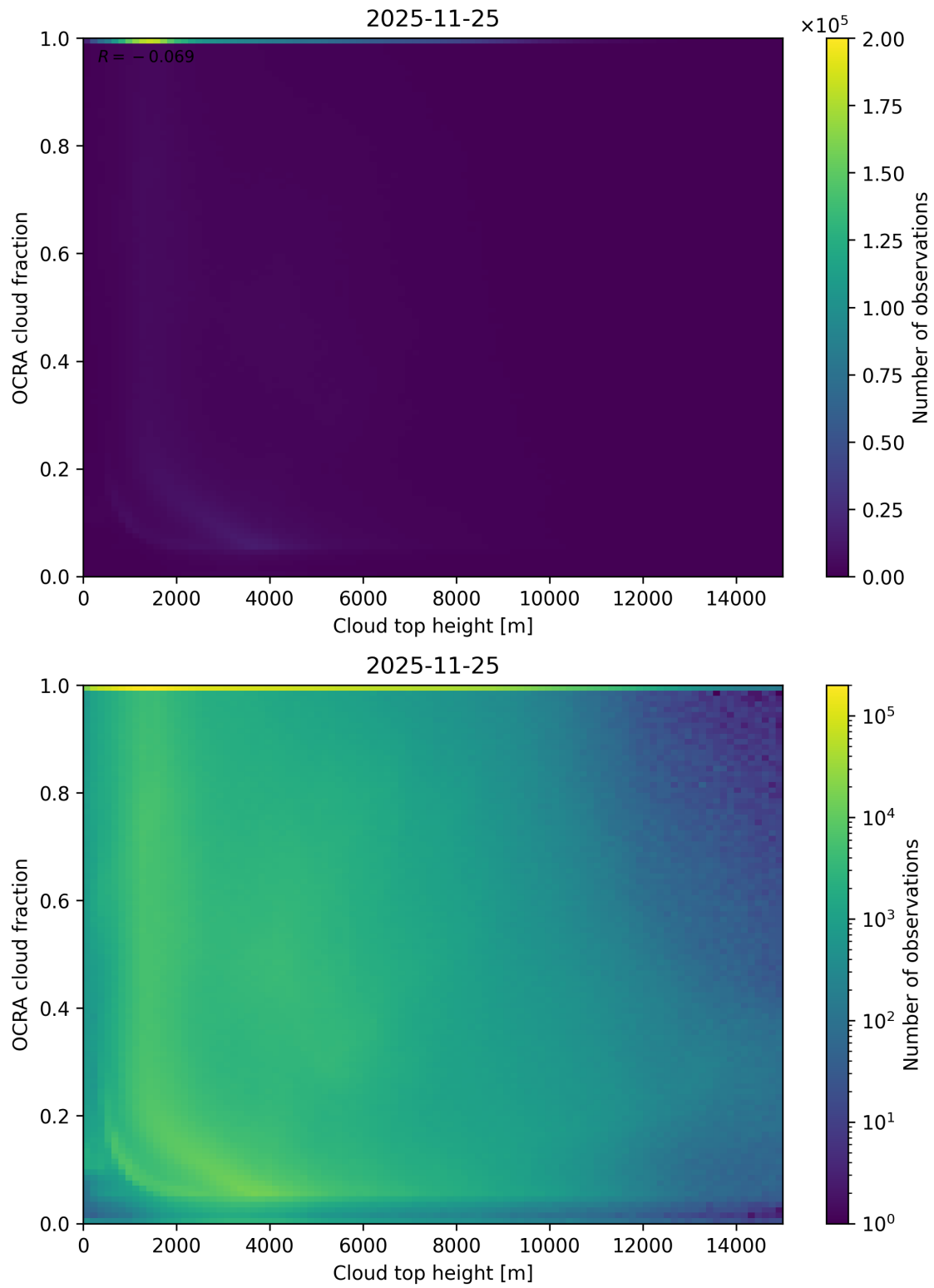
Figure 87: Scatter density plot of “Cloud top height” against “OCRA cloud fraction” for 2025-11-24 to 2025-11-26.
