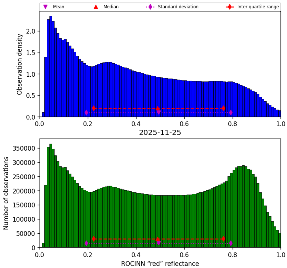
Figure 53: Histogram of “ROCINN “red” reflectance” for 2025-11-24 to 2025-11-26
