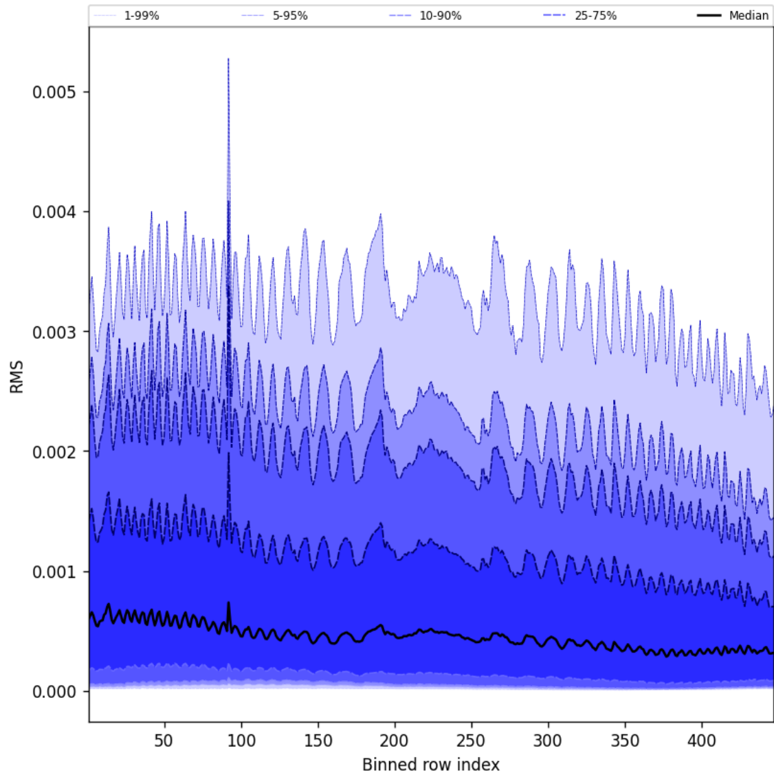
Figure 63: Along track statistics of “RMS” for 2025-11-24 to 2025-11-26
