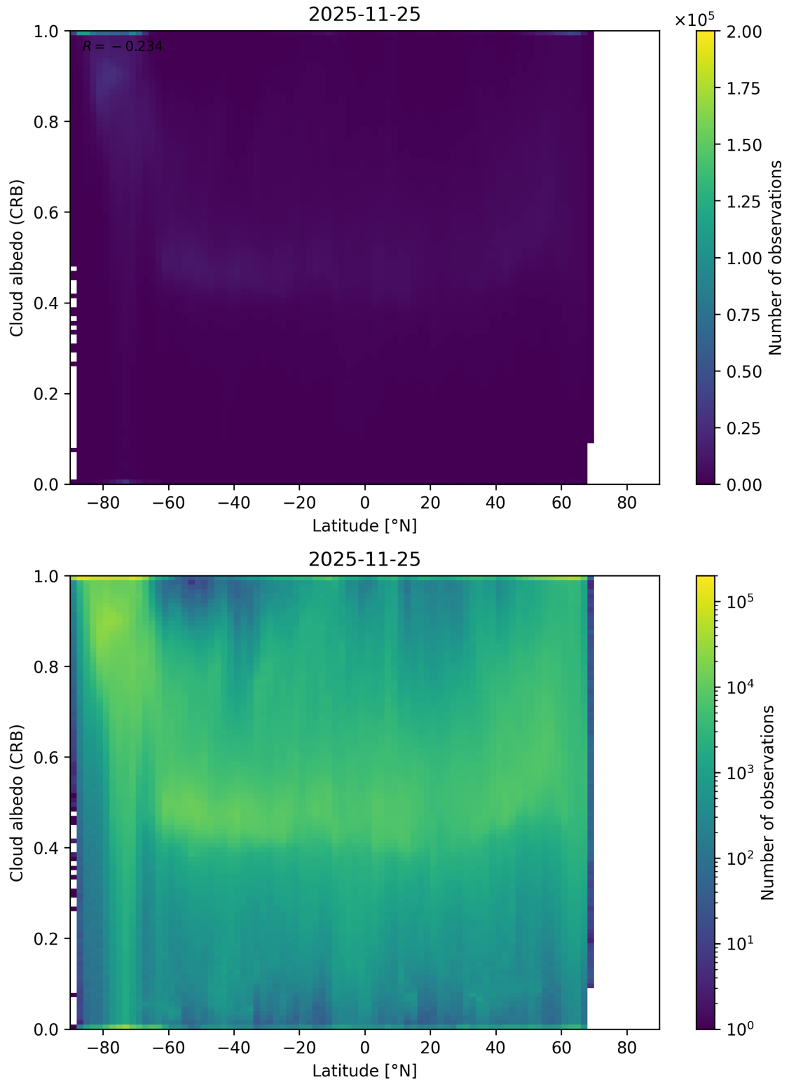
Figure 91: Scatter density plot of “Latitude” against “Cloud albedo (CRB)” for 2025-11-24 to 2025-11-26.
