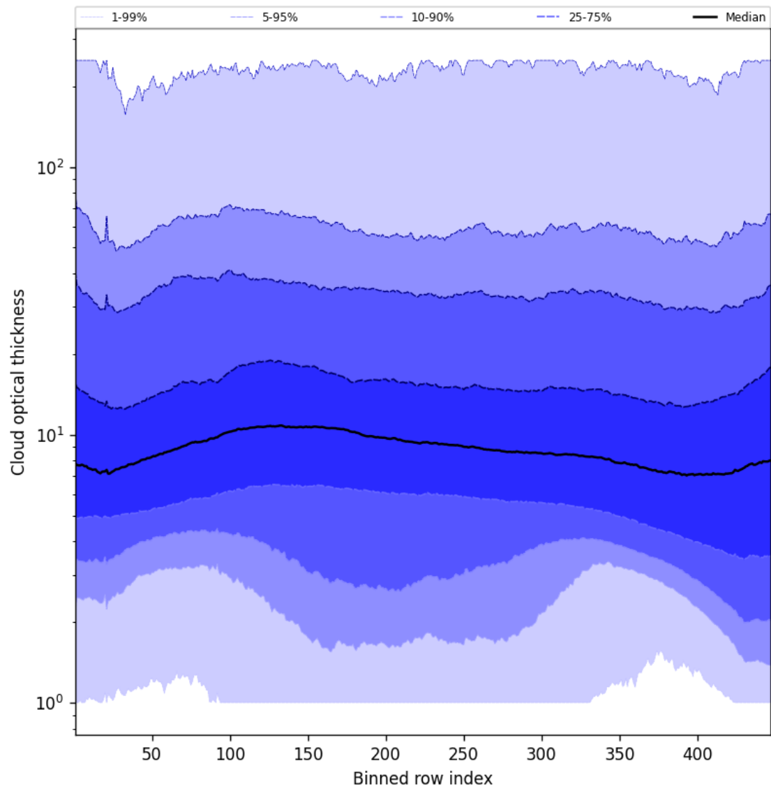
Figure 57: Along track statistics of “Cloud optical thickness” for 2025-11-24 to 2025-11-26
