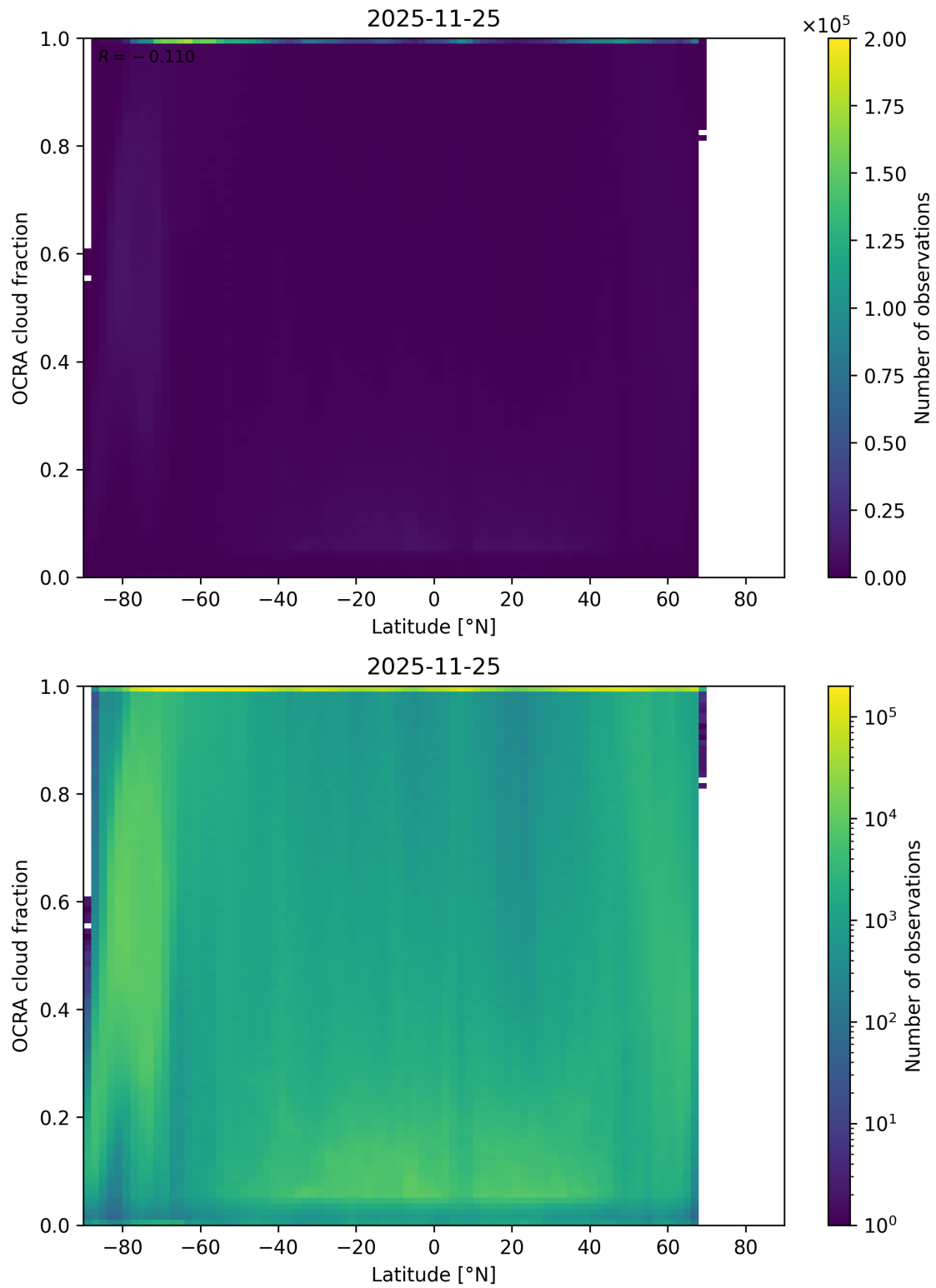
Figure 93: Scatter density plot of “Latitude” against “OCRA cloud fraction” for 2025-11-24 to 2025-11-26.
