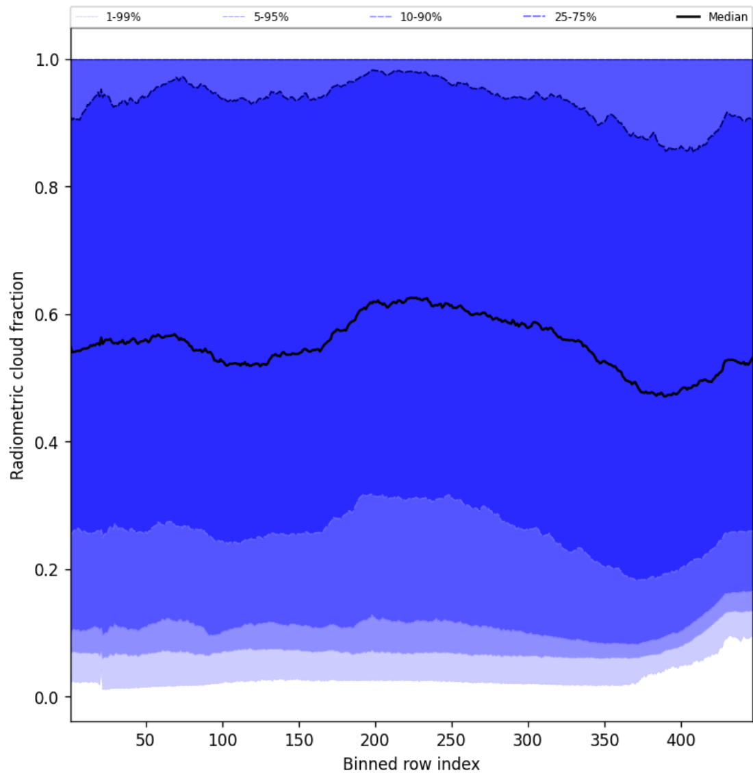
Figure 55: Along track statistics of “Radiometric cloud fraction” for 2025-11-24 to 2025-11-26
