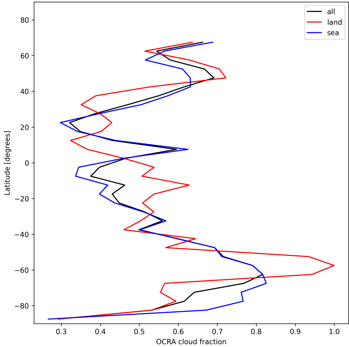
Figure 34: Zonal average of “OCRA cloud fraction” for 2025-11-24 to 2025-11-26.
