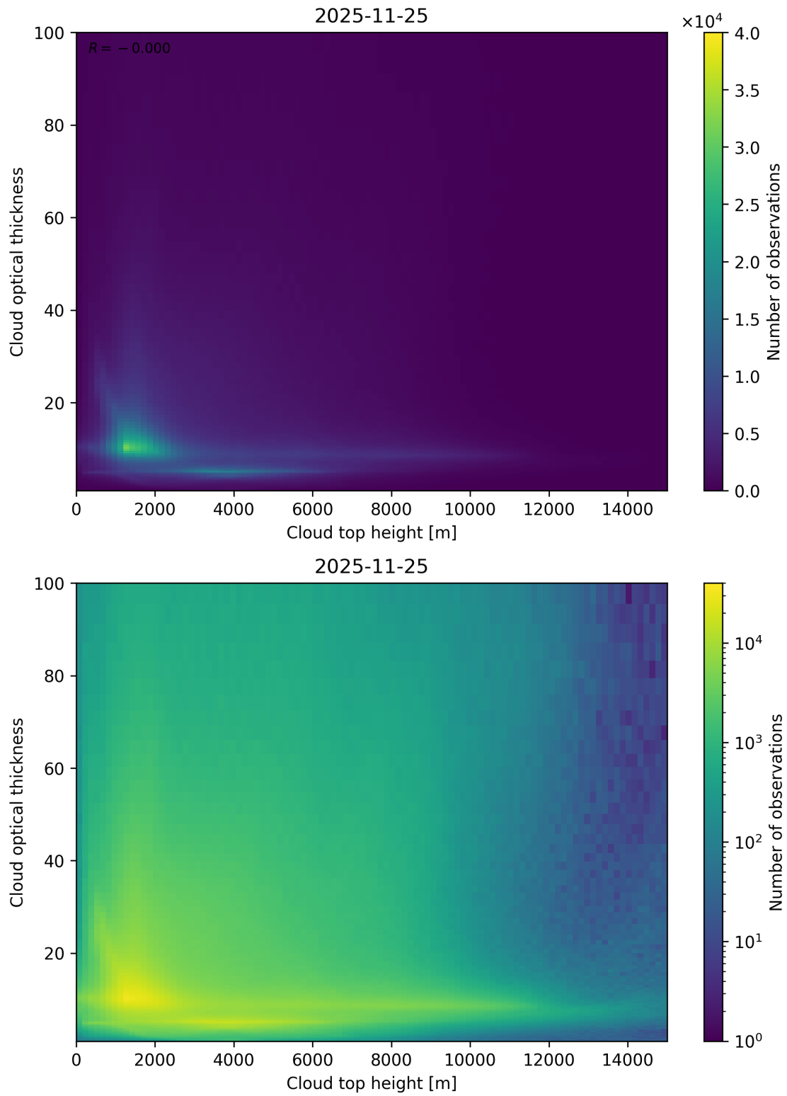
Figure 90: Scatter density plot of “Cloud top height” against “Cloud optical thickness” for 2025-11-24 to 2025-11-26.
