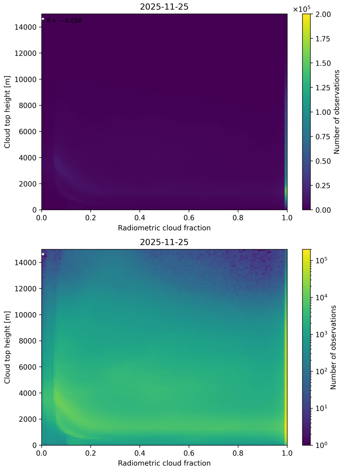
Figure 76: Scatter density plot of “Radiometric cloud fraction” against “Cloud top height” for 2025-11-24 to 2025-11-26.
