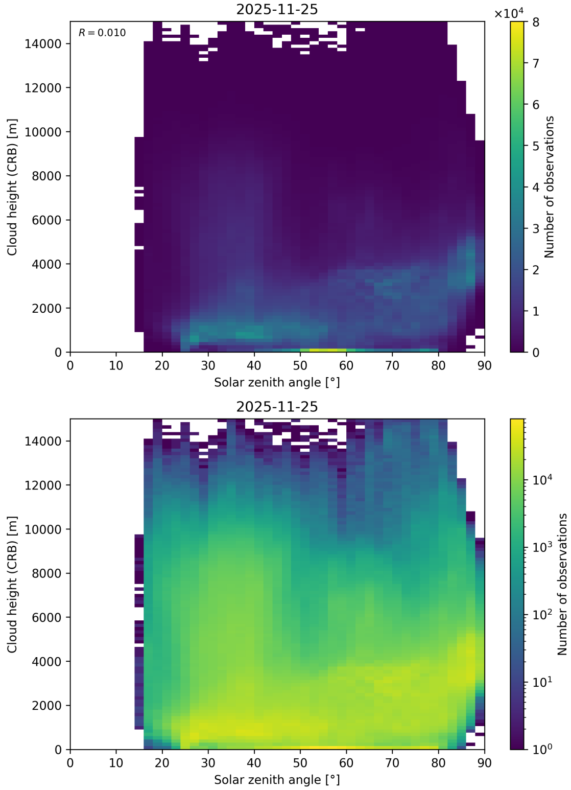
Figure 102: Scatter density plot of “Solar zenith angle” against “Cloud height (CRB)” for 2025-11-24 to 2025-11-26.
