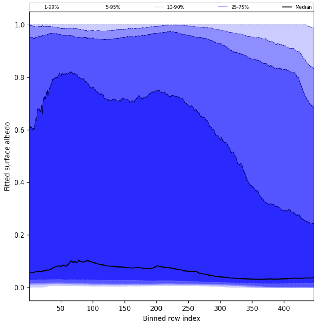
Figure 61: Along track statistics of “Fitted surface albedo” for 2025-11-24 to 2025-11-26
