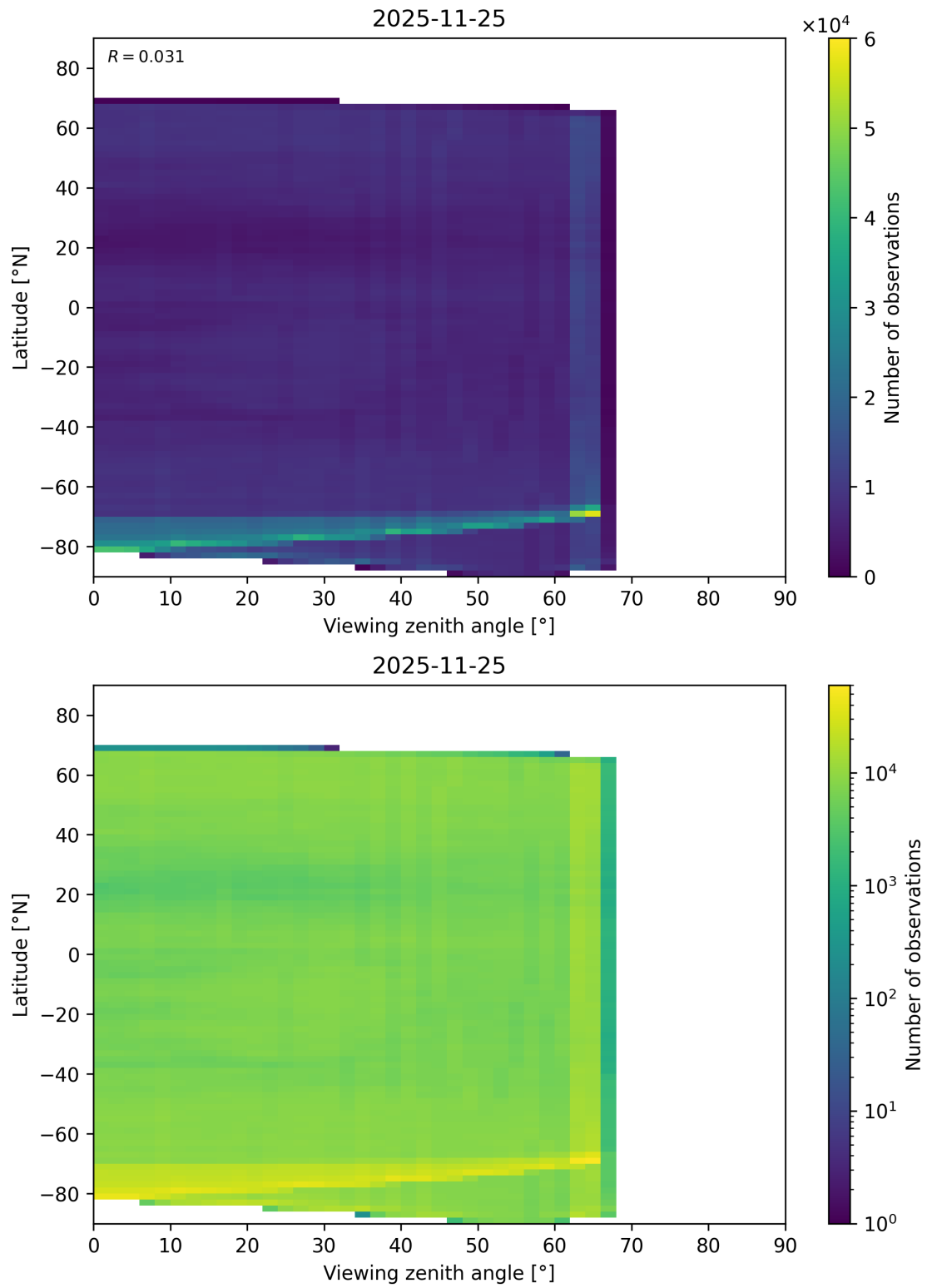
Figure 113: Scatter density plot of “Viewing zenith angle” against “Latitude” for 2025-11-24 to 2025-11-26.
