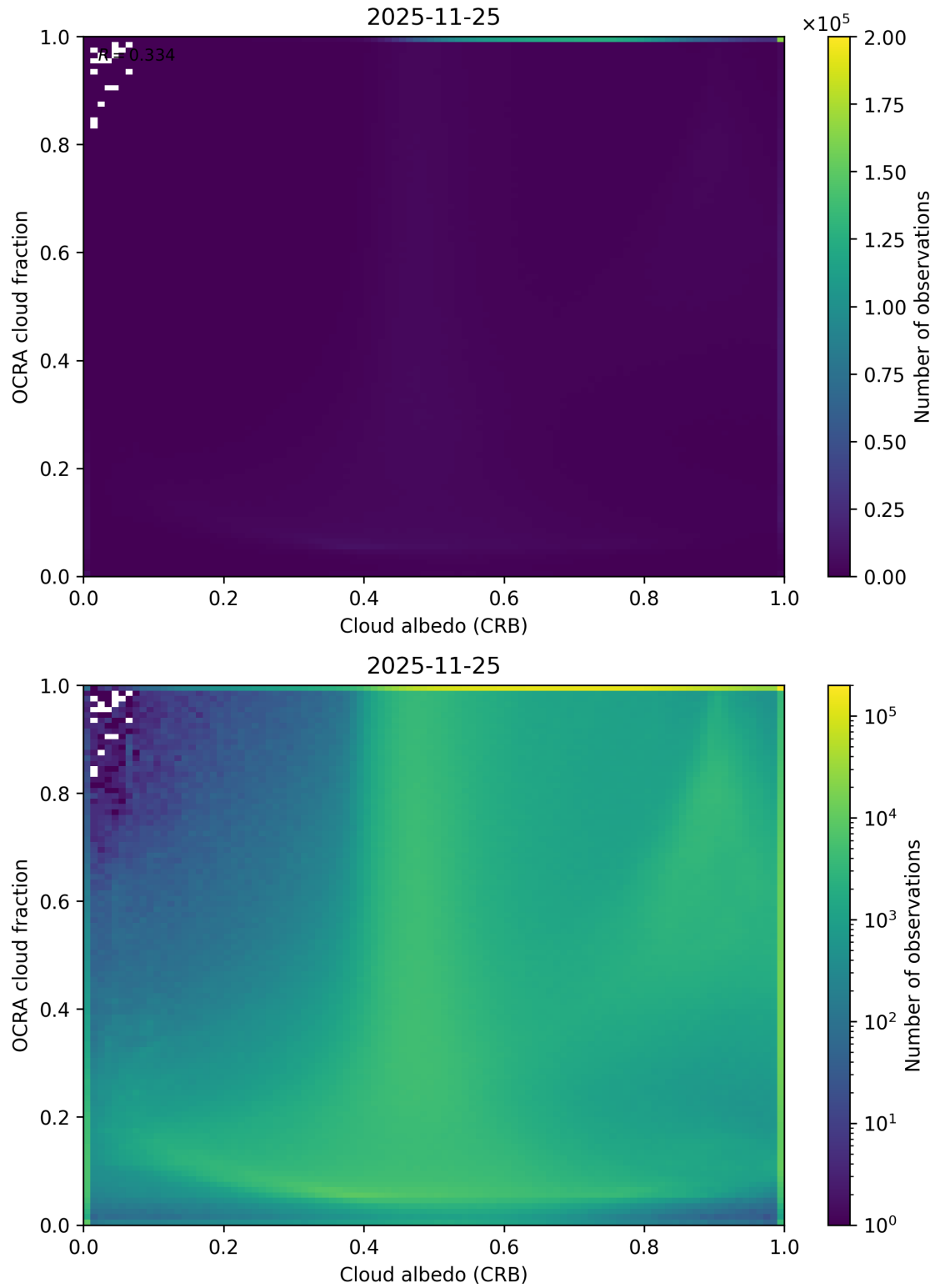
Figure 70: Scatter density plot of “Cloud albedo (CRB)” against “OCRA cloud fraction” for 2025-11-24 to 2025-11-26.
