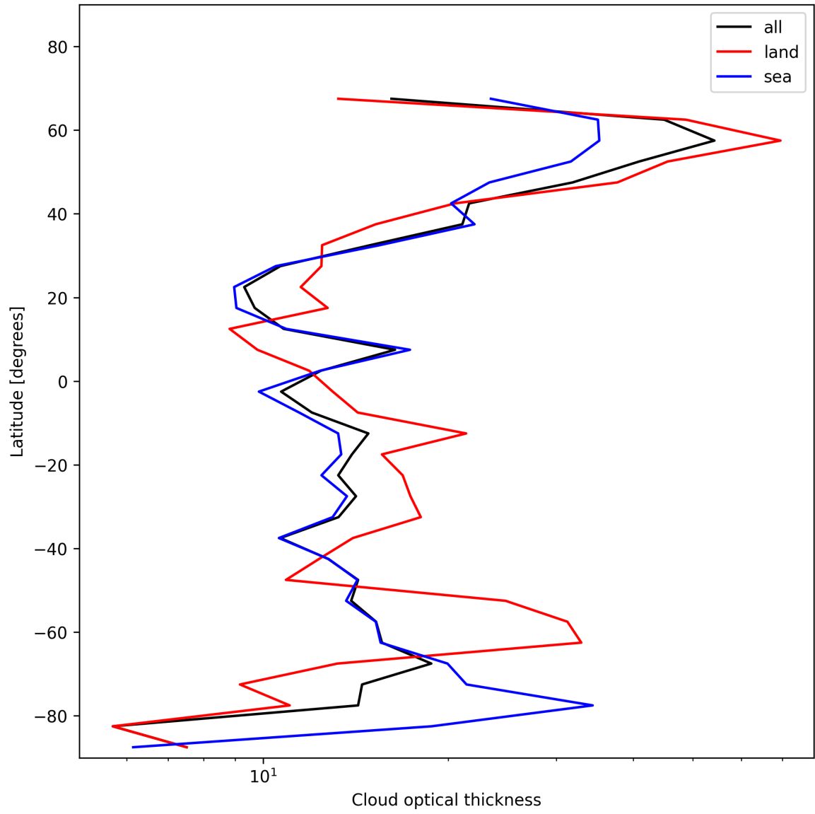
Figure 25: Zonal average of “Cloud optical thickness” for 2025-11-24 to 2025-11-26.
