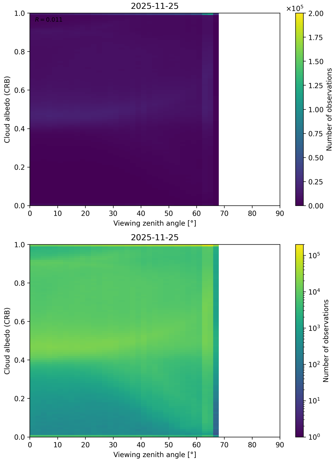
Figure 106: Scatter density plot of “Viewing zenith angle” against “Cloud albedo (CRB)” for 2025-11-24 to 2025-11-26.
