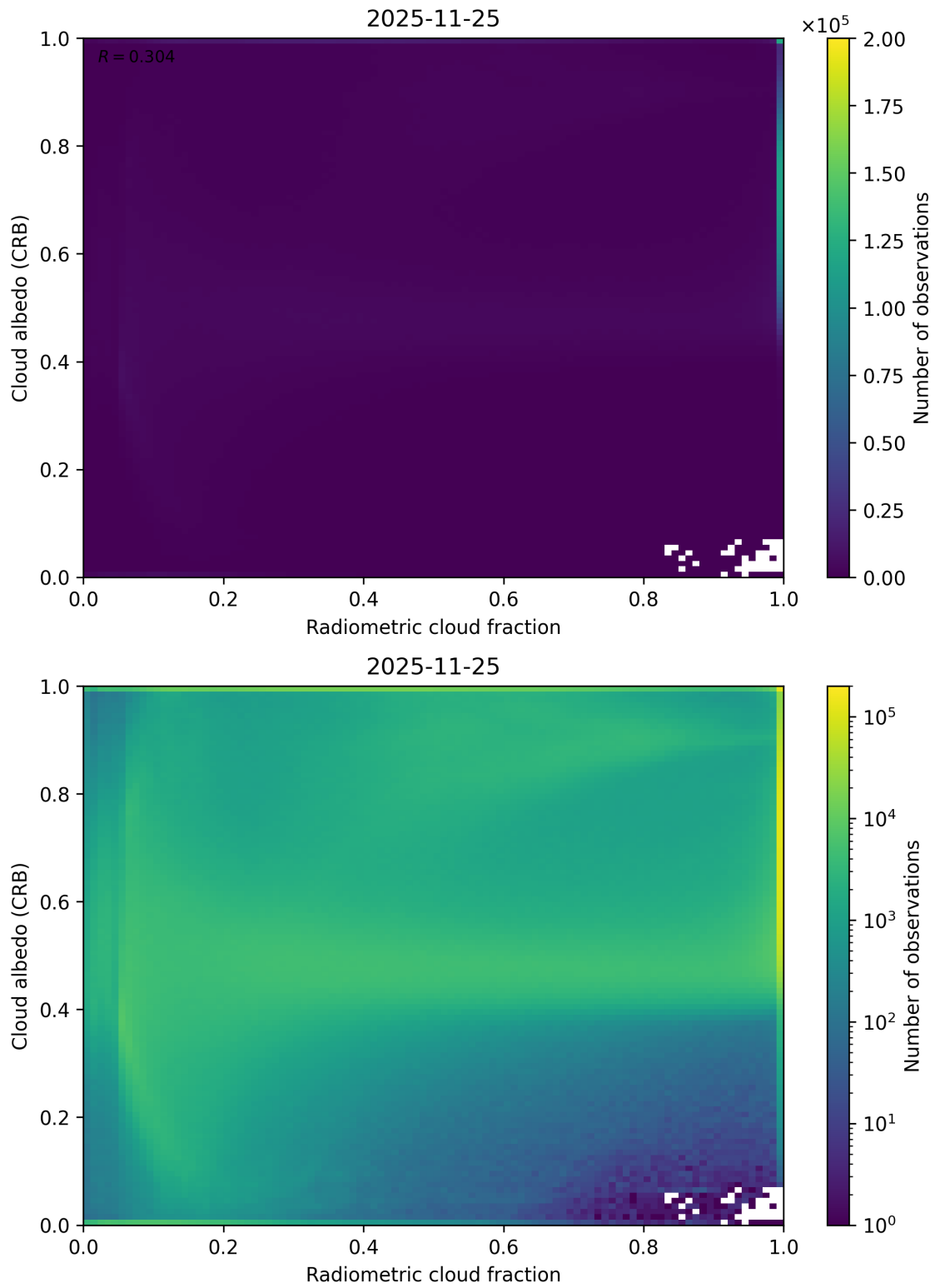
Figure 71: Scatter density plot of “Radiometric cloud fraction” against “Cloud albedo (CRB)” for 2025-11-24 to 2025-11-26.
