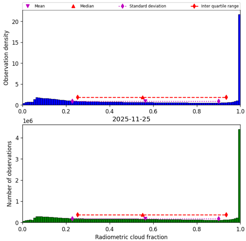
Figure 39: Histogram of “Radiometric cloud fraction” for 2025-11-24 to 2025-11-26
