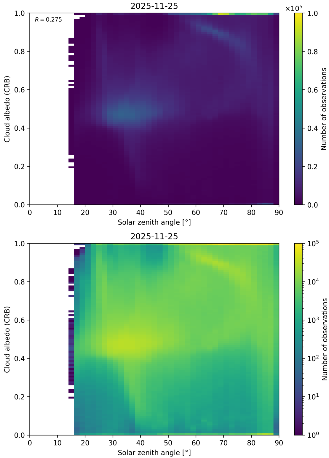
Figure 98: Scatter density plot of “Solar zenith angle” against “Cloud albedo (CRB)” for 2025-11-24 to 2025-11-26.
