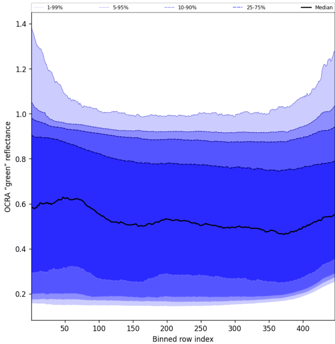
Figure 68: Along track statistics of "OCRA "green" reflectance" for 2025-11-24 to 2025-11-26
