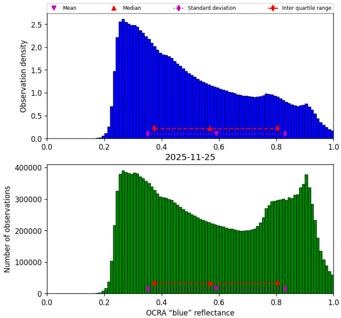
Figure 51: Histogram of “OCRA “blue” reflectance” for 2025-11-24 to 2025-11-26
