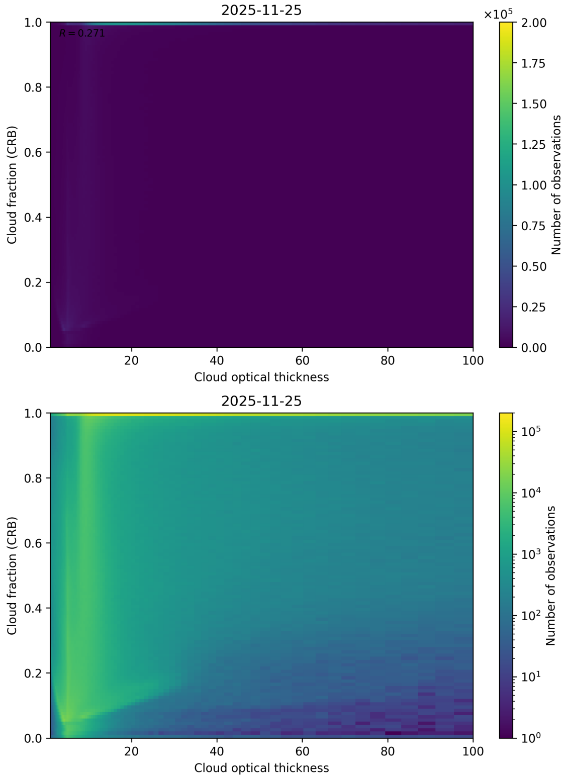
Figure 84: Scatter density plot of “Cloud optical thickness” against “Cloud fraction (CRB)” for 2025-11-24 to 2025-11-26.
