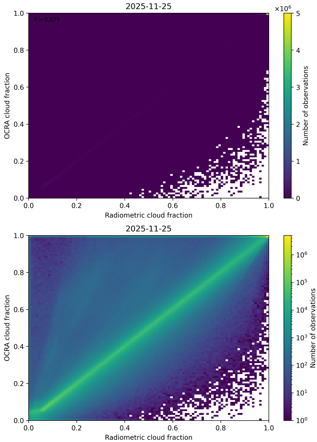
Figure 72: Scatter density plot of “Radiometric cloud fraction” against “OCRA cloud fraction” for 2025-11-24 to 2025-11-26.
