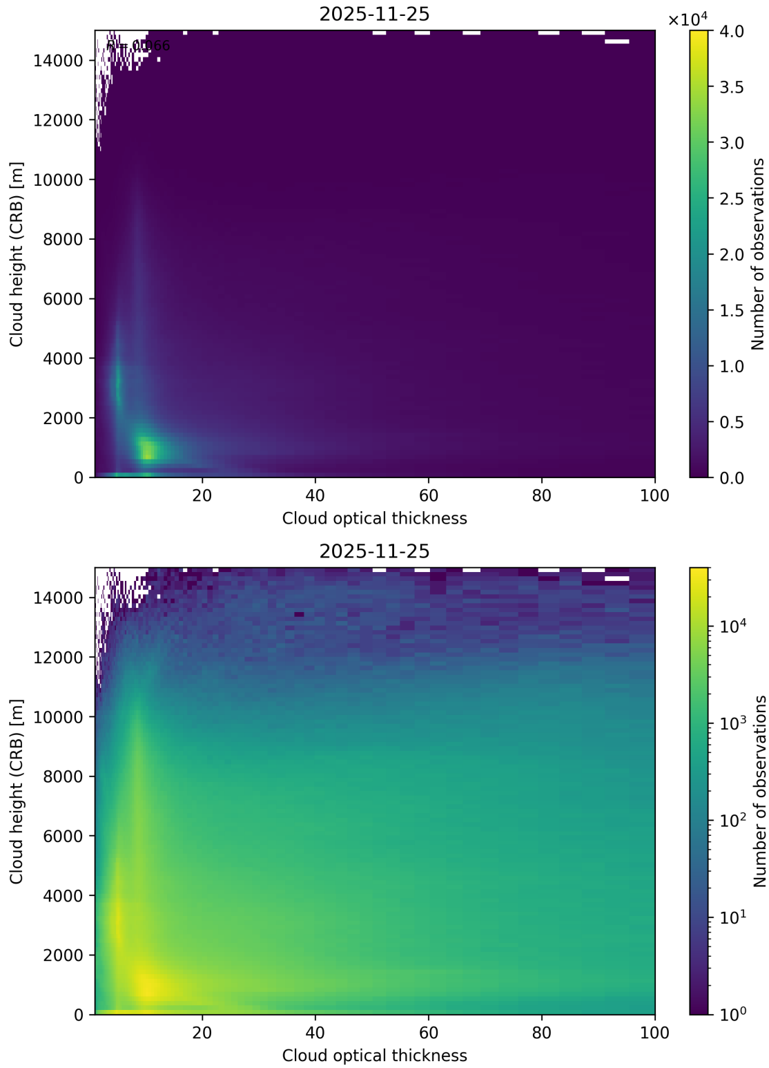
Figure 85: Scatter density plot of “Cloud optical thickness” against “Cloud height (CRB)” for 2025-11-24 to 2025-11-26.
