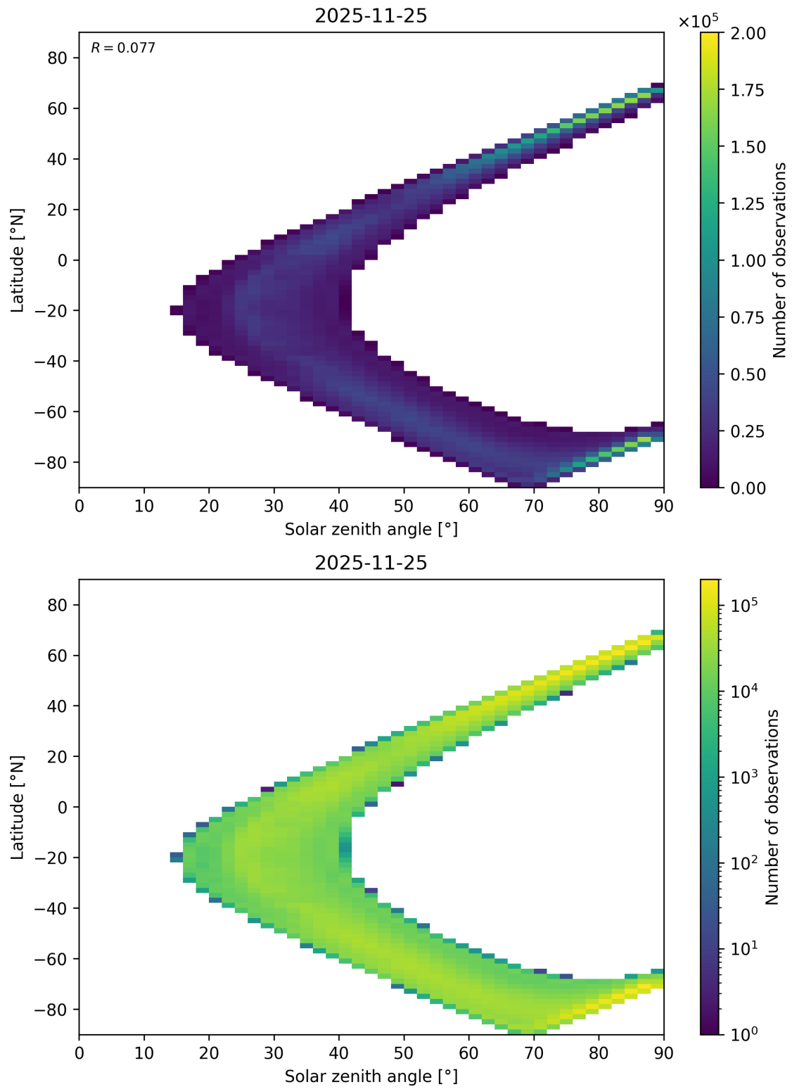
Figure 105: Scatter density plot of “Solar zenith angle” against “Latitude” for 2025-11-24 to 2025-11-26.
