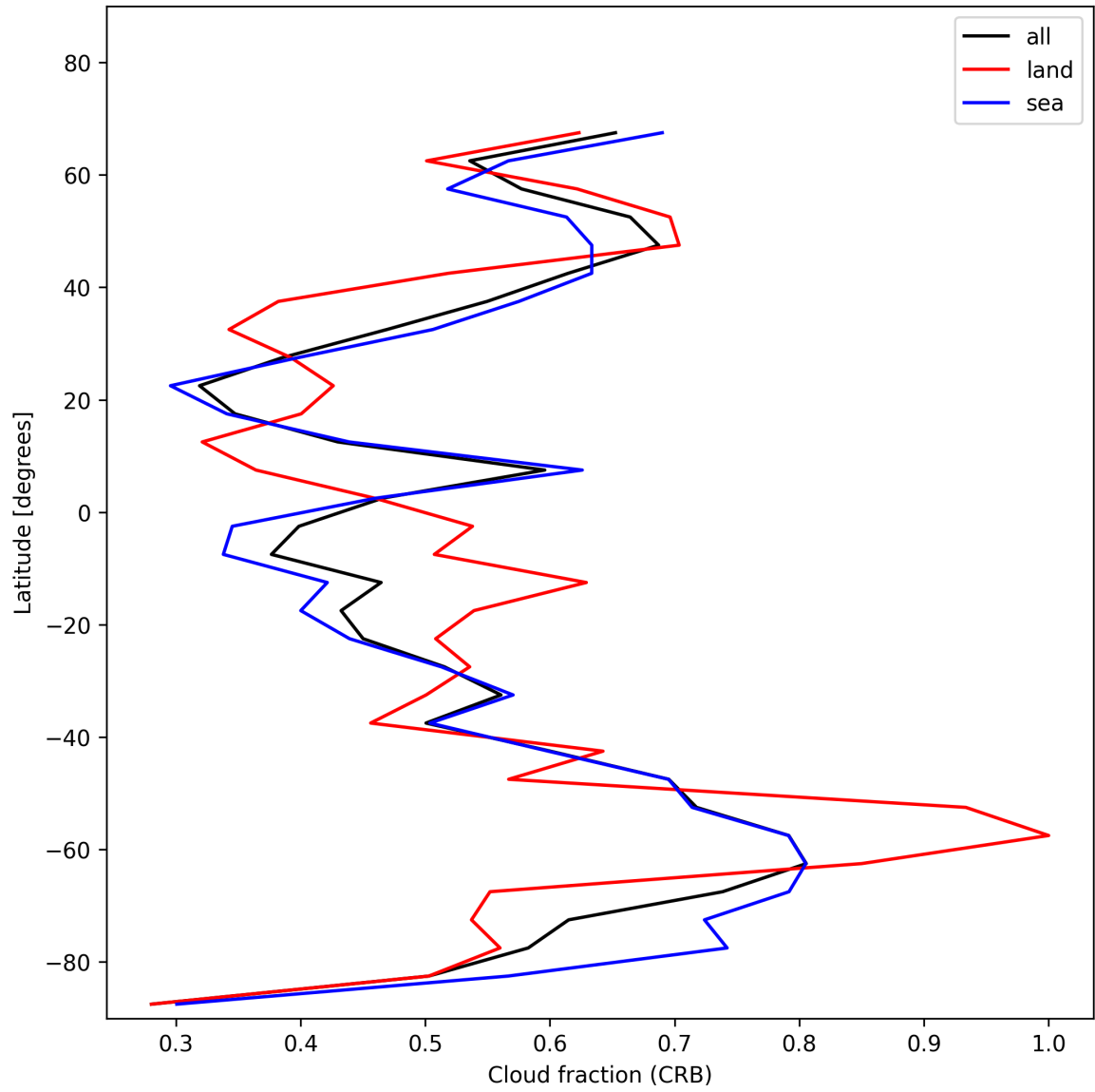
Figure 26: Zonal average of “Cloud fraction (CRB)” for 2025-11-24 to 2025-11-26.
