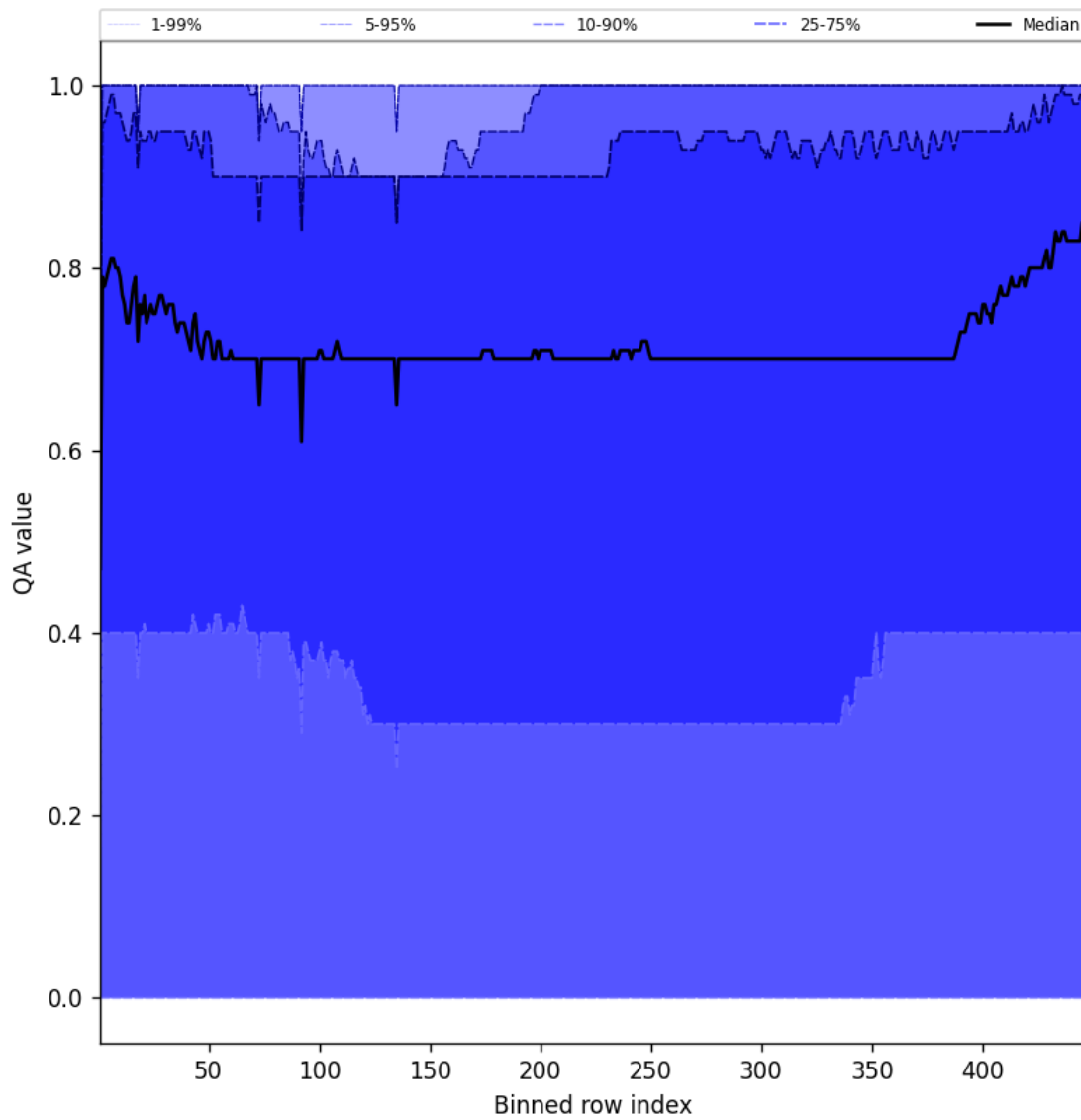
Figure 54: Along track statistics of “QA value” for 2025-11-24 to 2025-11-26
