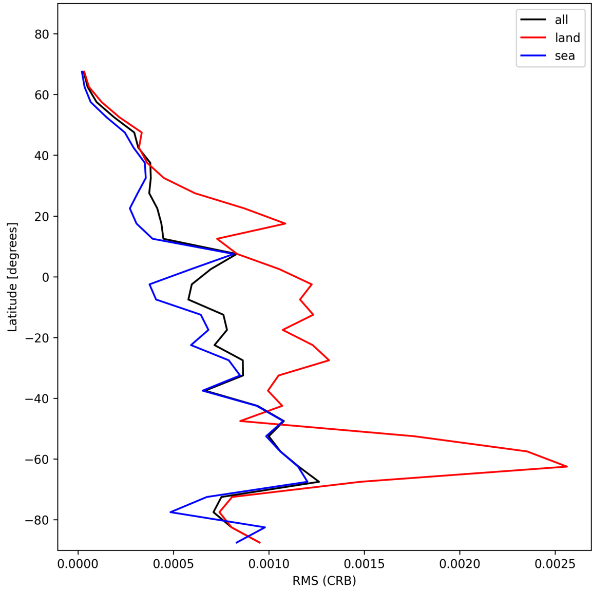
Figure 32: Zonal average of “RMS (CRB)” for 2025-11-24 to 2025-11-26.
