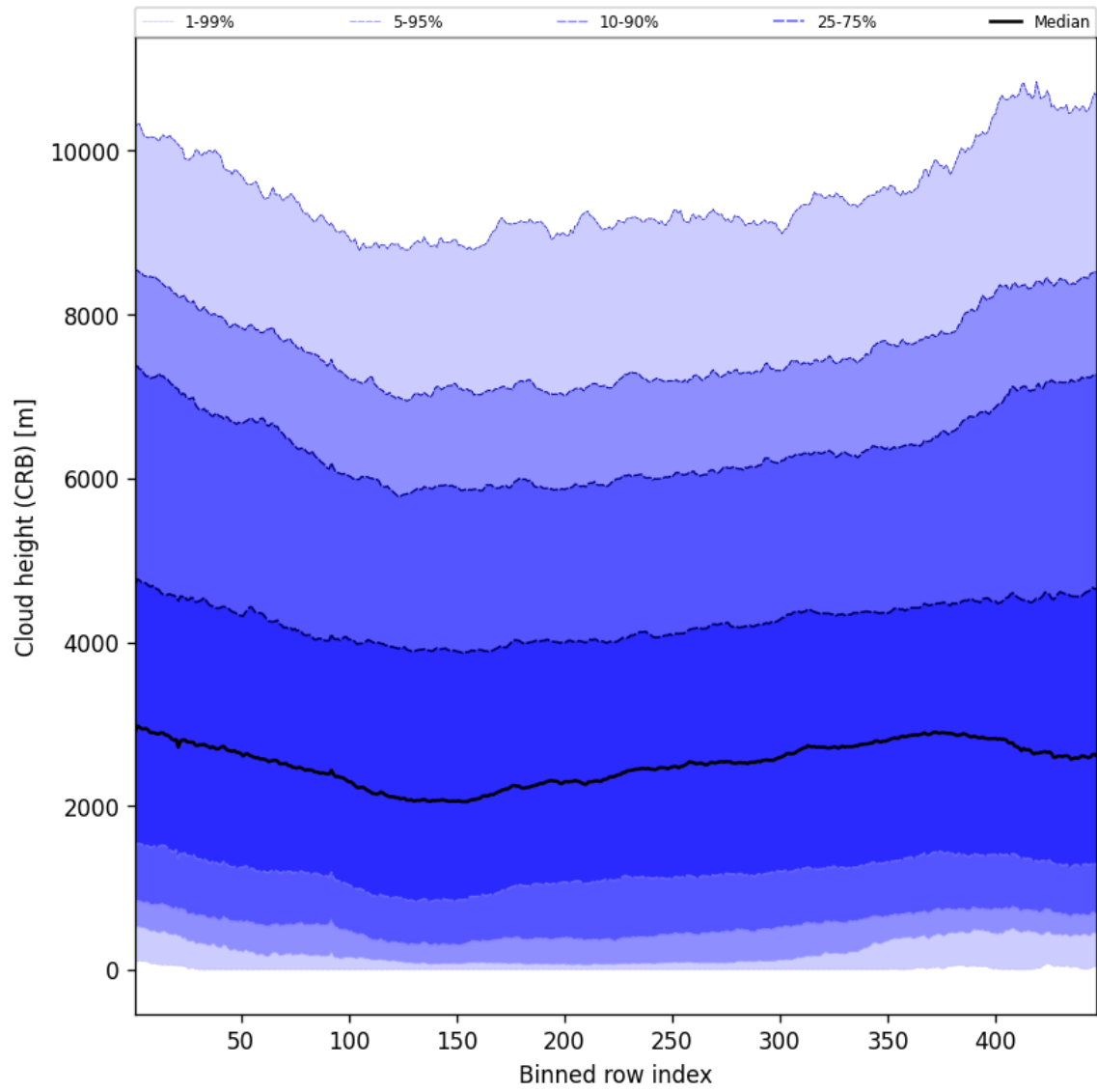
Figure 59: Along track statistics of “Cloud height (CRB)” for 2025-11-24 to 2025-11-26
