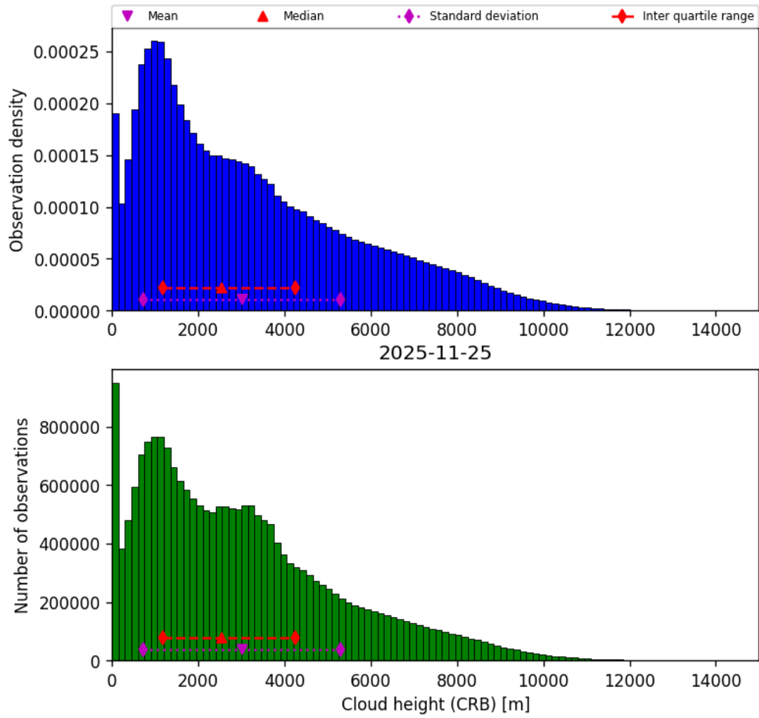
Figure 43: Histogram of “Cloud height (CRB)” for 2025-11-24 to 2025-11-26
