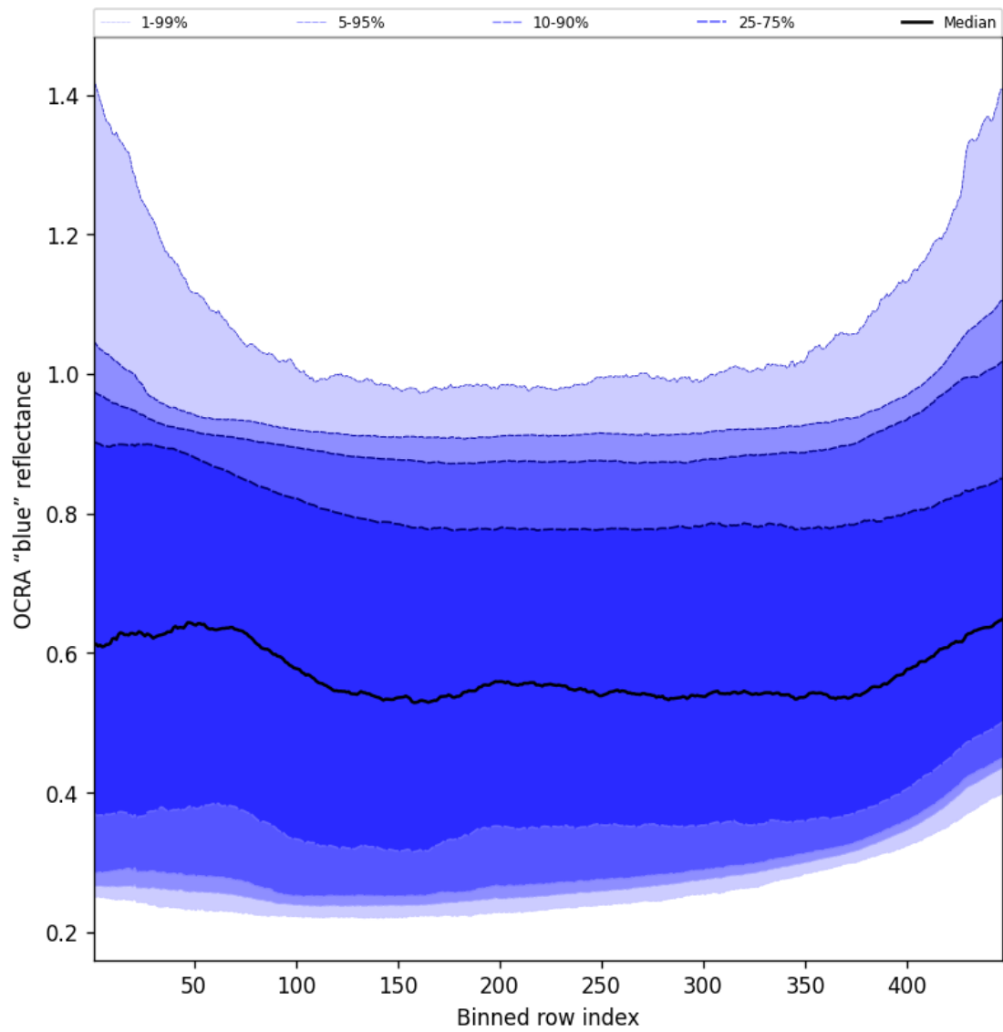
Figure 67: Along track statistics of “OCRA “blue” reflectance” for 2025-11-24 to 2025-11-26
