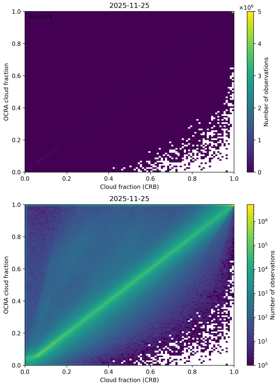
Figure 78: Scatter density plot of “Cloud fraction (CRB)” against “OCRA cloud fraction” for 2025-11-24 to 2025-11-26.
