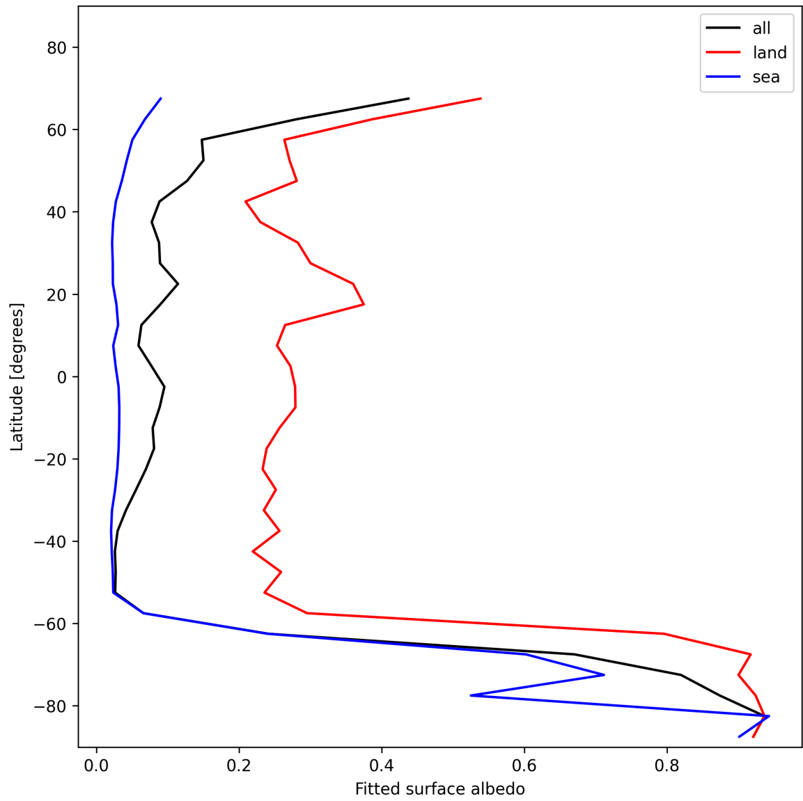
Figure 29: Zonal average of “Fitted surface albedo” for 2025-11-24 to 2025-11-26.
