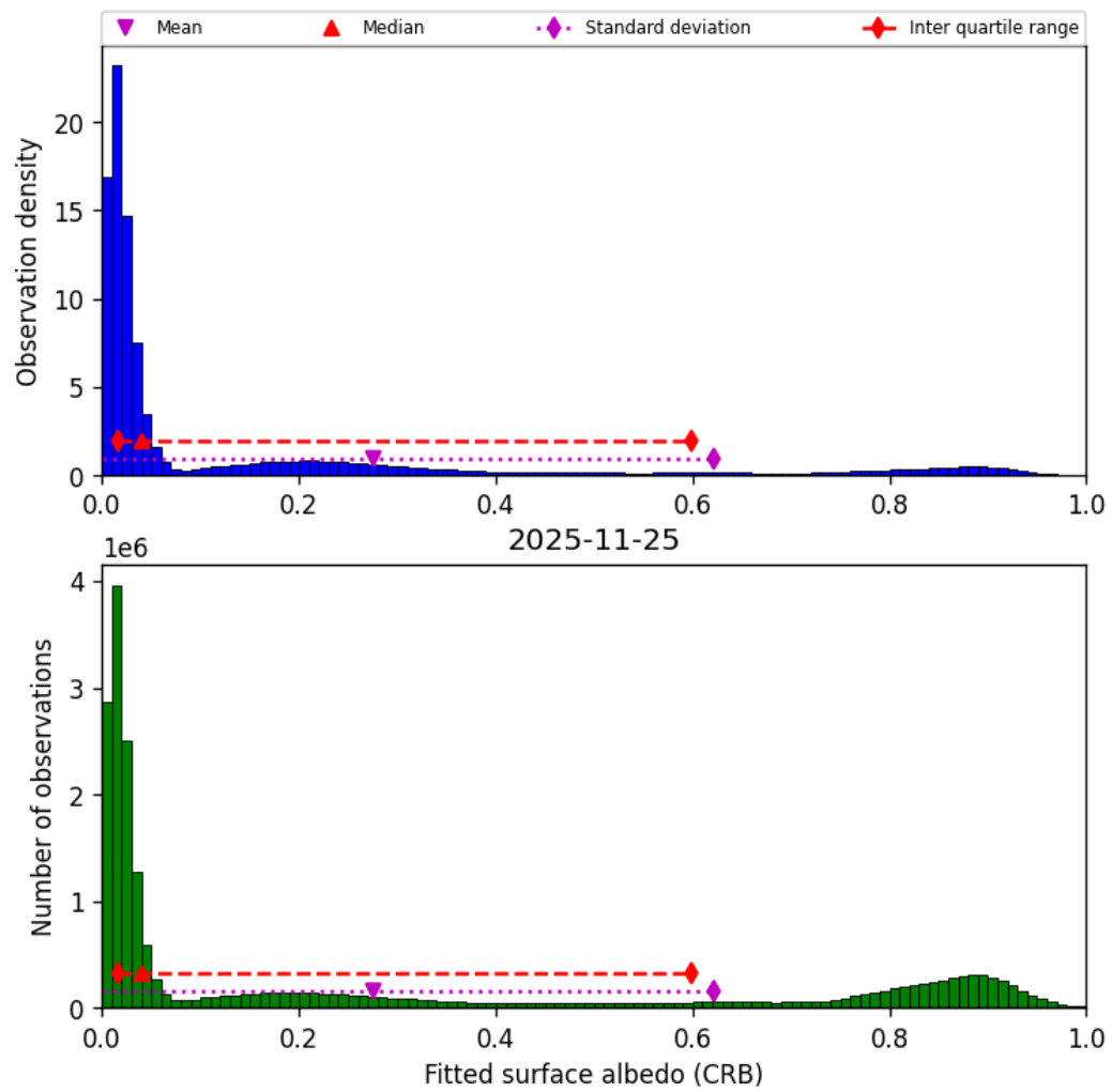
Figure 46: Histogram of “Fitted surface albedo (CRB)” for 2025-11-24 to 2025-11-26
