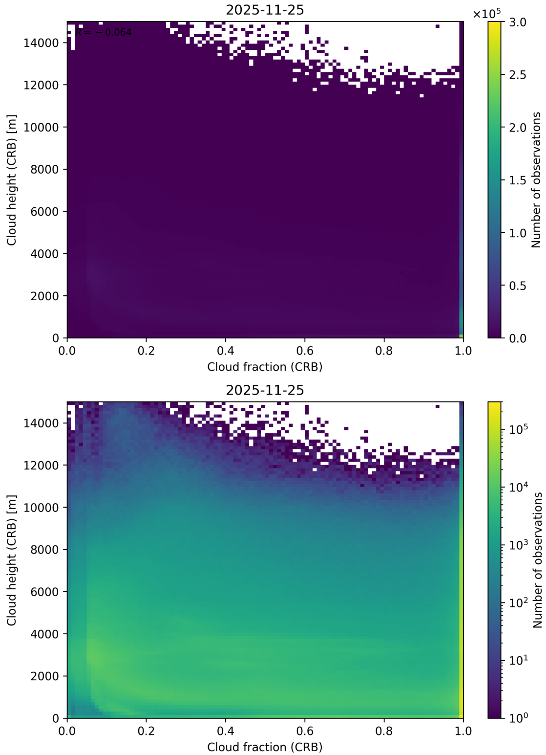
Figure 79: Scatter density plot of “Cloud fraction (CRB)” against “Cloud height (CRB)” for 2025-11-24 to 2025-11-26.
