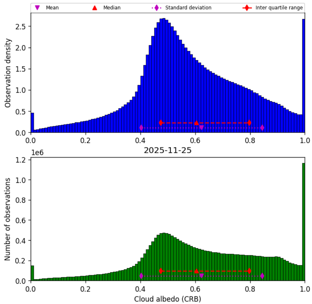
Figure 44: Histogram of “Cloud albedo (CRB)” for 2025-11-24 to 2025-11-26
