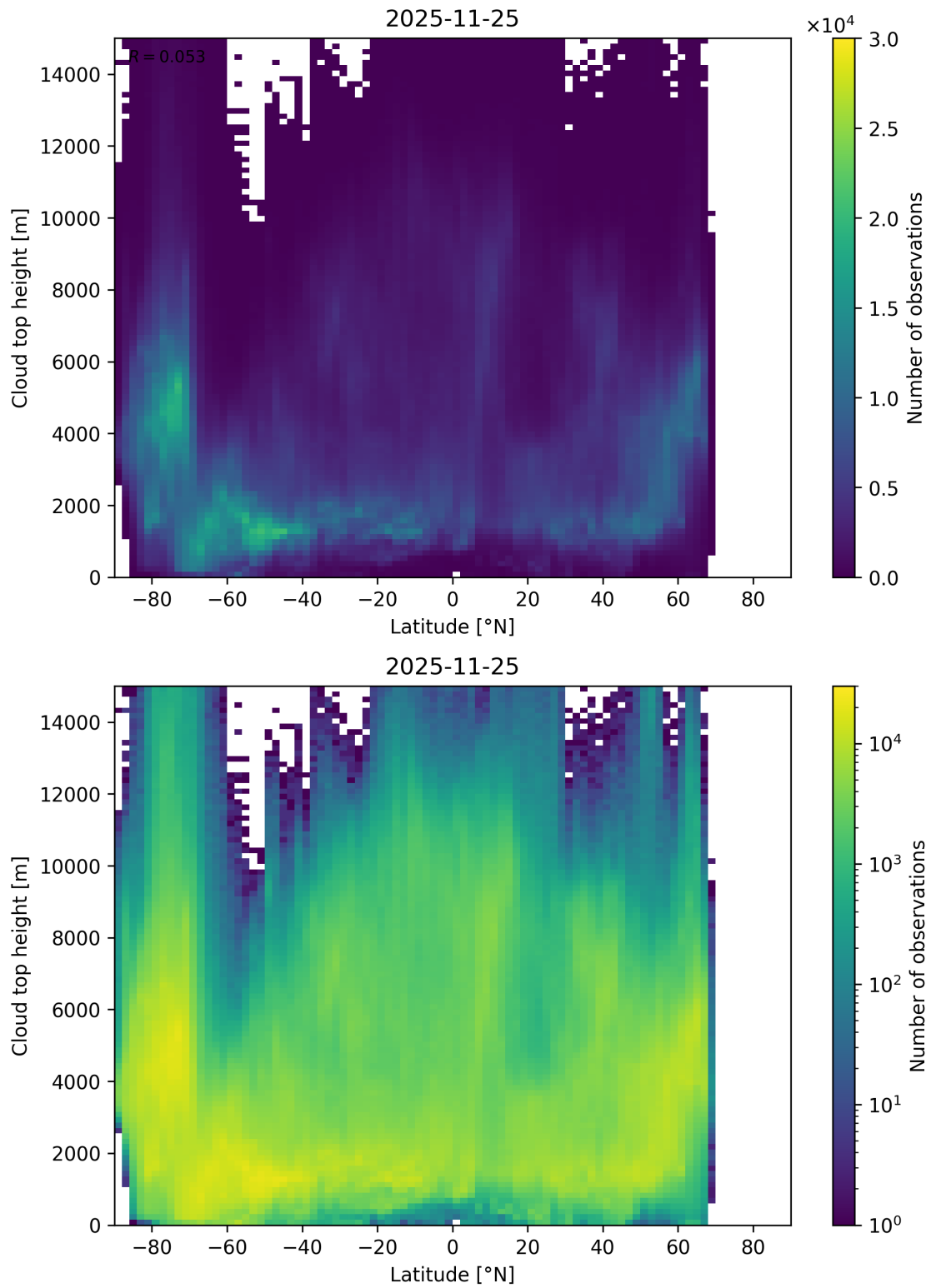
Figure 97: Scatter density plot of “Latitude” against “Cloud top height” for 2025-11-24 to 2025-11-26.
