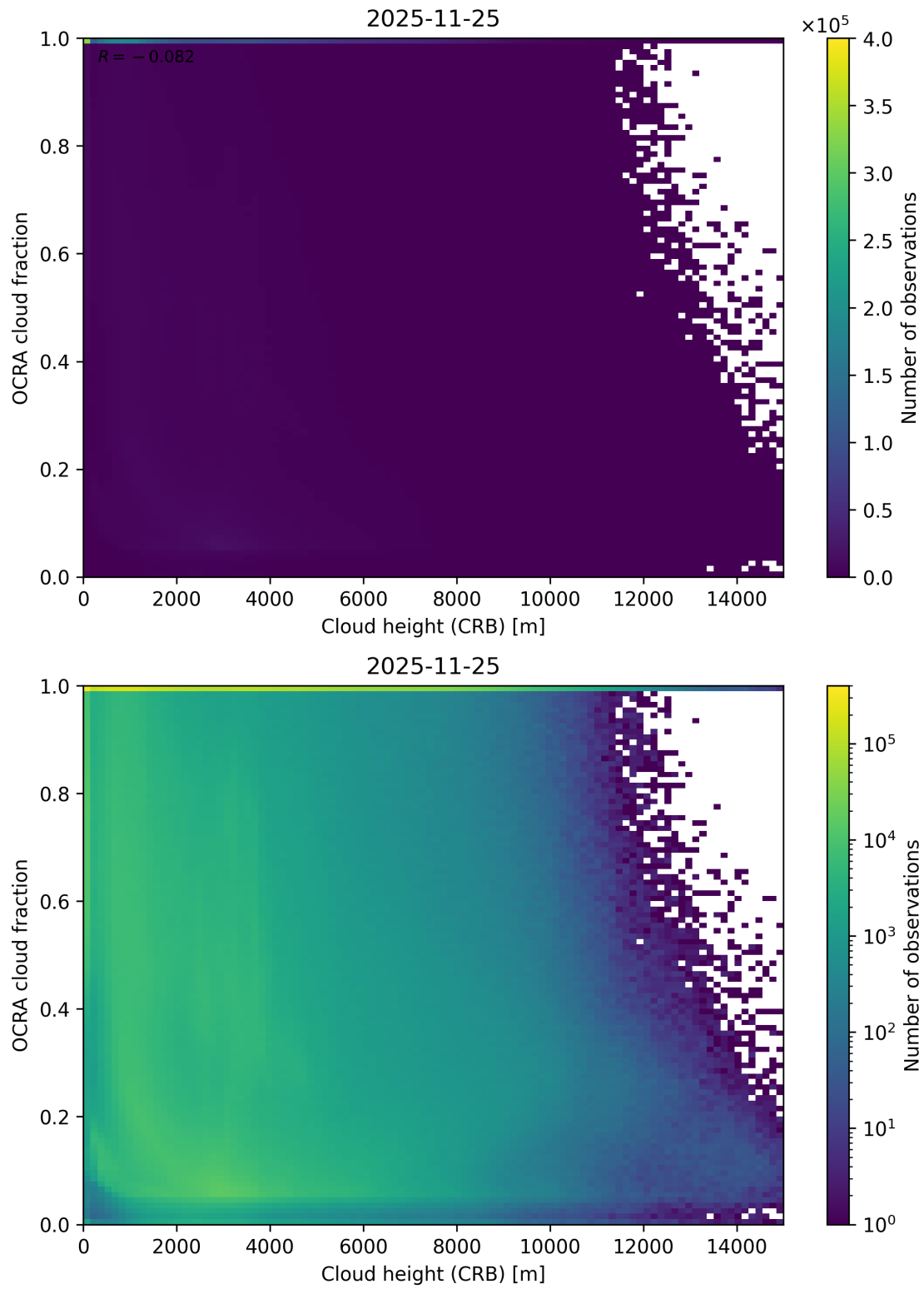
Figure 81: Scatter density plot of “Cloud height (CRB)” against “OCRA cloud fraction” for 2025-11-24 to 2025-11-26.
