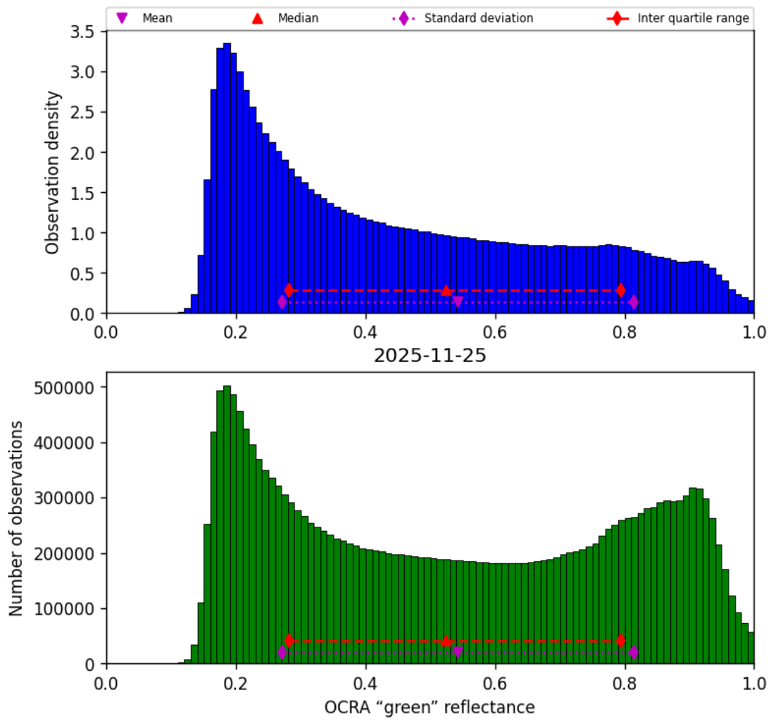
Figure 52: Histogram of “OCRA “green” reflectance” for 2025-11-24 to 2025-11-26
