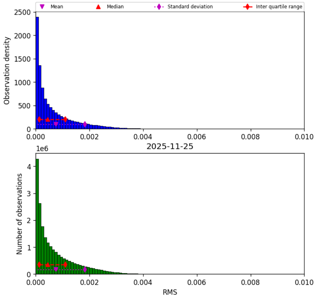
Figure 47: Histogram of “RMS” for 2025-11-24 to 2025-11-26
