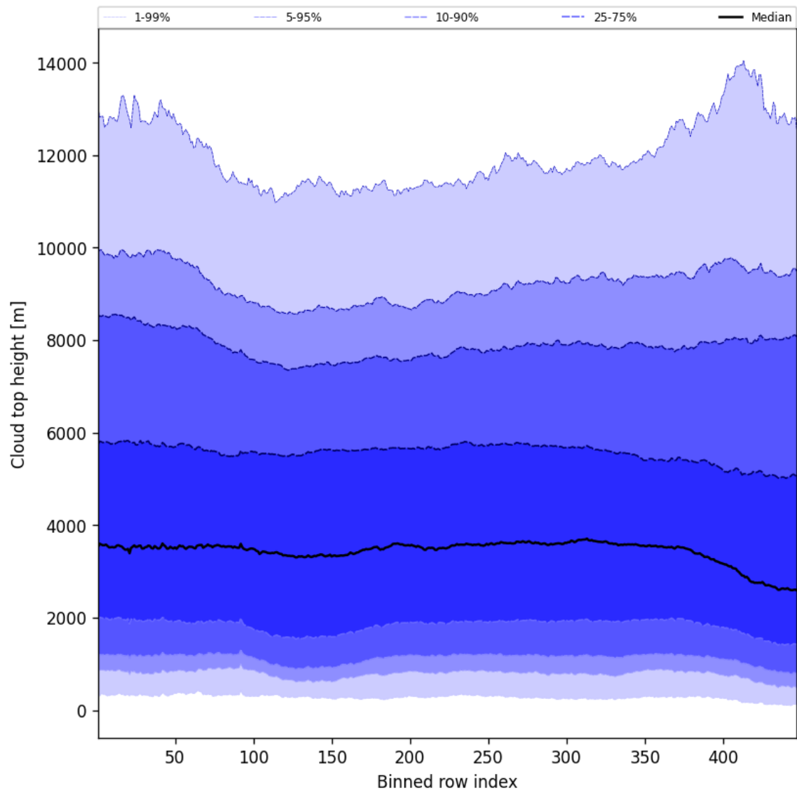
Figure 56: Along track statistics of “Cloud top height” for 2025-11-24 to 2025-11-26
