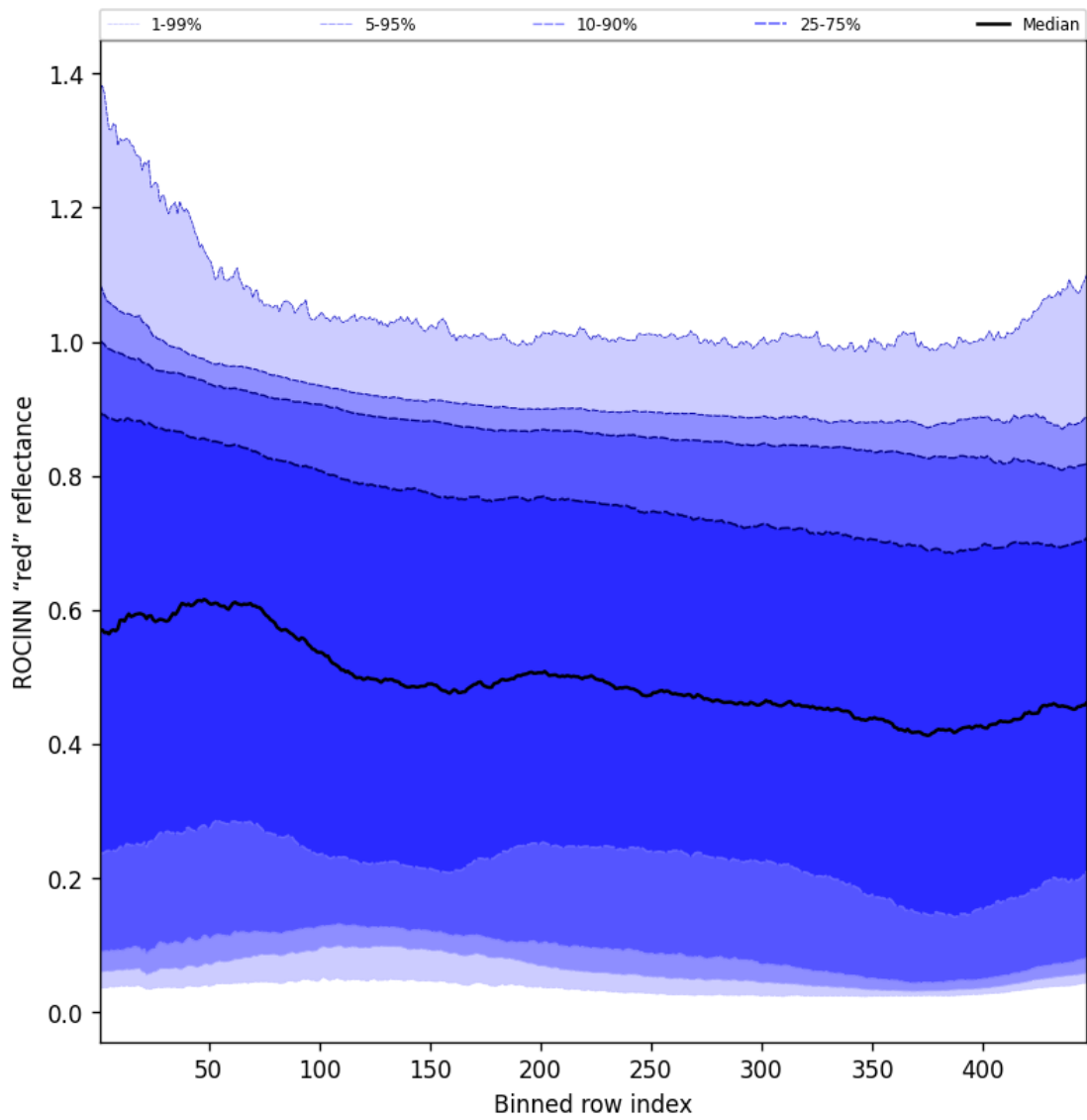
Figure 69: Along track statistics of “ROCINN “red” reflectance” for 2025-11-24 to 2025-11-26
