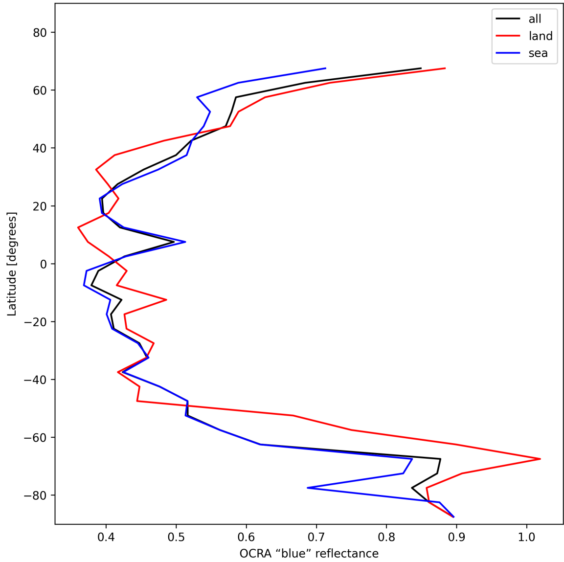
Figure 35: Zonal average of “OCRA “blue” reflectance” for 2025-11-24 to 2025-11-26.
