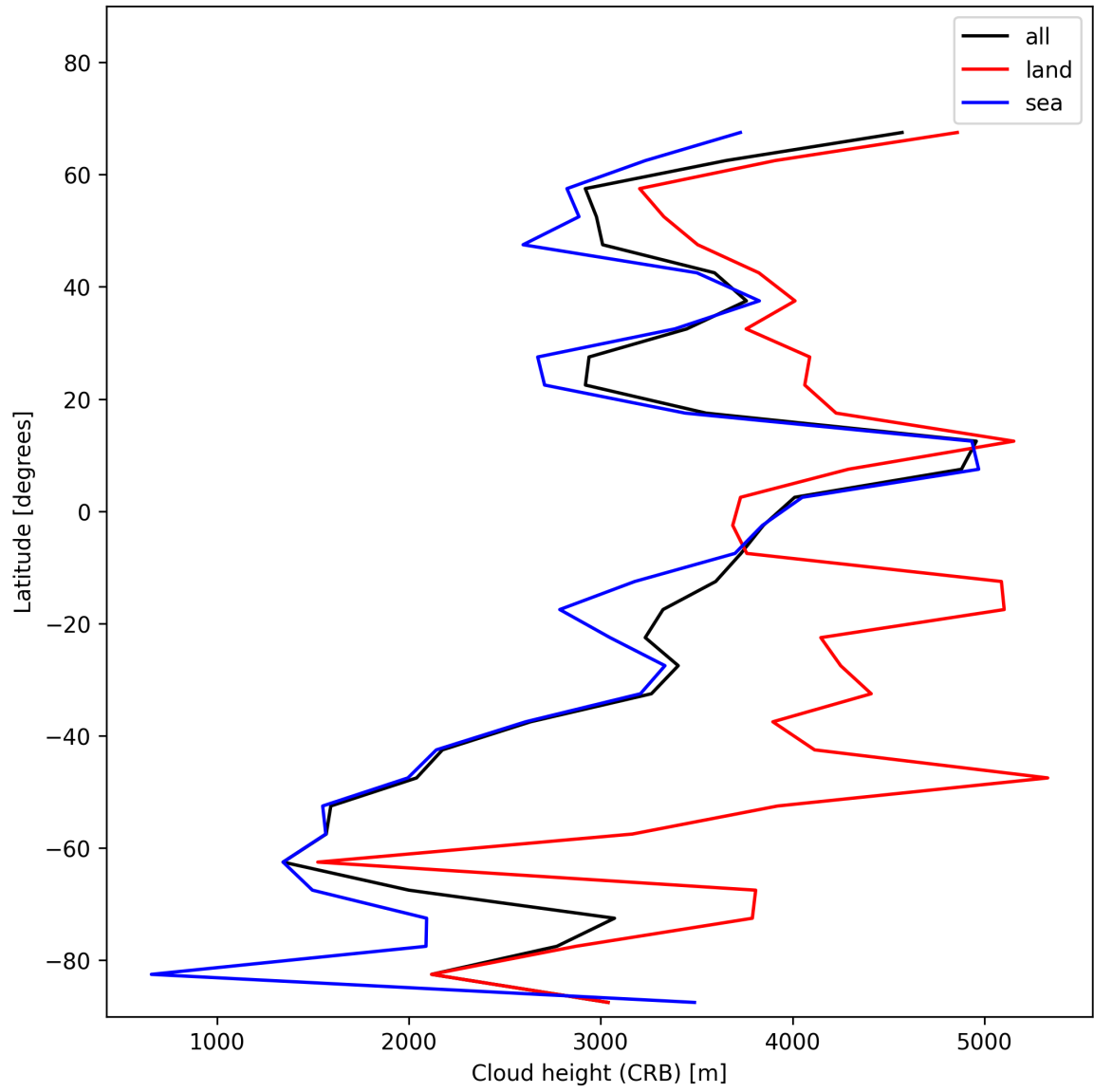
Figure 27: Zonal average of “Cloud height (CRB)” for 2025-11-24 to 2025-11-26.
