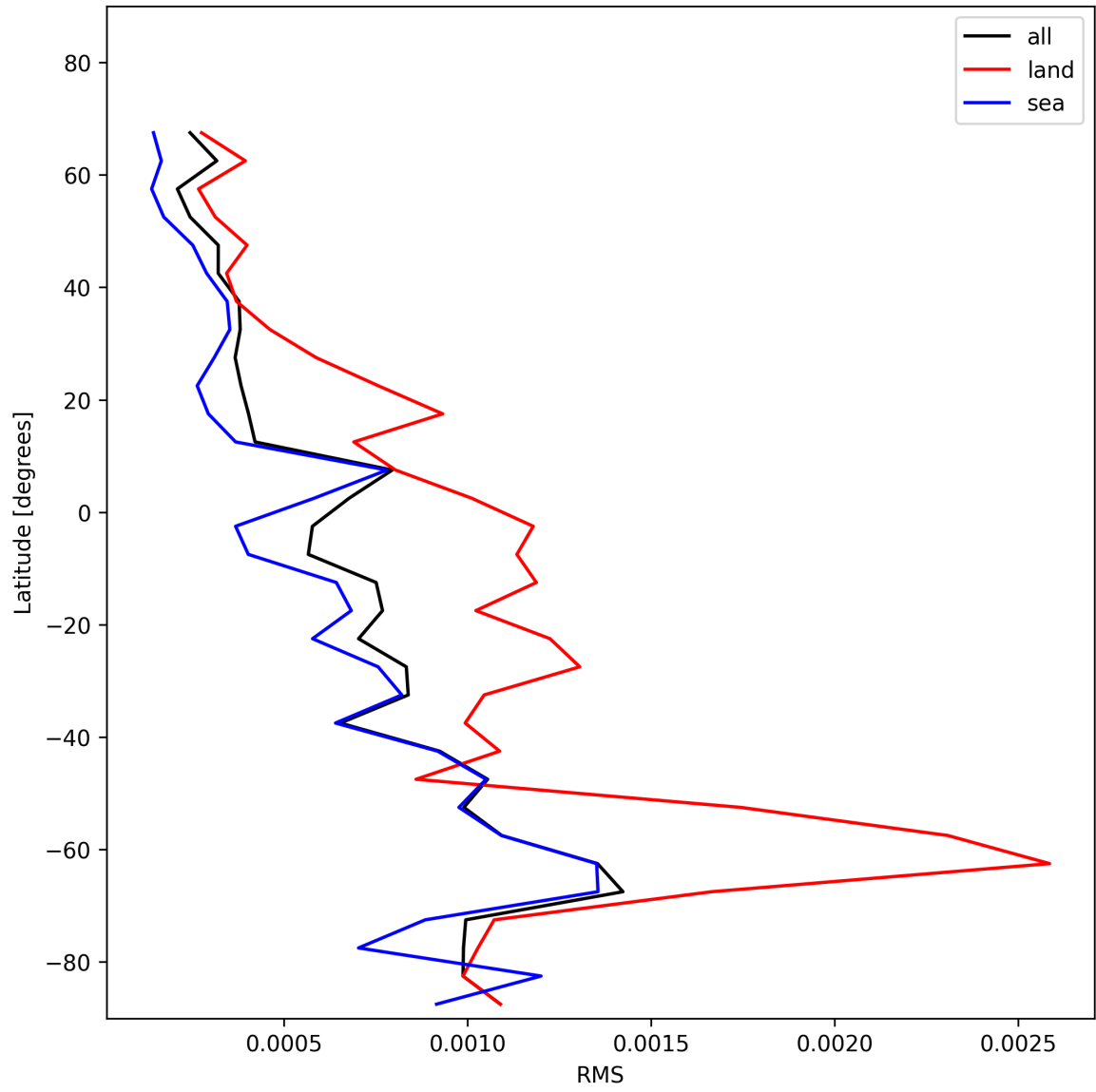
Figure 31: Zonal average of “RMS” for 2025-11-24 to 2025-11-26.
