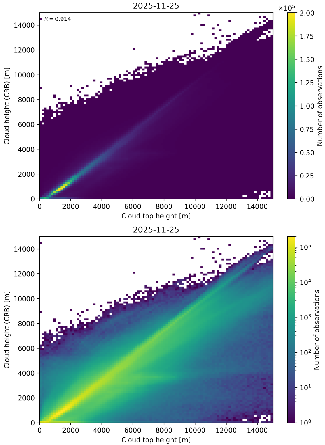
Figure 89: Scatter density plot of “Cloud top height” against “Cloud height (CRB)” for 2025-11-24 to 2025-11-26.
