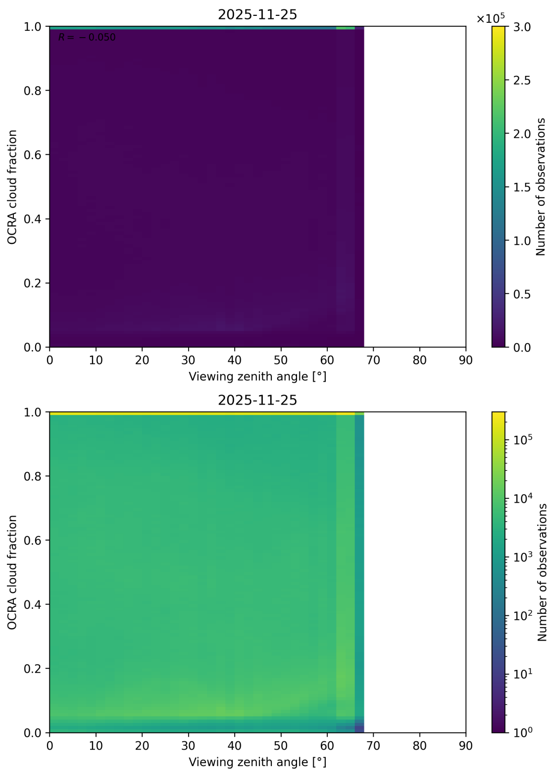
Figure 108: Scatter density plot of “Viewing zenith angle” against “OCRA cloud fraction” for 2025-11-24 to 2025-11-26.
