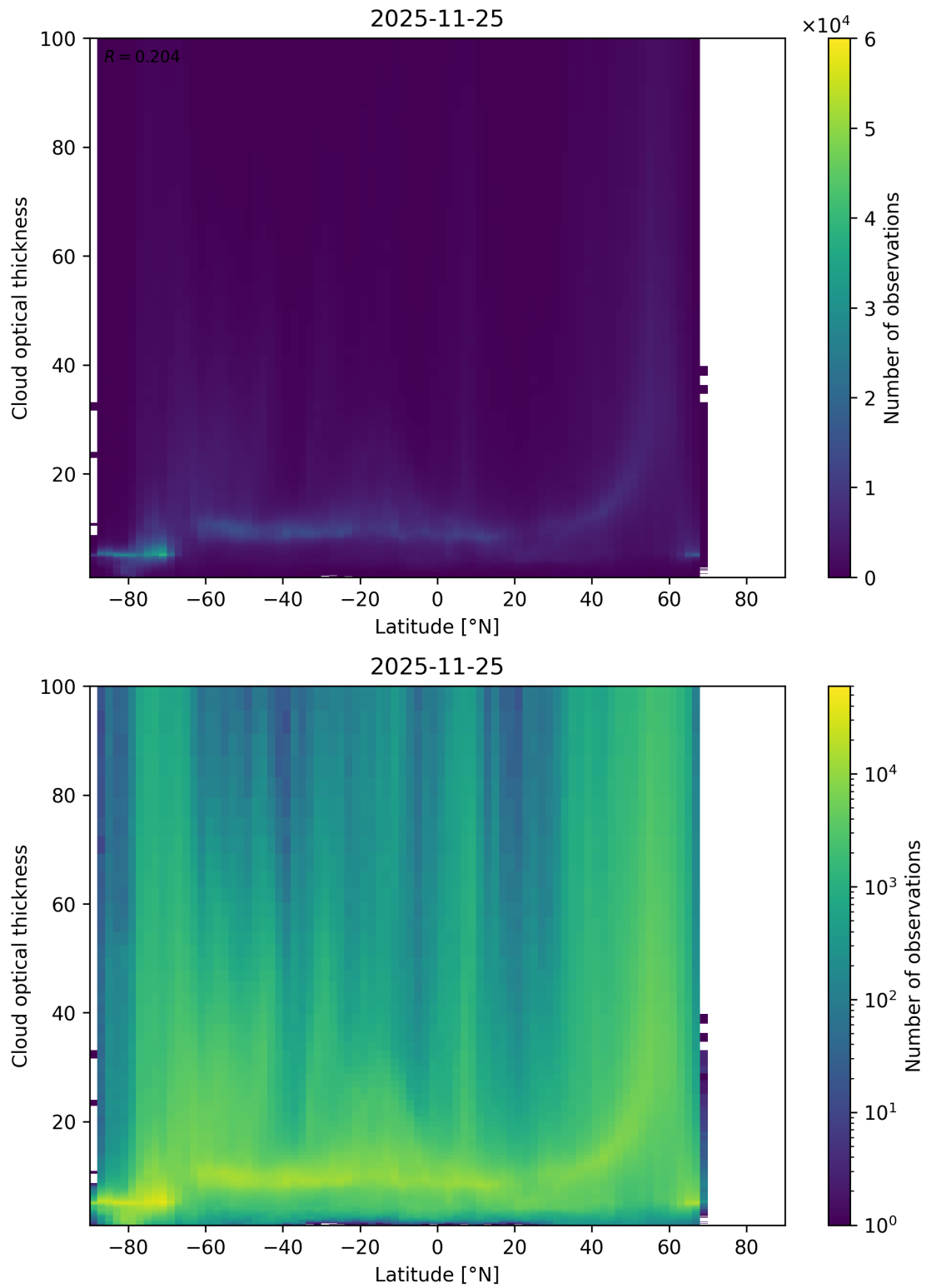
Figure 96: Scatter density plot of “Latitude” against “Cloud optical thickness” for 2025-11-24 to 2025-11-26.
