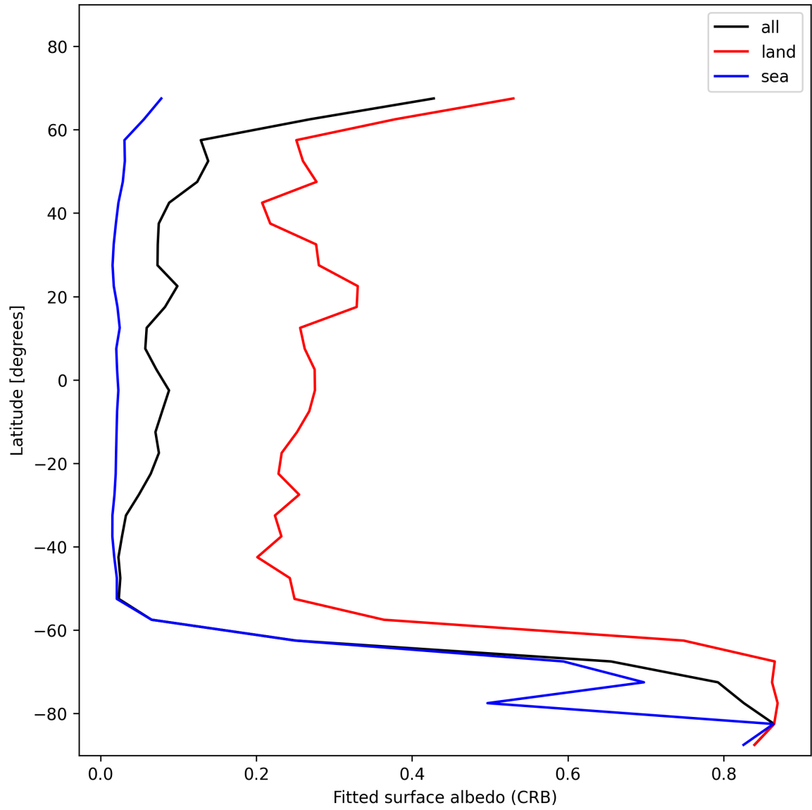
Figure 30: Zonal average of “Fitted surface albedo (CRB)” for 2025-11-25 to 2025-11-27.
