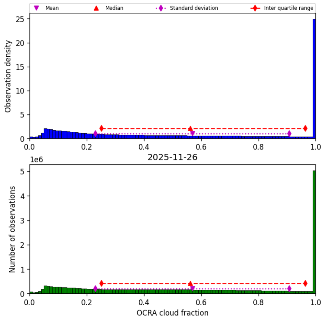
Figure 50: Histogram of “OCRA cloud fraction” for 2025-11-25 to 2025-11-27
