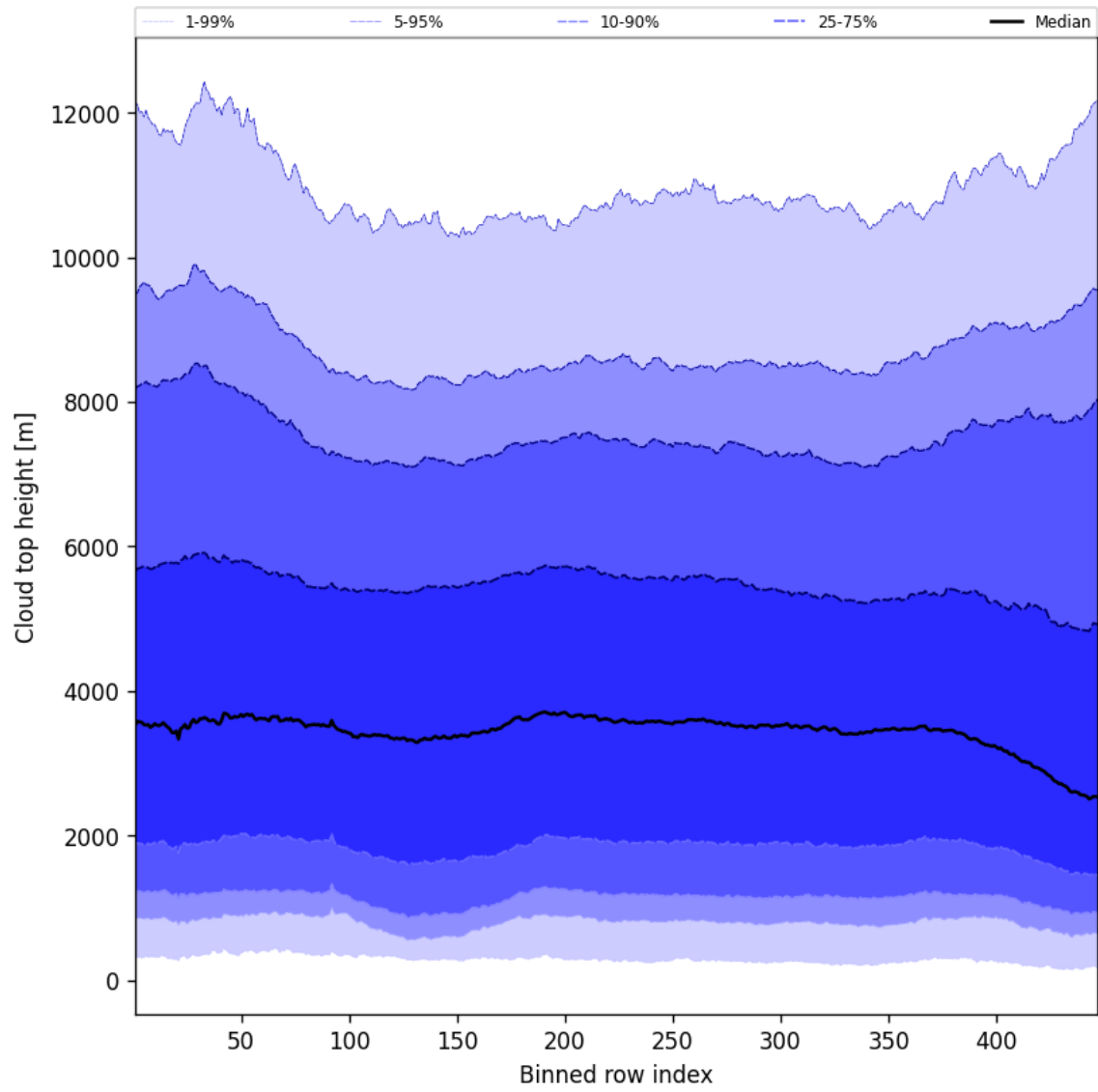
Figure 56: Along track statistics of “Cloud top height” for 2025-11-25 to 2025-11-27
