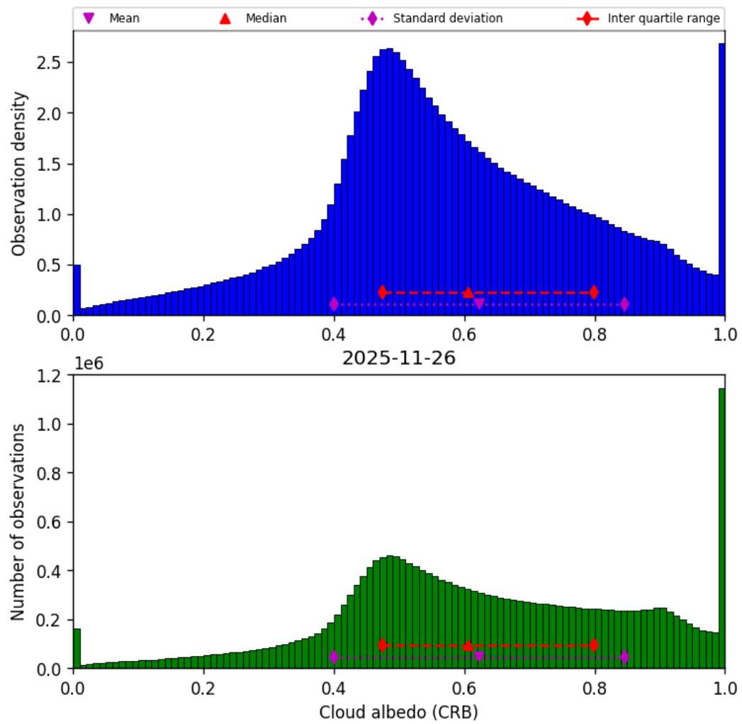
Figure 44: Histogram of “Cloud albedo (CRB)” for 2025-11-25 to 2025-11-27
