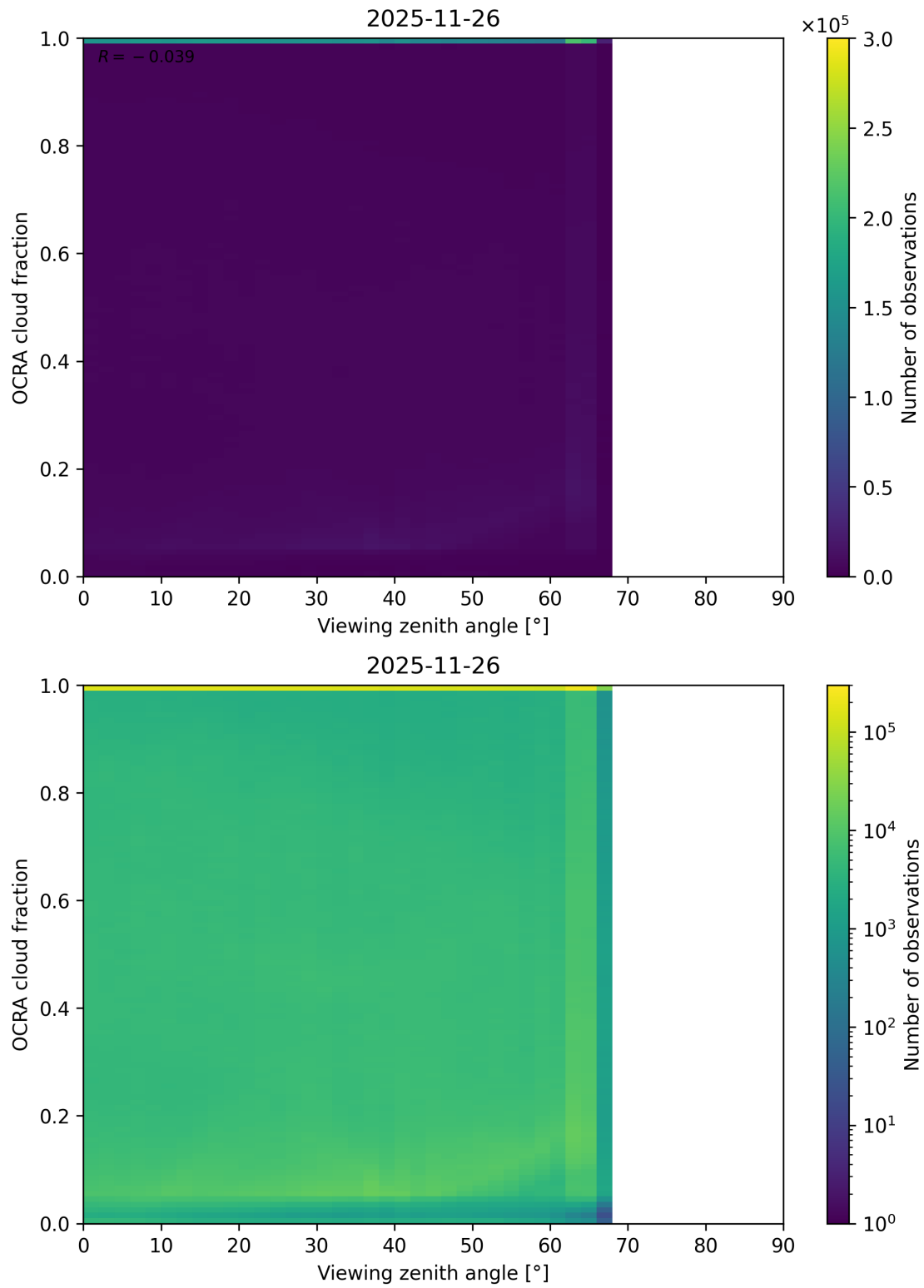
Figure 108: Scatter density plot of “Viewing zenith angle” against “OCRA cloud fraction” for 2025-11-25 to 2025-11-27.
