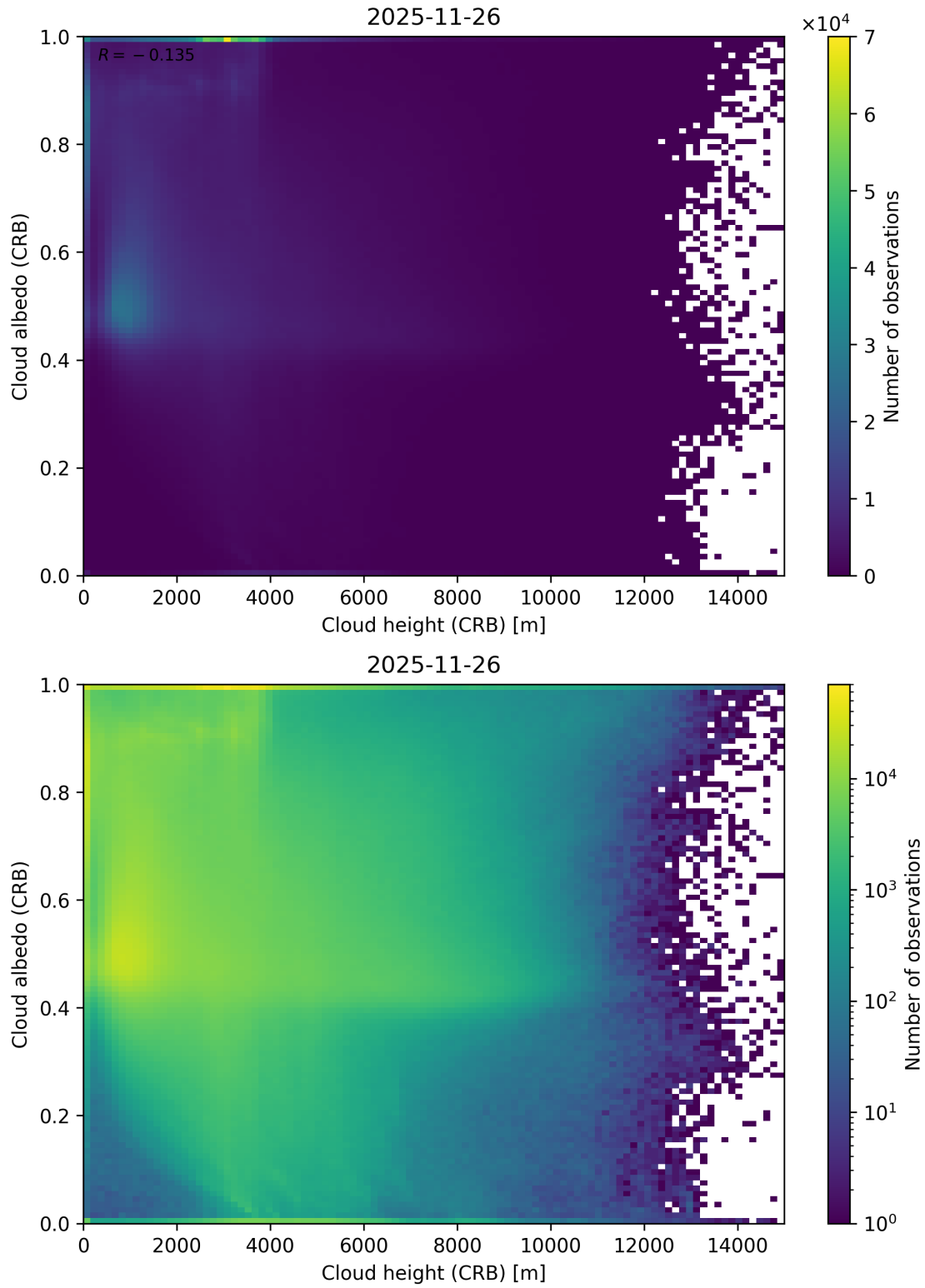
Figure 80: Scatter density plot of “Cloud height (CRB)” against “Cloud albedo (CRB)” for 2025-11-25 to 2025-11-27.
