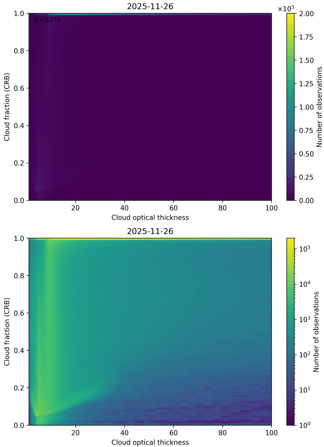
Figure 84: Scatter density plot of “Cloud optical thickness” against “Cloud fraction (CRB)” for 2025-11-25 to 2025-11-27.
