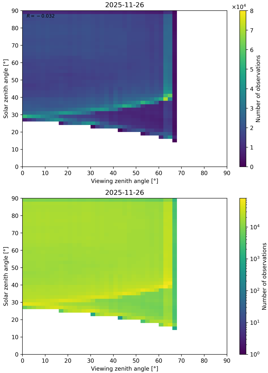
Figure 114: Scatter density plot of “Viewing zenith angle” against “Solar zenith angle” for 2025-11-25 to 2025-11-27.
