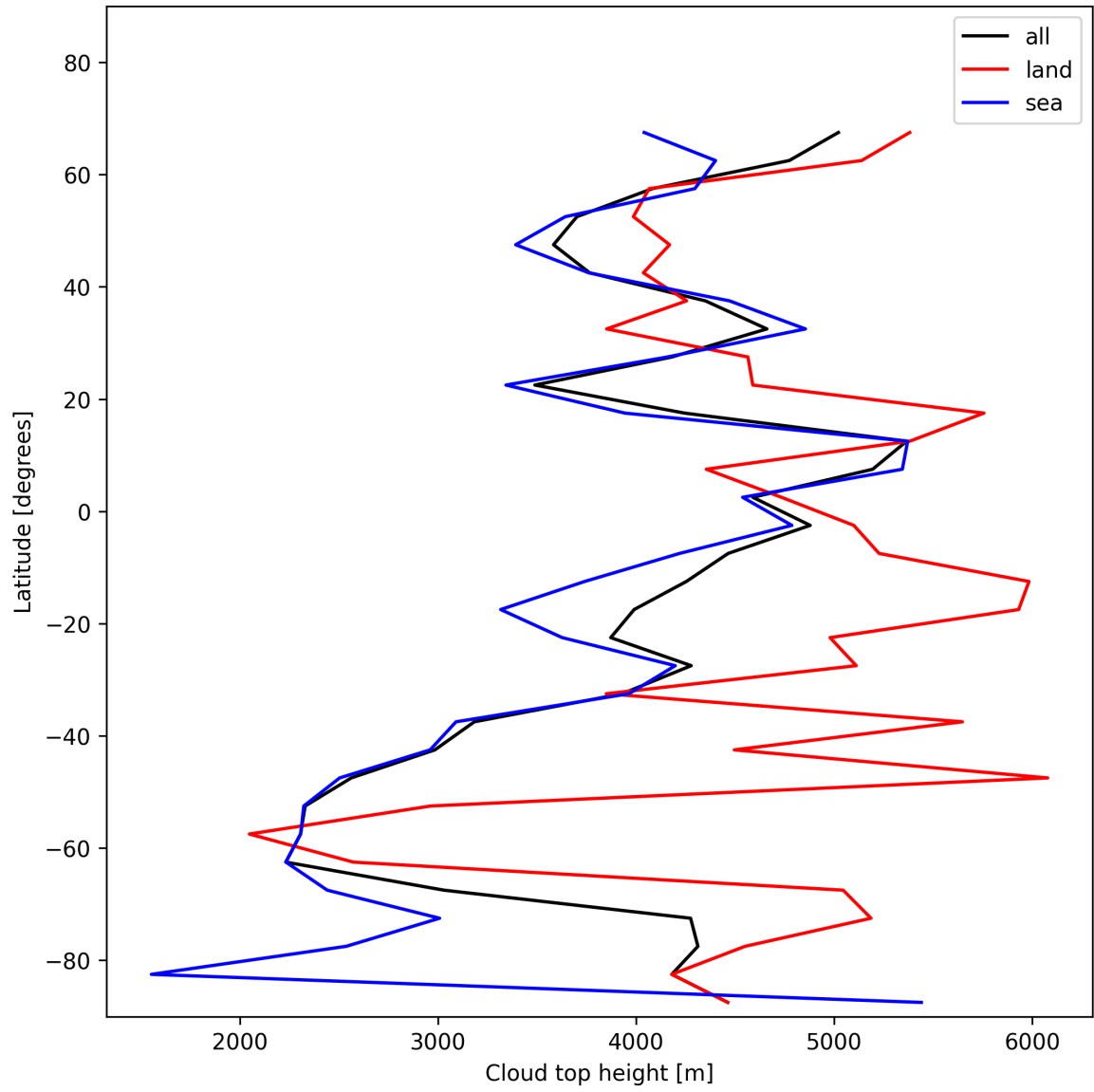
Figure 24: Zonal average of “Cloud top height” for 2025-11-25 to 2025-11-27.
