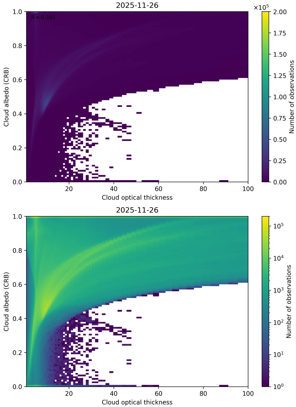
Figure 82: Scatter density plot of “Cloud optical thickness” against “Cloud albedo (CRB)” for 2025-11-25 to 2025-11-27.
