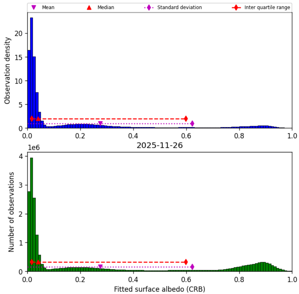
Figure 46: Histogram of “Fitted surface albedo (CRB)” for 2025-11-25 to 2025-11-27
