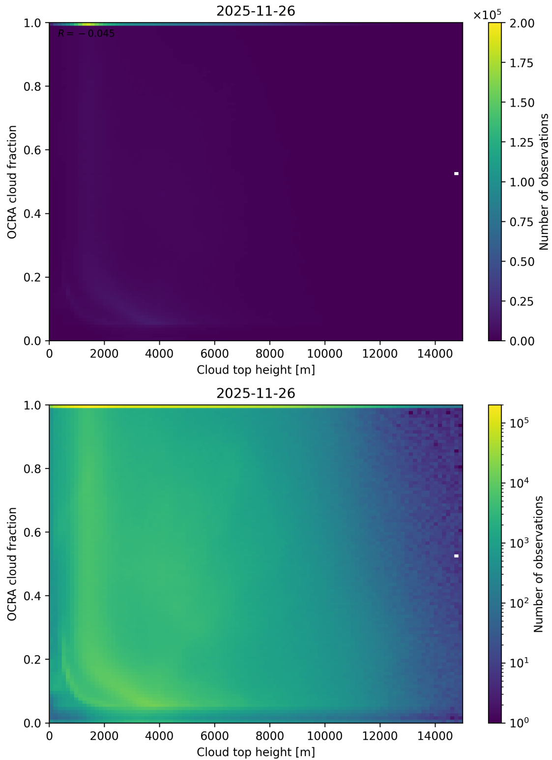
Figure 87: Scatter density plot of “Cloud top height” against “OCRA cloud fraction” for 2025-11-25 to 2025-11-27.
