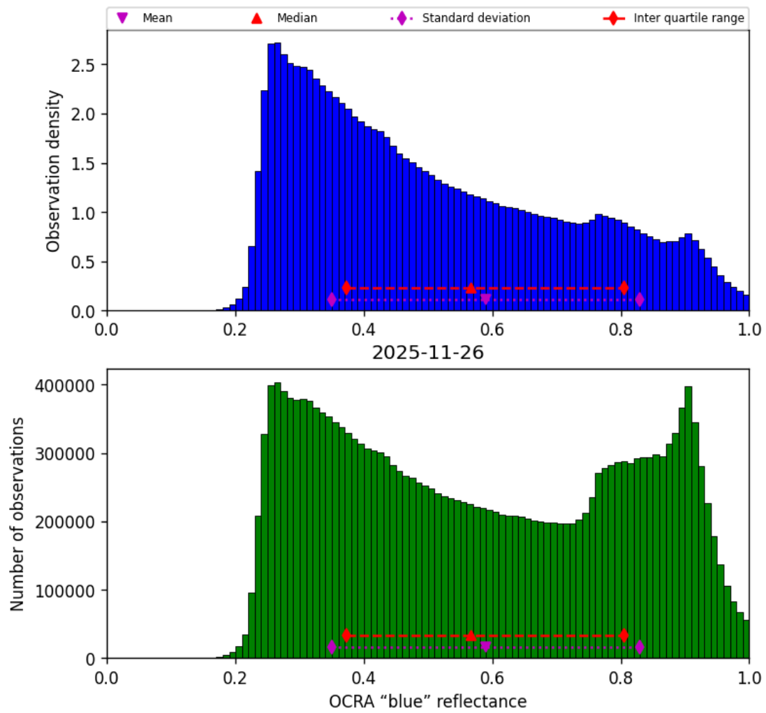
Figure 51: Histogram of “OCRA “blue” reflectance” for 2025-11-25 to 2025-11-27
