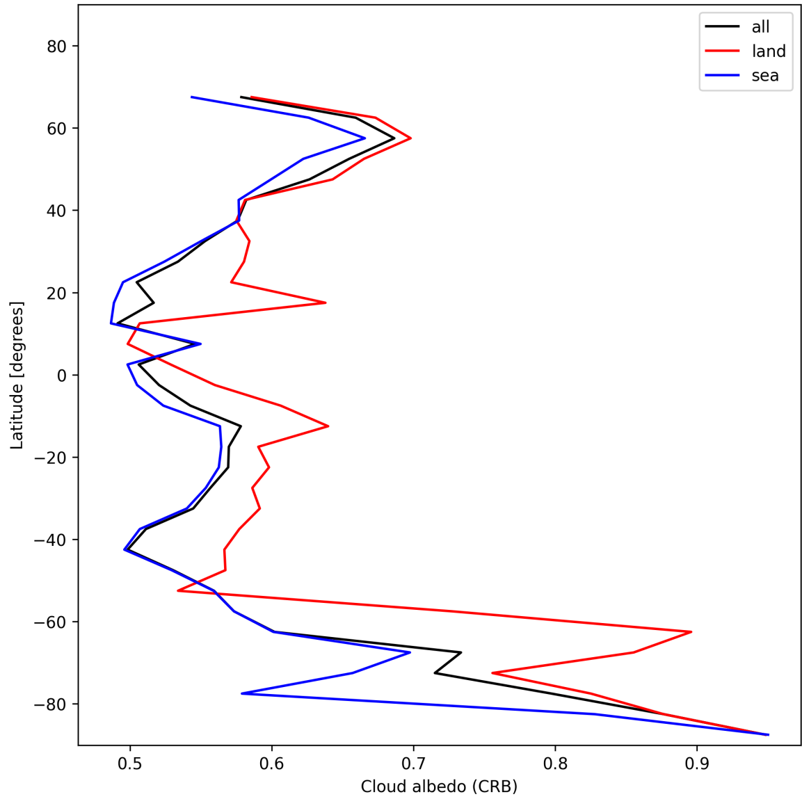
Figure 28: Zonal average of “Cloud albedo (CRB)” for 2025-11-25 to 2025-11-27.
