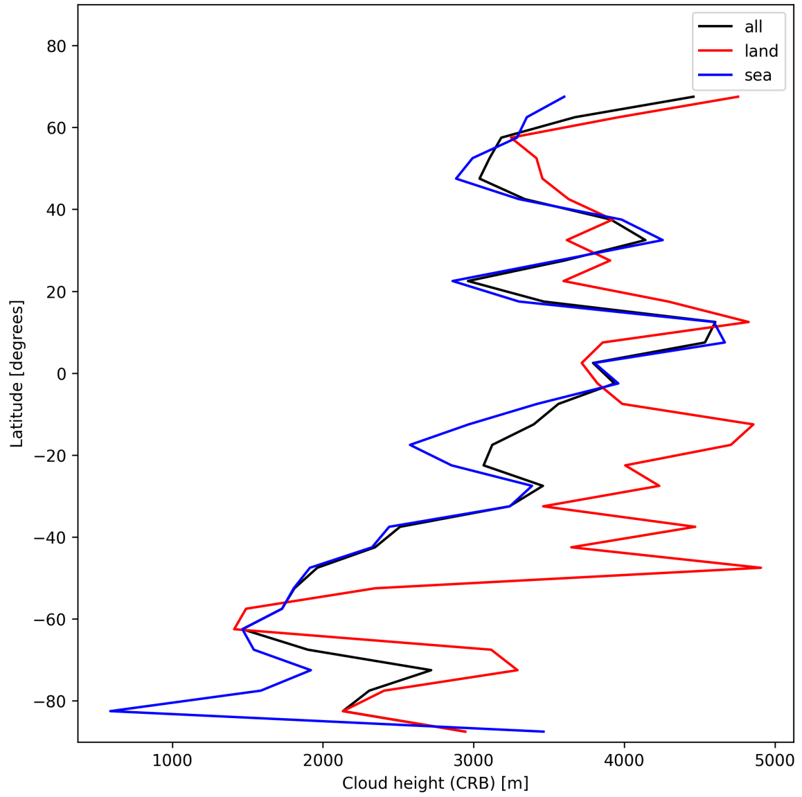
Figure 27: Zonal average of “Cloud height (CRB)” for 2025-11-25 to 2025-11-27.
