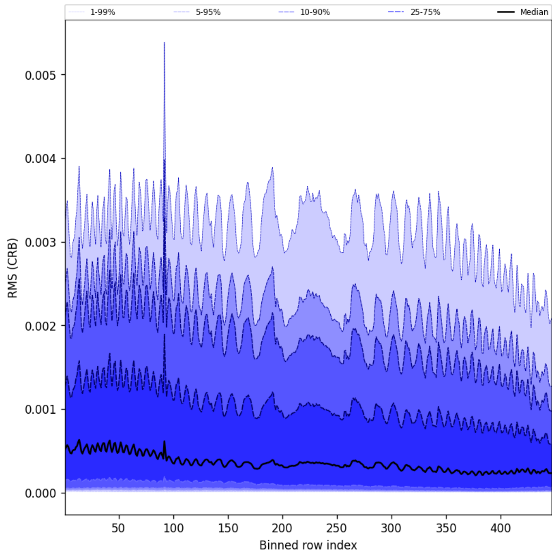
Figure 64: Along track statistics of “RMS (CRB)” for 2025-11-25 to 2025-11-27
