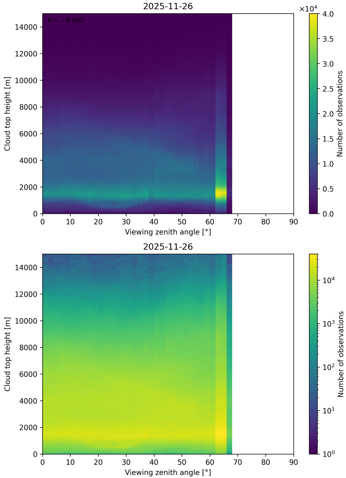
Figure 112: Scatter density plot of “Viewing zenith angle” against “Cloud top height” for 2025-11-25 to 2025-11-27.
