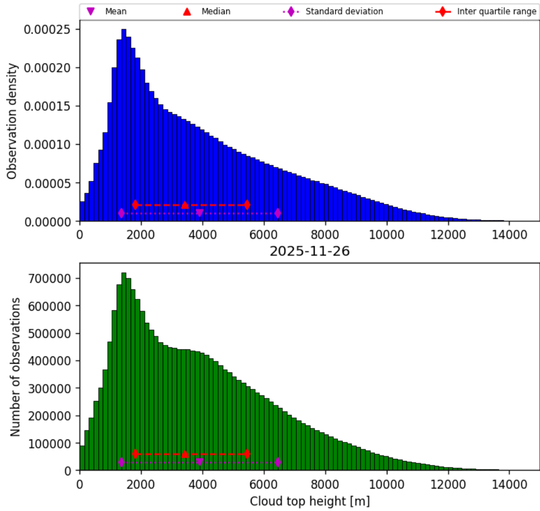
Figure 40: Histogram of “Cloud top height” for 2025-11-25 to 2025-11-27
