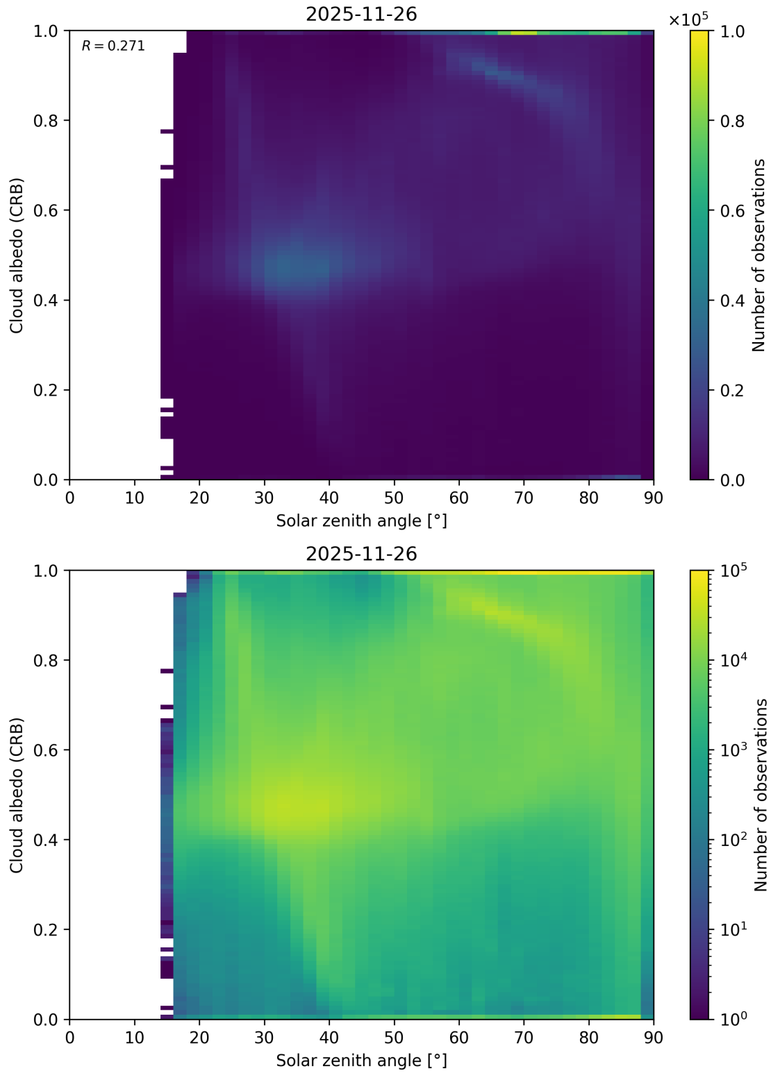
Figure 98: Scatter density plot of “Solar zenith angle” against “Cloud albedo (CRB)” for 2025-11-25 to 2025-11-27.
