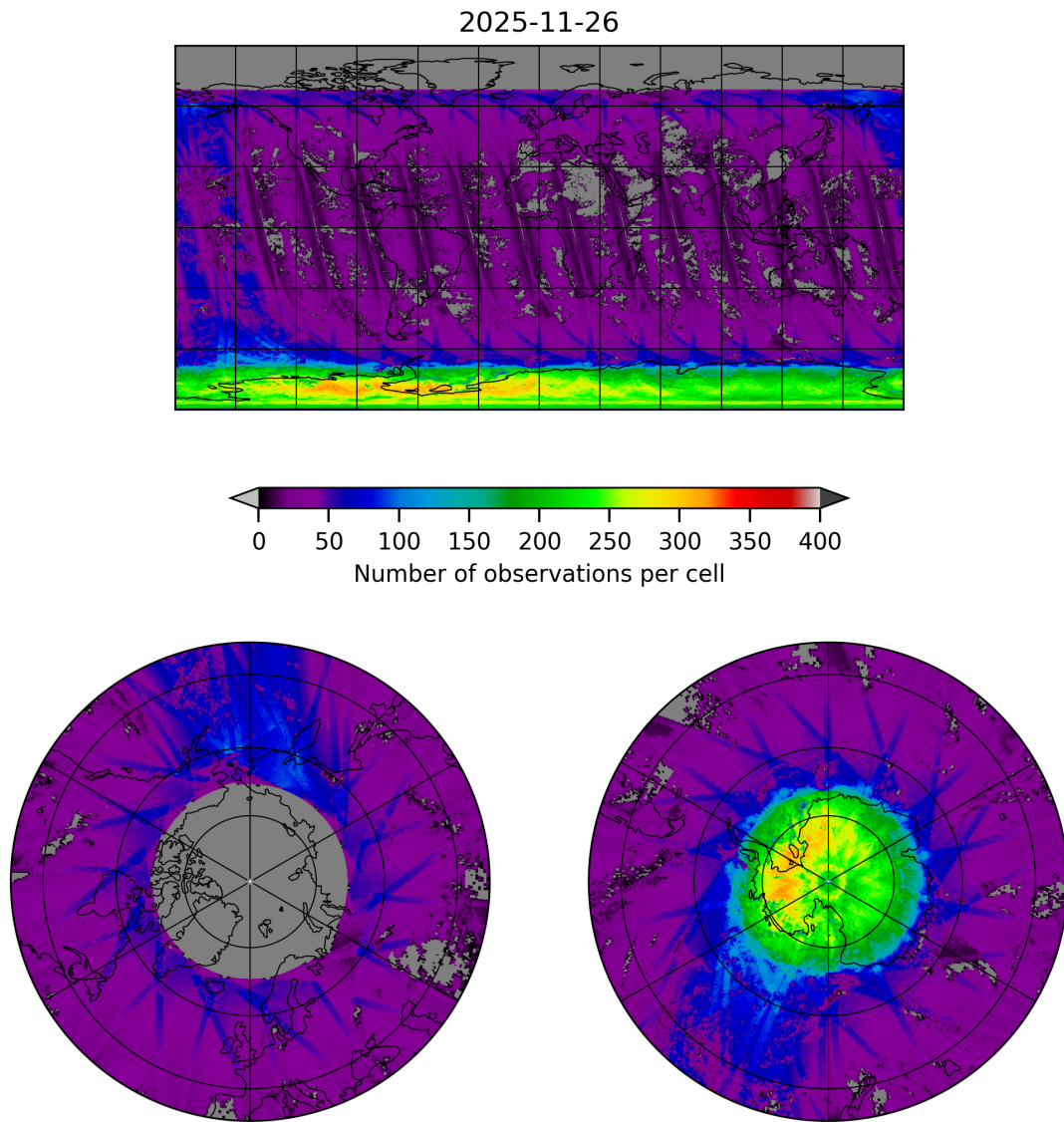
Figure 21: Map of the number of observations for 2025-11-25 to 2025-11-27
