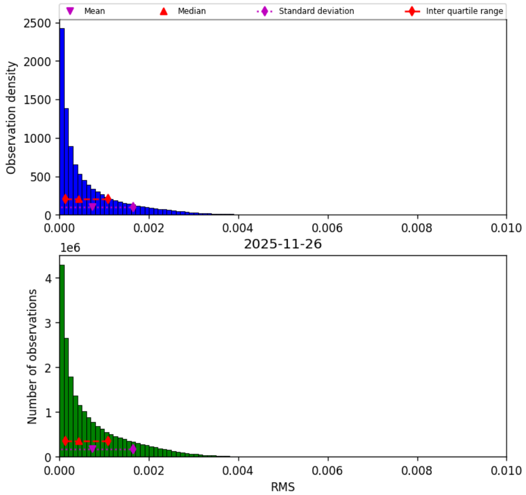
Figure 47: Histogram of “RMS” for 2025-11-25 to 2025-11-27
