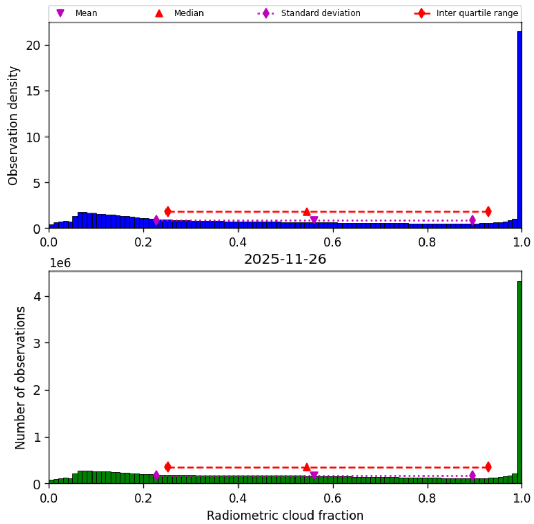
Figure 39: Histogram of “Radiometric cloud fraction” for 2025-11-25 to 2025-11-27
