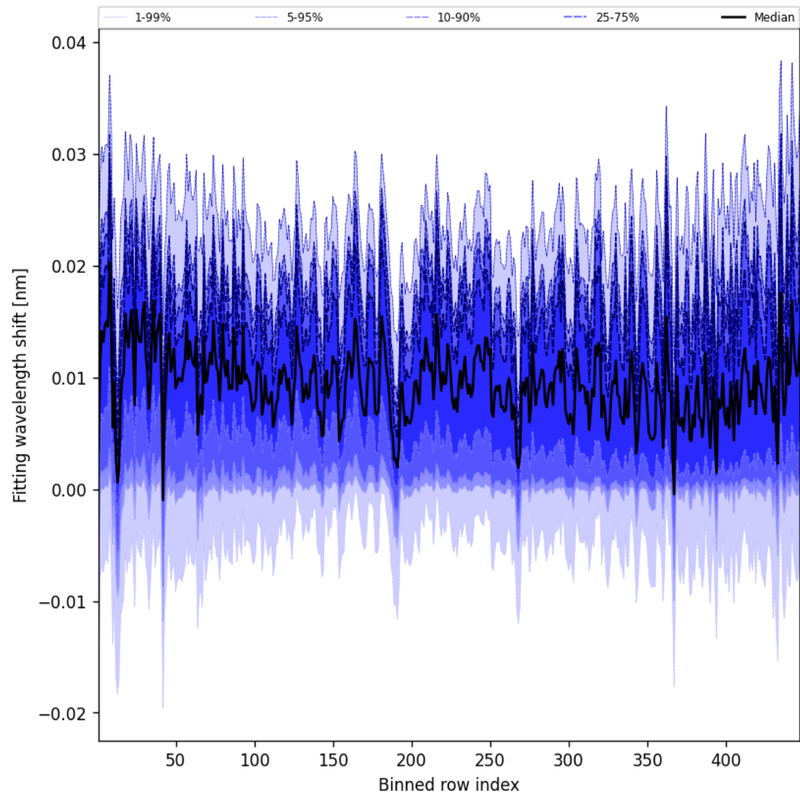
Figure 65: Along track statistics of “Fitting wavelength shift” for 2025-11-25 to 2025-11-27
