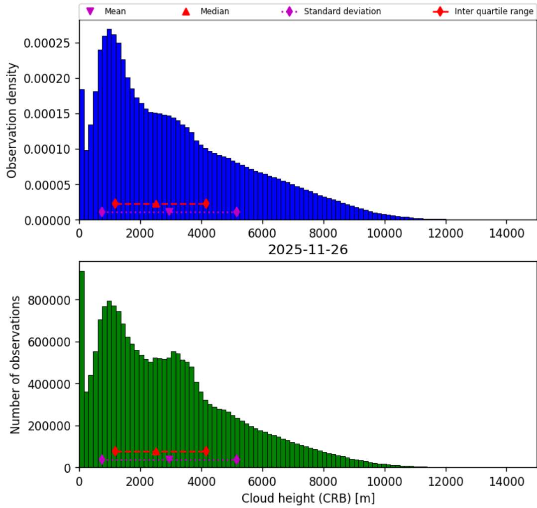
Figure 43: Histogram of “Cloud height (CRB)” for 2025-11-25 to 2025-11-27
