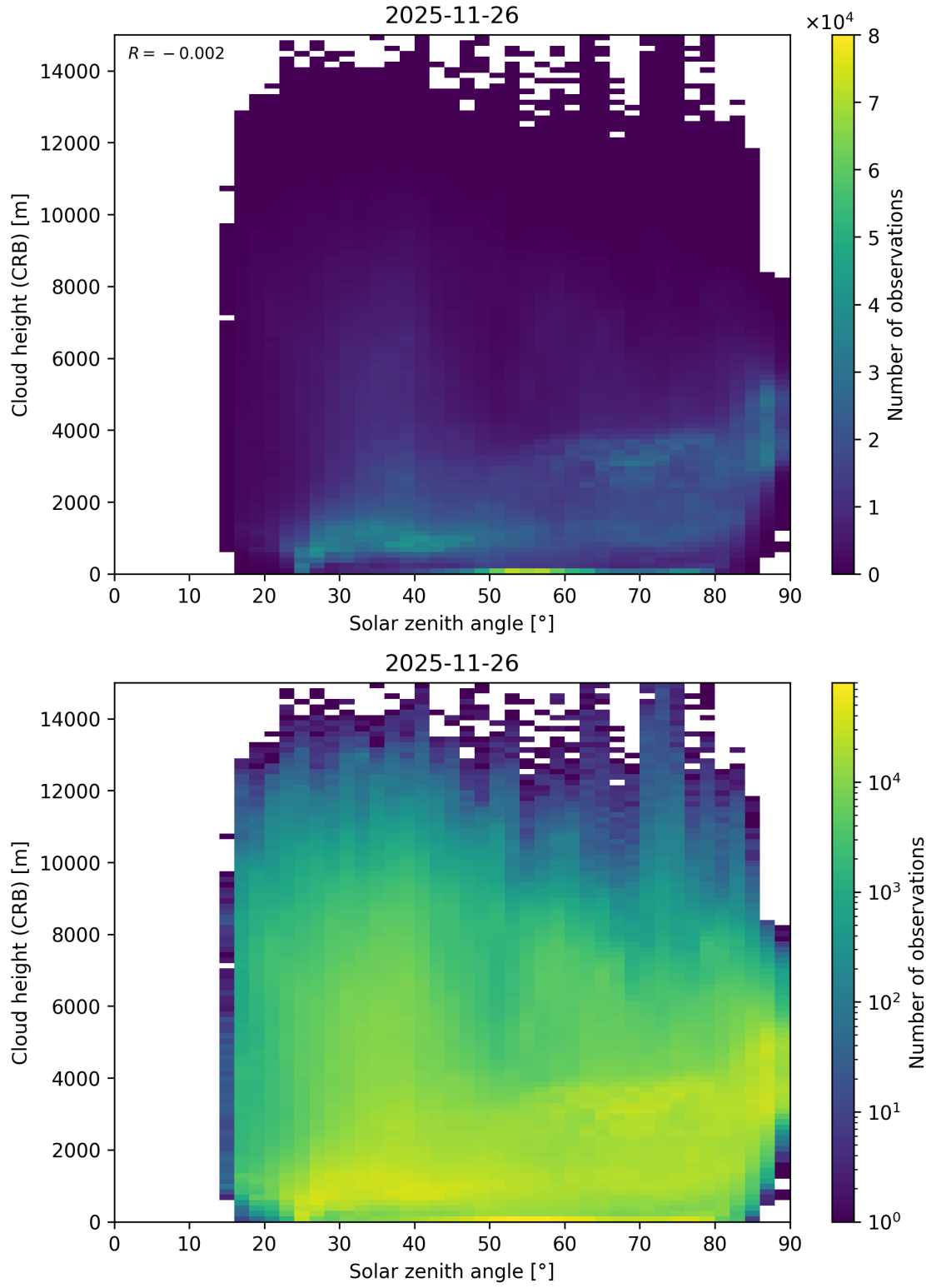
Figure 102: Scatter density plot of “Solar zenith angle” against “Cloud height (CRB)” for 2025-11-25 to 2025-11-27.
