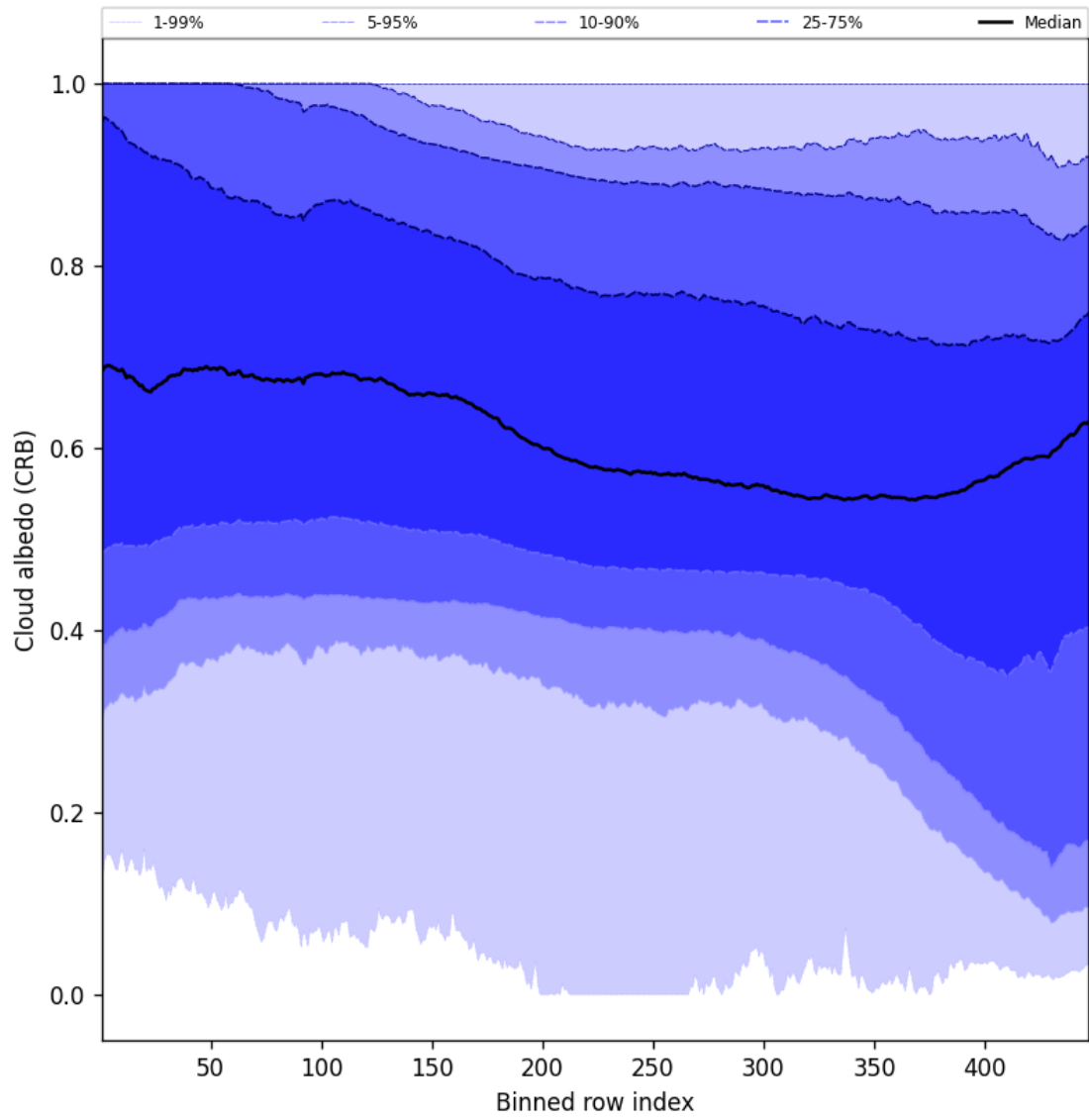
Figure 60: Along track statistics of “Cloud albedo (CRB)” for 2025-11-25 to 2025-11-27
