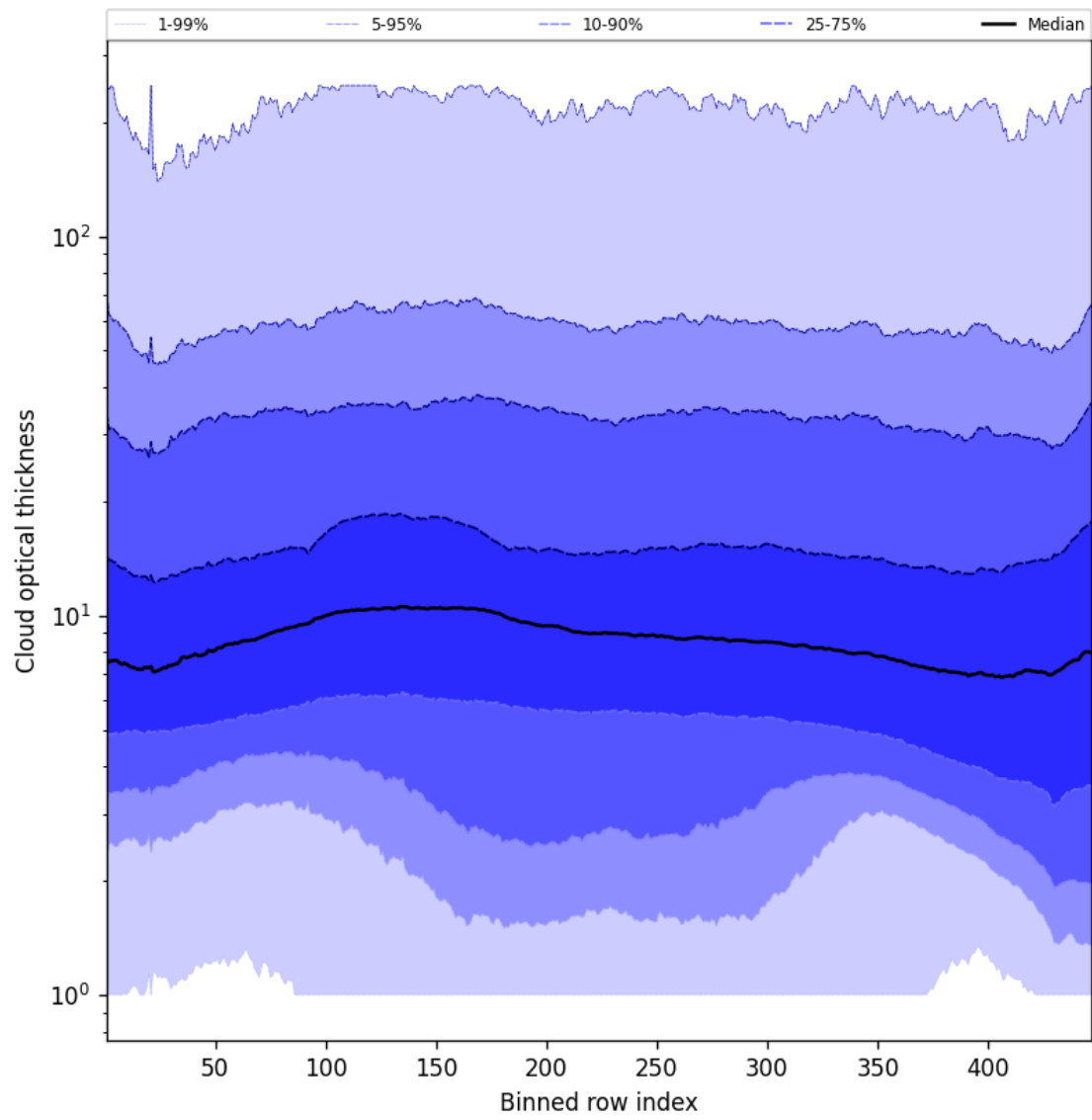
Figure 57: Along track statistics of “Cloud optical thickness” for 2025-11-25 to 2025-11-27
