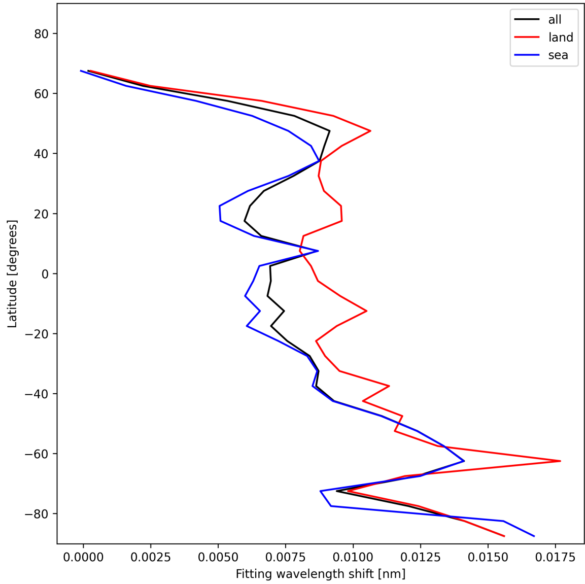
Figure 33: Zonal average of “Fitting wavelength shift” for 2025-11-25 to 2025-11-27.
