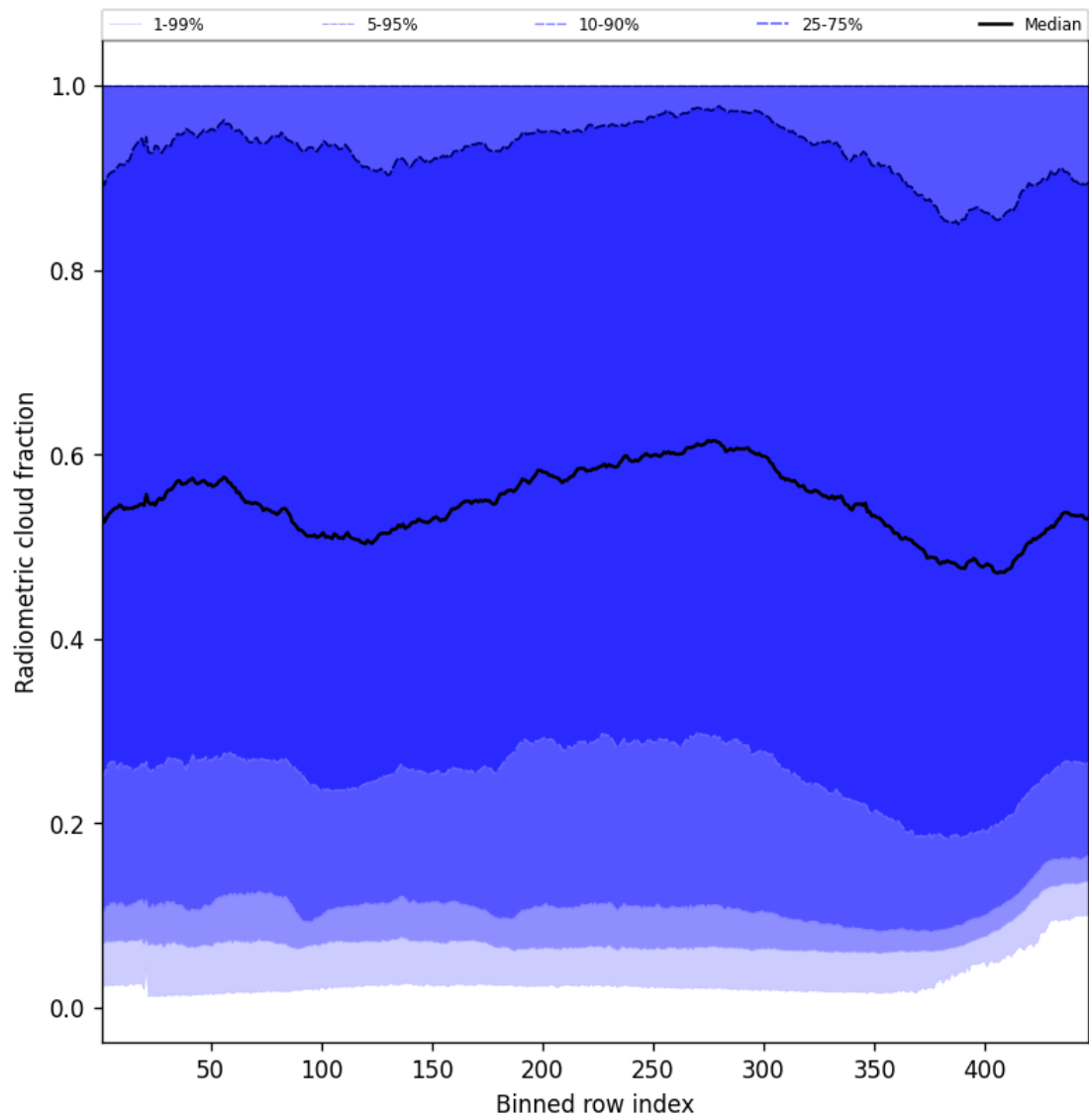
Figure 55: Along track statistics of “Radiometric cloud fraction” for 2025-11-25 to 2025-11-27
