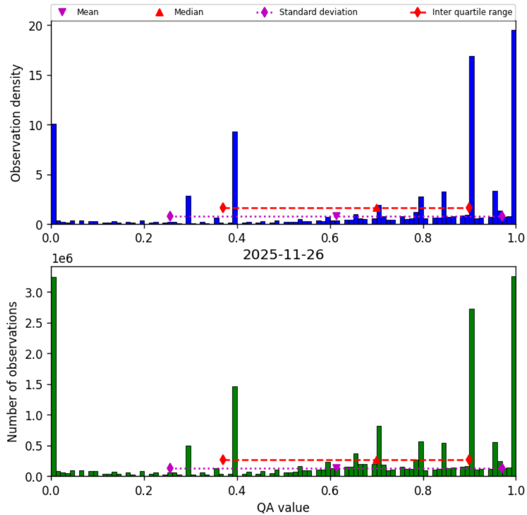
Figure 38: Histogram of “QA value” for 2025-11-25 to 2025-11-27
