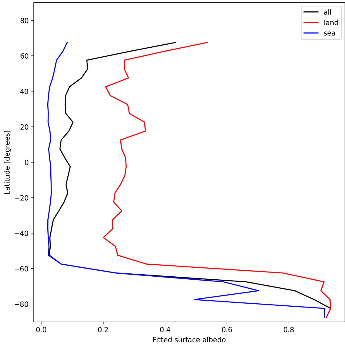
Figure 29: Zonal average of “Fitted surface albedo” for 2025-11-25 to 2025-11-27.
