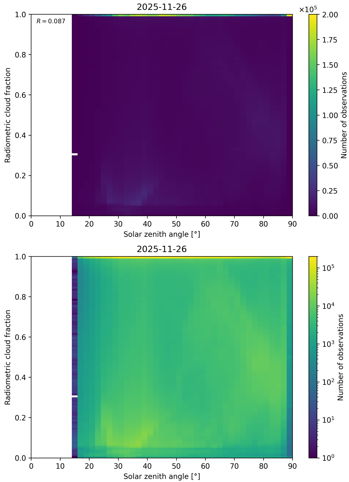
Figure 99: Scatter density plot of “Solar zenith angle” against “Radiometric cloud fraction” for 2025-11-25 to 2025-11-27.
