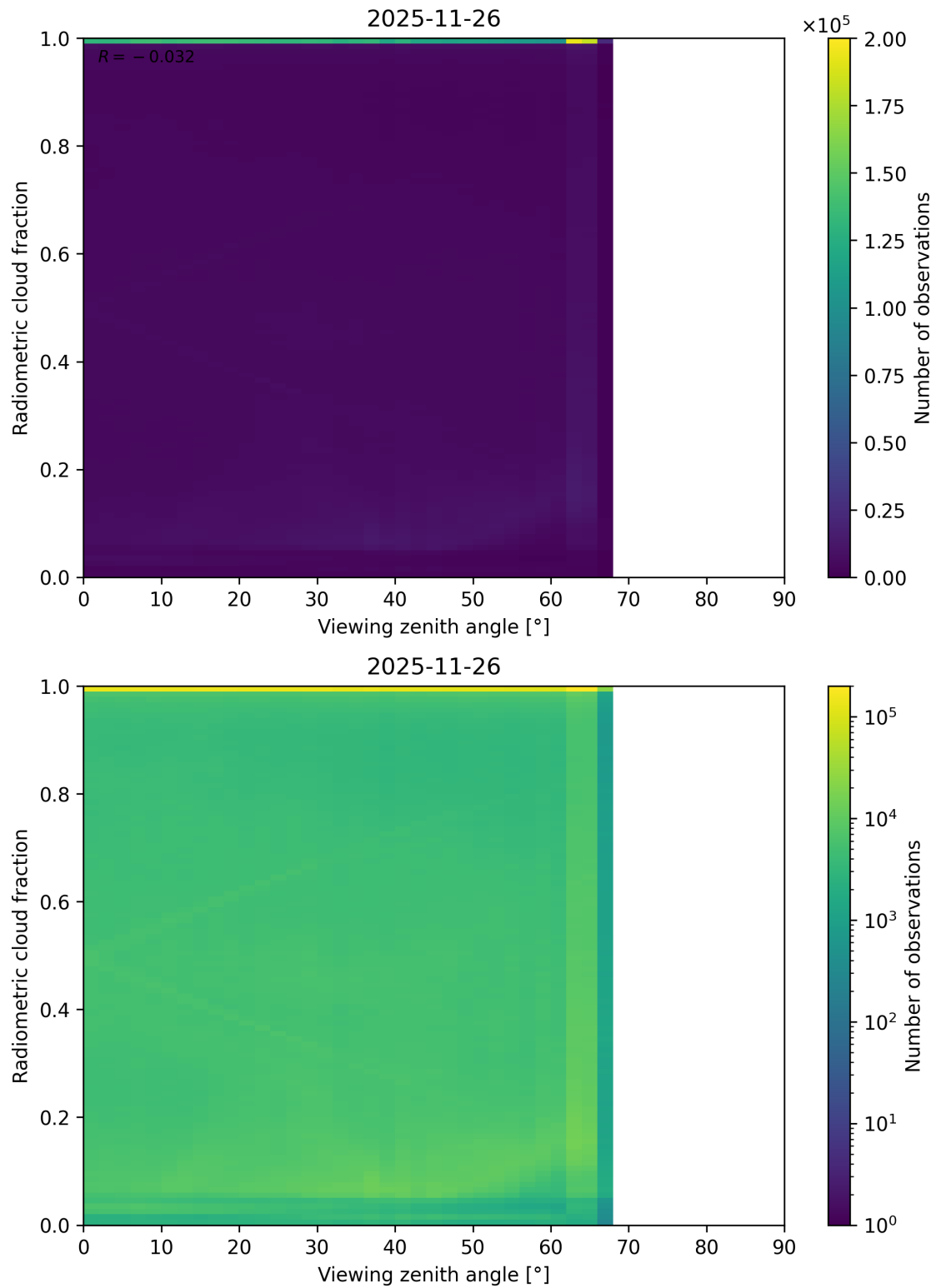
Figure 107: Scatter density plot of “Viewing zenith angle” against “Radiometric cloud fraction” for 2025-11-25 to 2025-11-27.
