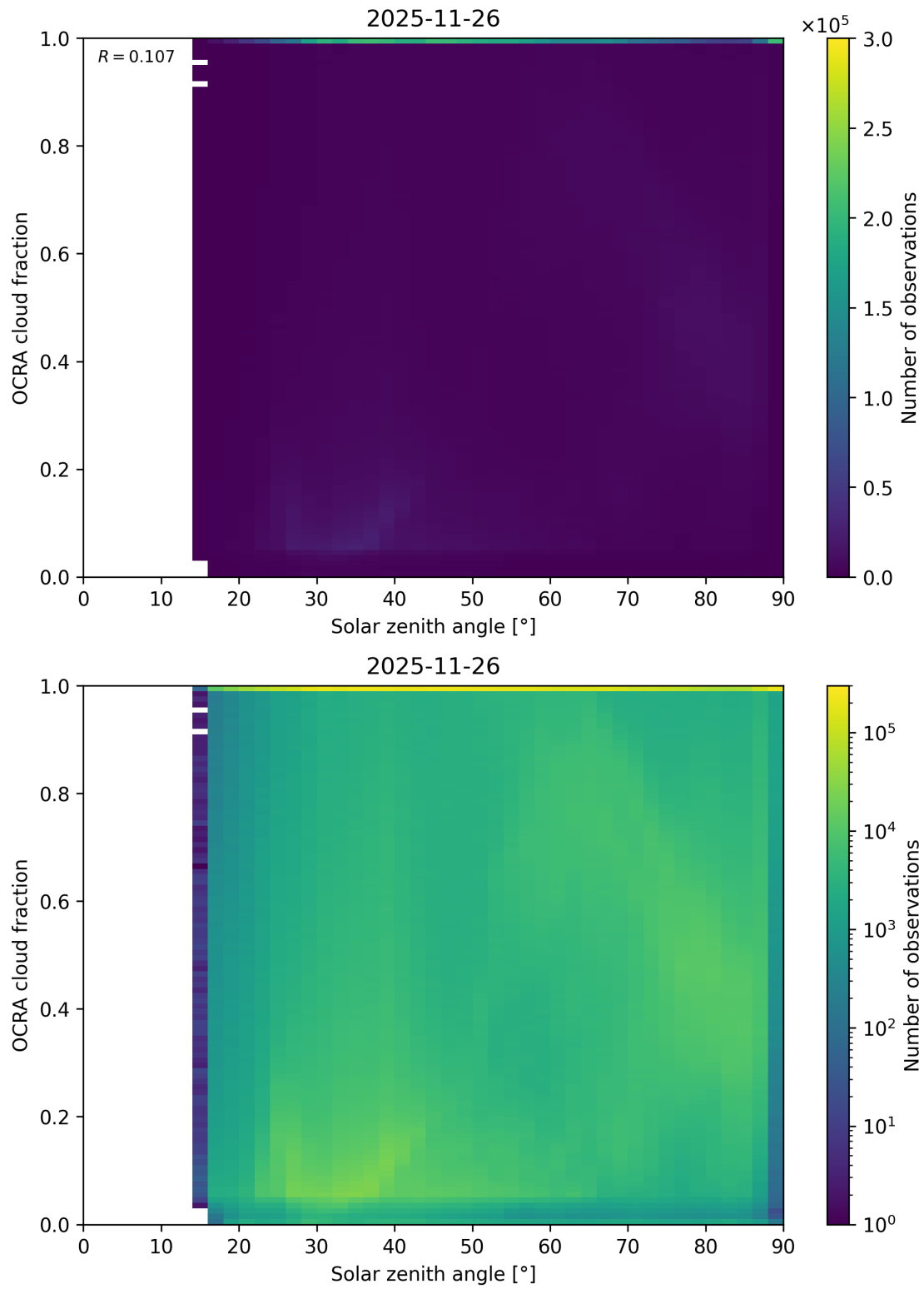
Figure 100: Scatter density plot of “Solar zenith angle” against “OCRA cloud fraction” for 2025-11-25 to 2025-11-27.
