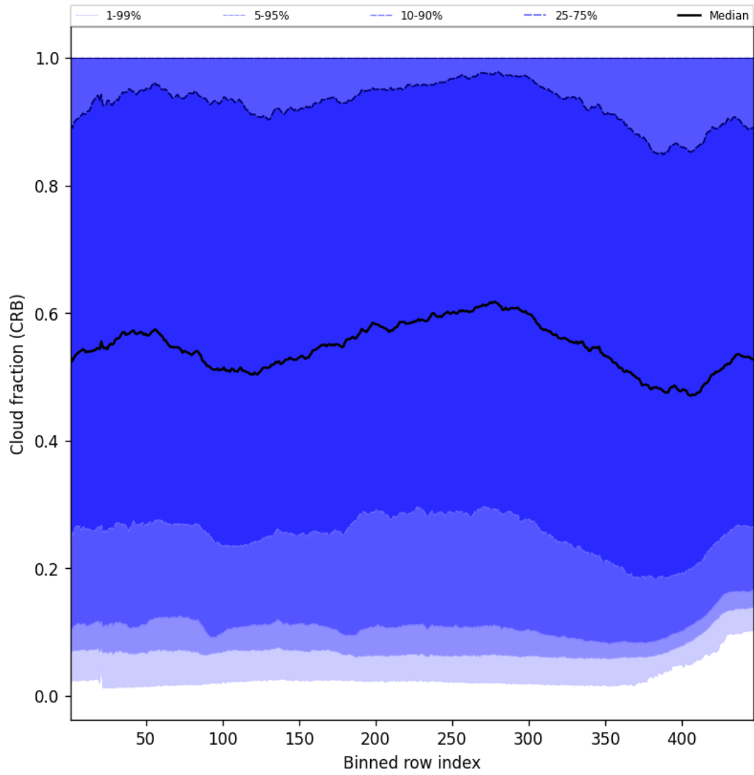
Figure 58: Along track statistics of “Cloud fraction (CRB)” for 2025-11-25 to 2025-11-27
