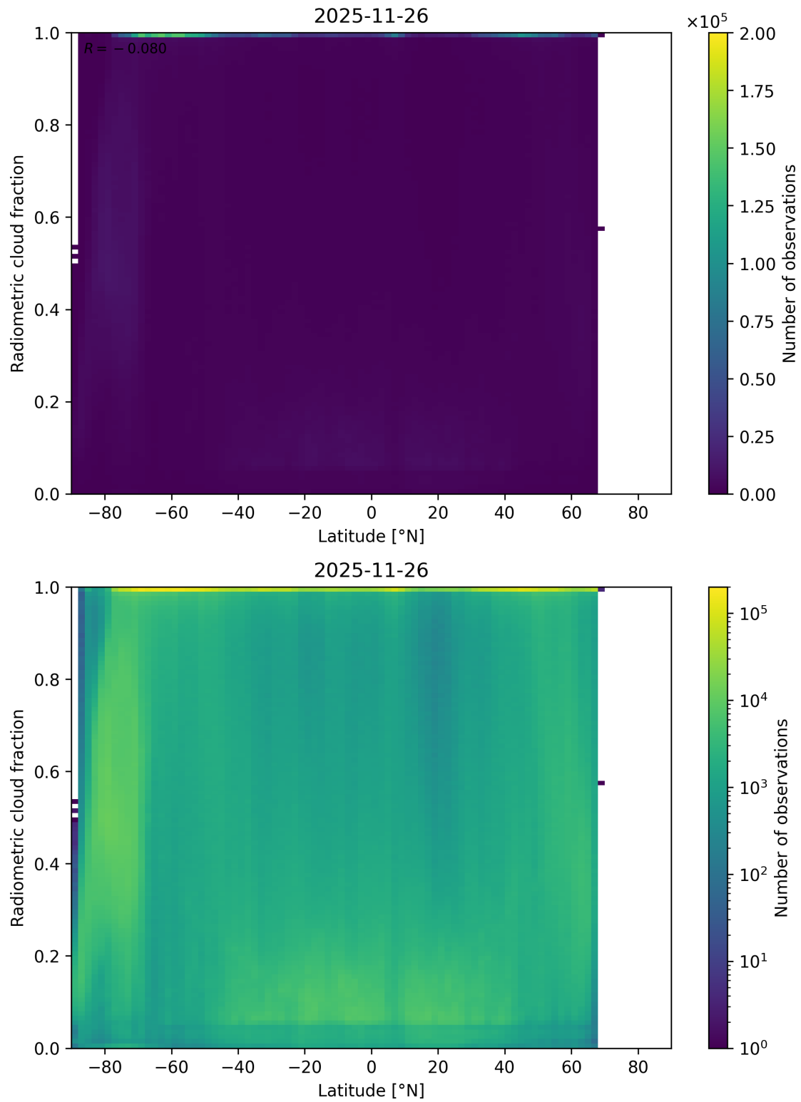
Figure 92: Scatter density plot of “Latitude” against “Radiometric cloud fraction” for 2025-11-25 to 2025-11-27.
