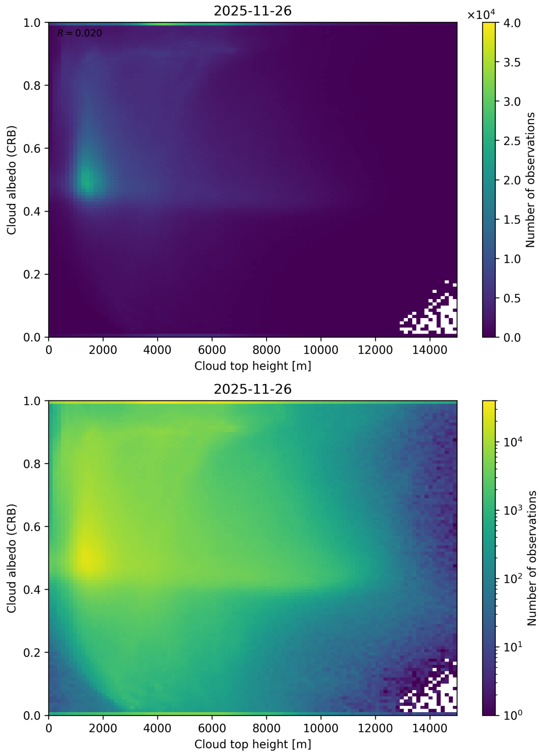
Figure 86: Scatter density plot of “Cloud top height” against “Cloud albedo (CRB)” for 2025-11-25 to 2025-11-27.
