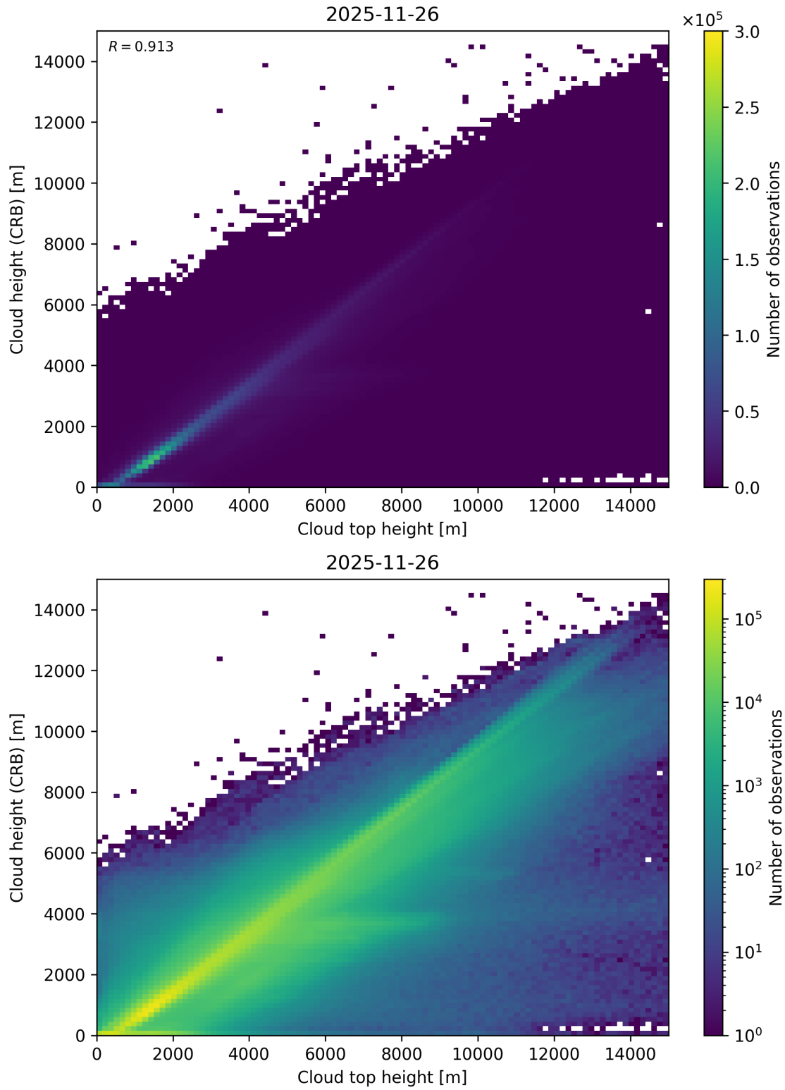
Figure 89: Scatter density plot of “Cloud top height” against “Cloud height (CRB)” for 2025-11-25 to 2025-11-27.
