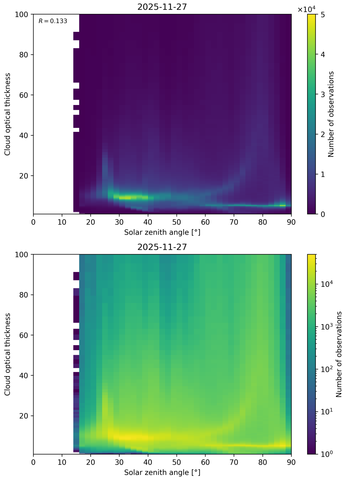
Figure 103: Scatter density plot of “Solar zenith angle” against “Cloud optical thickness” for 2025-11-26 to 2025-11-28.
