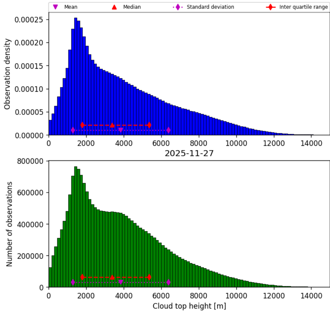
Figure 40: Histogram of “Cloud top height” for 2025-11-26 to 2025-11-28
