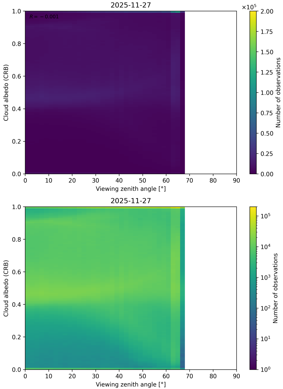
Figure 106: Scatter density plot of “Viewing zenith angle” against “Cloud albedo (CRB)” for 2025-11-26 to 2025-11-28.
