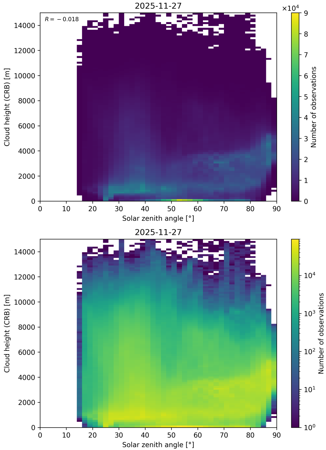
Figure 102: Scatter density plot of “Solar zenith angle” against “Cloud height (CRB)” for 2025-11-26 to 2025-11-28.
