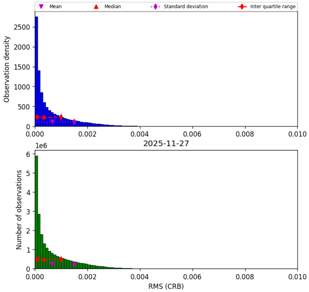
Figure 48: Histogram of “RMS (CRB)” for 2025-11-26 to 2025-11-28
