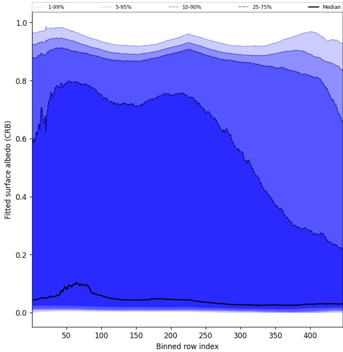
Figure 62: Along track statistics of “Fitted surface albedo (CRB)” for 2025-11-26 to 2025-11-28
