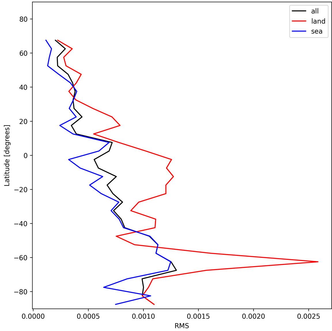
Figure 31: Zonal average of “RMS” for 2025-11-26 to 2025-11-28.
