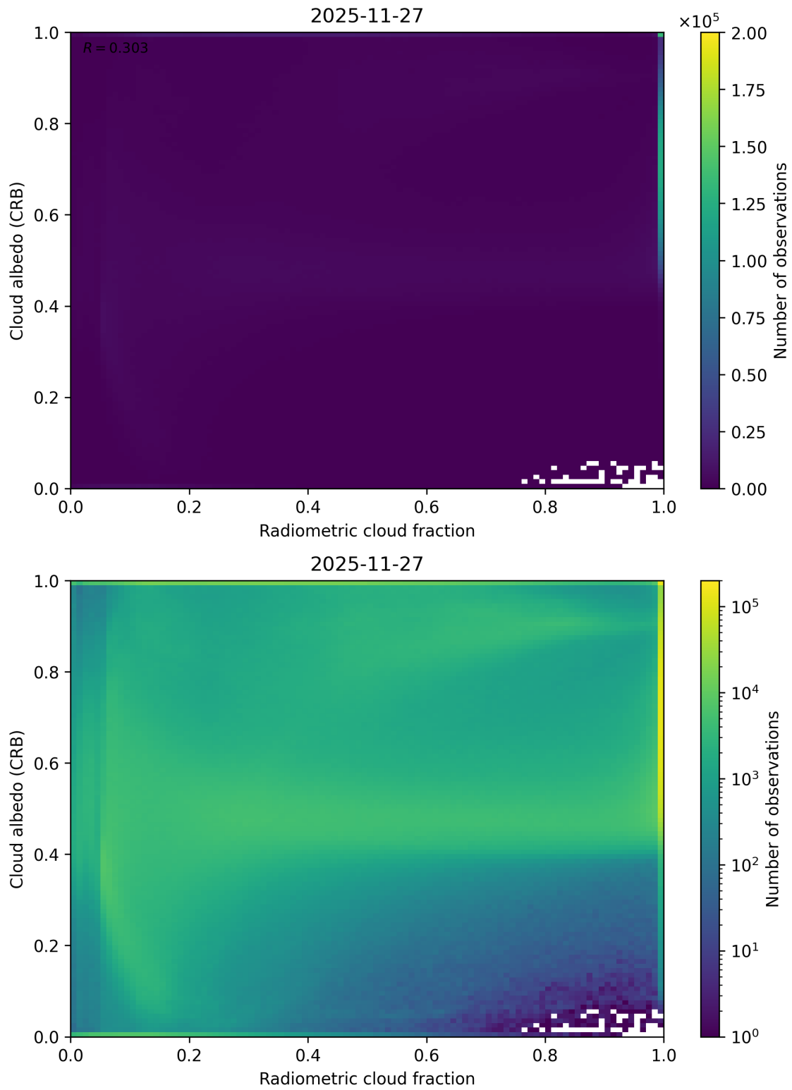
Figure 71: Scatter density plot of “Radiometric cloud fraction” against “Cloud albedo (CRB)” for 2025-11-26 to 2025-11-28.
