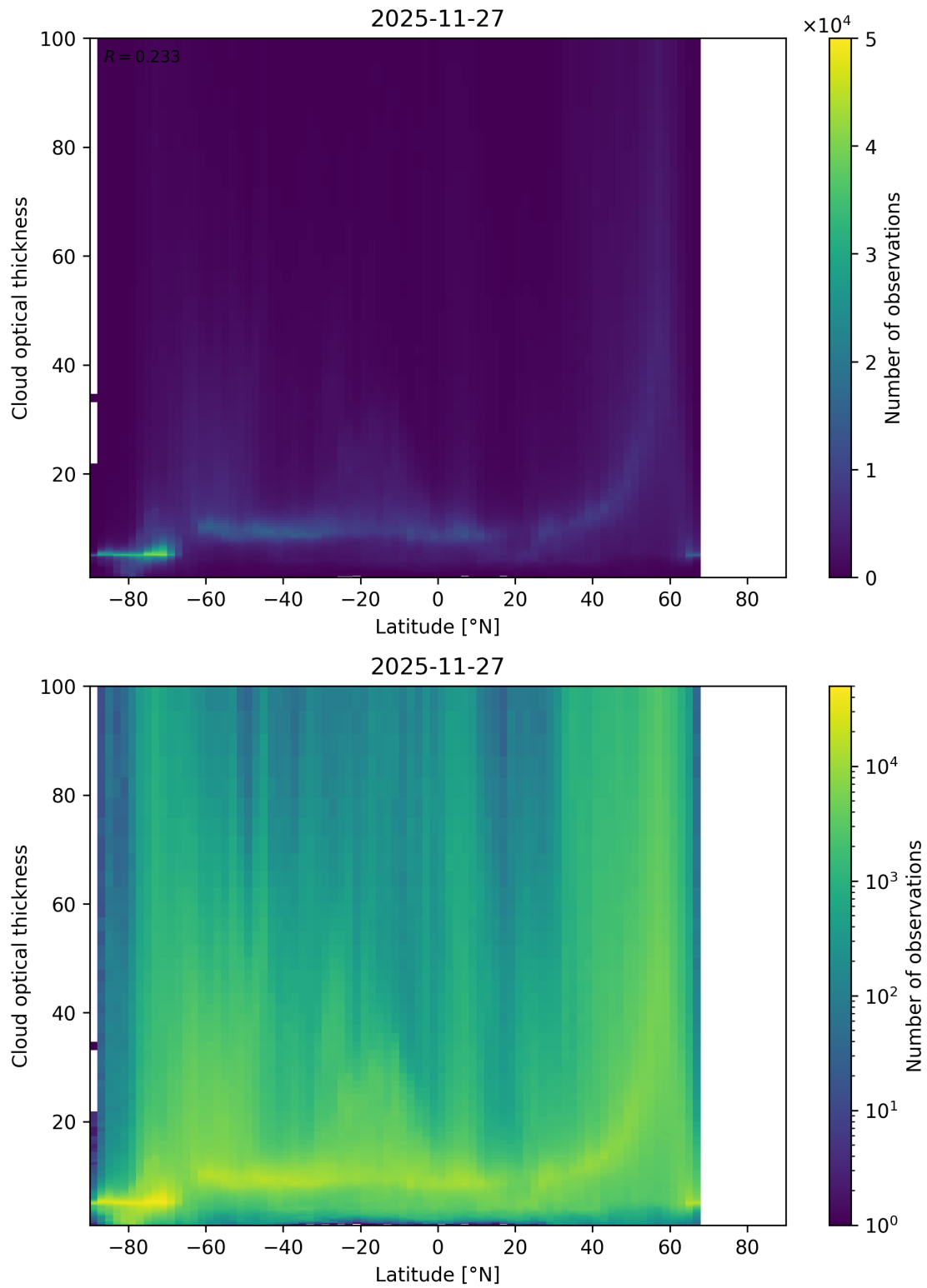
Figure 96: Scatter density plot of “Latitude” against “Cloud optical thickness” for 2025-11-26 to 2025-11-28.
