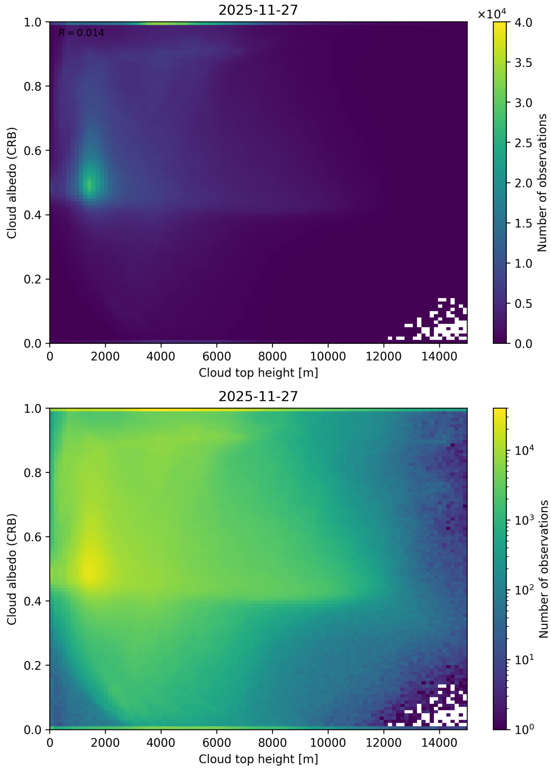
Figure 86: Scatter density plot of “Cloud top height” against “Cloud albedo (CRB)” for 2025-11-26 to 2025-11-28.
