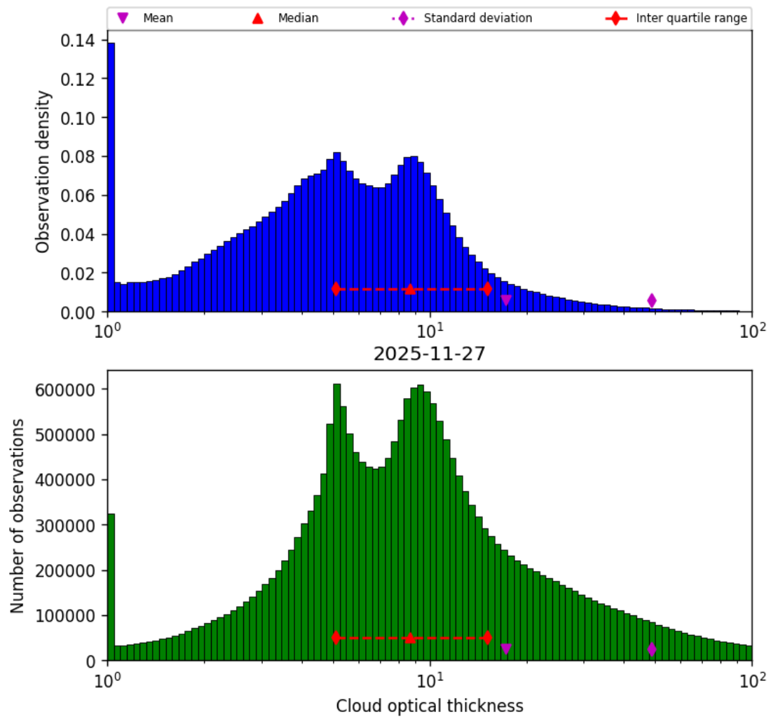
Figure 41: Histogram of “Cloud optical thickness” for 2025-11-26 to 2025-11-28
