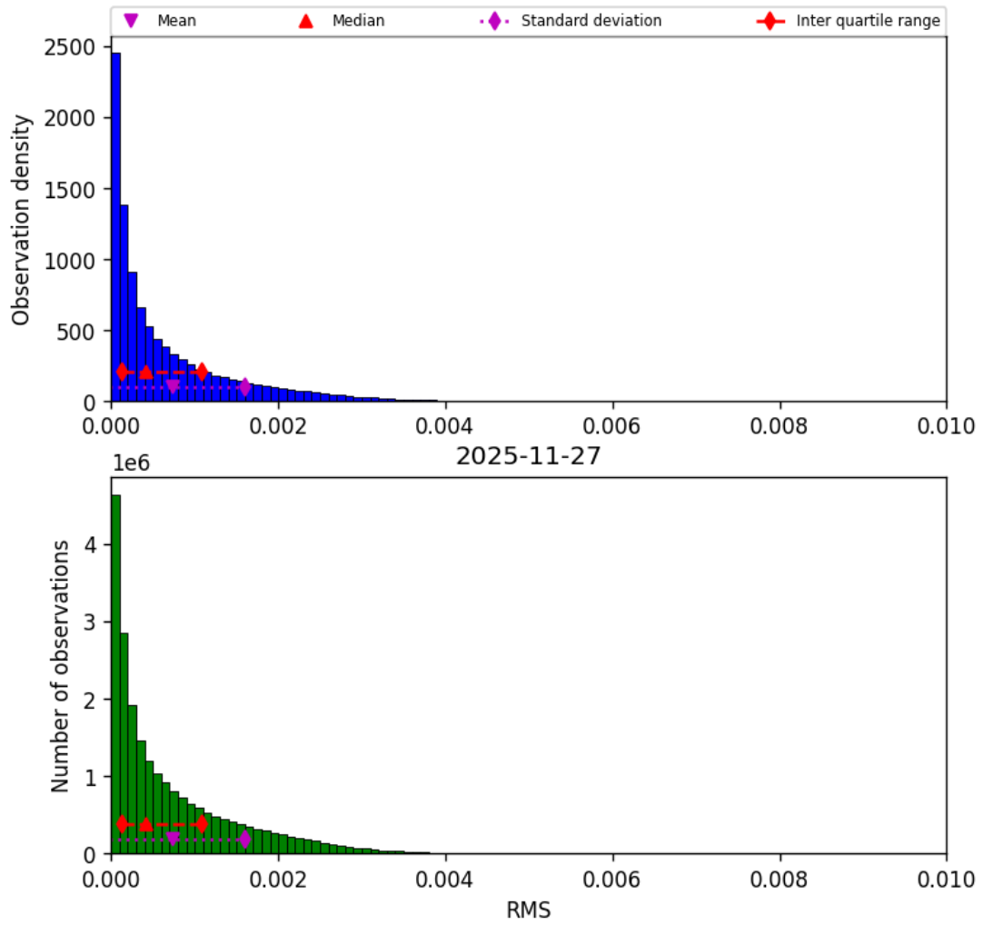
Figure 47: Histogram of “RMS” for 2025-11-26 to 2025-11-28
