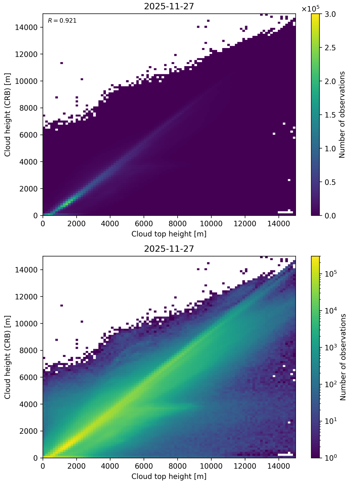
Figure 89: Scatter density plot of “Cloud top height” against “Cloud height (CRB)” for 2025-11-26 to 2025-11-28.
