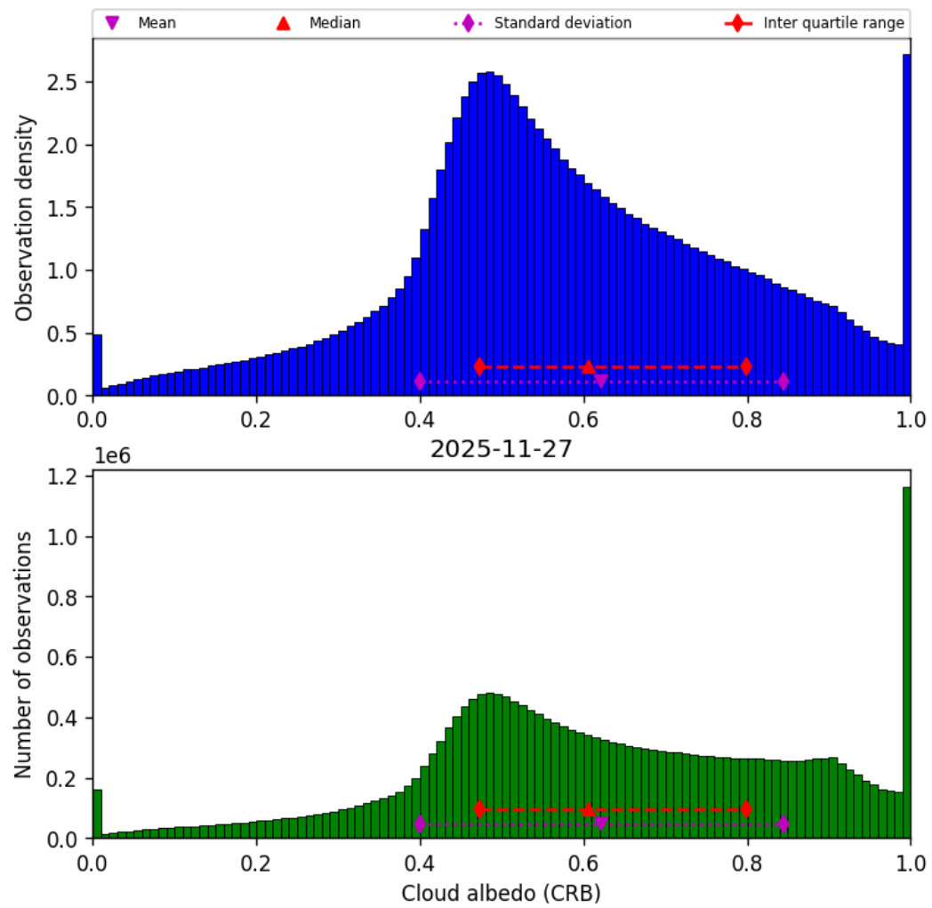
Figure 44: Histogram of “Cloud albedo (CRB)” for 2025-11-26 to 2025-11-28
