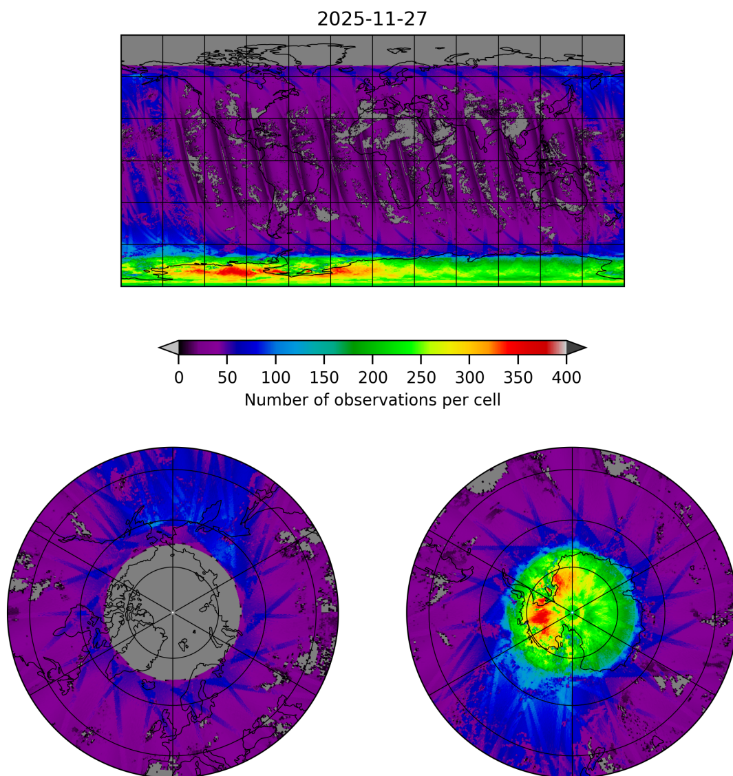
Figure 21: Map of the number of observations for 2025-11-26 to 2025-11-28
