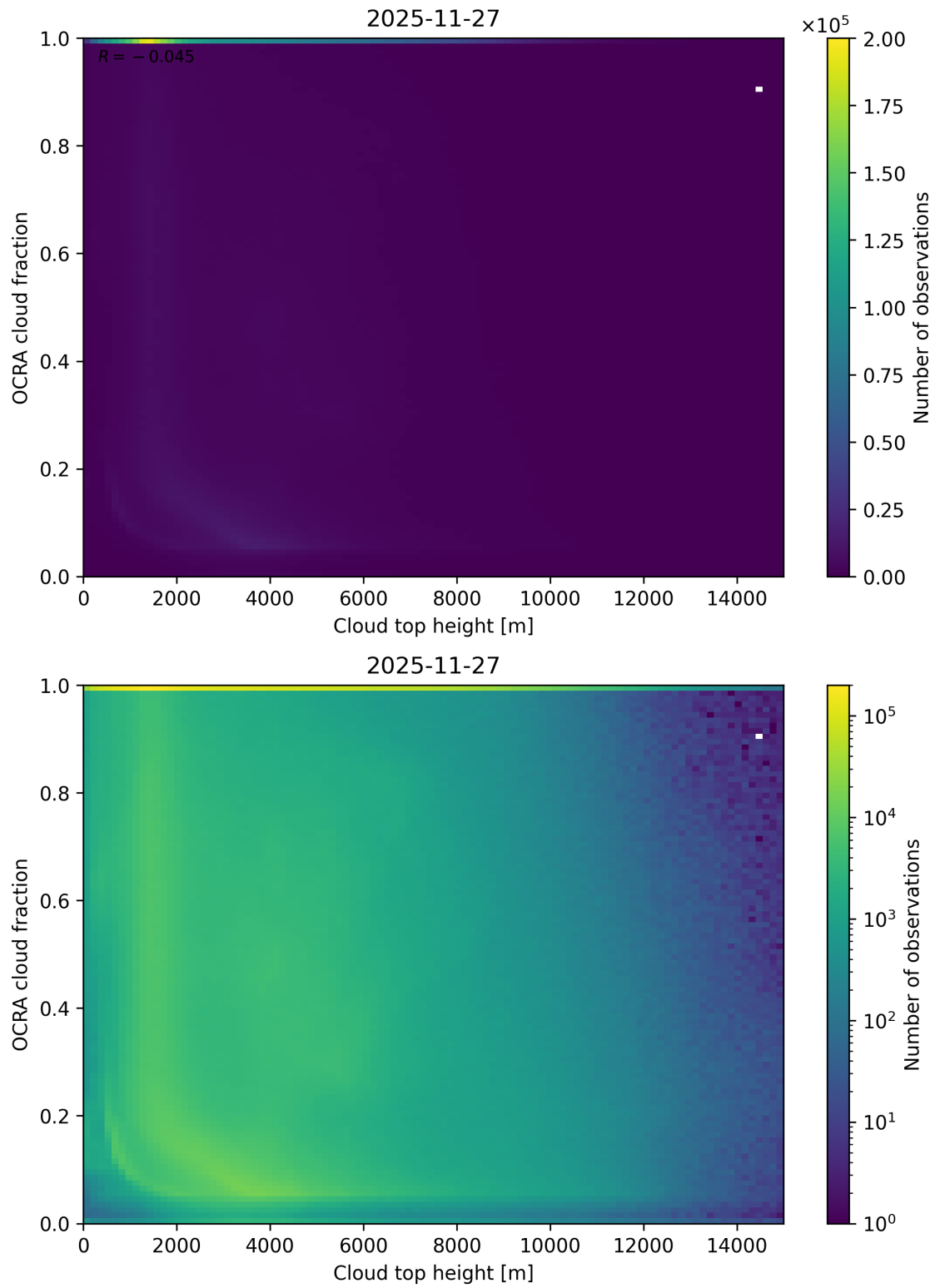
Figure 87: Scatter density plot of “Cloud top height” against “OCRA cloud fraction” for 2025-11-26 to 2025-11-28.
