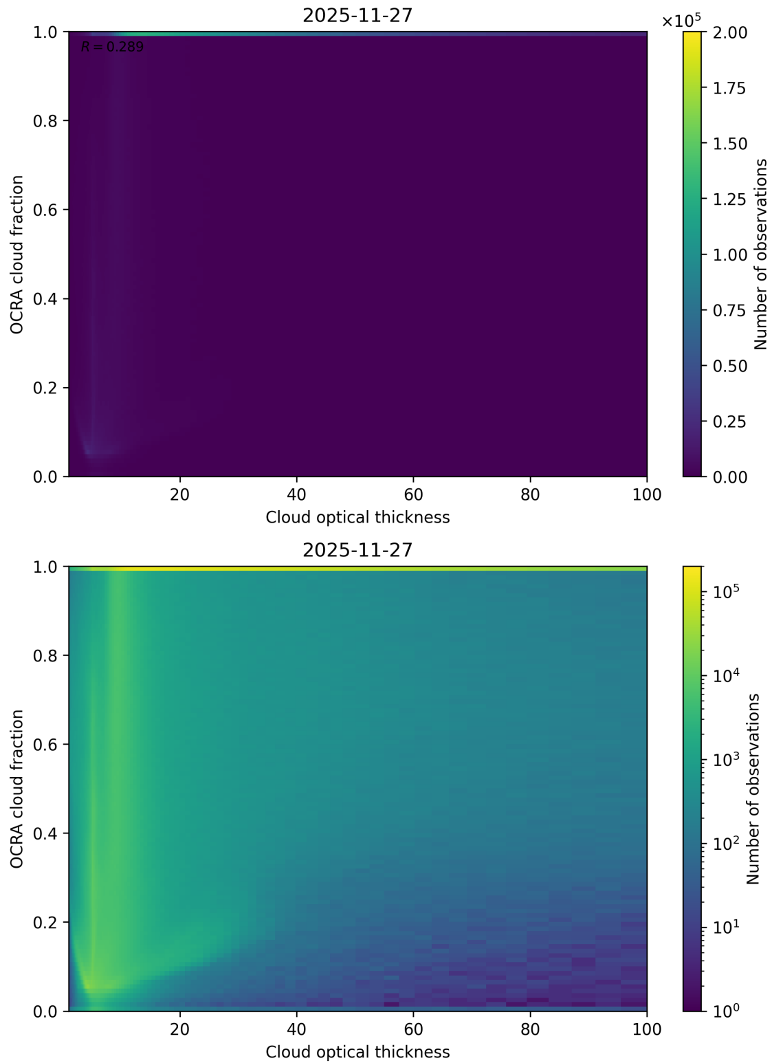
Figure 83: Scatter density plot of “Cloud optical thickness” against “OCRA cloud fraction” for 2025-11-26 to 2025-11-28.
