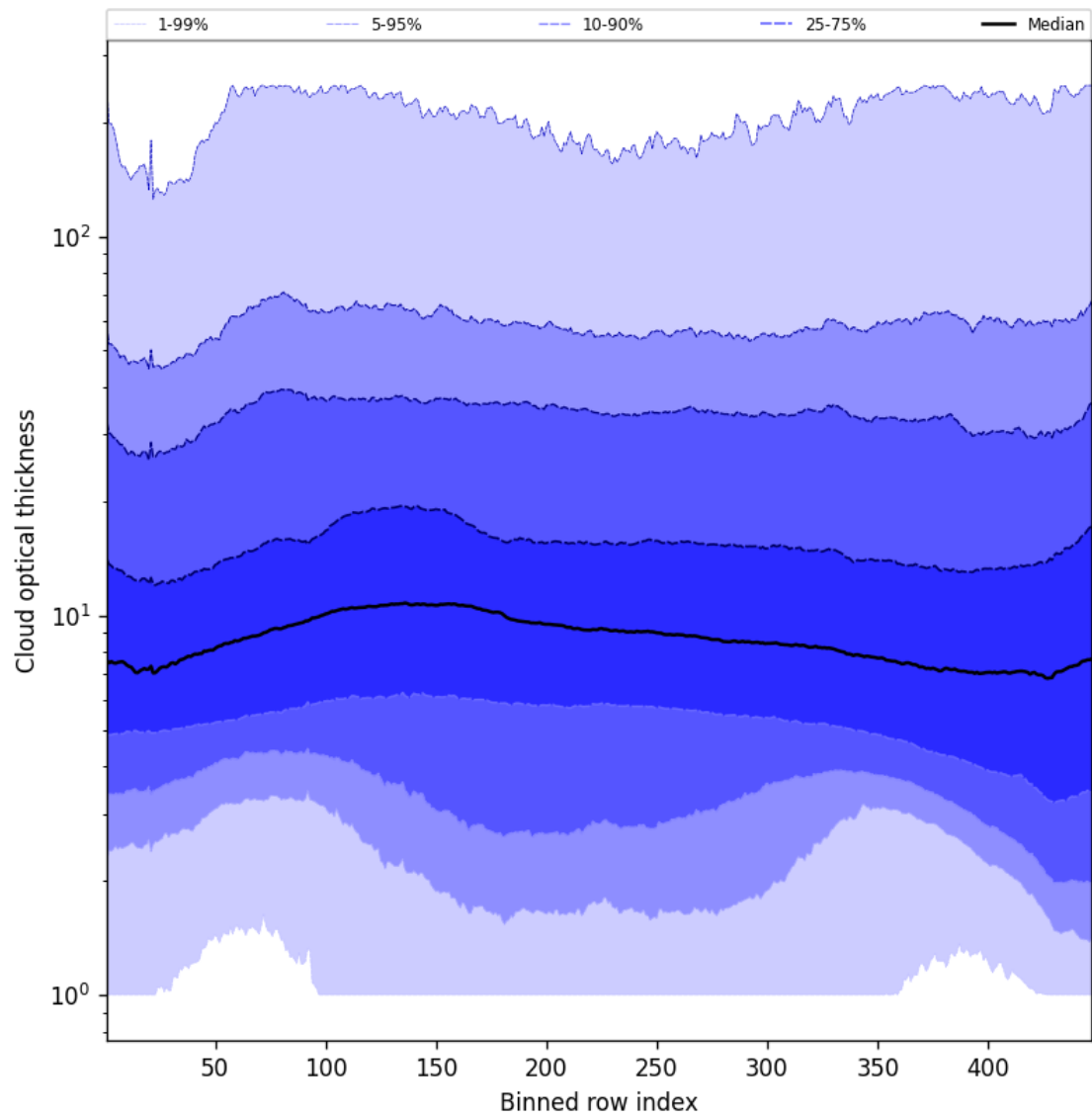
Figure 57: Along track statistics of “Cloud optical thickness” for 2025-11-26 to 2025-11-28
