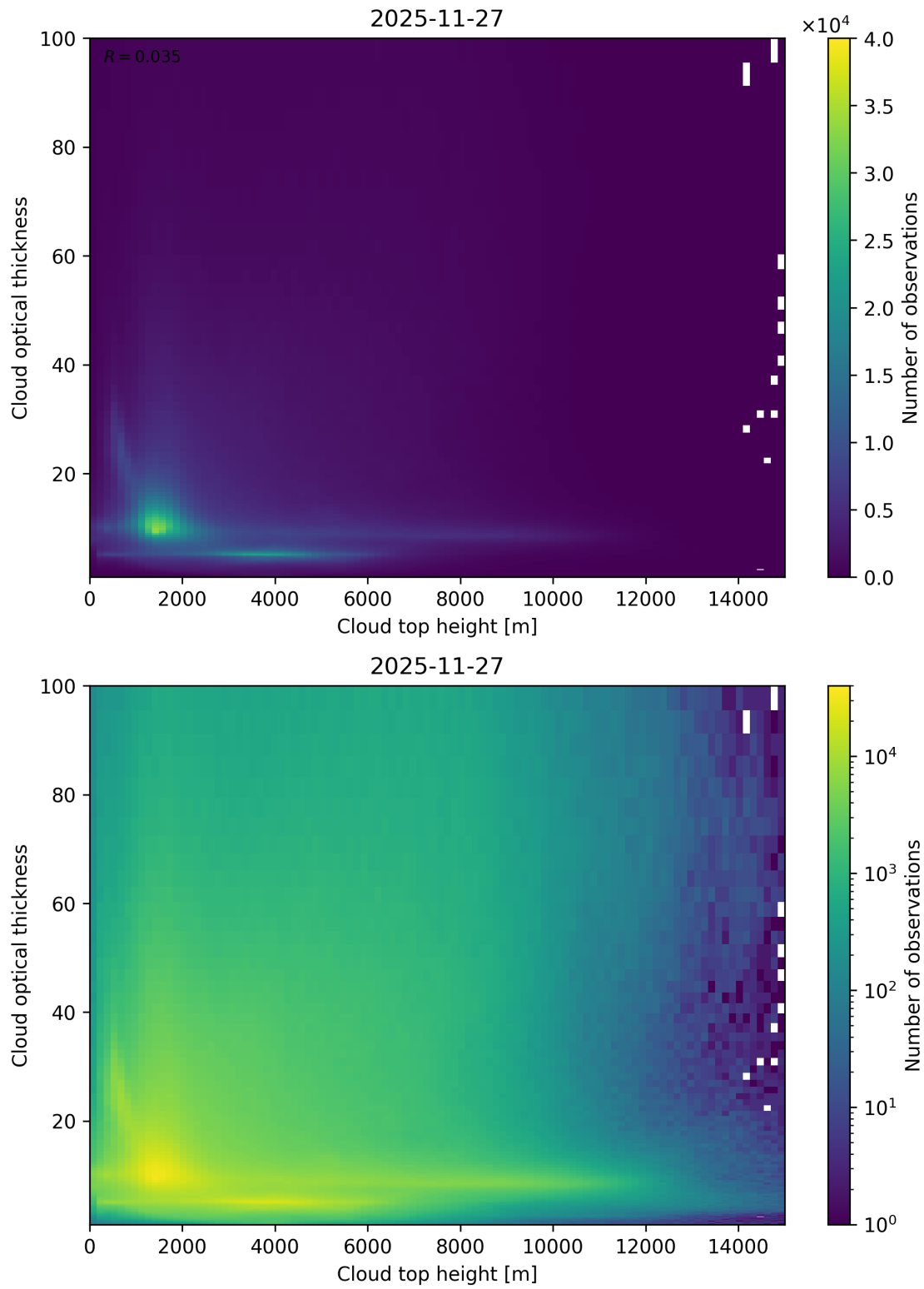
Figure 90: Scatter density plot of “Cloud top height” against “Cloud optical thickness” for 2025-11-26 to 2025-11-28.
