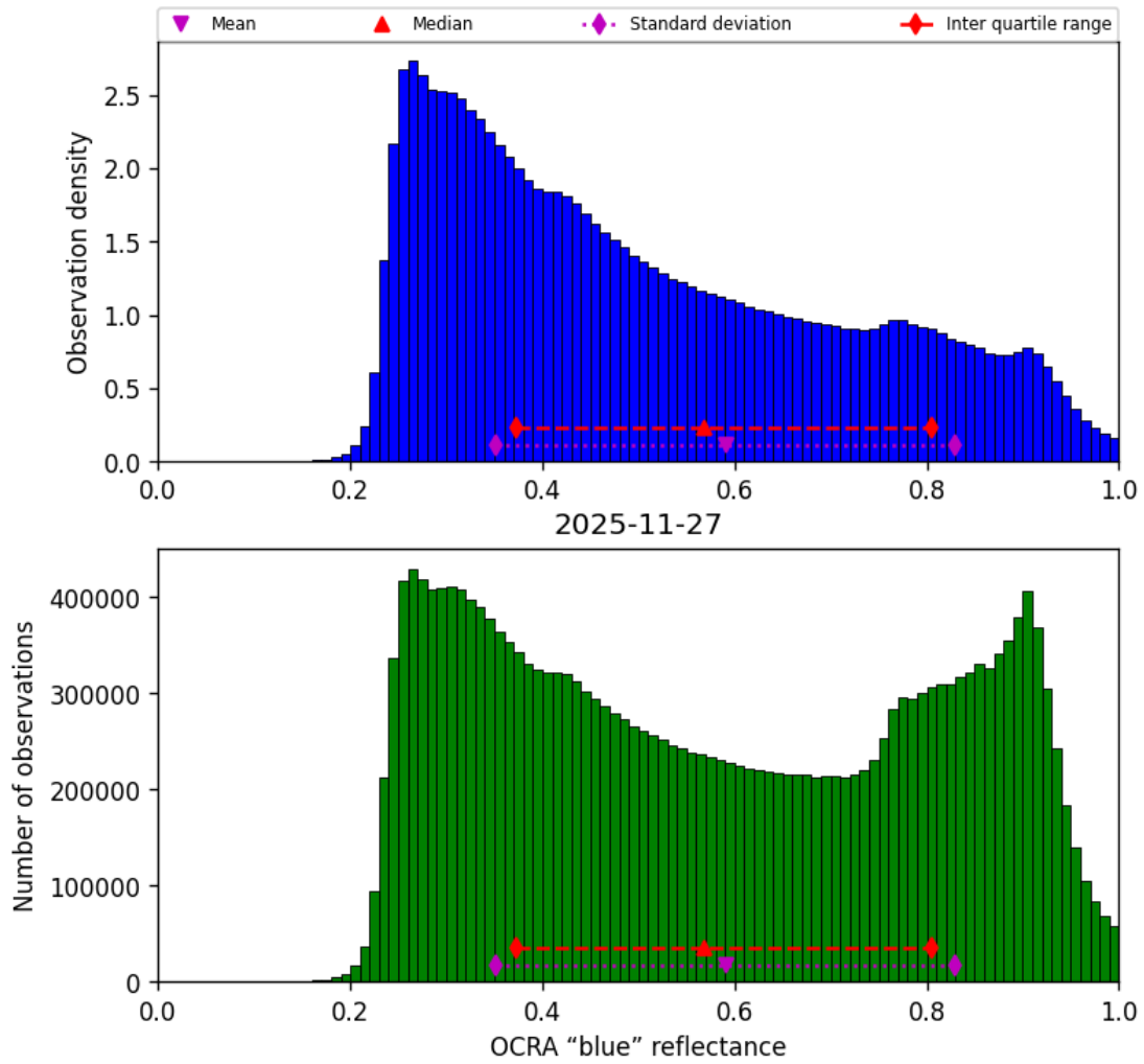
Figure 51: Histogram of “OCRA “blue” reflectance” for 2025-11-26 to 2025-11-28
