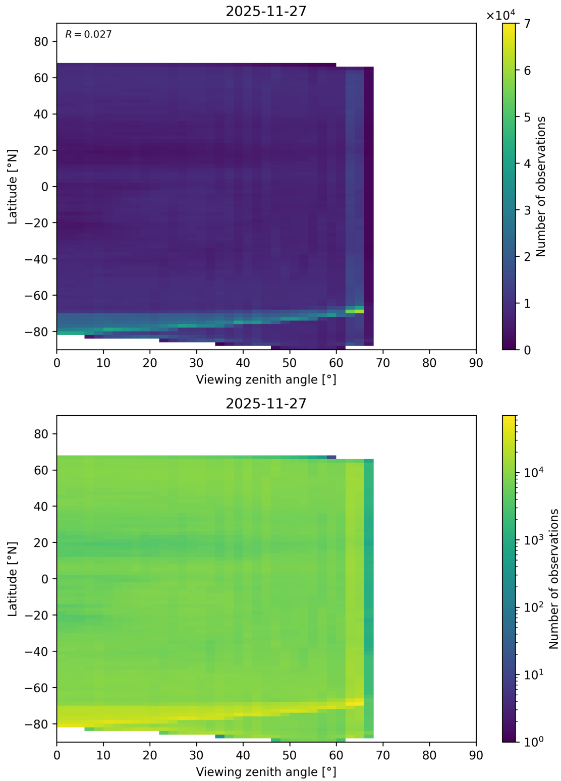
Figure 113: Scatter density plot of “Viewing zenith angle” against “Latitude” for 2025-11-26 to 2025-11-28.
