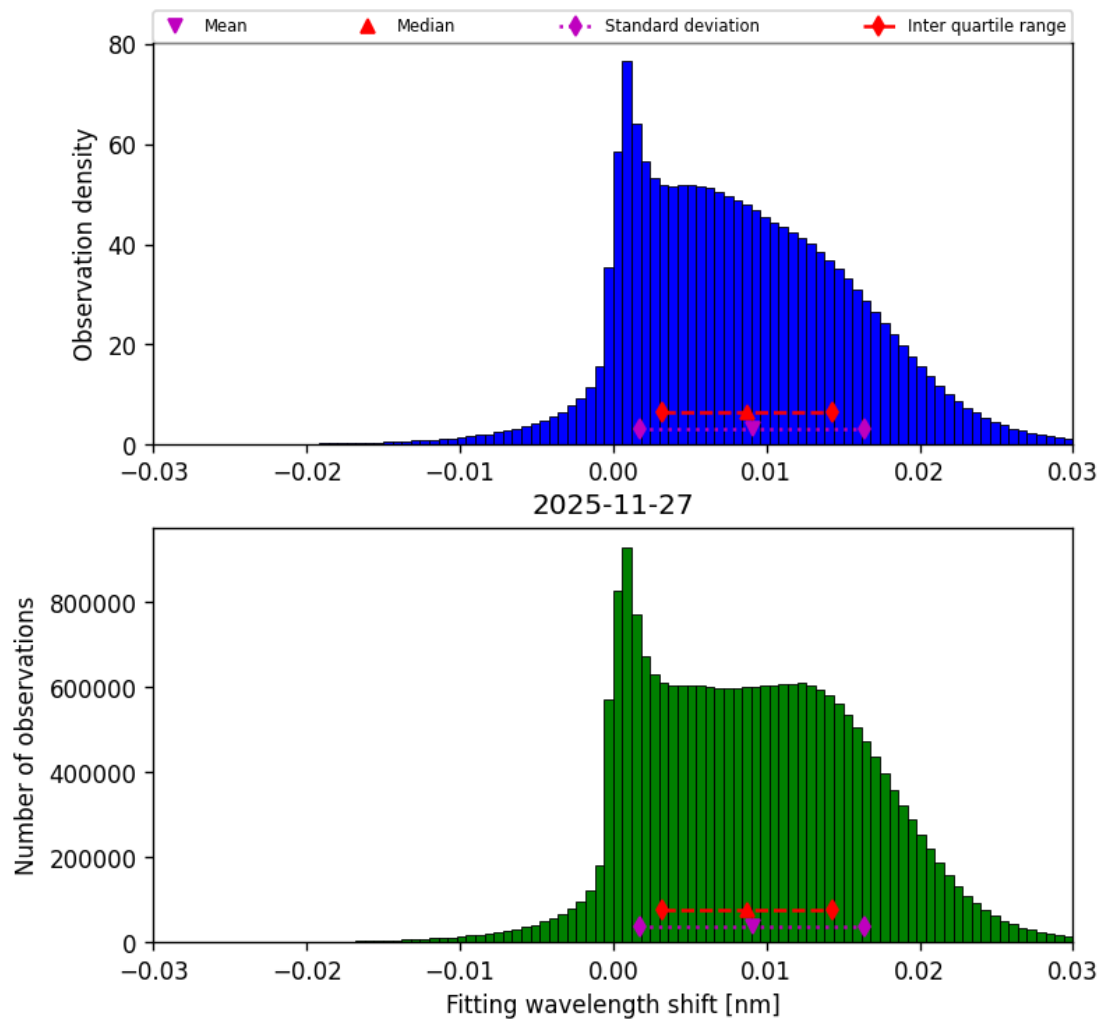
Figure 49: Histogram of “Fitting wavelength shift” for 2025-11-26 to 2025-11-28
