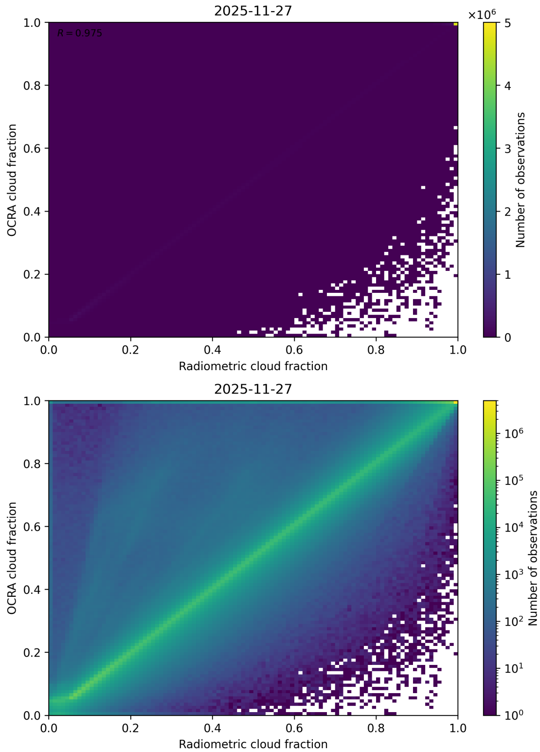
Figure 72: Scatter density plot of “Radiometric cloud fraction” against “OCRA cloud fraction” for 2025-11-26 to 2025-11-28.
