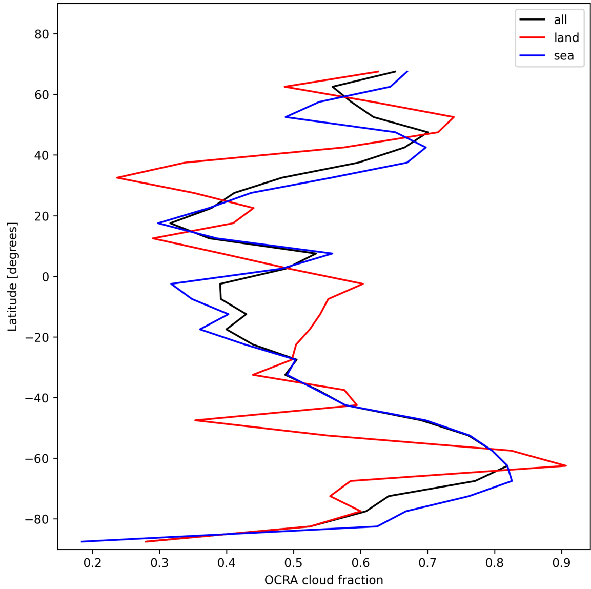
Figure 34: Zonal average of “OCRA cloud fraction” for 2025-11-26 to 2025-11-28.
