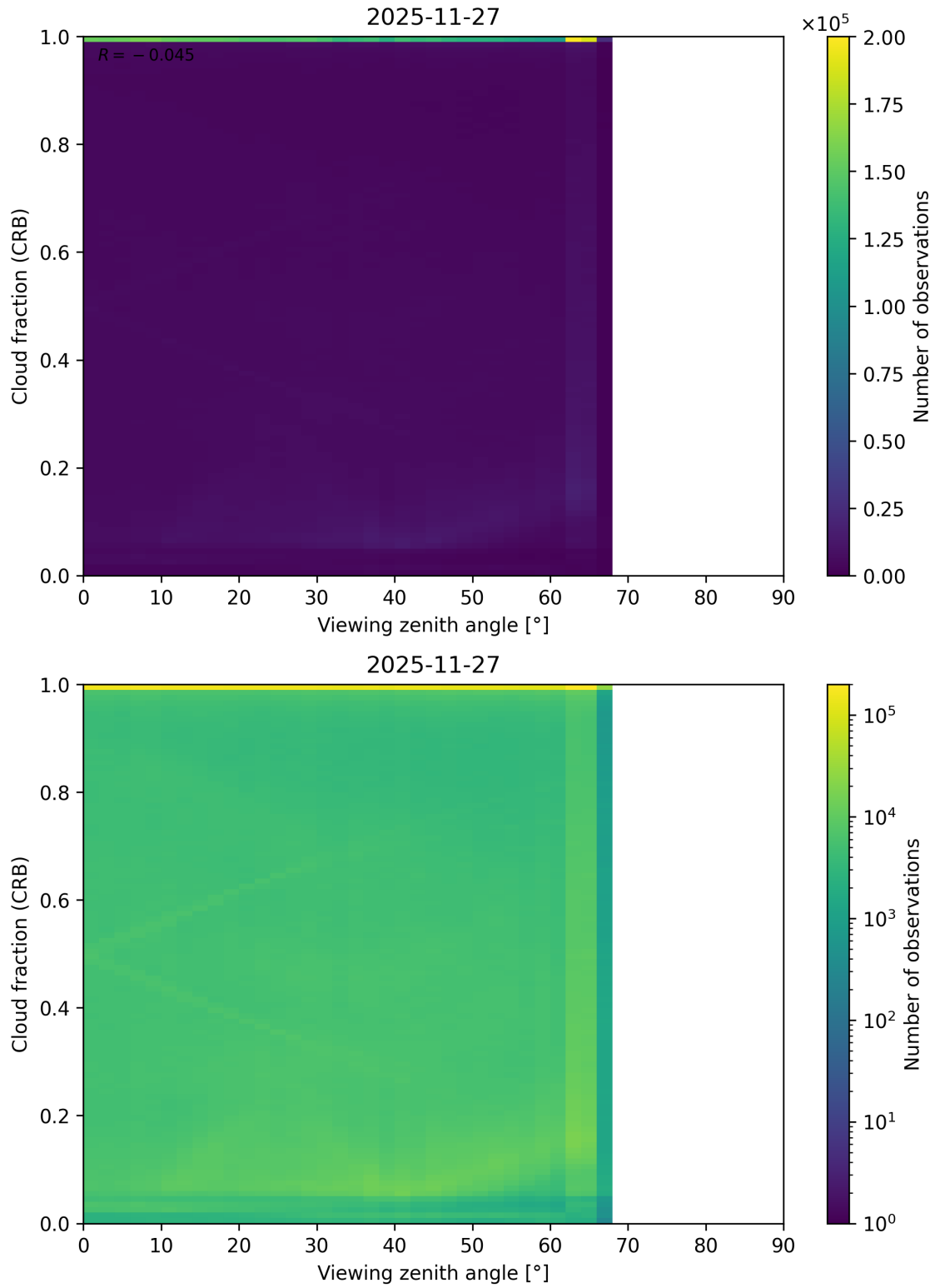
Figure 109: Scatter density plot of “Viewing zenith angle” against “Cloud fraction (CRB)” for 2025-11-26 to 2025-11-28.
