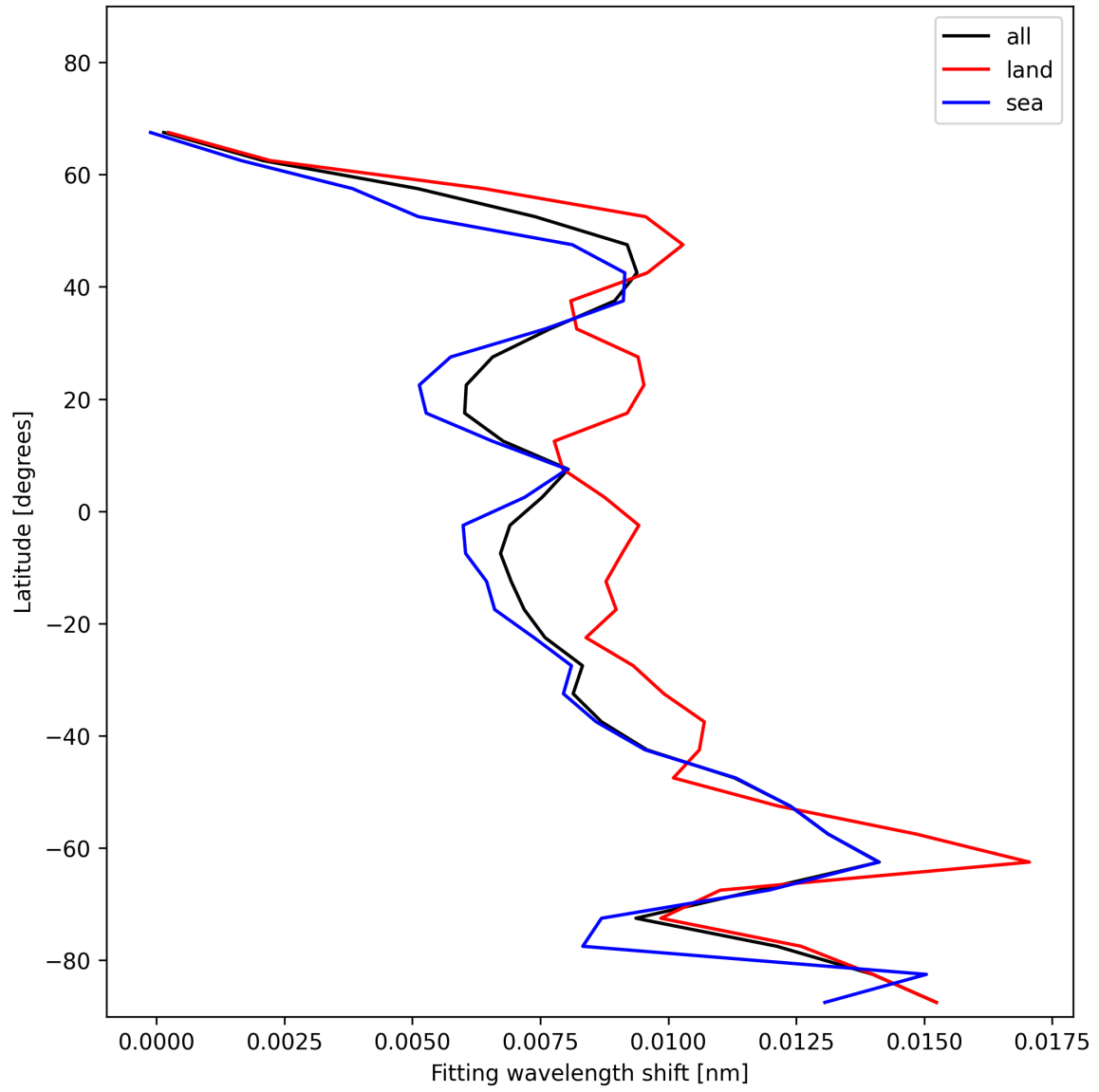
Figure 33: Zonal average of “Fitting wavelength shift” for 2025-11-26 to 2025-11-28.
