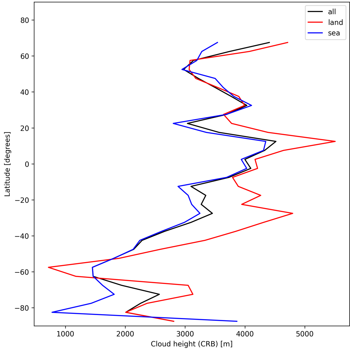
Figure 27: Zonal average of “Cloud height (CRB)” for 2025-11-26 to 2025-11-28.
