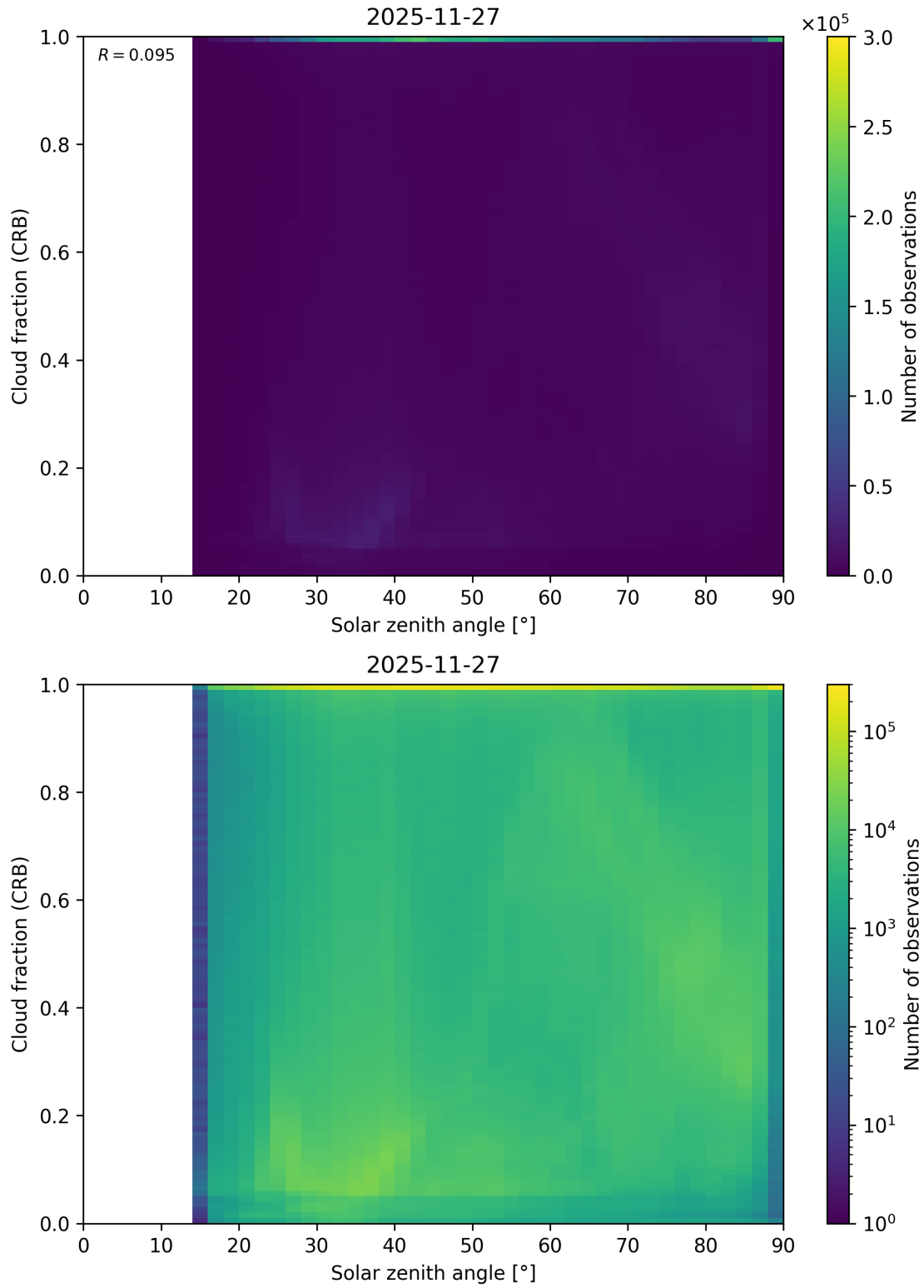
Figure 101: Scatter density plot of “Solar zenith angle” against “Cloud fraction (CRB)” for 2025-11-26 to 2025-11-28.
