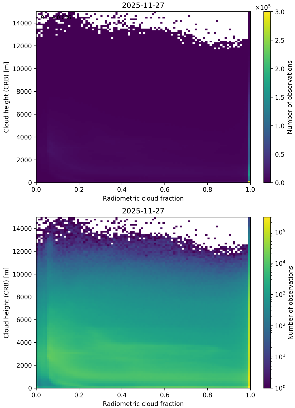
Figure 74: Scatter density plot of “Radiometric cloud fraction” against “Cloud height (CRB)” for 2025-11-26 to 2025-11-28.
