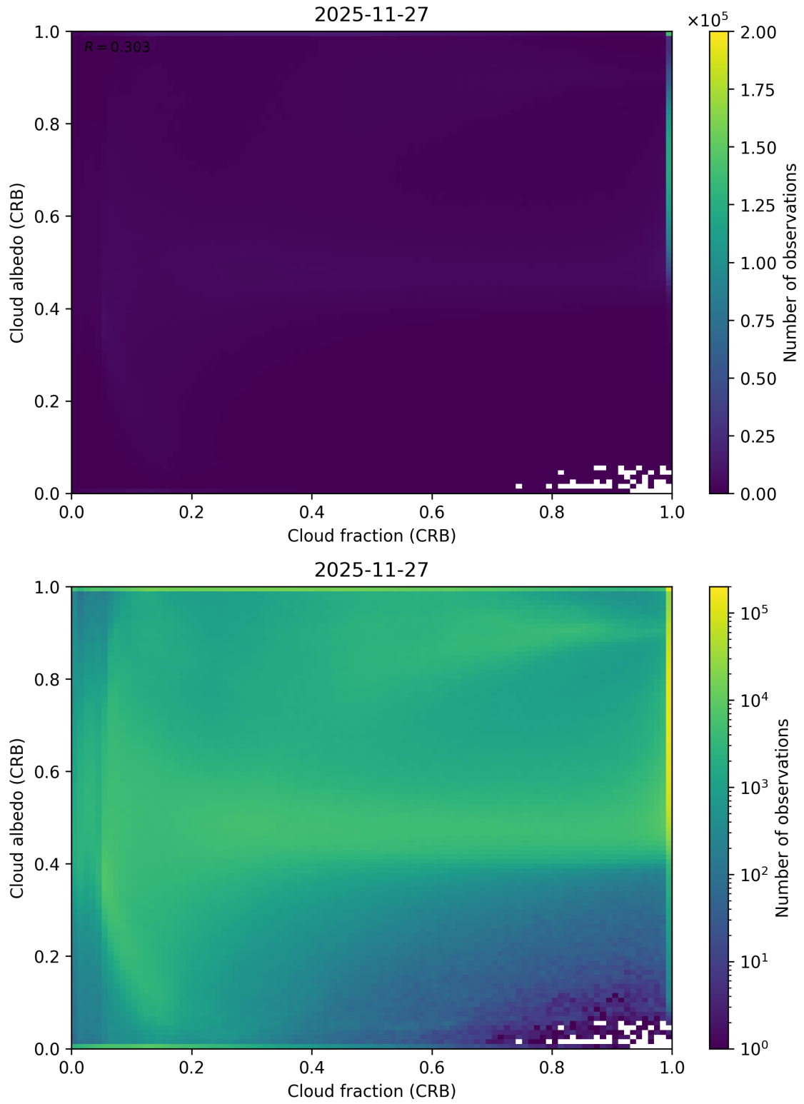
Figure 77: Scatter density plot of “Cloud fraction (CRB)” against “Cloud albedo (CRB)” for 2025-11-26 to 2025-11-28.
