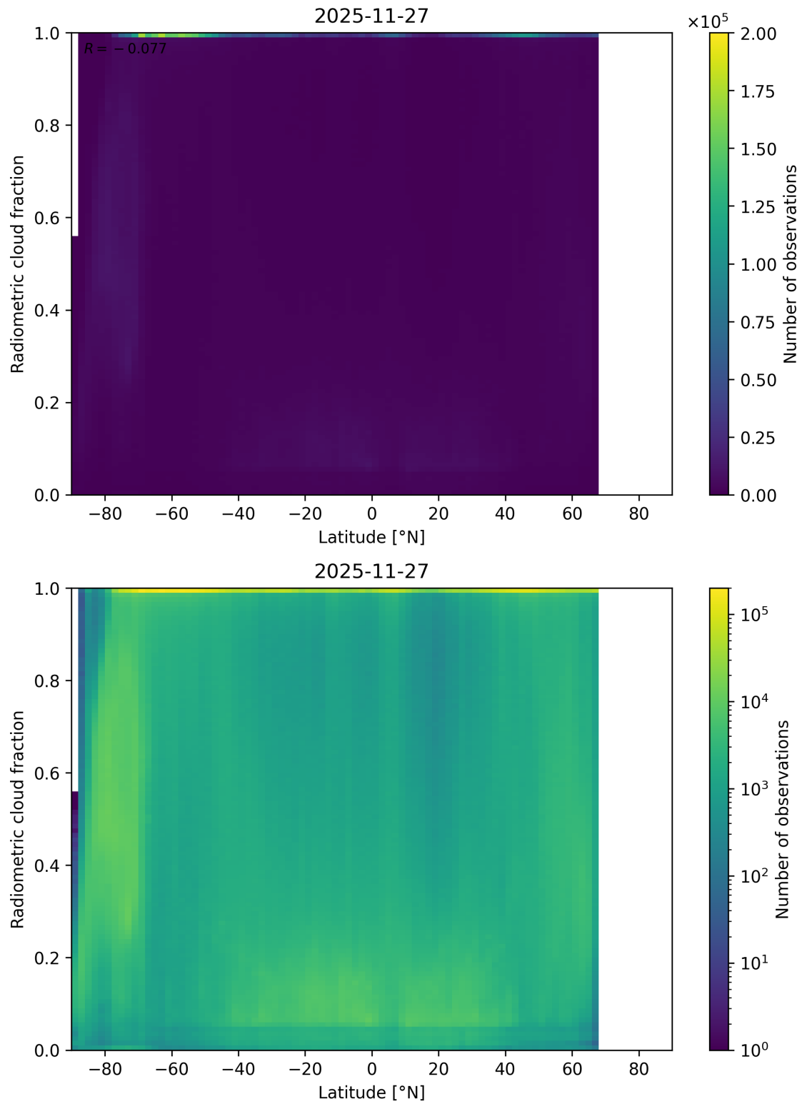
Figure 92: Scatter density plot of “Latitude” against “Radiometric cloud fraction” for 2025-11-26 to 2025-11-28.
