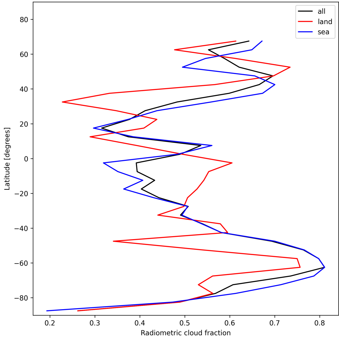
Figure 23: Zonal average of “Radiometric cloud fraction” for 2025-11-26 to 2025-11-28.
