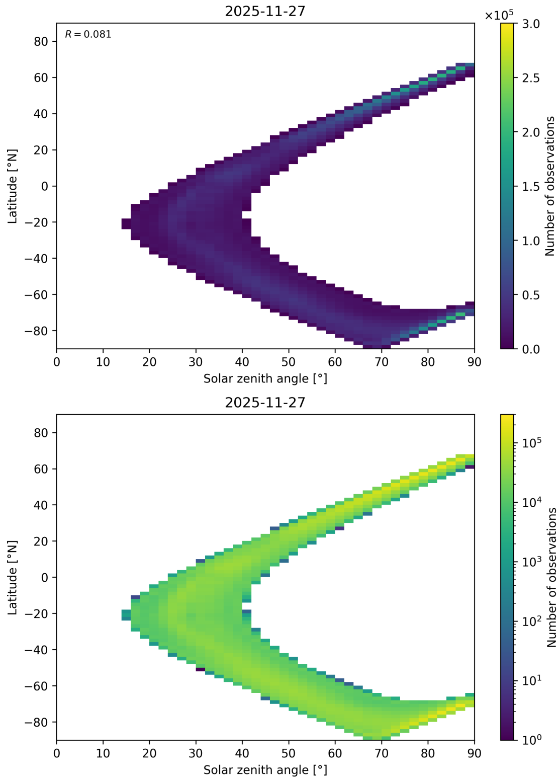
Figure 105: Scatter density plot of “Solar zenith angle” against “Latitude” for 2025-11-26 to 2025-11-28.
