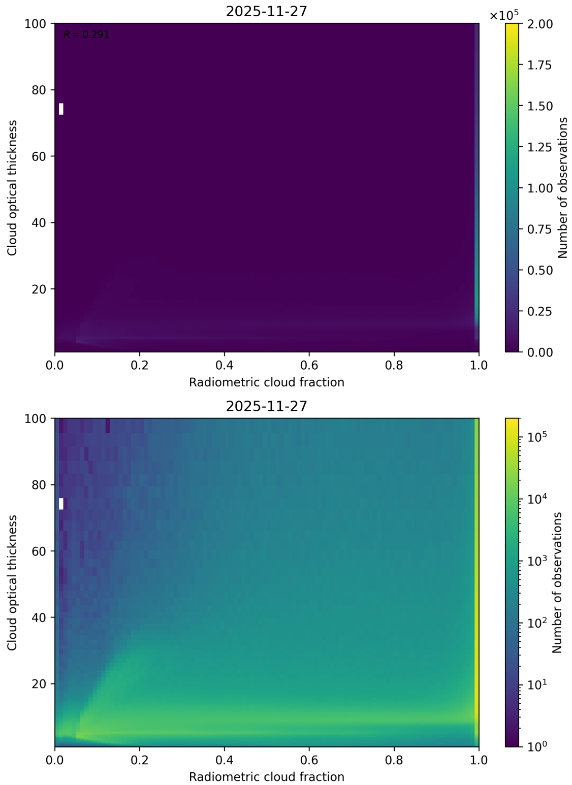
Figure 75: Scatter density plot of “Radiometric cloud fraction” against “Cloud optical thickness” for 2025-11-26 to 2025-11-28.
