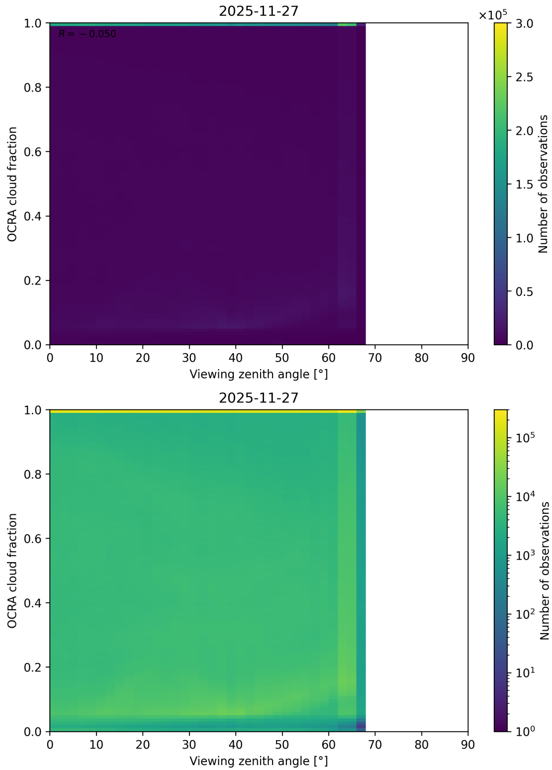
Figure 108: Scatter density plot of “Viewing zenith angle” against “OCRA cloud fraction” for 2025-11-26 to 2025-11-28.
