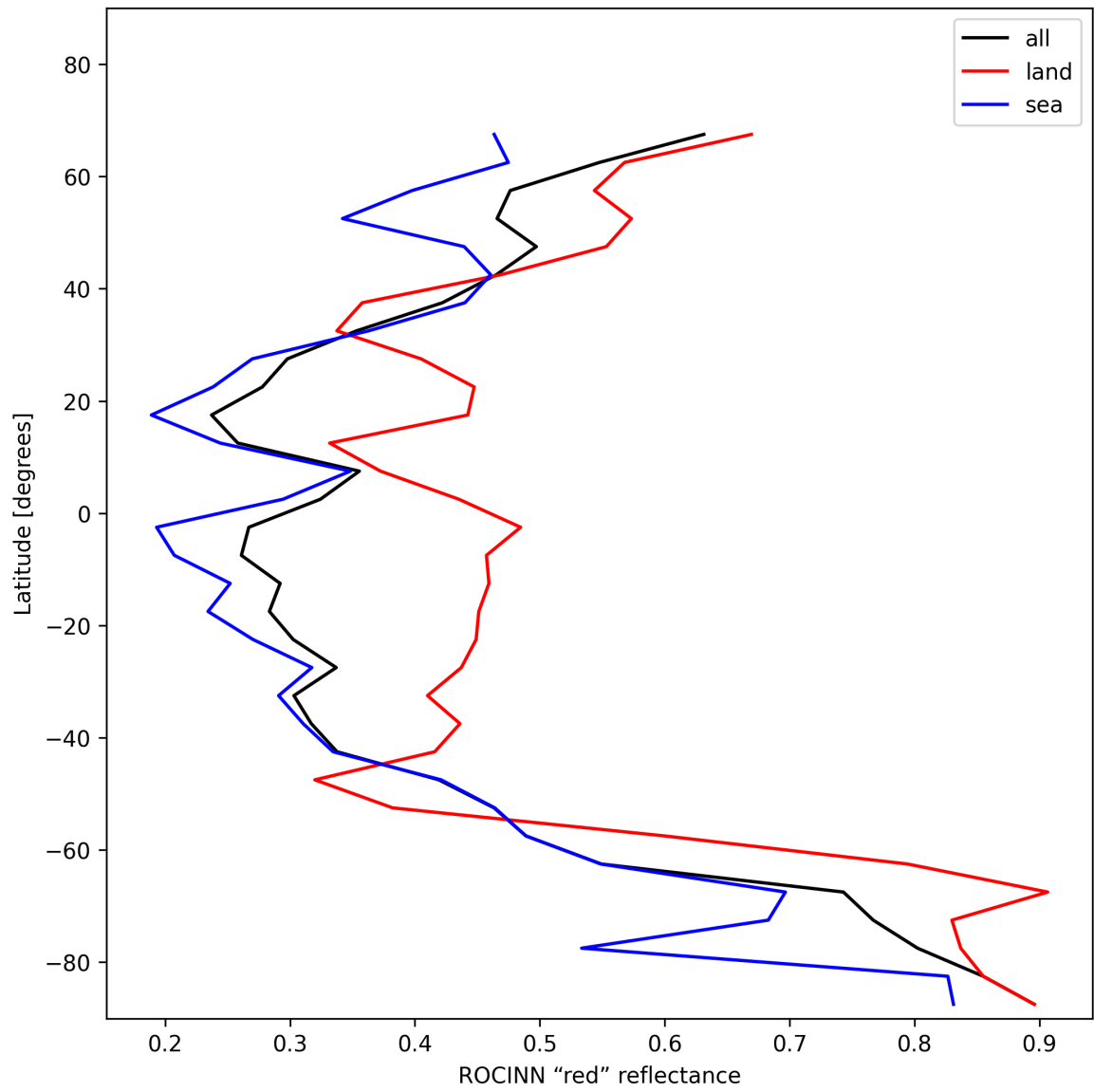
Figure 37: Zonal average of “ROCINN “red” reflectance” for 2025-11-26 to 2025-11-28.
