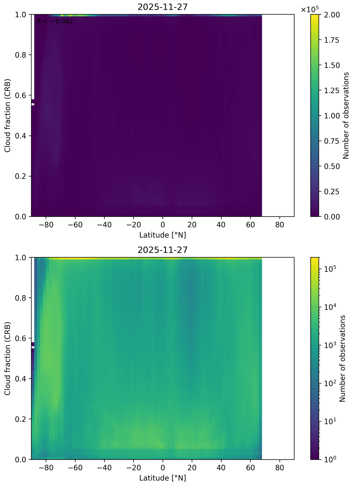
Figure 94: Scatter density plot of “Latitude” against “Cloud fraction (CRB)” for 2025-11-26 to 2025-11-28.
