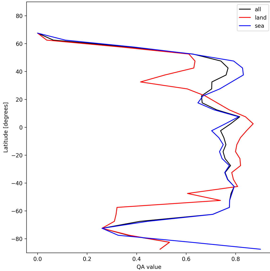
Figure 22: Zonal average of “QA value” for 2025-11-26 to 2025-11-28.
