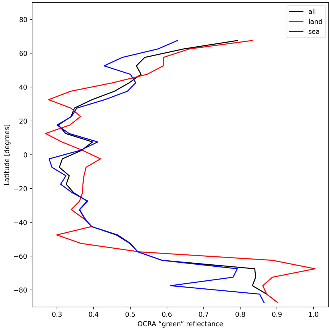
Figure 36: Zonal average of “OCRA “green” reflectance” for 2025-11-26 to 2025-11-28.
