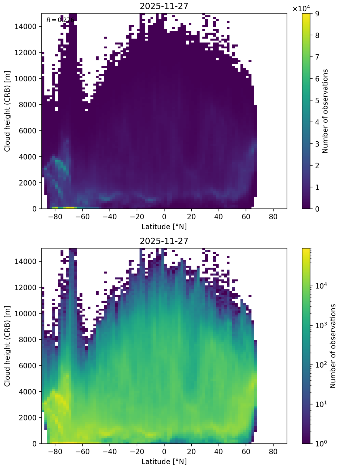
Figure 95: Scatter density plot of “Latitude” against “Cloud height (CRB)” for 2025-11-26 to 2025-11-28.
