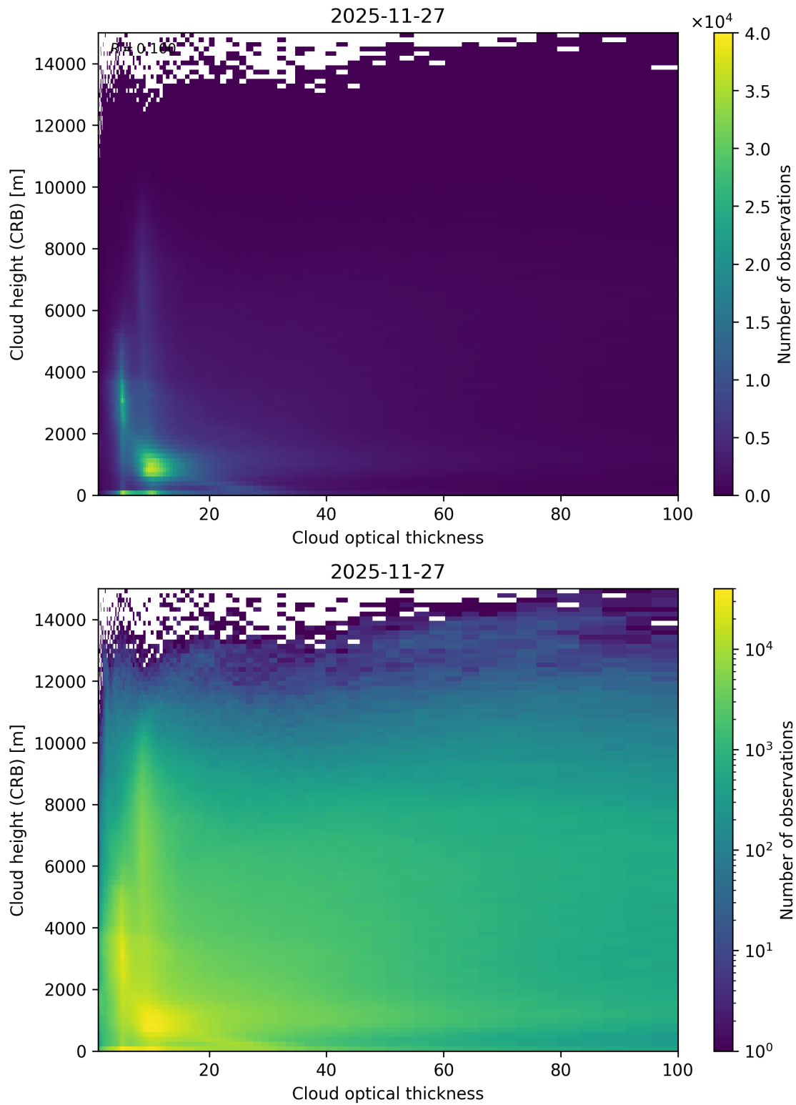
Figure 85: Scatter density plot of “Cloud optical thickness” against “Cloud height (CRB)” for 2025-11-26 to 2025-11-28.
