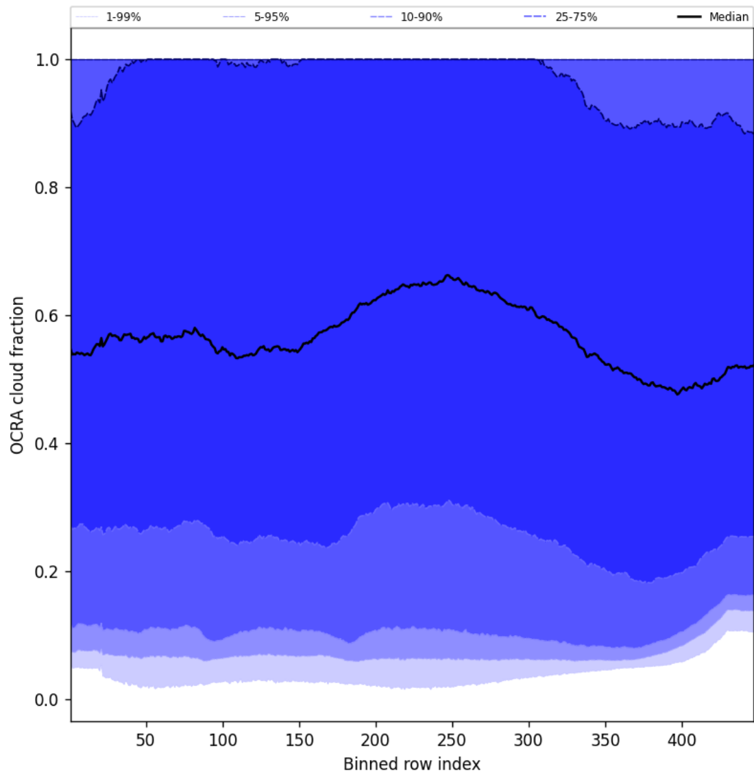
Figure 66: Along track statistics of “OCRA cloud fraction” for 2025-11-26 to 2025-11-28
