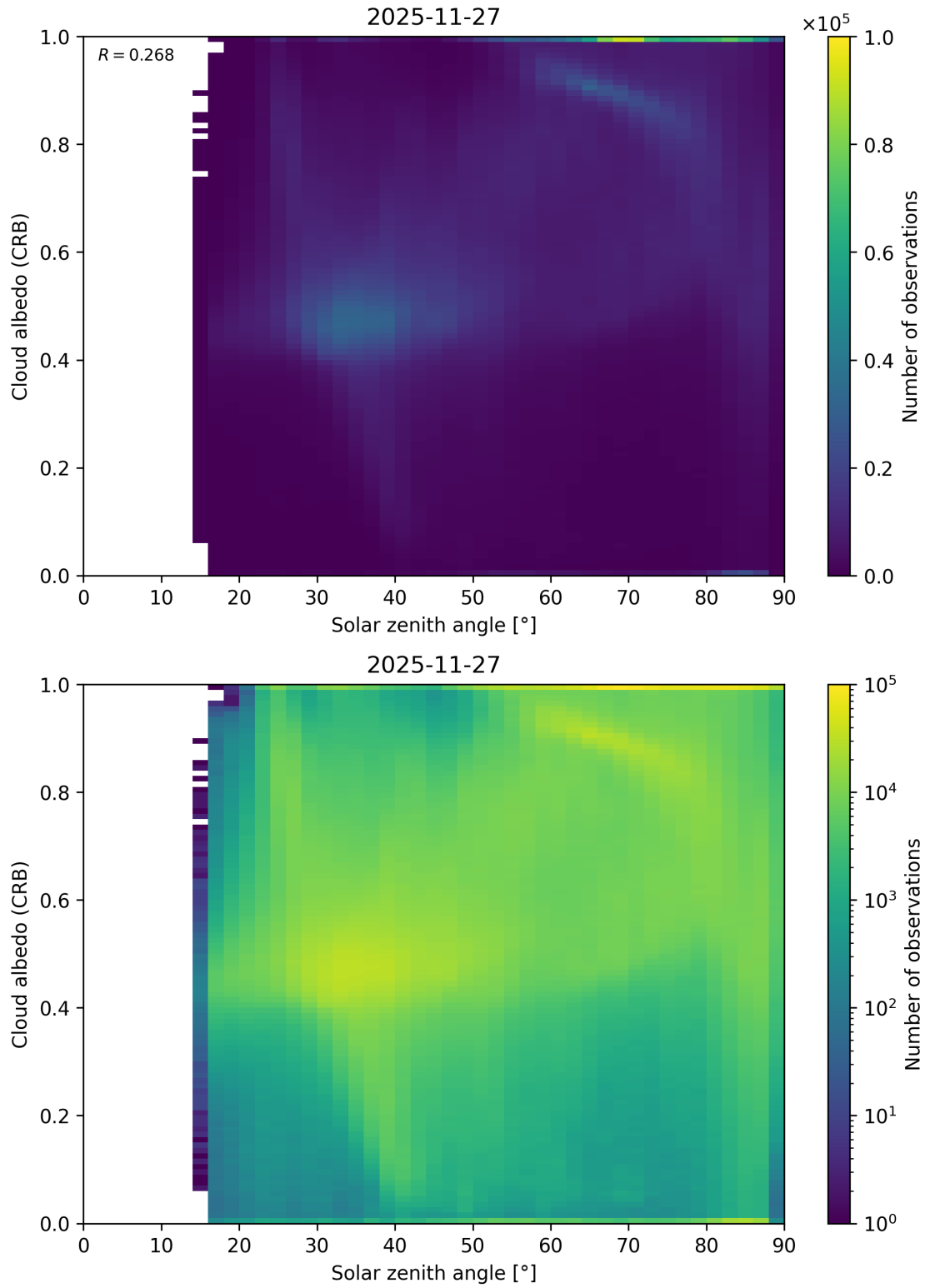
Figure 98: Scatter density plot of “Solar zenith angle” against “Cloud albedo (CRB)” for 2025-11-26 to 2025-11-28.
