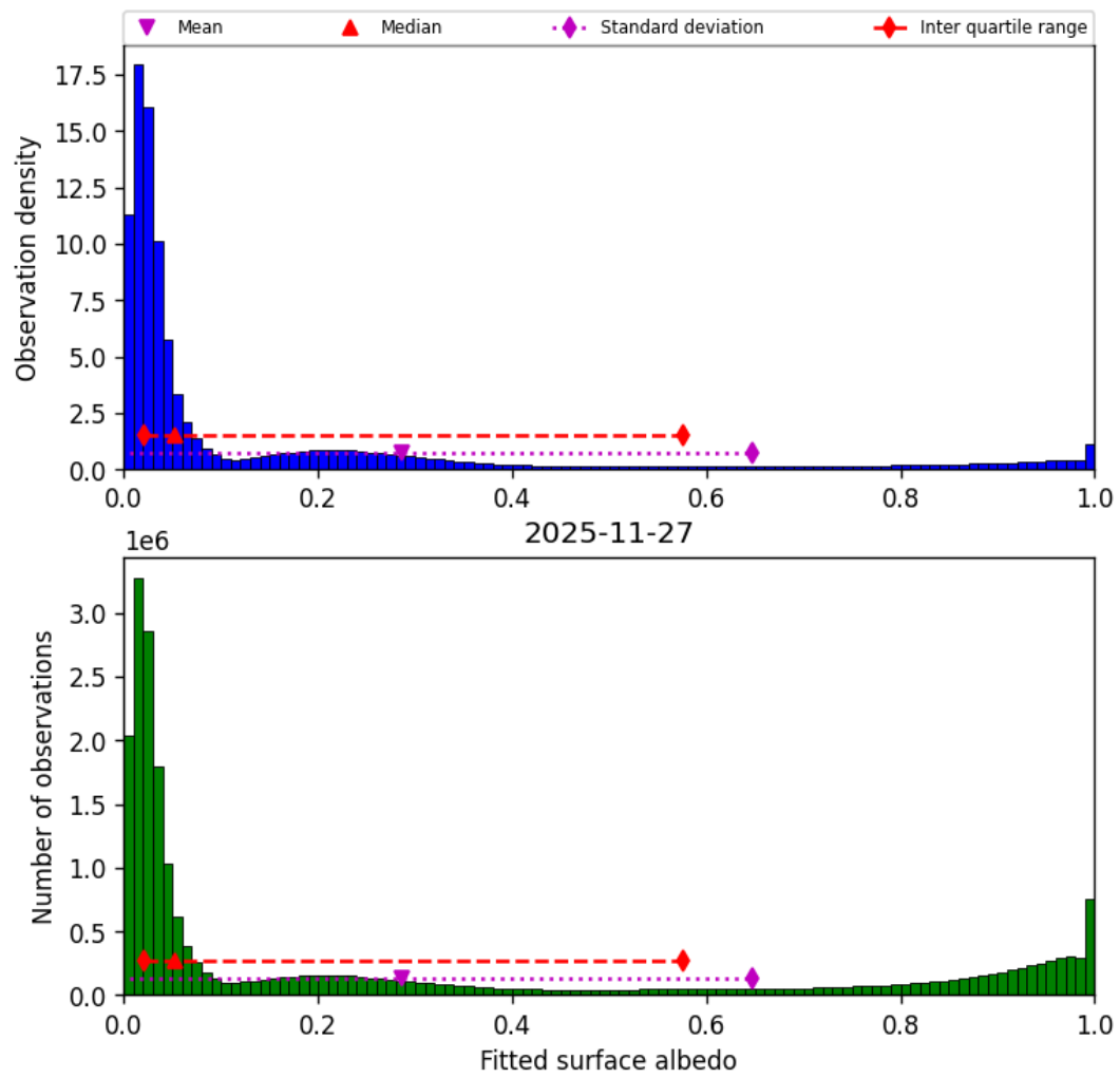
Figure 45: Histogram of “Fitted surface albedo” for 2025-11-26 to 2025-11-28
