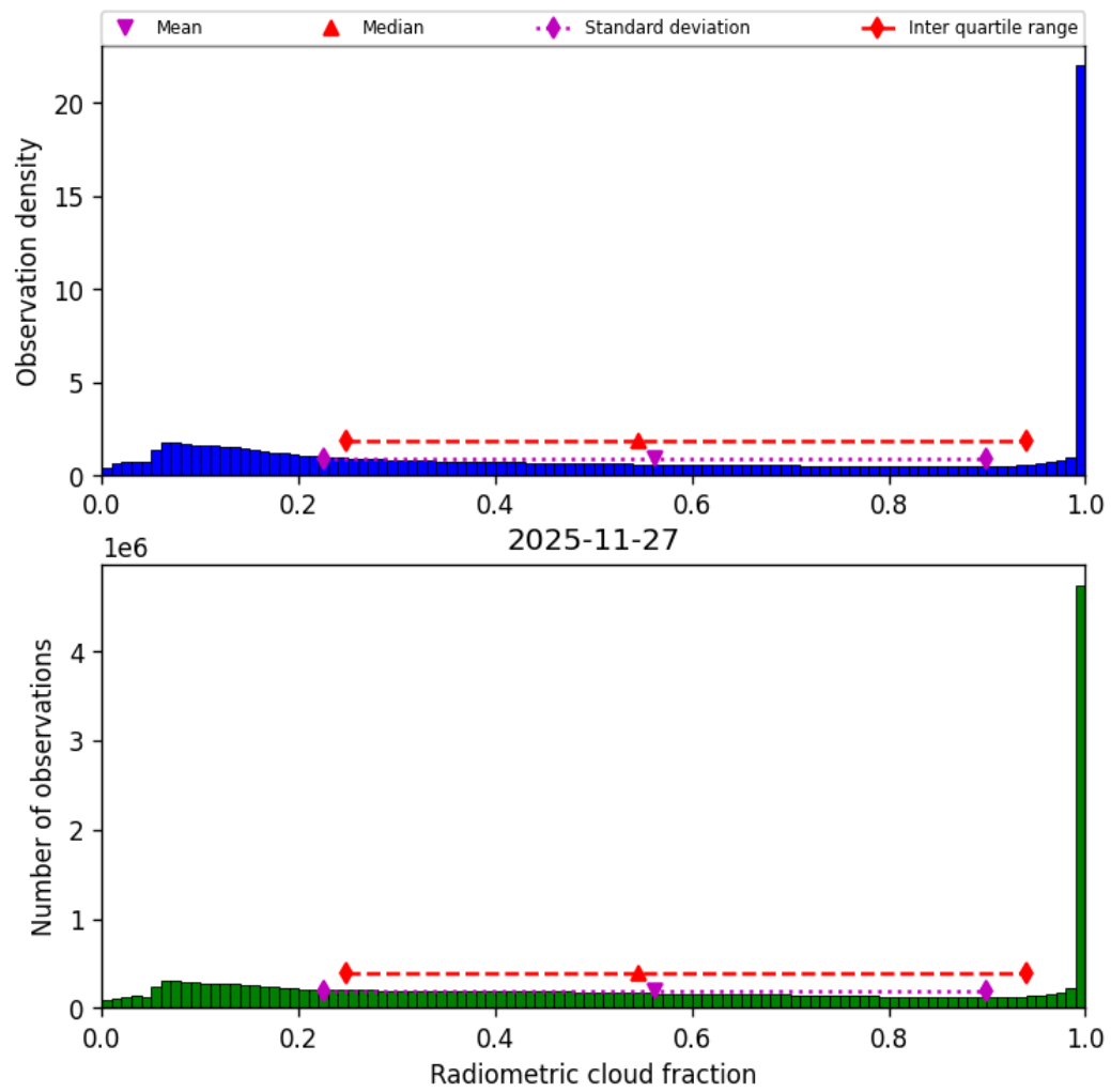
Figure 39: Histogram of “Radiometric cloud fraction” for 2025-11-26 to 2025-11-28
