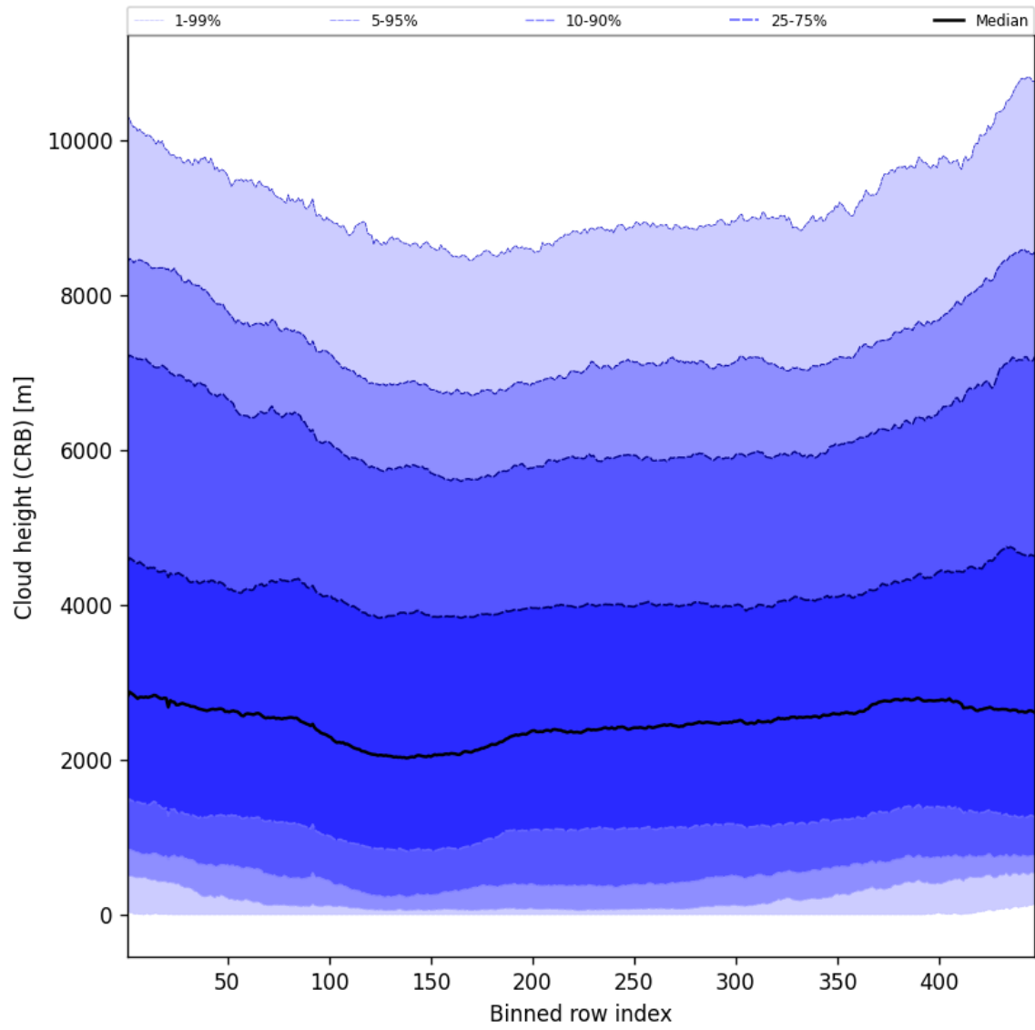
Figure 59: Along track statistics of “Cloud height (CRB)” for 2025-11-26 to 2025-11-28
