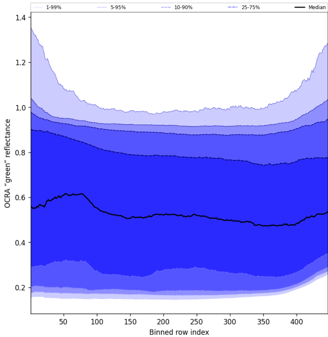
Figure 68: Along track statistics of “OCRA “green” reflectance” for 2025-11-26 to 2025-11-28
