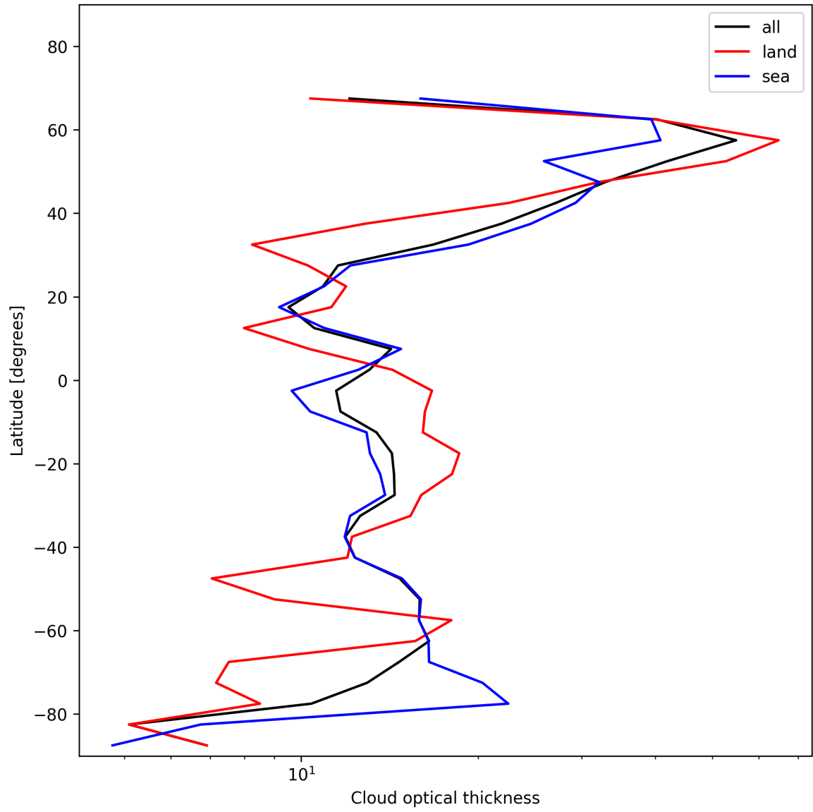
Figure 25: Zonal average of “Cloud optical thickness” for 2025-11-26 to 2025-11-28.
