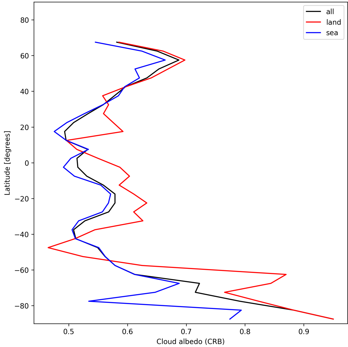
Figure 28: Zonal average of “Cloud albedo (CRB)” for 2025-11-26 to 2025-11-28.
