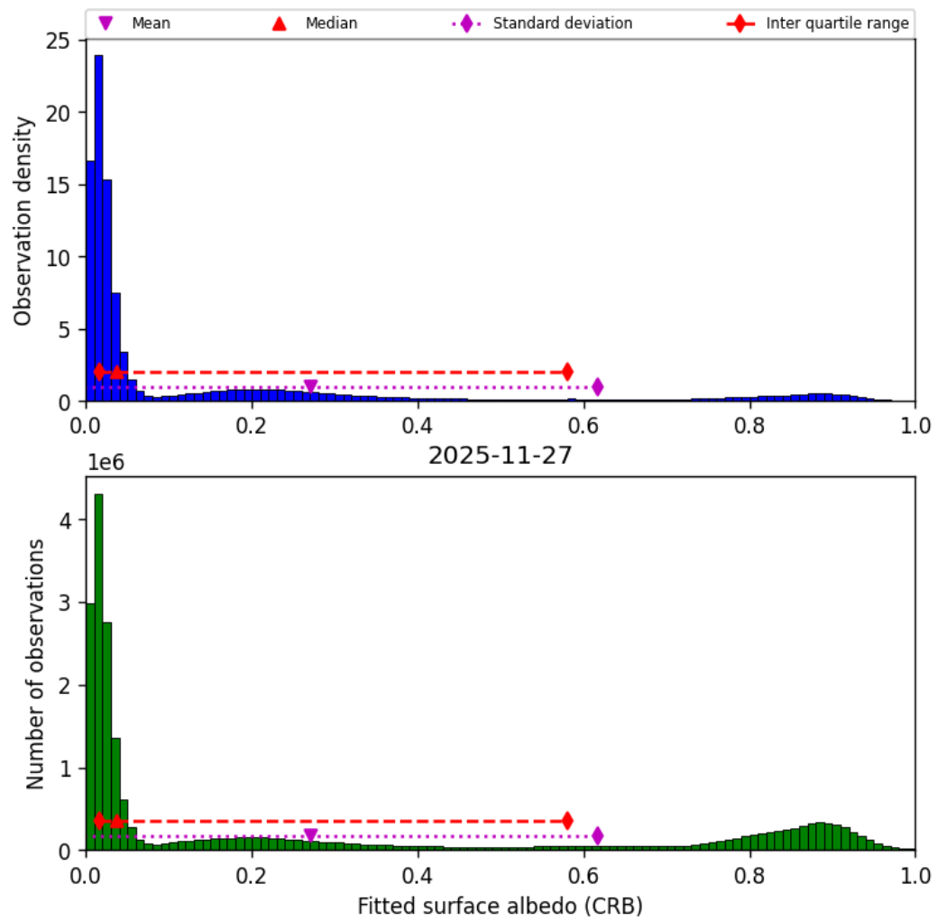
Figure 46: Histogram of “Fitted surface albedo (CRB)” for 2025-11-26 to 2025-11-28
