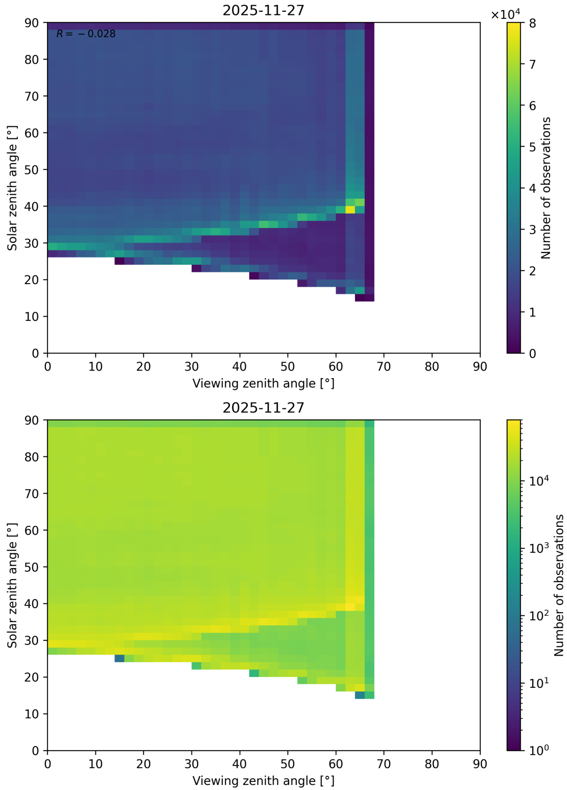
Figure 114: Scatter density plot of “Viewing zenith angle” against “Solar zenith angle” for 2025-11-26 to 2025-11-28.
