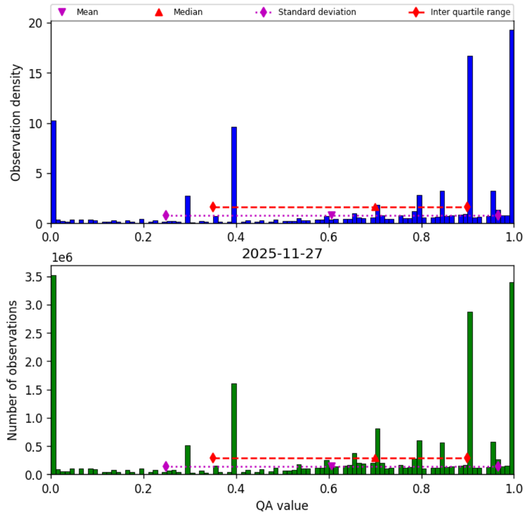
Figure 38: Histogram of “QA value” for 2025-11-26 to 2025-11-28
