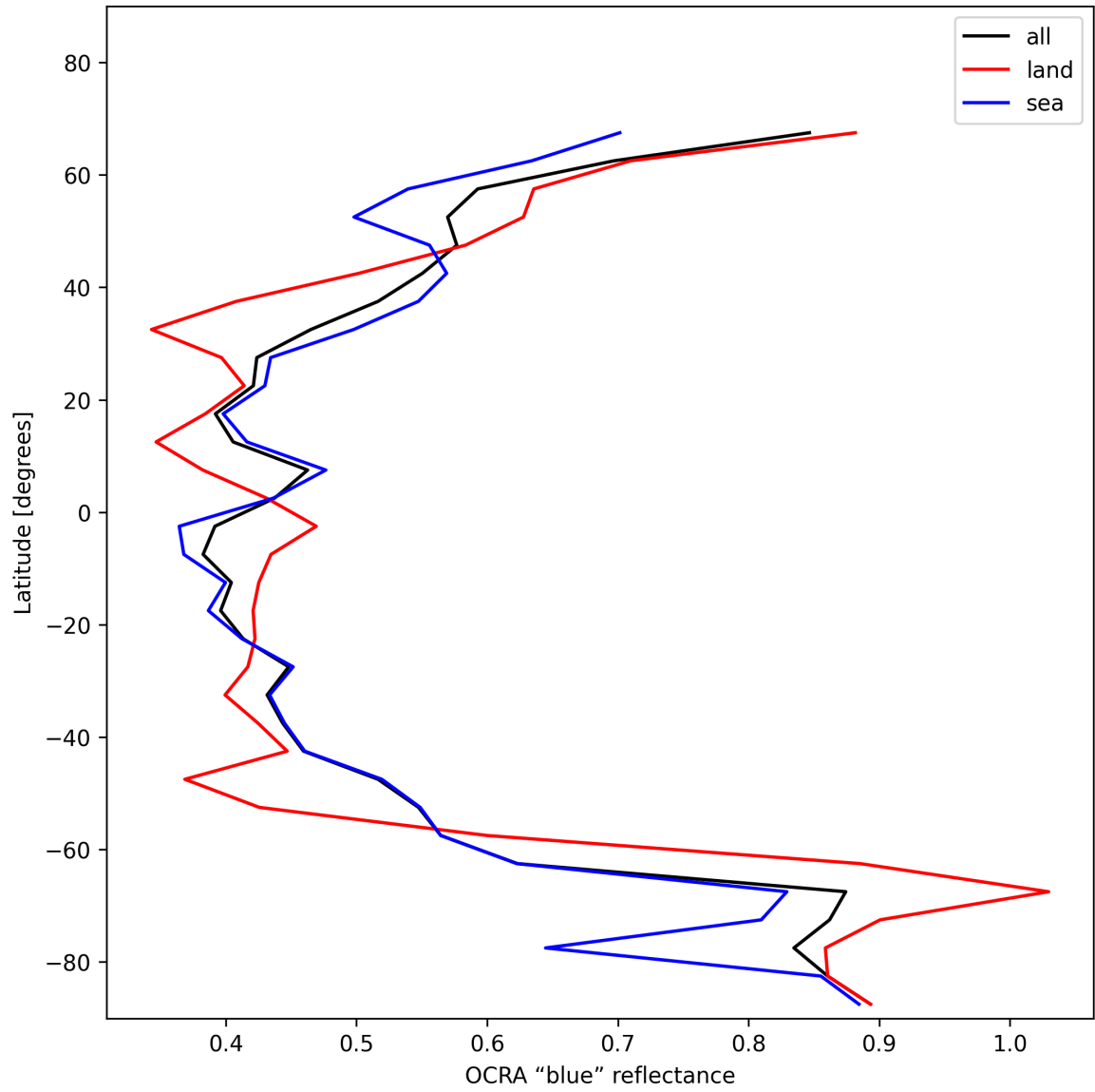
Figure 35: Zonal average of “OCRA “blue” reflectance” for 2025-11-26 to 2025-11-28.
