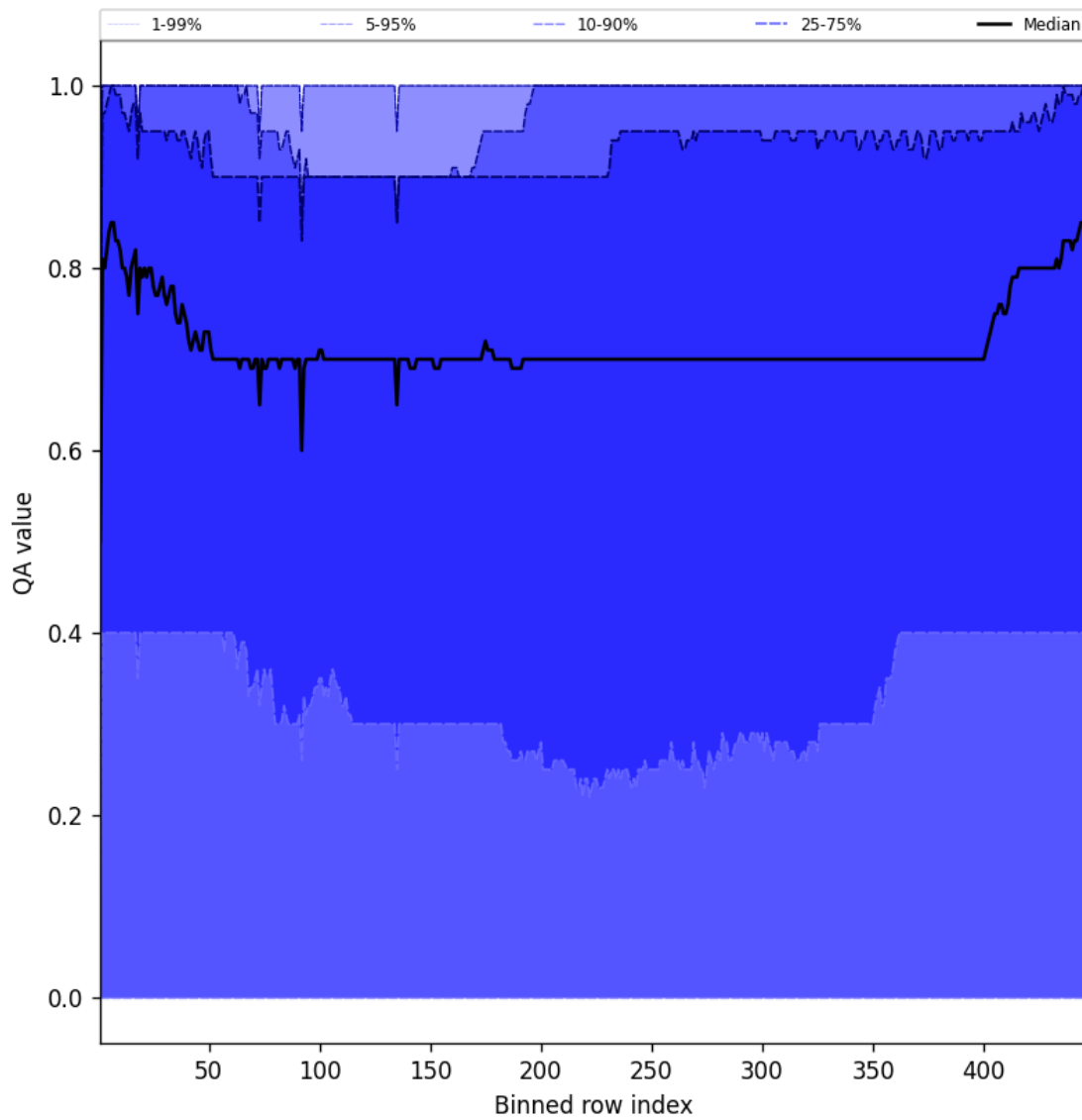
Figure 54: Along track statistics of “QA value” for 2025-11-26 to 2025-11-28
