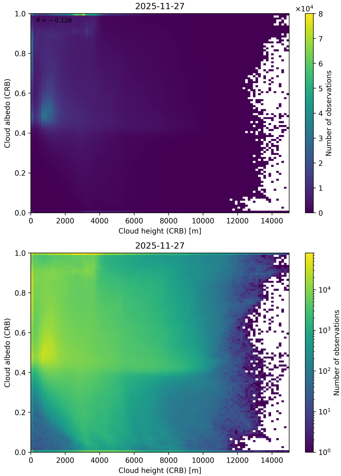
Figure 80: Scatter density plot of “Cloud height (CRB)” against “Cloud albedo (CRB)” for 2025-11-26 to 2025-11-28.
