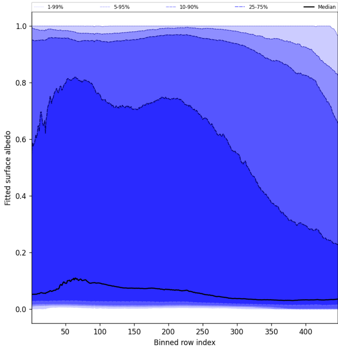
Figure 61: Along track statistics of “Fitted surface albedo” for 2025-11-26 to 2025-11-28
