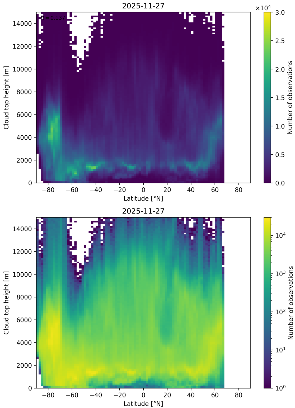
Figure 97: Scatter density plot of “Latitude” against “Cloud top height” for 2025-11-26 to 2025-11-28.
