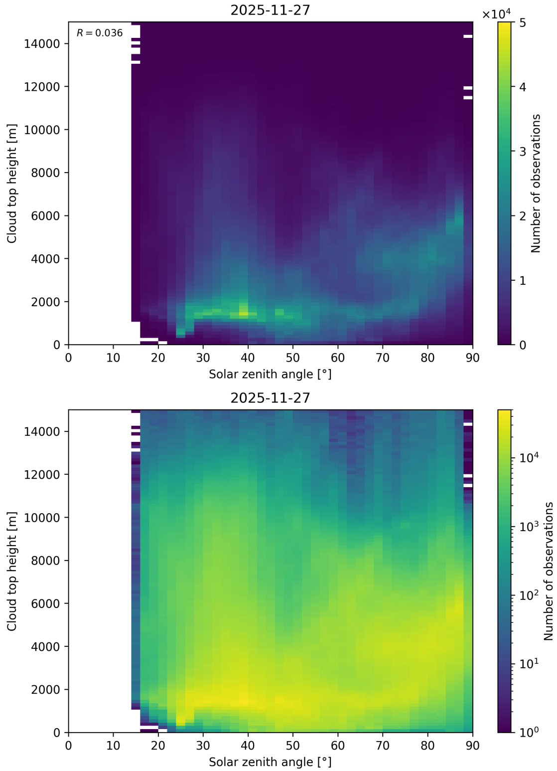
Figure 104: Scatter density plot of “Solar zenith angle” against “Cloud top height” for 2025-11-26 to 2025-11-28.
