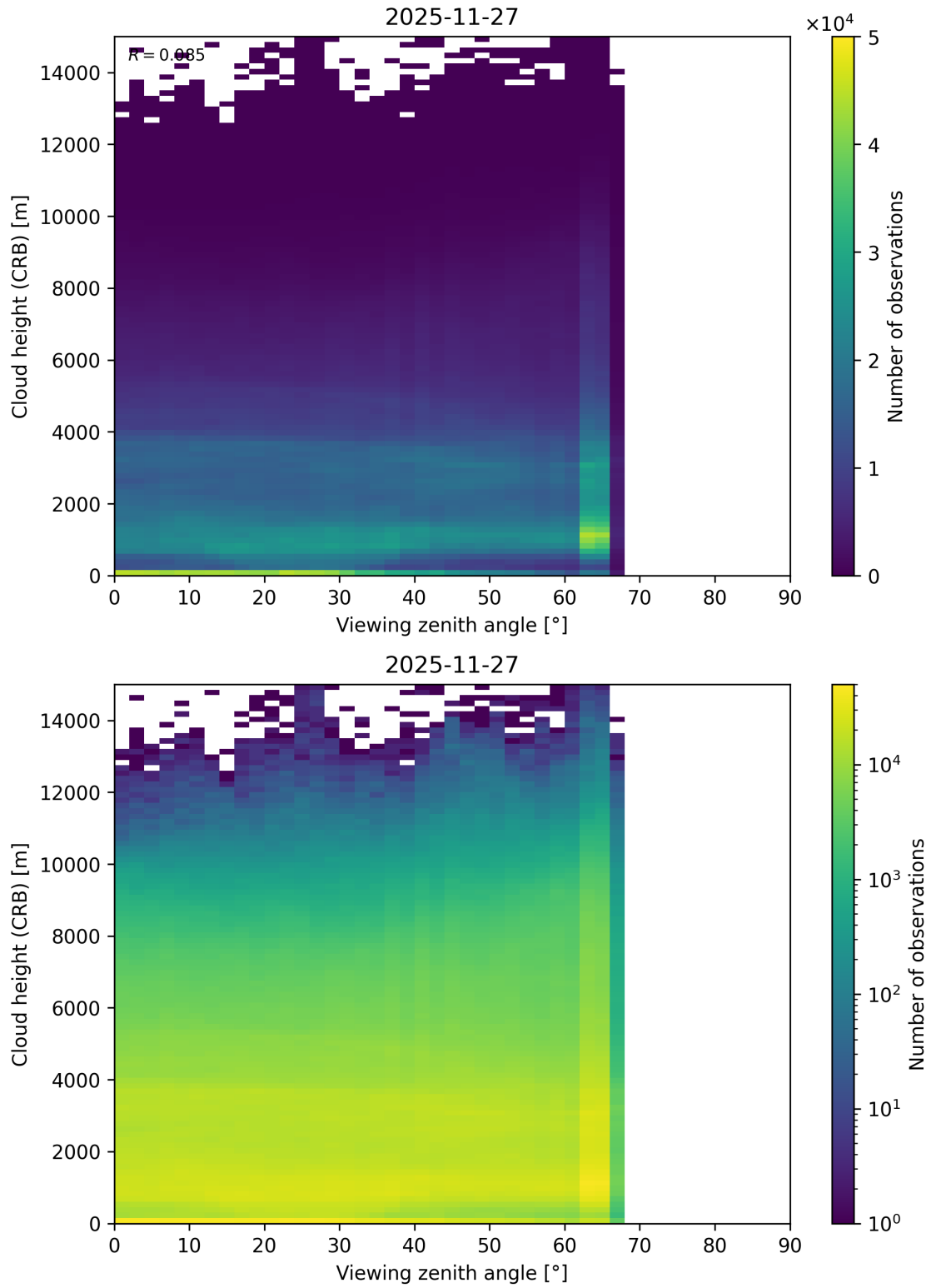
Figure 110: Scatter density plot of “Viewing zenith angle” against “Cloud height (CRB)” for 2025-11-26 to 2025-11-28.
