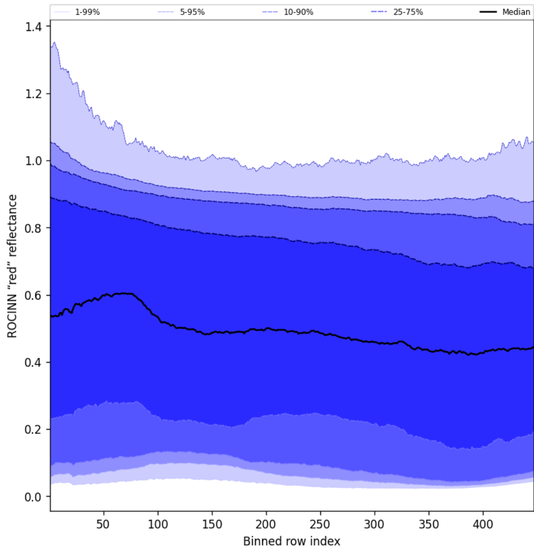
Figure 69: Along track statistics of “ROCINN “red” reflectance” for 2025-11-26 to 2025-11-28
