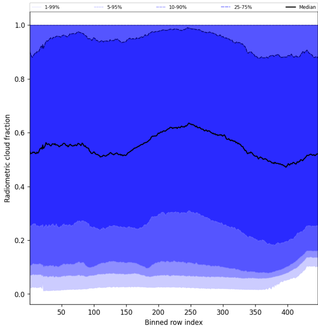
Figure 55: Along track statistics of “Radiometric cloud fraction” for 2025-11-26 to 2025-11-28
