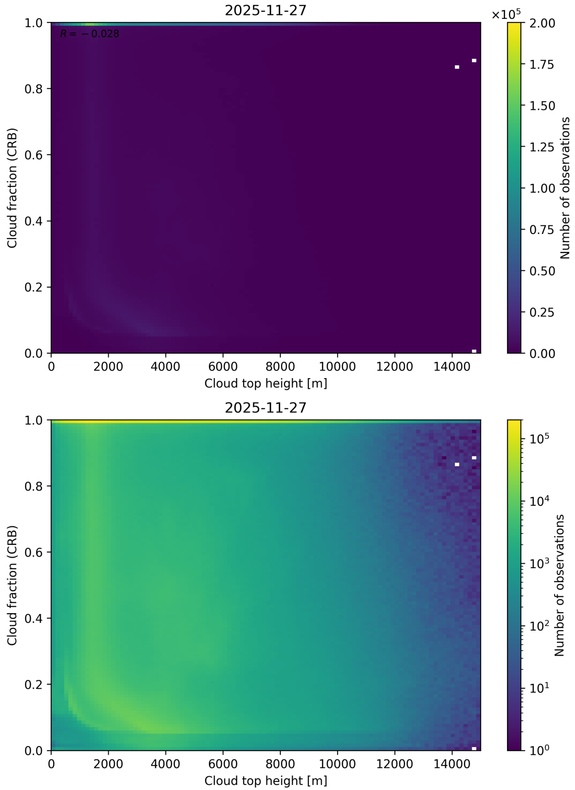
Figure 88: Scatter density plot of “Cloud top height” against “Cloud fraction (CRB)” for 2025-11-26 to 2025-11-28.
