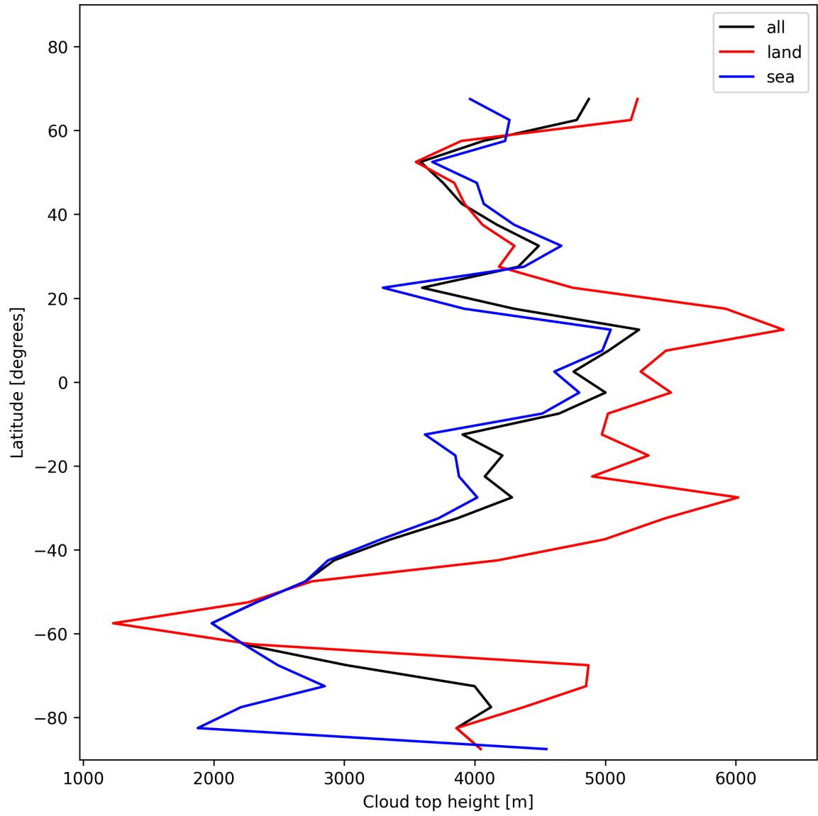
Figure 24: Zonal average of “Cloud top height” for 2025-11-26 to 2025-11-28.
