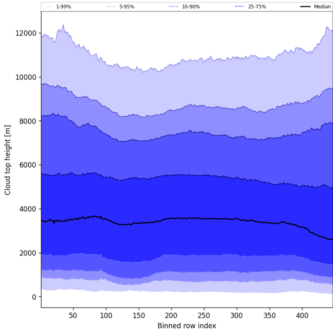
Figure 56: Along track statistics of “Cloud top height” for 2025-11-26 to 2025-11-28
