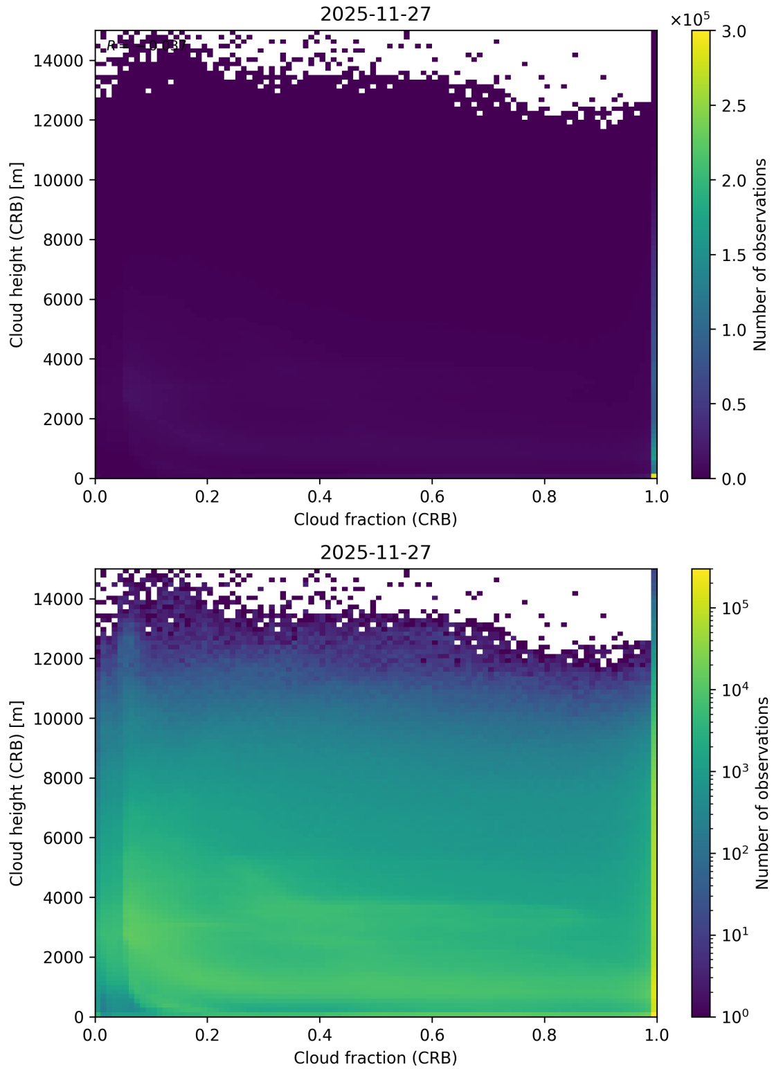
Figure 79: Scatter density plot of “Cloud fraction (CRB)” against “Cloud height (CRB)” for 2025-11-26 to 2025-11-28.
