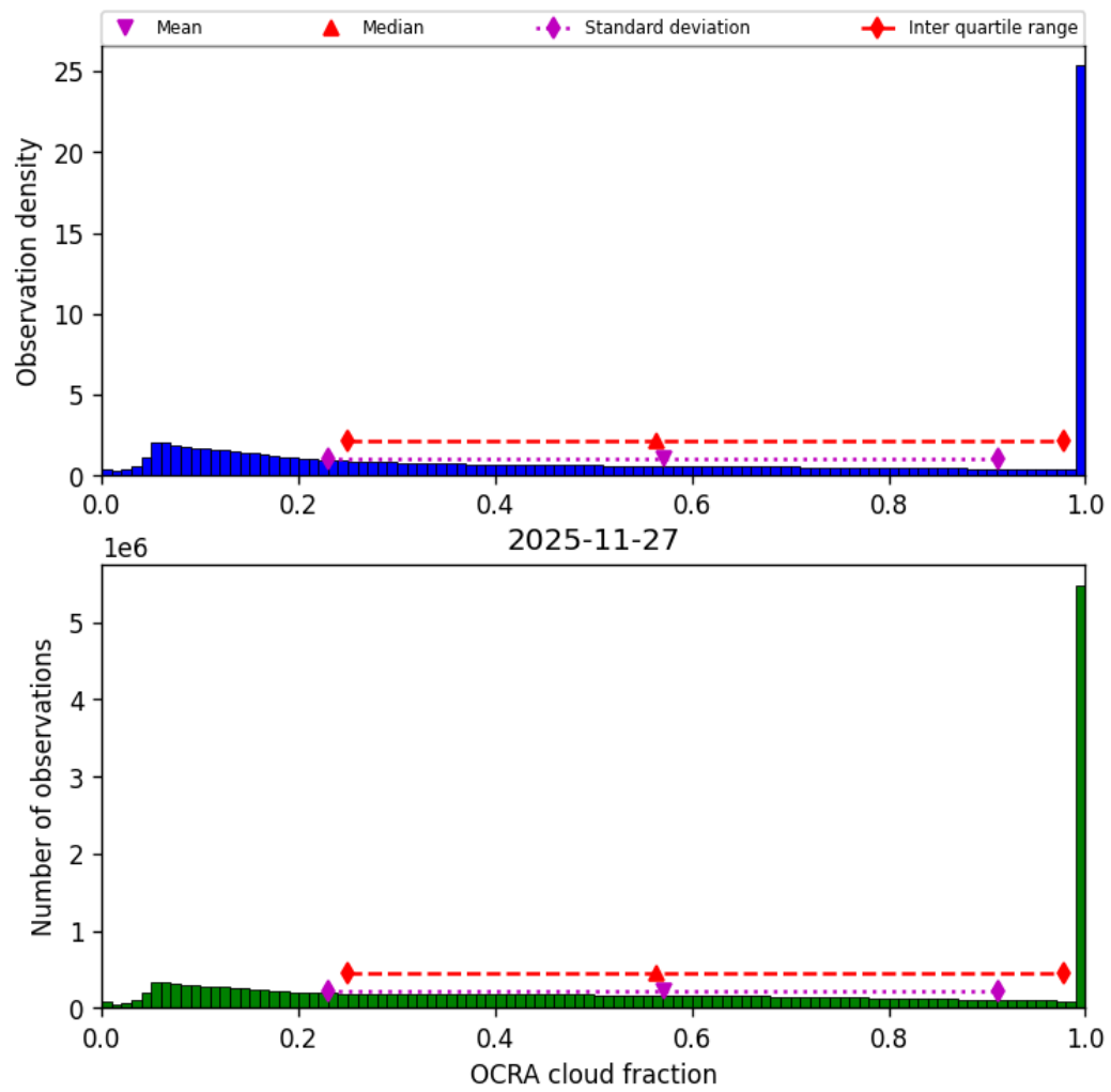
Figure 50: Histogram of “OCRA cloud fraction” for 2025-11-26 to 2025-11-28
