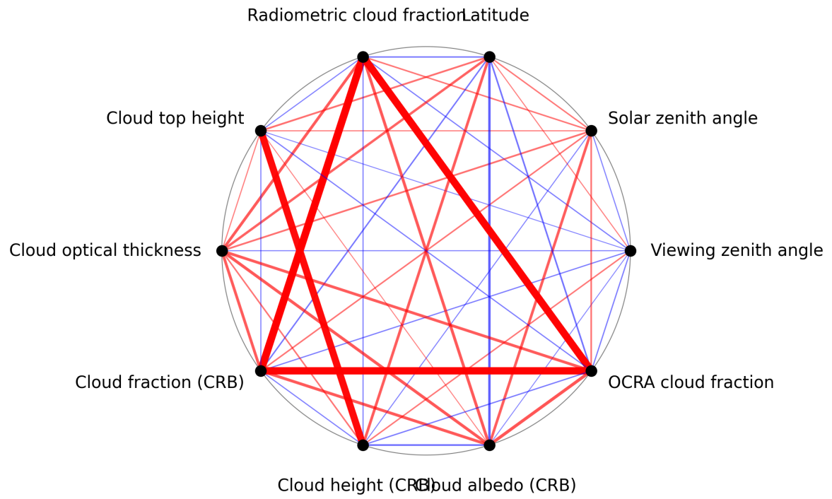
Figure 1: Map of correlation graph for 2025-11-26 to 2025-11-28.
