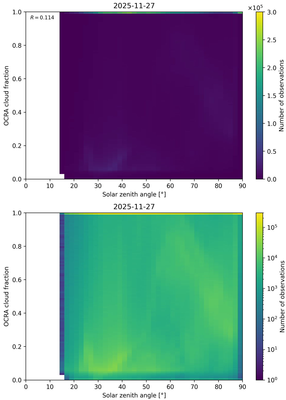
Figure 100: Scatter density plot of “Solar zenith angle” against “OCRA cloud fraction” for 2025-11-26 to 2025-11-28.
