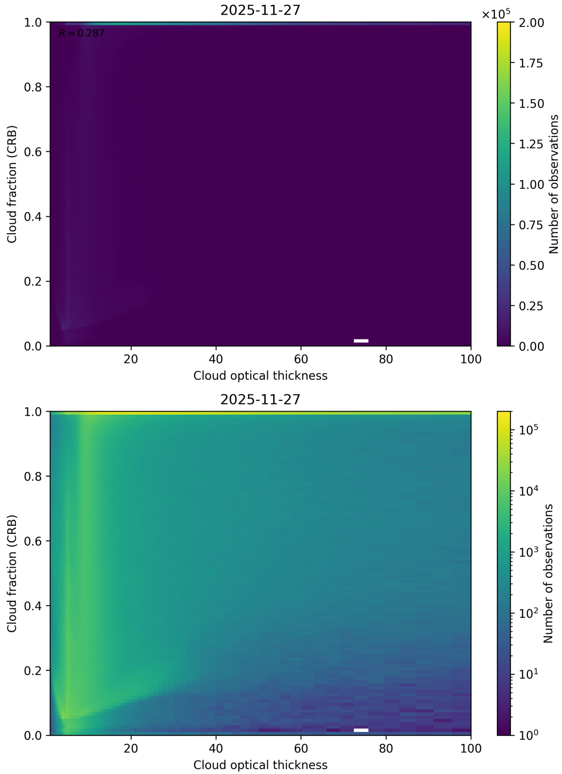
Figure 84: Scatter density plot of “Cloud optical thickness” against “Cloud fraction (CRB)” for 2025-11-26 to 2025-11-28.
