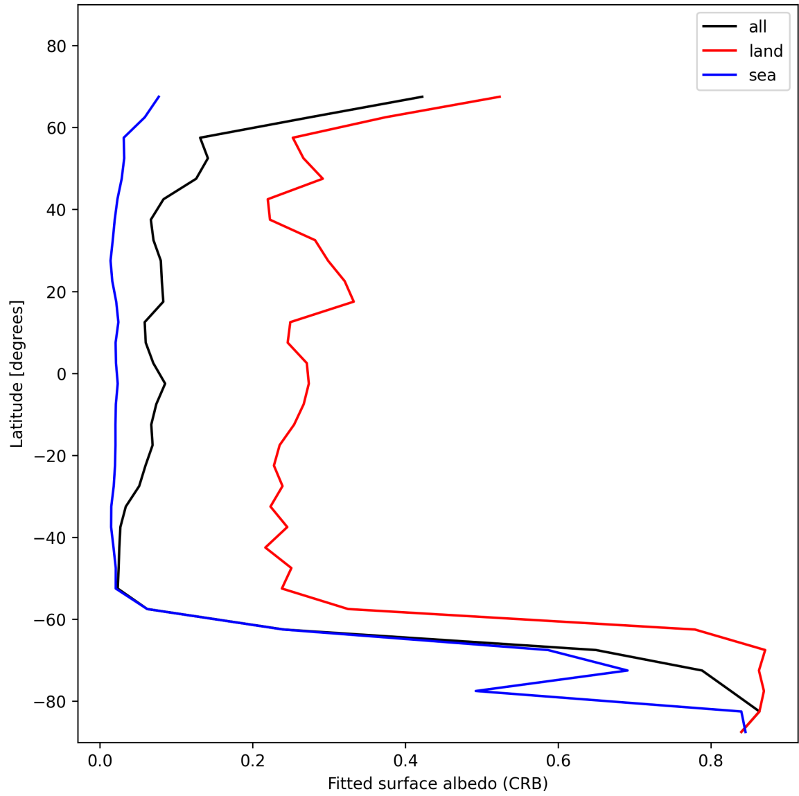
Figure 30: Zonal average of “Fitted surface albedo (CRB)” for 2025-11-26 to 2025-11-28.
