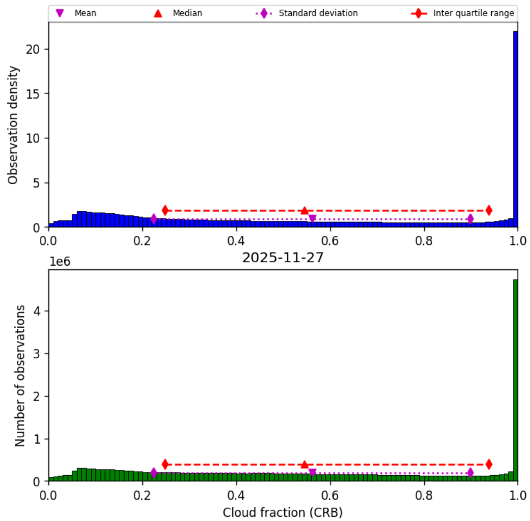
Figure 42: Histogram of “Cloud fraction (CRB)” for 2025-11-26 to 2025-11-28
