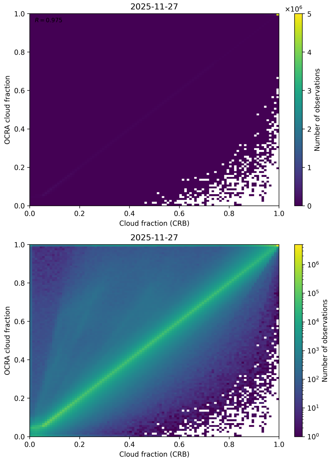
Figure 78: Scatter density plot of “Cloud fraction (CRB)” against “OCRA cloud fraction” for 2025-11-26 to 2025-11-28.
