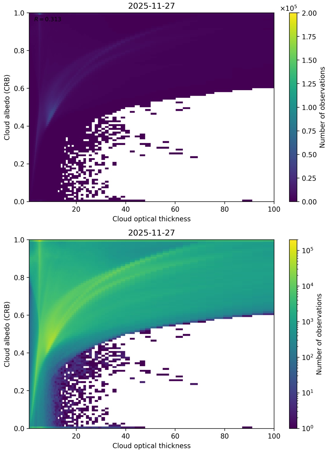
Figure 82: Scatter density plot of “Cloud optical thickness” against “Cloud albedo (CRB)” for 2025-11-26 to 2025-11-28.
