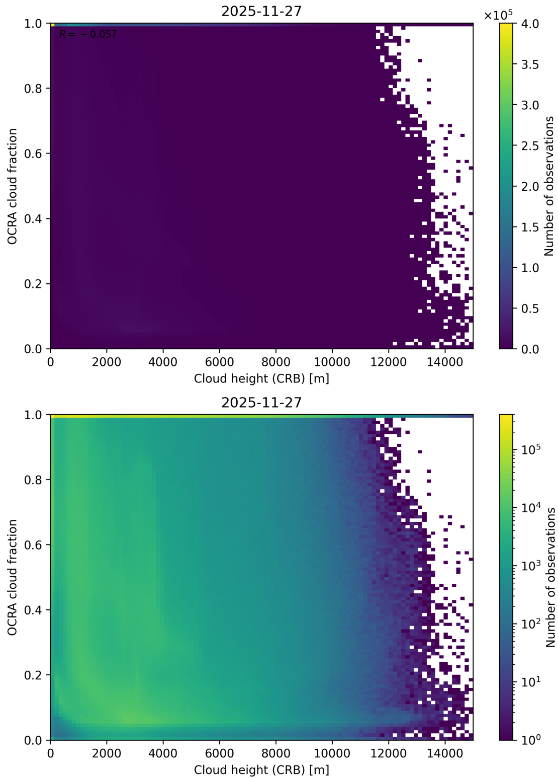
Figure 81: Scatter density plot of “Cloud height (CRB)” against “OCRA cloud fraction” for 2025-11-26 to 2025-11-28.
