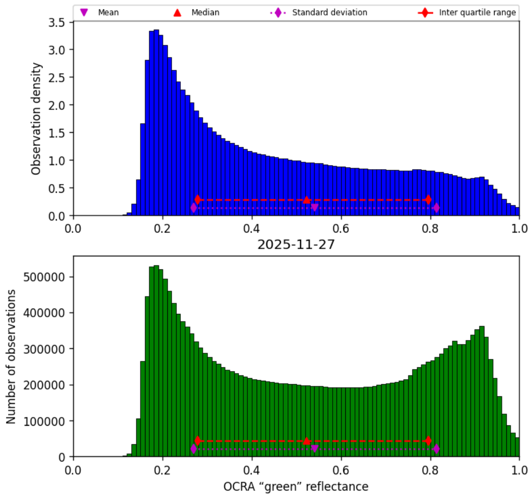
Figure 52: Histogram of “OCRA “green” reflectance” for 2025-11-26 to 2025-11-28
