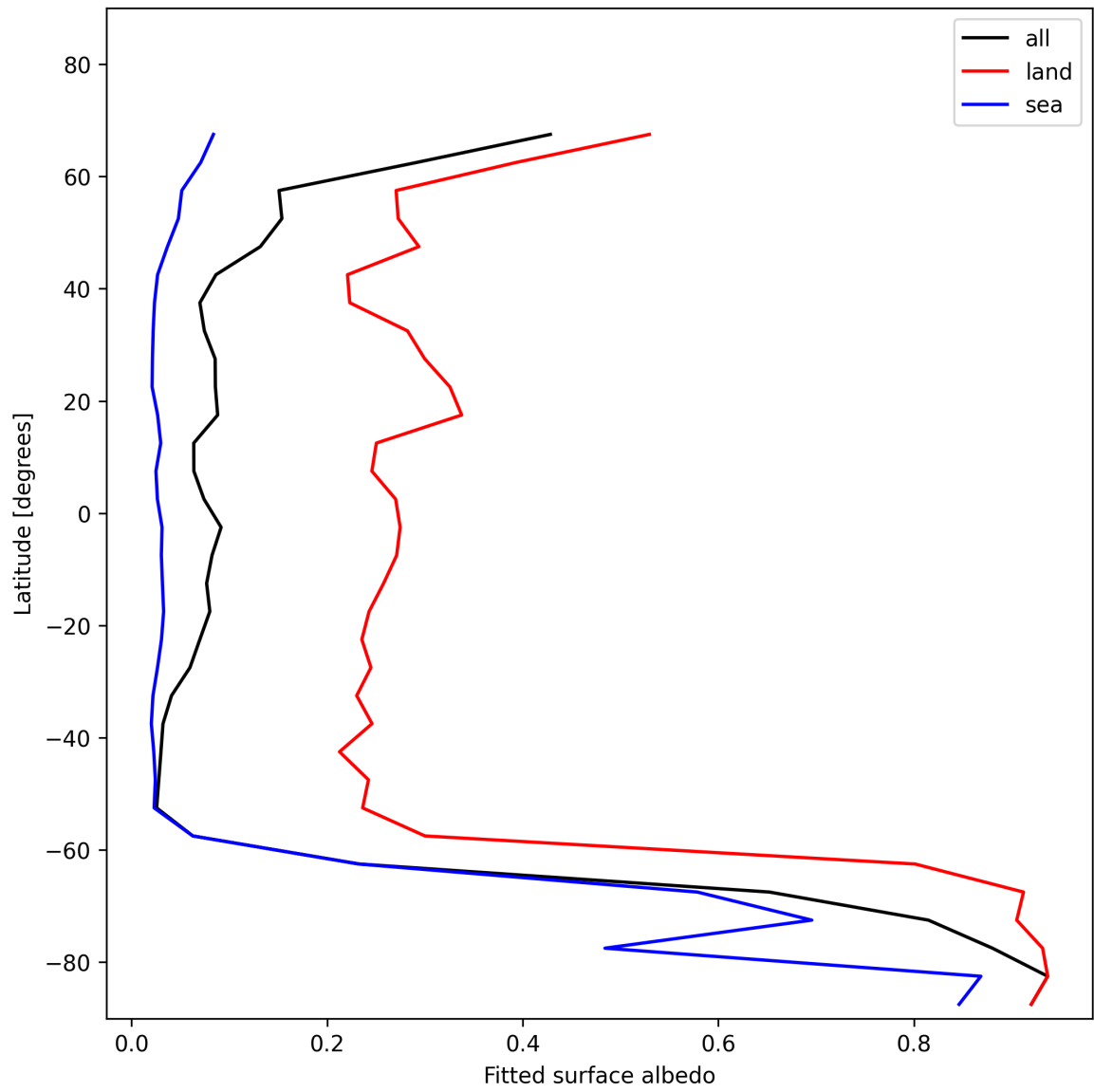
Figure 29: Zonal average of “Fitted surface albedo” for 2025-11-26 to 2025-11-28.
