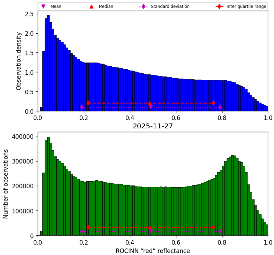
Figure 53: Histogram of “ROCINN “red” reflectance” for 2025-11-26 to 2025-11-28
