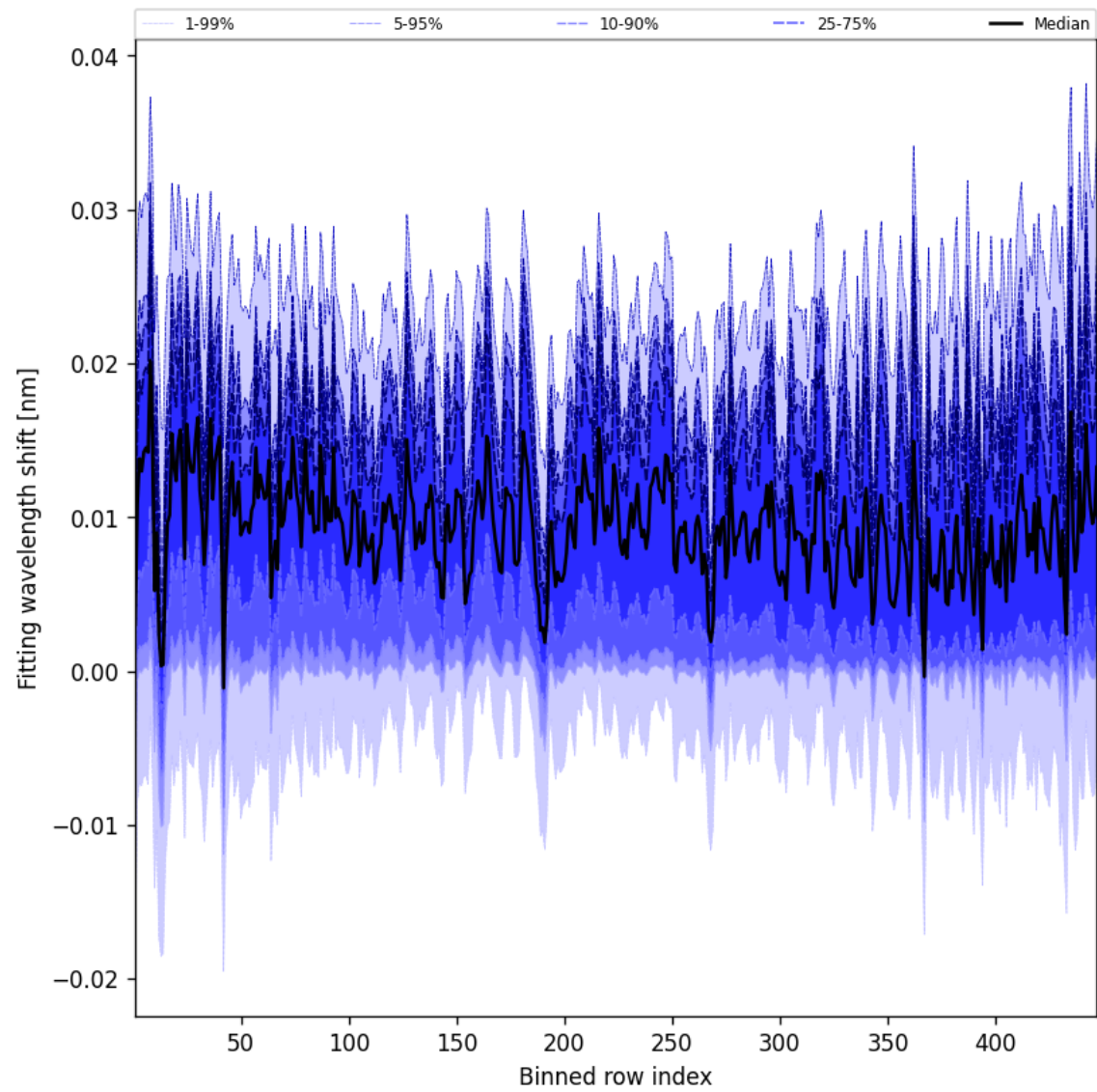
Figure 65: Along track statistics of “Fitting wavelength shift” for 2025-11-26 to 2025-11-28
