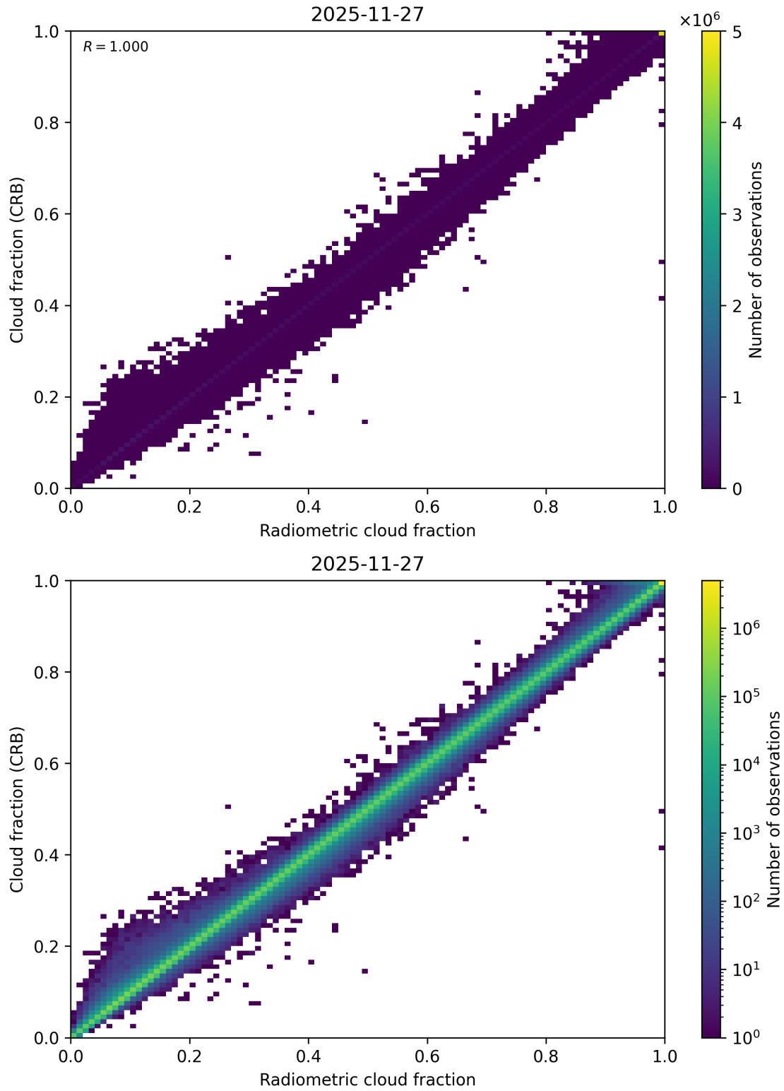
Figure 73: Scatter density plot of “Radiometric cloud fraction” against “Cloud fraction (CRB)” for 2025-11-26 to 2025-11-28.
