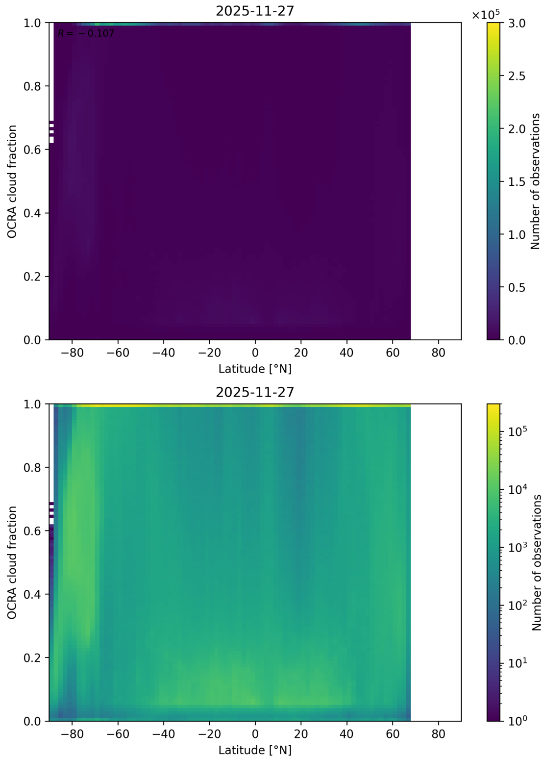
Figure 93: Scatter density plot of “Latitude” against “OCRA cloud fraction” for 2025-11-26 to 2025-11-28.
