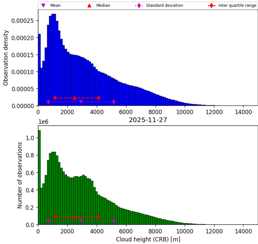
Figure 43: Histogram of “Cloud height (CRB)” for 2025-11-26 to 2025-11-28
