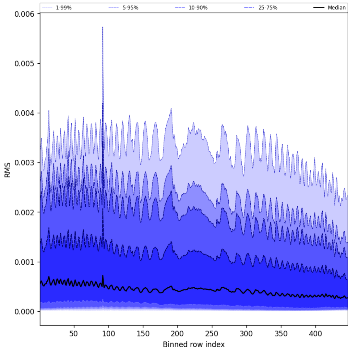
Figure 63: Along track statistics of “RMS” for 2025-11-26 to 2025-11-28
