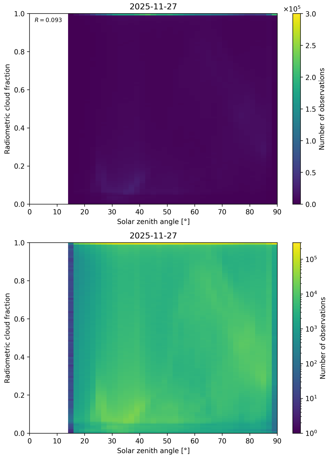
Figure 99: Scatter density plot of “Solar zenith angle” against “Radiometric cloud fraction” for 2025-11-26 to 2025-11-28.
