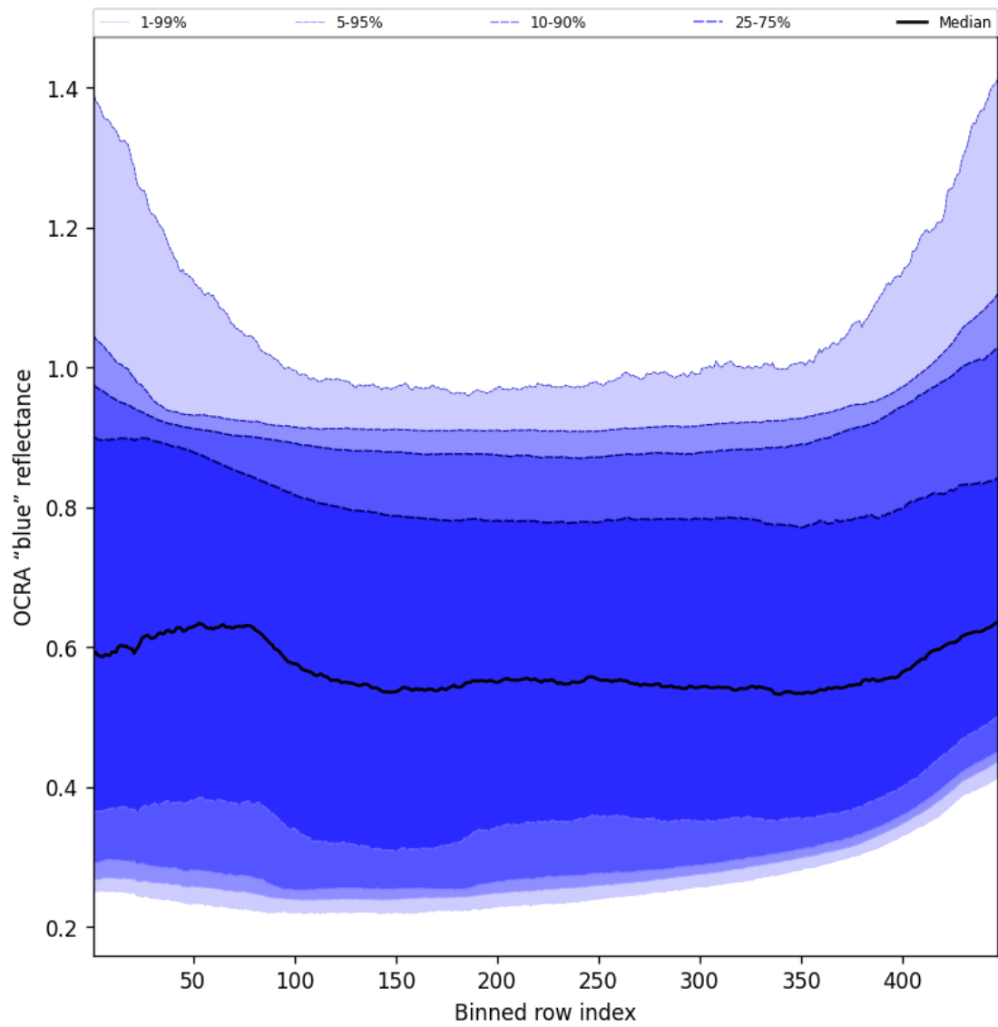
Figure 67: Along track statistics of “OCRA “blue” reflectance” for 2025-11-26 to 2025-11-28
