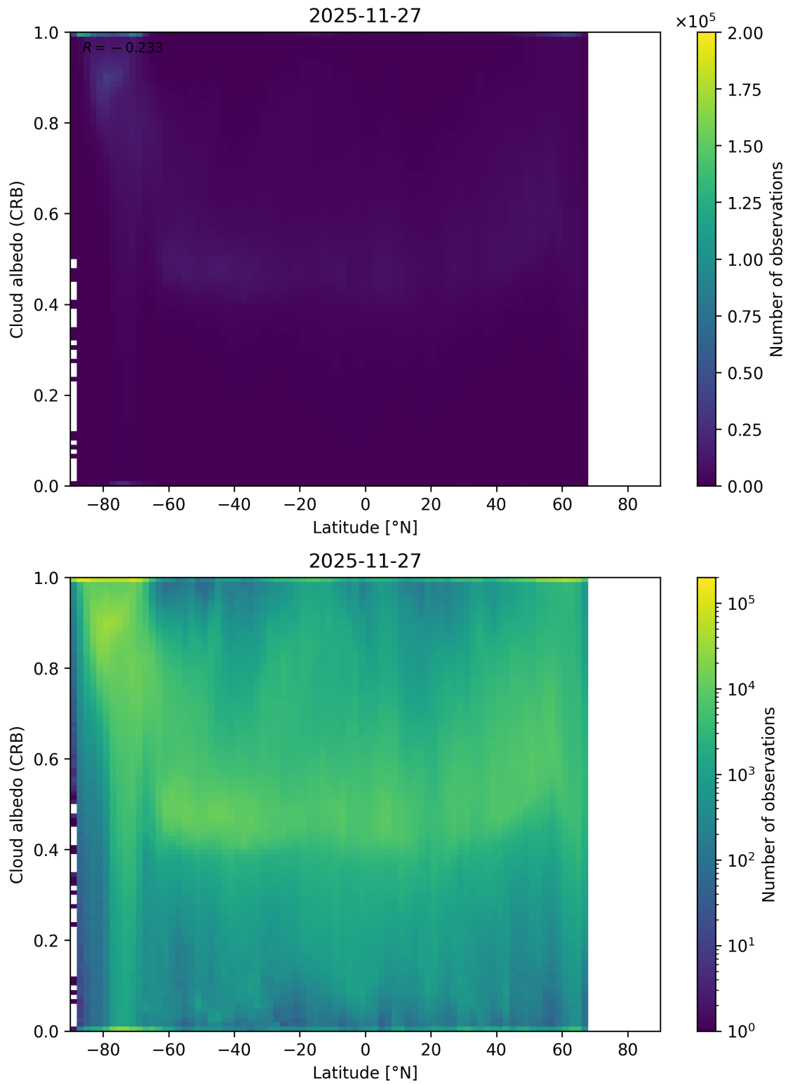
Figure 91: Scatter density plot of “Latitude” against “Cloud albedo (CRB)” for 2025-11-26 to 2025-11-28.
