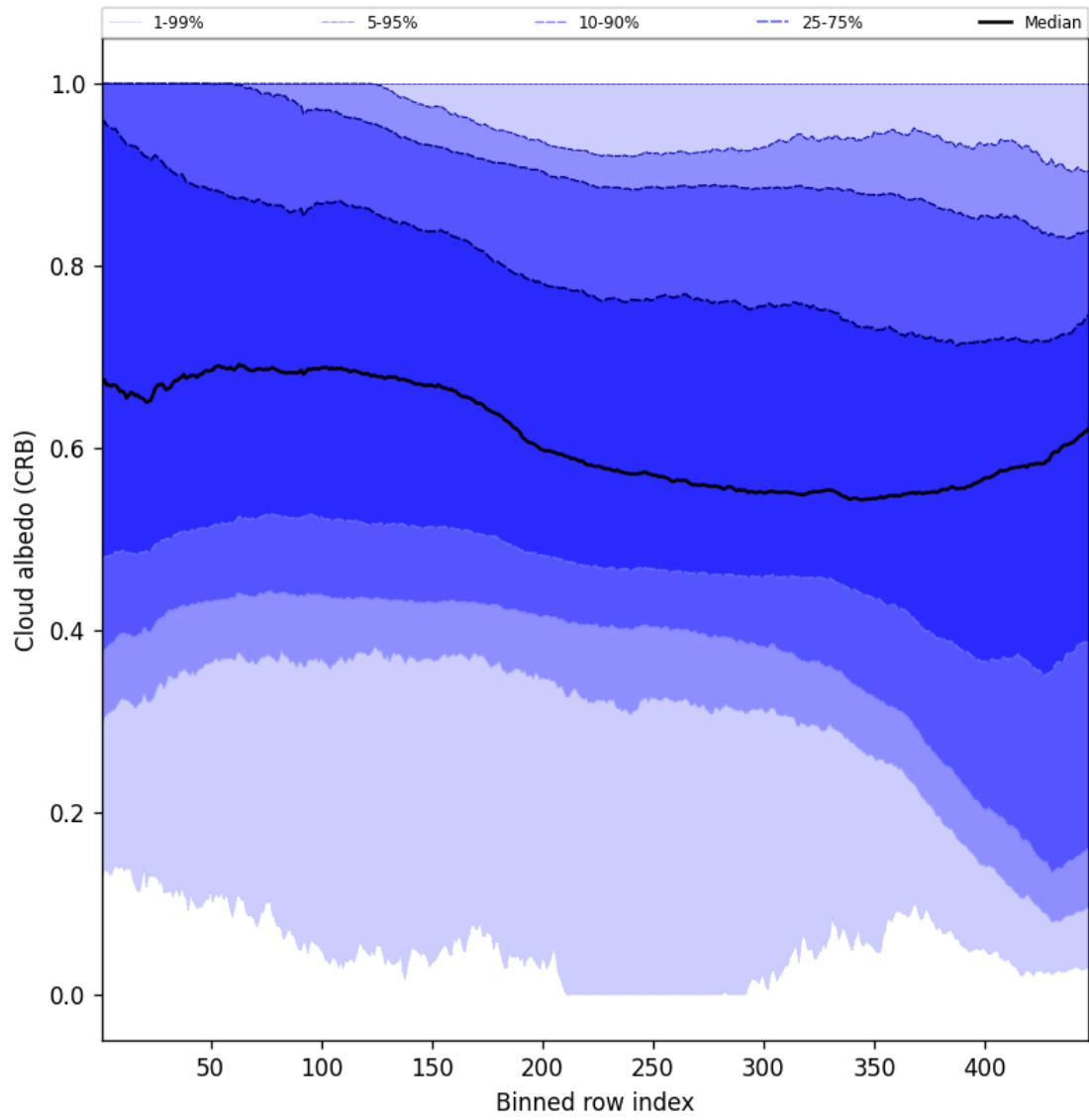
Figure 60: Along track statistics of “Cloud albedo (CRB)” for 2025-11-26 to 2025-11-28
