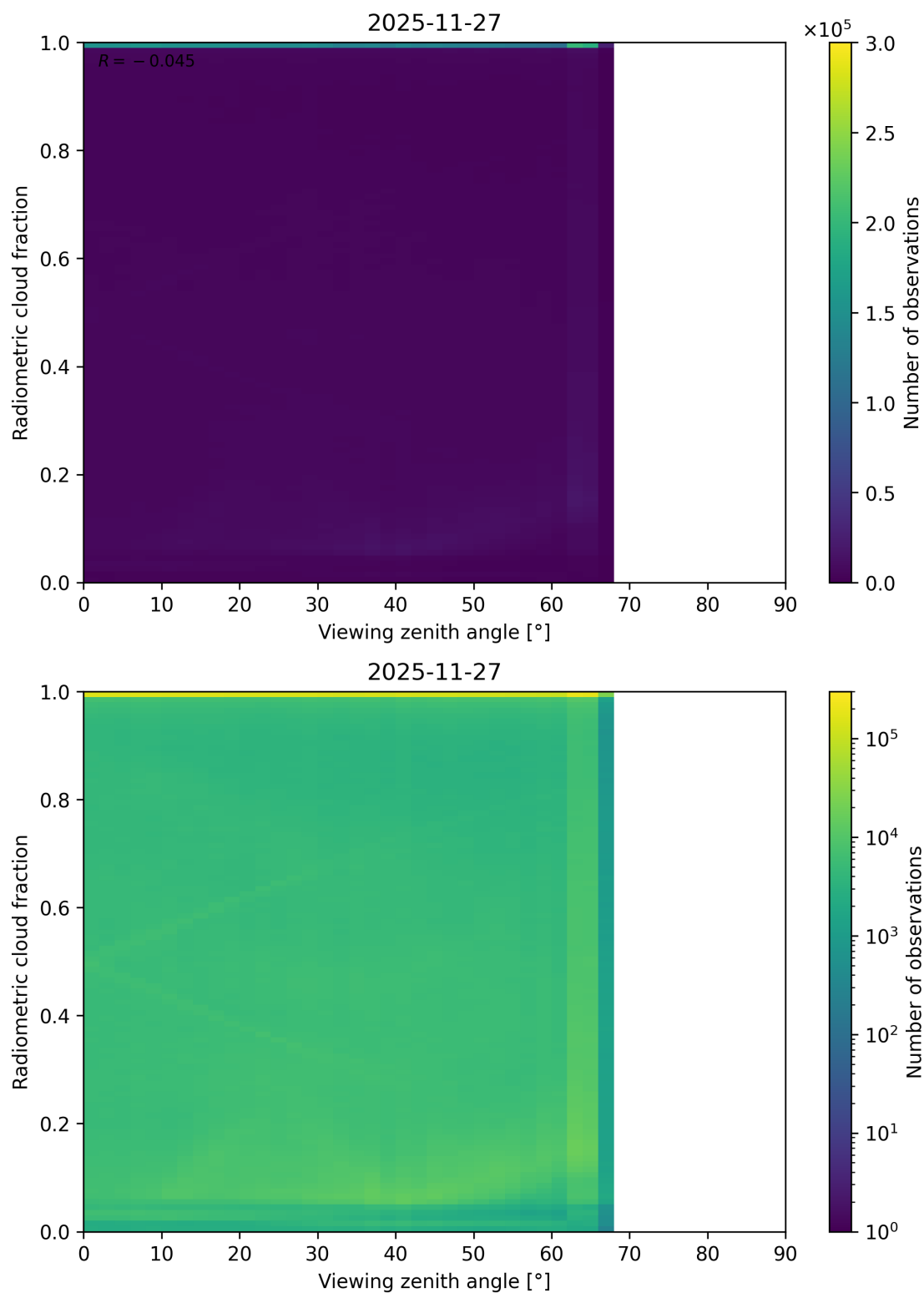
Figure 107: Scatter density plot of “Viewing zenith angle” against “Radiometric cloud fraction” for 2025-11-26 to 2025-11-28.
