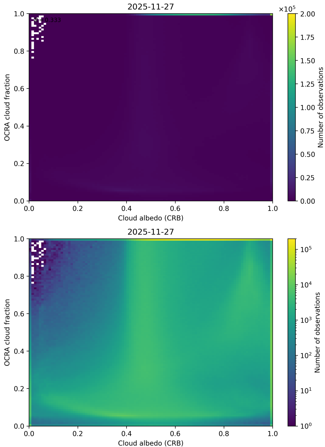
Figure 70: Scatter density plot of “Cloud albedo (CRB)” against “OCRA cloud fraction” for 2025-11-26 to 2025-11-28.
