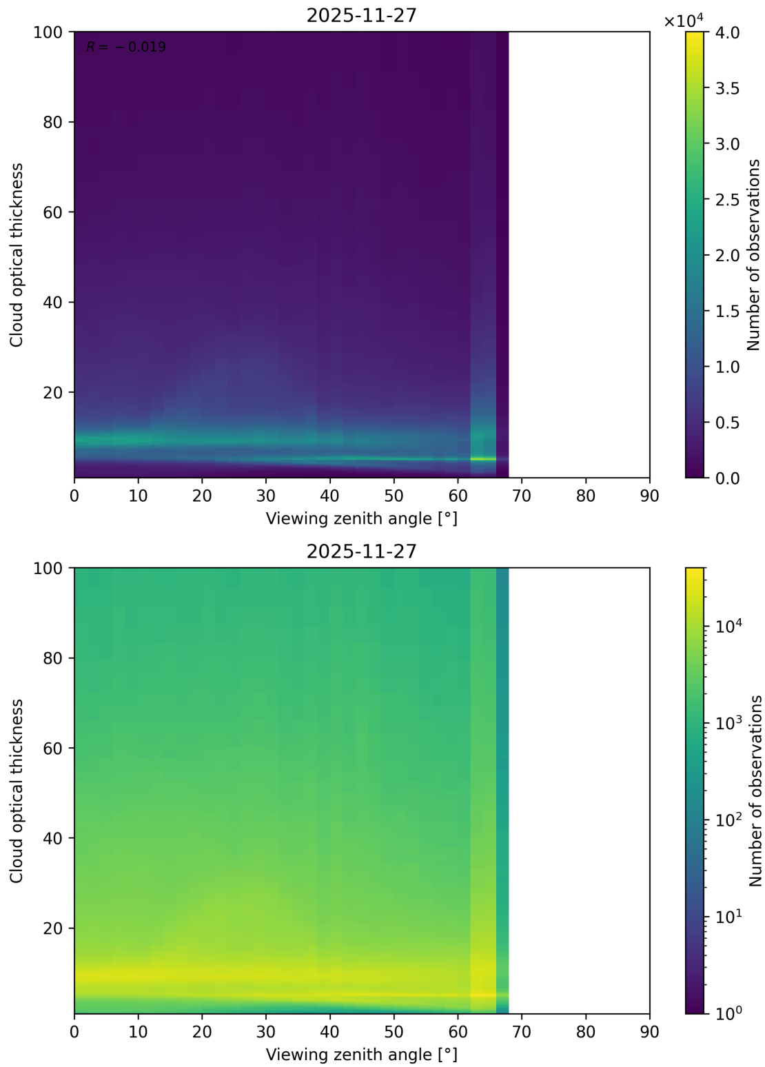
Figure 111: Scatter density plot of “Viewing zenith angle” against “Cloud optical thickness” for 2025-11-26 to 2025-11-28.
