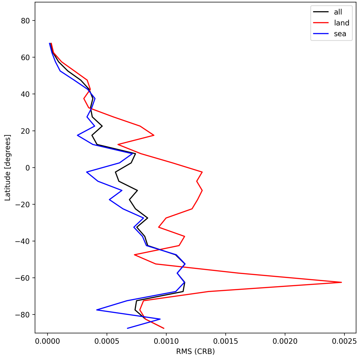
Figure 32: Zonal average of “RMS (CRB)” for 2025-11-26 to 2025-11-28.
