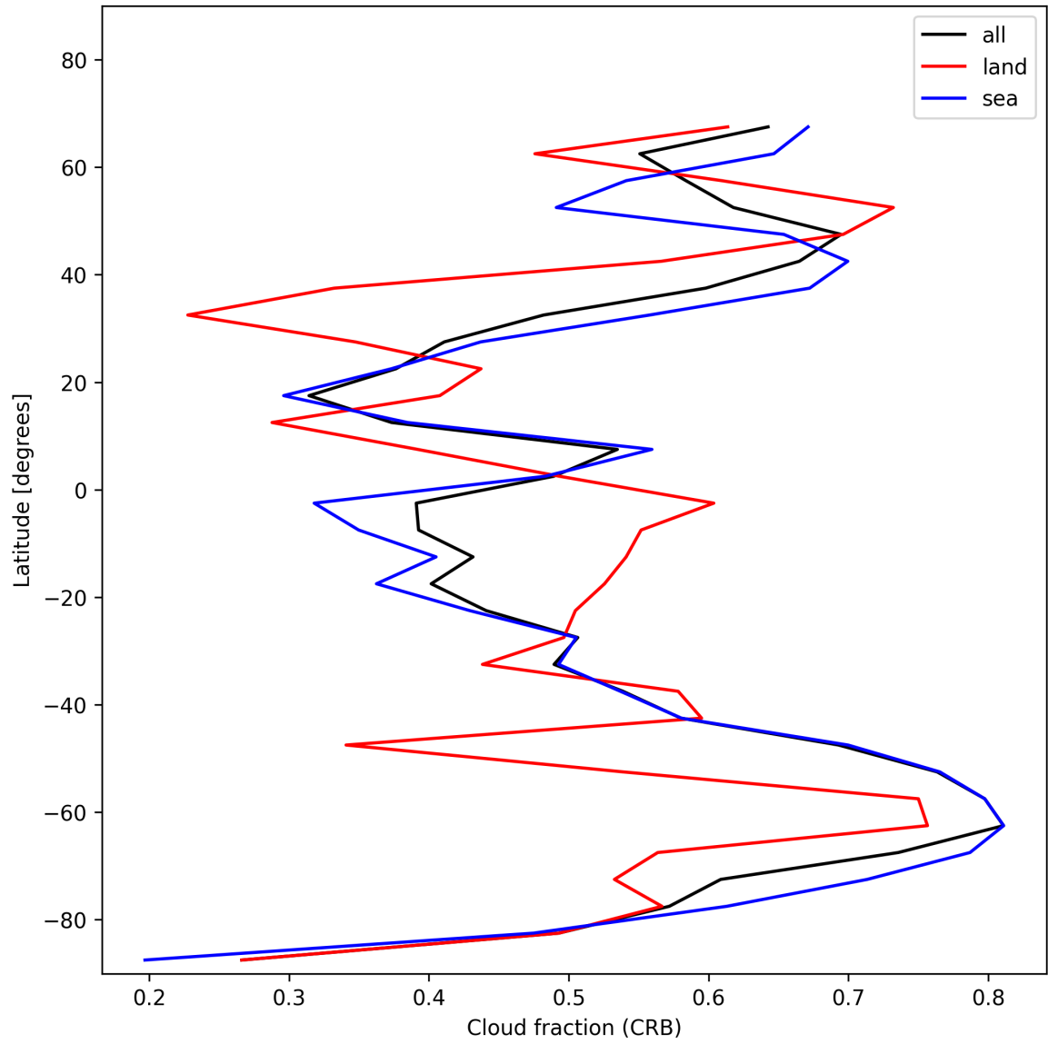
Figure 26: Zonal average of “Cloud fraction (CRB)” for 2025-11-26 to 2025-11-28.
