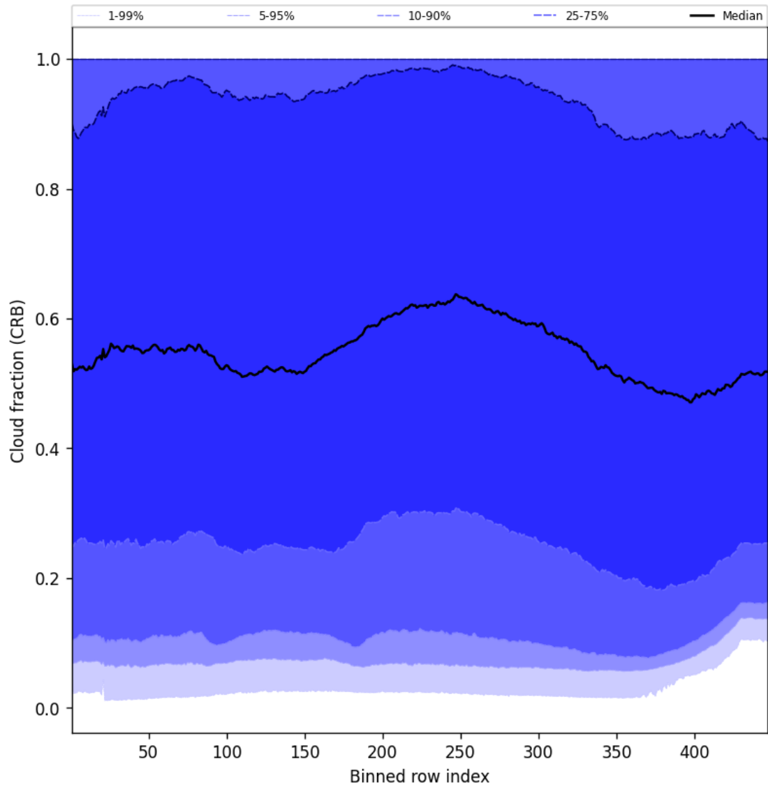
Figure 58: Along track statistics of “Cloud fraction (CRB)” for 2025-11-26 to 2025-11-28
