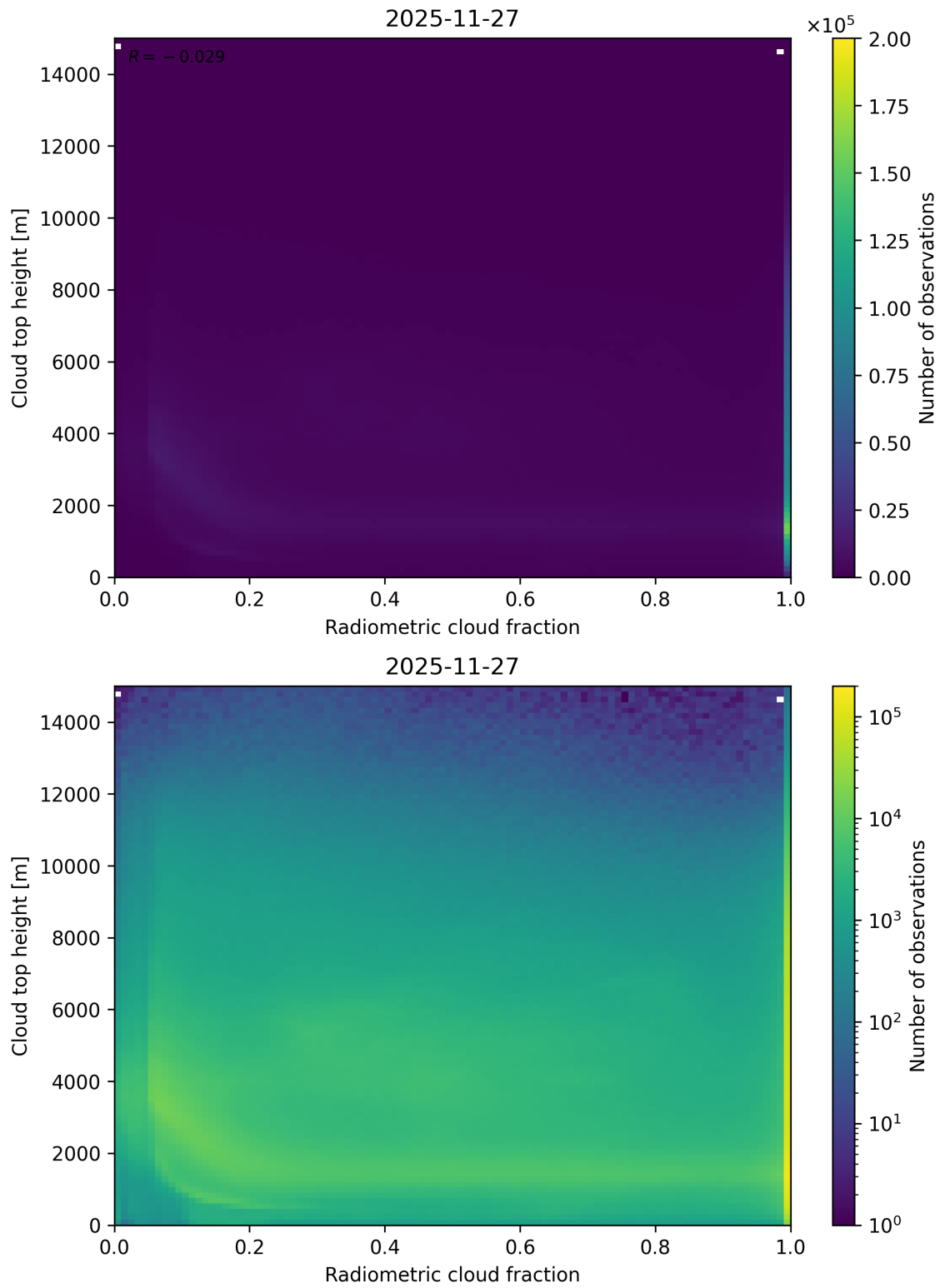
Figure 76: Scatter density plot of “Radiometric cloud fraction” against “Cloud top height” for 2025-11-26 to 2025-11-28.
