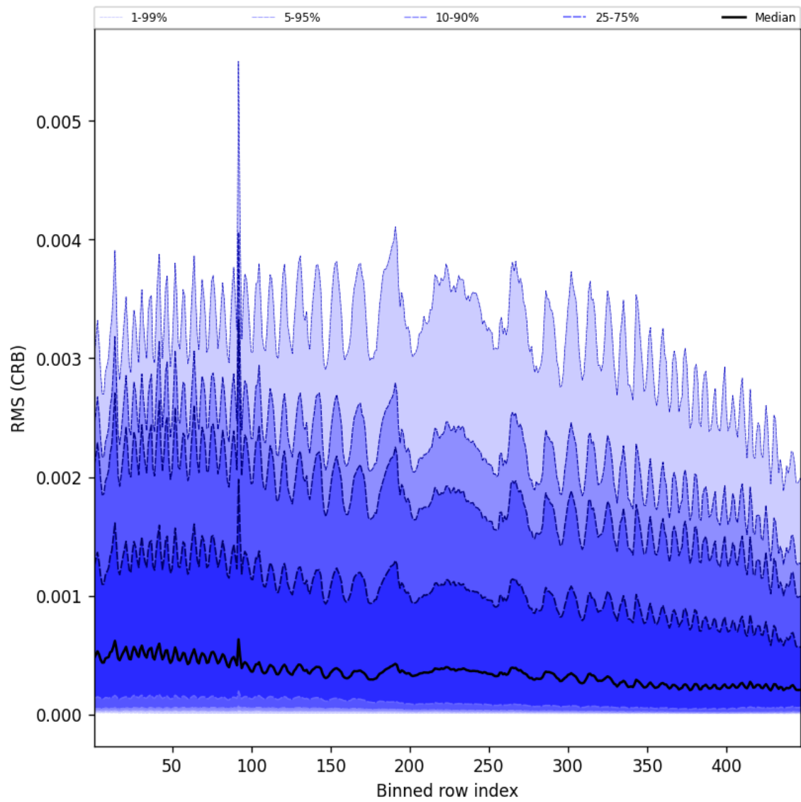
Figure 64: Along track statistics of “RMS (CRB)” for 2025-11-26 to 2025-11-28
