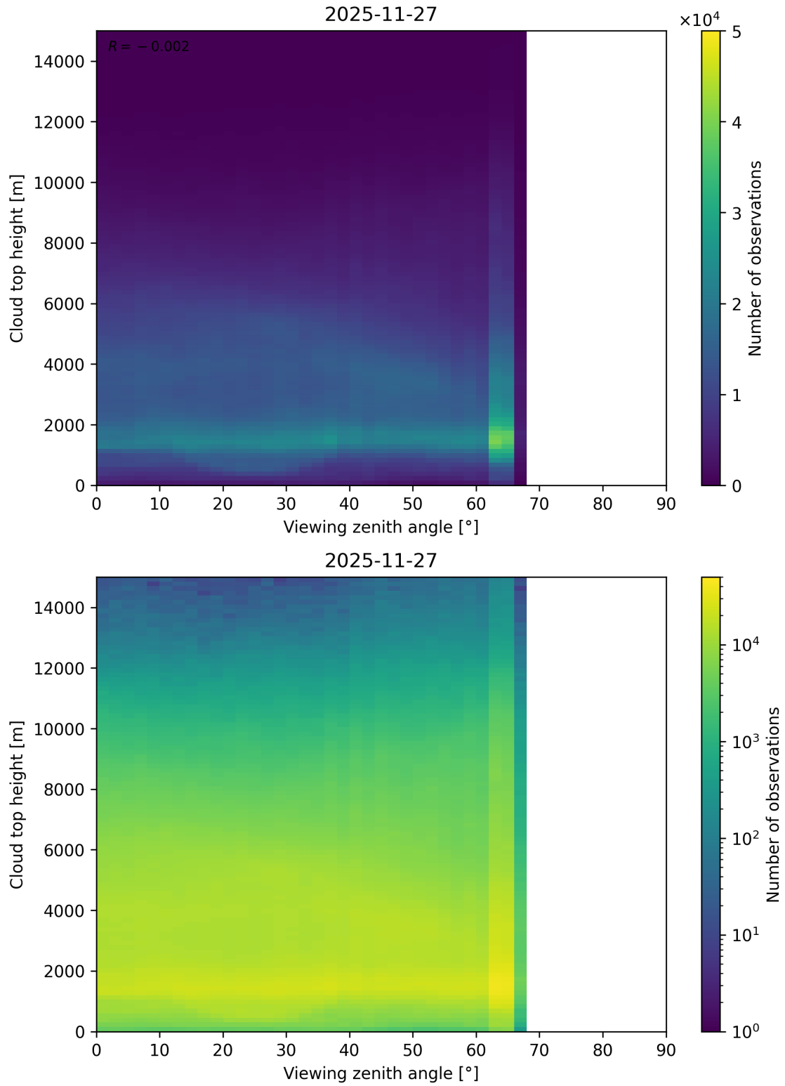
Figure 112: Scatter density plot of “Viewing zenith angle” against “Cloud top height” for 2025-11-26 to 2025-11-28.
