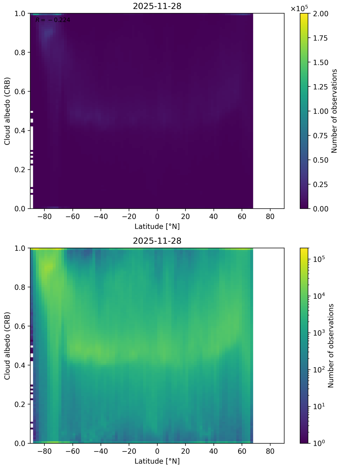
Figure 91: Scatter density plot of “Latitude” against “Cloud albedo (CRB)” for 2025-11-28 to 2025-11-29.
