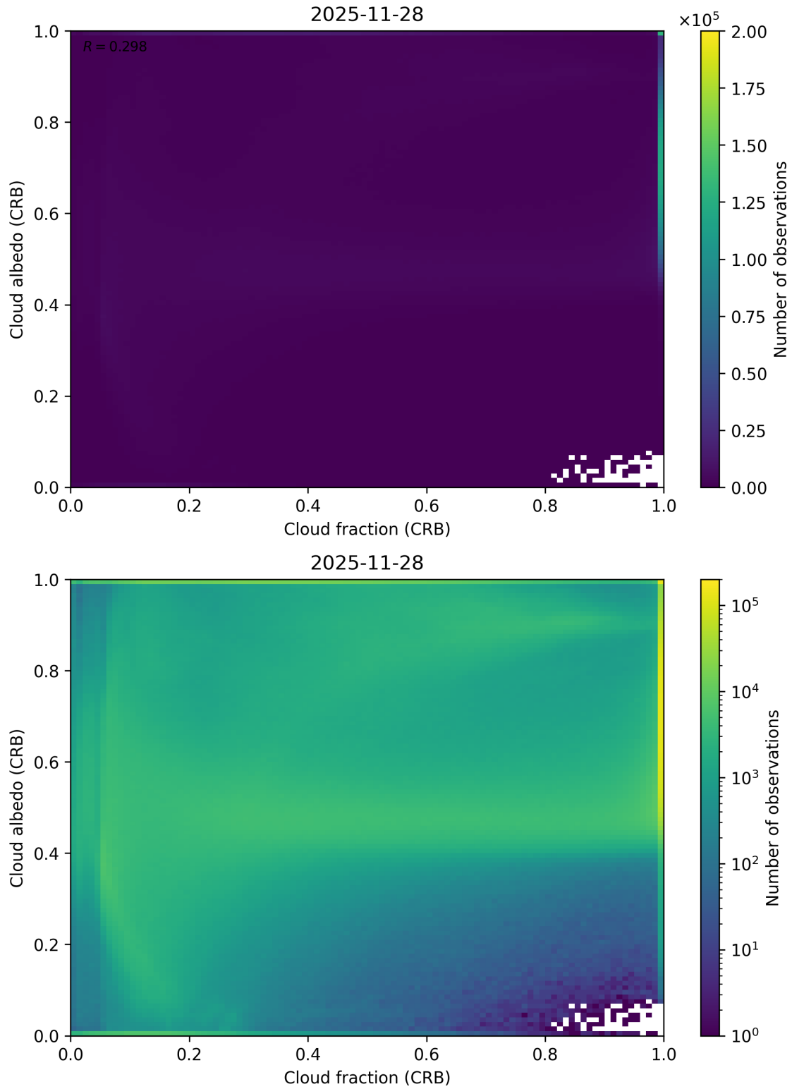
Figure 77: Scatter density plot of “Cloud fraction (CRB)” against “Cloud albedo (CRB)” for 2025-11-28 to 2025-11-29.
