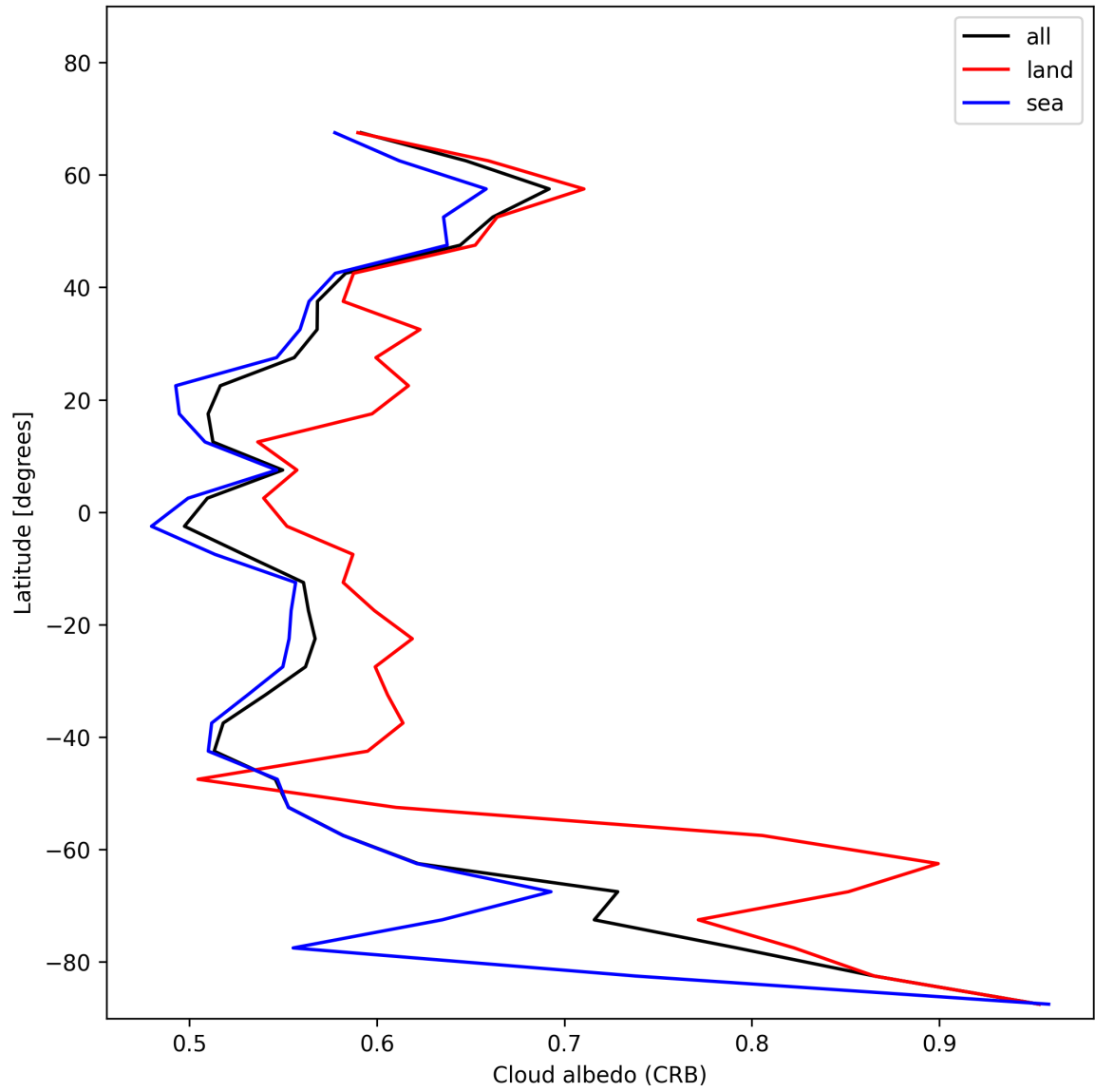
Figure 28: Zonal average of “Cloud albedo (CRB)” for 2025-11-28 to 2025-11-29.
