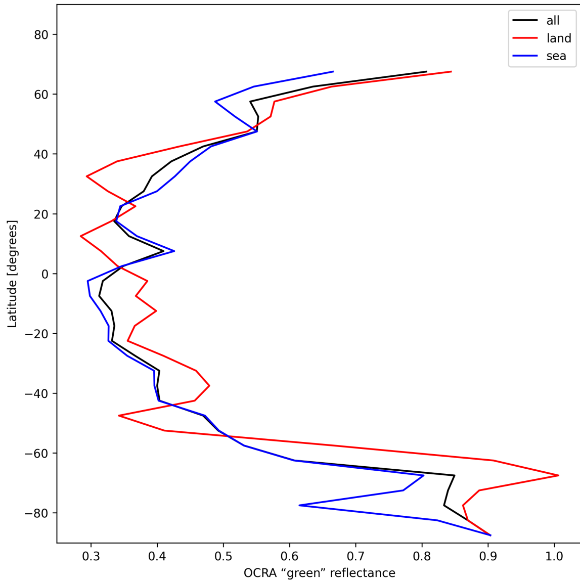
Figure 36: Zonal average of “OCRA “green” reflectance” for 2025-11-28 to 2025-11-29.
