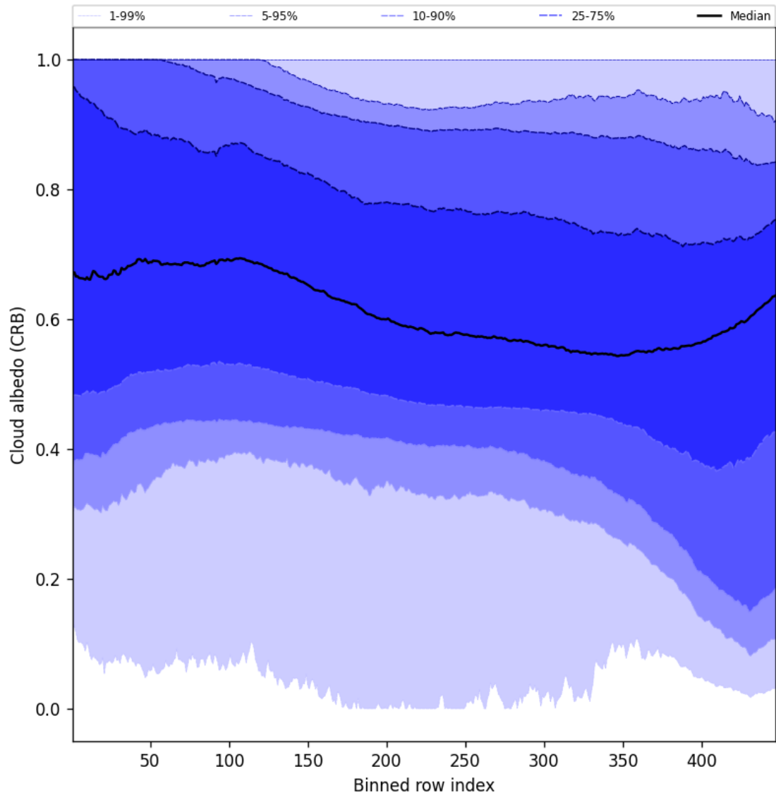
Figure 60: Along track statistics of “Cloud albedo (CRB)” for 2025-11-28 to 2025-11-29
