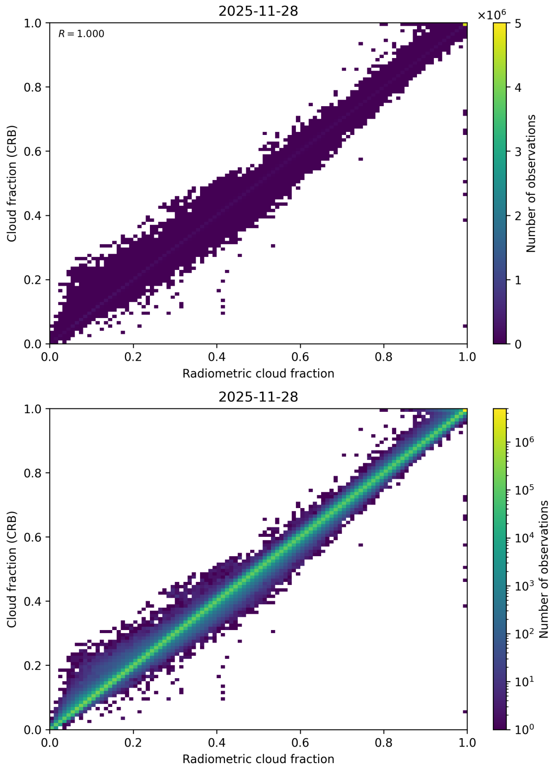
Figure 73: Scatter density plot of “Radiometric cloud fraction” against “Cloud fraction (CRB)” for 2025-11-28 to 2025-11-29.
