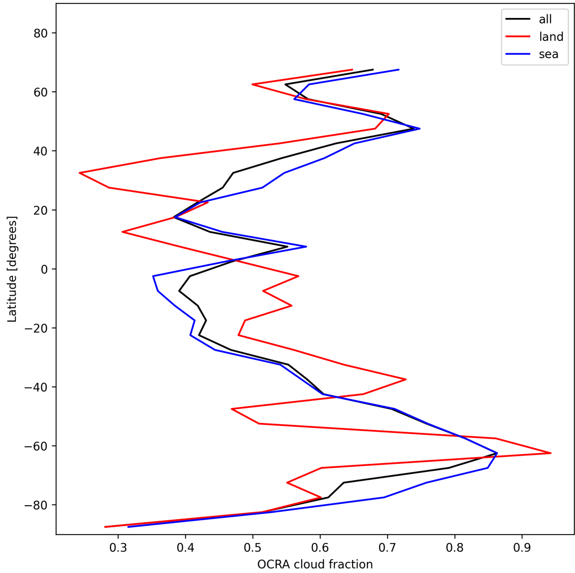
Figure 34: Zonal average of “OCRA cloud fraction” for 2025-11-28 to 2025-11-29.
