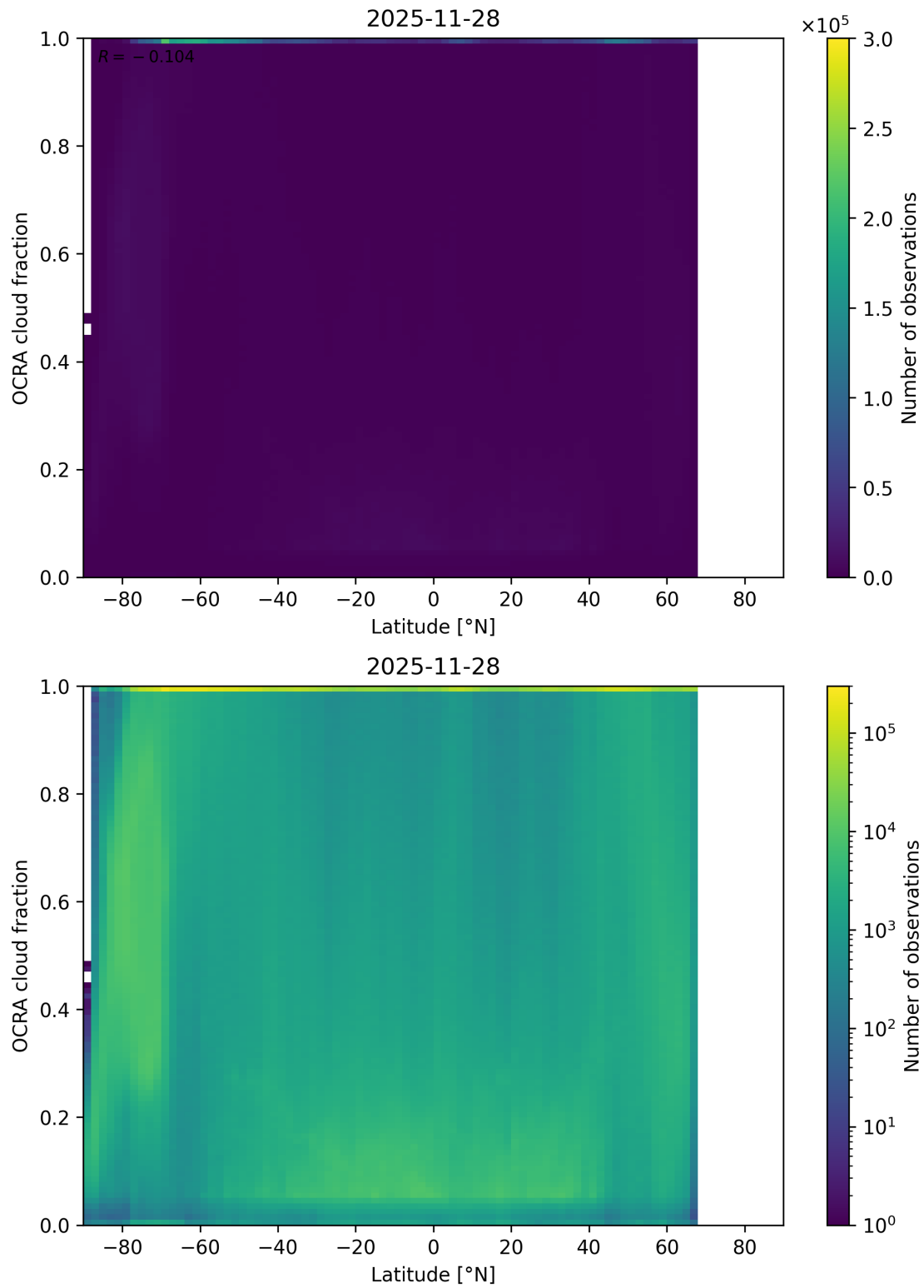
Figure 93: Scatter density plot of “Latitude” against “OCRA cloud fraction” for 2025-11-28 to 2025-11-29.
