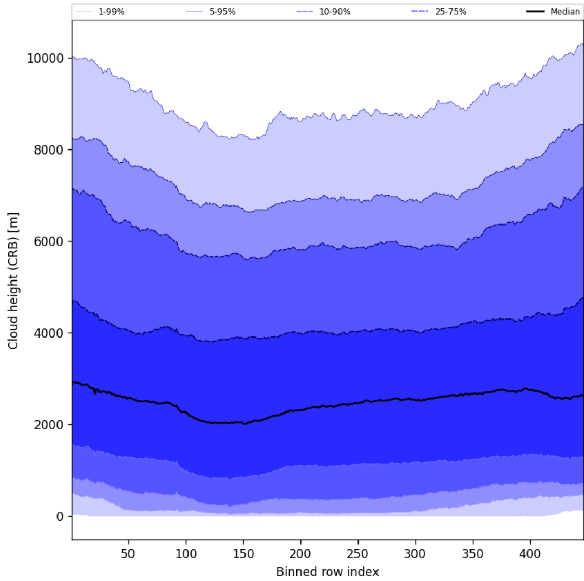
Figure 59: Along track statistics of “Cloud height (CRB)” for 2025-11-28 to 2025-11-29
