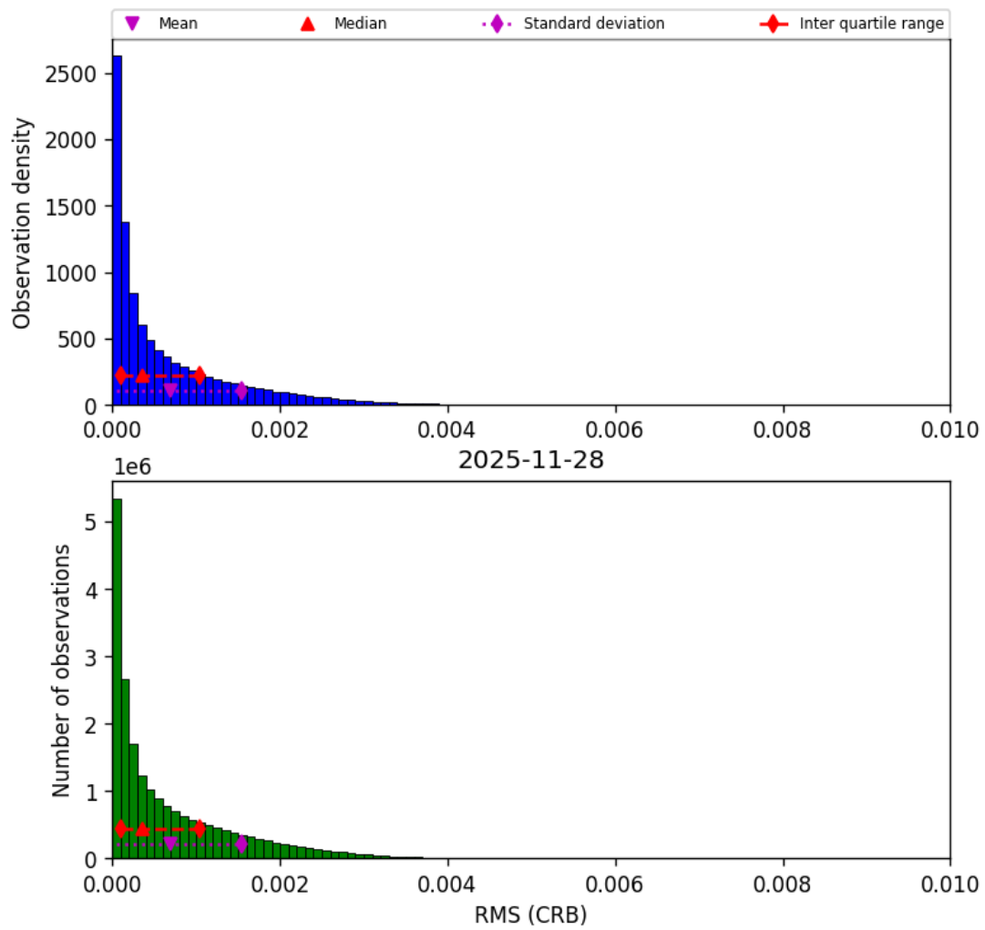
Figure 48: Histogram of "RMS (CRB)" for 2025-11-28 to 2025-11-29
