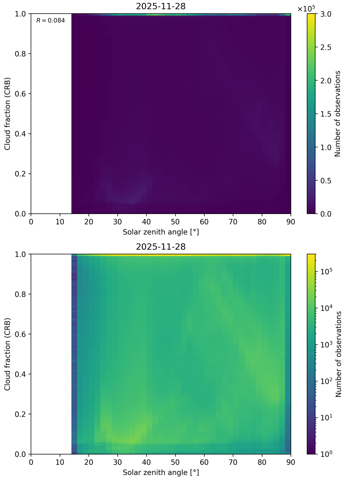
Figure 101: Scatter density plot of “Solar zenith angle” against “Cloud fraction (CRB)” for 2025-11-28 to 2025-11-29.
