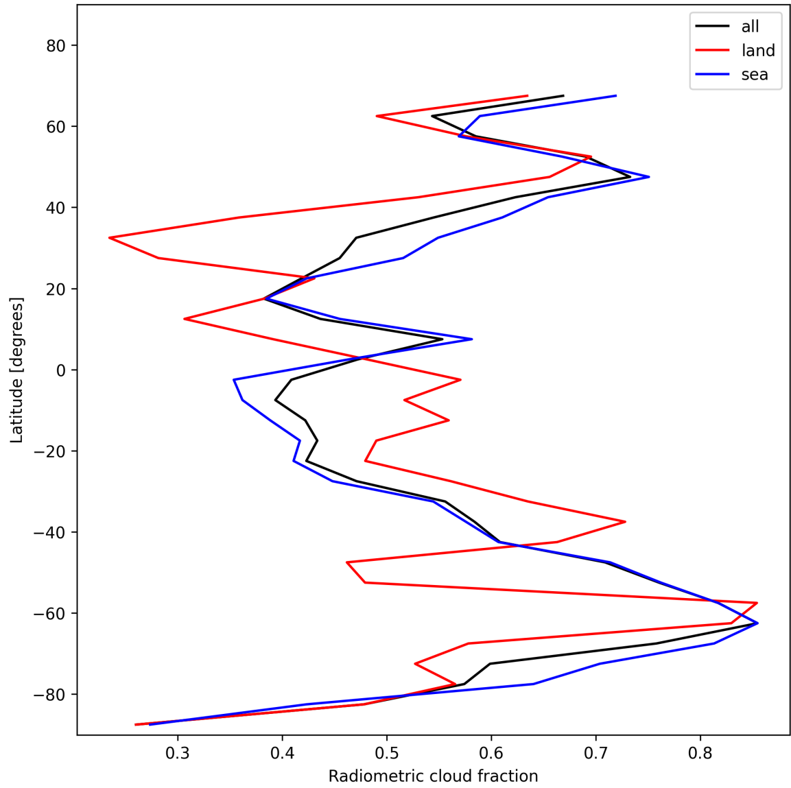
Figure 23: Zonal average of “Radiometric cloud fraction” for 2025-11-28 to 2025-11-29.
