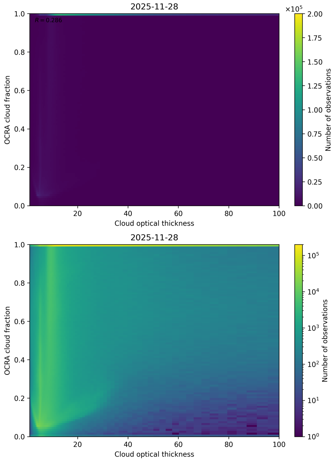
Figure 83: Scatter density plot of “Cloud optical thickness” against “OCRA cloud fraction” for 2025-11-28 to 2025-11-29.
