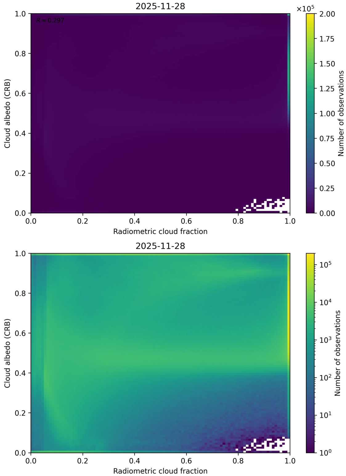
Figure 71: Scatter density plot of “Radiometric cloud fraction” against “Cloud albedo (CRB)” for 2025-11-28 to 2025-11-29.
