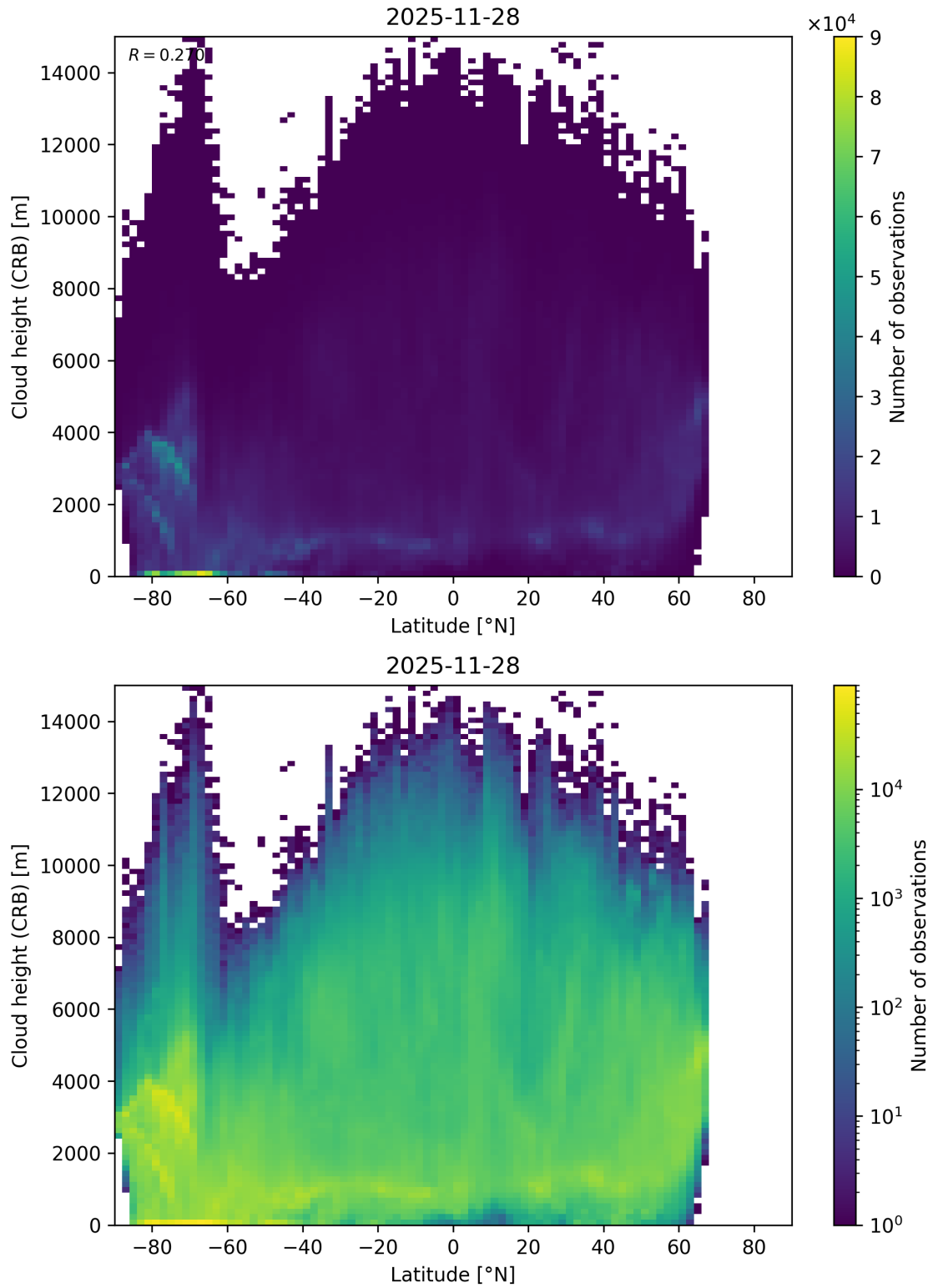
Figure 95: Scatter density plot of “Latitude” against “Cloud height (CRB)” for 2025-11-28 to 2025-11-29.
