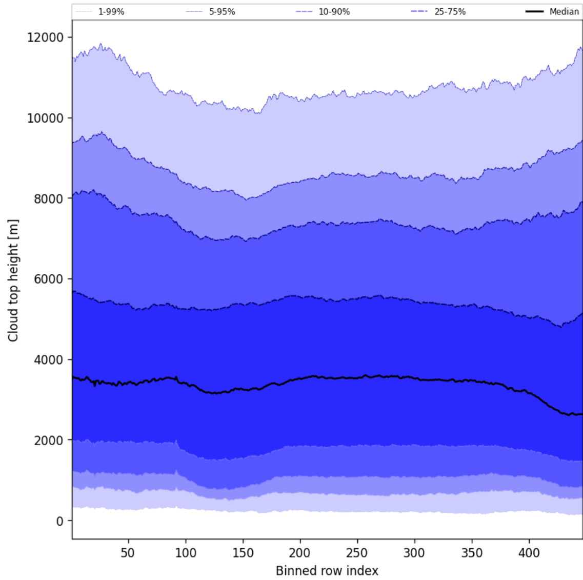
Figure 56: Along track statistics of “Cloud top height” for 2025-11-28 to 2025-11-29
