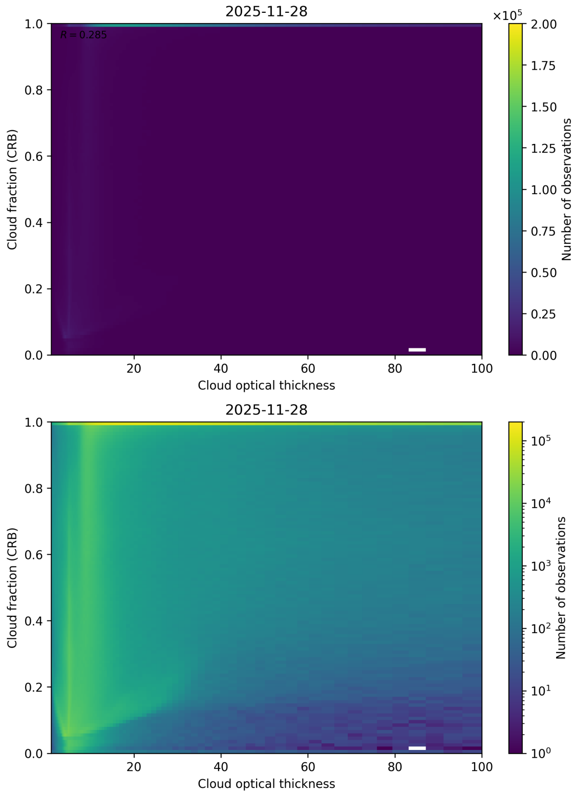
Figure 84: Scatter density plot of “Cloud optical thickness” against “Cloud fraction (CRB)” for 2025-11-28 to 2025-11-29.
