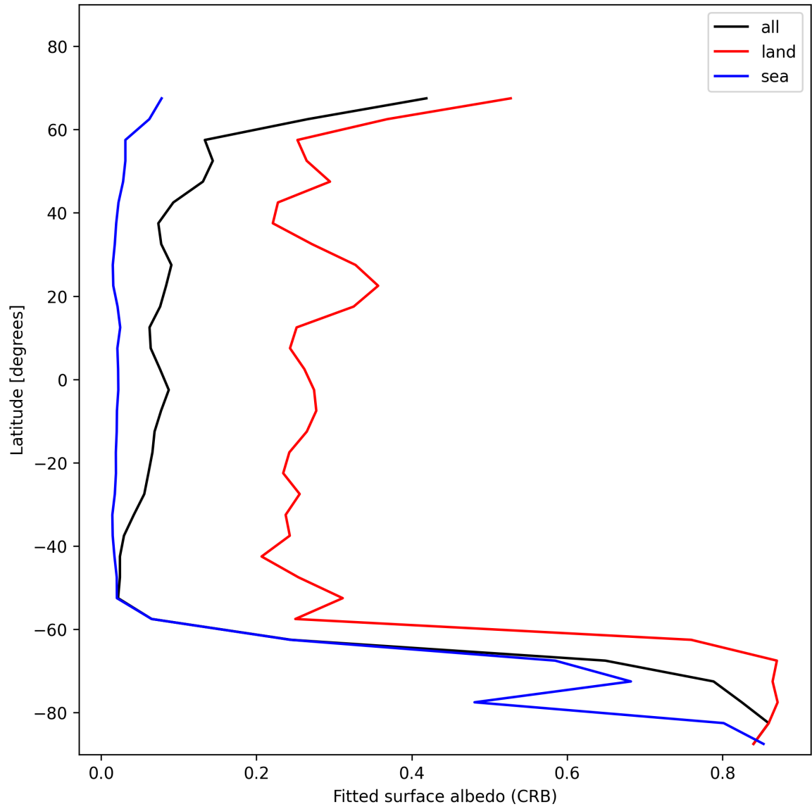
Figure 30: Zonal average of “Fitted surface albedo (CRB)” for 2025-11-28 to 2025-11-29.
