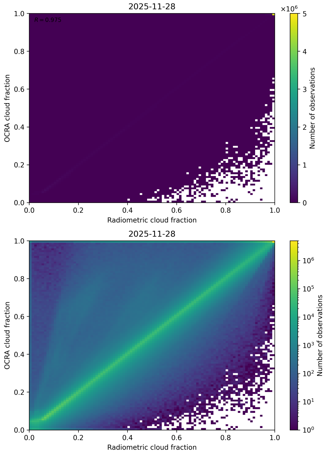
Figure 72: Scatter density plot of “Radiometric cloud fraction” against “OCRA cloud fraction” for 2025-11-28 to 2025-11-29.
