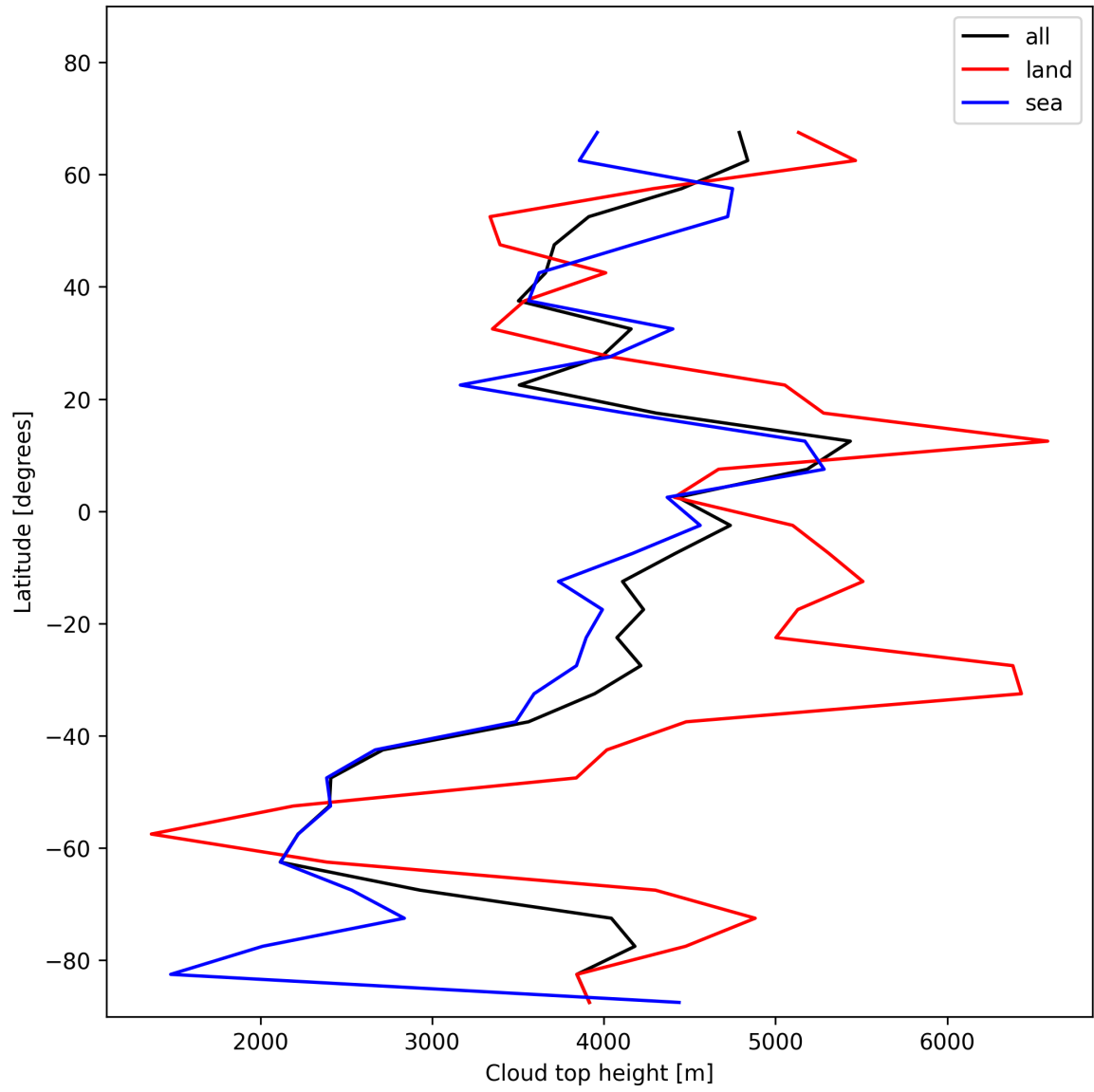
Figure 24: Zonal average of “Cloud top height” for 2025-11-28 to 2025-11-29.
