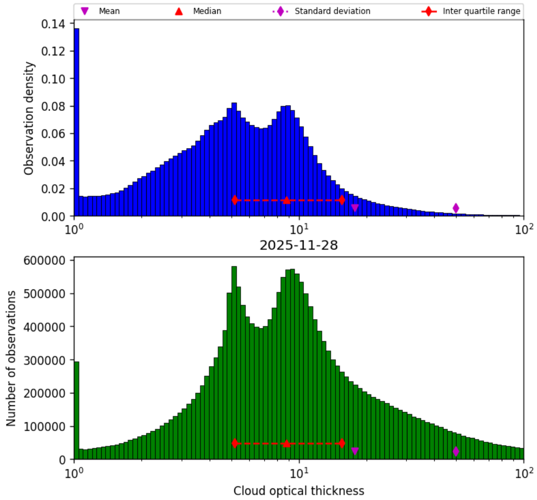
Figure 41: Histogram of “Cloud optical thickness” for 2025-11-28 to 2025-11-29
