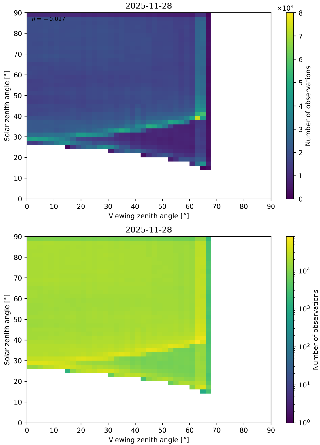
Figure 114: Scatter density plot of “Viewing zenith angle” against “Solar zenith angle” for 2025-11-28 to 2025-11-29.
