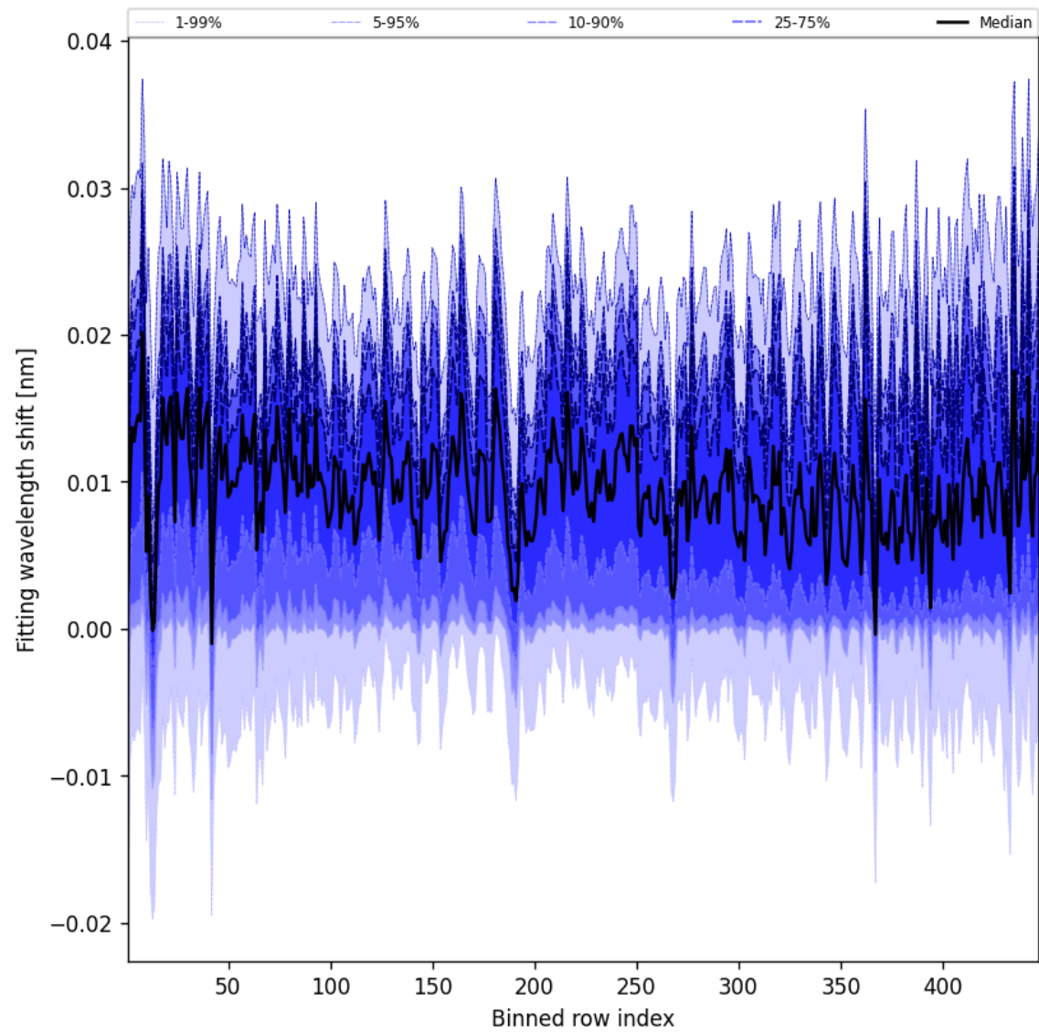
Figure 65: Along track statistics of “Fitting wavelength shift” for 2025-11-28 to 2025-11-29
