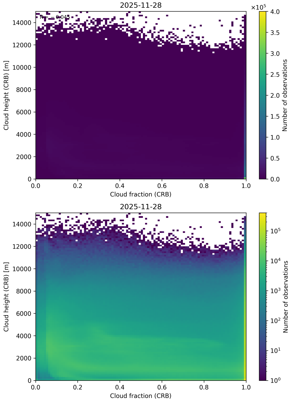
Figure 79: Scatter density plot of “Cloud fraction (CRB)” against “Cloud height (CRB)” for 2025-11-28 to 2025-11-29.
