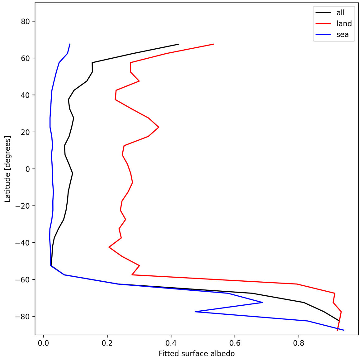
Figure 29: Zonal average of “Fitted surface albedo” for 2025-11-28 to 2025-11-29.
