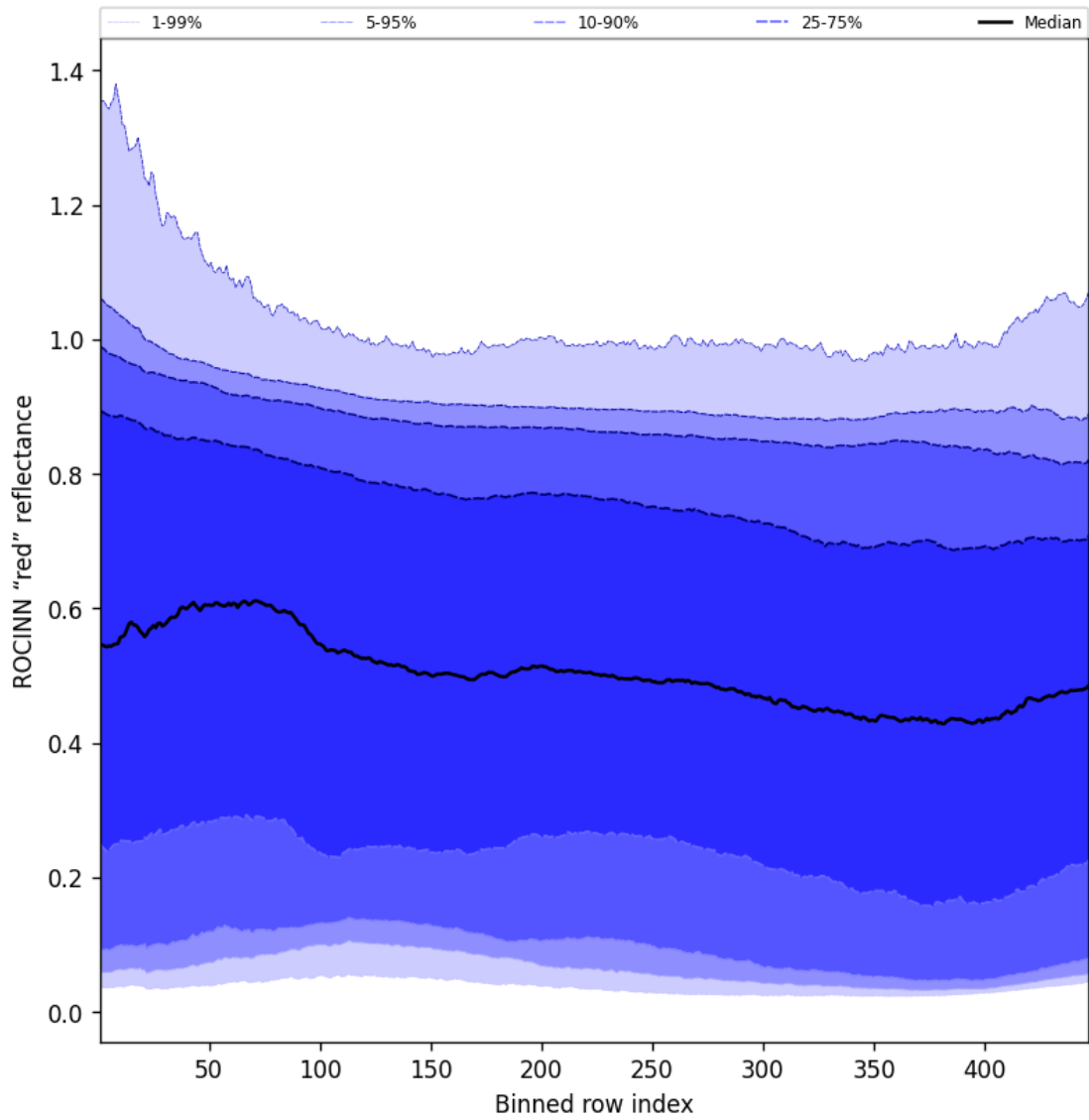
Figure 69: Along track statistics of "ROCINN "red" reflectance" for 2025-11-28 to 2025-11-29
