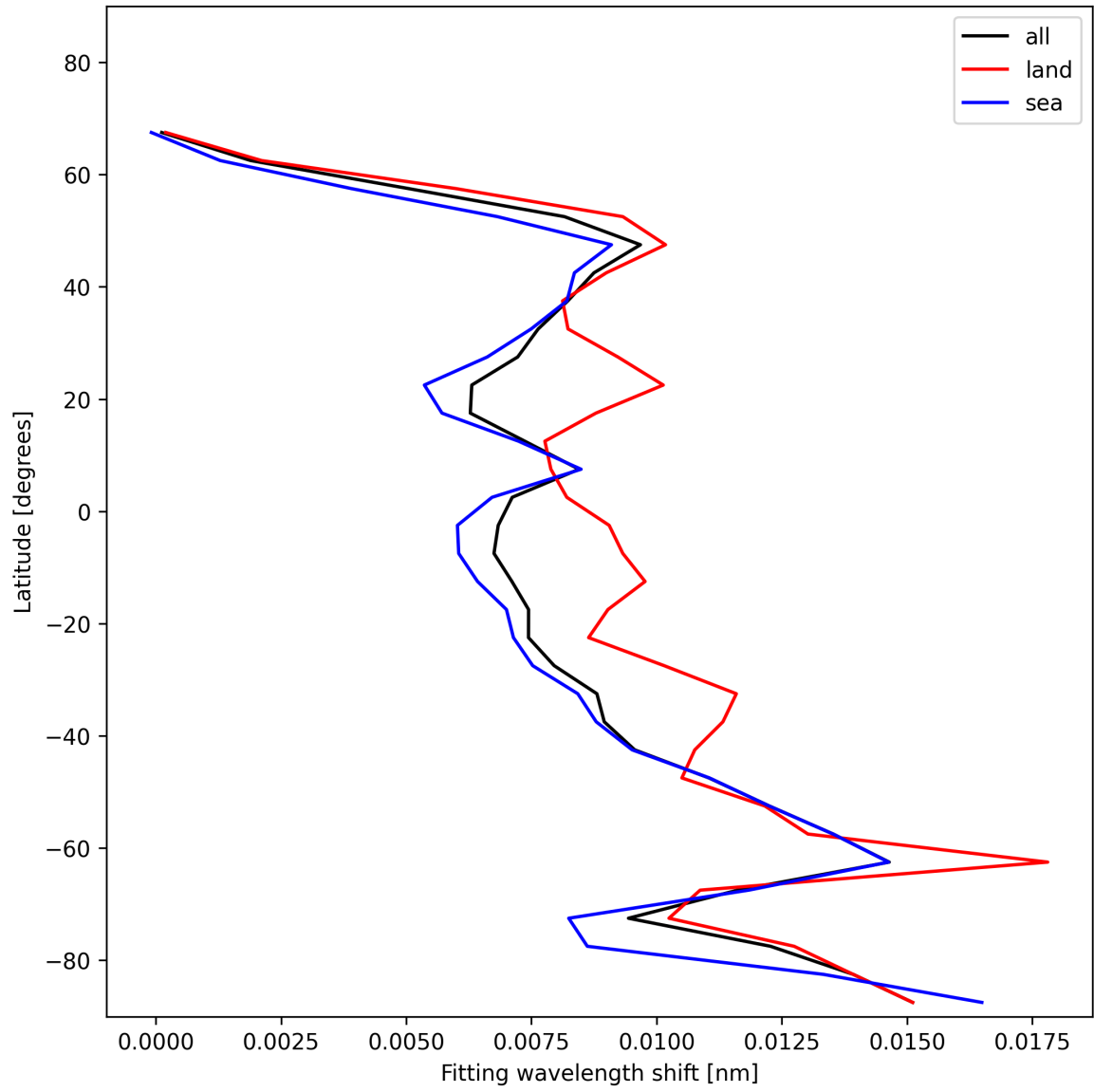
Figure 33: Zonal average of “Fitting wavelength shift” for 2025-11-28 to 2025-11-29.
