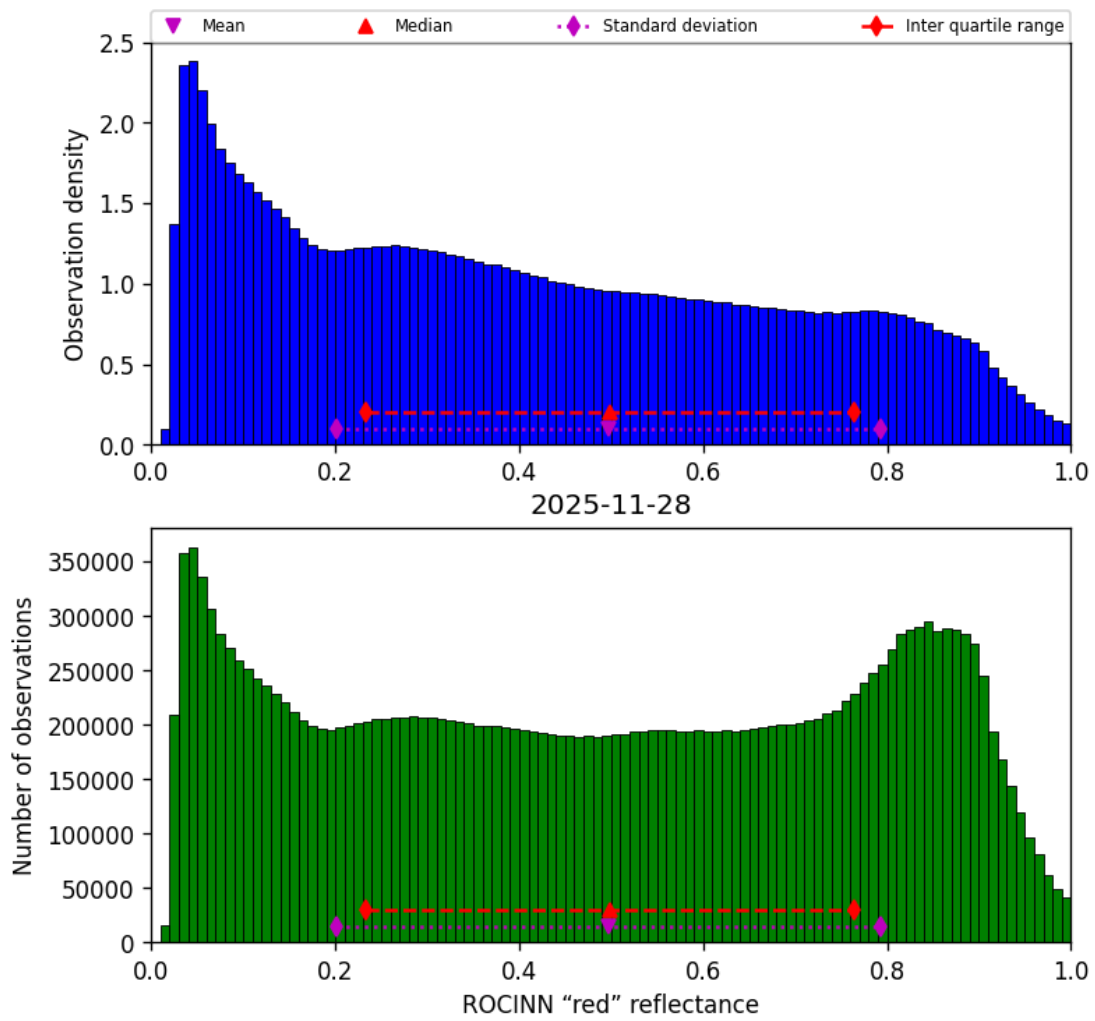
Figure 53: Histogram of “ROCINN “red” reflectance” for 2025-11-28 to 2025-11-29
