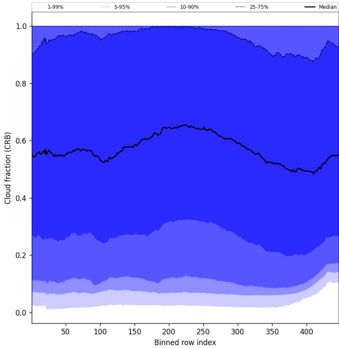
Figure 58: Along track statistics of “Cloud fraction (CRB)” for 2025-11-28 to 2025-11-29
