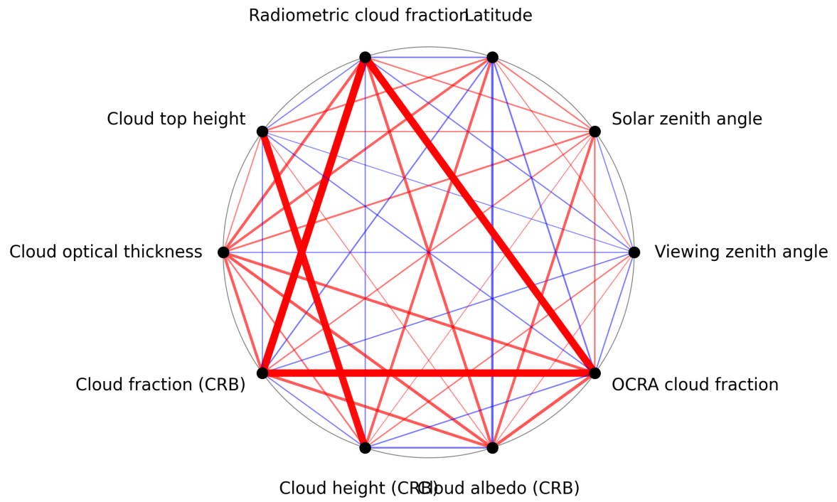
Figure 1: Map of correlation graph for 2025-11-28 to 2025-11-29.
