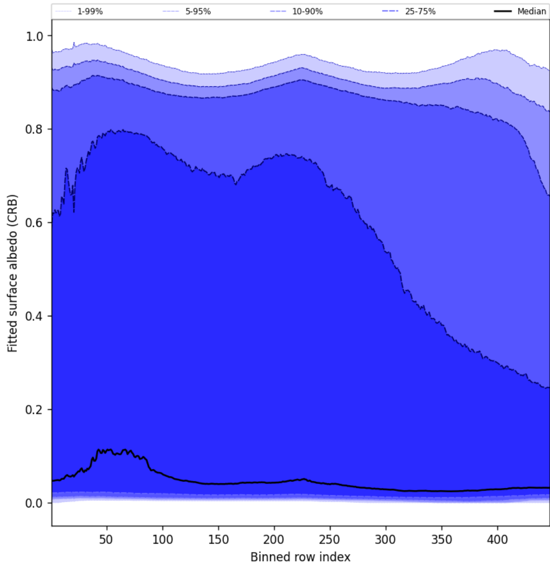
Figure 62: Along track statistics of “Fitted surface albedo (CRB)” for 2025-11-28 to 2025-11-29
