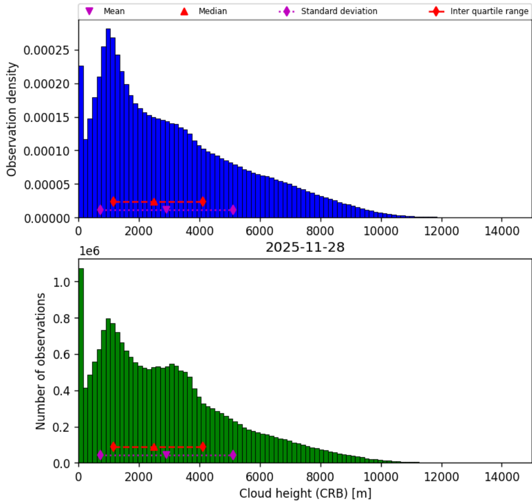
Figure 43: Histogram of “Cloud height (CRB)” for 2025-11-28 to 2025-11-29
