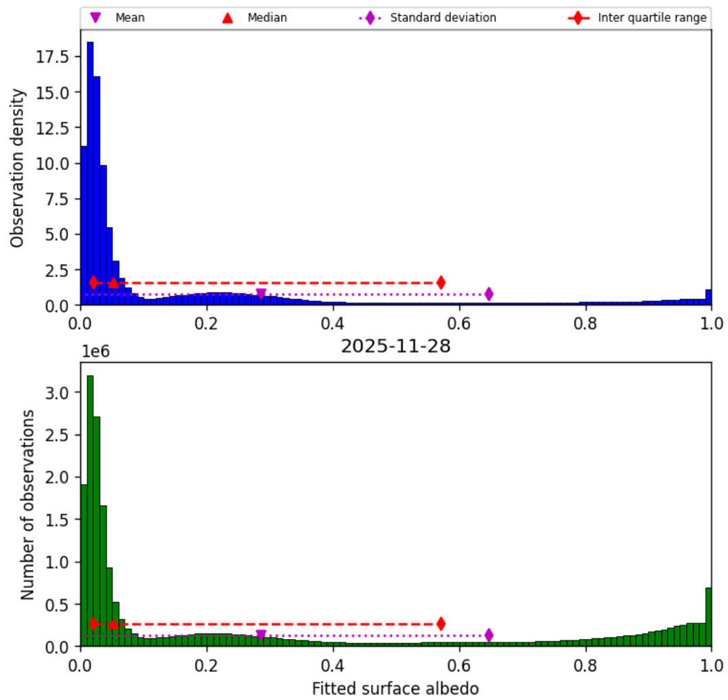
Figure 45: Histogram of “Fitted surface albedo” for 2025-11-28 to 2025-11-29
