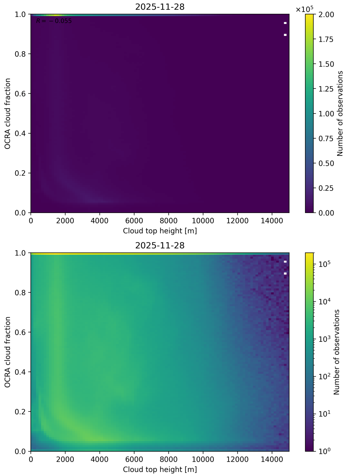
Figure 87: Scatter density plot of “Cloud top height” against “OCRA cloud fraction” for 2025-11-28 to 2025-11-29.
