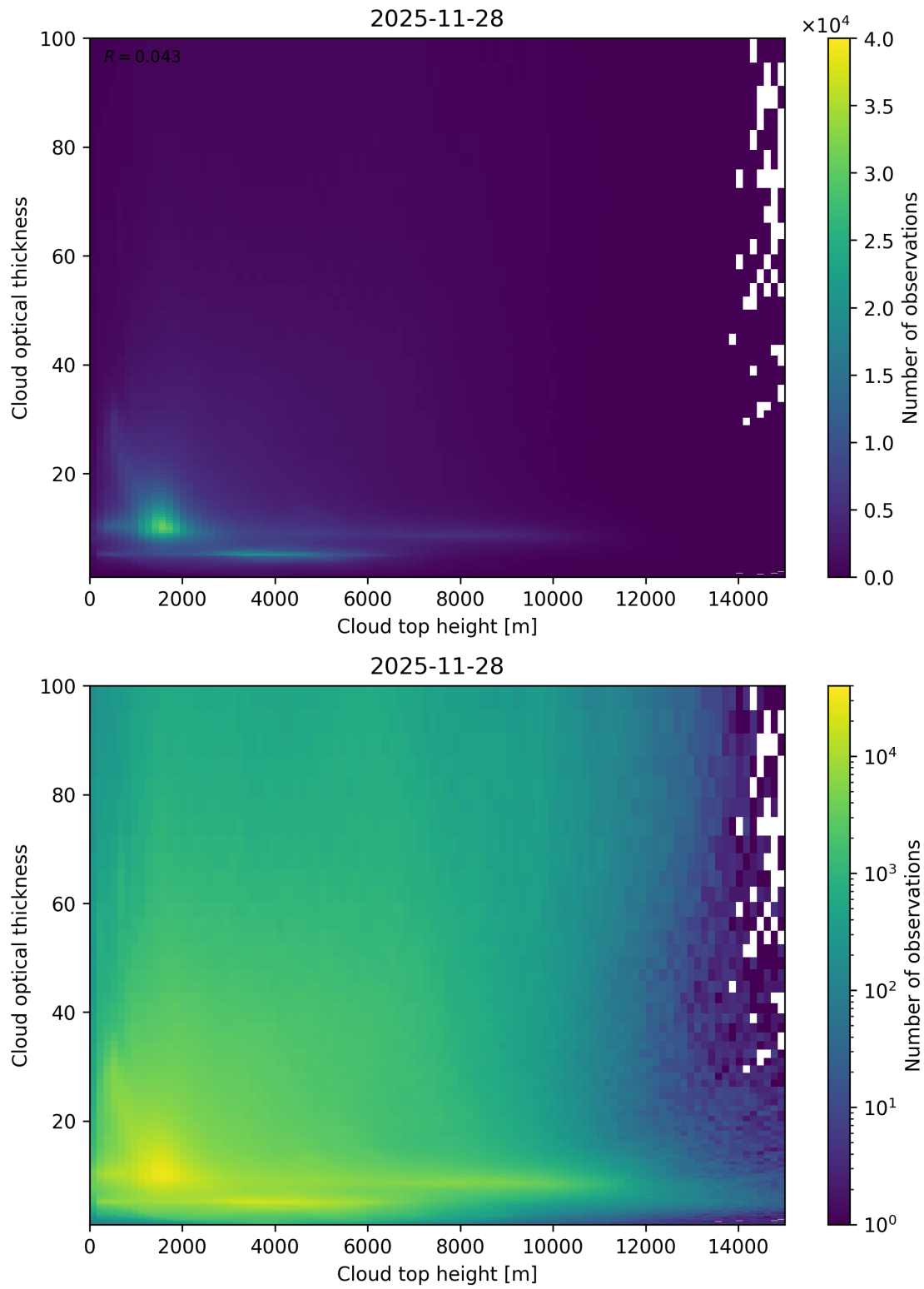
Figure 90: Scatter density plot of “Cloud top height” against “Cloud optical thickness” for 2025-11-28 to 2025-11-29.
