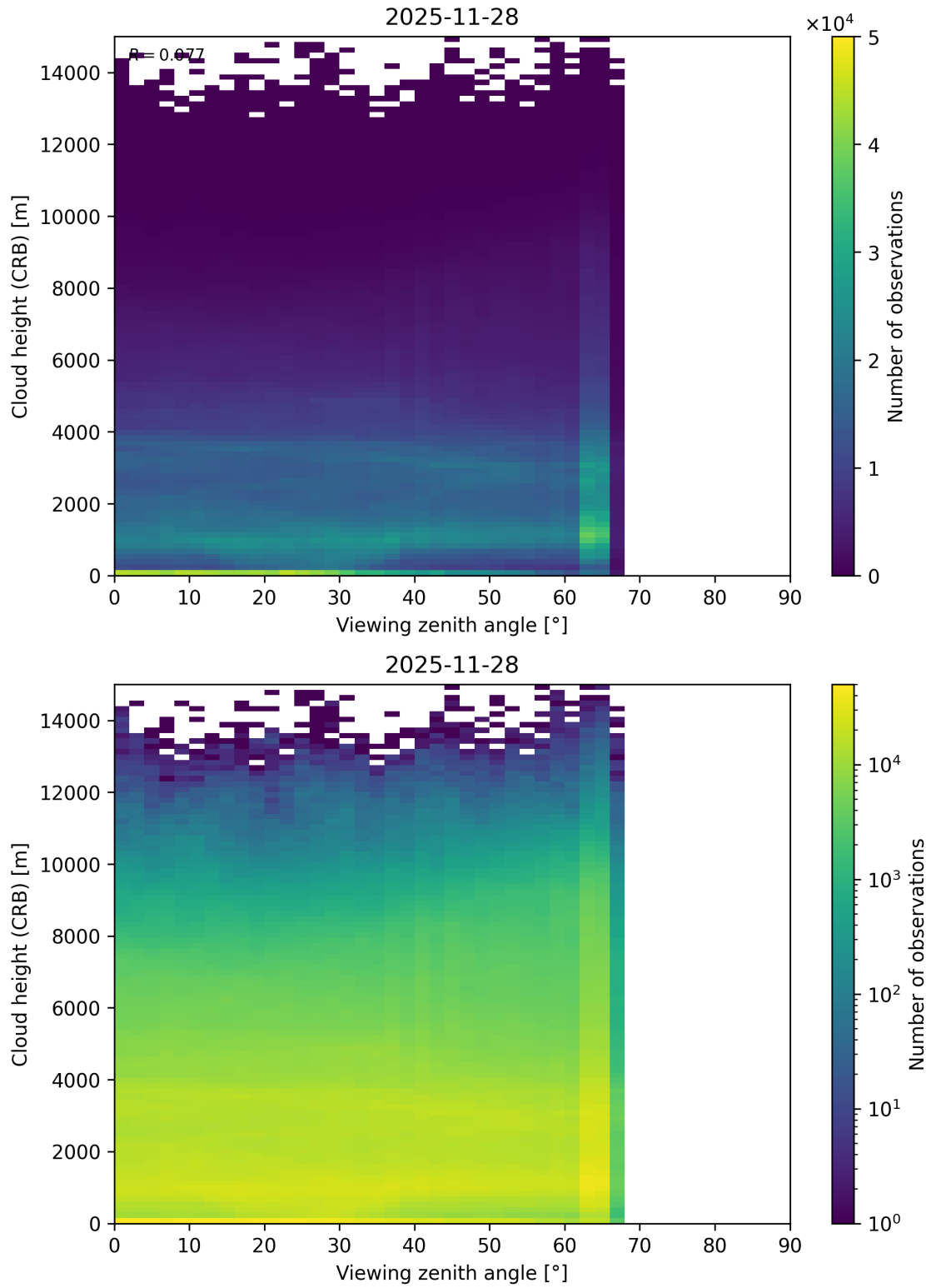
Figure 110: Scatter density plot of “Viewing zenith angle” against “Cloud height (CRB)” for 2025-11-28 to 2025-11-29.
