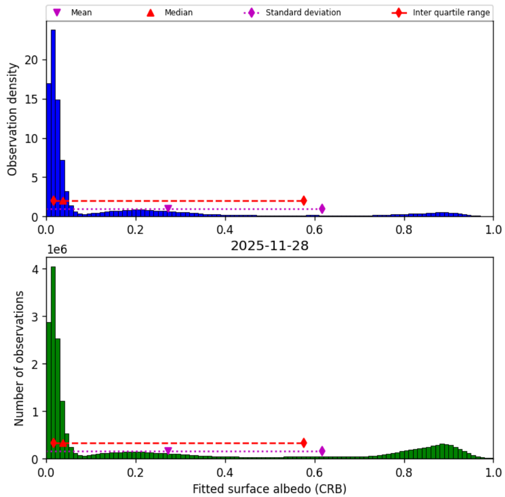
Figure 46: Histogram of “Fitted surface albedo (CRB)” for 2025-11-28 to 2025-11-29
