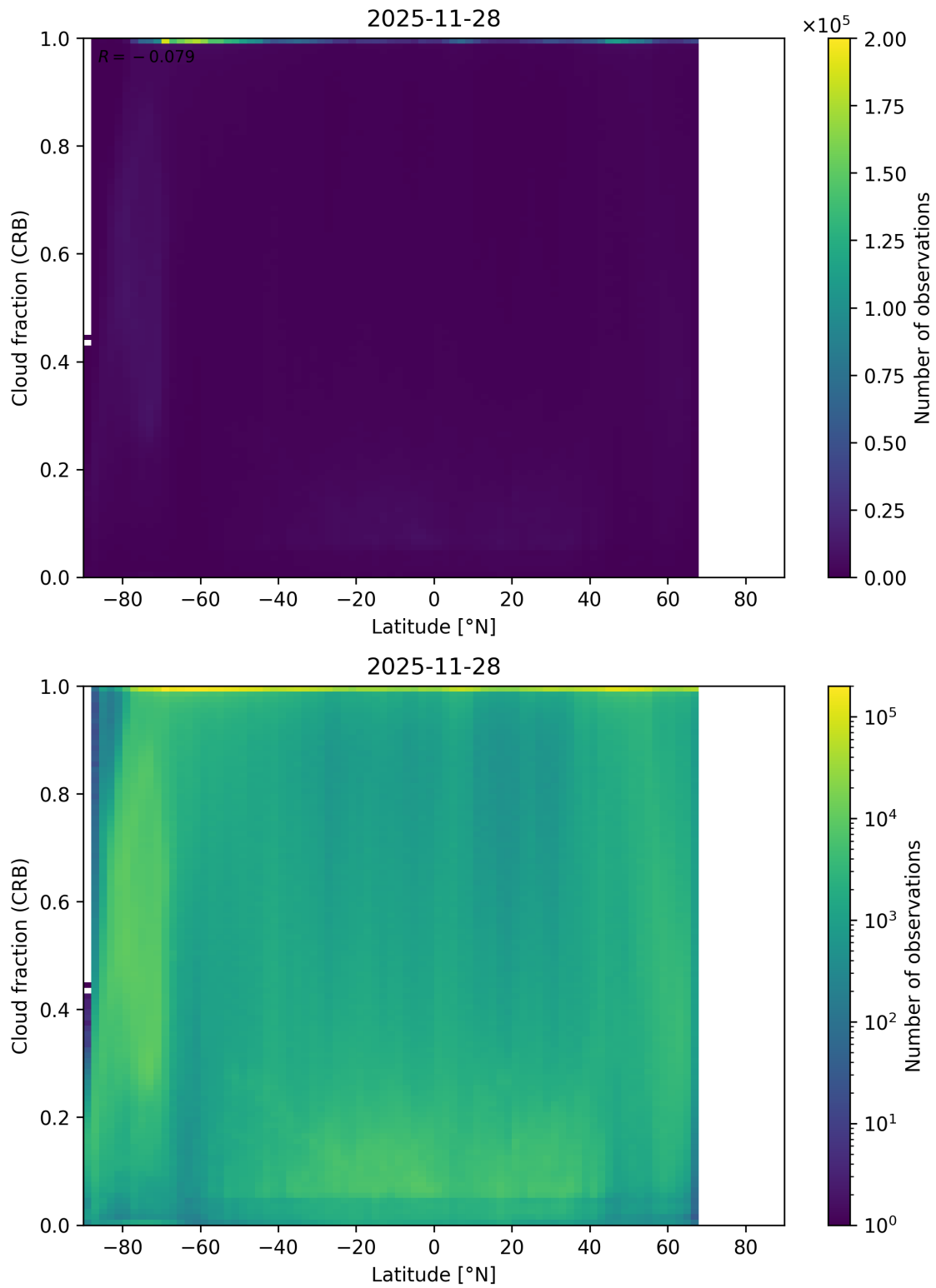
Figure 94: Scatter density plot of “Latitude” against “Cloud fraction (CRB)” for 2025-11-28 to 2025-11-29.
