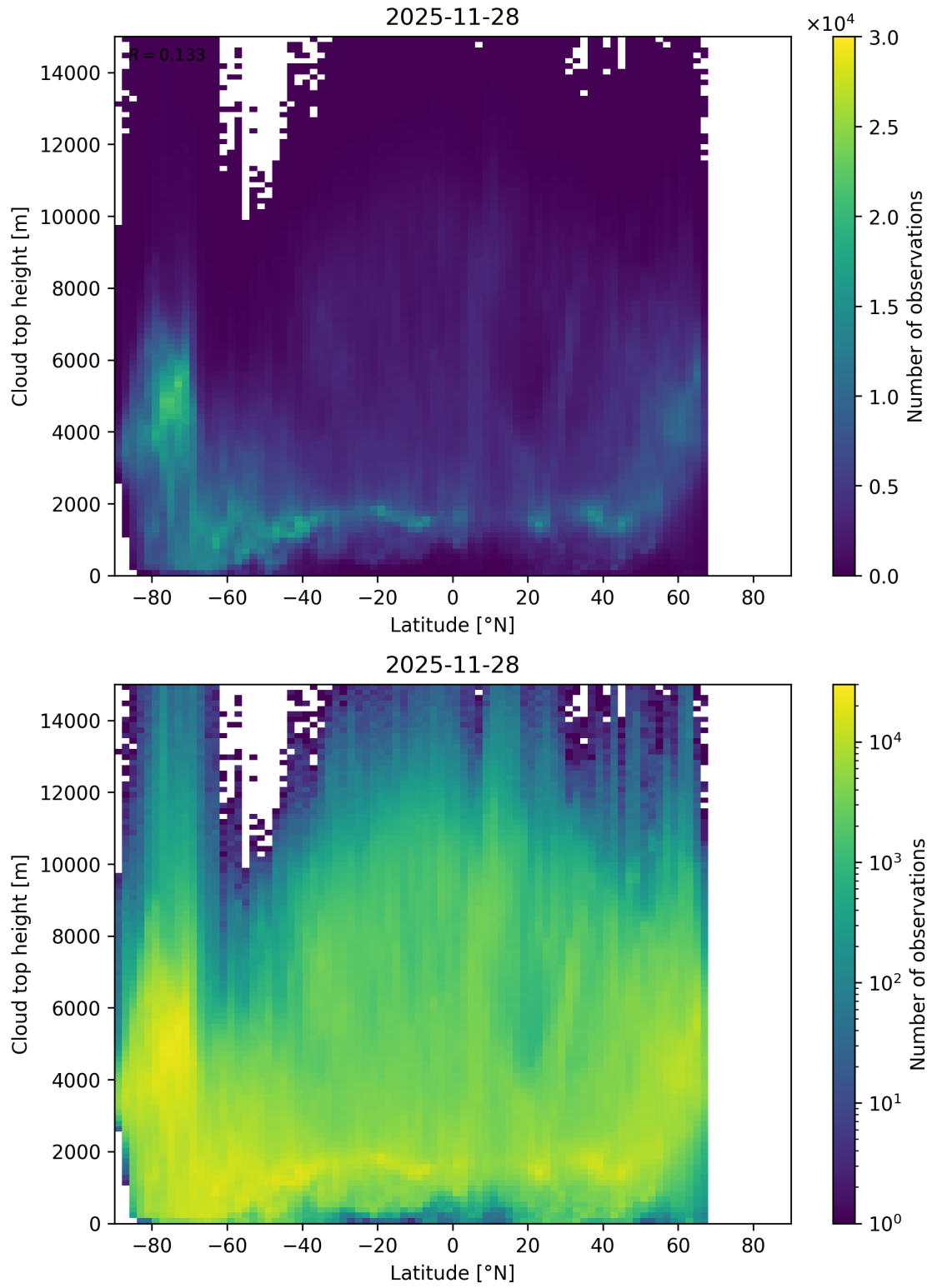
Figure 97: Scatter density plot of “Latitude” against “Cloud top height” for 2025-11-28 to 2025-11-29.
