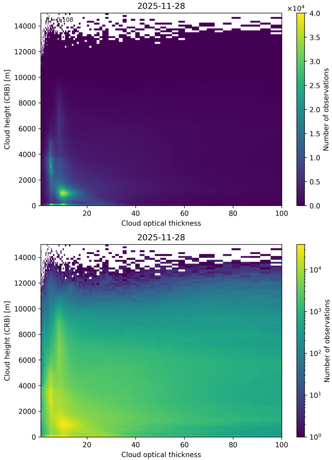
Figure 85: Scatter density plot of “Cloud optical thickness” against “Cloud height (CRB)” for 2025-11-28 to 2025-11-29.
