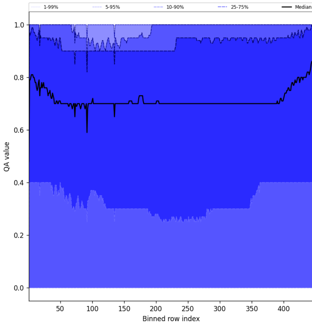
Figure 54: Along track statistics of “QA value” for 2025-11-28 to 2025-11-29
