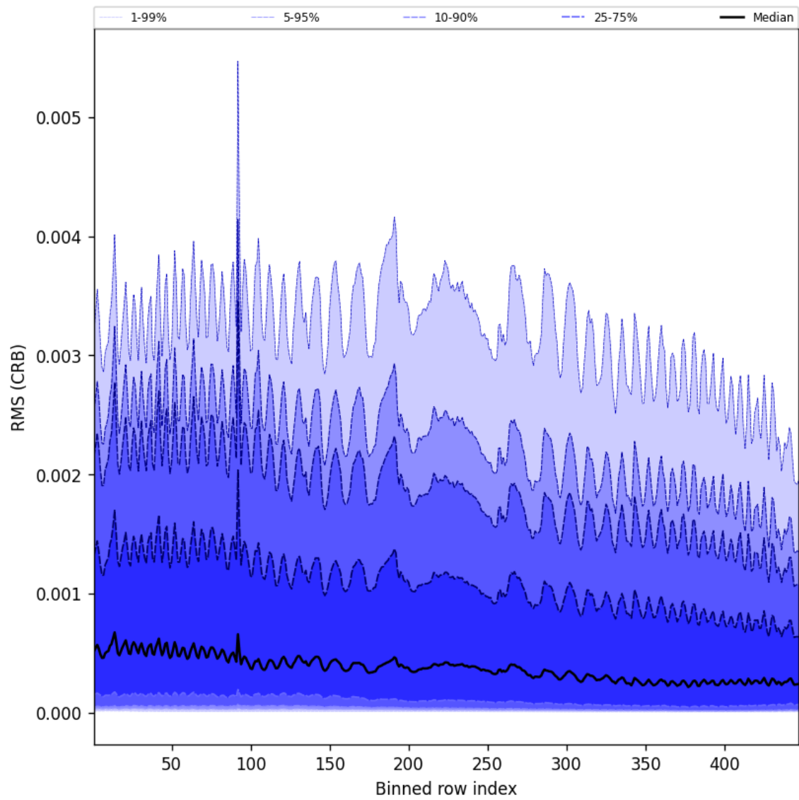
Figure 64: Along track statistics of “RMS (CRB)” for 2025-11-28 to 2025-11-29
