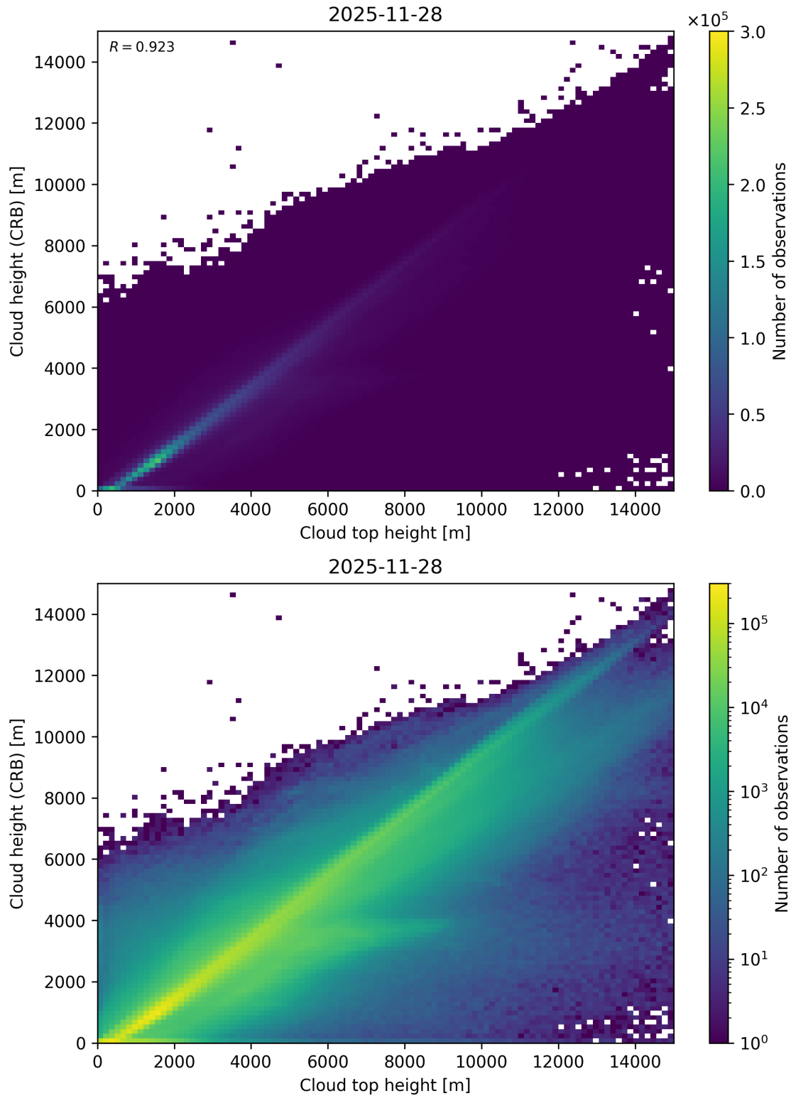
Figure 89: Scatter density plot of “Cloud top height” against “Cloud height (CRB)” for 2025-11-28 to 2025-11-29.
