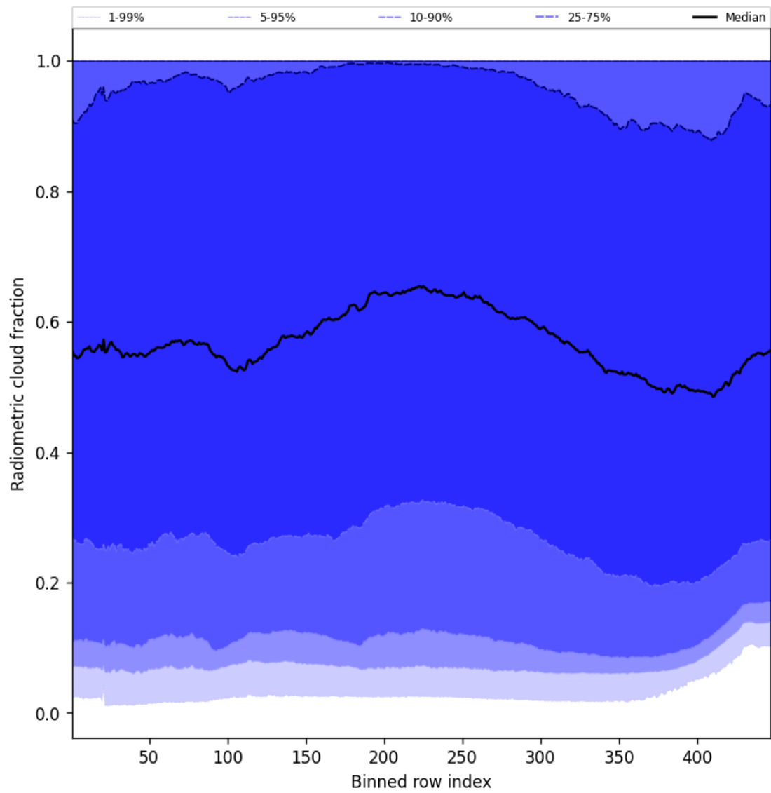
Figure 55: Along track statistics of “Radiometric cloud fraction” for 2025-11-28 to 2025-11-29
