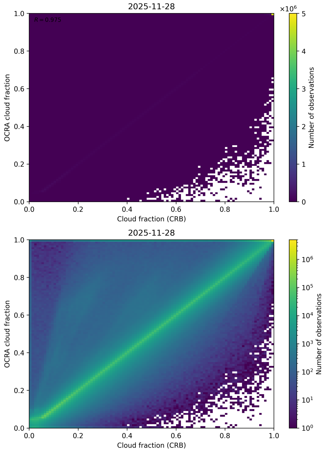
Figure 78: Scatter density plot of “Cloud fraction (CRB)” against “OCRA cloud fraction” for 2025-11-28 to 2025-11-29.
