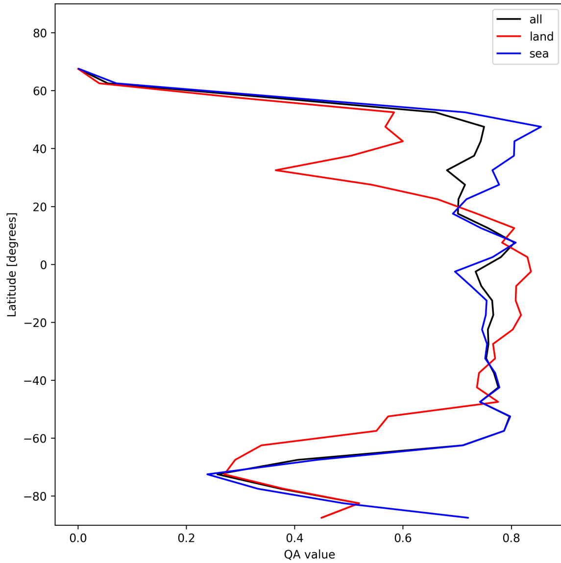
Figure 22: Zonal average of “QA value” for 2025-11-28 to 2025-11-29.
