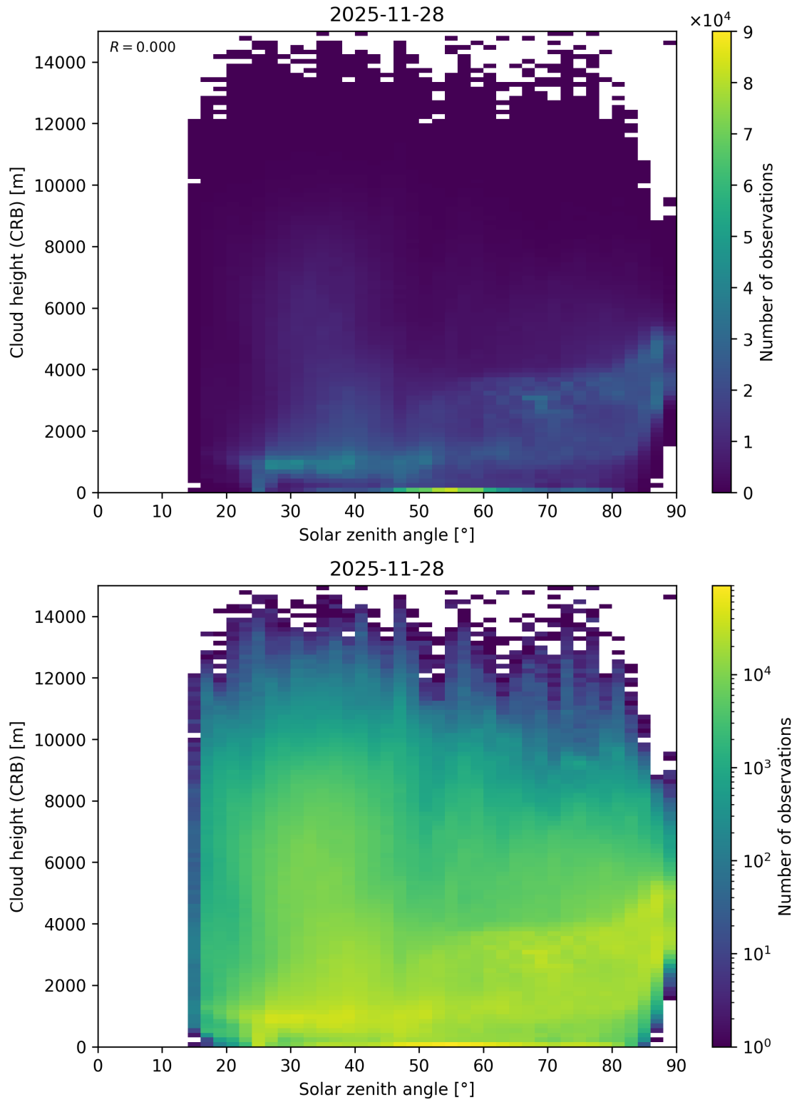
Figure 102: Scatter density plot of “Solar zenith angle” against “Cloud height (CRB)” for 2025-11-28 to 2025-11-29.
