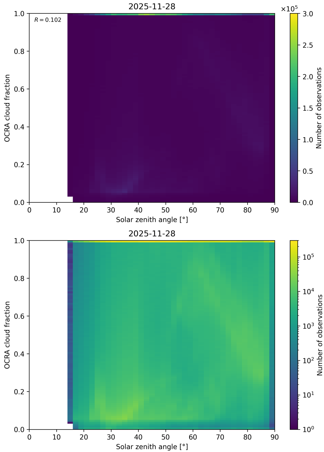
Figure 100: Scatter density plot of “Solar zenith angle” against “OCRA cloud fraction” for 2025-11-28 to 2025-11-29.
