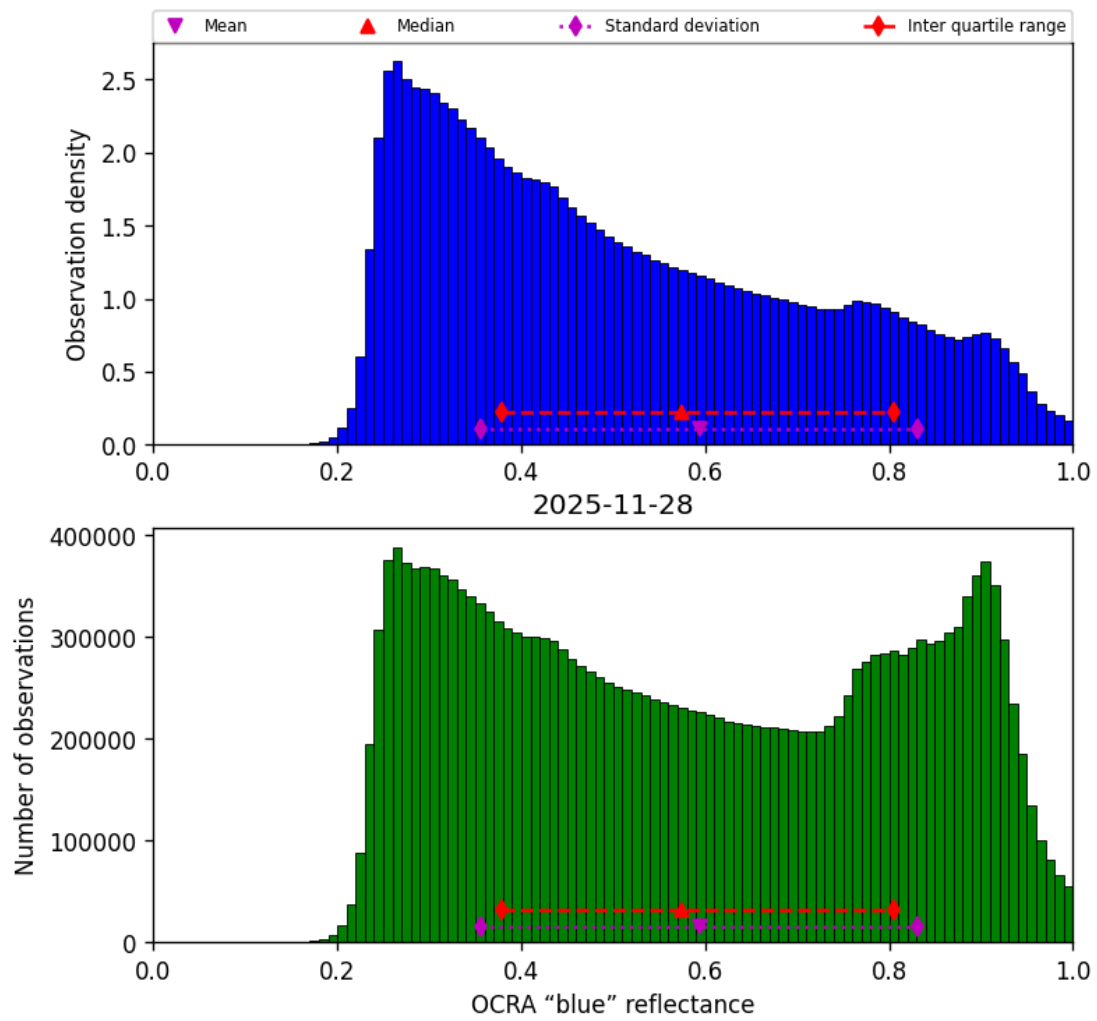
Figure 51: Histogram of “OCRA “blue” reflectance” for 2025-11-28 to 2025-11-29
