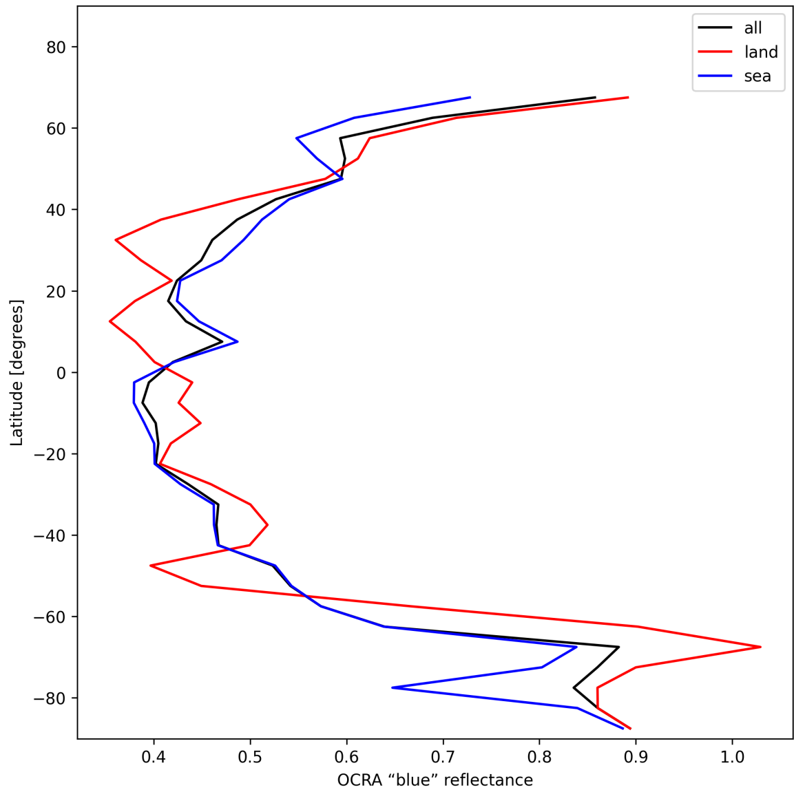
Figure 35: Zonal average of “OCRA “blue” reflectance” for 2025-11-28 to 2025-11-29.
