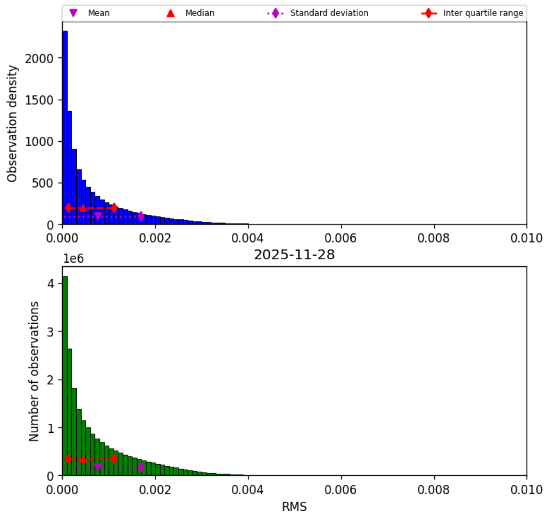
Figure 47: Histogram of “RMS” for 2025-11-28 to 2025-11-29
