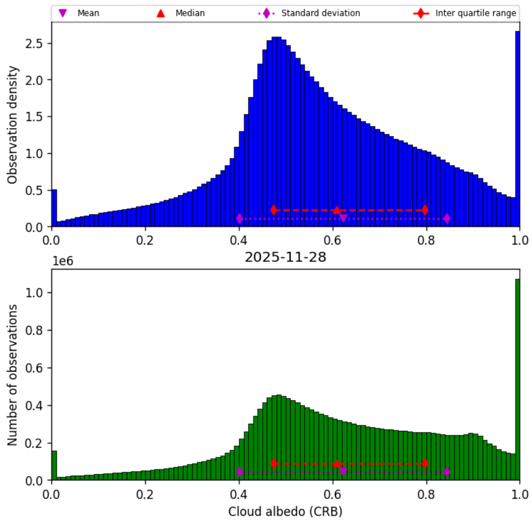
Figure 44: Histogram of “Cloud albedo (CRB)” for 2025-11-28 to 2025-11-29
