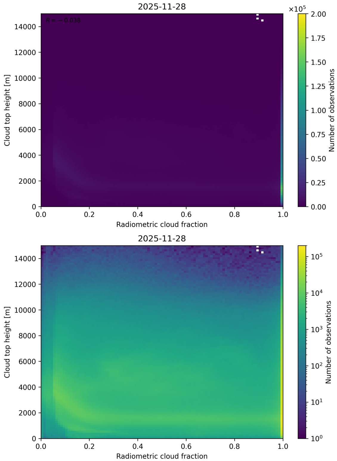
Figure 76: Scatter density plot of “Radiometric cloud fraction” against “Cloud top height” for 2025-11-28 to 2025-11-29.
