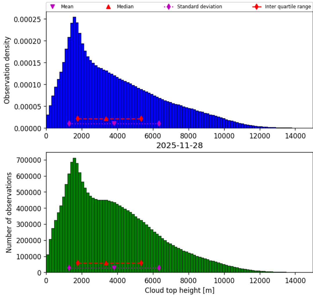
Figure 40: Histogram of “Cloud top height” for 2025-11-28 to 2025-11-29
