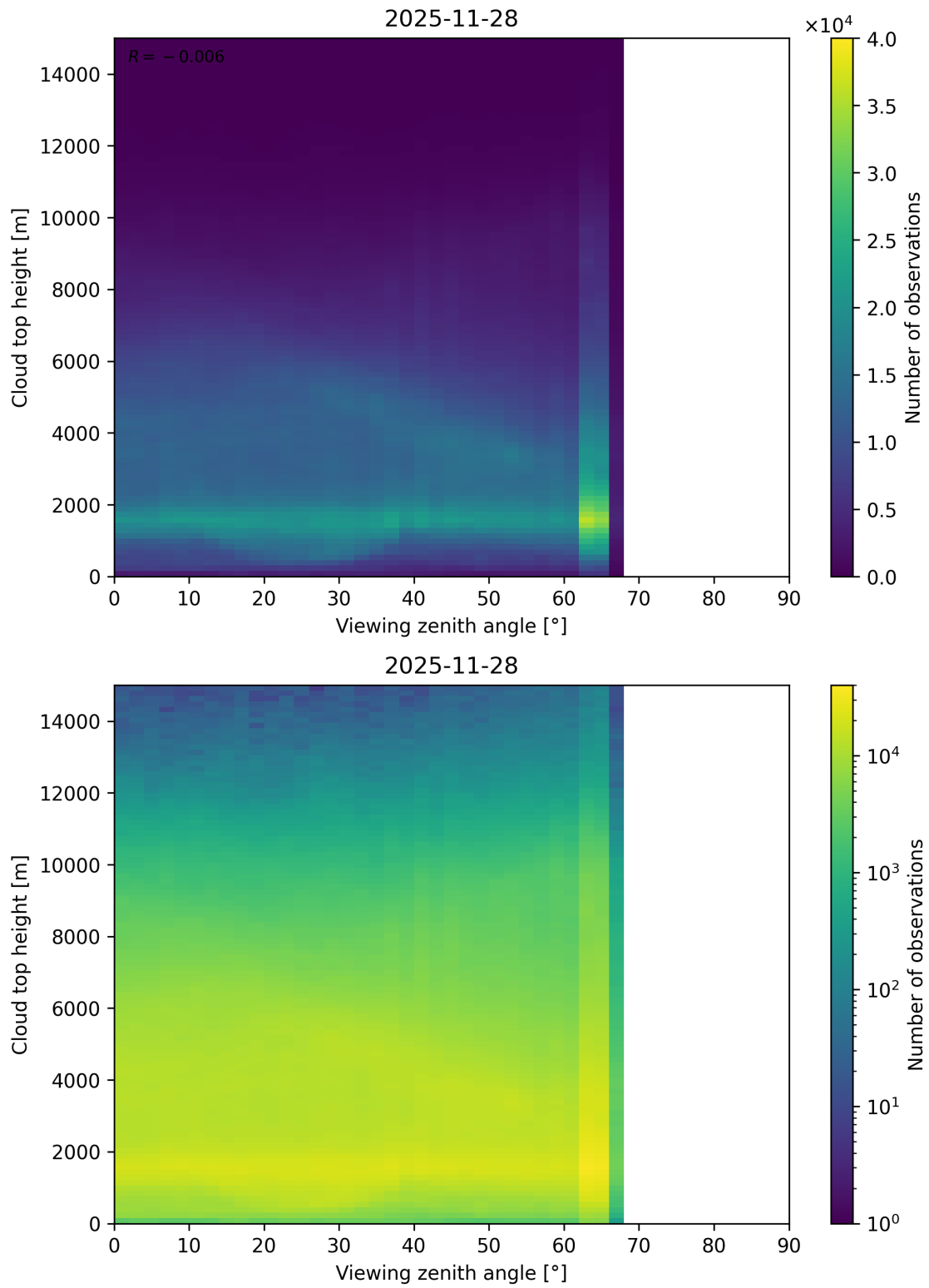
Figure 112: Scatter density plot of “Viewing zenith angle” against “Cloud top height” for 2025-11-28 to 2025-11-29.
