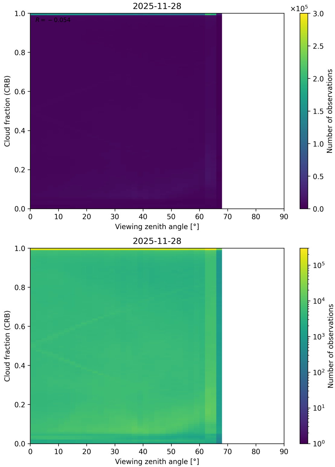
Figure 109: Scatter density plot of “Viewing zenith angle” against “Cloud fraction (CRB)” for 2025-11-28 to 2025-11-29.
