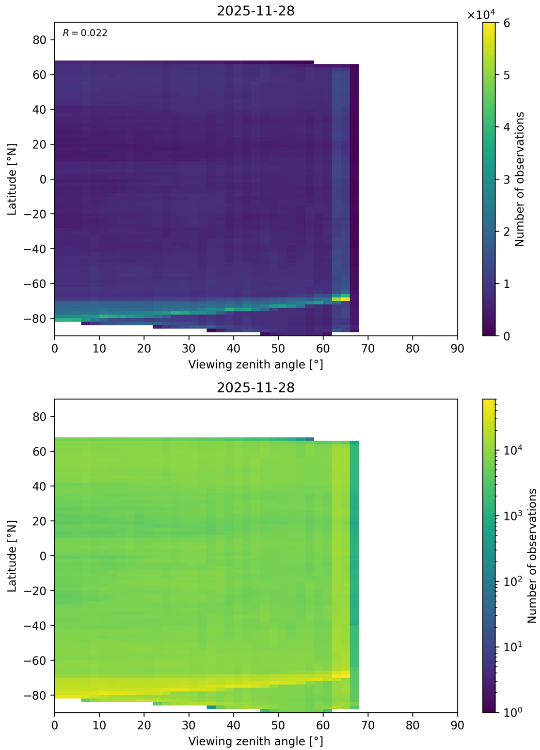
Figure 113: Scatter density plot of “Viewing zenith angle” against “Latitude” for 2025-11-28 to 2025-11-29.
