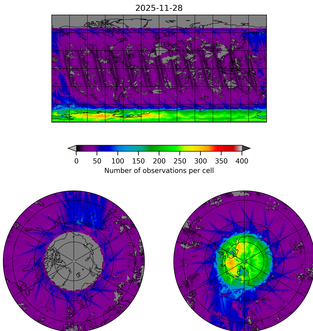
Figure 21: Map of the number of observations for 2025-11-28 to 2025-11-29
