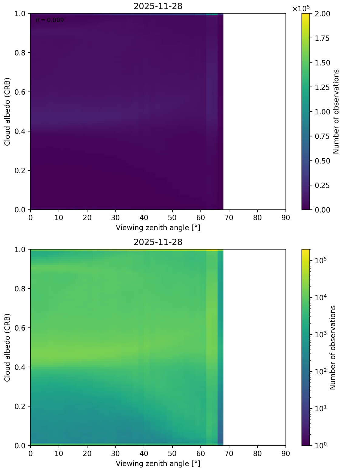
Figure 106: Scatter density plot of “Viewing zenith angle” against “Cloud albedo (CRB)” for 2025-11-28 to 2025-11-29.
