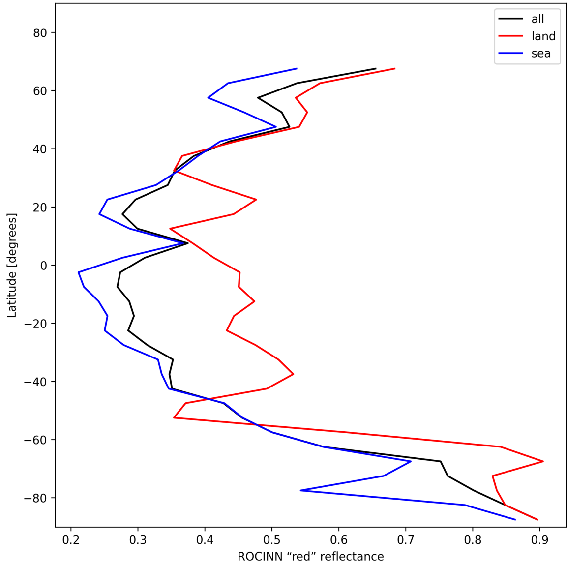
Figure 37: Zonal average of "ROCINN "red" reflectance" for 2025-11-28 to 2025-11-29.
