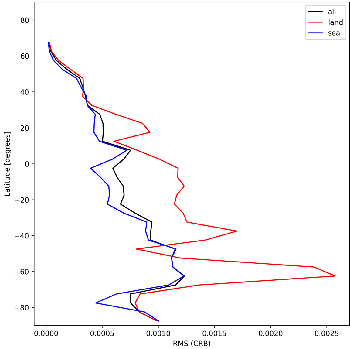
Figure 32: Zonal average of “RMS (CRB)” for 2025-11-28 to 2025-11-29.
