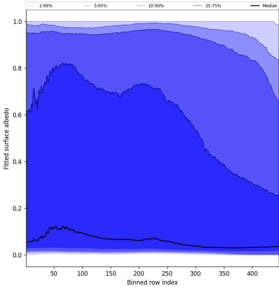
Figure 61: Along track statistics of “Fitted surface albedo” for 2025-11-28 to 2025-11-29
