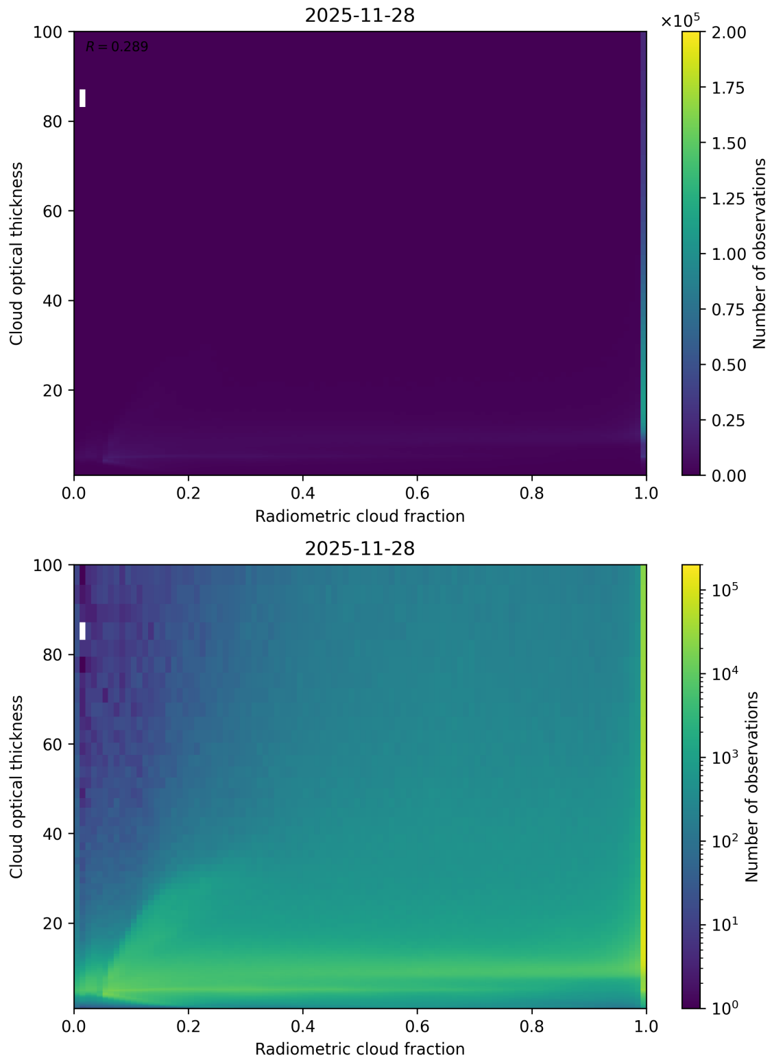
Figure 75: Scatter density plot of “Radiometric cloud fraction” against “Cloud optical thickness” for 2025-11-28 to 2025-11-29.
