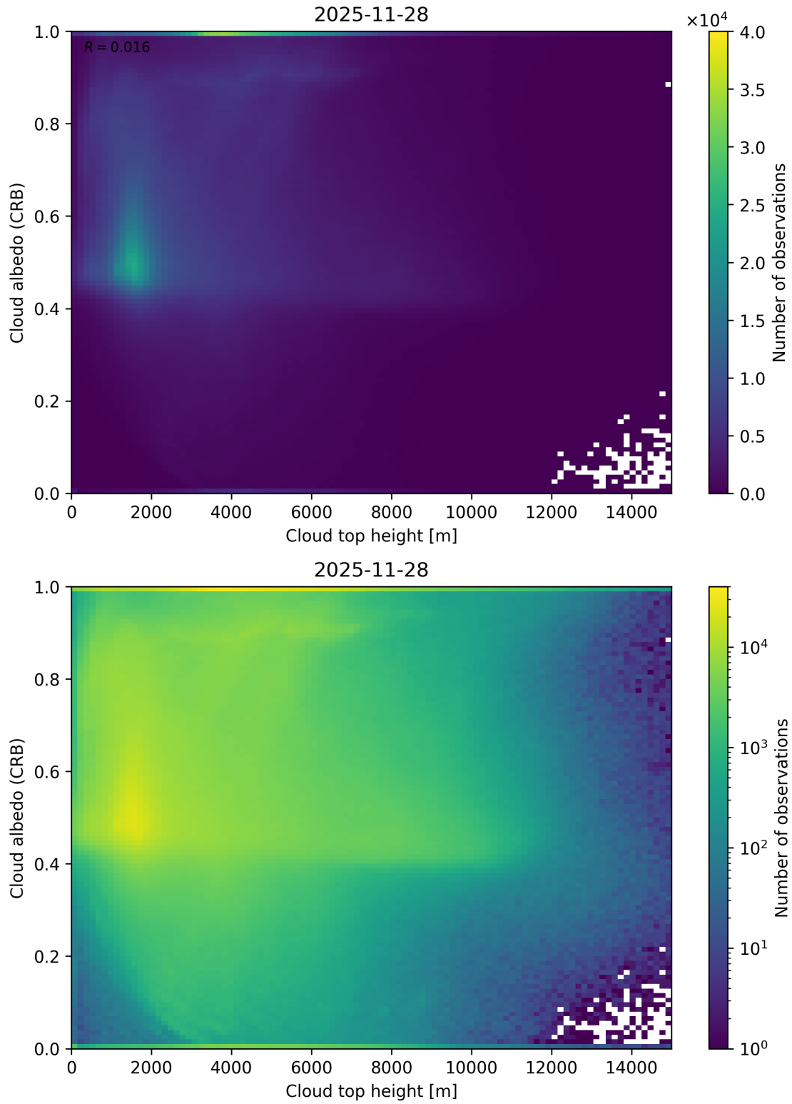
Figure 86: Scatter density plot of “Cloud top height” against “Cloud albedo (CRB)” for 2025-11-28 to 2025-11-29.
