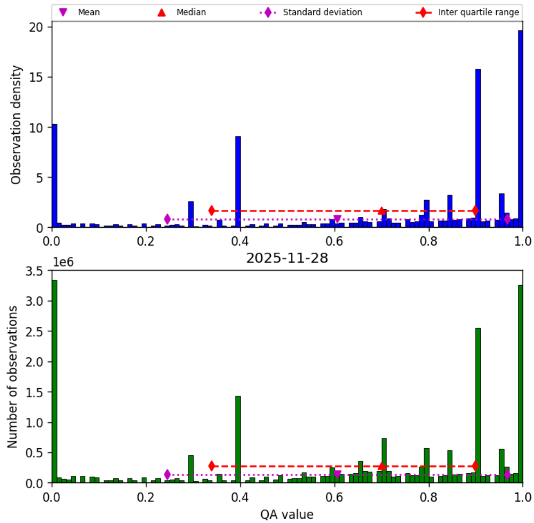
Figure 38: Histogram of “QA value” for 2025-11-28 to 2025-11-29
