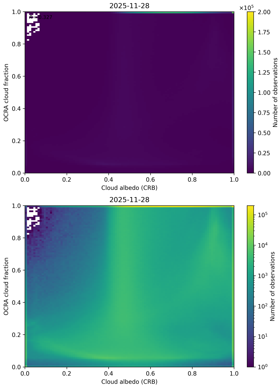
Figure 70: Scatter density plot of “Cloud albedo (CRB)” against “OCRA cloud fraction” for 2025-11-28 to 2025-11-29.
