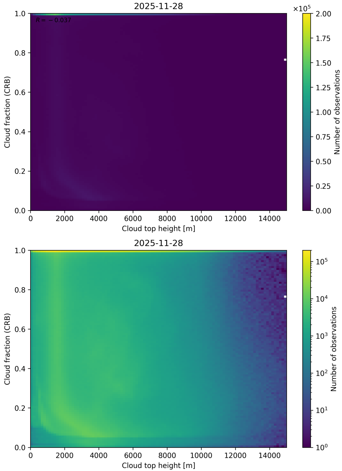
Figure 88: Scatter density plot of “Cloud top height” against “Cloud fraction (CRB)” for 2025-11-28 to 2025-11-29.
