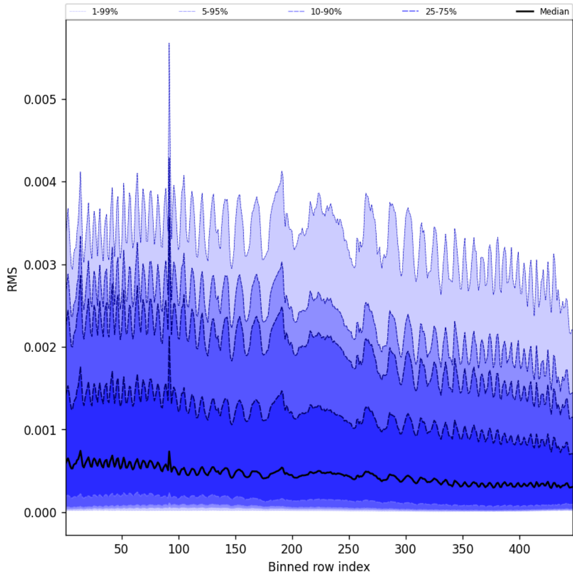
Figure 63: Along track statistics of “RMS” for 2025-11-28 to 2025-11-29
