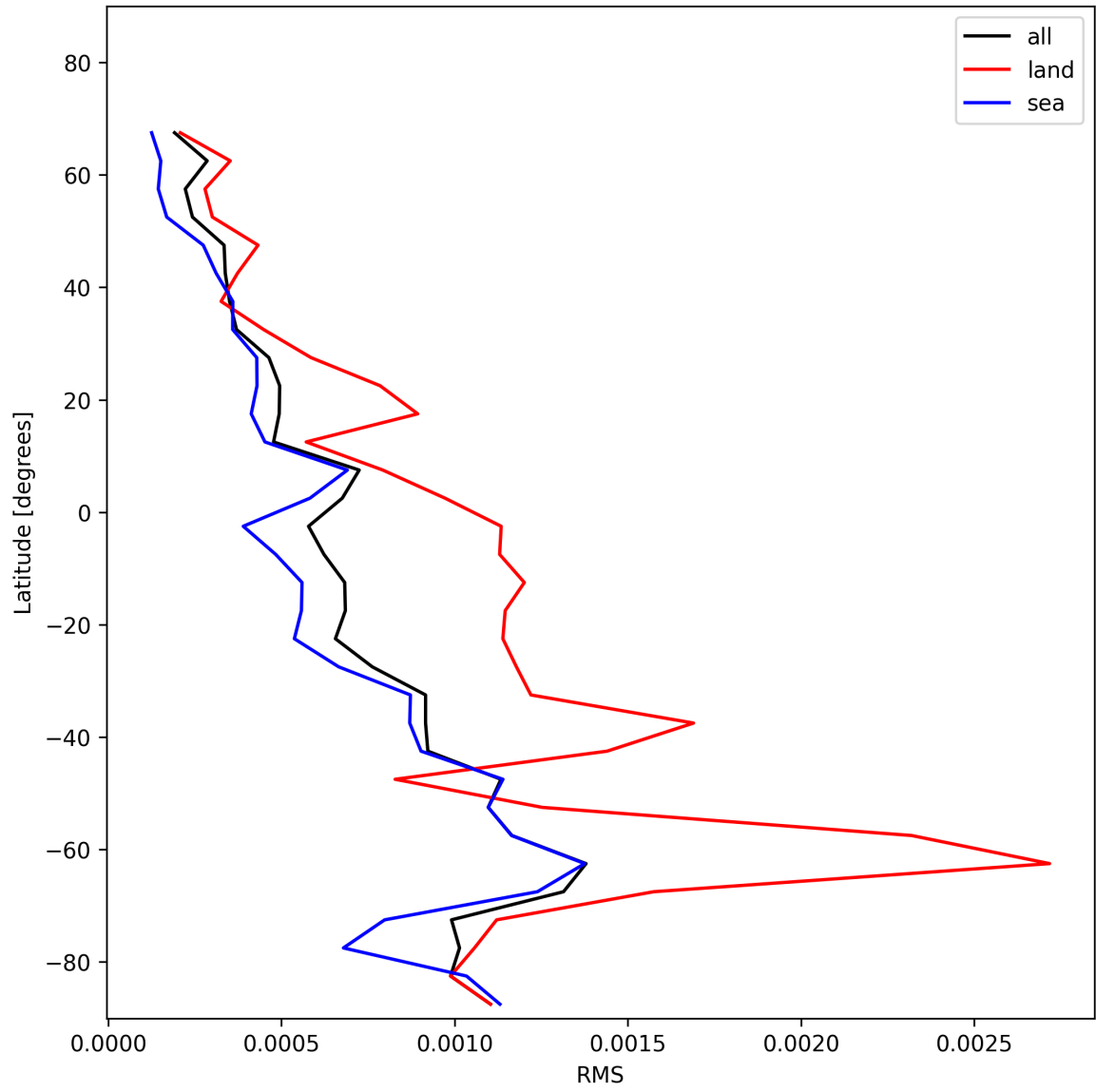
Figure 31: Zonal average of “RMS” for 2025-11-28 to 2025-11-29.
