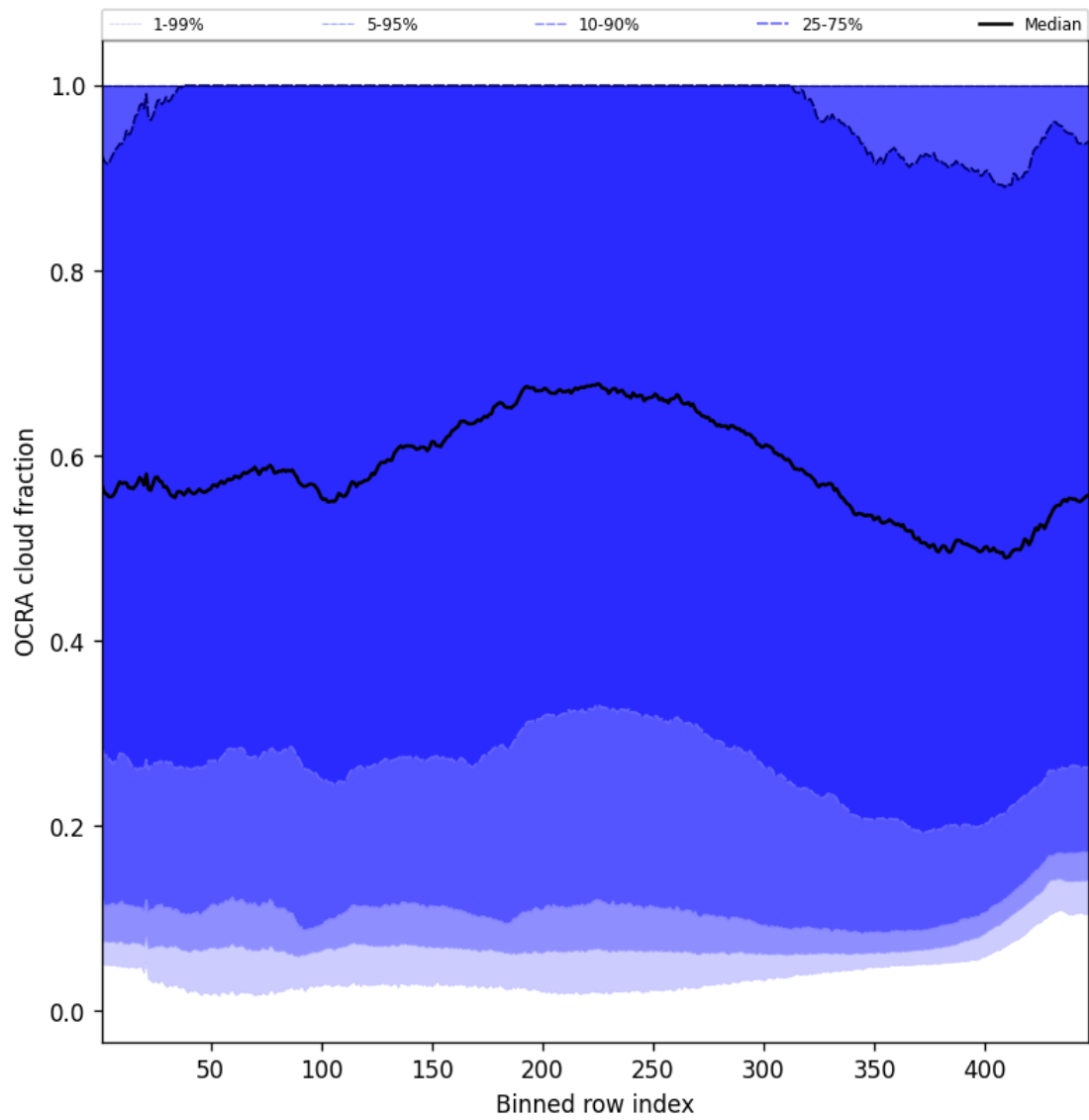
Figure 66: Along track statistics of “OCRA cloud fraction” for 2025-11-28 to 2025-11-29
