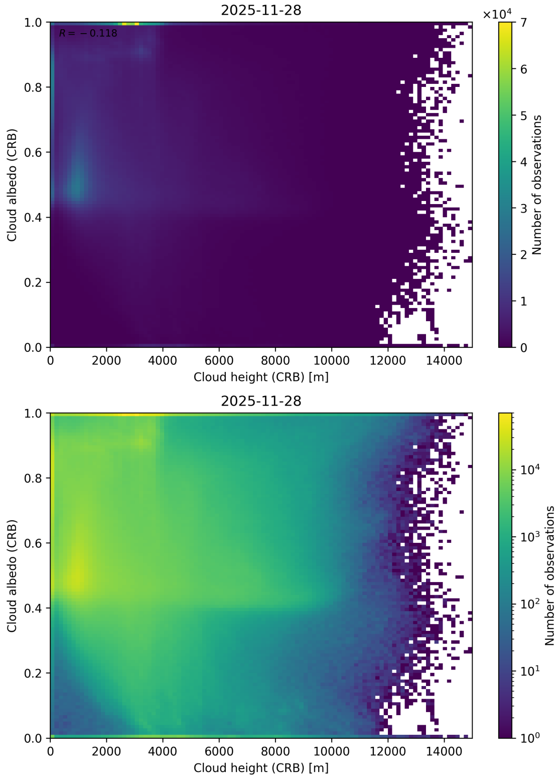
Figure 80: Scatter density plot of “Cloud height (CRB)” against “Cloud albedo (CRB)” for 2025-11-28 to 2025-11-29.
