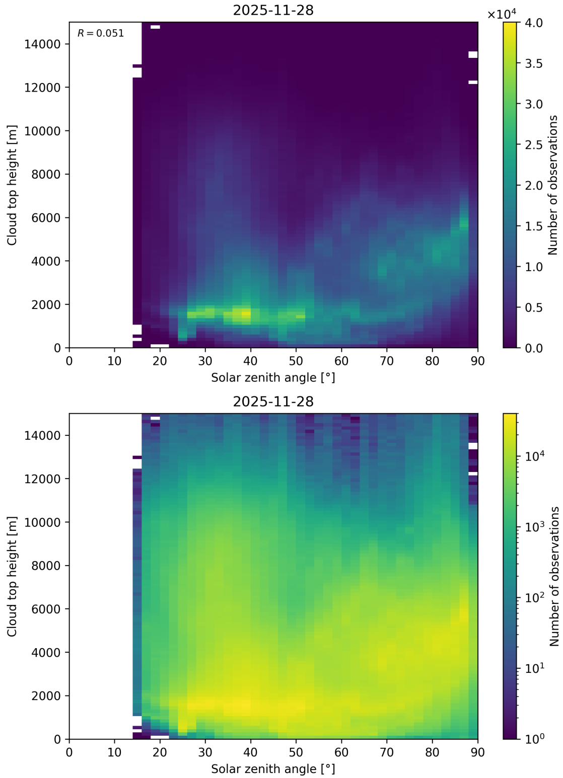
Figure 104: Scatter density plot of “Solar zenith angle” against “Cloud top height” for 2025-11-28 to 2025-11-29.
