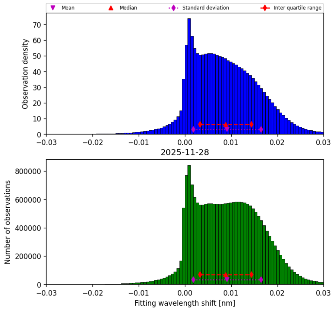
Figure 49: Histogram of “Fitting wavelength shift” for 2025-11-28 to 2025-11-29
