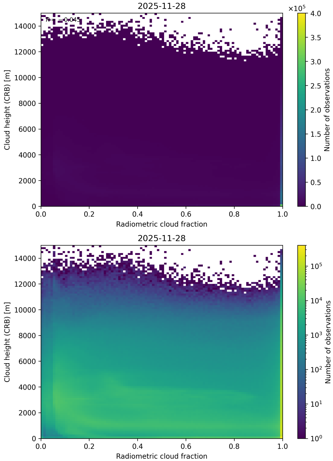
Figure 74: Scatter density plot of “Radiometric cloud fraction” against “Cloud height (CRB)” for 2025-11-28 to 2025-11-29.
