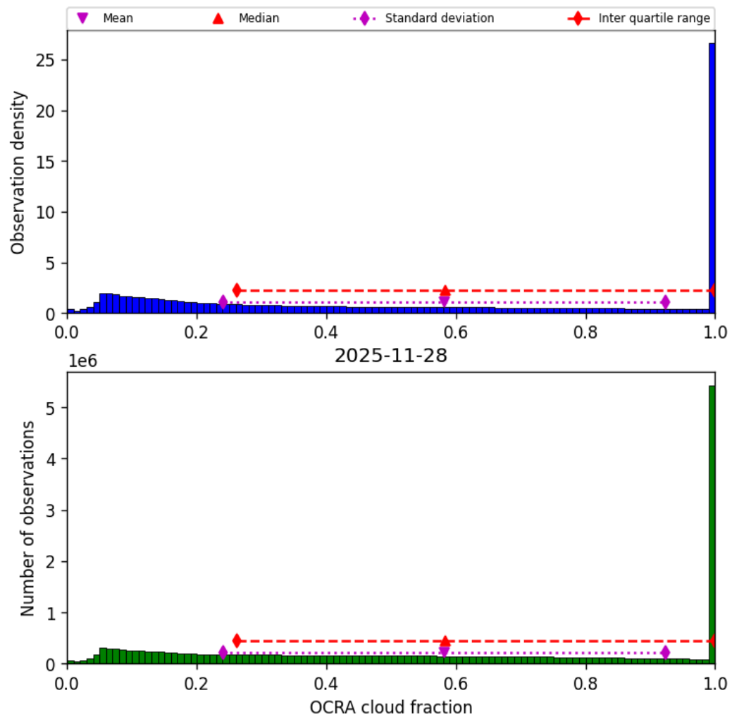
Figure 50: Histogram of “OCRA cloud fraction” for 2025-11-28 to 2025-11-29
