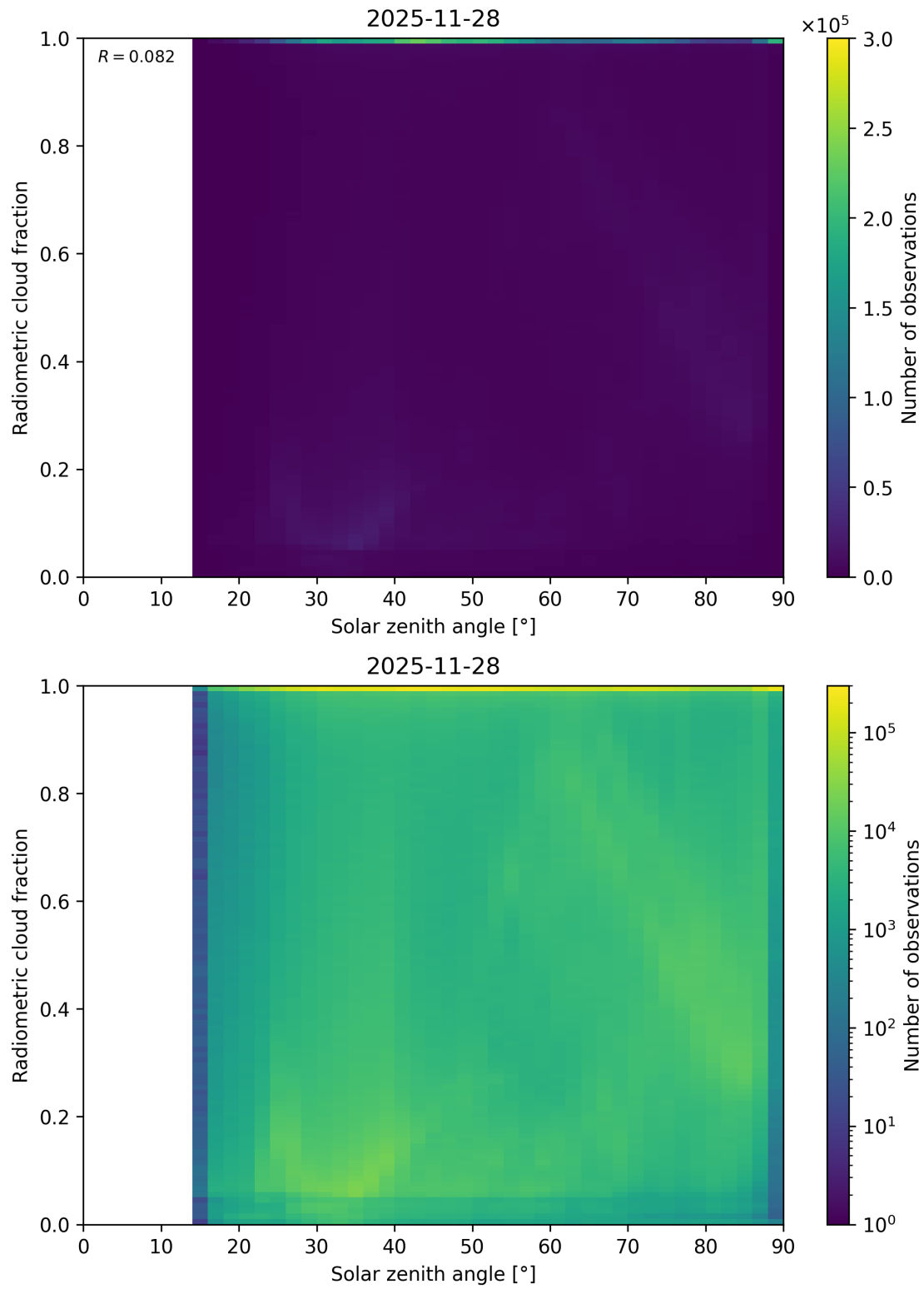
Figure 99: Scatter density plot of “Solar zenith angle” against “Radiometric cloud fraction” for 2025-11-28 to 2025-11-29.
