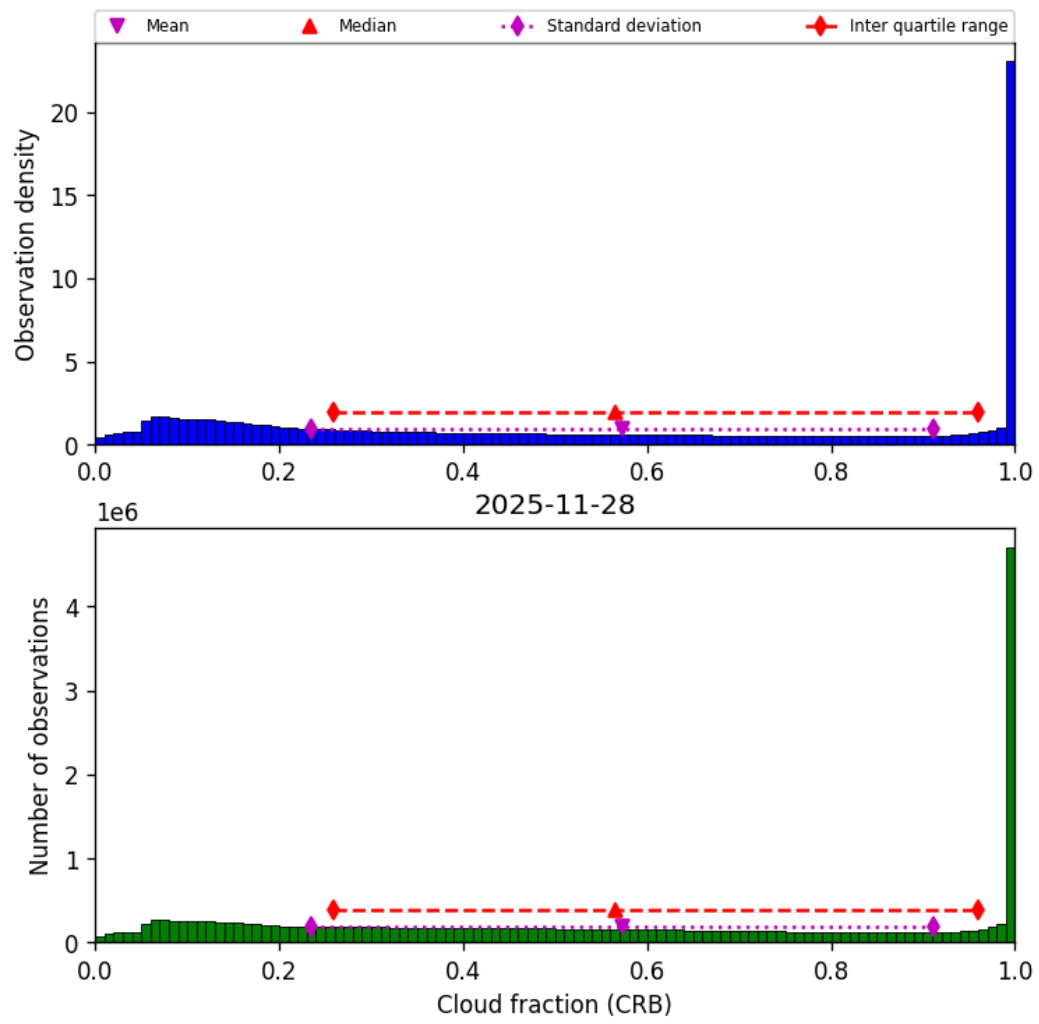
Figure 42: Histogram of “Cloud fraction (CRB)” for 2025-11-28 to 2025-11-29
