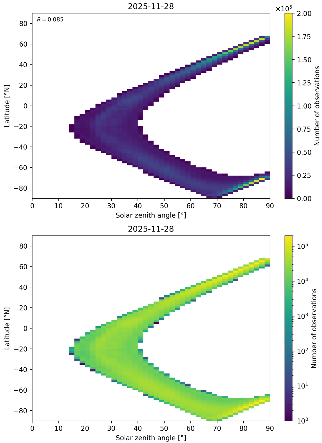
Figure 105: Scatter density plot of “Solar zenith angle” against “Latitude” for 2025-11-28 to 2025-11-29.
