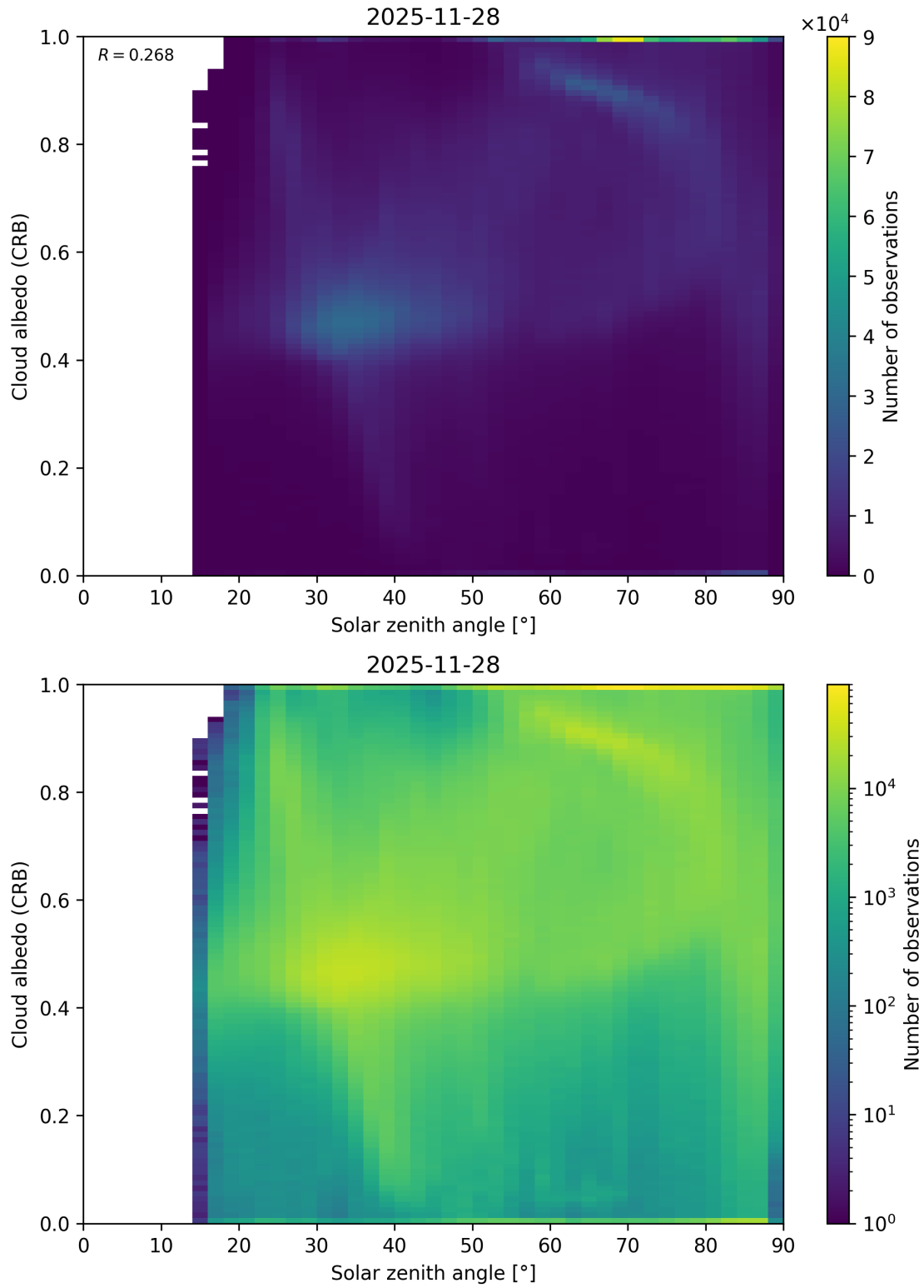
Figure 98: Scatter density plot of “Solar zenith angle” against “Cloud albedo (CRB)” for 2025-11-28 to 2025-11-29.
