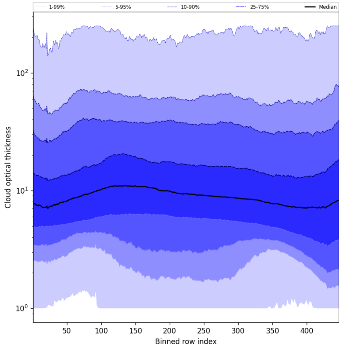
Figure 57: Along track statistics of “Cloud optical thickness” for 2025-11-28 to 2025-11-29
