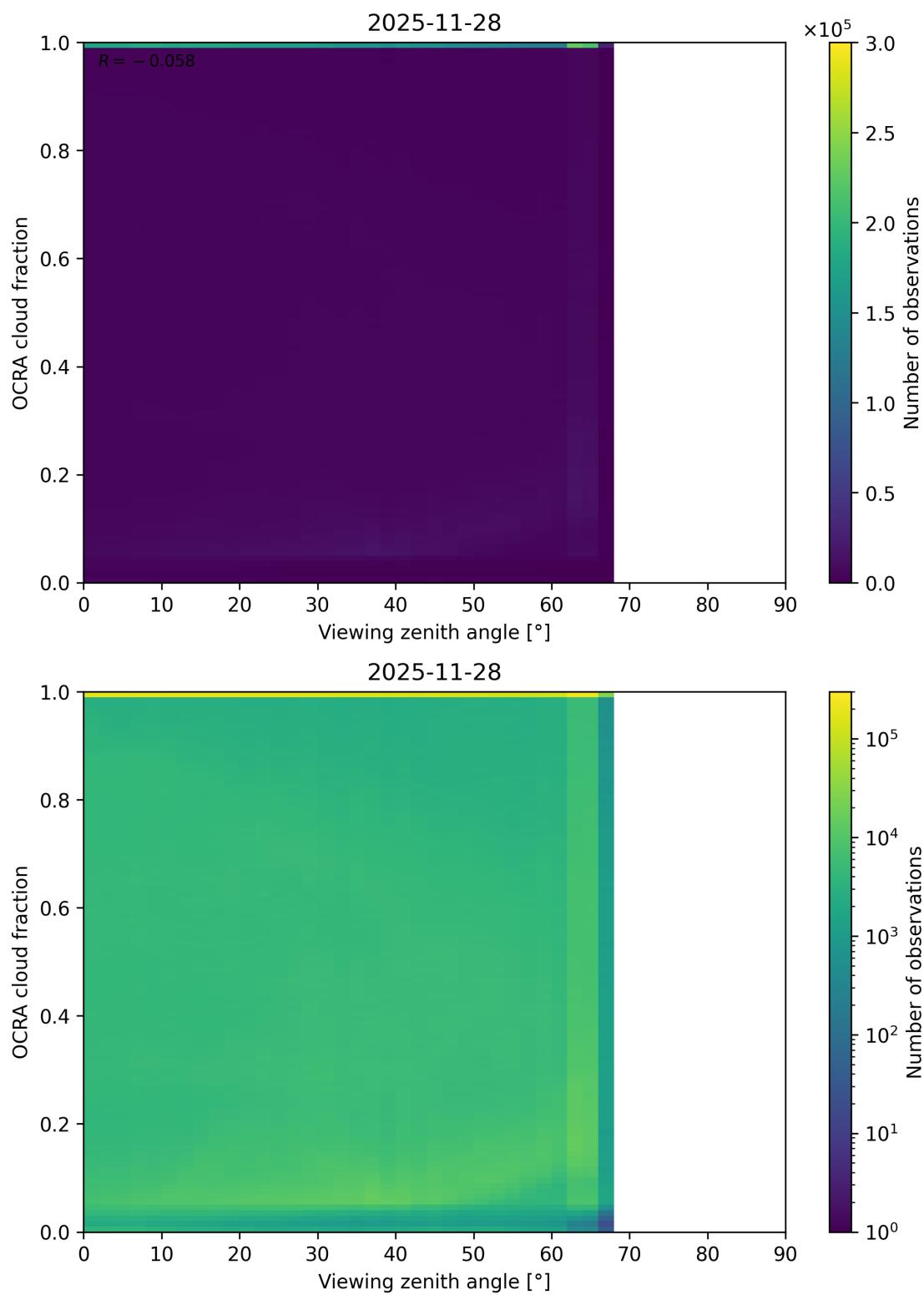
Figure 108: Scatter density plot of “Viewing zenith angle” against “OCRA cloud fraction” for 2025-11-28 to 2025-11-29.
