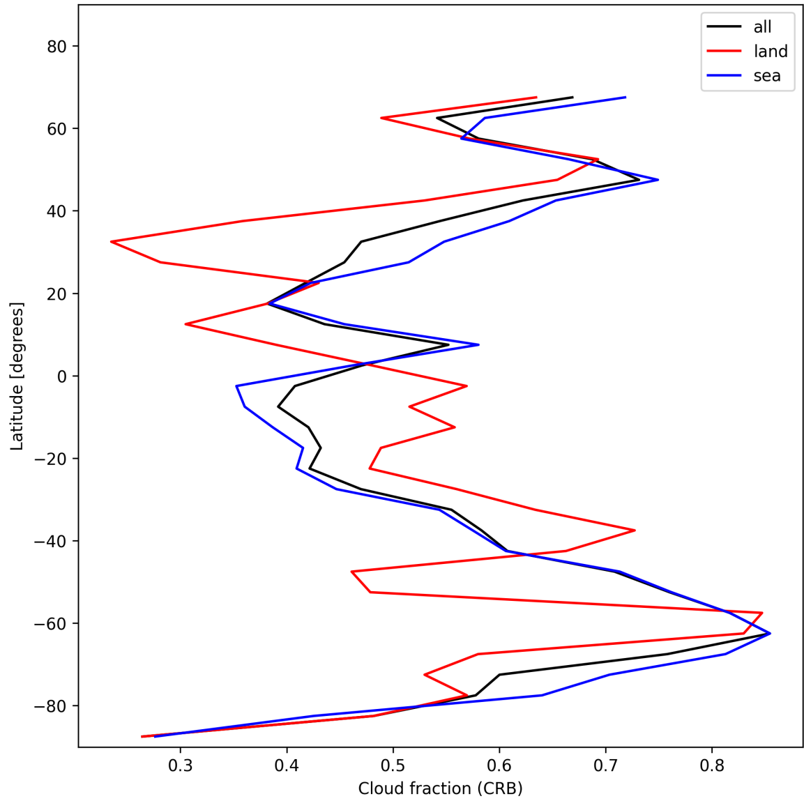
Figure 26: Zonal average of “Cloud fraction (CRB)” for 2025-11-28 to 2025-11-29.
