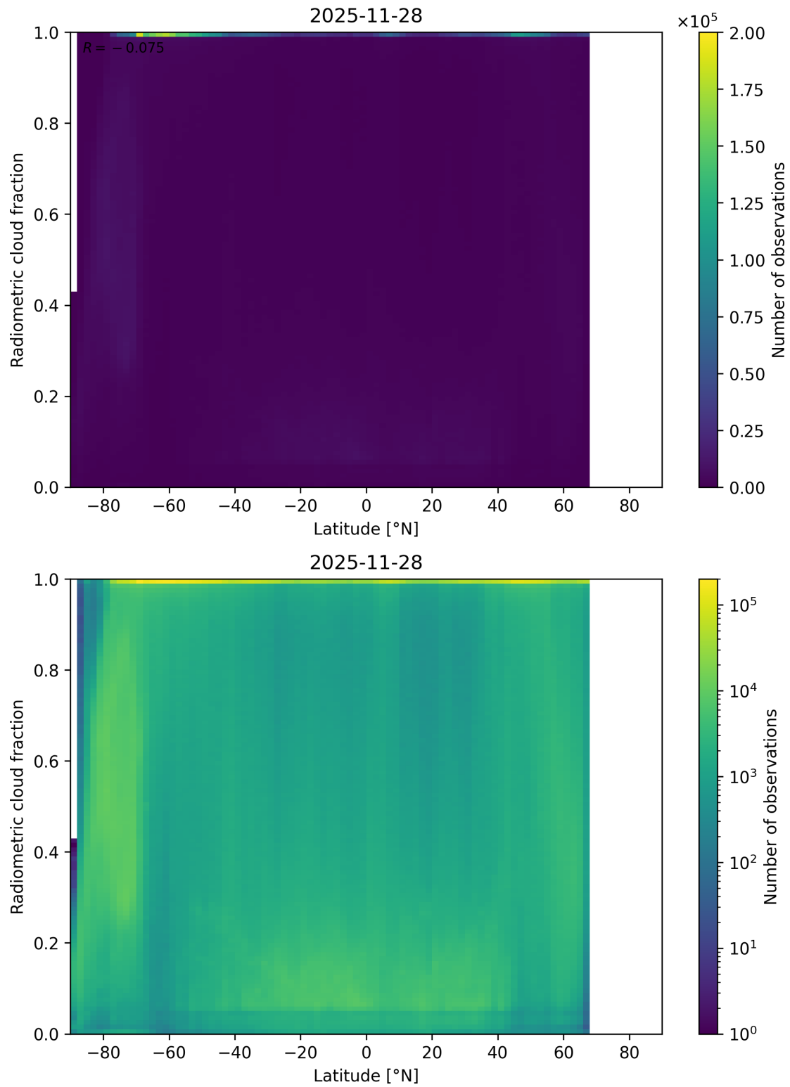
Figure 92: Scatter density plot of “Latitude” against “Radiometric cloud fraction” for 2025-11-28 to 2025-11-29.
