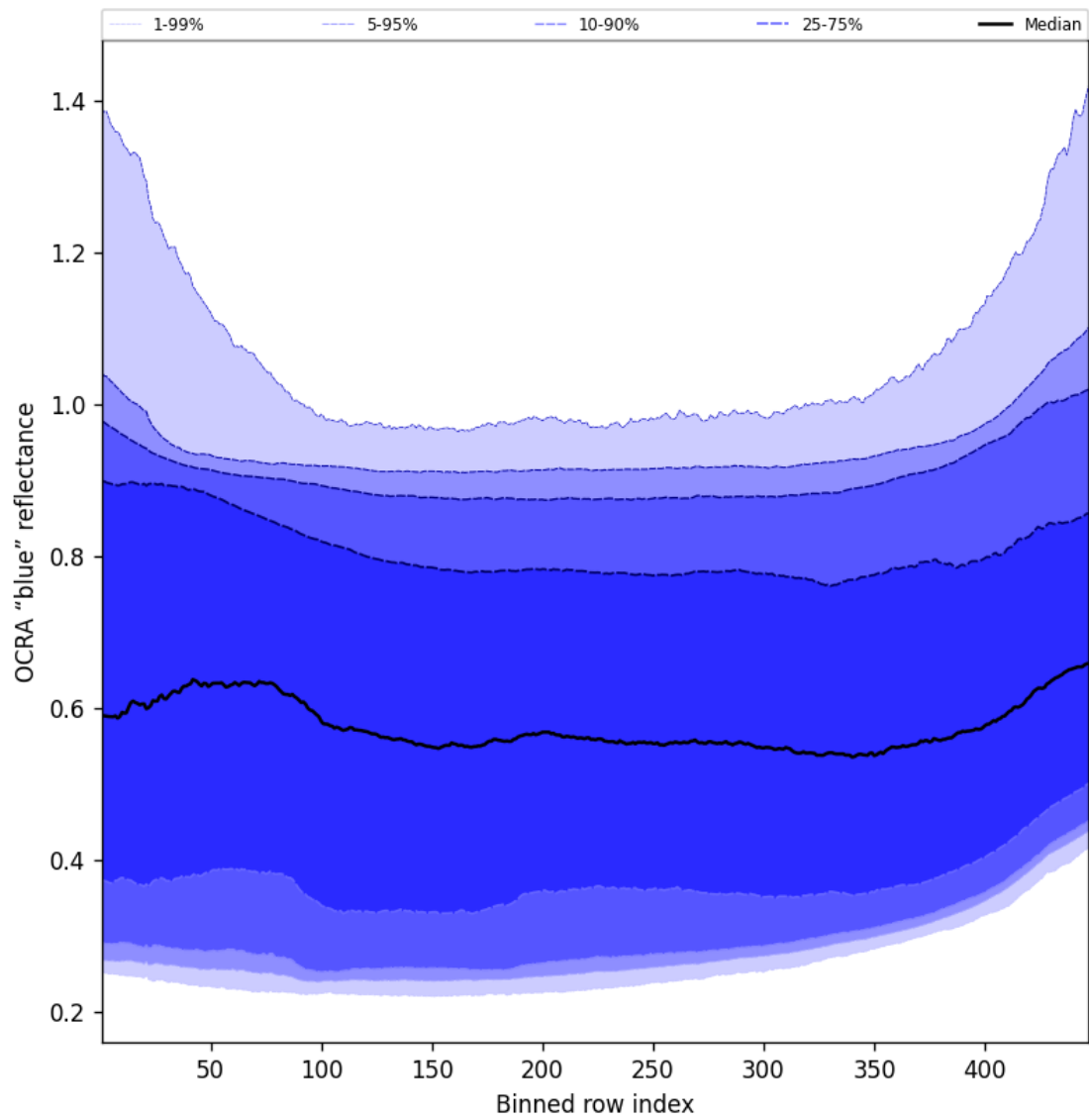
Figure 67: Along track statistics of “OCRA “blue” reflectance” for 2025-11-28 to 2025-11-29
