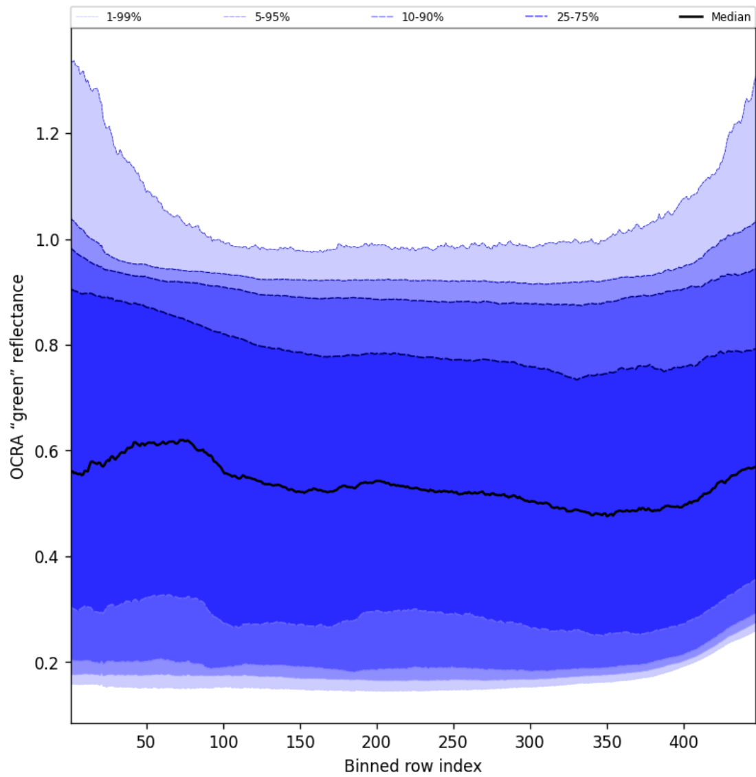
Figure 68: Along track statistics of "OCRA "green" reflectance" for 2025-11-28 to 2025-11-29
