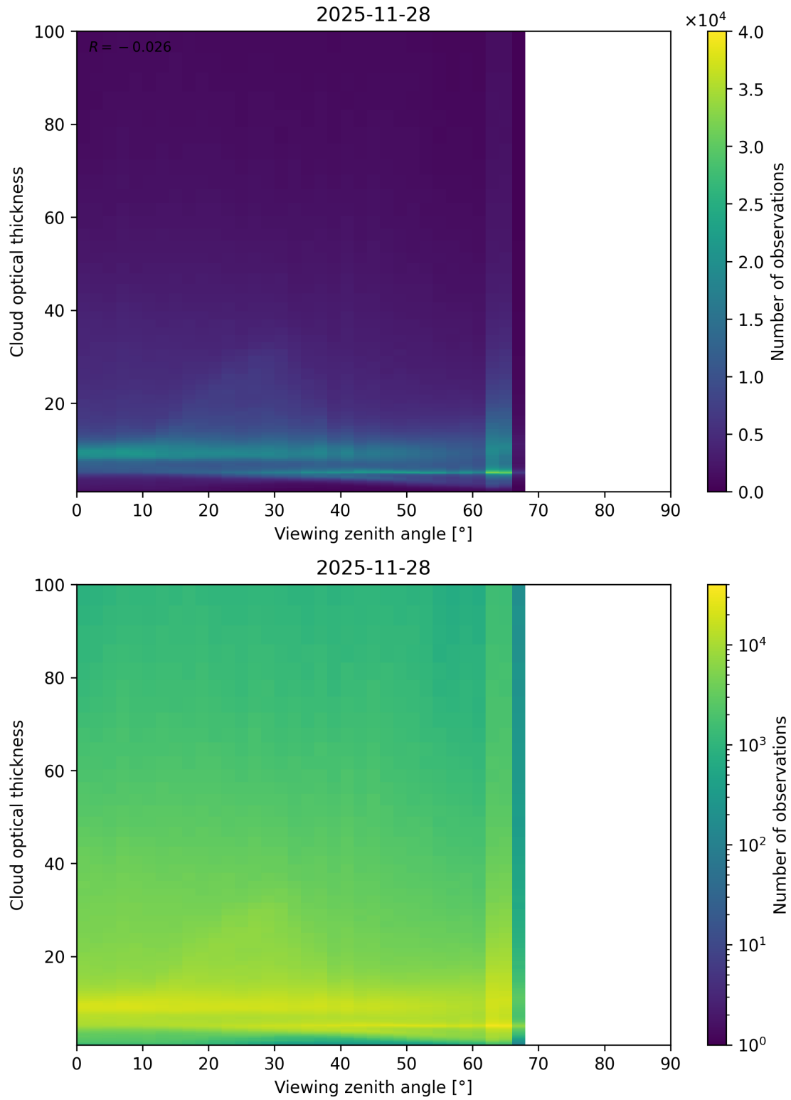
Figure 111: Scatter density plot of “Viewing zenith angle” against “Cloud optical thickness” for 2025-11-28 to 2025-11-29.
