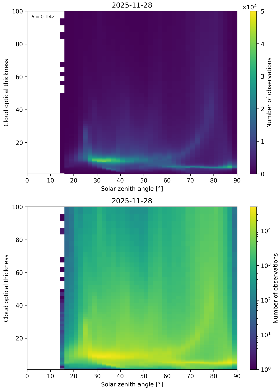
Figure 103: Scatter density plot of “Solar zenith angle” against “Cloud optical thickness” for 2025-11-28 to 2025-11-29.
