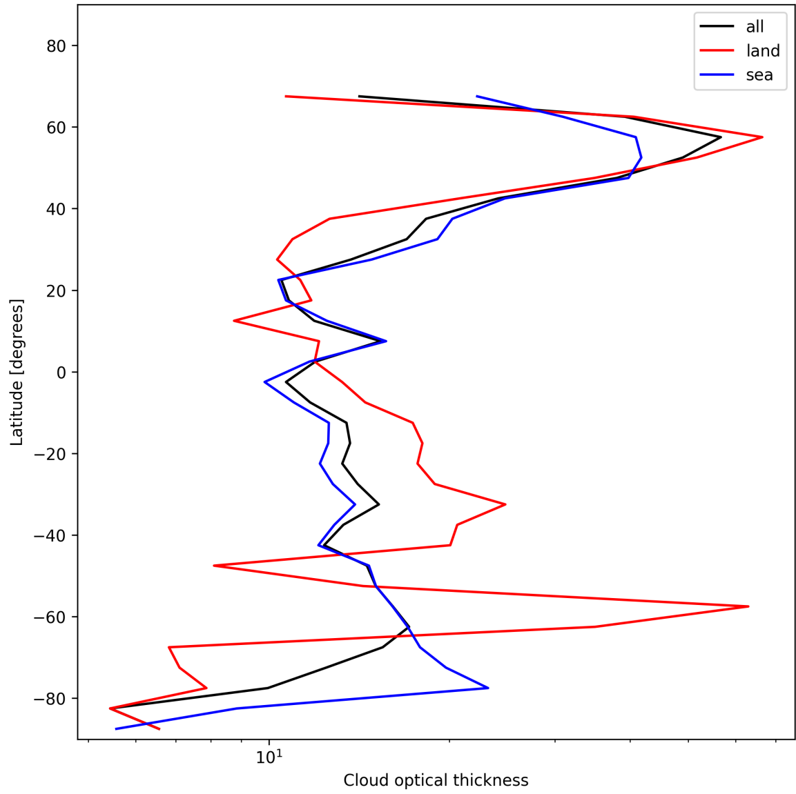
Figure 25: Zonal average of “Cloud optical thickness” for 2025-11-28 to 2025-11-29.
