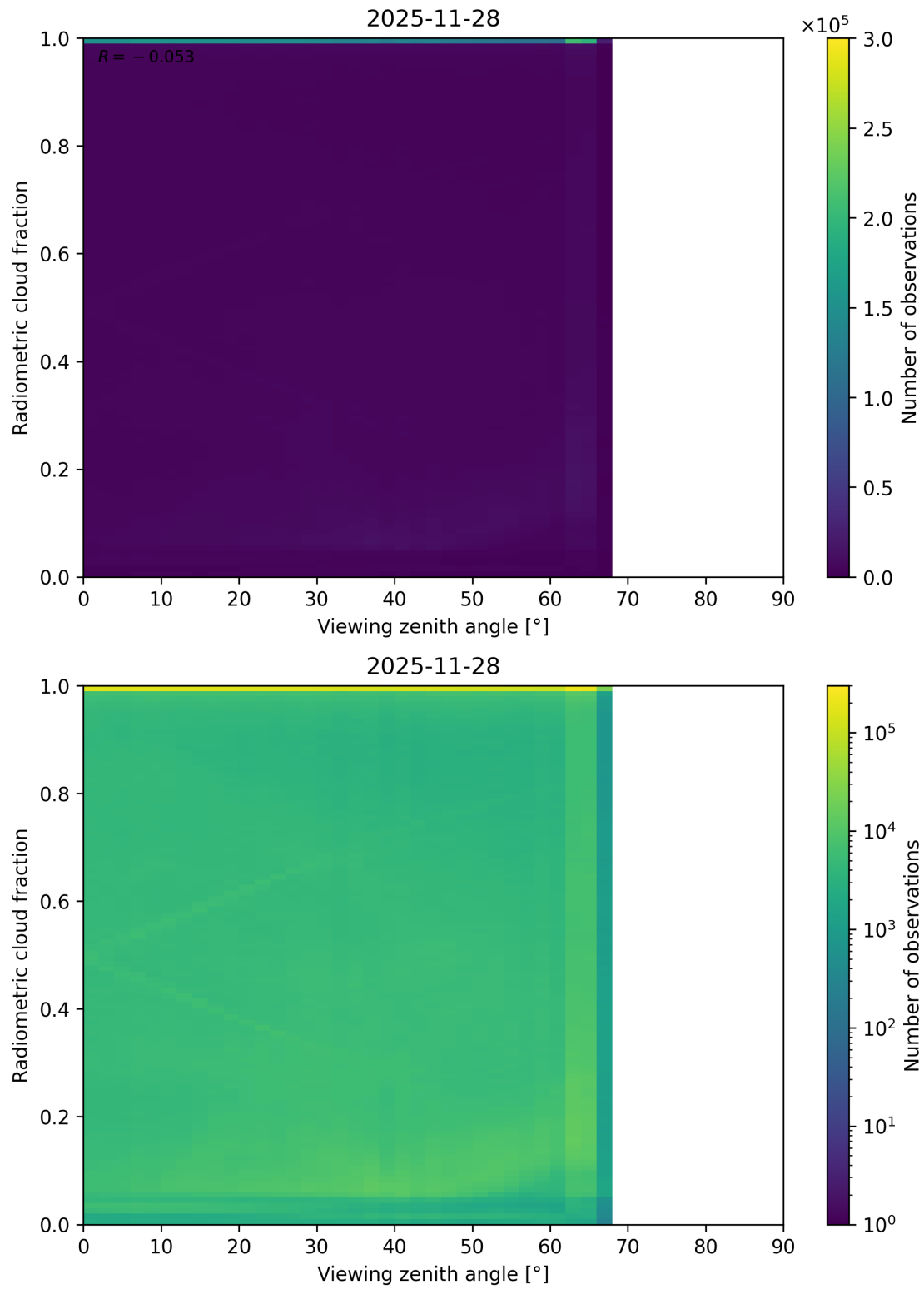
Figure 107: Scatter density plot of “Viewing zenith angle” against “Radiometric cloud fraction” for 2025-11-28 to 2025-11-29.
