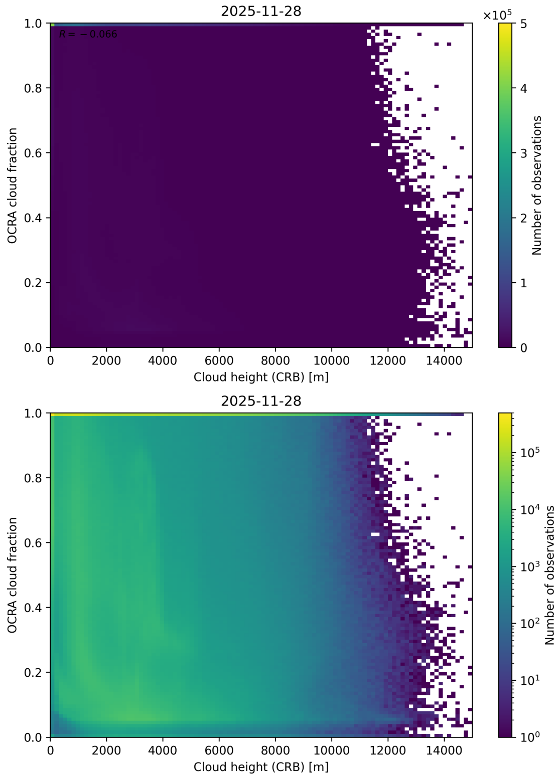
Figure 81: Scatter density plot of “Cloud height (CRB)” against “OCRA cloud fraction” for 2025-11-28 to 2025-11-29.
