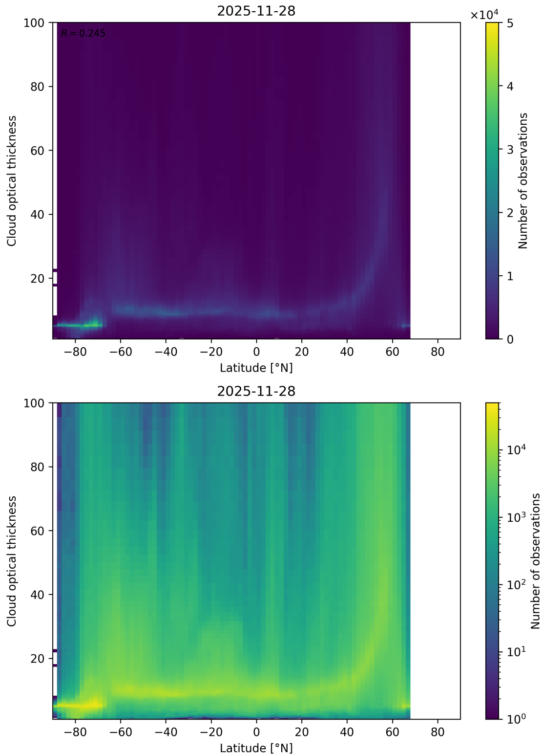
Figure 96: Scatter density plot of “Latitude” against “Cloud optical thickness” for 2025-11-28 to 2025-11-29.
