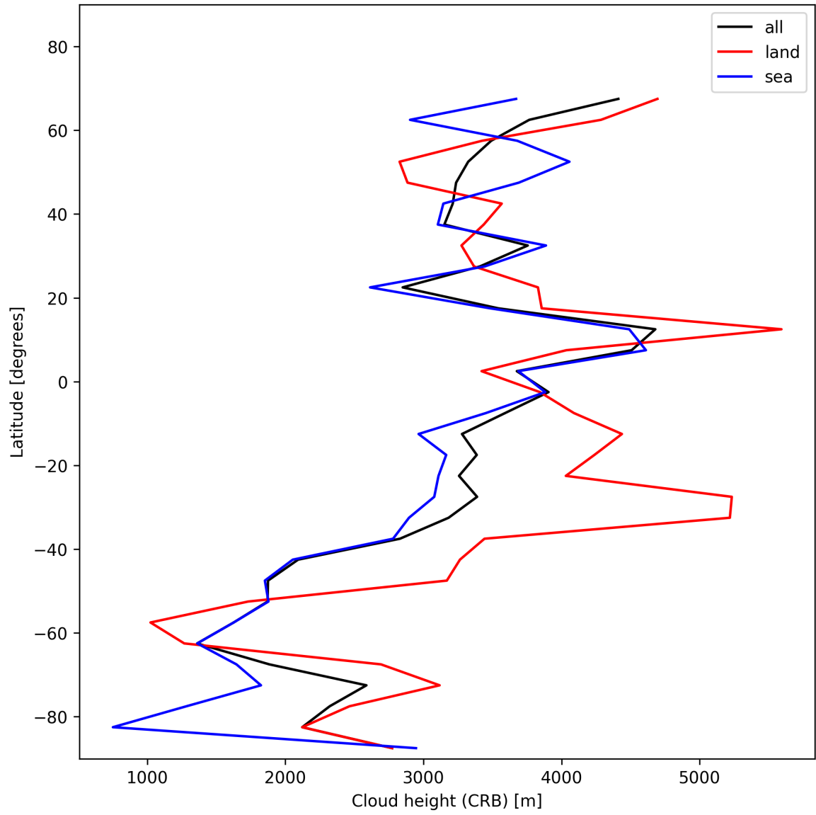
Figure 27: Zonal average of “Cloud height (CRB)” for 2025-11-28 to 2025-11-29.
