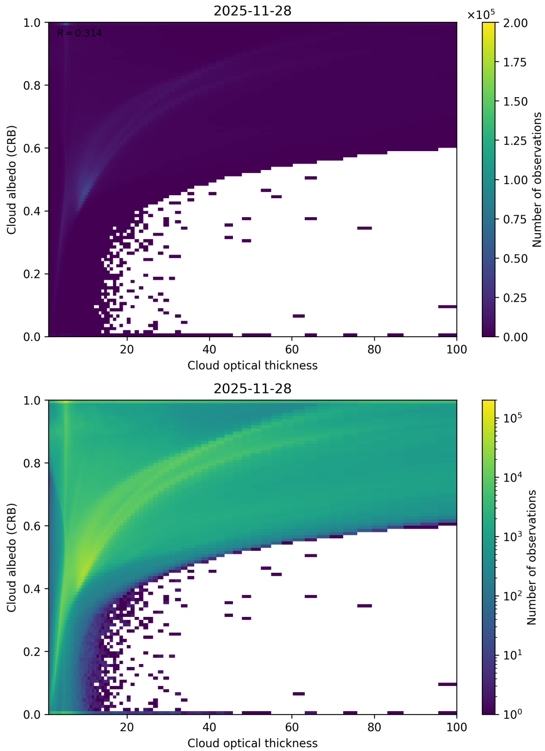
Figure 82: Scatter density plot of “Cloud optical thickness” against “Cloud albedo (CRB)” for 2025-11-28 to 2025-11-29.
