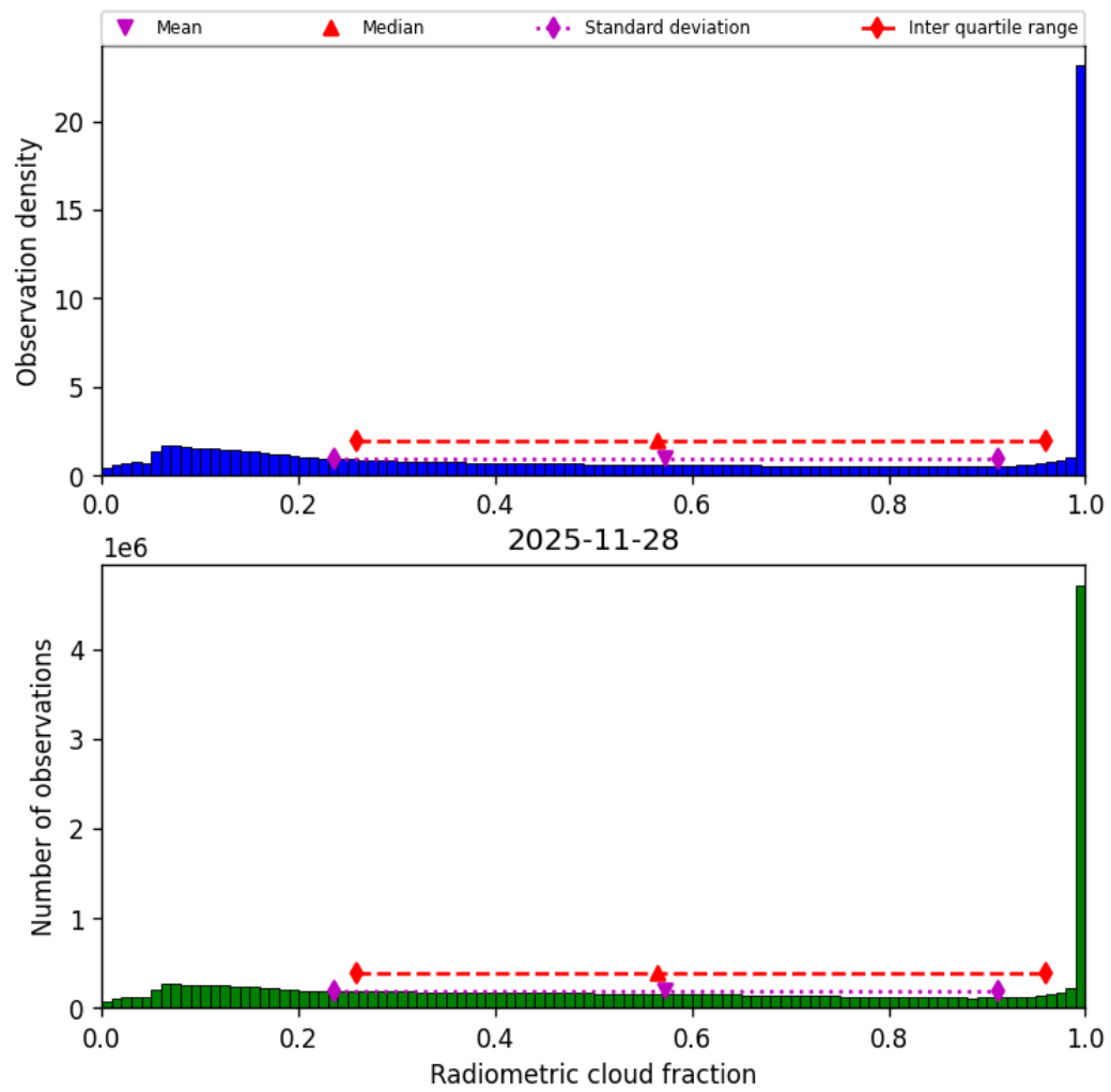
Figure 39: Histogram of “Radiometric cloud fraction” for 2025-11-28 to 2025-11-29
