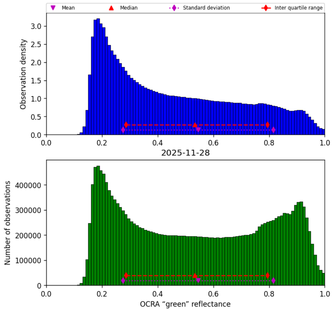
Figure 52: Histogram of “OCRA “green” reflectance” for 2025-11-28 to 2025-11-29
