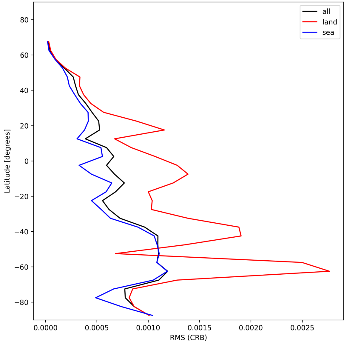
Figure 32: Zonal average of “RMS (CRB)” for 2025-11-29 to 2025-12-01.
