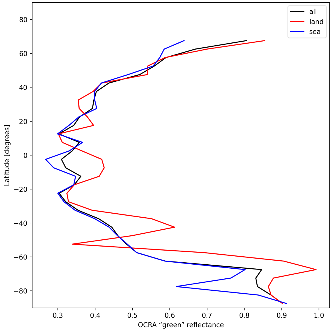
Figure 36: Zonal average of “OCRA “green” reflectance” for 2025-11-29 to 2025-12-01.
