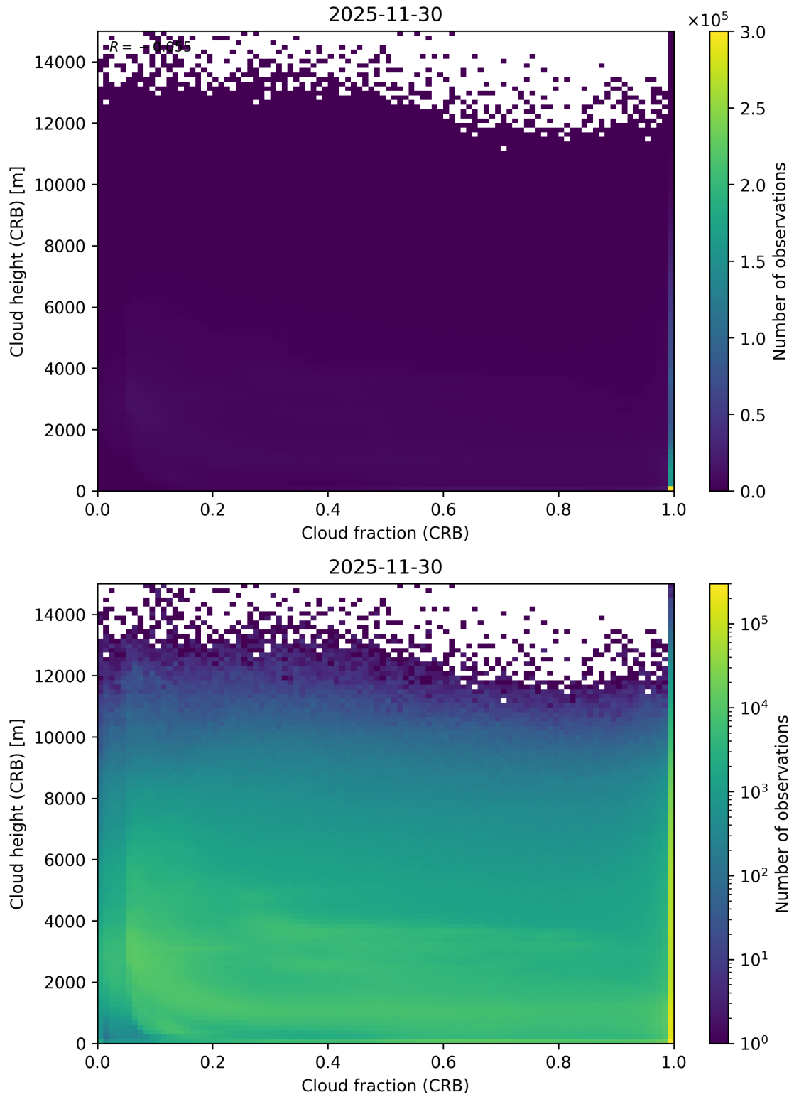
Figure 79: Scatter density plot of “Cloud fraction (CRB)” against “Cloud height (CRB)” for 2025-11-29 to 2025-12-01.
