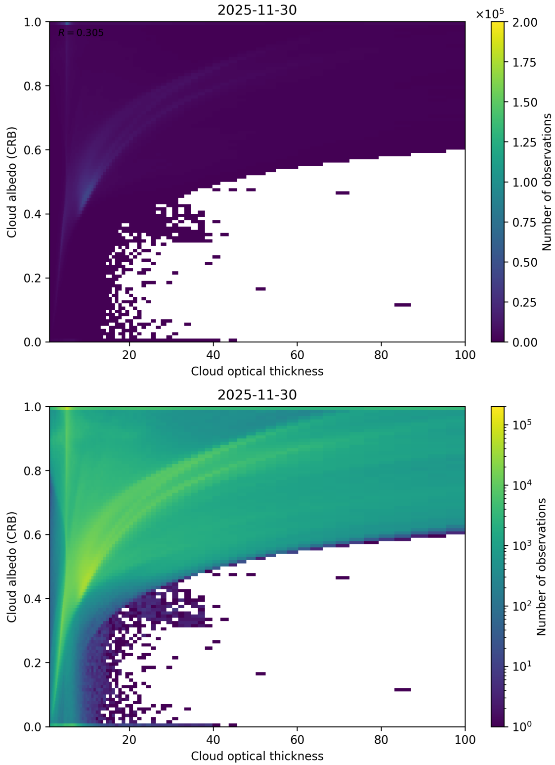
Figure 82: Scatter density plot of “Cloud optical thickness” against “Cloud albedo (CRB)” for 2025-11-29 to 2025-12-01.
