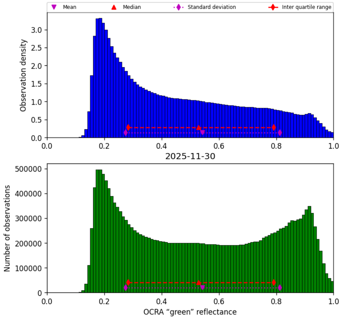
Figure 52: Histogram of “OCRA “green” reflectance” for 2025-11-29 to 2025-12-01
