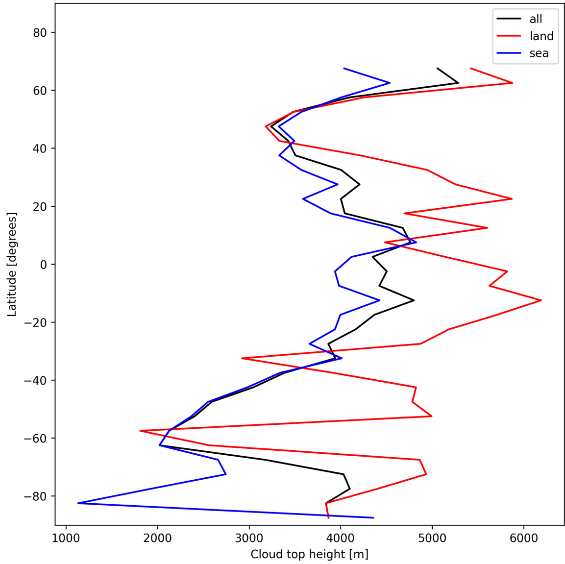
Figure 24: Zonal average of “Cloud top height” for 2025-11-29 to 2025-12-01.
