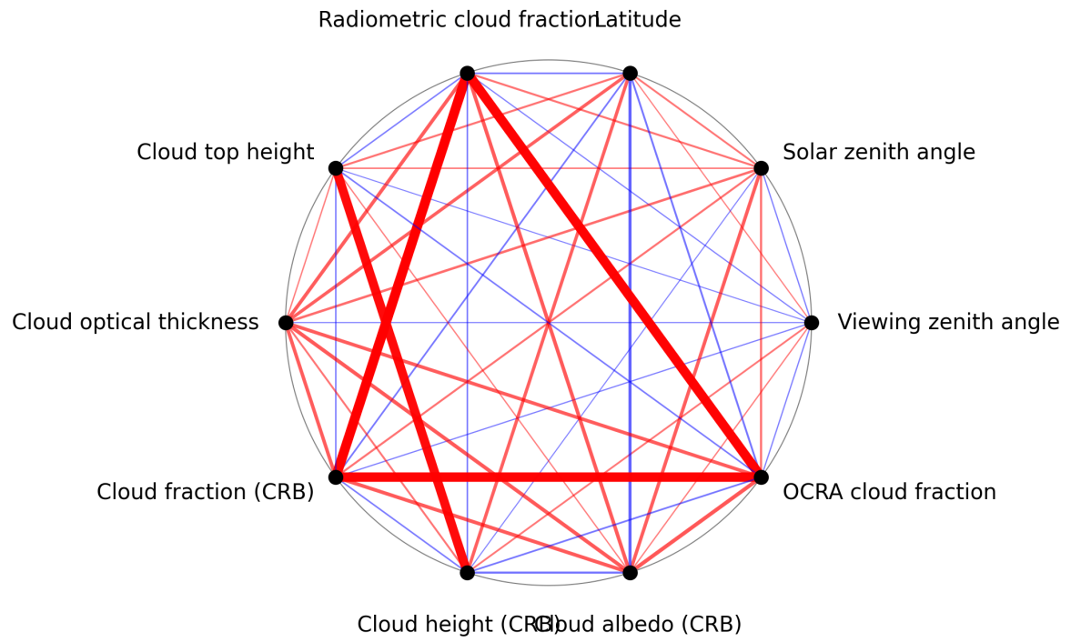
Figure 1: Map of correlation graph for 2025-11-29 to 2025-12-01.
