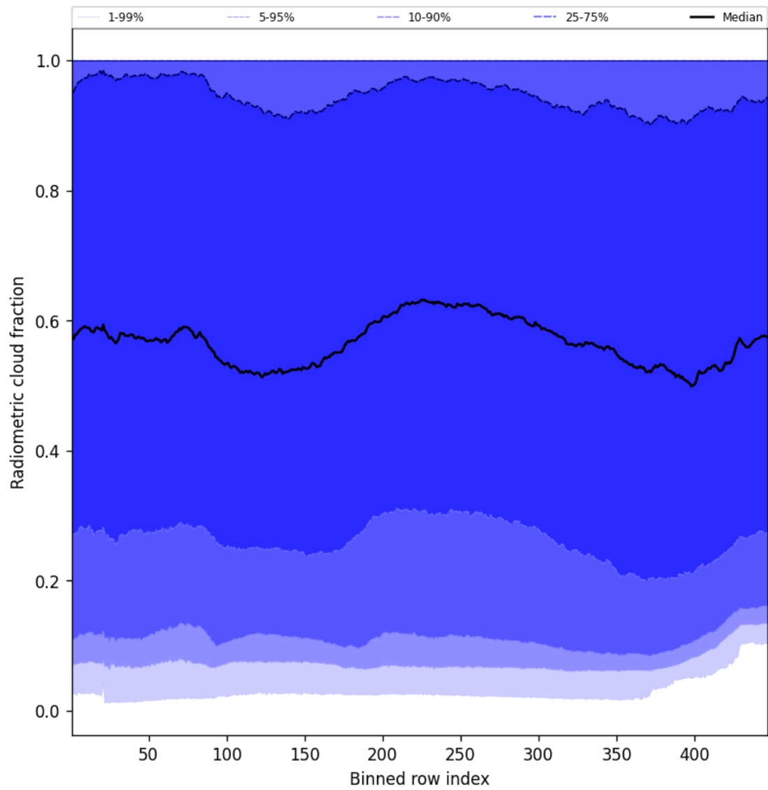
Figure 55: Along track statistics of “Radiometric cloud fraction” for 2025-11-29 to 2025-12-01
