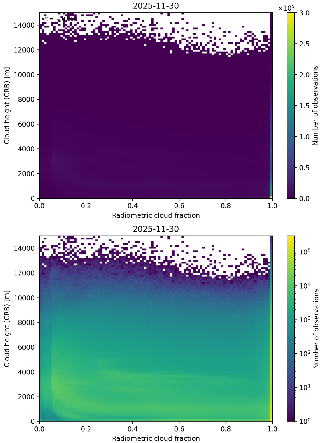
Figure 74: Scatter density plot of “Radiometric cloud fraction” against “Cloud height (CRB)” for 2025-11-29 to 2025-12-01.
