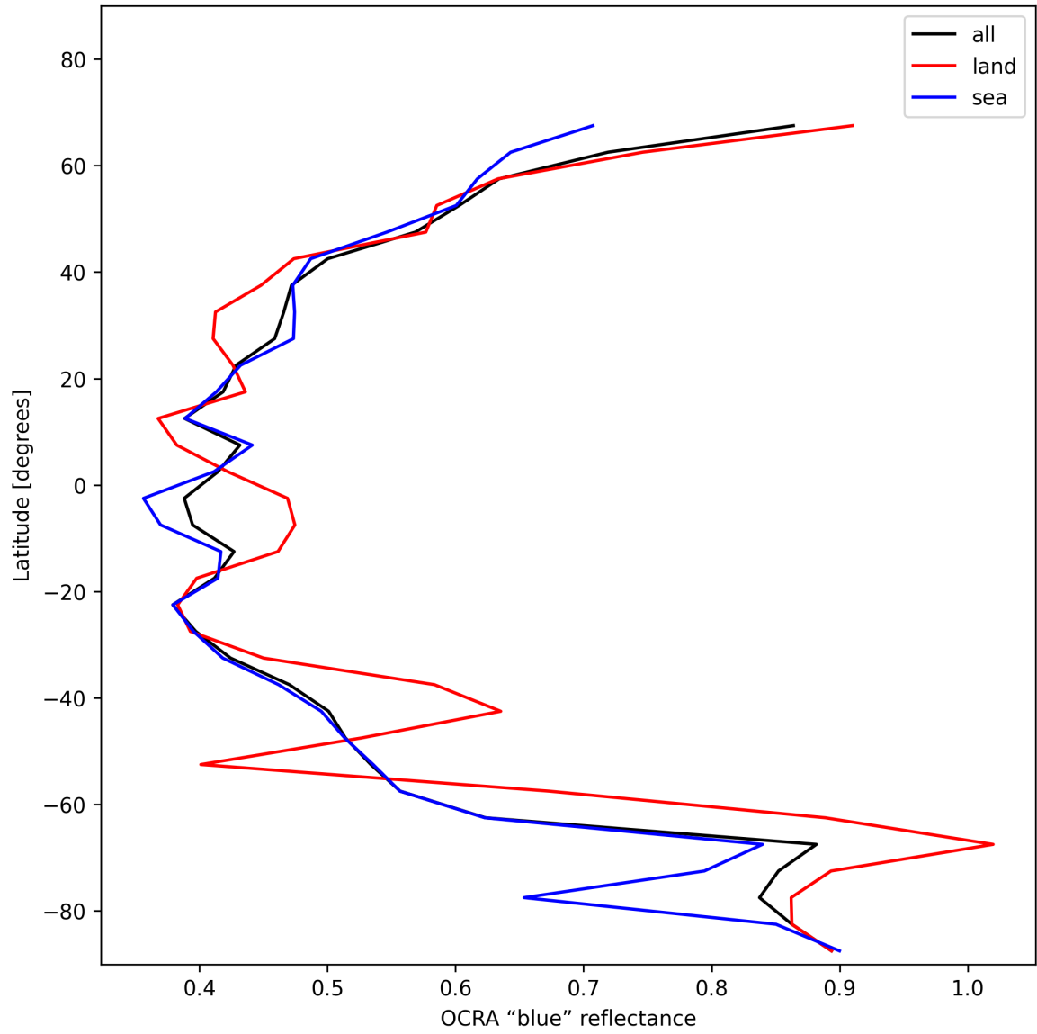
Figure 35: Zonal average of “OCRA “blue” reflectance” for 2025-11-29 to 2025-12-01.
