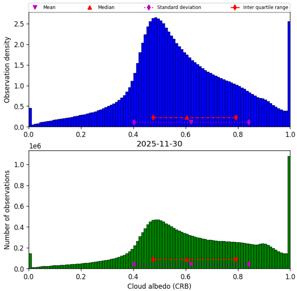
Figure 44: Histogram of “Cloud albedo (CRB)” for 2025-11-29 to 2025-12-01
