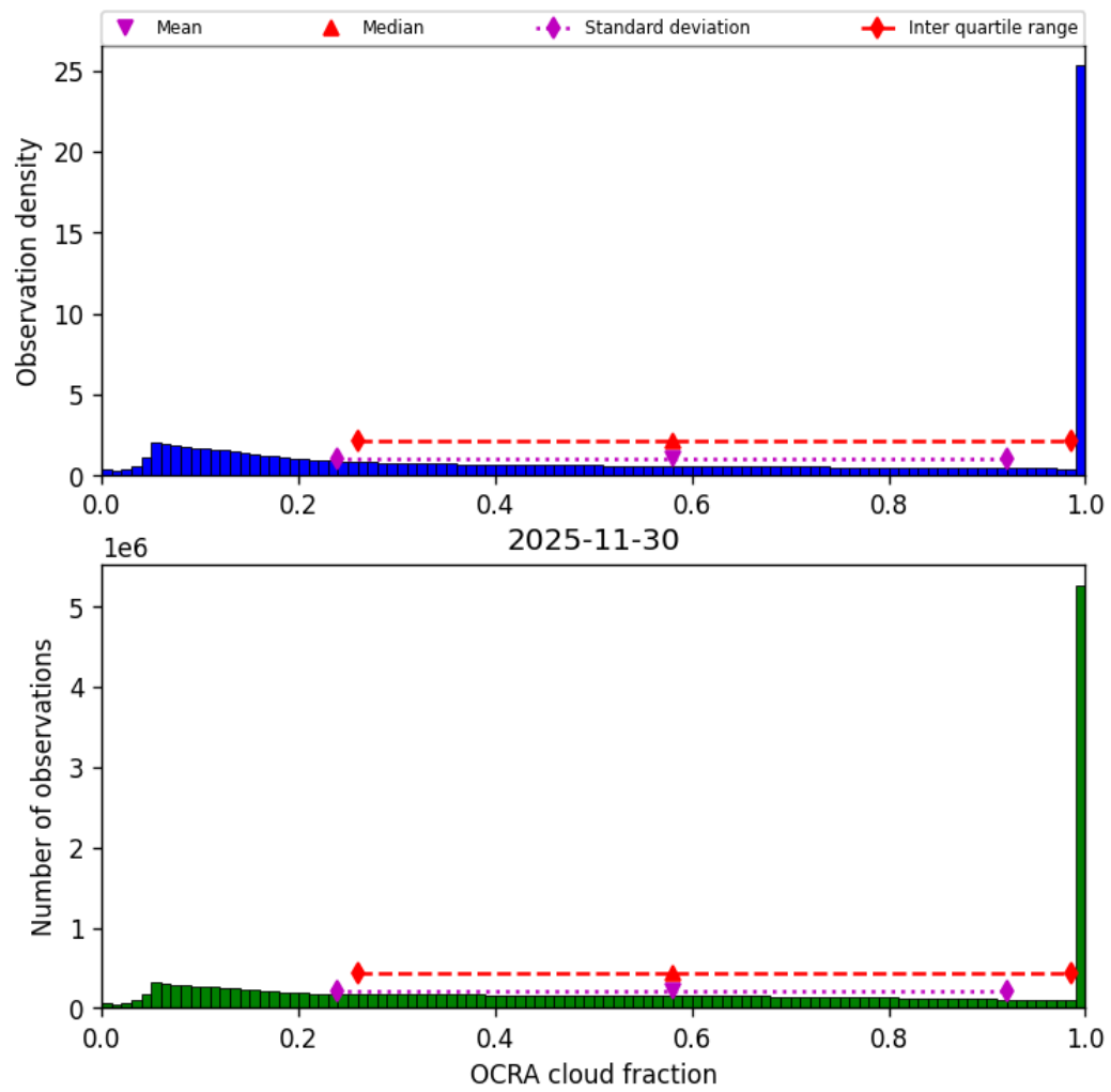
Figure 50: Histogram of “OCRA cloud fraction” for 2025-11-29 to 2025-12-01
