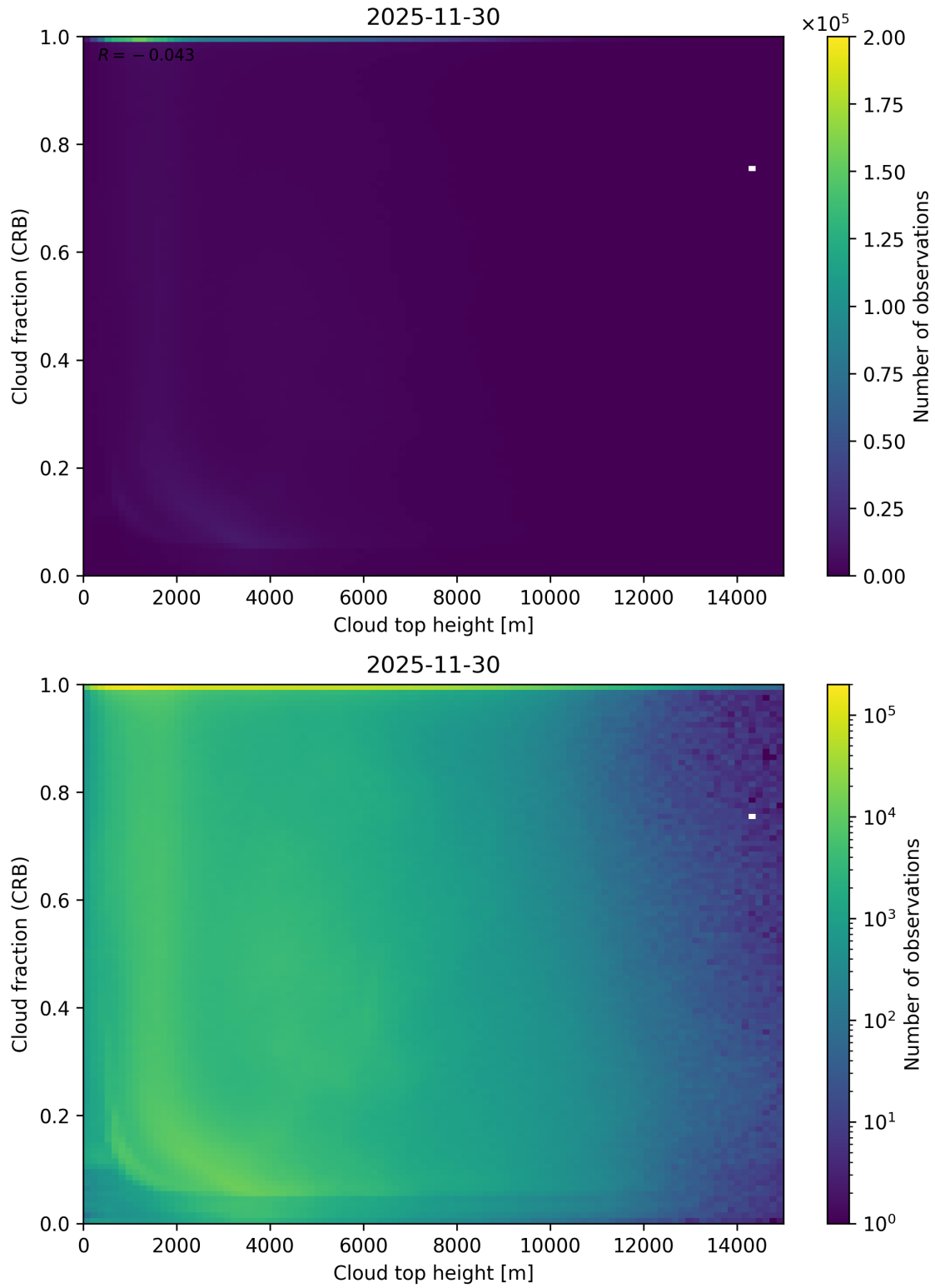
Figure 88: Scatter density plot of “Cloud top height” against “Cloud fraction (CRB)” for 2025-11-29 to 2025-12-01.
