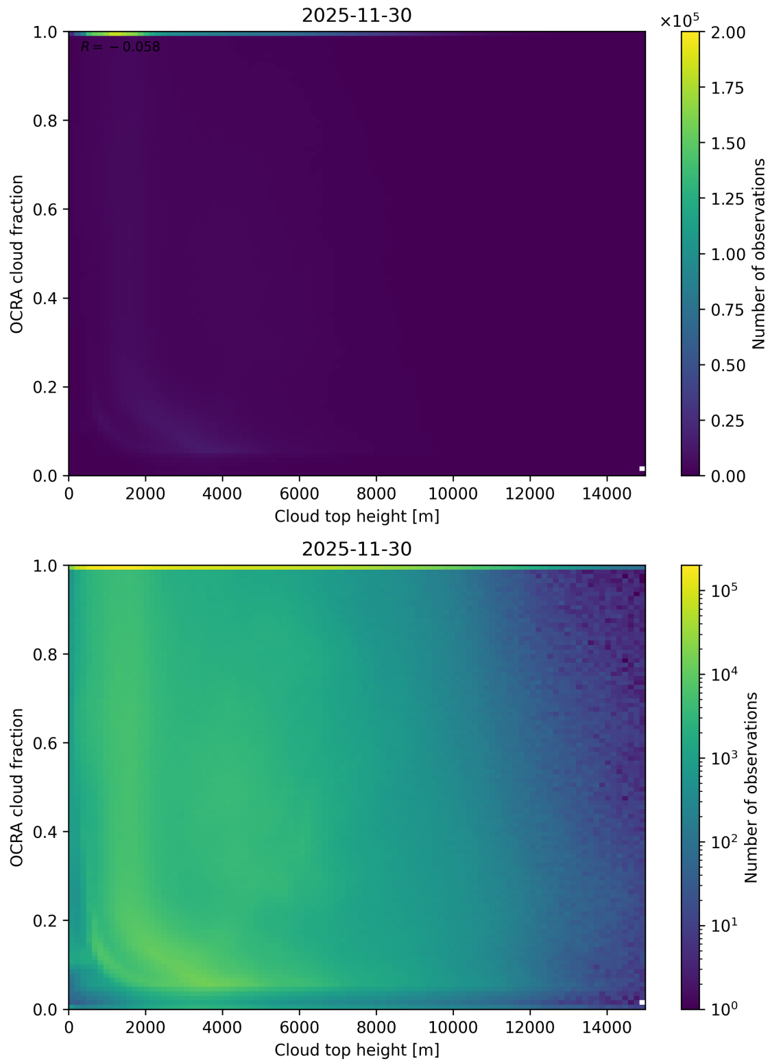
Figure 87: Scatter density plot of “Cloud top height” against “OCRA cloud fraction” for 2025-11-29 to 2025-12-01.
