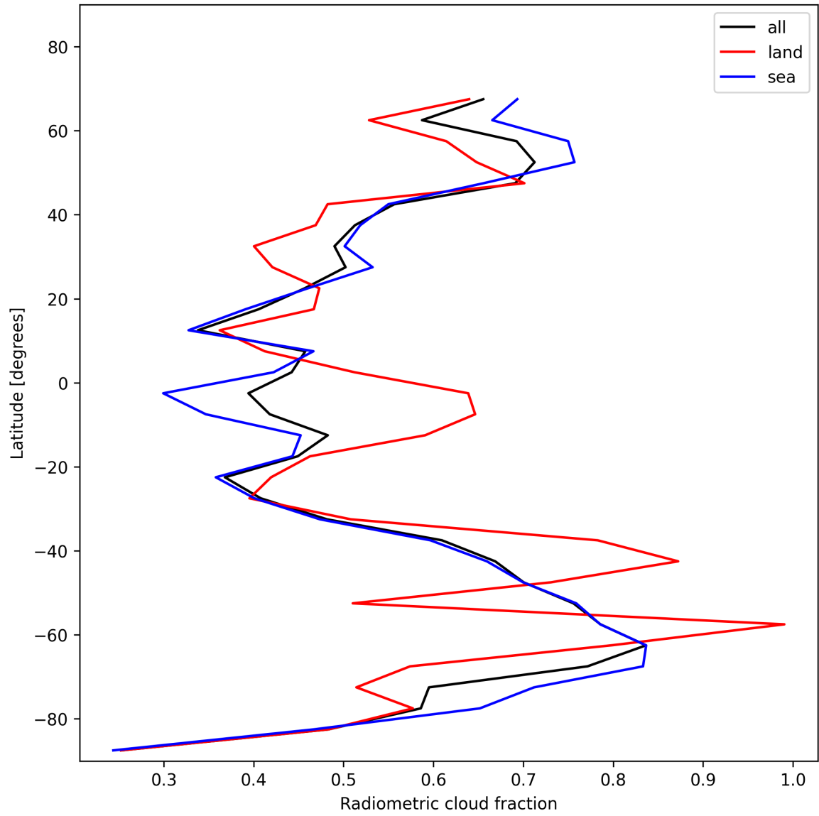
Figure 23: Zonal average of “Radiometric cloud fraction” for 2025-11-29 to 2025-12-01.
