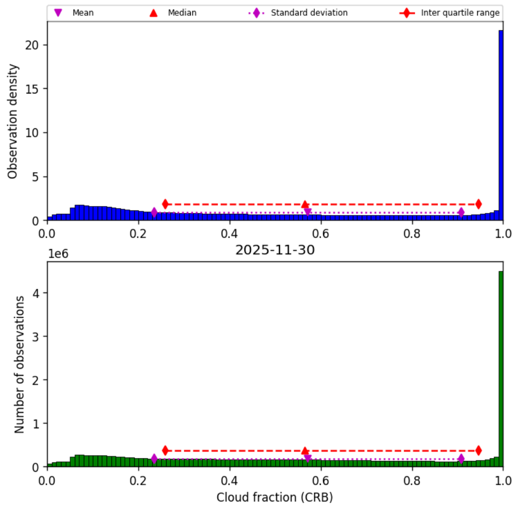
Figure 42: Histogram of “Cloud fraction (CRB)” for 2025-11-29 to 2025-12-01
