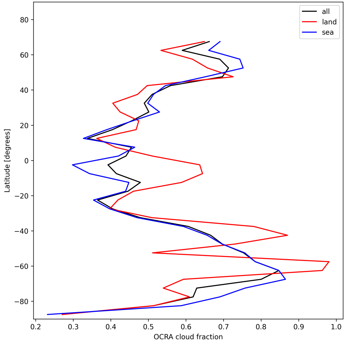
Figure 34: Zonal average of “OCRA cloud fraction” for 2025-11-29 to 2025-12-01.
