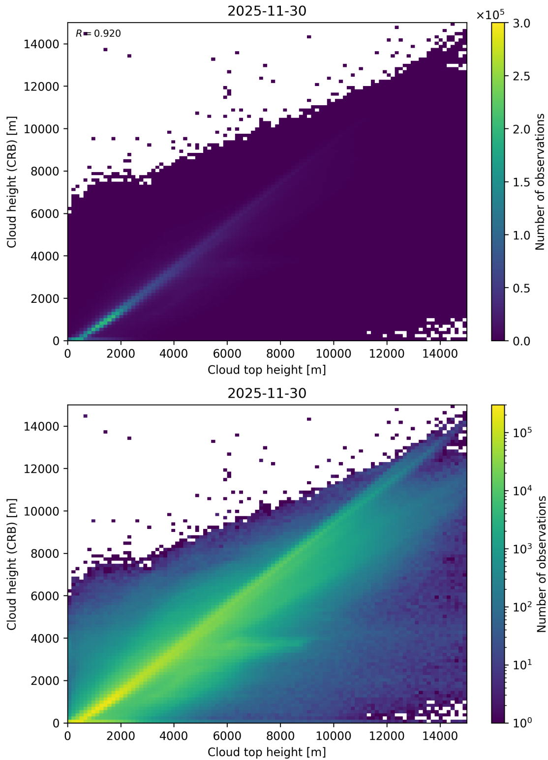
Figure 89: Scatter density plot of “Cloud top height” against “Cloud height (CRB)” for 2025-11-29 to 2025-12-01.
