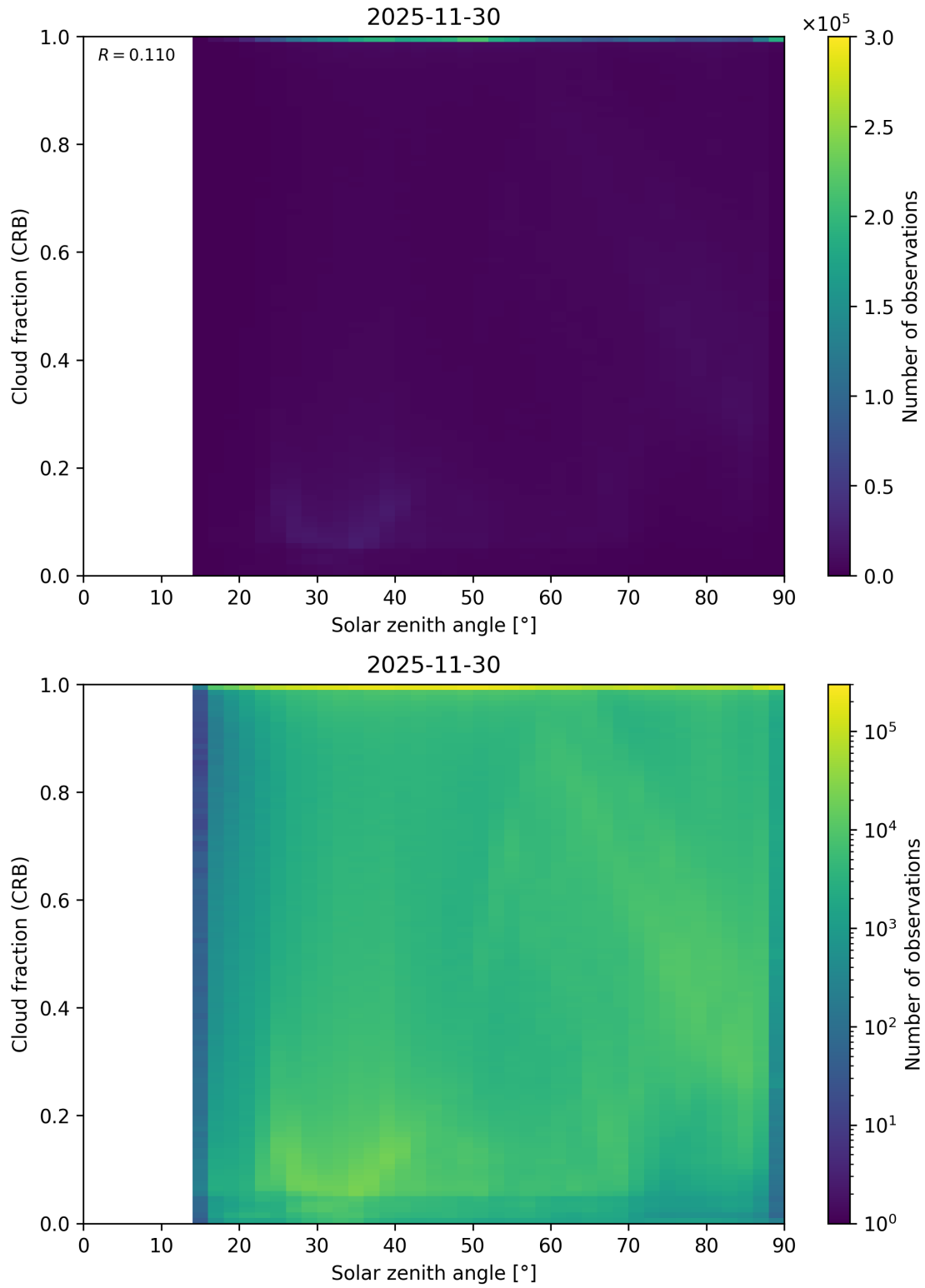
Figure 101: Scatter density plot of “Solar zenith angle” against “Cloud fraction (CRB)” for 2025-11-29 to 2025-12-01.
