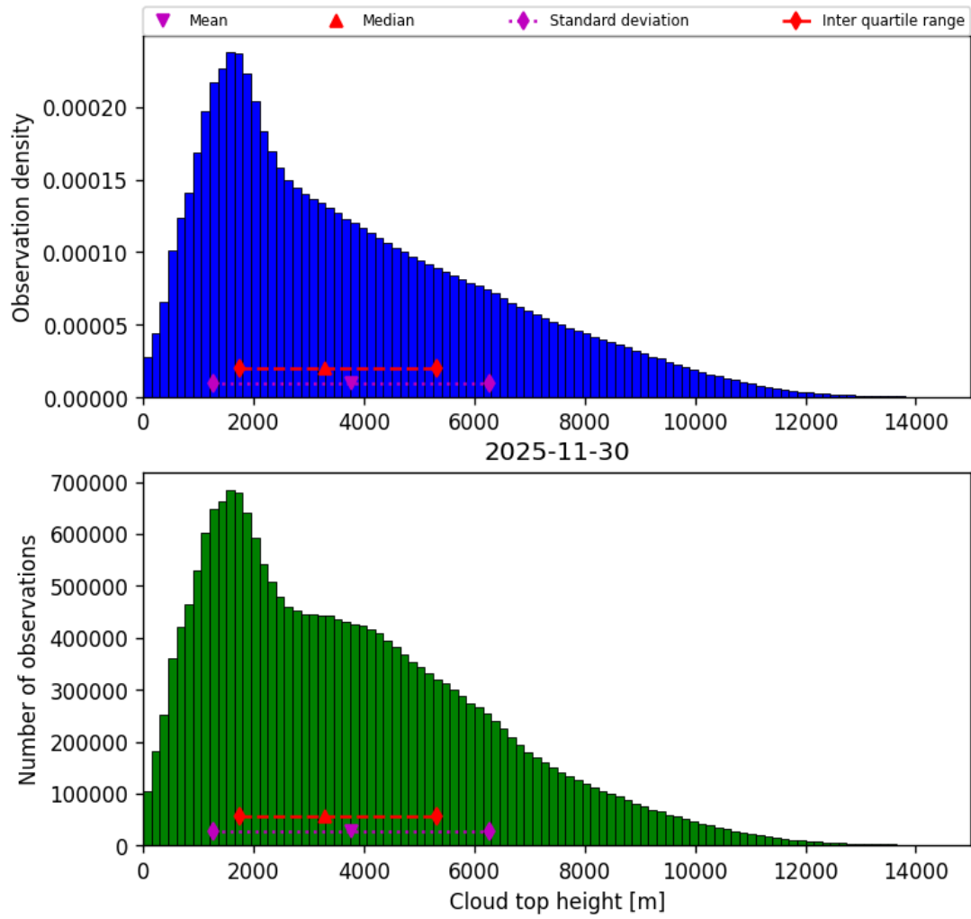
Figure 40: Histogram of “Cloud top height” for 2025-11-29 to 2025-12-01
