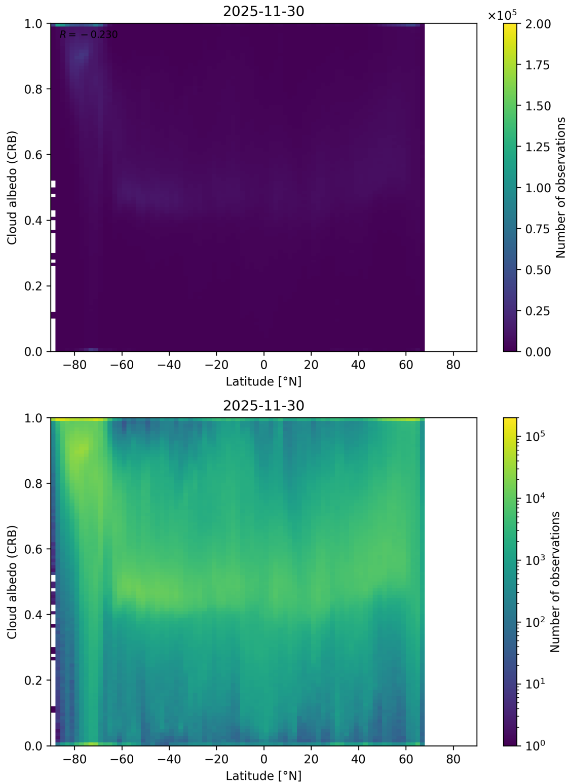
Figure 91: Scatter density plot of “Latitude” against “Cloud albedo (CRB)” for 2025-11-29 to 2025-12-01.
