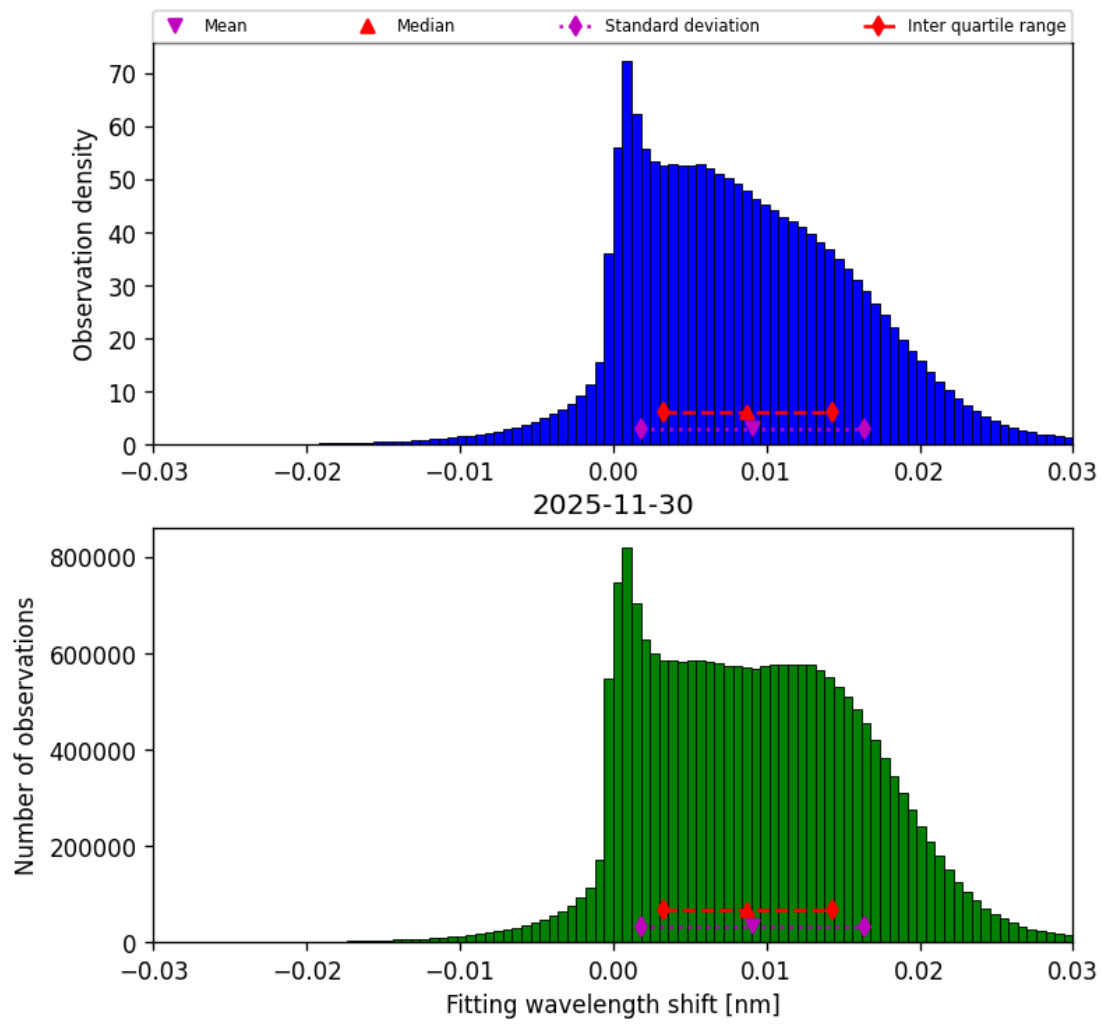
Figure 49: Histogram of “Fitting wavelength shift” for 2025-11-29 to 2025-12-01
