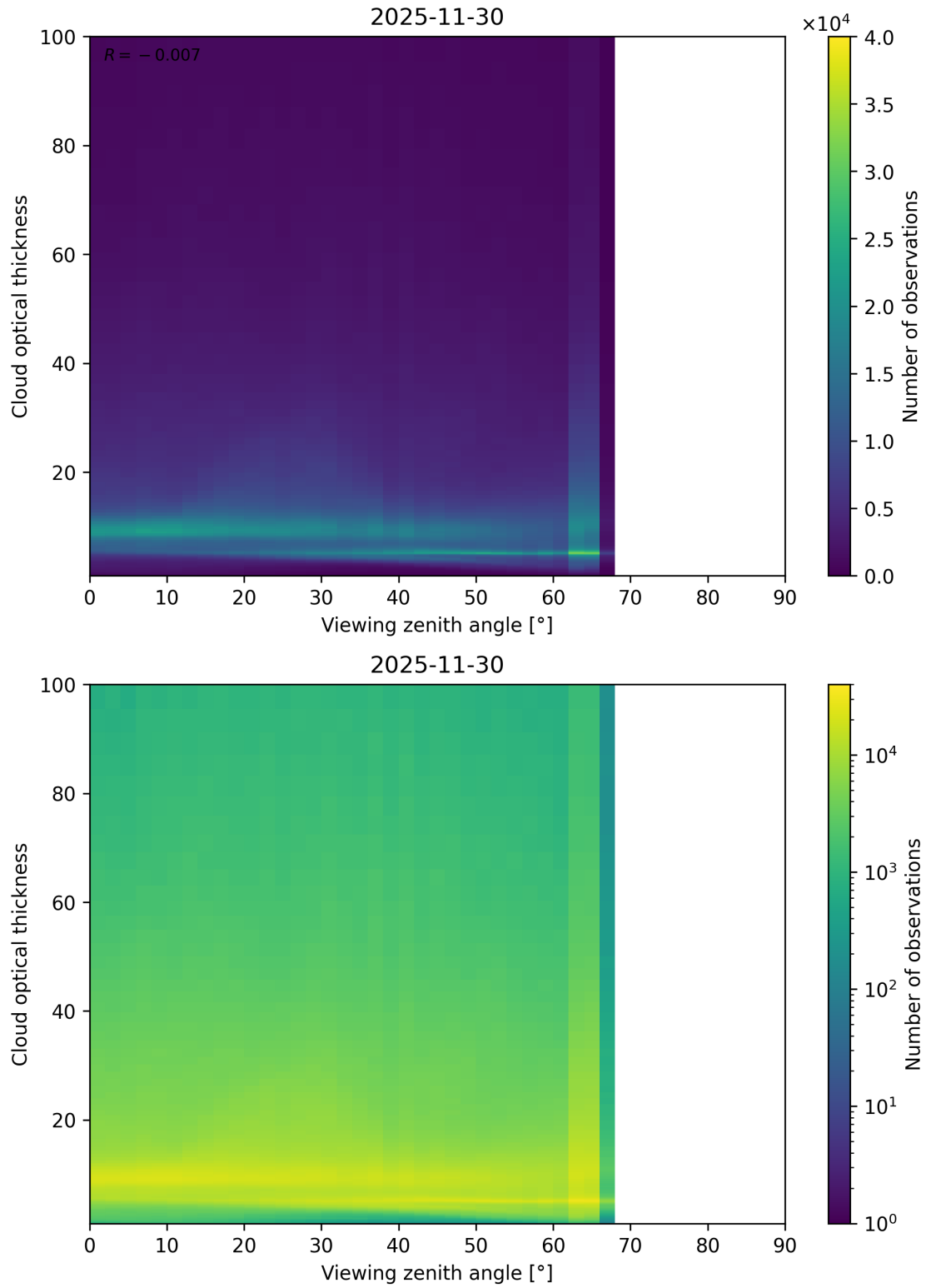
Figure 111: Scatter density plot of “Viewing zenith angle” against “Cloud optical thickness” for 2025-11-29 to 2025-12-01.
