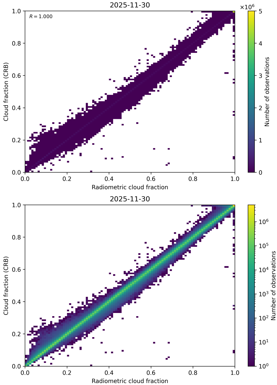
Figure 73: Scatter density plot of “Radiometric cloud fraction” against “Cloud fraction (CRB)” for 2025-11-29 to 2025-12-01.
