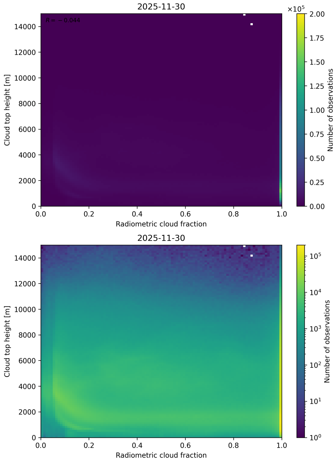
Figure 76: Scatter density plot of “Radiometric cloud fraction” against “Cloud top height” for 2025-11-29 to 2025-12-01.
