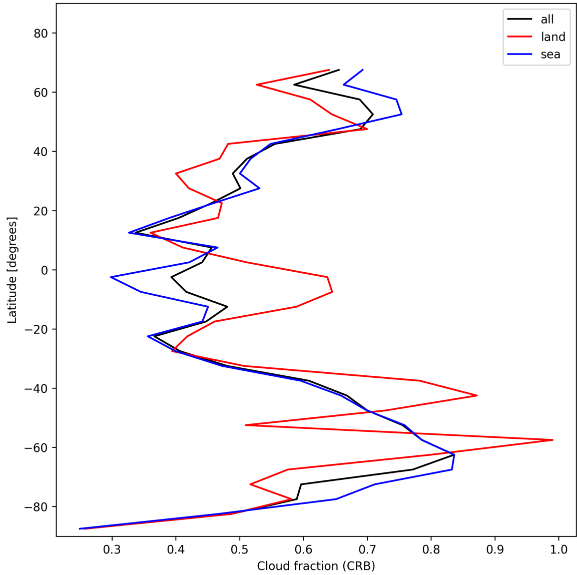
Figure 26: Zonal average of “Cloud fraction (CRB)” for 2025-11-29 to 2025-12-01.
