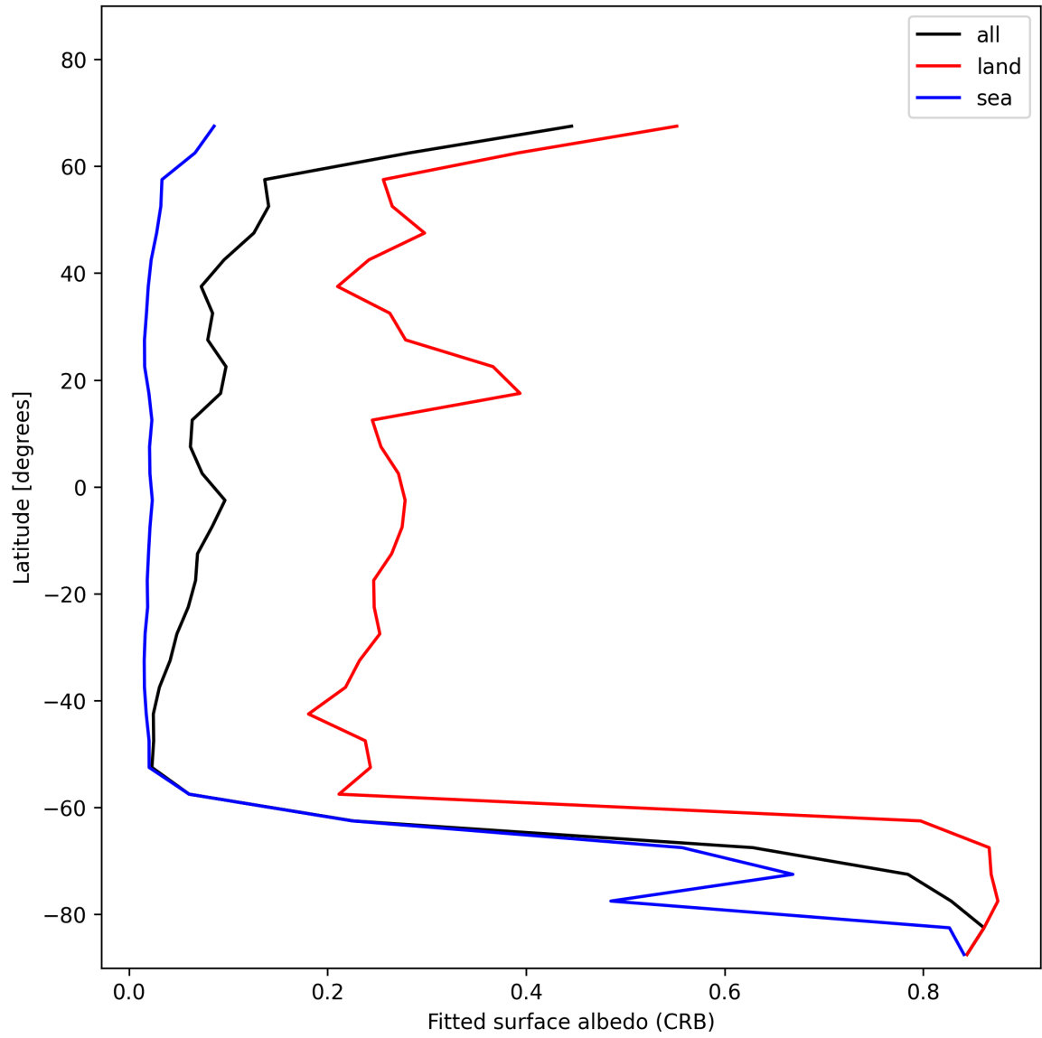
Figure 30: Zonal average of “Fitted surface albedo (CRB)” for 2025-11-29 to 2025-12-01.
