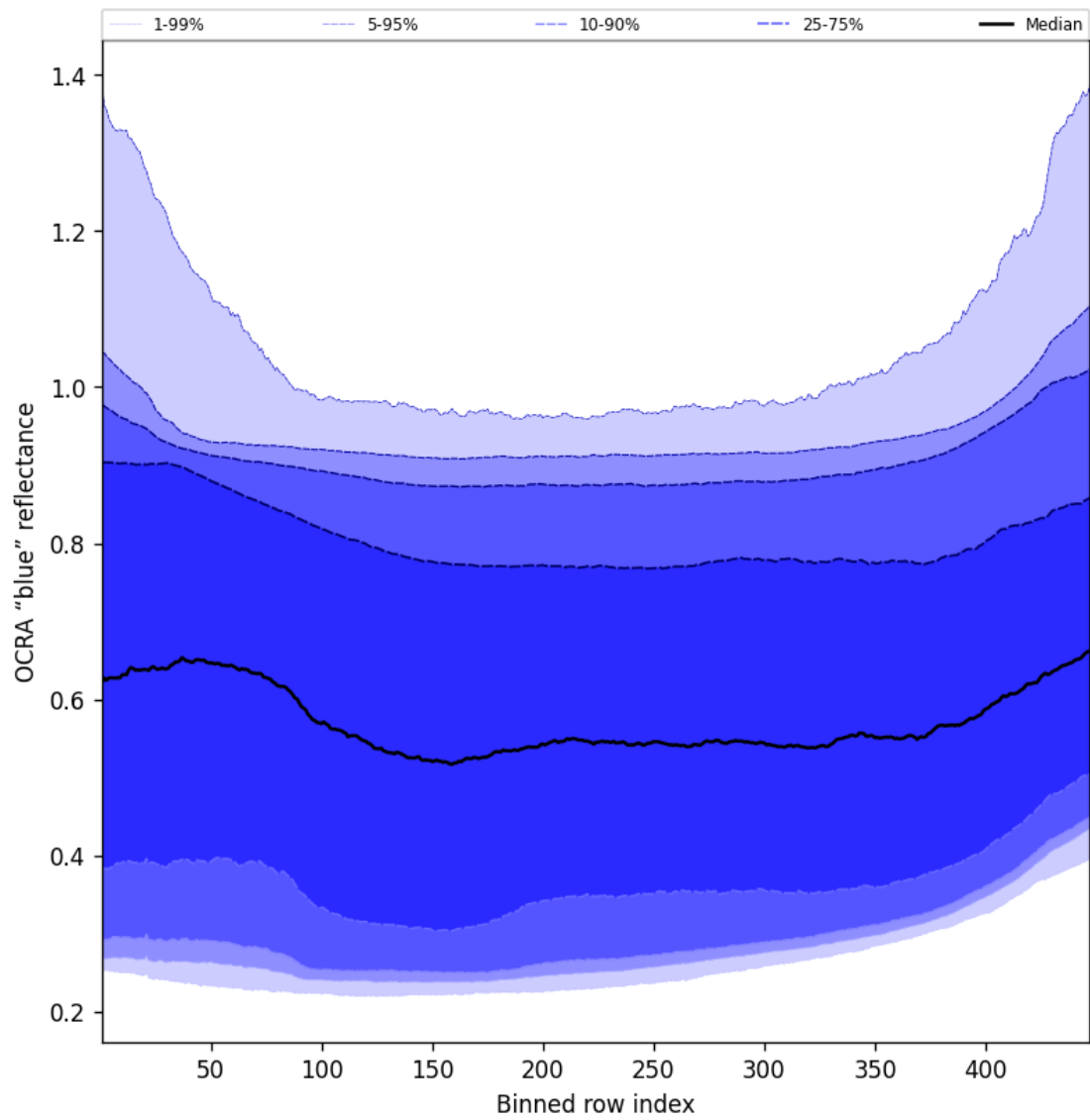
Figure 67: Along track statistics of “OCRA “blue” reflectance” for 2025-11-29 to 2025-12-01
