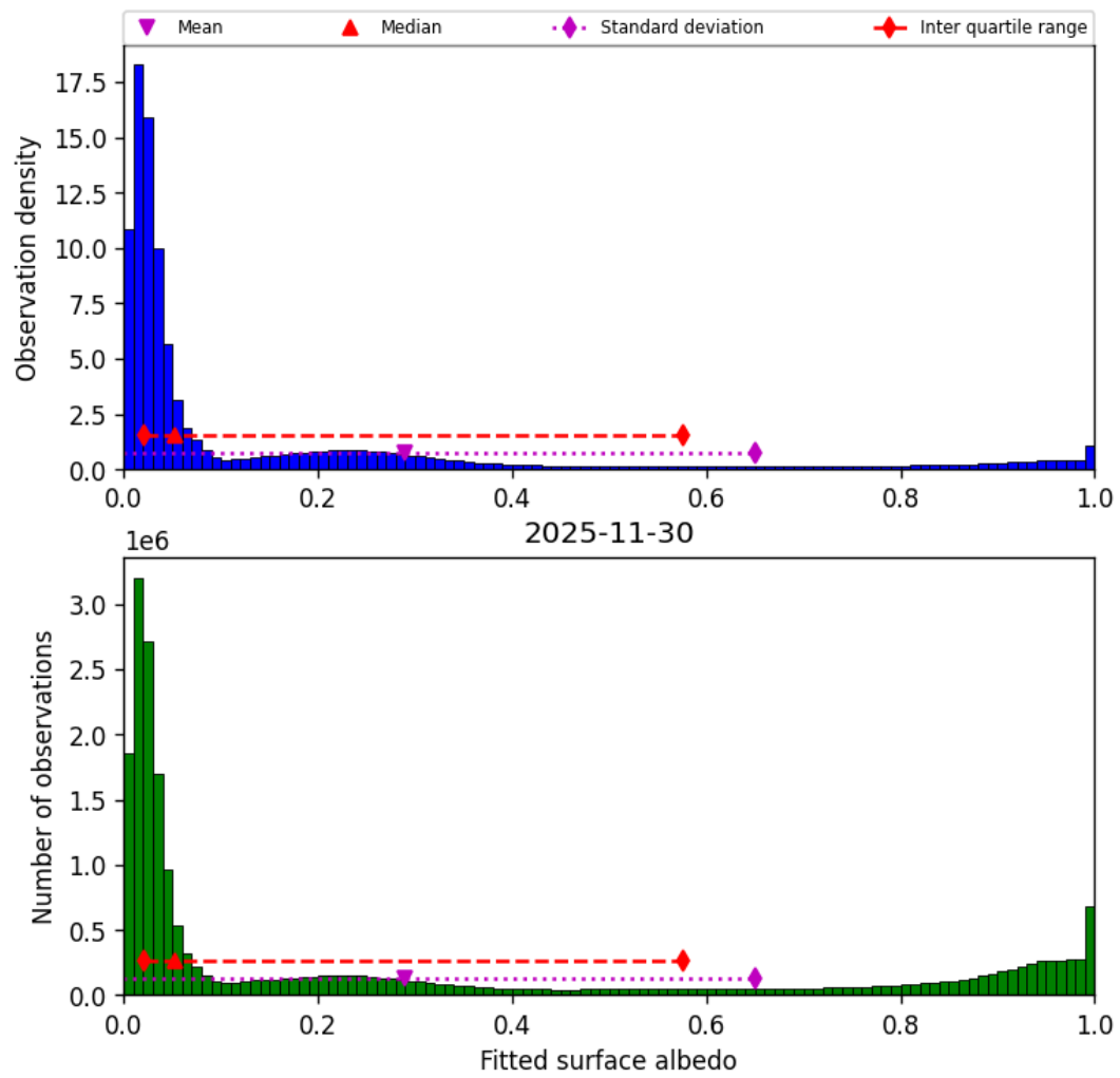
Figure 45: Histogram of “Fitted surface albedo” for 2025-11-29 to 2025-12-01
