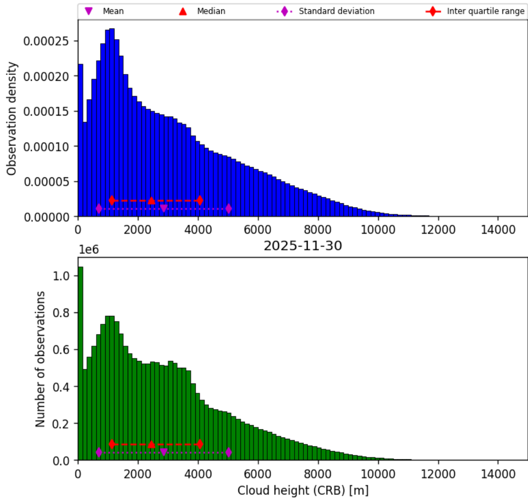
Figure 43: Histogram of “Cloud height (CRB)” for 2025-11-29 to 2025-12-01
