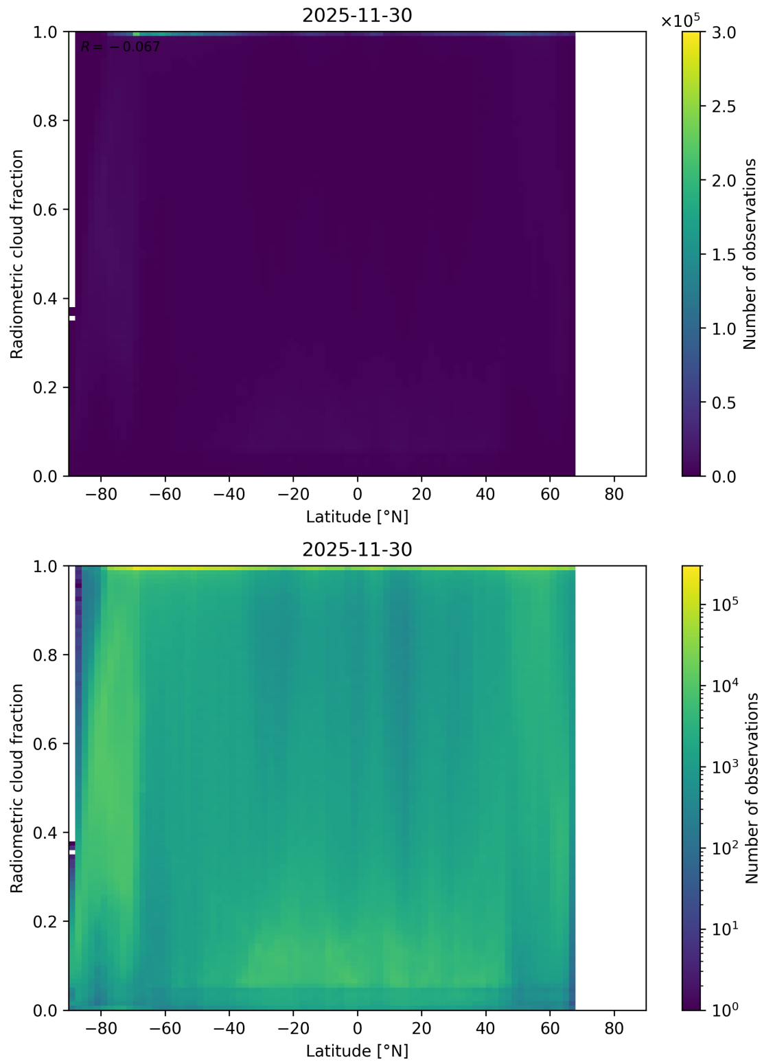
Figure 92: Scatter density plot of “Latitude” against “Radiometric cloud fraction” for 2025-11-29 to 2025-12-01.
