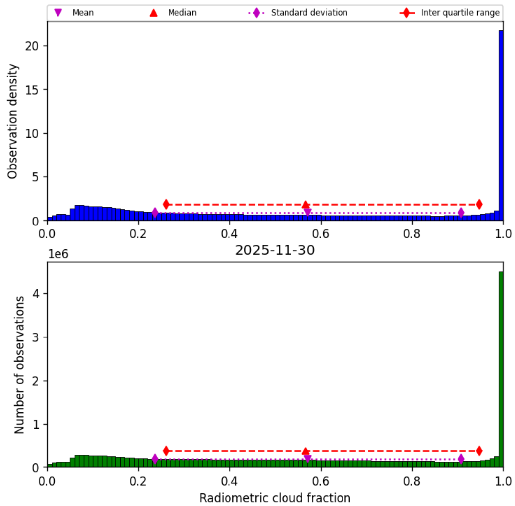
Figure 39: Histogram of “Radiometric cloud fraction” for 2025-11-29 to 2025-12-01
