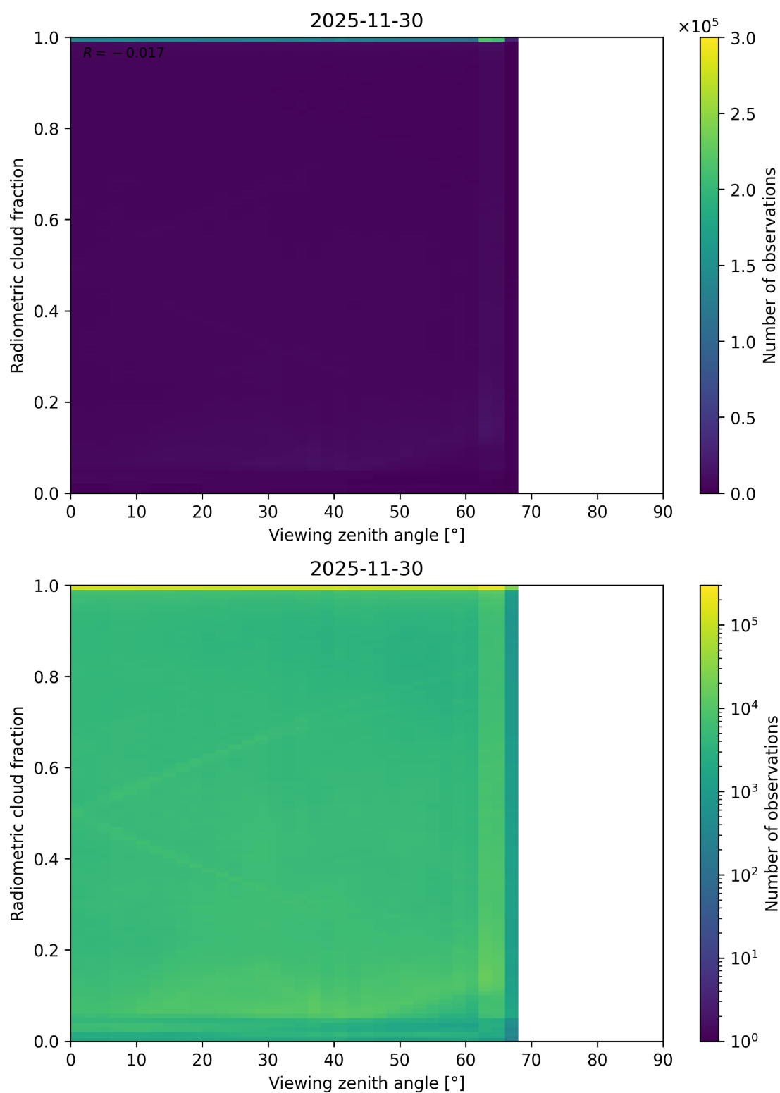
Figure 107: Scatter density plot of “Viewing zenith angle” against “Radiometric cloud fraction” for 2025-11-29 to 2025-12-01.
