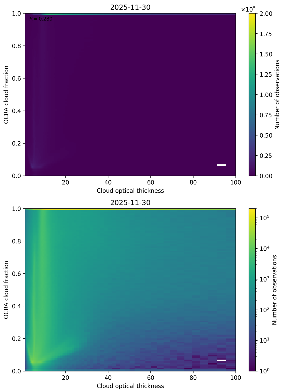
Figure 83: Scatter density plot of “Cloud optical thickness” against “OCRA cloud fraction” for 2025-11-29 to 2025-12-01.
