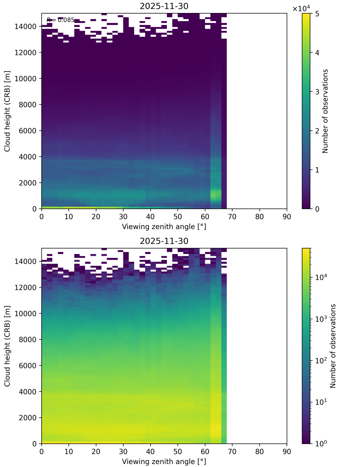
Figure 110: Scatter density plot of “Viewing zenith angle” against “Cloud height (CRB)” for 2025-11-29 to 2025-12-01.
