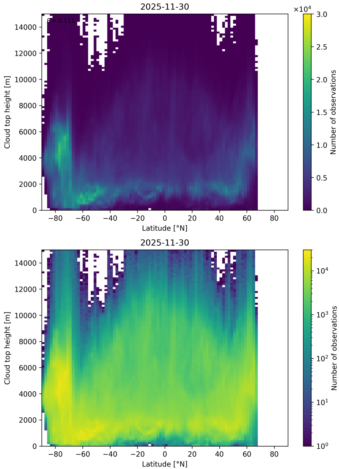
Figure 97: Scatter density plot of “Latitude” against “Cloud top height” for 2025-11-29 to 2025-12-01.
