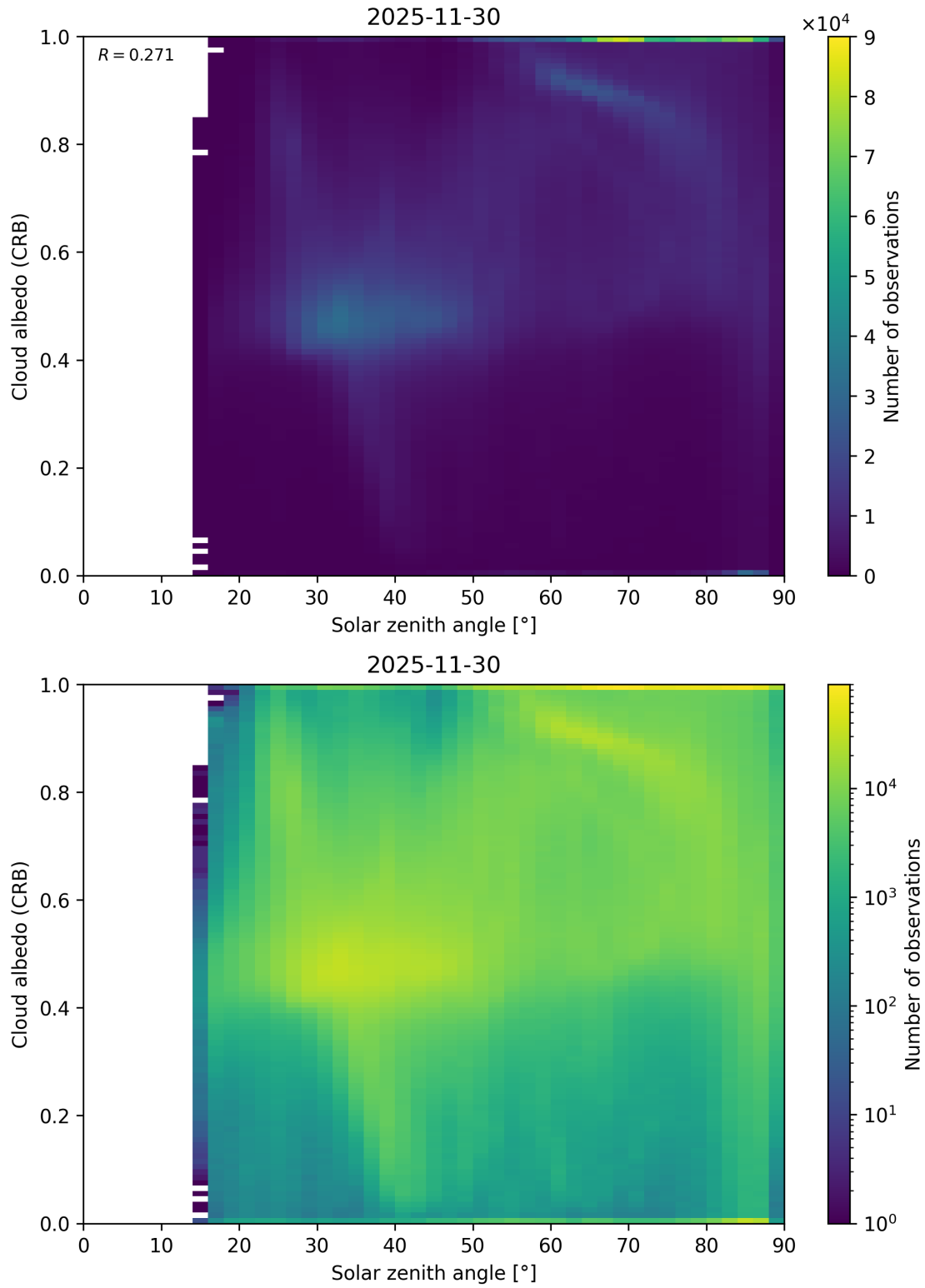
Figure 98: Scatter density plot of “Solar zenith angle” against “Cloud albedo (CRB)” for 2025-11-29 to 2025-12-01.
