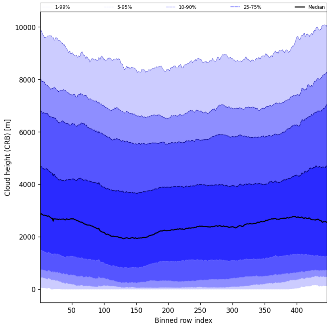
Figure 59: Along track statistics of “Cloud height (CRB)” for 2025-11-29 to 2025-12-01
