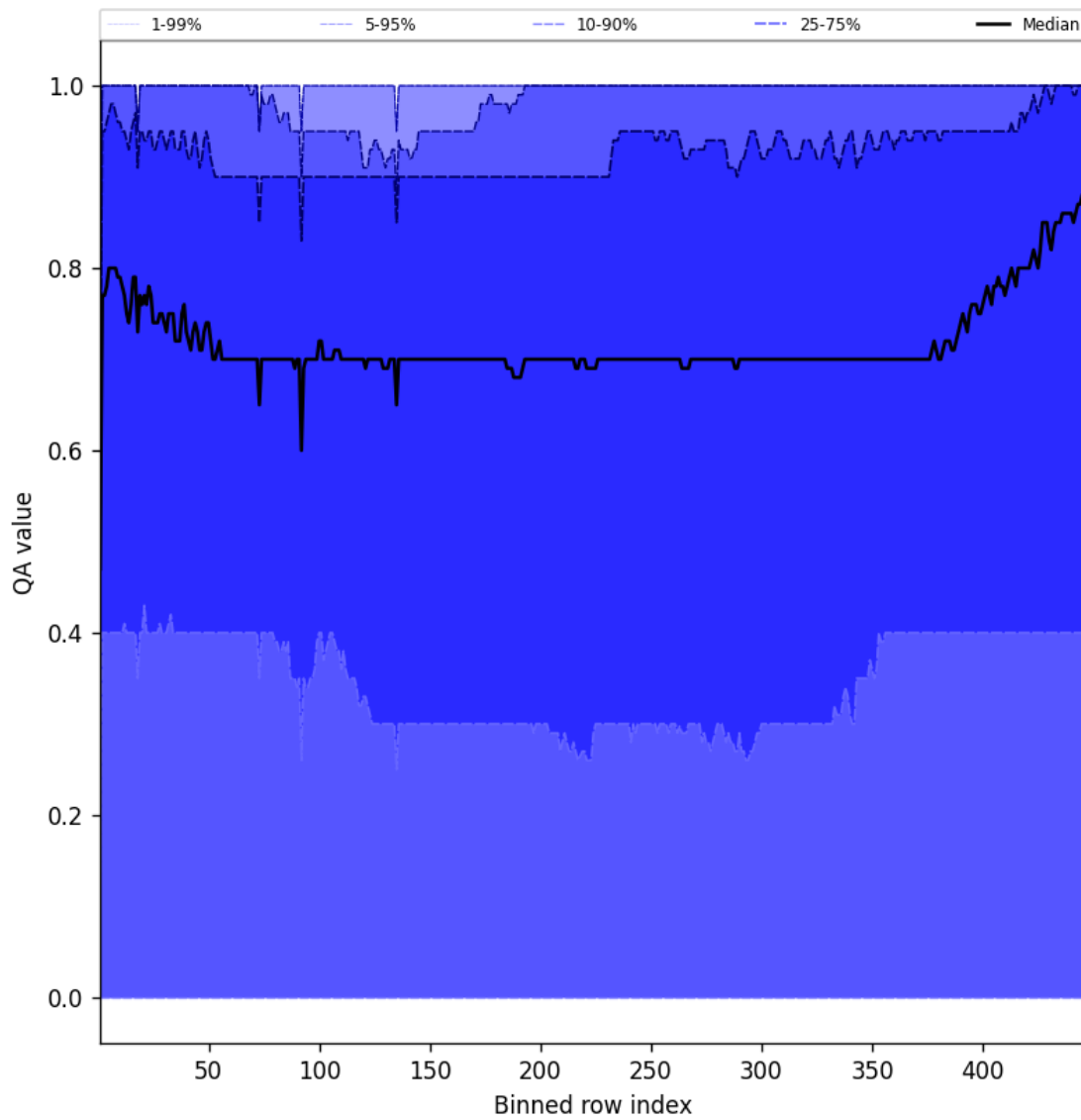
Figure 54: Along track statistics of “QA value” for 2025-11-29 to 2025-12-01
