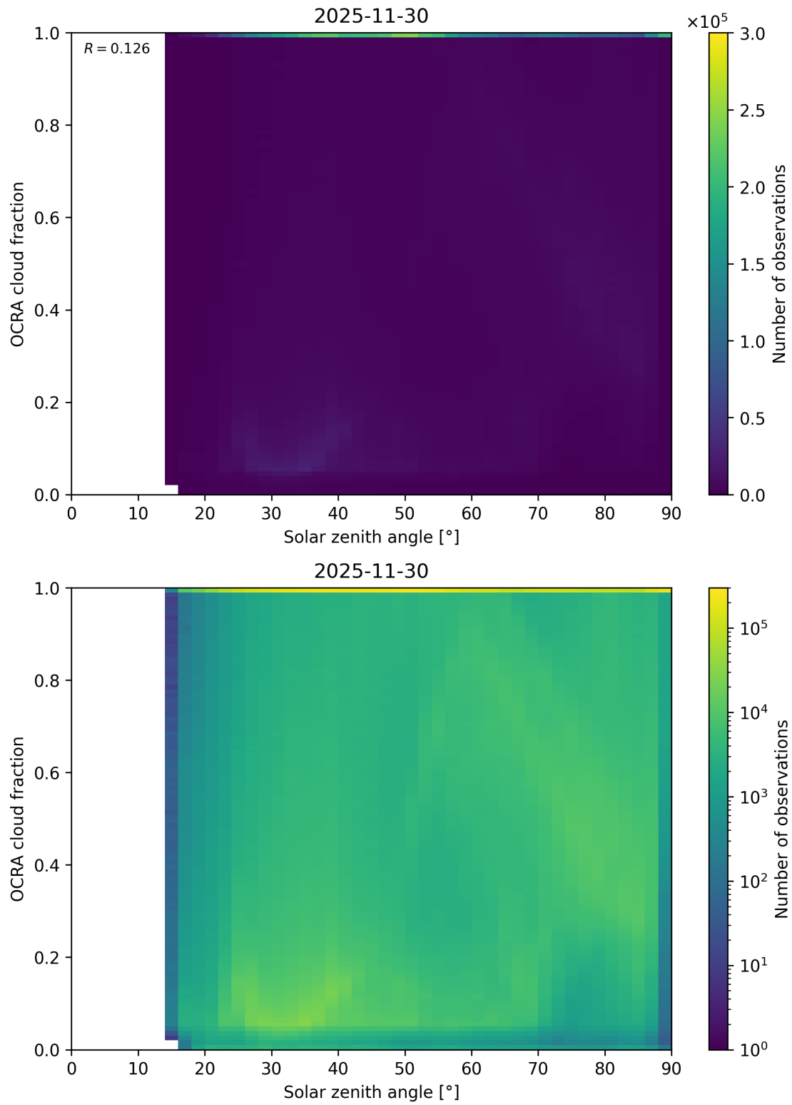
Figure 100: Scatter density plot of “Solar zenith angle” against “OCRA cloud fraction” for 2025-11-29 to 2025-12-01.
