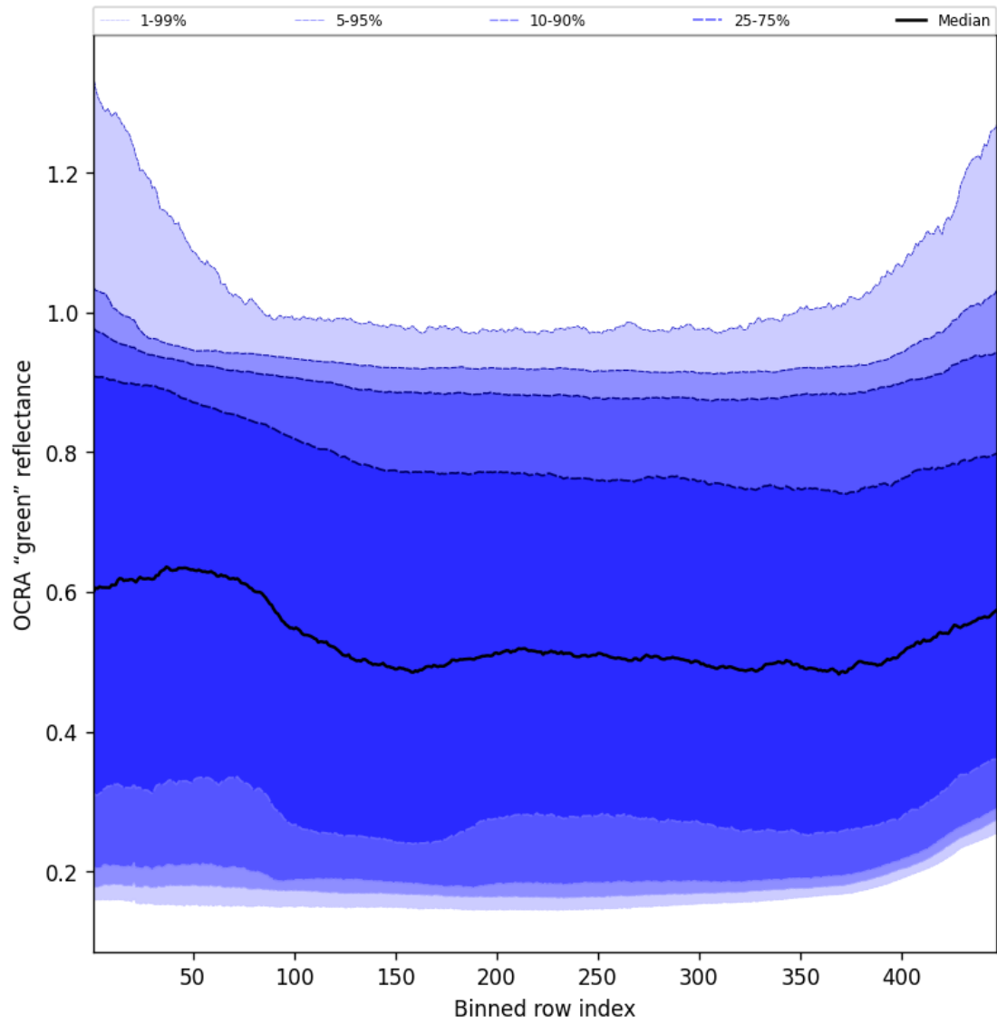
Figure 68: Along track statistics of “OCRA “green” reflectance” for 2025-11-29 to 2025-12-01
