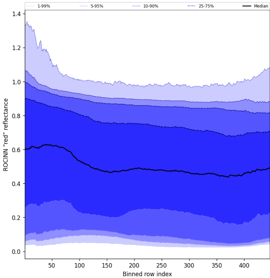
Figure 69: Along track statistics of “ROCINN “red” reflectance” for 2025-11-29 to 2025-12-01
