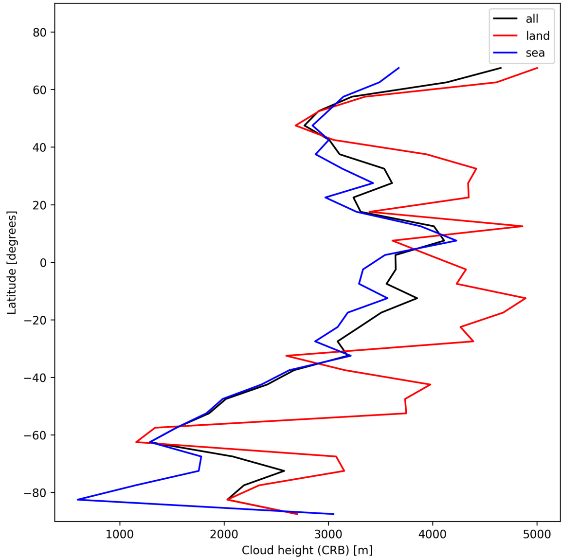
Figure 27: Zonal average of “Cloud height (CRB)” for 2025-11-29 to 2025-12-01.
