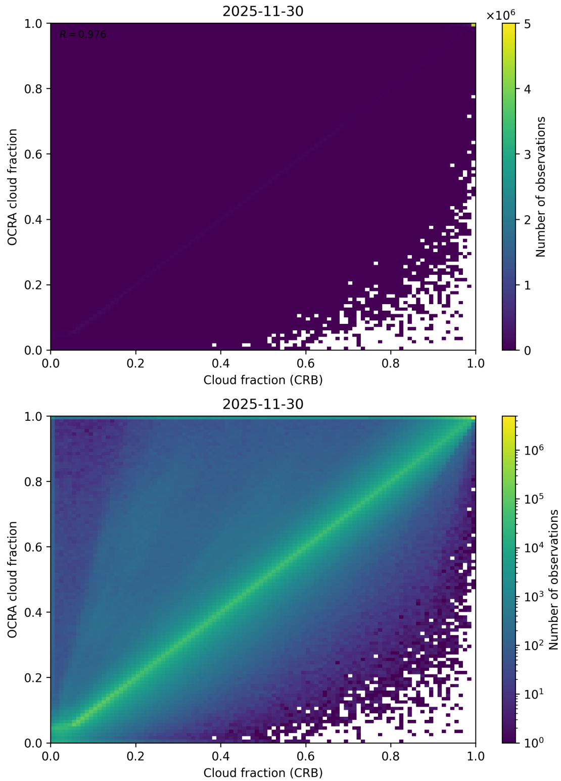
Figure 78: Scatter density plot of “Cloud fraction (CRB)” against “OCRA cloud fraction” for 2025-11-29 to 2025-12-01.
