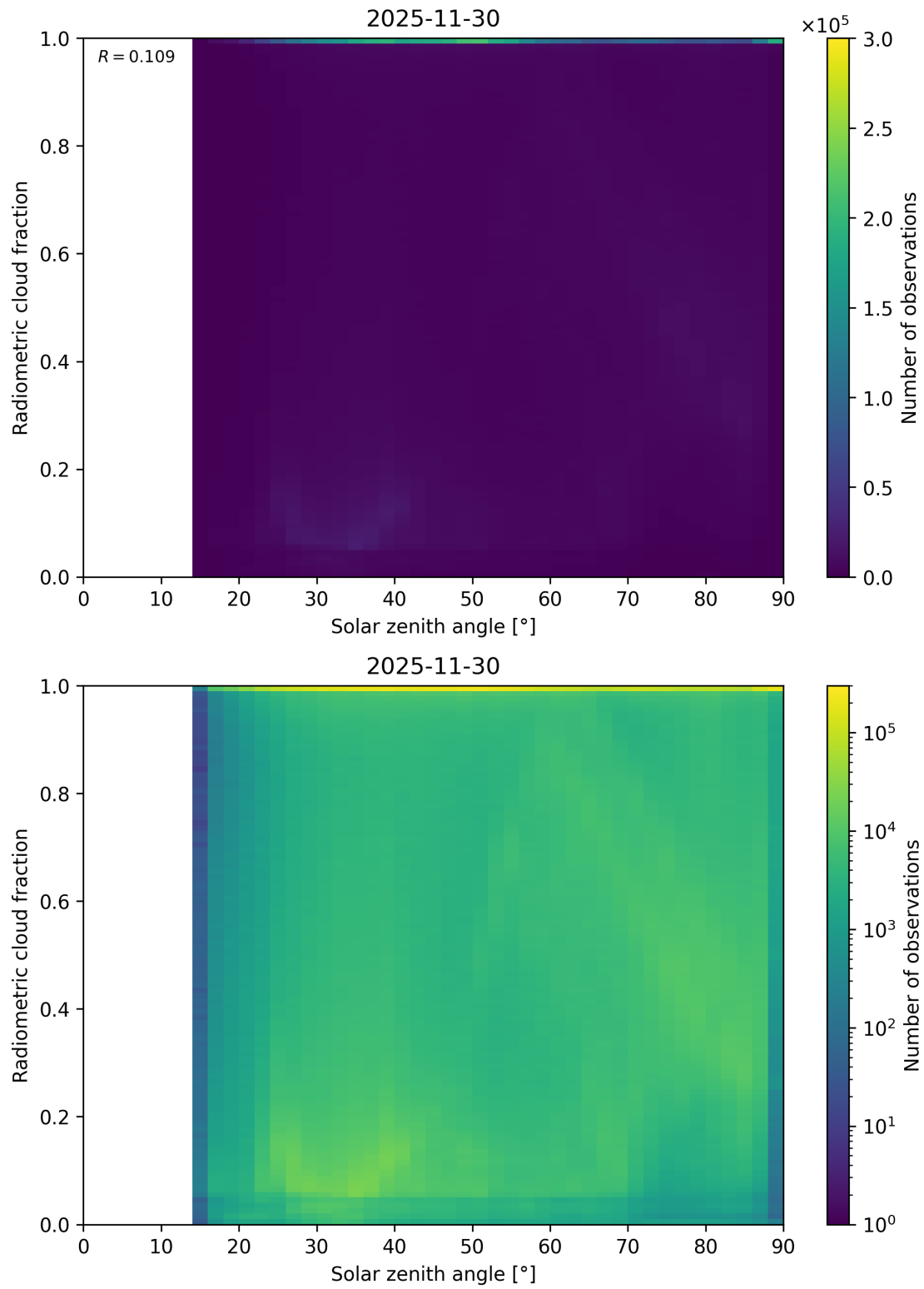
Figure 99: Scatter density plot of “Solar zenith angle” against “Radiometric cloud fraction” for 2025-11-29 to 2025-12-01.
