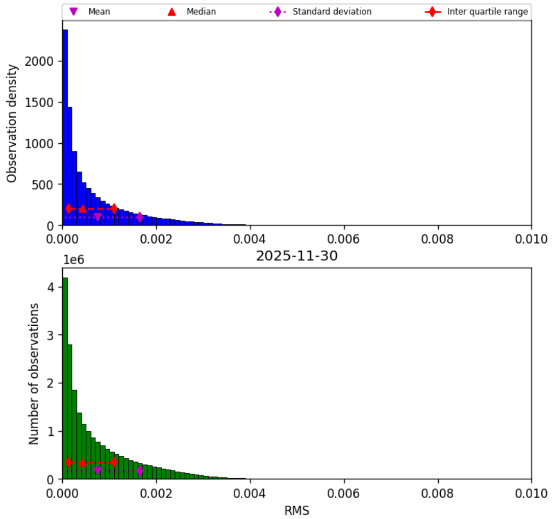
Figure 47: Histogram of “RMS” for 2025-11-29 to 2025-12-01
