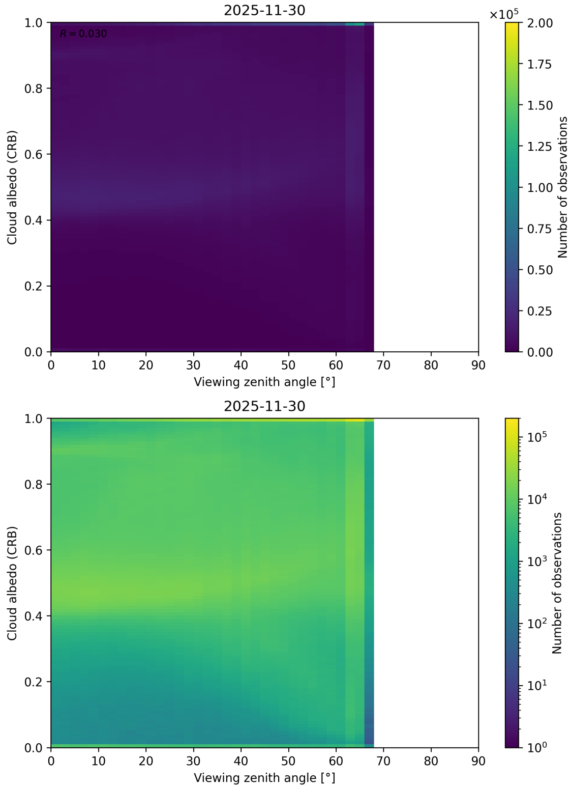
Figure 106: Scatter density plot of “Viewing zenith angle” against “Cloud albedo (CRB)” for 2025-11-29 to 2025-12-01.
