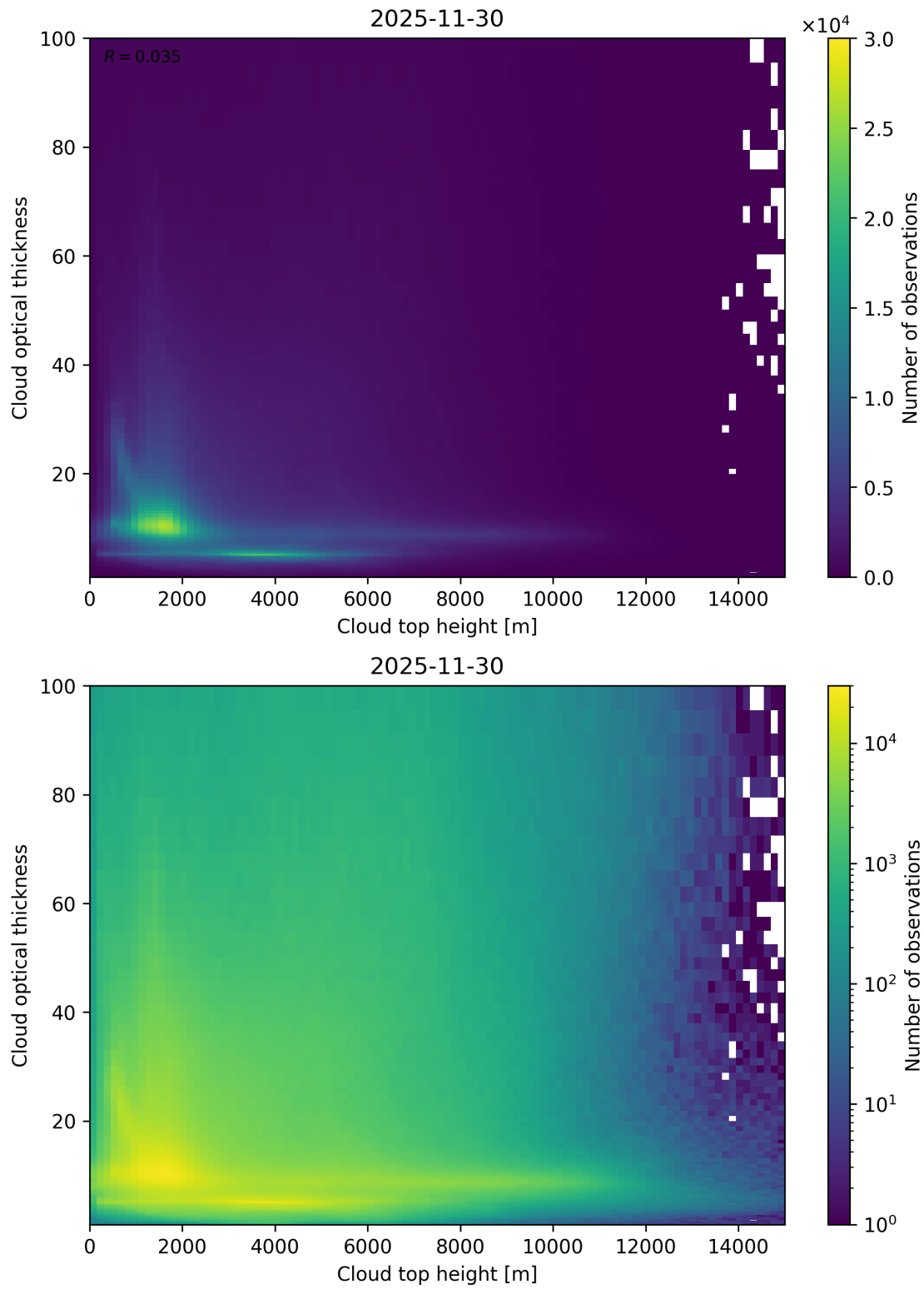
Figure 90: Scatter density plot of “Cloud top height” against “Cloud optical thickness” for 2025-11-29 to 2025-12-01.
