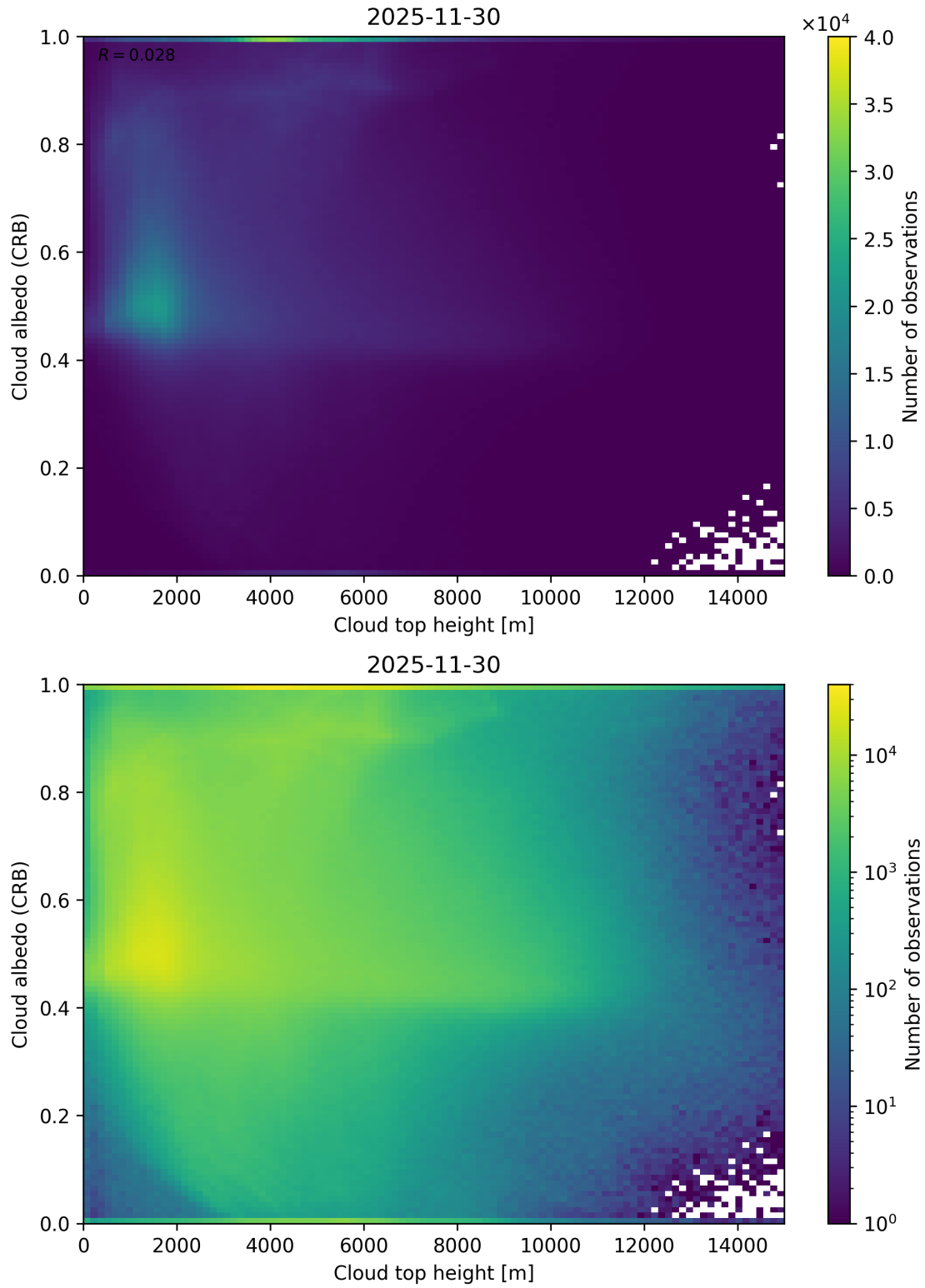
Figure 86: Scatter density plot of “Cloud top height” against “Cloud albedo (CRB)” for 2025-11-29 to 2025-12-01.
