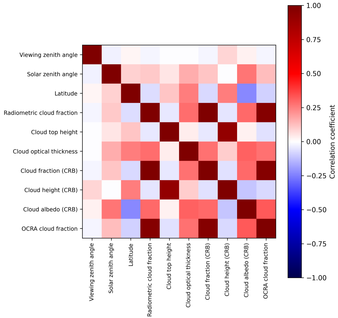
Figure 2: Map of correlation matrix for 2025-11-29 to 2025-12-01.
