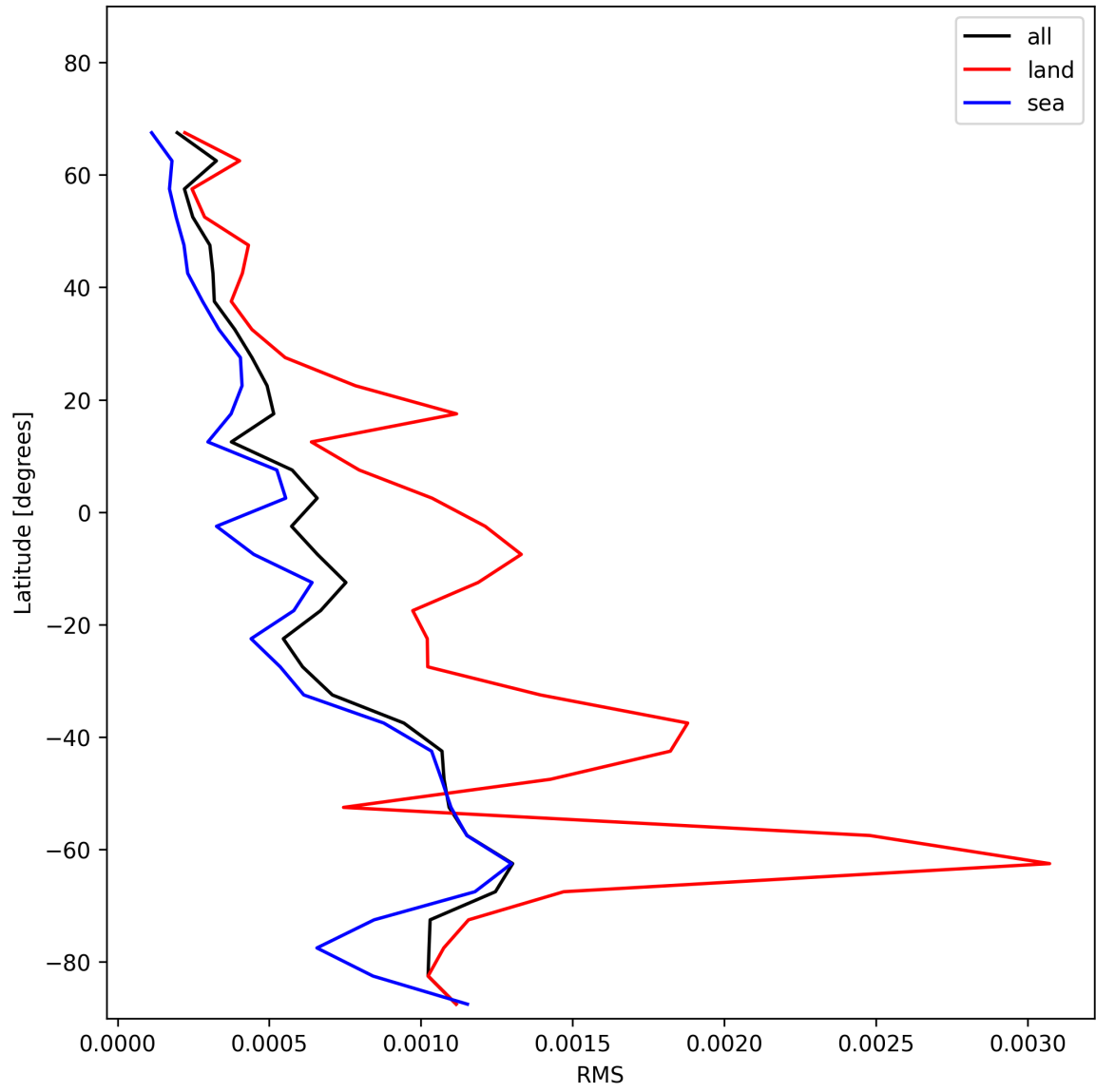
Figure 31: Zonal average of “RMS” for 2025-11-29 to 2025-12-01.
