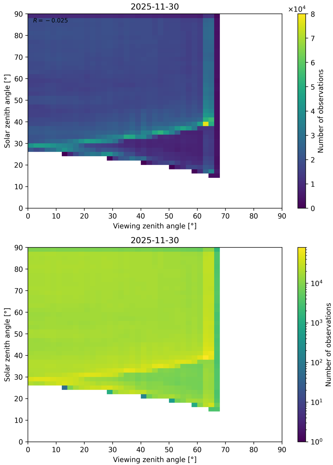
Figure 114: Scatter density plot of “Viewing zenith angle” against “Solar zenith angle” for 2025-11-29 to 2025-12-01.
