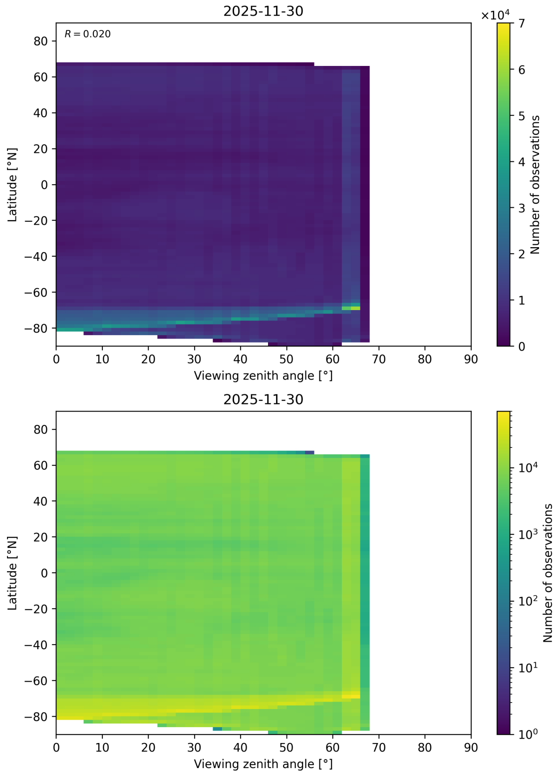
Figure 113: Scatter density plot of “Viewing zenith angle” against “Latitude” for 2025-11-29 to 2025-12-01.
