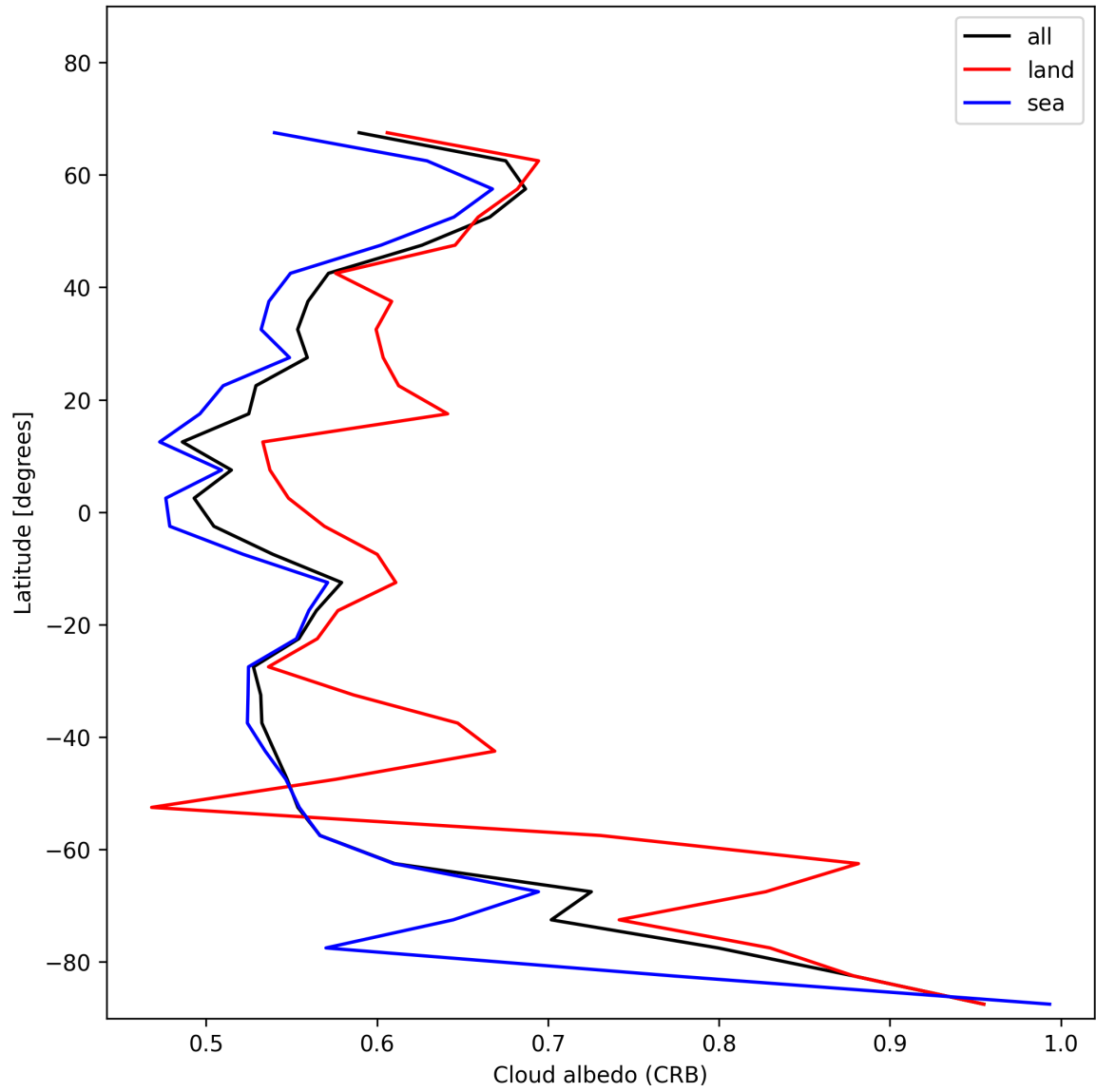
Figure 28: Zonal average of “Cloud albedo (CRB)” for 2025-11-29 to 2025-12-01.
