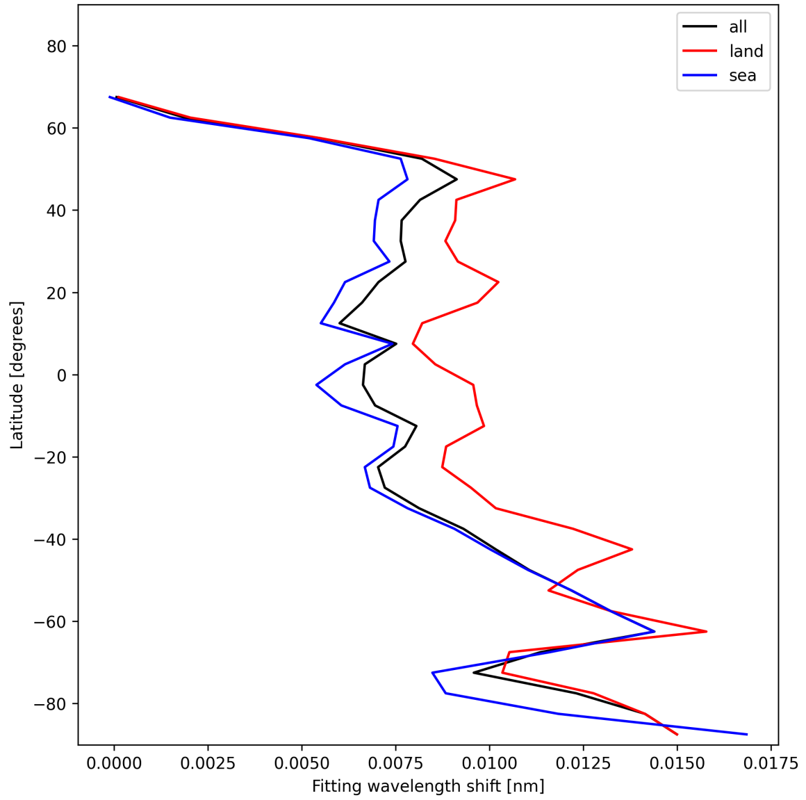
Figure 33: Zonal average of “Fitting wavelength shift” for 2025-11-29 to 2025-12-01.
