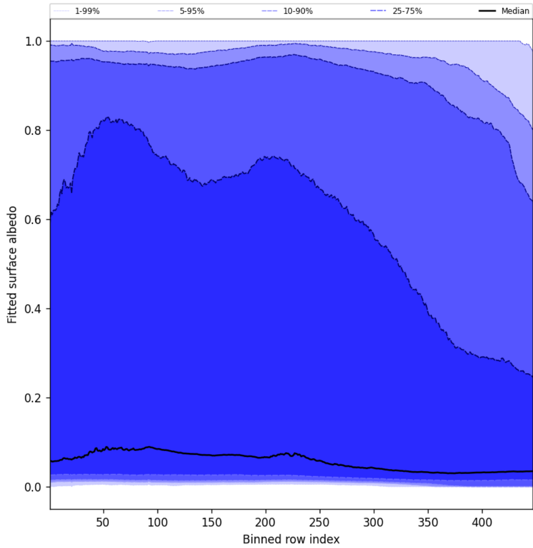
Figure 61: Along track statistics of “Fitted surface albedo” for 2025-11-29 to 2025-12-01
