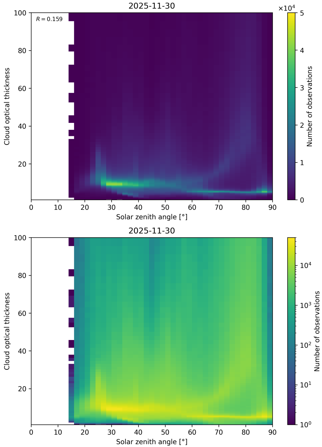
Figure 103: Scatter density plot of “Solar zenith angle” against “Cloud optical thickness” for 2025-11-29 to 2025-12-01.
