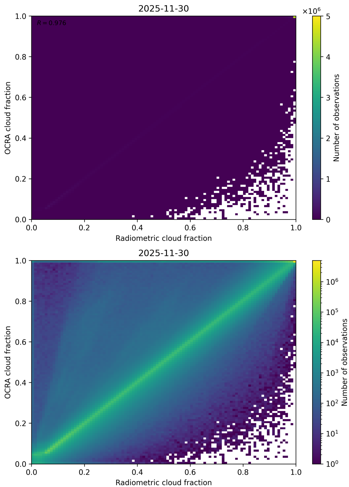
Figure 72: Scatter density plot of “Radiometric cloud fraction” against “OCRA cloud fraction” for 2025-11-29 to 2025-12-01.
