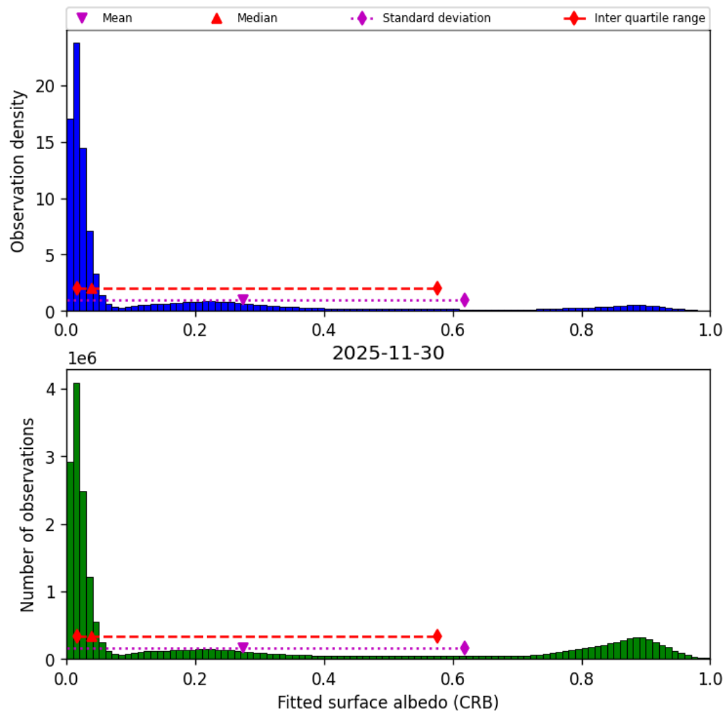
Figure 46: Histogram of “Fitted surface albedo (CRB)” for 2025-11-29 to 2025-12-01
