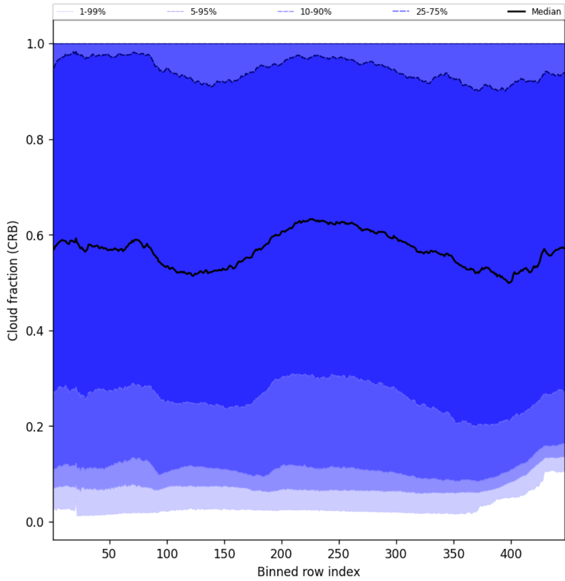
Figure 58: Along track statistics of “Cloud fraction (CRB)” for 2025-11-29 to 2025-12-01
