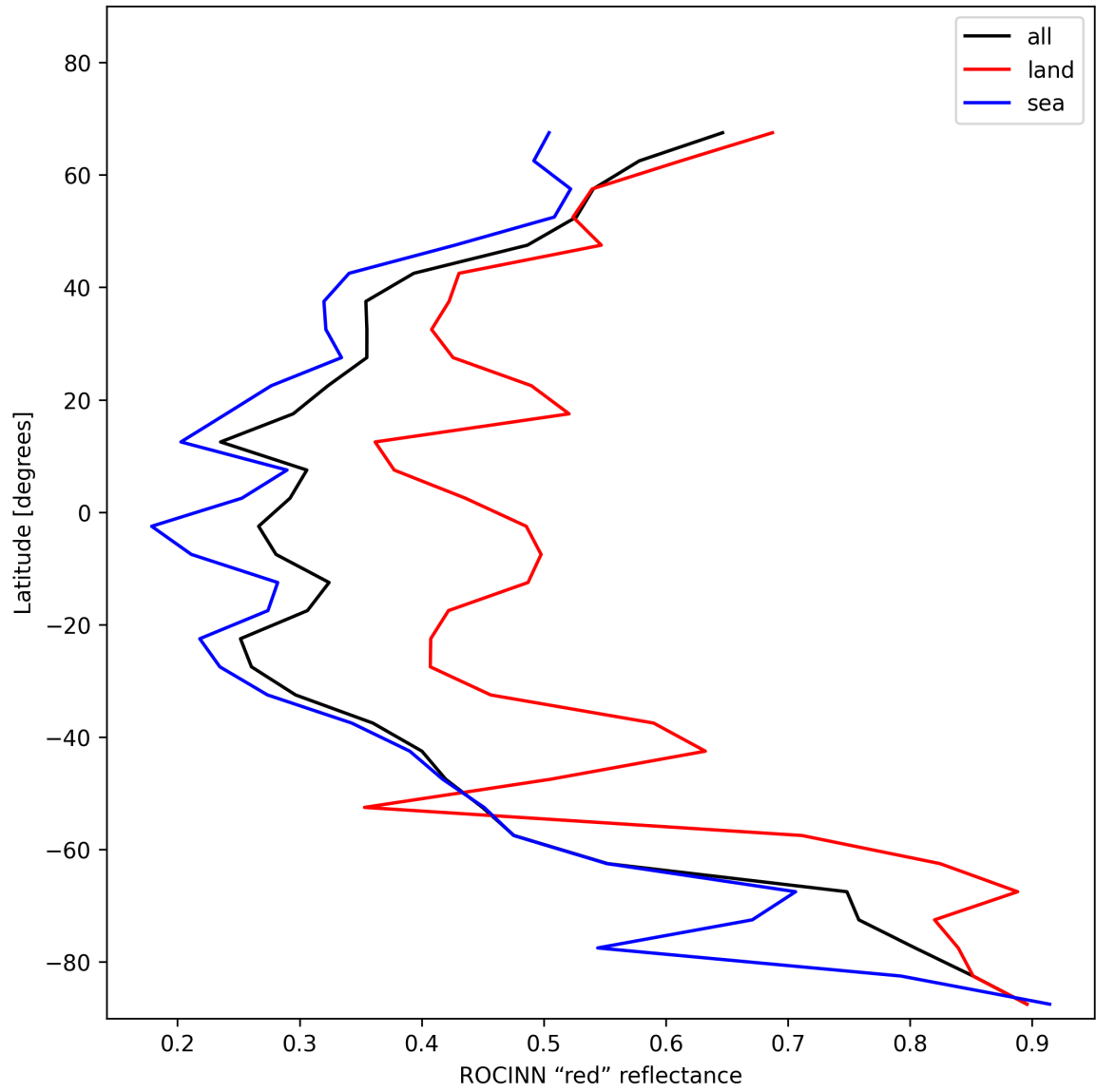
Figure 37: Zonal average of “ROCINN “red” reflectance” for 2025-11-29 to 2025-12-01.
