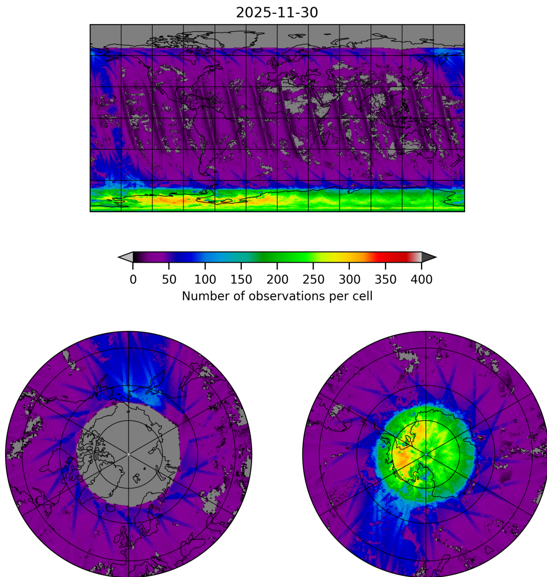
Figure 21: Map of the number of observations for 2025-11-29 to 2025-12-01
