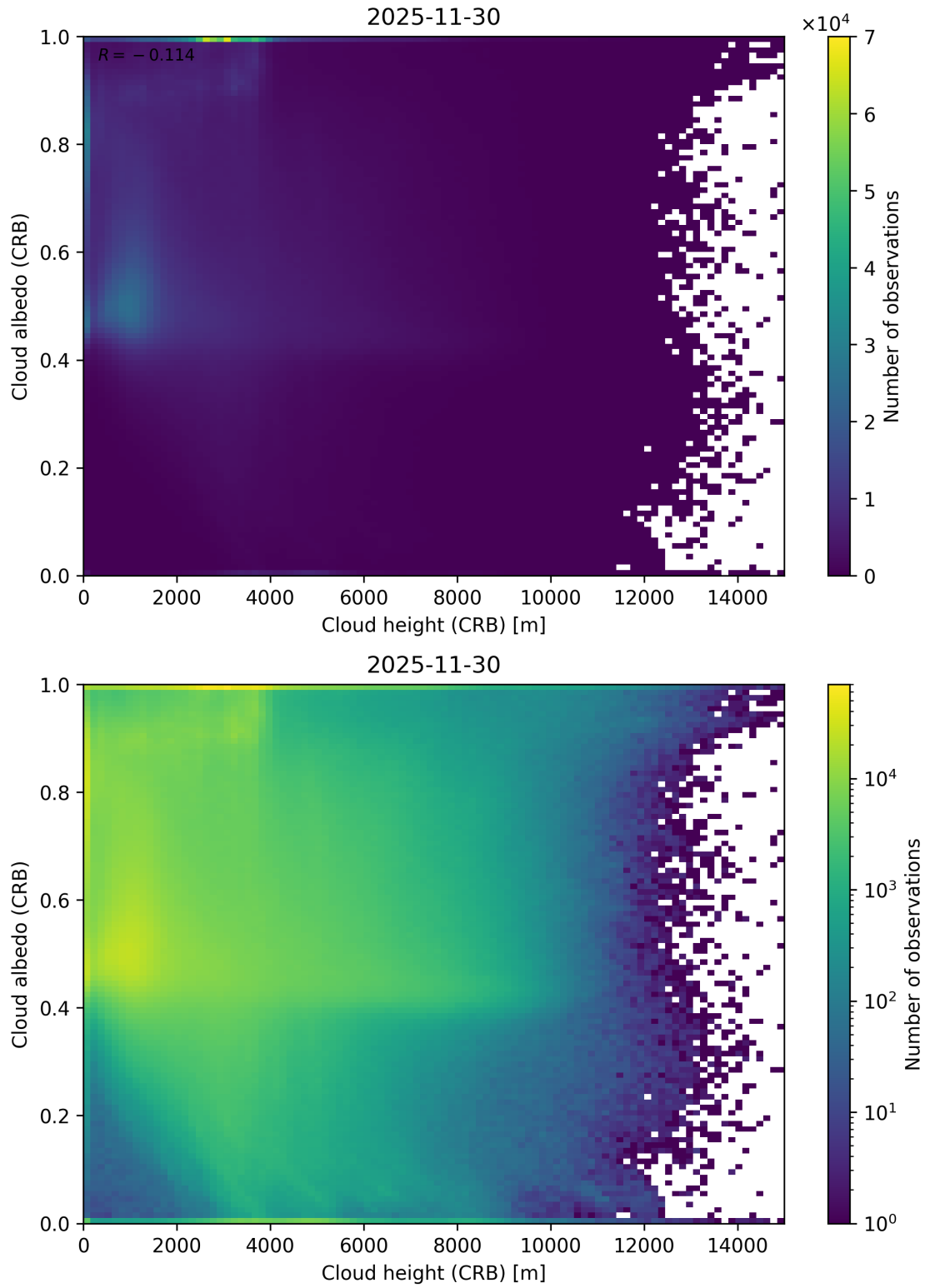
Figure 80: Scatter density plot of “Cloud height (CRB)” against “Cloud albedo (CRB)” for 2025-11-29 to 2025-12-01.
