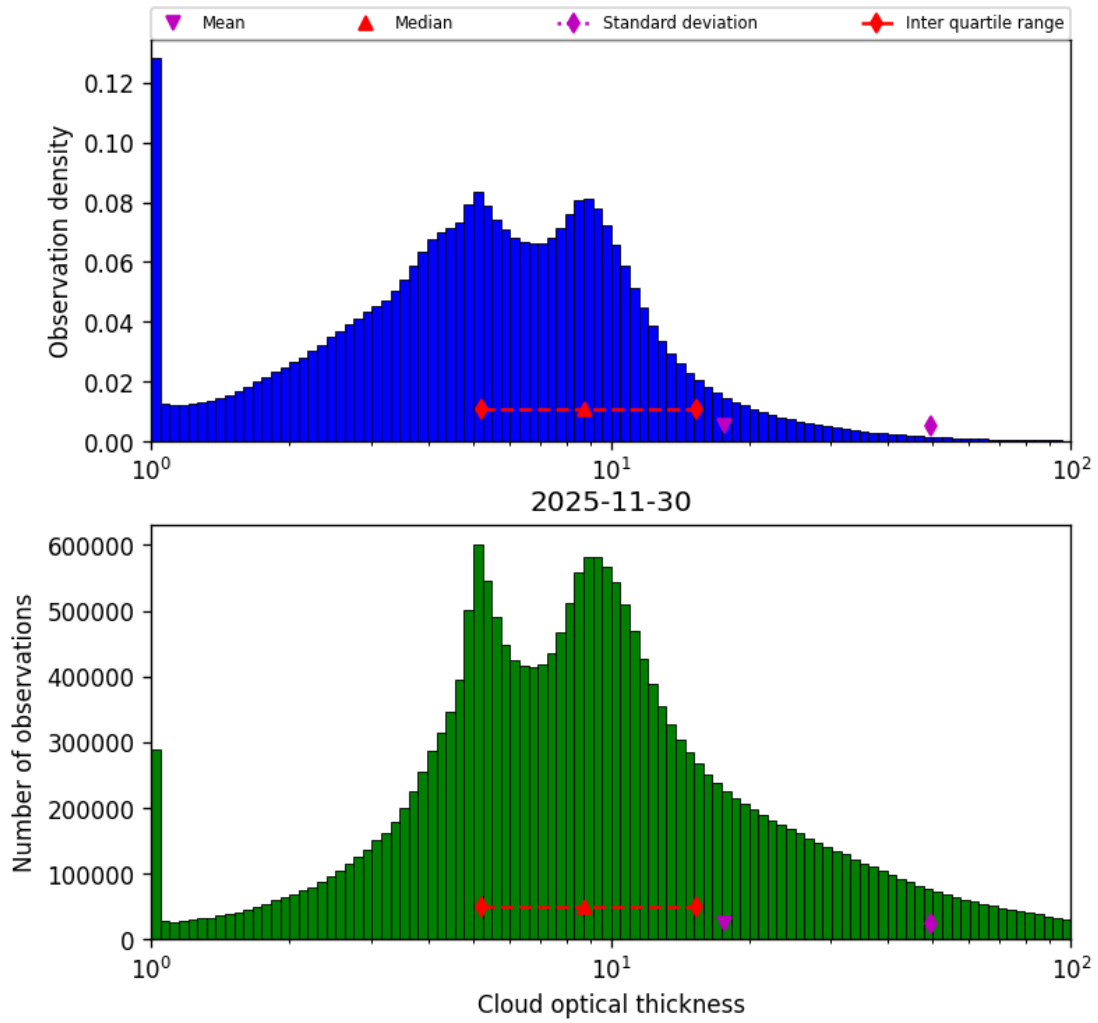
Figure 41: Histogram of “Cloud optical thickness” for 2025-11-29 to 2025-12-01
