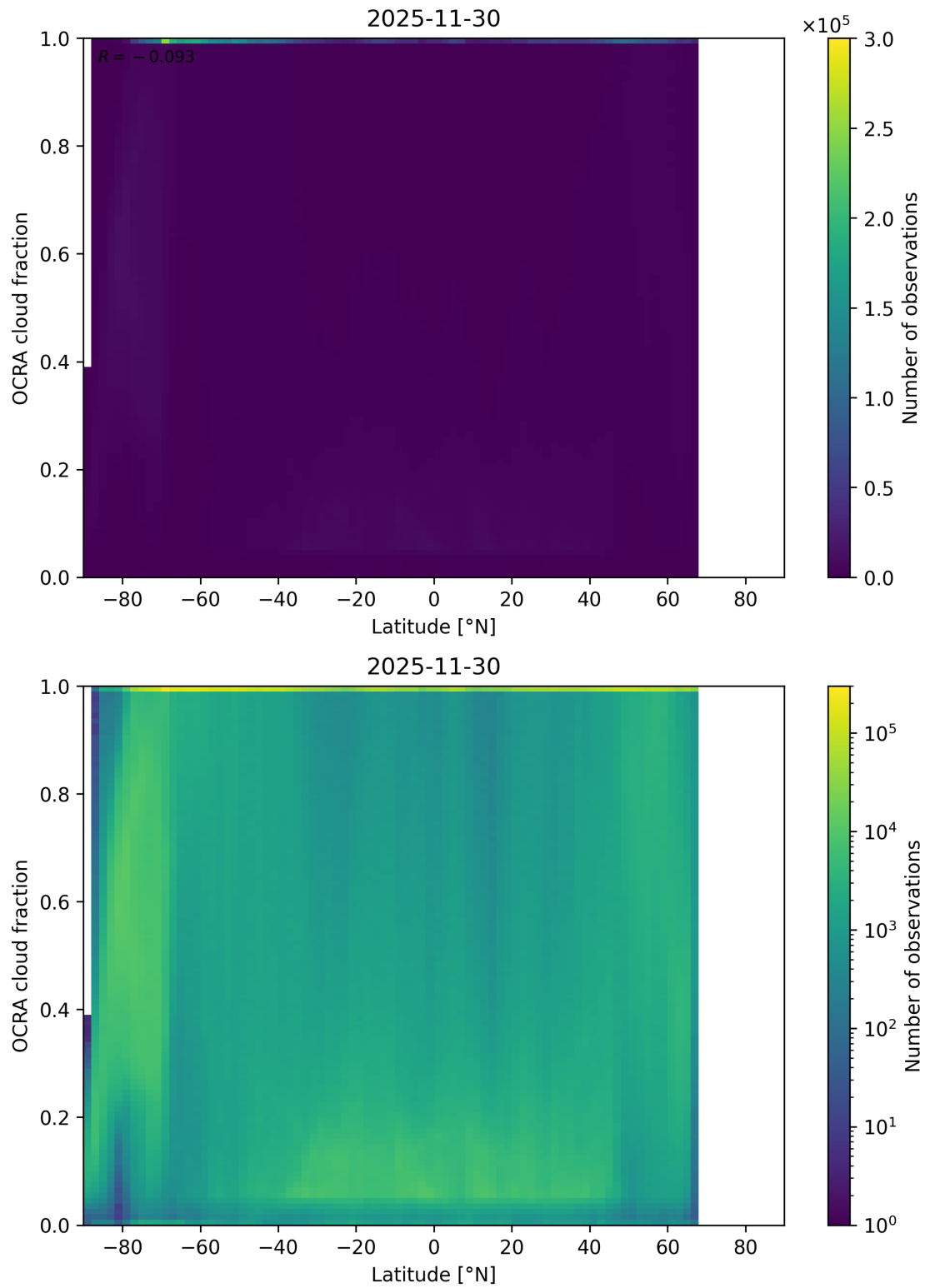
Figure 93: Scatter density plot of “Latitude” against “OCRA cloud fraction” for 2025-11-29 to 2025-12-01.
