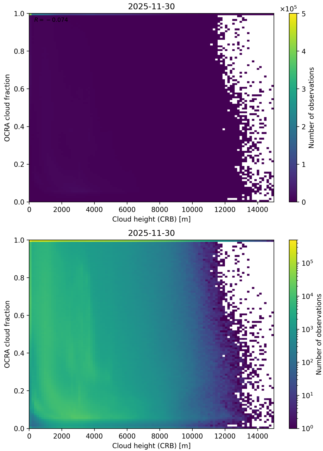
Figure 81: Scatter density plot of “Cloud height (CRB)” against “OCRA cloud fraction” for 2025-11-29 to 2025-12-01.
