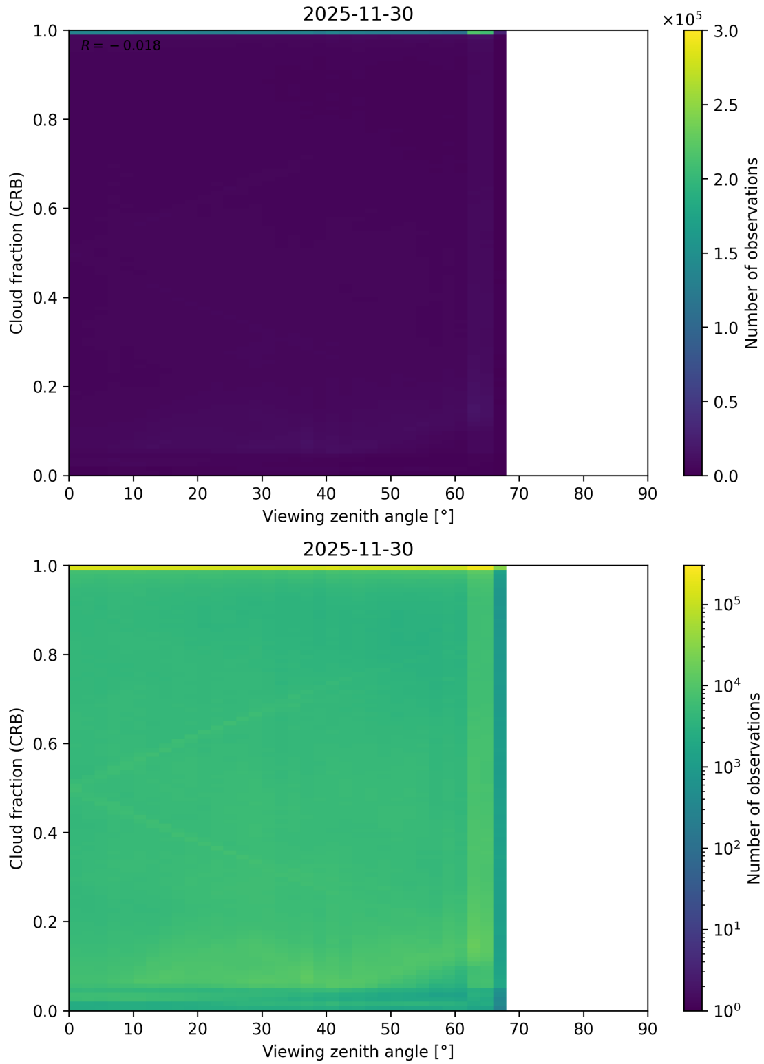
Figure 109: Scatter density plot of “Viewing zenith angle” against “Cloud fraction (CRB)” for 2025-11-29 to 2025-12-01.
