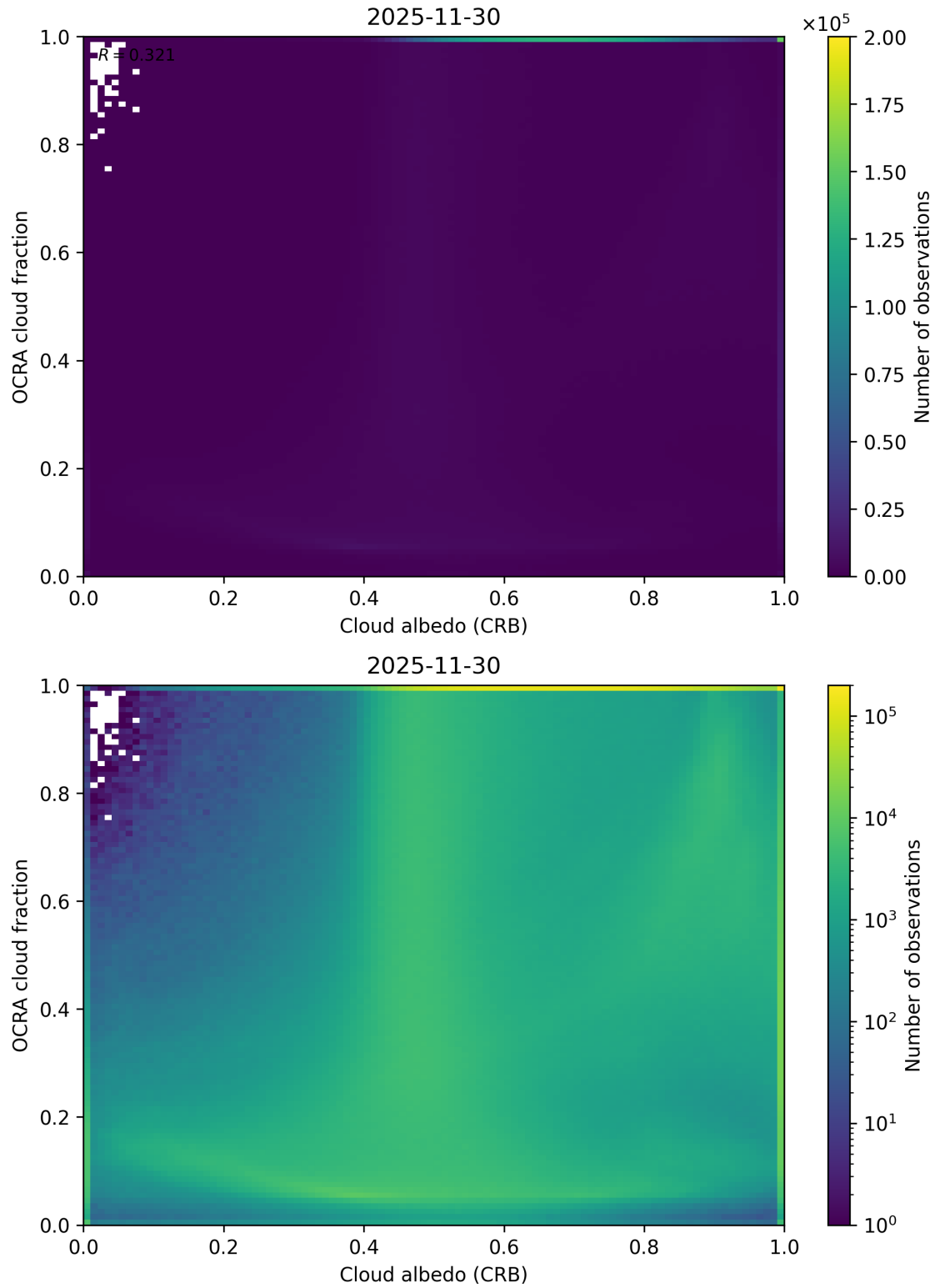
Figure 70: Scatter density plot of “Cloud albedo (CRB)” against “OCRA cloud fraction” for 2025-11-29 to 2025-12-01.
