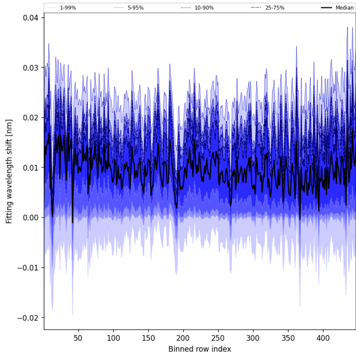
Figure 65: Along track statistics of “Fitting wavelength shift” for 2025-11-29 to 2025-12-01
