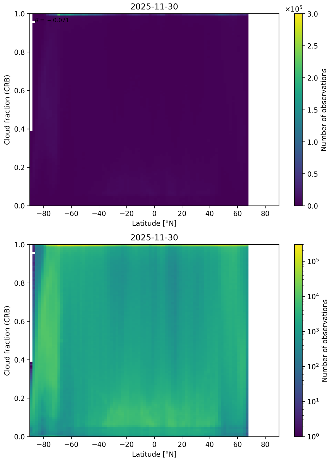
Figure 94: Scatter density plot of “Latitude” against “Cloud fraction (CRB)” for 2025-11-29 to 2025-12-01.
