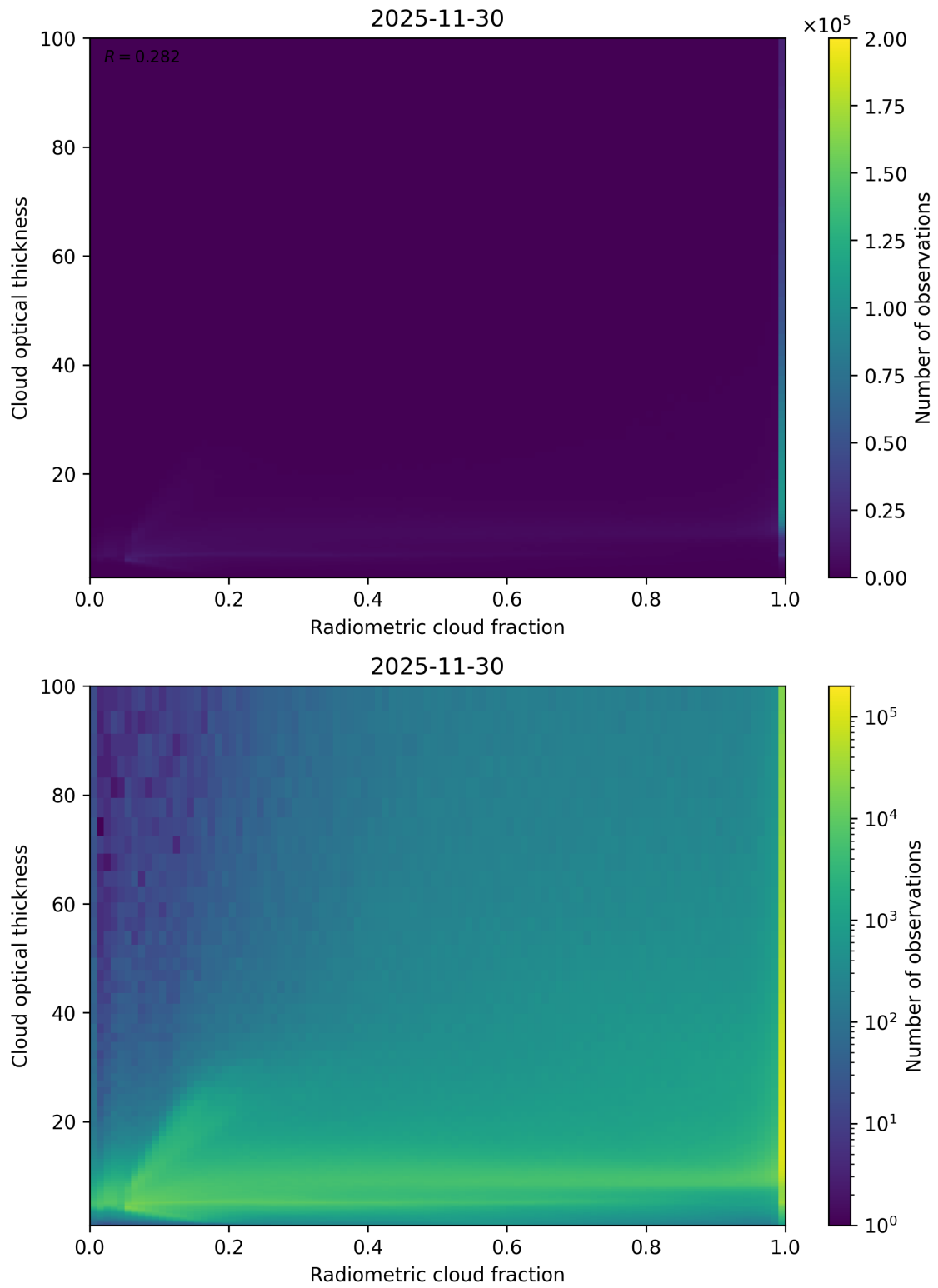
Figure 75: Scatter density plot of “Radiometric cloud fraction” against “Cloud optical thickness” for 2025-11-29 to 2025-12-01.
