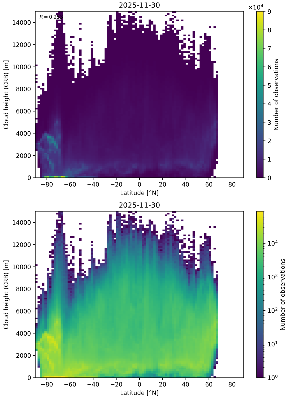
Figure 95: Scatter density plot of “Latitude” against “Cloud height (CRB)” for 2025-11-29 to 2025-12-01.
