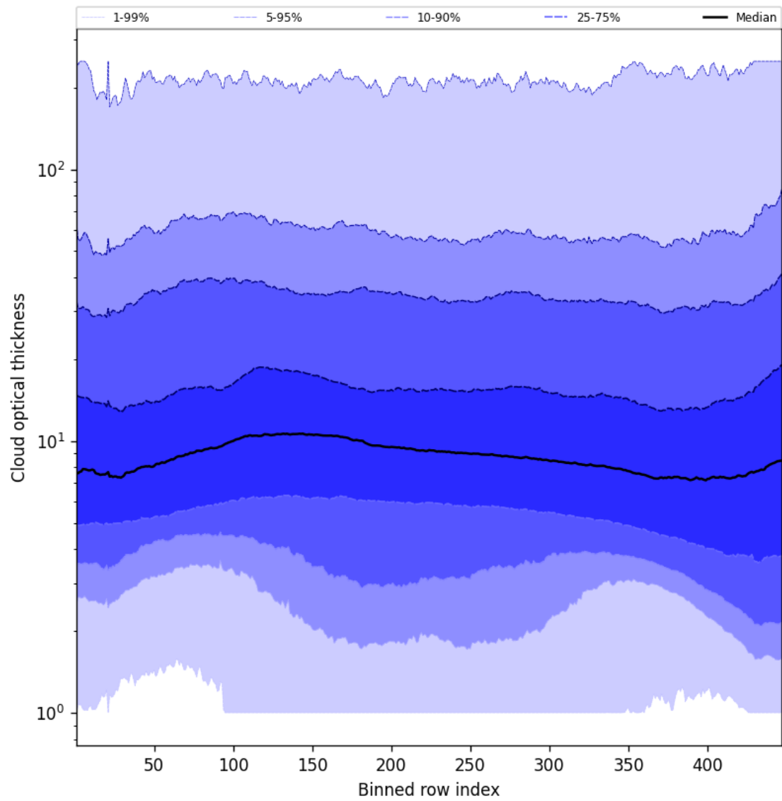
Figure 57: Along track statistics of “Cloud optical thickness” for 2025-11-29 to 2025-12-01
