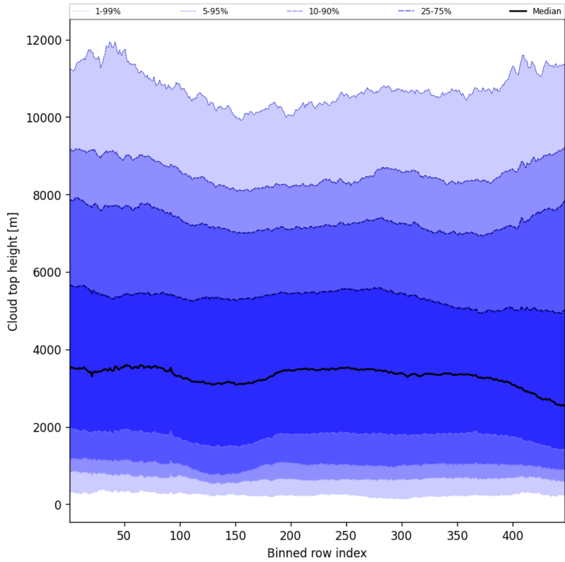
Figure 56: Along track statistics of “Cloud top height” for 2025-11-29 to 2025-12-01
