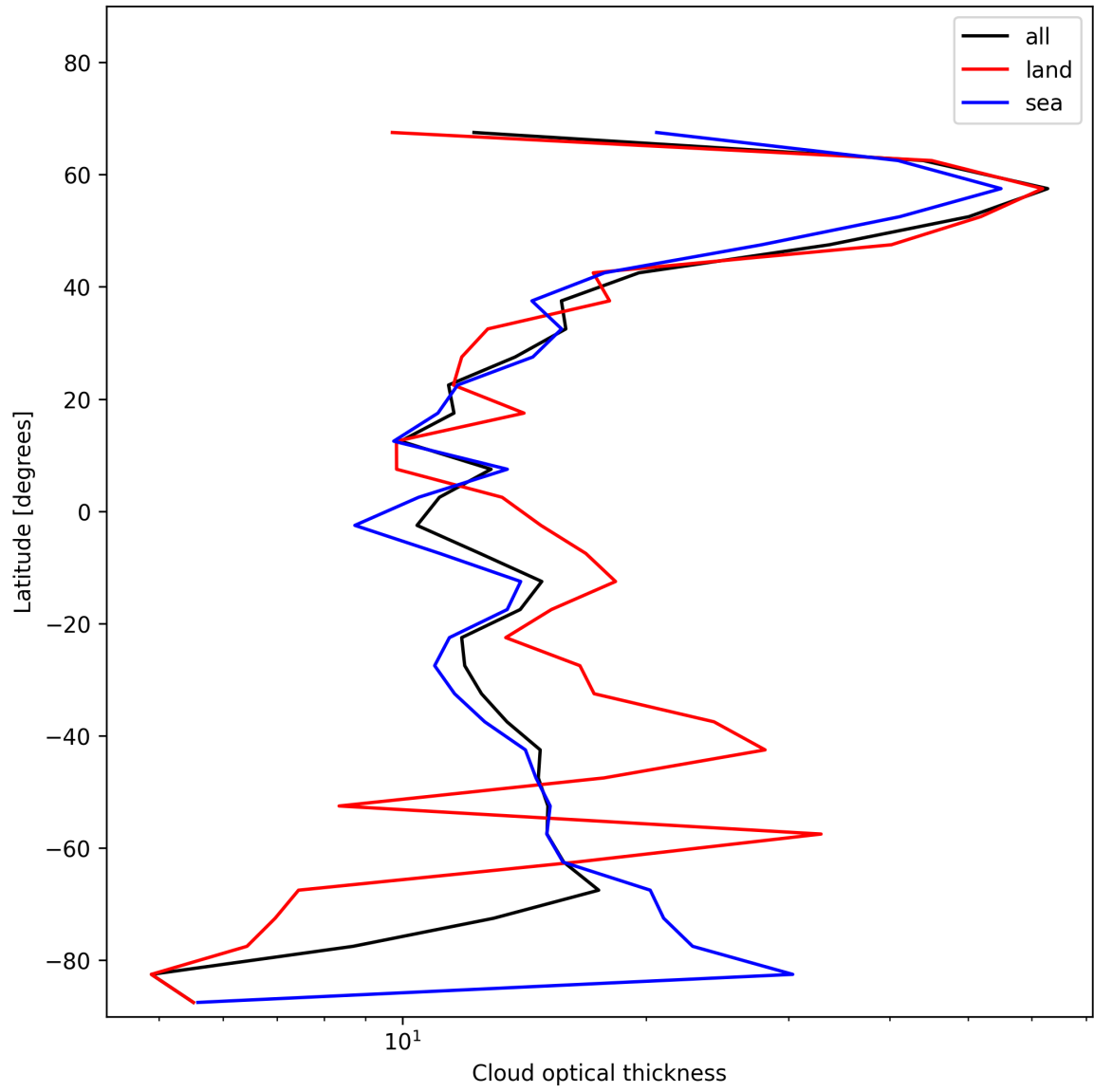
Figure 25: Zonal average of “Cloud optical thickness” for 2025-11-29 to 2025-12-01.
