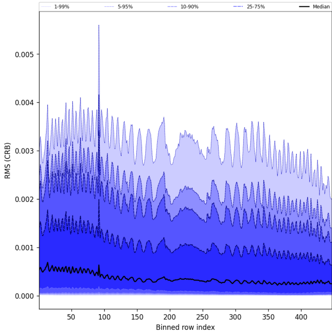
Figure 64: Along track statistics of “RMS (CRB)” for 2025-11-29 to 2025-12-01
