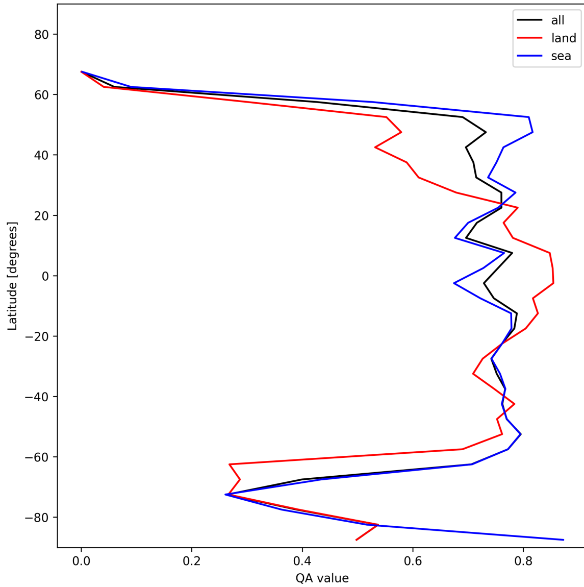
Figure 22: Zonal average of “QA value” for 2025-11-29 to 2025-12-01.
