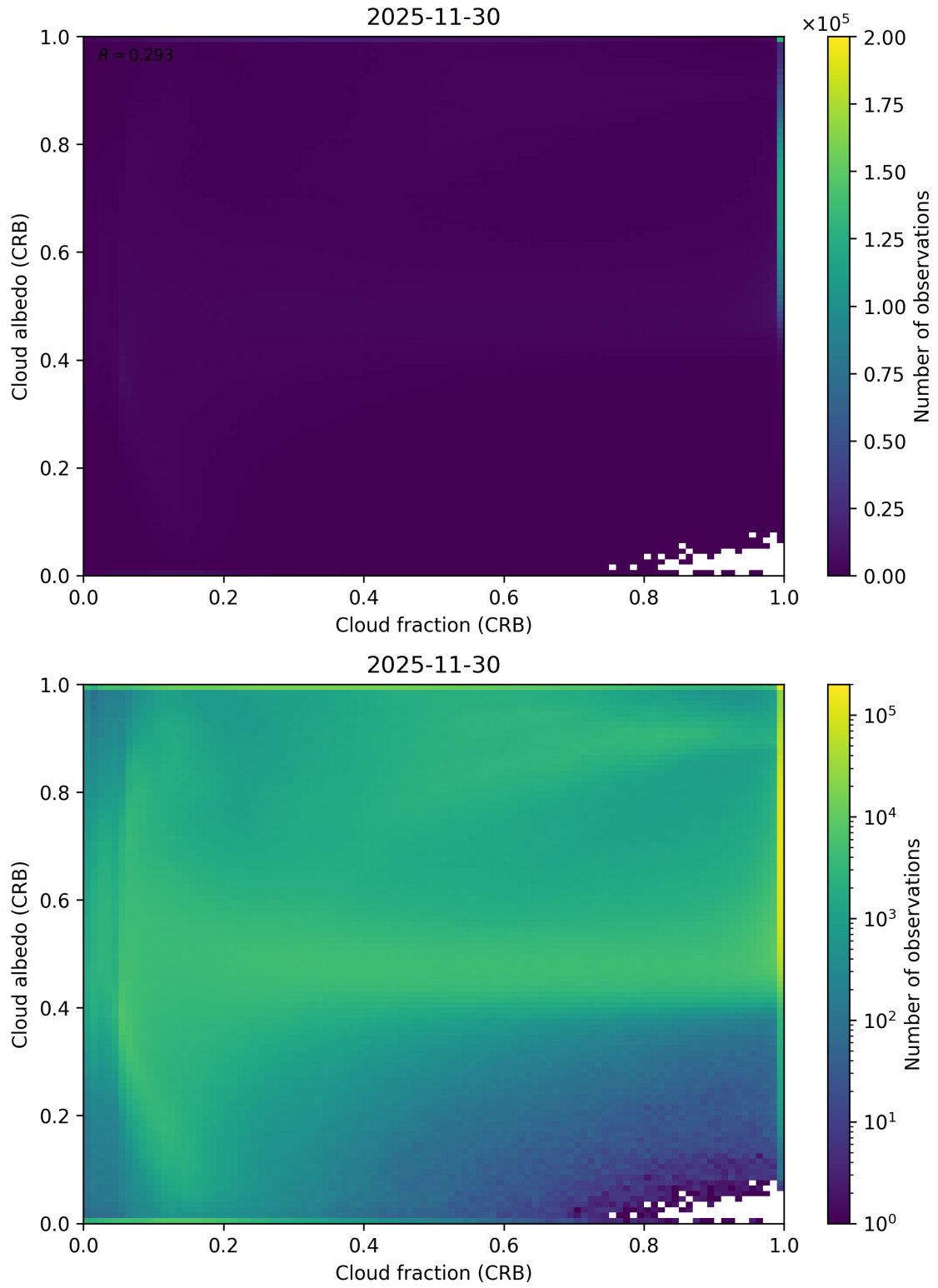
Figure 77: Scatter density plot of “Cloud fraction (CRB)” against “Cloud albedo (CRB)” for 2025-11-29 to 2025-12-01.
