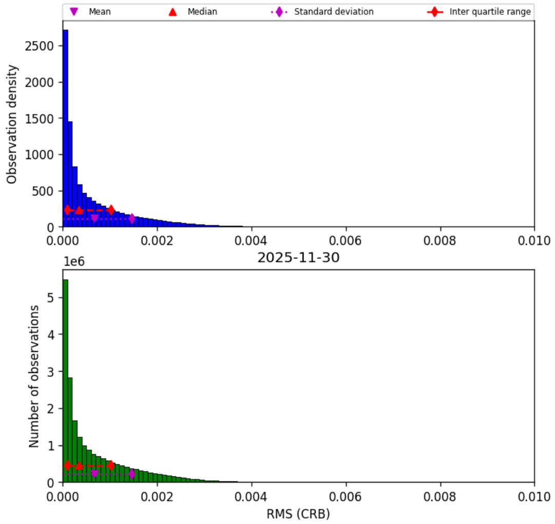
Figure 48: Histogram of “RMS (CRB)” for 2025-11-29 to 2025-12-01
