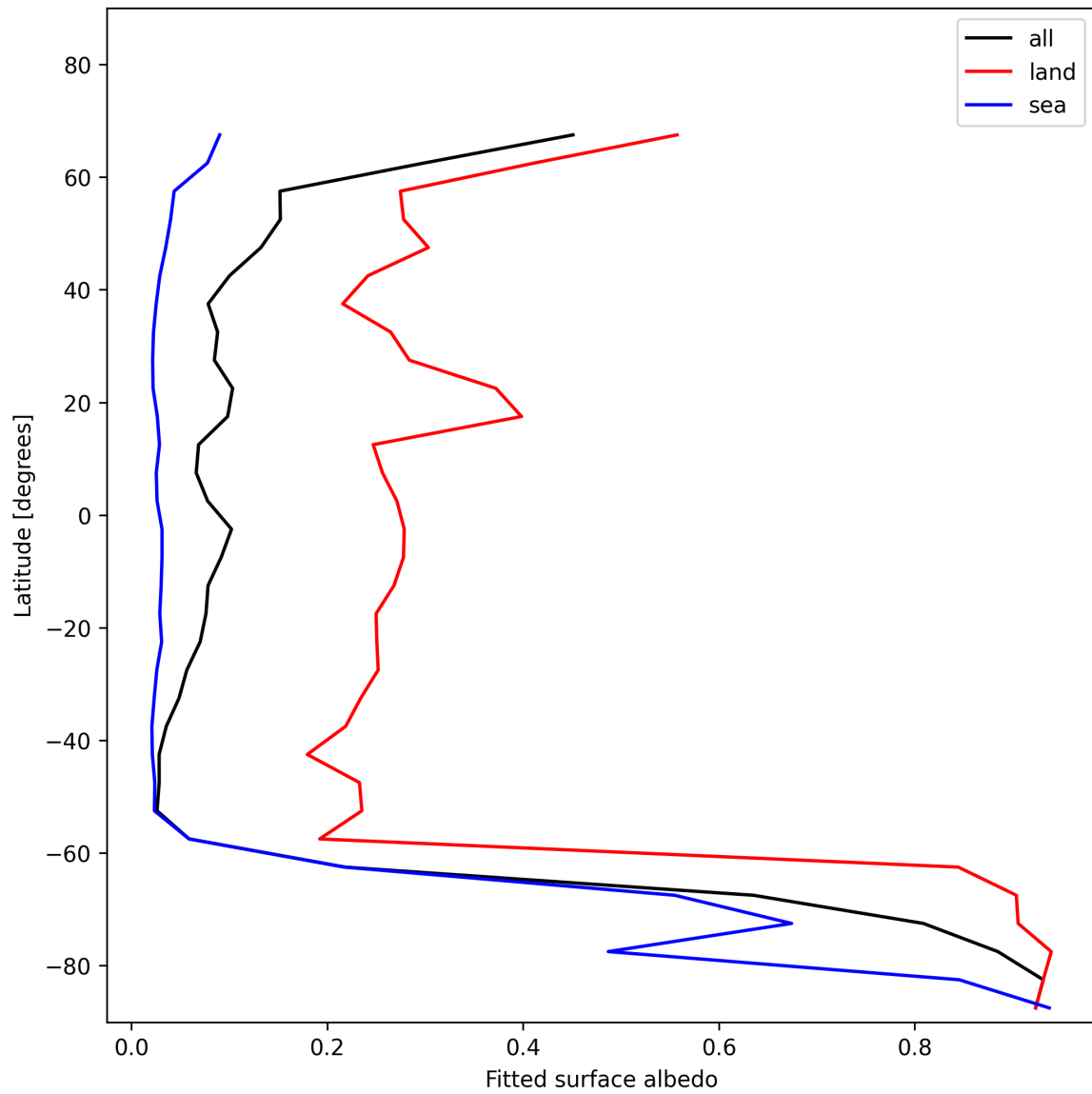
Figure 29: Zonal average of “Fitted surface albedo” for 2025-11-29 to 2025-12-01.
