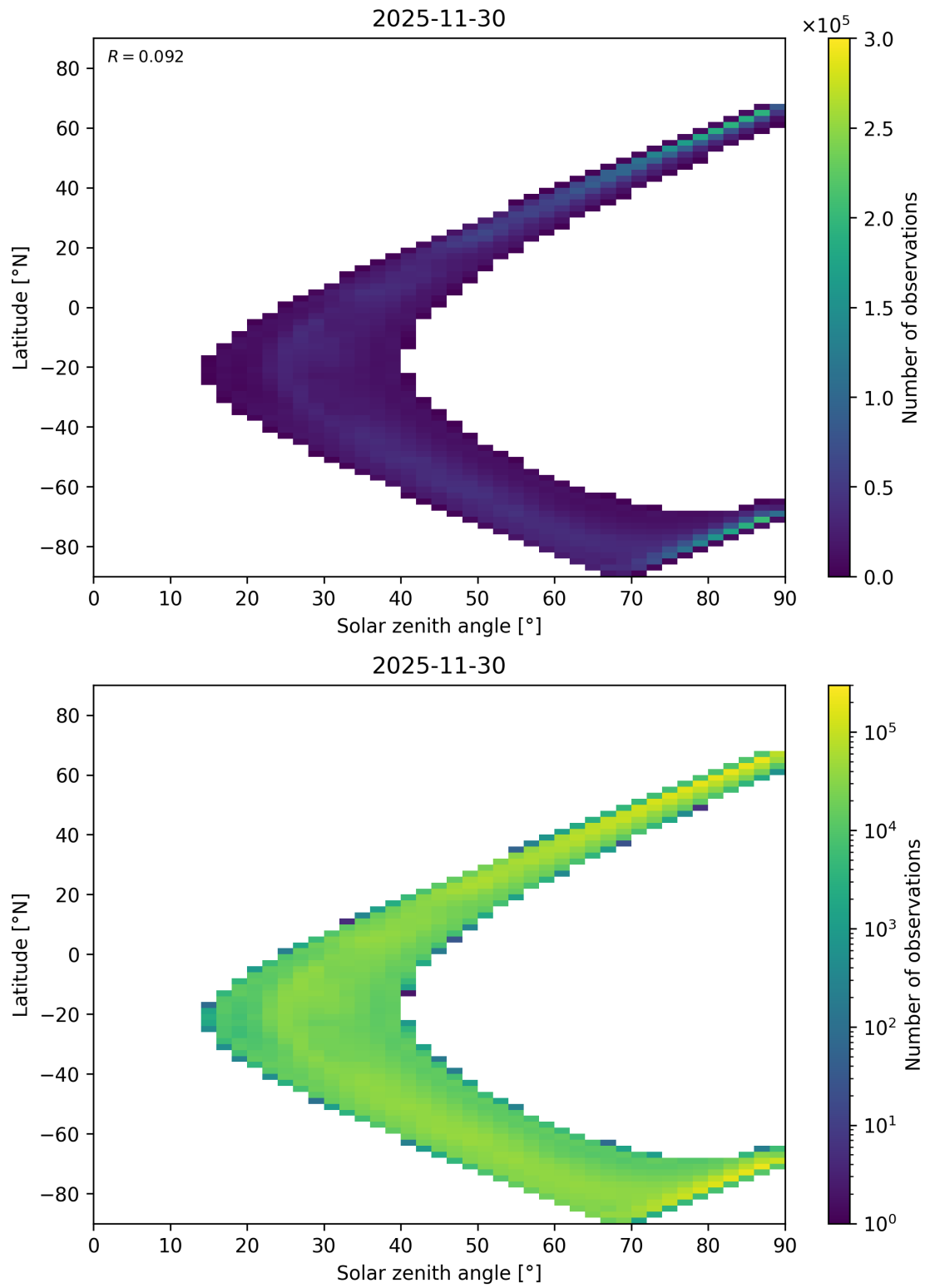
Figure 105: Scatter density plot of “Solar zenith angle” against “Latitude” for 2025-11-29 to 2025-12-01.
