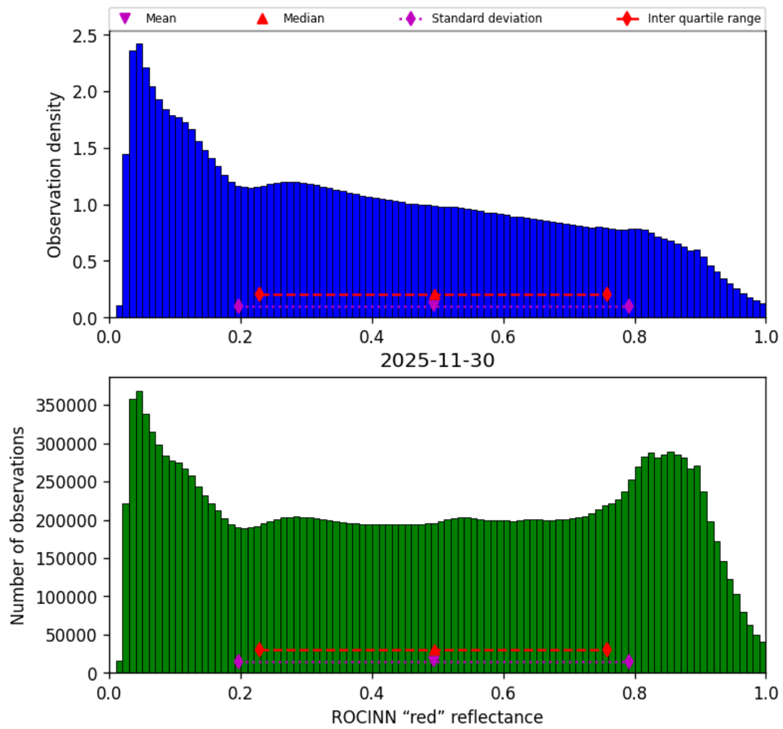
Figure 53: Histogram of “ROCINN “red” reflectance” for 2025-11-29 to 2025-12-01
