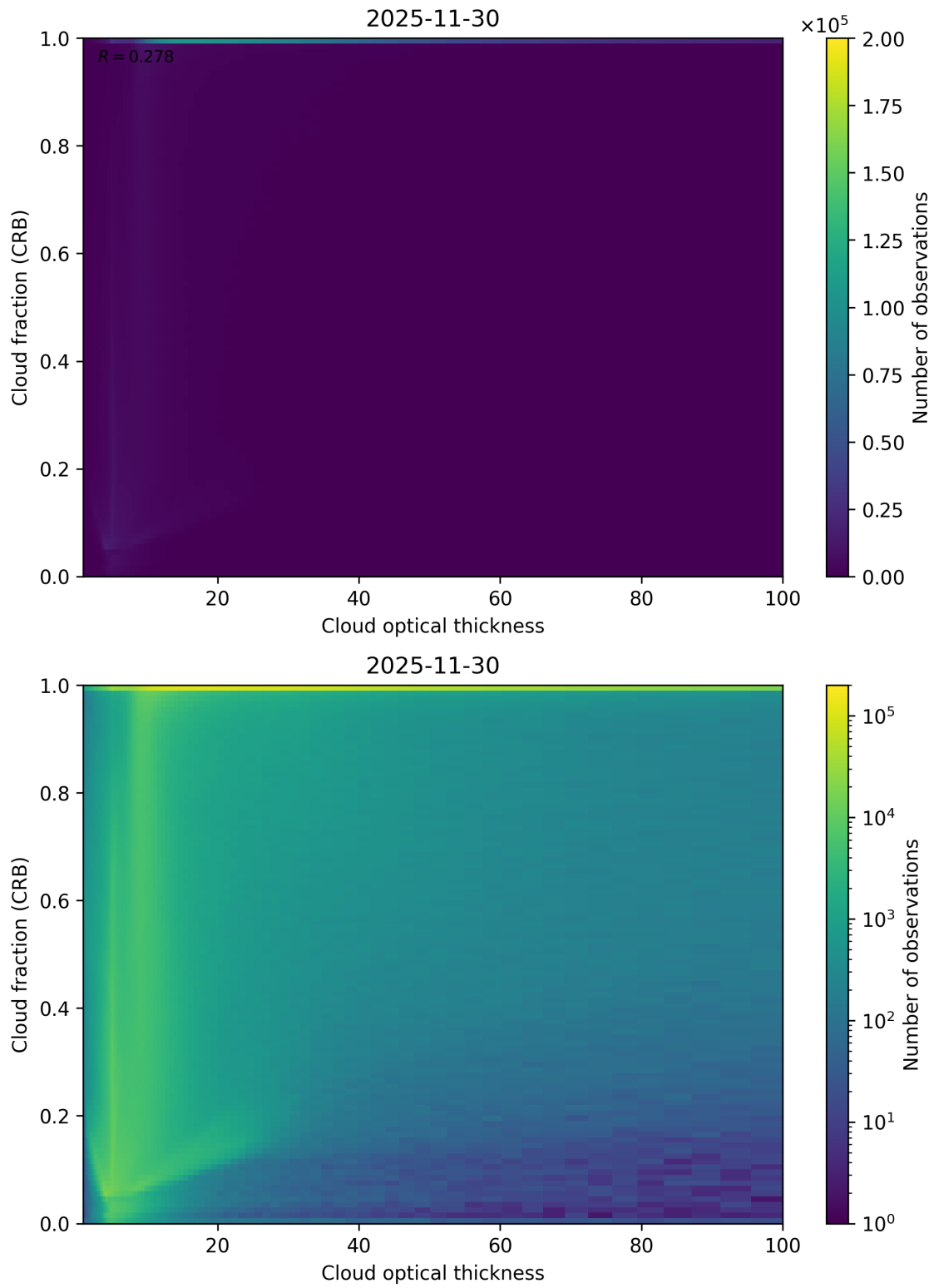
Figure 84: Scatter density plot of “Cloud optical thickness” against “Cloud fraction (CRB)” for 2025-11-29 to 2025-12-01.
