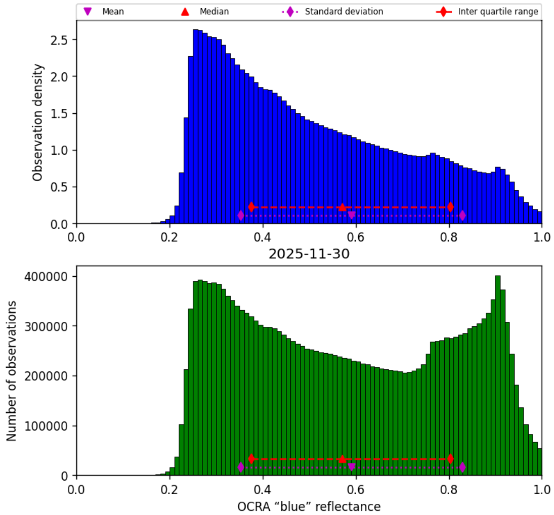
Figure 51: Histogram of “OCRA “blue” reflectance” for 2025-11-29 to 2025-12-01
