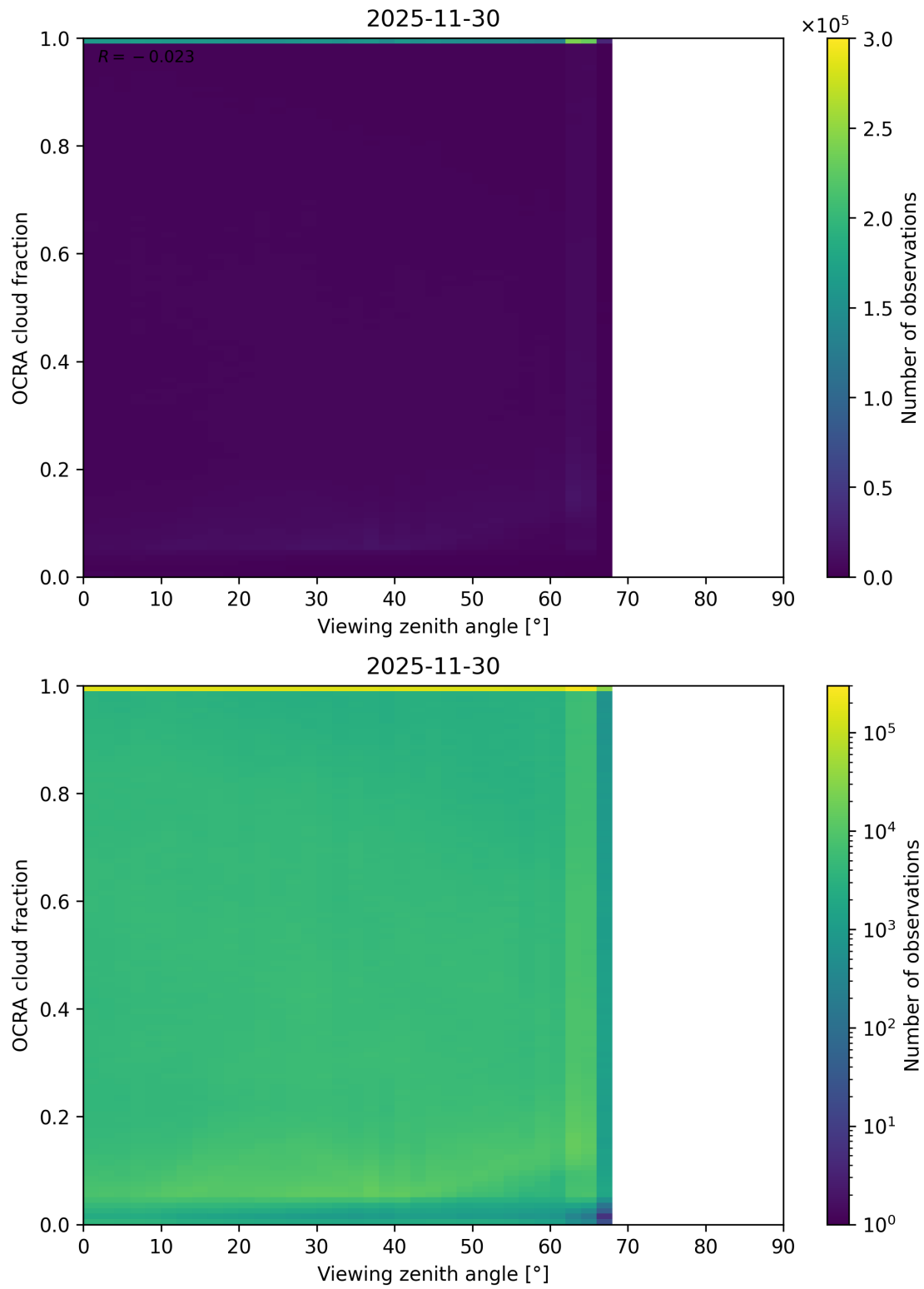
Figure 108: Scatter density plot of “Viewing zenith angle” against “OCRA cloud fraction” for 2025-11-29 to 2025-12-01.
