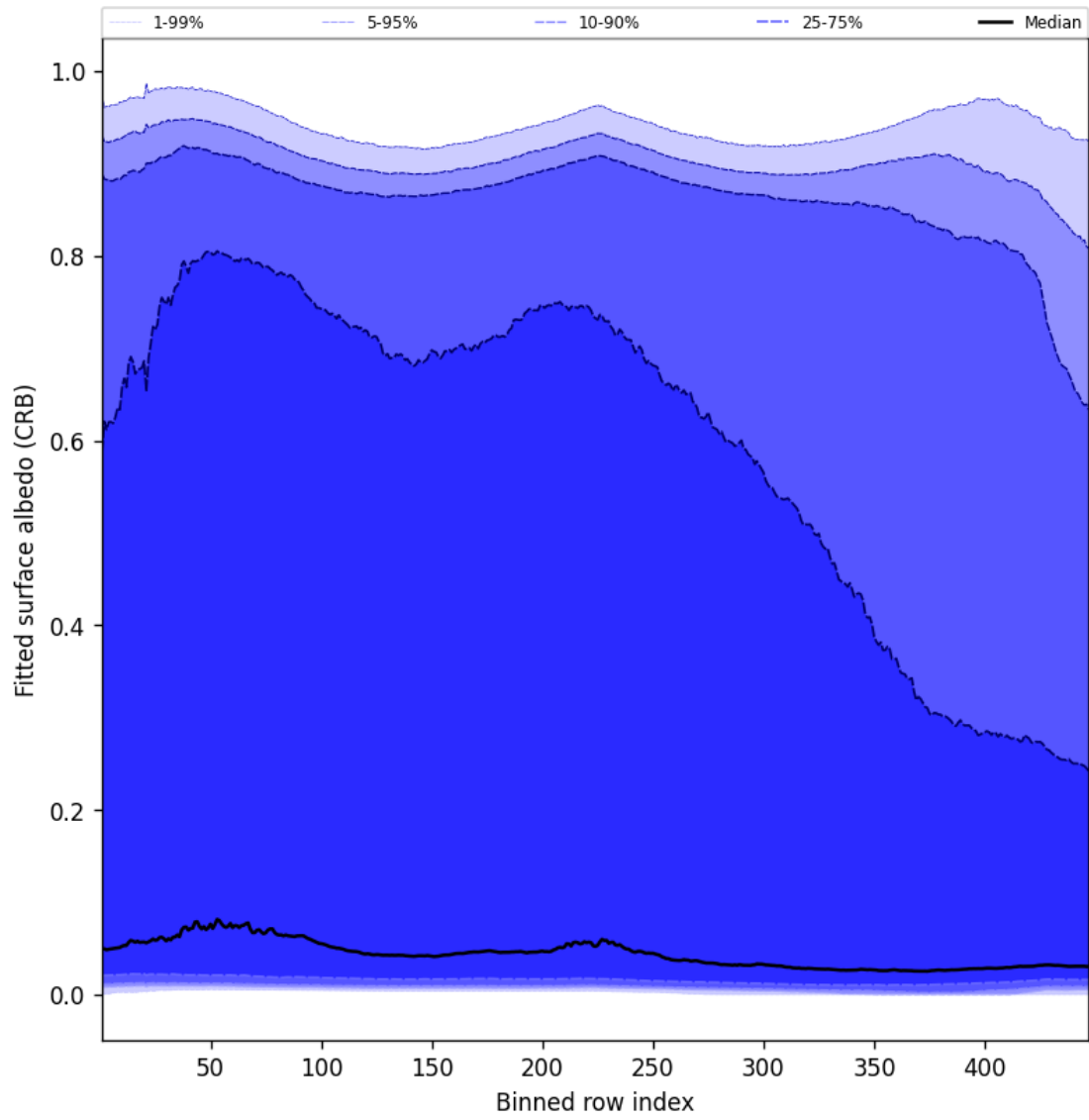
Figure 62: Along track statistics of “Fitted surface albedo (CRB)” for 2025-11-29 to 2025-12-01
