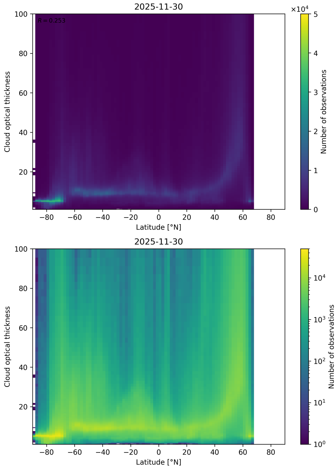
Figure 96: Scatter density plot of “Latitude” against “Cloud optical thickness” for 2025-11-29 to 2025-12-01.
