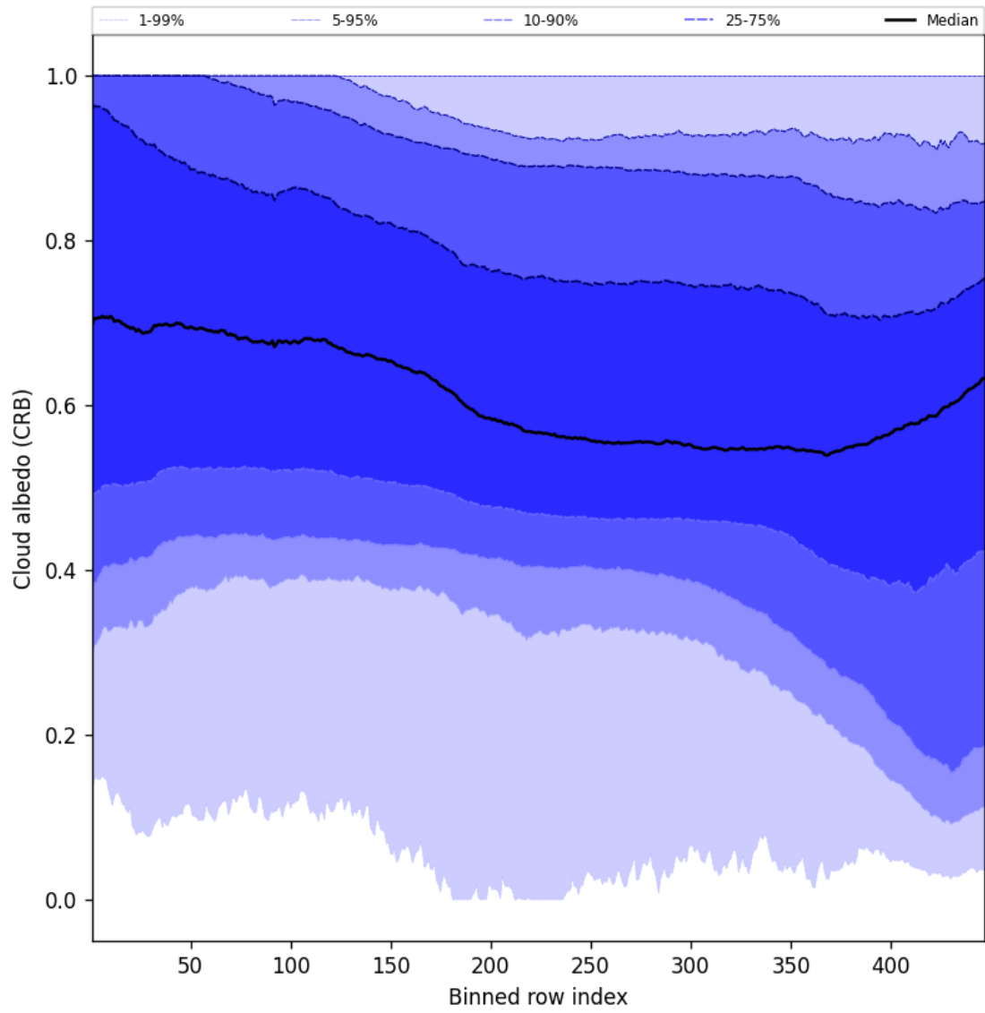
Figure 60: Along track statistics of “Cloud albedo (CRB)” for 2025-11-29 to 2025-12-01
