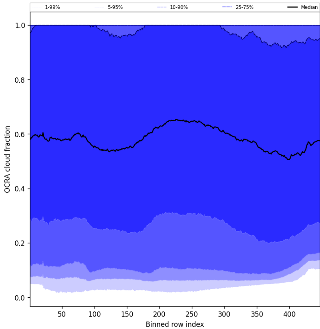
Figure 66: Along track statistics of “OCRA cloud fraction” for 2025-11-29 to 2025-12-01
