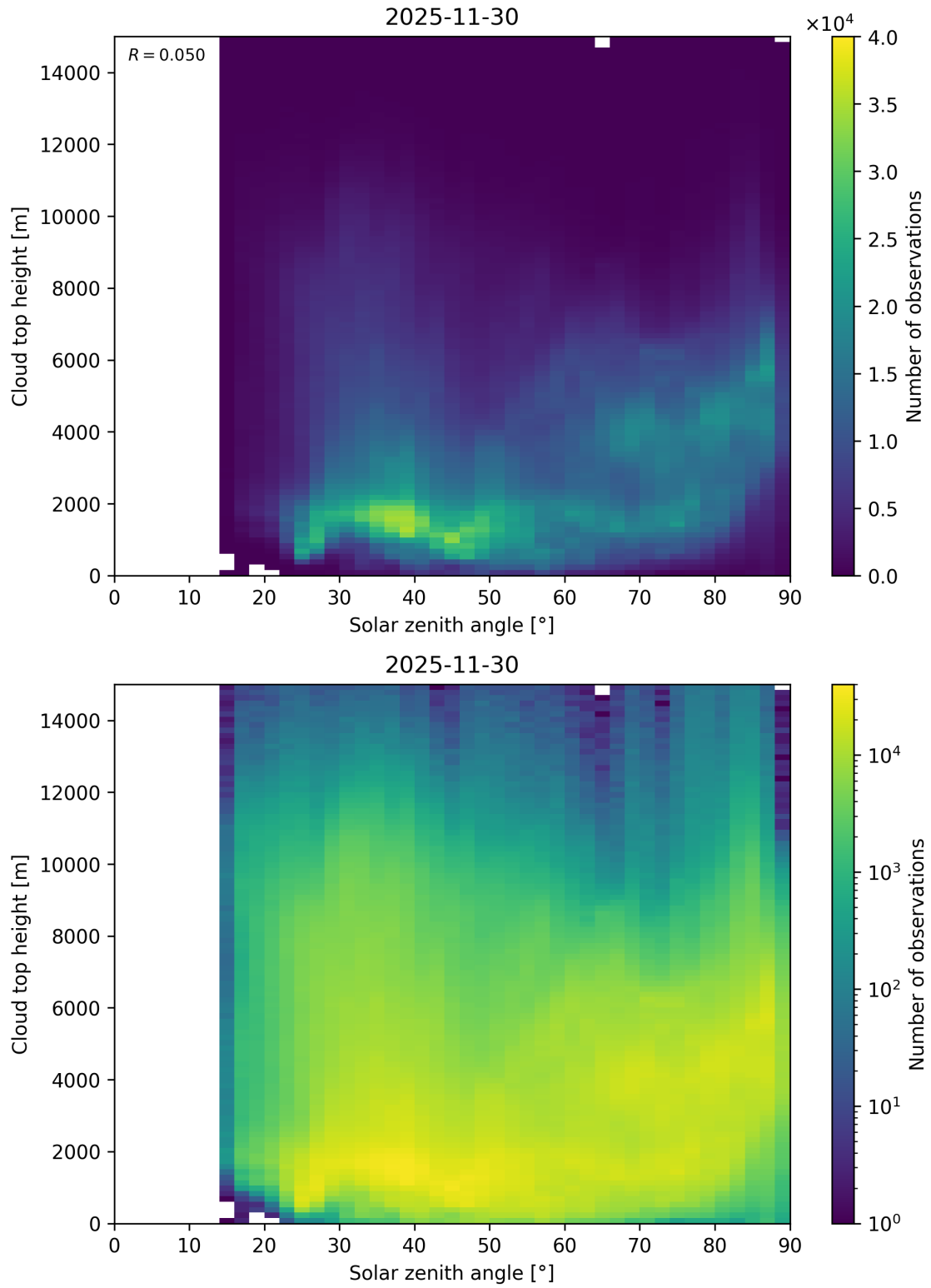
Figure 104: Scatter density plot of “Solar zenith angle” against “Cloud top height” for 2025-11-29 to 2025-12-01.
