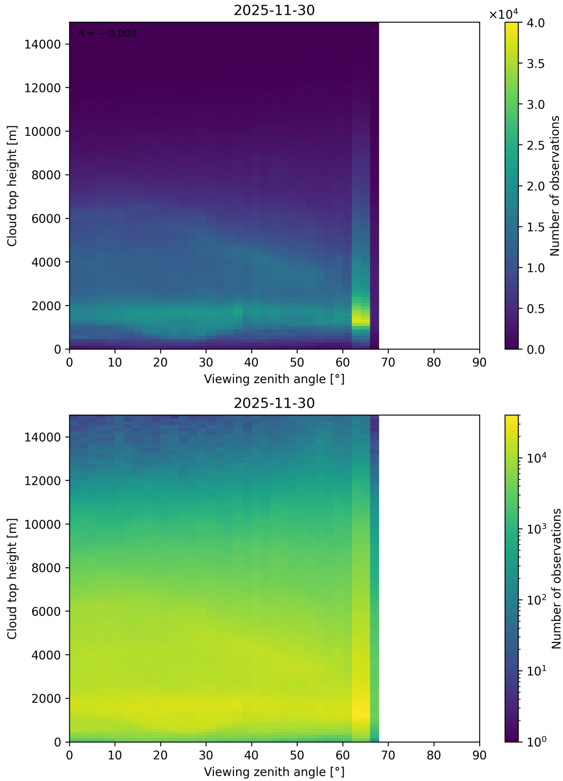
Figure 112: Scatter density plot of “Viewing zenith angle” against “Cloud top height” for 2025-11-29 to 2025-12-01.
