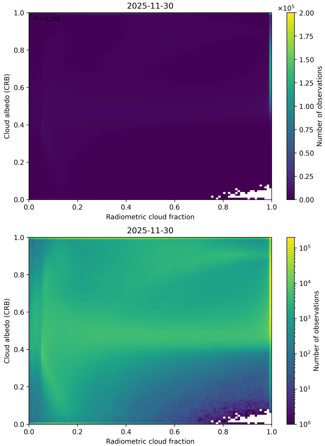
Figure 71: Scatter density plot of “Radiometric cloud fraction” against “Cloud albedo (CRB)” for 2025-11-29 to 2025-12-01.
