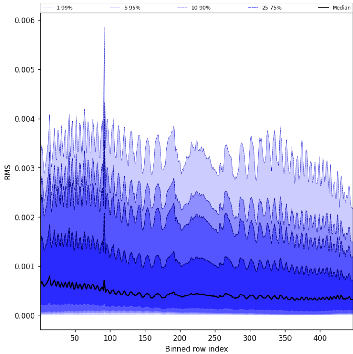
Figure 63: Along track statistics of “RMS” for 2025-11-29 to 2025-12-01
