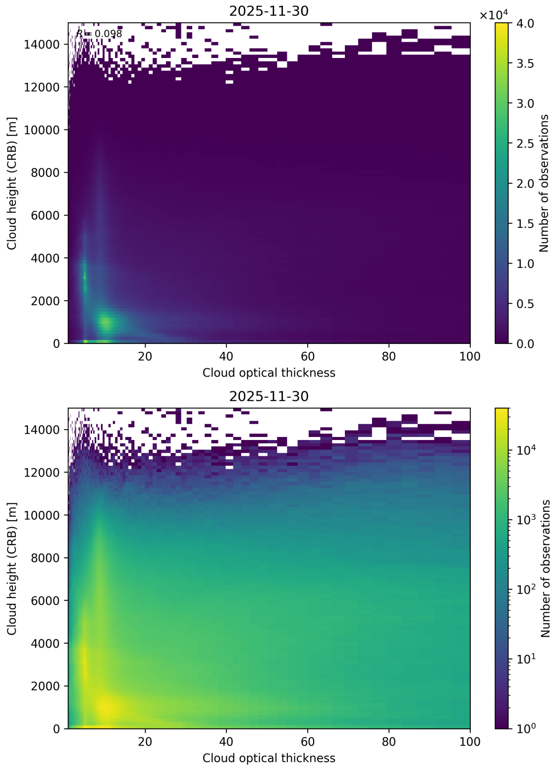
Figure 85: Scatter density plot of “Cloud optical thickness” against “Cloud height (CRB)” for 2025-11-29 to 2025-12-01.
