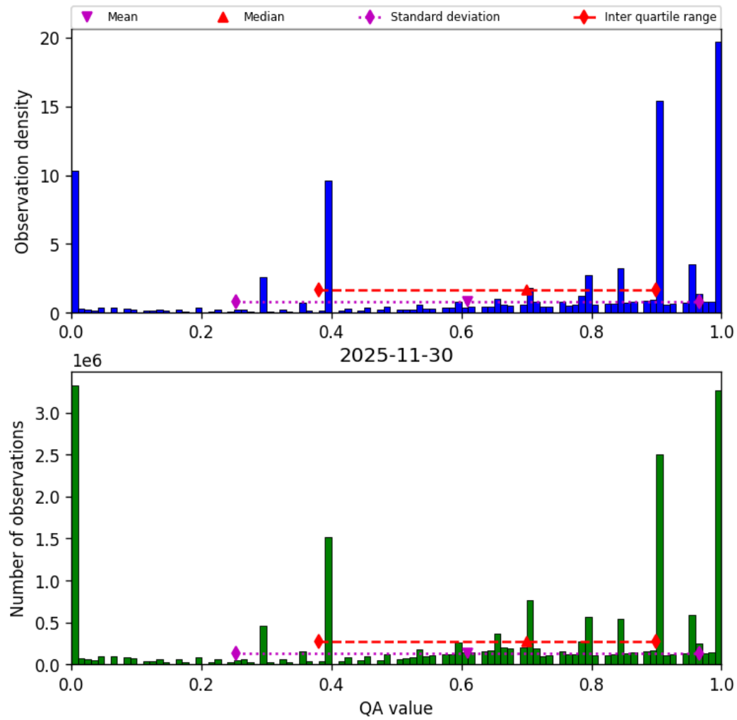
Figure 38: Histogram of “QA value” for 2025-11-29 to 2025-12-01
