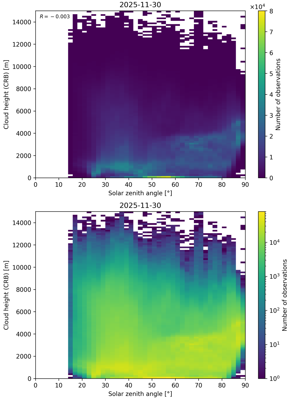
Figure 102: Scatter density plot of “Solar zenith angle” against “Cloud height (CRB)” for 2025-11-29 to 2025-12-01.
