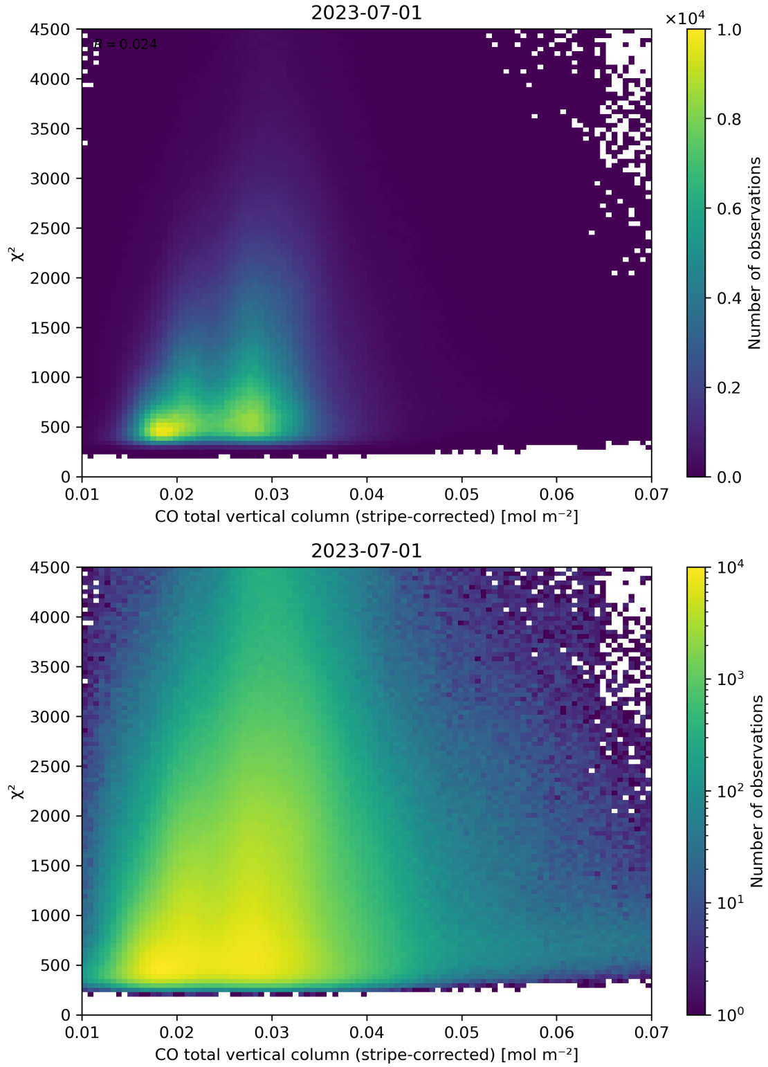
Figure 37: Scatter density plot of “CO total vertical column (stripe-corrected)” against “ \chi^2 ” for 2023-06-30 to 2023-07-02.
