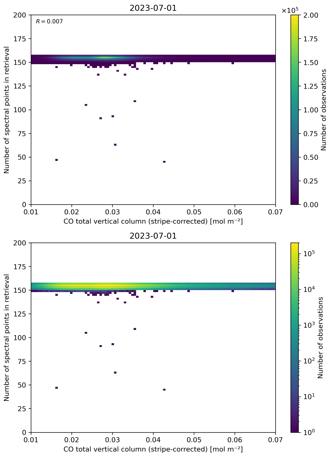
Figure 40: Scatter density plot of “CO total vertical column (stripe-corrected)” against “Number of spectral points in retrieval” for 2023-06-30 to 2023-07-02.
