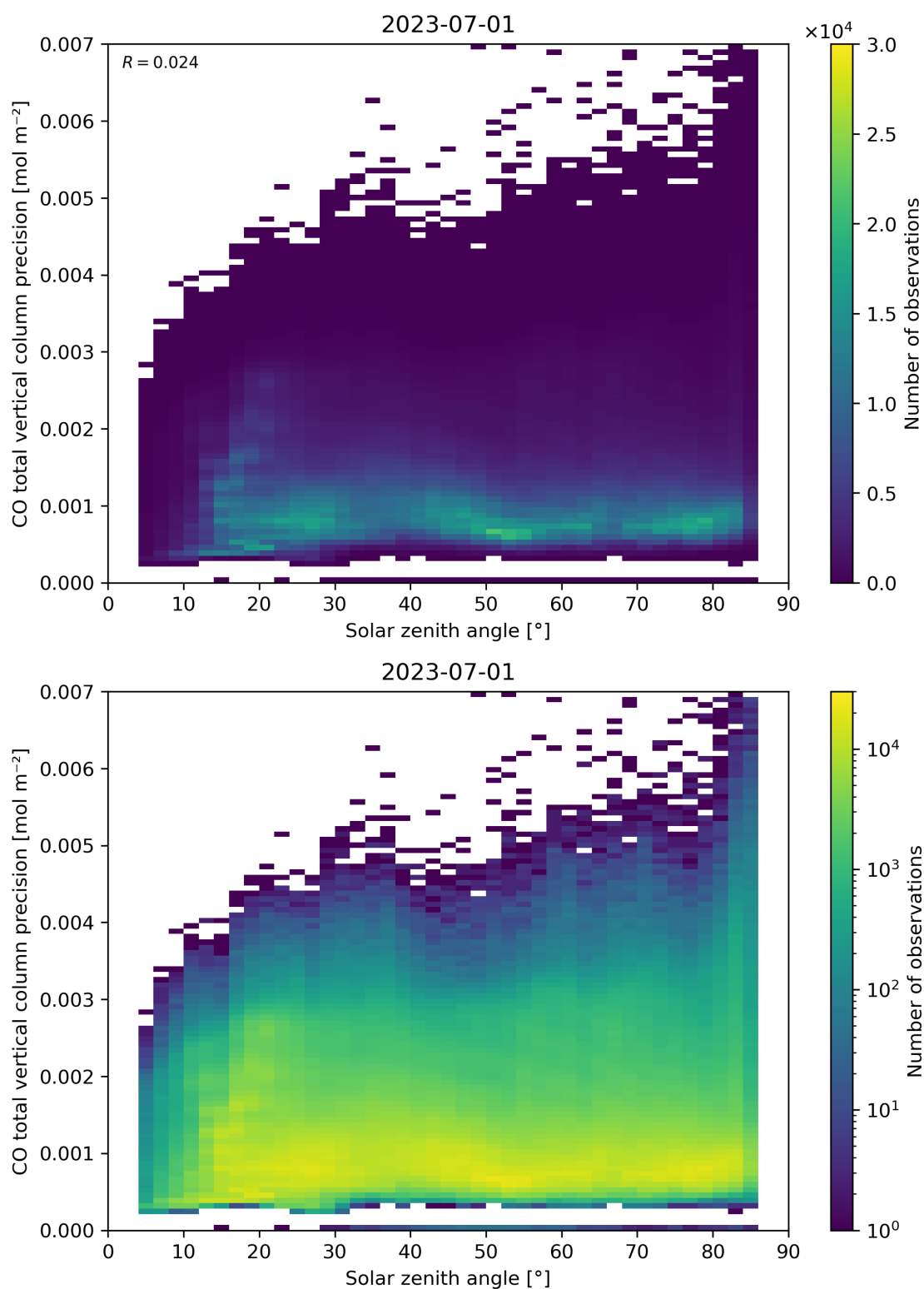
Figure 63: Scatter density plot of “Solar zenith angle” against “CO total vertical column precision” for 2023-06-30 to 2023-07-02.
