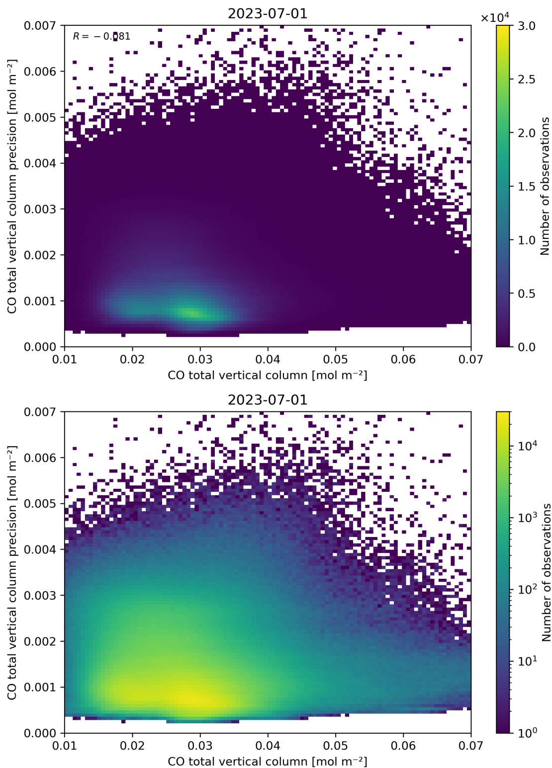
Figure 34: Scatter density plot of “CO total vertical column” against “CO total vertical column precision” for 2023-06-30 to 2023-07-02.
