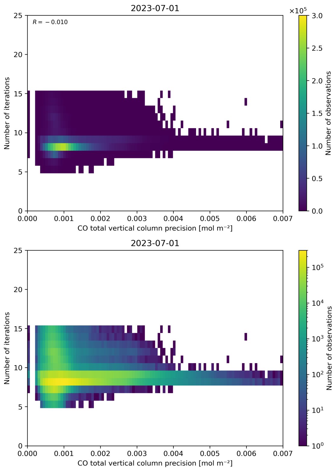
Figure 46: Scatter density plot of “CO total vertical column precision” against “Number of iterations” for 2023-06-30 to 2023-07-02.
