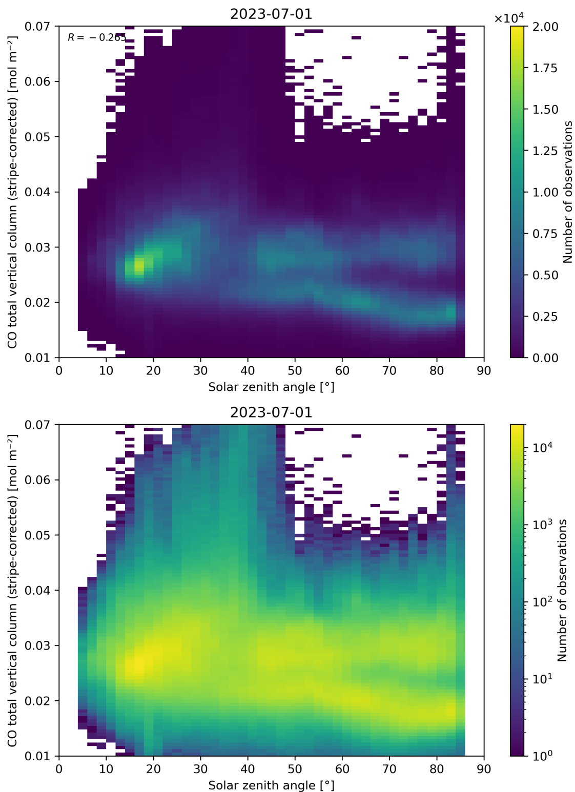
Figure 62: Scatter density plot of “Solar zenith angle” against “CO total vertical column (stripe-corrected)” for 2023-06-30 to 2023-07-02.
