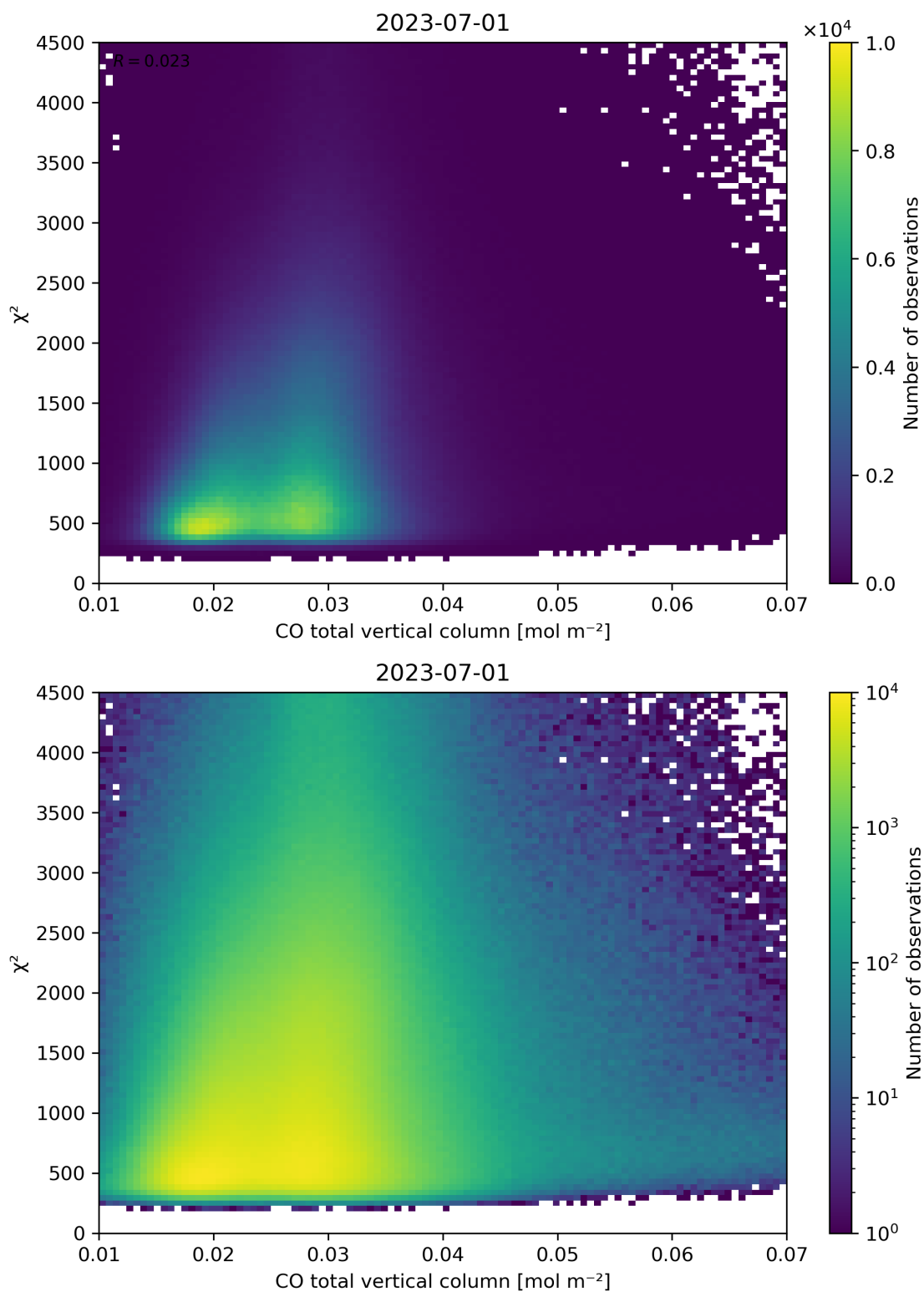
Figure 35: Scatter density plot of “CO total vertical column” against “ \chi^2 ” for 2023-06-30 to 2023-07-02.
