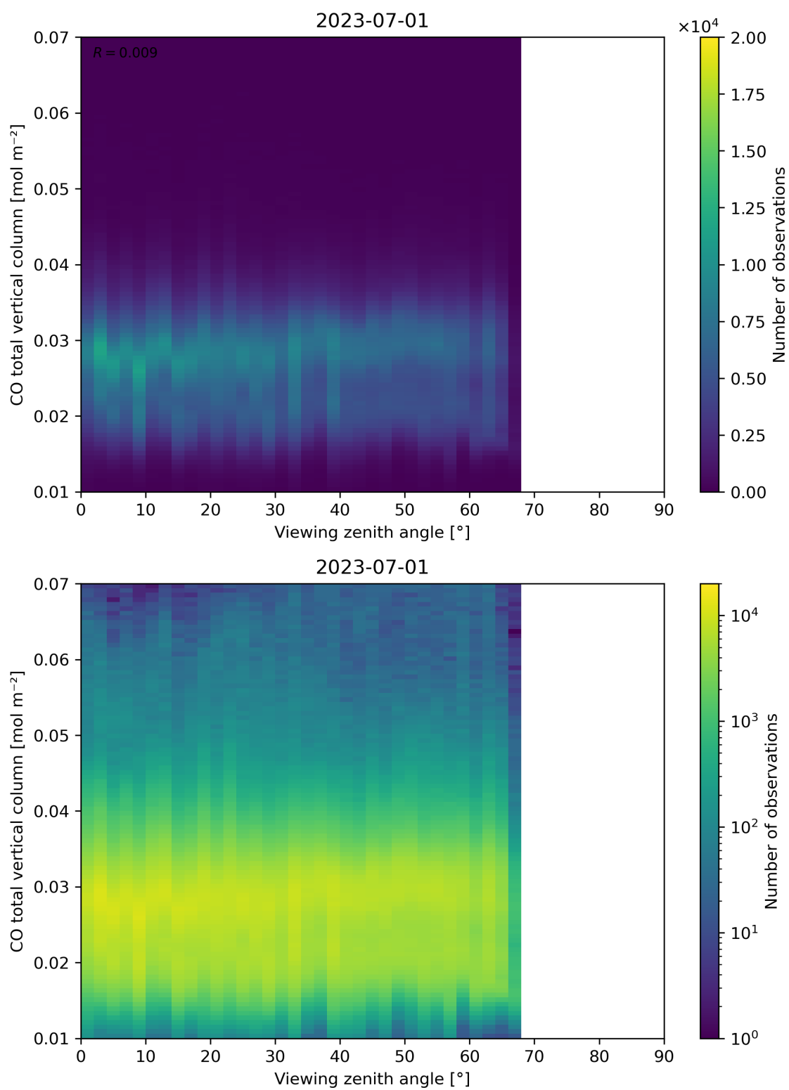
Figure 69: Scatter density plot of “Viewing zenith angle” against “CO total vertical column” for 2023-06-30 to 2023-07-02.
