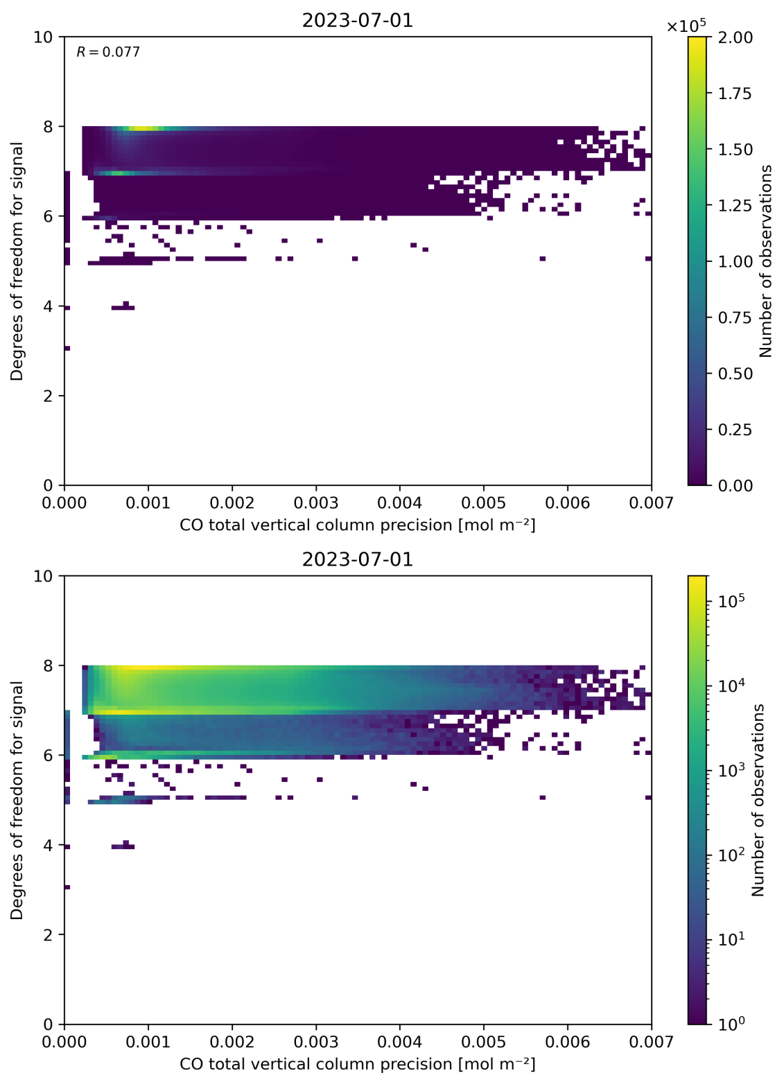
Figure 45: Scatter density plot of “CO total vertical column precision” against “Degrees of freedom for signal” for 2023-06-30 to 2023-07-02.
