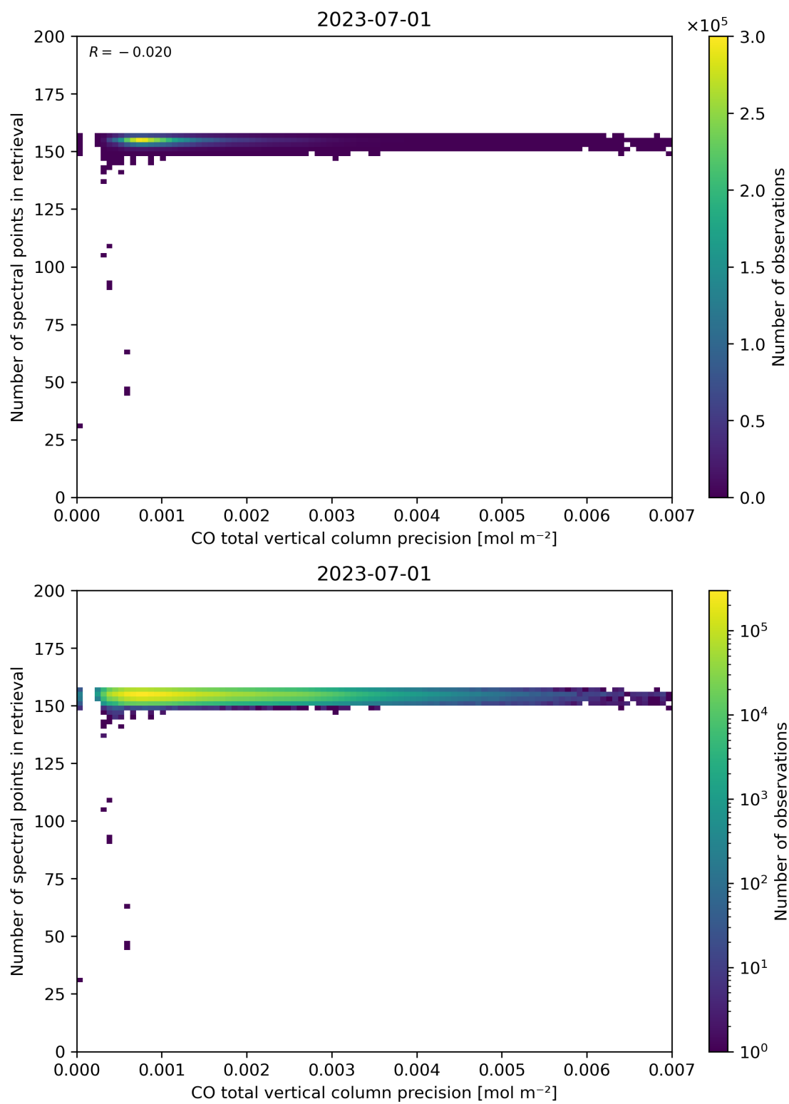
Figure 47: Scatter density plot of “CO total vertical column precision” against “Number of spectral points in retrieval” for 2023-06-30 to 2023-07-02.
