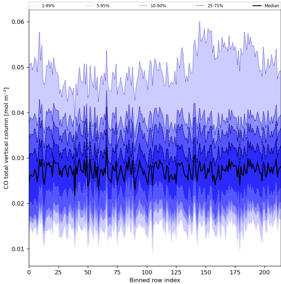
Figure 26: Along track statistics of “CO total vertical column” for 2023-06-30 to 2023-07-02
