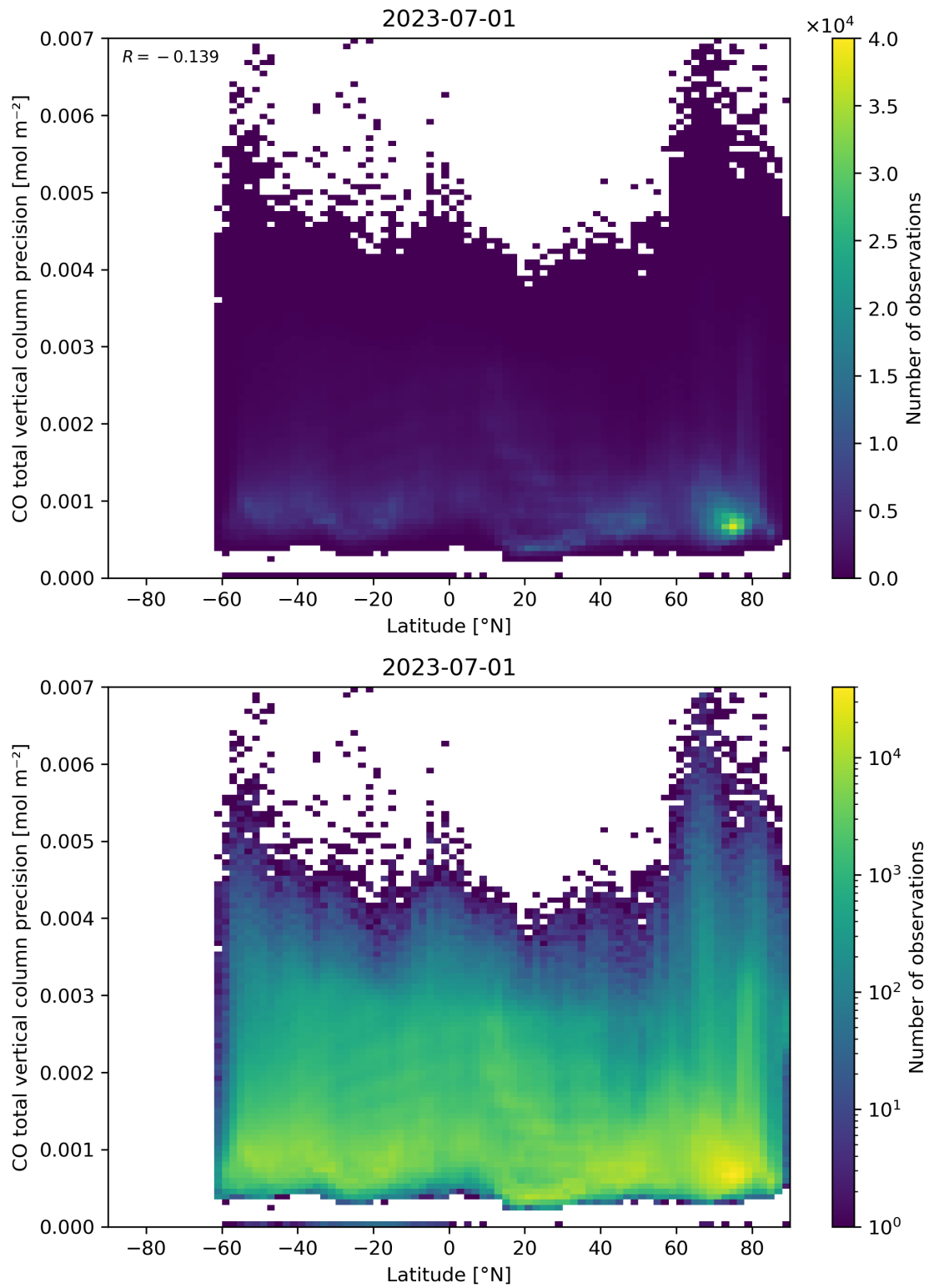
Figure 53: Scatter density plot of “Latitude” against “CO total vertical column precision” for 2023-06-30 to 2023-07-02.
