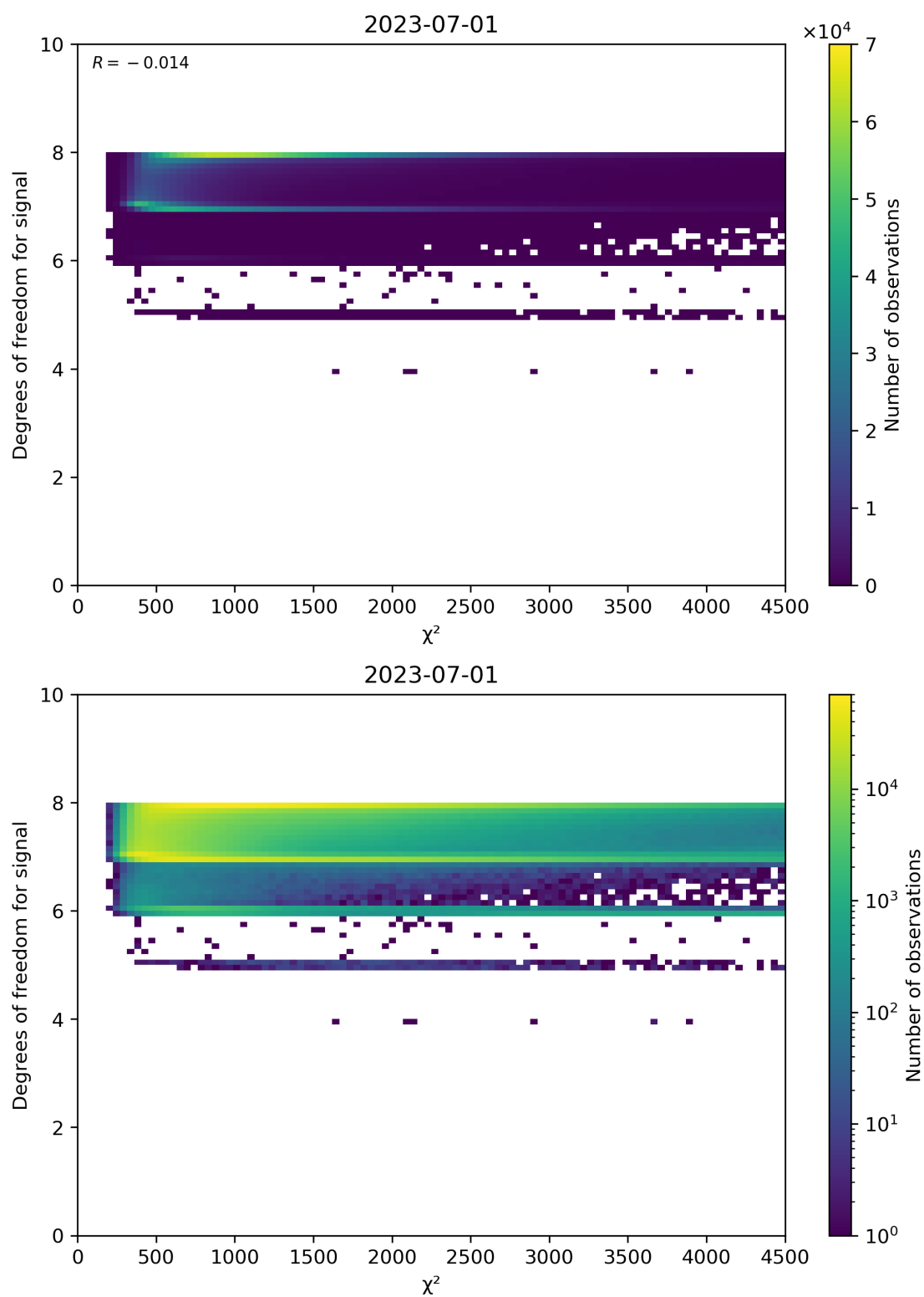
Figure 48: Scatter density plot of “ \chi^2 ” against “Degrees of freedom for signal” for 2023-06-30 to 2023-07-02.
