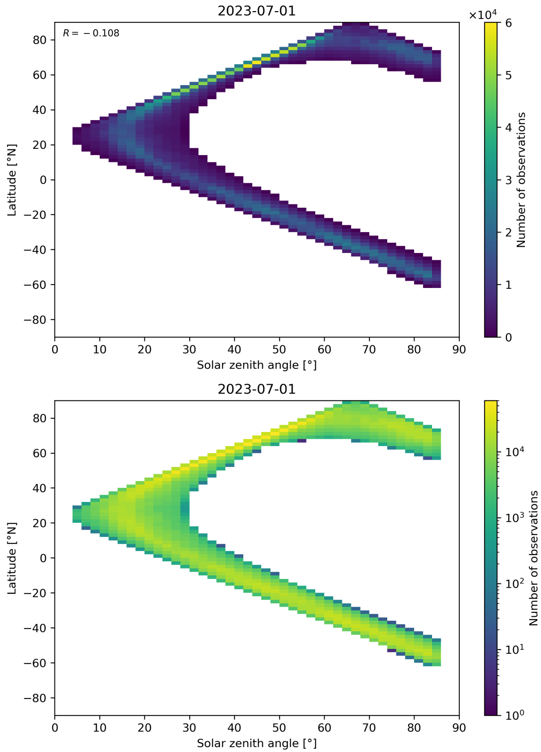
Figure 66: Scatter density plot of “Solar zenith angle” against “Latitude” for 2023-06-30 to 2023-07-02.
