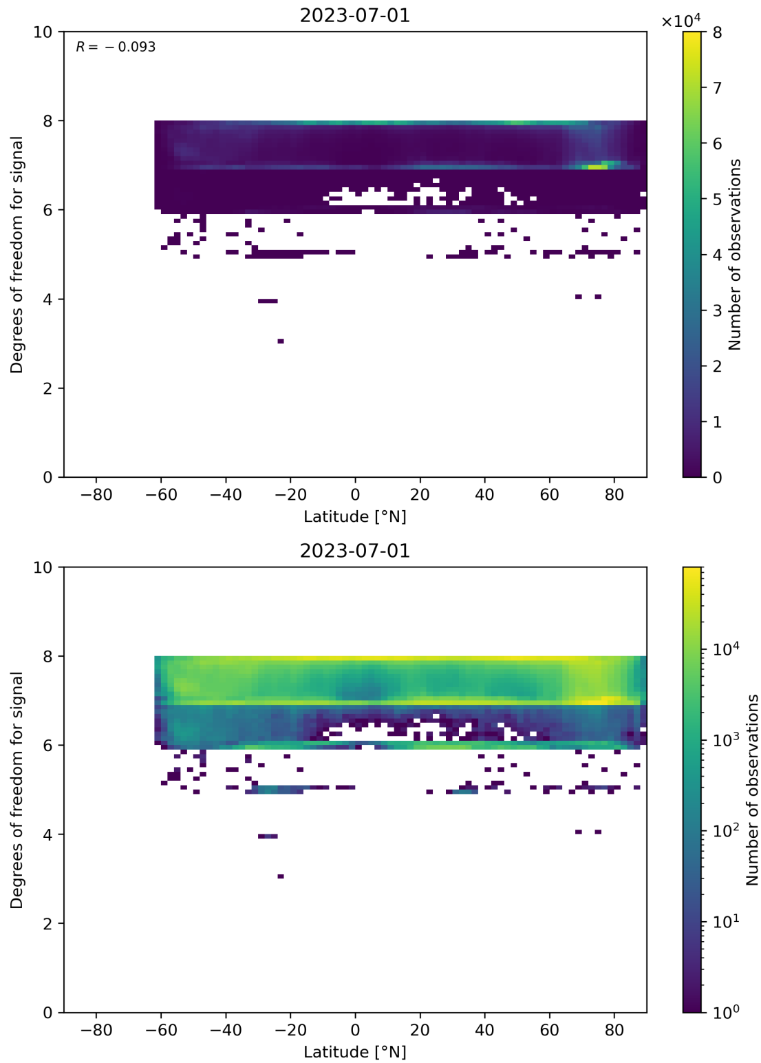
Figure 55: Scatter density plot of “Latitude” against “Degrees of freedom for signal” for 2023-06-30 to 2023-07-02.
