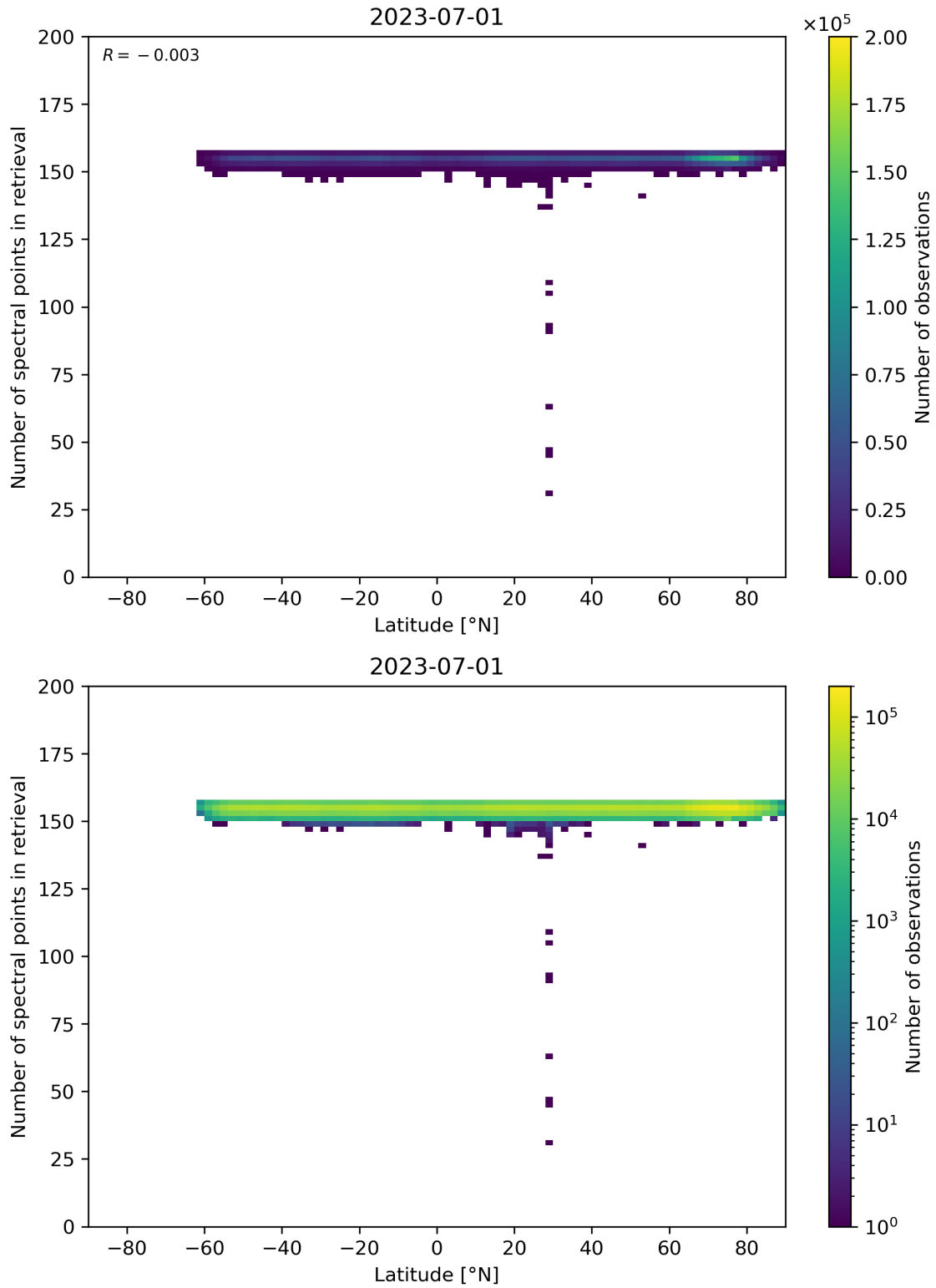
Figure 57: Scatter density plot of “Latitude” against “Number of spectral points in retrieval” for 2023-06-30 to 2023-07-02.
