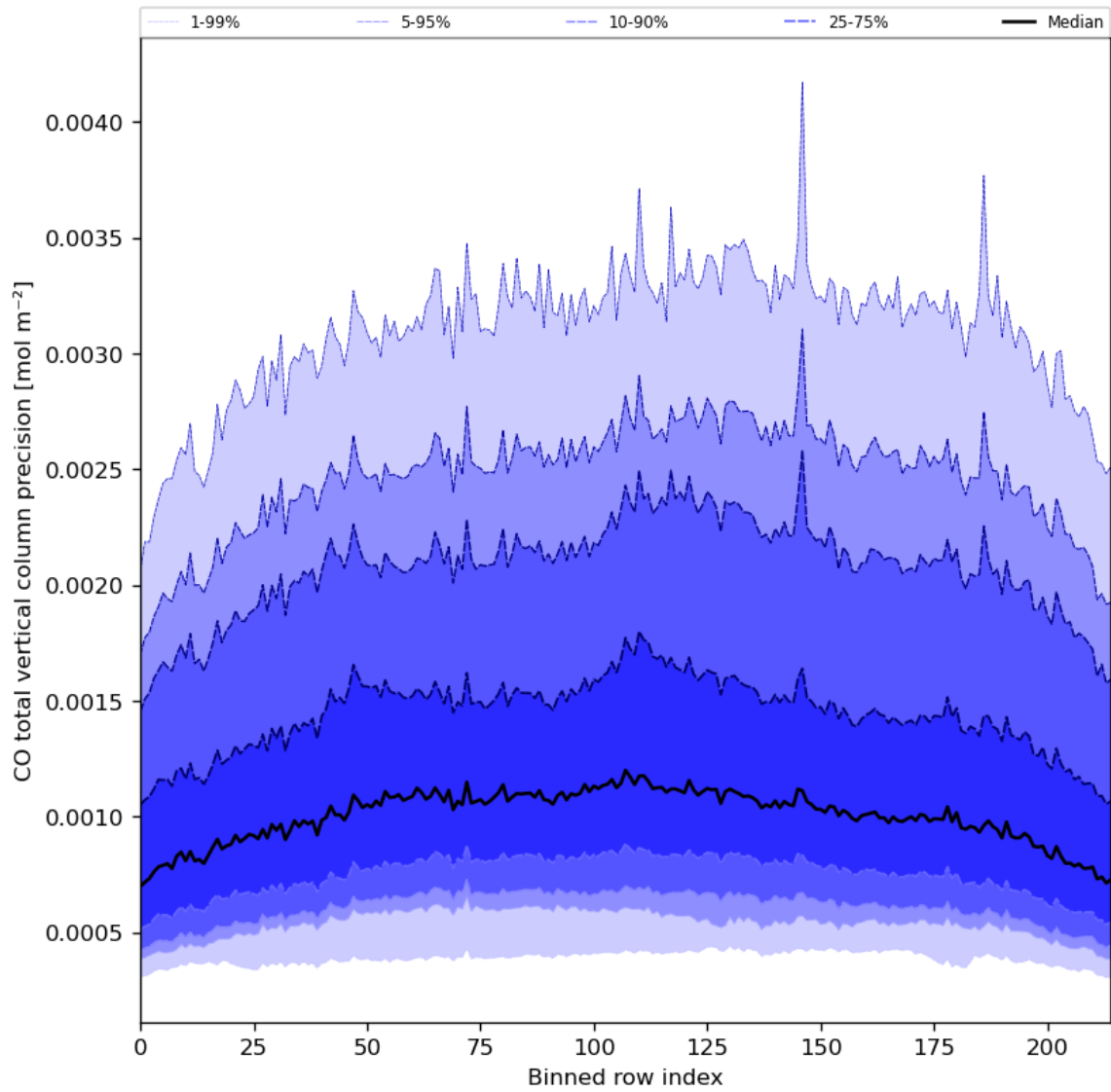
Figure 28: Along track statistics of “CO total vertical column precision” for 2023-06-30 to 2023-07-02
