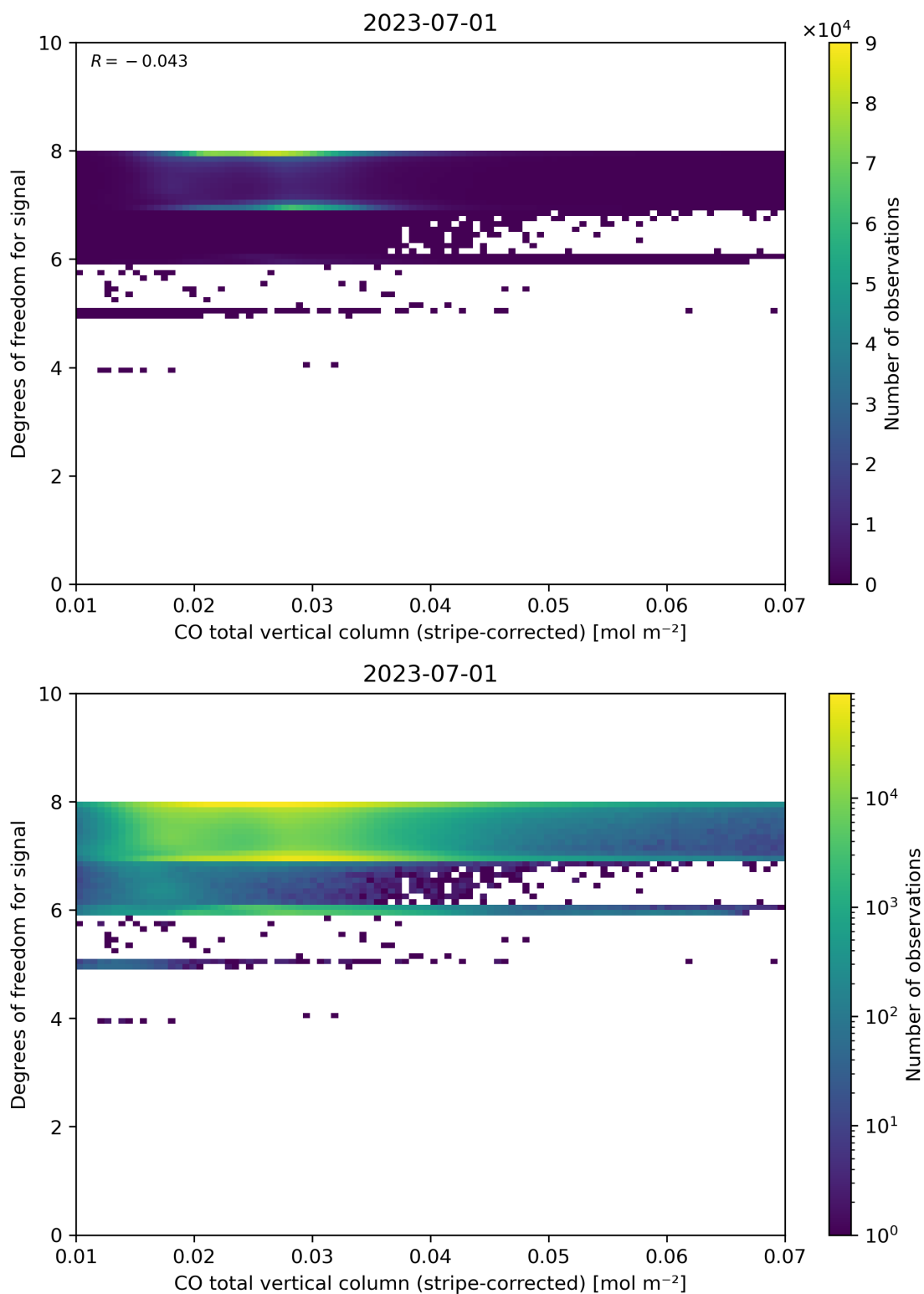
Figure 38: Scatter density plot of “CO total vertical column (stripe-corrected)” against “Degrees of freedom for signal” for 2023-06-30 to 2023-07-02.
