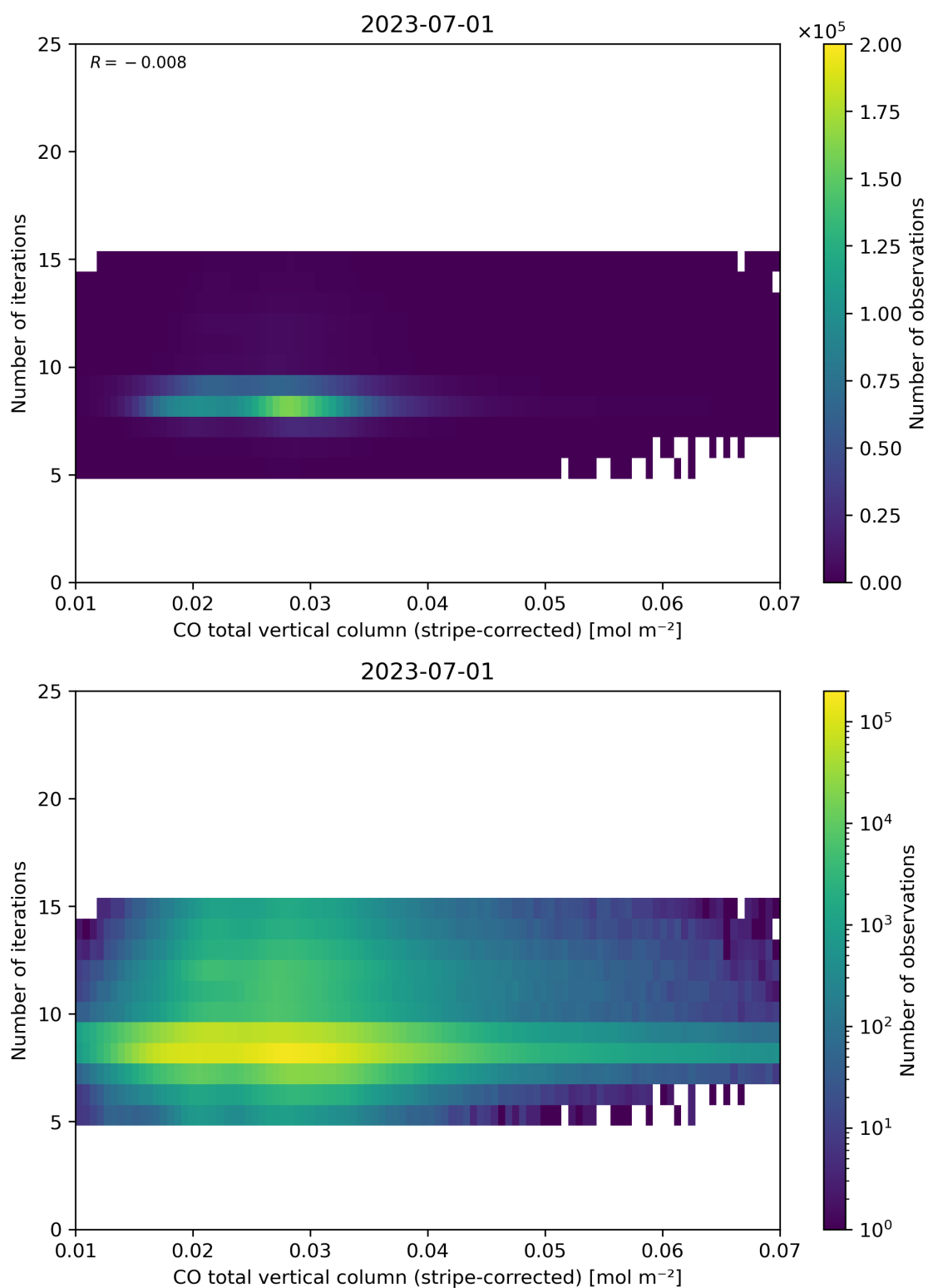
Figure 39: Scatter density plot of “CO total vertical column (stripe-corrected)” against “Number of iterations” for 2023-06-30 to 2023-07-02.
