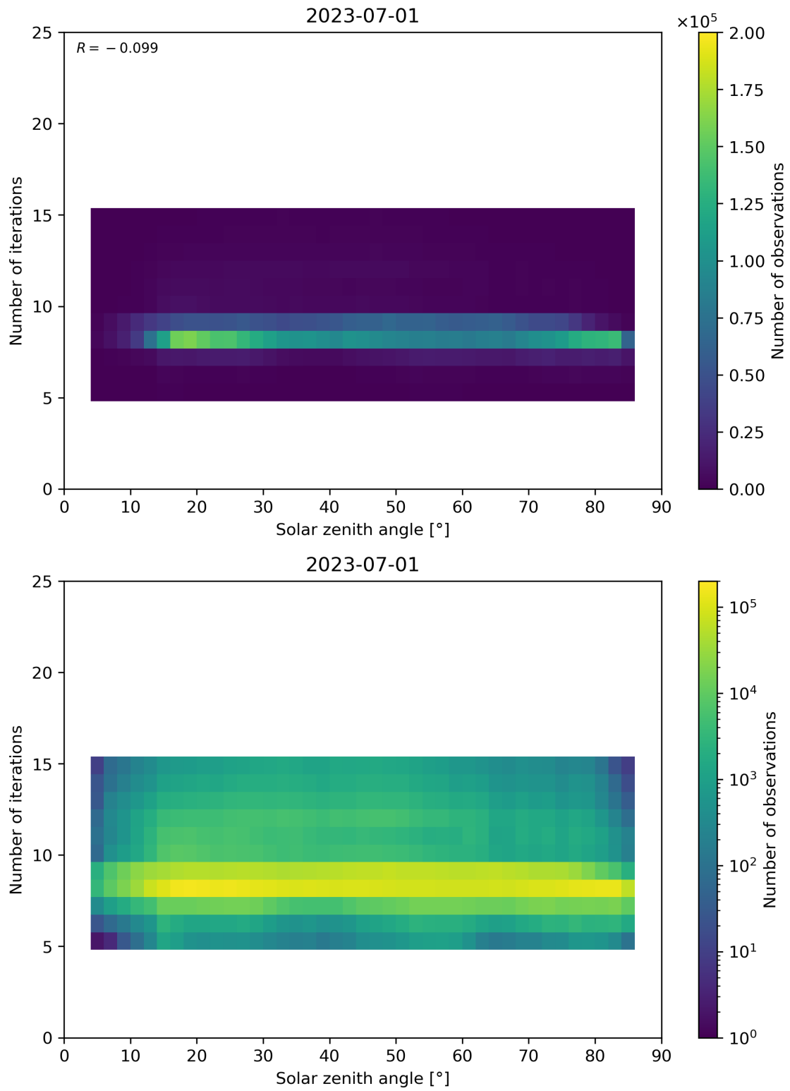
Figure 67: Scatter density plot of “Solar zenith angle” against “Number of iterations” for 2023-06-30 to 2023-07-02.
