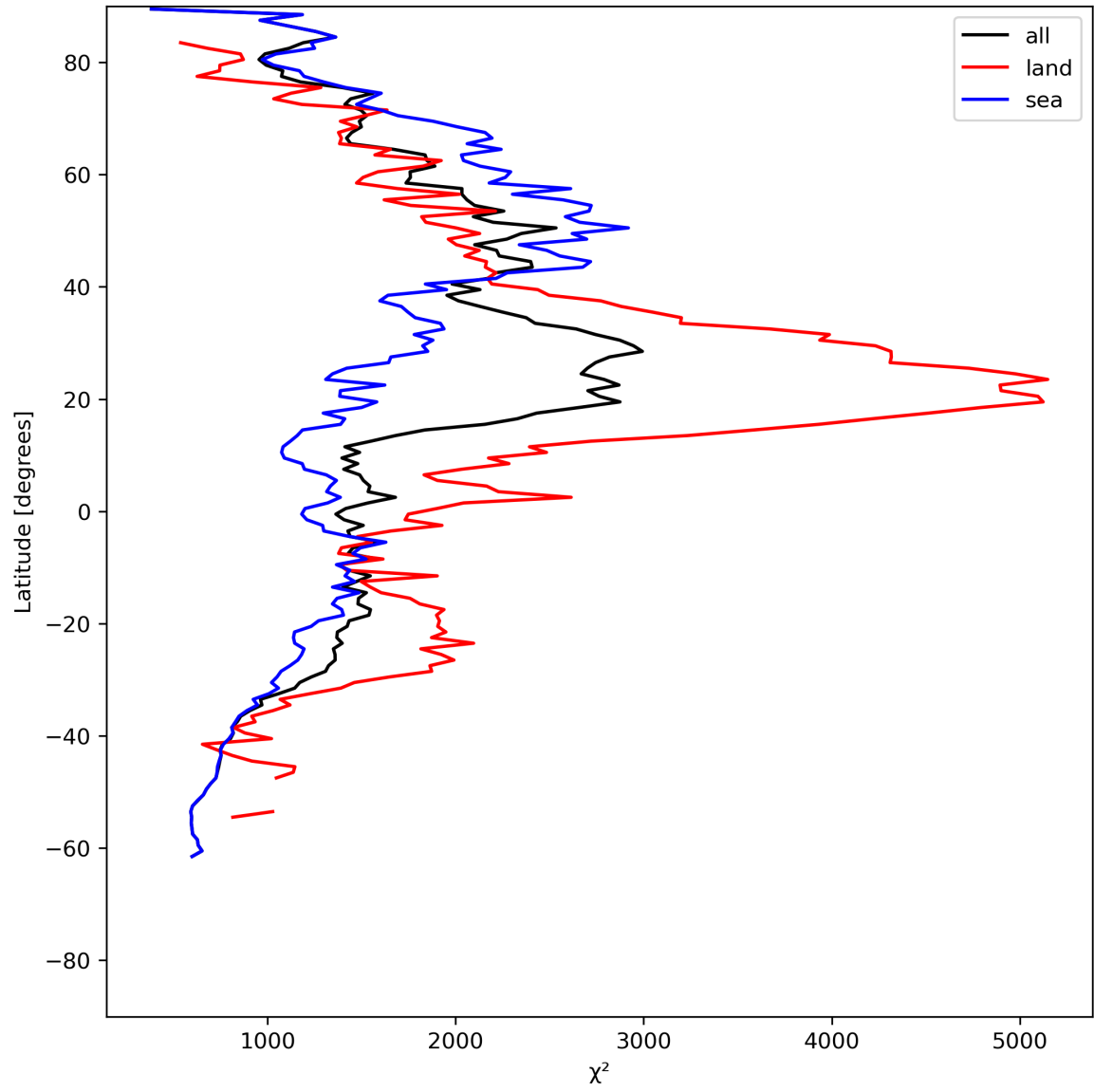
Figure 14: Zonal average of “ \chi^2 ” for 2023-06-30 to 2023-07-02.
