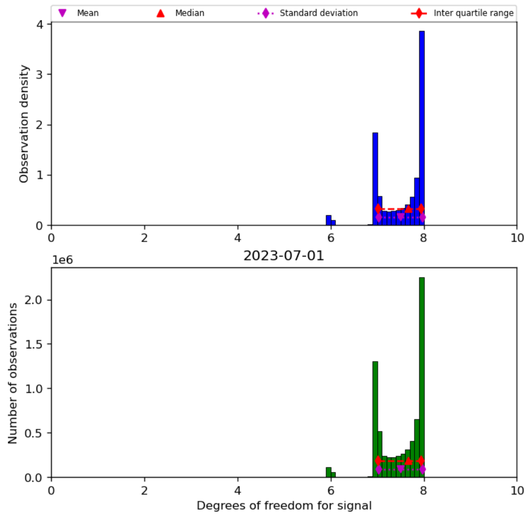
Figure 23: Histogram of “Degrees of freedom for signal” for 2023-06-30 to 2023-07-02
