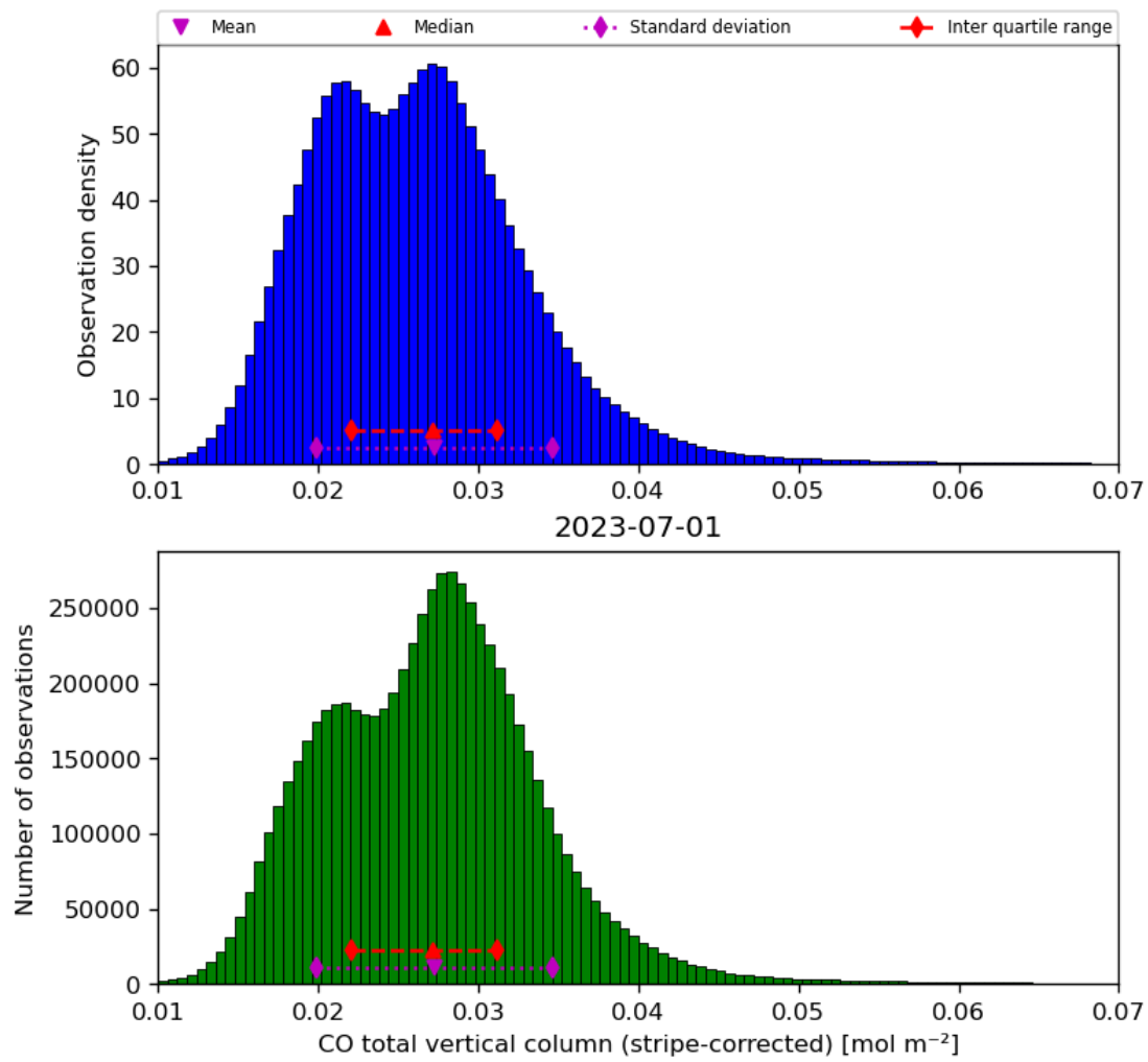
Figure 19: Histogram of “CO total vertical column (stripe-corrected)” for 2023-06-30 to 2023-07-02
