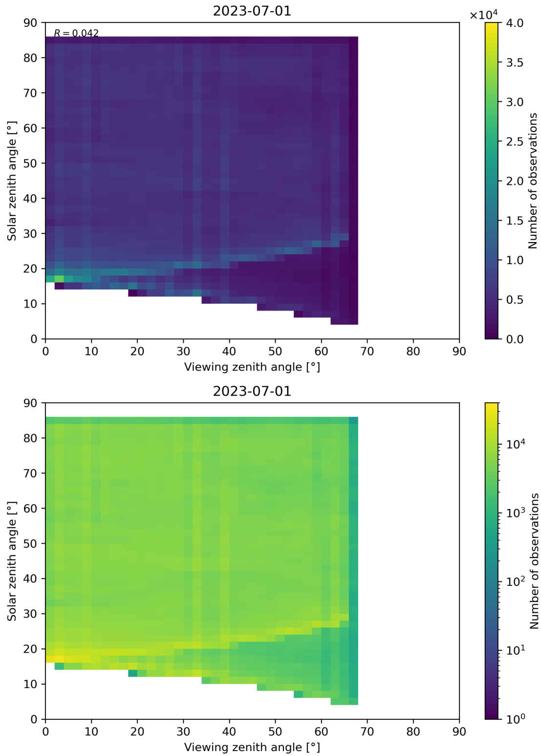
Figure 77: Scatter density plot of “Viewing zenith angle” against “Solar zenith angle” for 2023-06-30 to 2023-07-02.
