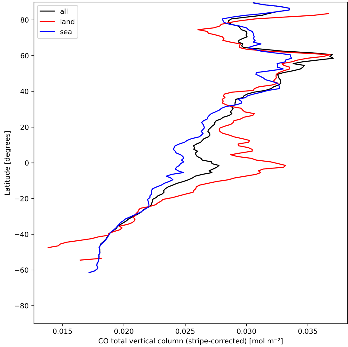
Figure 11: Zonal average of “CO total vertical column (stripe-corrected)” for 2023-06-30 to 2023-07-02.
