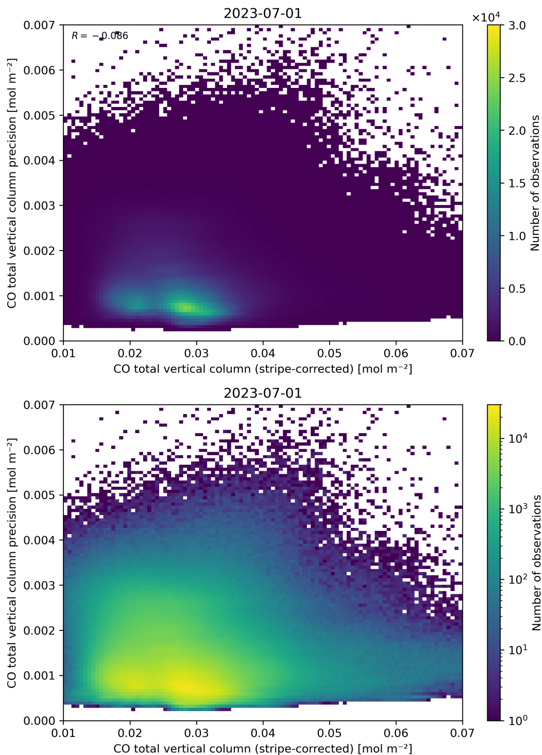
Figure 36: Scatter density plot of “CO total vertical column (stripe-corrected)” against “CO total vertical column precision” for 2023-06-30 to 2023-07-02.
