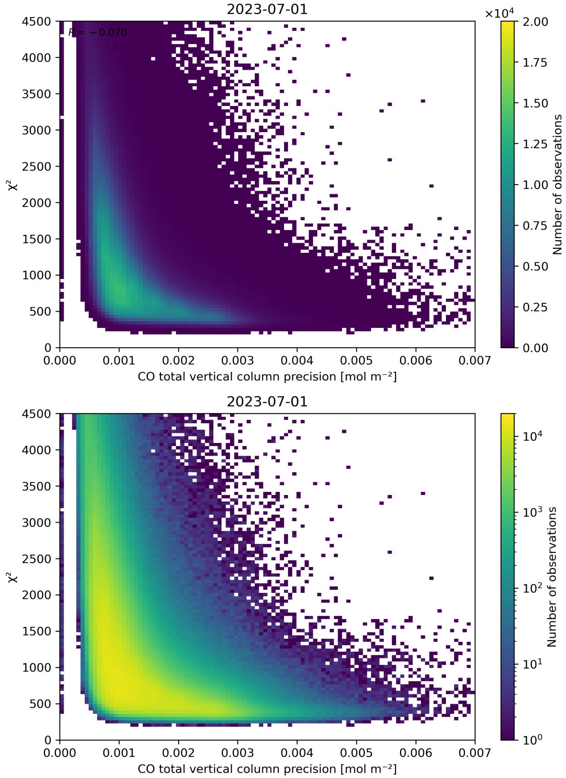
Figure 44: Scatter density plot of “CO total vertical column precision” against “ \chi^2 ” for 2023-06-30 to 2023-07-02.
