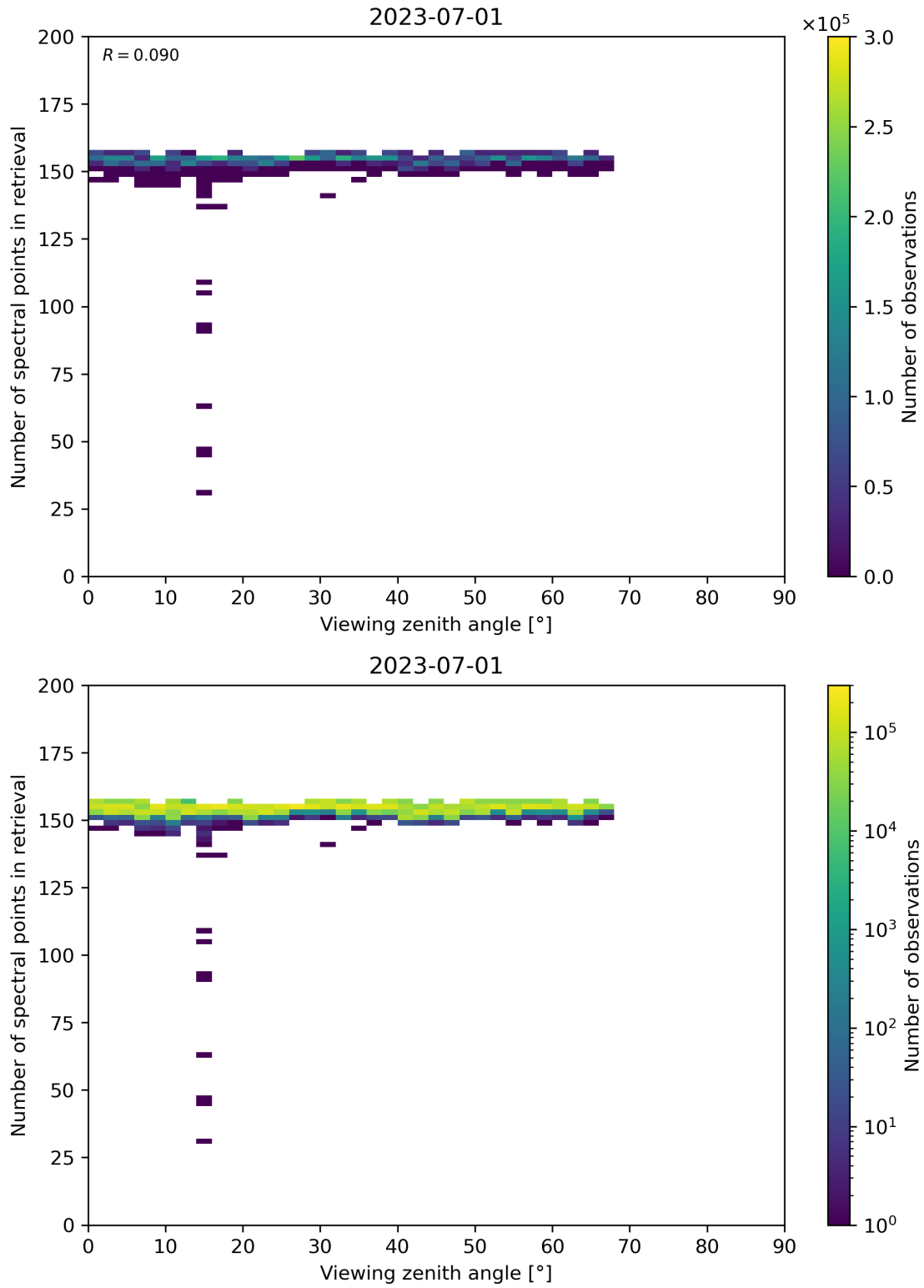
Figure 76: Scatter density plot of “Viewing zenith angle” against “Number of spectral points in retrieval” for 2023-06-30 to 2023-07-02.
