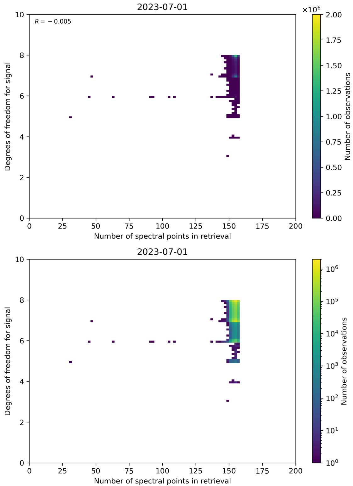
Figure 59: Scatter density plot of “Number of spectral points in retrieval” against “Degrees of freedom for signal” for 2023-06-30 to 2023-07-02.
