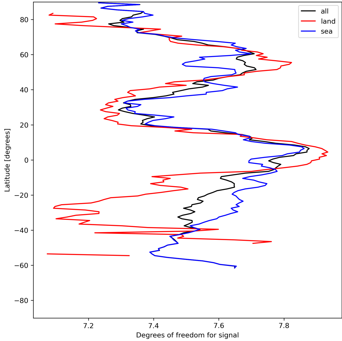
Figure 15: Zonal average of “Degrees of freedom for signal” for 2023-06-30 to 2023-07-02.
