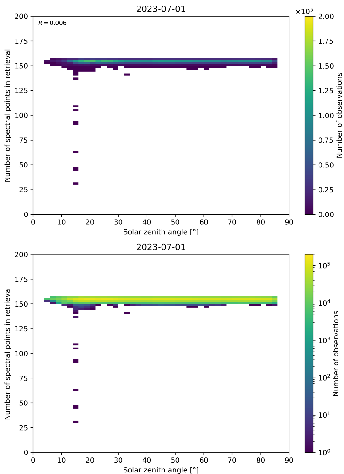
Figure 68: Scatter density plot of “Solar zenith angle” against “Number of spectral points in retrieval” for 2023-06-30 to 2023-07-02.
