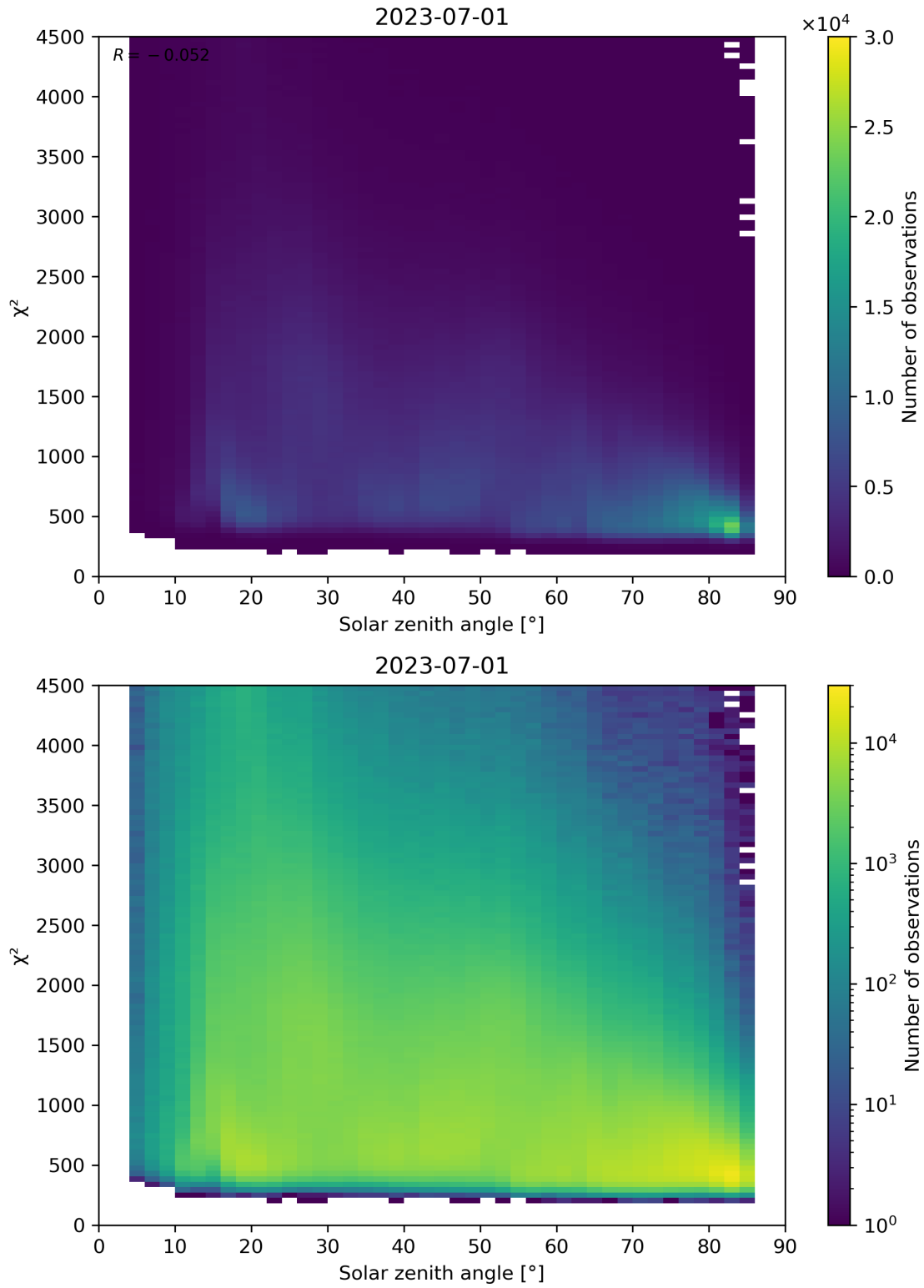
Figure 64: Scatter density plot of “Solar zenith angle” against “ \chi^2 ” for 2023-06-30 to 2023-07-02.
