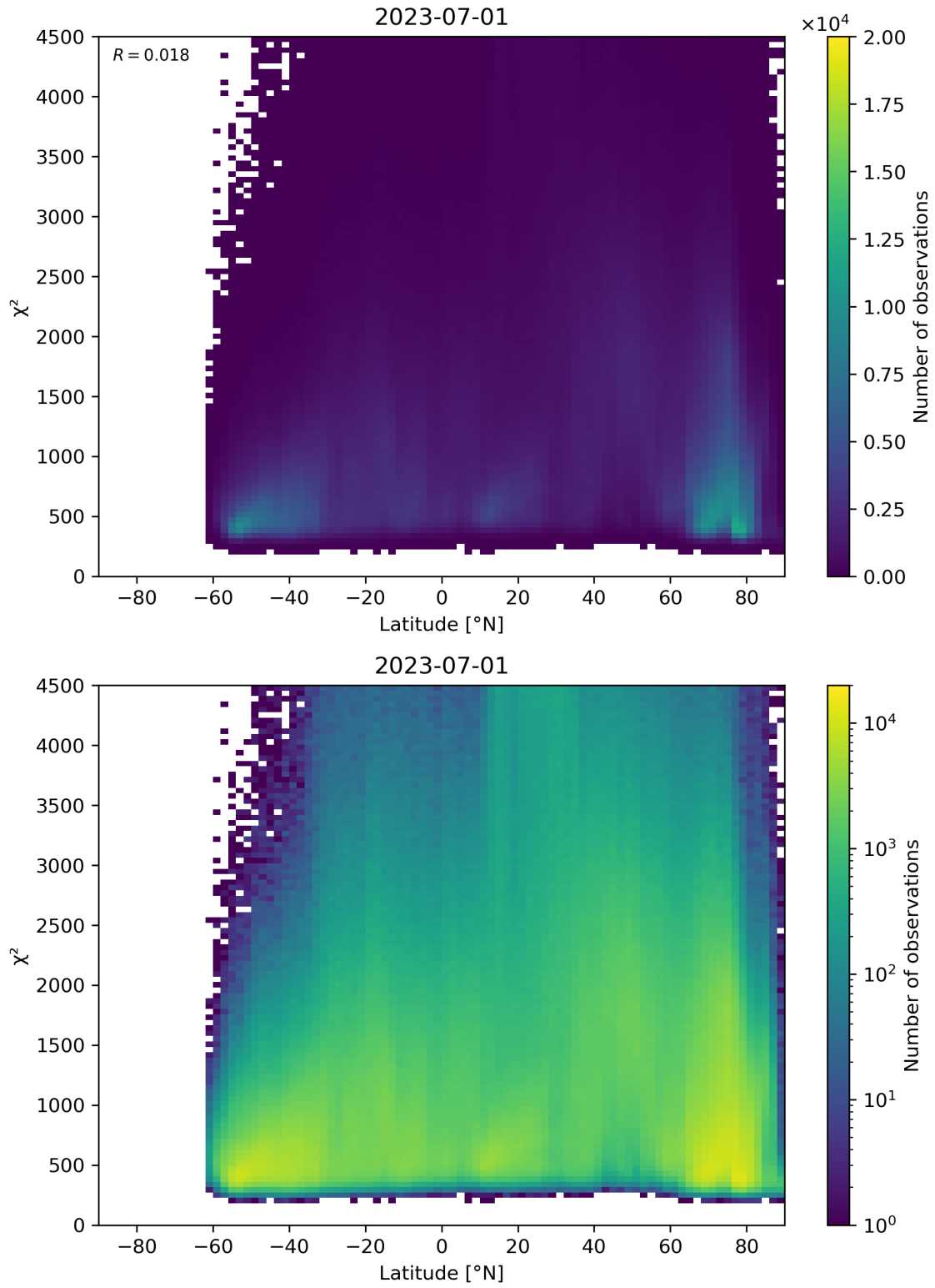
Figure 54: Scatter density plot of “Latitude” against “ \chi^2 ” for 2023-06-30 to 2023-07-02.
