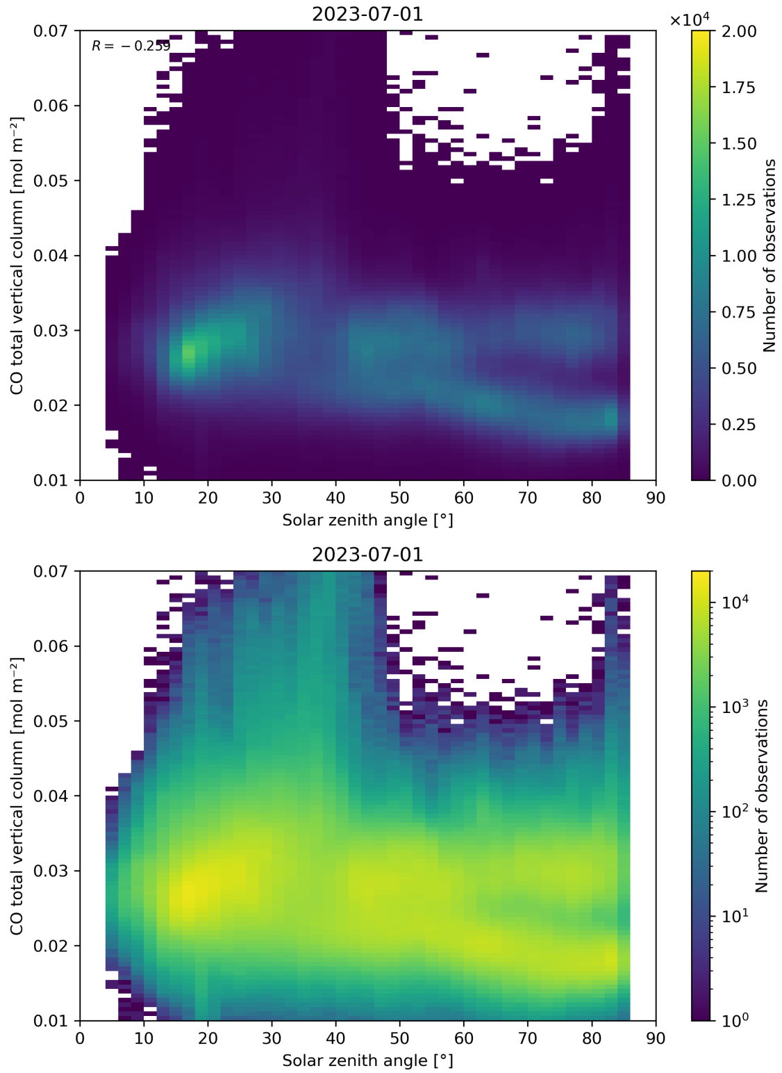
Figure 61: Scatter density plot of “Solar zenith angle” against “CO total vertical column” for 2023-06-30 to 2023-07-02.
