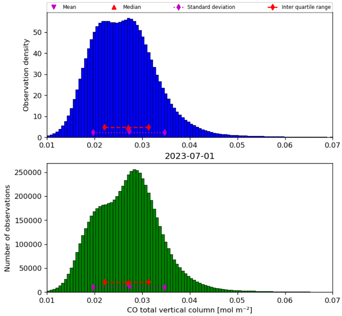
Figure 18: Histogram of “CO total vertical column” for 2023-06-30 to 2023-07-02
