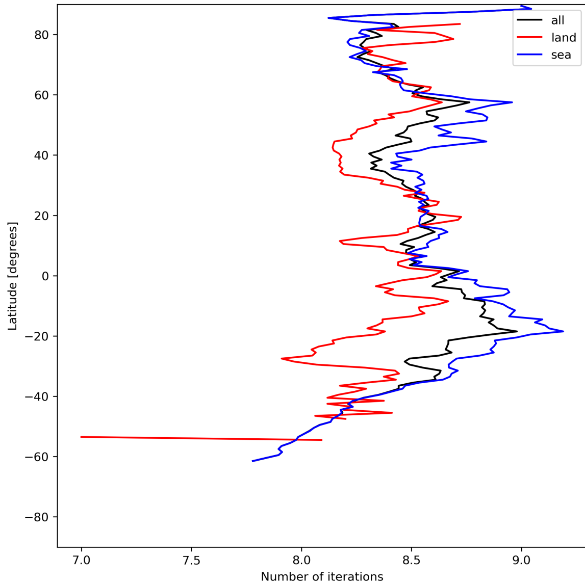
Figure 16: Zonal average of “Number of iterations” for 2023-06-30 to 2023-07-02.
