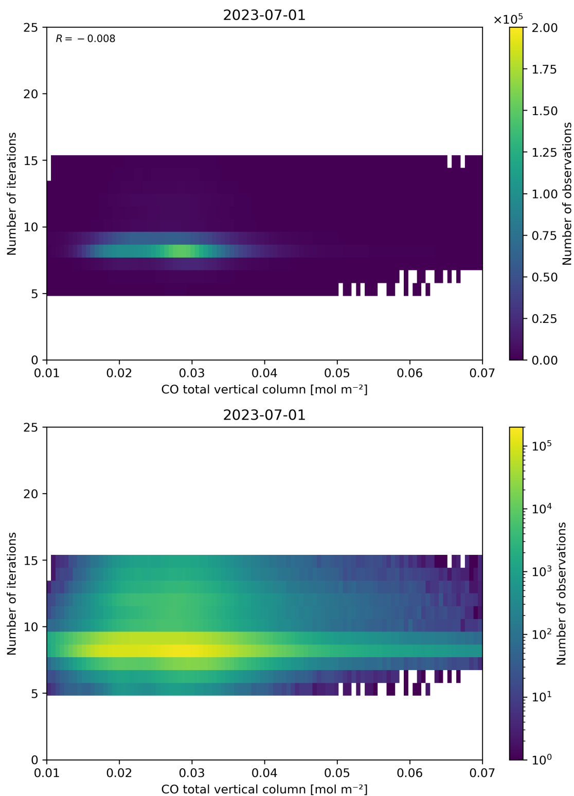
Figure 42: Scatter density plot of “CO total vertical column” against “Number of iterations” for 2023-06-30 to 2023-07-02.
