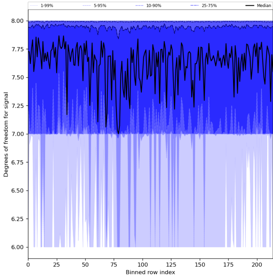
Figure 31: Along track statistics of “Degrees of freedom for signal” for 2023-06-30 to 2023-07-02
