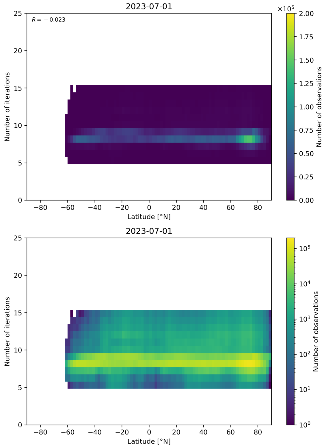
Figure 56: Scatter density plot of “Latitude” against “Number of iterations” for 2023-06-30 to 2023-07-02.
