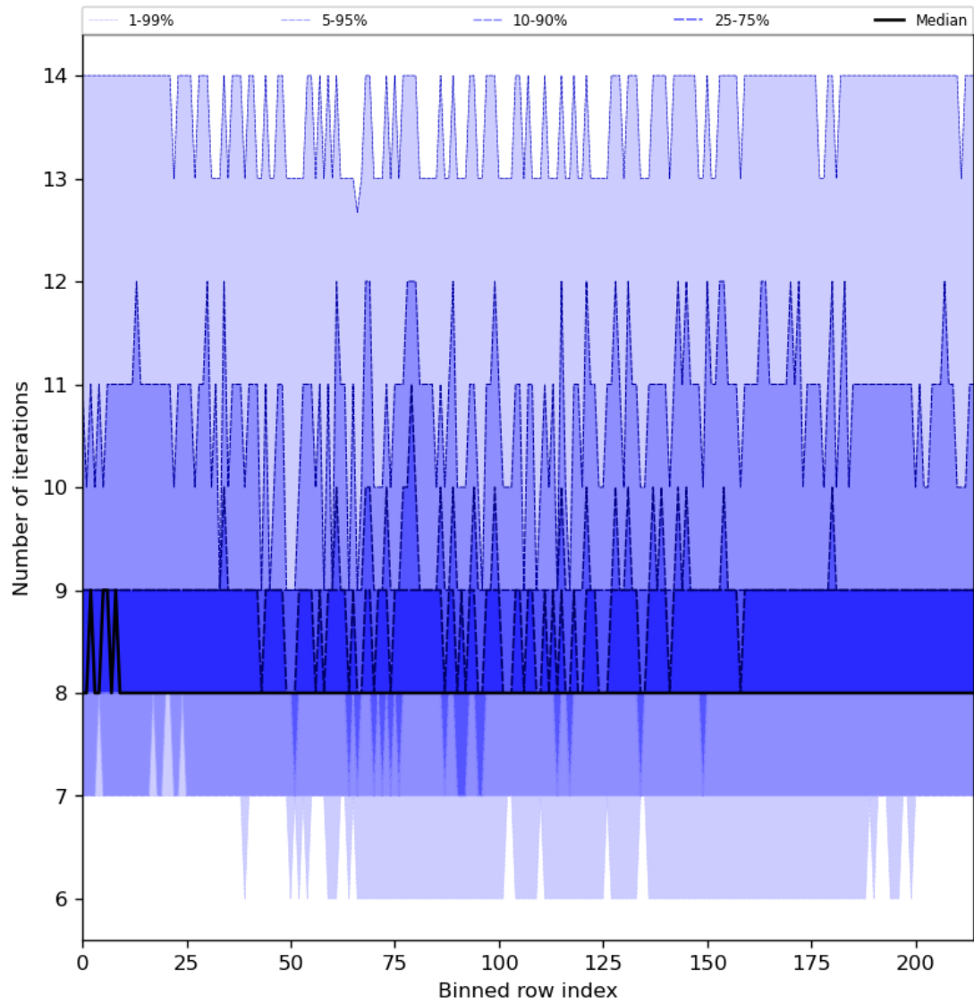
Figure 32: Along track statistics of “Number of iterations” for 2023-06-30 to 2023-07-02
