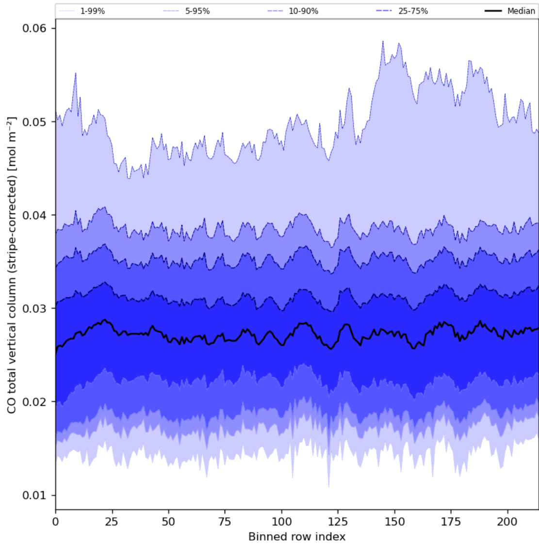
Figure 27: Along track statistics of "CO total vertical column (stripe-corrected)" for 2023-06-30 to 2023-07-02
