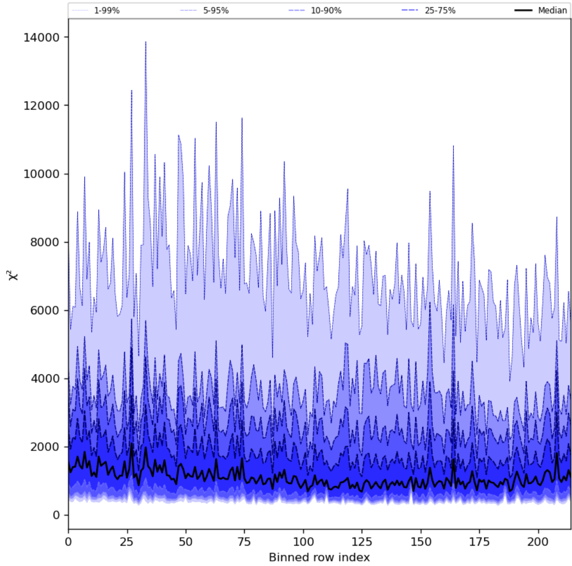
Figure 30: Along track statistics of “ \chi^2 ” for 2023-06-30 to 2023-07-02
