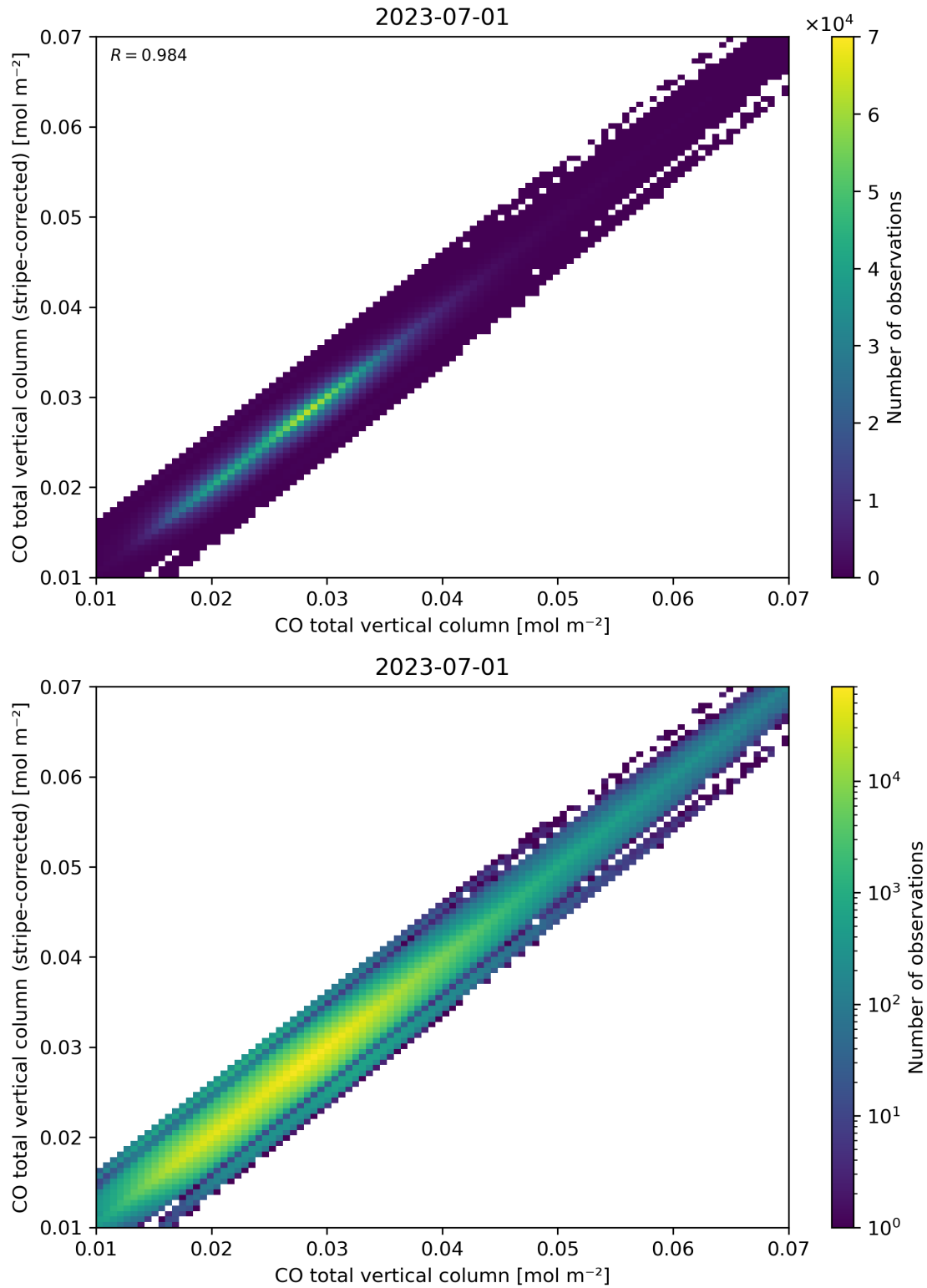
Figure 33: Scatter density plot of “CO total vertical column” against “CO total vertical column (stripe-corrected)” for 2023-06-30 to 2023-07-02.
