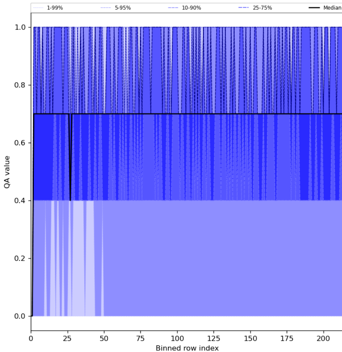
Figure 25: Along track statistics of “QA value” for 2023-06-30 to 2023-07-02
