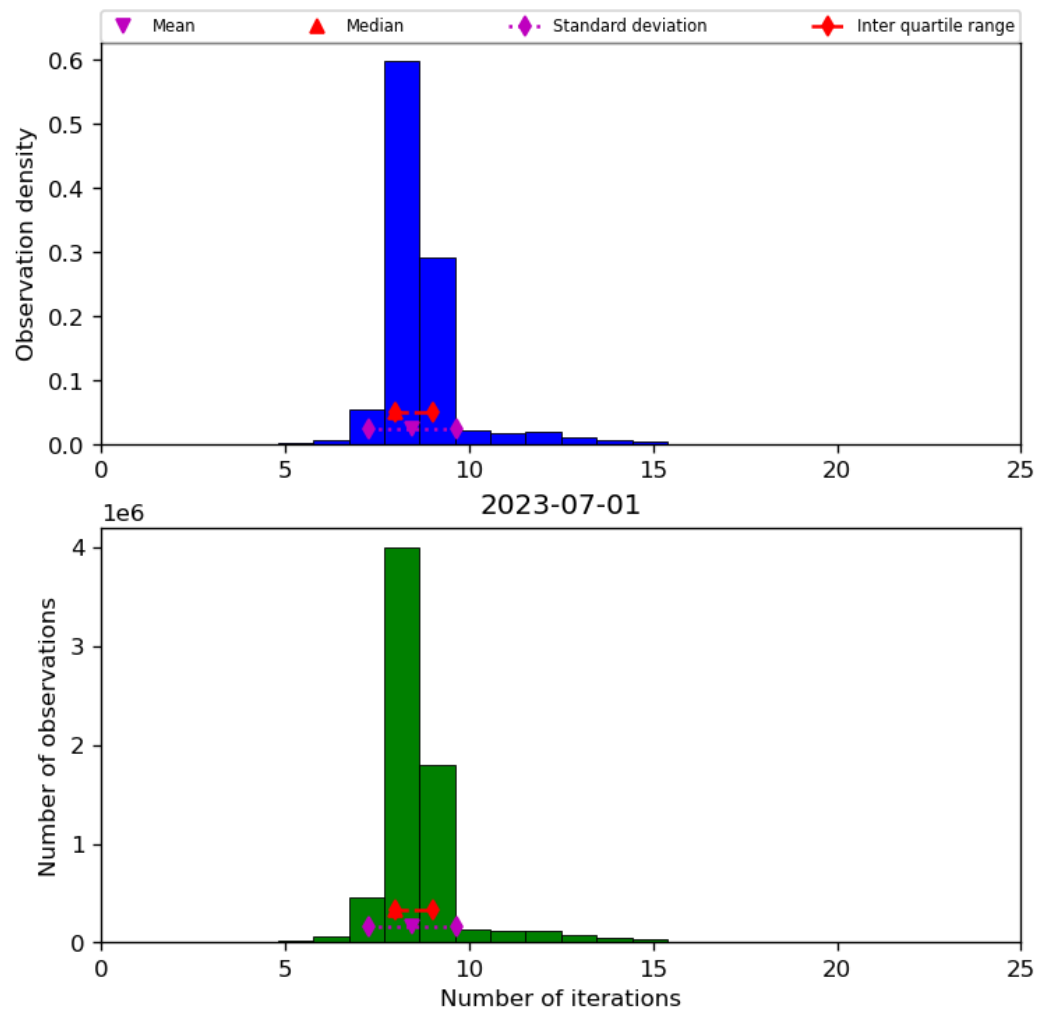
Figure 24: Histogram of “Number of iterations” for 2023-06-30 to 2023-07-02
