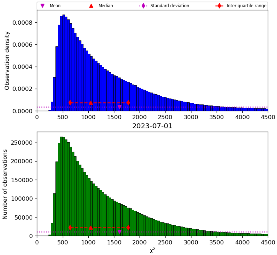
Figure 22: Histogram of “ \chi^2 ” for 2023-06-30 to 2023-07-02
