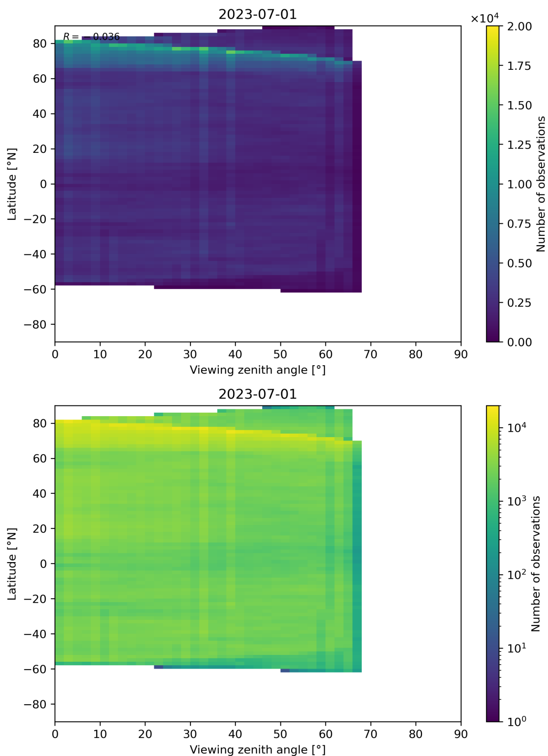
Figure 74: Scatter density plot of “Viewing zenith angle” against “Latitude” for 2023-06-30 to 2023-07-02.
