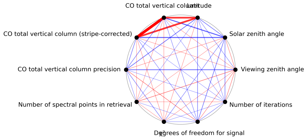
Figure 1: Map of correlation graph for 2023-06-30 to 2023-07-02.
