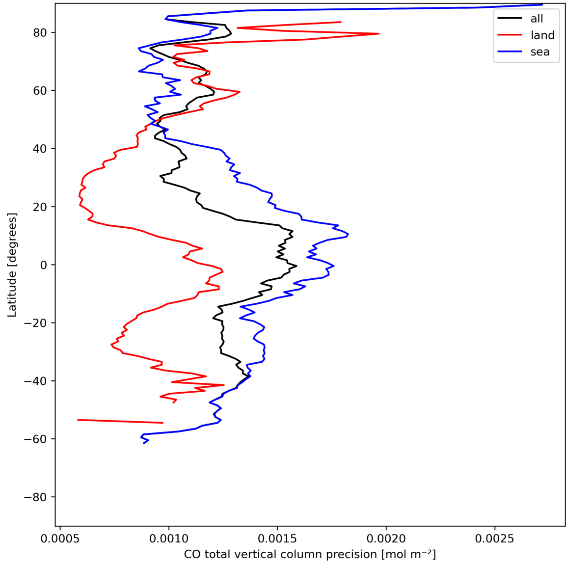
Figure 12: Zonal average of “CO total vertical column precision” for 2023-06-30 to 2023-07-02.
