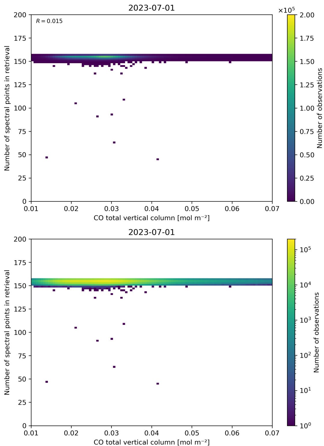
Figure 43: Scatter density plot of “CO total vertical column” against “Number of spectral points in retrieval” for 2023-06-30 to 2023-07-02.
