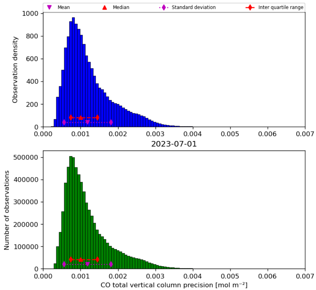
Figure 20: Histogram of “CO total vertical column precision” for 2023-06-30 to 2023-07-02
