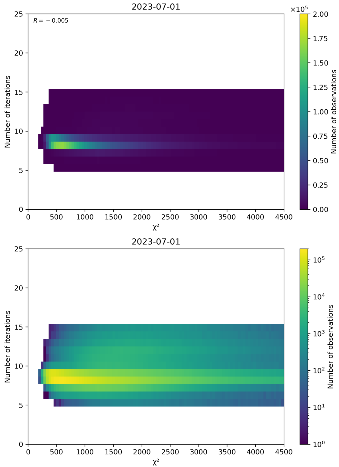
Figure 49: Scatter density plot of “ \chi^2 ” against “Number of iterations” for 2023-06-30 to 2023-07-02.
