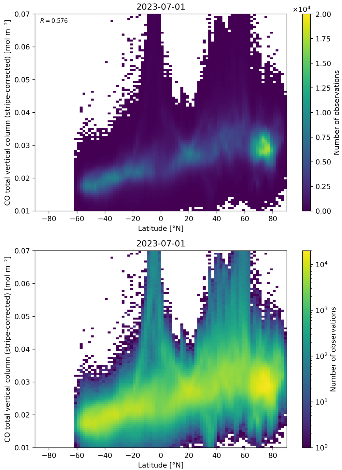
Figure 52: Scatter density plot of “Latitude” against “CO total vertical column (stripe-corrected)” for 2023-06-30 to 2023-07-02.
