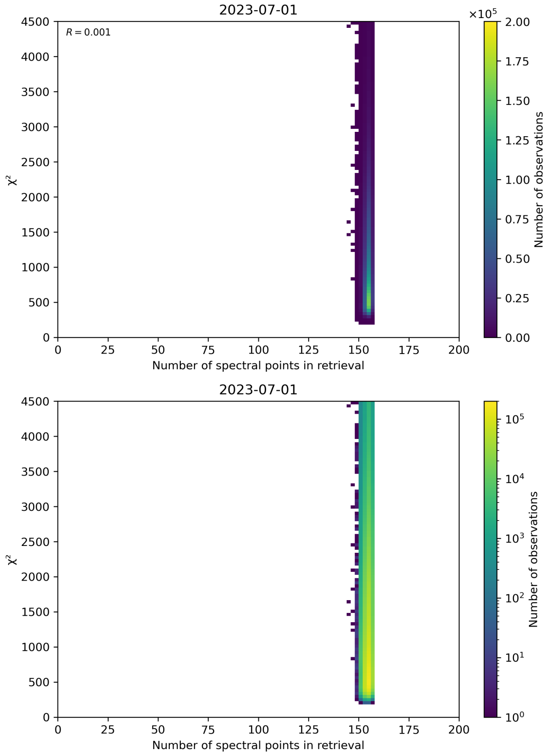
Figure 58: Scatter density plot of “Number of spectral points in retrieval” against “ \chi^2 ” for 2023-06-30 to 2023-07-02.
