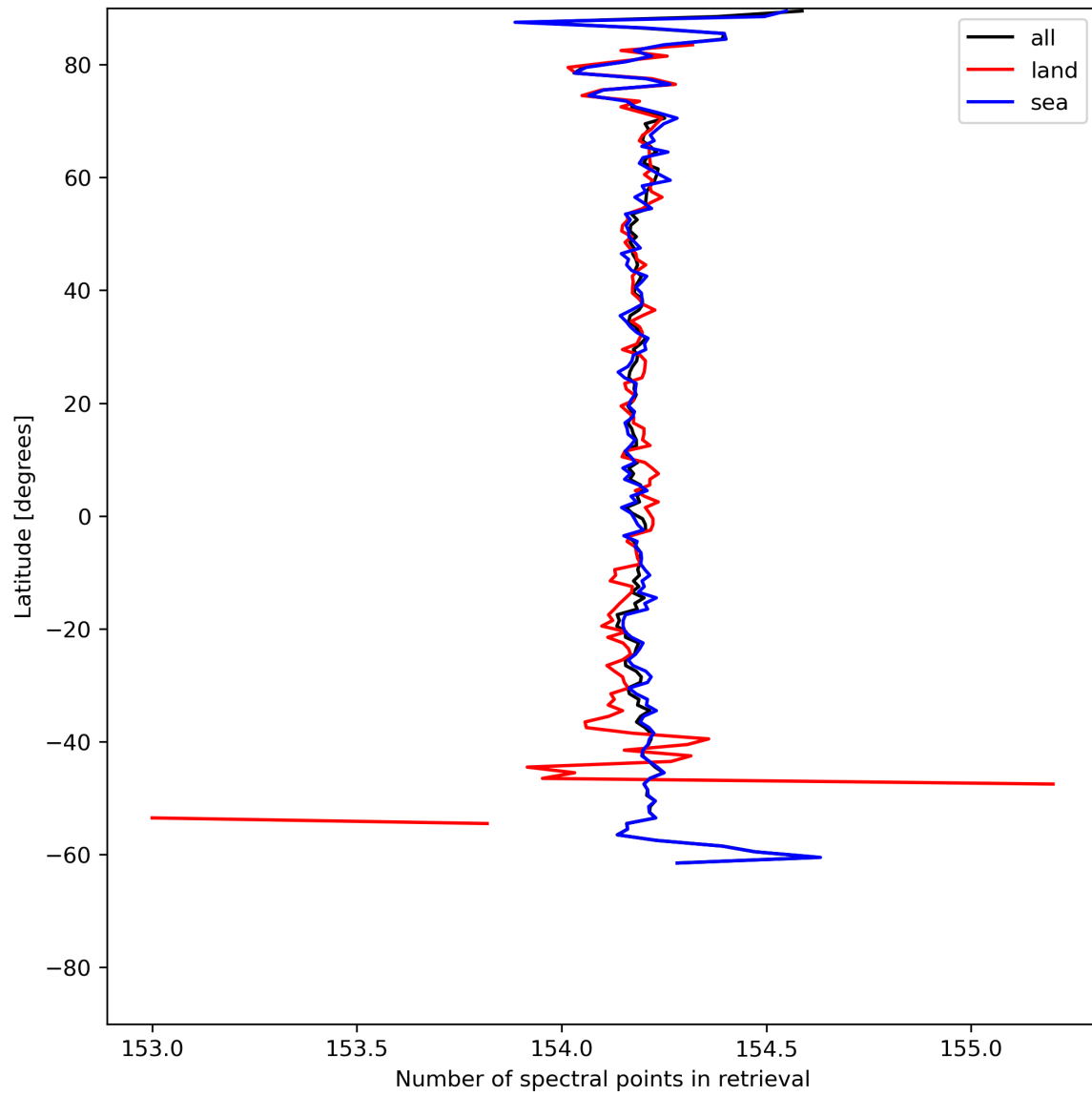
Figure 13: Zonal average of “Number of spectral points in retrieval” for 2023-06-30 to 2023-07-02.
