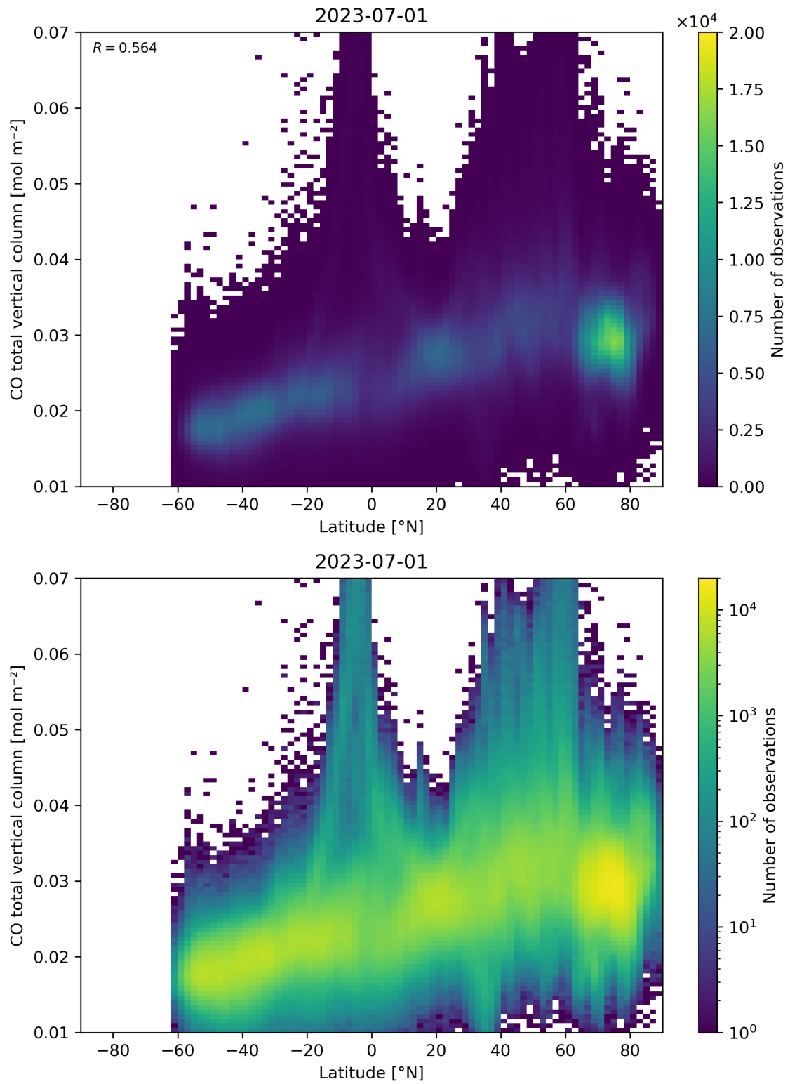
Figure 51: Scatter density plot of “Latitude” against “CO total vertical column” for 2023-06-30 to 2023-07-02.
