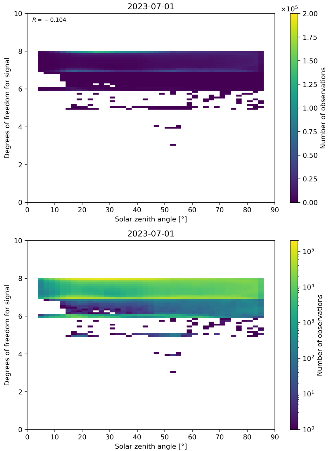
Figure 65: Scatter density plot of “Solar zenith angle” against “Degrees of freedom for signal” for 2023-06-30 to 2023-07-02.
