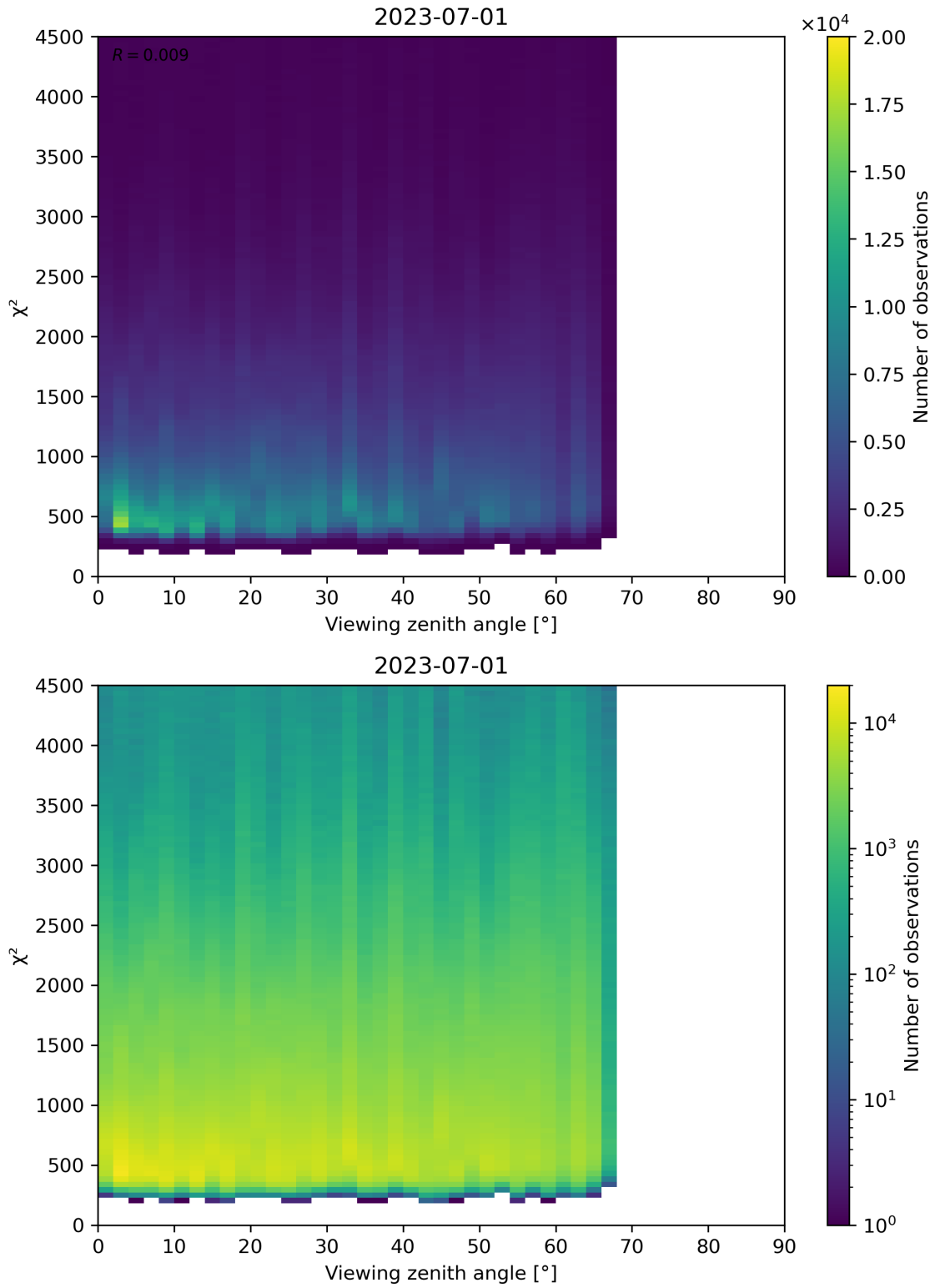
Figure 72: Scatter density plot of “Viewing zenith angle” against “ \chi^2 ” for 2023-06-30 to 2023-07-02.
