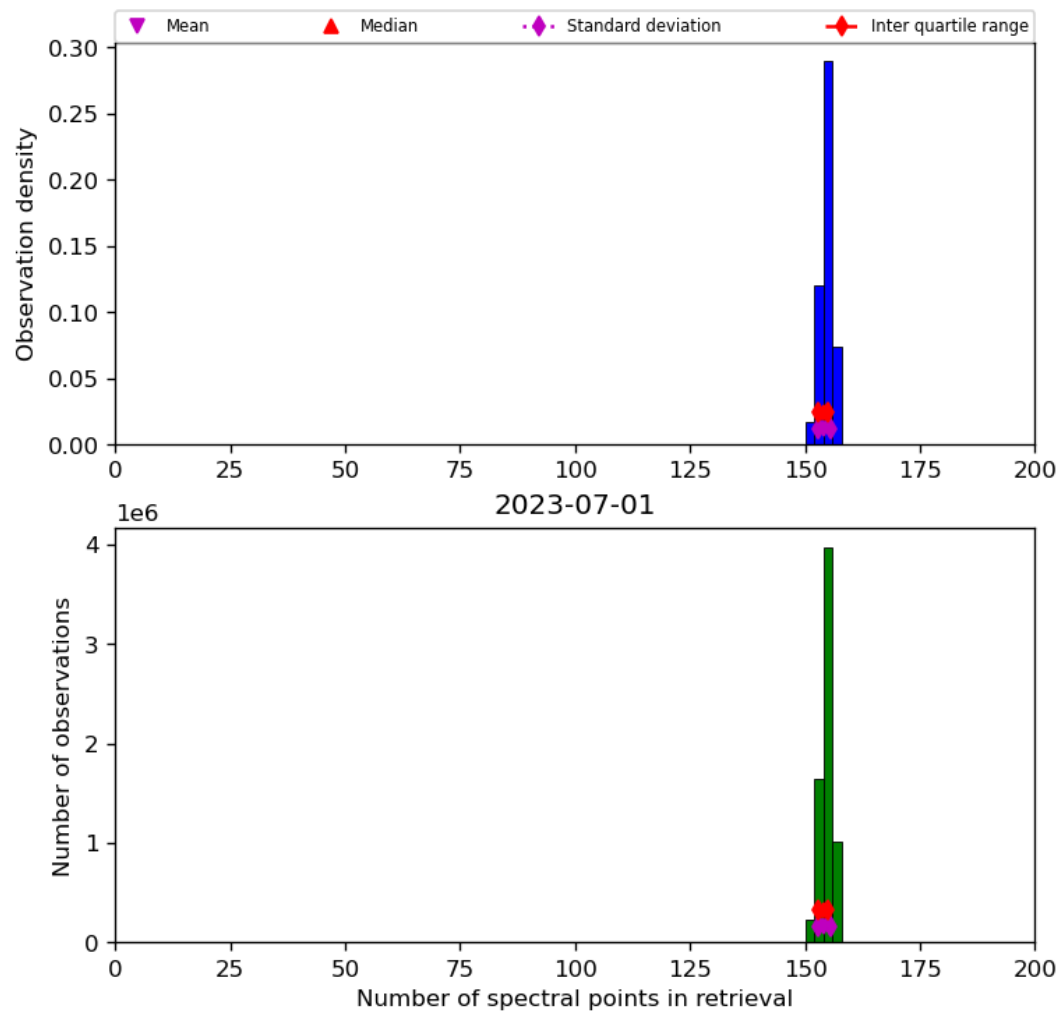
Figure 21: Histogram of “Number of spectral points in retrieval” for 2023-06-30 to 2023-07-02
