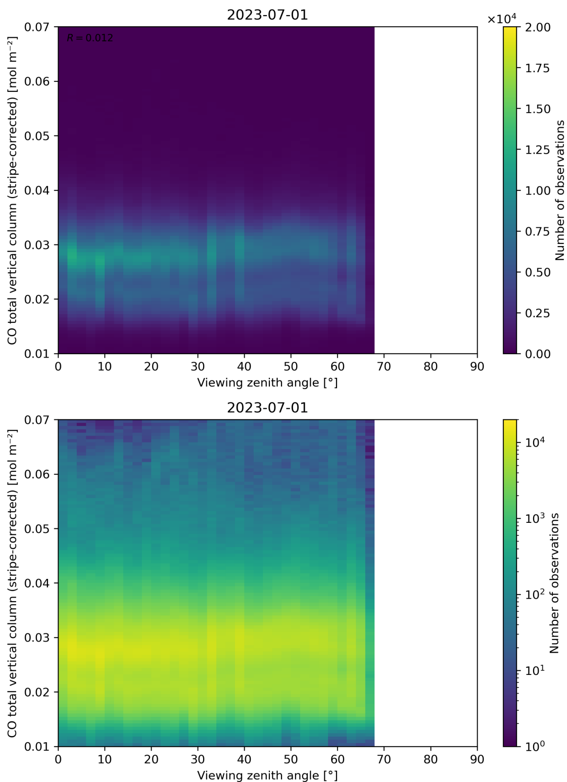
Figure 70: Scatter density plot of “Viewing zenith angle” against “CO total vertical column (stripe-corrected)” for 2023-06-30 to 2023-07-02.
