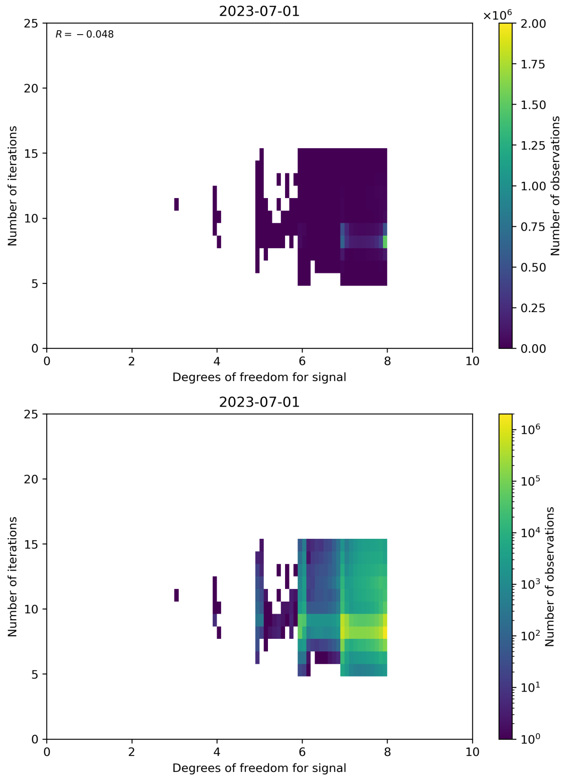
Figure 50: Scatter density plot of “Degrees of freedom for signal” against “Number of iterations” for 2023-06-30 to 2023-07-02.
