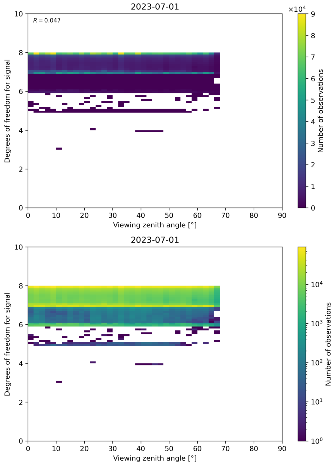
Figure 73: Scatter density plot of “Viewing zenith angle” against “Degrees of freedom for signal” for 2023-06-30 to 2023-07-02.
