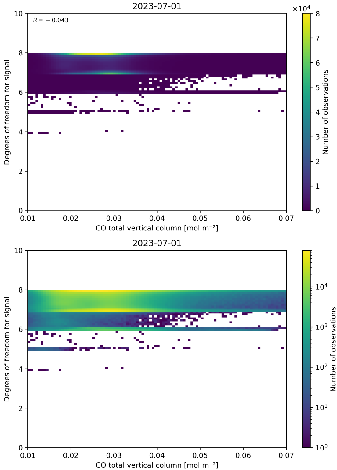
Figure 41: Scatter density plot of “CO total vertical column” against “Degrees of freedom for signal” for 2023-06-30 to 2023-07-02.
