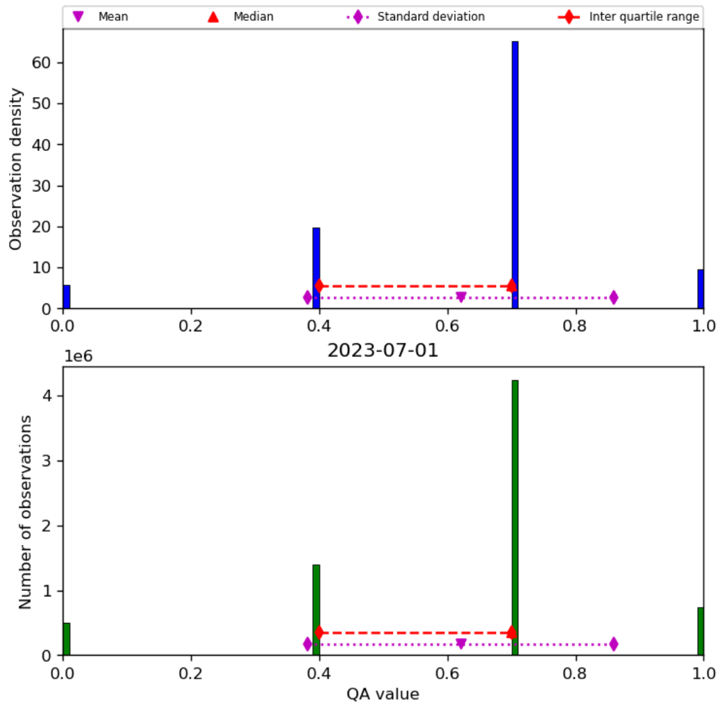
Figure 17: Histogram of “QA value” for 2023-06-30 to 2023-07-02
