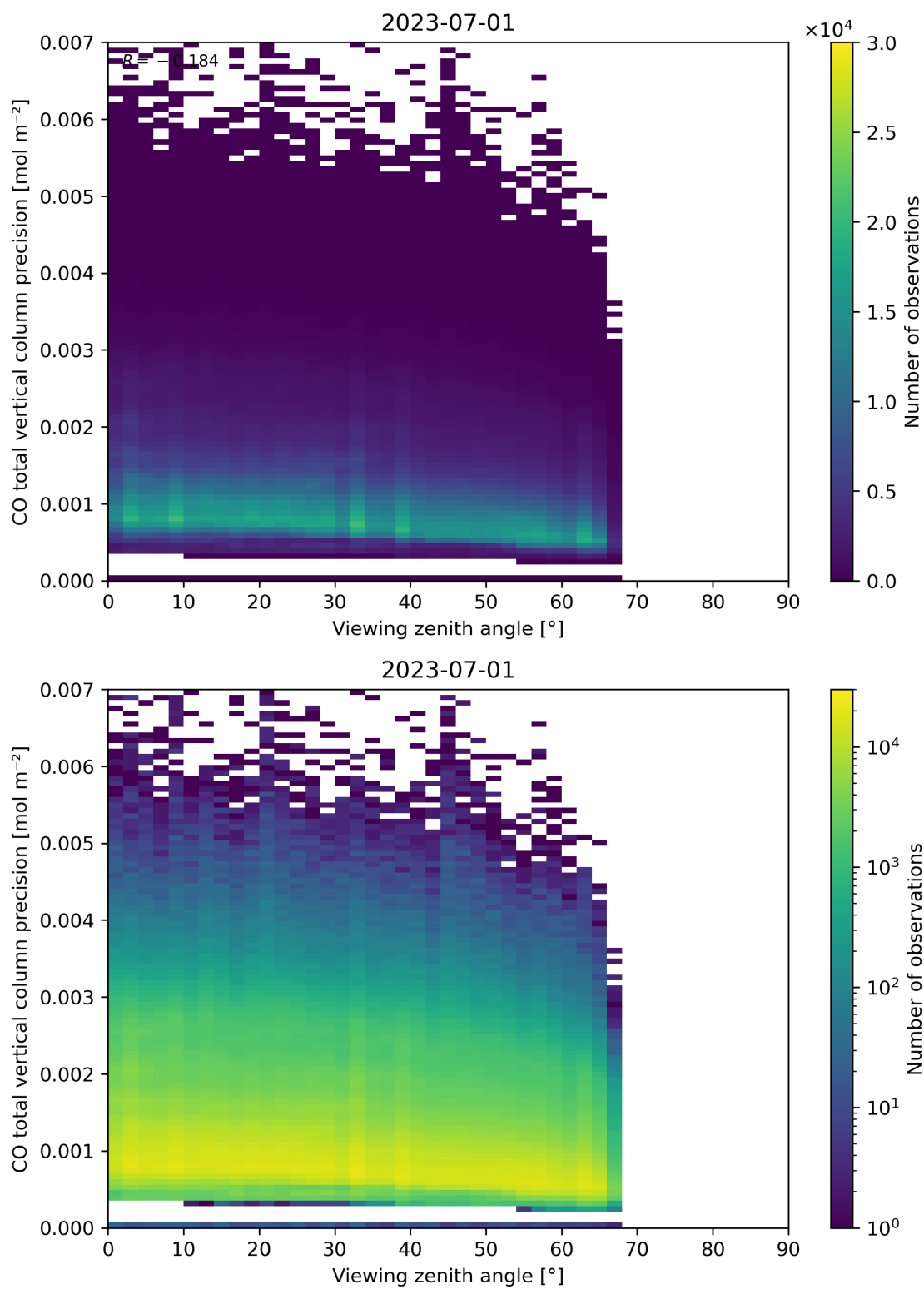
Figure 71: Scatter density plot of “Viewing zenith angle” against “CO total vertical column precision” for 2023-06-30 to 2023-07-02.
