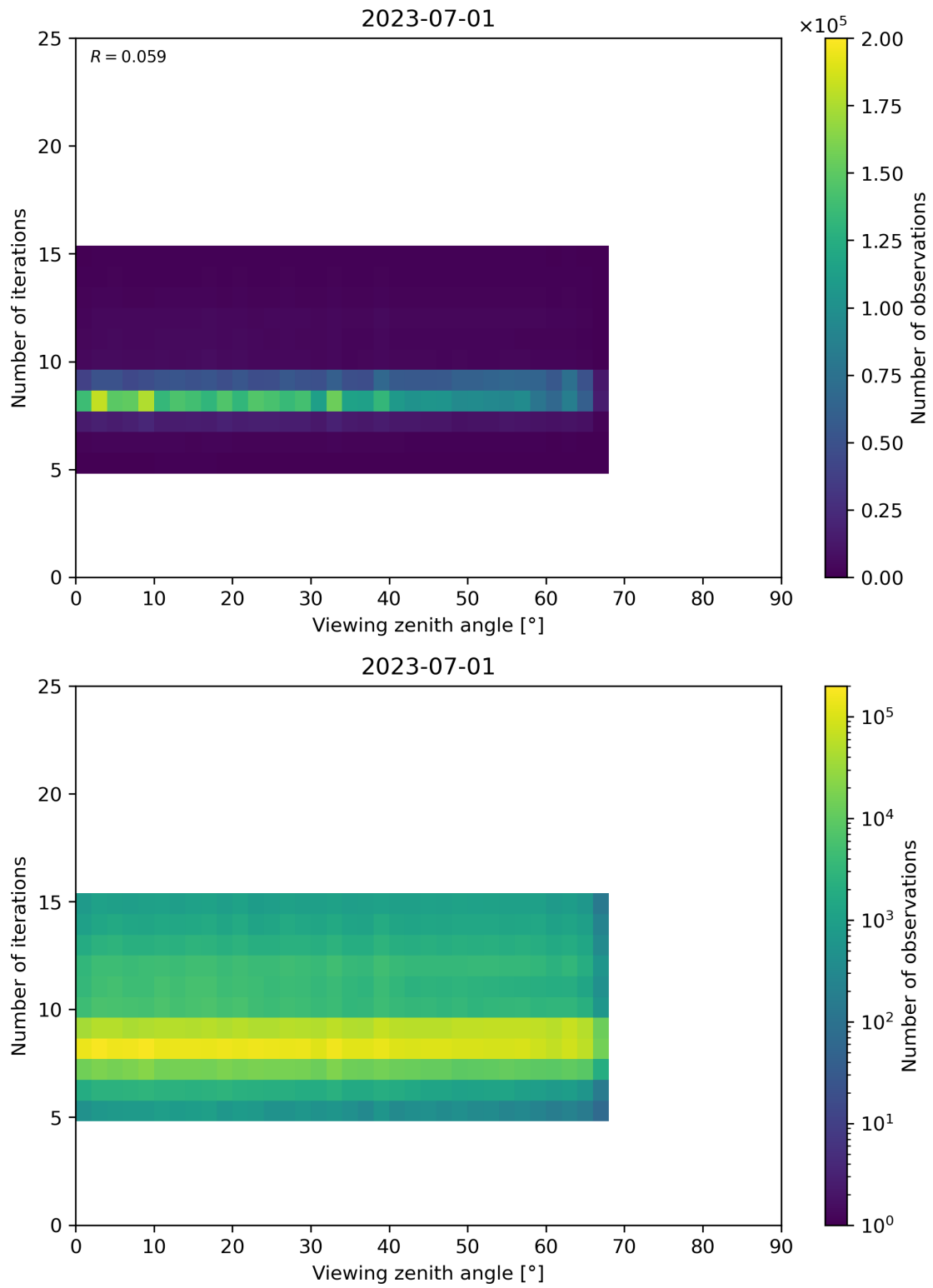
Figure 75: Scatter density plot of “Viewing zenith angle” against “Number of iterations” for 2023-06-30 to 2023-07-02.
