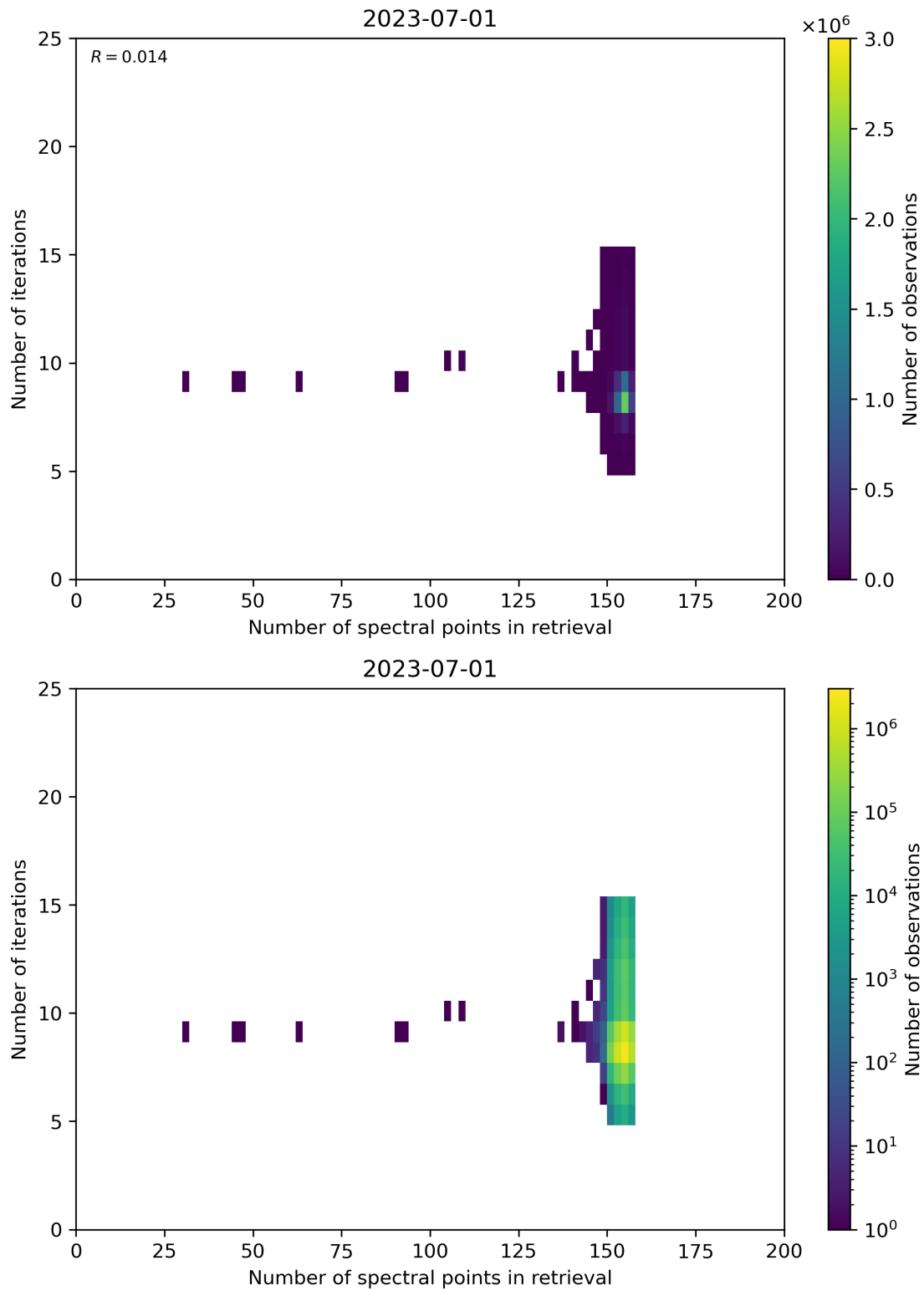
Figure 60: Scatter density plot of “Number of spectral points in retrieval” against “Number of iterations” for 2023-06-30 to 2023-07-02.
