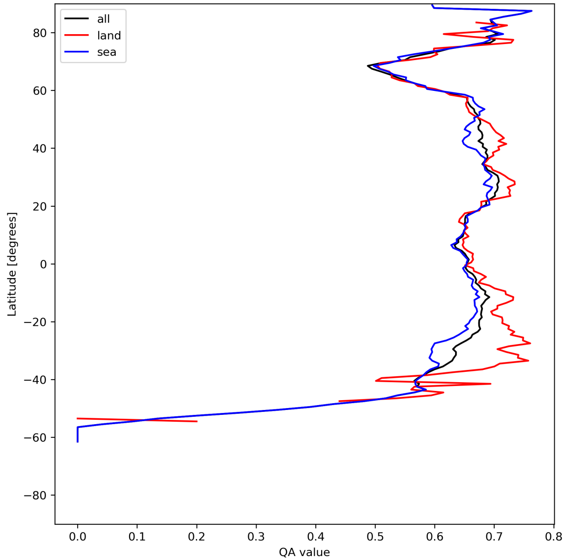
Figure 9: Zonal average of “QA value” for 2023-06-30 to 2023-07-02.
