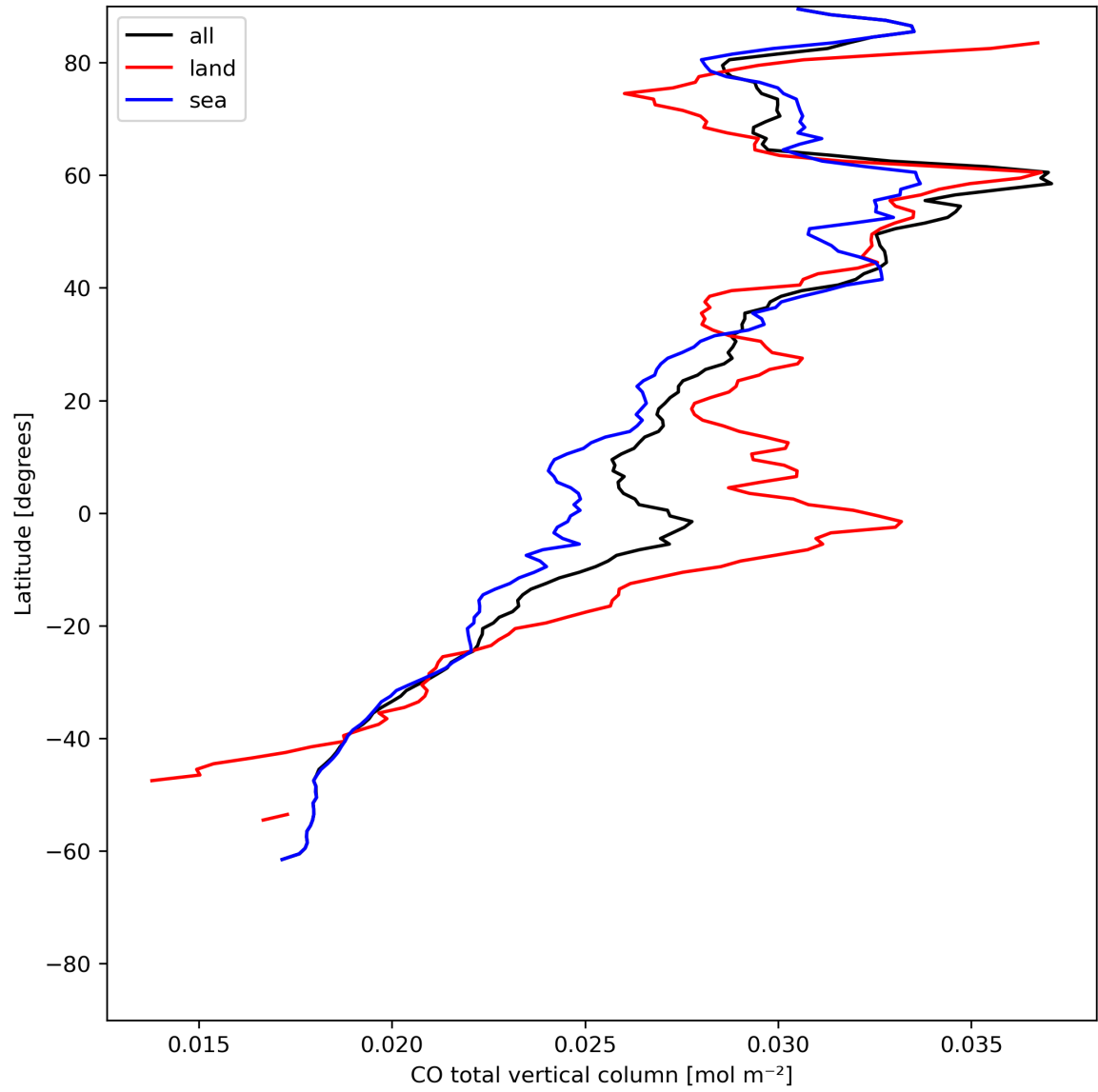
Figure 10: Zonal average of “CO total vertical column” for 2023-06-30 to 2023-07-02.
