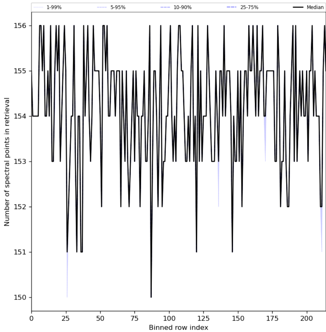
Figure 29: Along track statistics of “Number of spectral points in retrieval” for 2023-06-30 to 2023-07-02
