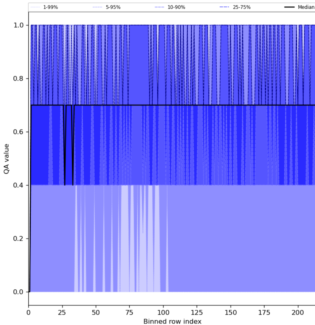
Figure 25: Along track statistics of “QA value” for 2023-07-01 to 2023-07-03
