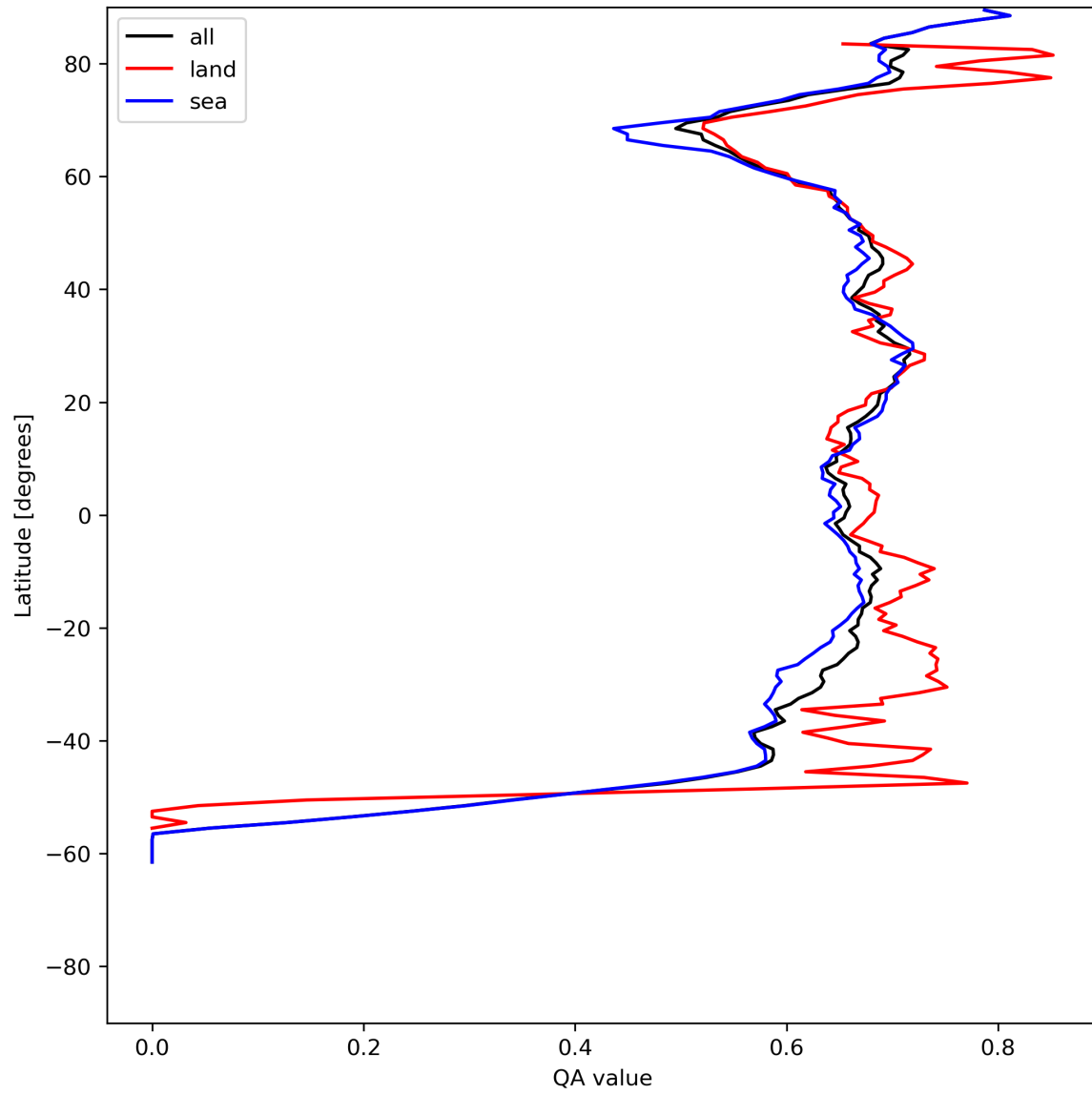
Figure 9: Zonal average of “QA value” for 2023-07-01 to 2023-07-03.
