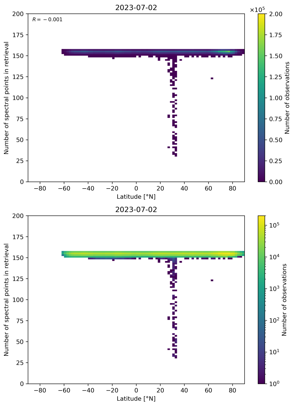
Figure 57: Scatter density plot of “Latitude” against “Number of spectral points in retrieval” for 2023-07-01 to 2023-07-03.
