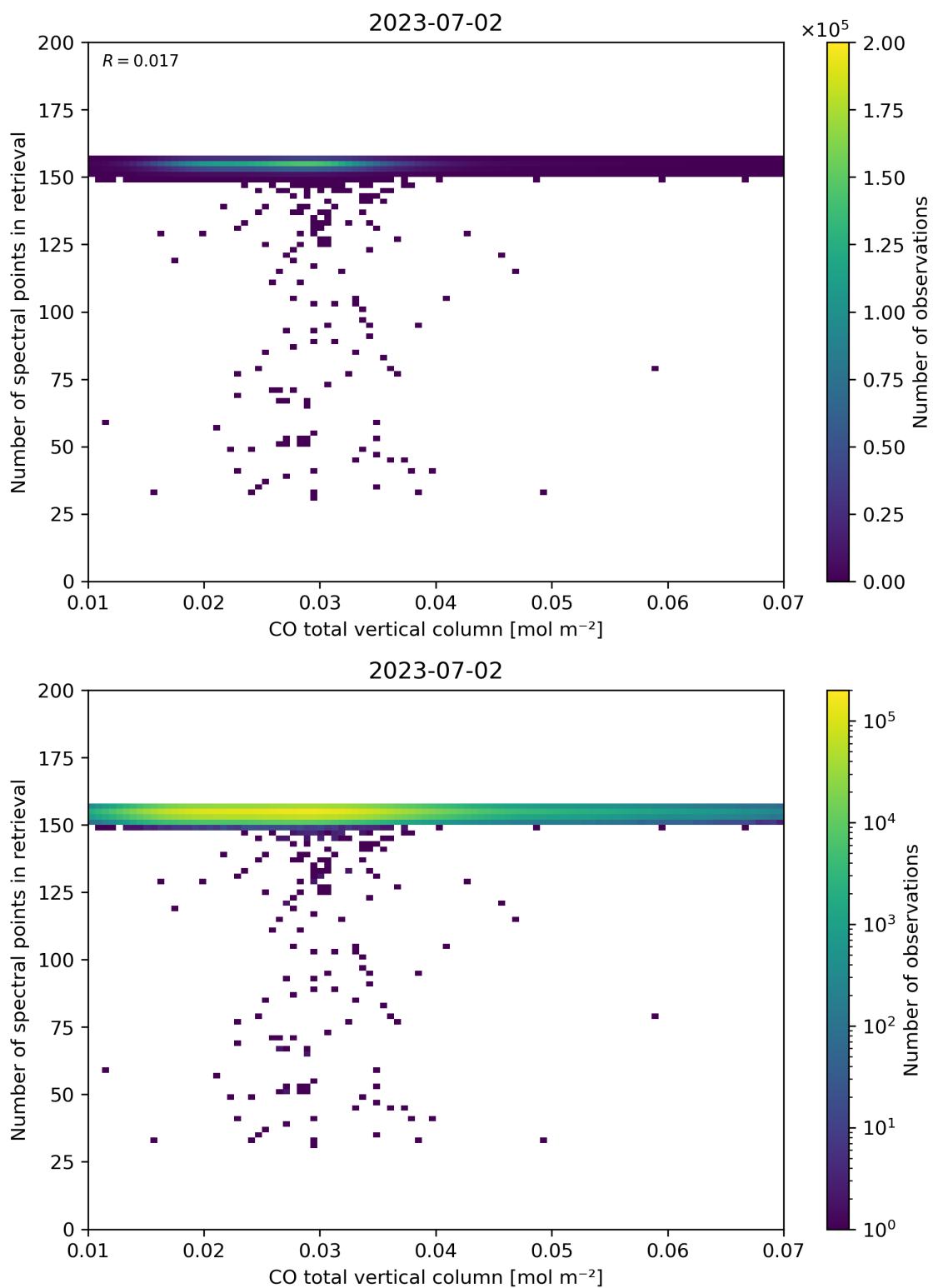
Figure 43: Scatter density plot of “CO total vertical column” against “Number of spectral points in retrieval” for 2023-07-01 to 2023-07-03.
