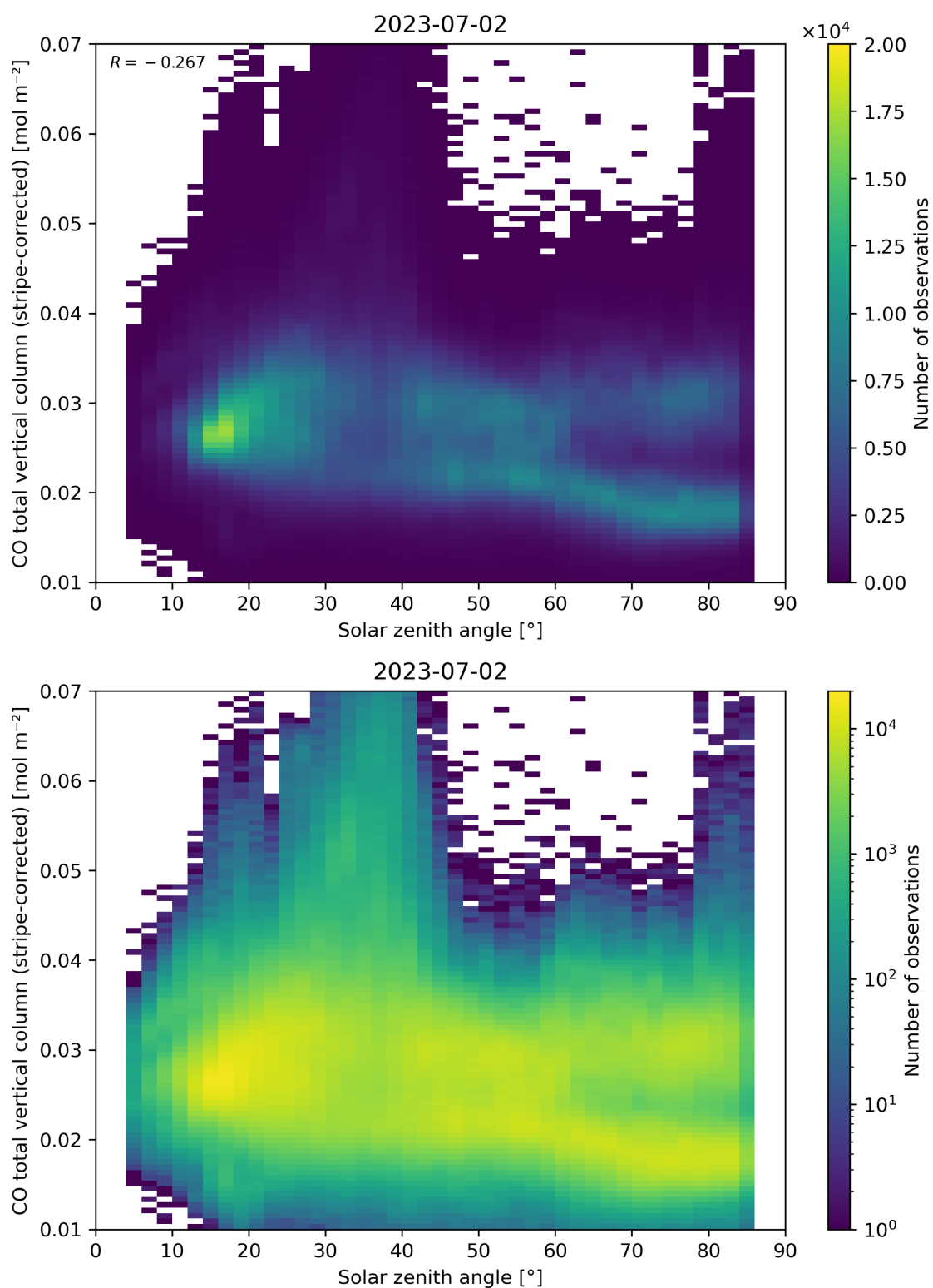
Figure 62: Scatter density plot of “Solar zenith angle” against “CO total vertical column (stripe-corrected)” for 2023-07-01 to 2023-07-03.
