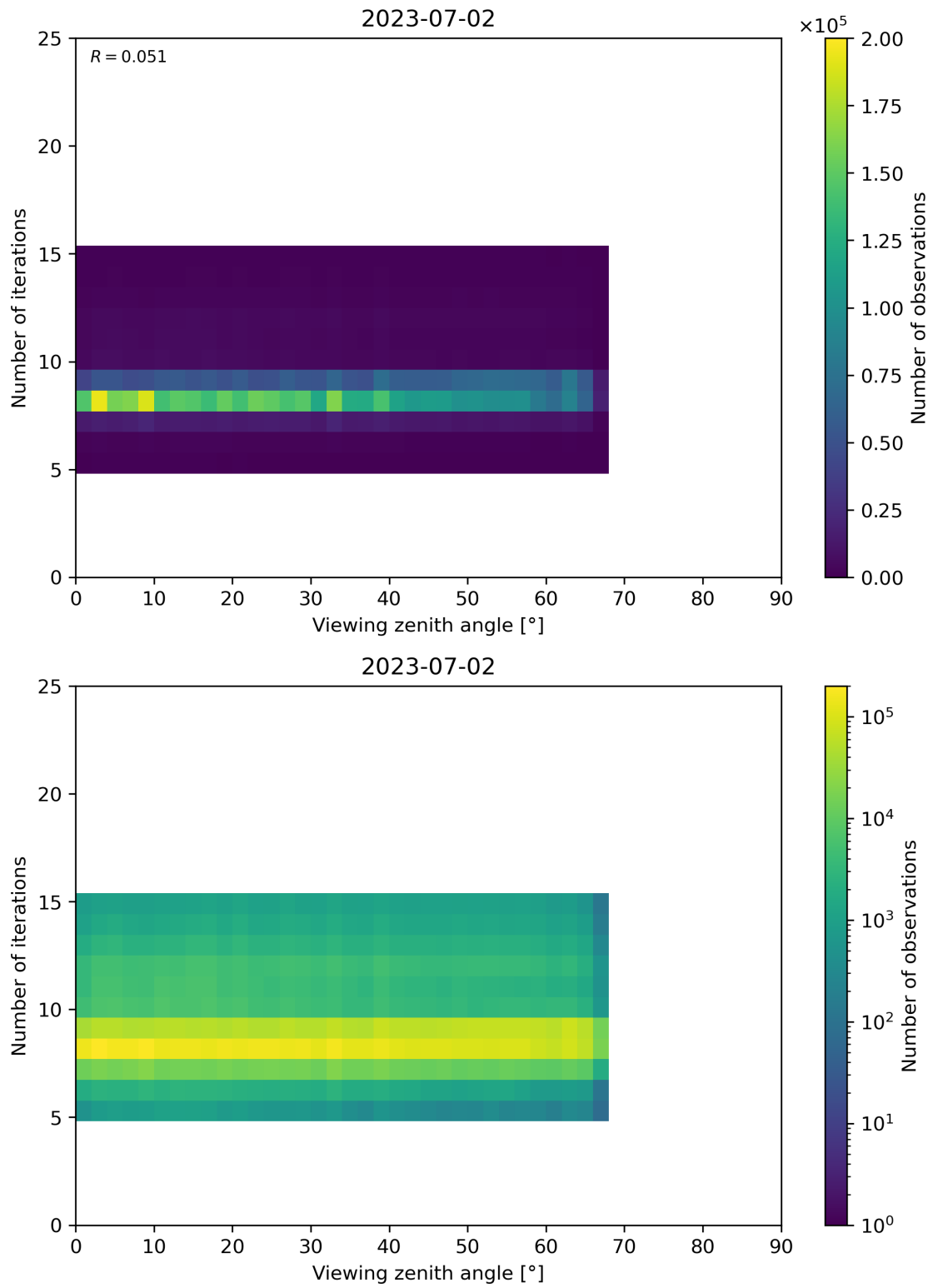
Figure 75: Scatter density plot of “Viewing zenith angle” against “Number of iterations” for 2023-07-01 to 2023-07-03.
