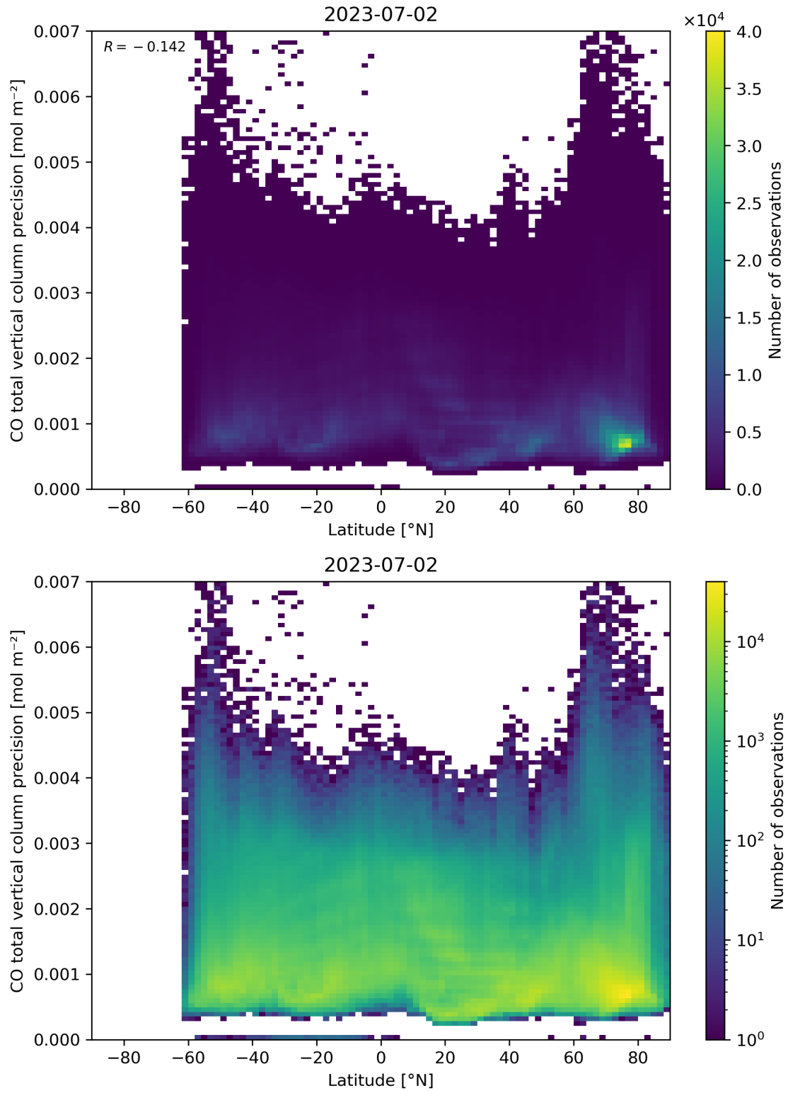
Figure 53: Scatter density plot of “Latitude” against “CO total vertical column precision” for 2023-07-01 to 2023-07-03.
