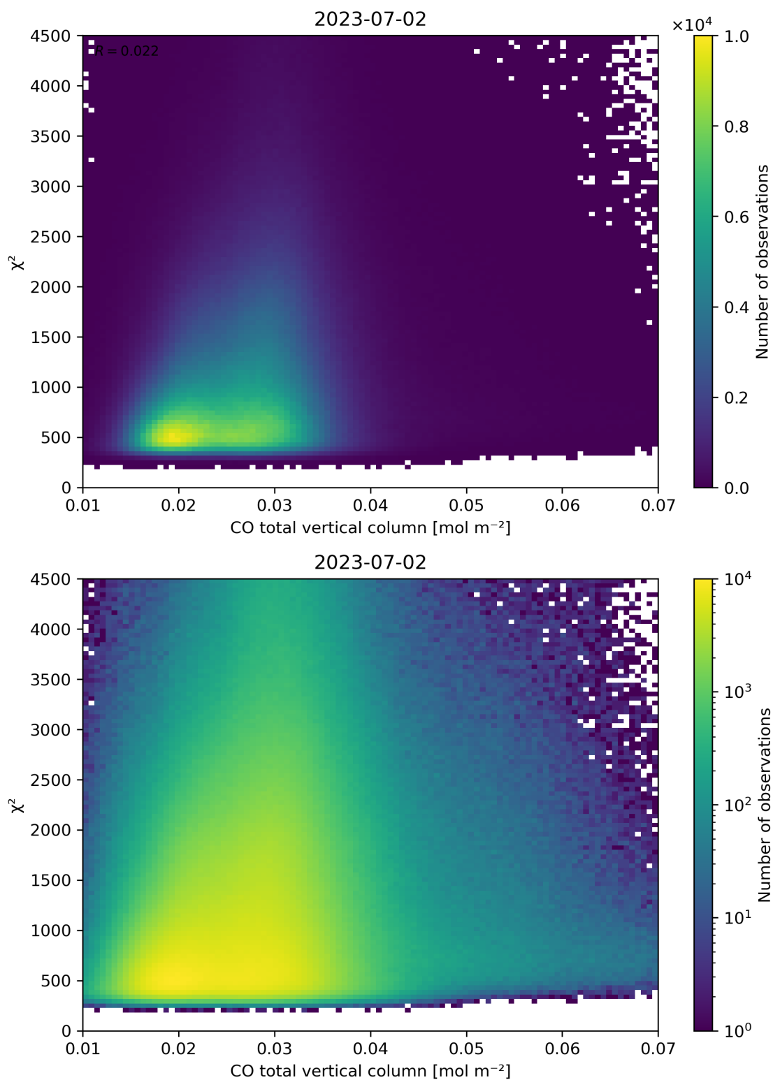
Figure 35: Scatter density plot of “CO total vertical column” against “ \chi^2 ” for 2023-07-01 to 2023-07-03.
