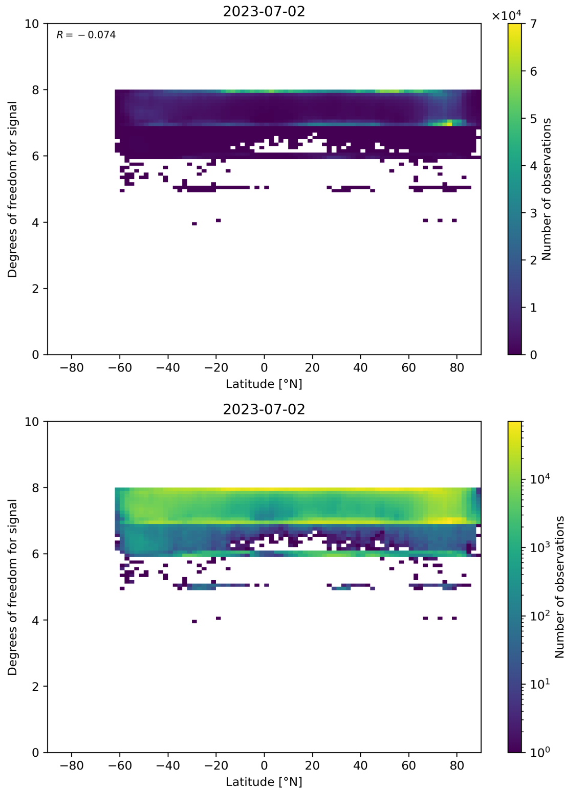
Figure 55: Scatter density plot of “Latitude” against “Degrees of freedom for signal” for 2023-07-01 to 2023-07-03.
