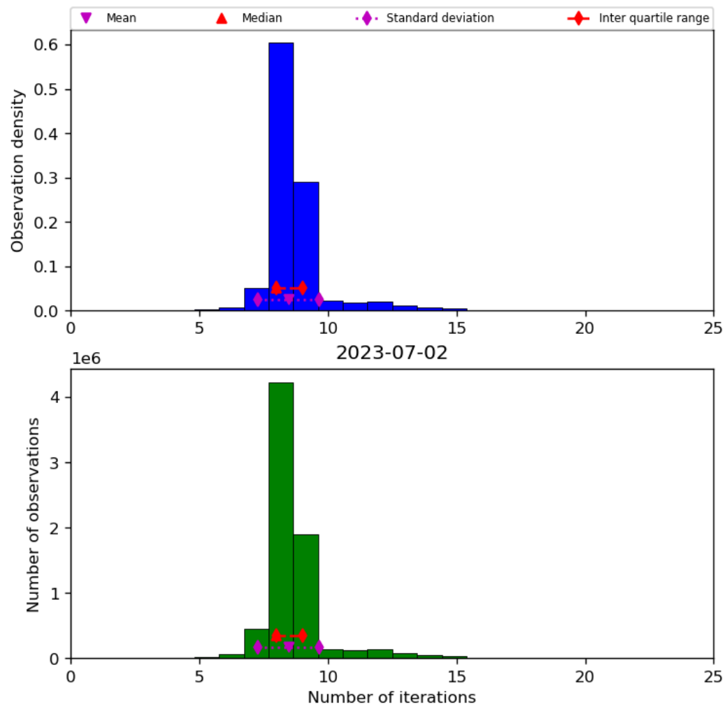
Figure 24: Histogram of “Number of iterations” for 2023-07-01 to 2023-07-03
