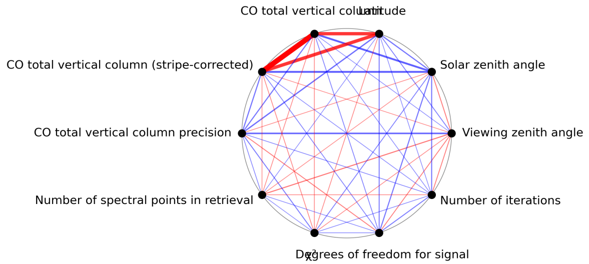
Figure 1: Map of correlation graph for 2023-07-01 to 2023-07-03.
