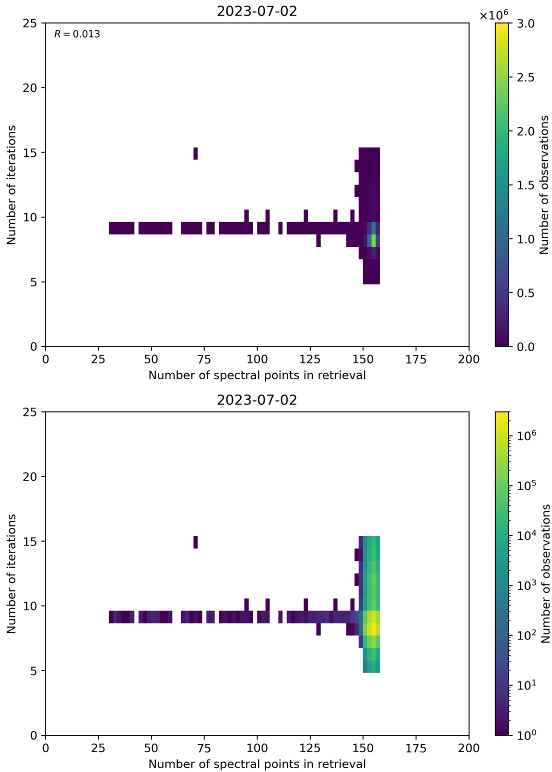
Figure 60: Scatter density plot of “Number of spectral points in retrieval” against “Number of iterations” for 2023-07-01 to 2023-07-03.
