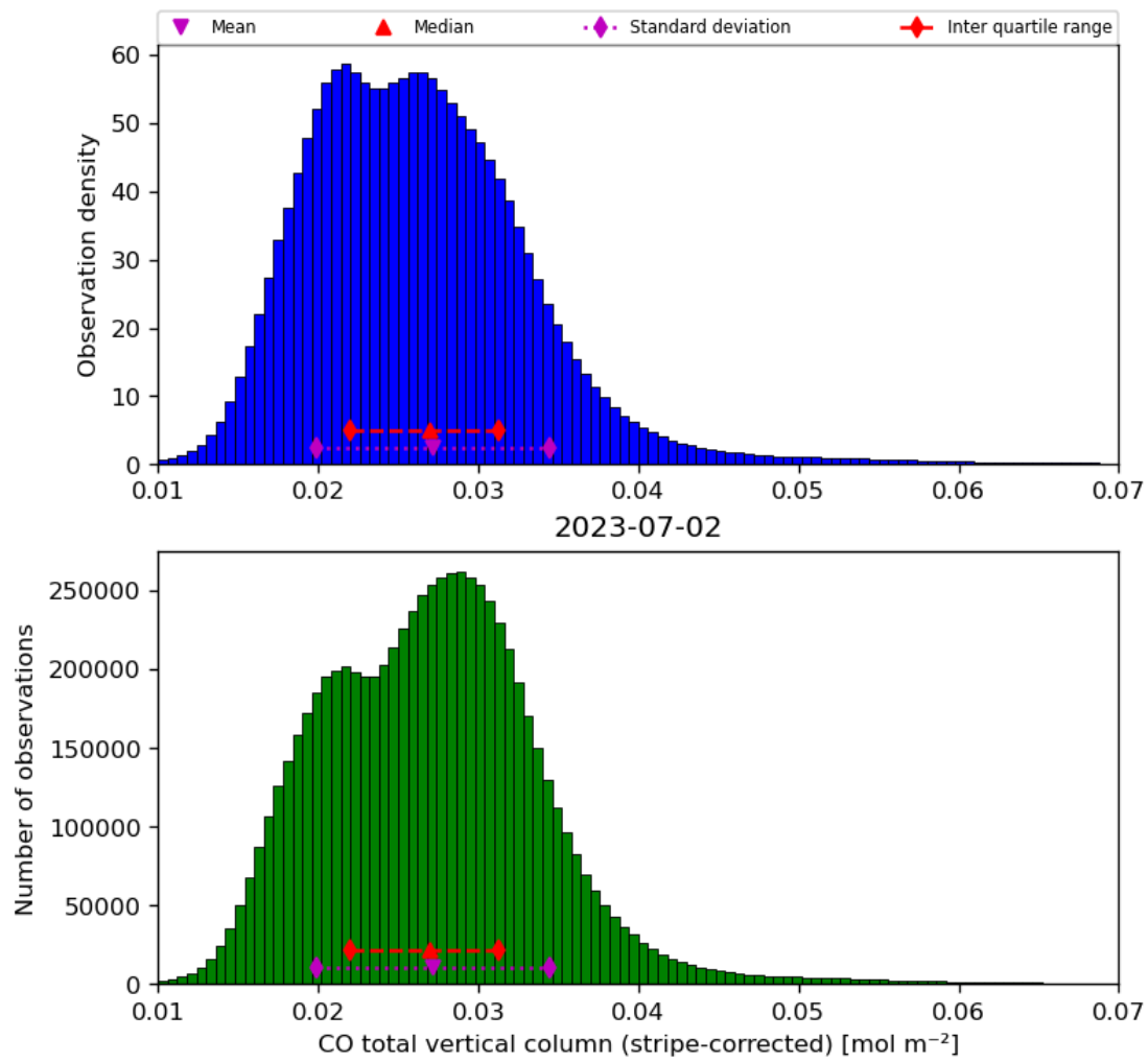
Figure 19: Histogram of “CO total vertical column (stripe-corrected)” for 2023-07-01 to 2023-07-03
