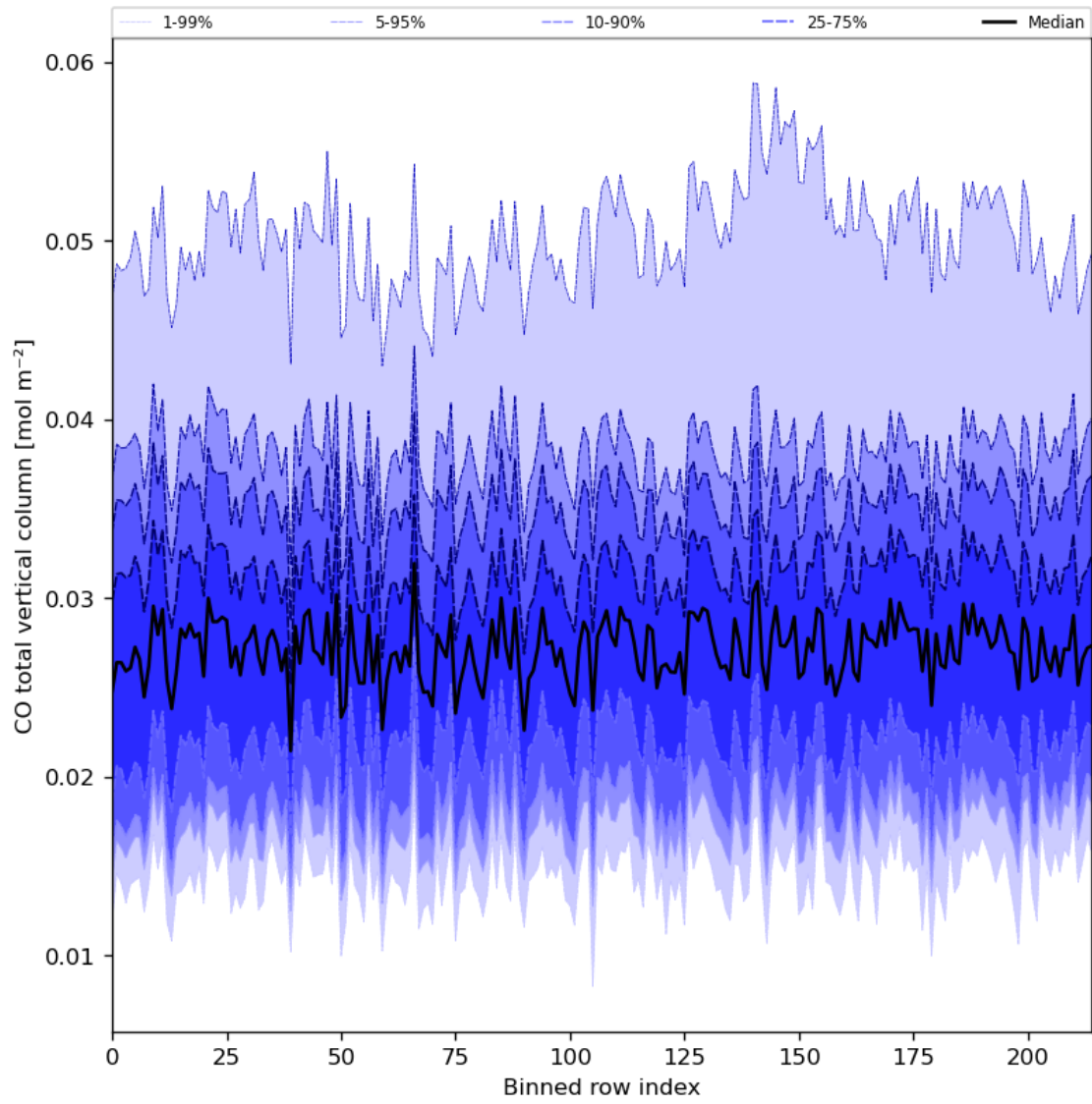
Figure 26: Along track statistics of “CO total vertical column” for 2023-07-01 to 2023-07-03
