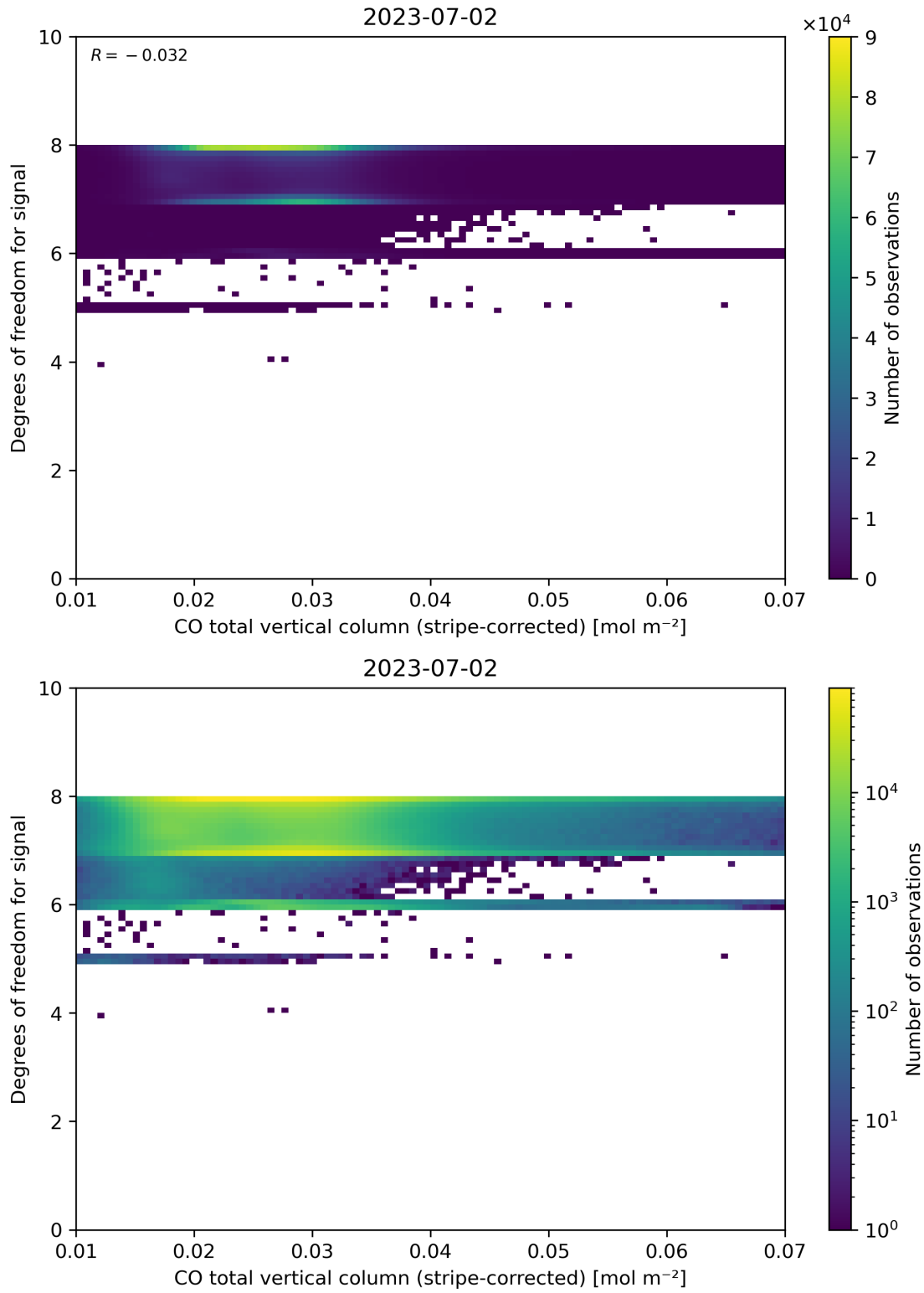
Figure 38: Scatter density plot of “CO total vertical column (stripe-corrected)” against “Degrees of freedom for signal” for 2023-07-01 to 2023-07-03.
