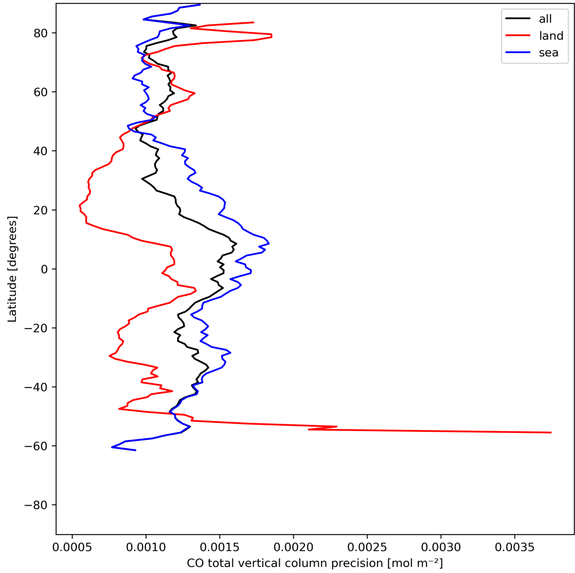
Figure 12: Zonal average of “CO total vertical column precision” for 2023-07-01 to 2023-07-03.
