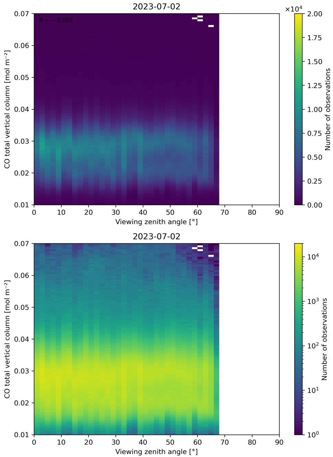
Figure 69: Scatter density plot of “Viewing zenith angle” against “CO total vertical column” for 2023-07-01 to 2023-07-03.
