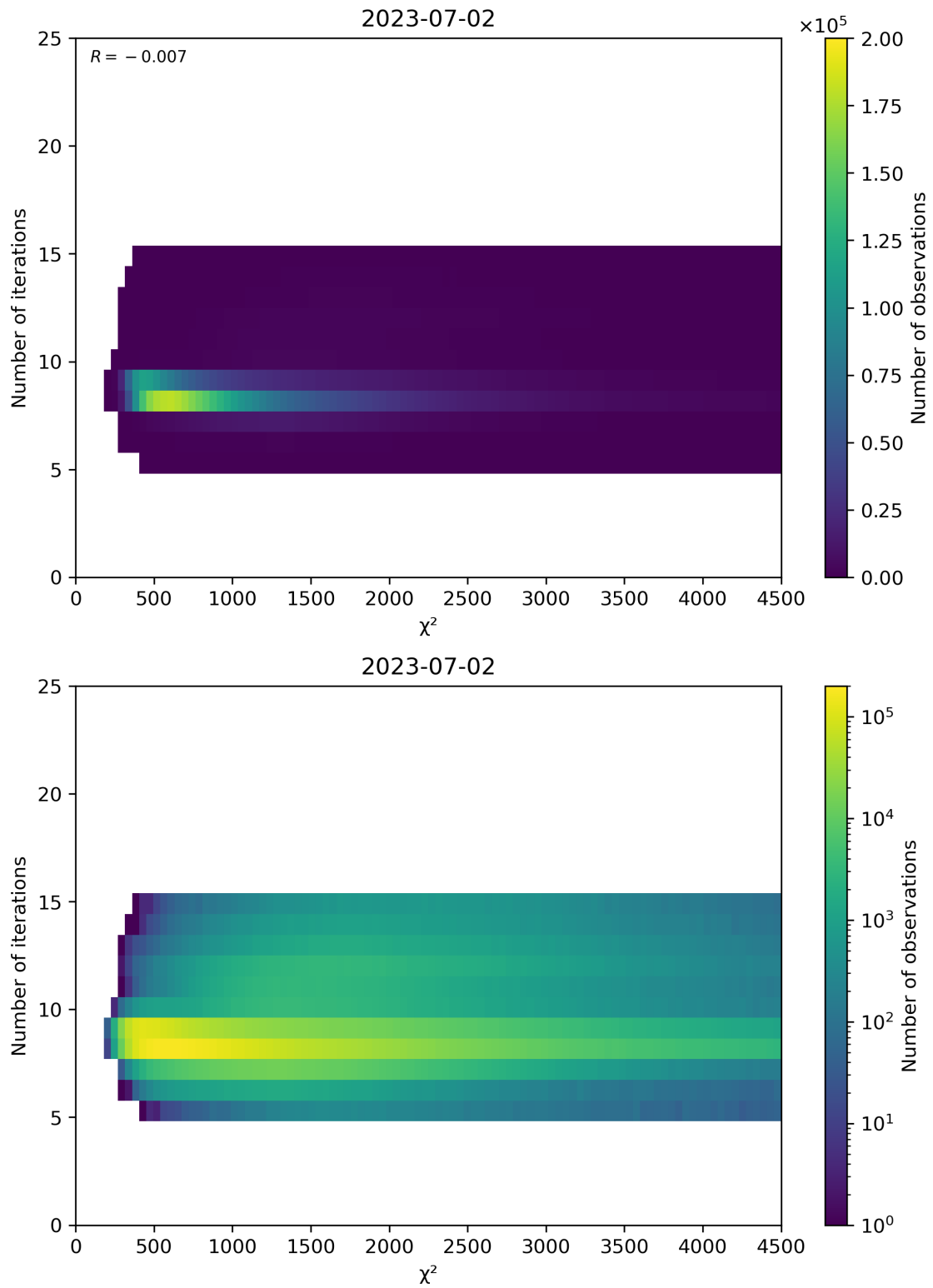
Figure 49: Scatter density plot of “ \chi^2 ” against “Number of iterations” for 2023-07-01 to 2023-07-03.
