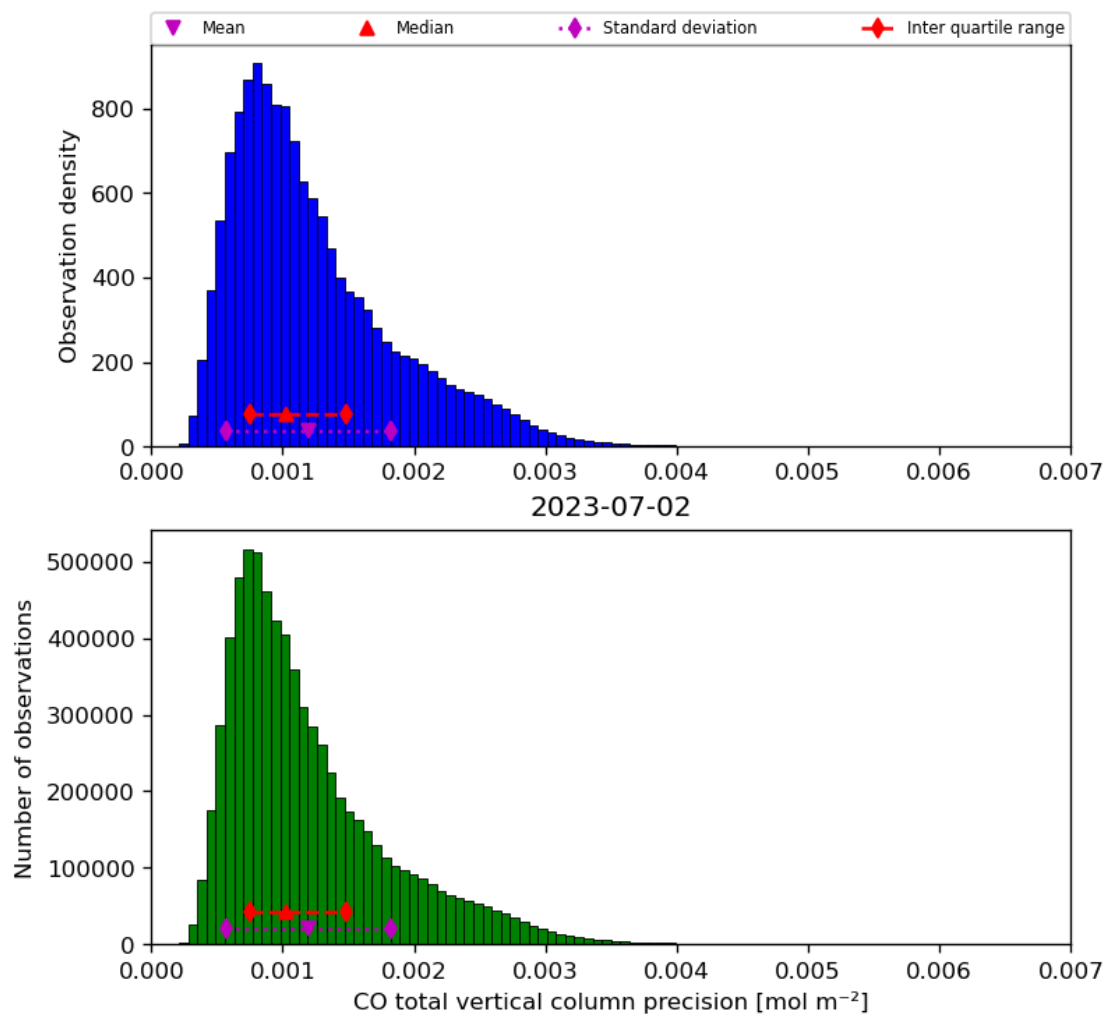
Figure 20: Histogram of “CO total vertical column precision” for 2023-07-01 to 2023-07-03
