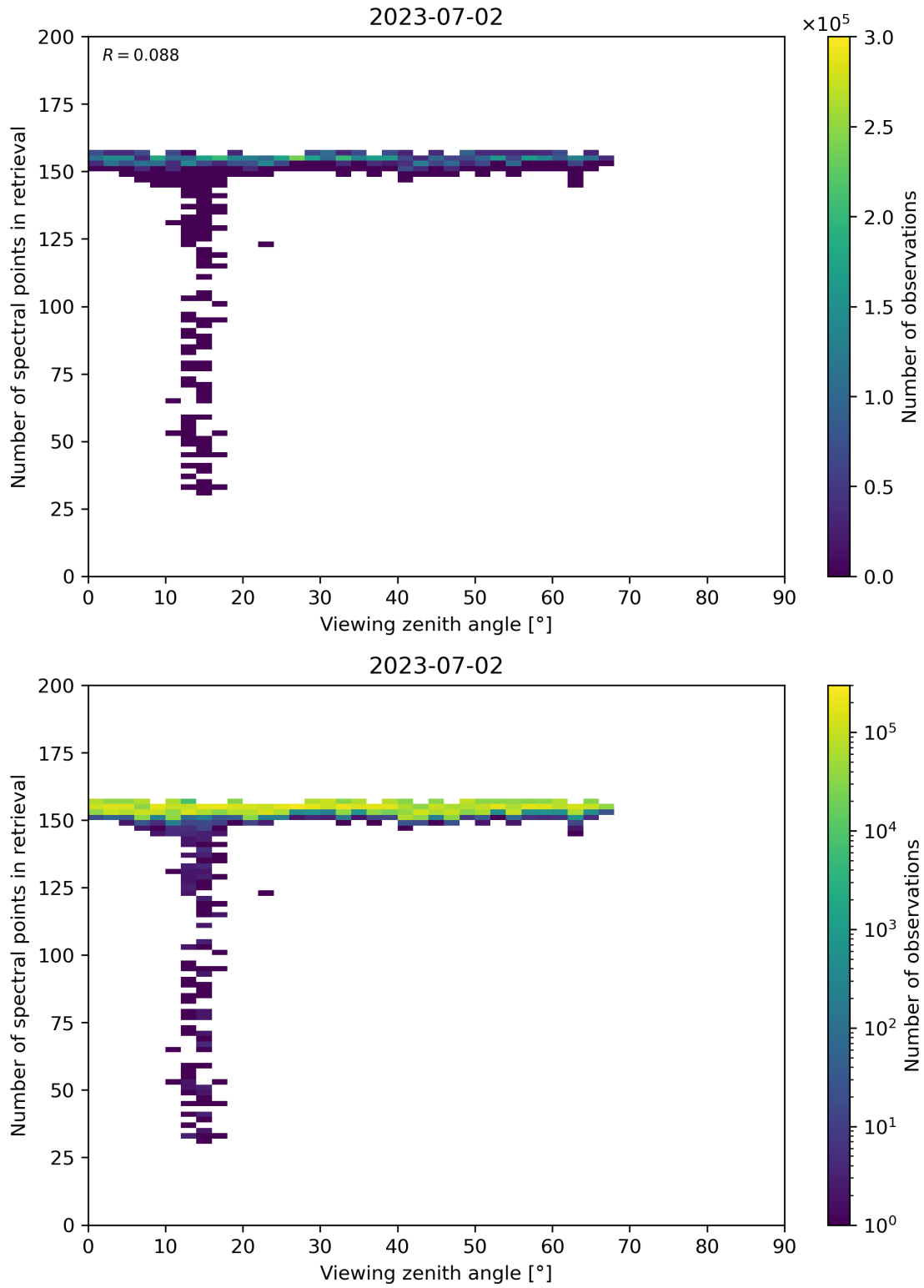
Figure 76: Scatter density plot of “Viewing zenith angle” against “Number of spectral points in retrieval” for 2023-07-01 to 2023-07-03.
