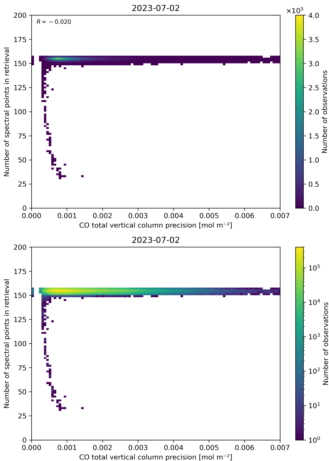
Figure 47: Scatter density plot of “CO total vertical column precision” against “Number of spectral points in retrieval” for 2023-07-01 to 2023-07-03.
