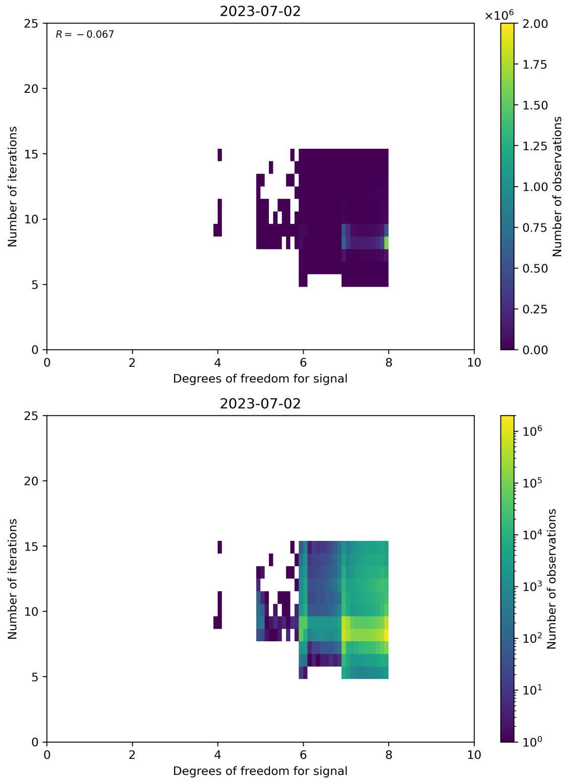
Figure 50: Scatter density plot of “Degrees of freedom for signal” against “Number of iterations” for 2023-07-01 to 2023-07-03.
