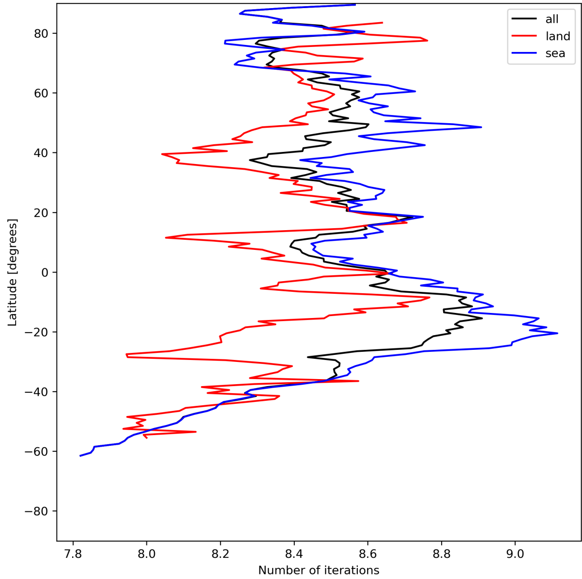
Figure 16: Zonal average of “Number of iterations” for 2023-07-01 to 2023-07-03.
