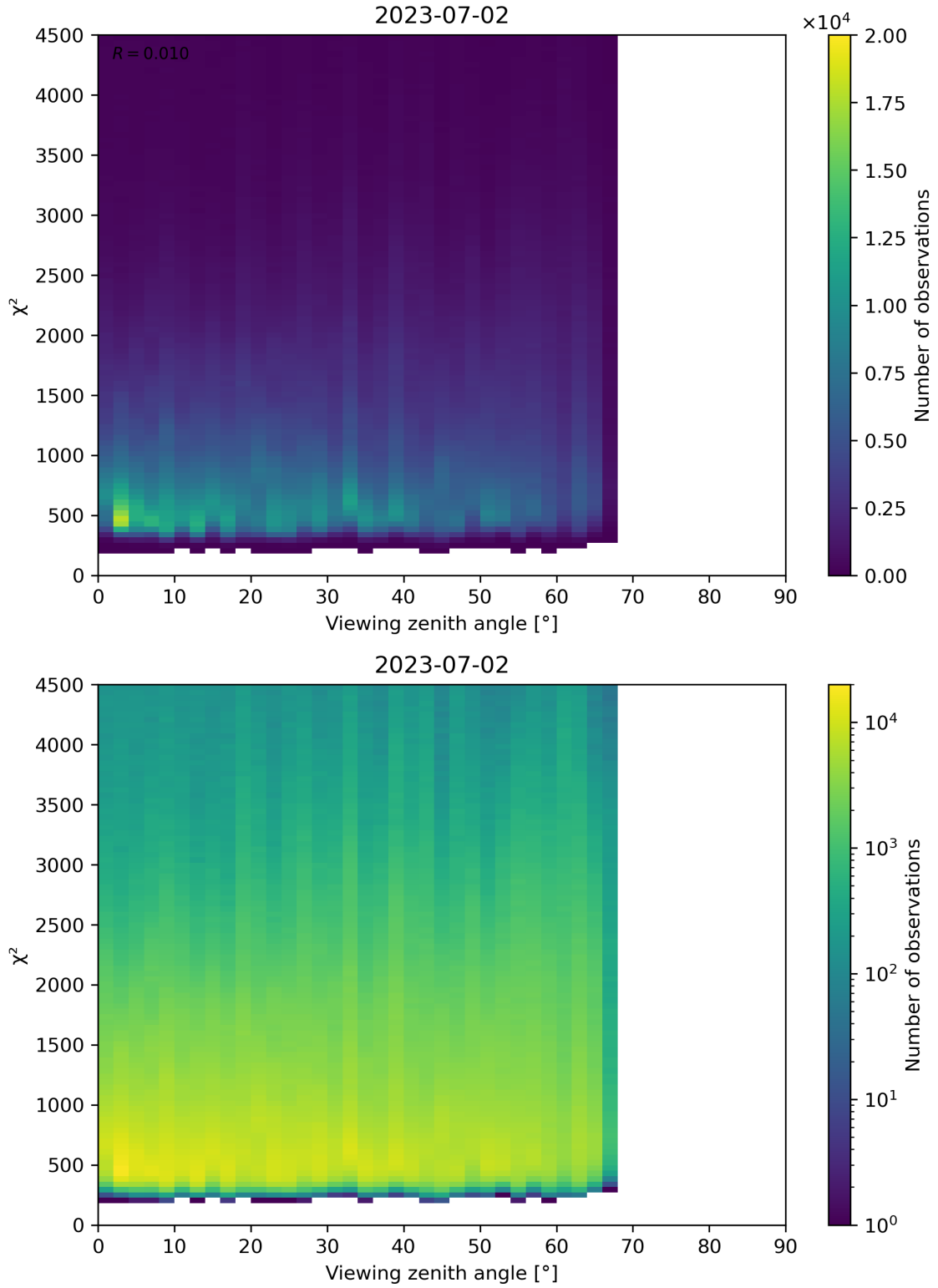
Figure 72: Scatter density plot of “Viewing zenith angle” against “ \chi^2 ” for 2023-07-01 to 2023-07-03.
