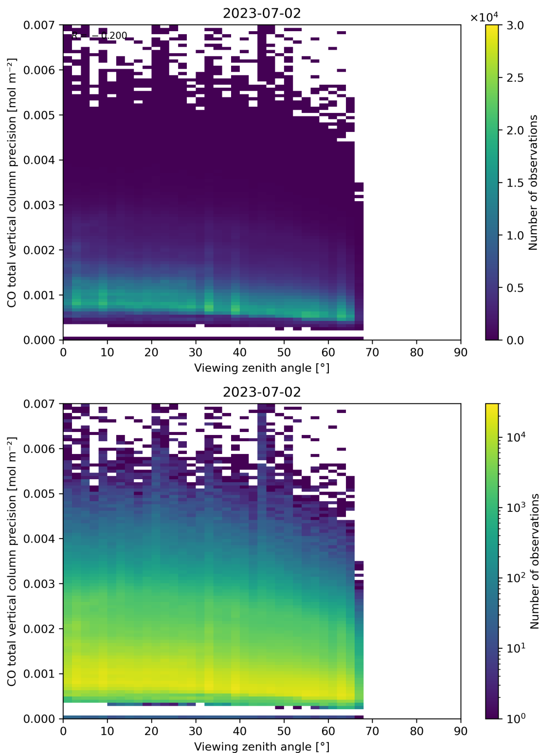
Figure 71: Scatter density plot of “Viewing zenith angle” against “CO total vertical column precision” for 2023-07-01 to 2023-07-03.
