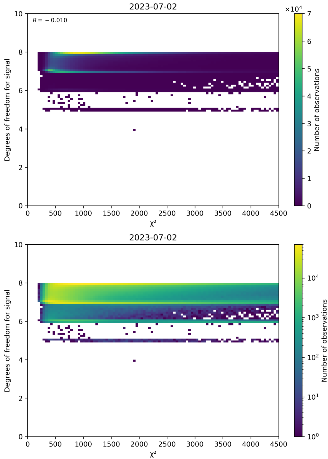
Figure 48: Scatter density plot of “ \chi^2 ” against “Degrees of freedom for signal” for 2023-07-01 to 2023-07-03.
