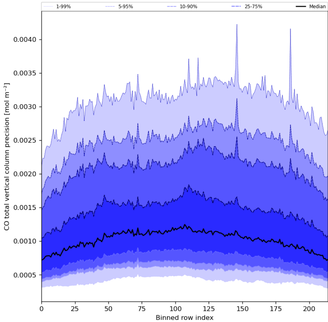
Figure 28: Along track statistics of “CO total vertical column precision” for 2023-07-01 to 2023-07-03
