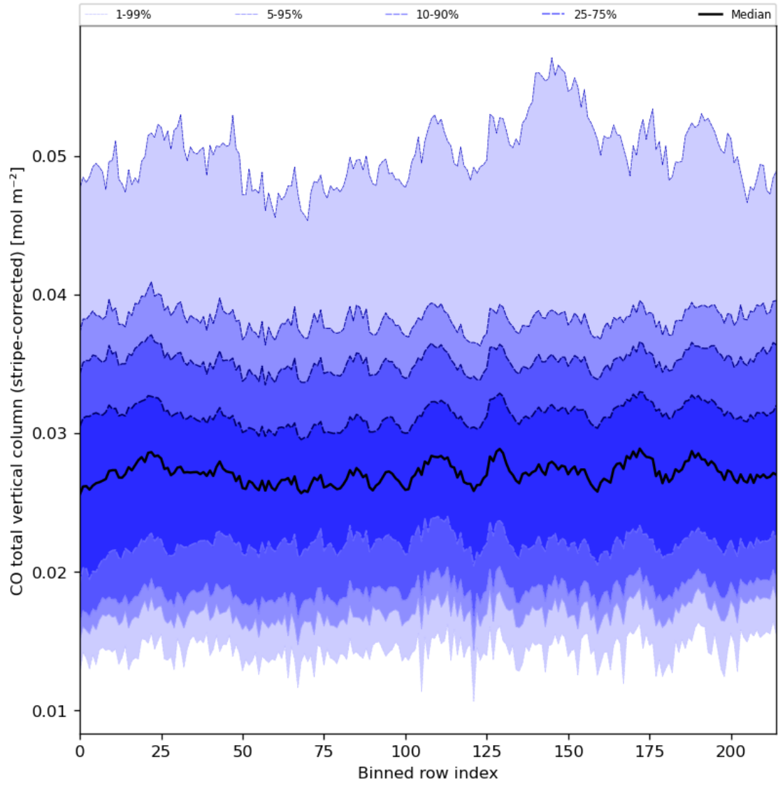
Figure 27: Along track statistics of “CO total vertical column (stripe-corrected)” for 2023-07-01 to 2023-07-03
