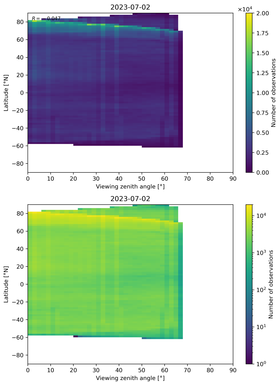
Figure 74: Scatter density plot of “Viewing zenith angle” against “Latitude” for 2023-07-01 to 2023-07-03.
