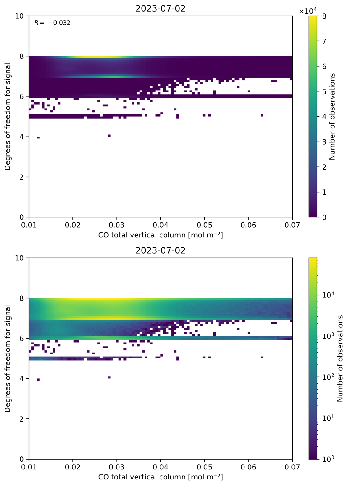
Figure 41: Scatter density plot of “CO total vertical column” against “Degrees of freedom for signal” for 2023-07-01 to 2023-07-03.
