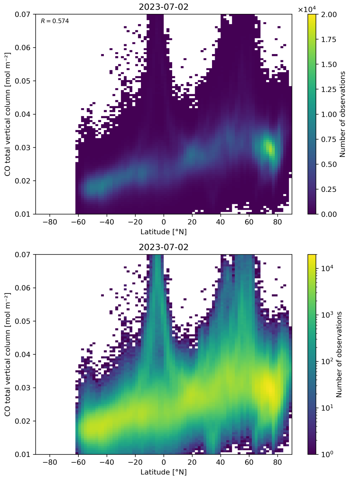
Figure 51: Scatter density plot of “Latitude” against “CO total vertical column” for 2023-07-01 to 2023-07-03.
