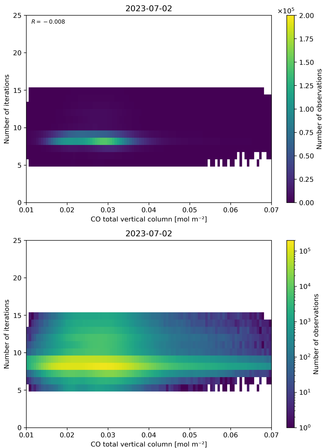
Figure 42: Scatter density plot of “CO total vertical column” against “Number of iterations” for 2023-07-01 to 2023-07-03.
