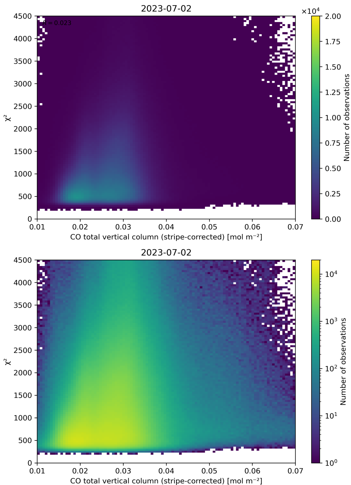
Figure 37: Scatter density plot of “CO total vertical column (stripe-corrected)” against “ \chi^2 ” for 2023-07-01 to 2023-07-03.
