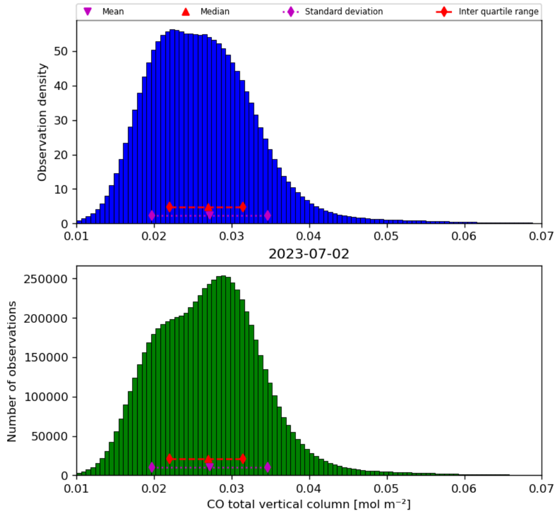
Figure 18: Histogram of “CO total vertical column” for 2023-07-01 to 2023-07-03
