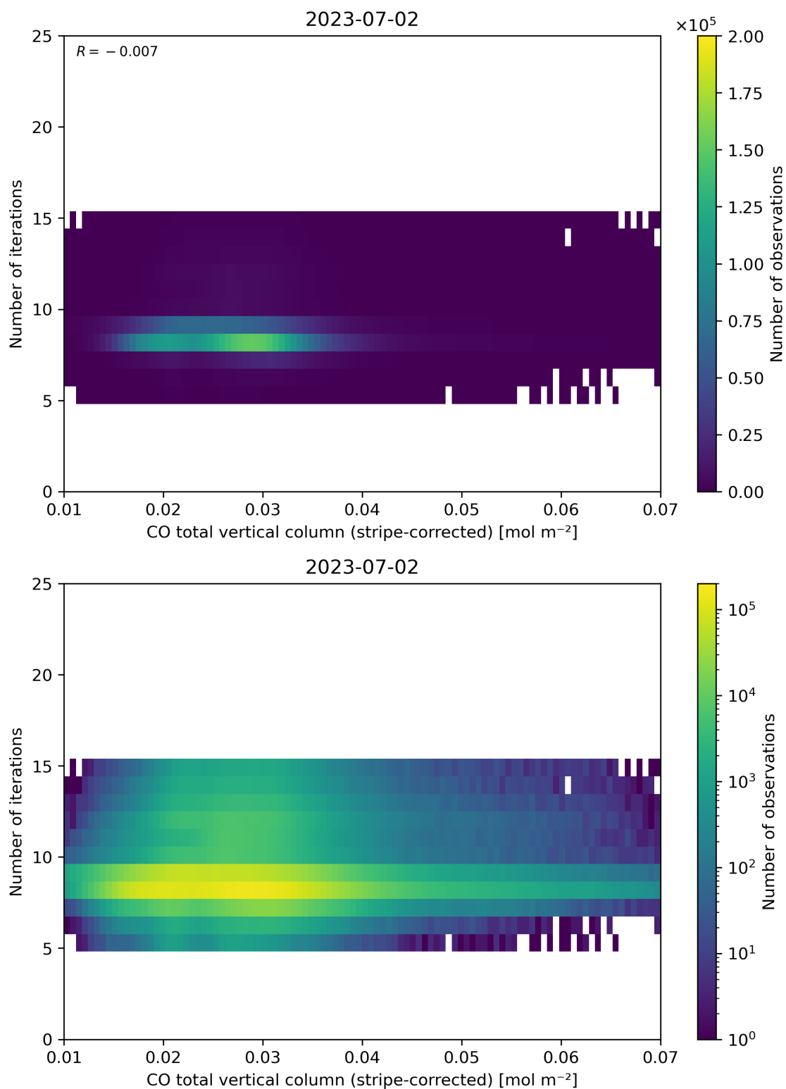
Figure 39: Scatter density plot of “CO total vertical column (stripe-corrected)” against “Number of iterations” for 2023-07-01 to 2023-07-03.
