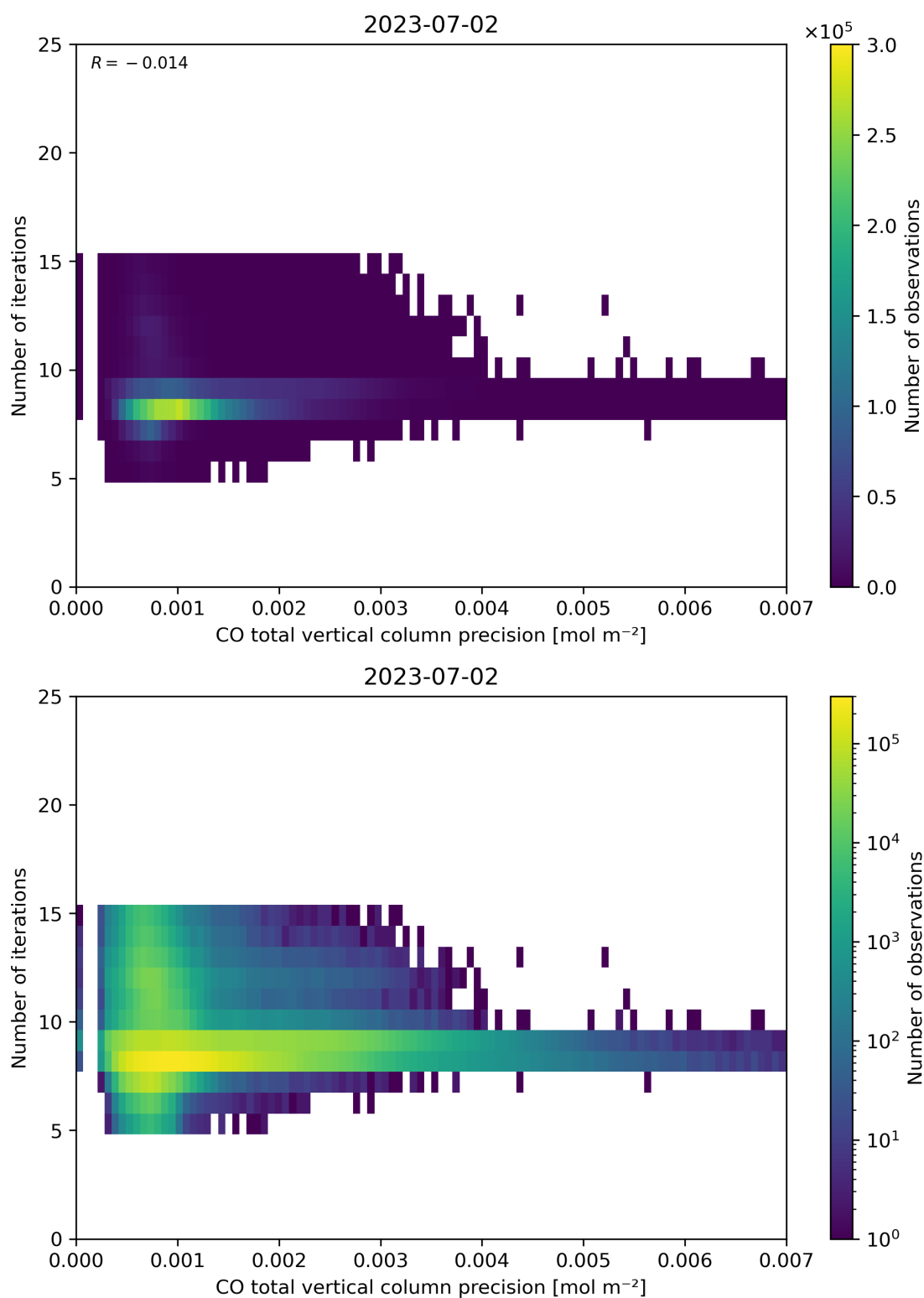
Figure 46: Scatter density plot of “CO total vertical column precision” against “Number of iterations” for 2023-07-01 to 2023-07-03.
