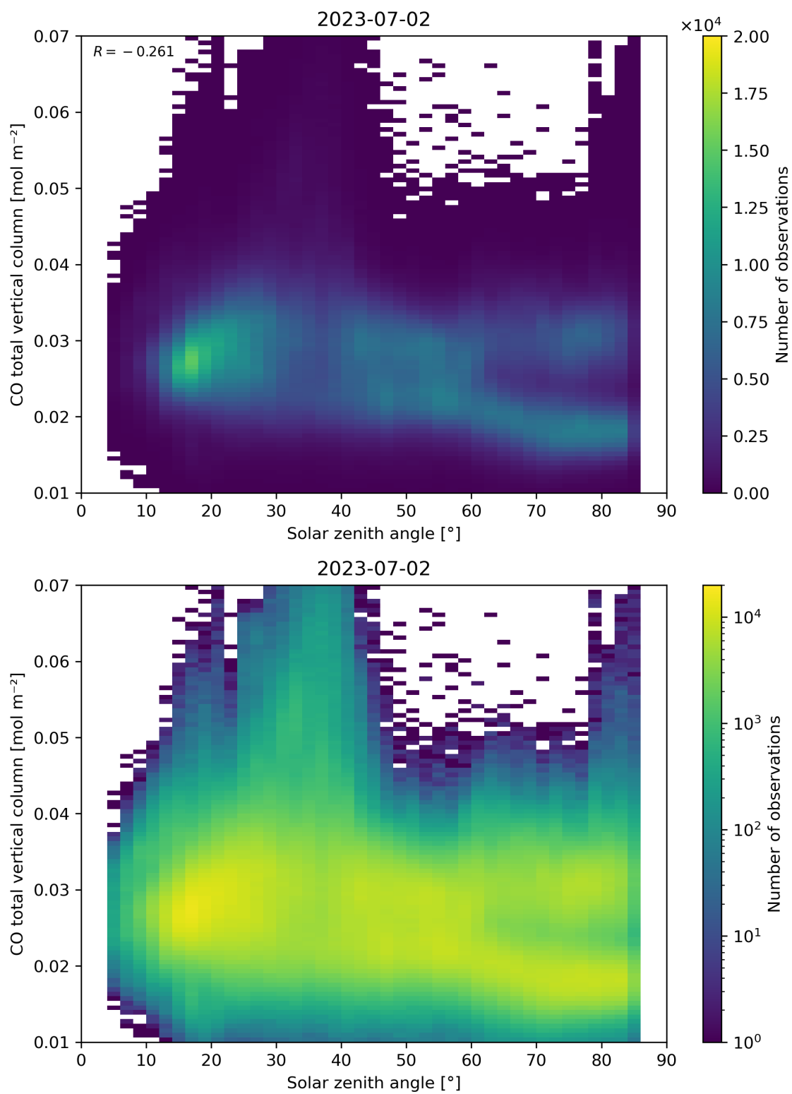
Figure 61: Scatter density plot of “Solar zenith angle” against “CO total vertical column” for 2023-07-01 to 2023-07-03.
