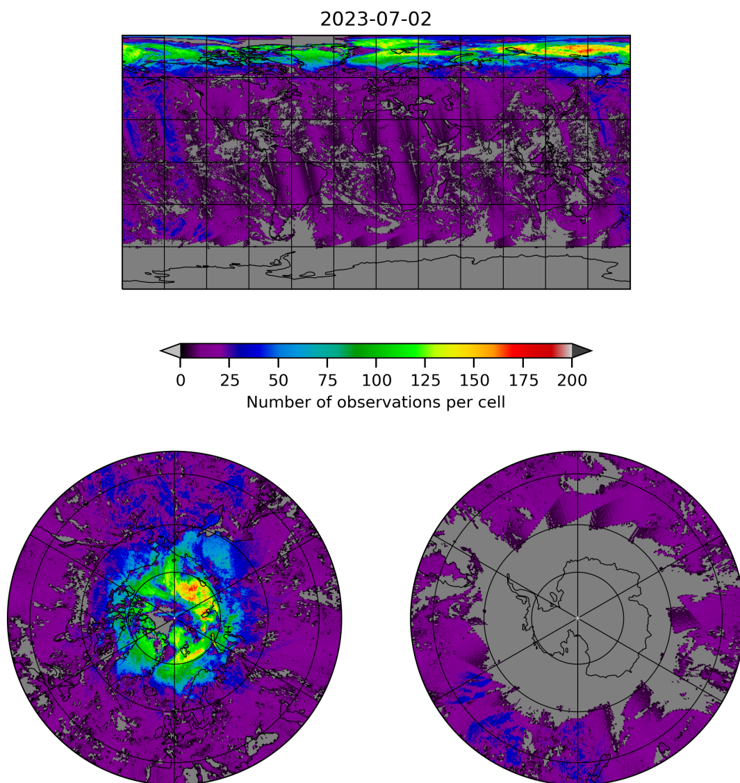
Figure 8: Map of the number of observations for 2023-07-01 to 2023-07-03
