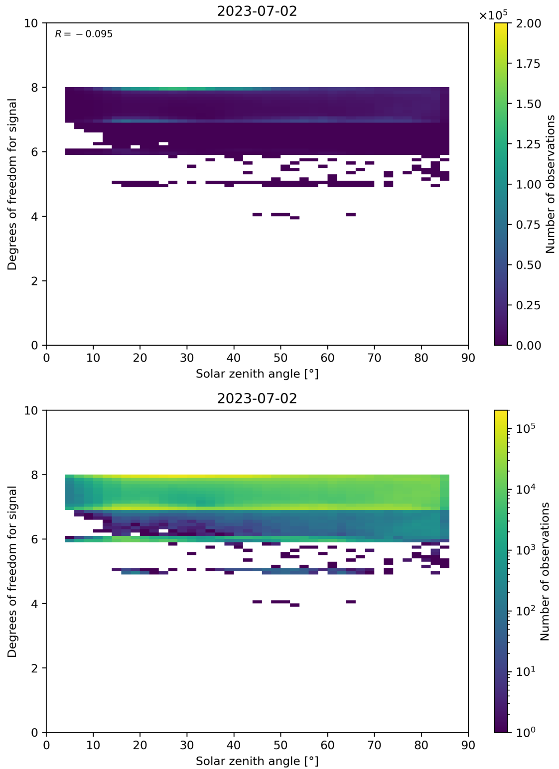
Figure 65: Scatter density plot of “Solar zenith angle” against “Degrees of freedom for signal” for 2023-07-01 to 2023-07-03.
