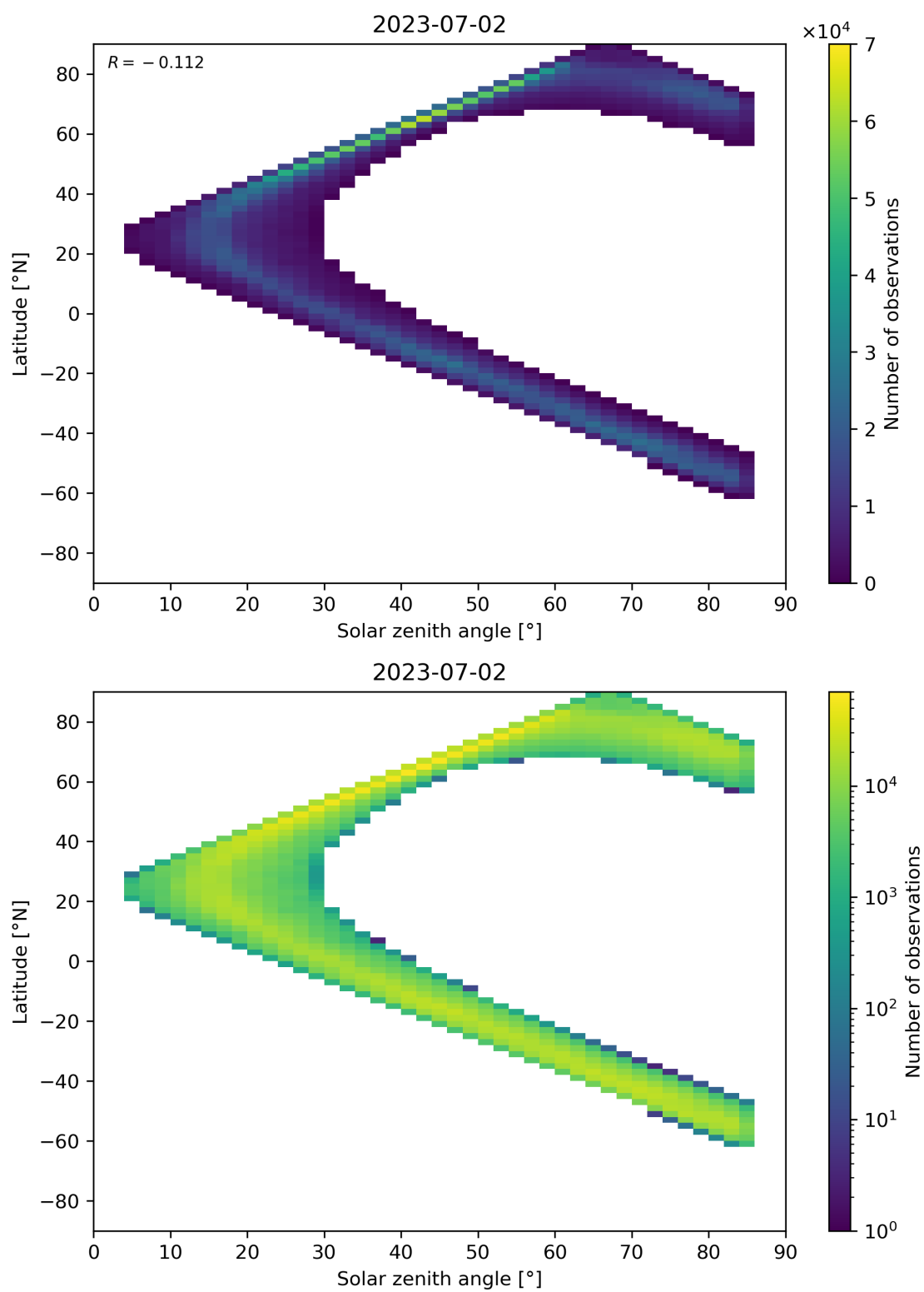
Figure 66: Scatter density plot of “Solar zenith angle” against “Latitude” for 2023-07-01 to 2023-07-03.
