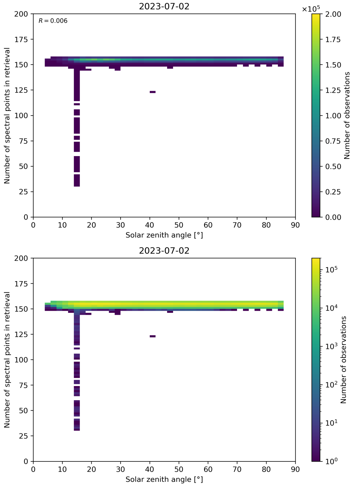
Figure 68: Scatter density plot of “Solar zenith angle” against “Number of spectral points in retrieval” for 2023-07-01 to 2023-07-03.
