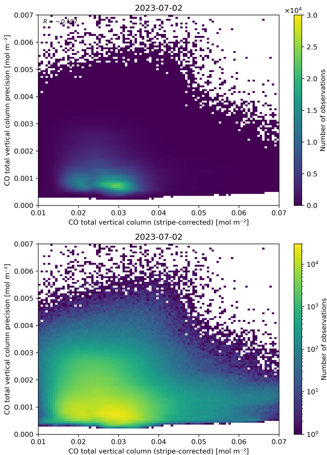
Figure 36: Scatter density plot of “CO total vertical column (stripe-corrected)” against “CO total vertical column precision” for 2023-07-01 to 2023-07-03.
