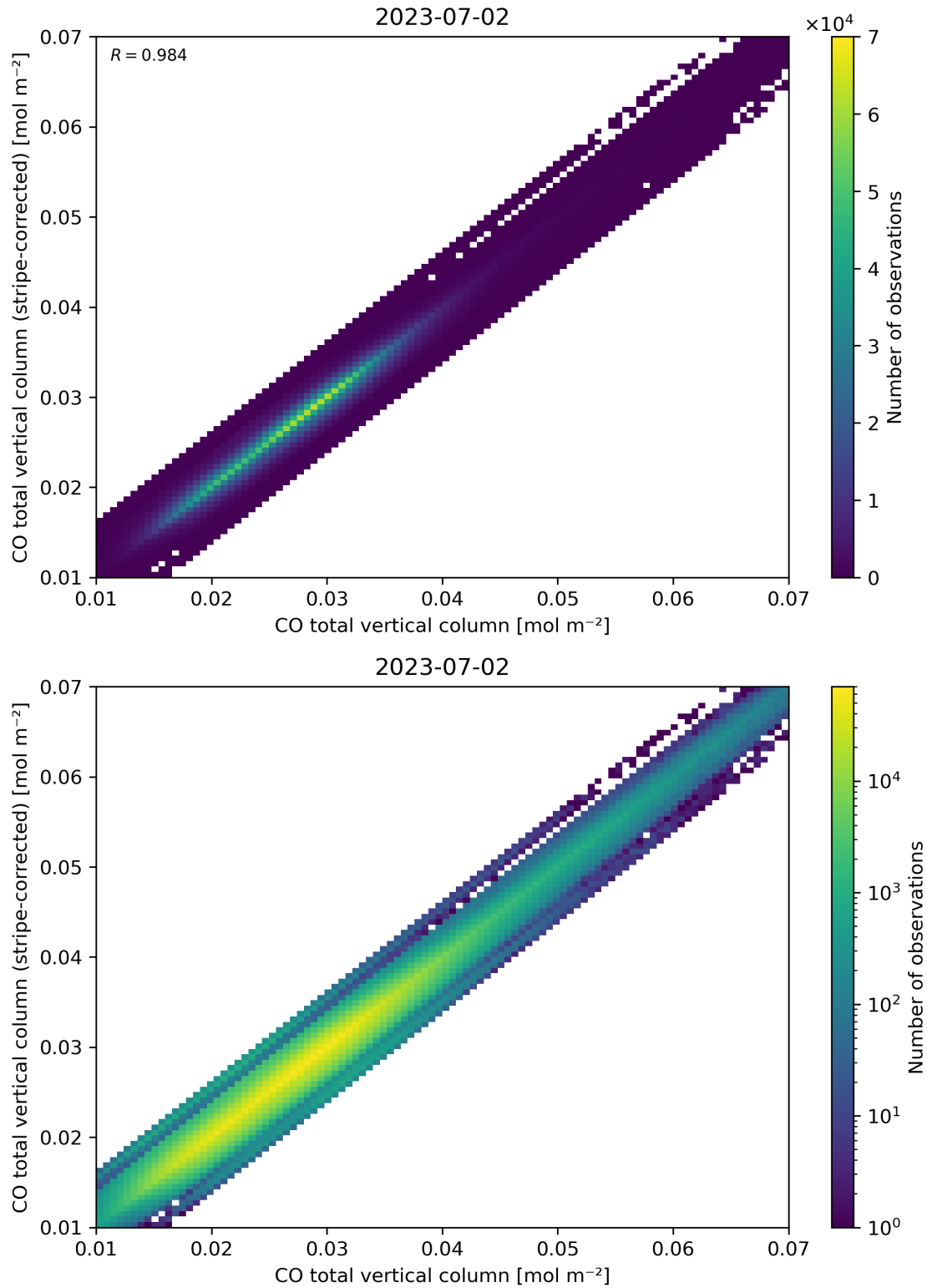
Figure 33: Scatter density plot of “CO total vertical column” against “CO total vertical column (stripe-corrected)” for 2023-07-01 to 2023-07-03.
