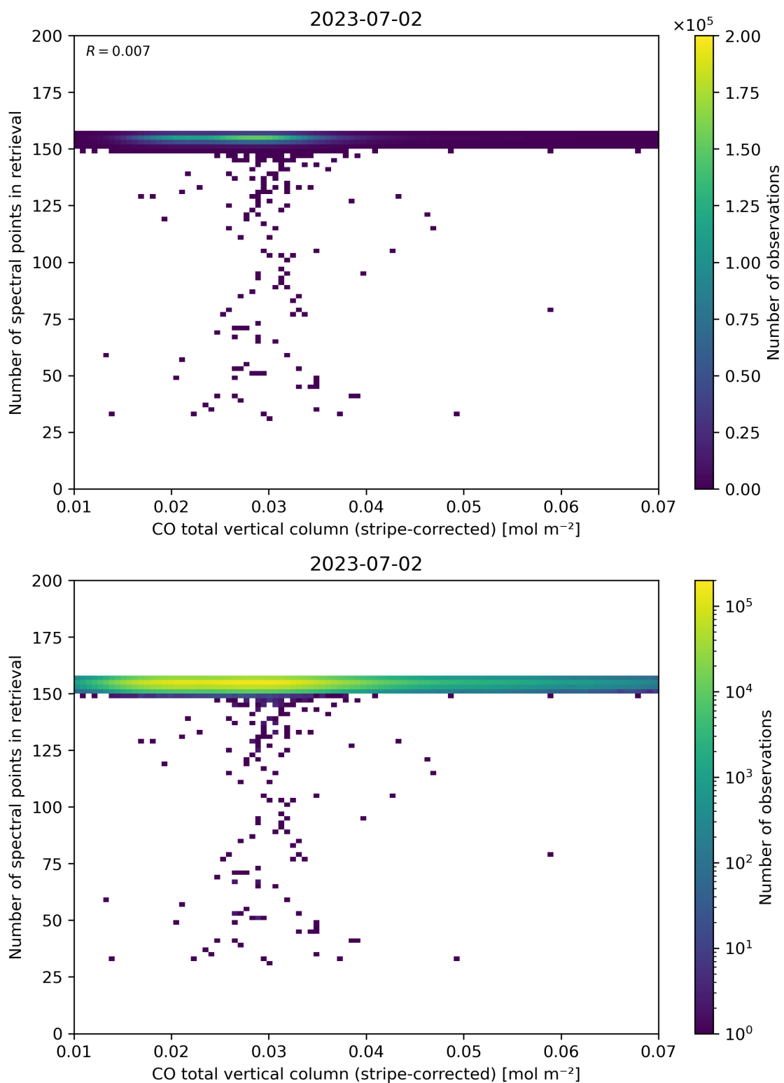
Figure 40: Scatter density plot of “CO total vertical column (stripe-corrected)” against “Number of spectral points in retrieval” for 2023-07-01 to 2023-07-03.
