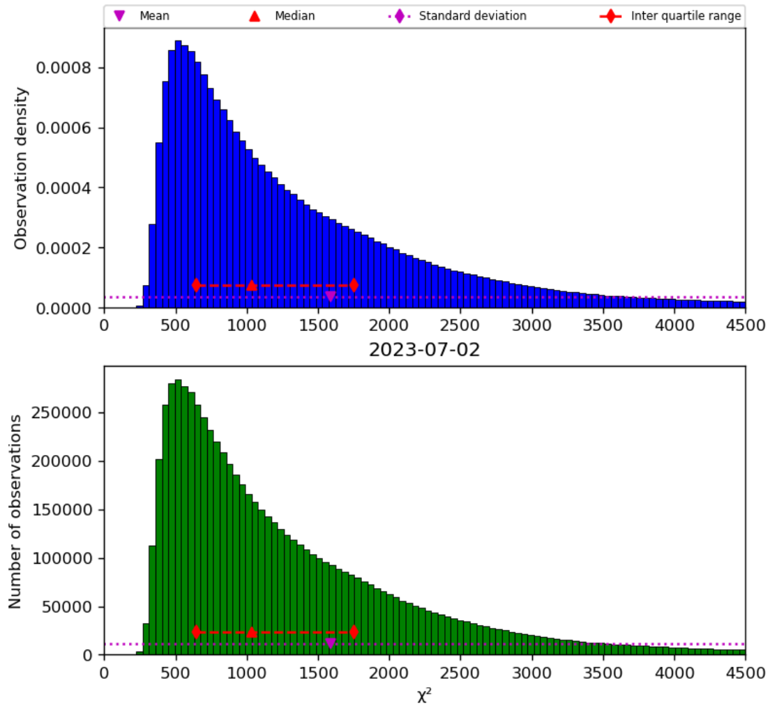
Figure 22: Histogram of “ \chi^2 ” for 2023-07-01 to 2023-07-03
