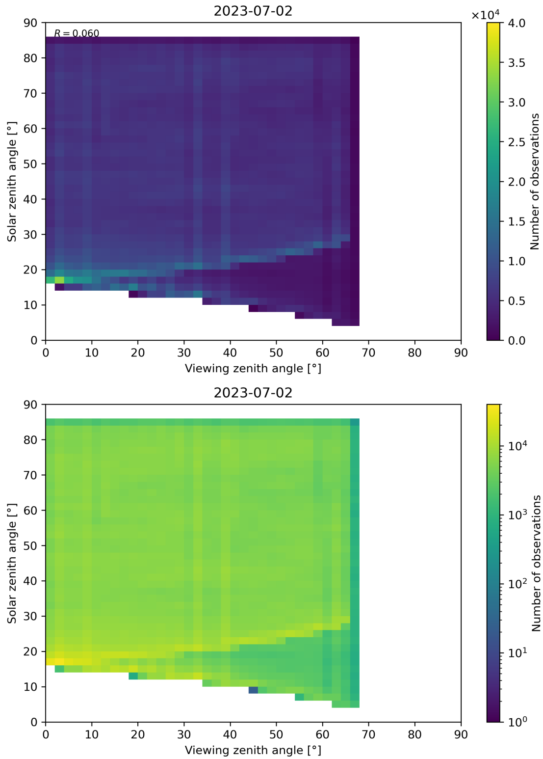
Figure 77: Scatter density plot of “Viewing zenith angle” against “Solar zenith angle” for 2023-07-01 to 2023-07-03.
