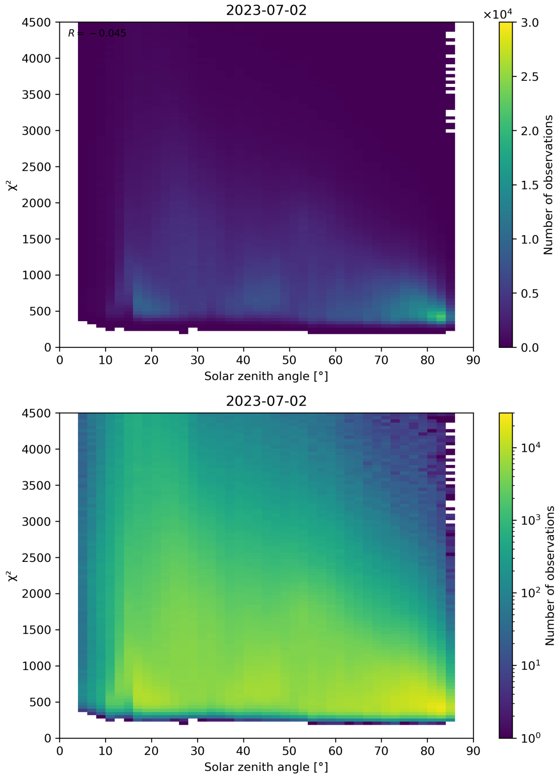
Figure 64: Scatter density plot of “Solar zenith angle” against “ \chi^2 ” for 2023-07-01 to 2023-07-03.
