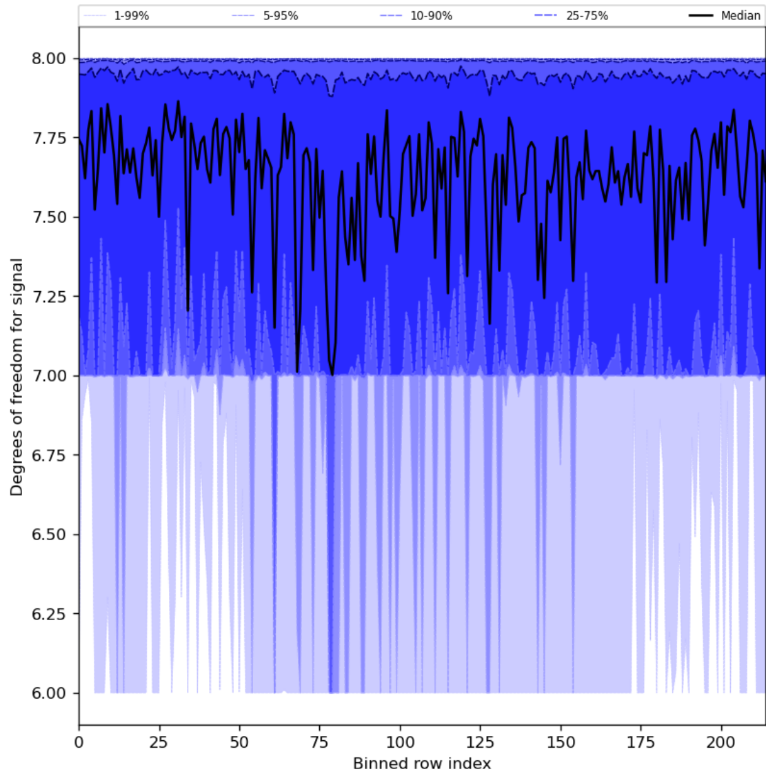
Figure 31: Along track statistics of “Degrees of freedom for signal” for 2023-07-01 to 2023-07-03
