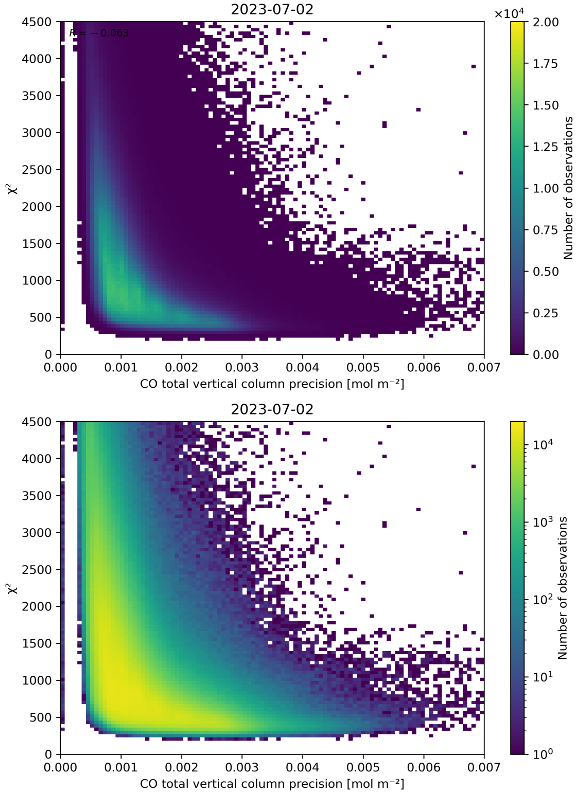
Figure 44: Scatter density plot of “CO total vertical column precision” against “ \chi^2 ” for 2023-07-01 to 2023-07-03.
