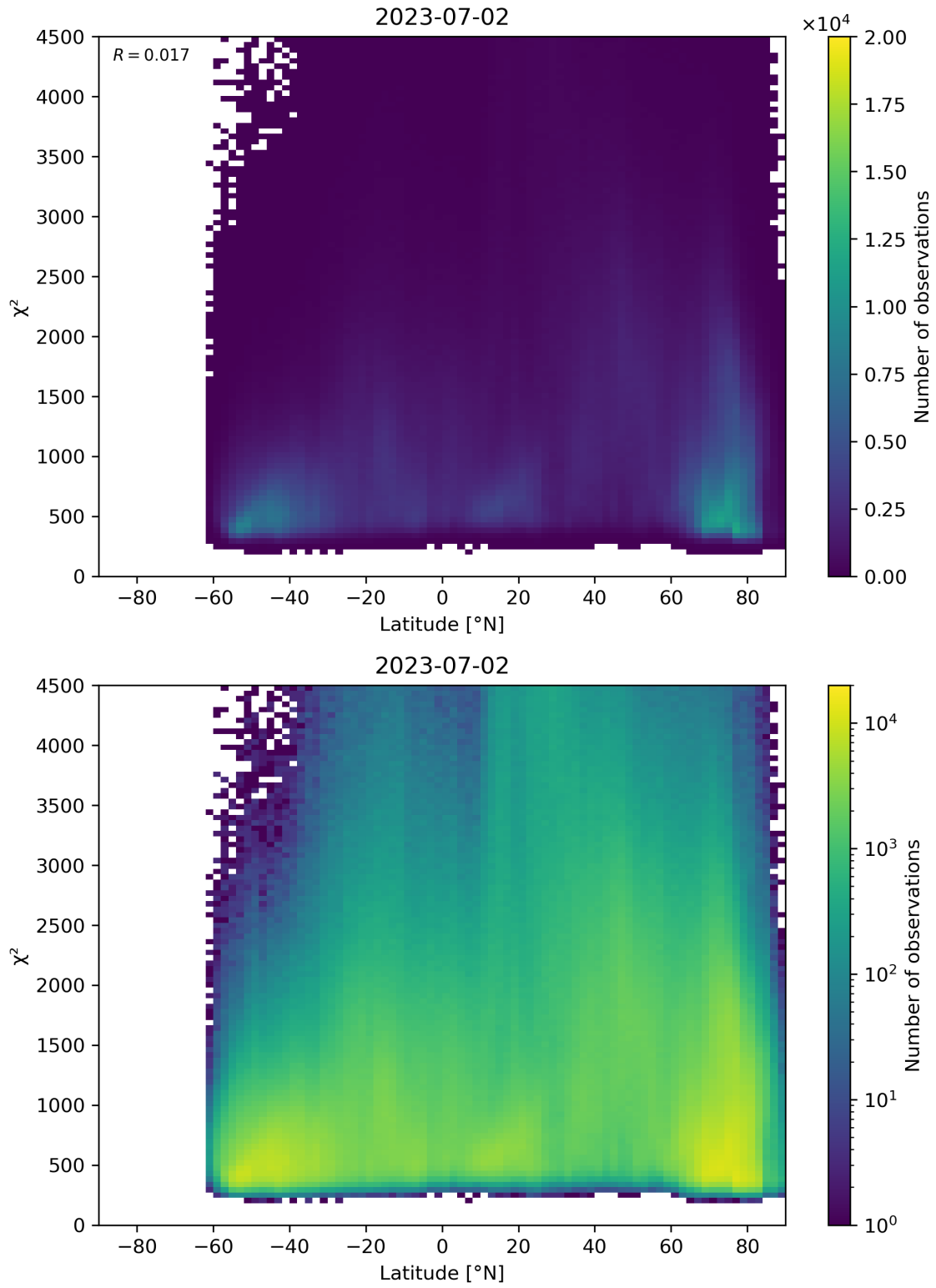
Figure 54: Scatter density plot of “Latitude” against “ \chi^2 ” for 2023-07-01 to 2023-07-03.
