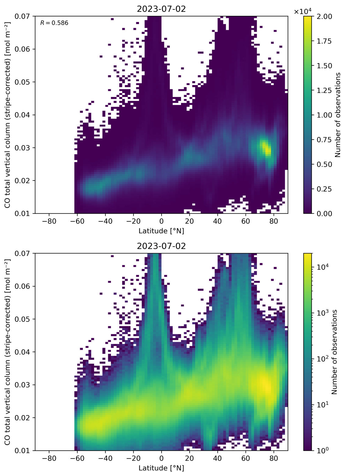
Figure 52: Scatter density plot of “Latitude” against “CO total vertical column (stripe-corrected)” for 2023-07-01 to 2023-07-03.
