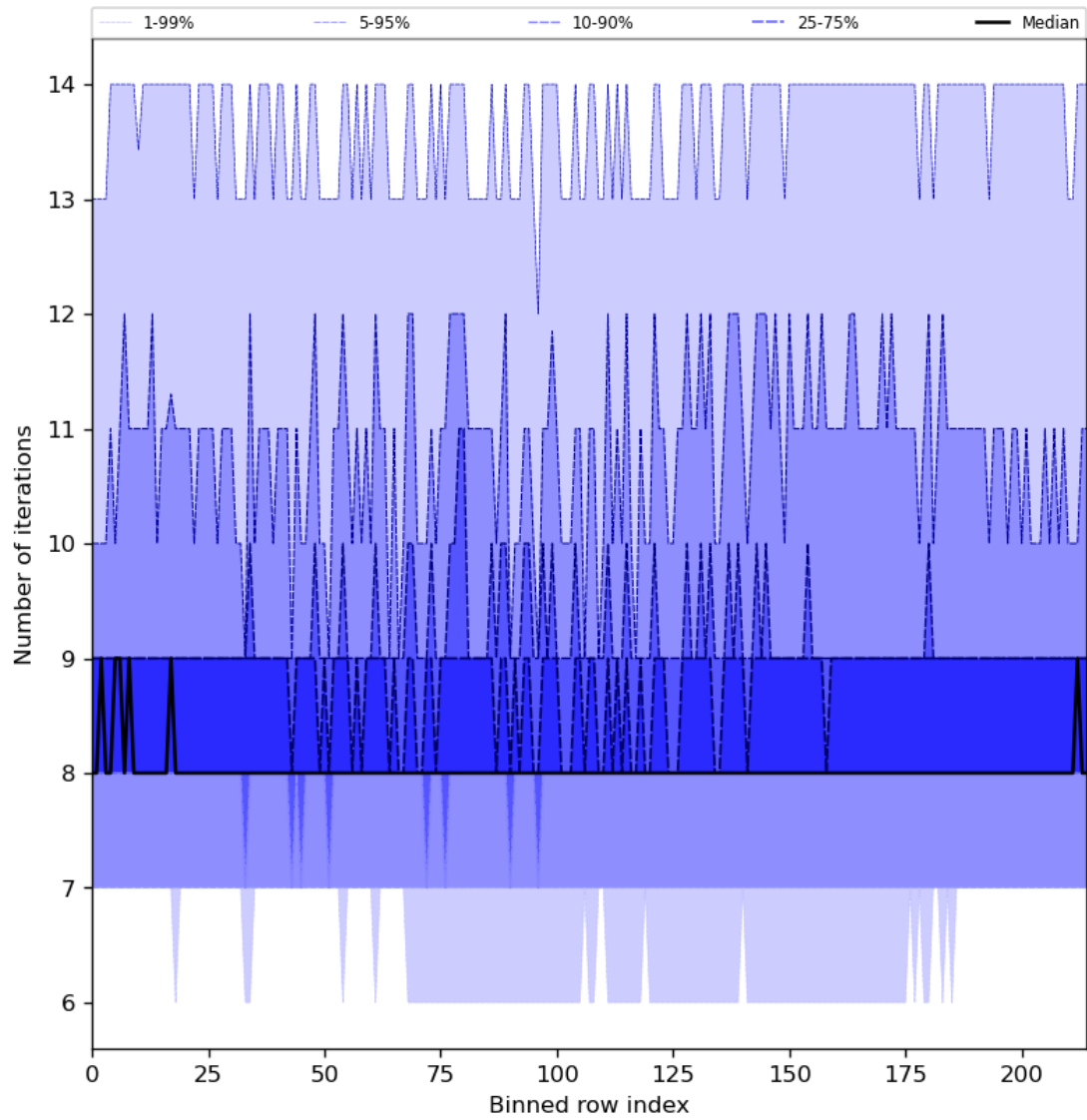
Figure 32: Along track statistics of “Number of iterations” for 2023-07-01 to 2023-07-03
