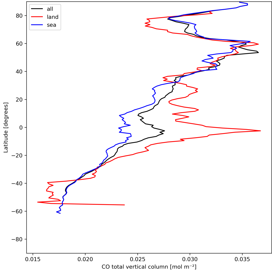
Figure 10: Zonal average of “CO total vertical column” for 2023-07-01 to 2023-07-03.
