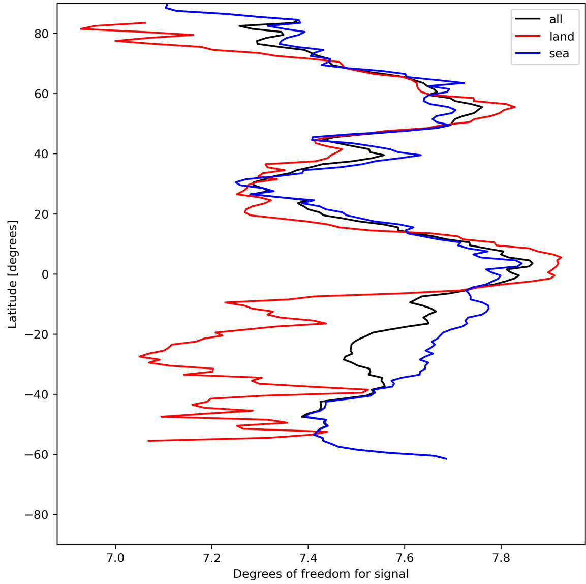
Figure 15: Zonal average of “Degrees of freedom for signal” for 2023-07-01 to 2023-07-03.
