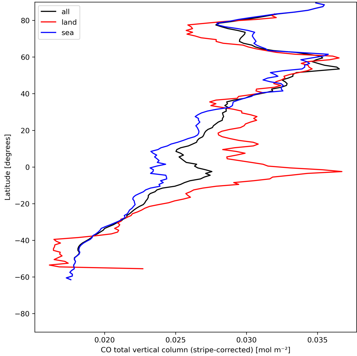
Figure 11: Zonal average of “CO total vertical column (stripe-corrected)” for 2023-07-01 to 2023-07-03.
