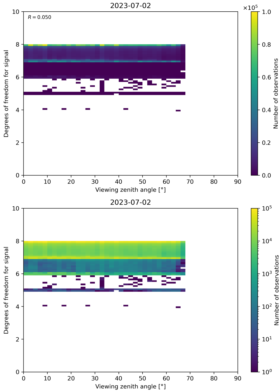
Figure 73: Scatter density plot of “Viewing zenith angle” against “Degrees of freedom for signal” for 2023-07-01 to 2023-07-03.
