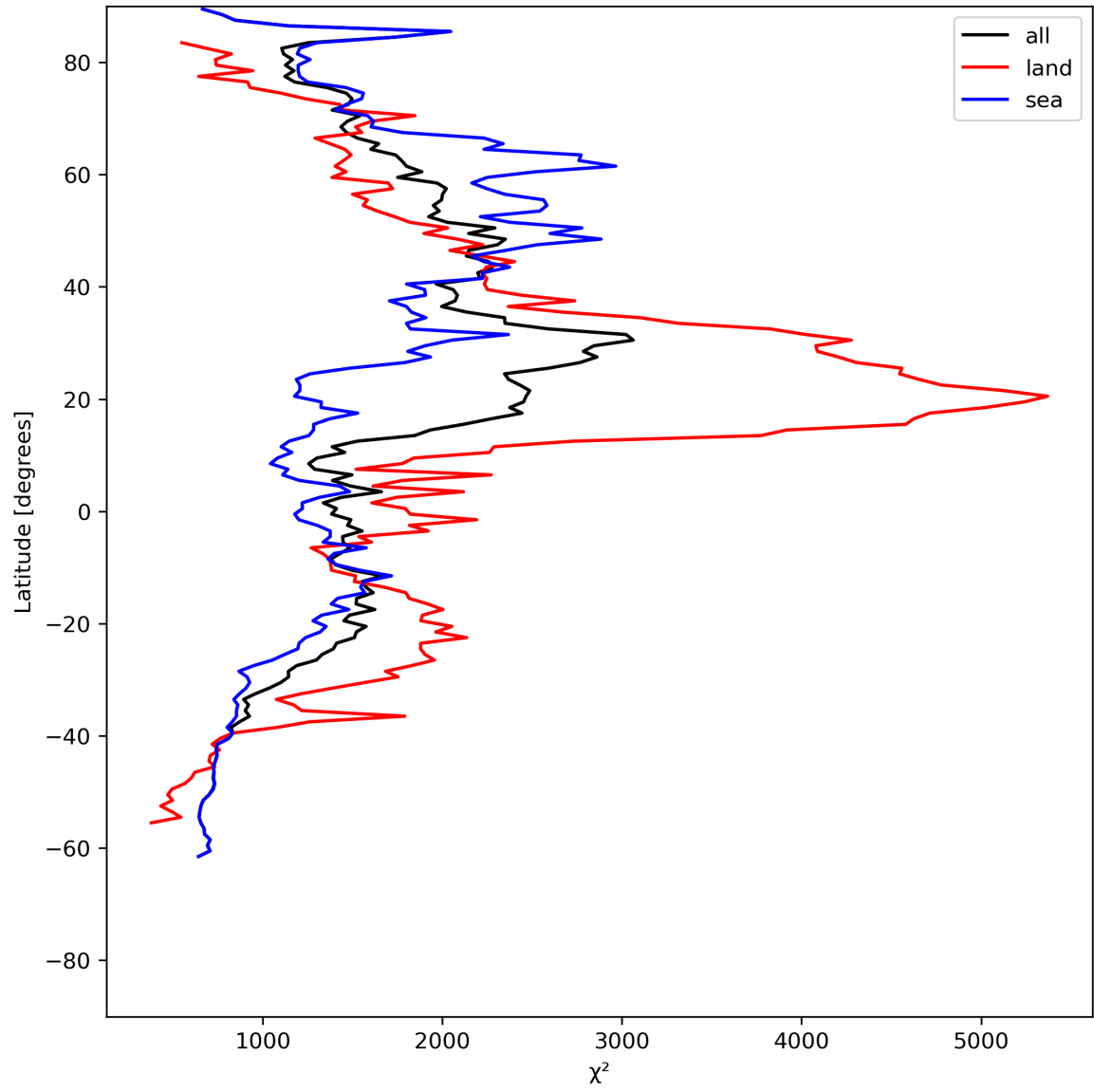
Figure 14: Zonal average of “ \chi^2 ” for 2023-07-01 to 2023-07-03.
