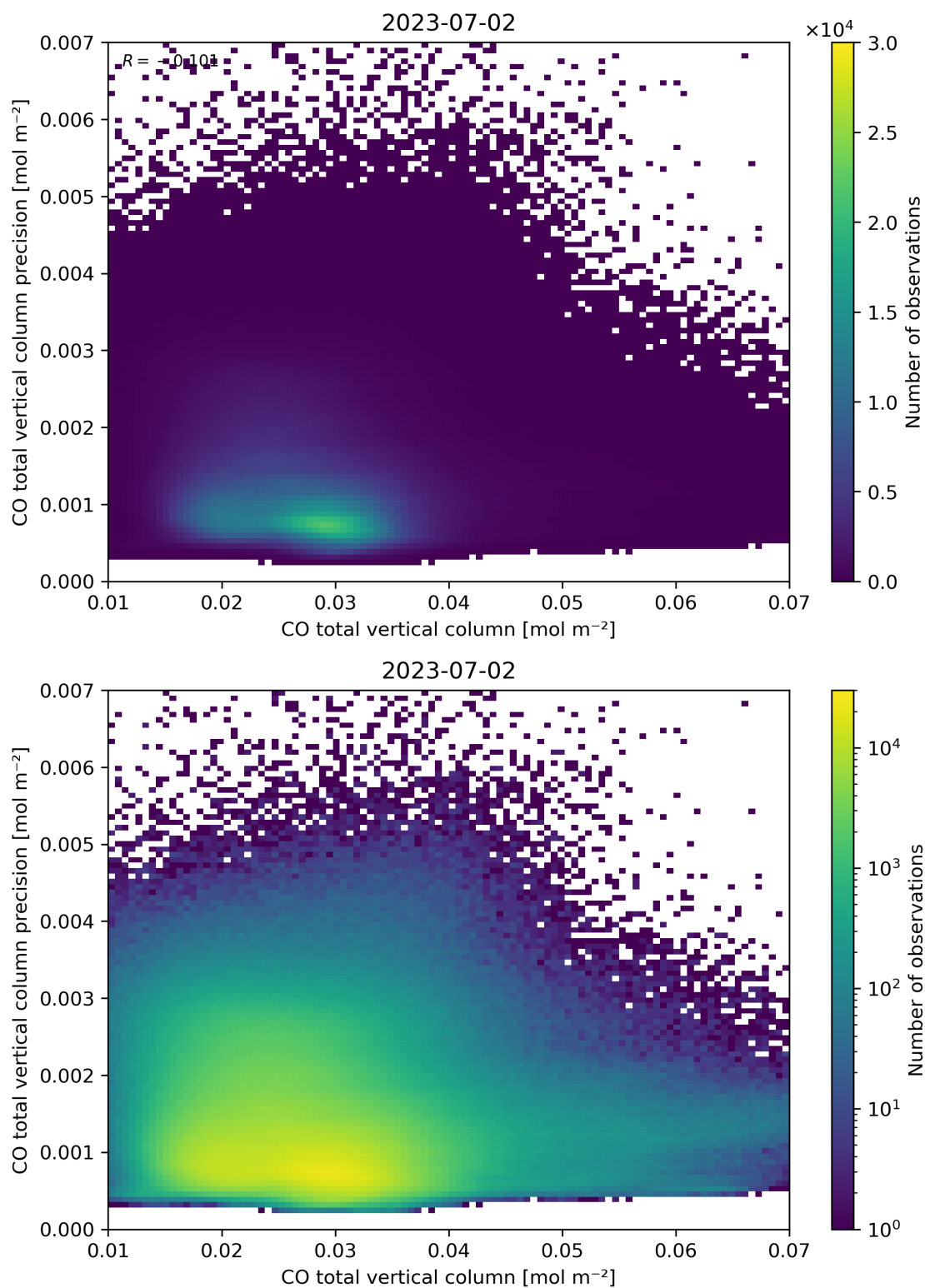
Figure 34: Scatter density plot of “CO total vertical column” against “CO total vertical column precision” for 2023-07-01 to 2023-07-03.
