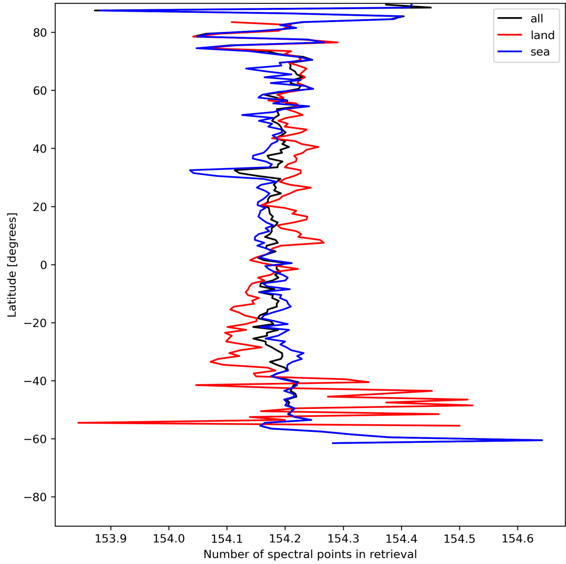
Figure 13: Zonal average of “Number of spectral points in retrieval” for 2023-07-01 to 2023-07-03.
