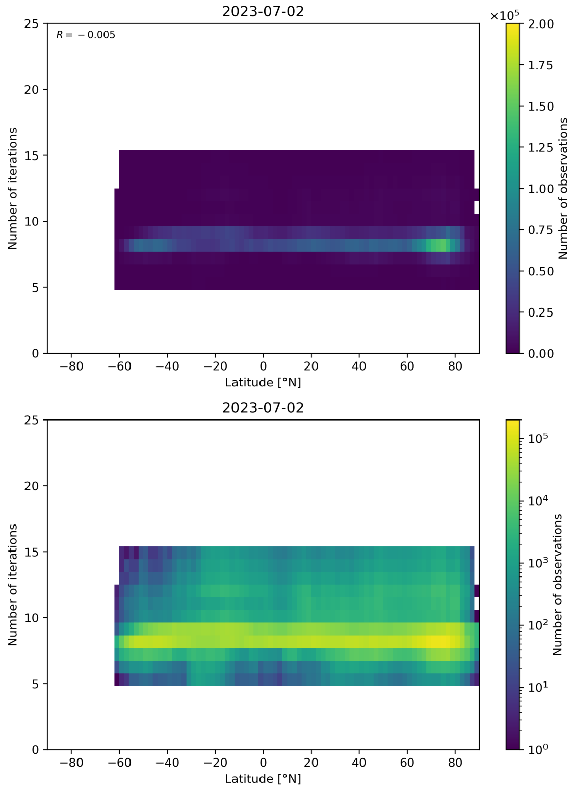
Figure 56: Scatter density plot of “Latitude” against “Number of iterations” for 2023-07-01 to 2023-07-03.
