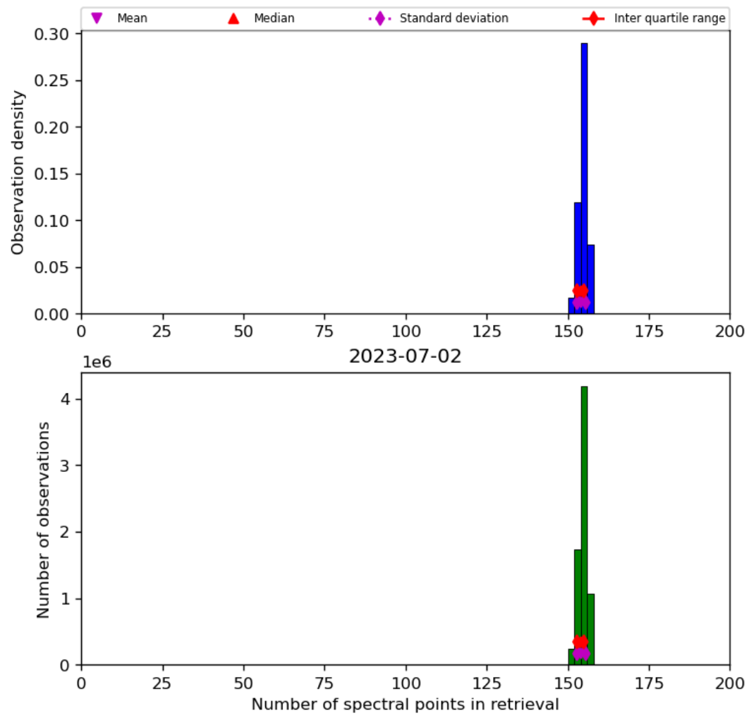
Figure 21: Histogram of “Number of spectral points in retrieval” for 2023-07-01 to 2023-07-03
