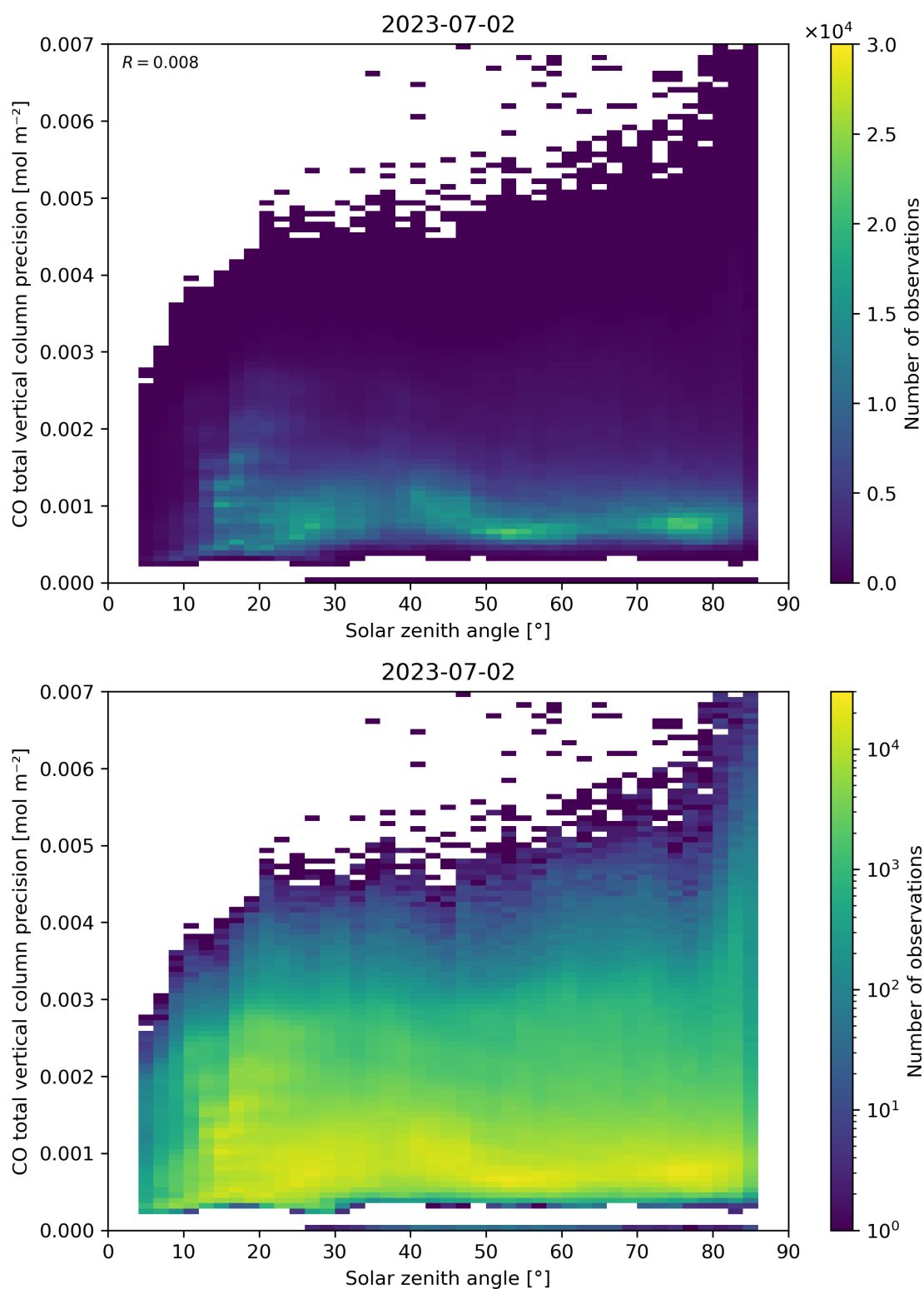
Figure 63: Scatter density plot of “Solar zenith angle” against “CO total vertical column precision” for 2023-07-01 to 2023-07-03.
