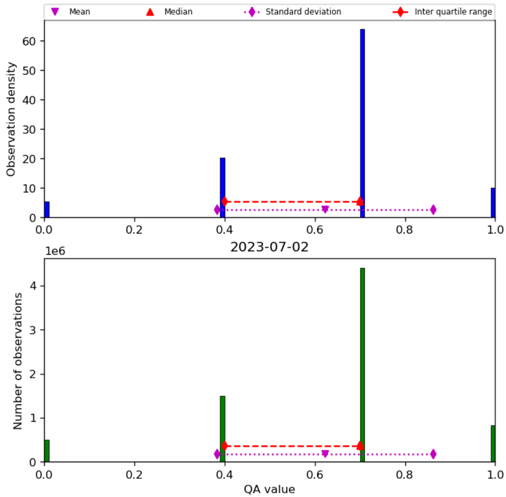
Figure 17: Histogram of “QA value” for 2023-07-01 to 2023-07-03
