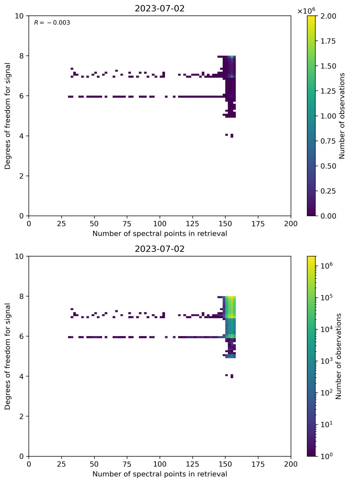
Figure 59: Scatter density plot of “Number of spectral points in retrieval” against “Degrees of freedom for signal” for 2023-07-01 to 2023-07-03.
