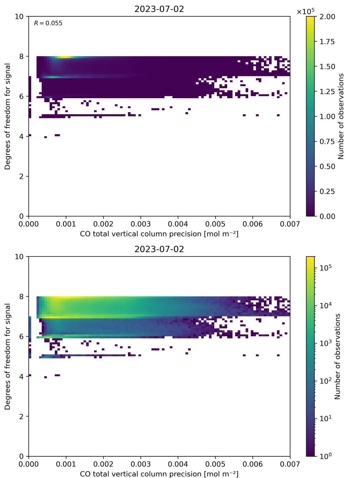
Figure 45: Scatter density plot of “CO total vertical column precision” against “Degrees of freedom for signal” for 2023-07-01 to 2023-07-03.
