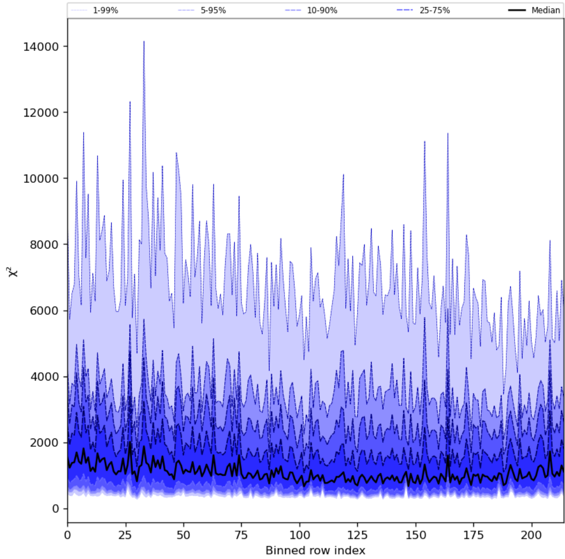
Figure 30: Along track statistics of “ \chi^2 ” for 2023-07-01 to 2023-07-03
