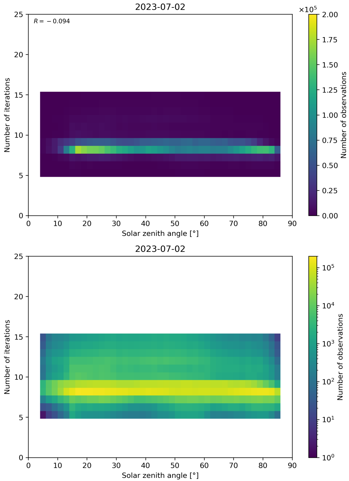
Figure 67: Scatter density plot of “Solar zenith angle” against “Number of iterations” for 2023-07-01 to 2023-07-03.
