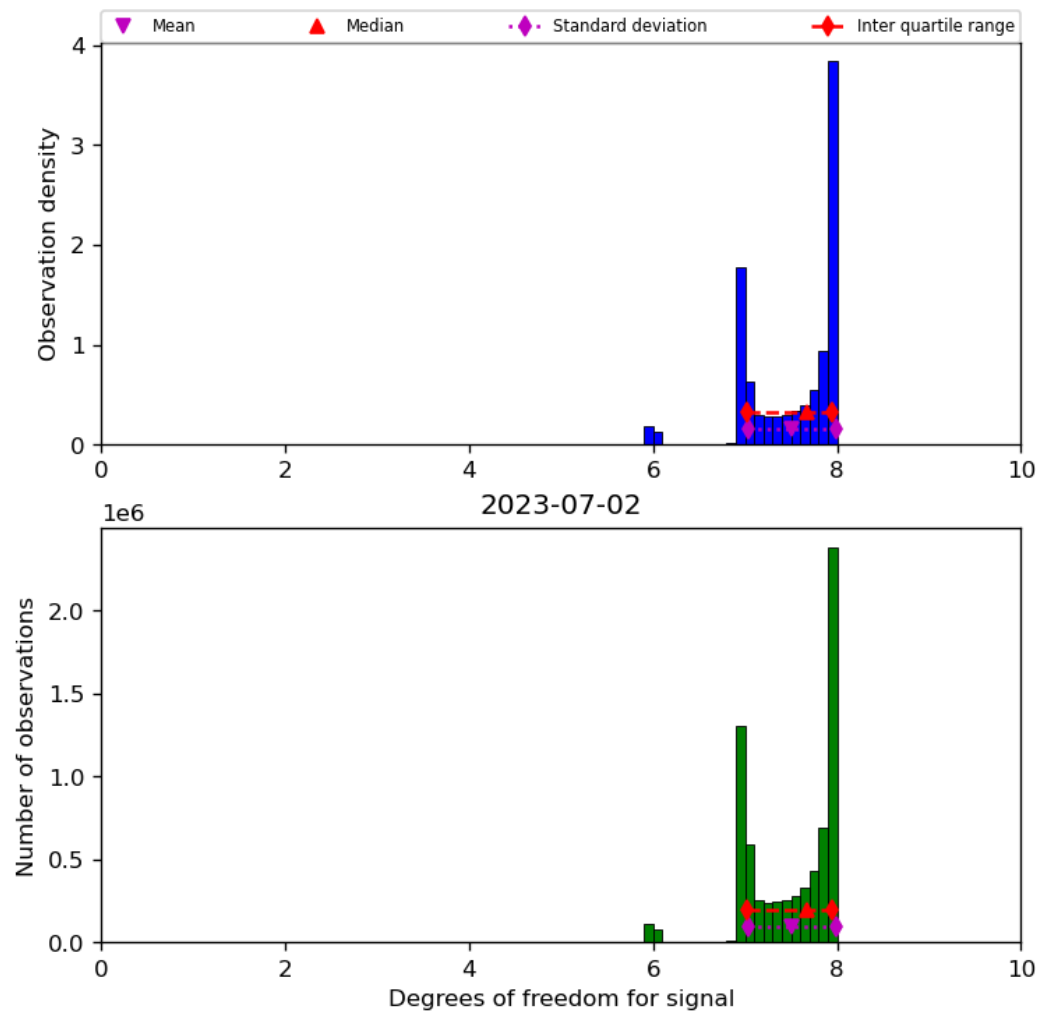
Figure 23: Histogram of “Degrees of freedom for signal” for 2023-07-01 to 2023-07-03
