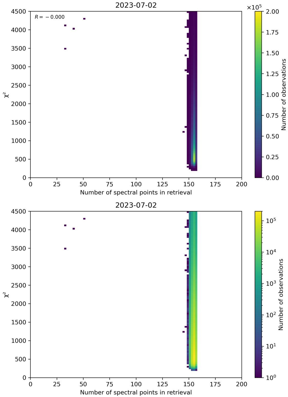
Figure 58: Scatter density plot of “Number of spectral points in retrieval” against “ \chi^2 ” for 2023-07-01 to 2023-07-03.
