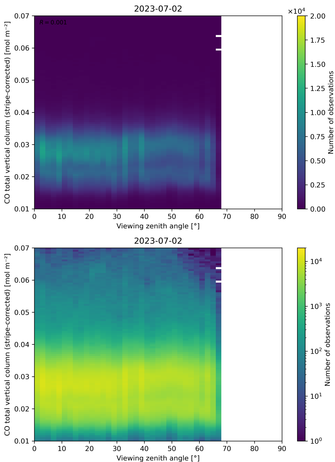
Figure 70: Scatter density plot of “Viewing zenith angle” against “CO total vertical column (stripe-corrected)” for 2023-07-01 to 2023-07-03.
