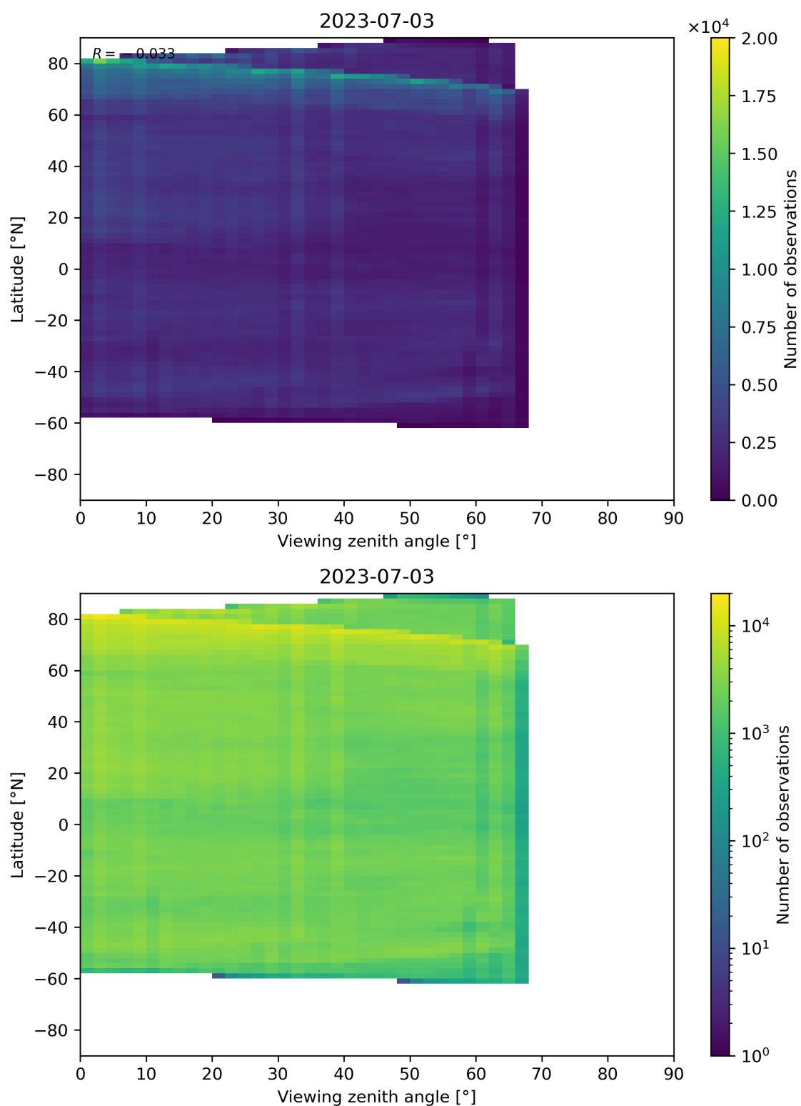
Figure 74: Scatter density plot of “Viewing zenith angle” against “Latitude” for 2023-07-03 to 2023-07-04.
