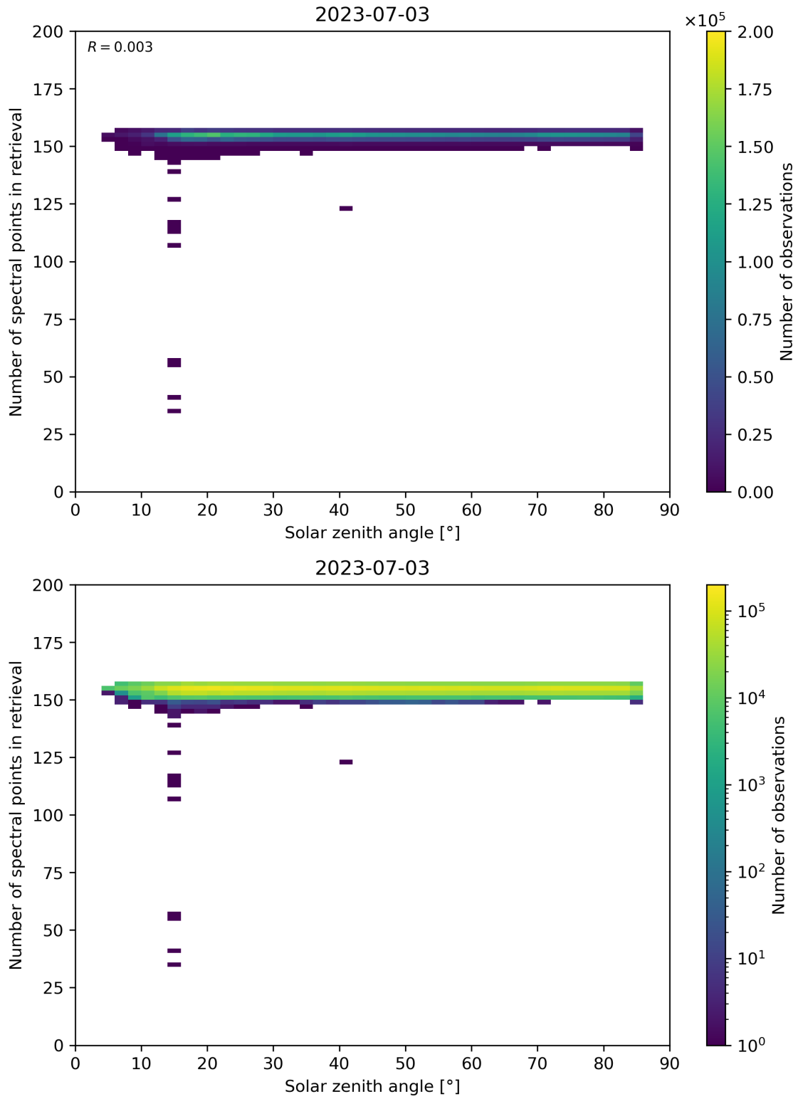
Figure 68: Scatter density plot of “Solar zenith angle” against “Number of spectral points in retrieval” for 2023-07-03 to 2023-07-04.
