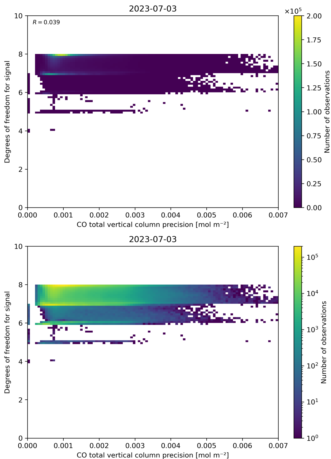
Figure 45: Scatter density plot of “CO total vertical column precision” against “Degrees of freedom for signal” for 2023-07-03 to 2023-07-04.
