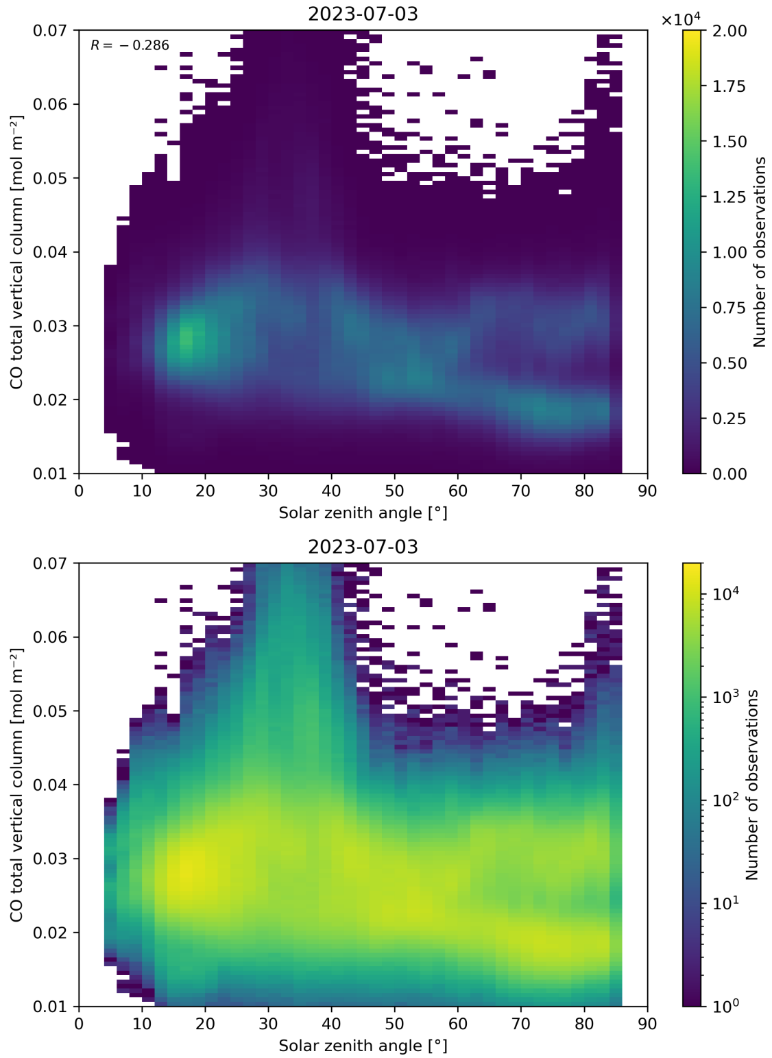
Figure 61: Scatter density plot of “Solar zenith angle” against “CO total vertical column” for 2023-07-03 to 2023-07-04.
