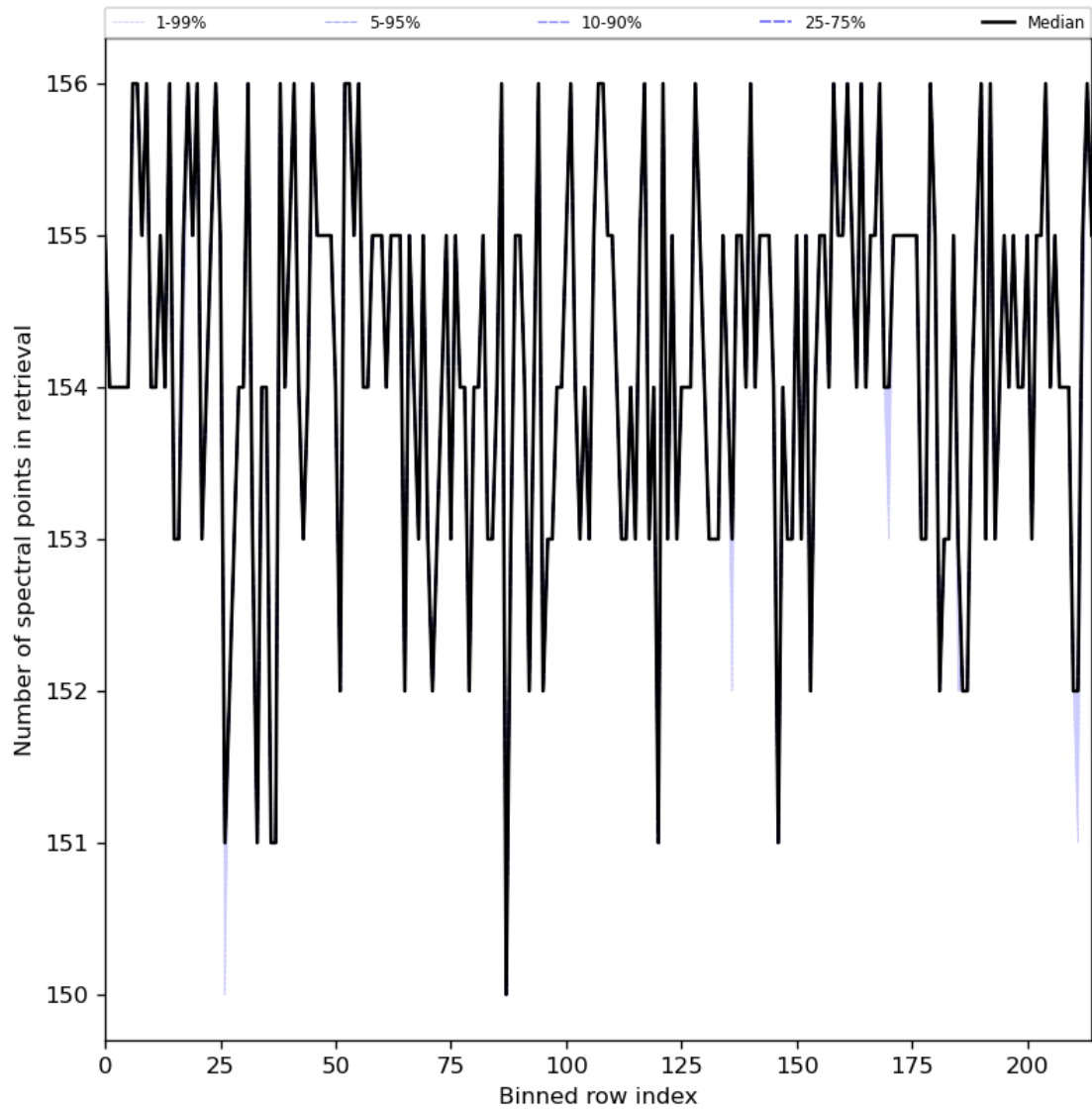
Figure 29: Along track statistics of “Number of spectral points in retrieval” for 2023-07-03 to 2023-07-04
