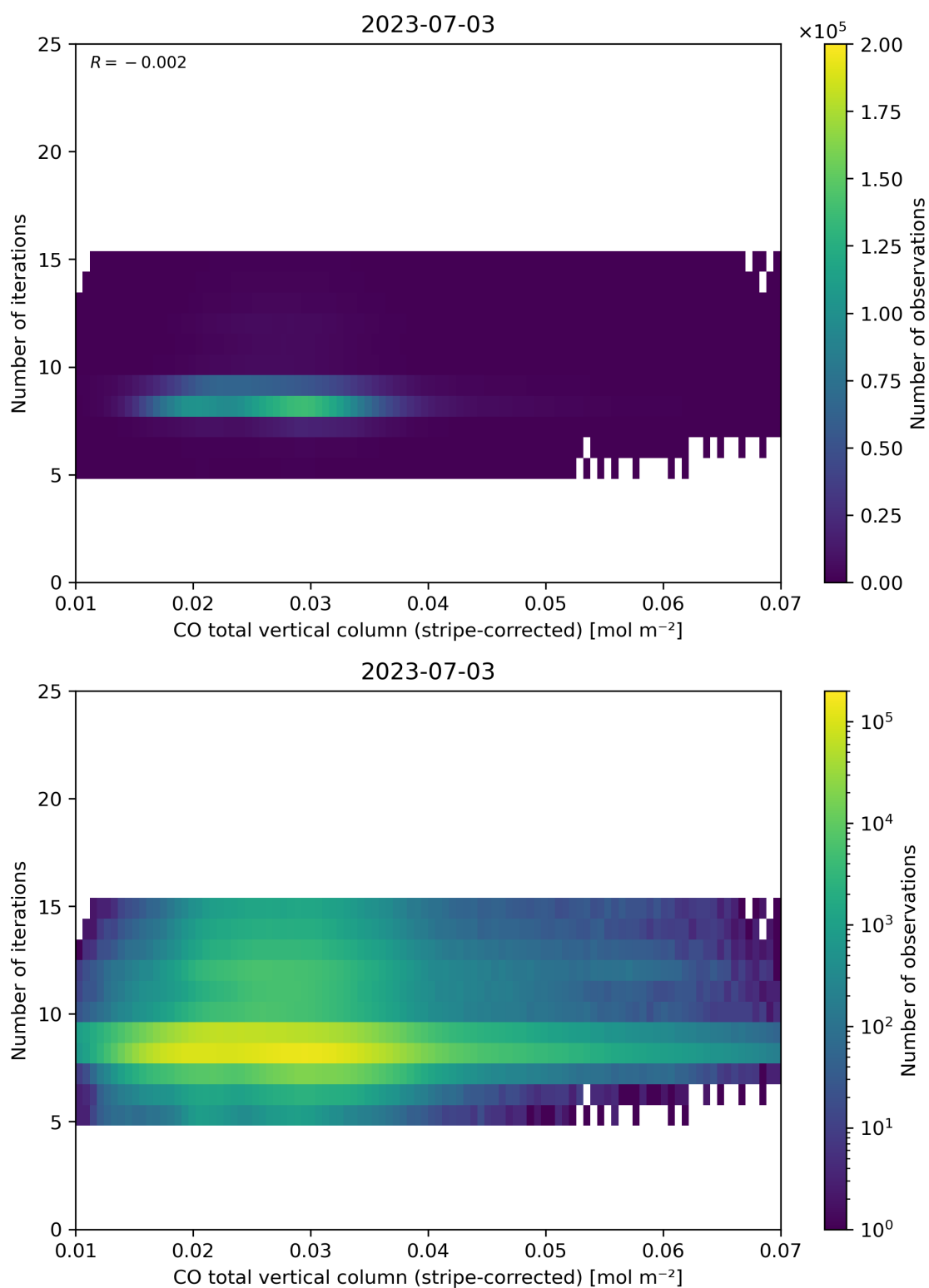
Figure 39: Scatter density plot of “CO total vertical column (stripe-corrected)” against “Number of iterations” for 2023-07-03 to 2023-07-04.
