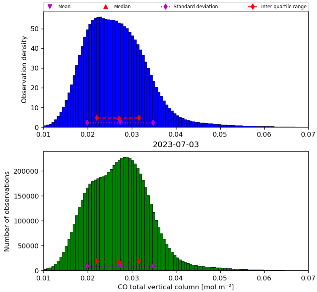
Figure 18: Histogram of “CO total vertical column” for 2023-07-03 to 2023-07-04
