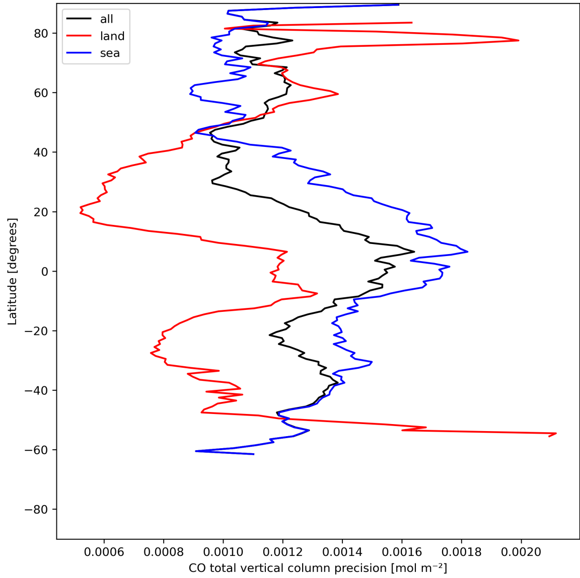
Figure 12: Zonal average of “CO total vertical column precision” for 2023-07-03 to 2023-07-04.
