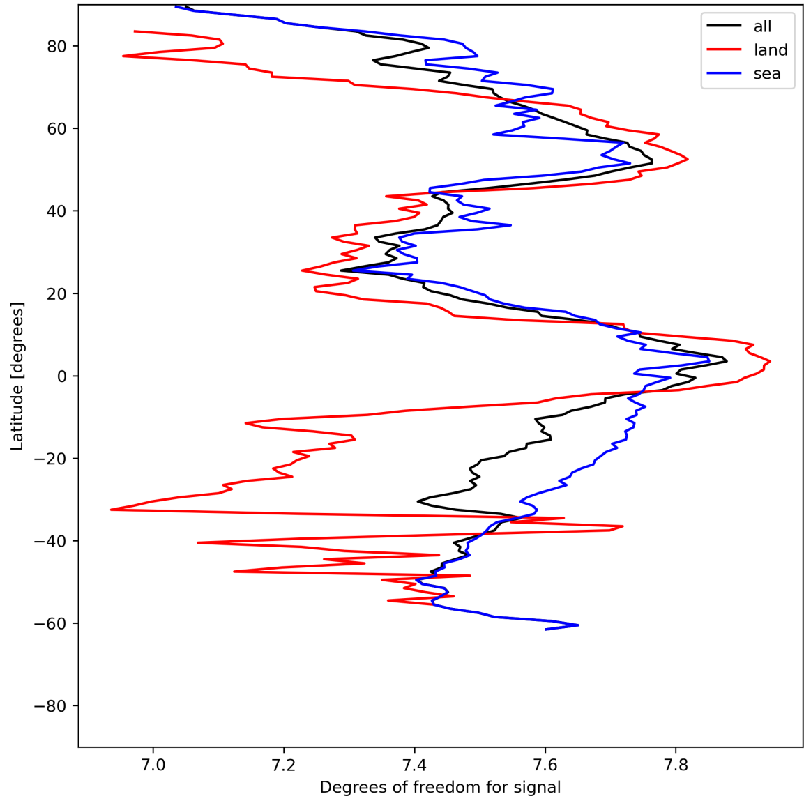
Figure 15: Zonal average of “Degrees of freedom for signal” for 2023-07-03 to 2023-07-04.
