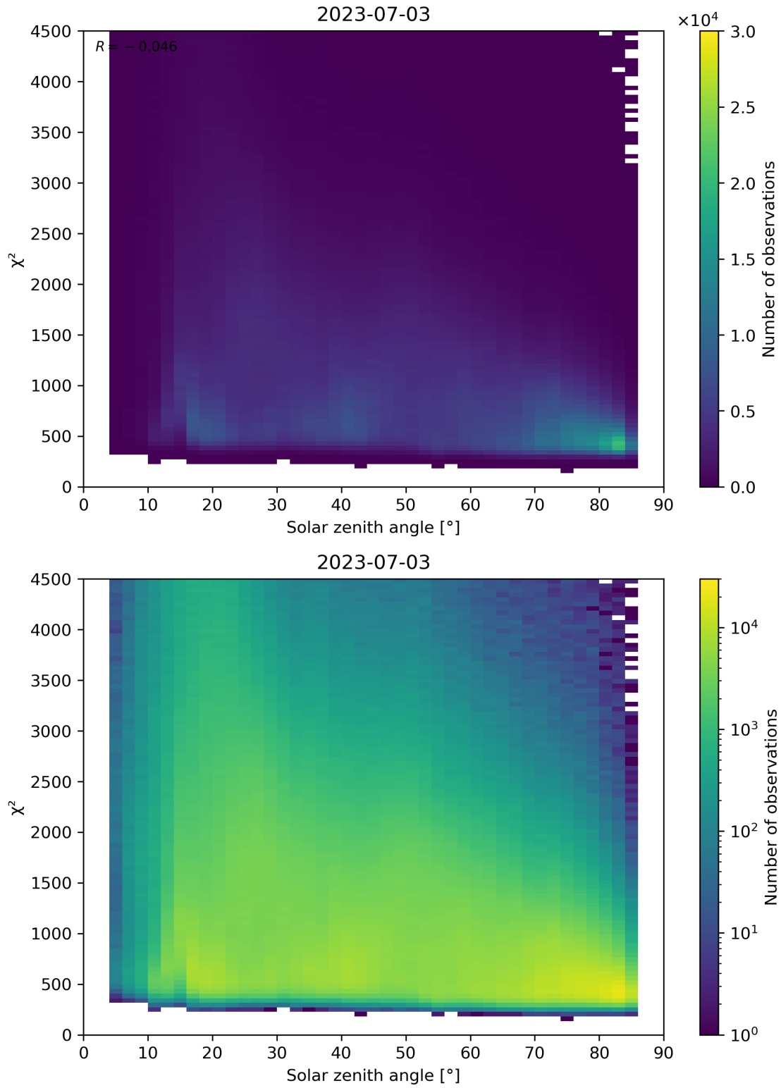
Figure 64: Scatter density plot of “Solar zenith angle” against “ \chi^2 ” for 2023-07-03 to 2023-07-04.
