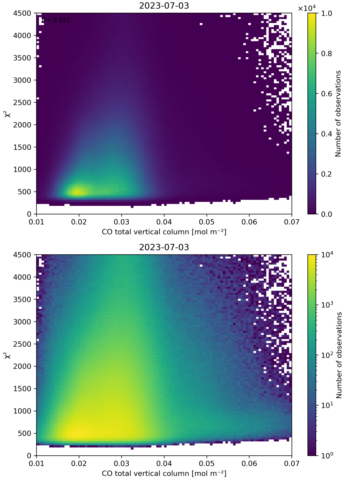
Figure 35: Scatter density plot of “CO total vertical column” against “ \chi^2 ” for 2023-07-03 to 2023-07-04.
