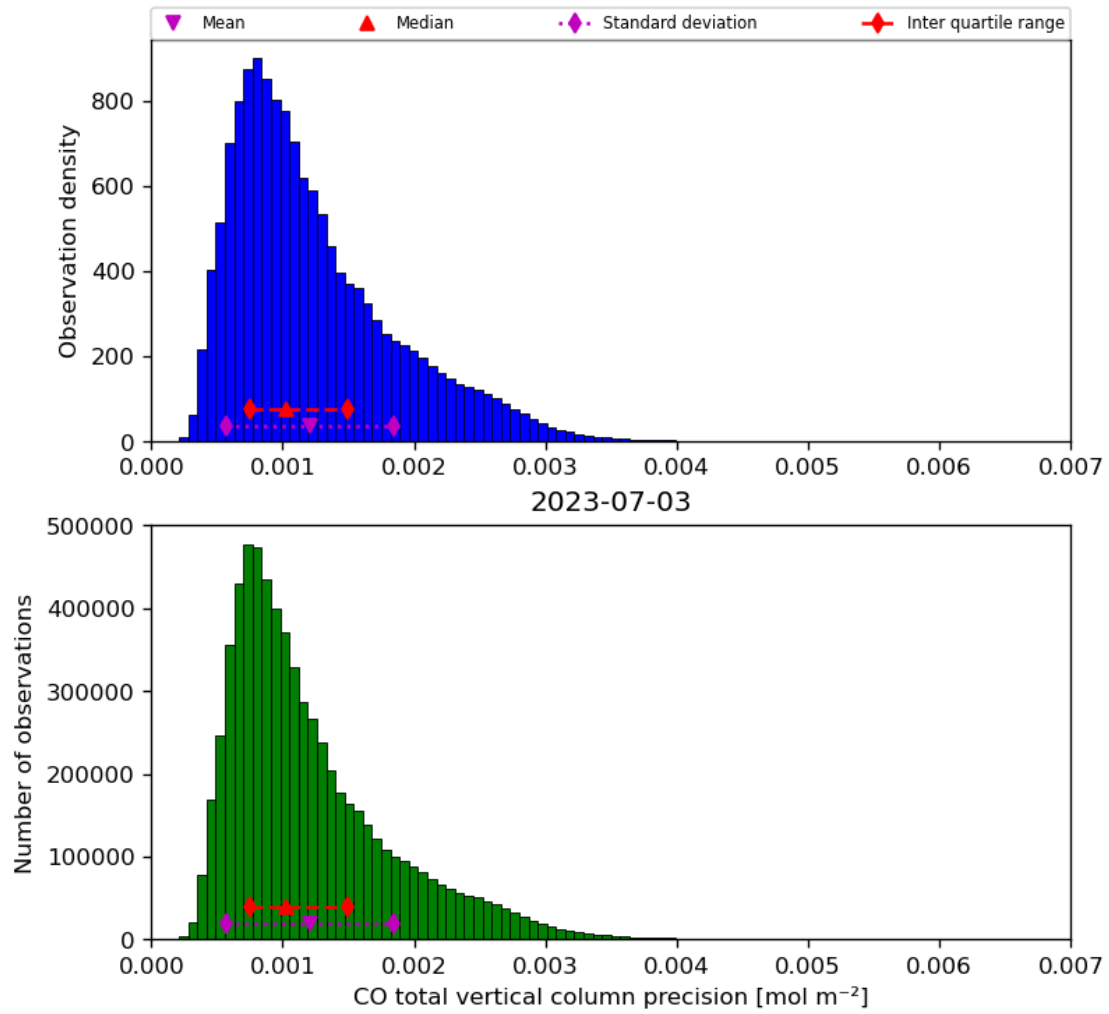
Figure 20: Histogram of “CO total vertical column precision” for 2023-07-03 to 2023-07-04
