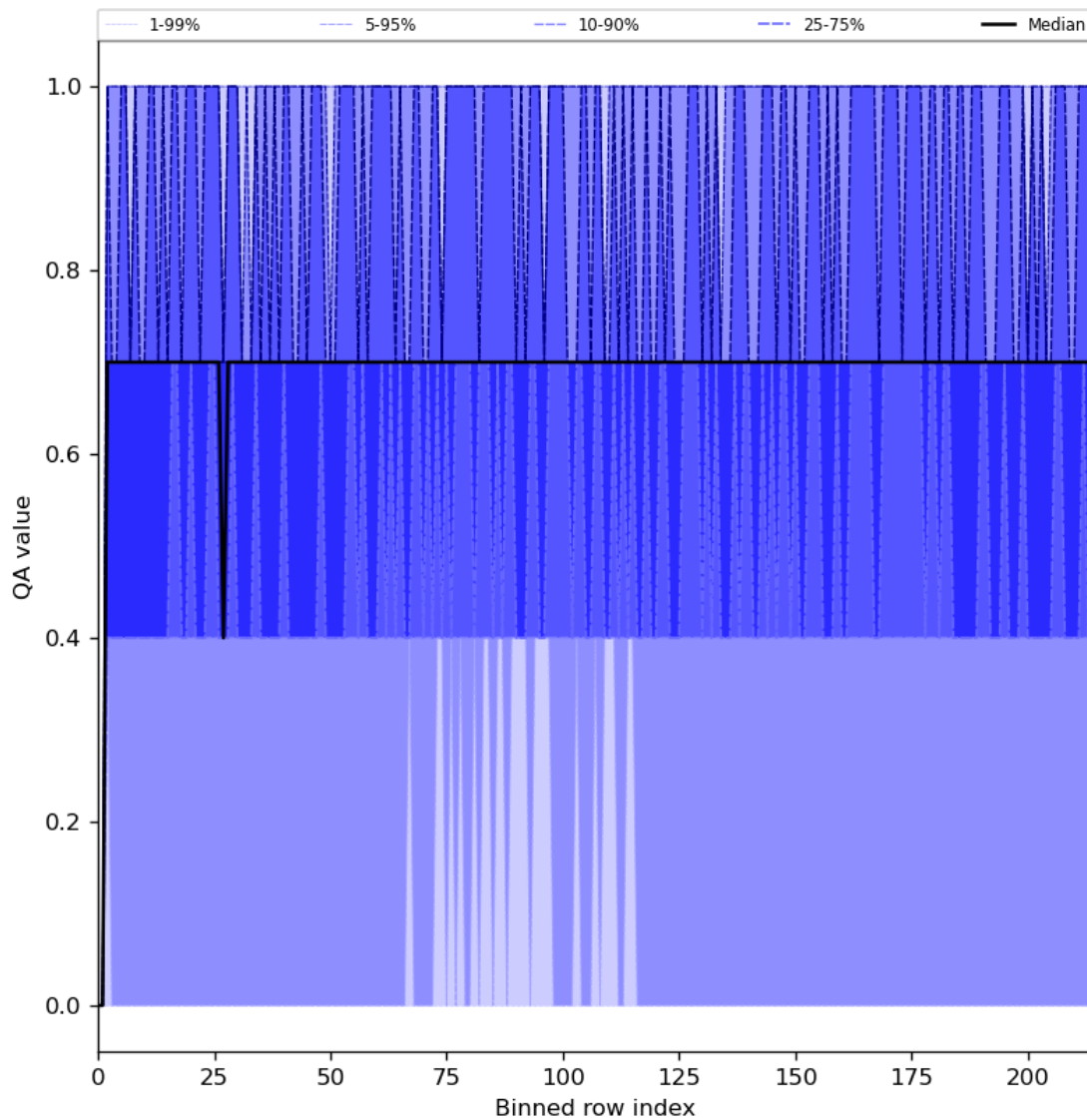
Figure 25: Along track statistics of “QA value” for 2023-07-03 to 2023-07-04
