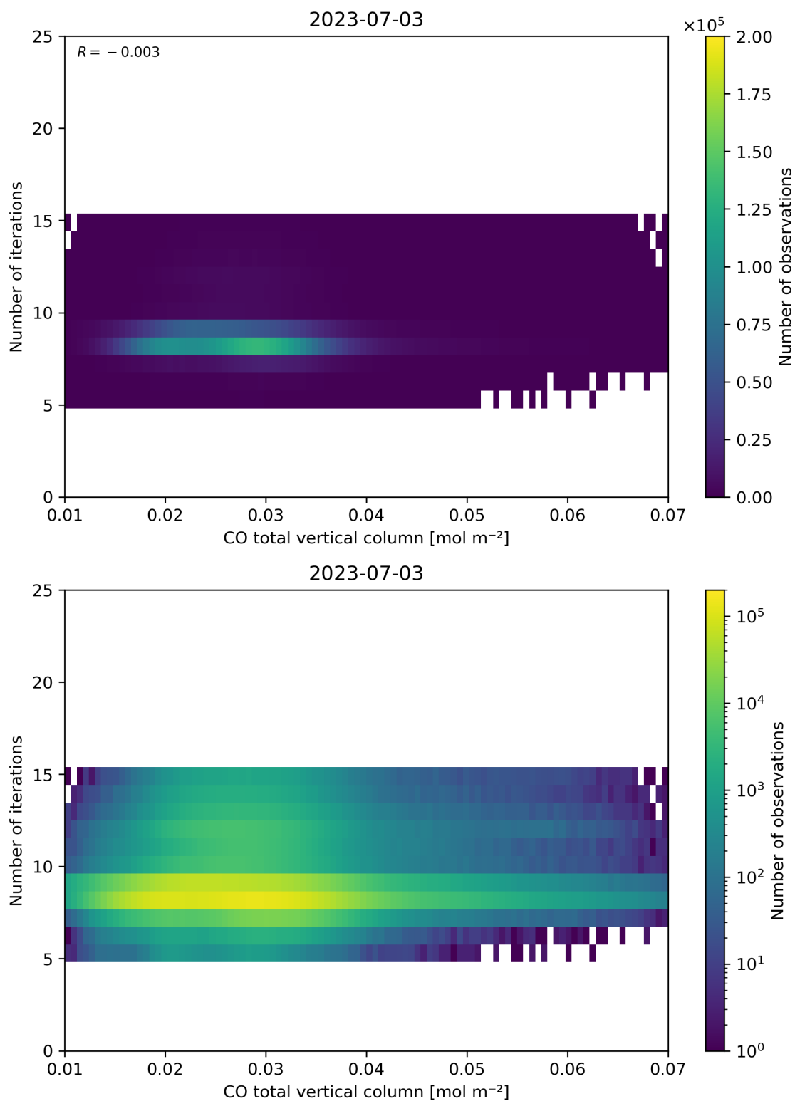
Figure 42: Scatter density plot of “CO total vertical column” against “Number of iterations” for 2023-07-03 to 2023-07-04.
