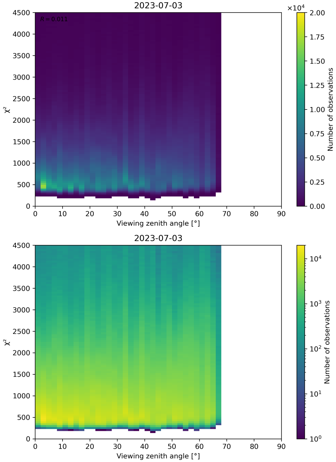
Figure 72: Scatter density plot of “Viewing zenith angle” against “ \chi^2 ” for 2023-07-03 to 2023-07-04.
