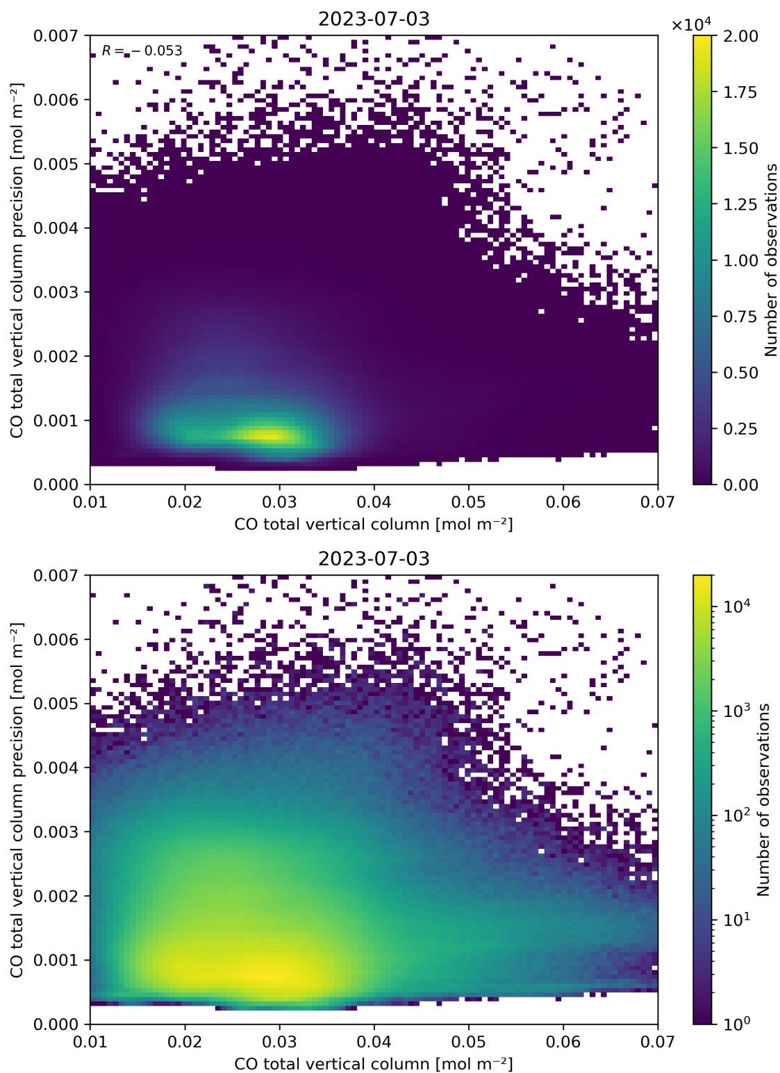
Figure 34: Scatter density plot of “CO total vertical column” against “CO total vertical column precision” for 2023-07-03 to 2023-07-04.
