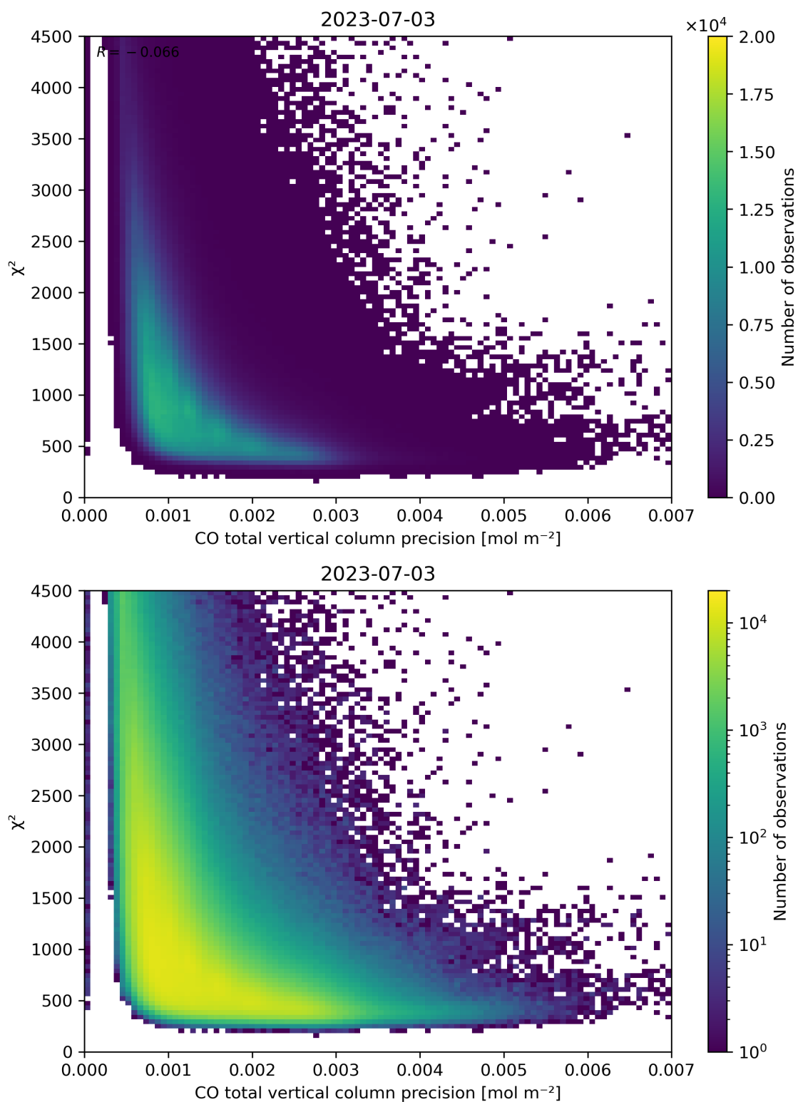
Figure 44: Scatter density plot of “CO total vertical column precision” against “ \chi^2 ” for 2023-07-03 to 2023-07-04.
