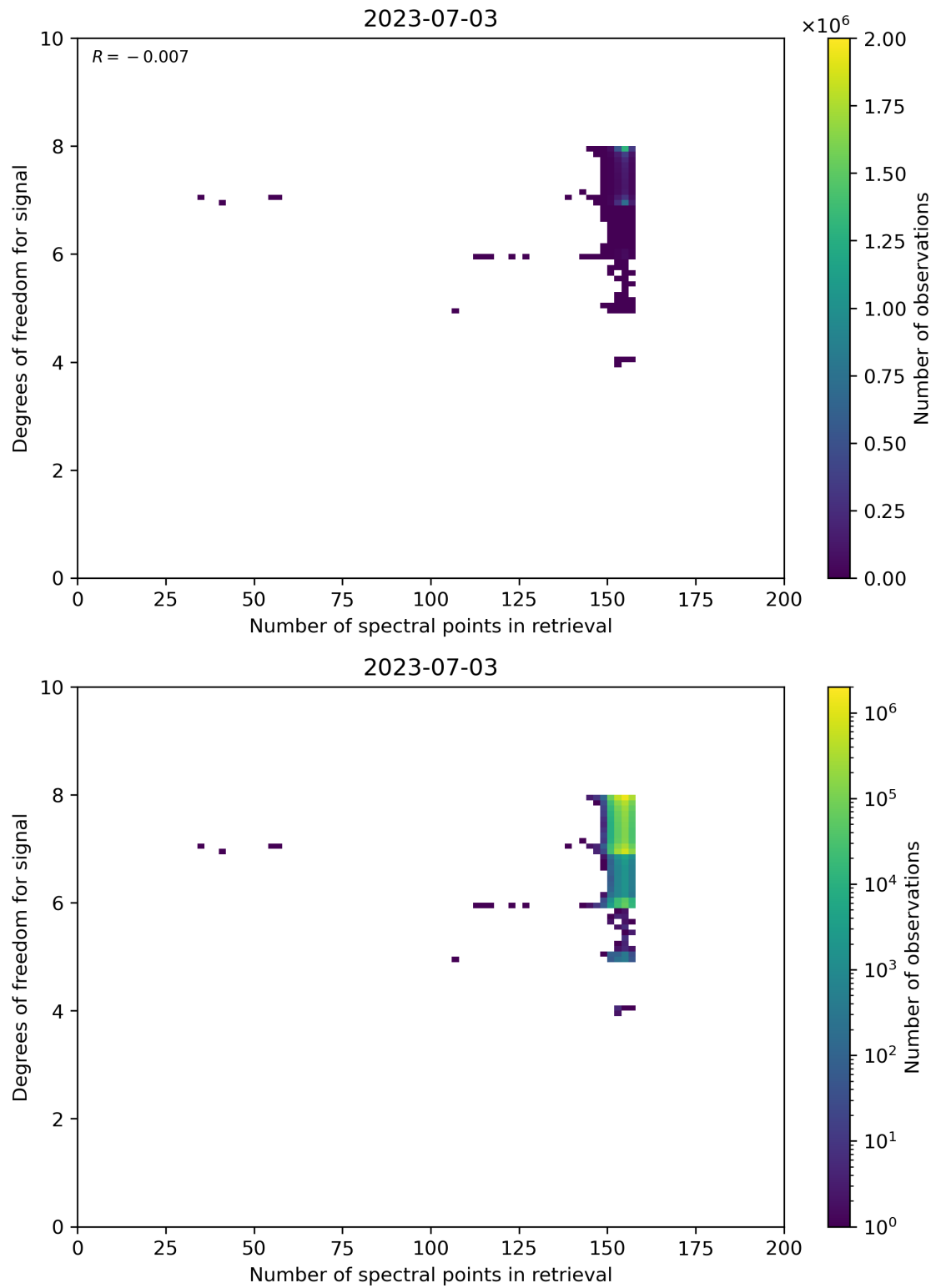
Figure 59: Scatter density plot of “Number of spectral points in retrieval” against “Degrees of freedom for signal” for 2023-07-03 to 2023-07-04.
