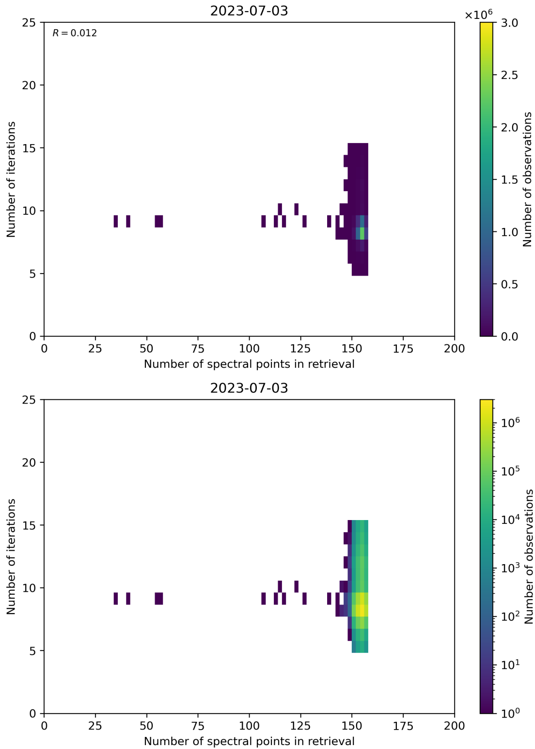
Figure 60: Scatter density plot of “Number of spectral points in retrieval” against “Number of iterations” for 2023-07-03 to 2023-07-04.
