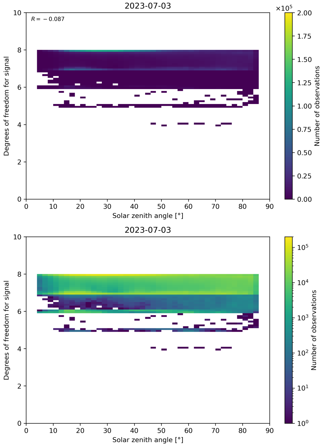
Figure 65: Scatter density plot of “Solar zenith angle” against “Degrees of freedom for signal” for 2023-07-03 to 2023-07-04.
