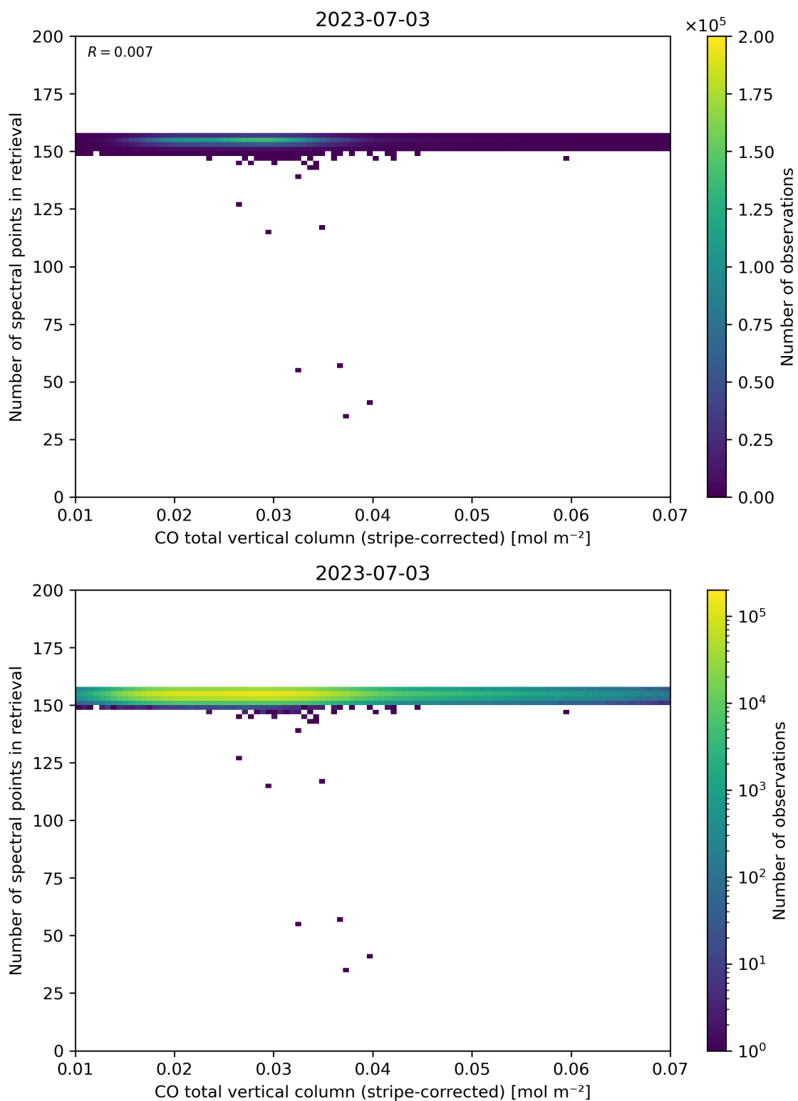
Figure 40: Scatter density plot of “CO total vertical column (stripe-corrected)” against “Number of spectral points in retrieval” for 2023-07-03 to 2023-07-04.
