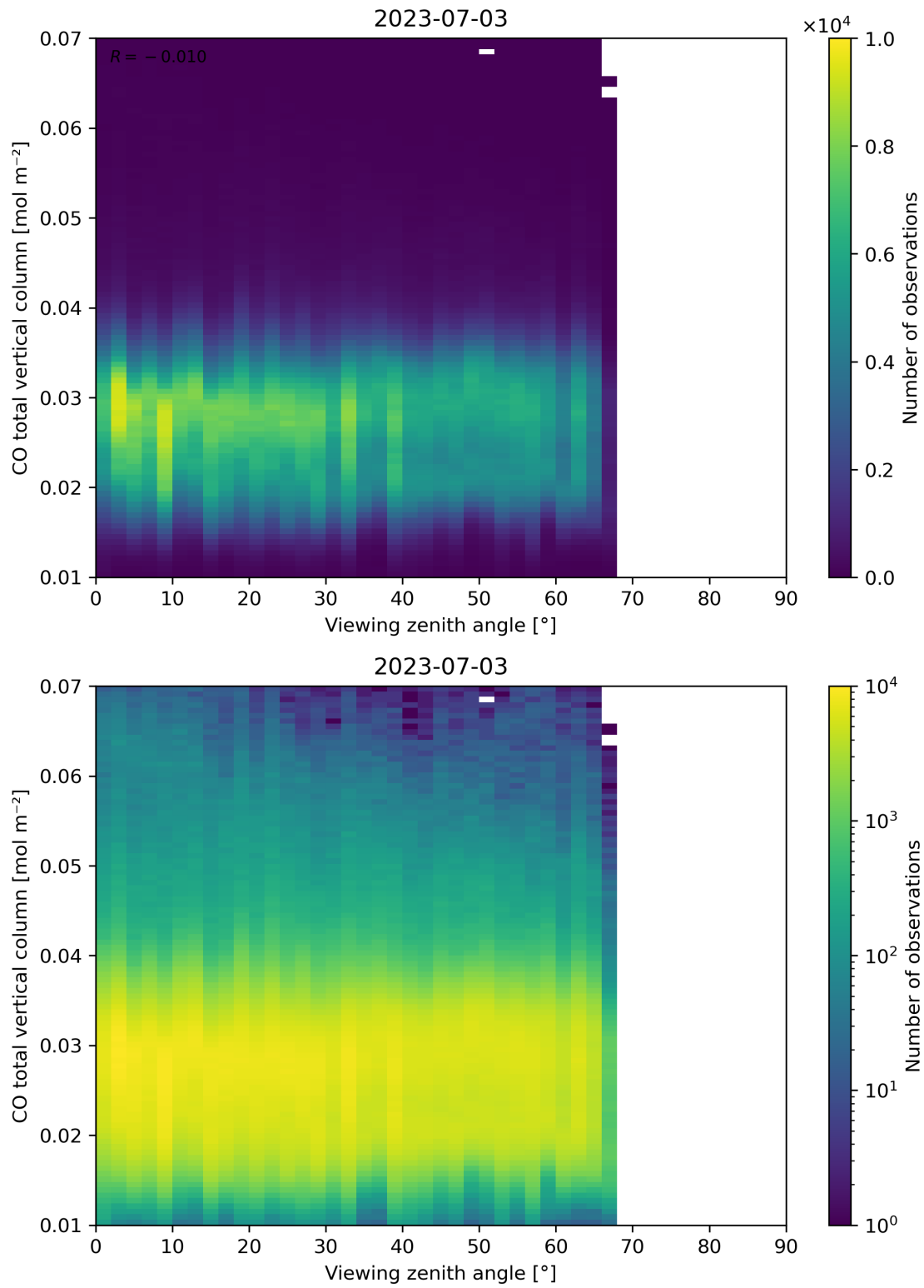
Figure 69: Scatter density plot of “Viewing zenith angle” against “CO total vertical column” for 2023-07-03 to 2023-07-04.
