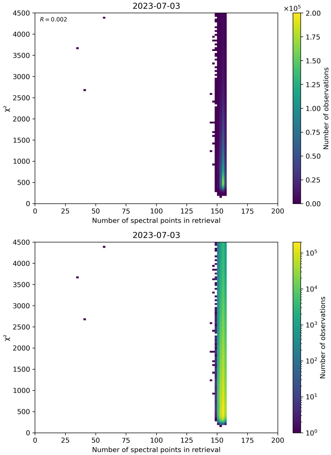
Figure 58: Scatter density plot of “Number of spectral points in retrieval” against “ \chi^2 ” for 2023-07-03 to 2023-07-04.
