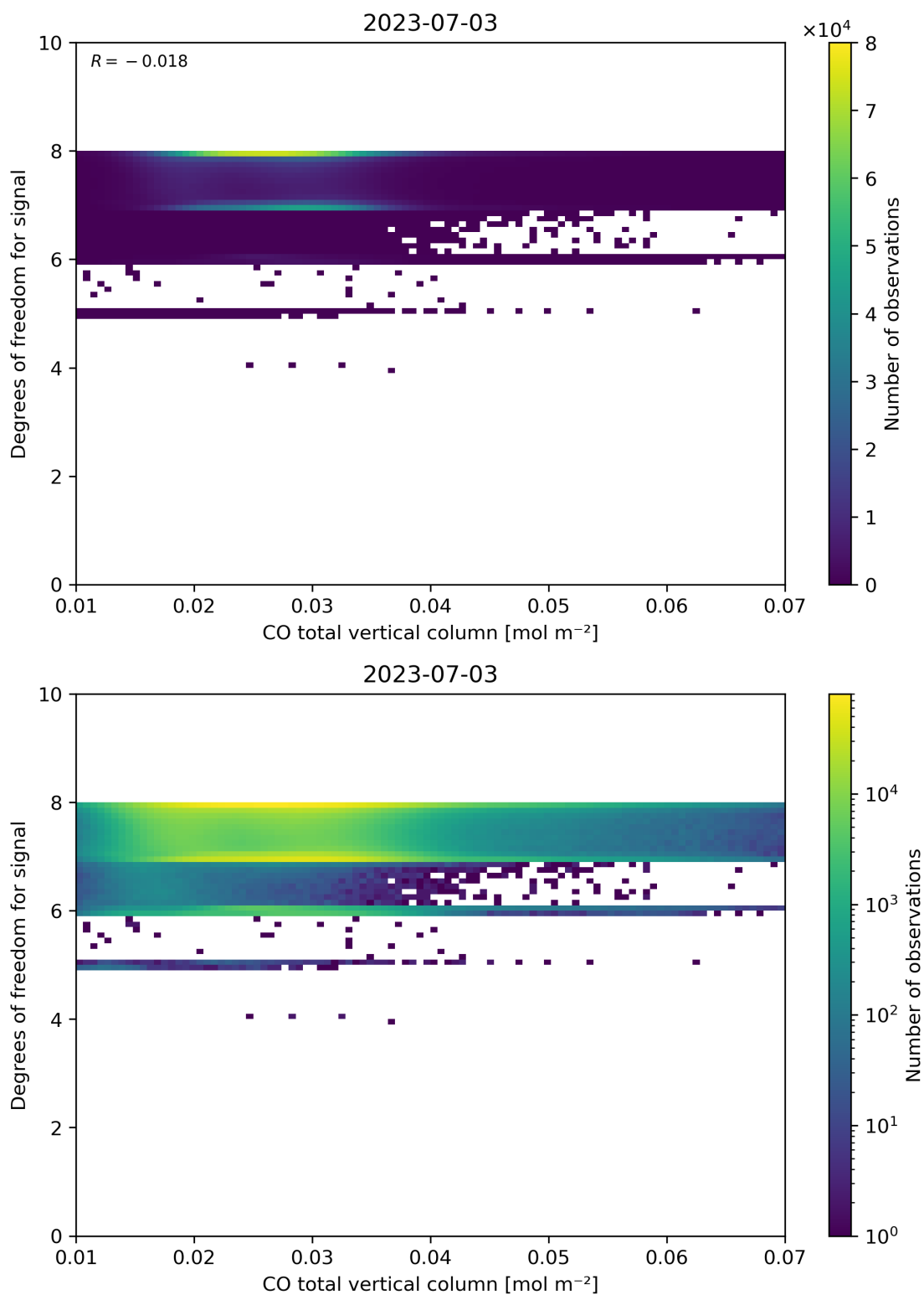
Figure 41: Scatter density plot of “CO total vertical column” against “Degrees of freedom for signal” for 2023-07-03 to 2023-07-04.
