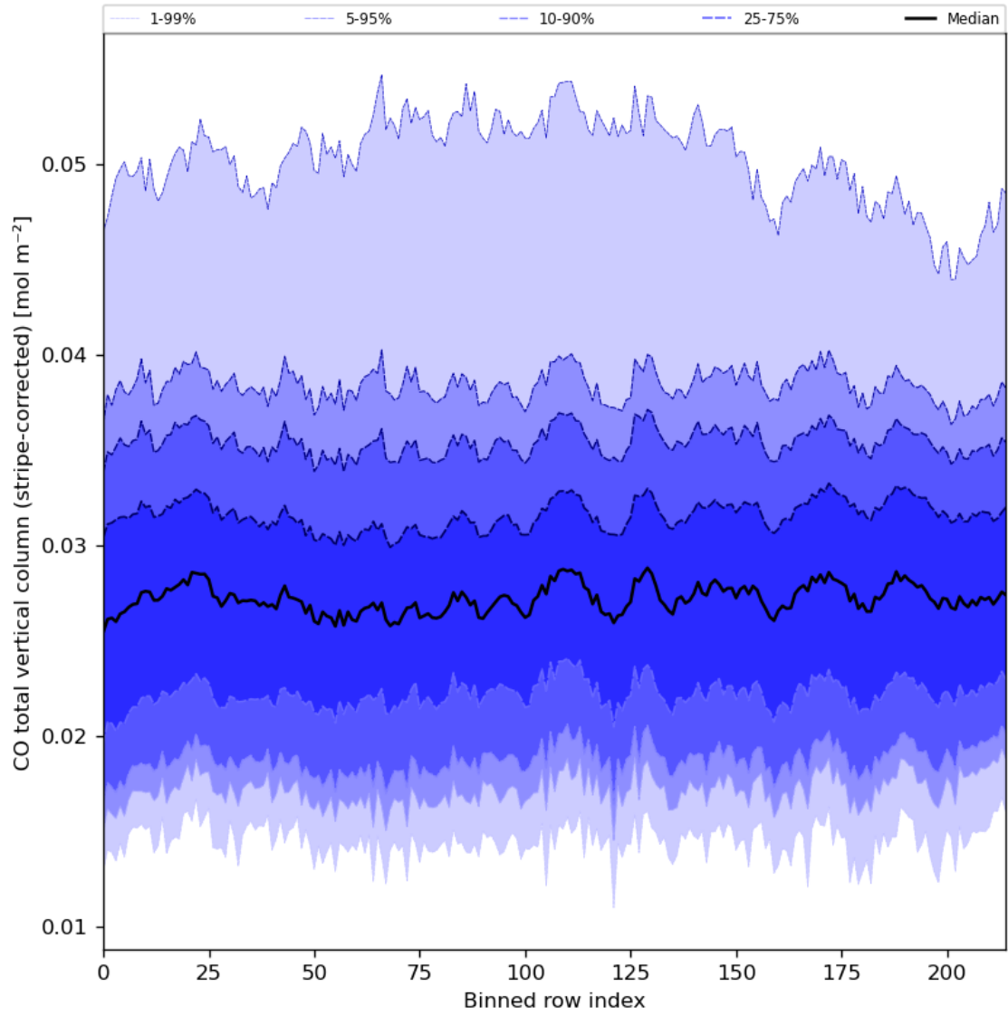
Figure 27: Along track statistics of “CO total vertical column (stripe-corrected)” for 2023-07-03 to 2023-07-04
