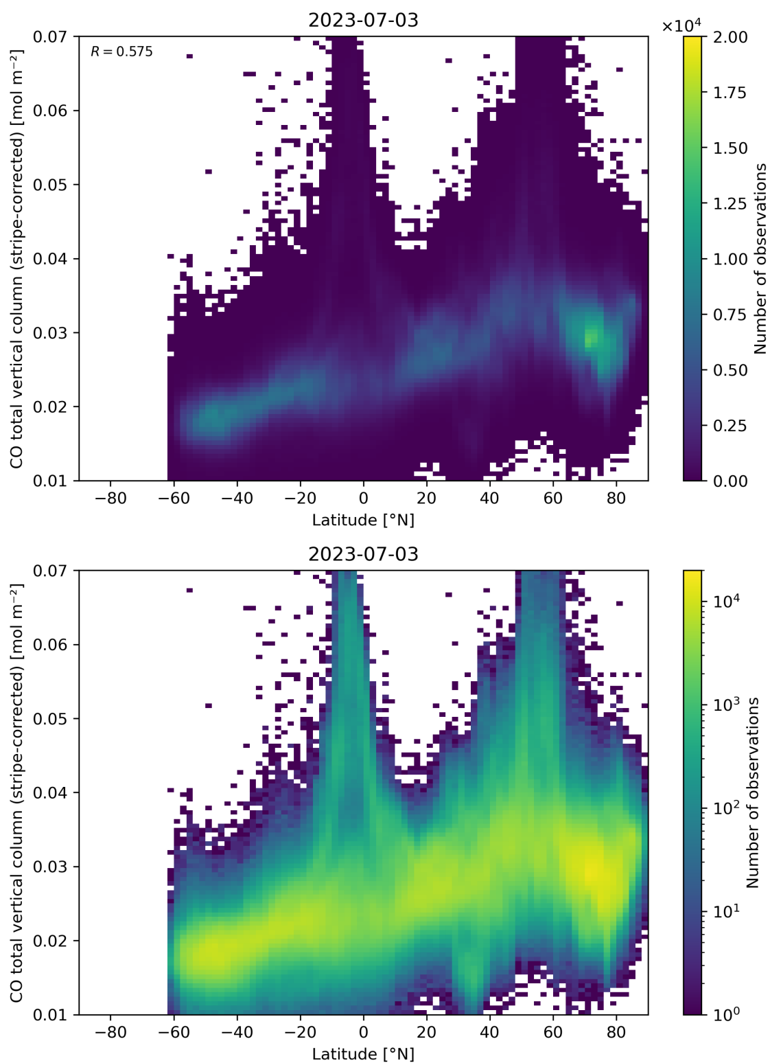
Figure 52: Scatter density plot of “Latitude” against “CO total vertical column (stripe-corrected)” for 2023-07-03 to 2023-07-04.
