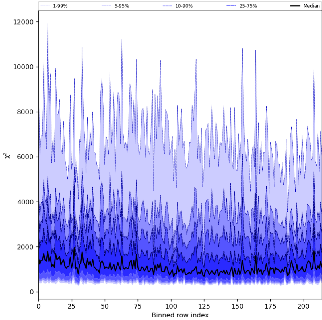
Figure 30: Along track statistics of “ \chi^2 ” for 2023-07-03 to 2023-07-04
