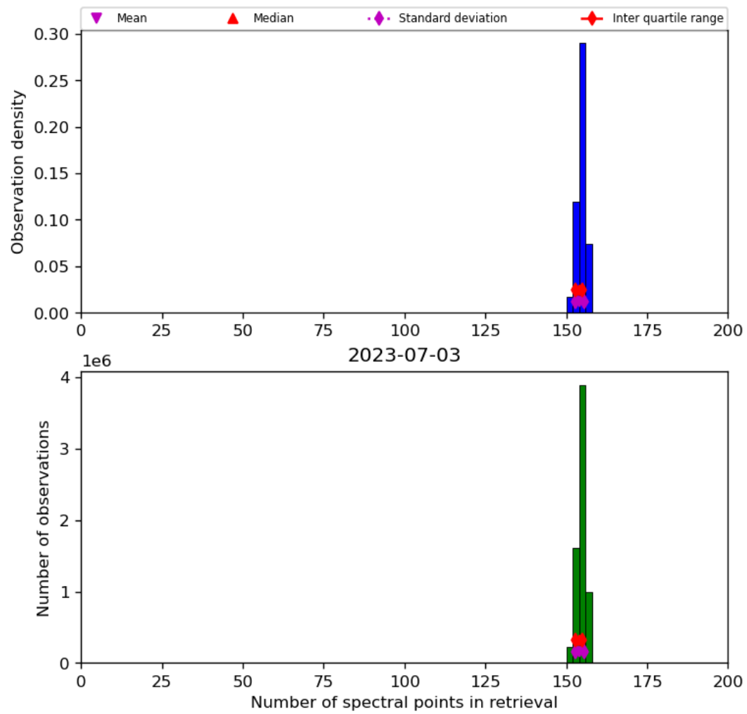
Figure 21: Histogram of “Number of spectral points in retrieval” for 2023-07-03 to 2023-07-04
