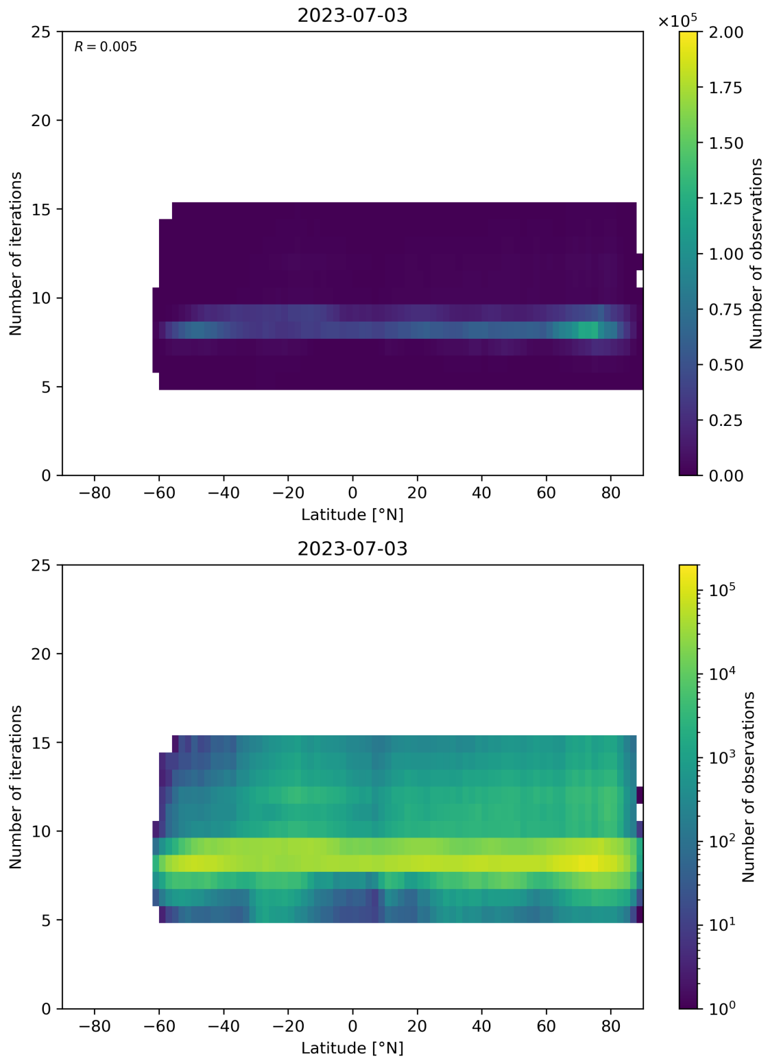
Figure 56: Scatter density plot of “Latitude” against “Number of iterations” for 2023-07-03 to 2023-07-04.
