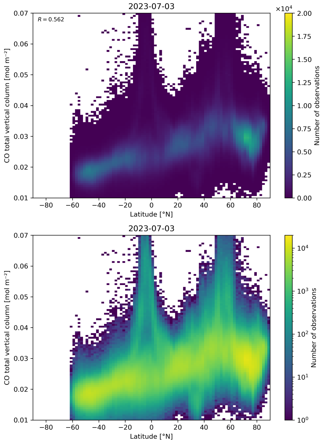
Figure 51: Scatter density plot of “Latitude” against “CO total vertical column” for 2023-07-03 to 2023-07-04.
