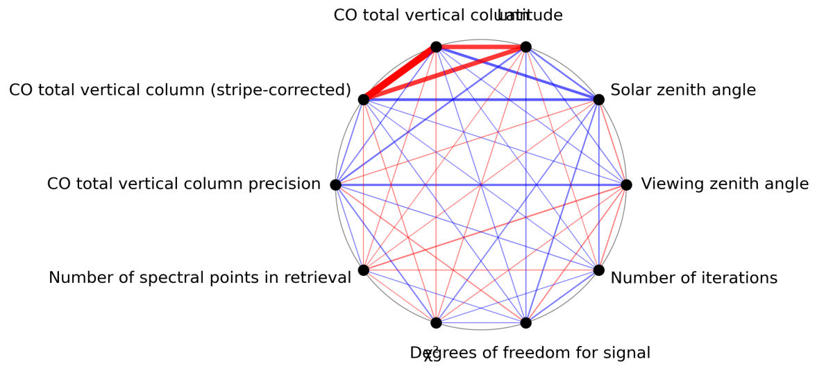
Figure 1: Map of correlation graph for 2023-07-03 to 2023-07-04.
