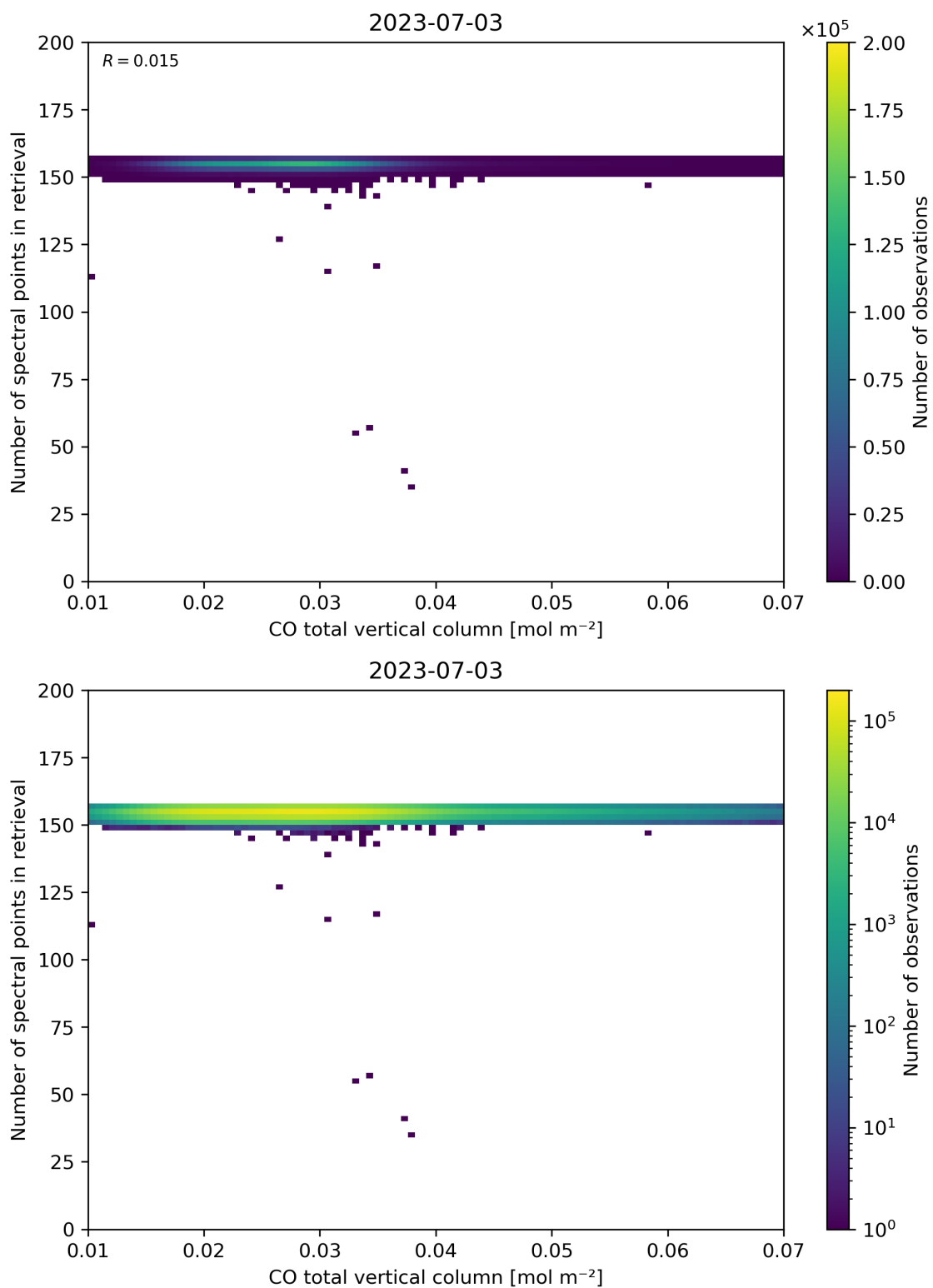
Figure 43: Scatter density plot of “CO total vertical column” against “Number of spectral points in retrieval” for 2023-07-03 to 2023-07-04.
