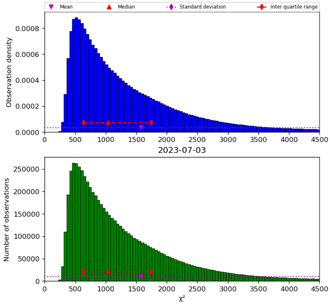
Figure 22: Histogram of " \chi^2 " for 2023-07-03 to 2023-07-04
