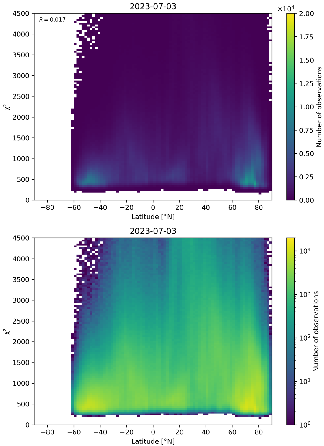
Figure 54: Scatter density plot of “Latitude” against “ \chi^2 ” for 2023-07-03 to 2023-07-04.
