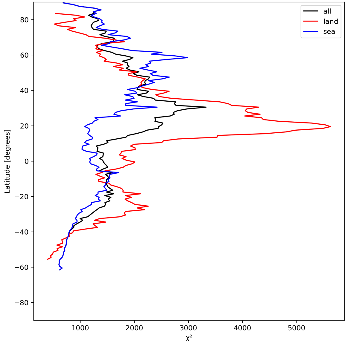
Figure 14: Zonal average of “ \chi^2 ” for 2023-07-03 to 2023-07-04.
