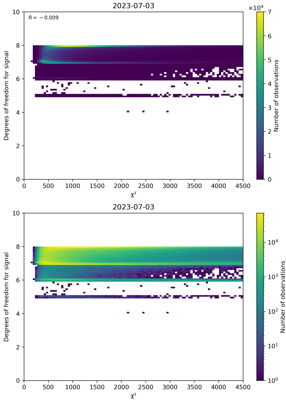
Figure 48: Scatter density plot of " \chi^2 " against "Degrees of freedom for signal" for 2023-07-03 to 2023-07-04.
