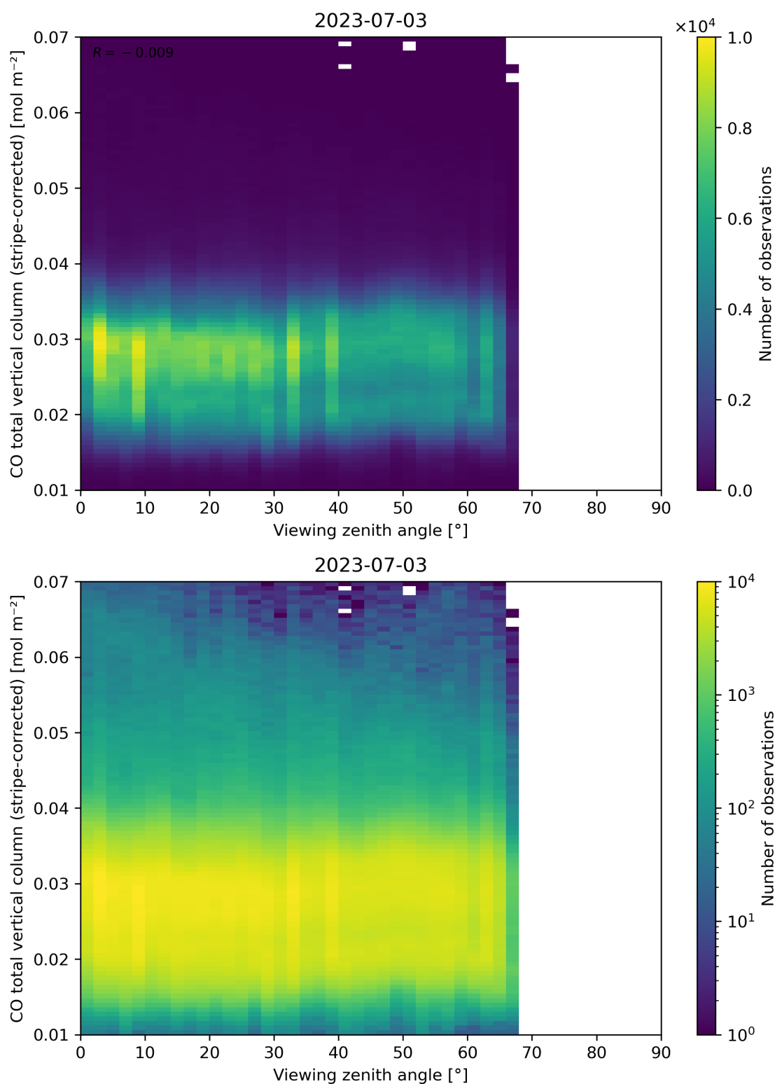
Figure 70: Scatter density plot of “Viewing zenith angle” against “CO total vertical column (stripe-corrected)” for 2023-07-03 to 2023-07-04.
