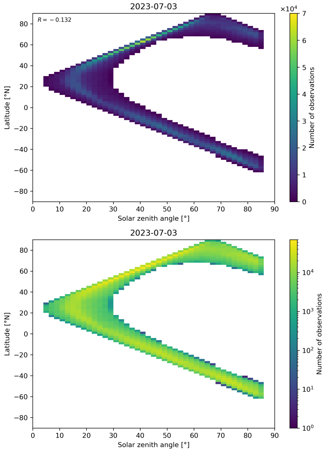
Figure 66: Scatter density plot of “Solar zenith angle” against “Latitude” for 2023-07-03 to 2023-07-04.
