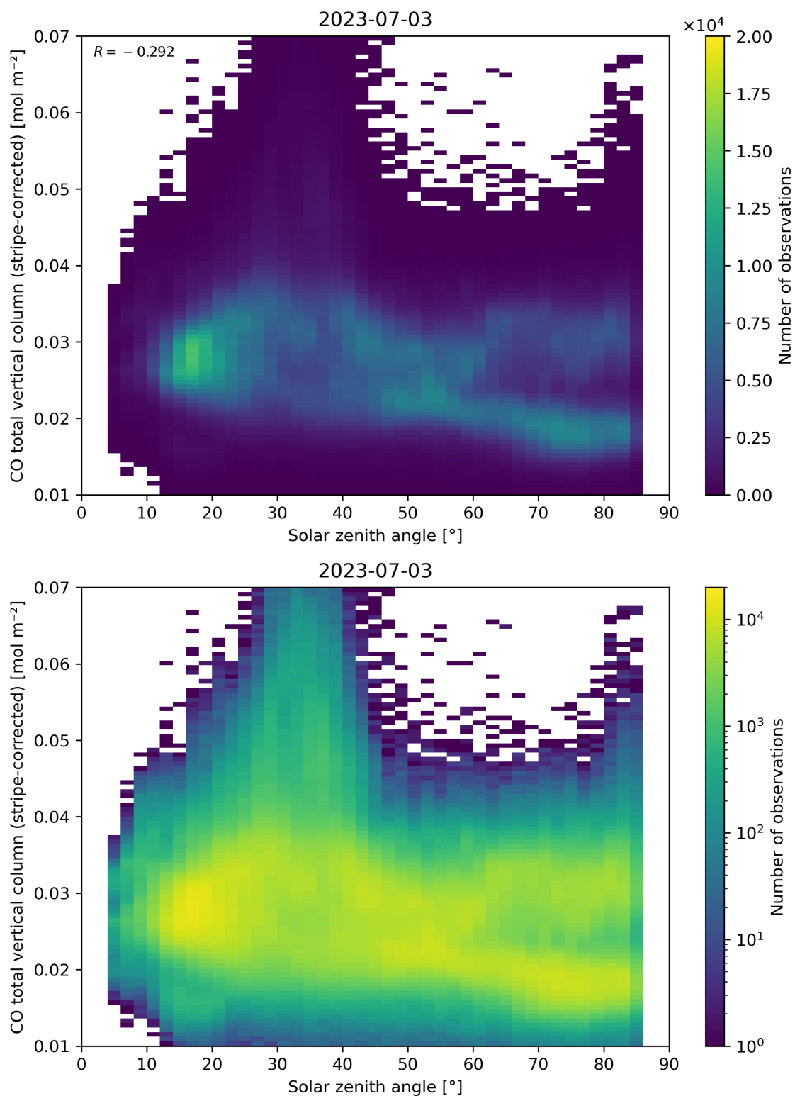
Figure 62: Scatter density plot of “Solar zenith angle” against “CO total vertical column (stripe-corrected)” for 2023-07-03 to 2023-07-04.
