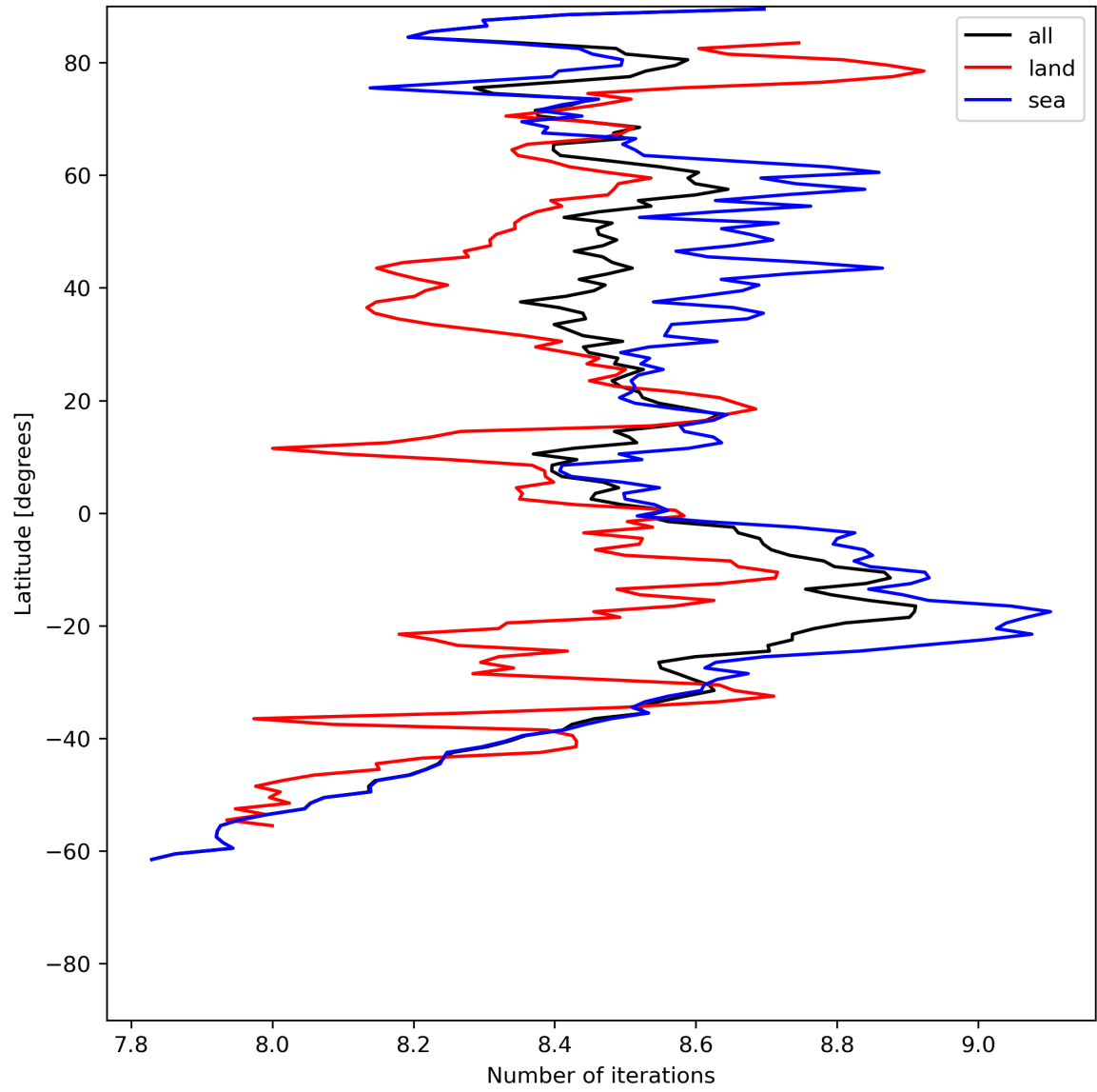
Figure 16: Zonal average of “Number of iterations” for 2023-07-03 to 2023-07-04.
