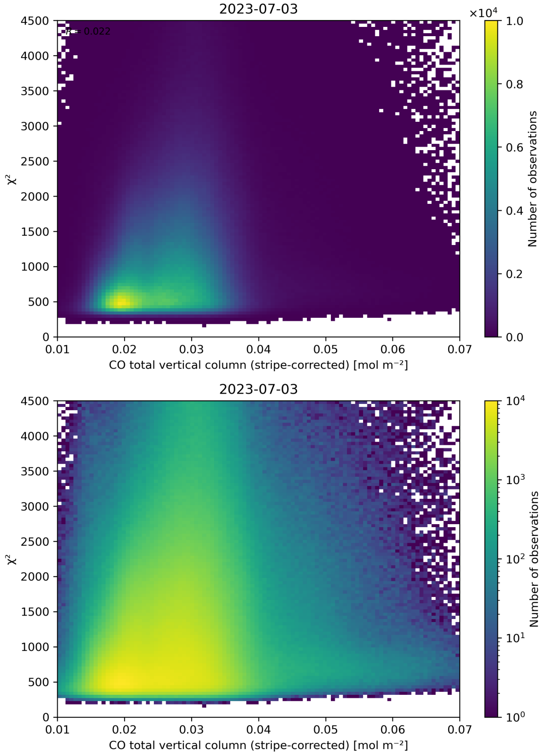
Figure 37: Scatter density plot of “CO total vertical column (stripe-corrected)” against “ \chi^2 ” for 2023-07-03 to 2023-07-04.
