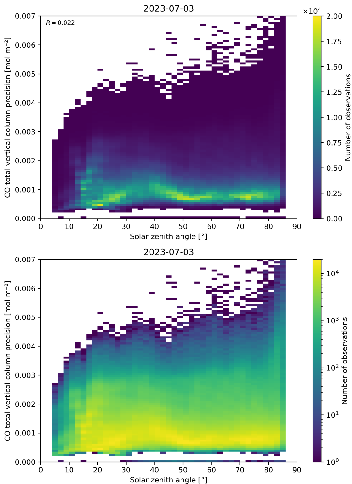
Figure 63: Scatter density plot of “Solar zenith angle” against “CO total vertical column precision” for 2023-07-03 to 2023-07-04.
