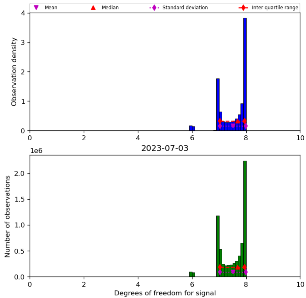
Figure 23: Histogram of “Degrees of freedom for signal” for 2023-07-03 to 2023-07-04
