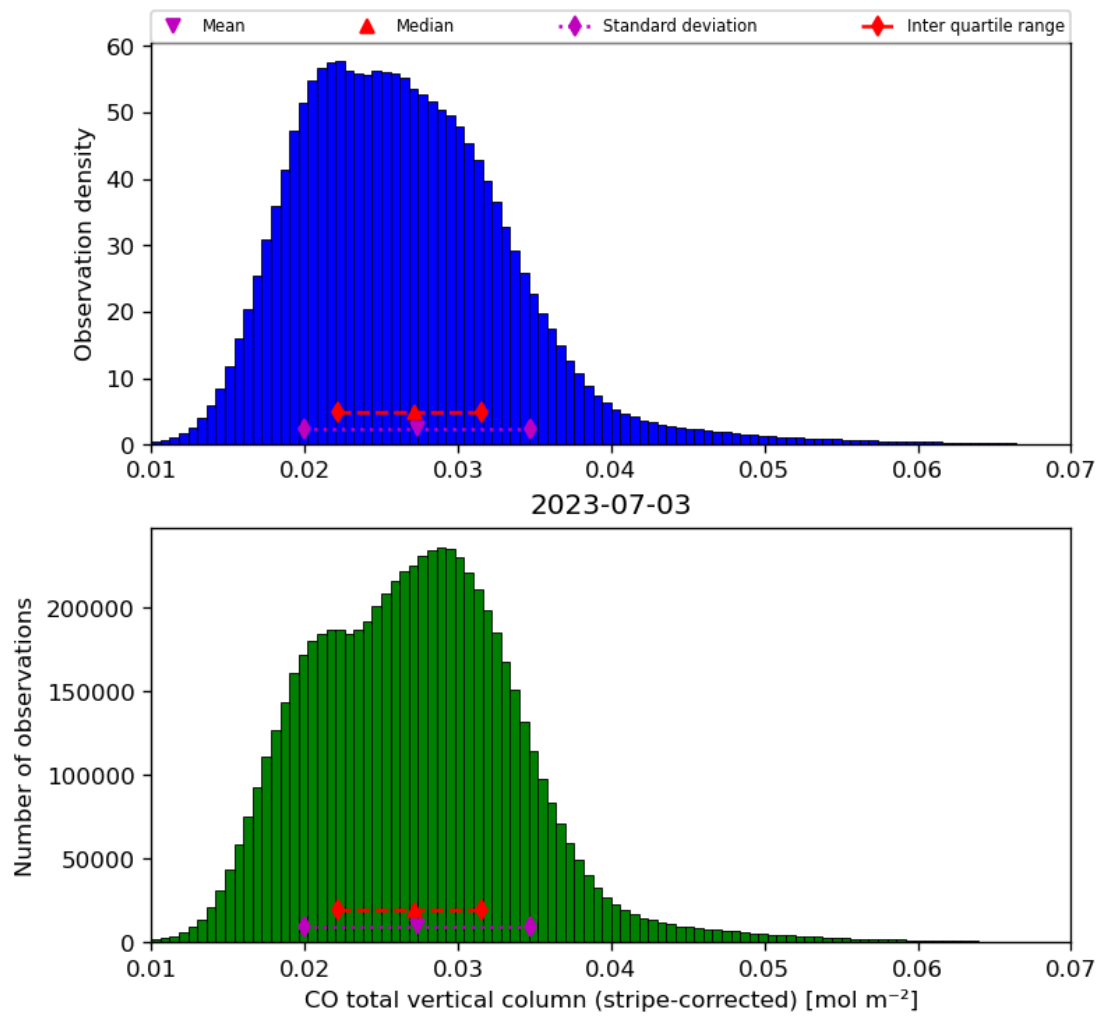
Figure 19: Histogram of “CO total vertical column (stripe-corrected)” for 2023-07-03 to 2023-07-04
