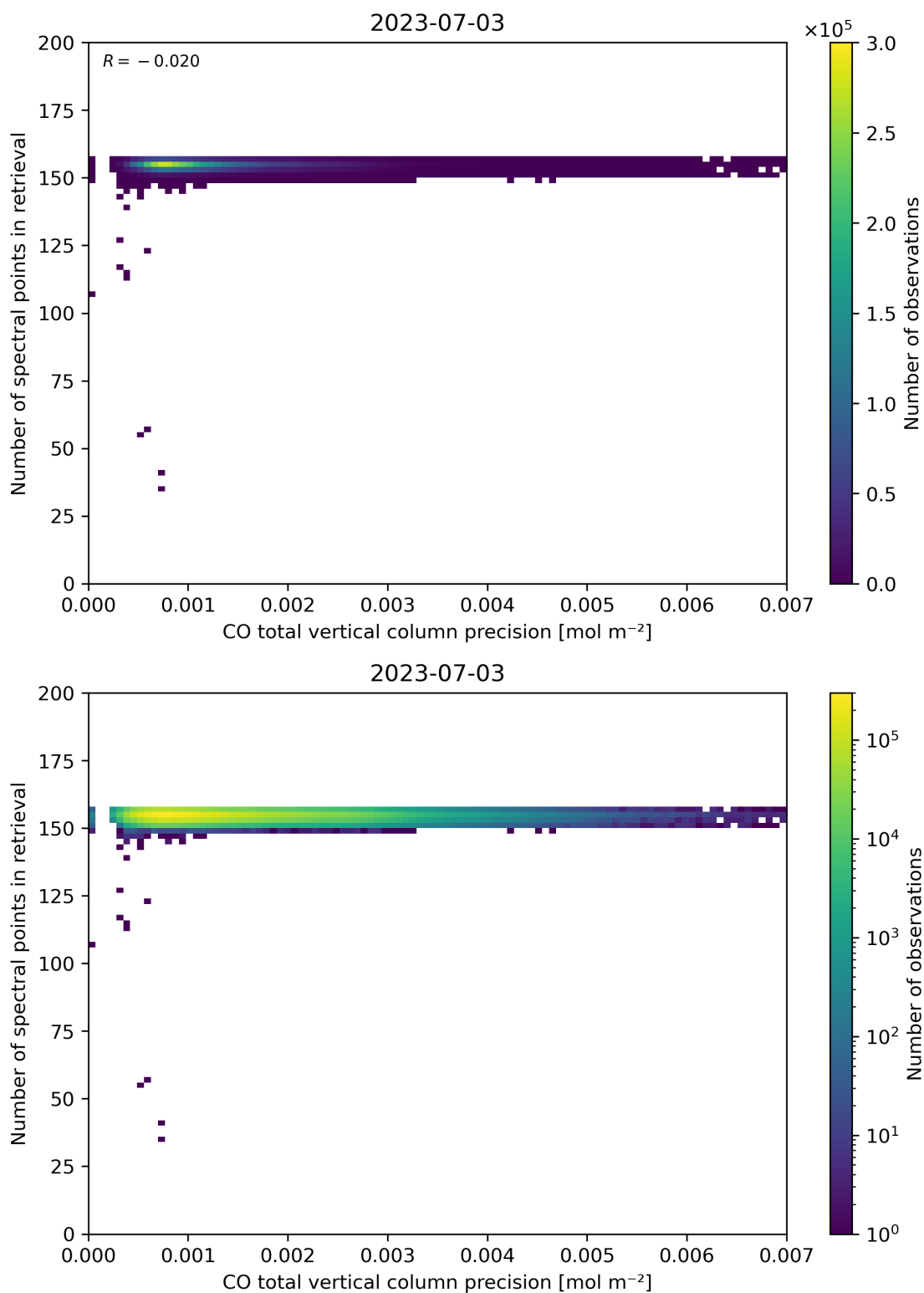
Figure 47: Scatter density plot of “CO total vertical column precision” against “Number of spectral points in retrieval” for 2023-07-03 to 2023-07-04.
