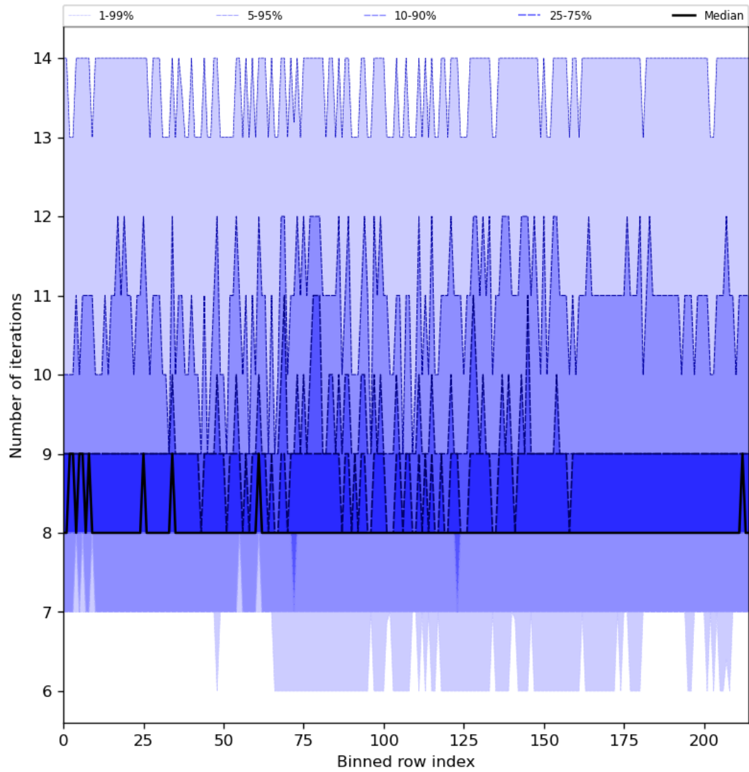
Figure 32: Along track statistics of “Number of iterations” for 2023-07-03 to 2023-07-04
