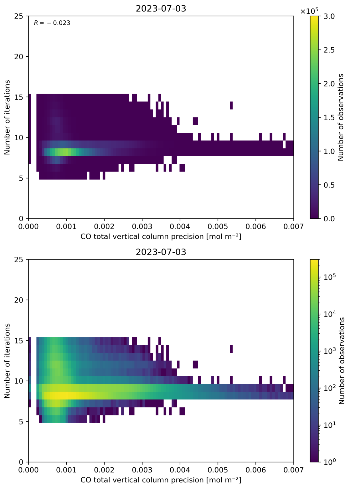
Figure 46: Scatter density plot of “CO total vertical column precision” against “Number of iterations” for 2023-07-03 to 2023-07-04.
