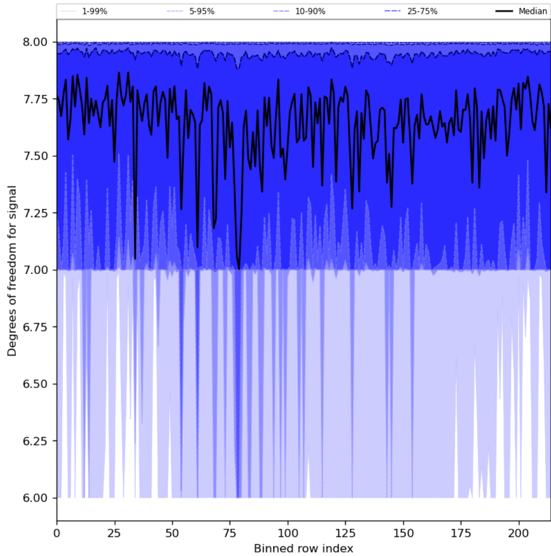
Figure 31: Along track statistics of “Degrees of freedom for signal” for 2023-07-03 to 2023-07-04
