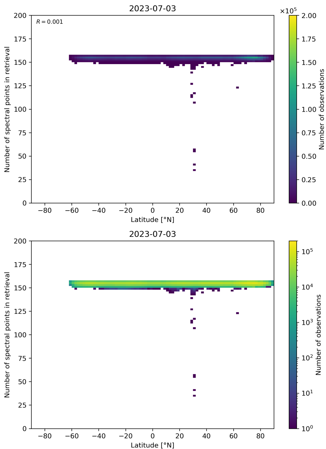
Figure 57: Scatter density plot of “Latitude” against “Number of spectral points in retrieval” for 2023-07-03 to 2023-07-04.
