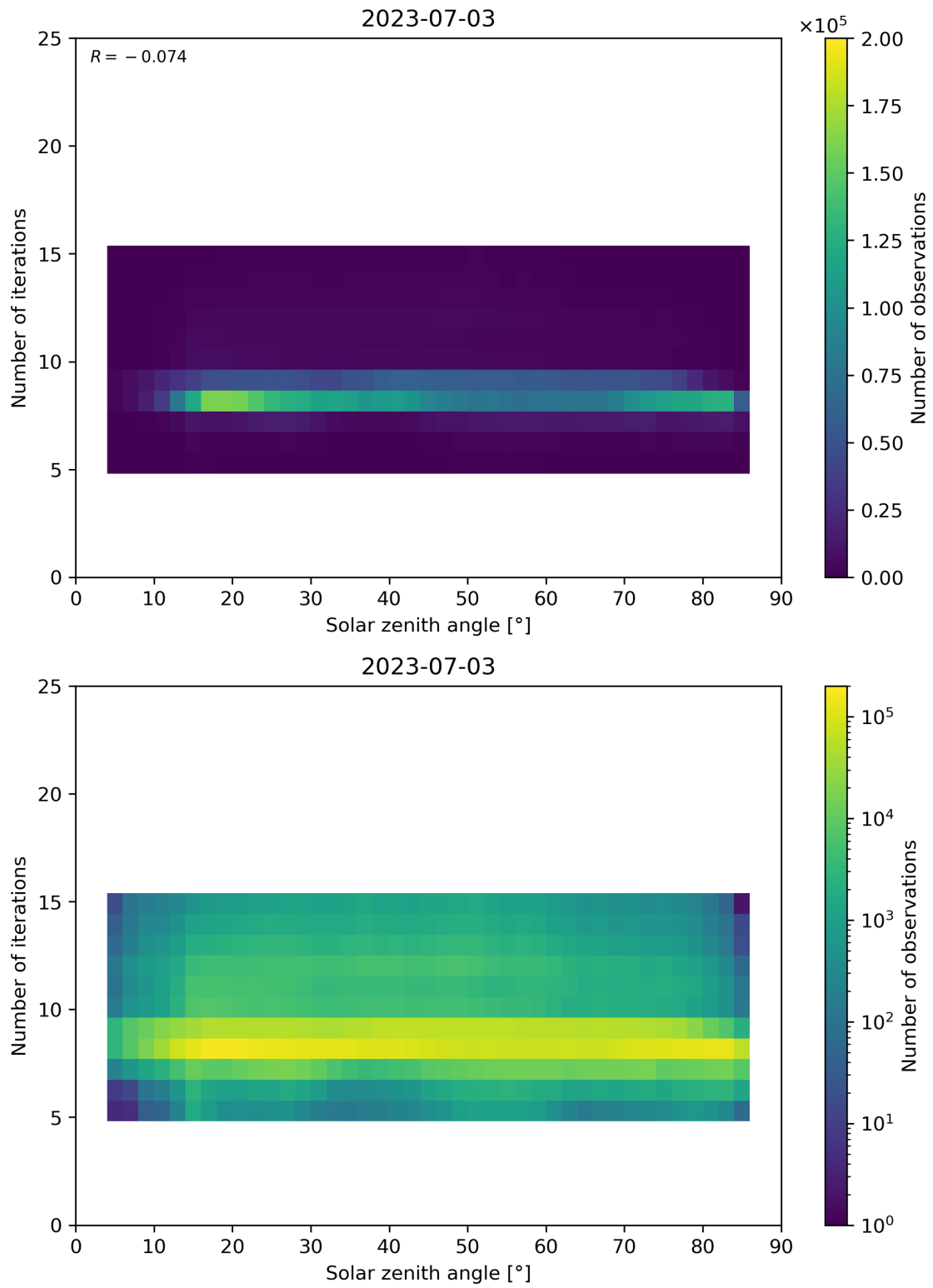
Figure 67: Scatter density plot of “Solar zenith angle” against “Number of iterations” for 2023-07-03 to 2023-07-04.
