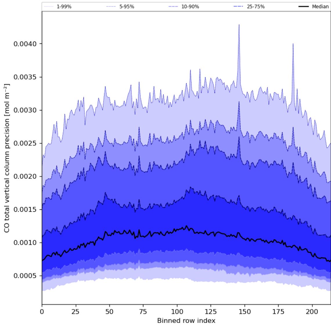
Figure 28: Along track statistics of “CO total vertical column precision” for 2023-07-03 to 2023-07-04
