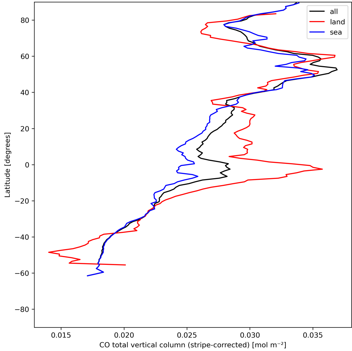
Figure 11: Zonal average of “CO total vertical column (stripe-corrected)” for 2023-07-03 to 2023-07-04.
