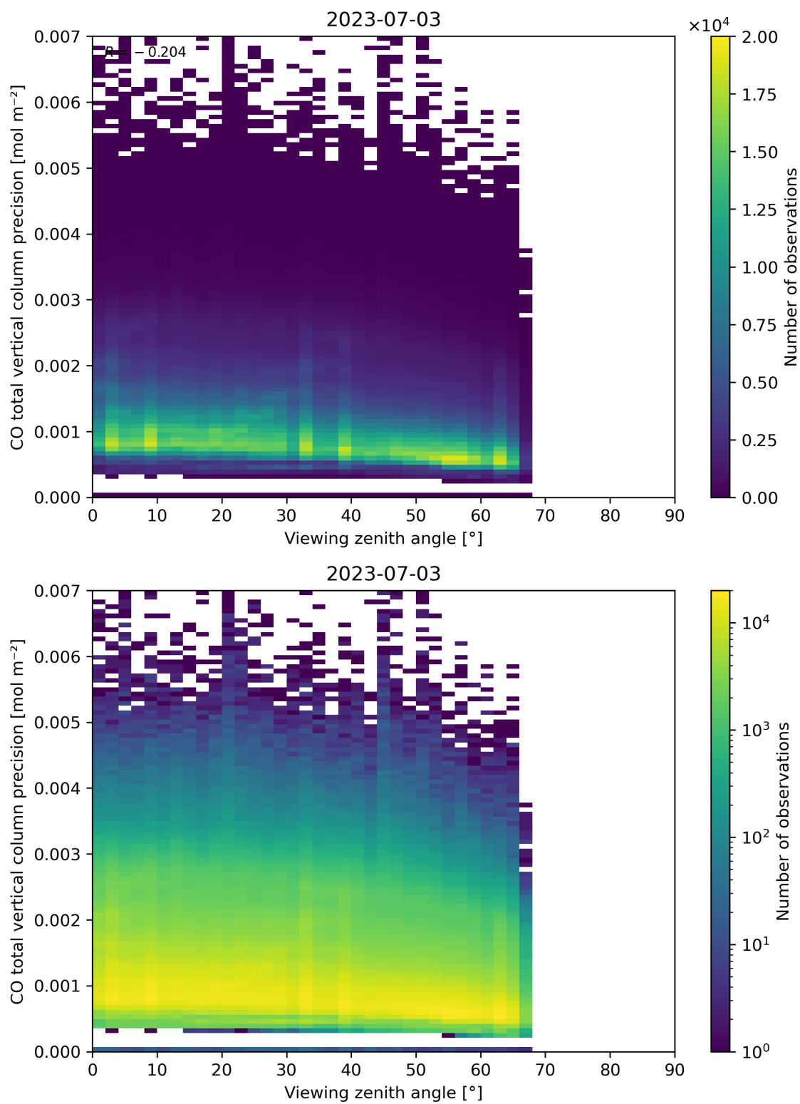
Figure 71: Scatter density plot of “Viewing zenith angle” against “CO total vertical column precision” for 2023-07-03 to 2023-07-04.
