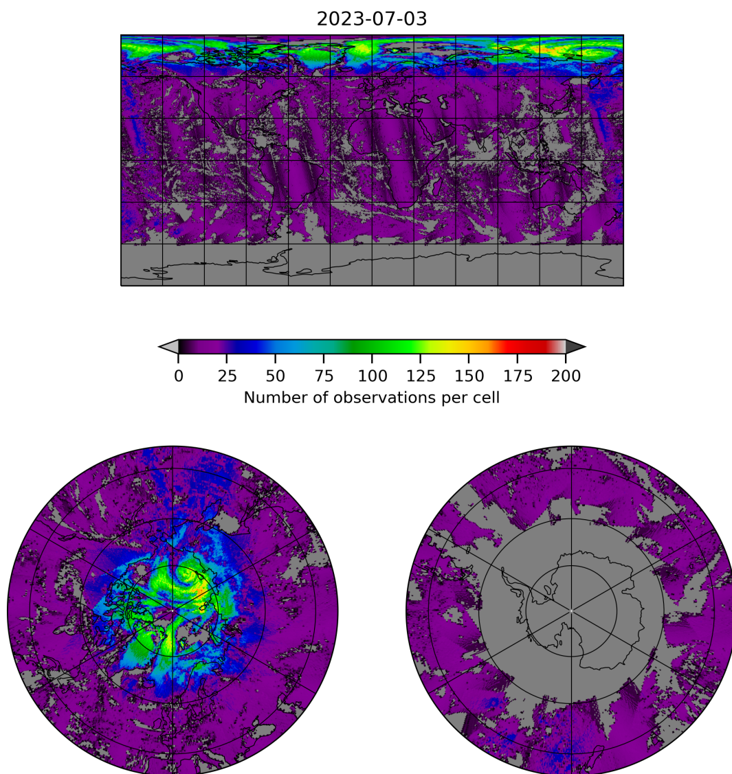
Figure 8: Map of the number of observations for 2023-07-03 to 2023-07-04
