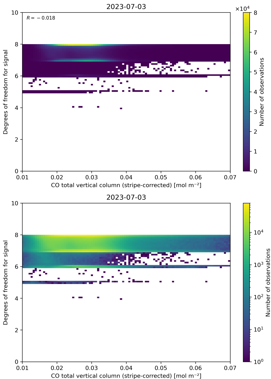
Figure 38: Scatter density plot of “CO total vertical column (stripe-corrected)” against “Degrees of freedom for signal” for 2023-07-03 to 2023-07-04.
