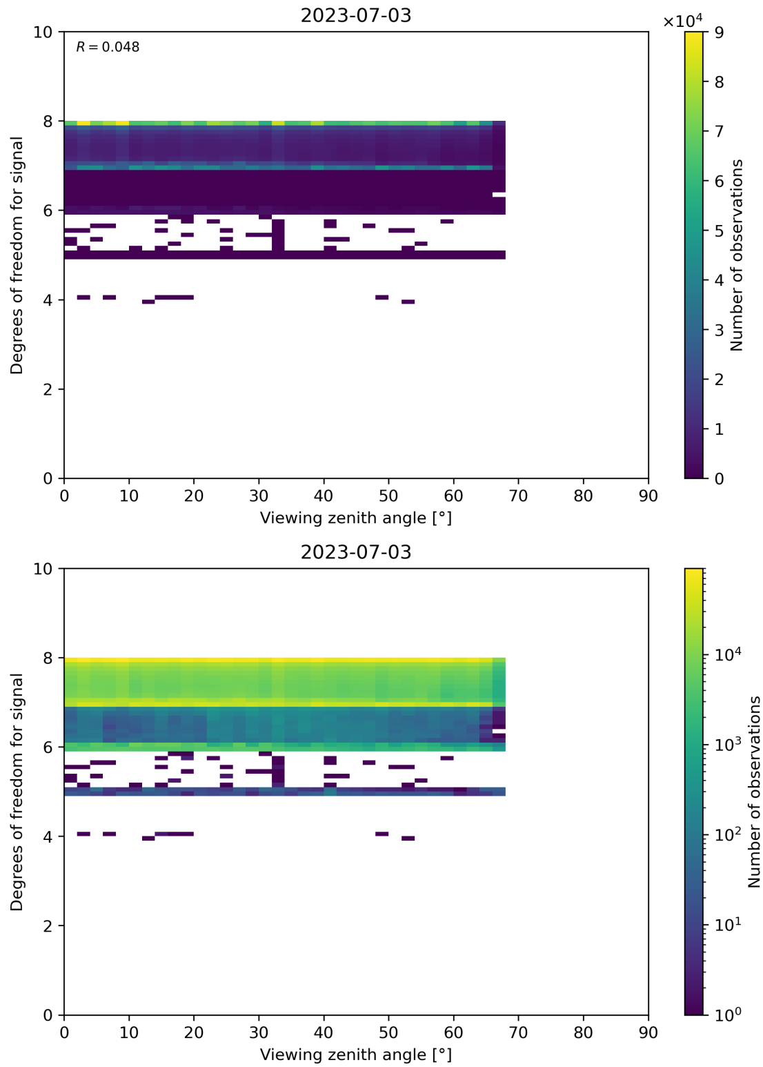
Figure 73: Scatter density plot of “Viewing zenith angle” against “Degrees of freedom for signal” for 2023-07-03 to 2023-07-04.
