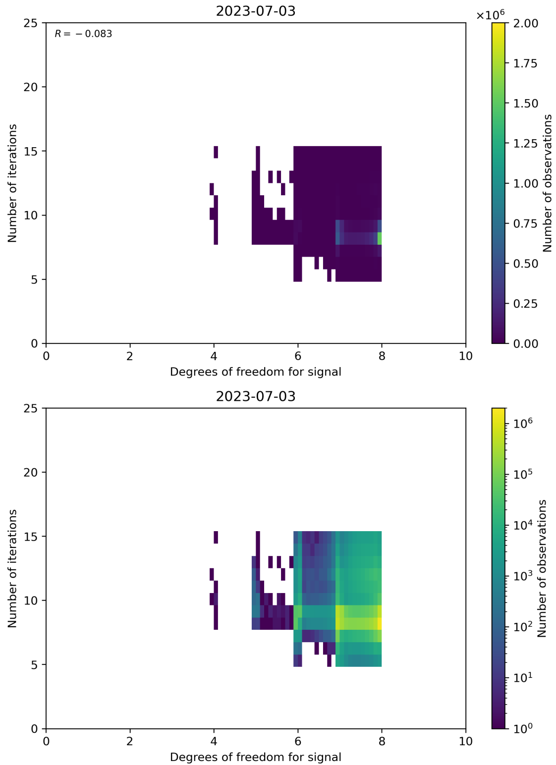
Figure 50: Scatter density plot of “Degrees of freedom for signal” against “Number of iterations” for 2023-07-03 to 2023-07-04.
