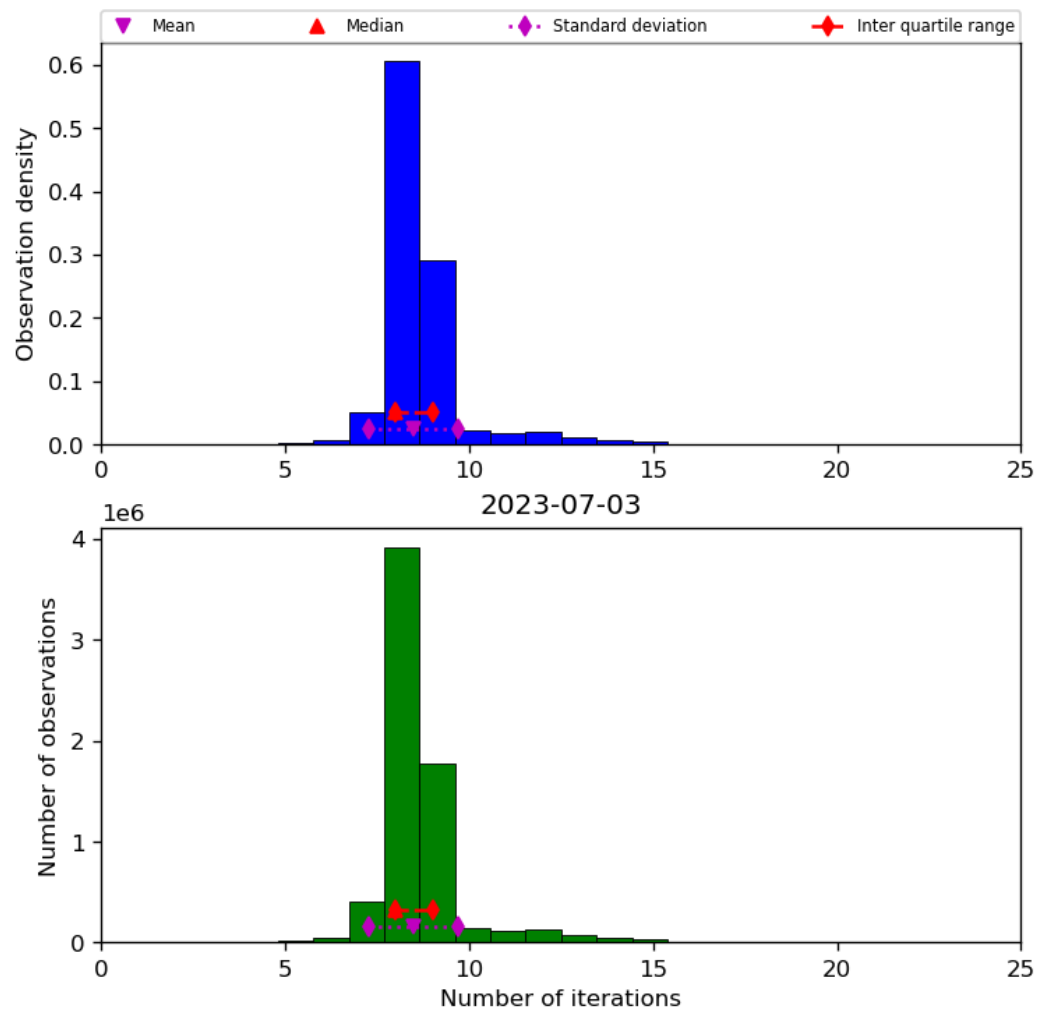
Figure 24: Histogram of “Number of iterations” for 2023-07-03 to 2023-07-04
