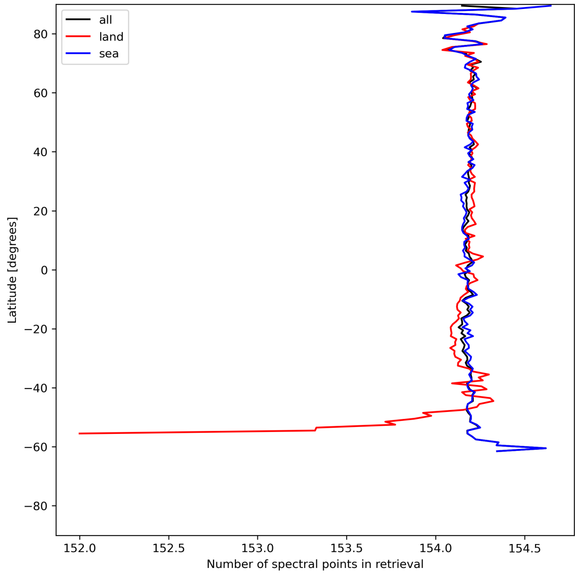
Figure 13: Zonal average of “Number of spectral points in retrieval” for 2023-07-03 to 2023-07-04.
