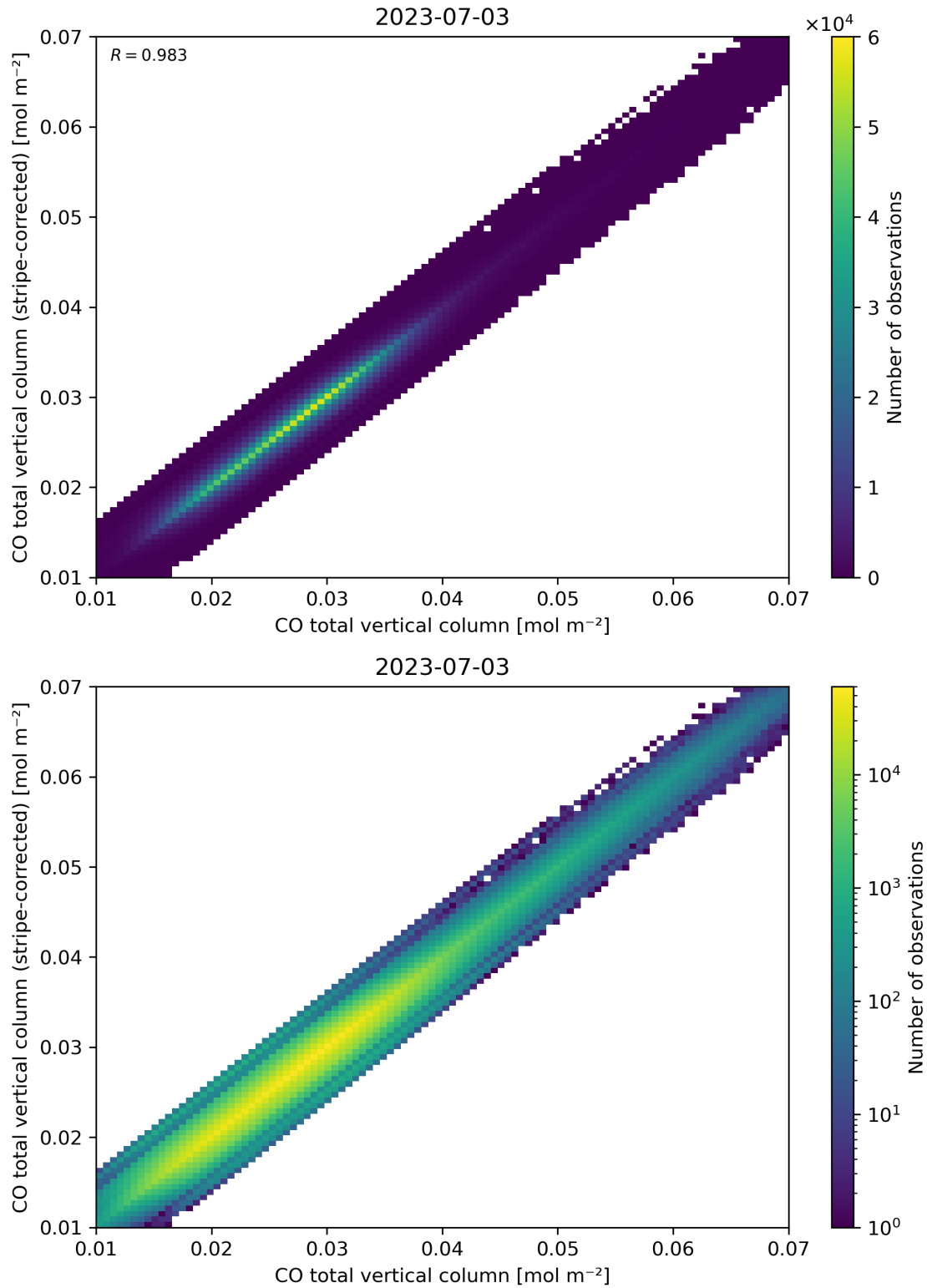
Figure 33: Scatter density plot of “CO total vertical column” against “CO total vertical column (stripe-corrected)” for 2023-07-03 to 2023-07-04.
