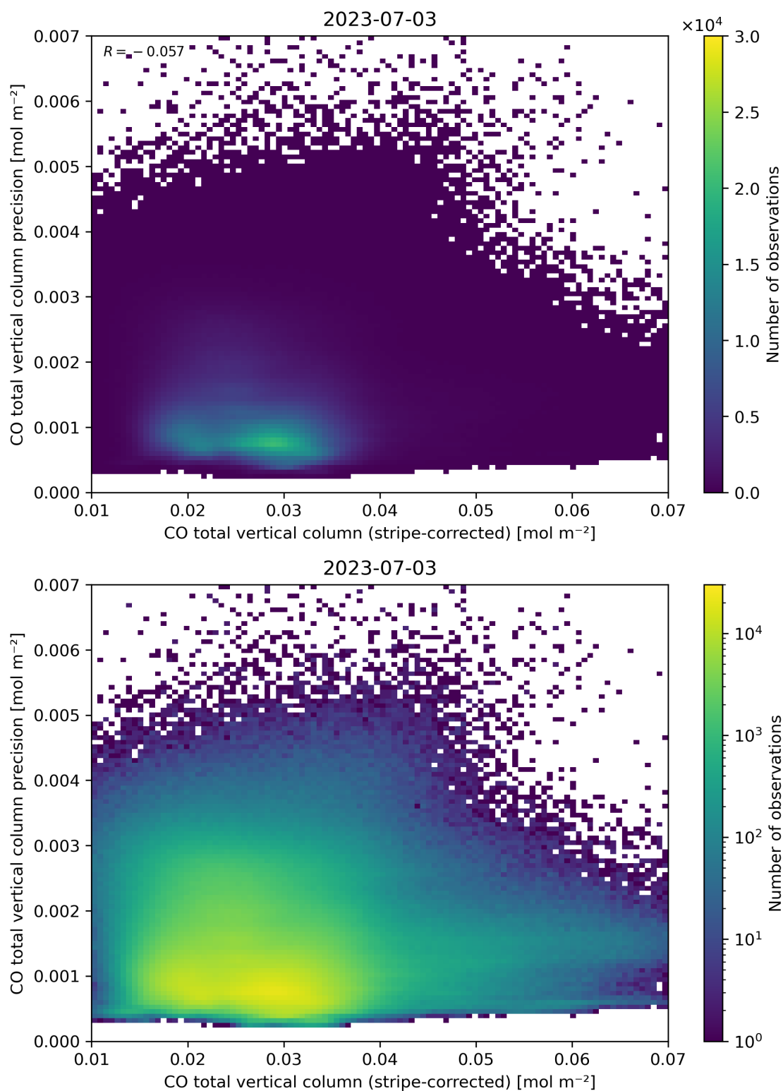
Figure 36: Scatter density plot of “CO total vertical column (stripe-corrected)” against “CO total vertical column precision” for 2023-07-03 to 2023-07-04.
