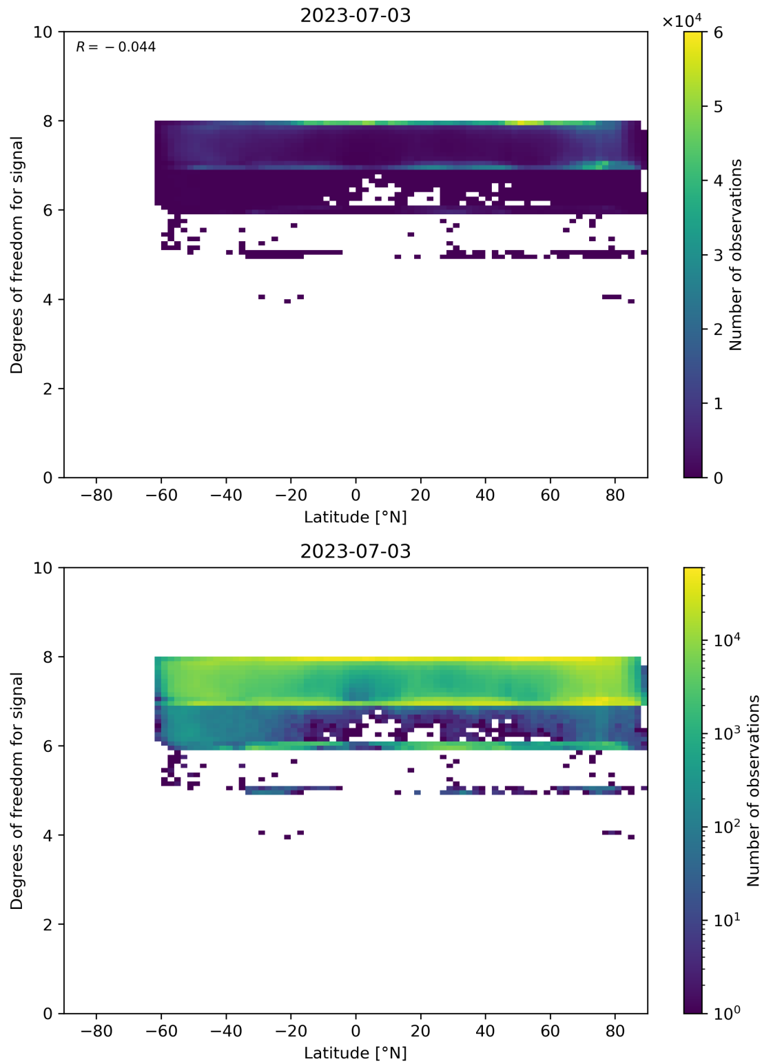
Figure 55: Scatter density plot of “Latitude” against “Degrees of freedom for signal” for 2023-07-03 to 2023-07-04.
