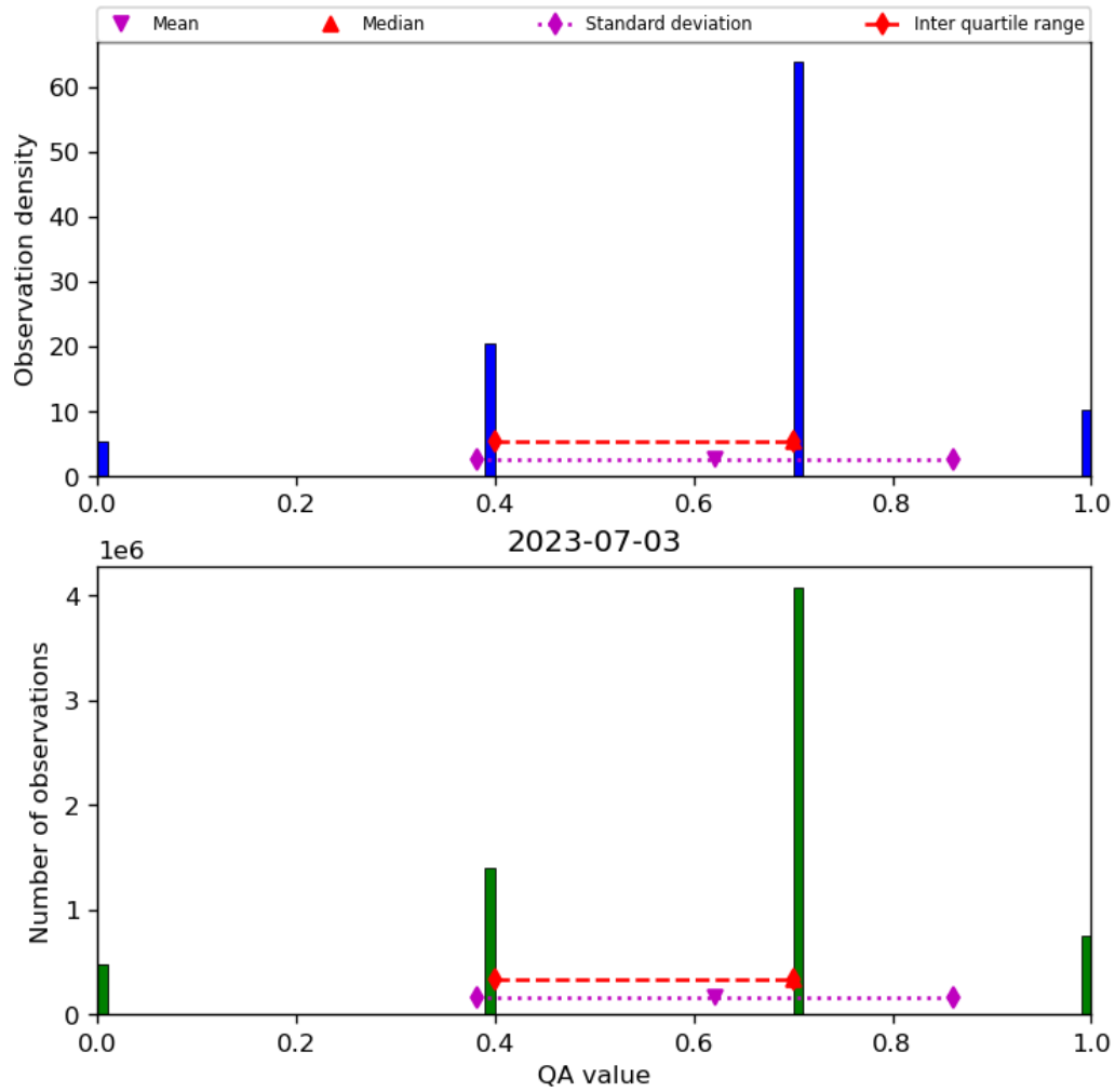
Figure 17: Histogram of “QA value” for 2023-07-03 to 2023-07-04
