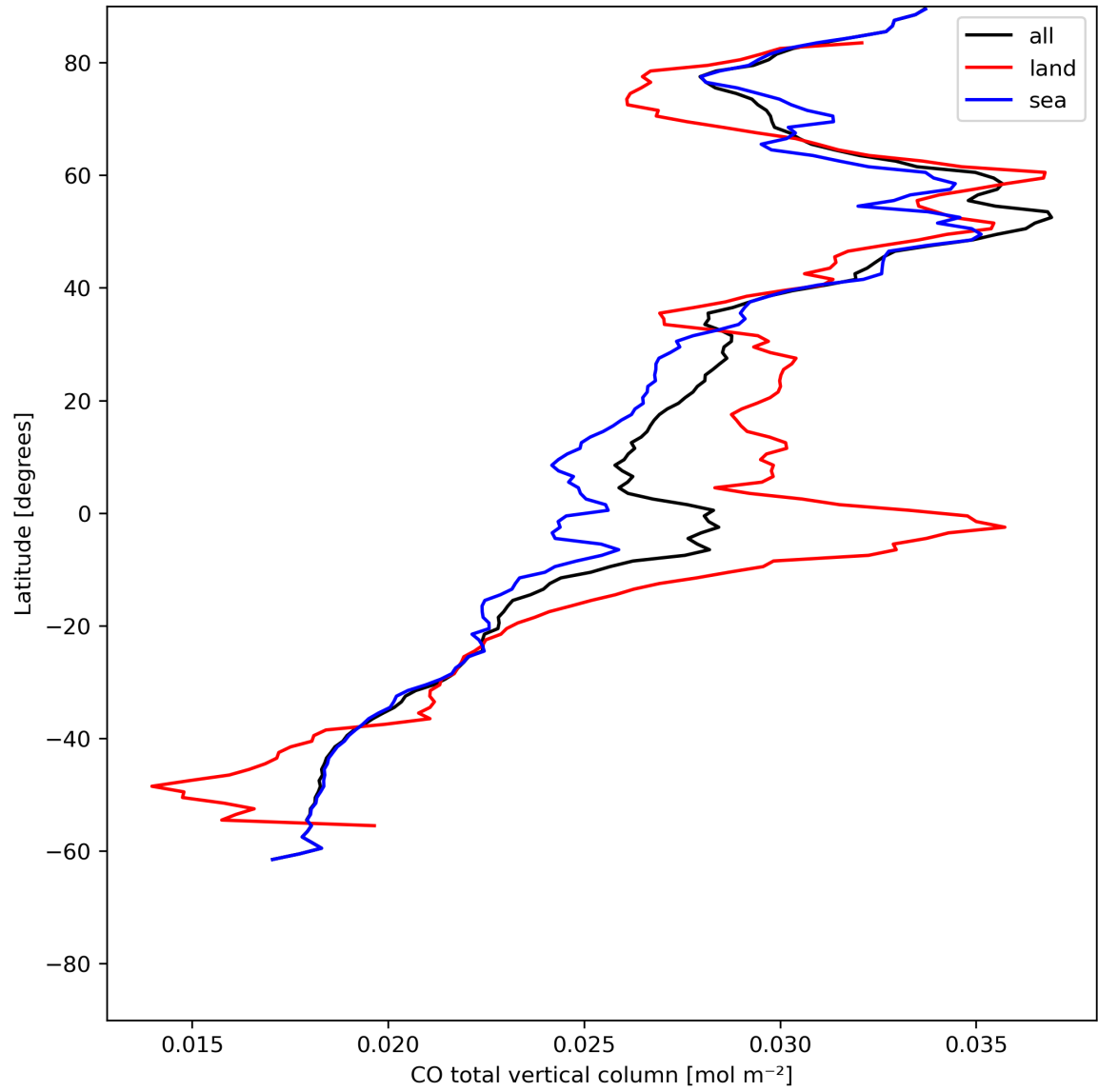
Figure 10: Zonal average of “CO total vertical column” for 2023-07-03 to 2023-07-04.
