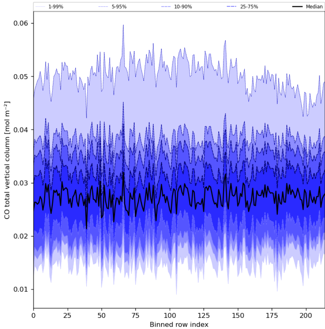
Figure 26: Along track statistics of “CO total vertical column” for 2023-07-03 to 2023-07-04
