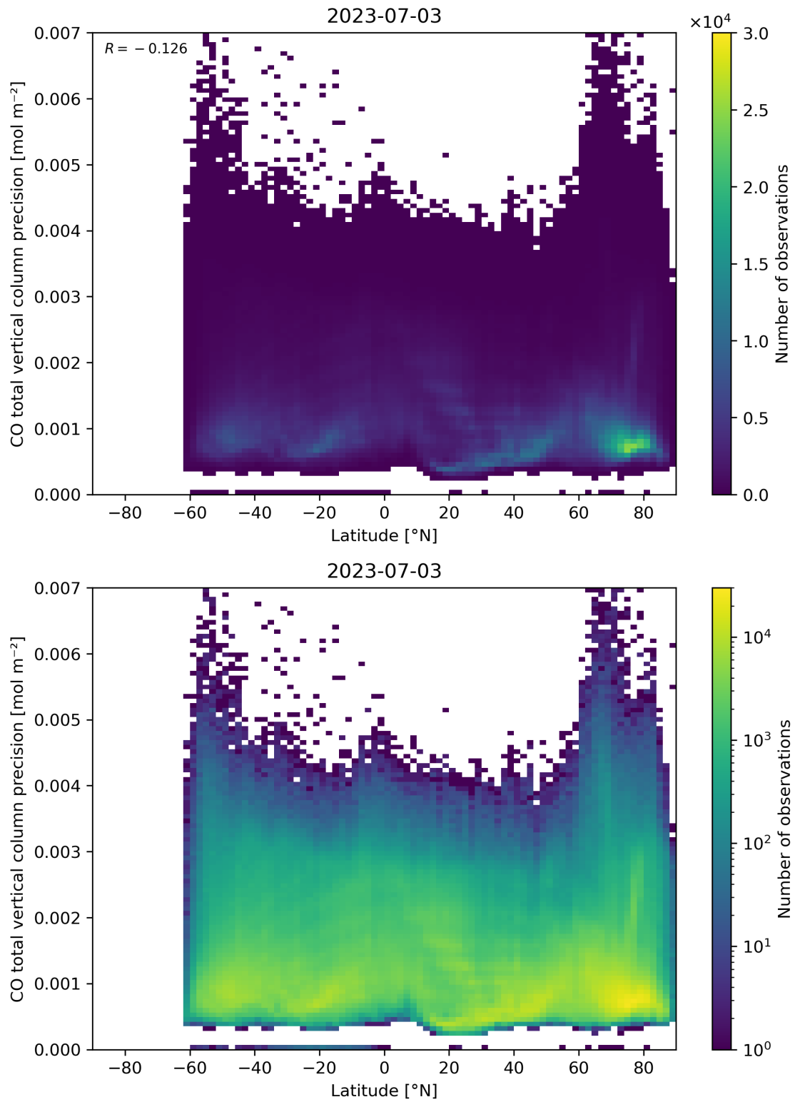
Figure 53: Scatter density plot of “Latitude” against “CO total vertical column precision” for 2023-07-03 to 2023-07-04.
