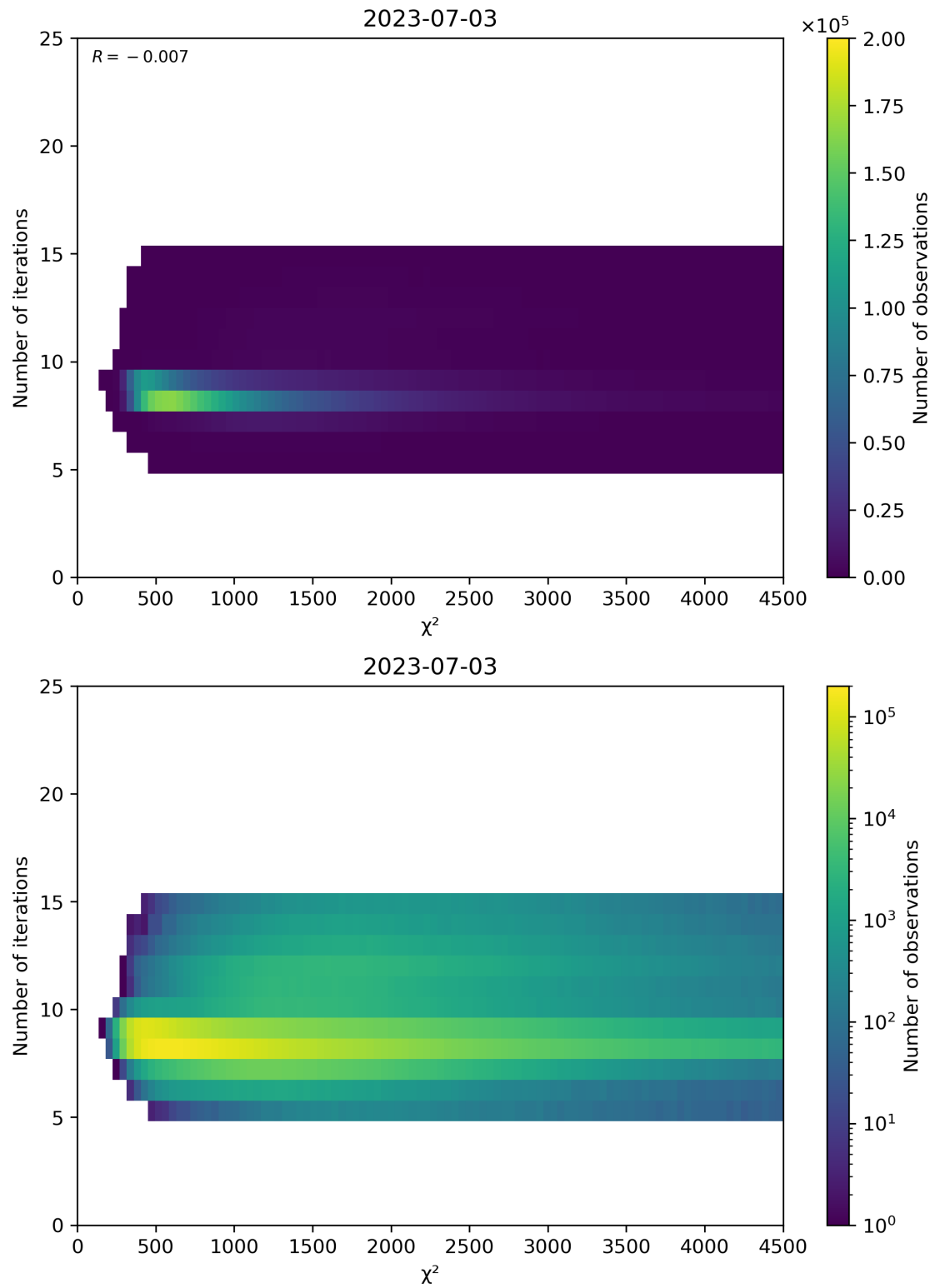
Figure 49: Scatter density plot of “ \chi^2 ” against “Number of iterations” for 2023-07-03 to 2023-07-04.
