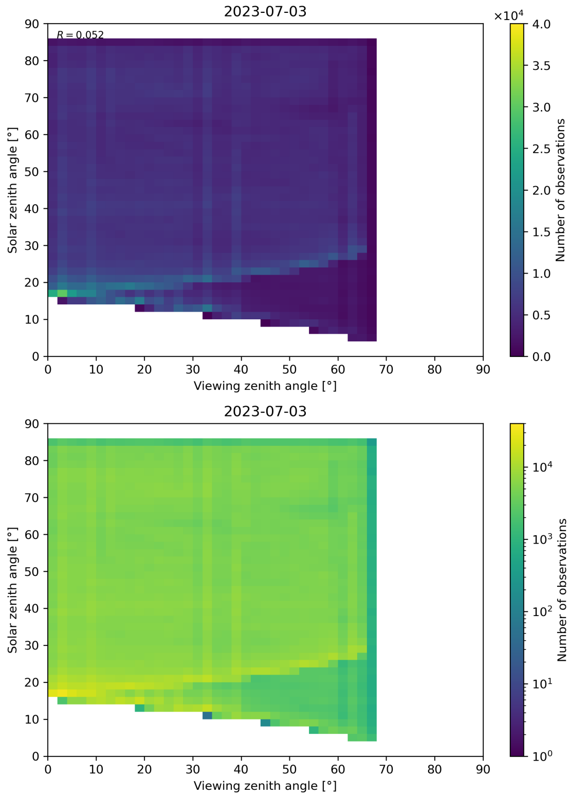
Figure 77: Scatter density plot of “Viewing zenith angle” against “Solar zenith angle” for 2023-07-03 to 2023-07-04.
