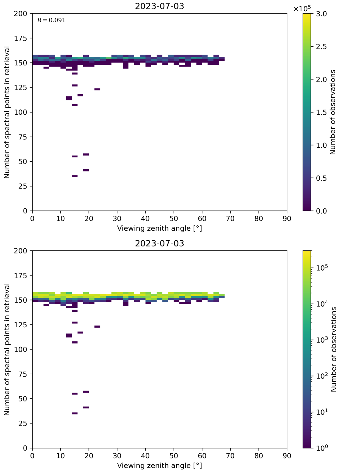
Figure 76: Scatter density plot of “Viewing zenith angle” against “Number of spectral points in retrieval” for 2023-07-03 to 2023-07-04.
