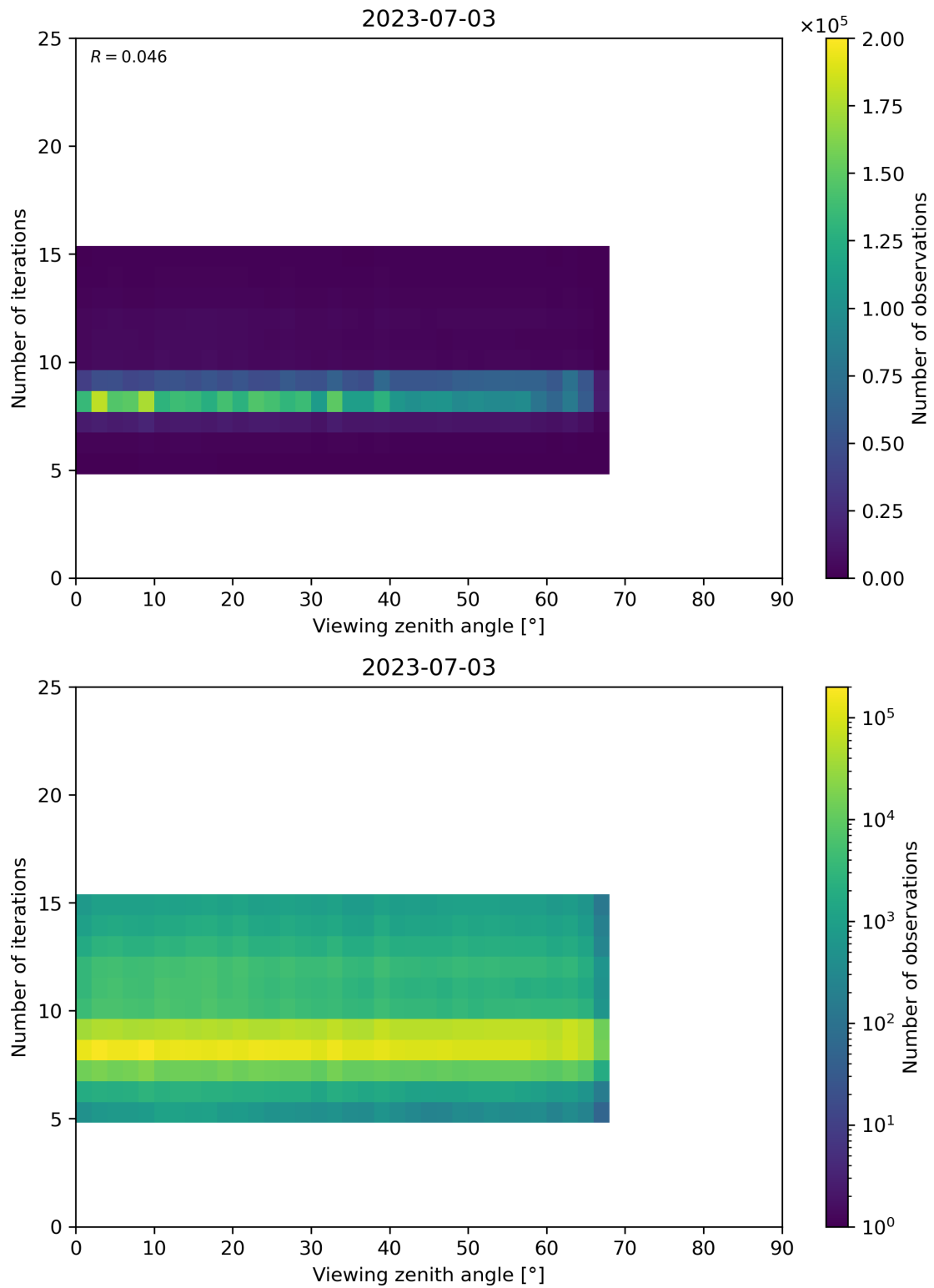
Figure 75: Scatter density plot of “Viewing zenith angle” against “Number of iterations” for 2023-07-03 to 2023-07-04.
