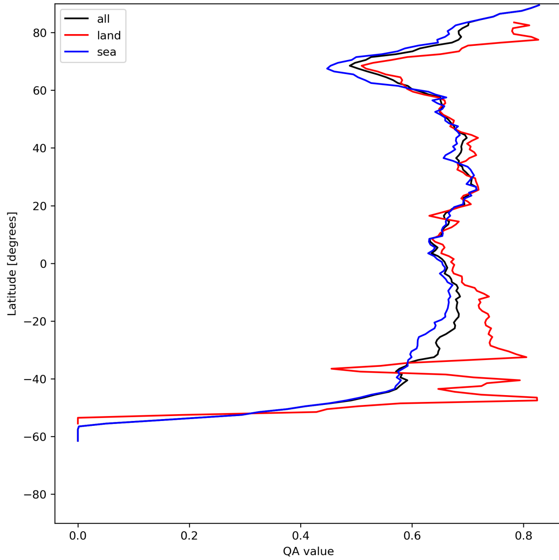
Figure 9: Zonal average of “QA value” for 2023-07-03 to 2023-07-04.
