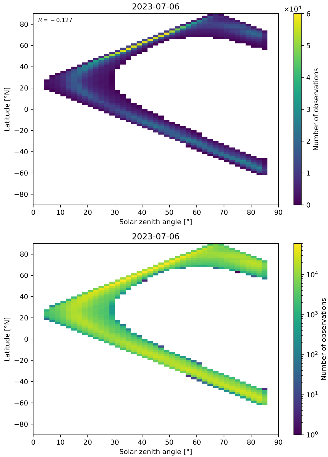
Figure 66: Scatter density plot of “Solar zenith angle” against “Latitude” for 2023-07-05 to 2023-07-07.
