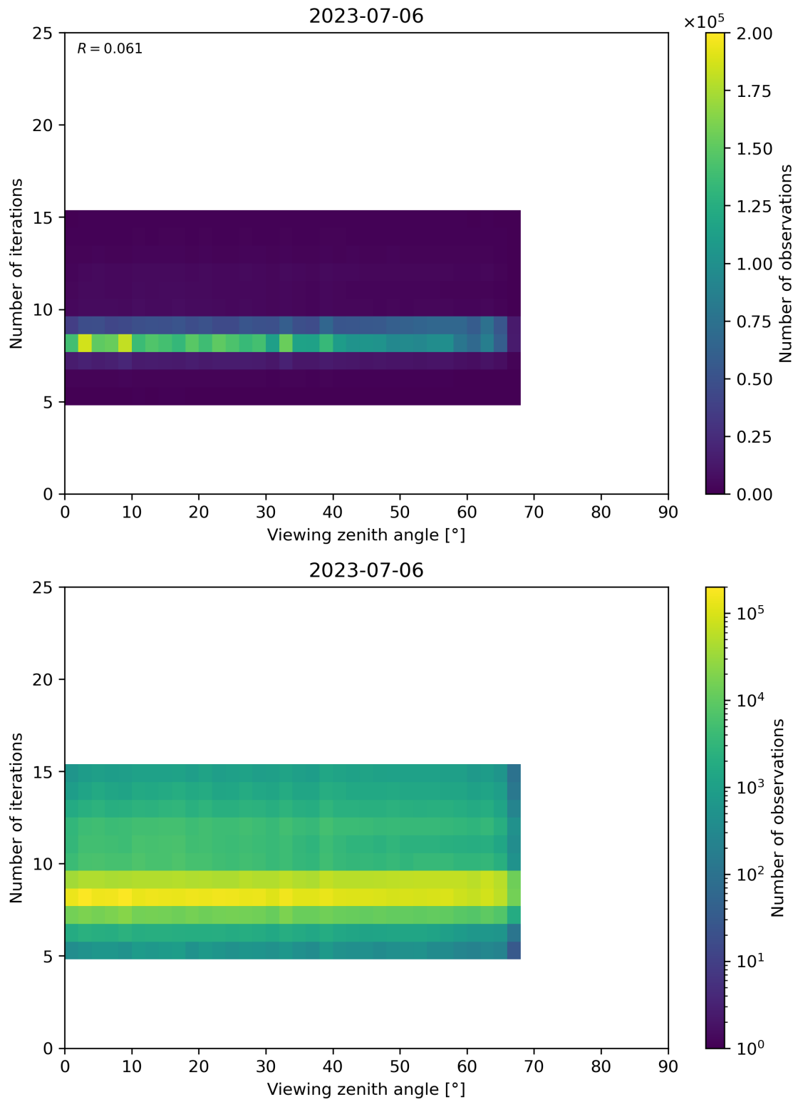
Figure 75: Scatter density plot of “Viewing zenith angle” against “Number of iterations” for 2023-07-05 to 2023-07-07.
