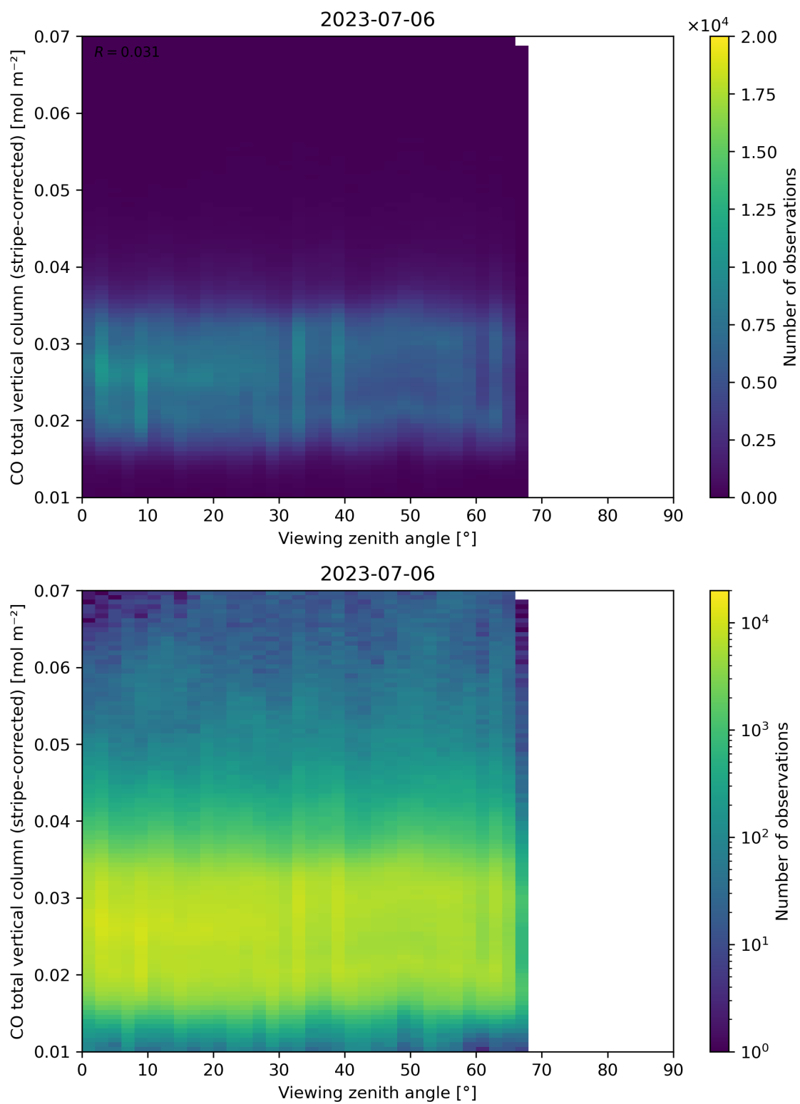
Figure 70: Scatter density plot of “Viewing zenith angle” against “CO total vertical column (stripe-corrected)” for 2023-07-05 to 2023-07-07.
