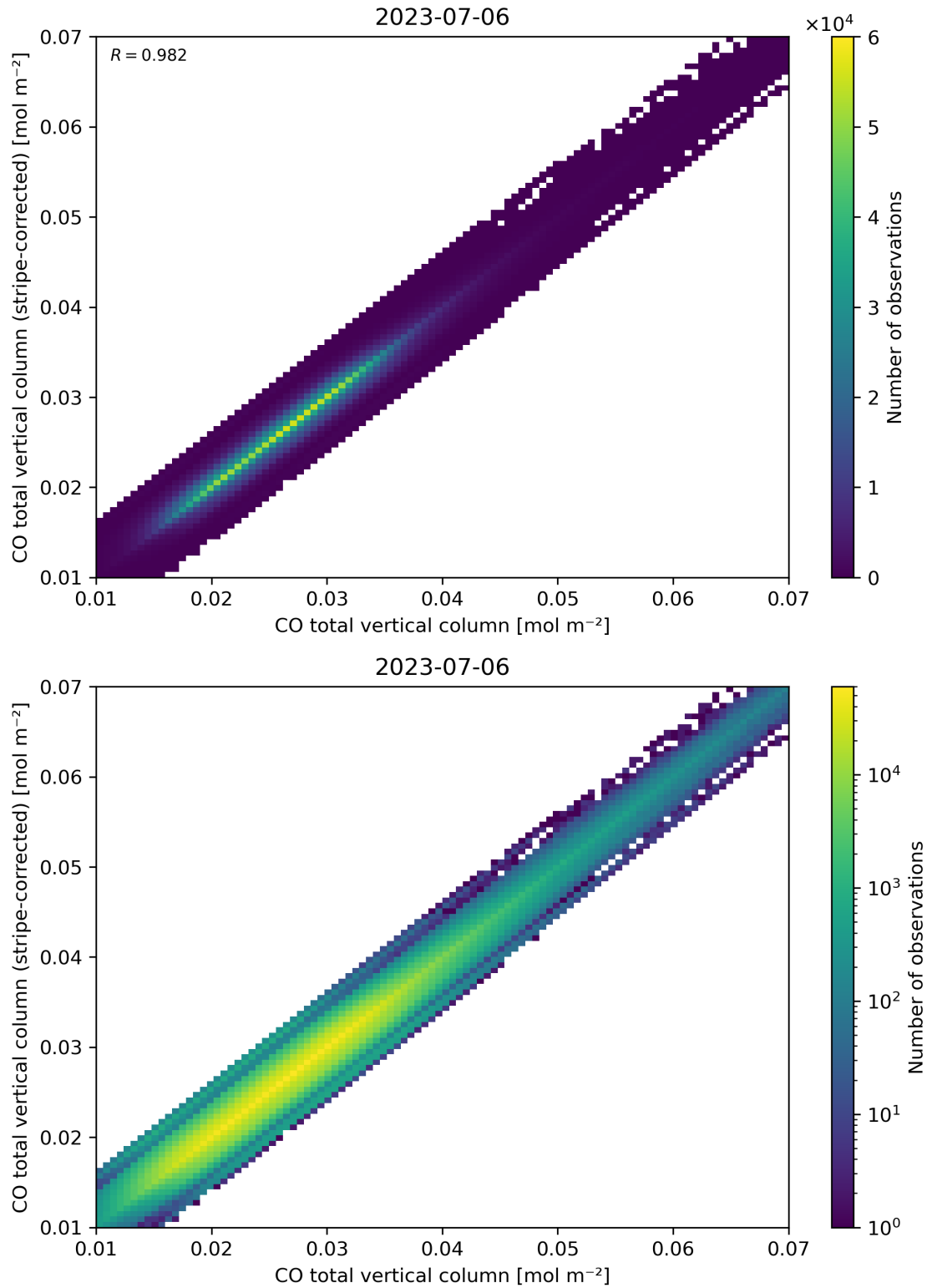
Figure 33: Scatter density plot of “CO total vertical column” against “CO total vertical column (stripe-corrected)” for 2023-07-05 to 2023-07-07.
