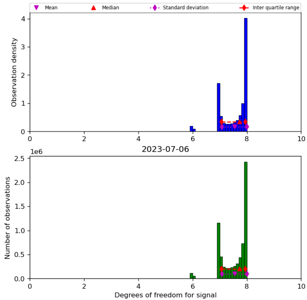
Figure 23: Histogram of “Degrees of freedom for signal” for 2023-07-05 to 2023-07-07
