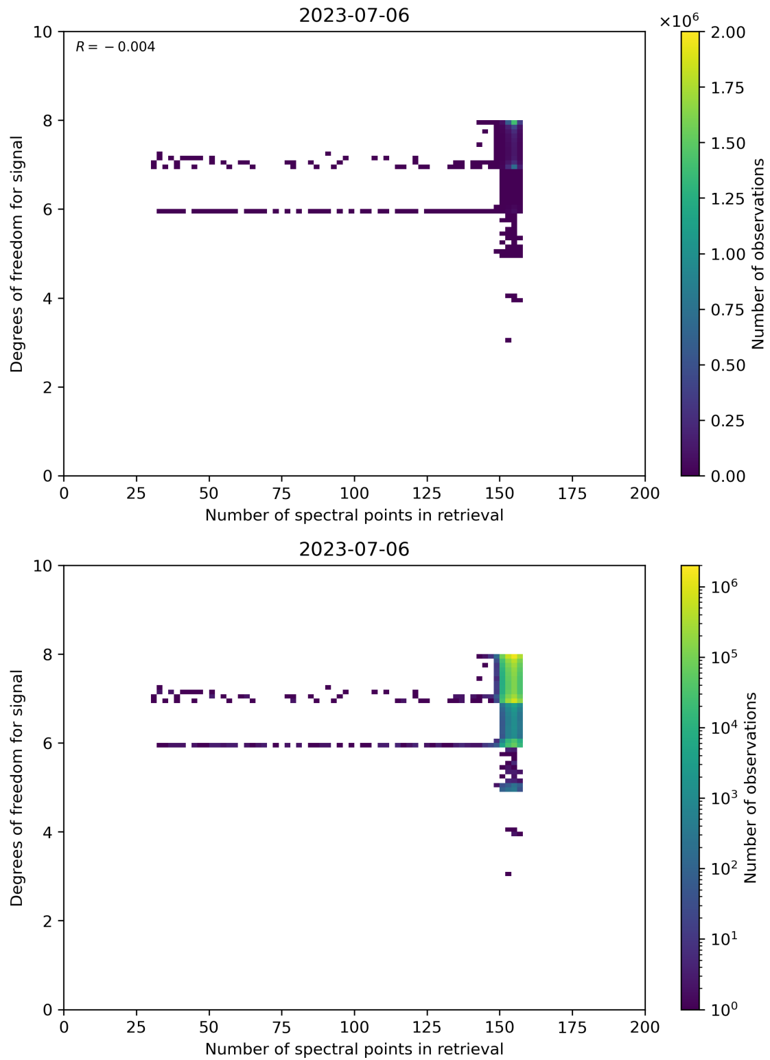
Figure 59: Scatter density plot of “Number of spectral points in retrieval” against “Degrees of freedom for signal” for 2023-07-05 to 2023-07-07.
