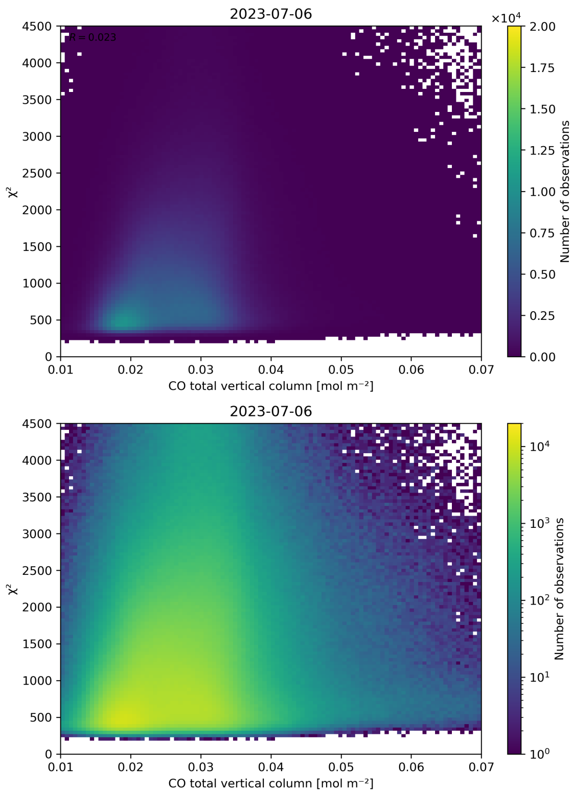
Figure 35: Scatter density plot of “CO total vertical column” against “ \chi^2 ” for 2023-07-05 to 2023-07-07.
