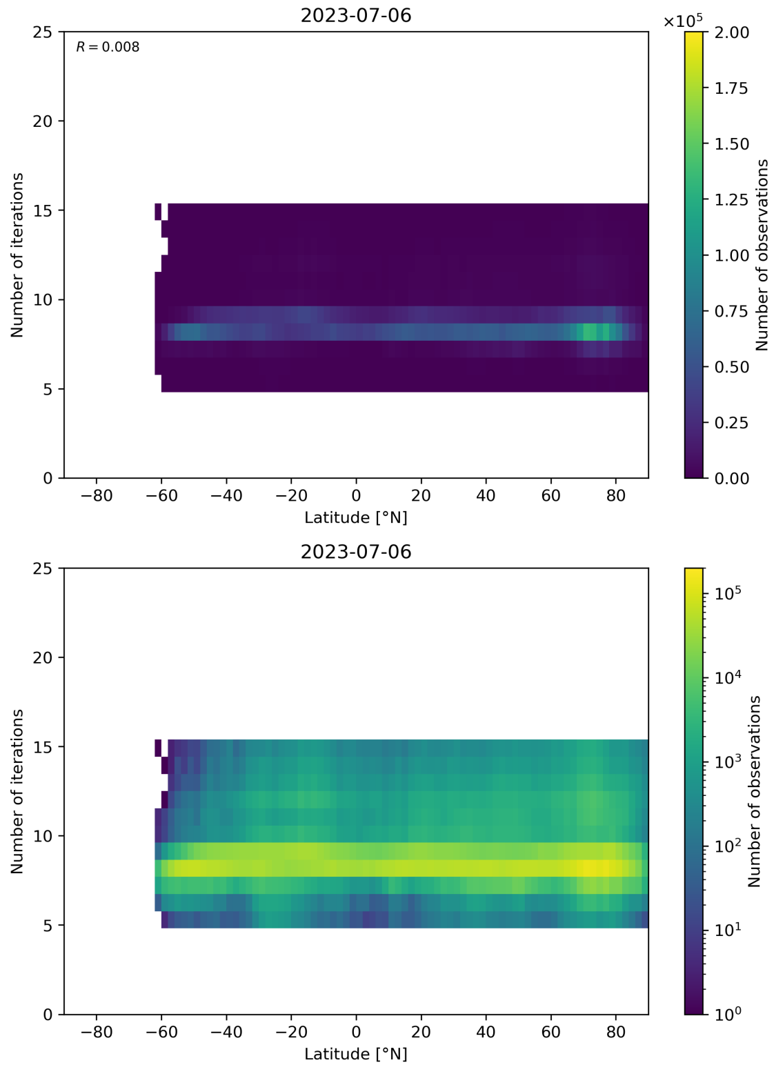
Figure 56: Scatter density plot of “Latitude” against “Number of iterations” for 2023-07-05 to 2023-07-07.
