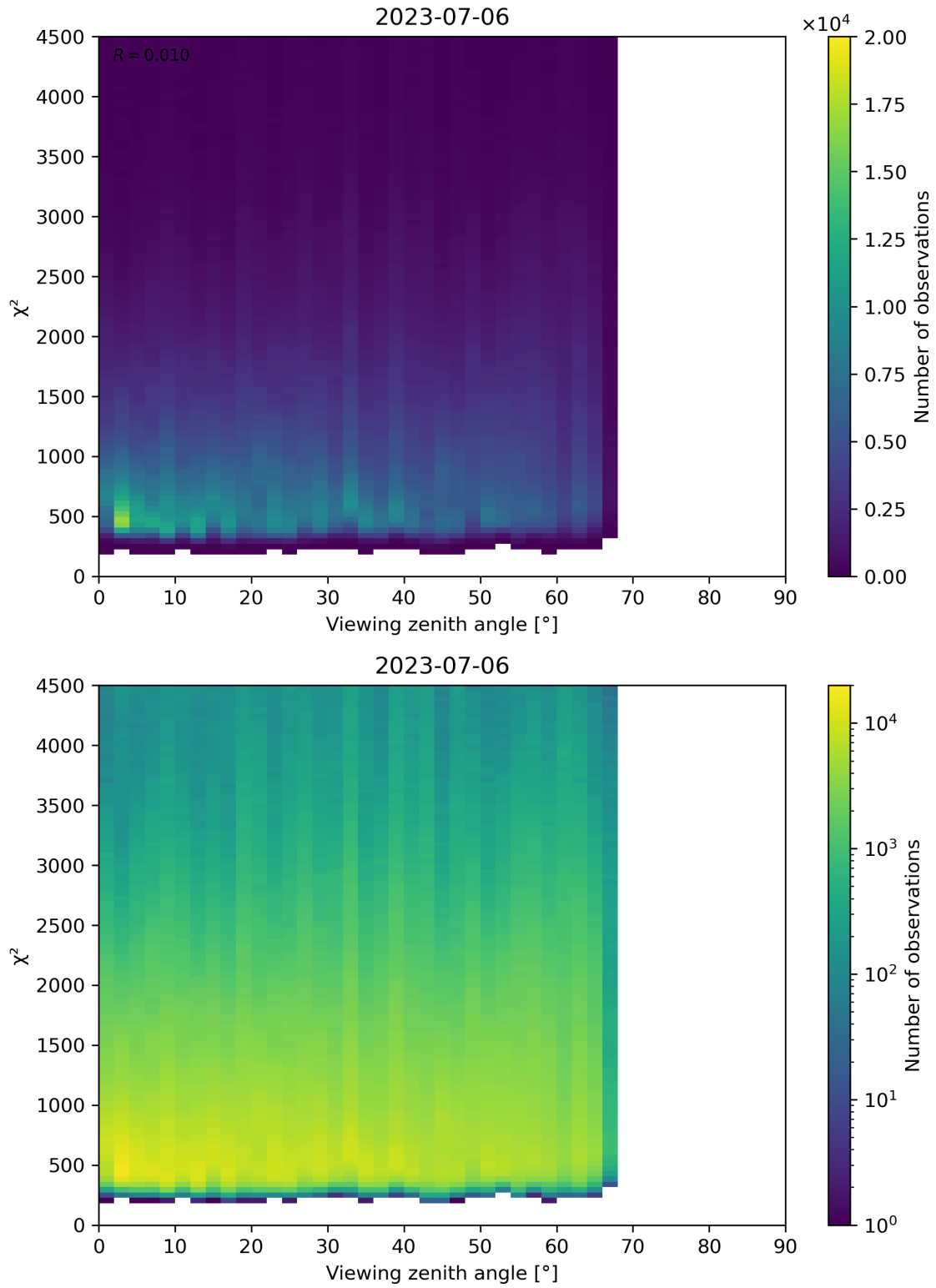
Figure 72: Scatter density plot of “Viewing zenith angle” against “ \chi^2 ” for 2023-07-05 to 2023-07-07.
