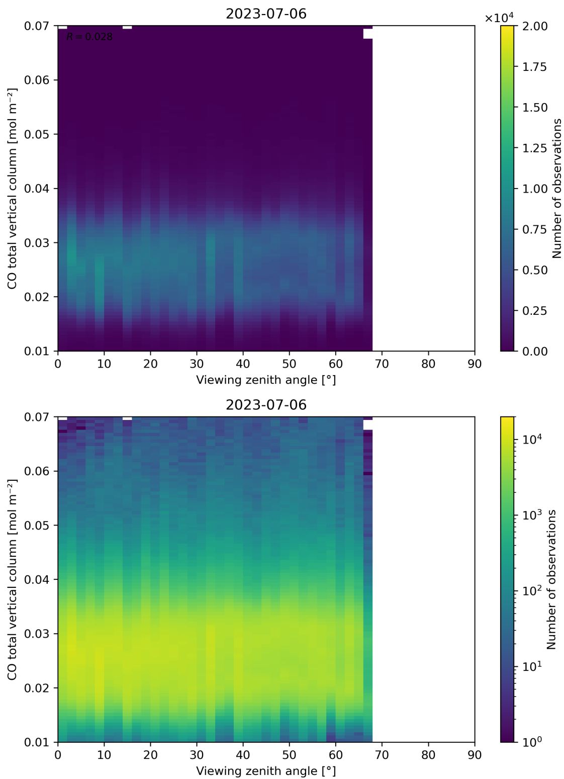
Figure 69: Scatter density plot of “Viewing zenith angle” against “CO total vertical column” for 2023-07-05 to 2023-07-07.
