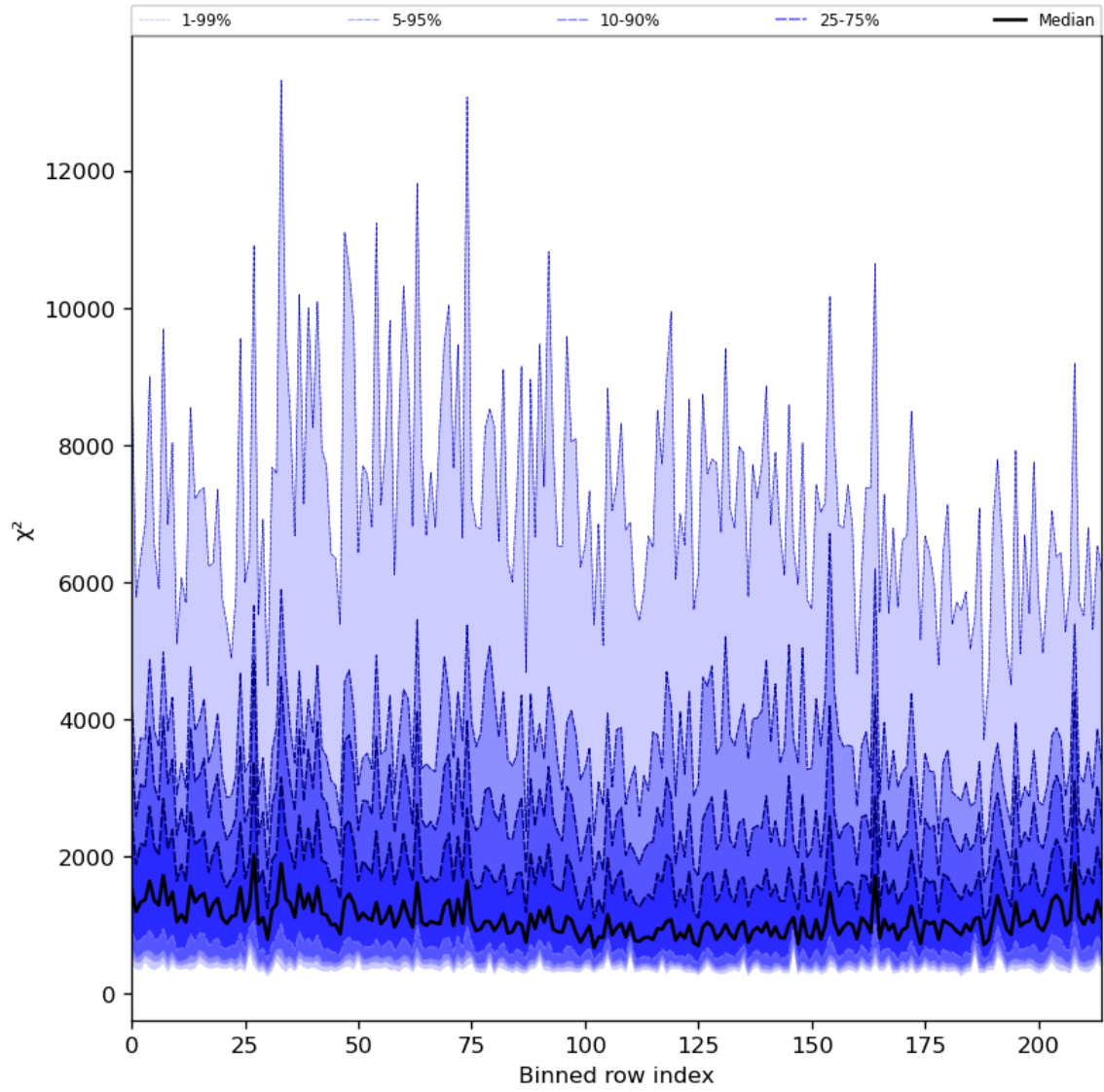
Figure 30: Along track statistics of “ \chi^2 ” for 2023-07-05 to 2023-07-07
