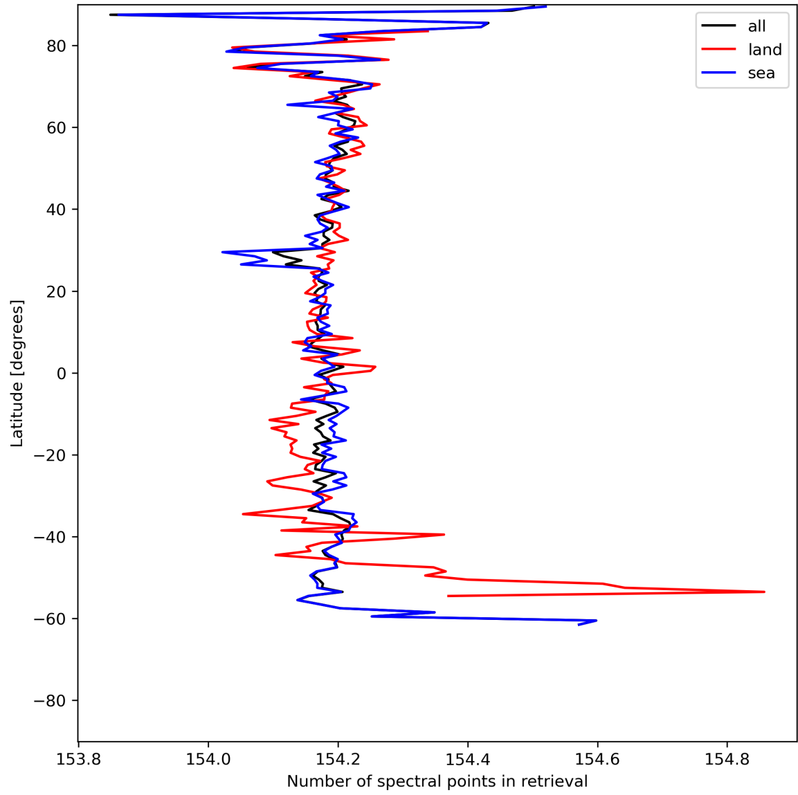
Figure 13: Zonal average of “Number of spectral points in retrieval” for 2023-07-05 to 2023-07-07.
