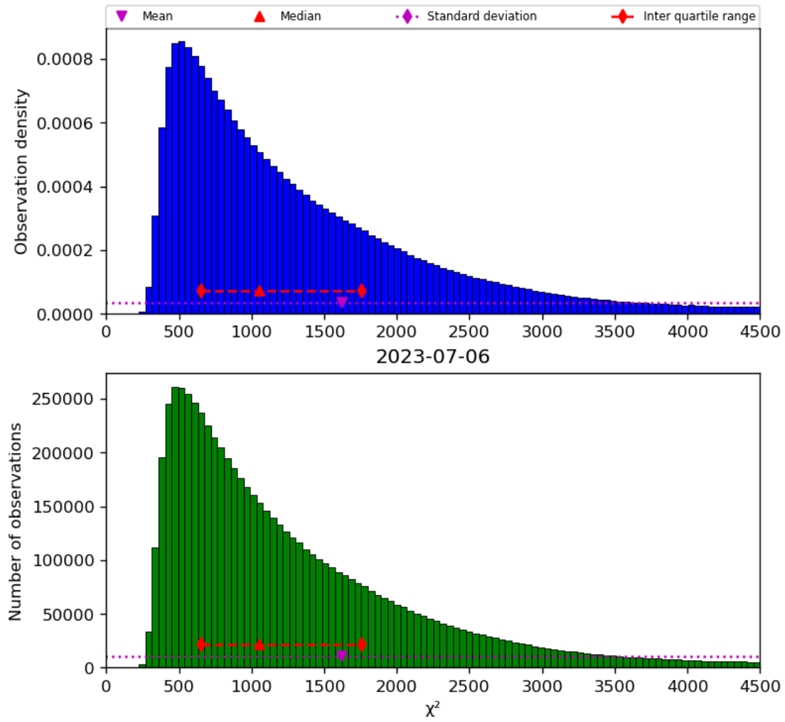
Figure 22: Histogram of “ \chi^2 ” for 2023-07-05 to 2023-07-07
