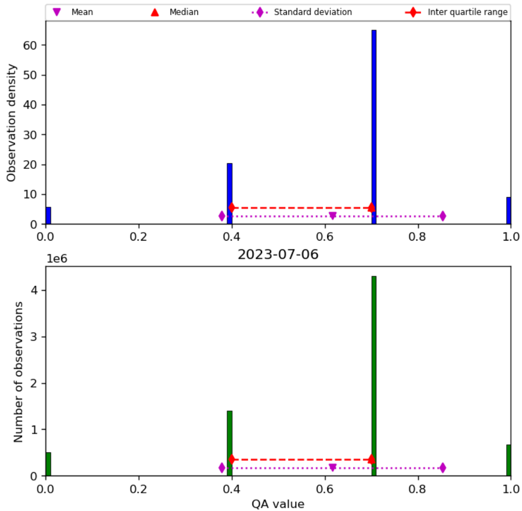
Figure 17: Histogram of “QA value” for 2023-07-05 to 2023-07-07
