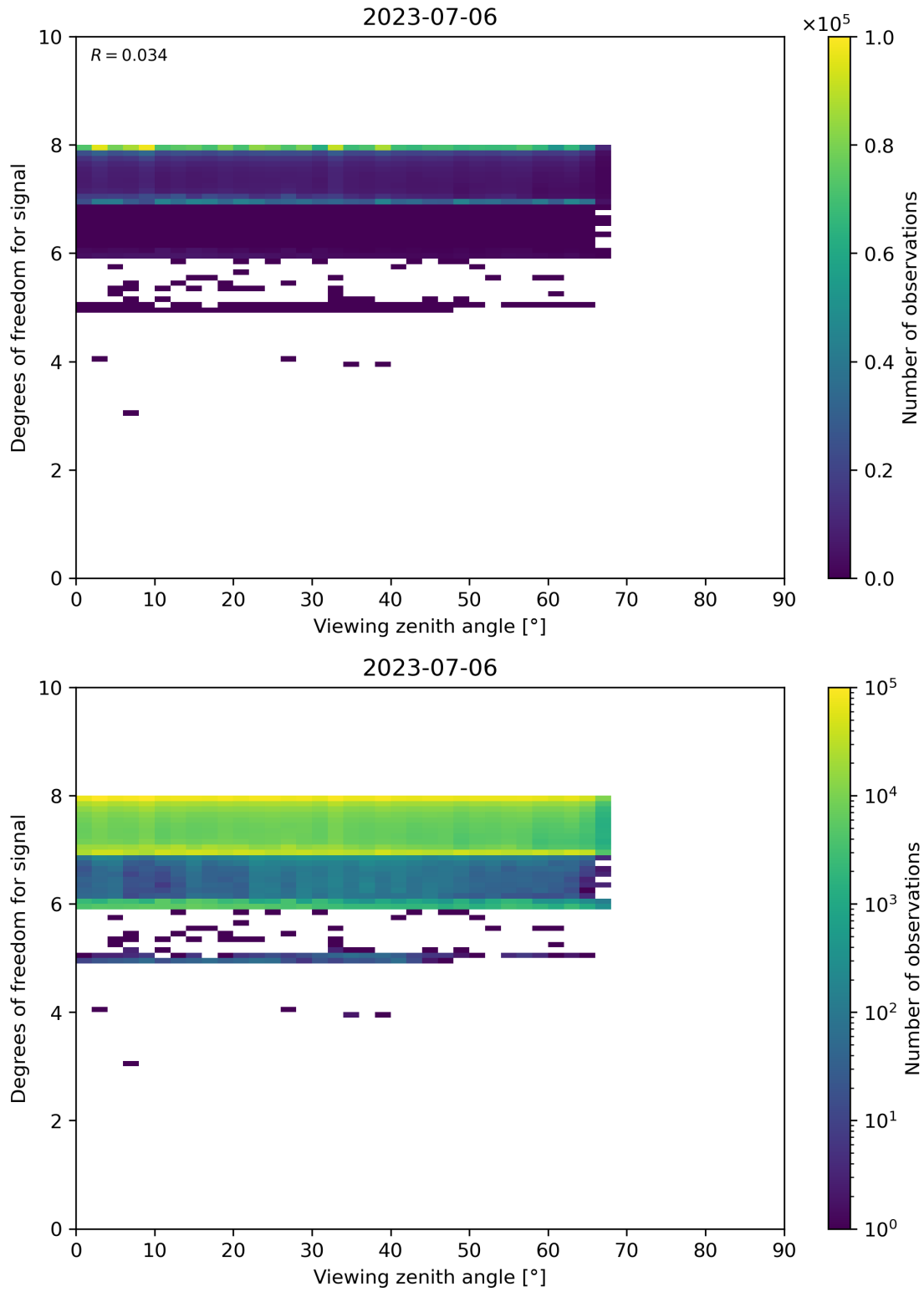
Figure 73: Scatter density plot of “Viewing zenith angle” against “Degrees of freedom for signal” for 2023-07-05 to 2023-07-07.
