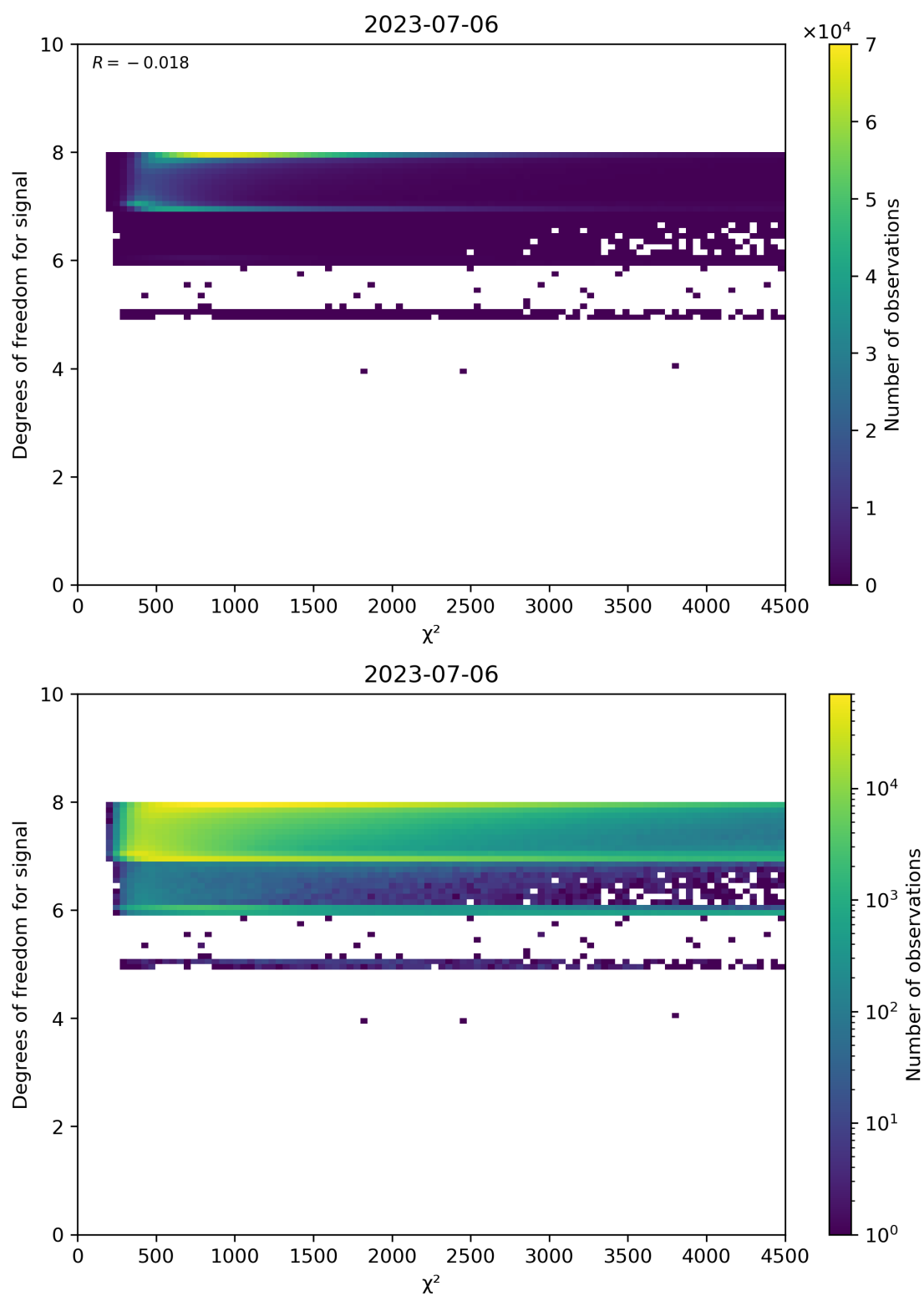
Figure 48: Scatter density plot of “ \chi^2 ” against “Degrees of freedom for signal” for 2023-07-05 to 2023-07-07.
