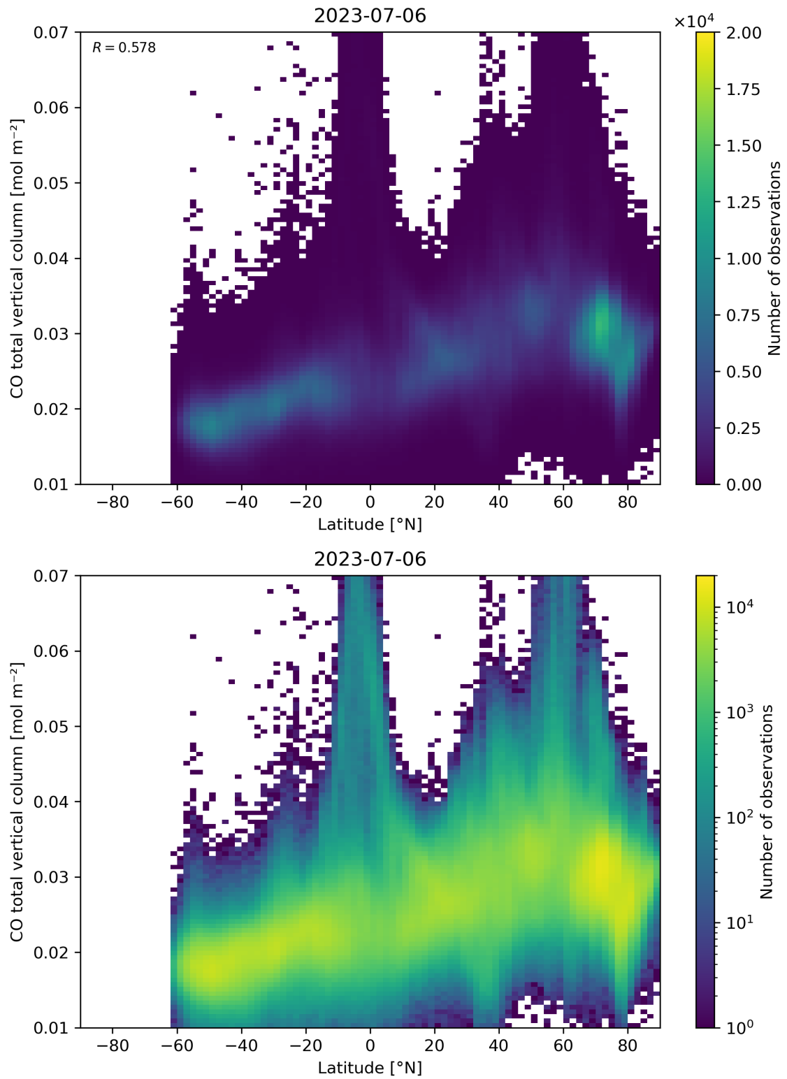
Figure 51: Scatter density plot of “Latitude” against “CO total vertical column” for 2023-07-05 to 2023-07-07.
