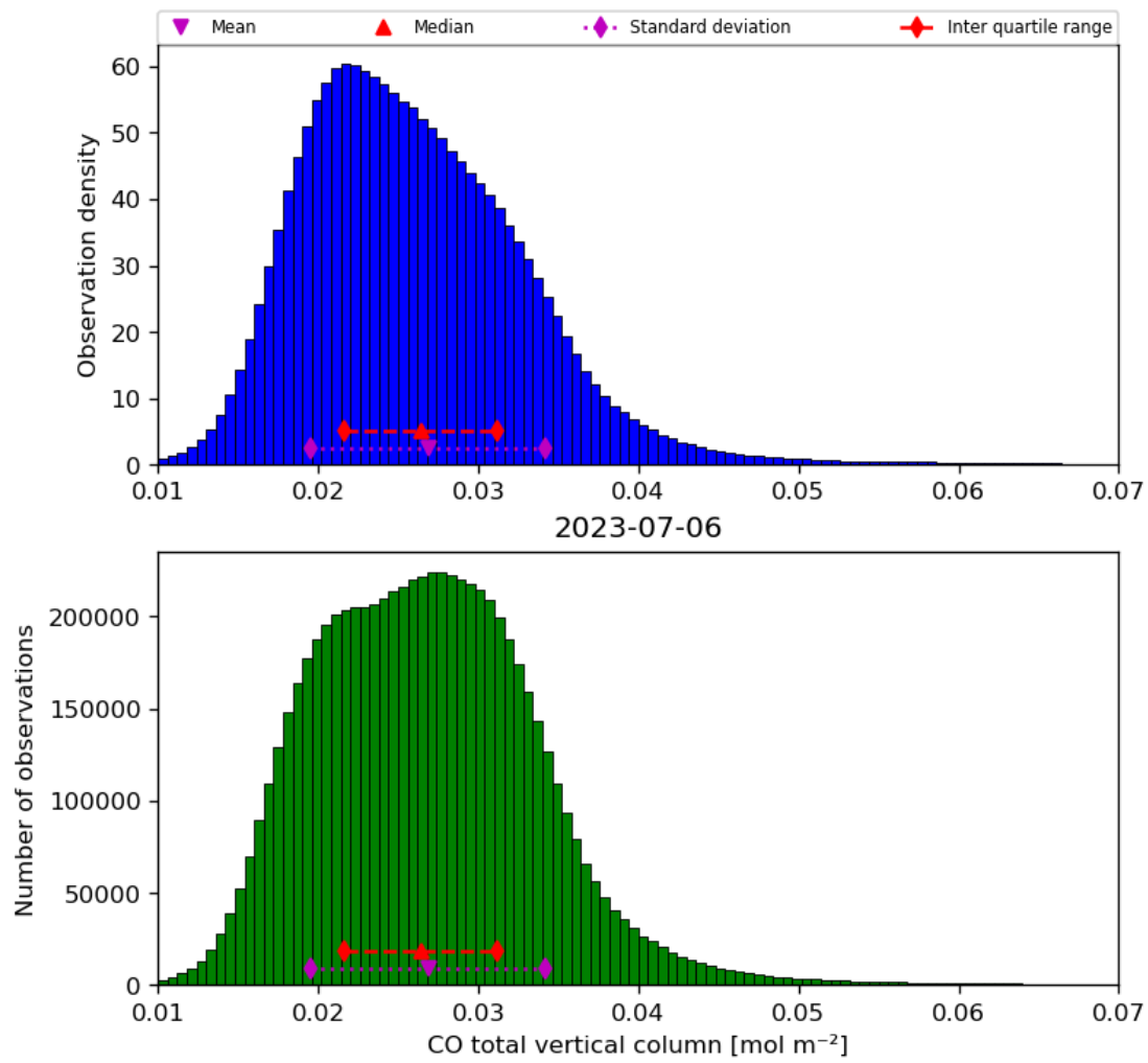
Figure 18: Histogram of “CO total vertical column” for 2023-07-05 to 2023-07-07
