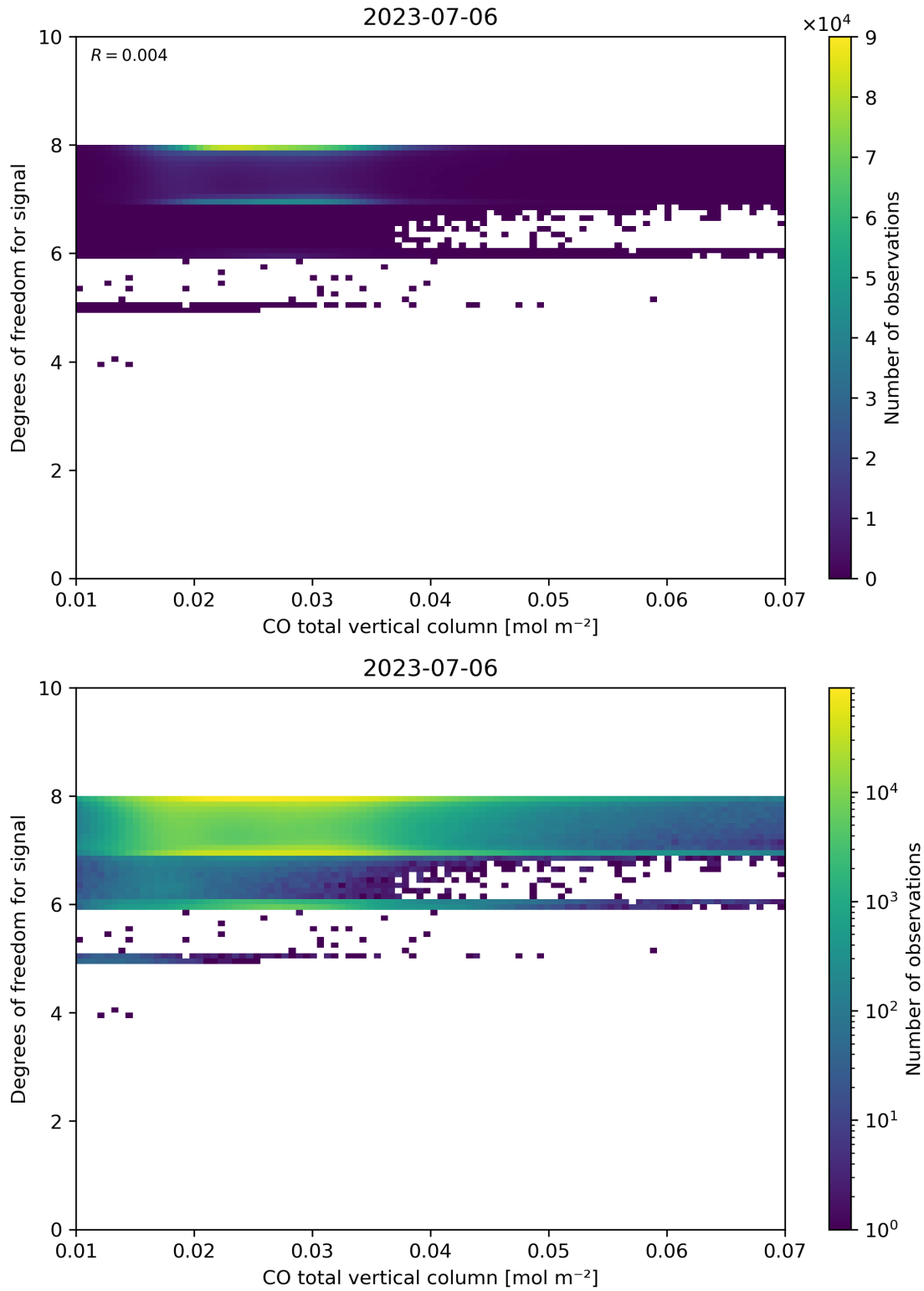
Figure 41: Scatter density plot of “CO total vertical column” against “Degrees of freedom for signal” for 2023-07-05 to 2023-07-07.
