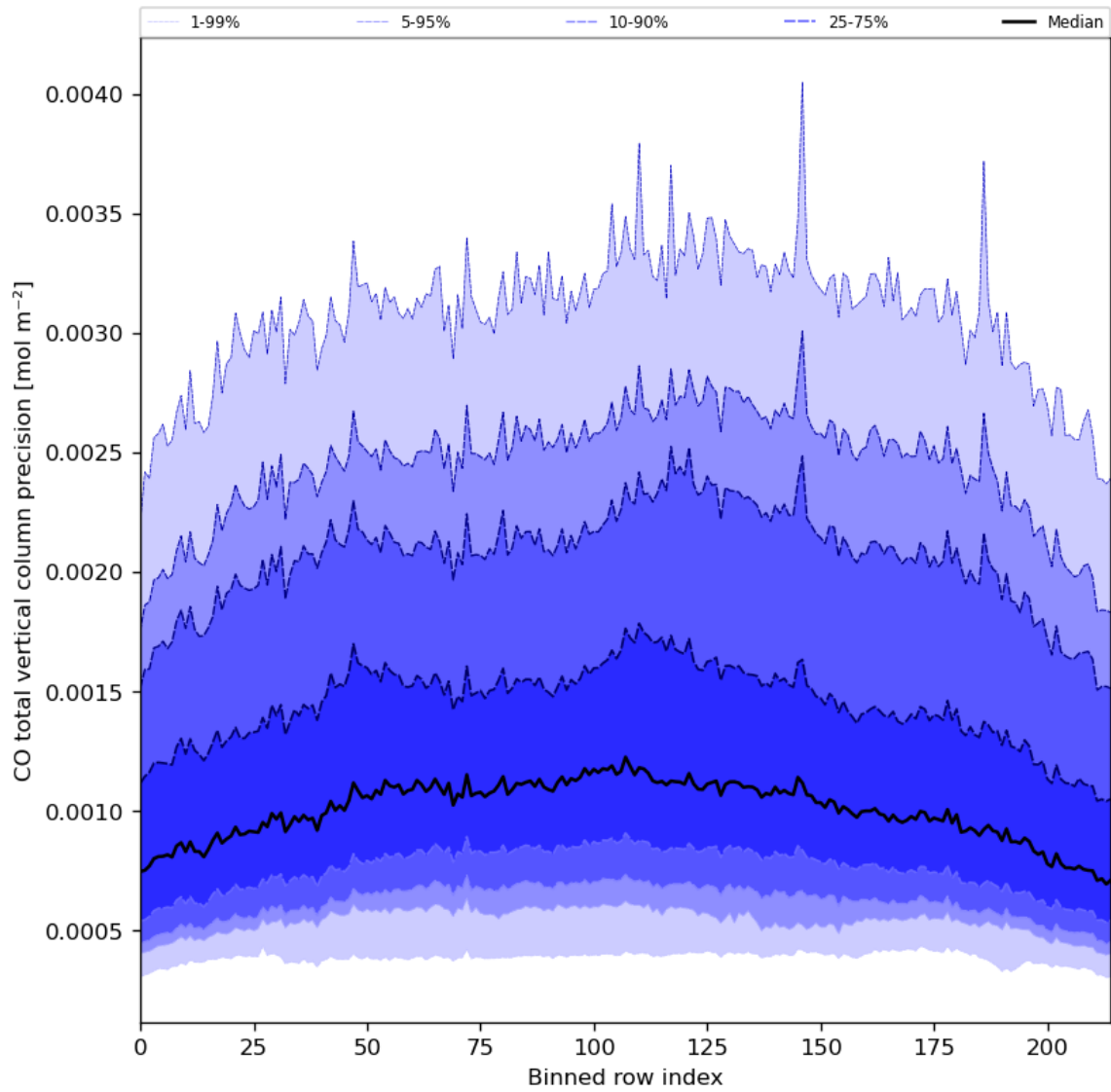
Figure 28: Along track statistics of “CO total vertical column precision” for 2023-07-05 to 2023-07-07
