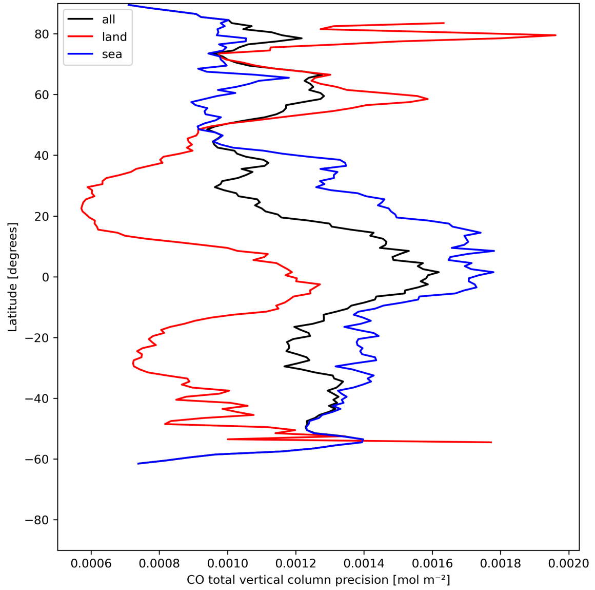
Figure 12: Zonal average of “CO total vertical column precision” for 2023-07-05 to 2023-07-07.
