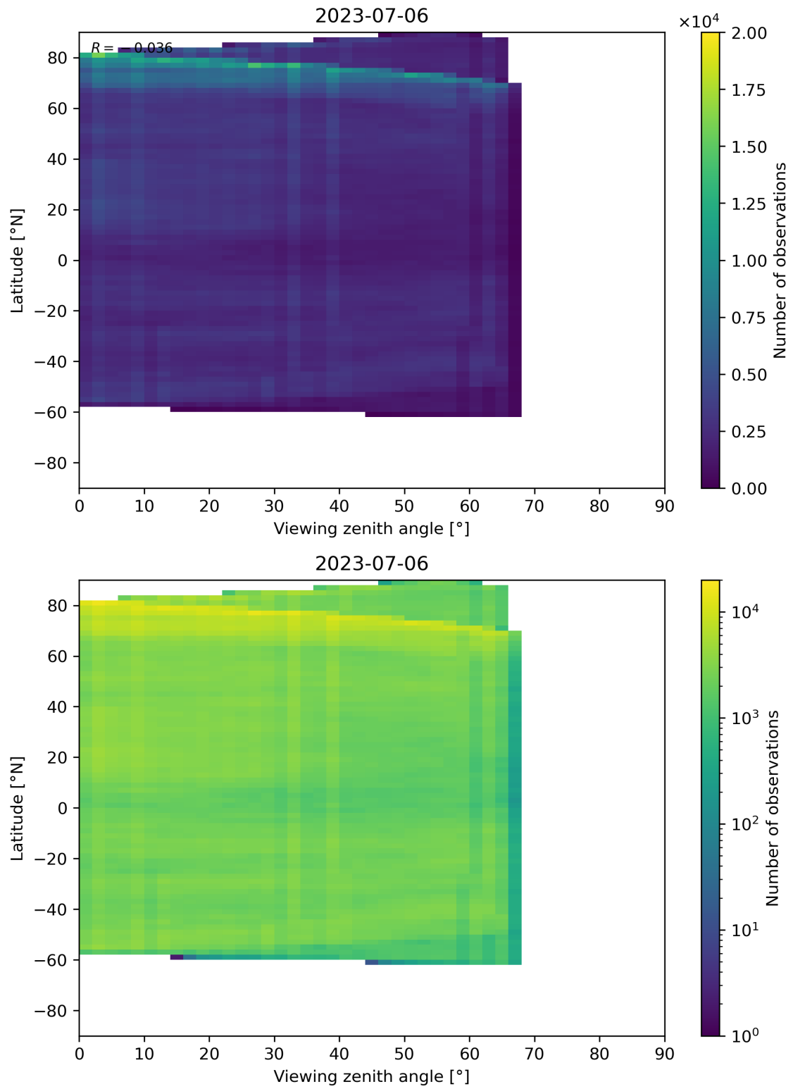
Figure 74: Scatter density plot of “Viewing zenith angle” against “Latitude” for 2023-07-05 to 2023-07-07.
