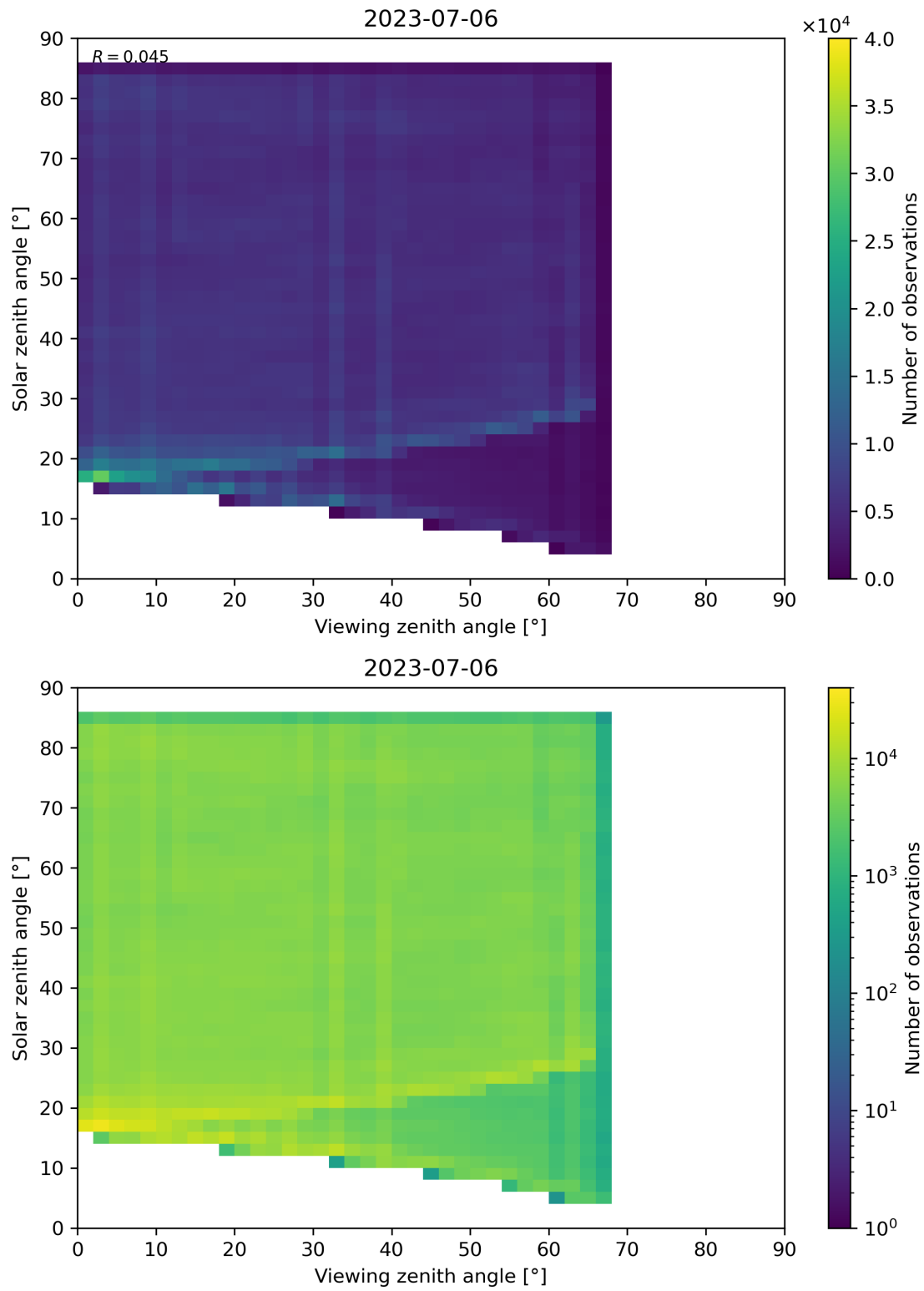
Figure 77: Scatter density plot of “Viewing zenith angle” against “Solar zenith angle” for 2023-07-05 to 2023-07-07.
