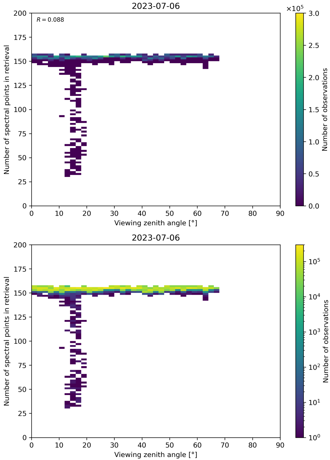
Figure 76: Scatter density plot of “Viewing zenith angle” against “Number of spectral points in retrieval” for 2023-07-05 to 2023-07-07.
