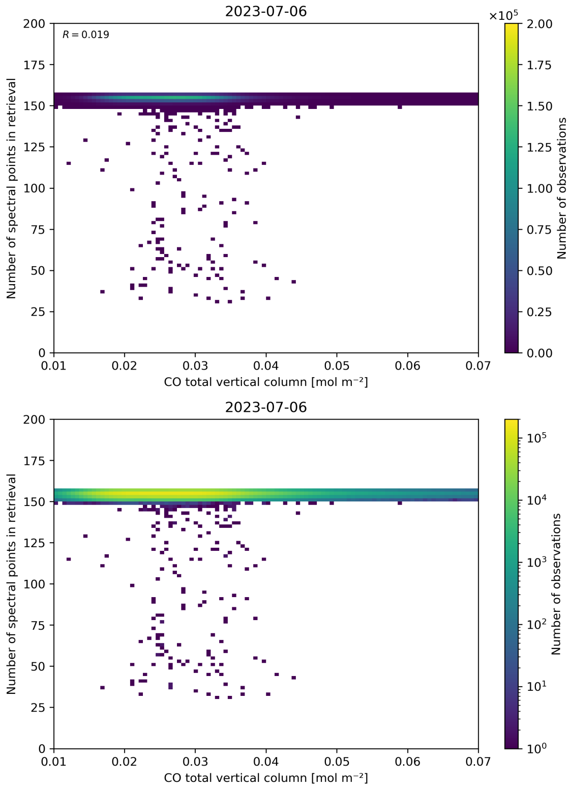
Figure 43: Scatter density plot of “CO total vertical column” against “Number of spectral points in retrieval” for 2023-07-05 to 2023-07-07.
