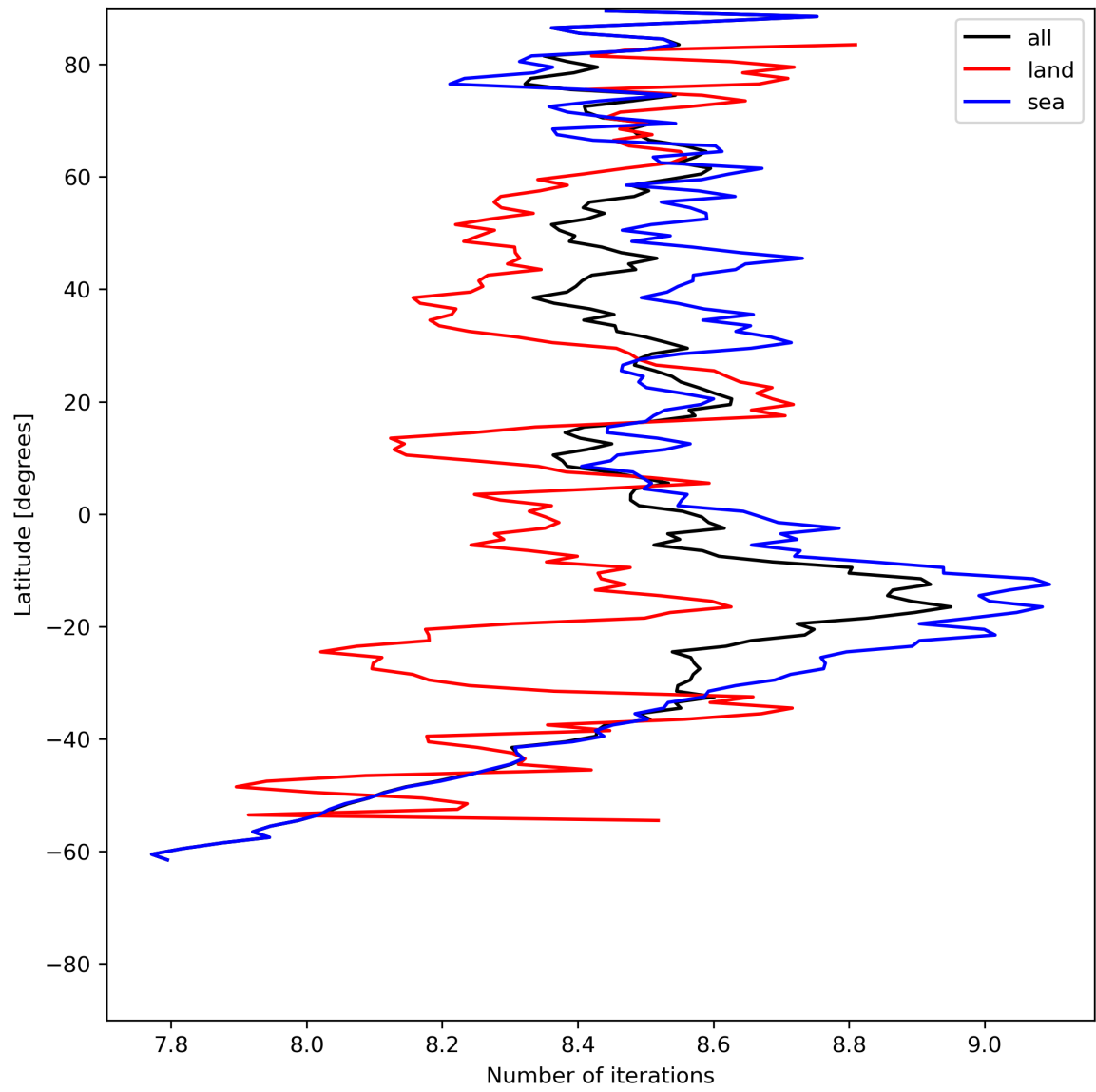
Figure 16: Zonal average of “Number of iterations” for 2023-07-05 to 2023-07-07.
