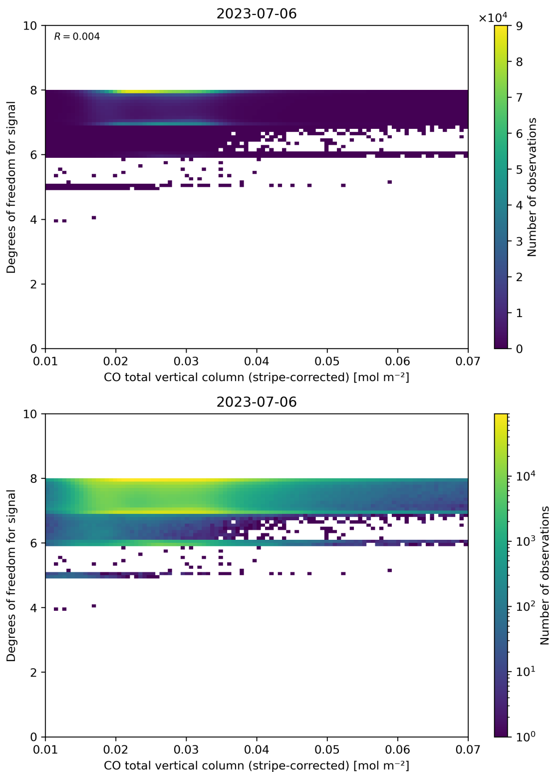
Figure 38: Scatter density plot of “CO total vertical column (stripe-corrected)” against “Degrees of freedom for signal” for 2023-07-05 to 2023-07-07.
