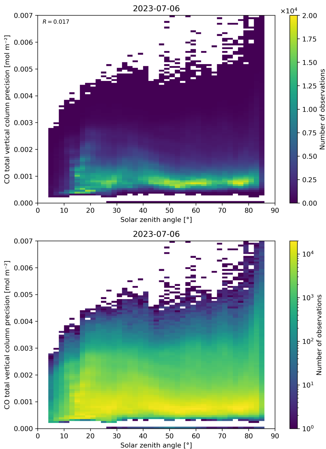
Figure 63: Scatter density plot of “Solar zenith angle” against “CO total vertical column precision” for 2023-07-05 to 2023-07-07.
