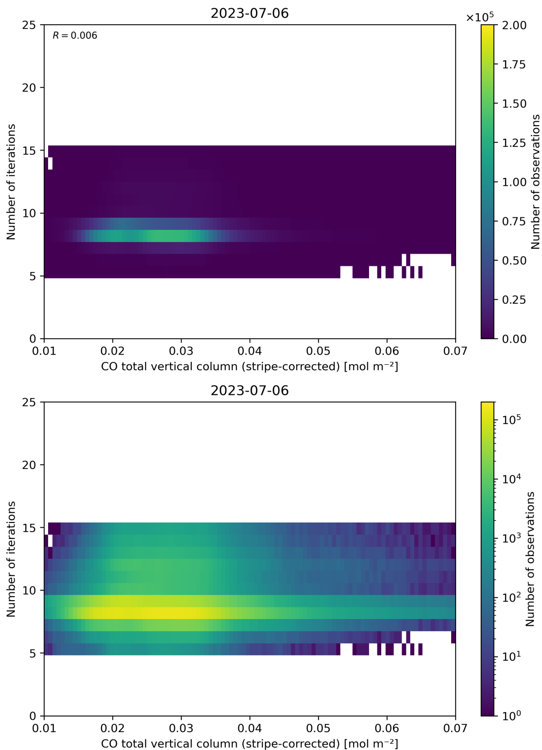
Figure 39: Scatter density plot of “CO total vertical column (stripe-corrected)” against “Number of iterations” for 2023-07-05 to 2023-07-07.
