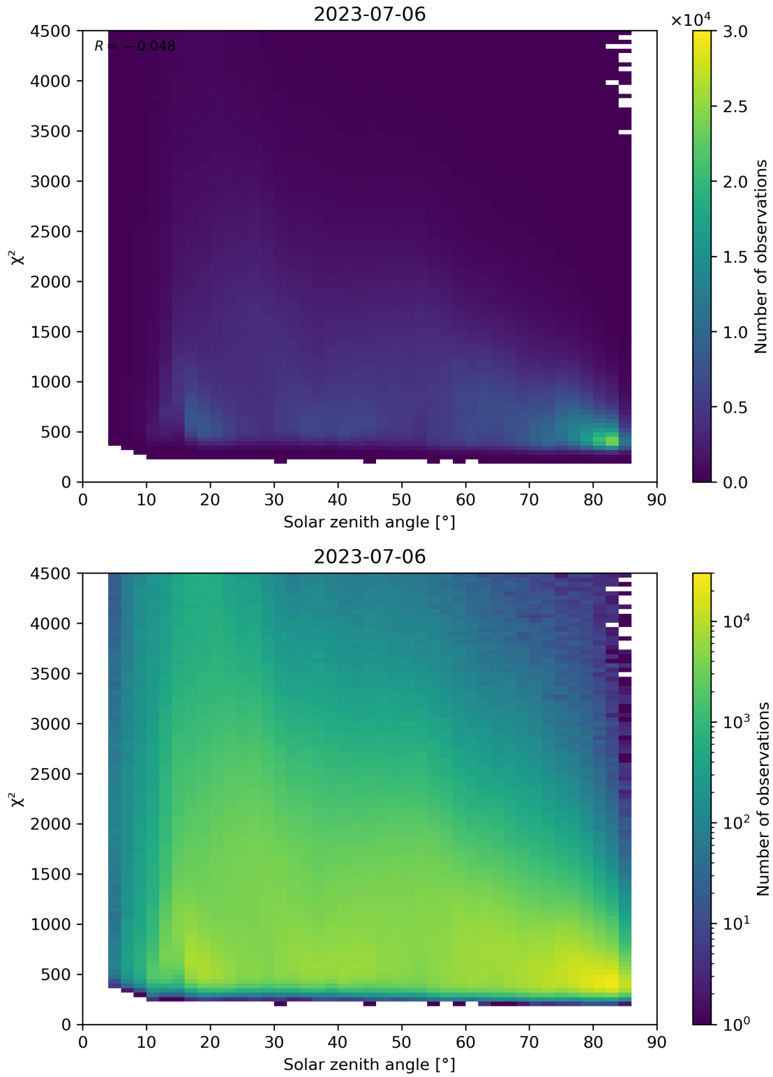
Figure 64: Scatter density plot of “Solar zenith angle” against “ \chi^2 ” for 2023-07-05 to 2023-07-07.
