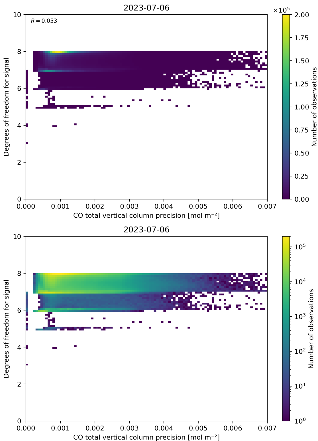
Figure 45: Scatter density plot of “CO total vertical column precision” against “Degrees of freedom for signal” for 2023-07-05 to 2023-07-07.
