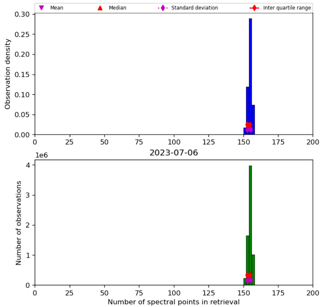
Figure 21: Histogram of “Number of spectral points in retrieval” for 2023-07-05 to 2023-07-07
