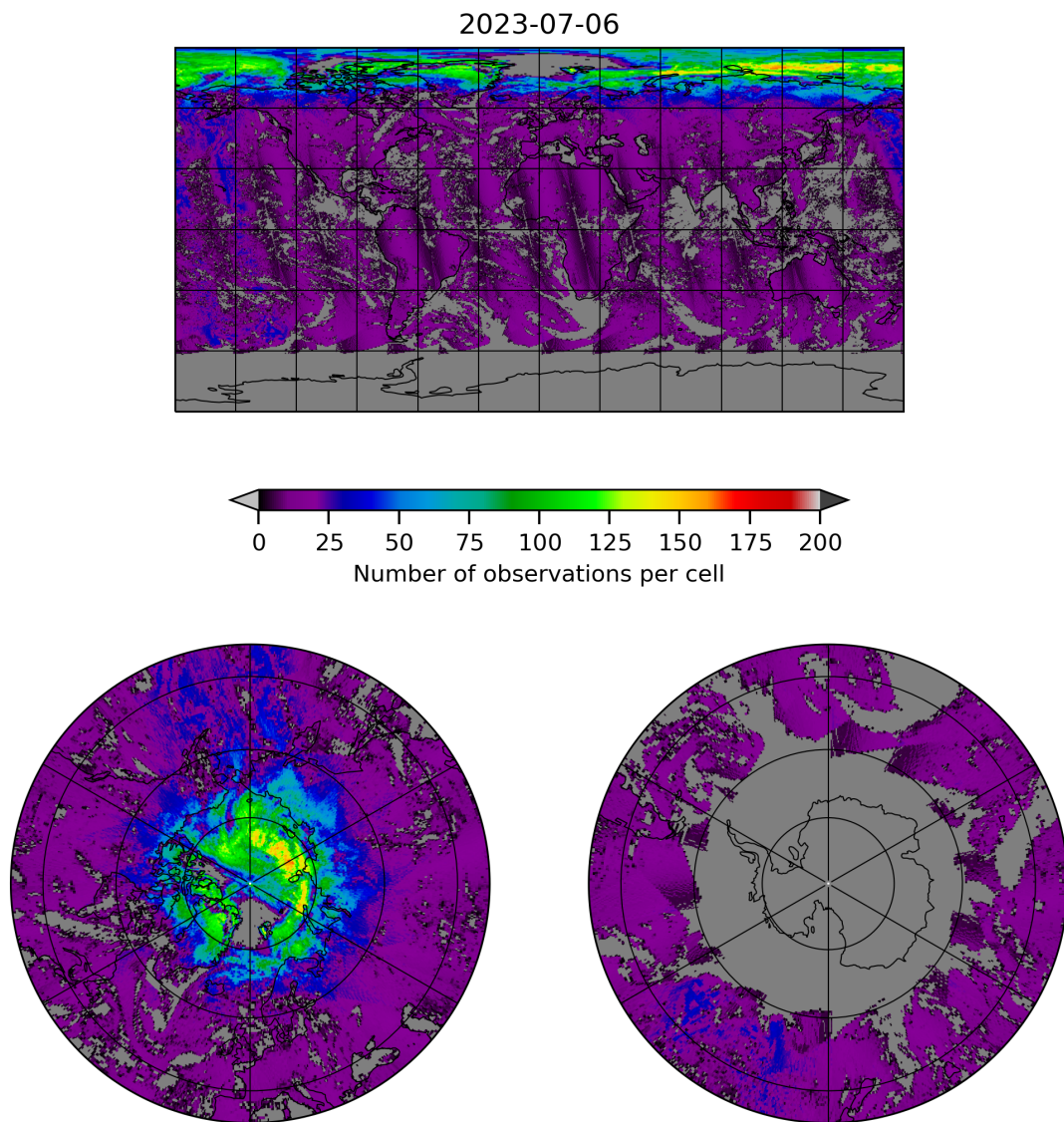
Figure 8: Map of the number of observations for 2023-07-05 to 2023-07-07
