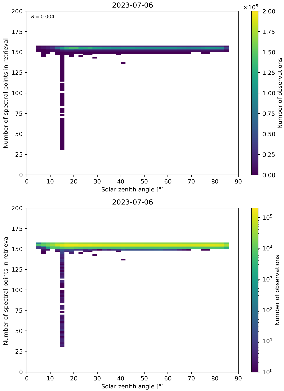
Figure 68: Scatter density plot of “Solar zenith angle” against “Number of spectral points in retrieval” for 2023-07-05 to 2023-07-07.
