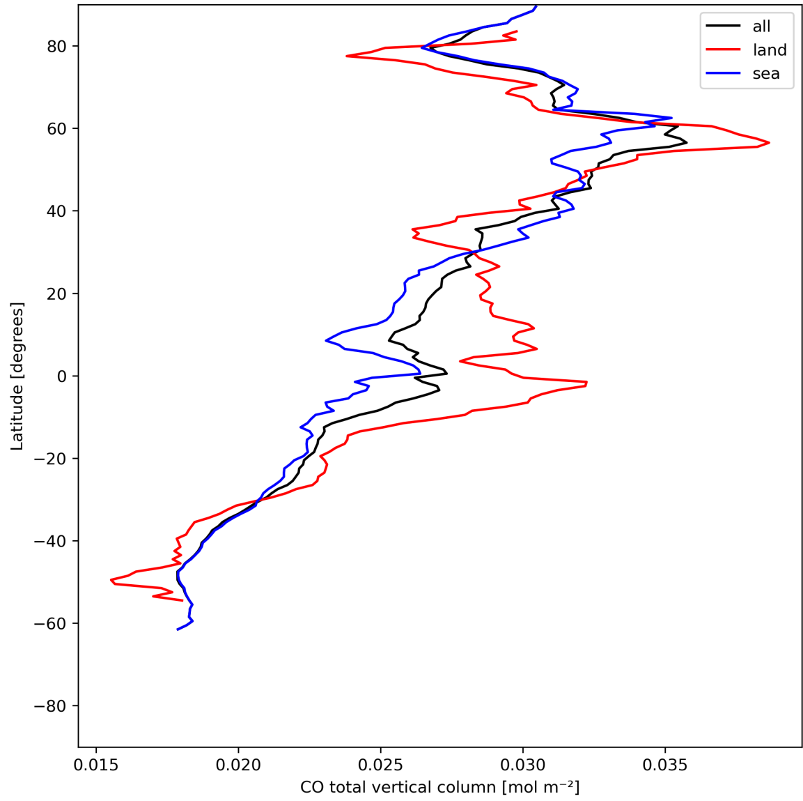
Figure 10: Zonal average of “CO total vertical column” for 2023-07-05 to 2023-07-07.
