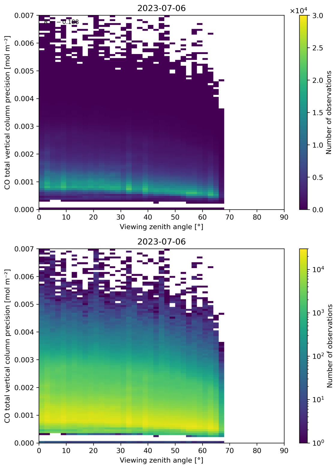
Figure 71: Scatter density plot of “Viewing zenith angle” against “CO total vertical column precision” for 2023-07-05 to 2023-07-07.
