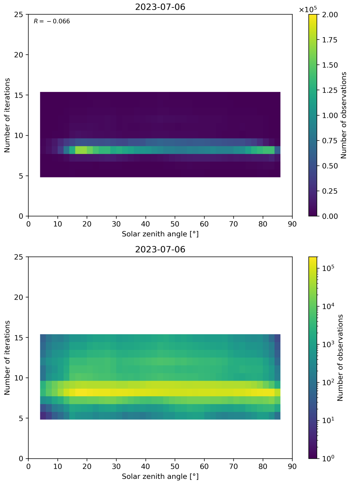
Figure 67: Scatter density plot of “Solar zenith angle” against “Number of iterations” for 2023-07-05 to 2023-07-07.
