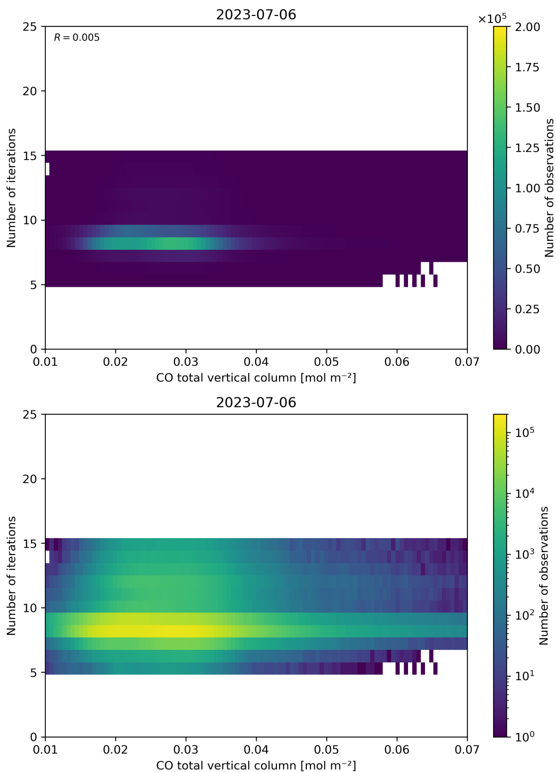
Figure 42: Scatter density plot of “CO total vertical column” against “Number of iterations” for 2023-07-05 to 2023-07-07.
