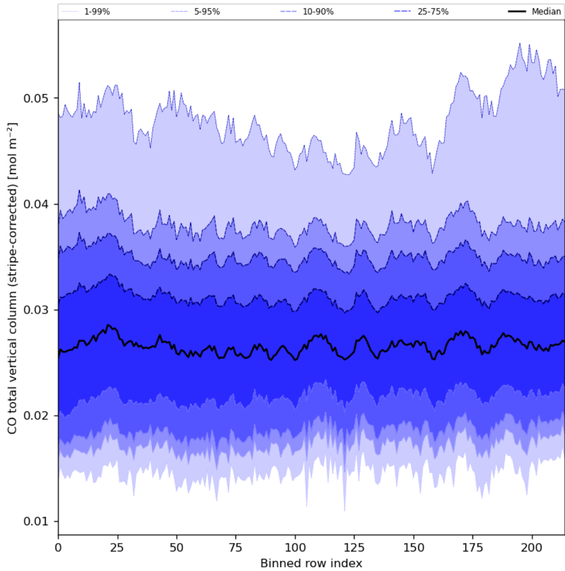
Figure 27: Along track statistics of “CO total vertical column (stripe-corrected)” for 2023-07-05 to 2023-07-07
