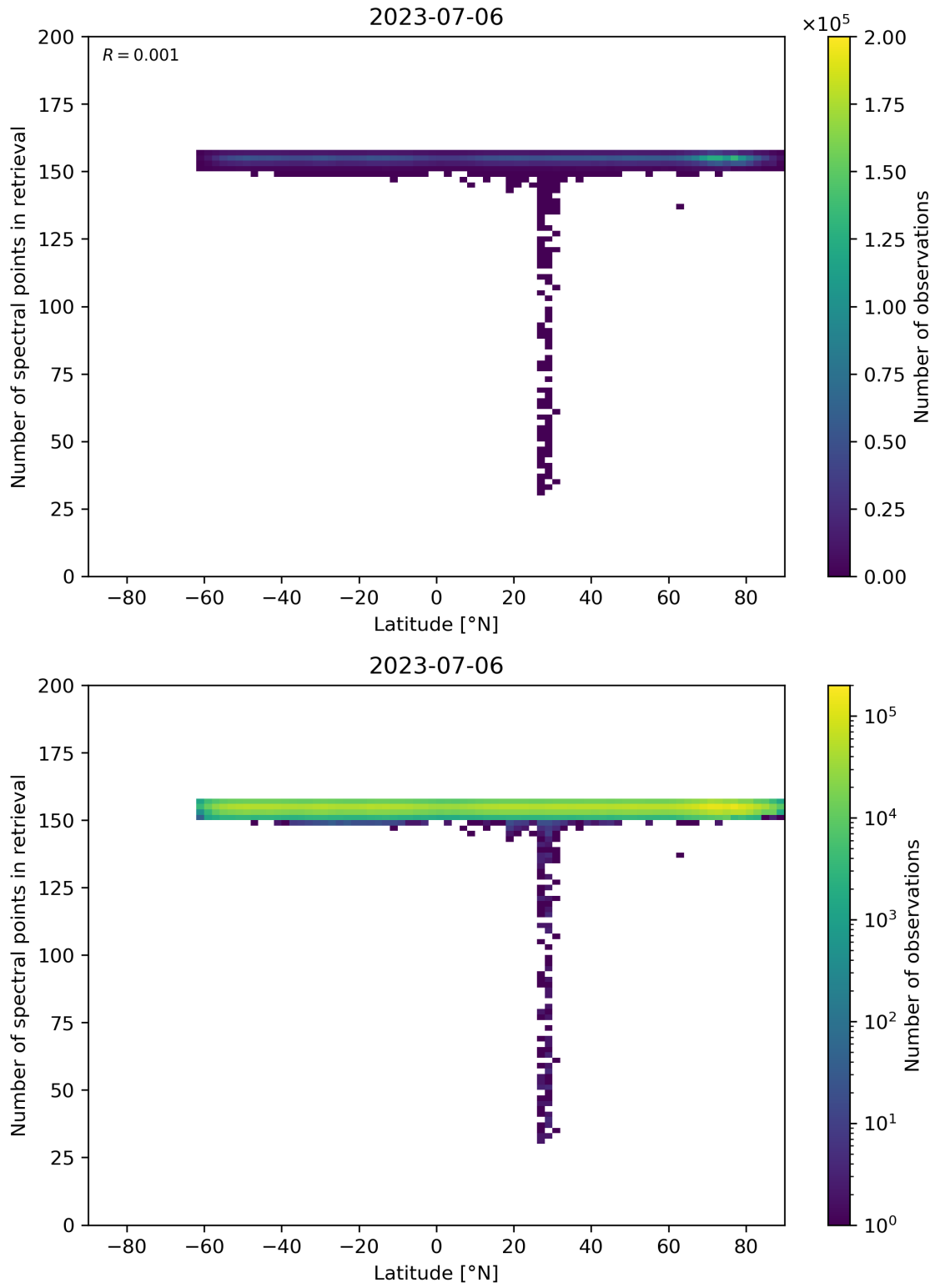
Figure 57: Scatter density plot of “Latitude” against “Number of spectral points in retrieval” for 2023-07-05 to 2023-07-07.
