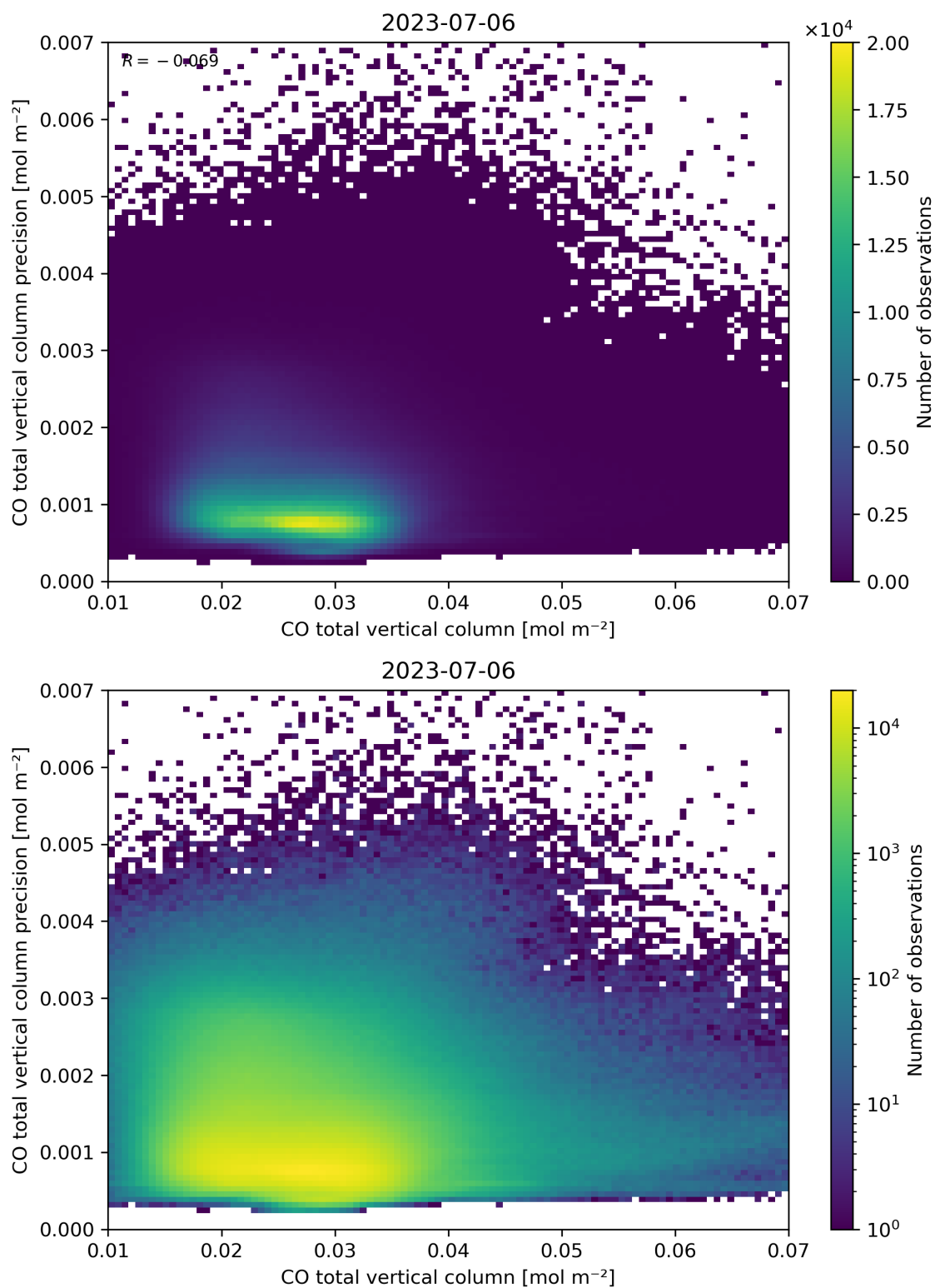
Figure 34: Scatter density plot of “CO total vertical column” against “CO total vertical column precision” for 2023-07-05 to 2023-07-07.
