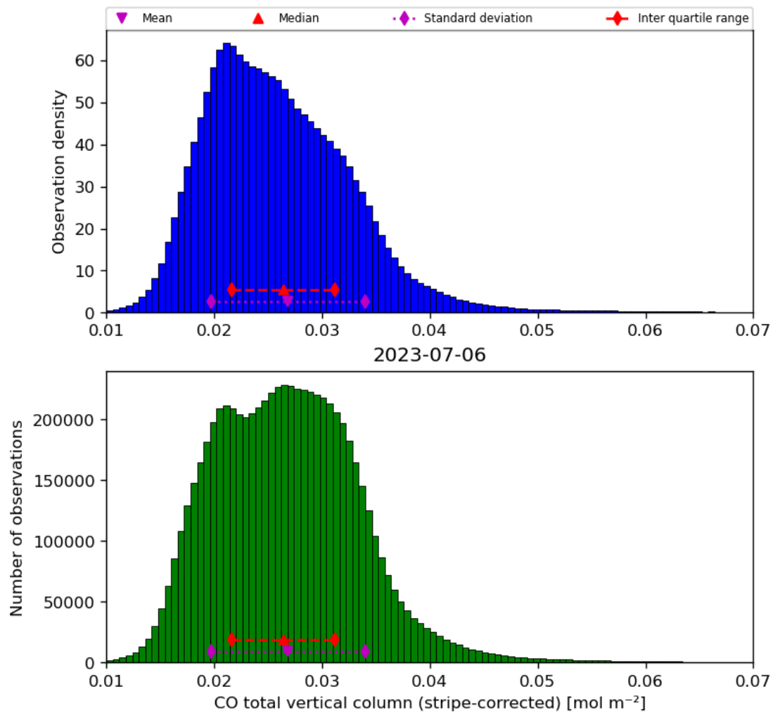
Figure 19: Histogram of “CO total vertical column (stripe-corrected)” for 2023-07-05 to 2023-07-07
