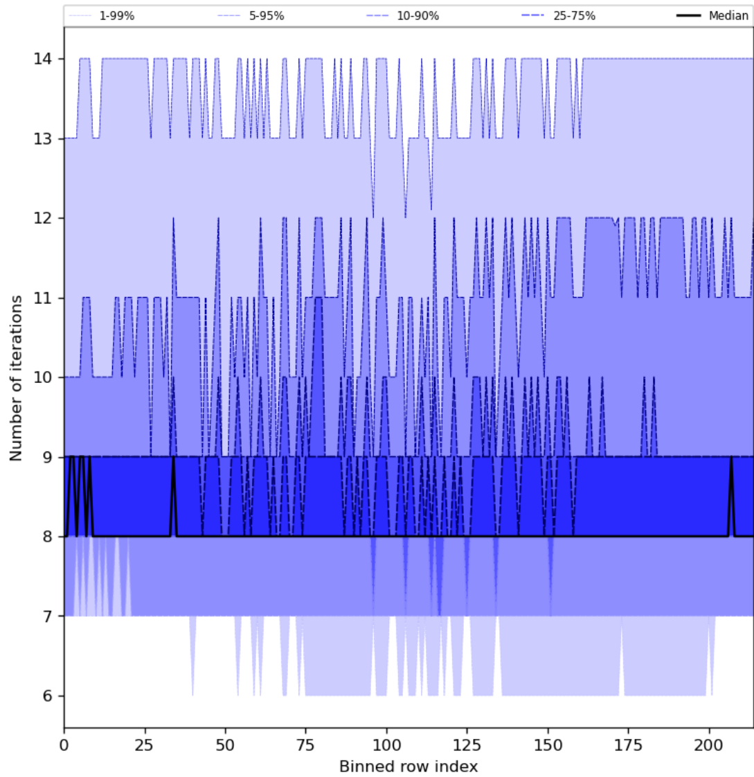
Figure 32: Along track statistics of “Number of iterations” for 2023-07-05 to 2023-07-07
