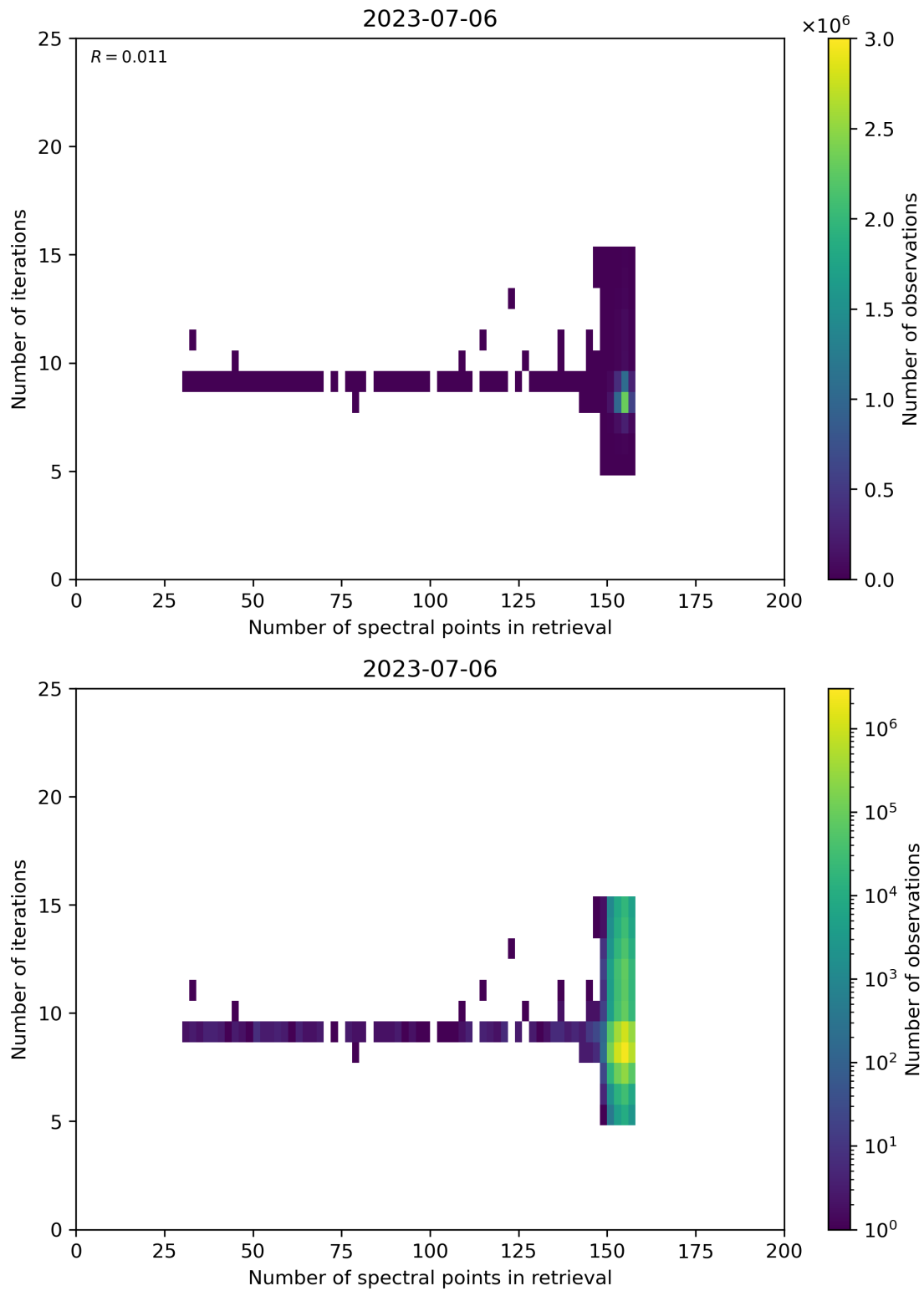
Figure 60: Scatter density plot of “Number of spectral points in retrieval” against “Number of iterations” for 2023-07-05 to 2023-07-07.
