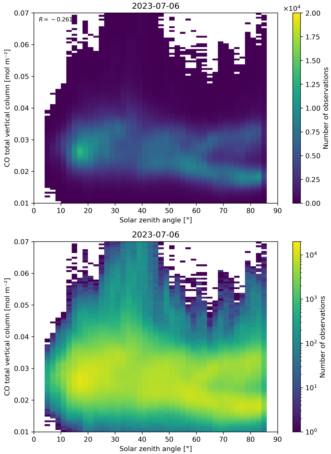
Figure 61: Scatter density plot of “Solar zenith angle” against “CO total vertical column” for 2023-07-05 to 2023-07-07.
