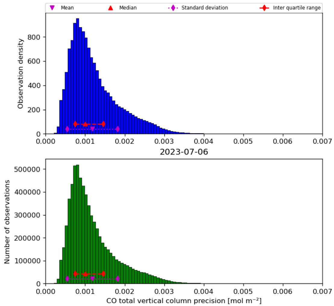
Figure 20: Histogram of “CO total vertical column precision” for 2023-07-05 to 2023-07-07
