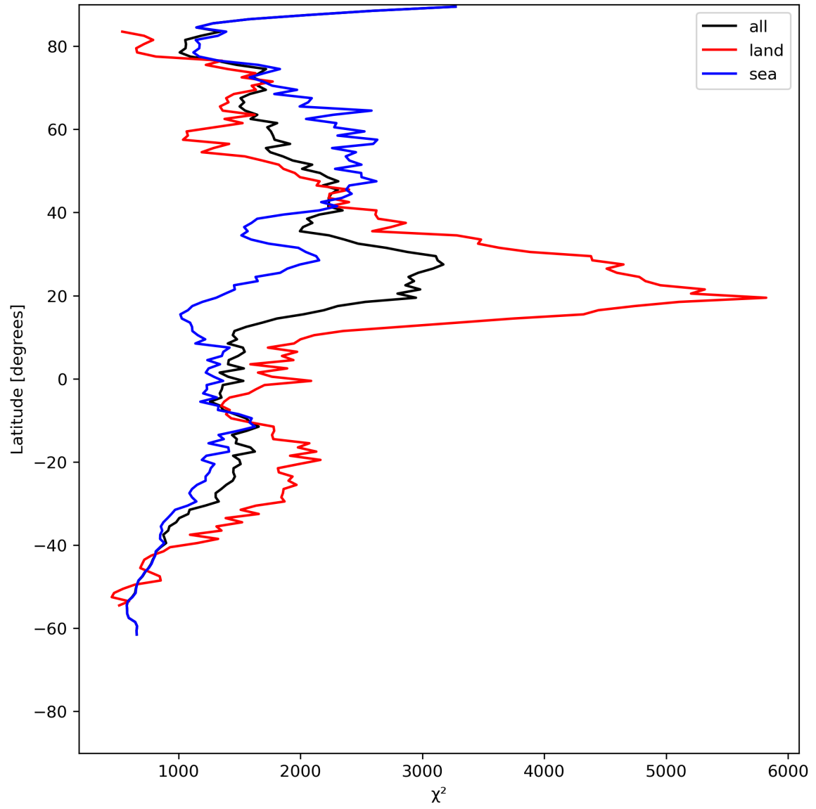
Figure 14: Zonal average of “ \chi^2 ” for 2023-07-05 to 2023-07-07.
