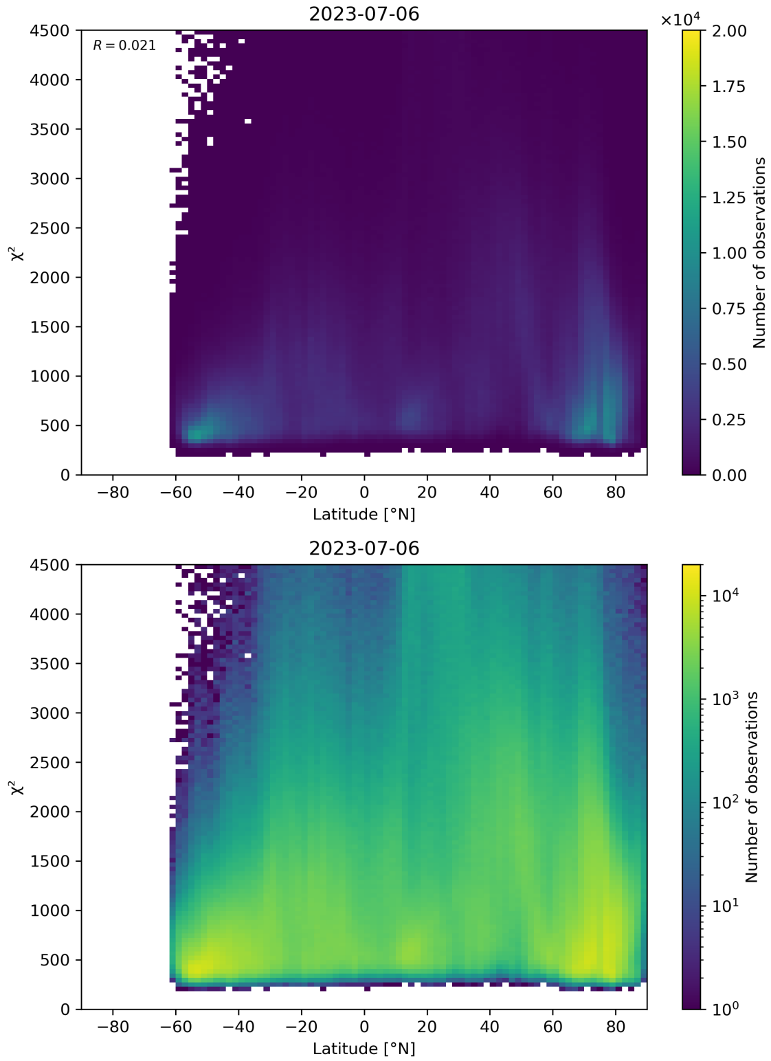
Figure 54: Scatter density plot of “Latitude” against “ \chi^2 ” for 2023-07-05 to 2023-07-07.
