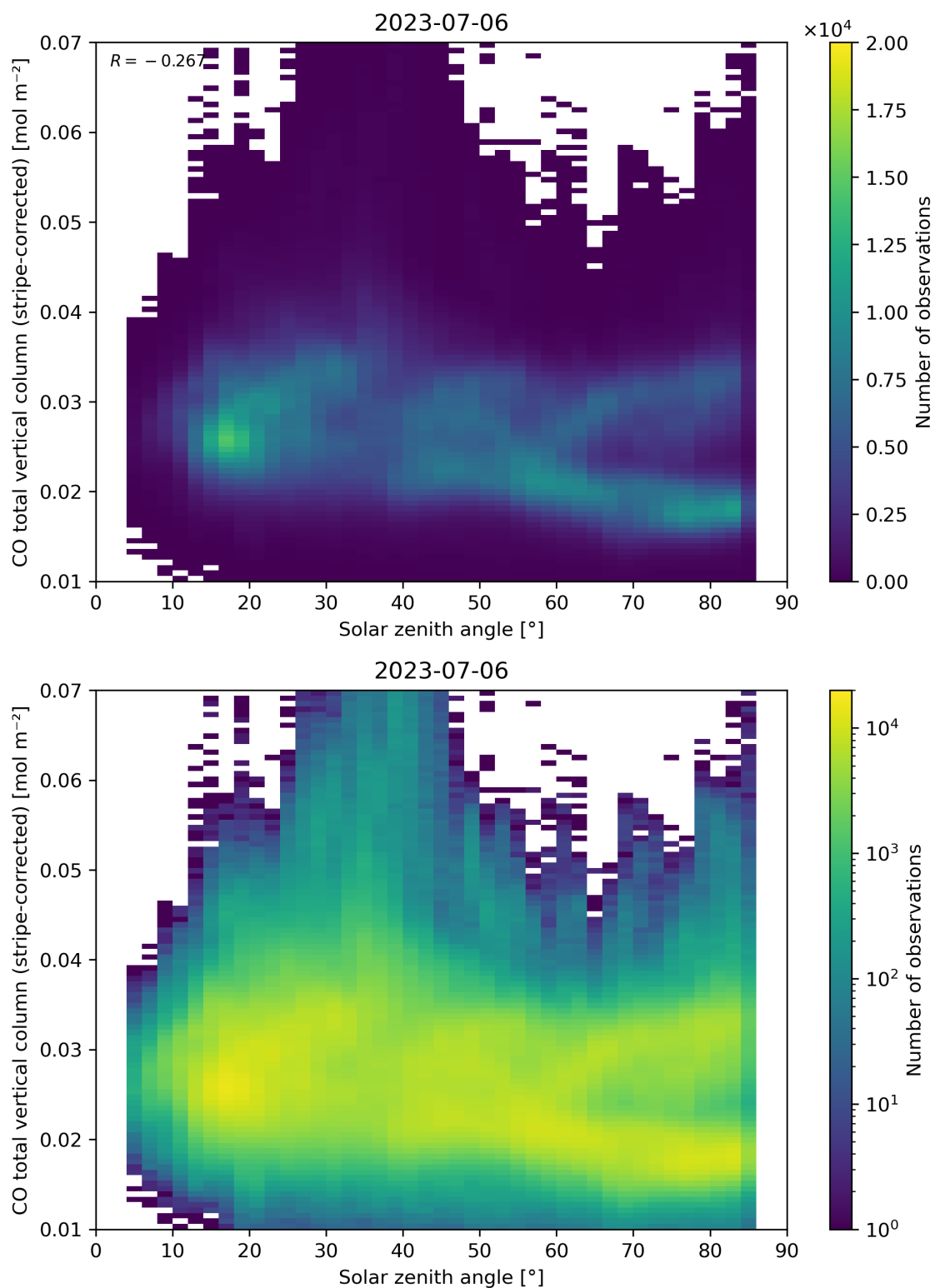
Figure 62: Scatter density plot of “Solar zenith angle” against “CO total vertical column (stripe-corrected)” for 2023-07-05 to 2023-07-07.
