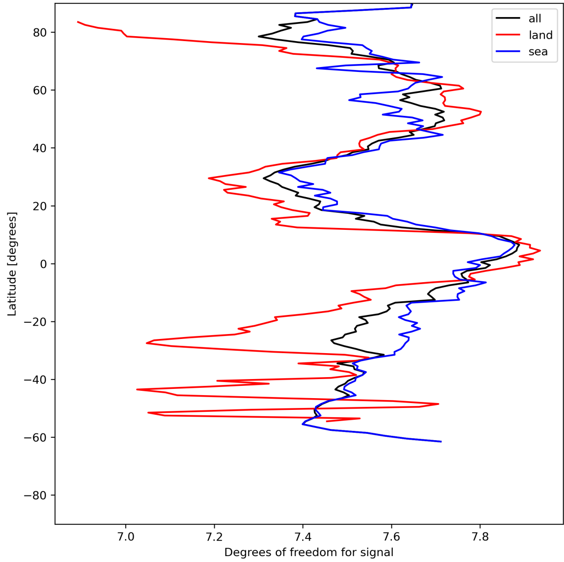
Figure 15: Zonal average of “Degrees of freedom for signal” for 2023-07-05 to 2023-07-07.
