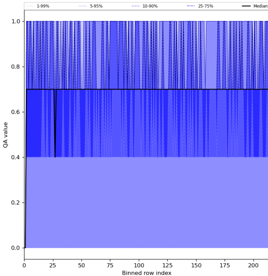
Figure 25: Along track statistics of “QA value” for 2023-07-05 to 2023-07-07
