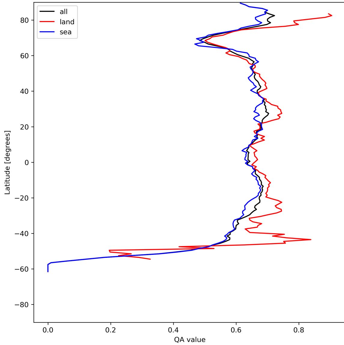
Figure 9: Zonal average of “QA value” for 2023-07-05 to 2023-07-07.
