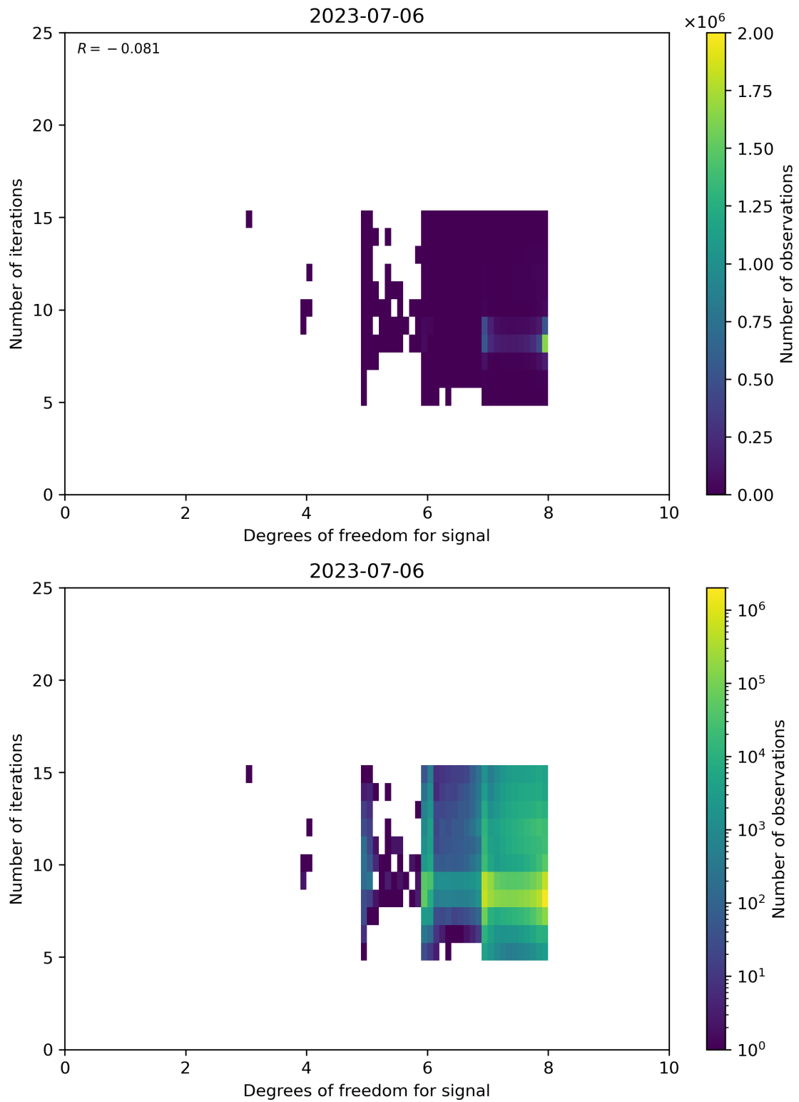
Figure 50: Scatter density plot of “Degrees of freedom for signal” against “Number of iterations” for 2023-07-05 to 2023-07-07.
