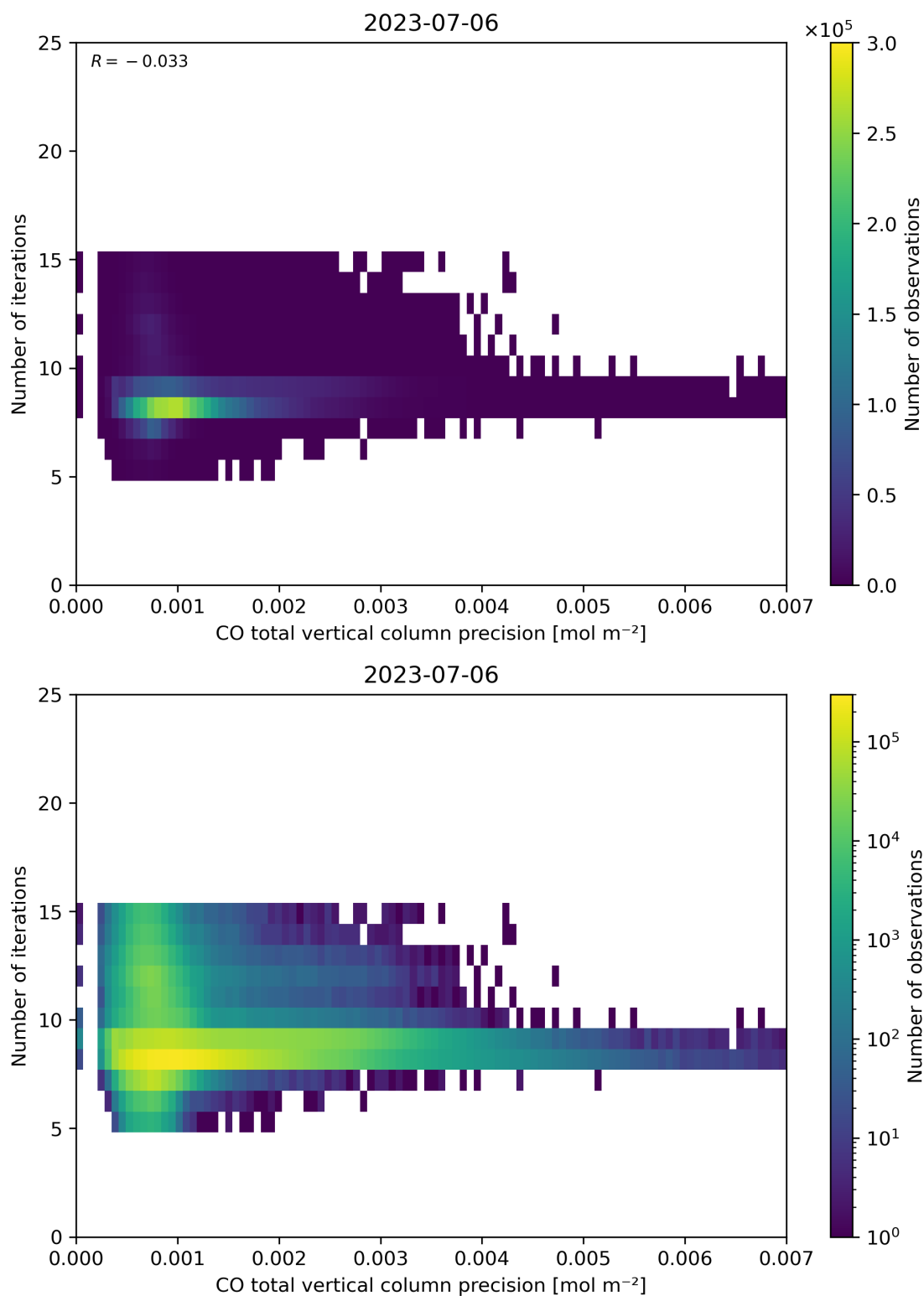
Figure 46: Scatter density plot of “CO total vertical column precision” against “Number of iterations” for 2023-07-05 to 2023-07-07.
