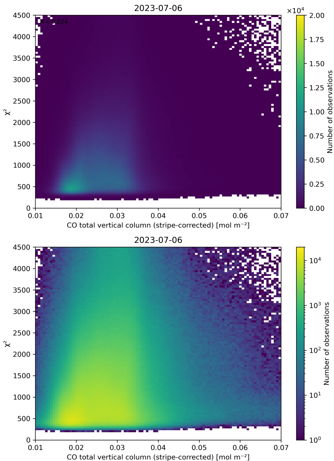
Figure 37: Scatter density plot of “CO total vertical column (stripe-corrected)” against “ \chi^2 ” for 2023-07-05 to 2023-07-07.
