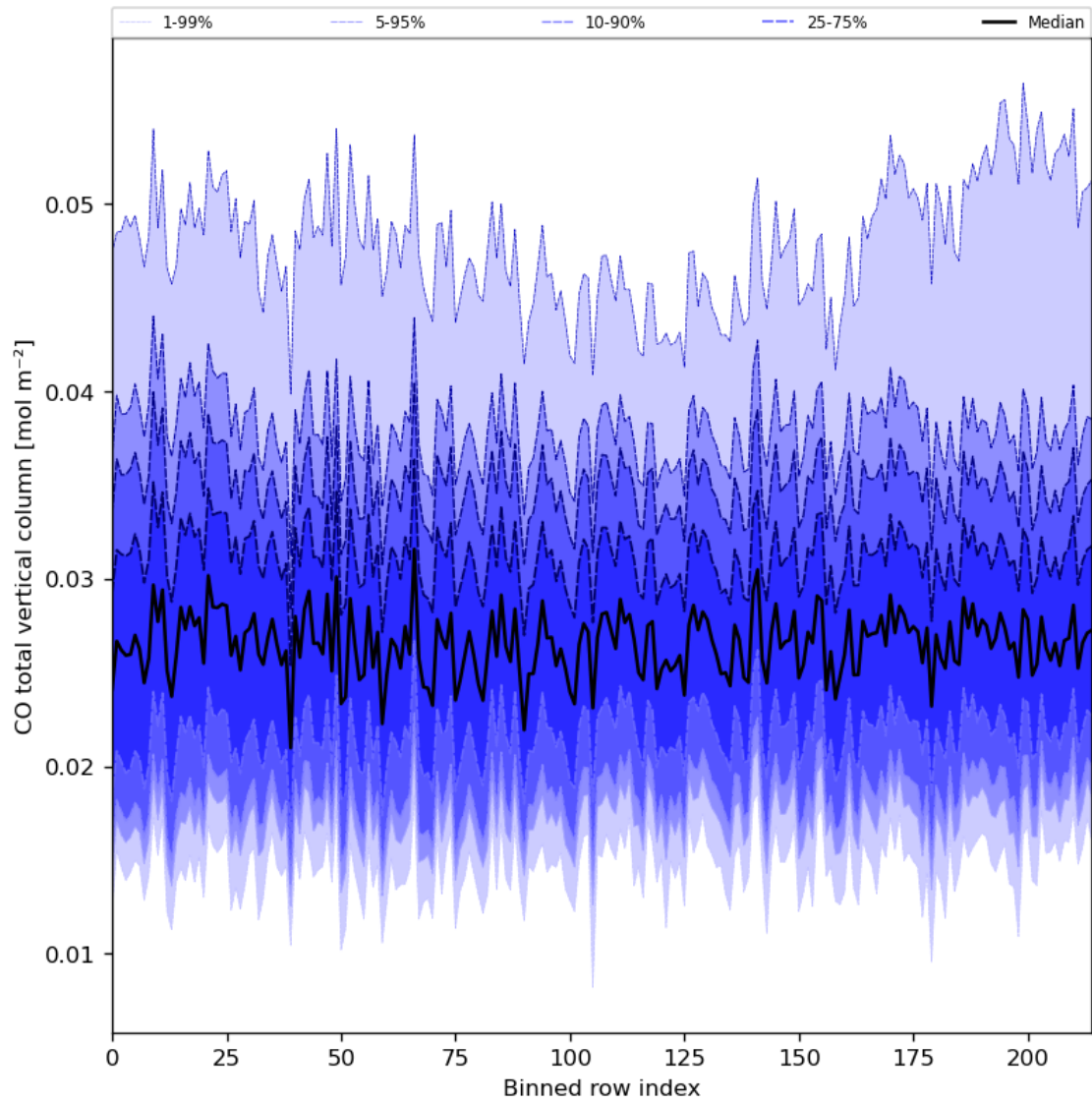
Figure 26: Along track statistics of “CO total vertical column” for 2023-07-05 to 2023-07-07
