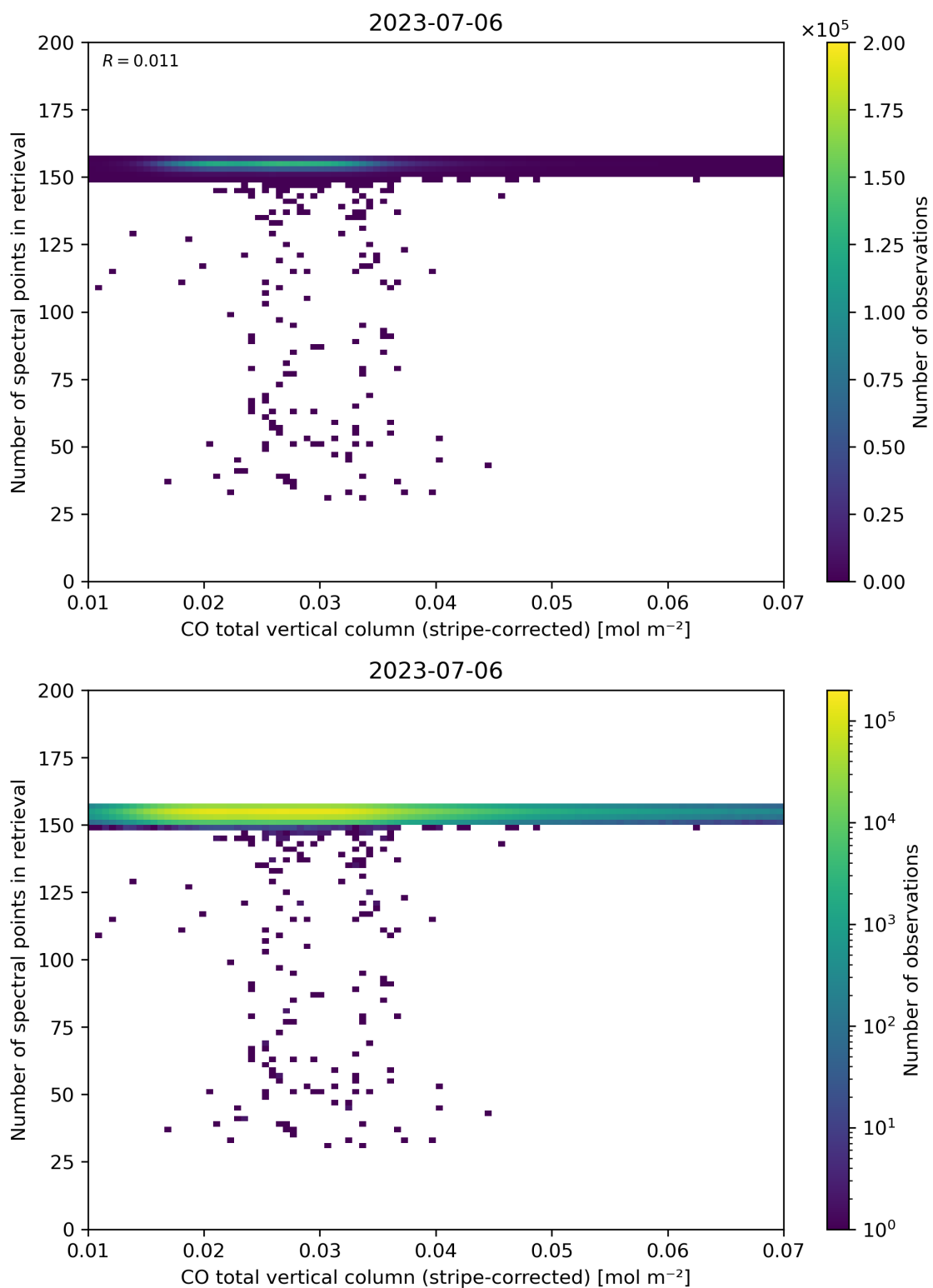
Figure 40: Scatter density plot of “CO total vertical column (stripe-corrected)” against “Number of spectral points in retrieval” for 2023-07-05 to 2023-07-07.
