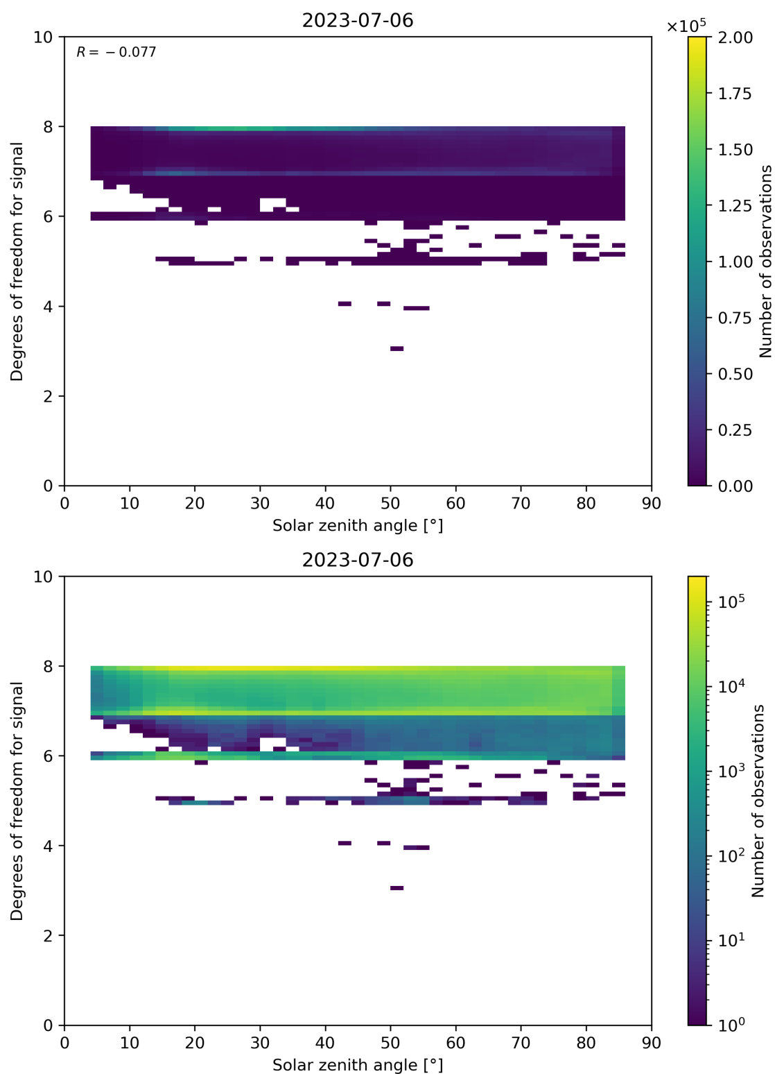
Figure 65: Scatter density plot of “Solar zenith angle” against “Degrees of freedom for signal” for 2023-07-05 to 2023-07-07.
