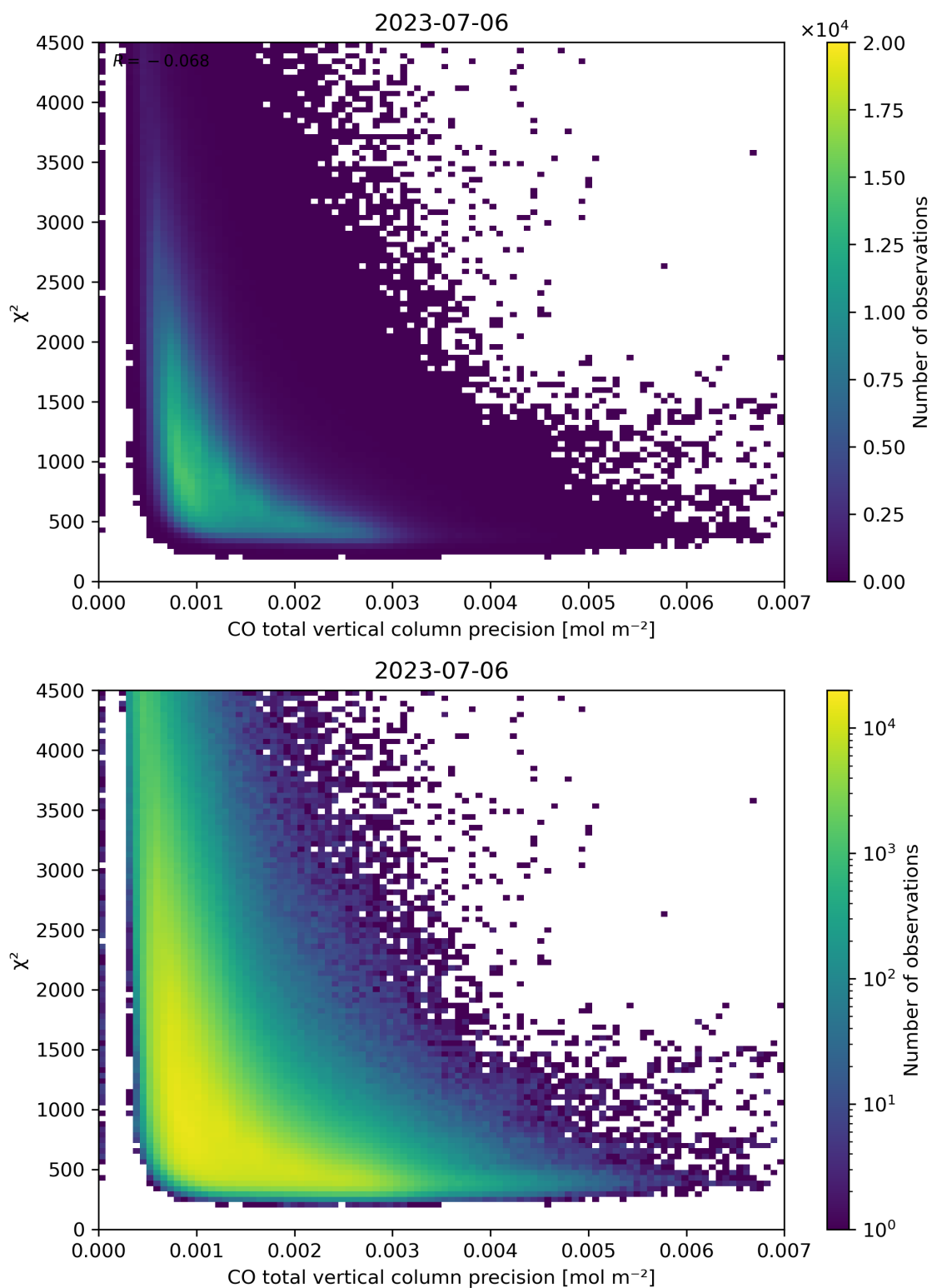
Figure 44: Scatter density plot of “CO total vertical column precision” against “ \chi^2 ” for 2023-07-05 to 2023-07-07.
