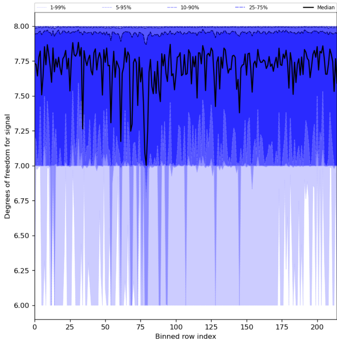
Figure 31: Along track statistics of “Degrees of freedom for signal” for 2023-07-05 to 2023-07-07
