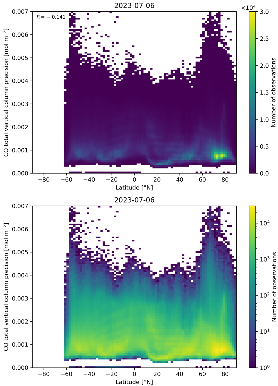
Figure 53: Scatter density plot of “Latitude” against “CO total vertical column precision” for 2023-07-05 to 2023-07-07.
