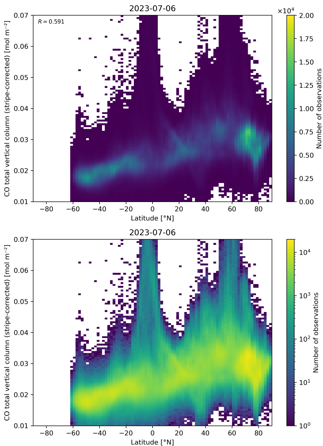
Figure 52: Scatter density plot of “Latitude” against “CO total vertical column (stripe-corrected)” for 2023-07-05 to 2023-07-07.
