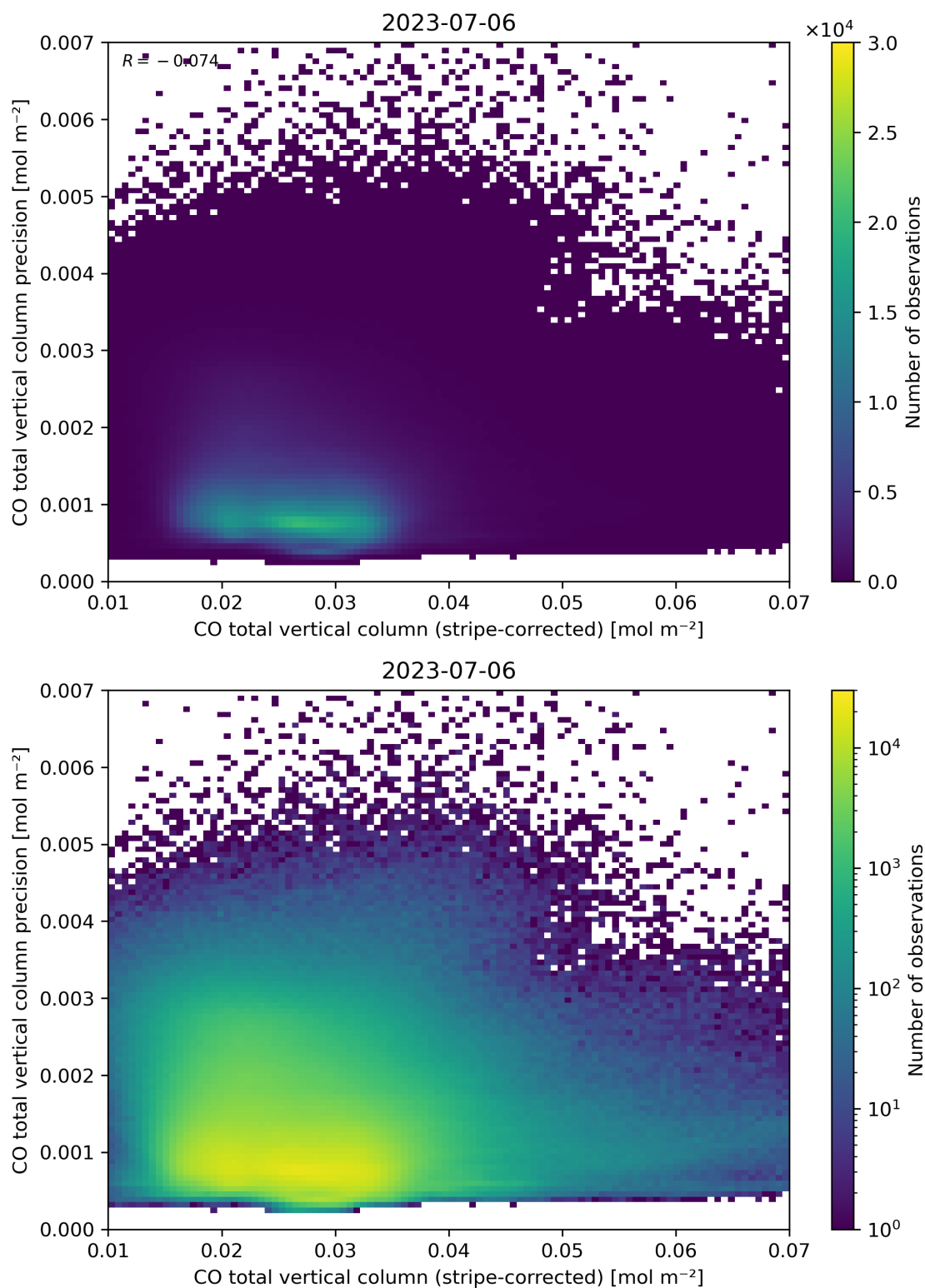
Figure 36: Scatter density plot of “CO total vertical column (stripe-corrected)” against “CO total vertical column precision” for 2023-07-05 to 2023-07-07.
