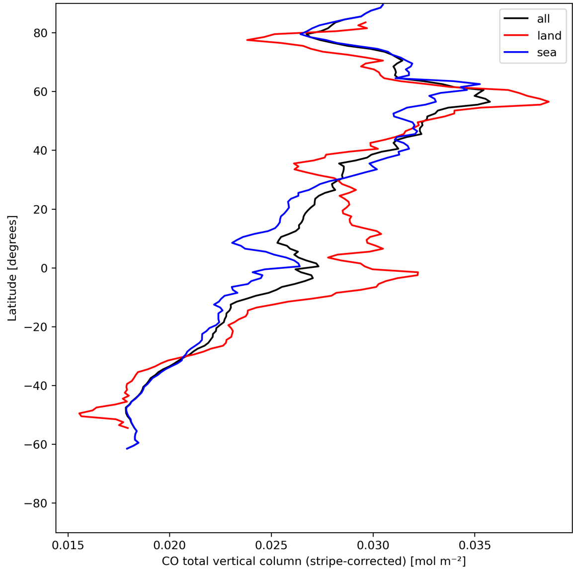
Figure 11: Zonal average of “CO total vertical column (stripe-corrected)” for 2023-07-05 to 2023-07-07.
