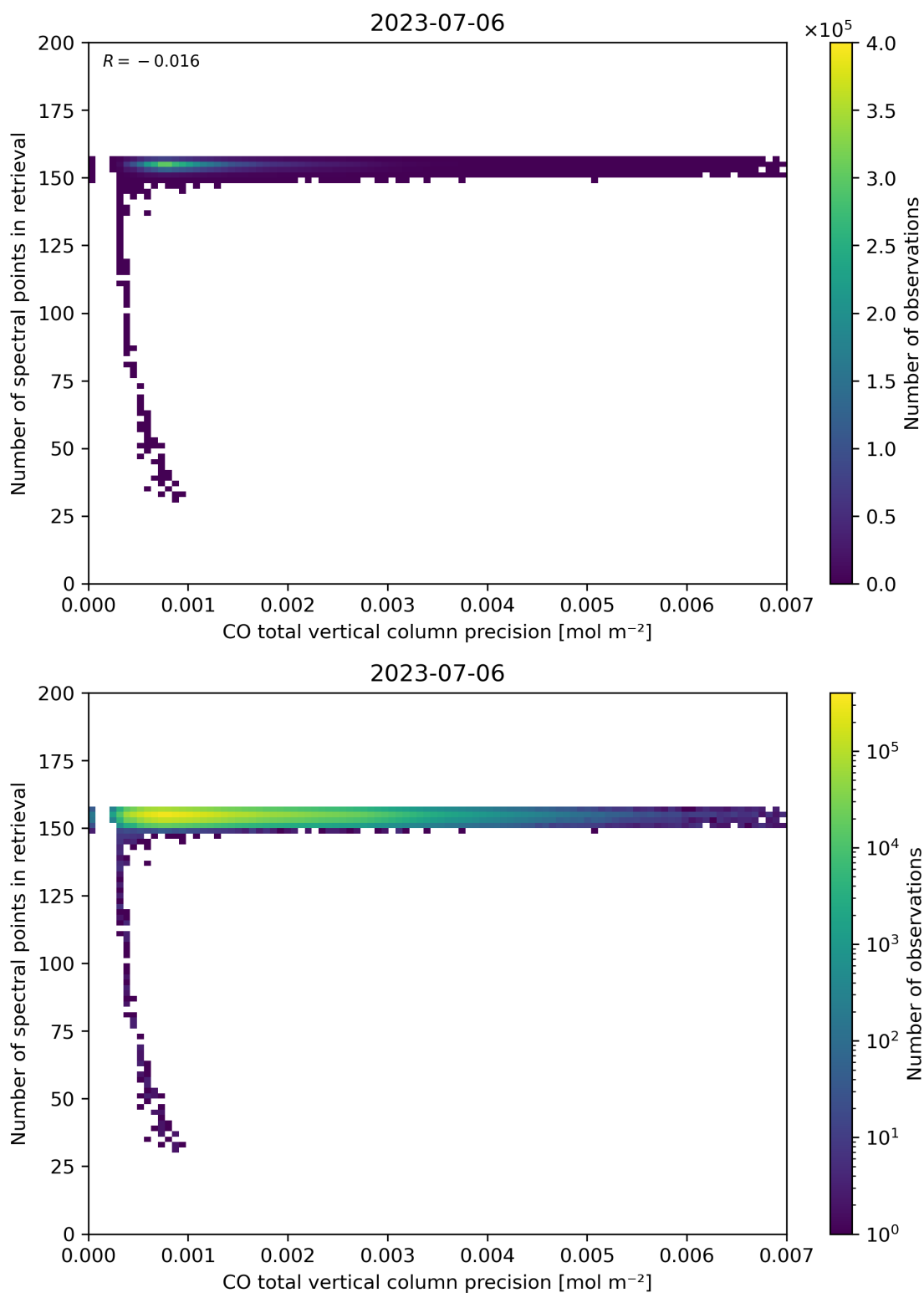
Figure 47: Scatter density plot of “CO total vertical column precision” against “Number of spectral points in retrieval” for 2023-07-05 to 2023-07-07.
