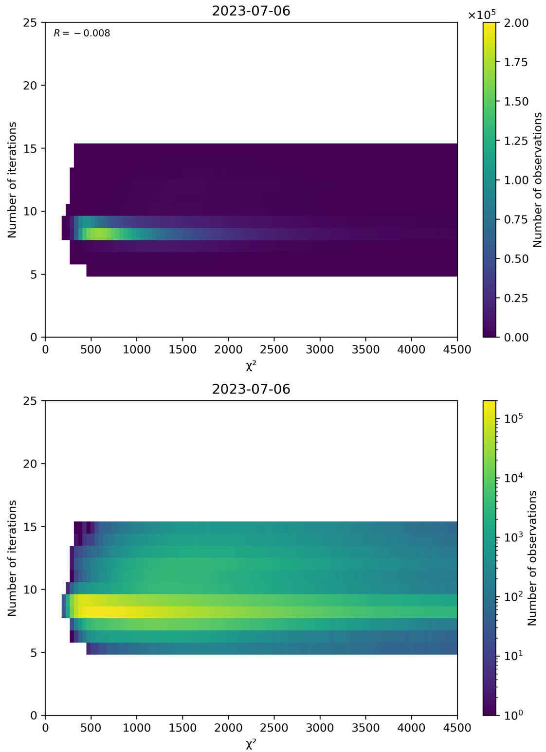
Figure 49: Scatter density plot of “ \chi^2 ” against “Number of iterations” for 2023-07-05 to 2023-07-07.
