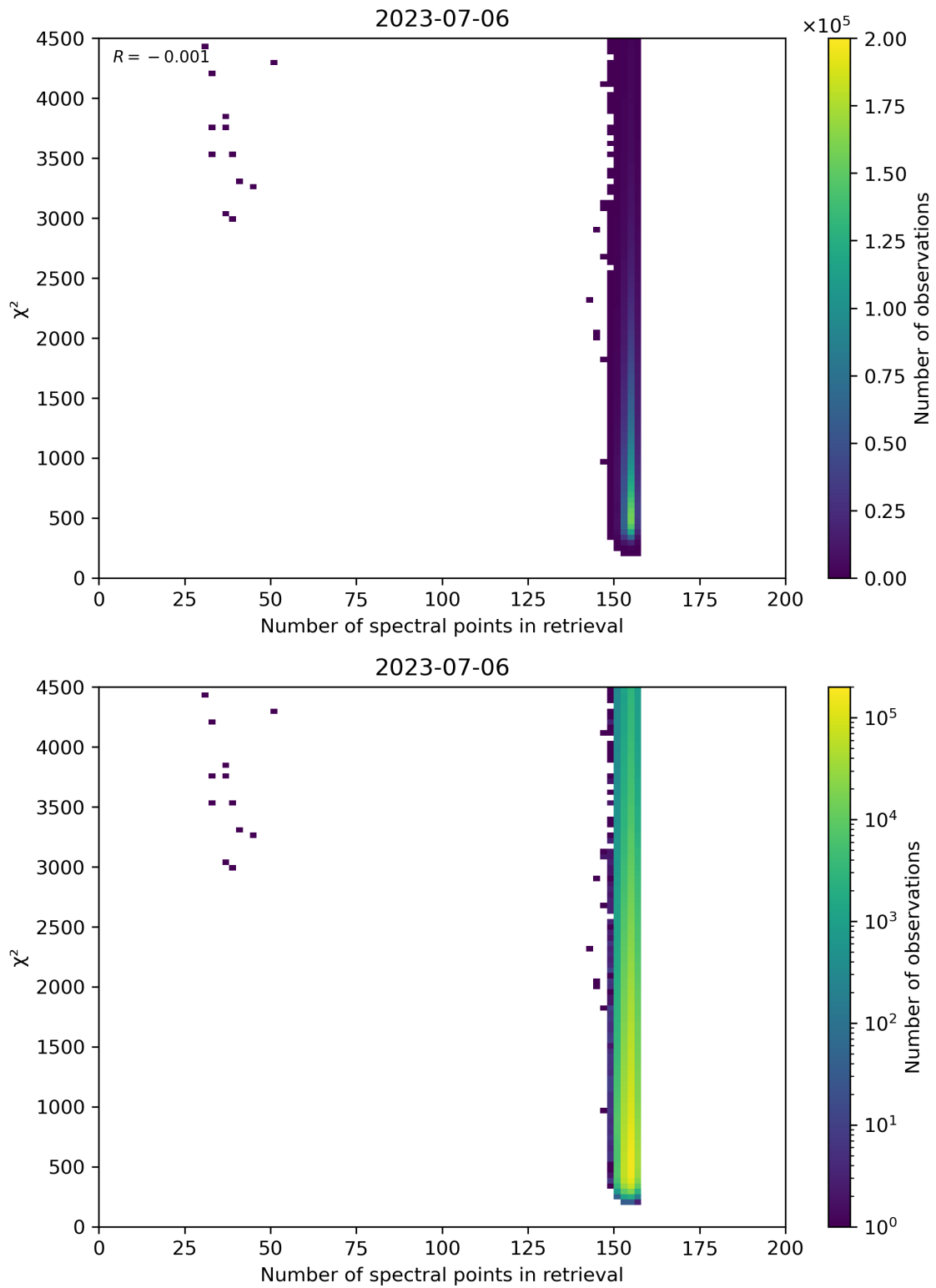
Figure 58: Scatter density plot of “Number of spectral points in retrieval” against “ \chi^2 ” for 2023-07-05 to 2023-07-07.
