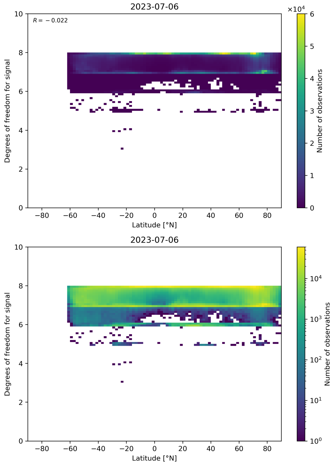
Figure 55: Scatter density plot of “Latitude” against “Degrees of freedom for signal” for 2023-07-05 to 2023-07-07.
