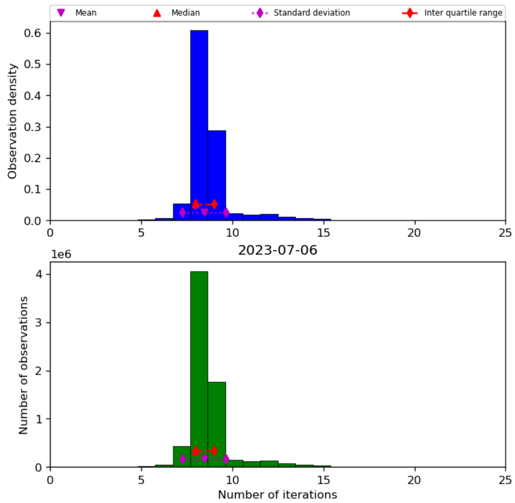
Figure 24: Histogram of “Number of iterations” for 2023-07-05 to 2023-07-07
