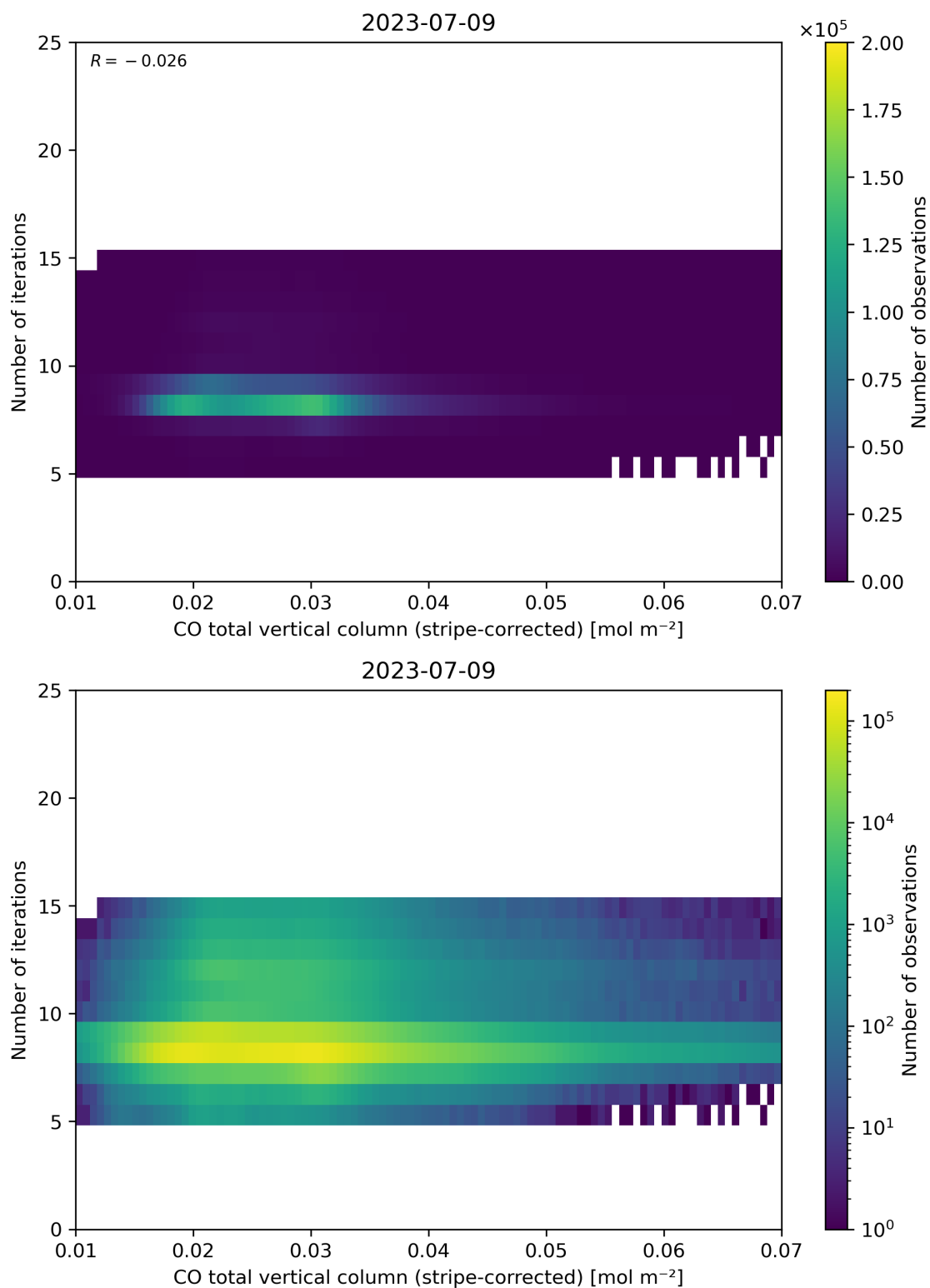
Figure 39: Scatter density plot of “CO total vertical column (stripe-corrected)” against “Number of iterations” for 2023-07-08 to 2023-07-10.
