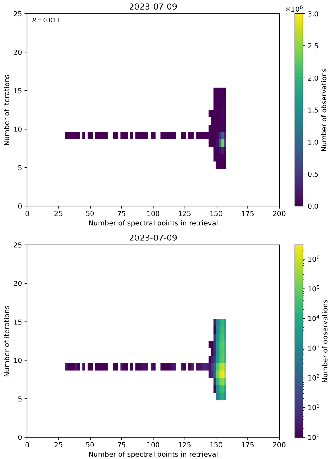
Figure 60: Scatter density plot of “Number of spectral points in retrieval” against “Number of iterations” for 2023-07-08 to 2023-07-10.
