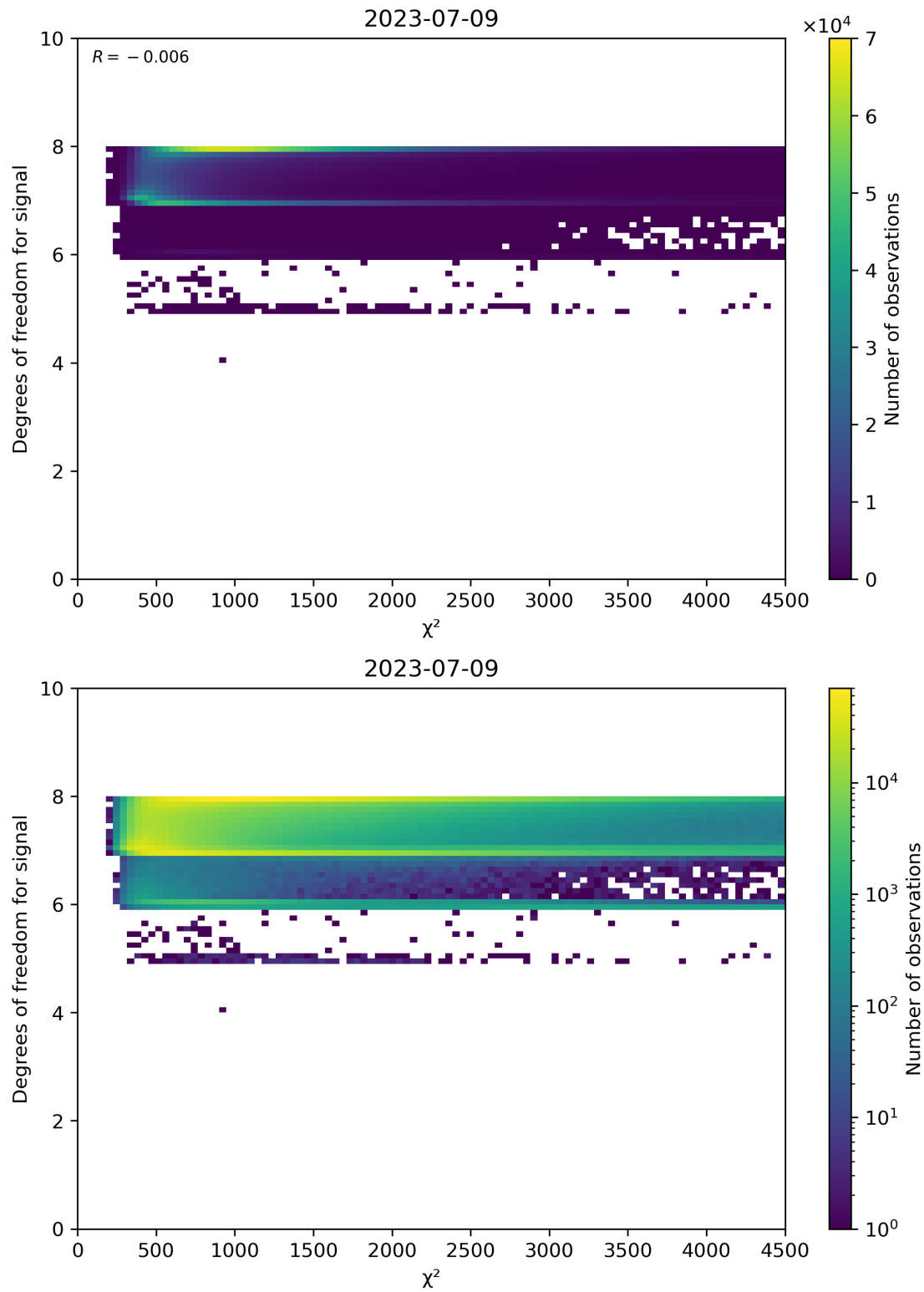
Figure 48: Scatter density plot of “ \chi^2 ” against “Degrees of freedom for signal” for 2023-07-08 to 2023-07-10.
