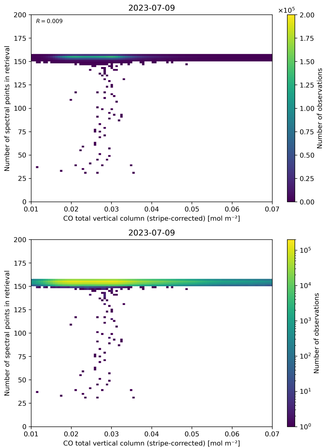
Figure 40: Scatter density plot of “CO total vertical column (stripe-corrected)” against “Number of spectral points in retrieval” for 2023-07-08 to 2023-07-10.
