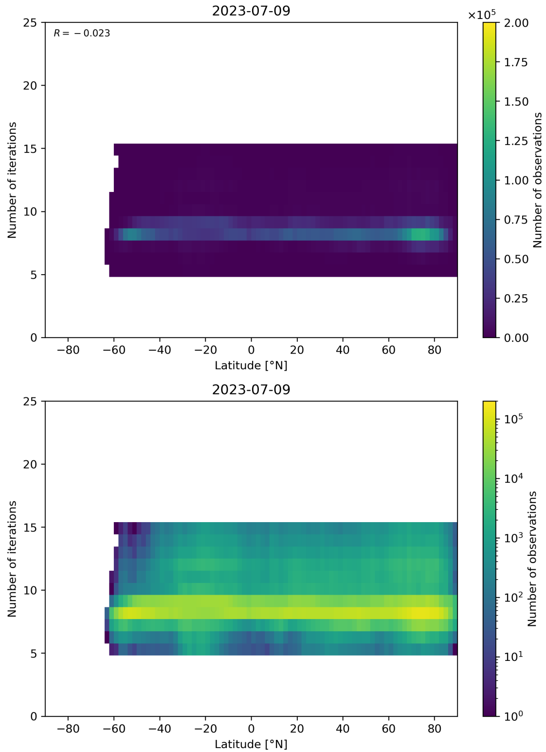
Figure 56: Scatter density plot of “Latitude” against “Number of iterations” for 2023-07-08 to 2023-07-10.
