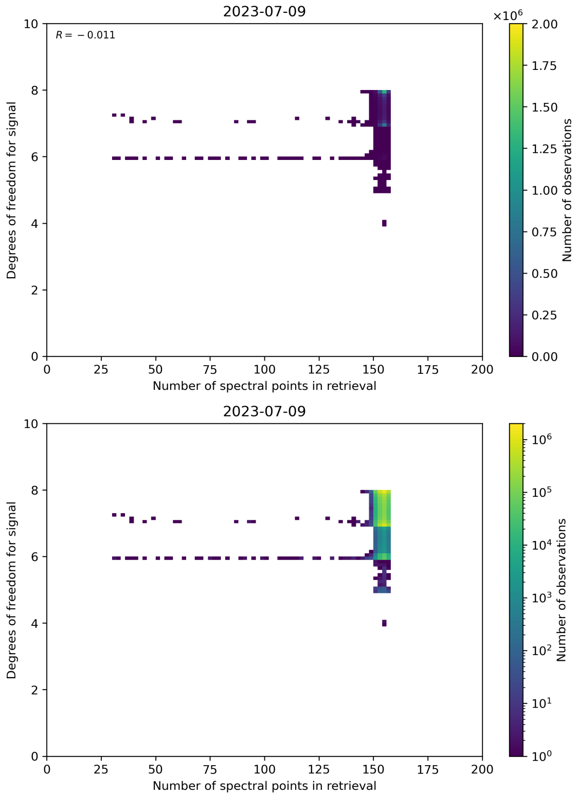
Figure 59: Scatter density plot of “Number of spectral points in retrieval” against “Degrees of freedom for signal” for 2023-07-08 to 2023-07-10.
