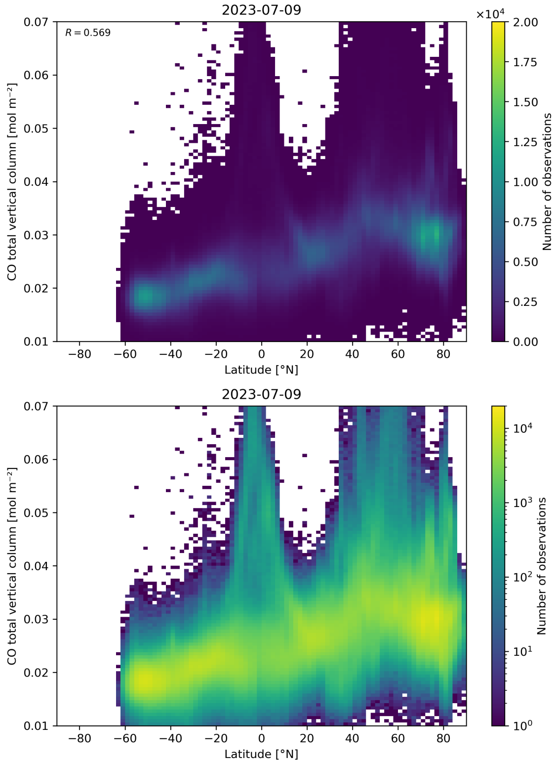
Figure 51: Scatter density plot of “Latitude” against “CO total vertical column” for 2023-07-08 to 2023-07-10.
