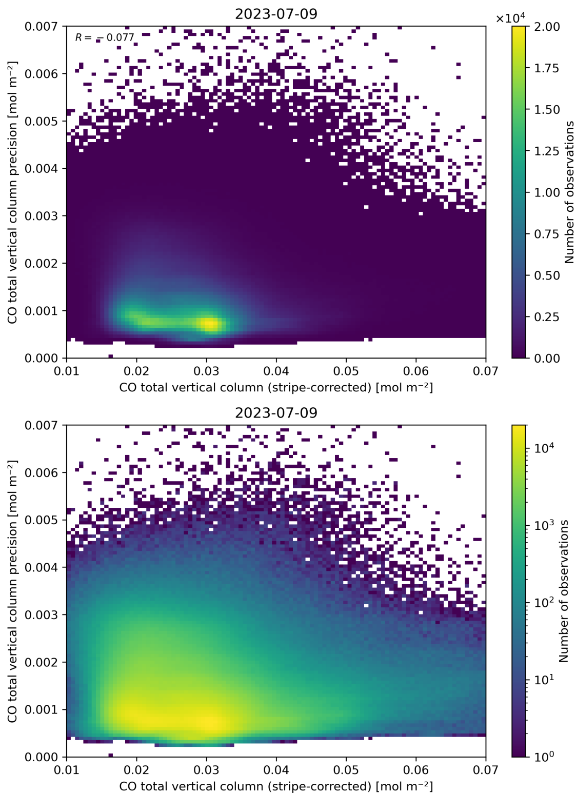
Figure 36: Scatter density plot of “CO total vertical column (stripe-corrected)” against “CO total vertical column precision” for 2023-07-08 to 2023-07-10.
