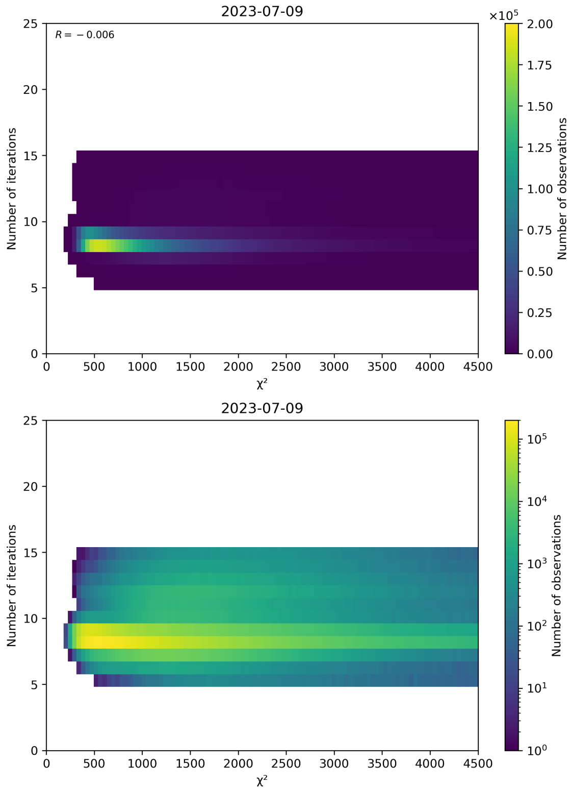
Figure 49: Scatter density plot of “ \chi^2 ” against “Number of iterations” for 2023-07-08 to 2023-07-10.
