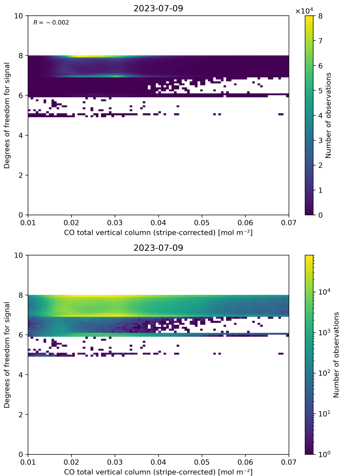
Figure 38: Scatter density plot of “CO total vertical column (stripe-corrected)” against “Degrees of freedom for signal” for 2023-07-08 to 2023-07-10.
