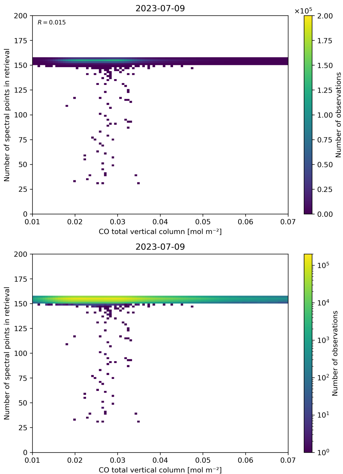
Figure 43: Scatter density plot of “CO total vertical column” against “Number of spectral points in retrieval” for 2023-07-08 to 2023-07-10.
