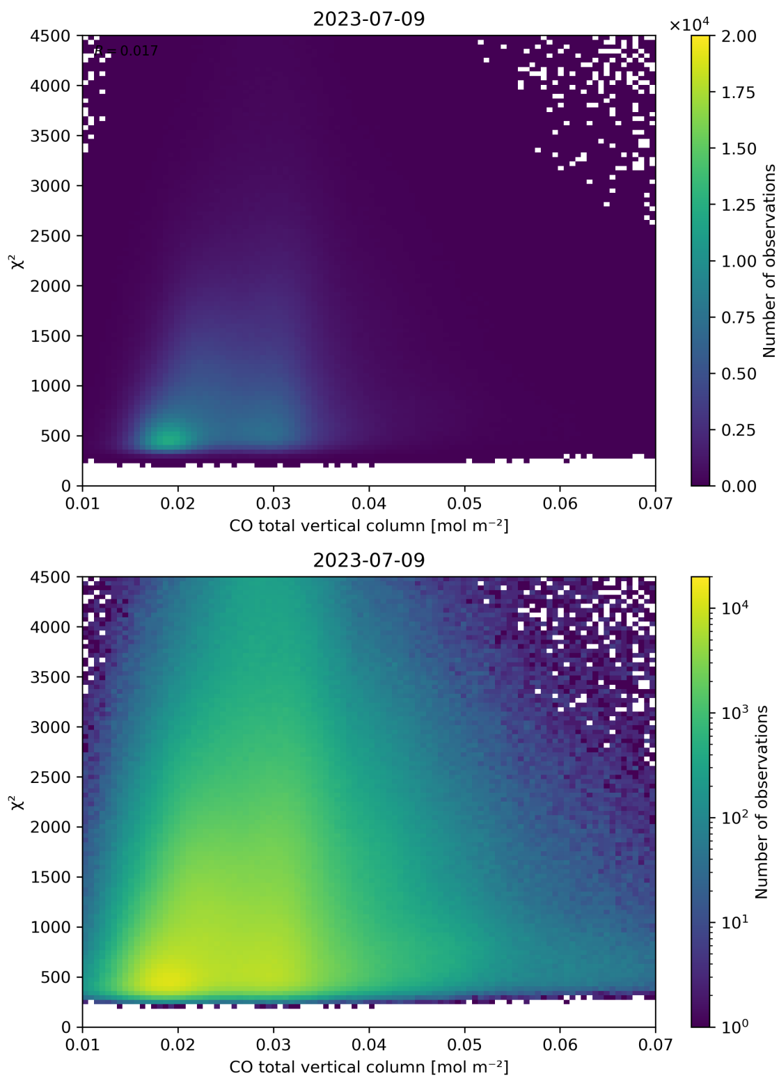
Figure 35: Scatter density plot of “CO total vertical column” against “ \chi^2 ” for 2023-07-08 to 2023-07-10.
