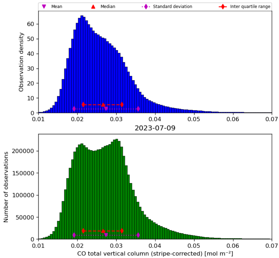
Figure 19: Histogram of “CO total vertical column (stripe-corrected)” for 2023-07-08 to 2023-07-10
