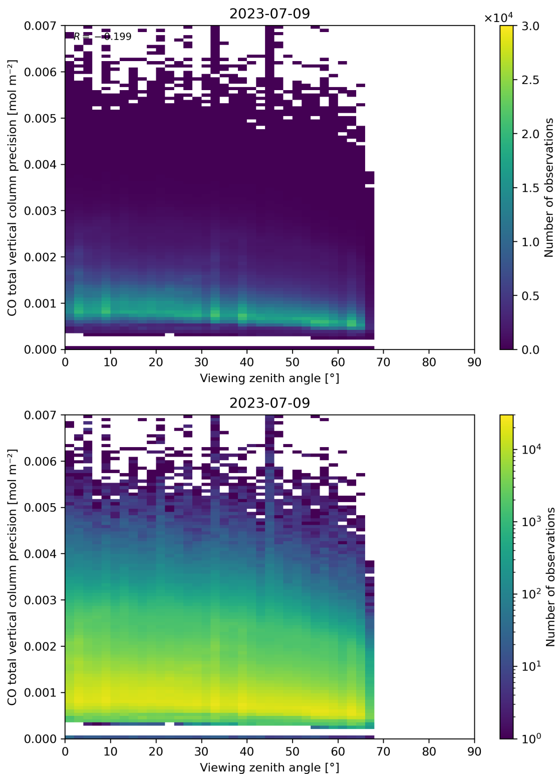
Figure 71: Scatter density plot of “Viewing zenith angle” against “CO total vertical column precision” for 2023-07-08 to 2023-07-10.
