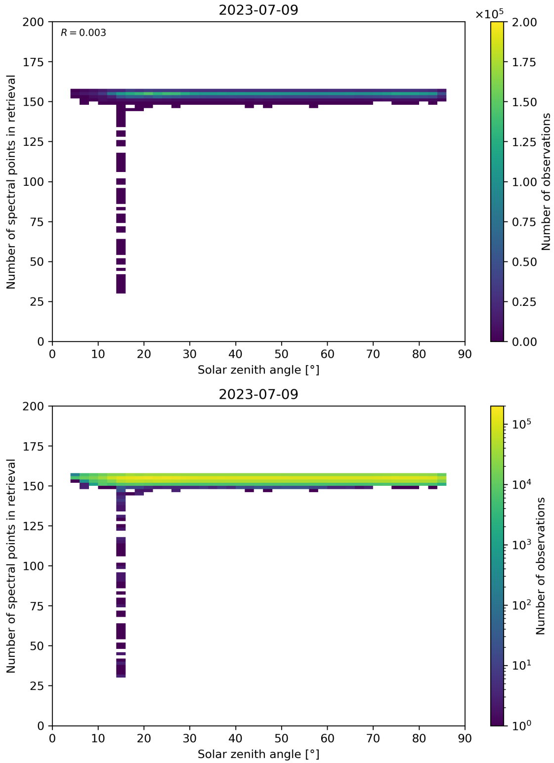
Figure 68: Scatter density plot of “Solar zenith angle” against “Number of spectral points in retrieval” for 2023-07-08 to 2023-07-10.
