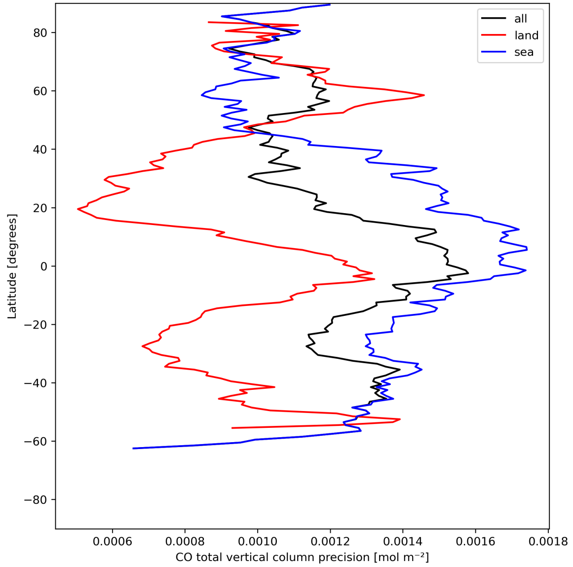
Figure 12: Zonal average of “CO total vertical column precision” for 2023-07-08 to 2023-07-10.
