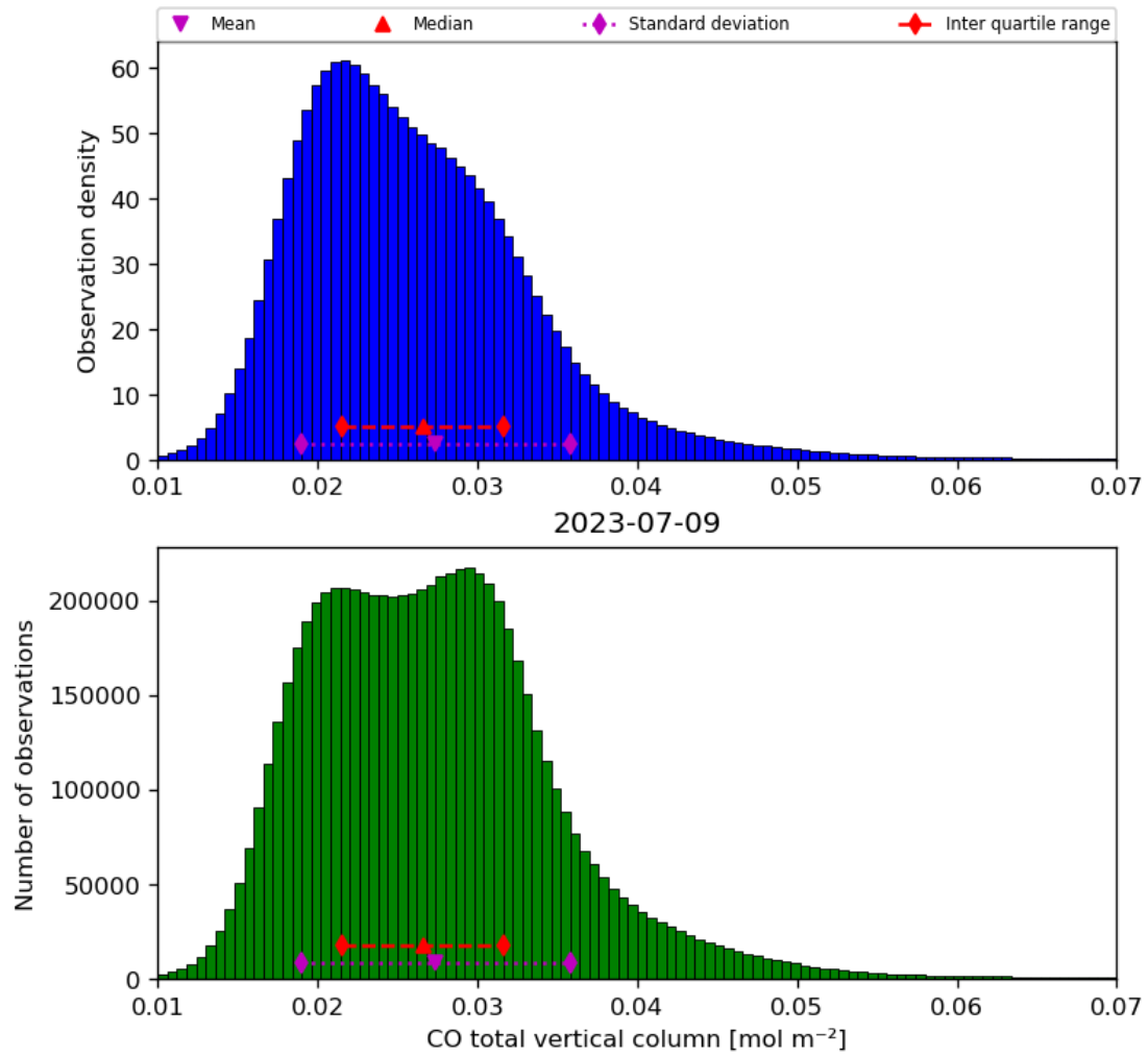
Figure 18: Histogram of “CO total vertical column” for 2023-07-08 to 2023-07-10
