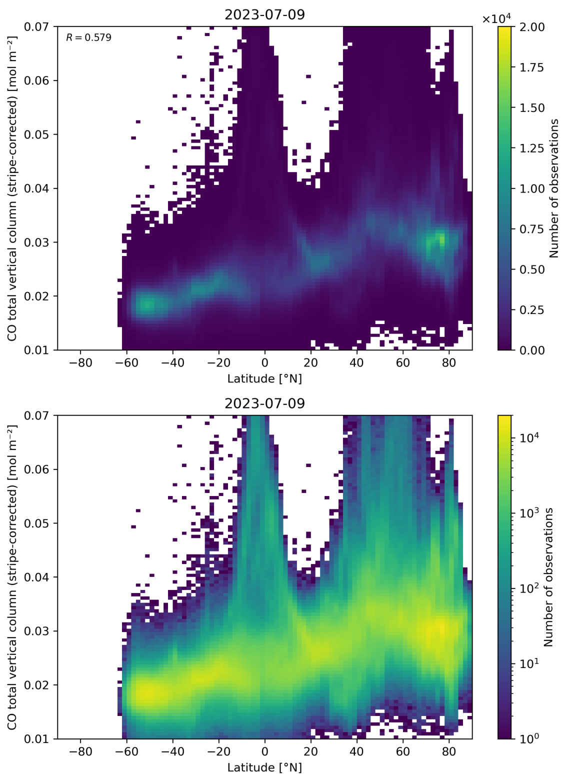
Figure 52: Scatter density plot of “Latitude” against “CO total vertical column (stripe-corrected)” for 2023-07-08 to 2023-07-10.
