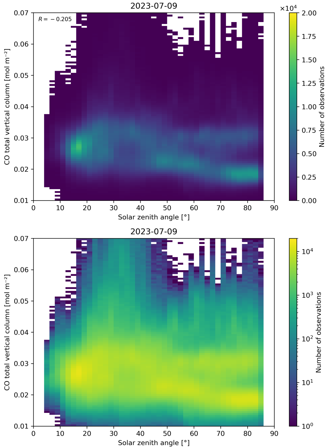
Figure 61: Scatter density plot of “Solar zenith angle” against “CO total vertical column” for 2023-07-08 to 2023-07-10.
