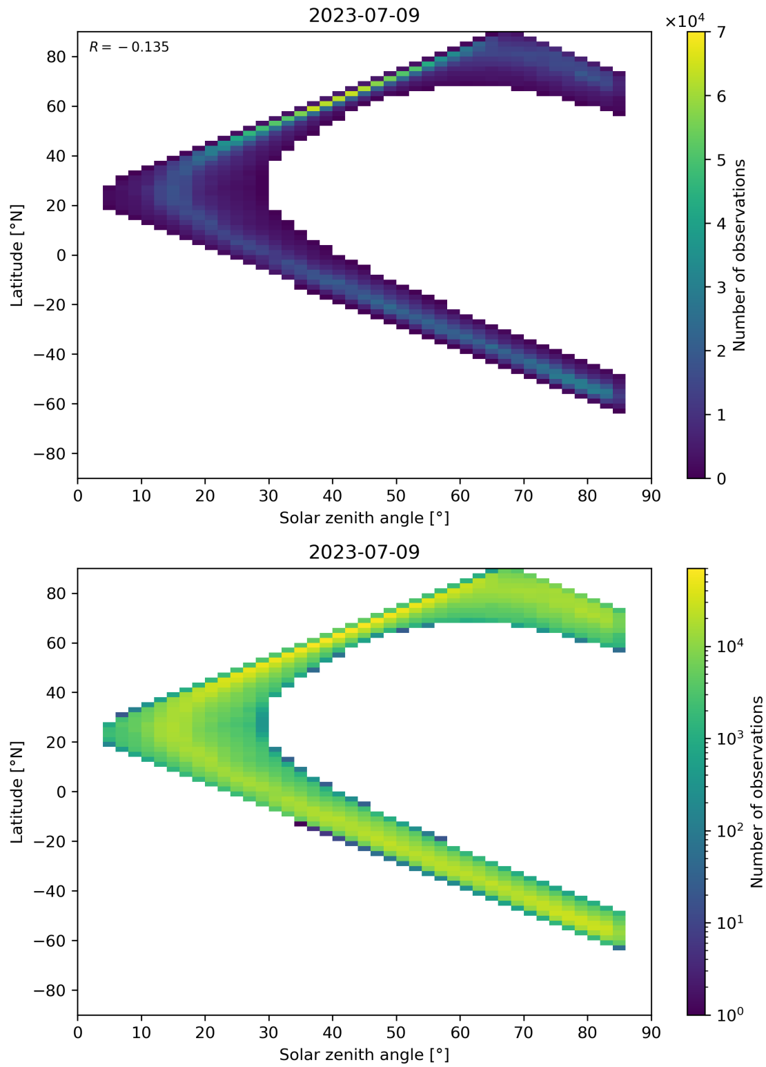
Figure 66: Scatter density plot of “Solar zenith angle” against “Latitude” for 2023-07-08 to 2023-07-10.
