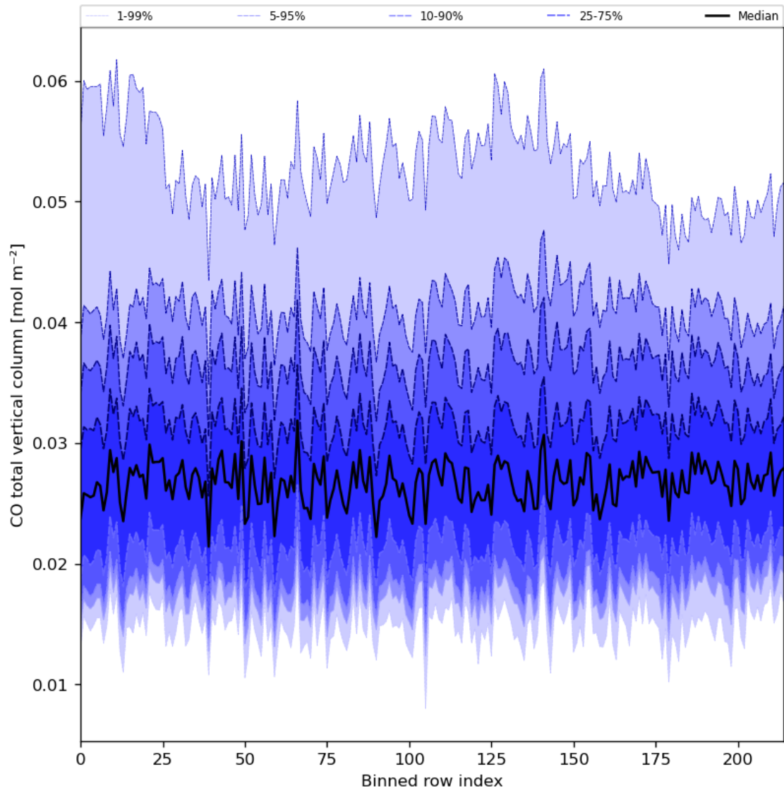
Figure 26: Along track statistics of “CO total vertical column” for 2023-07-08 to 2023-07-10
