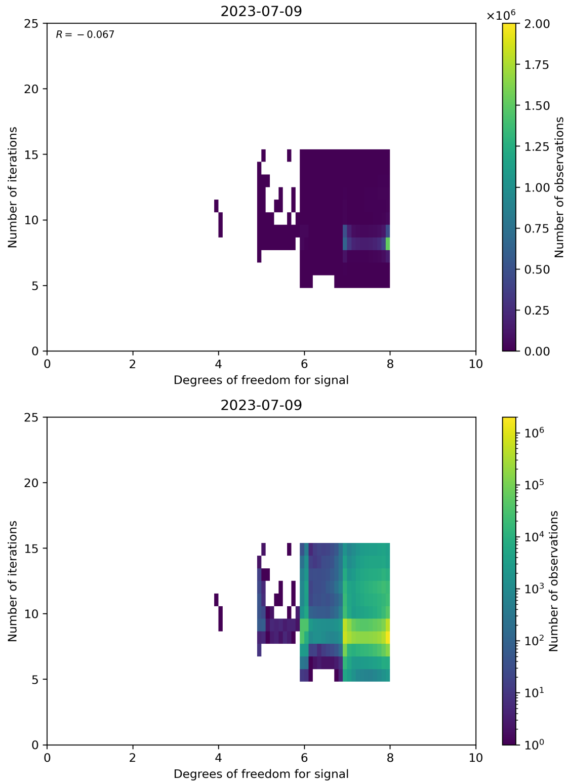
Figure 50: Scatter density plot of “Degrees of freedom for signal” against “Number of iterations” for 2023-07-08 to 2023-07-10.
