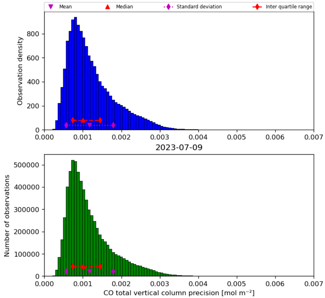
Figure 20: Histogram of “CO total vertical column precision” for 2023-07-08 to 2023-07-10
