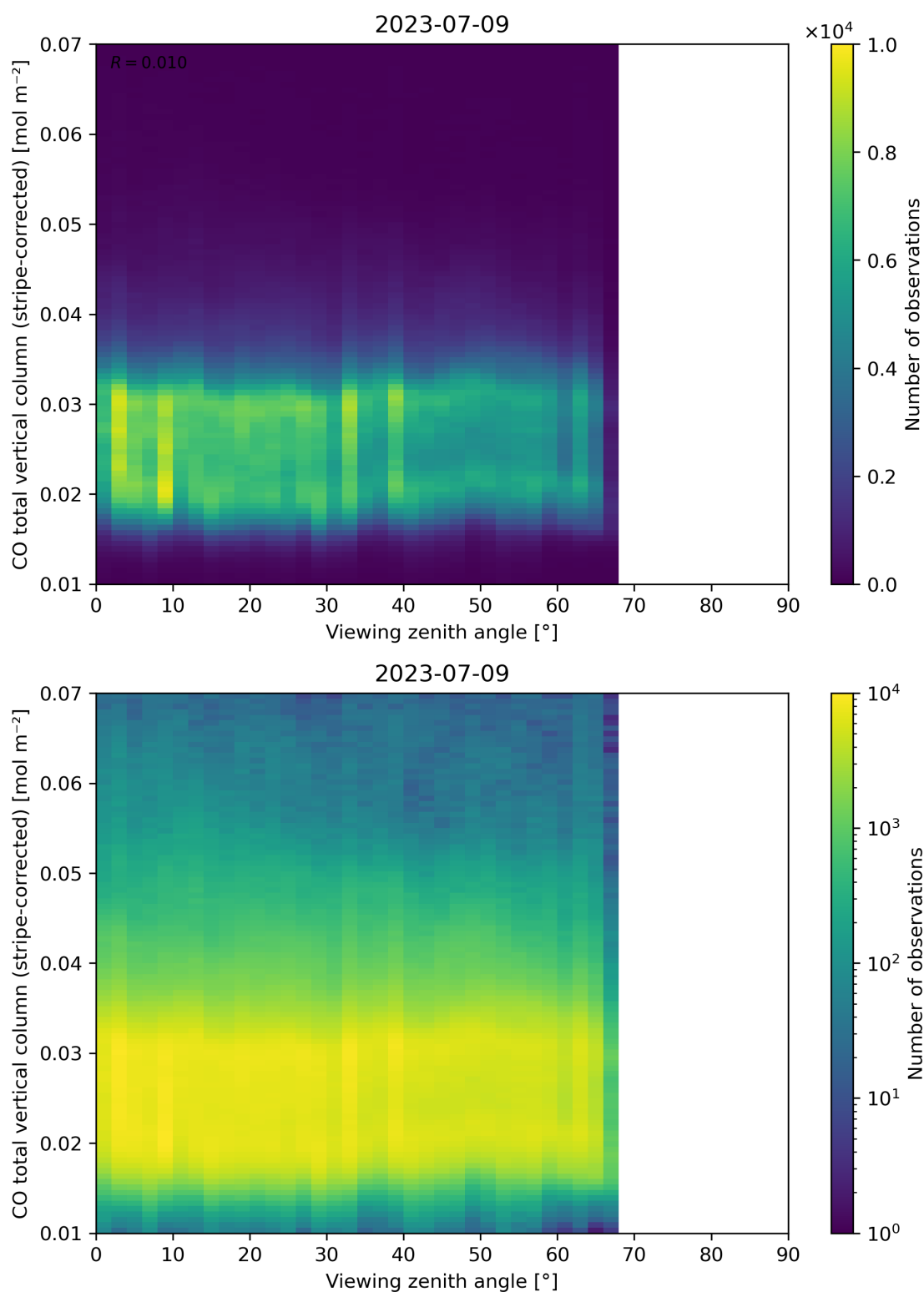
Figure 70: Scatter density plot of “Viewing zenith angle” against “CO total vertical column (stripe-corrected)” for 2023-07-08 to 2023-07-10.
