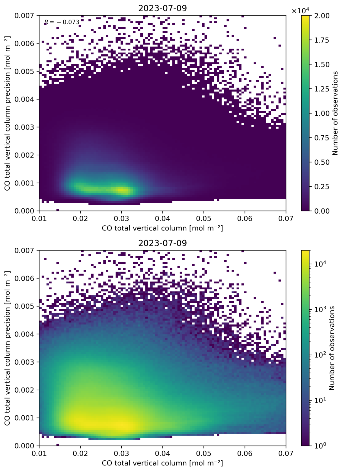
Figure 34: Scatter density plot of “CO total vertical column” against “CO total vertical column precision” for 2023-07-08 to 2023-07-10.
