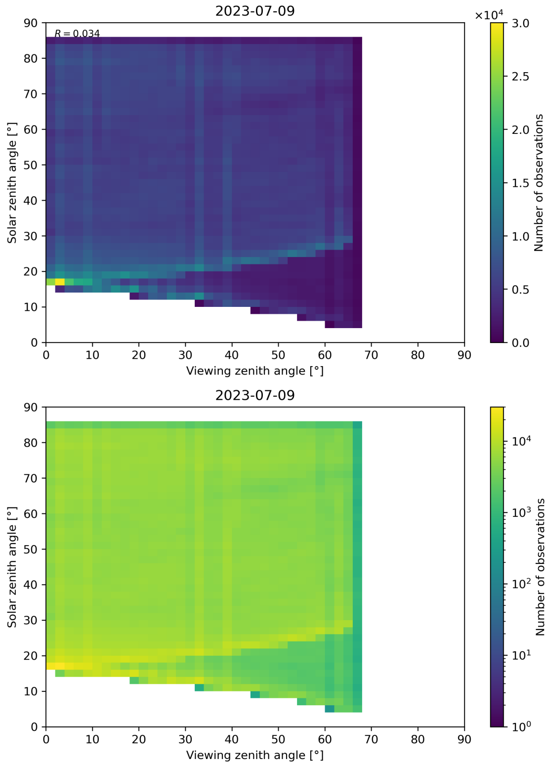
Figure 77: Scatter density plot of “Viewing zenith angle” against “Solar zenith angle” for 2023-07-08 to 2023-07-10.
