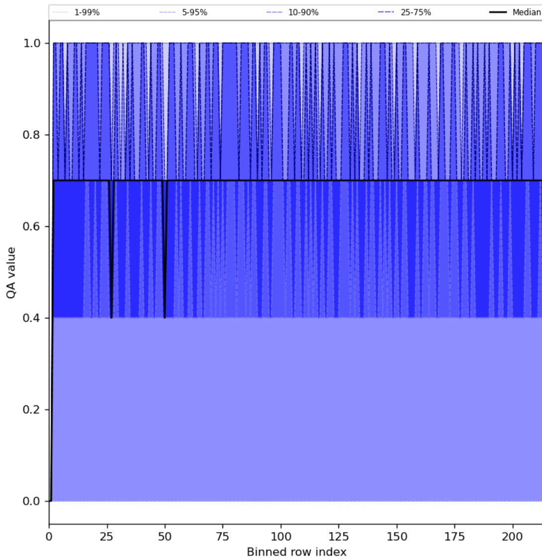
Figure 25: Along track statistics of “QA value” for 2023-07-08 to 2023-07-10
