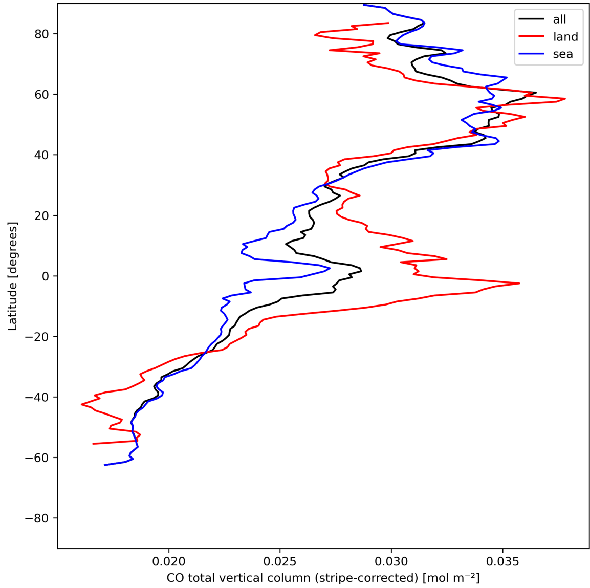
Figure 11: Zonal average of “CO total vertical column (stripe-corrected)” for 2023-07-08 to 2023-07-10.
