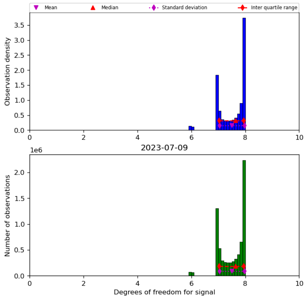
Figure 23: Histogram of “Degrees of freedom for signal” for 2023-07-08 to 2023-07-10
