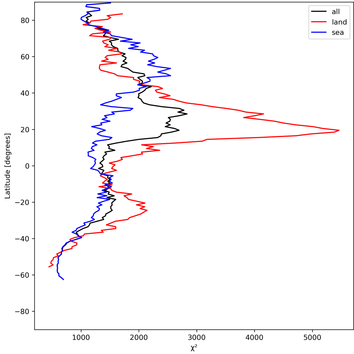
Figure 14: Zonal average of “ \chi^2 ” for 2023-07-08 to 2023-07-10.
