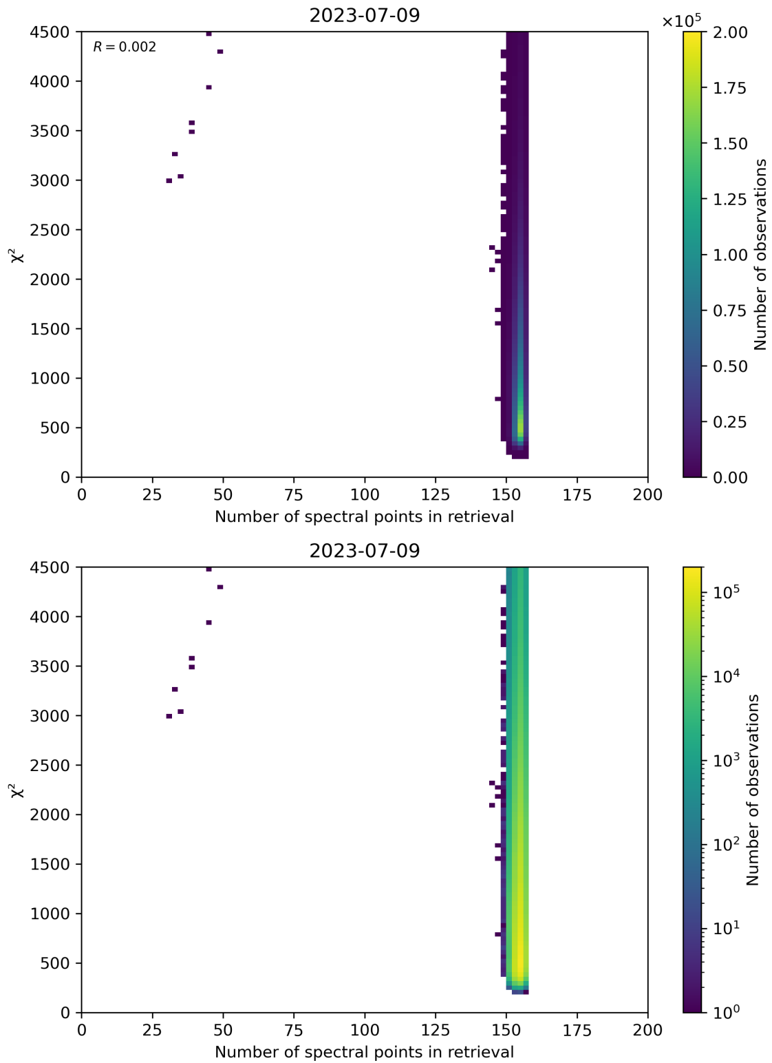
Figure 58: Scatter density plot of “Number of spectral points in retrieval” against “ \chi^2 ” for 2023-07-08 to 2023-07-10.
