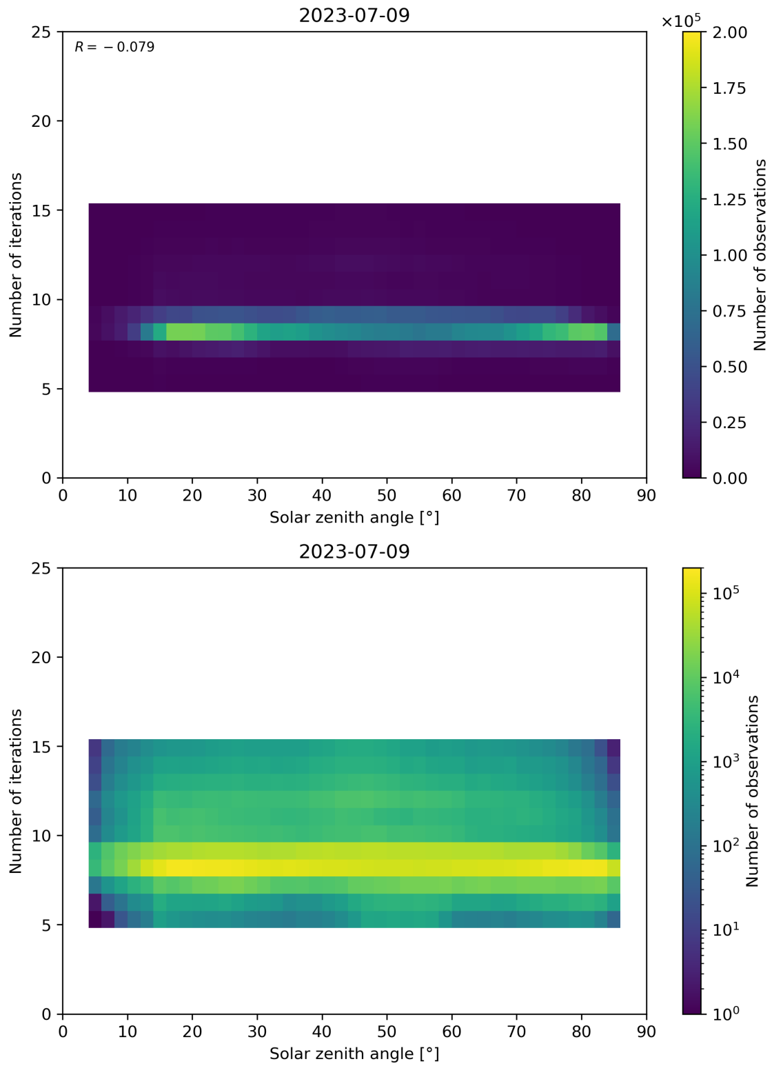
Figure 67: Scatter density plot of “Solar zenith angle” against “Number of iterations” for 2023-07-08 to 2023-07-10.
