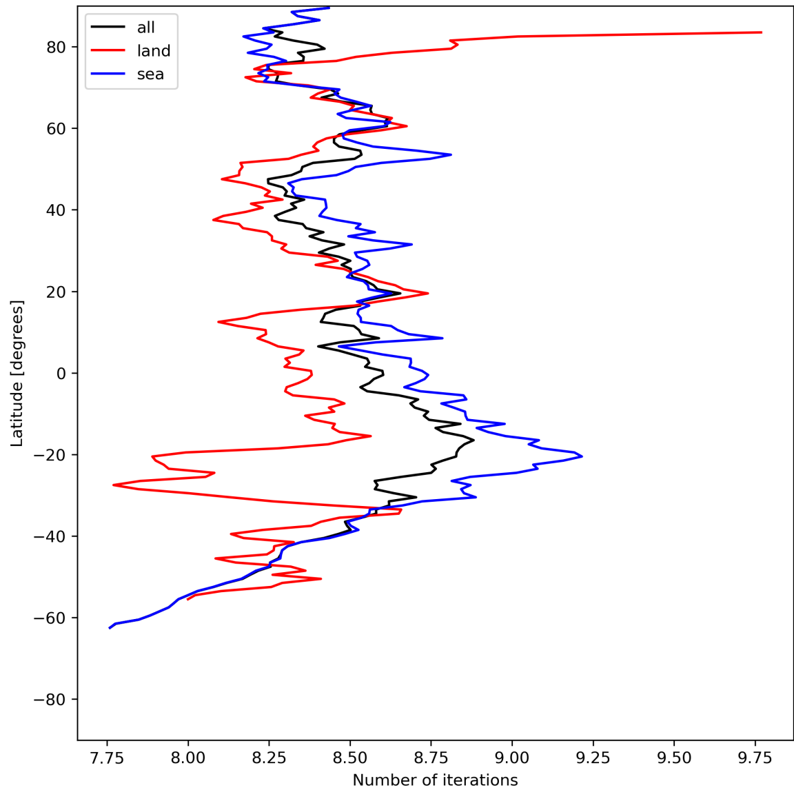
Figure 16: Zonal average of “Number of iterations” for 2023-07-08 to 2023-07-10.
