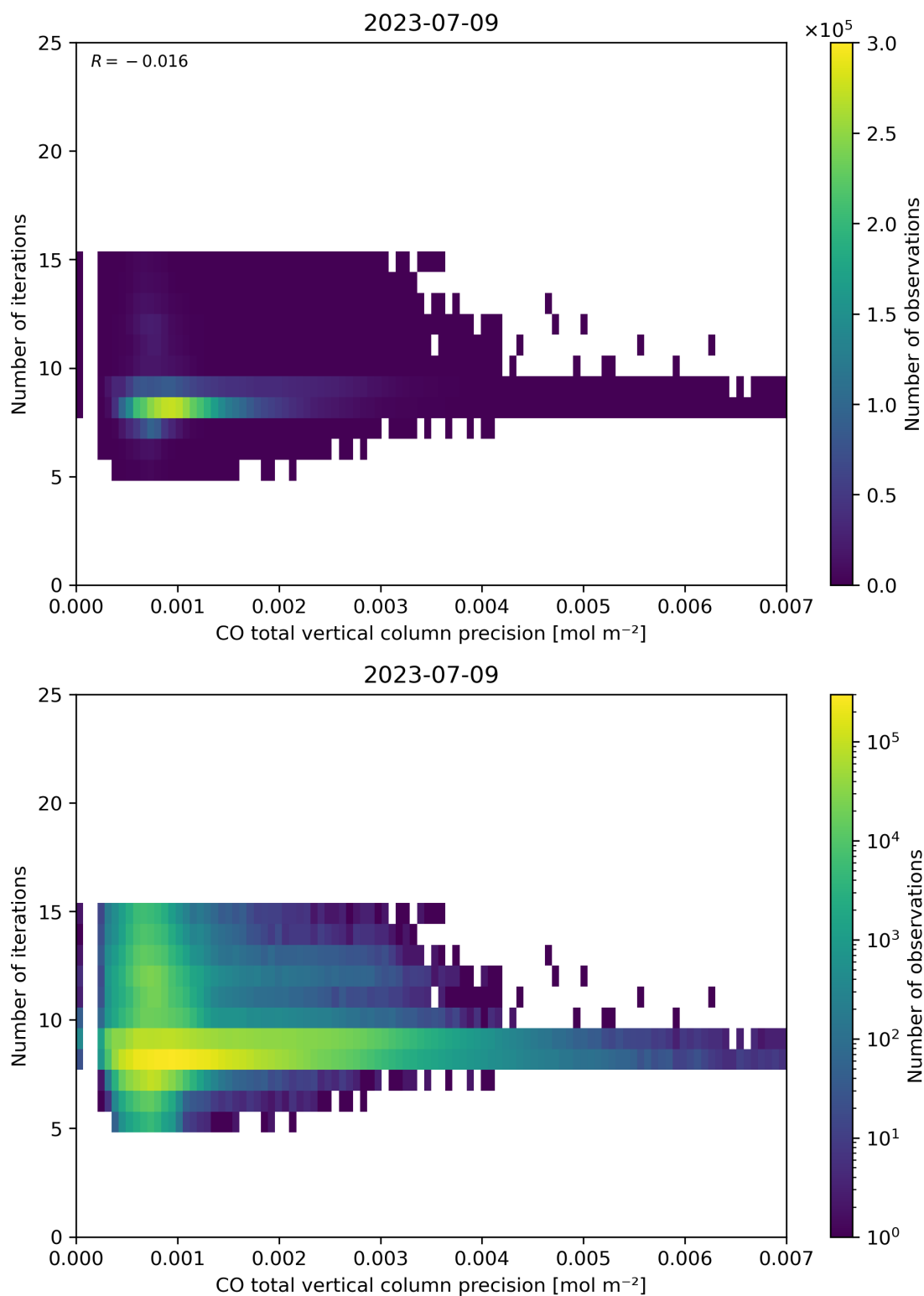
Figure 46: Scatter density plot of “CO total vertical column precision” against “Number of iterations” for 2023-07-08 to 2023-07-10.
