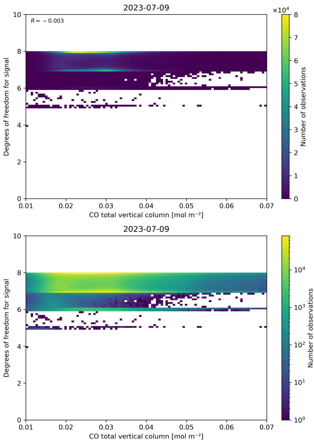
Figure 41: Scatter density plot of “CO total vertical column” against “Degrees of freedom for signal” for 2023-07-08 to 2023-07-10.
