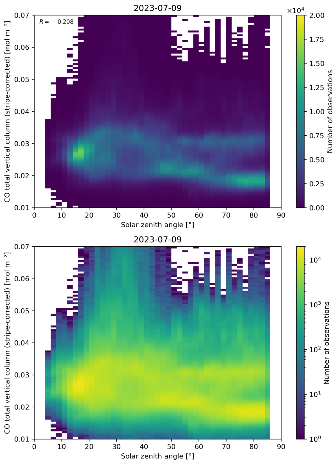
Figure 62: Scatter density plot of “Solar zenith angle” against “CO total vertical column (stripe-corrected)” for 2023-07-08 to 2023-07-10.
