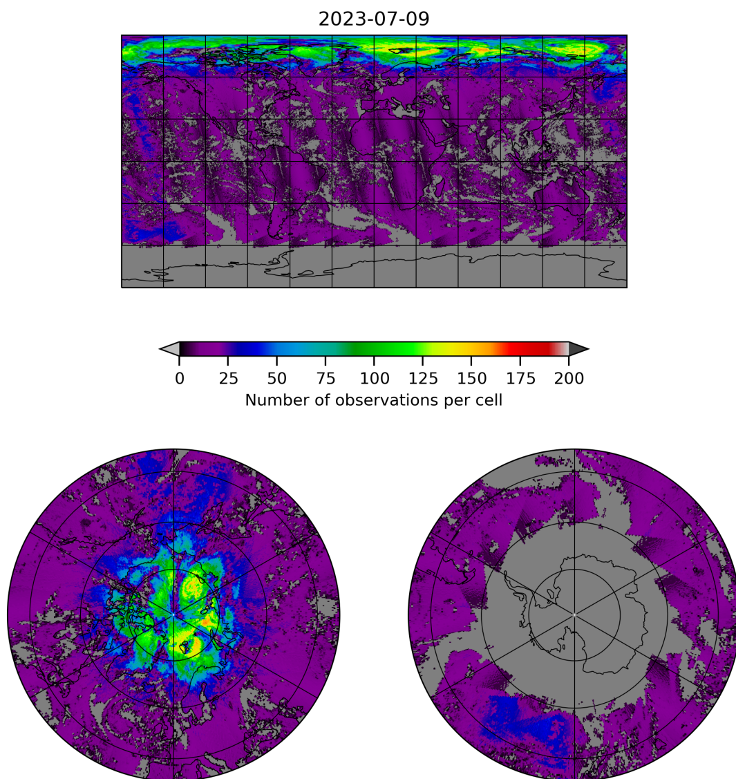
Figure 8: Map of the number of observations for 2023-07-08 to 2023-07-10
