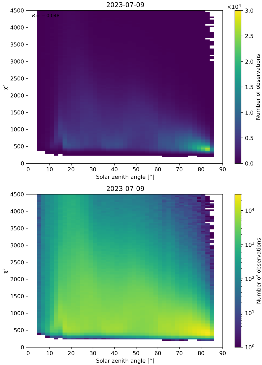
Figure 64: Scatter density plot of “Solar zenith angle” against “ \chi^2 ” for 2023-07-08 to 2023-07-10.
