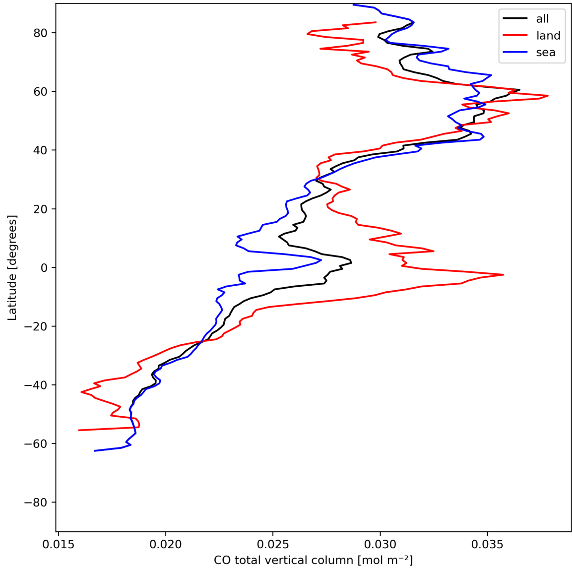
Figure 10: Zonal average of “CO total vertical column” for 2023-07-08 to 2023-07-10.
