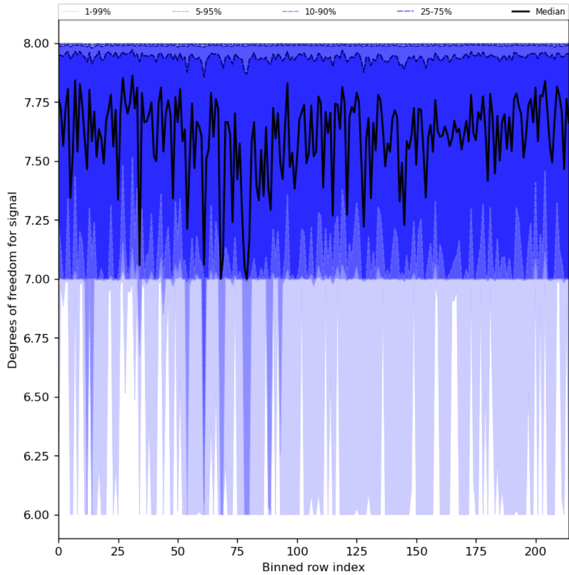
Figure 31: Along track statistics of “Degrees of freedom for signal” for 2023-07-08 to 2023-07-10
