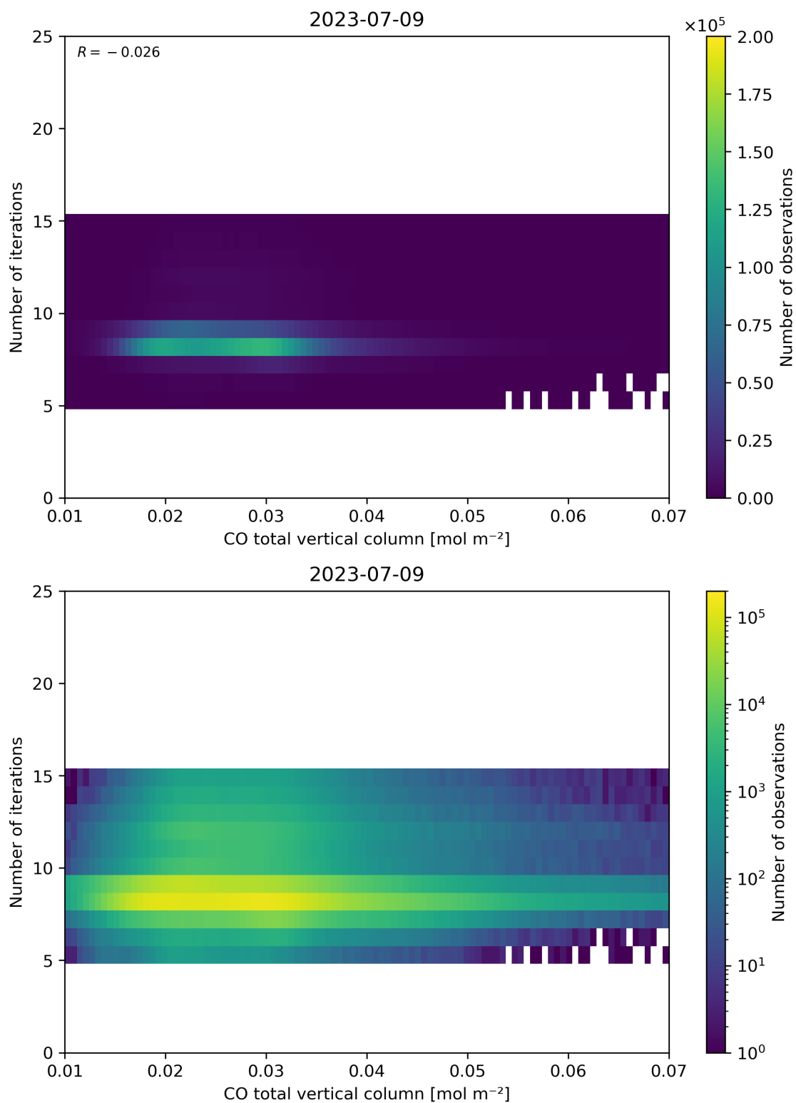
Figure 42: Scatter density plot of “CO total vertical column” against “Number of iterations” for 2023-07-08 to 2023-07-10.
