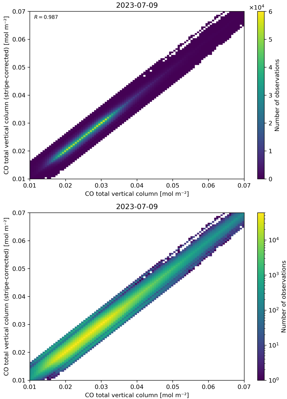
Figure 33: Scatter density plot of “CO total vertical column” against “CO total vertical column (stripe-corrected)” for 2023-07-08 to 2023-07-10.
