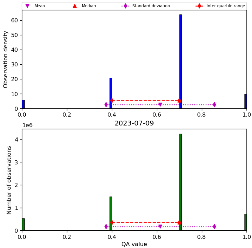
Figure 17: Histogram of “QA value” for 2023-07-08 to 2023-07-10
