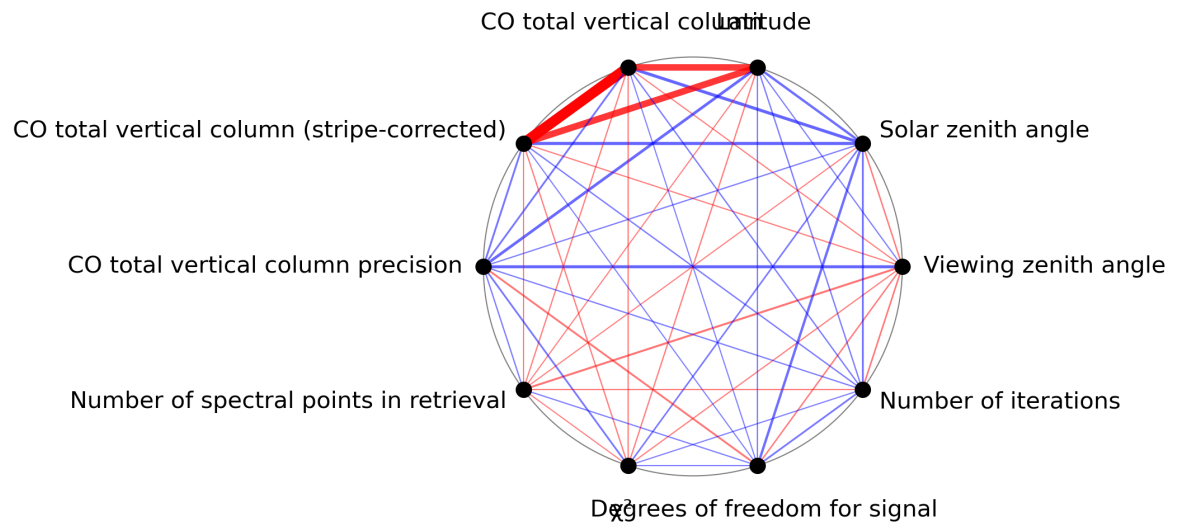
Figure 1: Map of correlation graph for 2023-07-08 to 2023-07-10.
