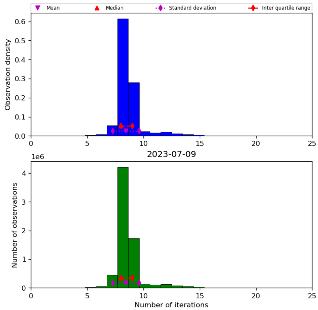
Figure 24: Histogram of “Number of iterations” for 2023-07-08 to 2023-07-10
