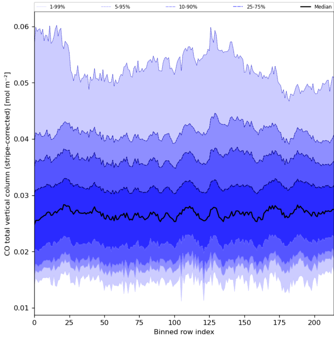
Figure 27: Along track statistics of “CO total vertical column (stripe-corrected)” for 2023-07-08 to 2023-07-10
