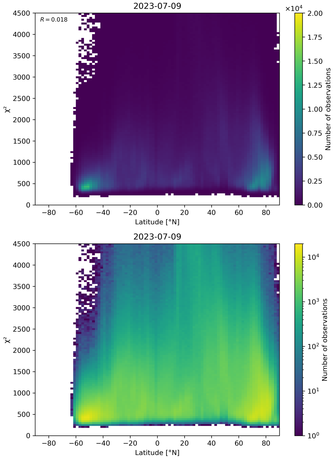
Figure 54: Scatter density plot of “Latitude” against “ \chi^2 ” for 2023-07-08 to 2023-07-10.
