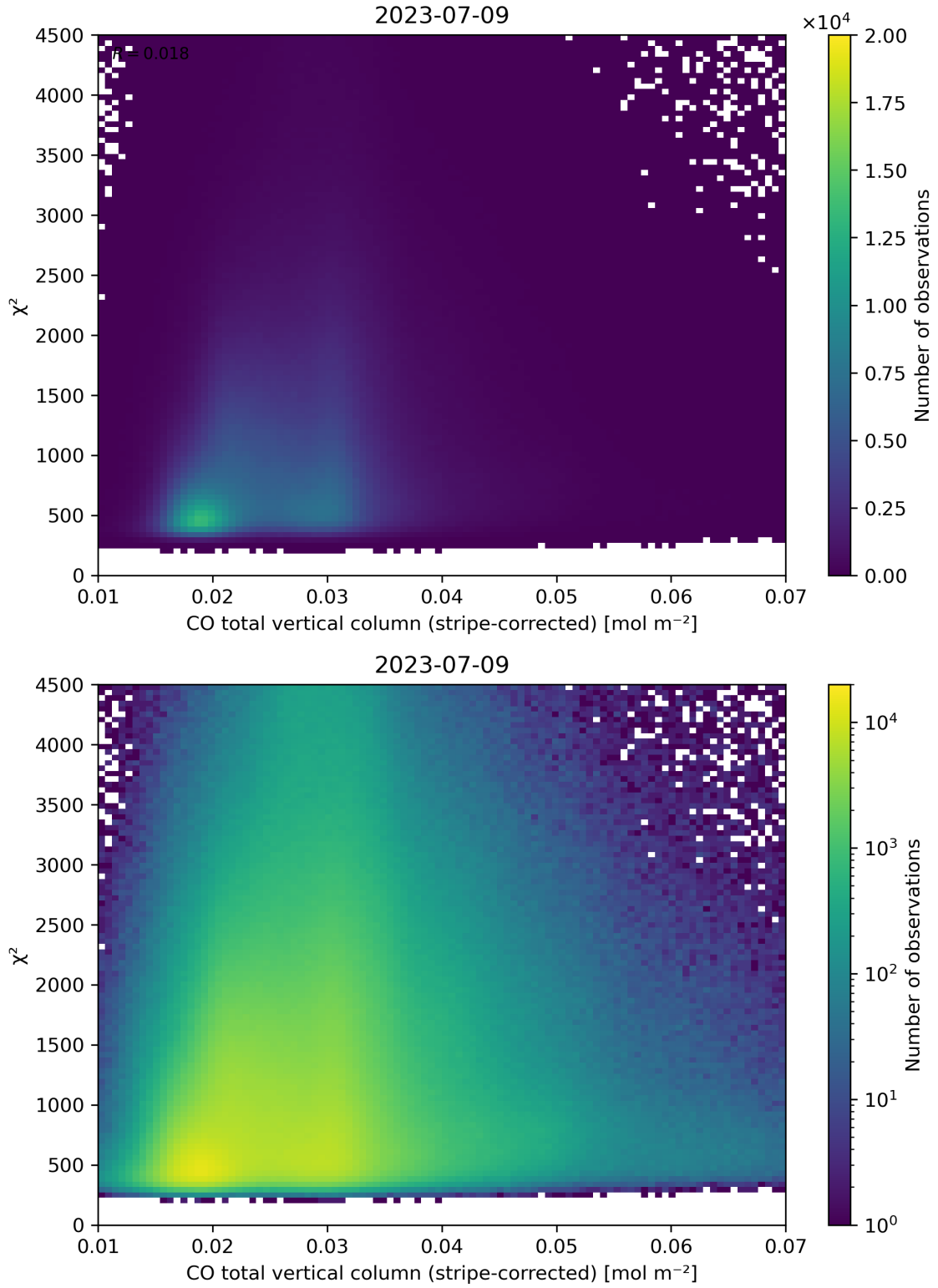
Figure 37: Scatter density plot of “CO total vertical column (stripe-corrected)” against “ \chi^2 ” for 2023-07-08 to 2023-07-10.
