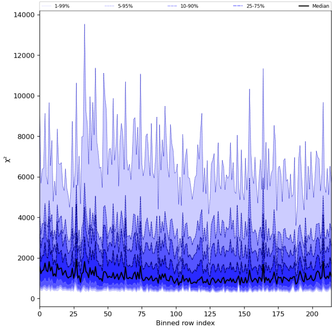
Figure 30: Along track statistics of “ \chi^2 ” for 2023-07-08 to 2023-07-10
