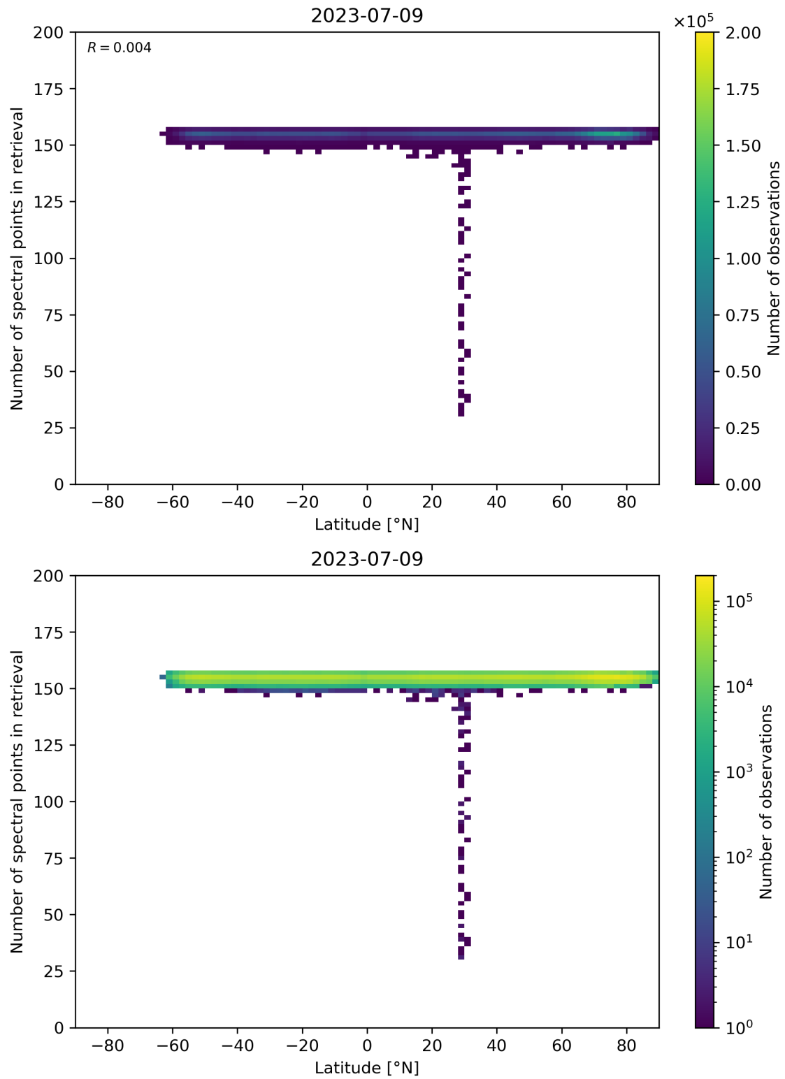
Figure 57: Scatter density plot of “Latitude” against “Number of spectral points in retrieval” for 2023-07-08 to 2023-07-10.
