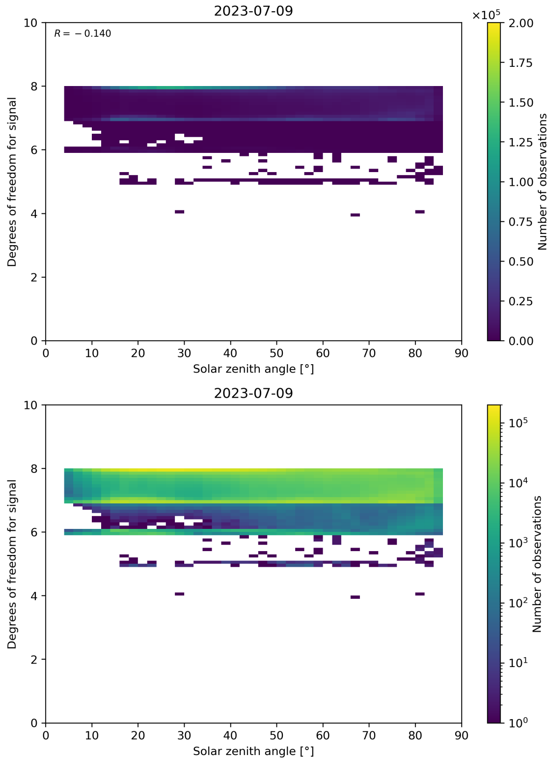
Figure 65: Scatter density plot of “Solar zenith angle” against “Degrees of freedom for signal” for 2023-07-08 to 2023-07-10.
