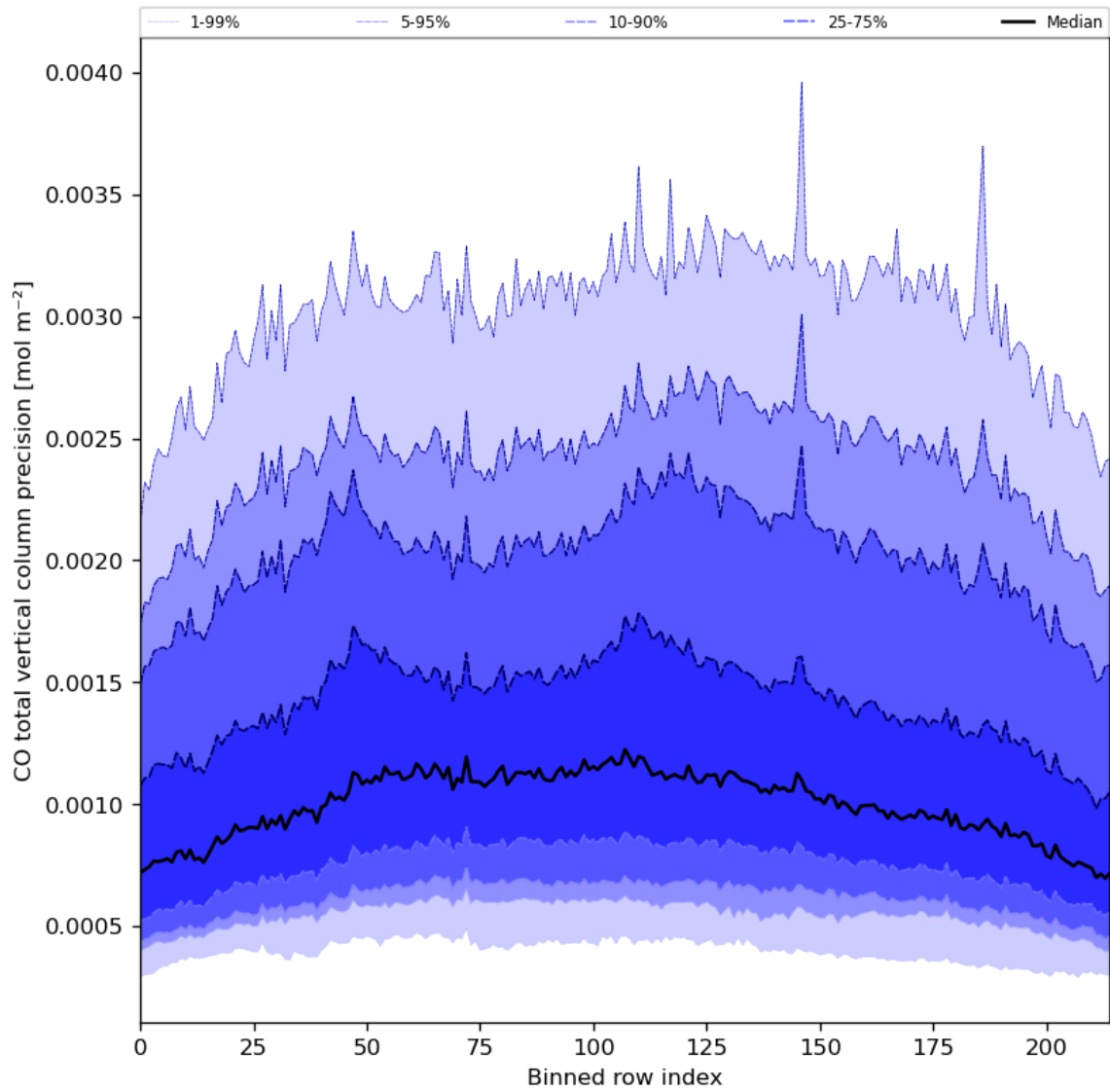
Figure 28: Along track statistics of “CO total vertical column precision” for 2023-07-08 to 2023-07-10
