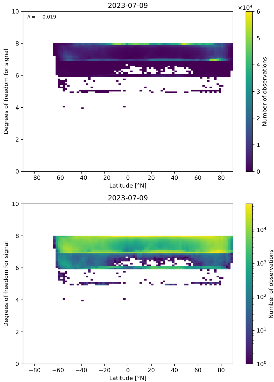
Figure 55: Scatter density plot of “Latitude” against “Degrees of freedom for signal” for 2023-07-08 to 2023-07-10.
