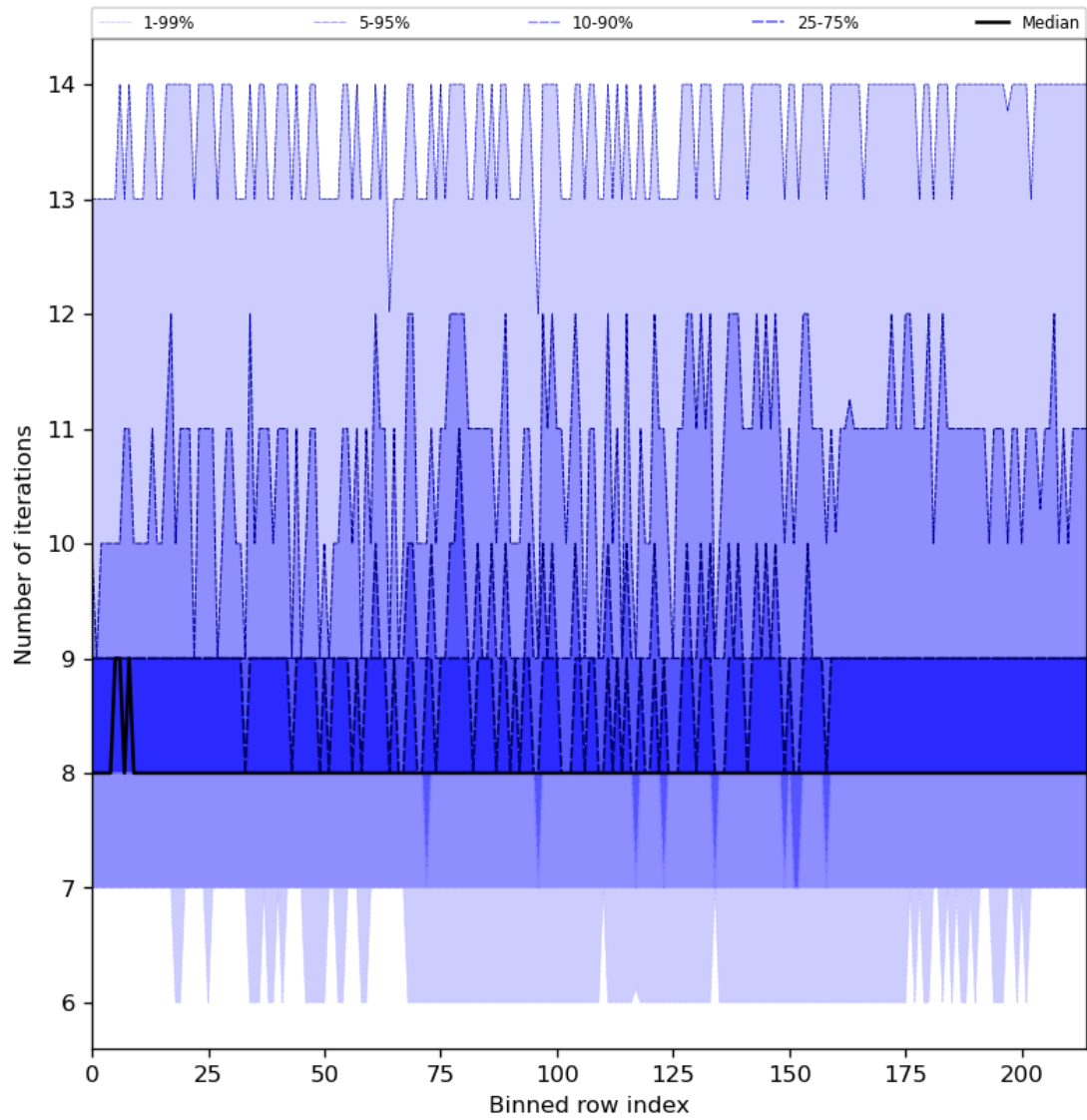
Figure 32: Along track statistics of “Number of iterations” for 2023-07-08 to 2023-07-10
