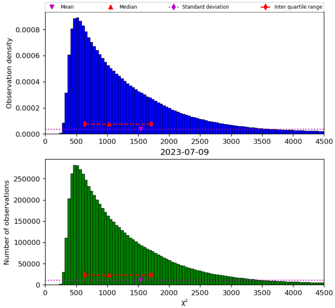
Figure 22: Histogram of “ \chi^2 ” for 2023-07-08 to 2023-07-10
