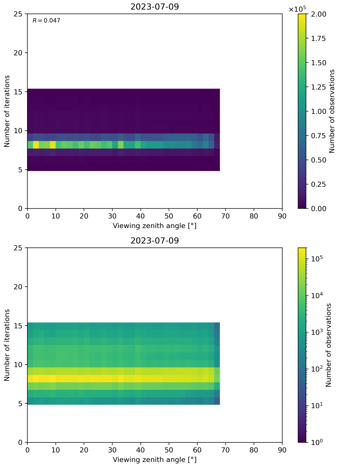
Figure 75: Scatter density plot of “Viewing zenith angle” against “Number of iterations” for 2023-07-08 to 2023-07-10.
