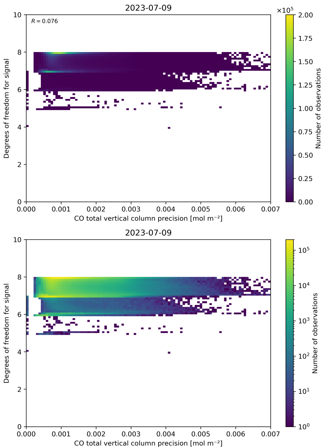
Figure 45: Scatter density plot of “CO total vertical column precision” against “Degrees of freedom for signal” for 2023-07-08 to 2023-07-10.
