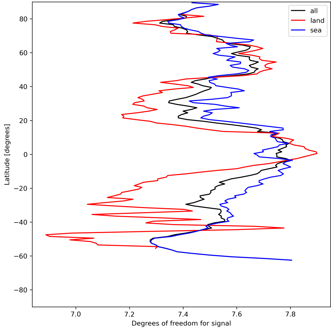
Figure 15: Zonal average of “Degrees of freedom for signal” for 2023-07-08 to 2023-07-10.
