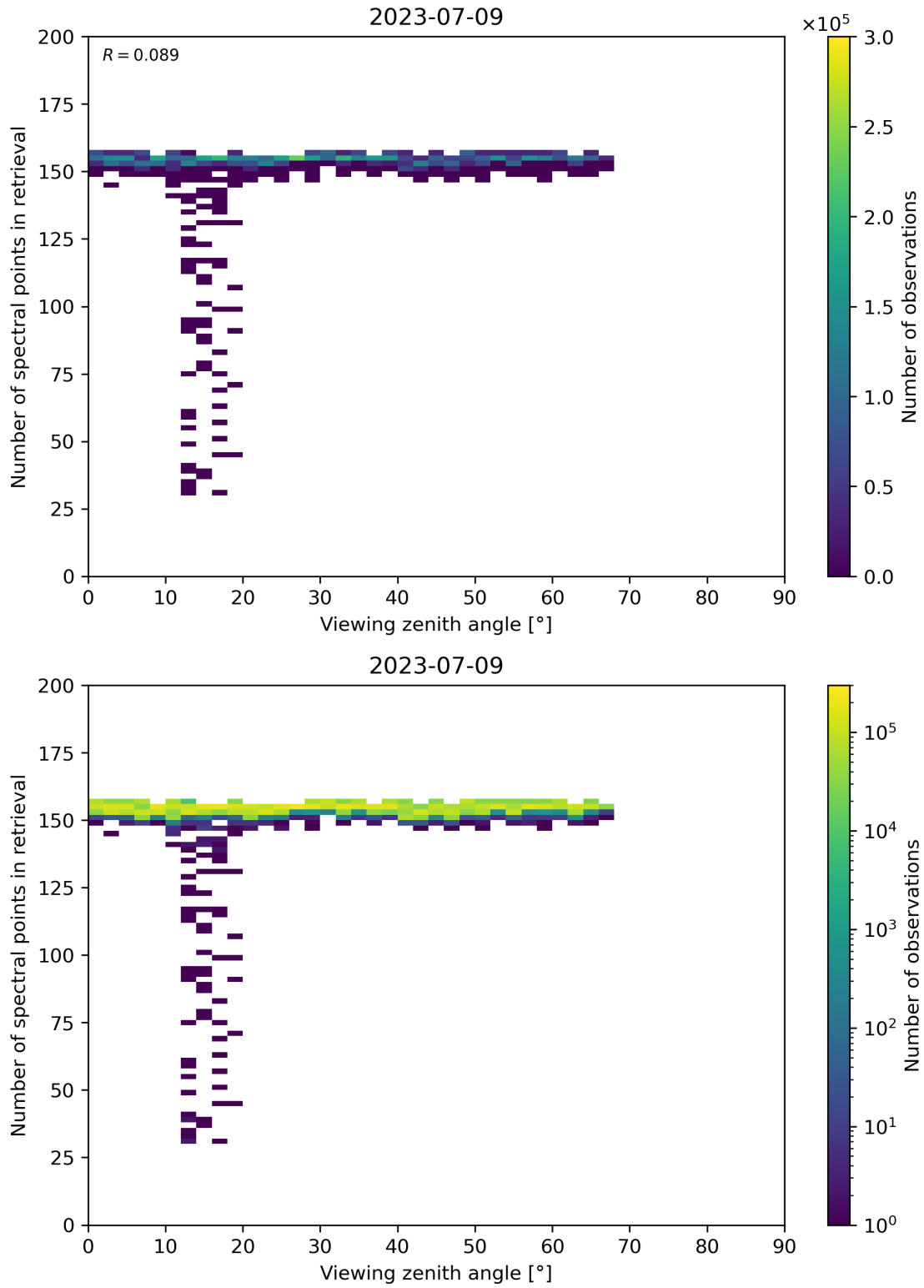
Figure 76: Scatter density plot of “Viewing zenith angle” against “Number of spectral points in retrieval” for 2023-07-08 to 2023-07-10.
