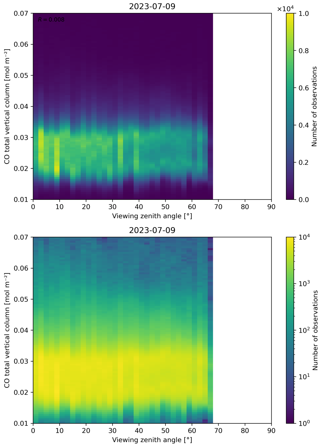
Figure 69: Scatter density plot of “Viewing zenith angle” against “CO total vertical column” for 2023-07-08 to 2023-07-10.
