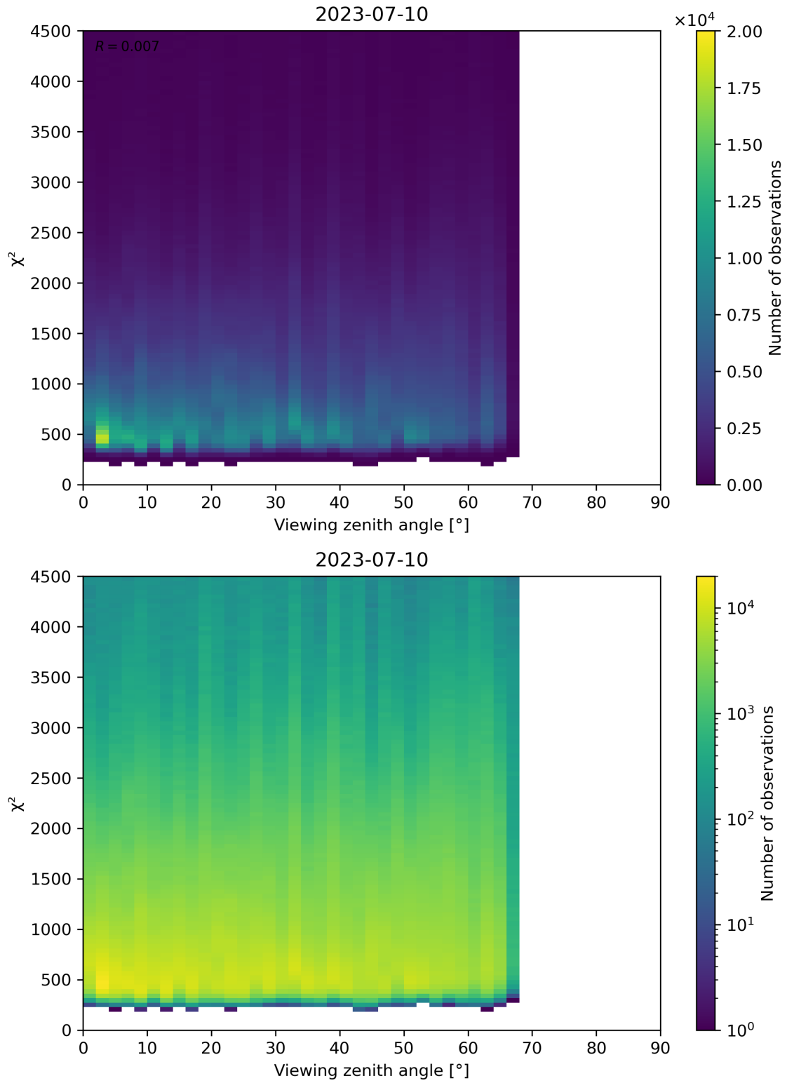
Figure 72: Scatter density plot of “Viewing zenith angle” against “ \chi^2 ” for 2023-07-09 to 2023-07-11.
