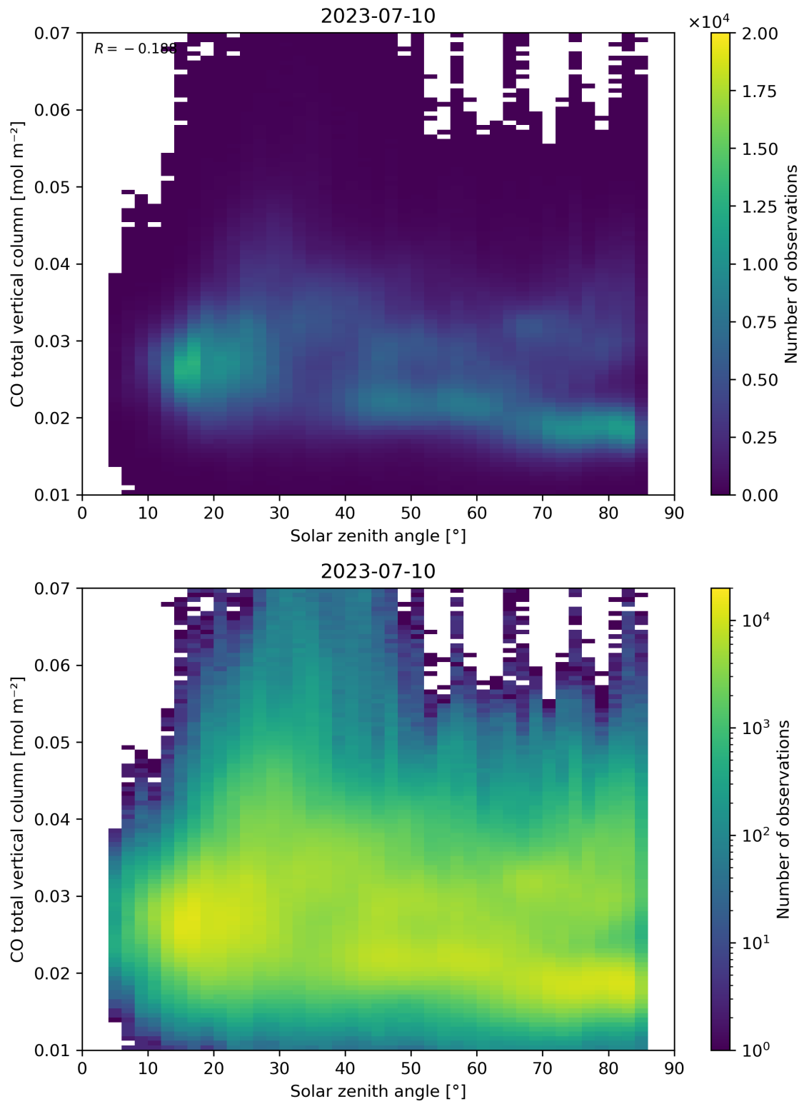
Figure 61: Scatter density plot of “Solar zenith angle” against “CO total vertical column” for 2023-07-09 to 2023-07-11.
