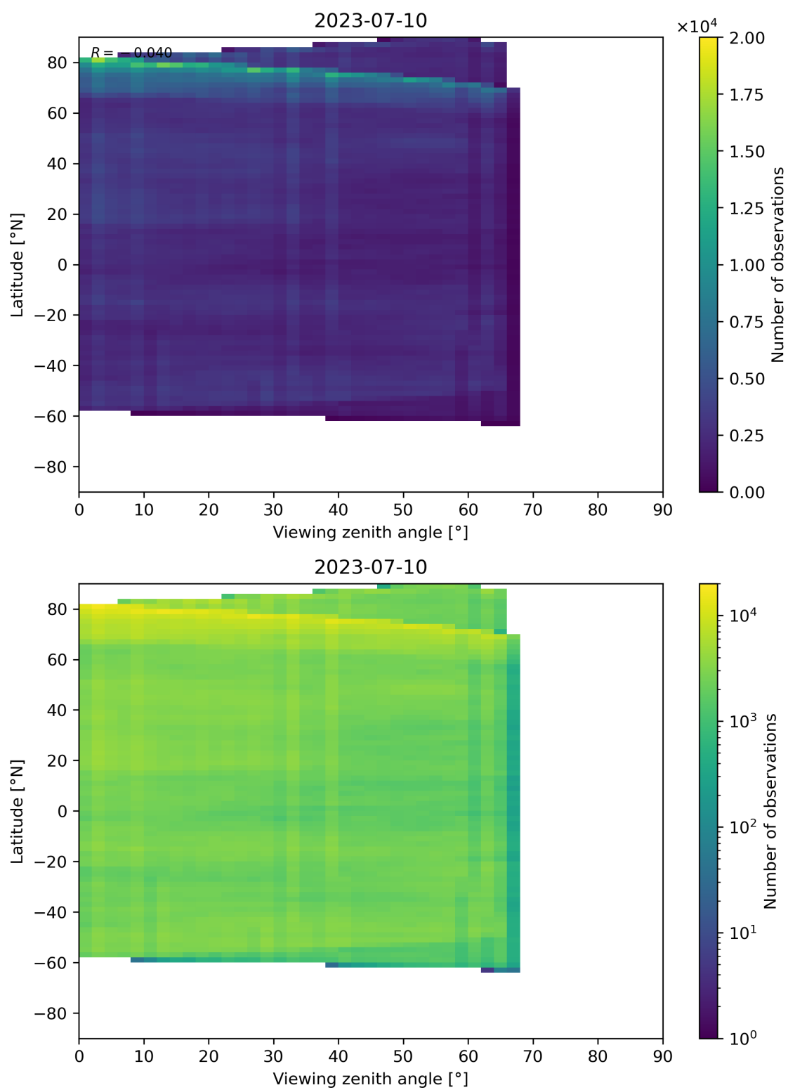
Figure 74: Scatter density plot of “Viewing zenith angle” against “Latitude” for 2023-07-09 to 2023-07-11.
