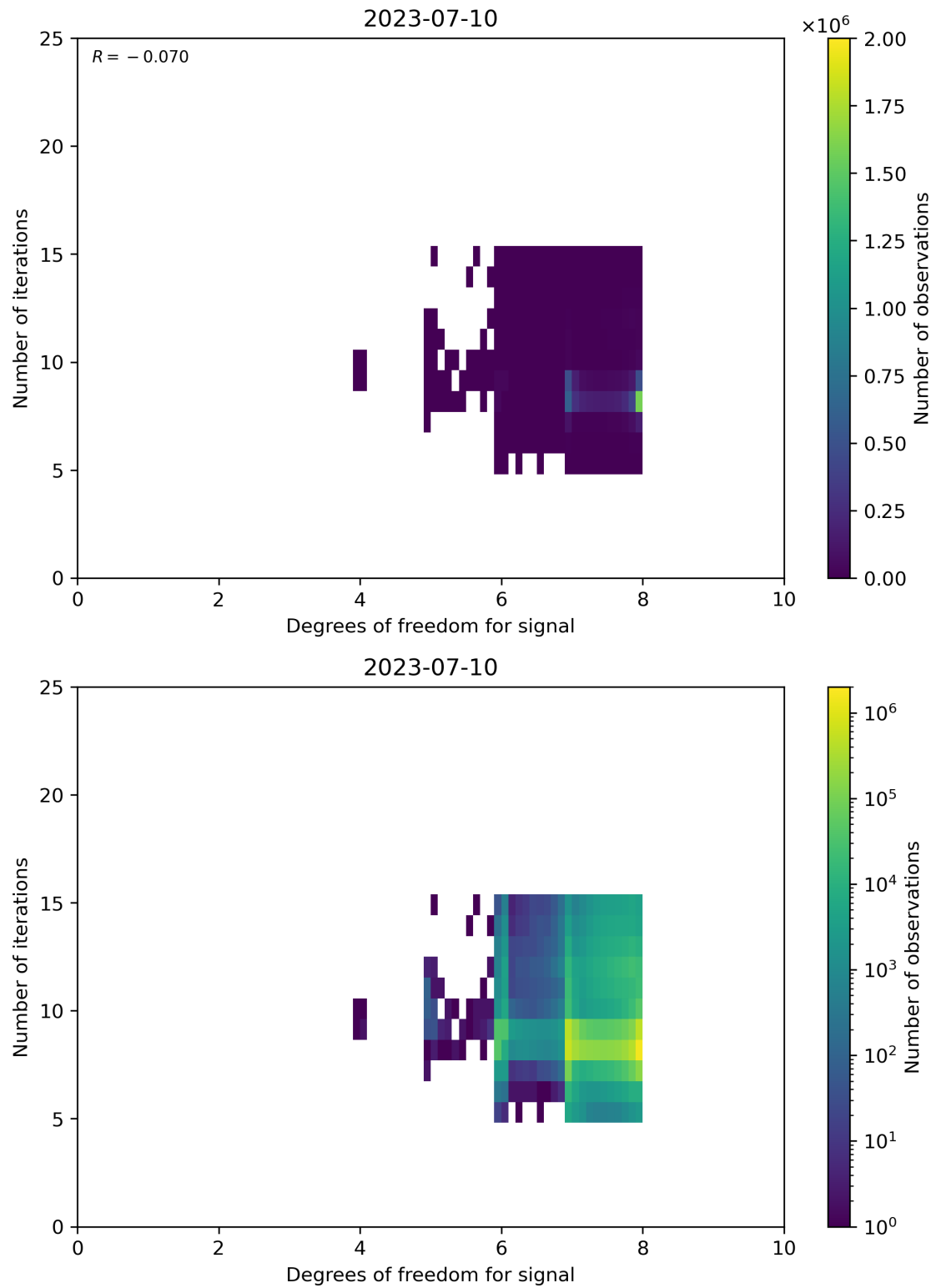
Figure 50: Scatter density plot of “Degrees of freedom for signal” against “Number of iterations” for 2023-07-09 to 2023-07-11.
