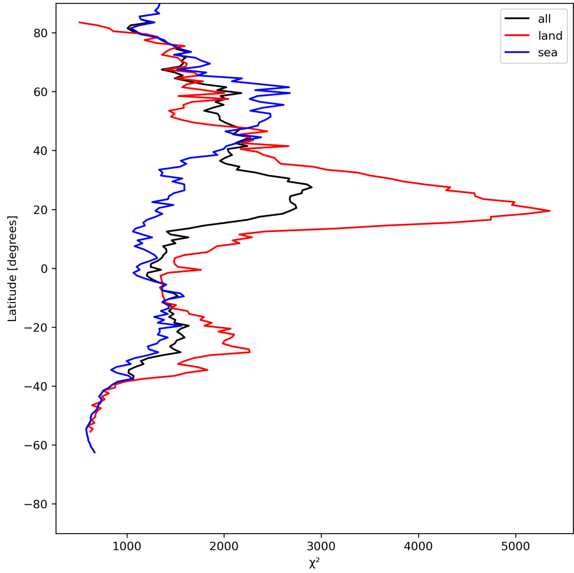
Figure 14: Zonal average of “ \chi^2 ” for 2023-07-09 to 2023-07-11.
