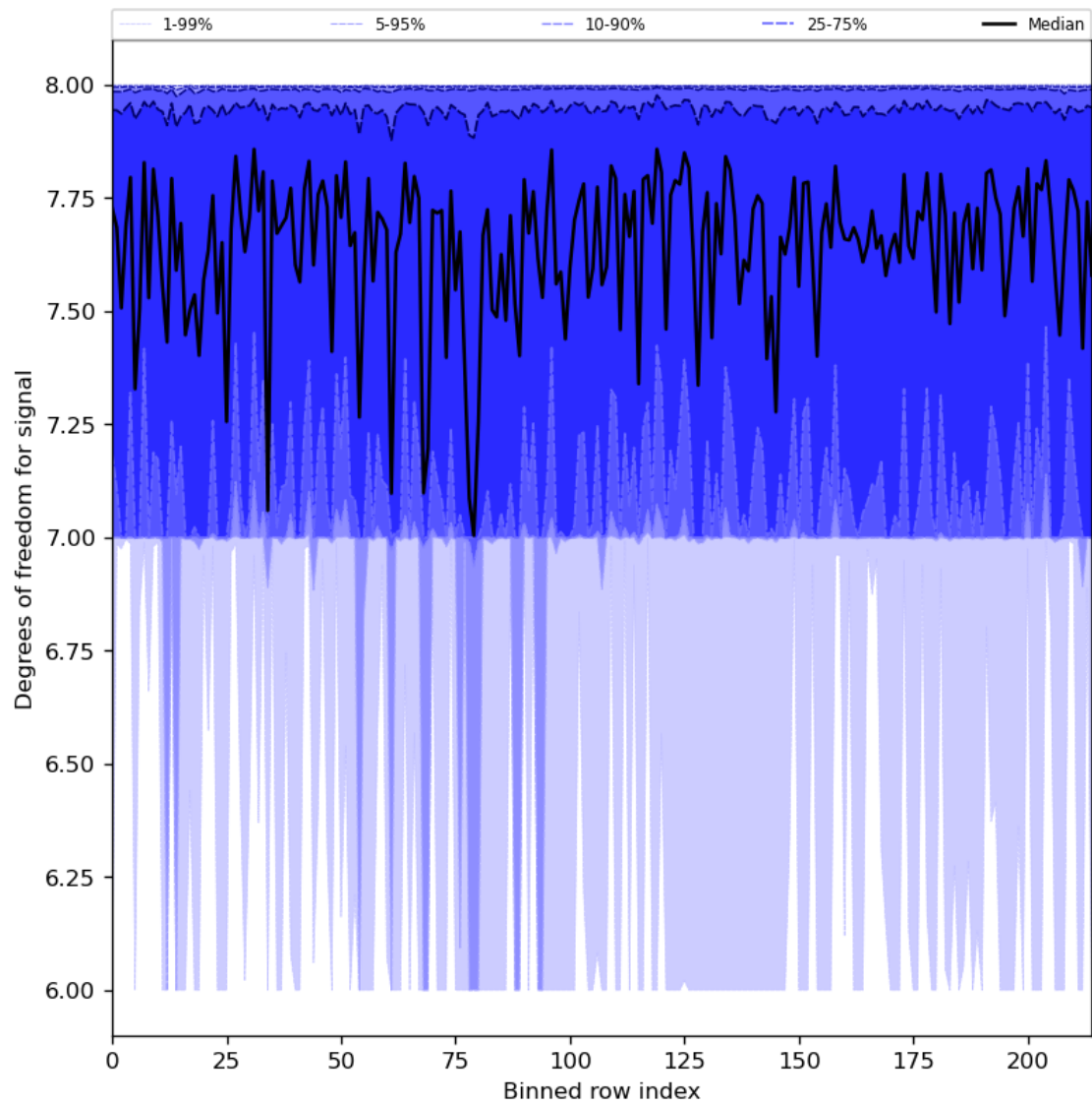
Figure 31: Along track statistics of “Degrees of freedom for signal” for 2023-07-09 to 2023-07-11
