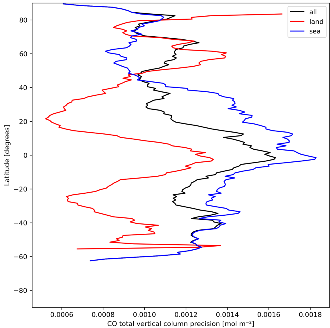
Figure 12: Zonal average of “CO total vertical column precision” for 2023-07-09 to 2023-07-11.
