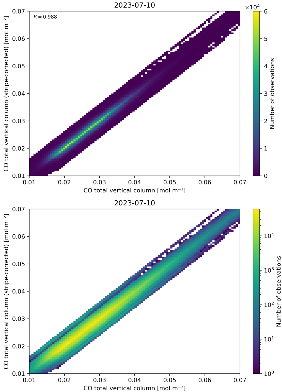
Figure 33: Scatter density plot of “CO total vertical column” against “CO total vertical column (stripe-corrected)” for 2023-07-09 to 2023-07-11.
