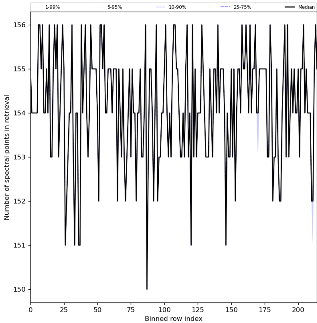
Figure 29: Along track statistics of “Number of spectral points in retrieval” for 2023-07-09 to 2023-07-11
