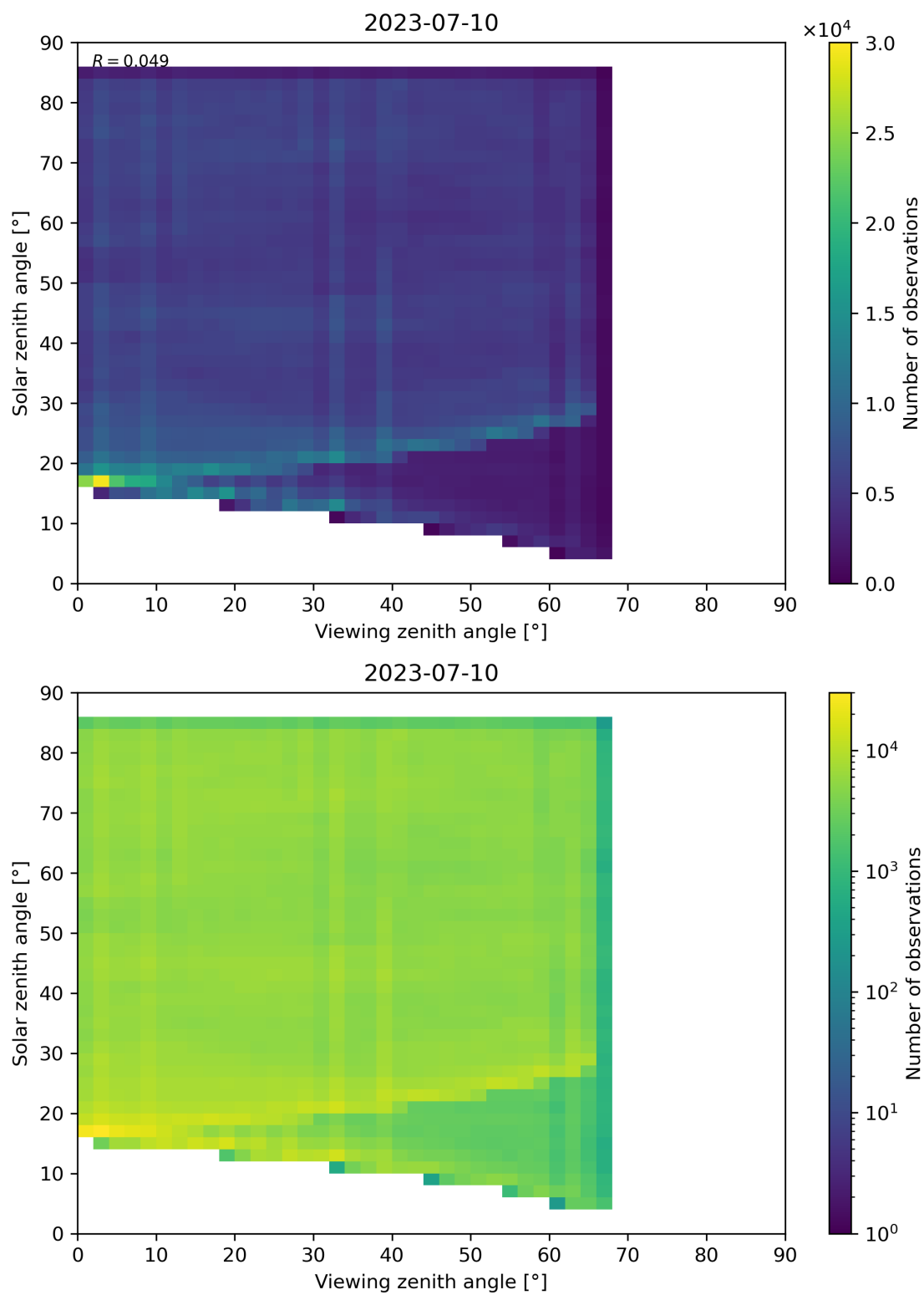
Figure 77: Scatter density plot of “Viewing zenith angle” against “Solar zenith angle” for 2023-07-09 to 2023-07-11.
