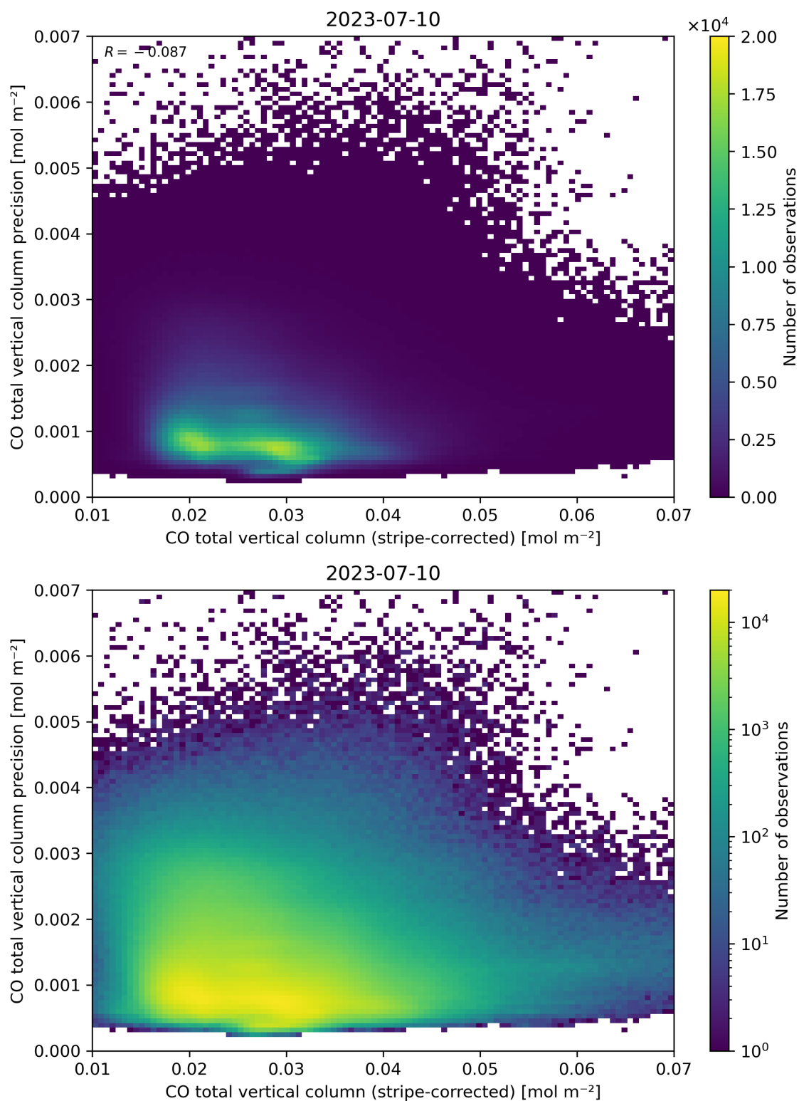
Figure 36: Scatter density plot of “CO total vertical column (stripe-corrected)” against “CO total vertical column precision” for 2023-07-09 to 2023-07-11.
