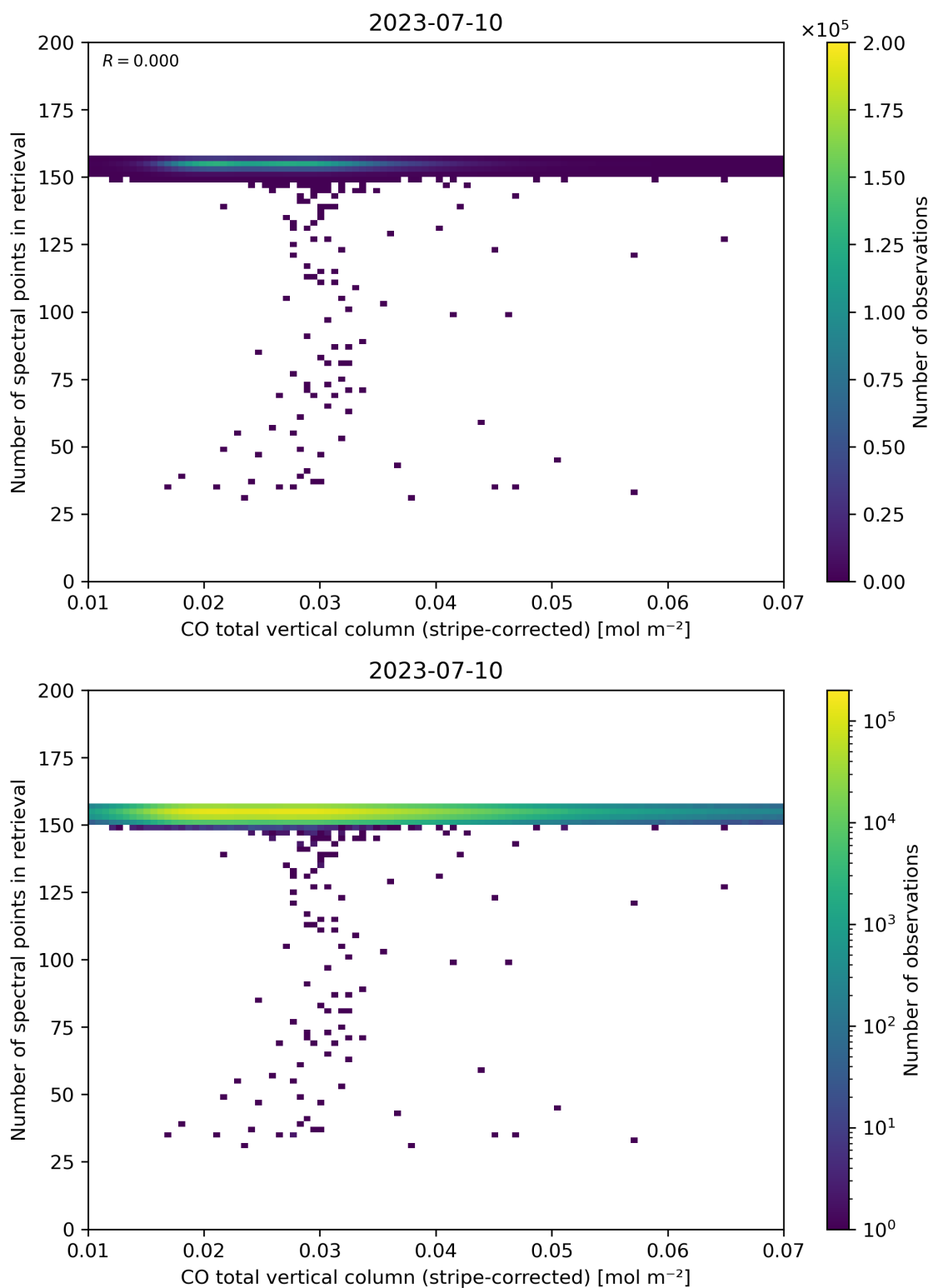
Figure 40: Scatter density plot of “CO total vertical column (stripe-corrected)” against “Number of spectral points in retrieval” for 2023-07-09 to 2023-07-11.
