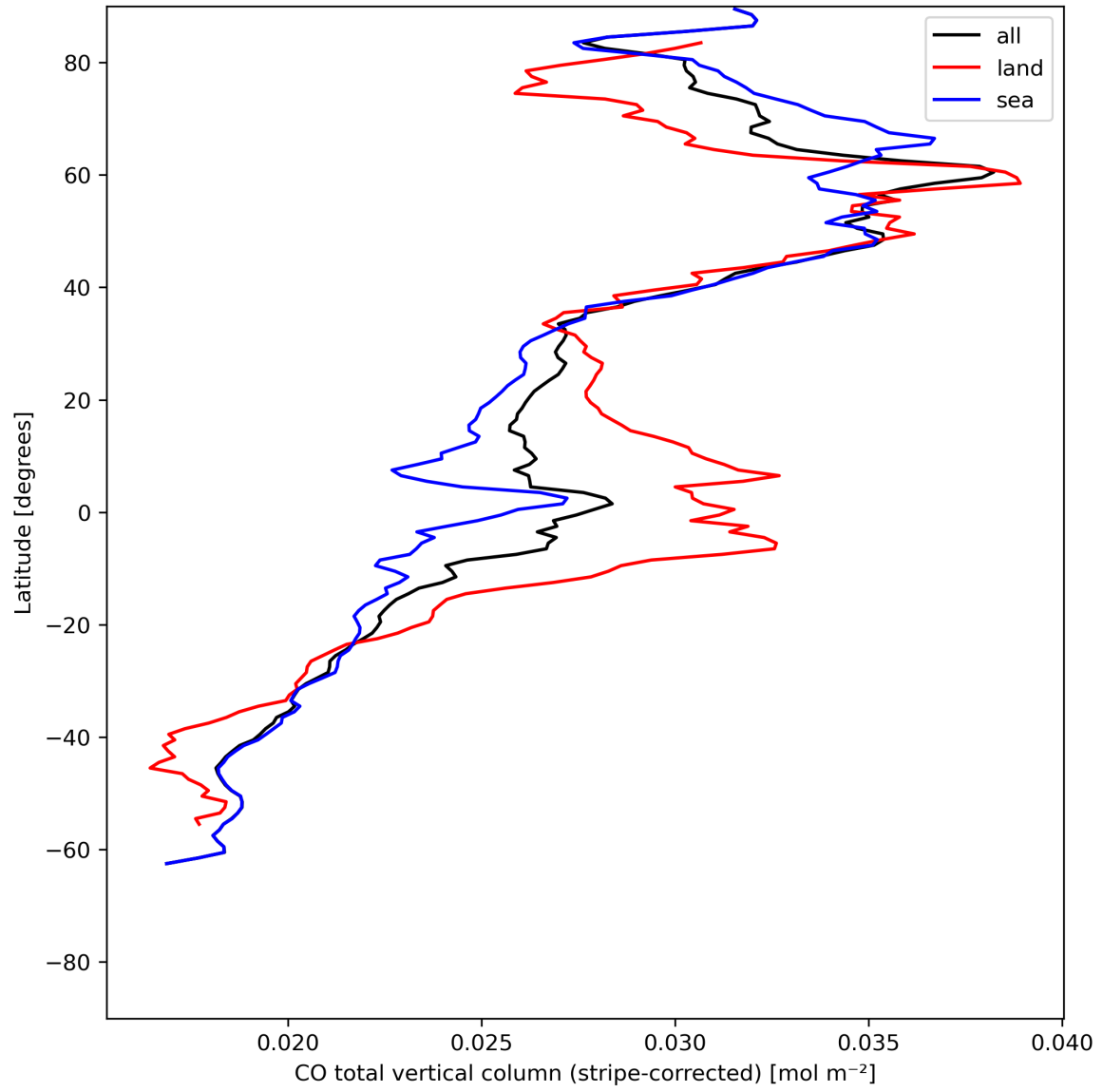
Figure 11: Zonal average of “CO total vertical column (stripe-corrected)” for 2023-07-09 to 2023-07-11.
