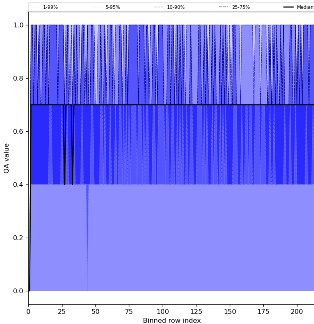
Figure 25: Along track statistics of “QA value” for 2023-07-09 to 2023-07-11
