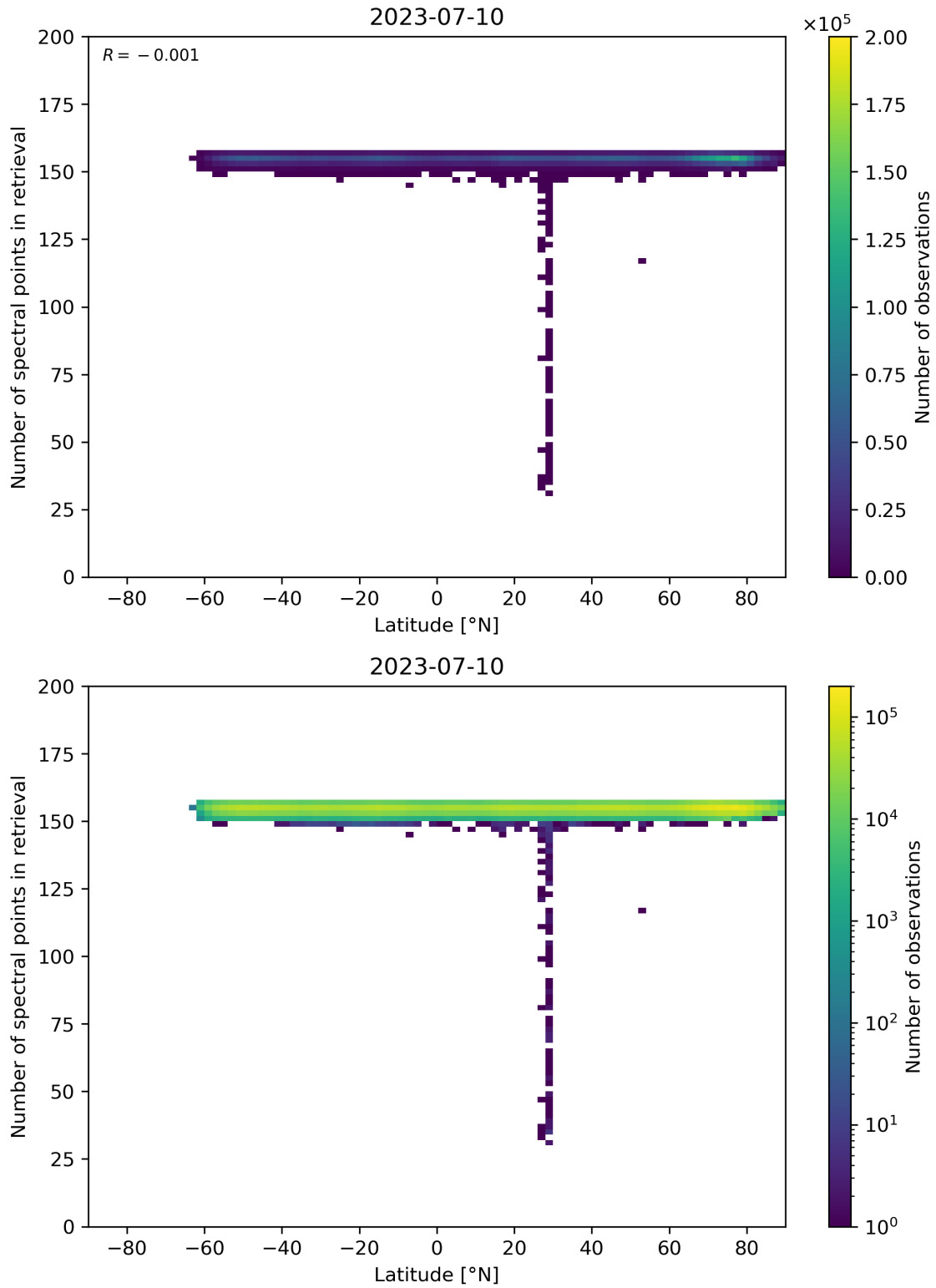
Figure 57: Scatter density plot of “Latitude” against “Number of spectral points in retrieval” for 2023-07-09 to 2023-07-11.
