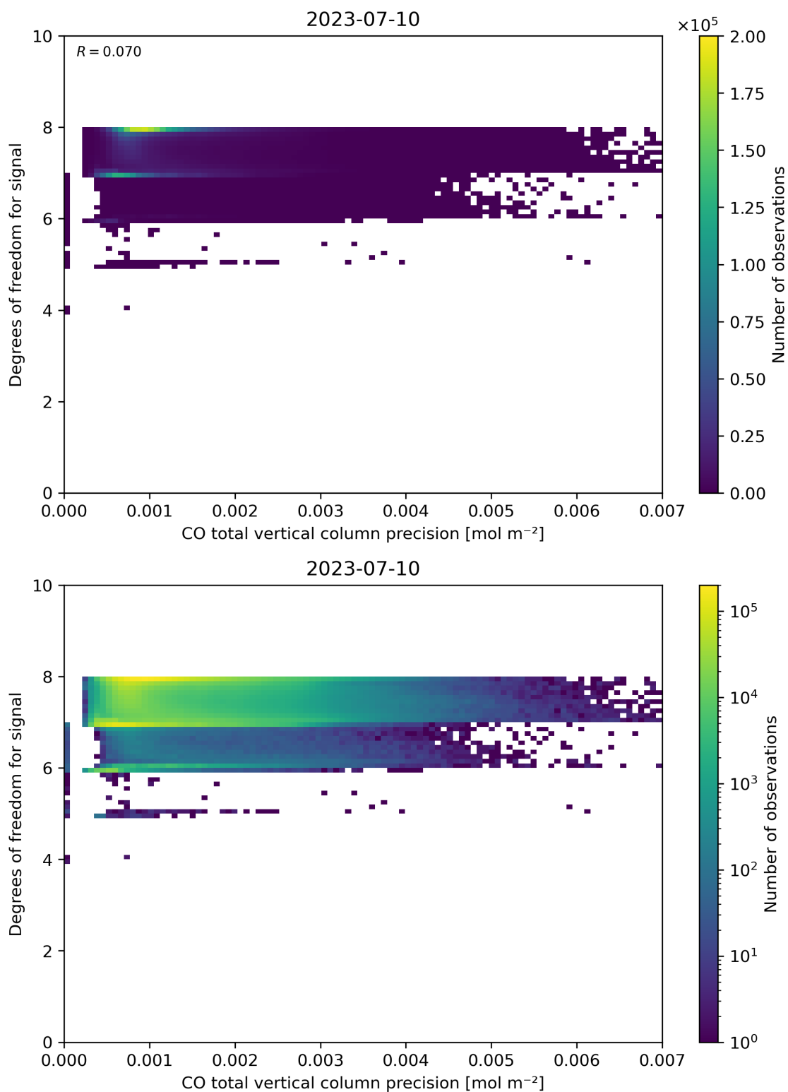
Figure 45: Scatter density plot of “CO total vertical column precision” against “Degrees of freedom for signal” for 2023-07-09 to 2023-07-11.
