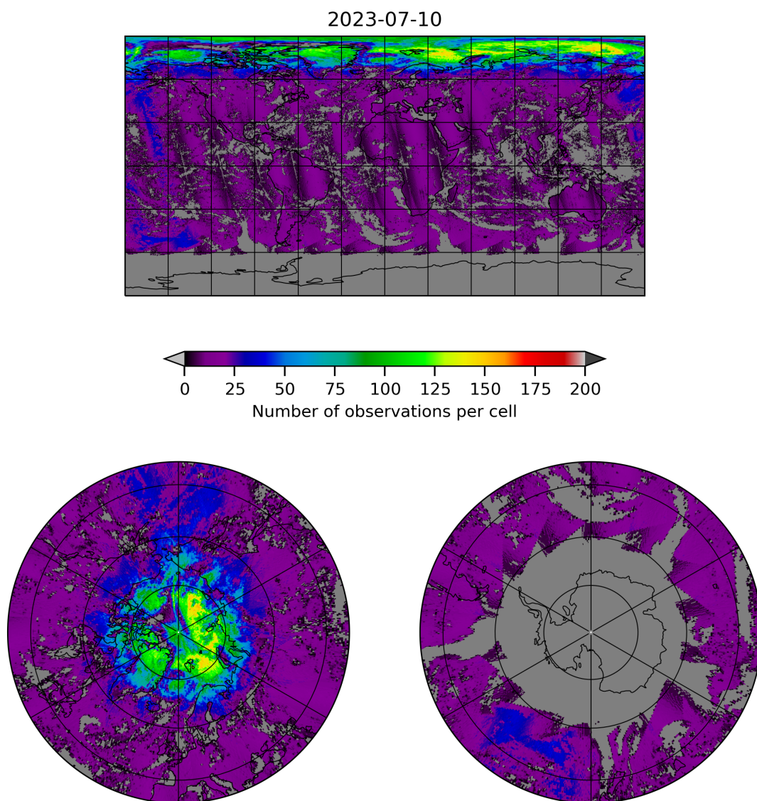
Figure 8: Map of the number of observations for 2023-07-09 to 2023-07-11
