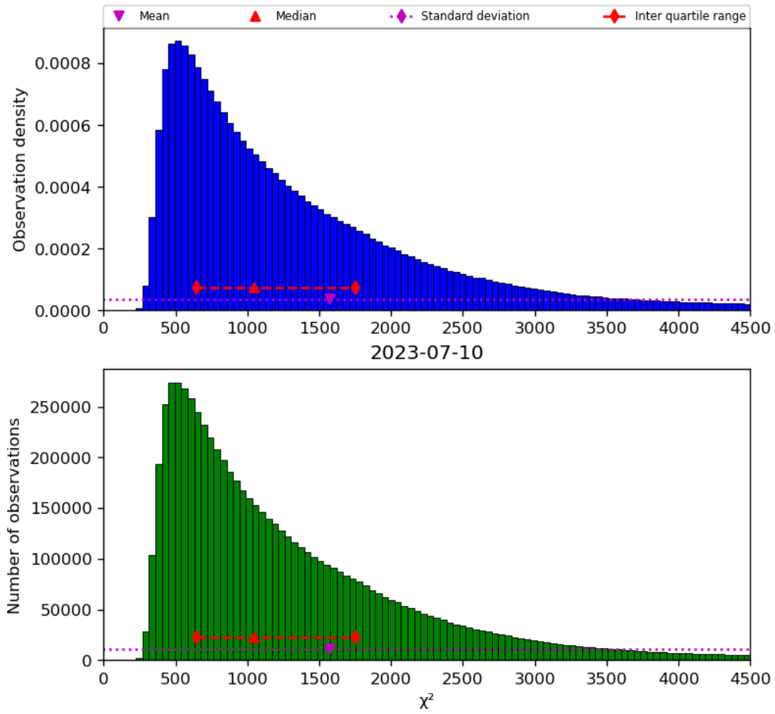
Figure 22: Histogram of “ \chi^2 ” for 2023-07-09 to 2023-07-11
