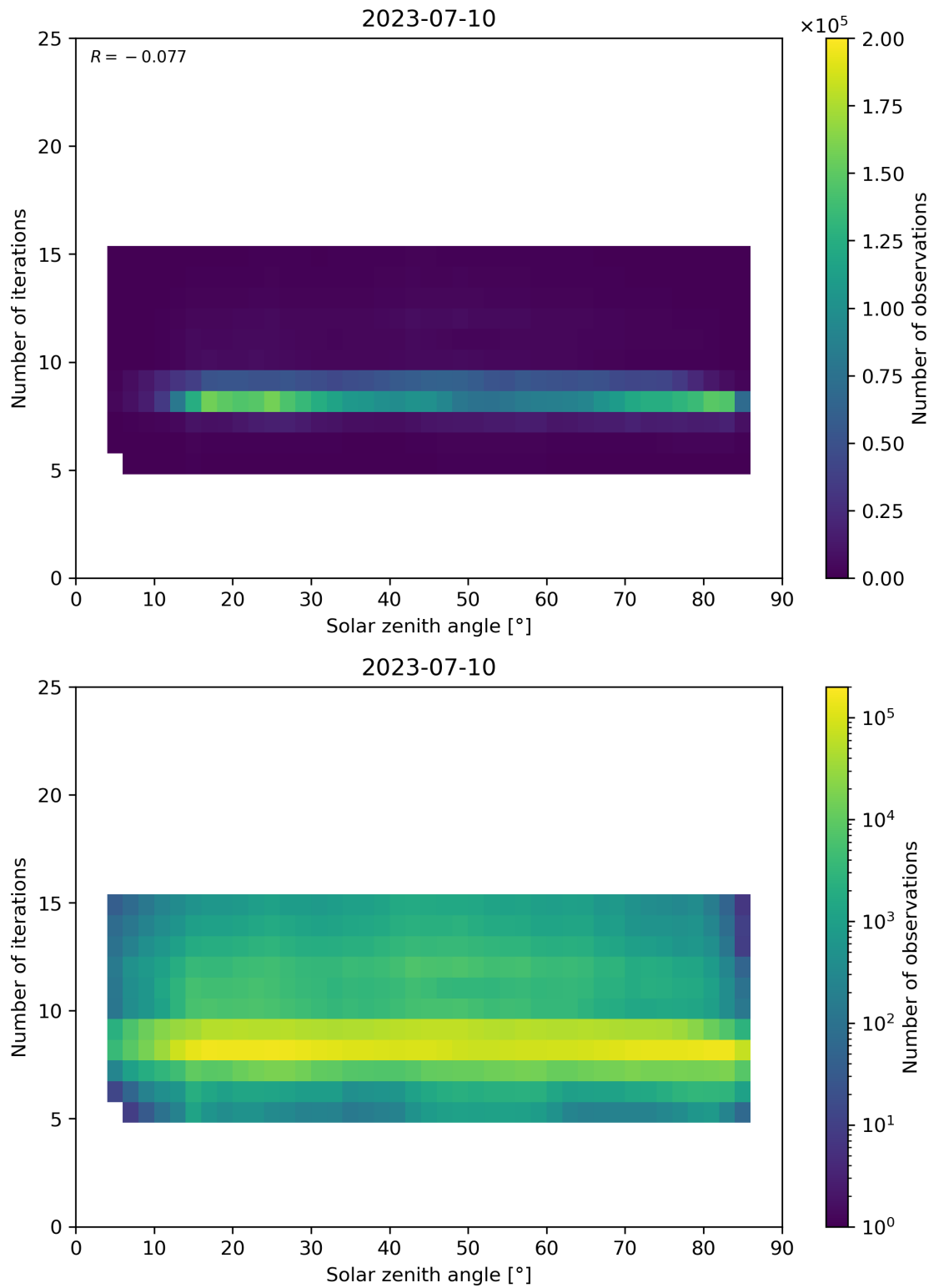
Figure 67: Scatter density plot of “Solar zenith angle” against “Number of iterations” for 2023-07-09 to 2023-07-11.
