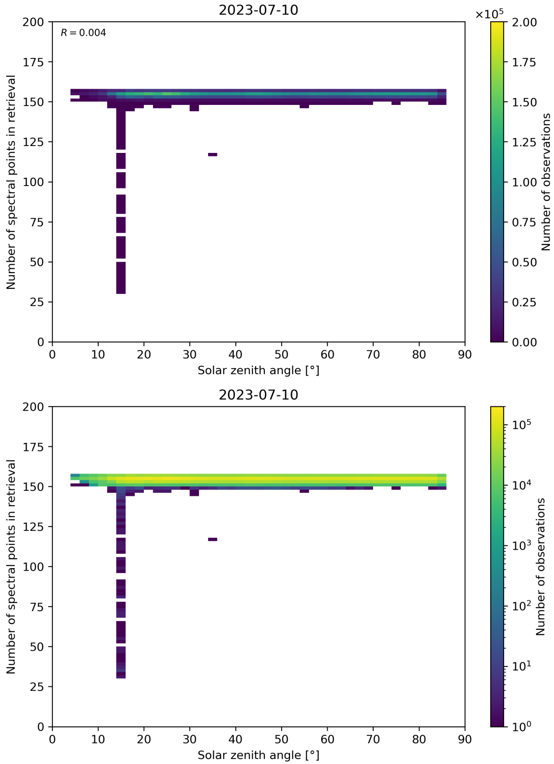
Figure 68: Scatter density plot of “Solar zenith angle” against “Number of spectral points in retrieval” for 2023-07-09 to 2023-07-11.
