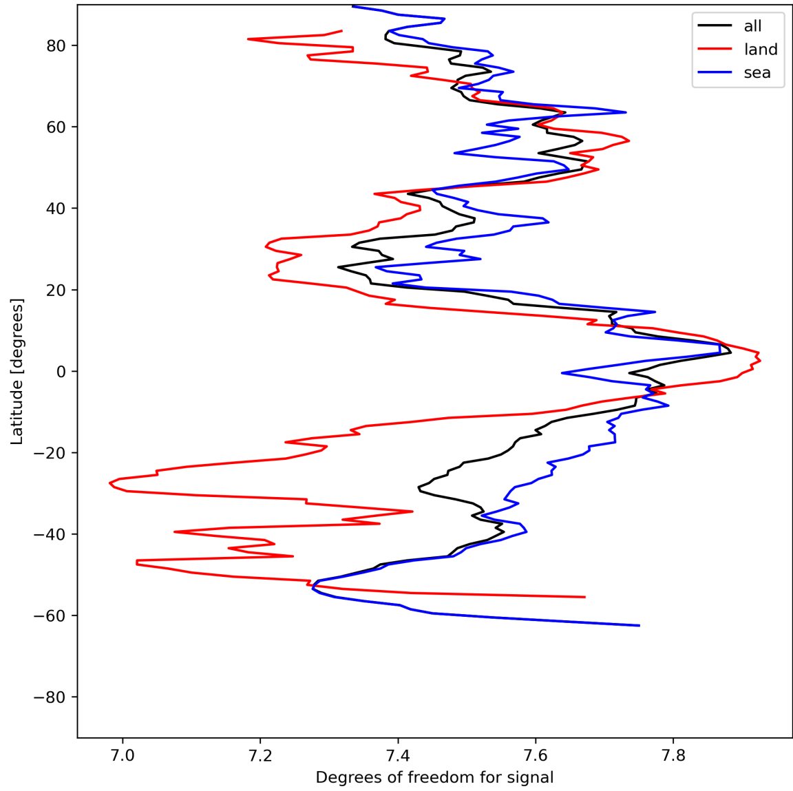
Figure 15: Zonal average of “Degrees of freedom for signal” for 2023-07-09 to 2023-07-11.
