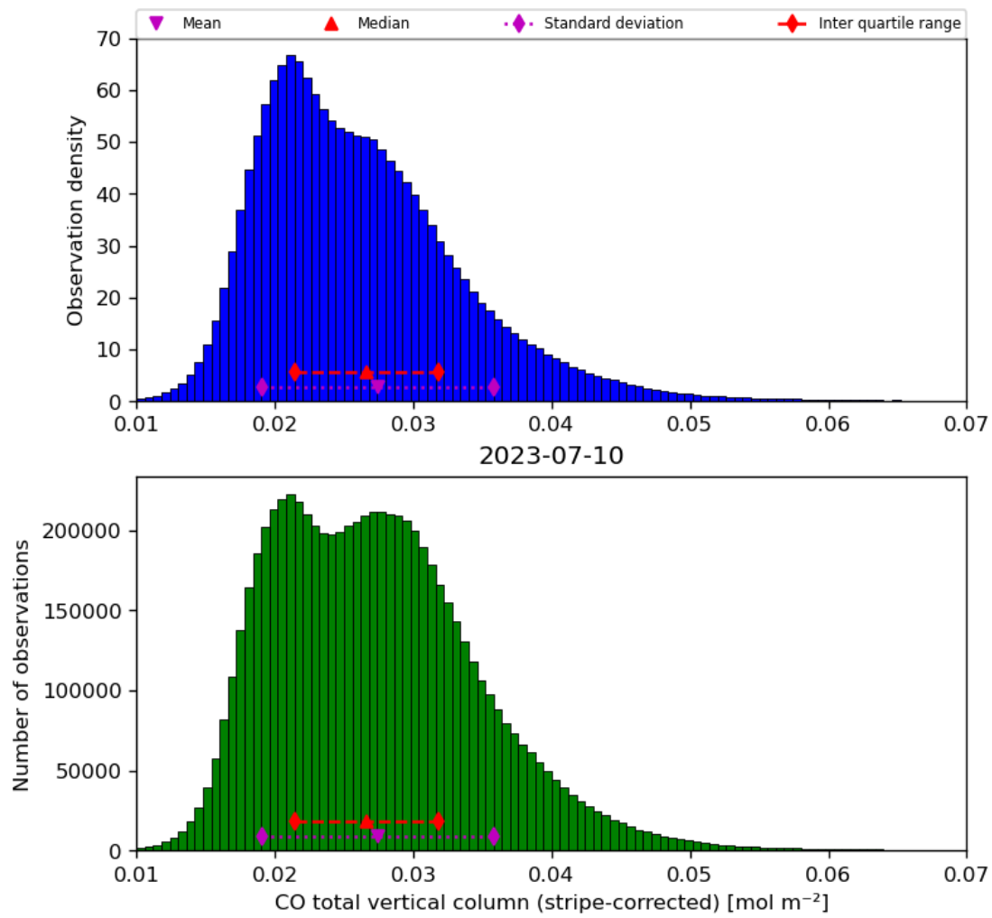
Figure 19: Histogram of “CO total vertical column (stripe-corrected)” for 2023-07-09 to 2023-07-11
