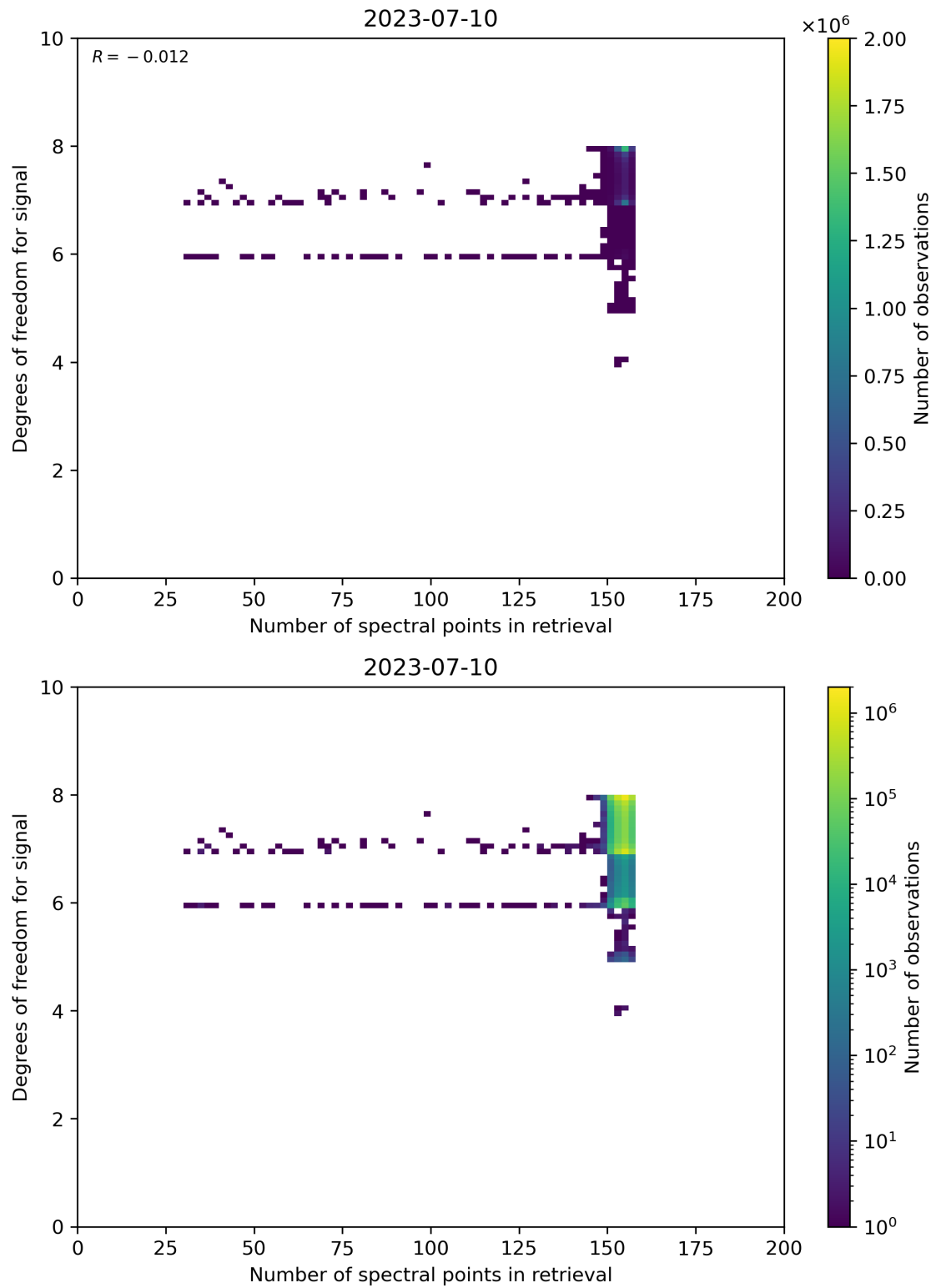
Figure 59: Scatter density plot of “Number of spectral points in retrieval” against “Degrees of freedom for signal” for 2023-07-09 to 2023-07-11.
