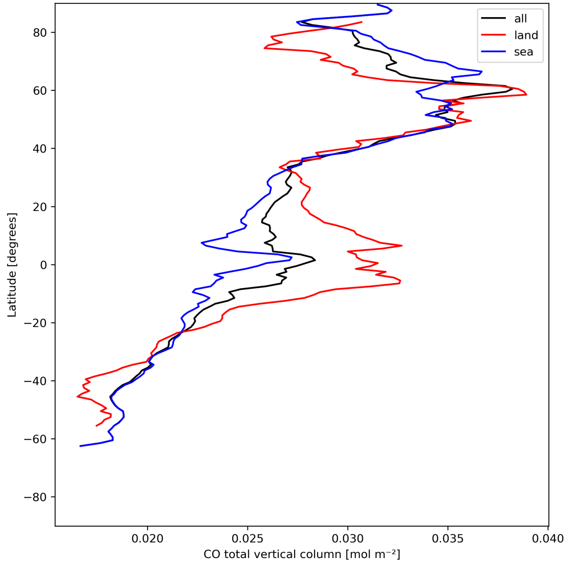
Figure 10: Zonal average of “CO total vertical column” for 2023-07-09 to 2023-07-11.
