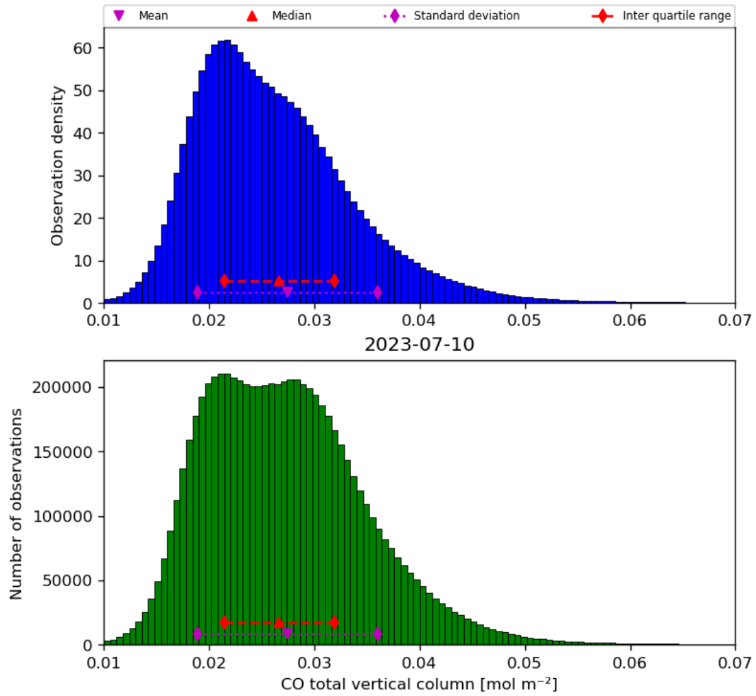
Figure 18: Histogram of “CO total vertical column” for 2023-07-09 to 2023-07-11
