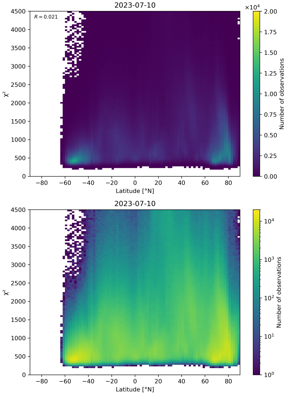
Figure 54: Scatter density plot of “Latitude” against “ \chi^2 ” for 2023-07-09 to 2023-07-11.
