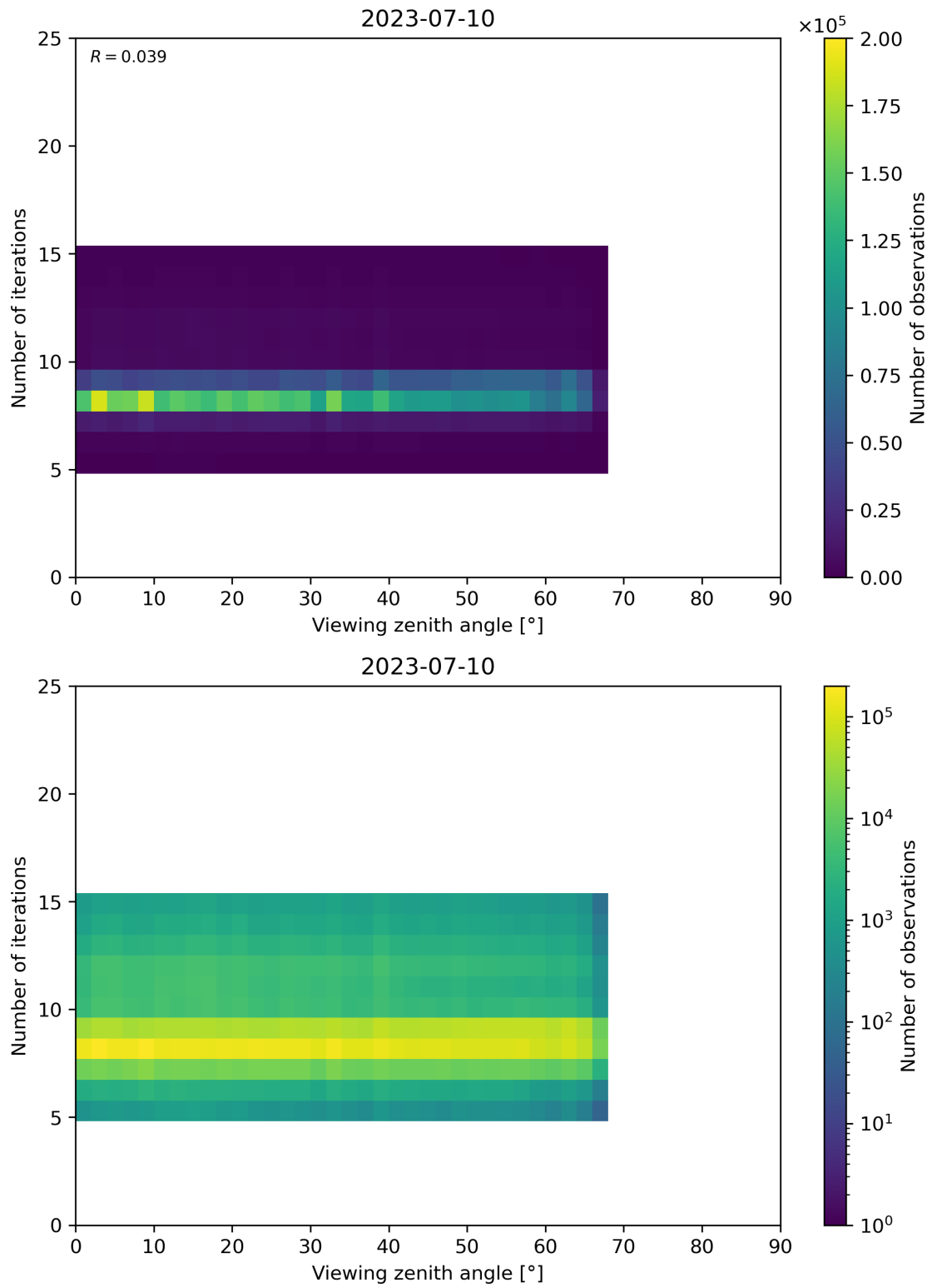
Figure 75: Scatter density plot of “Viewing zenith angle” against “Number of iterations” for 2023-07-09 to 2023-07-11.
