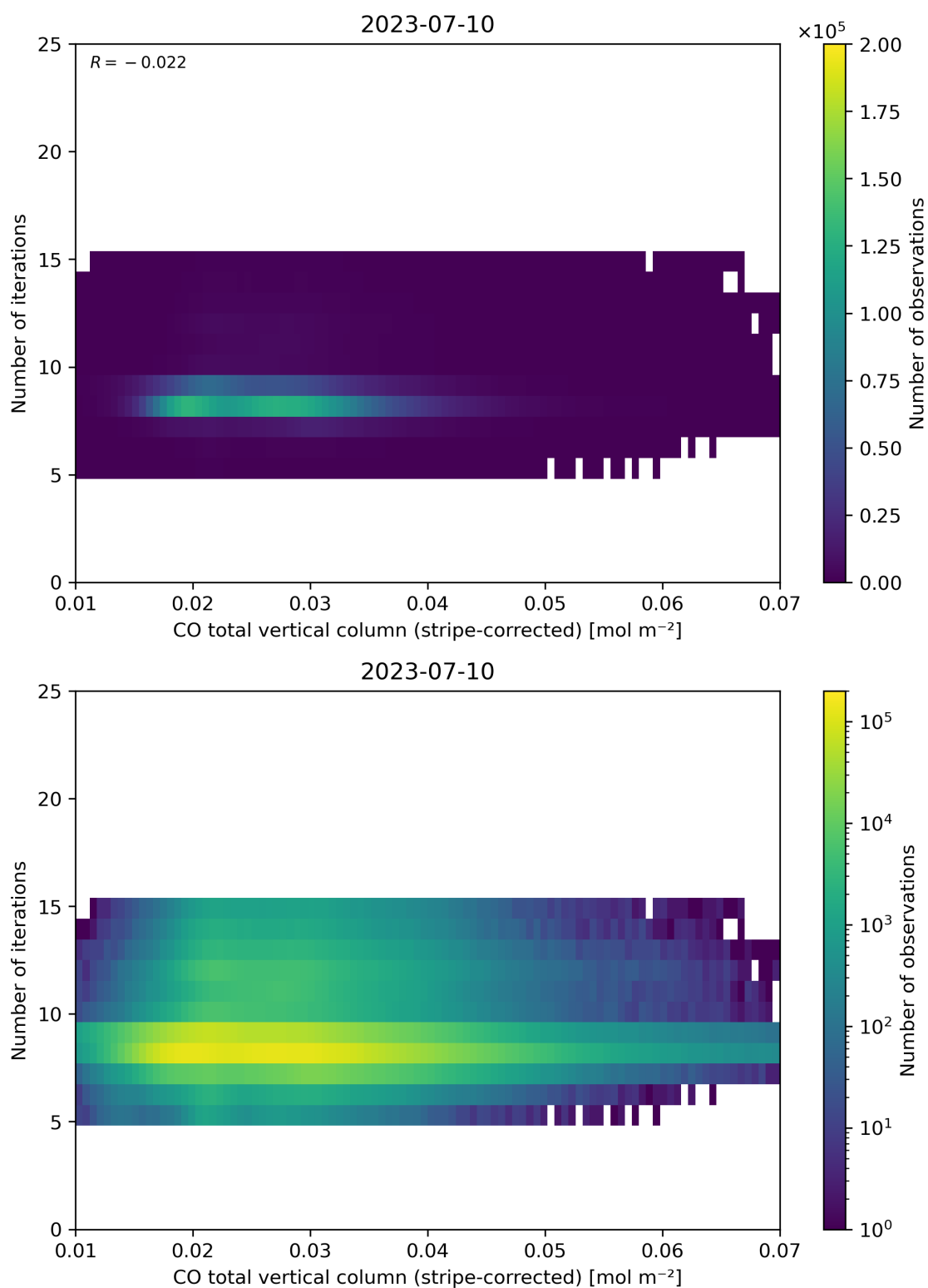
Figure 39: Scatter density plot of “CO total vertical column (stripe-corrected)” against “Number of iterations” for 2023-07-09 to 2023-07-11.
