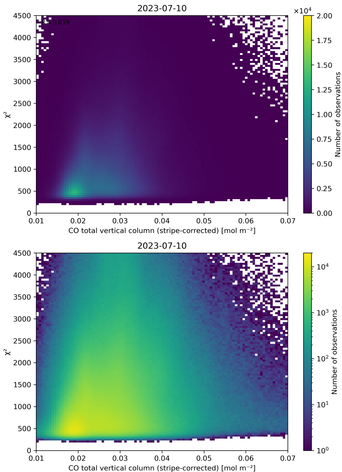
Figure 37: Scatter density plot of “CO total vertical column (stripe-corrected)” against “ \chi^2 ” for 2023-07-09 to 2023-07-11.
