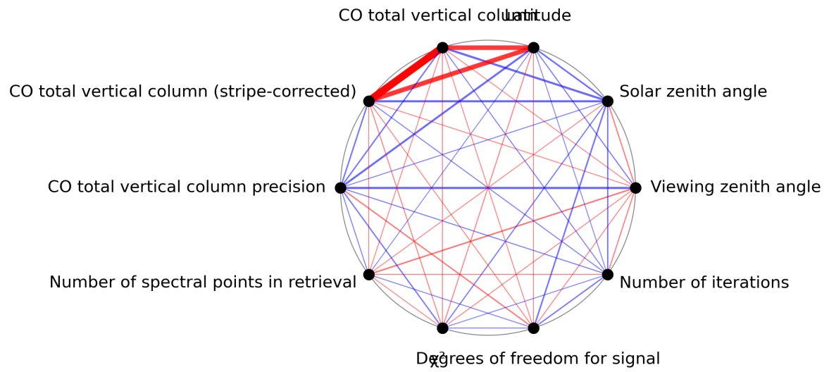
Figure 1: Map of correlation graph for 2023-07-09 to 2023-07-11.
