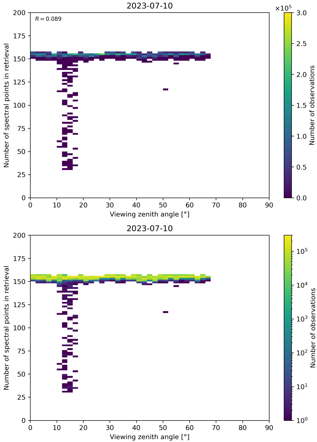
Figure 76: Scatter density plot of “Viewing zenith angle” against “Number of spectral points in retrieval” for 2023-07-09 to 2023-07-11.
