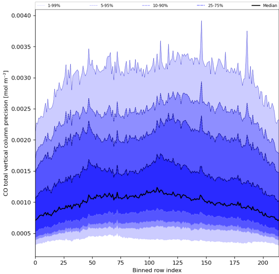
Figure 28: Along track statistics of “CO total vertical column precision” for 2023-07-09 to 2023-07-11
