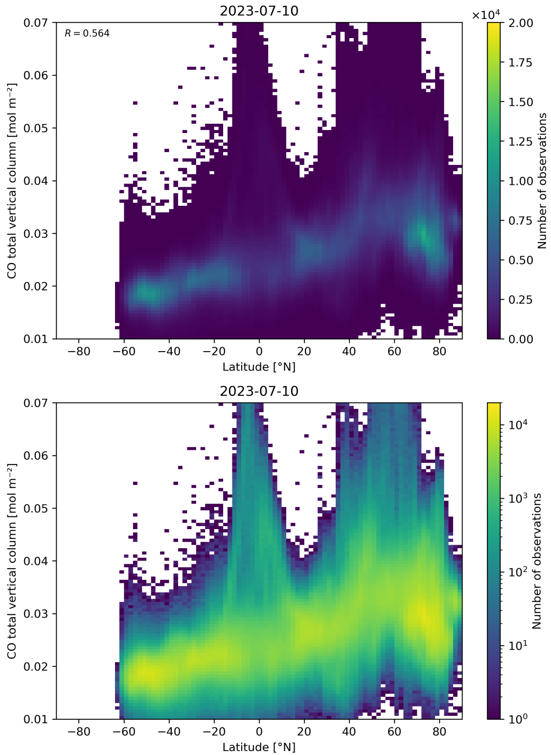
Figure 51: Scatter density plot of “Latitude” against “CO total vertical column” for 2023-07-09 to 2023-07-11.
