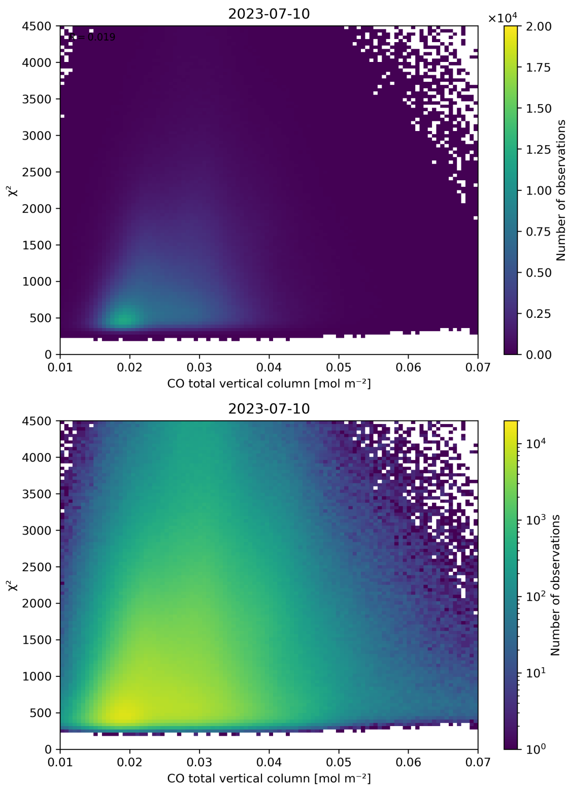
Figure 35: Scatter density plot of “CO total vertical column” against “ \chi^2 ” for 2023-07-09 to 2023-07-11.
