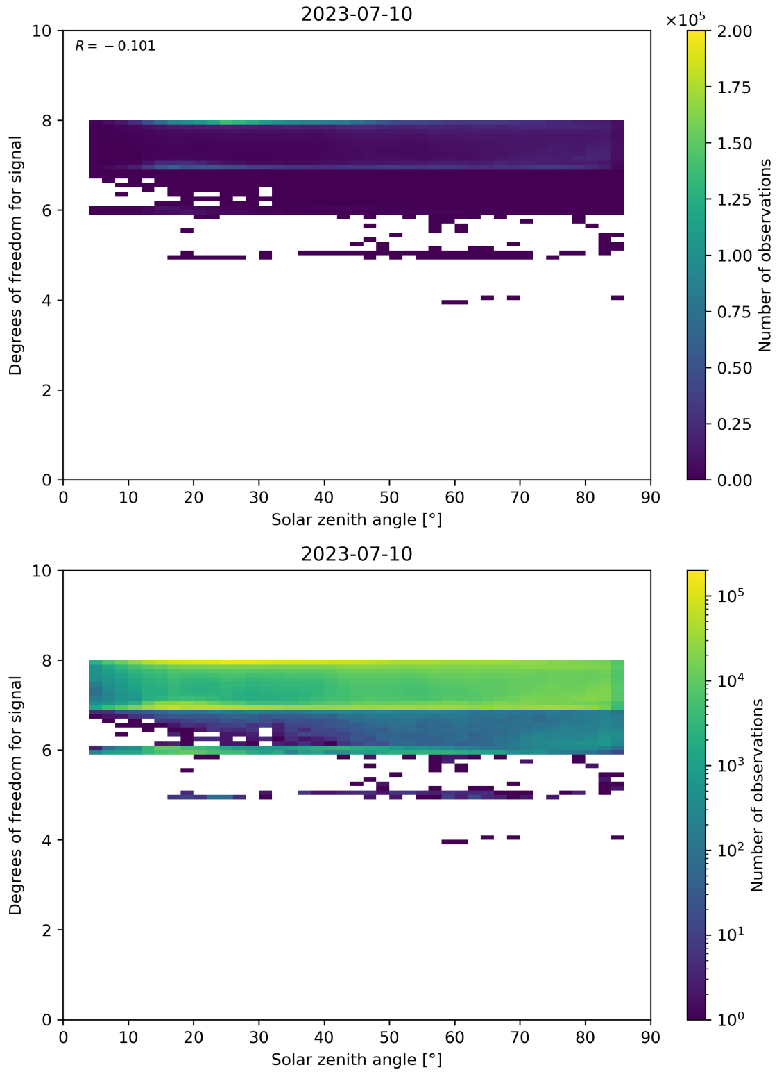
Figure 65: Scatter density plot of “Solar zenith angle” against “Degrees of freedom for signal” for 2023-07-09 to 2023-07-11.
