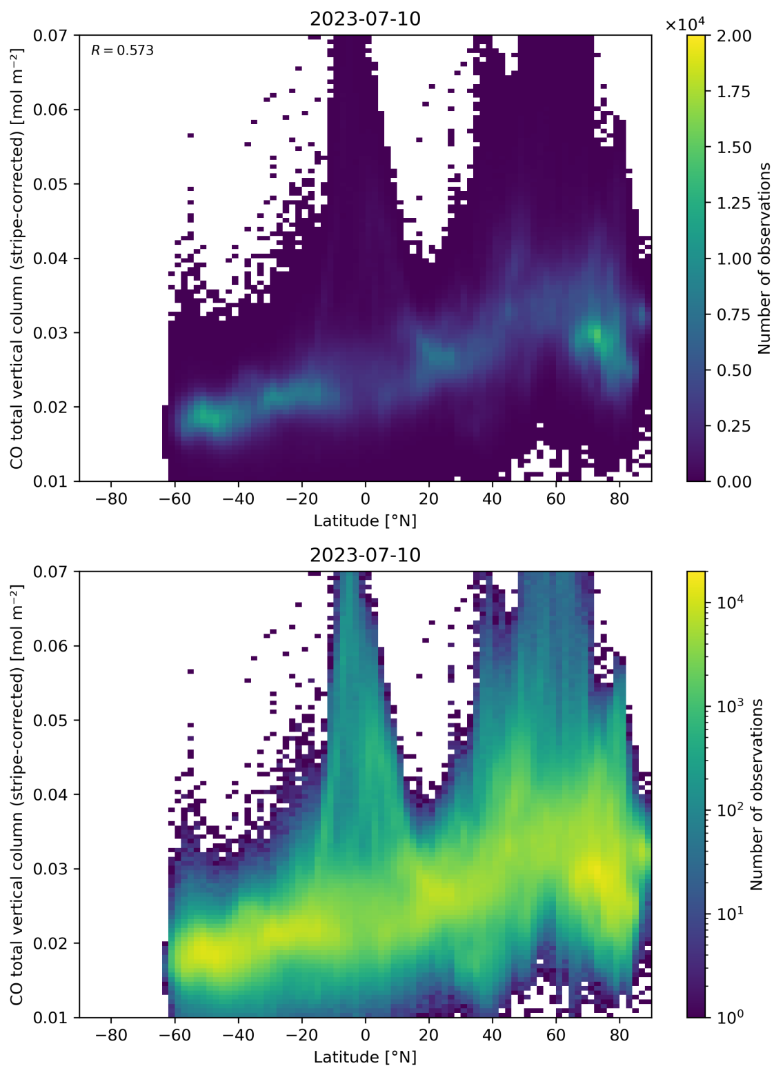
Figure 52: Scatter density plot of “Latitude” against “CO total vertical column (stripe-corrected)” for 2023-07-09 to 2023-07-11.
