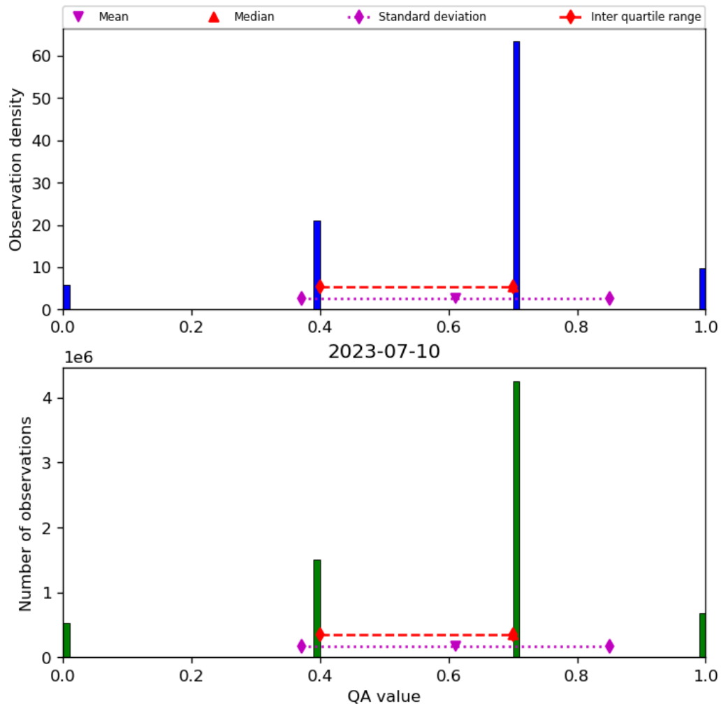
Figure 17: Histogram of “QA value” for 2023-07-09 to 2023-07-11
