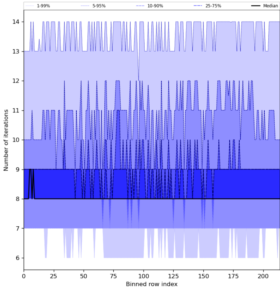
Figure 32: Along track statistics of “Number of iterations” for 2023-07-09 to 2023-07-11
