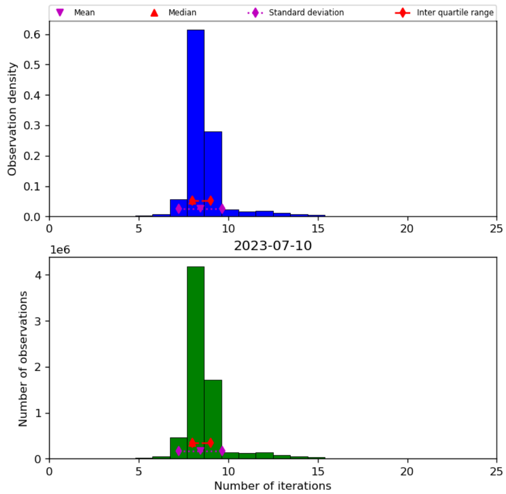
Figure 24: Histogram of "Number of iterations" for 2023-07-09 to 2023-07-11
