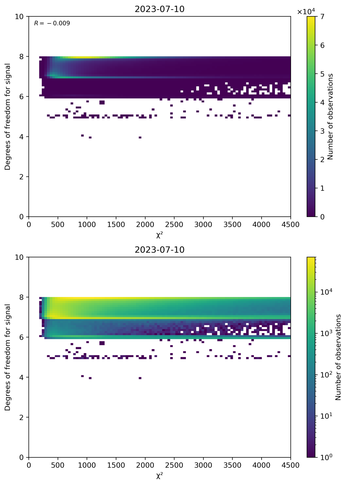
Figure 48: Scatter density plot of “ \chi^2 ” against “Degrees of freedom for signal” for 2023-07-09 to 2023-07-11.
