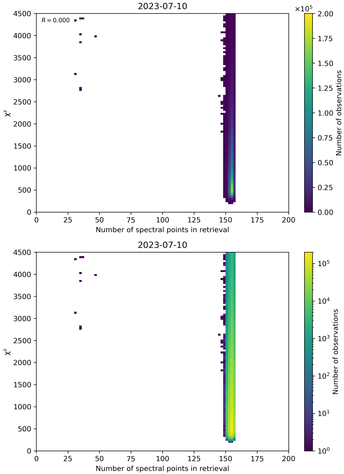
Figure 58: Scatter density plot of “Number of spectral points in retrieval” against “ \chi^2 ” for 2023-07-09 to 2023-07-11.
