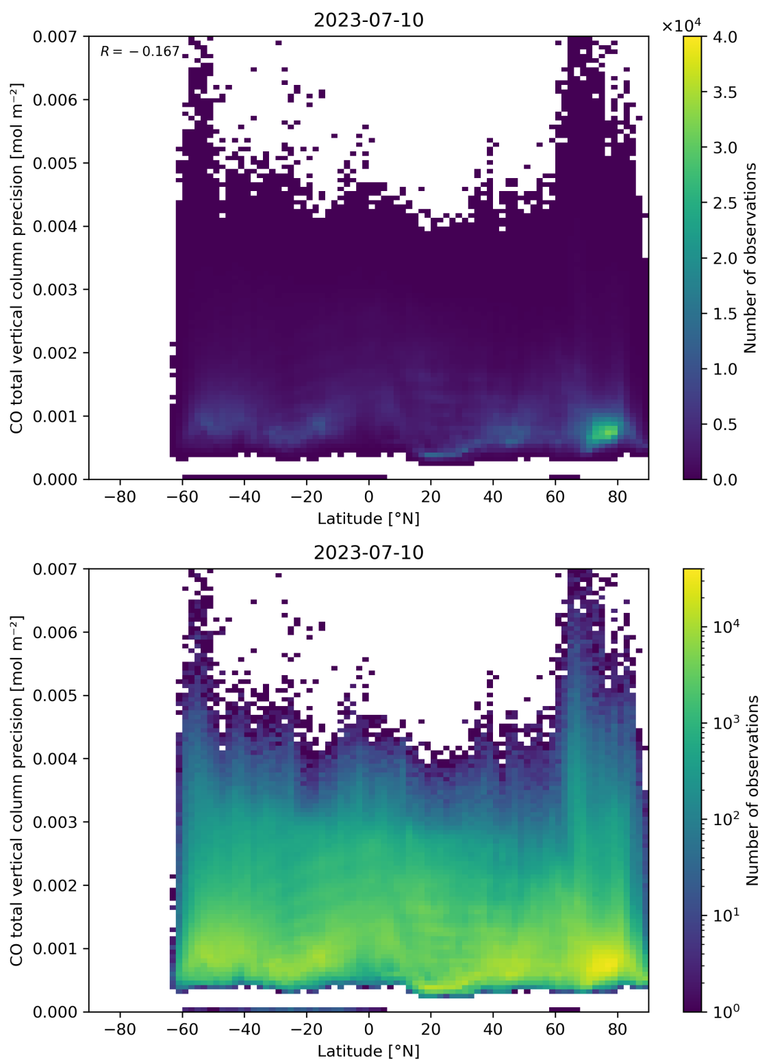
Figure 53: Scatter density plot of “Latitude” against “CO total vertical column precision” for 2023-07-09 to 2023-07-11.
