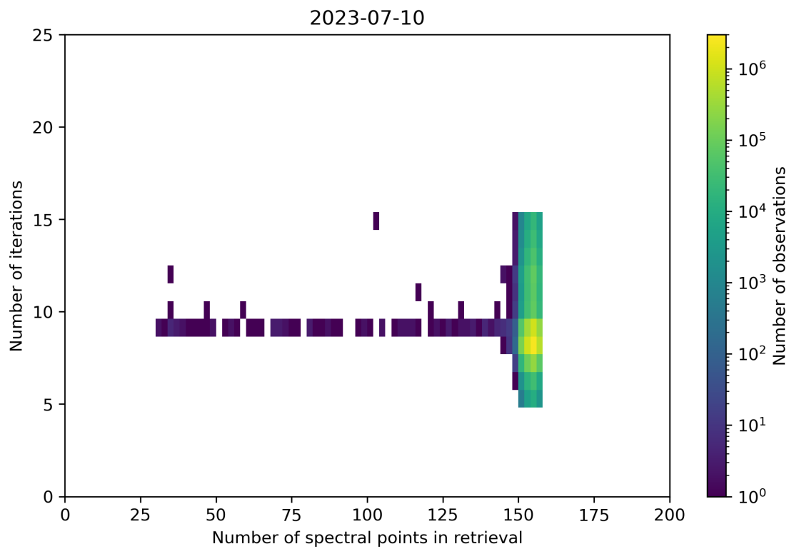
Figure 60: Scatter density plot of “Number of spectral points in retrieval” against “Number of iterations” for 2023-07-09 to 2023-07-11.
