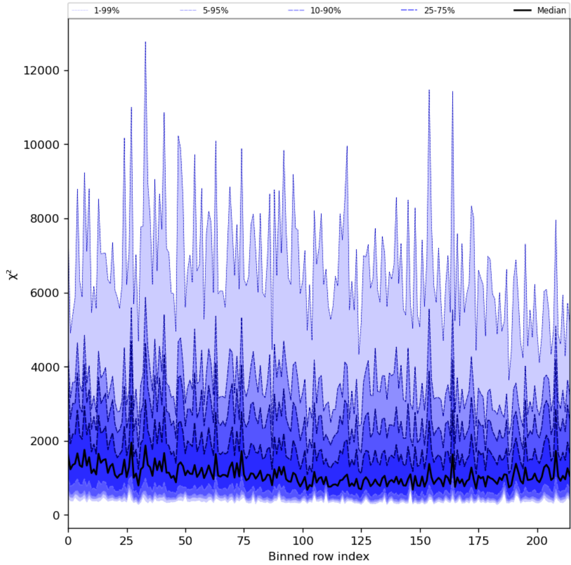
Figure 30: Along track statistics of “ \chi^2 ” for 2023-07-09 to 2023-07-11
