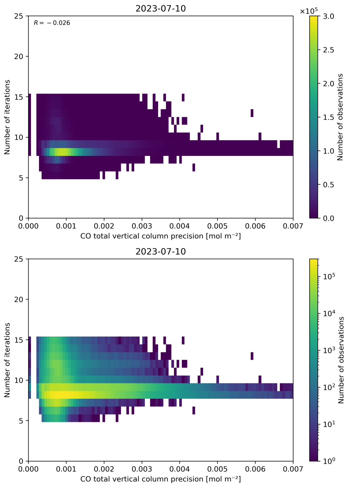
Figure 46: Scatter density plot of “CO total vertical column precision” against “Number of iterations” for 2023-07-09 to 2023-07-11.
