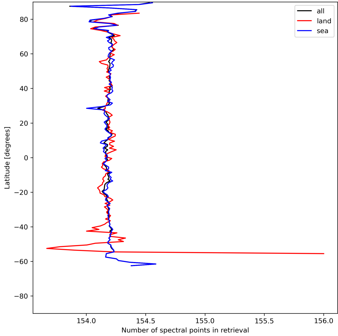
Figure 13: Zonal average of “Number of spectral points in retrieval” for 2023-07-09 to 2023-07-11.
