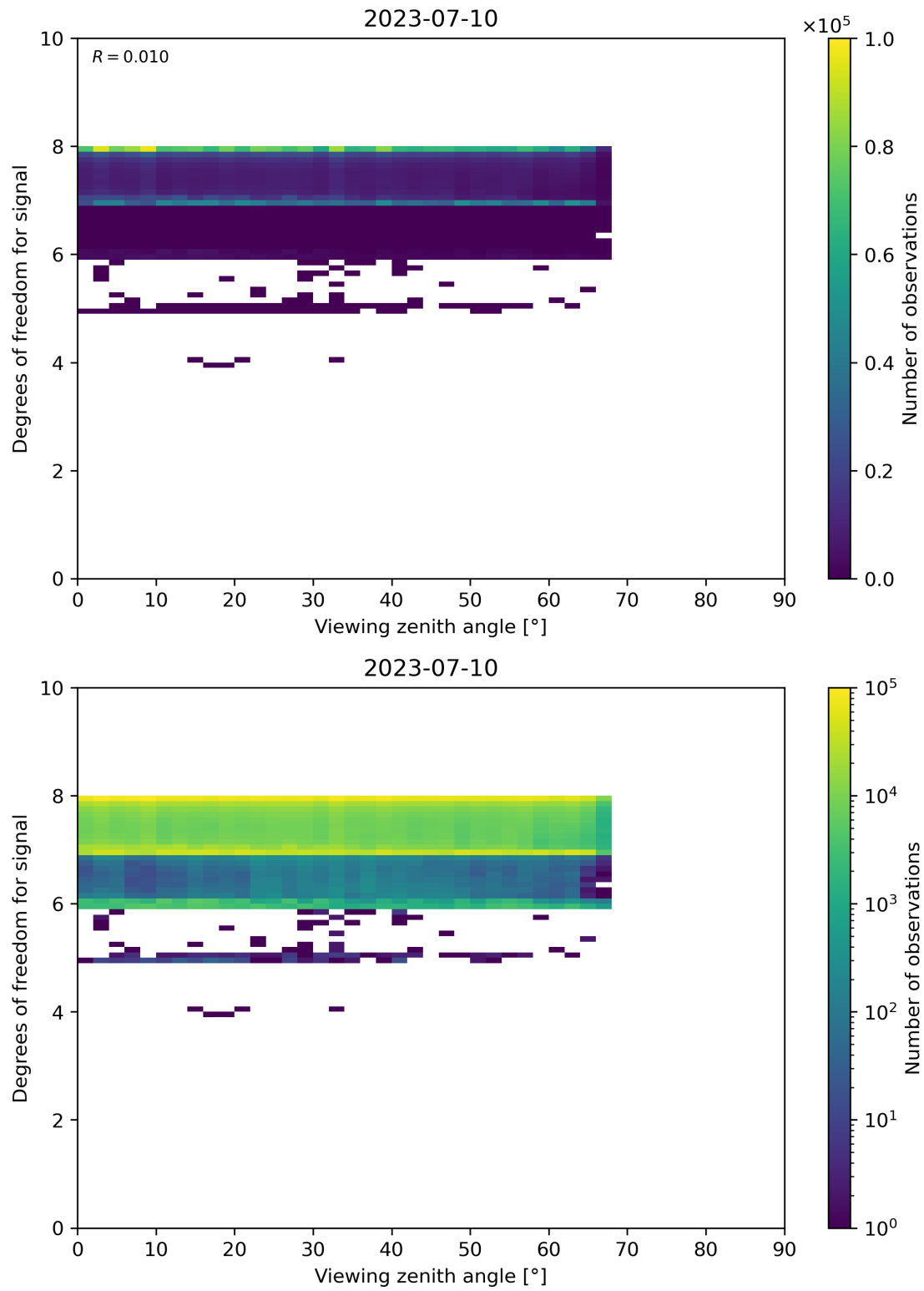
Figure 73: Scatter density plot of “Viewing zenith angle” against “Degrees of freedom for signal” for 2023-07-09 to 2023-07-11.
