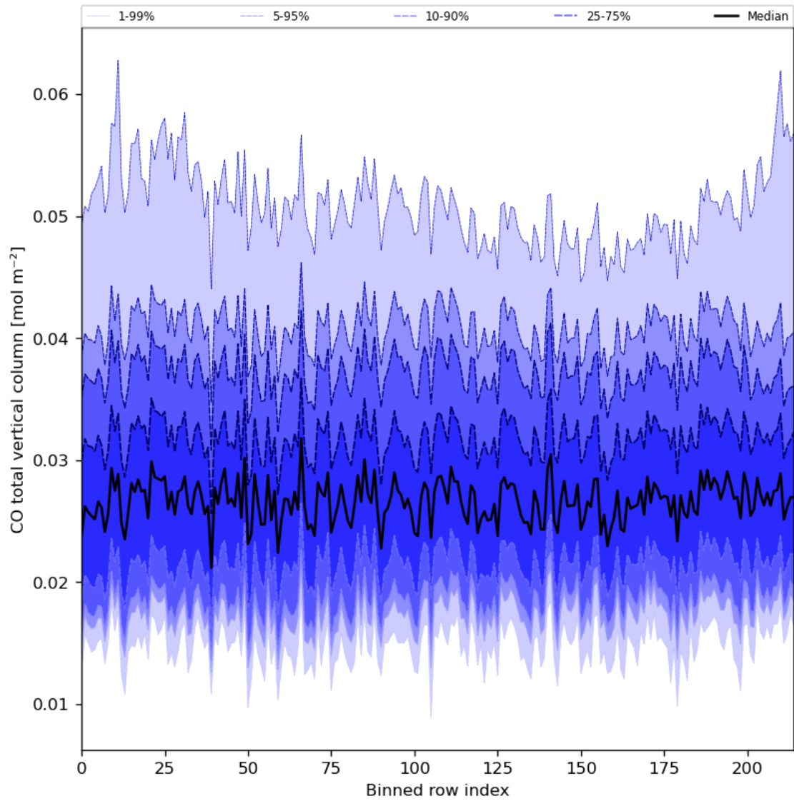
Figure 26: Along track statistics of “CO total vertical column” for 2023-07-09 to 2023-07-11
