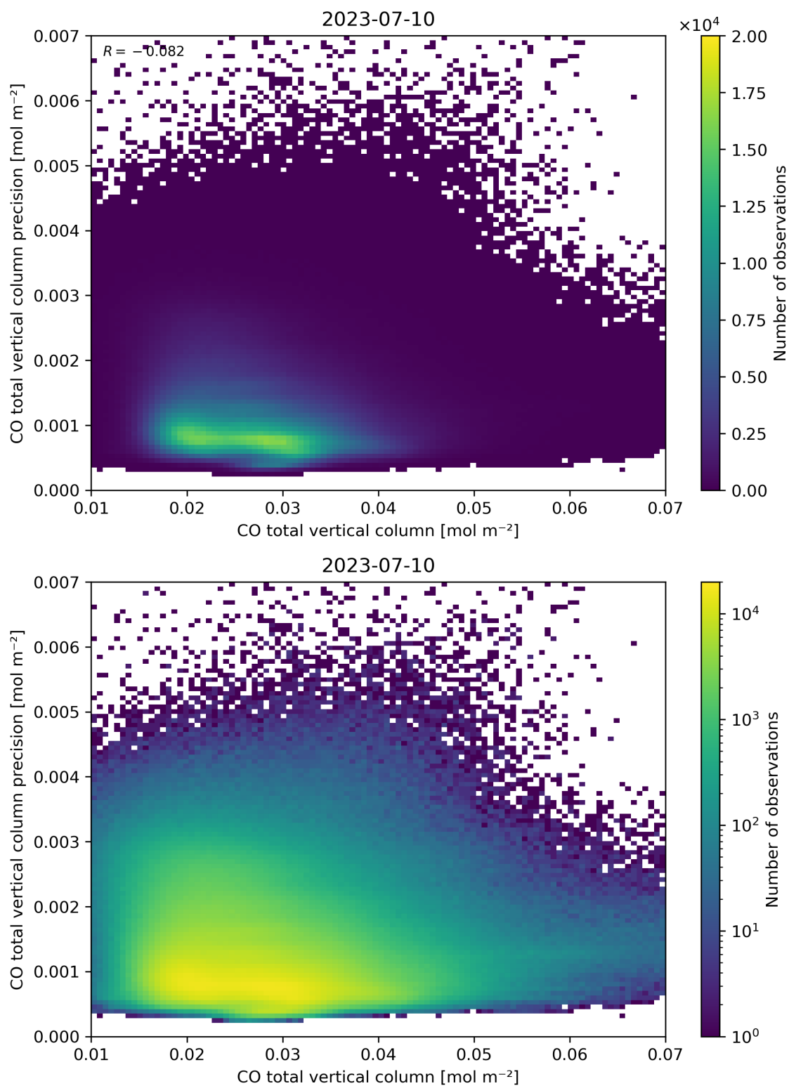
Figure 34: Scatter density plot of “CO total vertical column” against “CO total vertical column precision” for 2023-07-09 to 2023-07-11.
