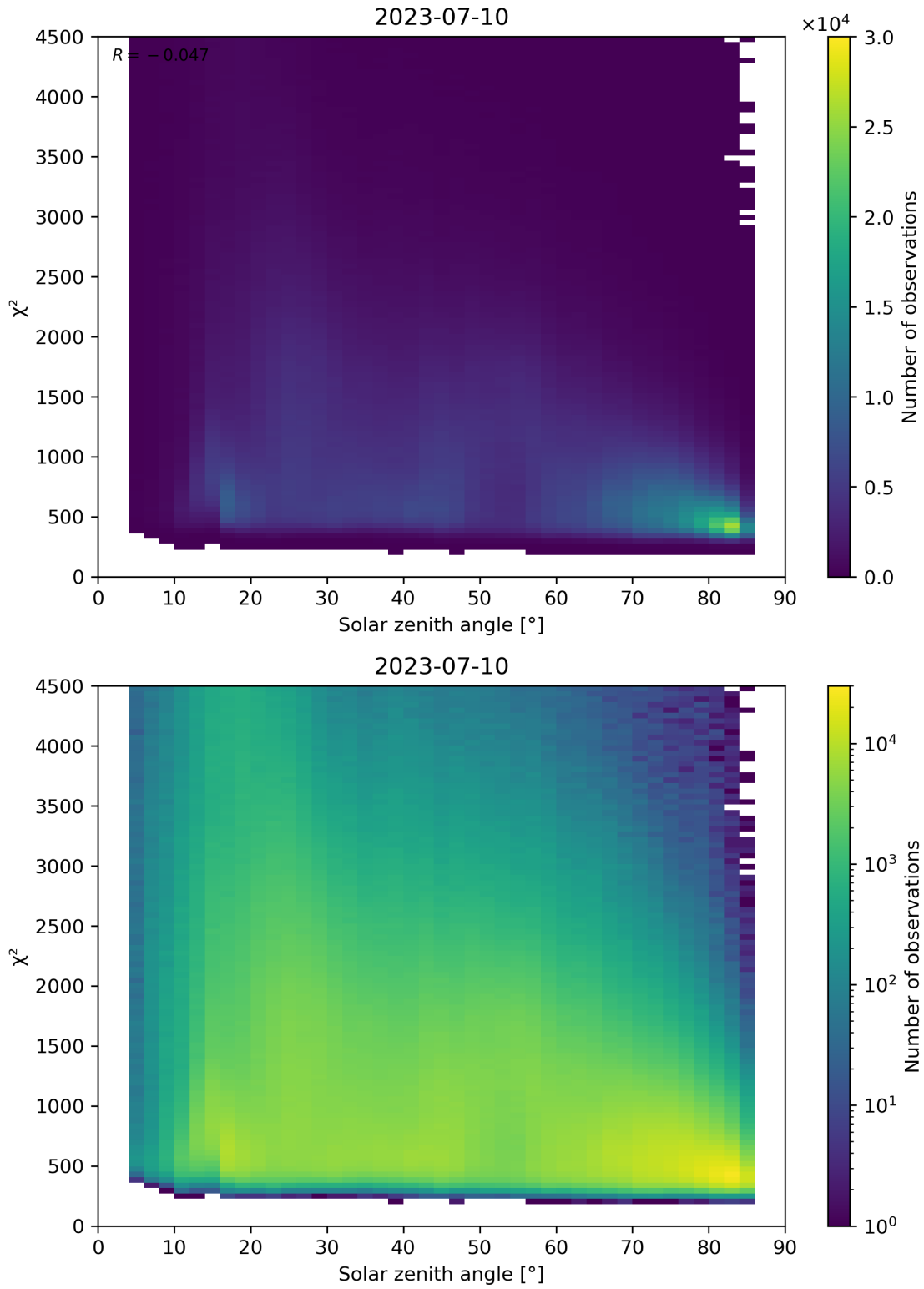
Figure 64: Scatter density plot of “Solar zenith angle” against “ \chi^2 ” for 2023-07-09 to 2023-07-11.
