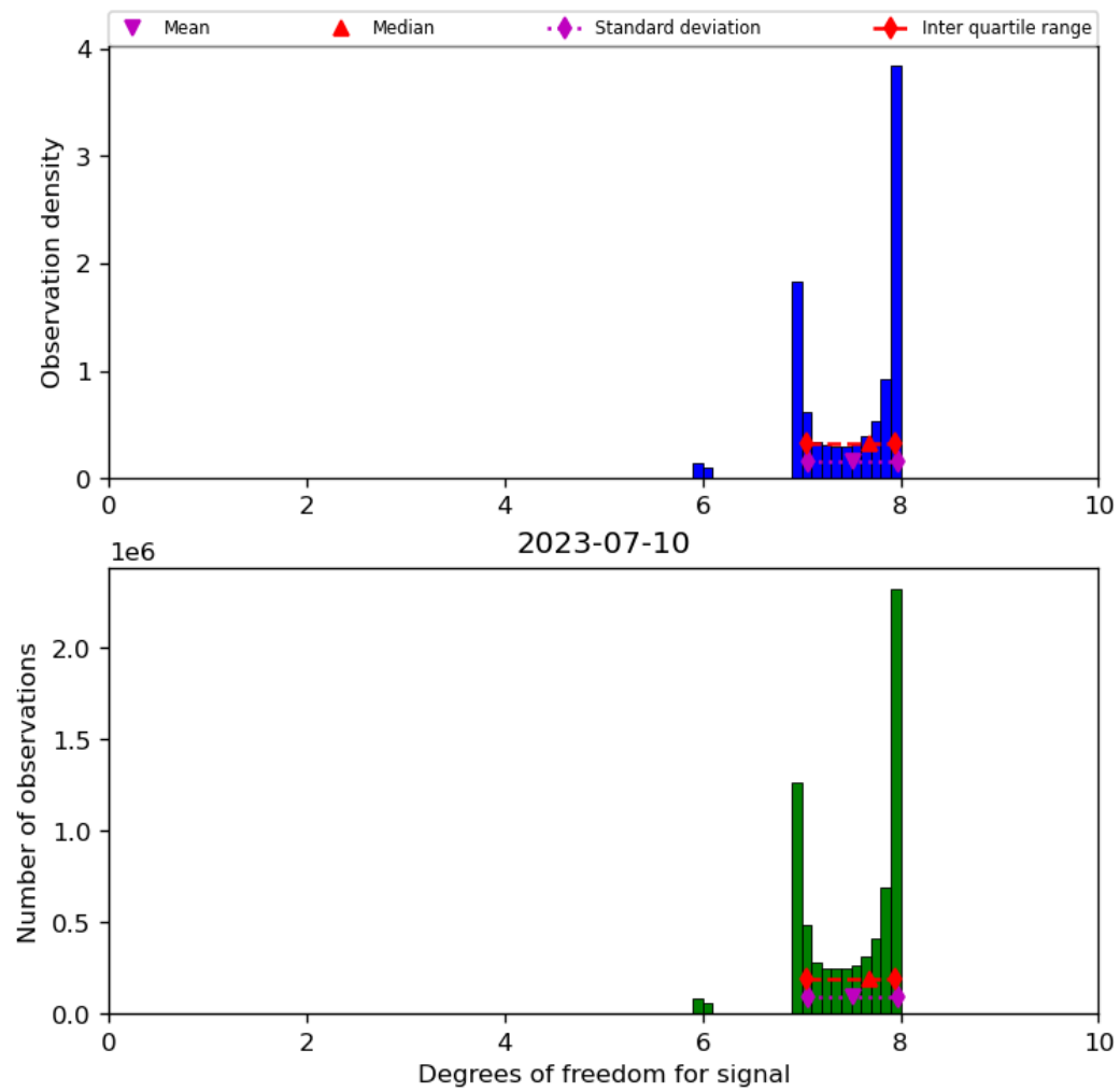
Figure 23: Histogram of “Degrees of freedom for signal” for 2023-07-09 to 2023-07-11
