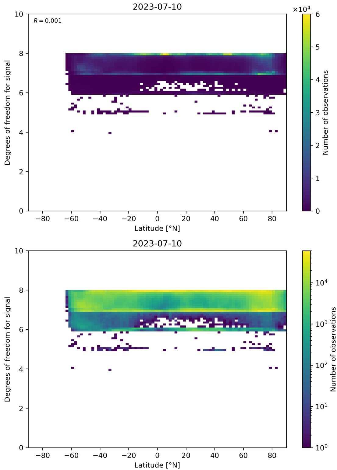
Figure 55: Scatter density plot of “Latitude” against “Degrees of freedom for signal” for 2023-07-09 to 2023-07-11.
