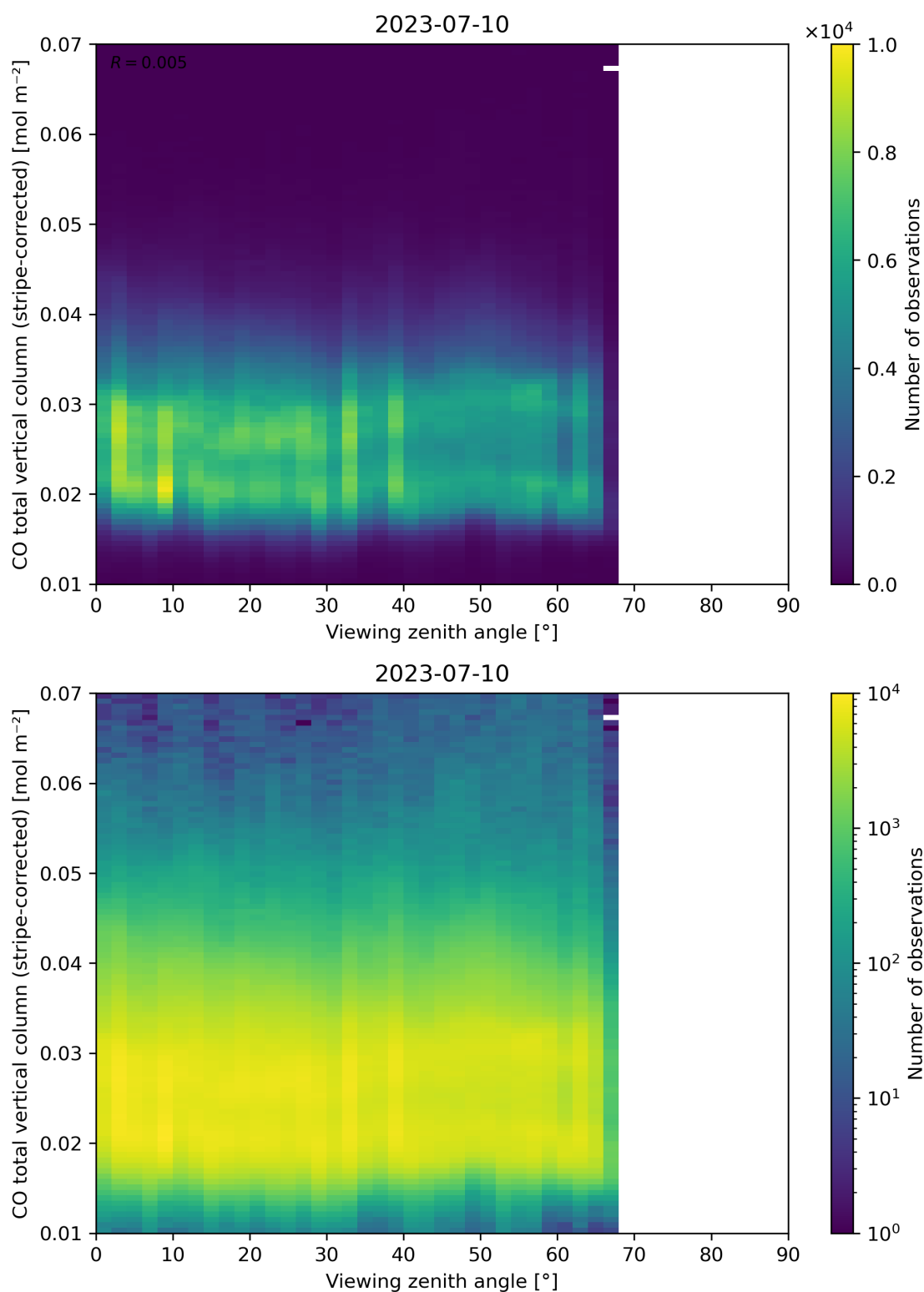
Figure 70: Scatter density plot of “Viewing zenith angle” against “CO total vertical column (stripe-corrected)” for 2023-07-09 to 2023-07-11.
