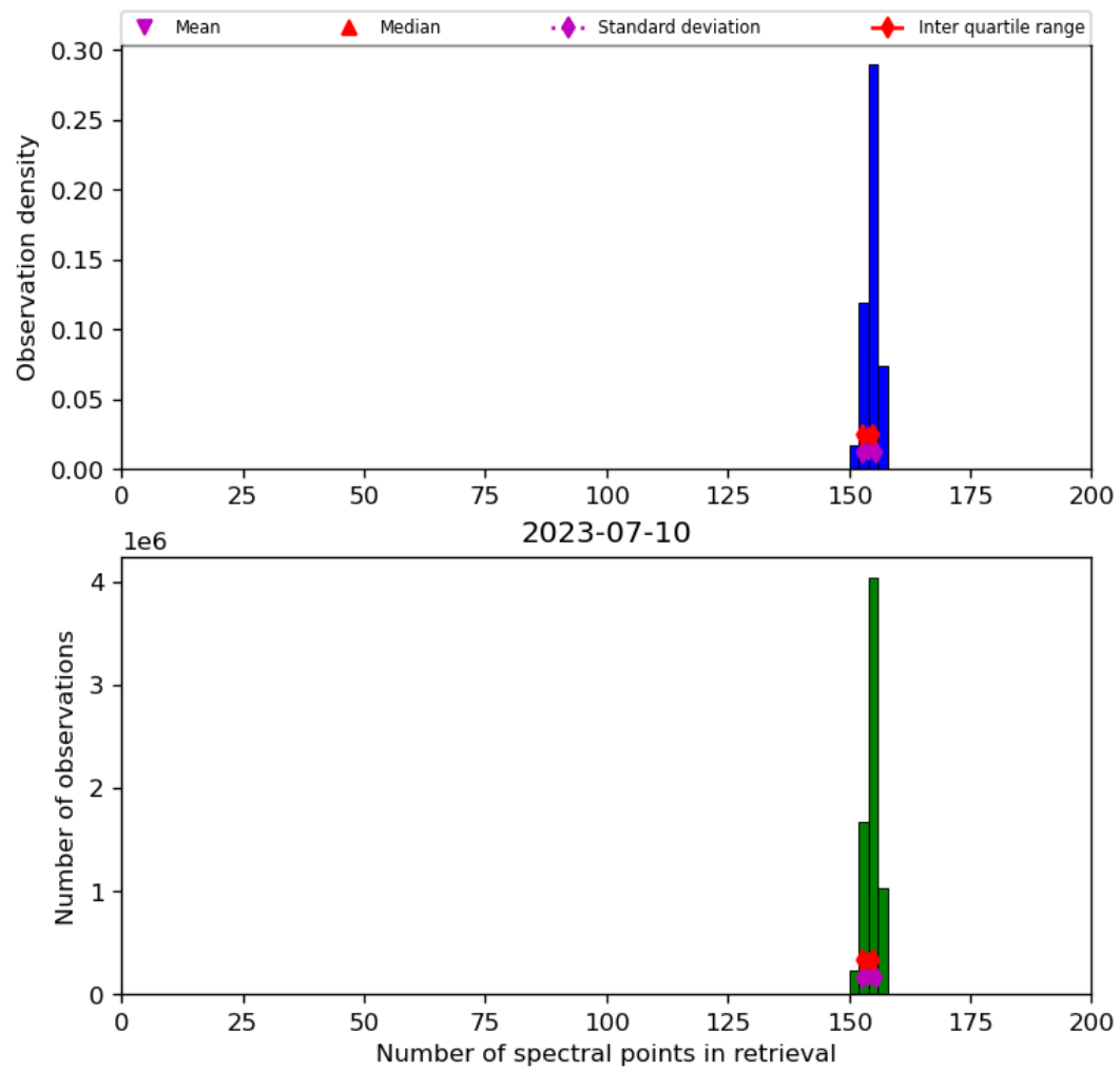
Figure 21: Histogram of “Number of spectral points in retrieval” for 2023-07-09 to 2023-07-11
