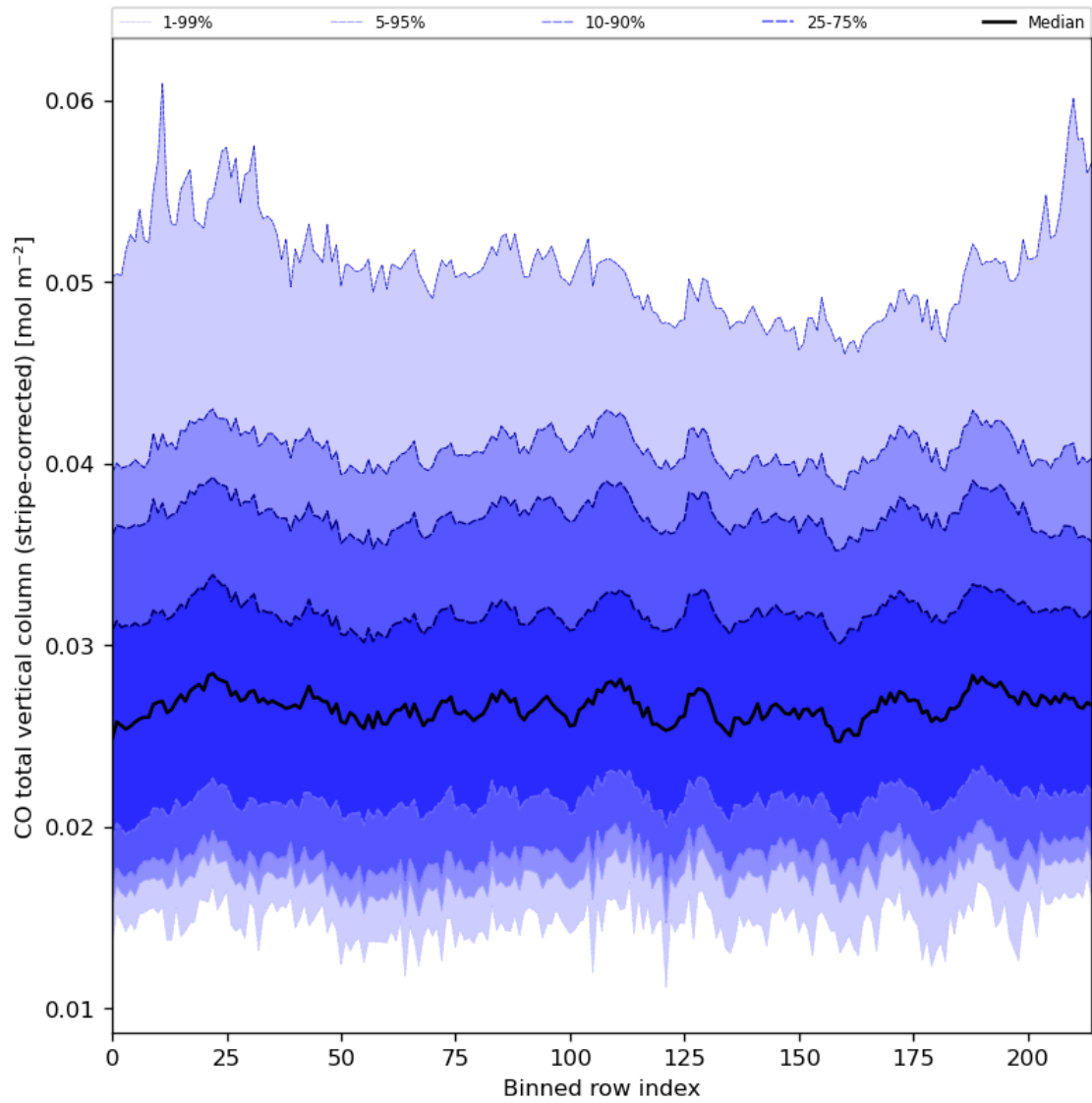
Figure 27: Along track statistics of “CO total vertical column (stripe-corrected)” for 2023-07-09 to 2023-07-11
