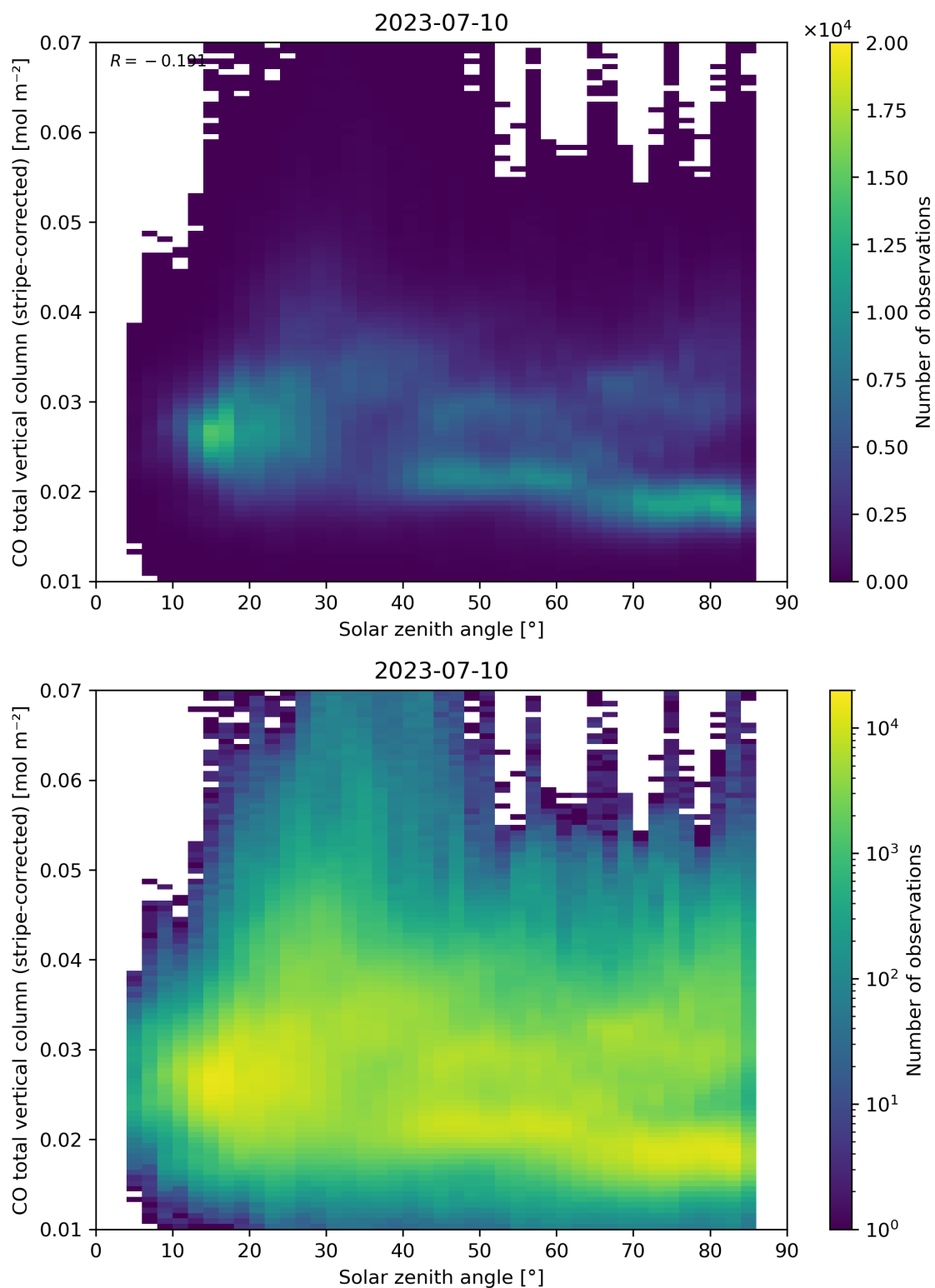
Figure 62: Scatter density plot of “Solar zenith angle” against “CO total vertical column (stripe-corrected)” for 2023-07-09 to 2023-07-11.
