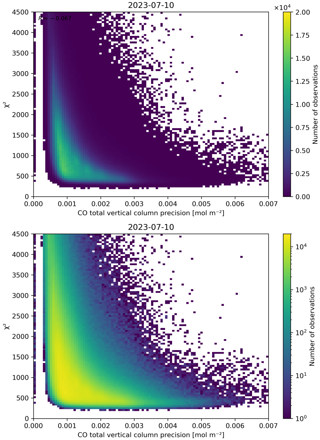
Figure 44: Scatter density plot of “CO total vertical column precision” against “ \chi^2 ” for 2023-07-09 to 2023-07-11.
