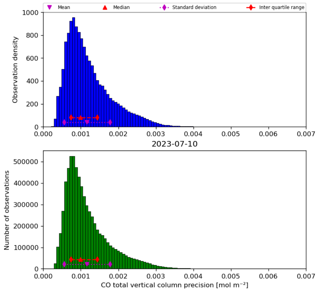
Figure 20: Histogram of “CO total vertical column precision” for 2023-07-09 to 2023-07-11
