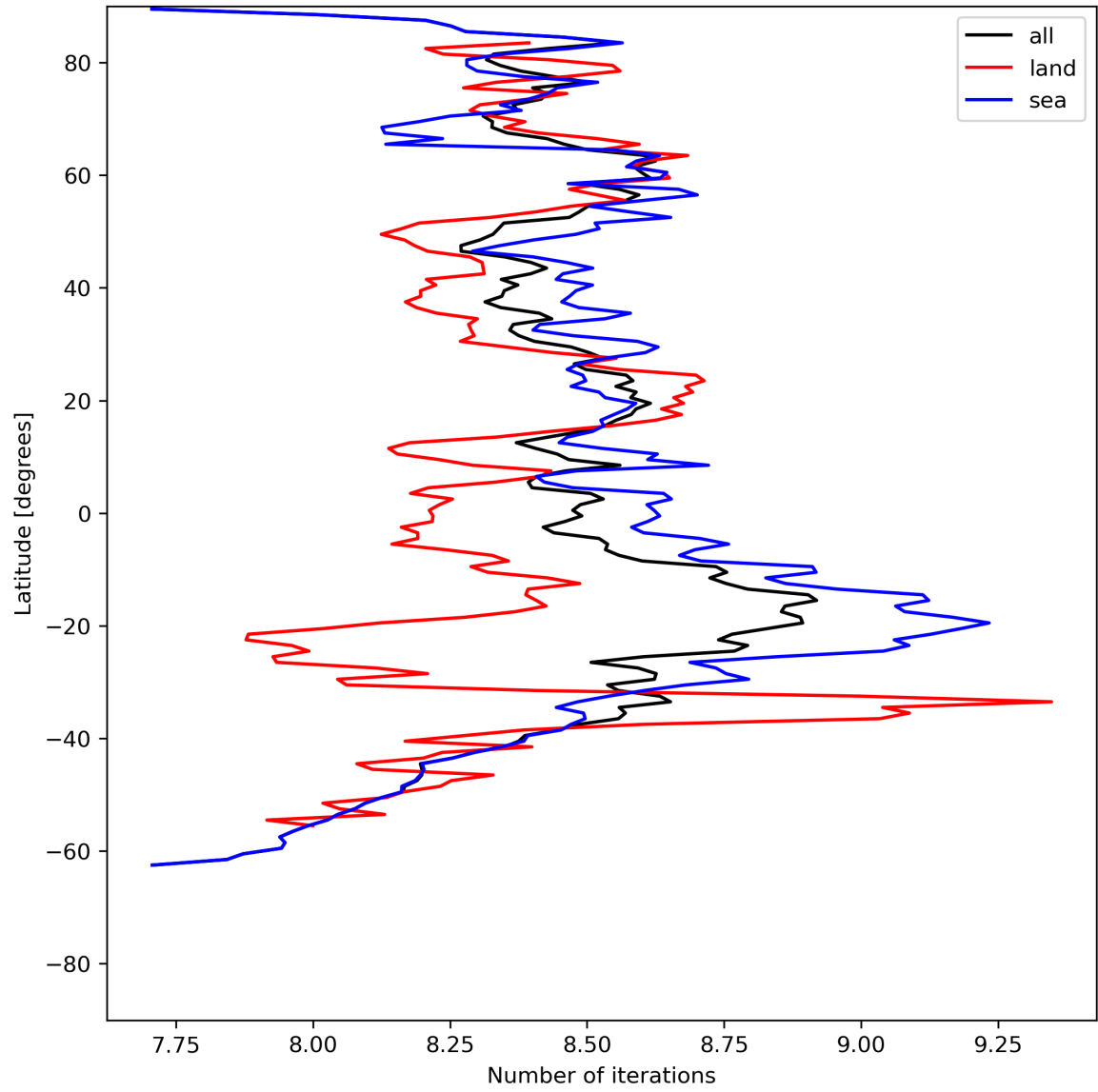
Figure 16: Zonal average of “Number of iterations” for 2023-07-09 to 2023-07-11.
