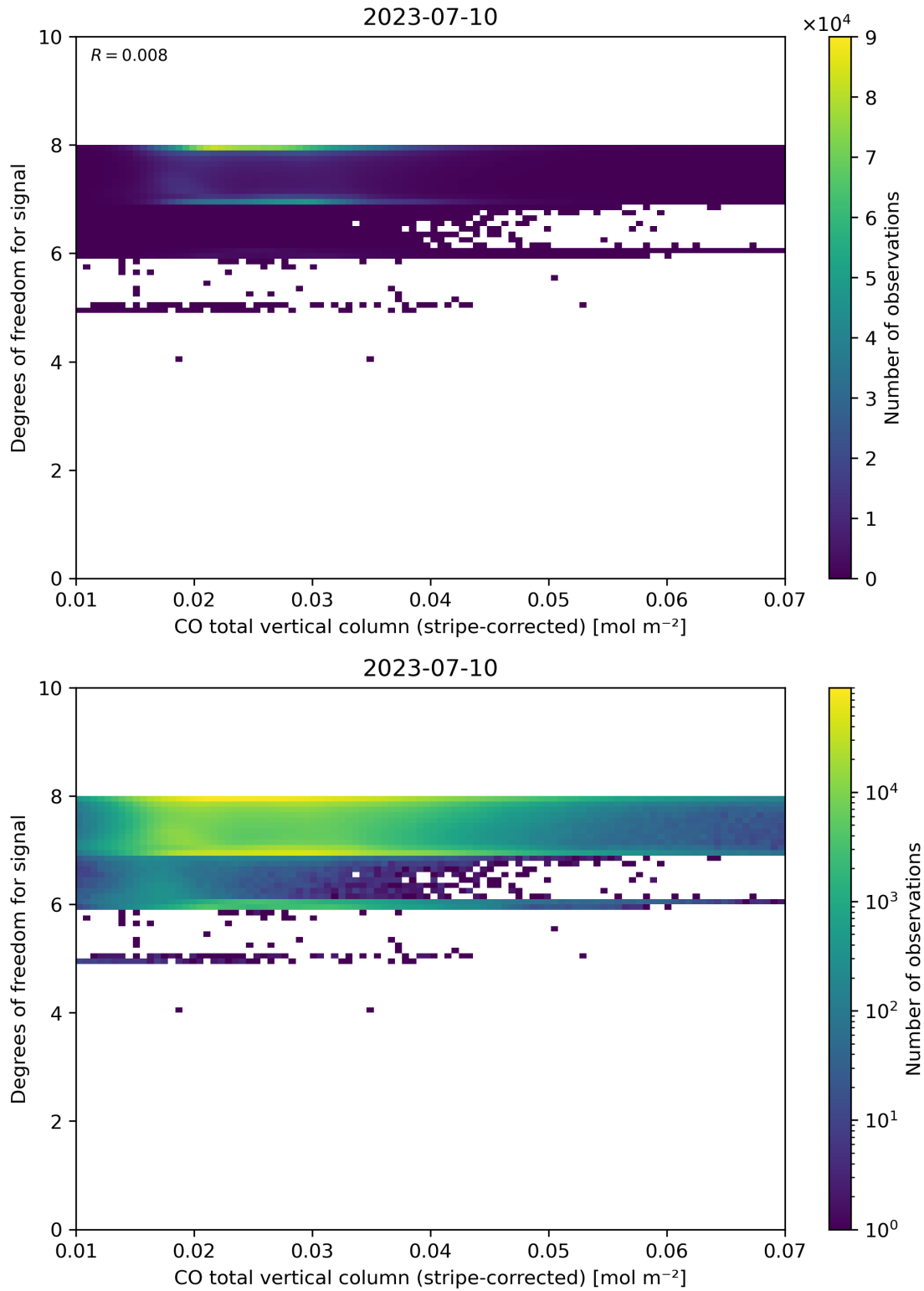
Figure 38: Scatter density plot of “CO total vertical column (stripe-corrected)” against “Degrees of freedom for signal” for 2023-07-09 to 2023-07-11.
