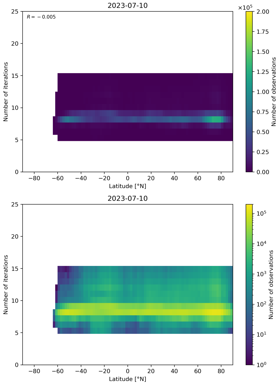
Figure 56: Scatter density plot of “Latitude” against “Number of iterations” for 2023-07-09 to 2023-07-11.
