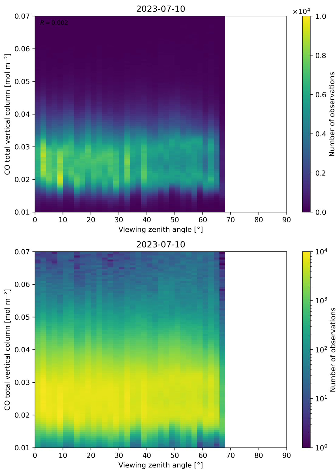
Figure 69: Scatter density plot of “Viewing zenith angle” against “CO total vertical column” for 2023-07-09 to 2023-07-11.
