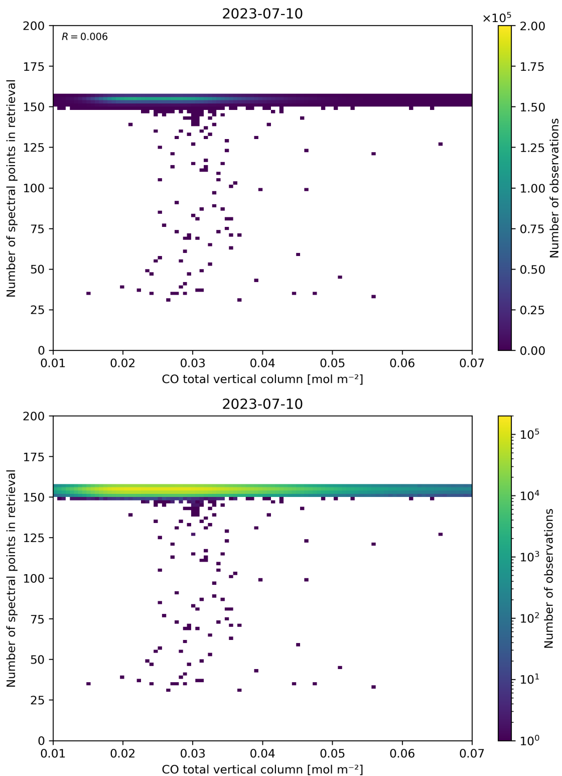
Figure 43: Scatter density plot of “CO total vertical column” against “Number of spectral points in retrieval” for 2023-07-09 to 2023-07-11.
