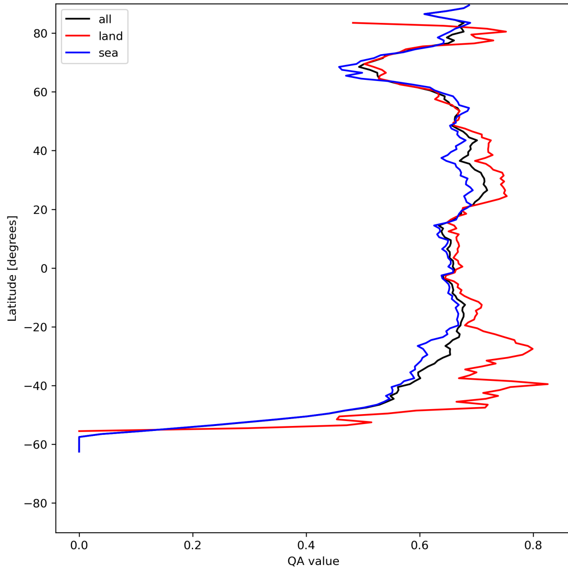
Figure 9: Zonal average of “QA value” for 2023-07-09 to 2023-07-11.
