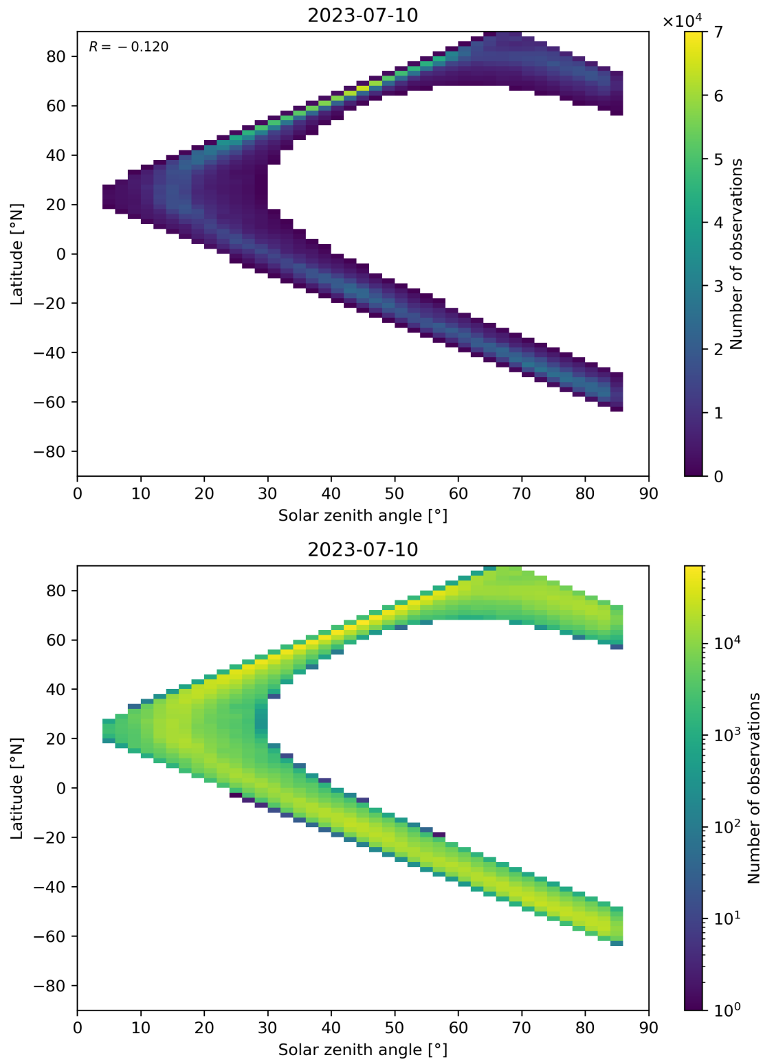
Figure 66: Scatter density plot of “Solar zenith angle” against “Latitude” for 2023-07-09 to 2023-07-11.
