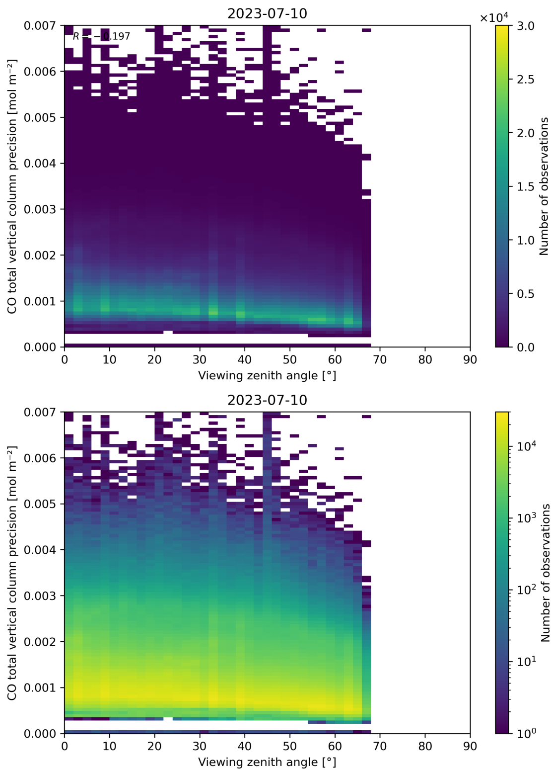
Figure 71: Scatter density plot of “Viewing zenith angle” against “CO total vertical column precision” for 2023-07-09 to 2023-07-11.
