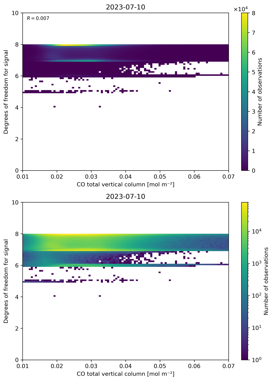
Figure 41: Scatter density plot of “CO total vertical column” against “Degrees of freedom for signal” for 2023-07-09 to 2023-07-11.
