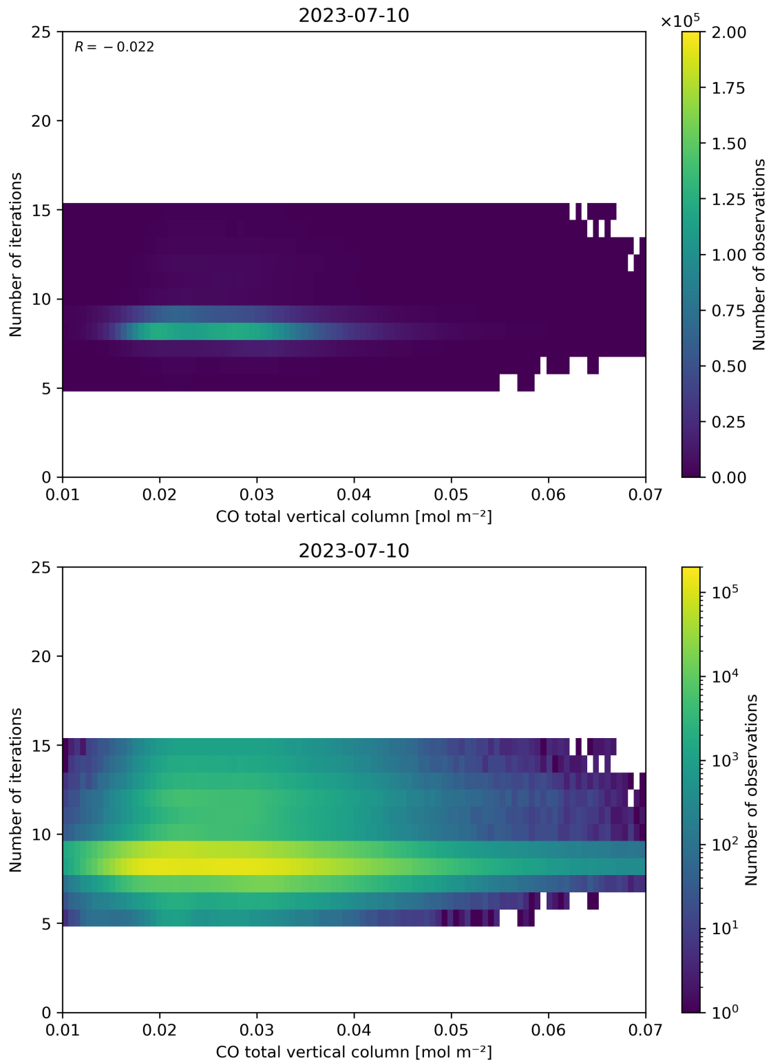
Figure 42: Scatter density plot of “CO total vertical column” against “Number of iterations” for 2023-07-09 to 2023-07-11.
