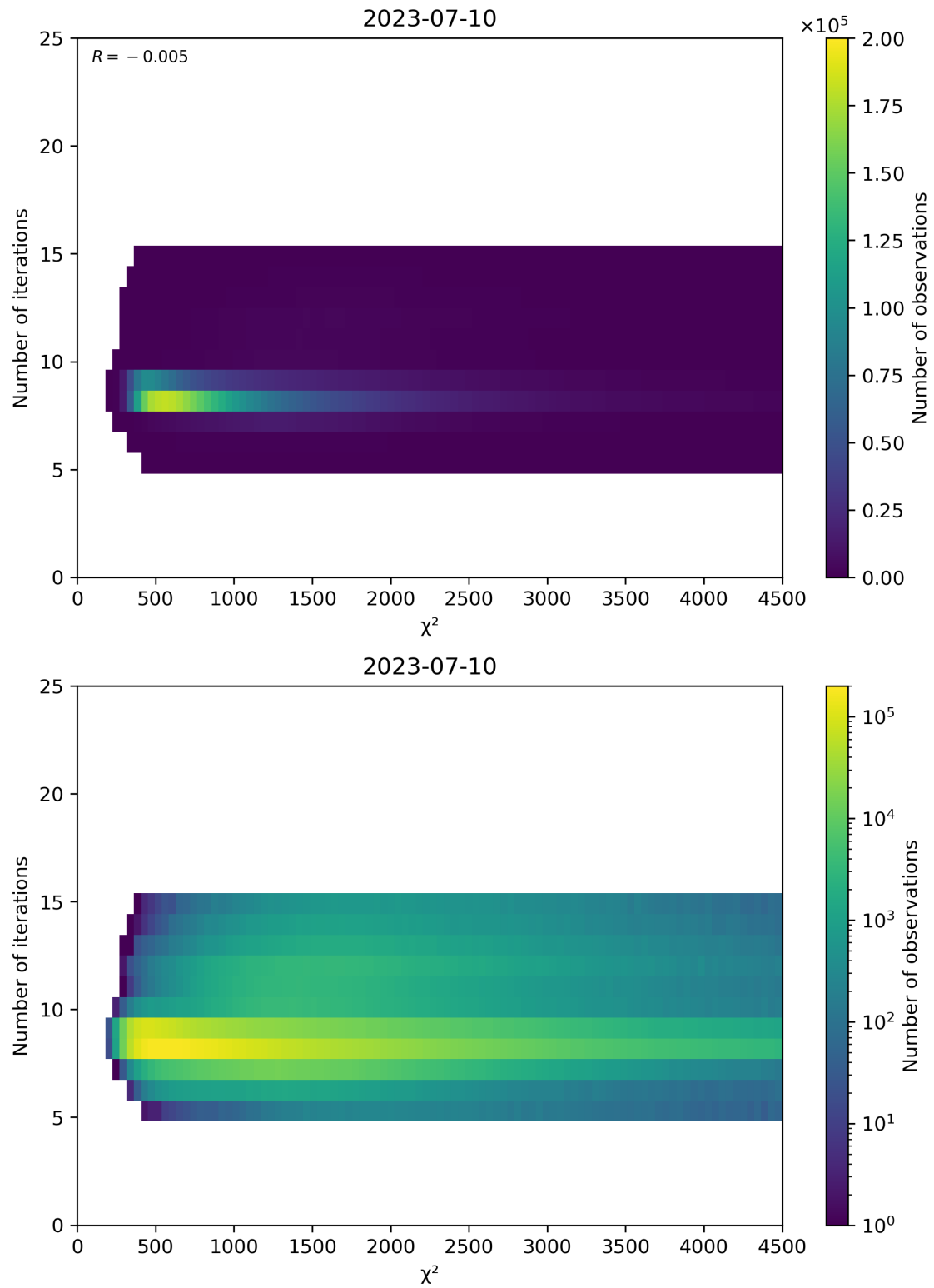
Figure 49: Scatter density plot of “ \chi^2 ” against “Number of iterations” for 2023-07-09 to 2023-07-11.
