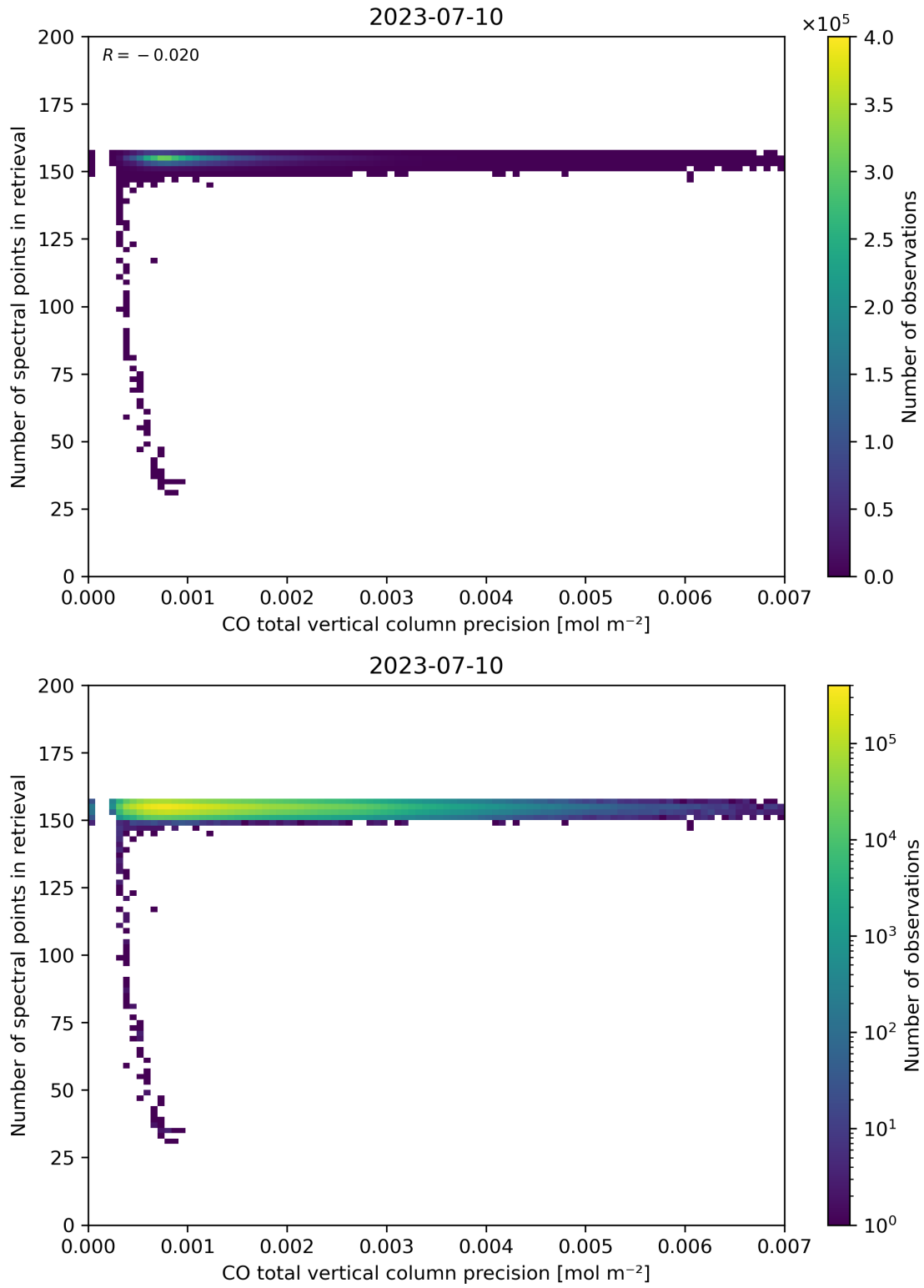
Figure 47: Scatter density plot of “CO total vertical column precision” against “Number of spectral points in retrieval” for 2023-07-09 to 2023-07-11.
