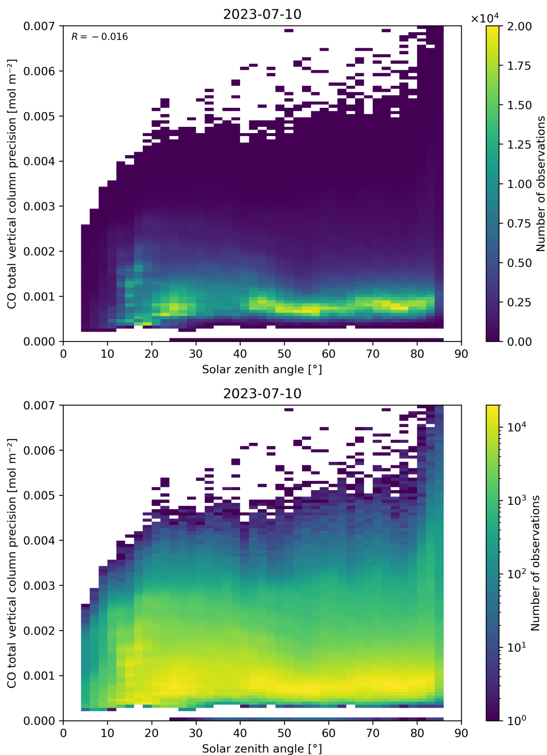
Figure 63: Scatter density plot of “Solar zenith angle” against “CO total vertical column precision” for 2023-07-09 to 2023-07-11.
