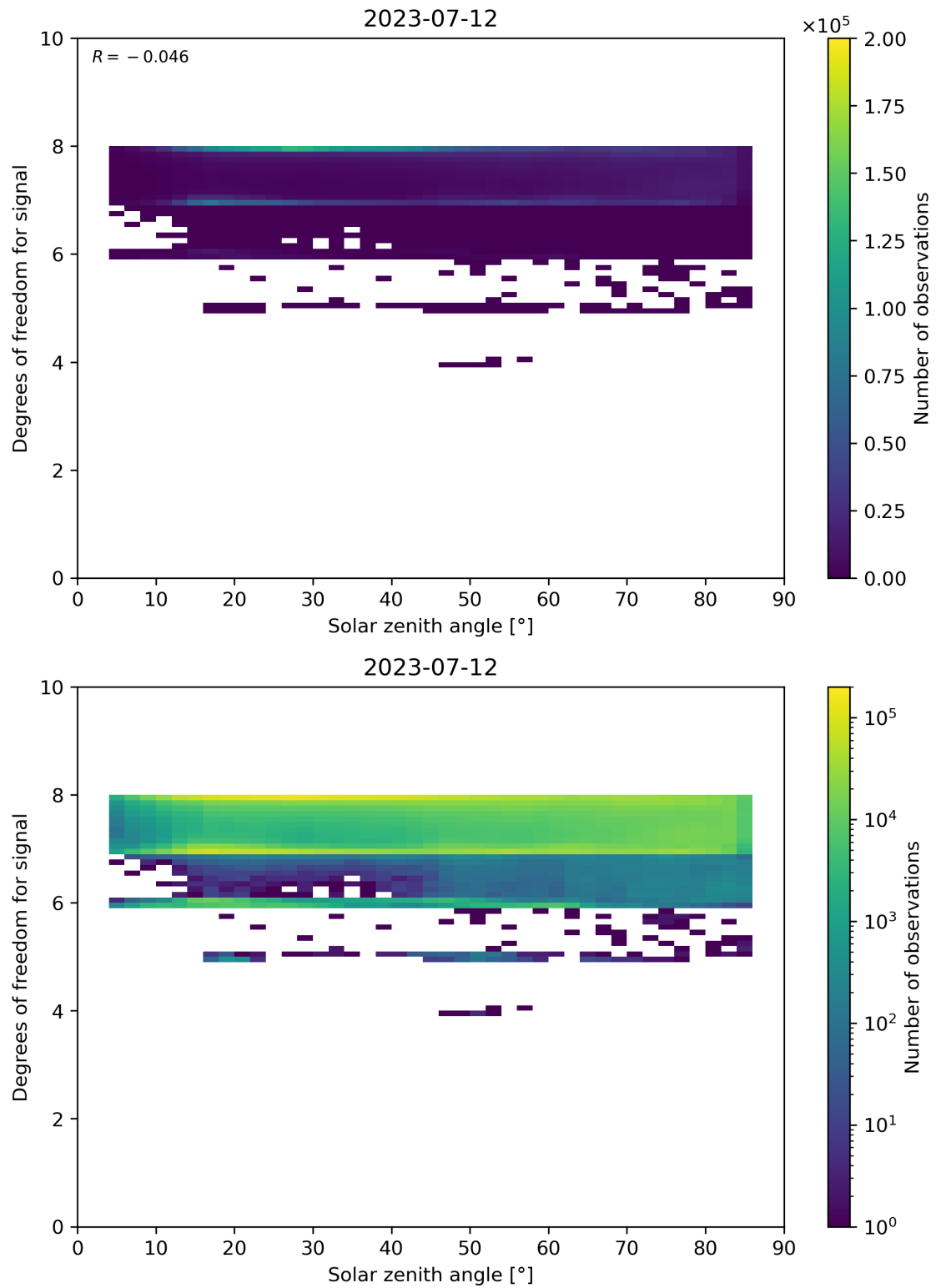
Figure 65: Scatter density plot of “Solar zenith angle” against “Degrees of freedom for signal” for 2023-07-11 to 2023-07-13.
