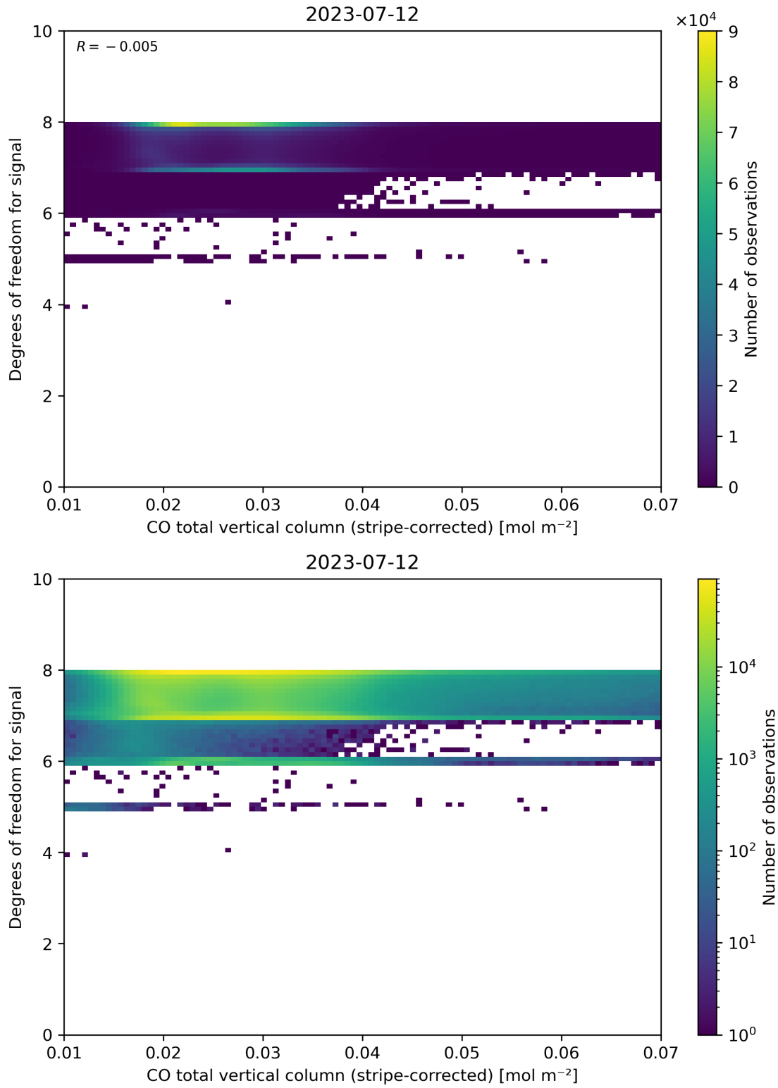
Figure 38: Scatter density plot of “CO total vertical column (stripe-corrected)” against “Degrees of freedom for signal” for 2023-07-11 to 2023-07-13.
