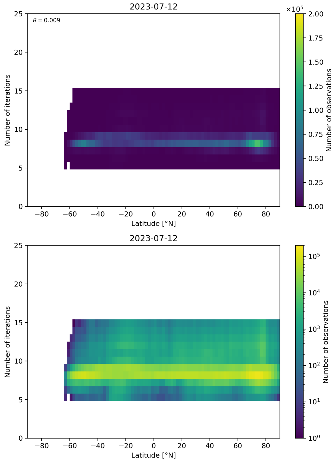
Figure 56: Scatter density plot of “Latitude” against “Number of iterations” for 2023-07-11 to 2023-07-13.
