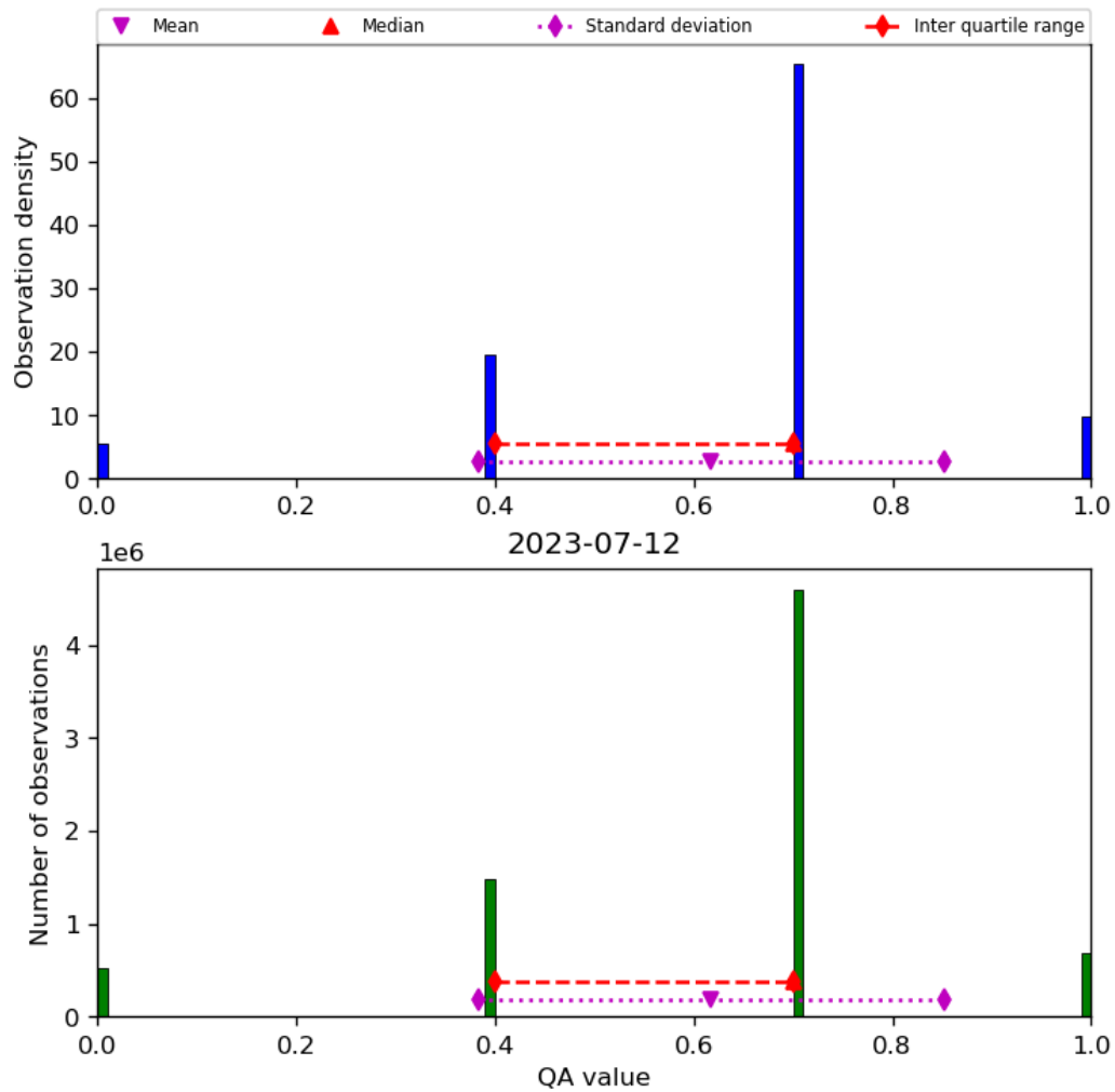
Figure 17: Histogram of “QA value” for 2023-07-11 to 2023-07-13
