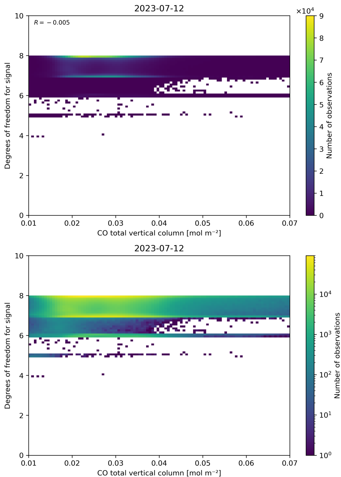
Figure 41: Scatter density plot of “CO total vertical column” against “Degrees of freedom for signal” for 2023-07-11 to 2023-07-13.
