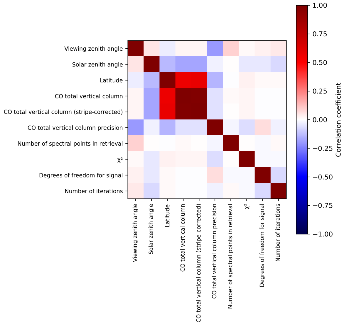
Figure 2: Map of correlation matrix for 2023-07-11 to 2023-07-13.
