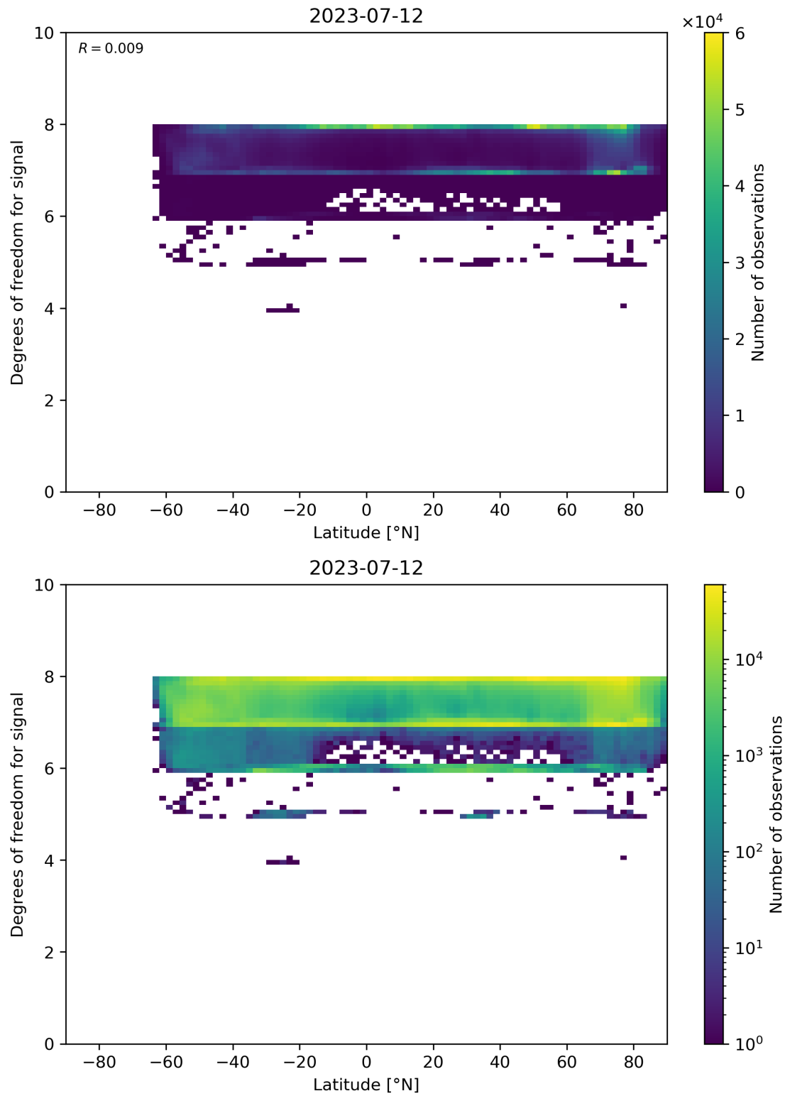
Figure 55: Scatter density plot of “Latitude” against “Degrees of freedom for signal” for 2023-07-11 to 2023-07-13.
