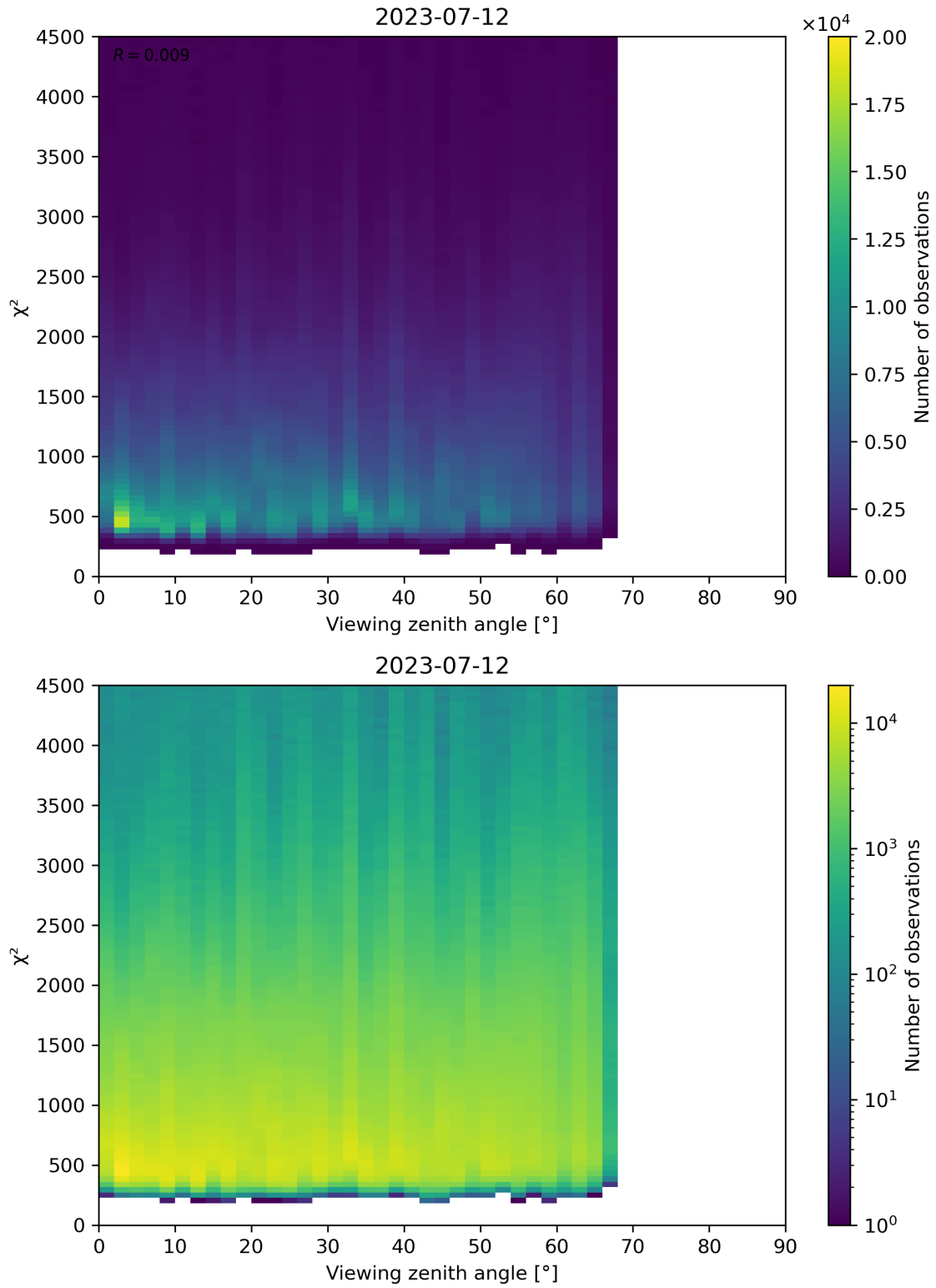
Figure 72: Scatter density plot of “Viewing zenith angle” against “ \chi^2 ” for 2023-07-11 to 2023-07-13.
