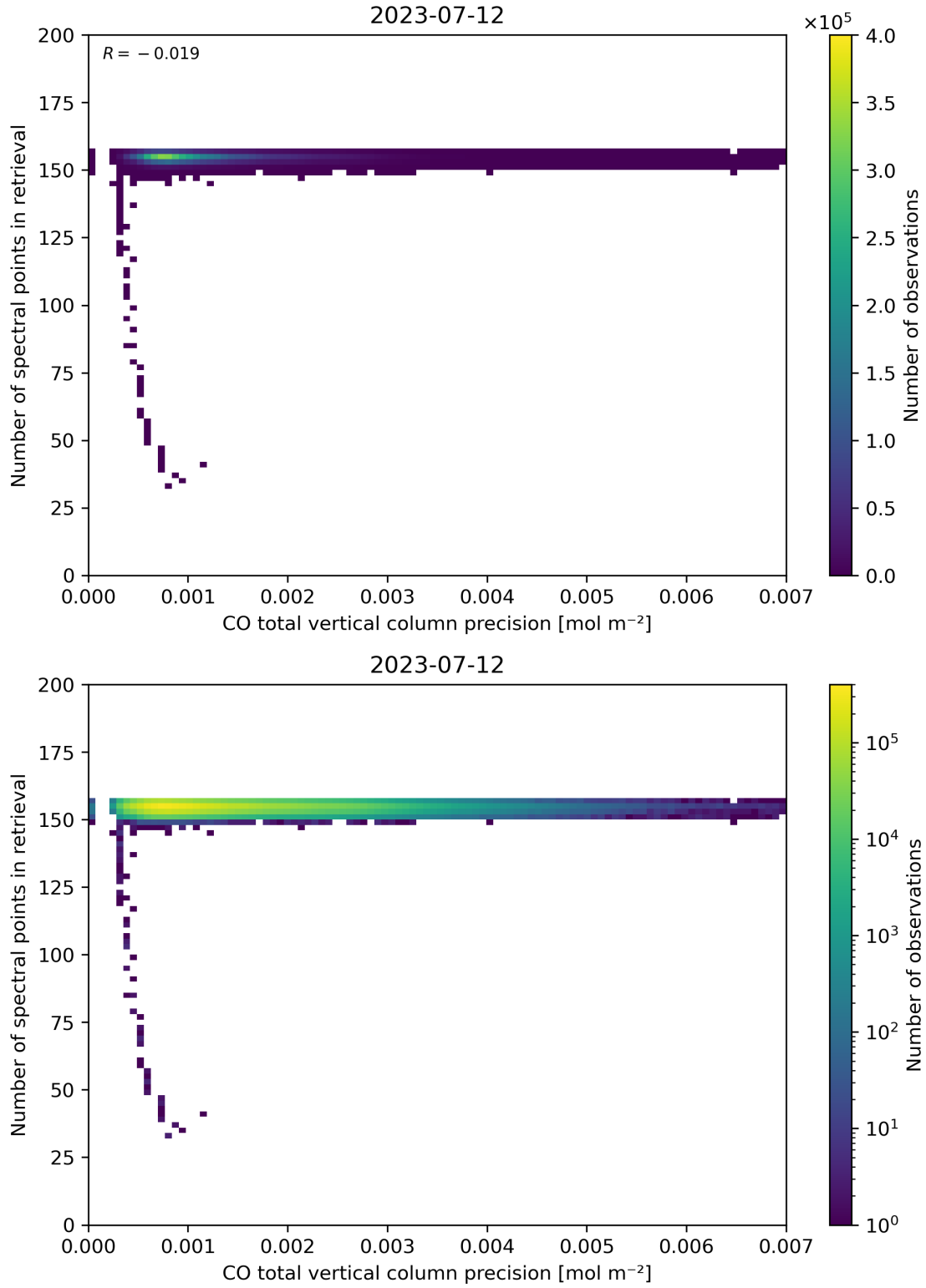
Figure 47: Scatter density plot of “CO total vertical column precision” against “Number of spectral points in retrieval” for 2023-07-11 to 2023-07-13.
