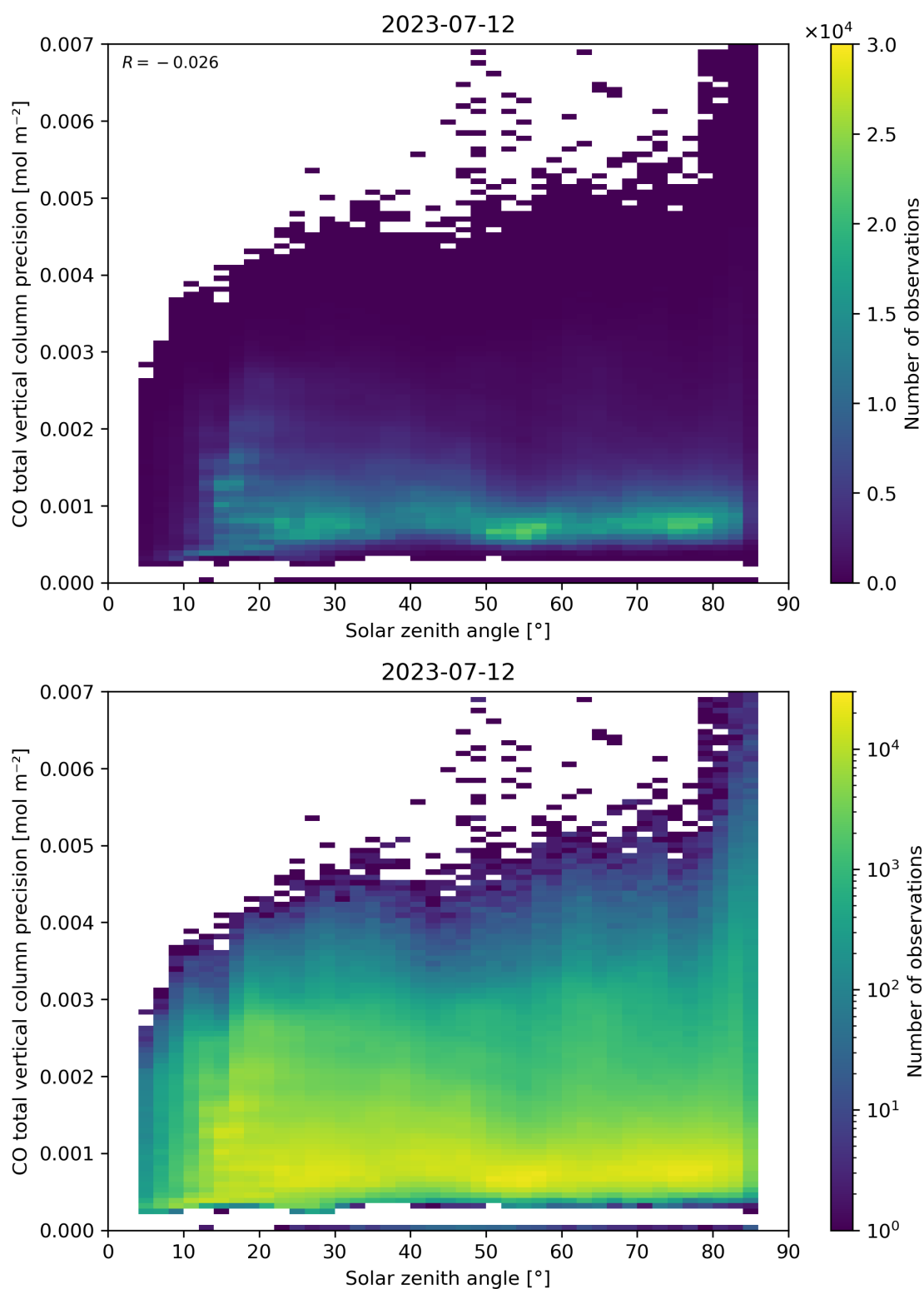
Figure 63: Scatter density plot of “Solar zenith angle” against “CO total vertical column precision” for 2023-07-11 to 2023-07-13.
