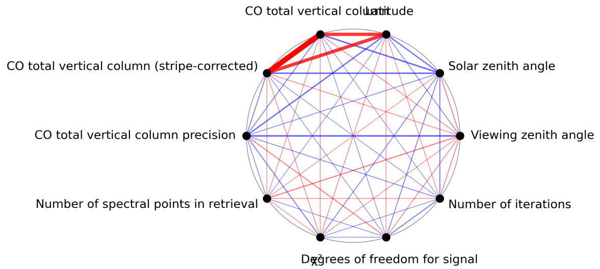
Figure 1: Map of correlation graph for 2023-07-11 to 2023-07-13.
