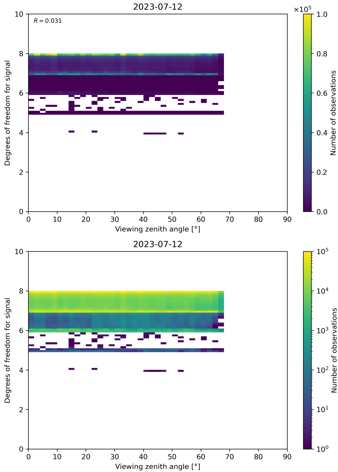
Figure 73: Scatter density plot of “Viewing zenith angle” against “Degrees of freedom for signal” for 2023-07-11 to 2023-07-13.
