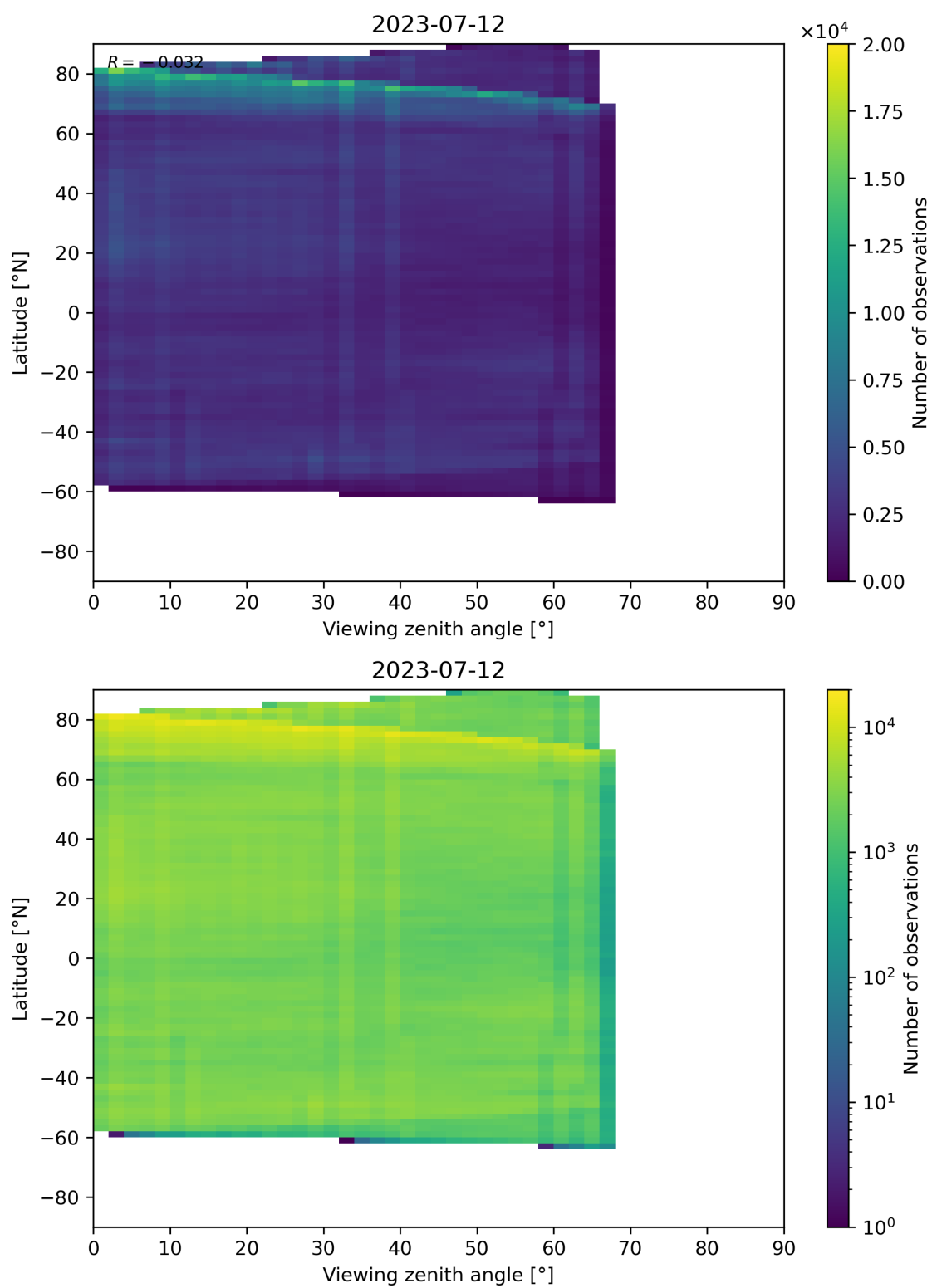
Figure 74: Scatter density plot of “Viewing zenith angle” against “Latitude” for 2023-07-11 to 2023-07-13.
