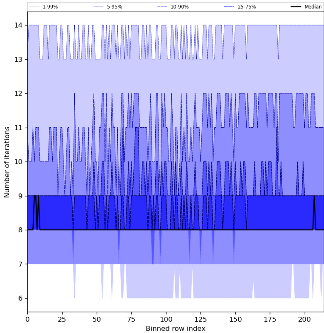
Figure 32: Along track statistics of “Number of iterations” for 2023-07-11 to 2023-07-13
