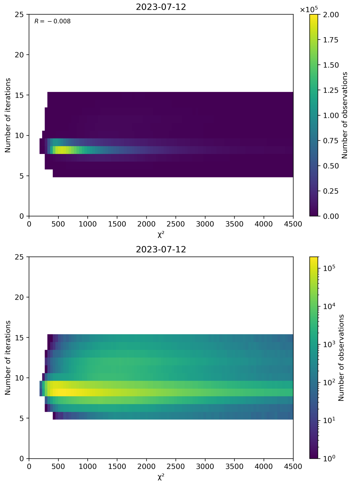
Figure 49: Scatter density plot of “ \chi^2 ” against “Number of iterations” for 2023-07-11 to 2023-07-13.
