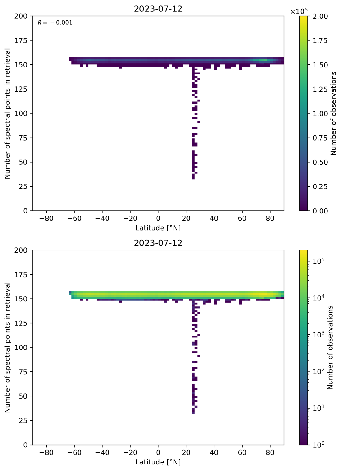
Figure 57: Scatter density plot of “Latitude” against “Number of spectral points in retrieval” for 2023-07-11 to 2023-07-13.
