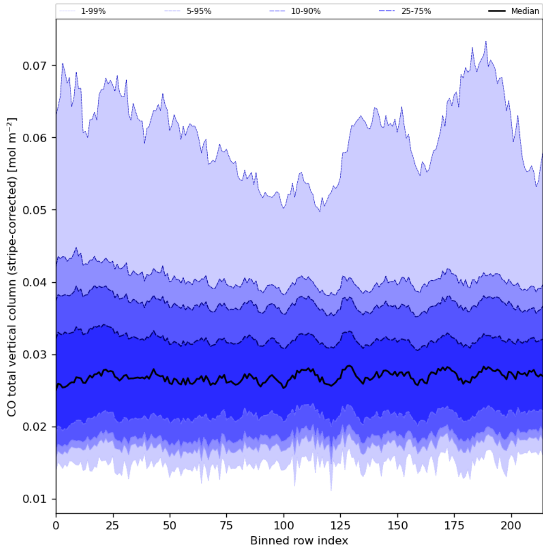
Figure 27: Along track statistics of “CO total vertical column (stripe-corrected)” for 2023-07-11 to 2023-07-13
