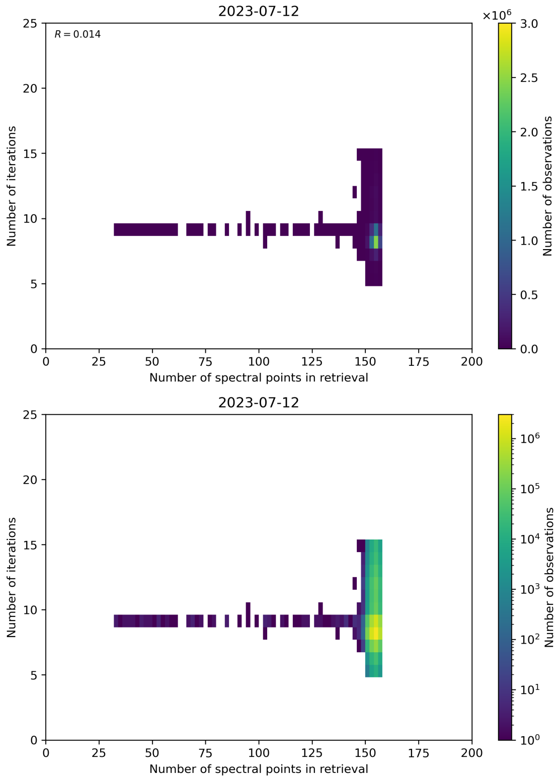
Figure 60: Scatter density plot of “Number of spectral points in retrieval” against “Number of iterations” for 2023-07-11 to 2023-07-13.
