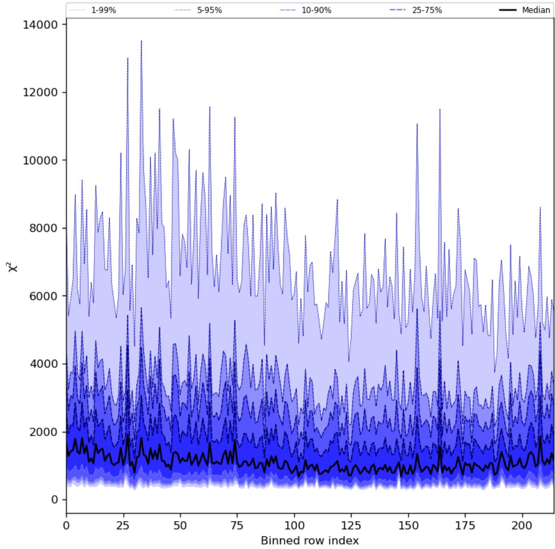
Figure 30: Along track statistics of “ \chi^2 ” for 2023-07-11 to 2023-07-13
