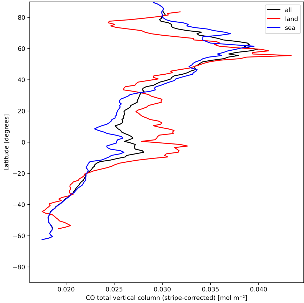
Figure 11: Zonal average of “CO total vertical column (stripe-corrected)” for 2023-07-11 to 2023-07-13.
