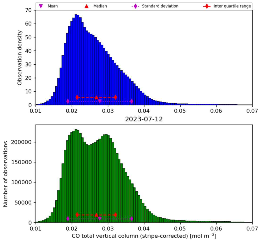
Figure 19: Histogram of “CO total vertical column (stripe-corrected)” for 2023-07-11 to 2023-07-13
