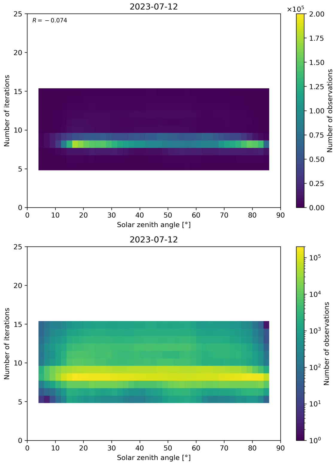
Figure 67: Scatter density plot of “Solar zenith angle” against “Number of iterations” for 2023-07-11 to 2023-07-13.
