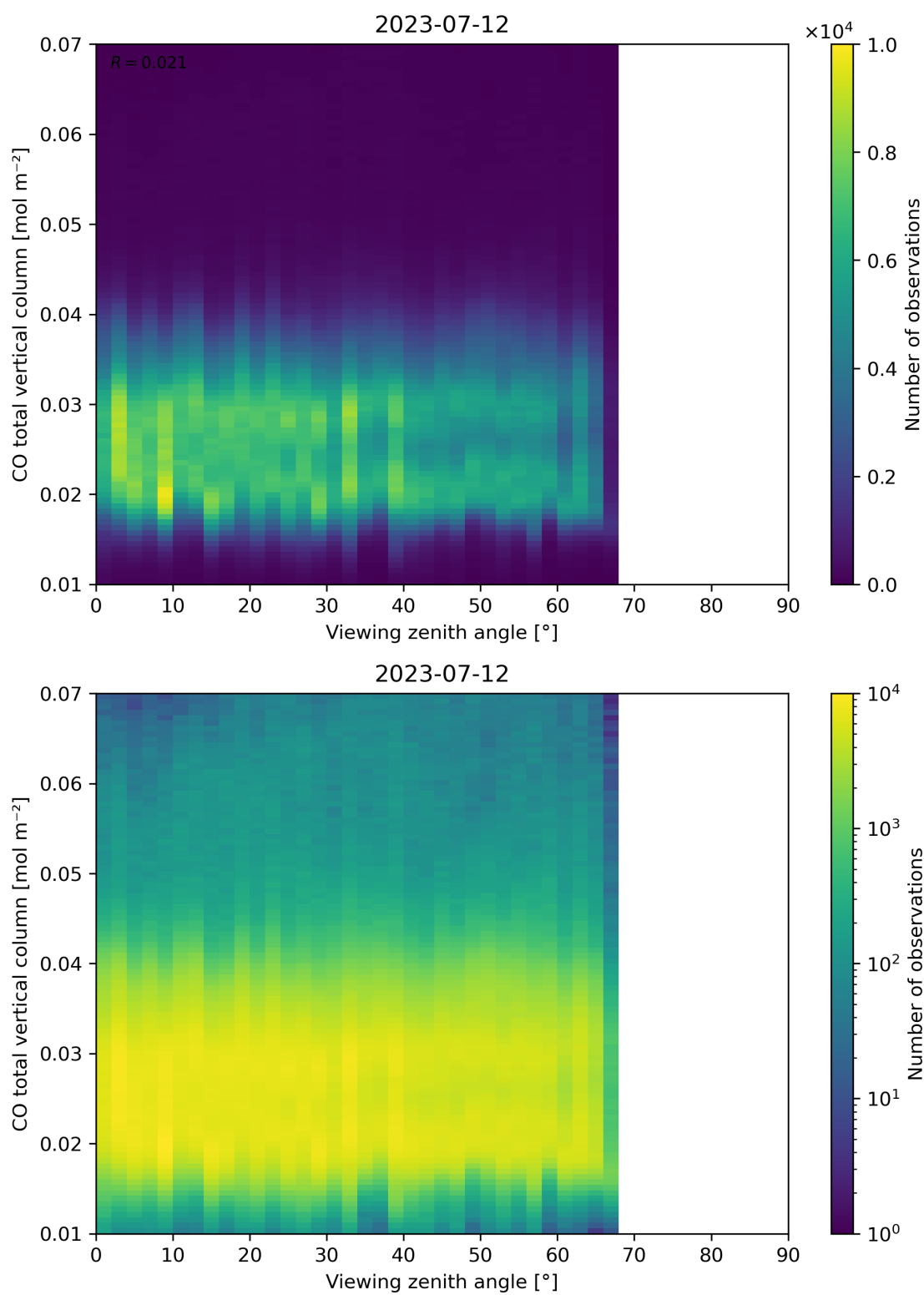
Figure 69: Scatter density plot of “Viewing zenith angle” against “CO total vertical column” for 2023-07-11 to 2023-07-13.
