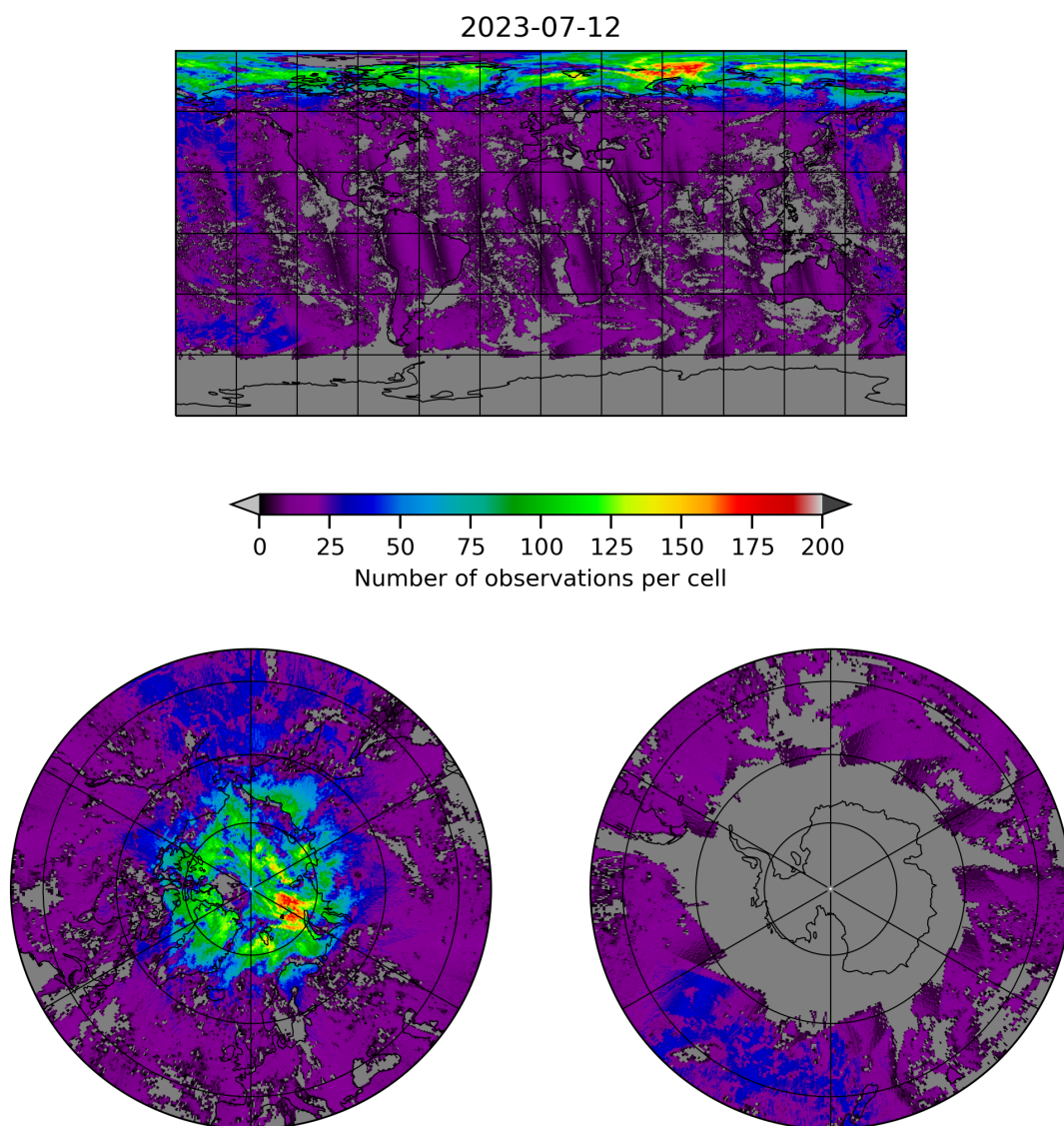
Figure 8: Map of the number of observations for 2023-07-11 to 2023-07-13
