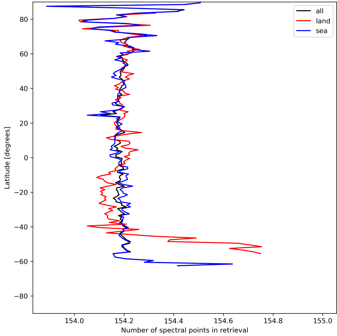
Figure 13: Zonal average of “Number of spectral points in retrieval” for 2023-07-11 to 2023-07-13.
