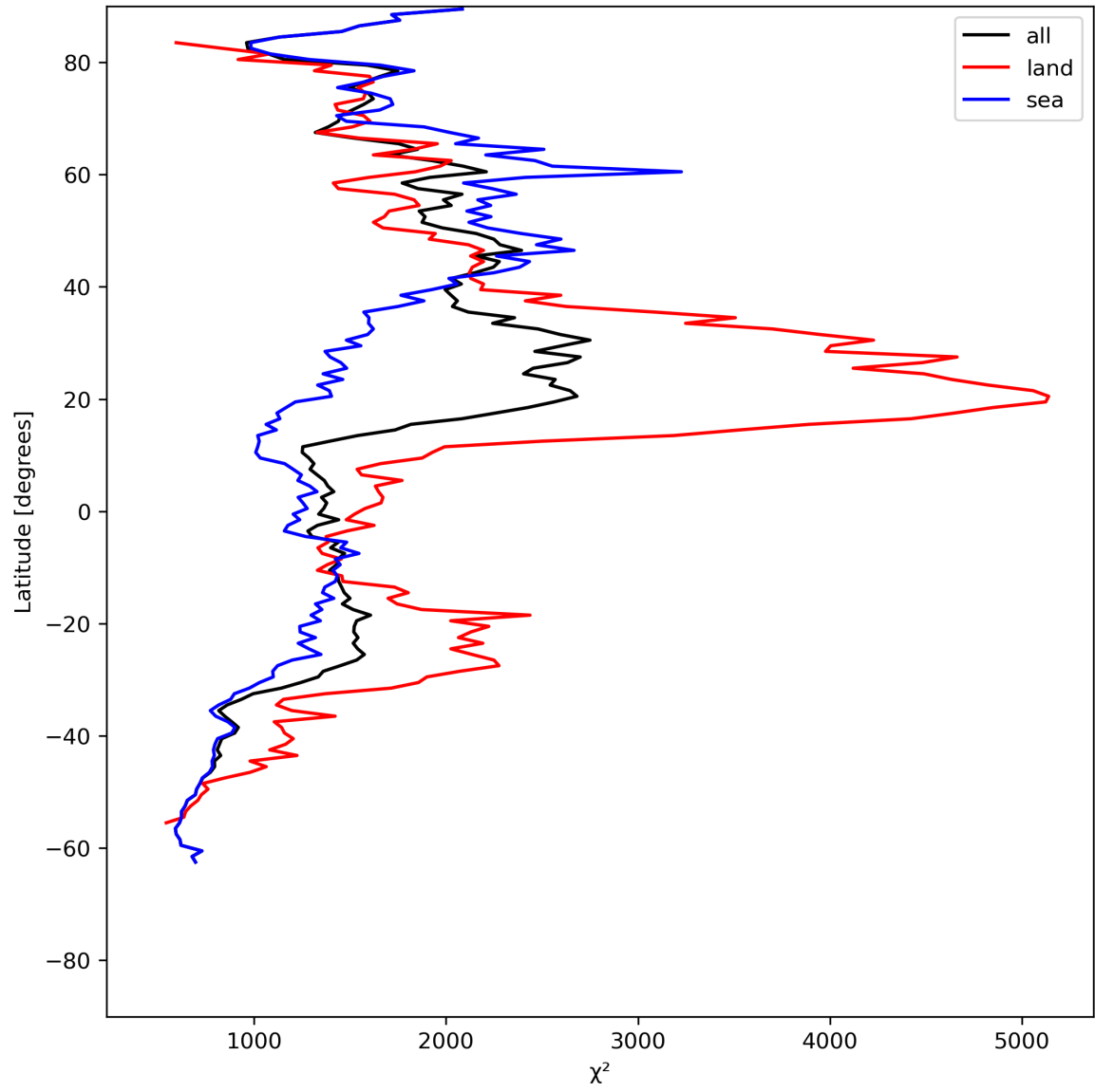
Figure 14: Zonal average of “ \chi^2 ” for 2023-07-11 to 2023-07-13.
