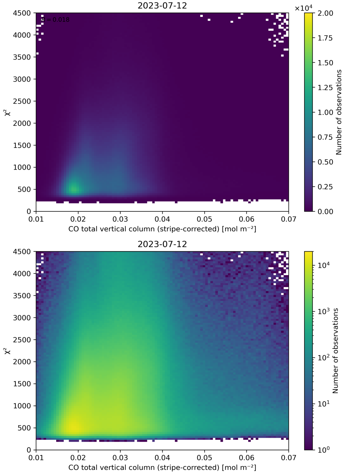
Figure 37: Scatter density plot of “CO total vertical column (stripe-corrected)” against “ \chi^2 ” for 2023-07-11 to 2023-07-13.
