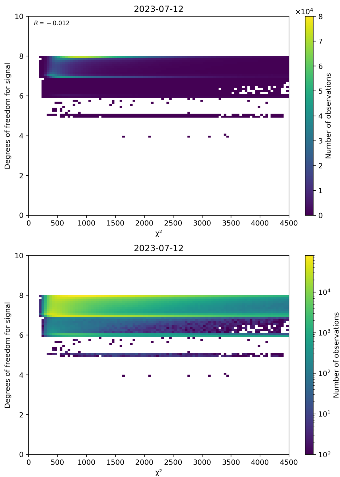
Figure 48: Scatter density plot of “ \chi^2 ” against “Degrees of freedom for signal” for 2023-07-11 to 2023-07-13.
