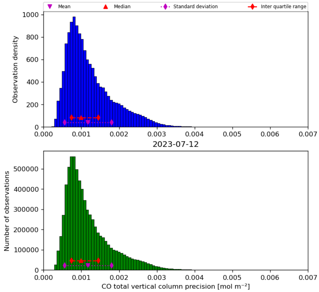
Figure 20: Histogram of “CO total vertical column precision” for 2023-07-11 to 2023-07-13
