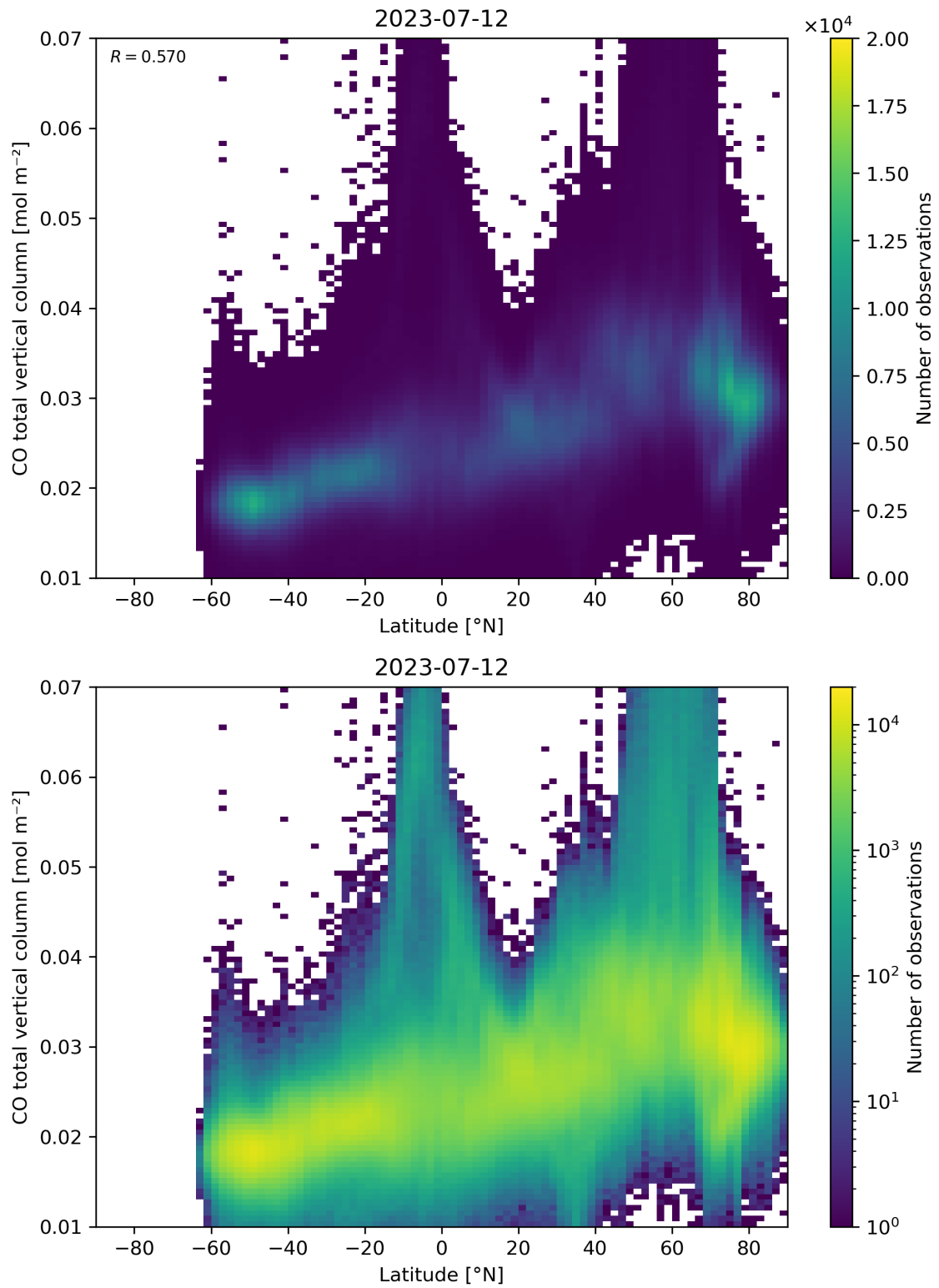
Figure 51: Scatter density plot of “Latitude” against “CO total vertical column” for 2023-07-11 to 2023-07-13.
