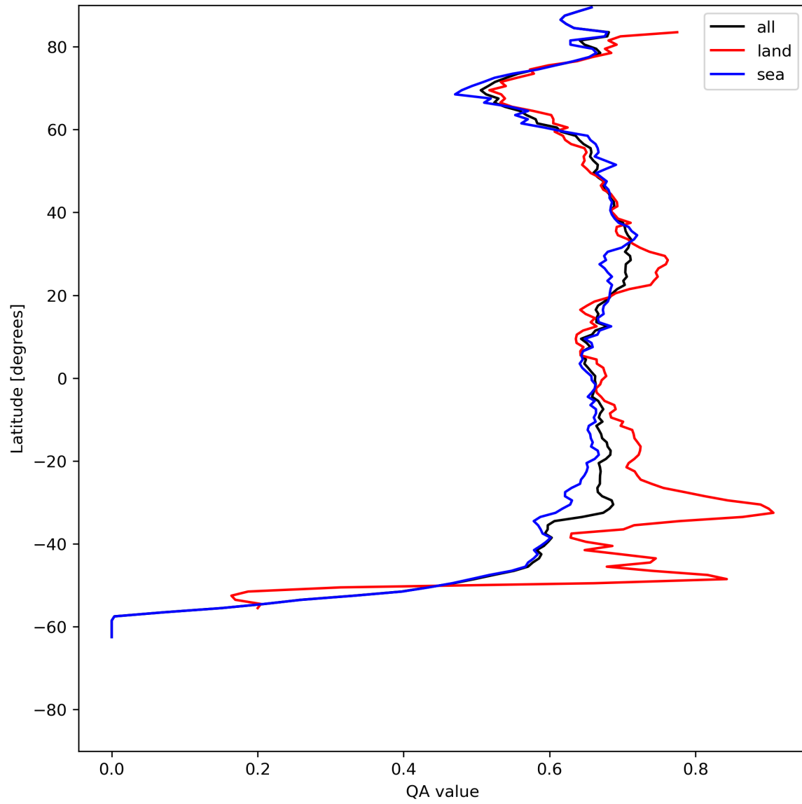
Figure 9: Zonal average of “QA value” for 2023-07-11 to 2023-07-13.
