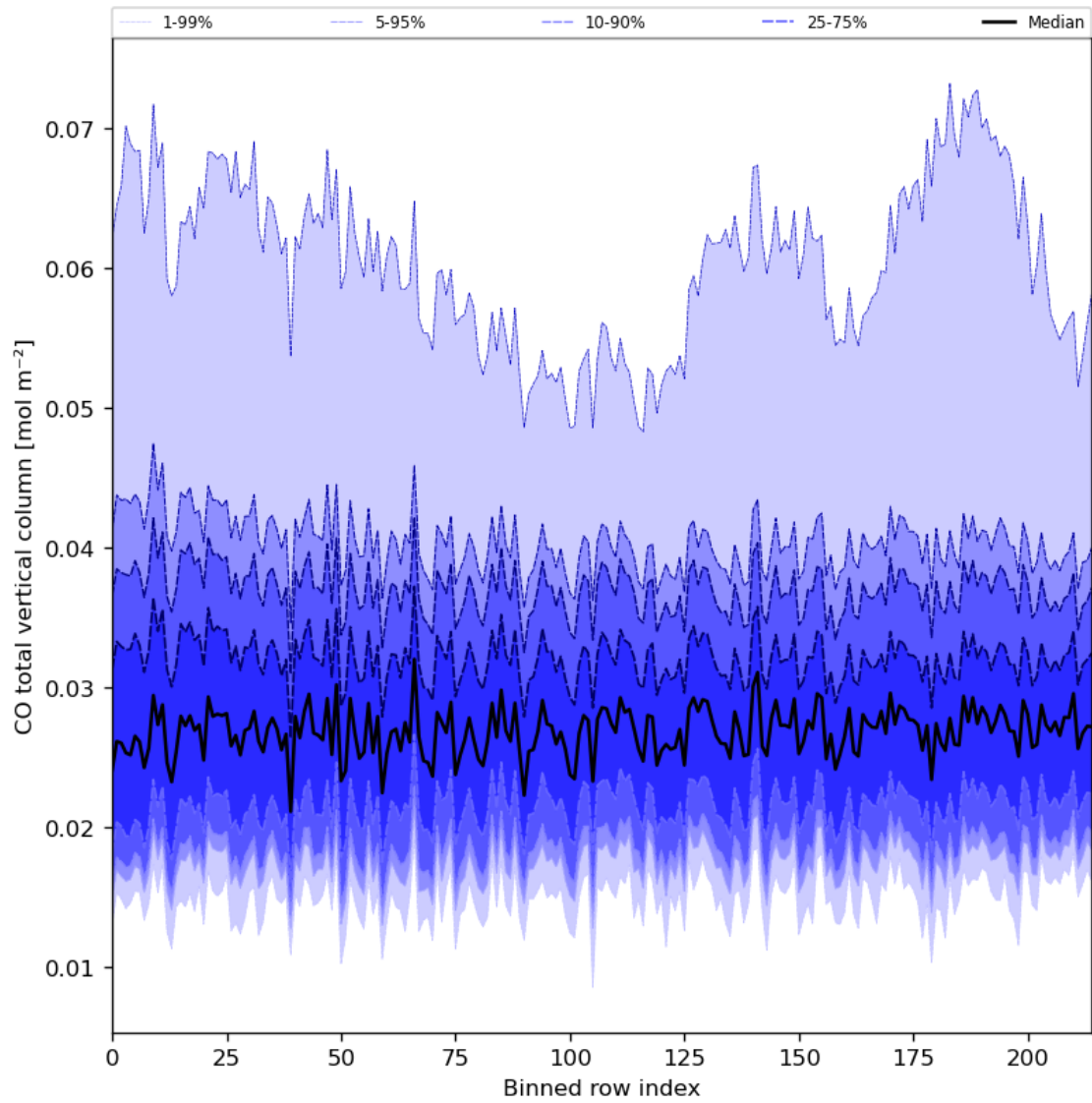
Figure 26: Along track statistics of “CO total vertical column” for 2023-07-11 to 2023-07-13
