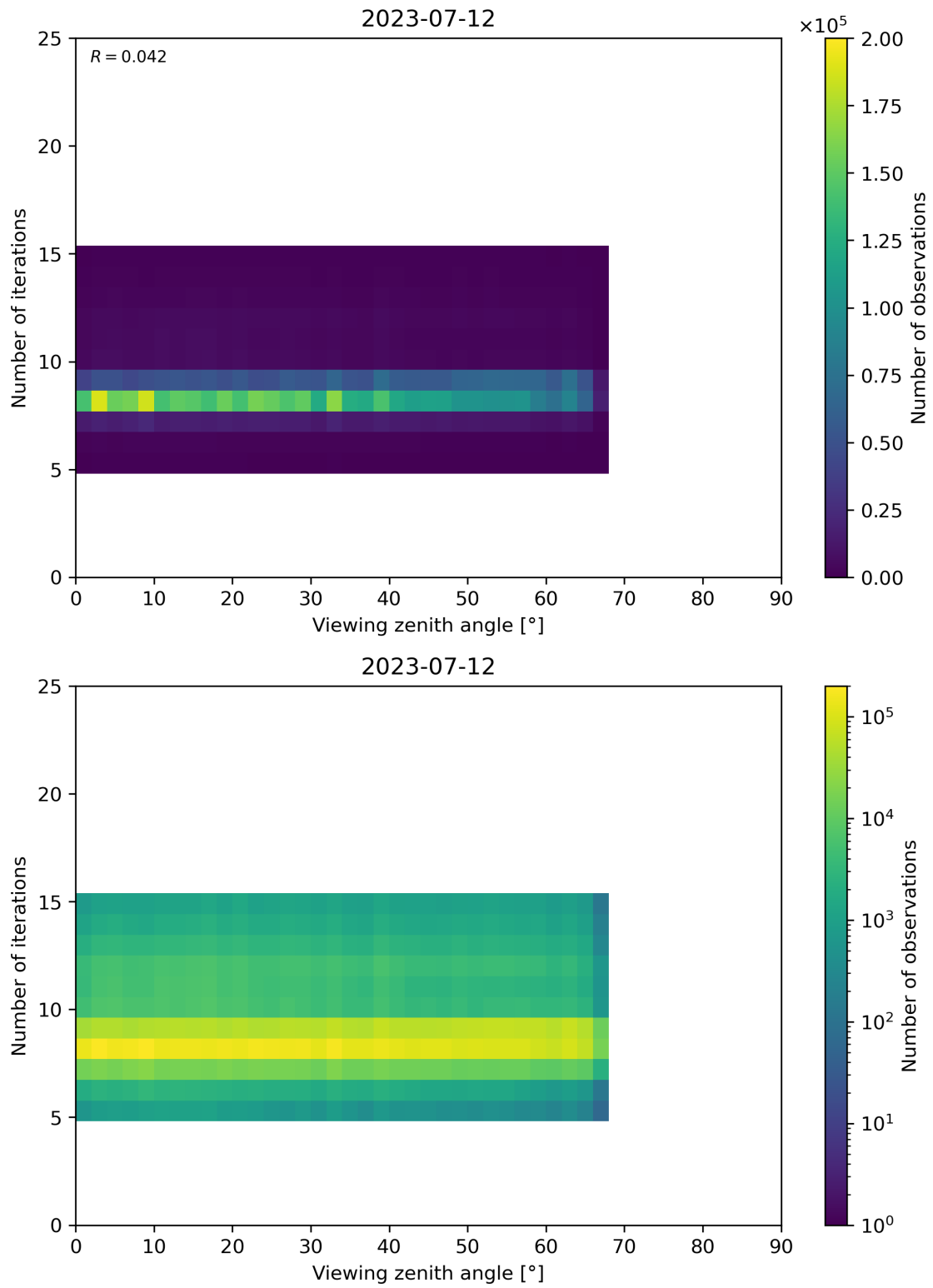
Figure 75: Scatter density plot of “Viewing zenith angle” against “Number of iterations” for 2023-07-11 to 2023-07-13.
