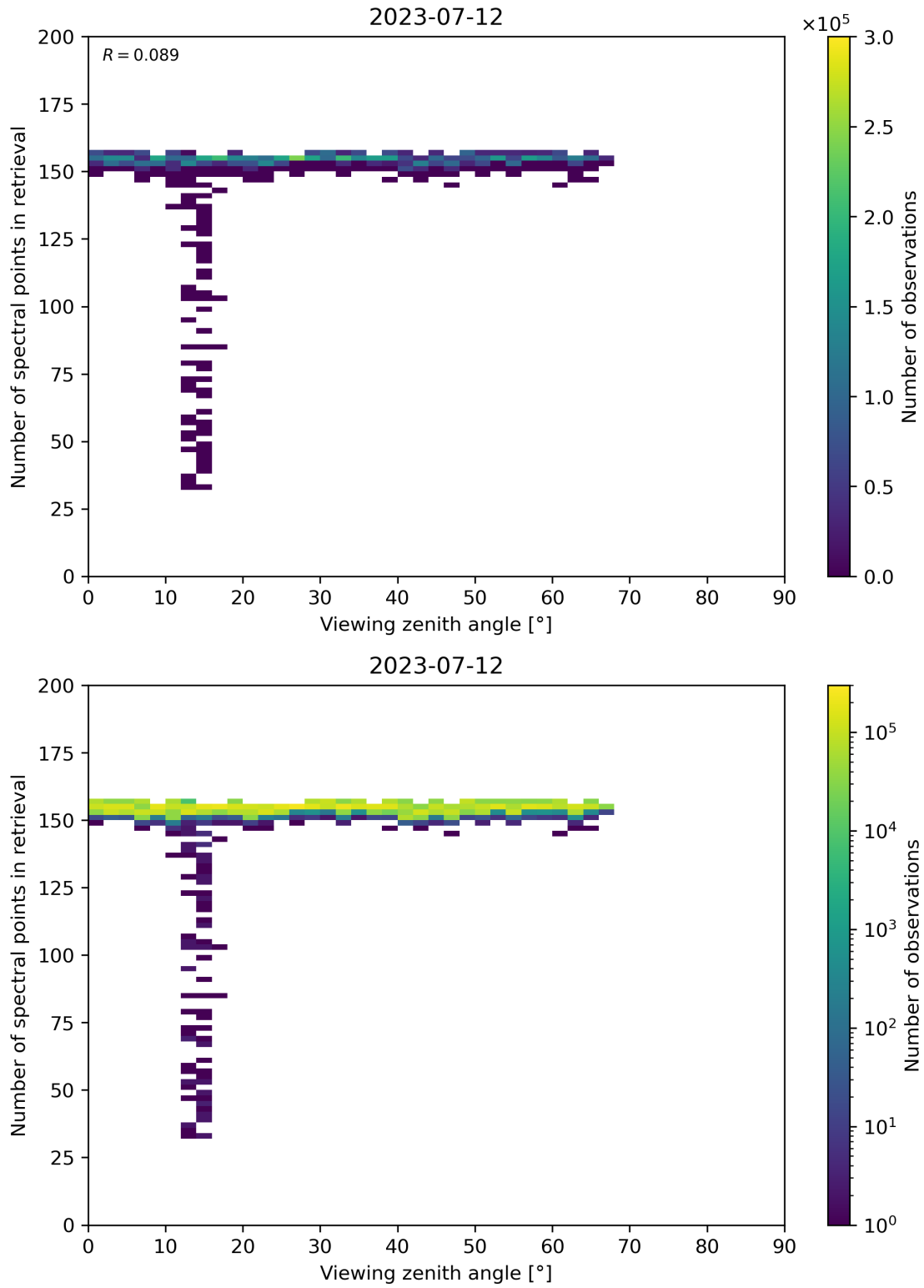
Figure 76: Scatter density plot of “Viewing zenith angle” against “Number of spectral points in retrieval” for 2023-07-11 to 2023-07-13.
