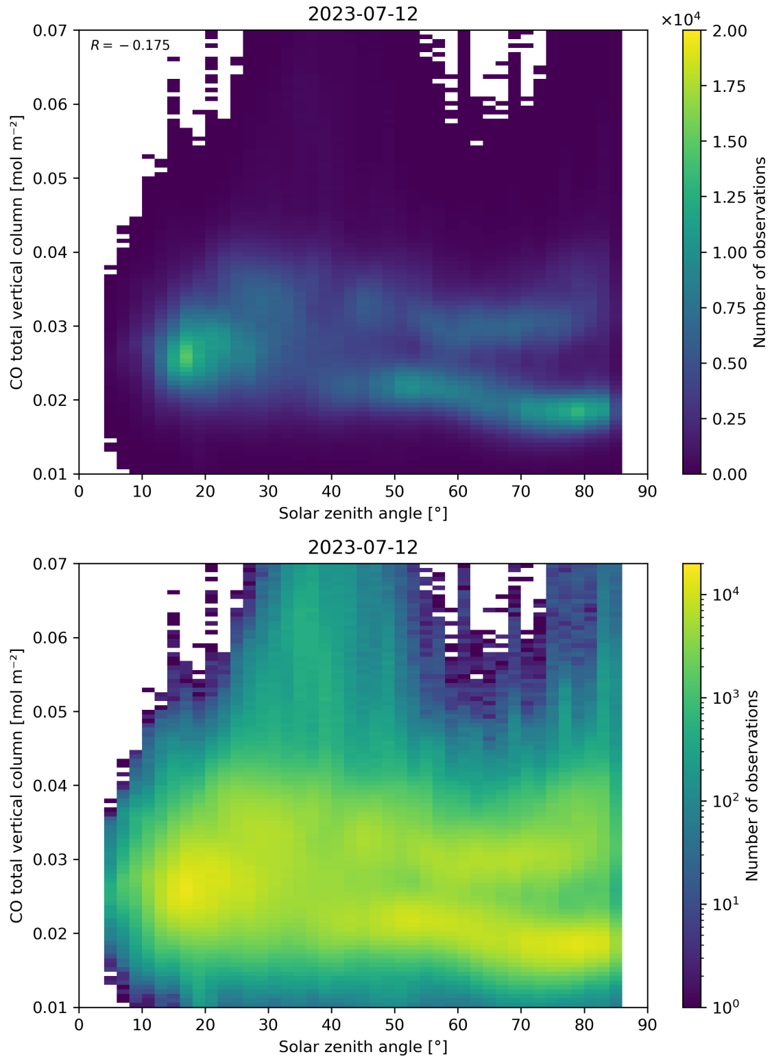
Figure 61: Scatter density plot of “Solar zenith angle” against “CO total vertical column” for 2023-07-11 to 2023-07-13.
