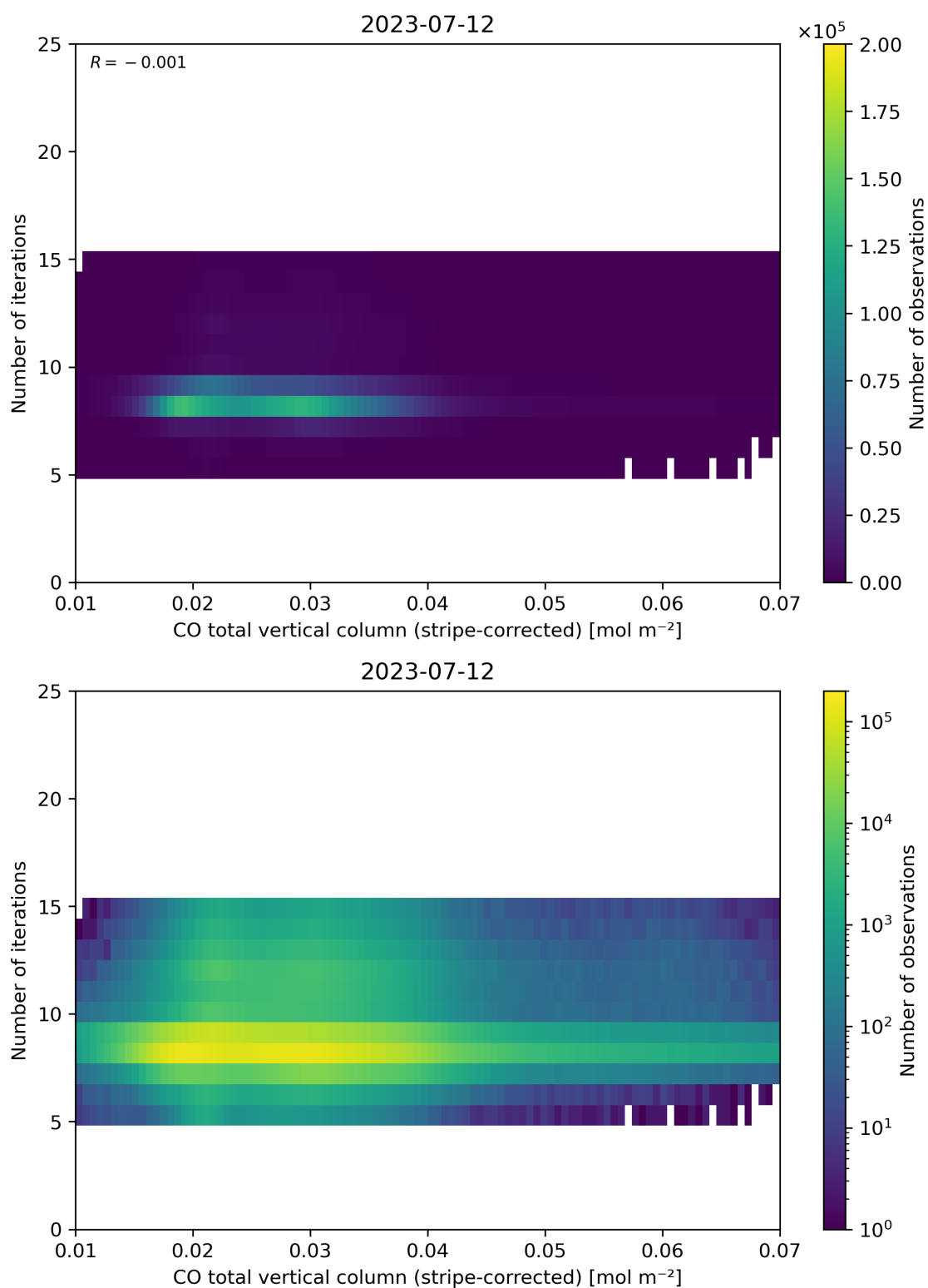
Figure 39: Scatter density plot of “CO total vertical column (stripe-corrected)” against “Number of iterations” for 2023-07-11 to 2023-07-13.
