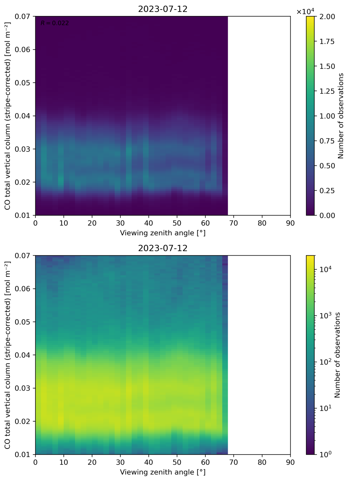
Figure 70: Scatter density plot of “Viewing zenith angle” against “CO total vertical column (stripe-corrected)” for 2023-07-11 to 2023-07-13.
