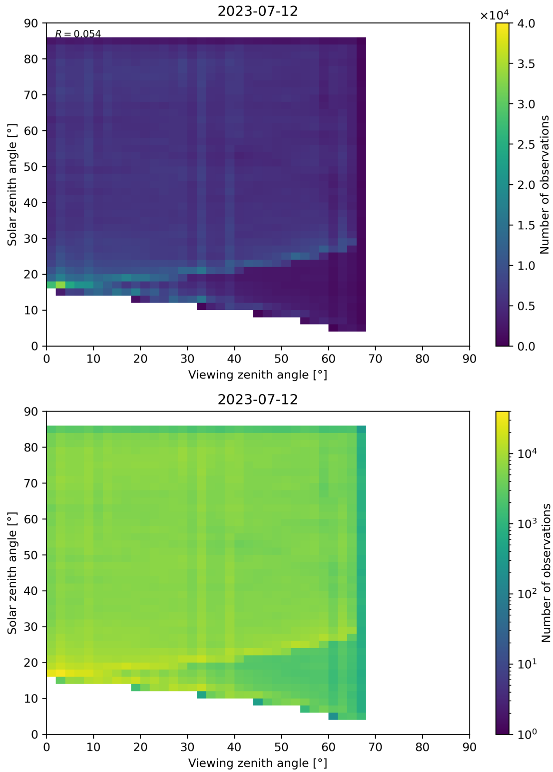
Figure 77: Scatter density plot of “Viewing zenith angle” against “Solar zenith angle” for 2023-07-11 to 2023-07-13.
