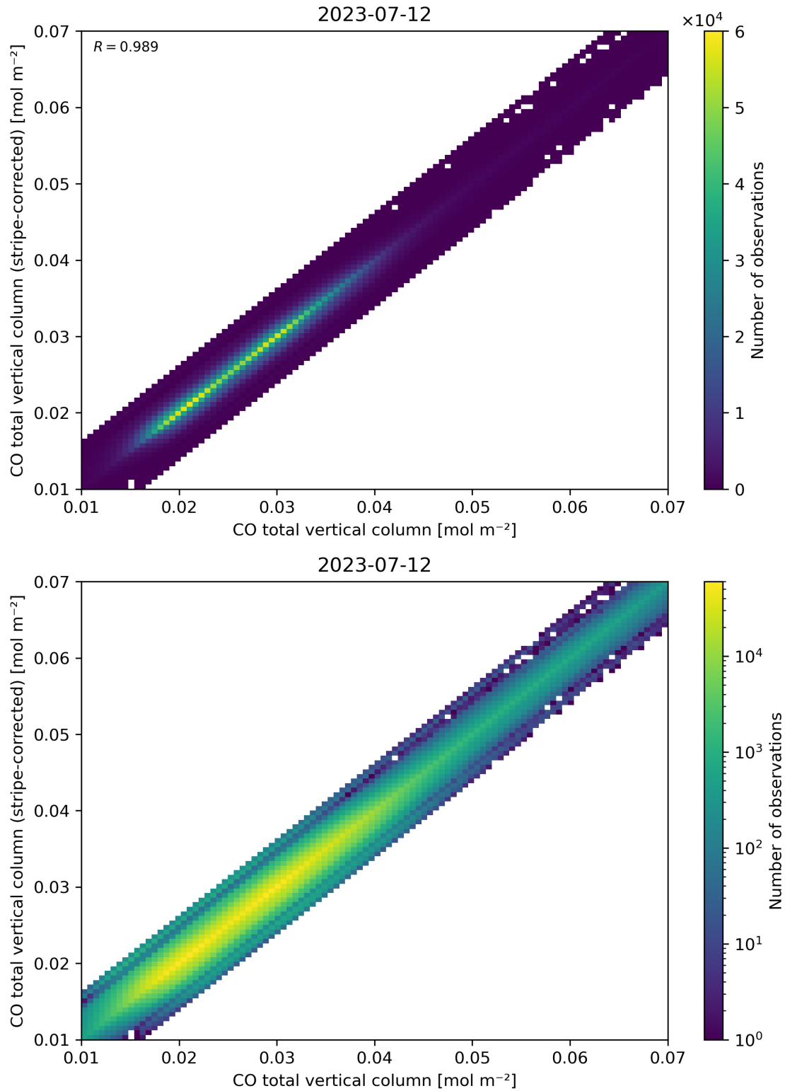
Figure 33: Scatter density plot of “CO total vertical column” against “CO total vertical column (stripe-corrected)” for 2023-07-11 to 2023-07-13.
