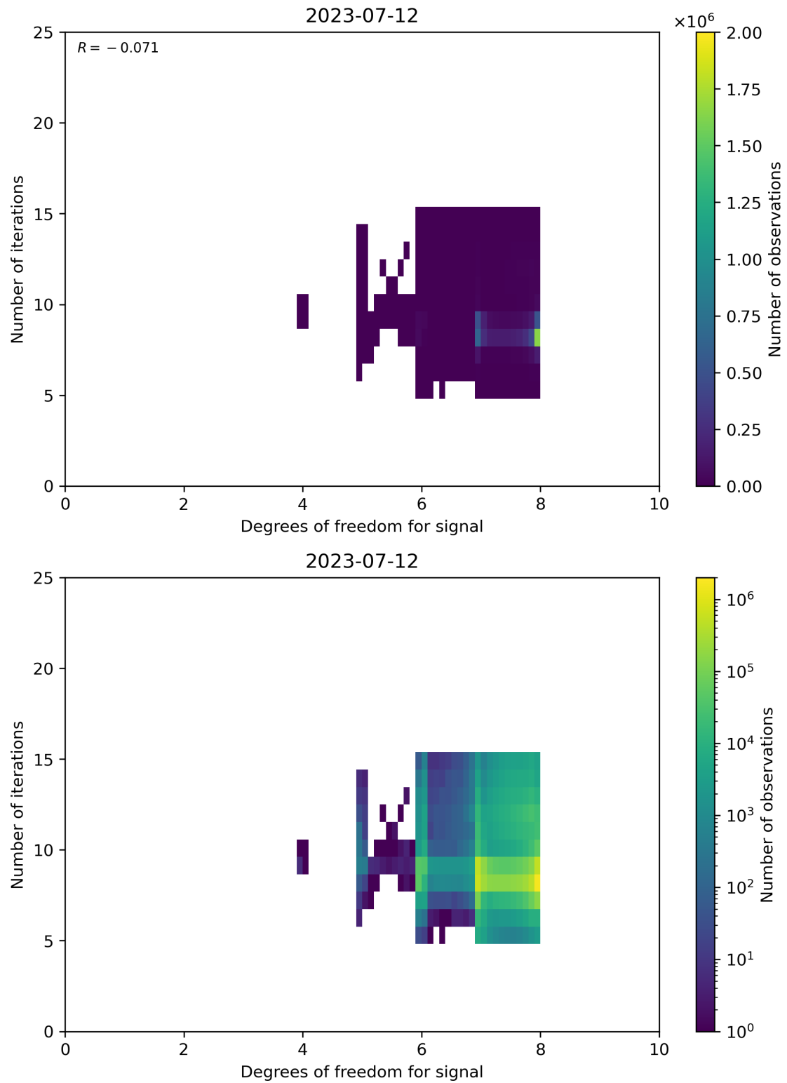
Figure 50: Scatter density plot of “Degrees of freedom for signal” against “Number of iterations” for 2023-07-11 to 2023-07-13.
