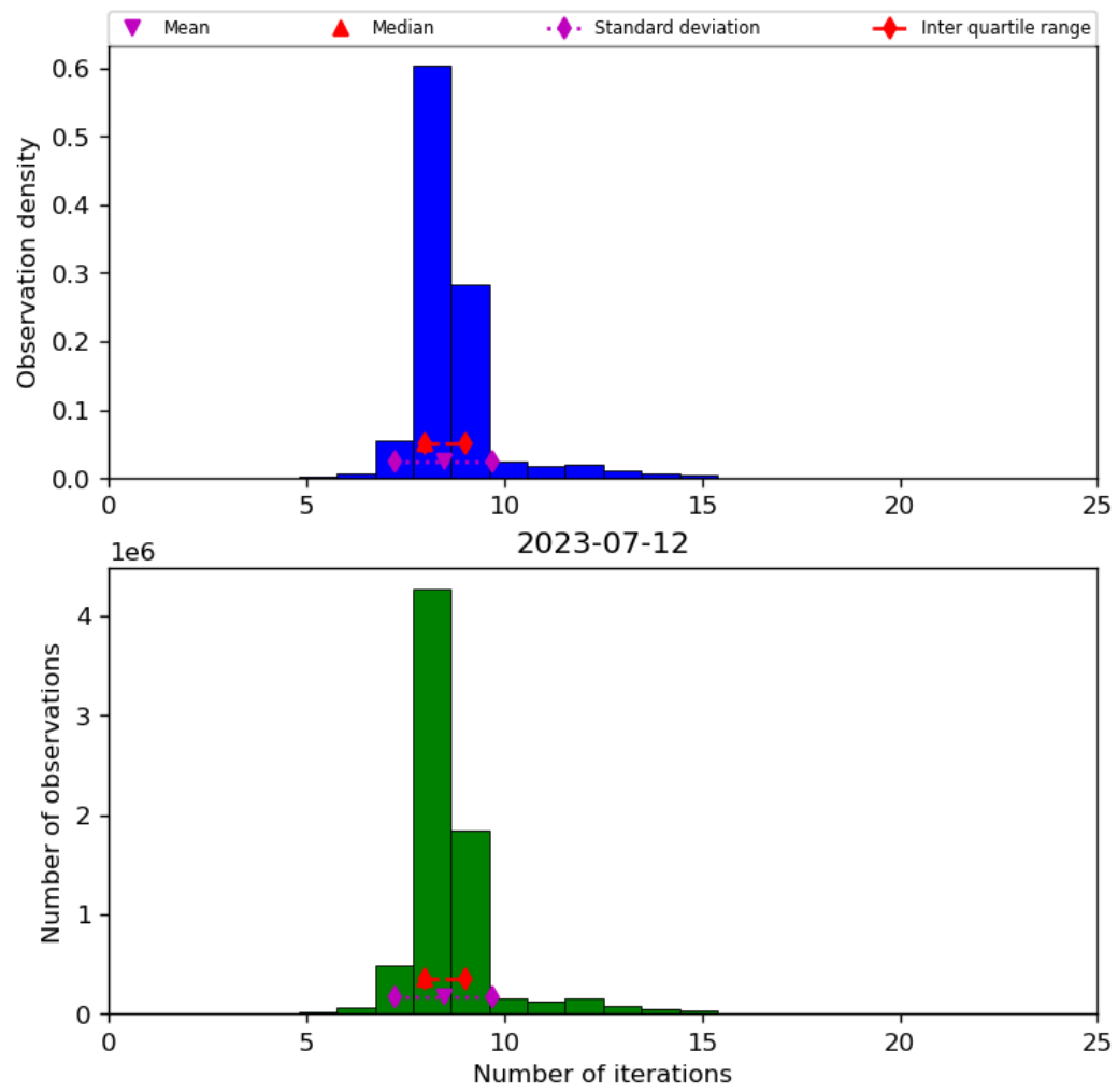
Figure 24: Histogram of "Number of iterations" for 2023-07-11 to 2023-07-13
