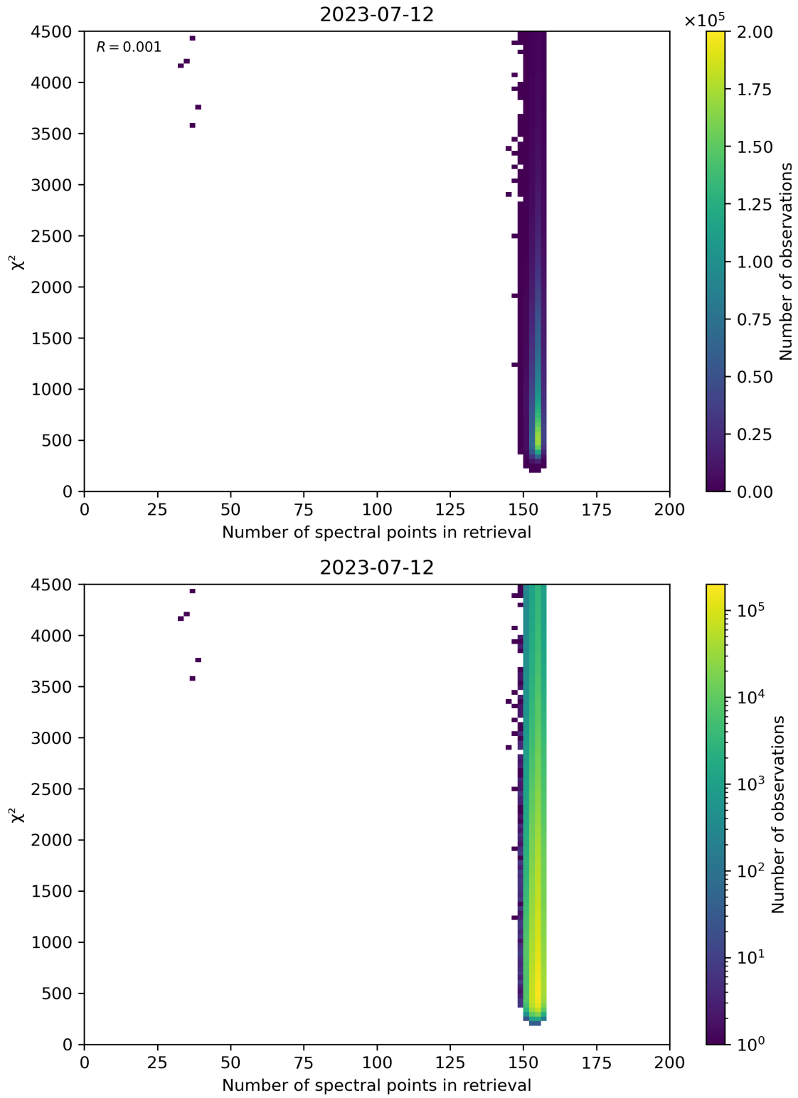
Figure 58: Scatter density plot of “Number of spectral points in retrieval” against “ \chi^2 ” for 2023-07-11 to 2023-07-13.
