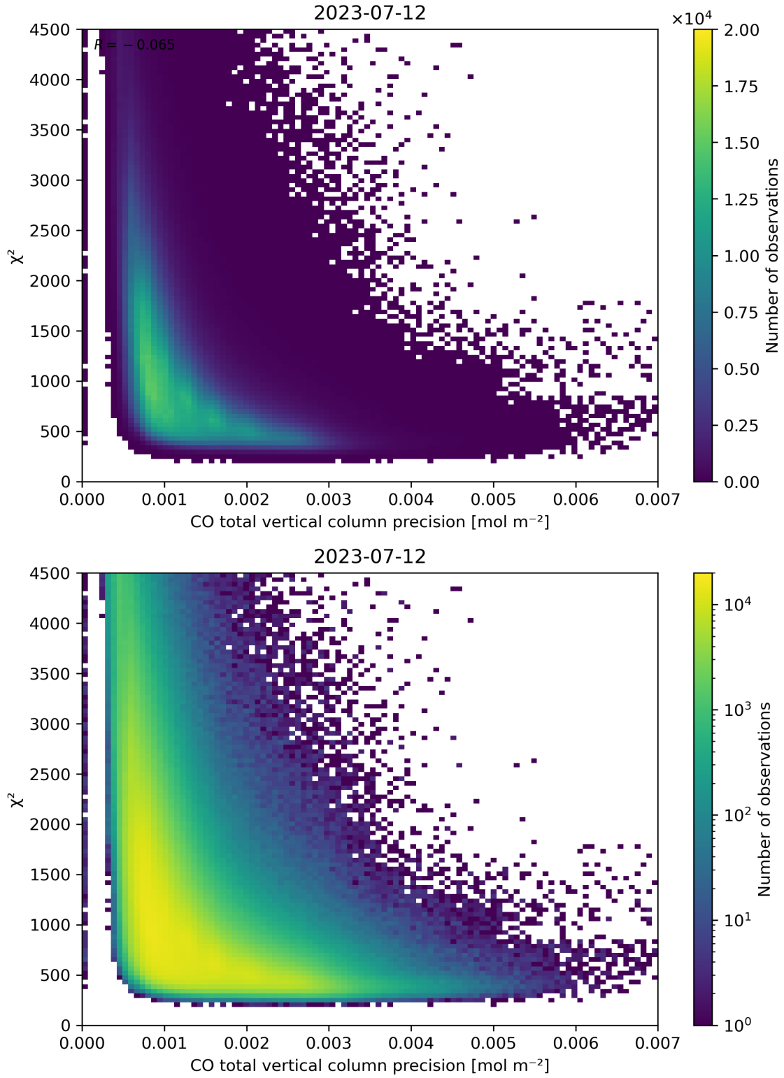
Figure 44: Scatter density plot of “CO total vertical column precision” against “ \chi^2 ” for 2023-07-11 to 2023-07-13.
