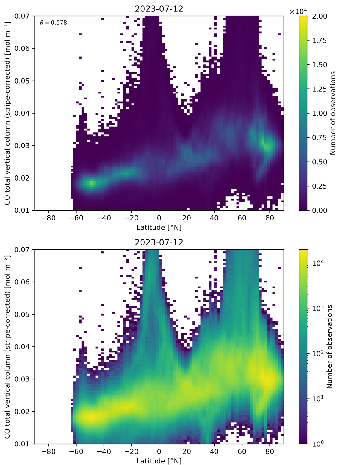
Figure 52: Scatter density plot of “Latitude” against “CO total vertical column (stripe-corrected)” for 2023-07-11 to 2023-07-13.
