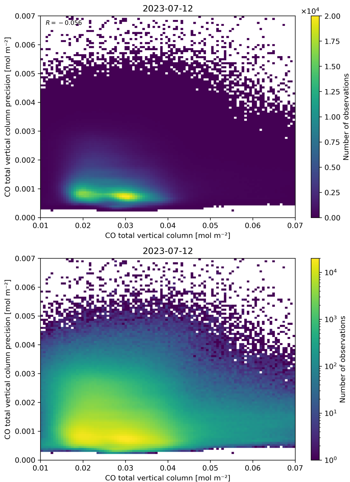
Figure 34: Scatter density plot of “CO total vertical column” against “CO total vertical column precision” for 2023-07-11 to 2023-07-13.
