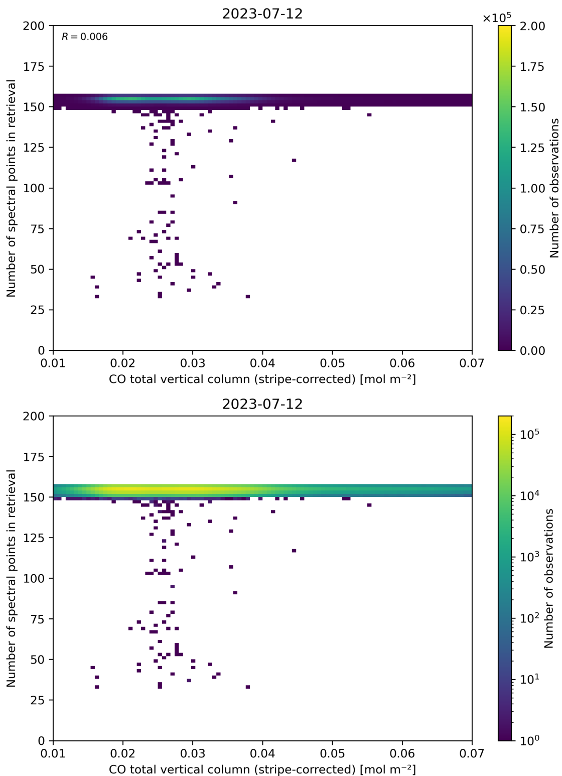
Figure 40: Scatter density plot of “CO total vertical column (stripe-corrected)” against “Number of spectral points in retrieval” for 2023-07-11 to 2023-07-13.
