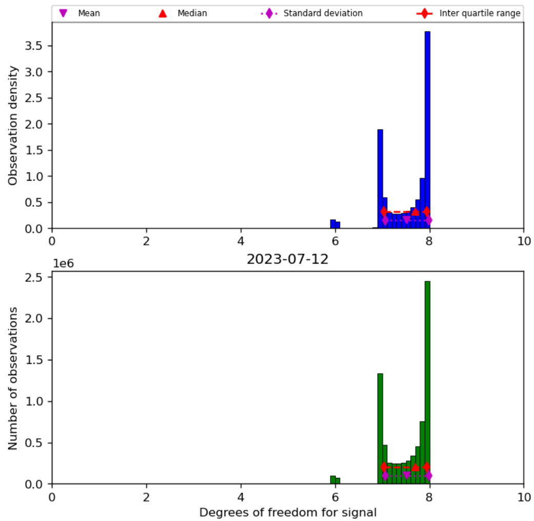
Figure 23: Histogram of “Degrees of freedom for signal” for 2023-07-11 to 2023-07-13
