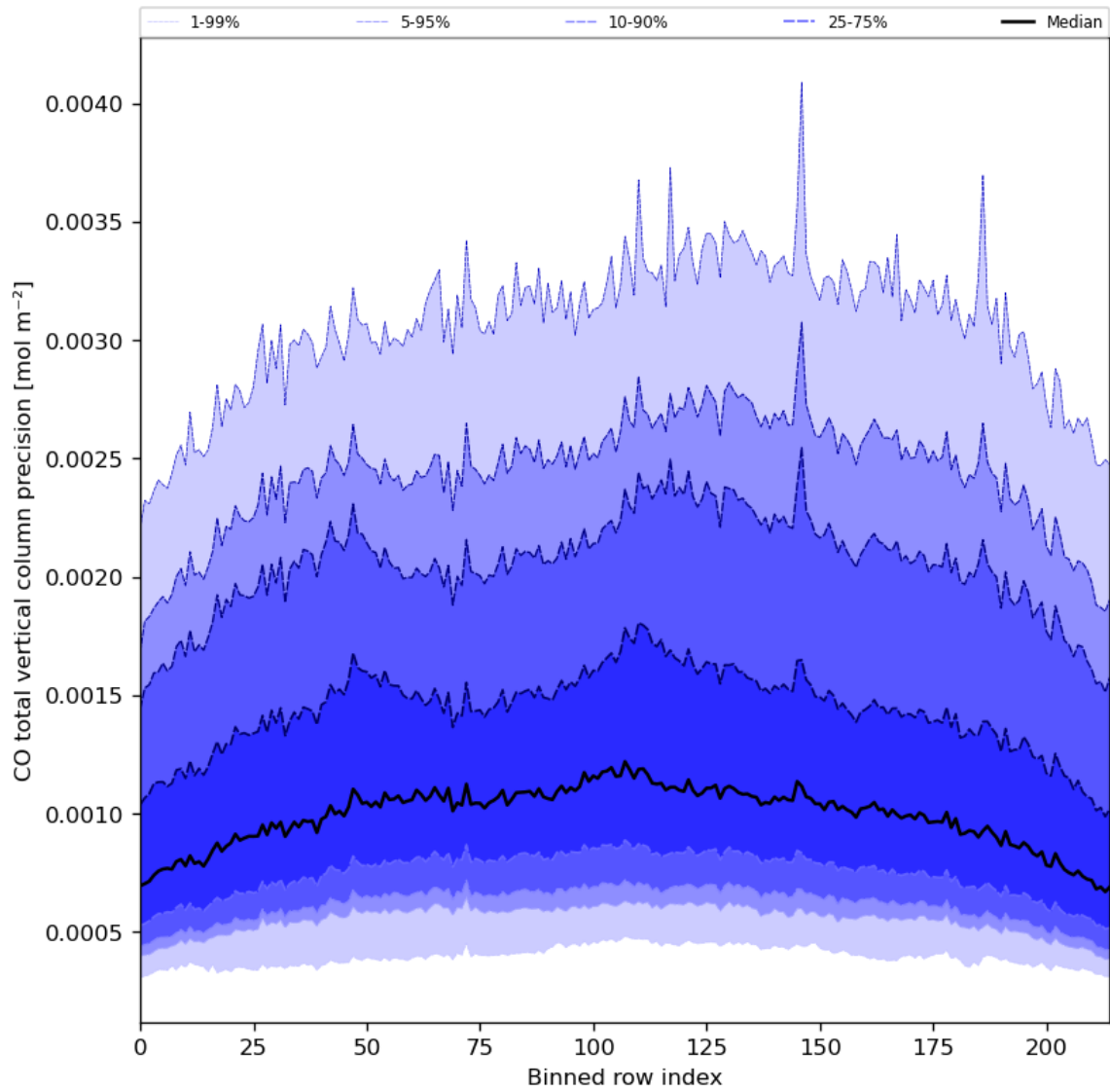
Figure 28: Along track statistics of “CO total vertical column precision” for 2023-07-11 to 2023-07-13
