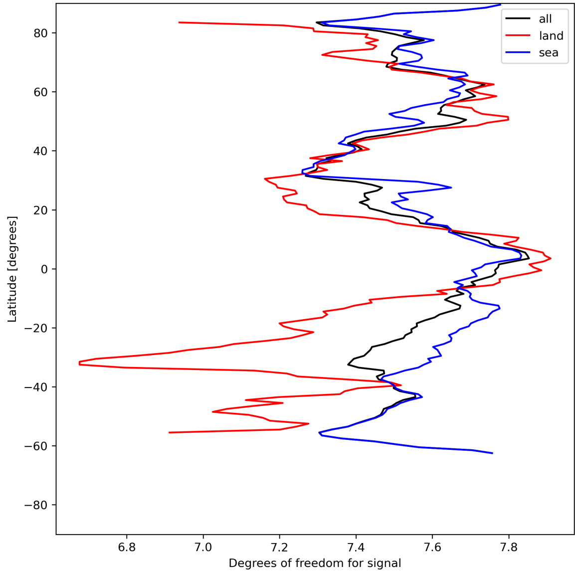
Figure 15: Zonal average of “Degrees of freedom for signal” for 2023-07-11 to 2023-07-13.
