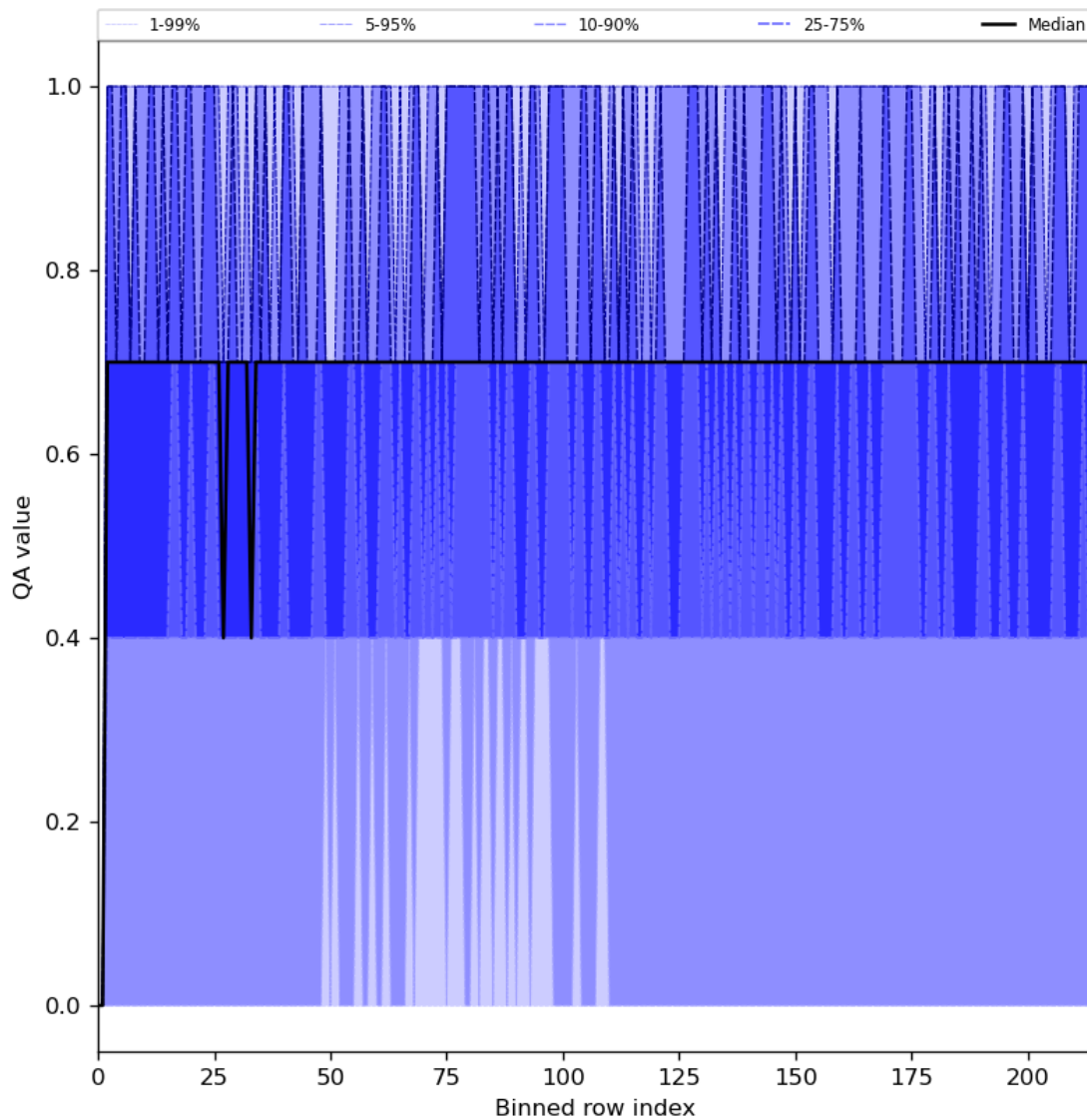
Figure 25: Along track statistics of “QA value” for 2023-07-11 to 2023-07-13
