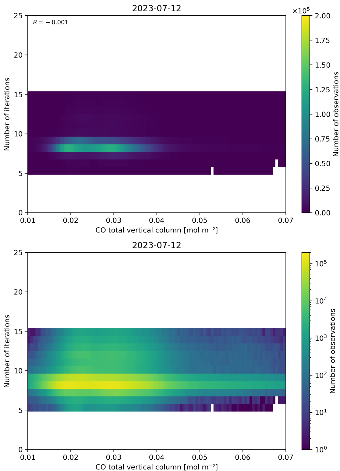
Figure 42: Scatter density plot of “CO total vertical column” against “Number of iterations” for 2023-07-11 to 2023-07-13.
