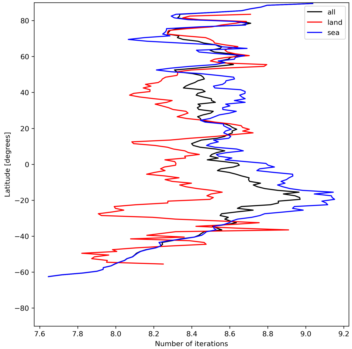
Figure 16: Zonal average of “Number of iterations” for 2023-07-11 to 2023-07-13.
