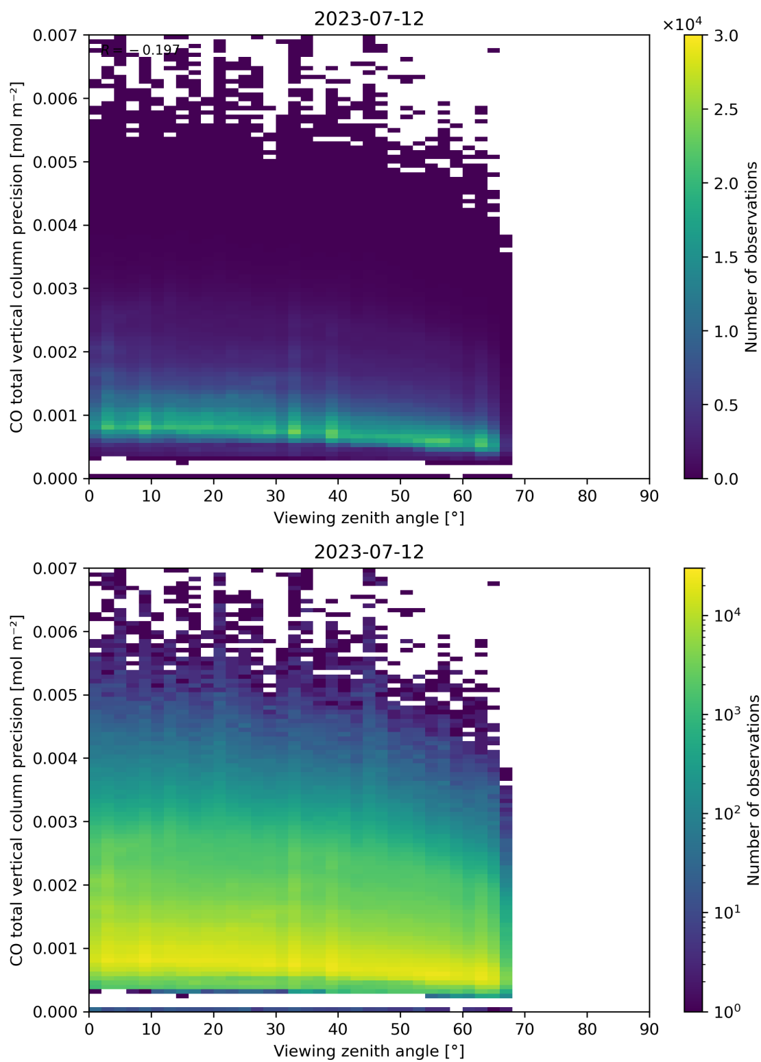
Figure 71: Scatter density plot of “Viewing zenith angle” against “CO total vertical column precision” for 2023-07-11 to 2023-07-13.
