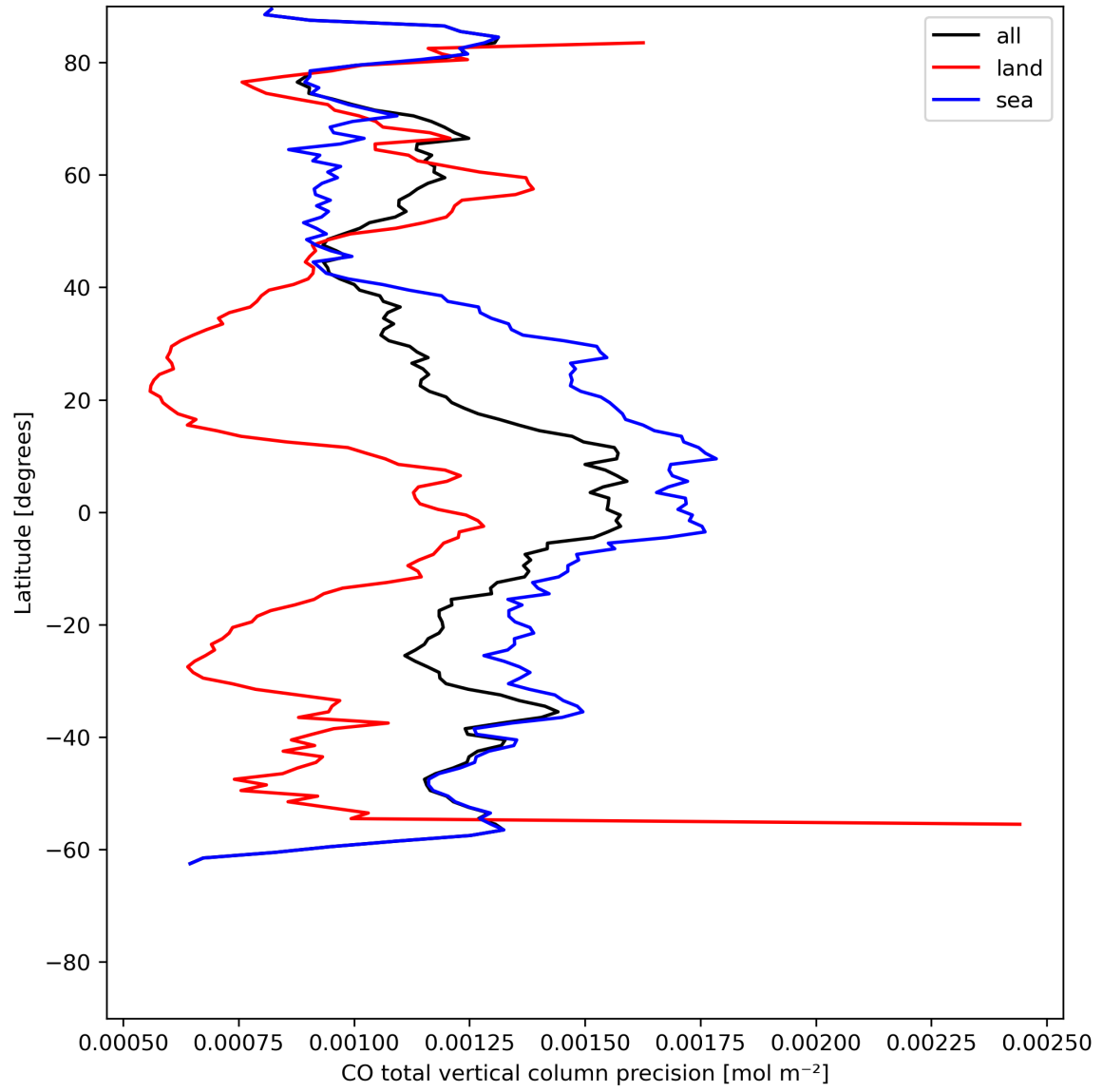
Figure 12: Zonal average of “CO total vertical column precision” for 2023-07-11 to 2023-07-13.
