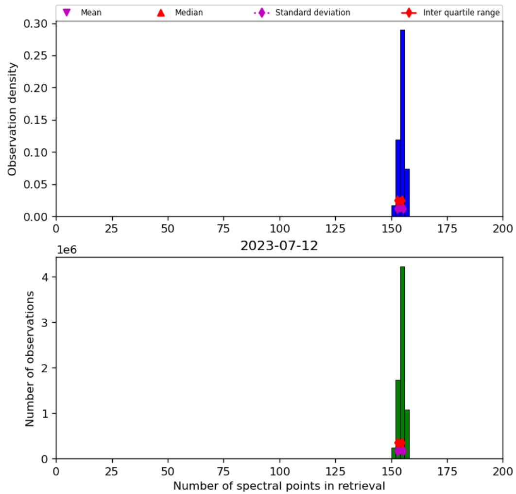
Figure 21: Histogram of “Number of spectral points in retrieval” for 2023-07-11 to 2023-07-13
