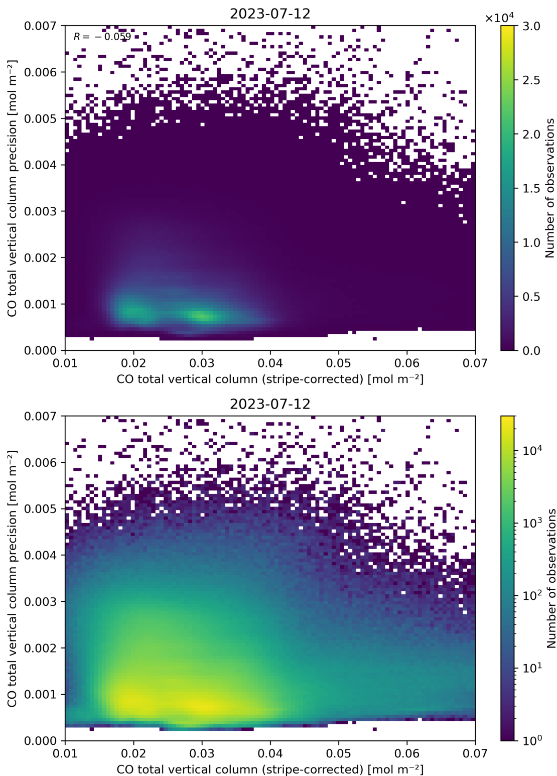
Figure 36: Scatter density plot of “CO total vertical column (stripe-corrected)” against “CO total vertical column precision” for 2023-07-11 to 2023-07-13.
