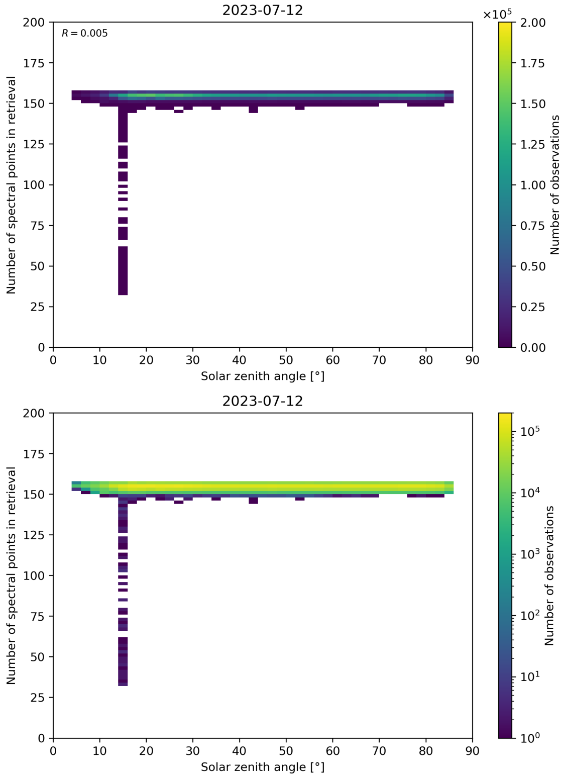
Figure 68: Scatter density plot of “Solar zenith angle” against “Number of spectral points in retrieval” for 2023-07-11 to 2023-07-13.
