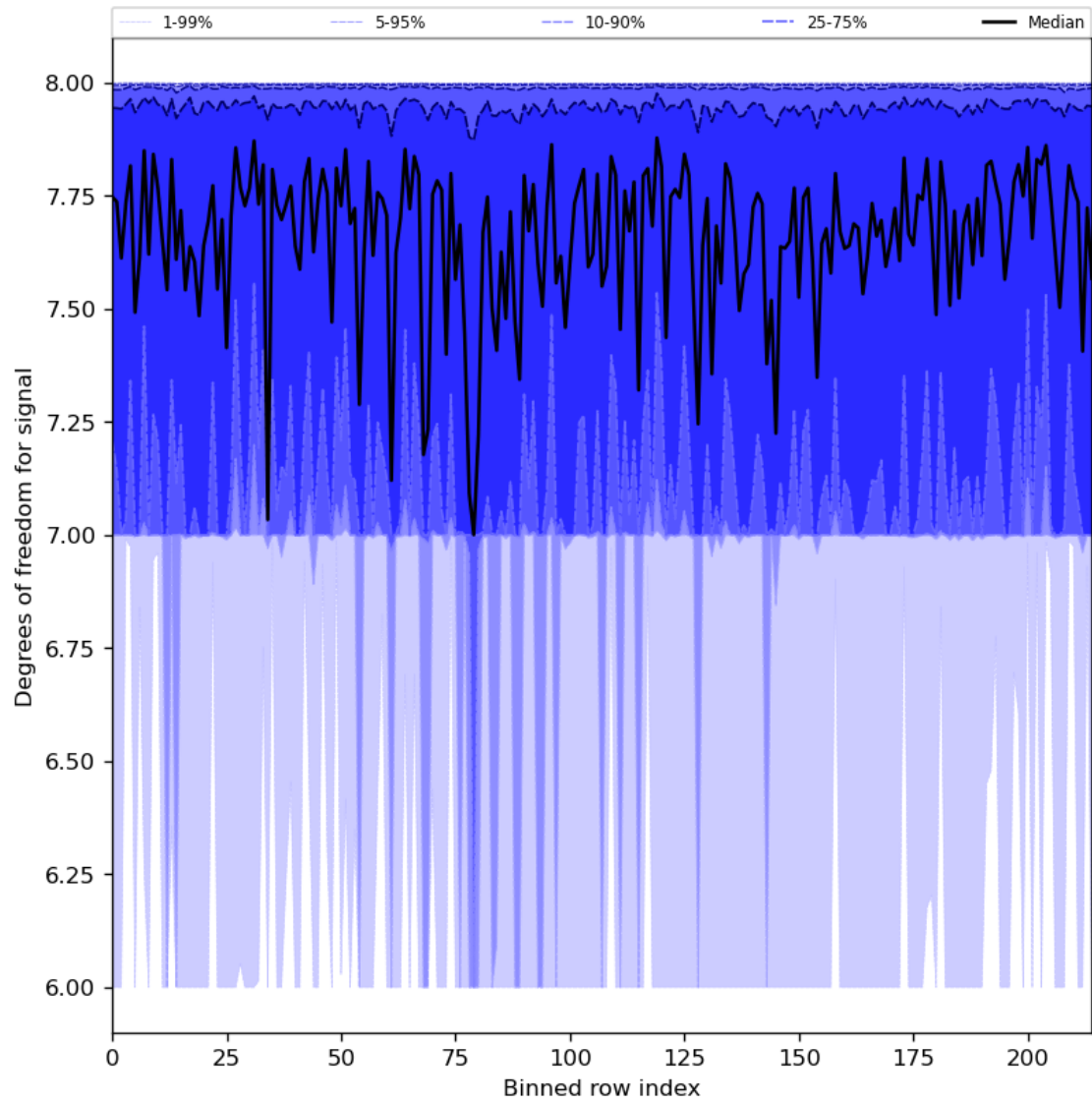
Figure 31: Along track statistics of “Degrees of freedom for signal” for 2023-07-11 to 2023-07-13
