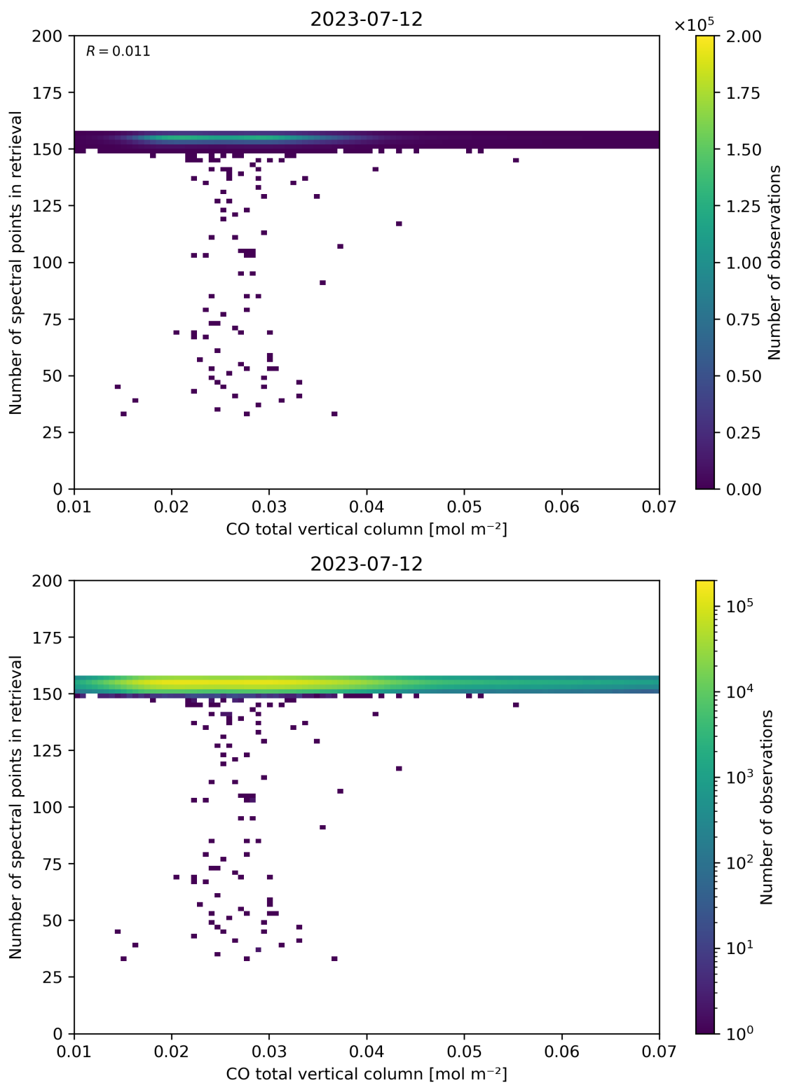
Figure 43: Scatter density plot of “CO total vertical column” against “Number of spectral points in retrieval” for 2023-07-11 to 2023-07-13.
