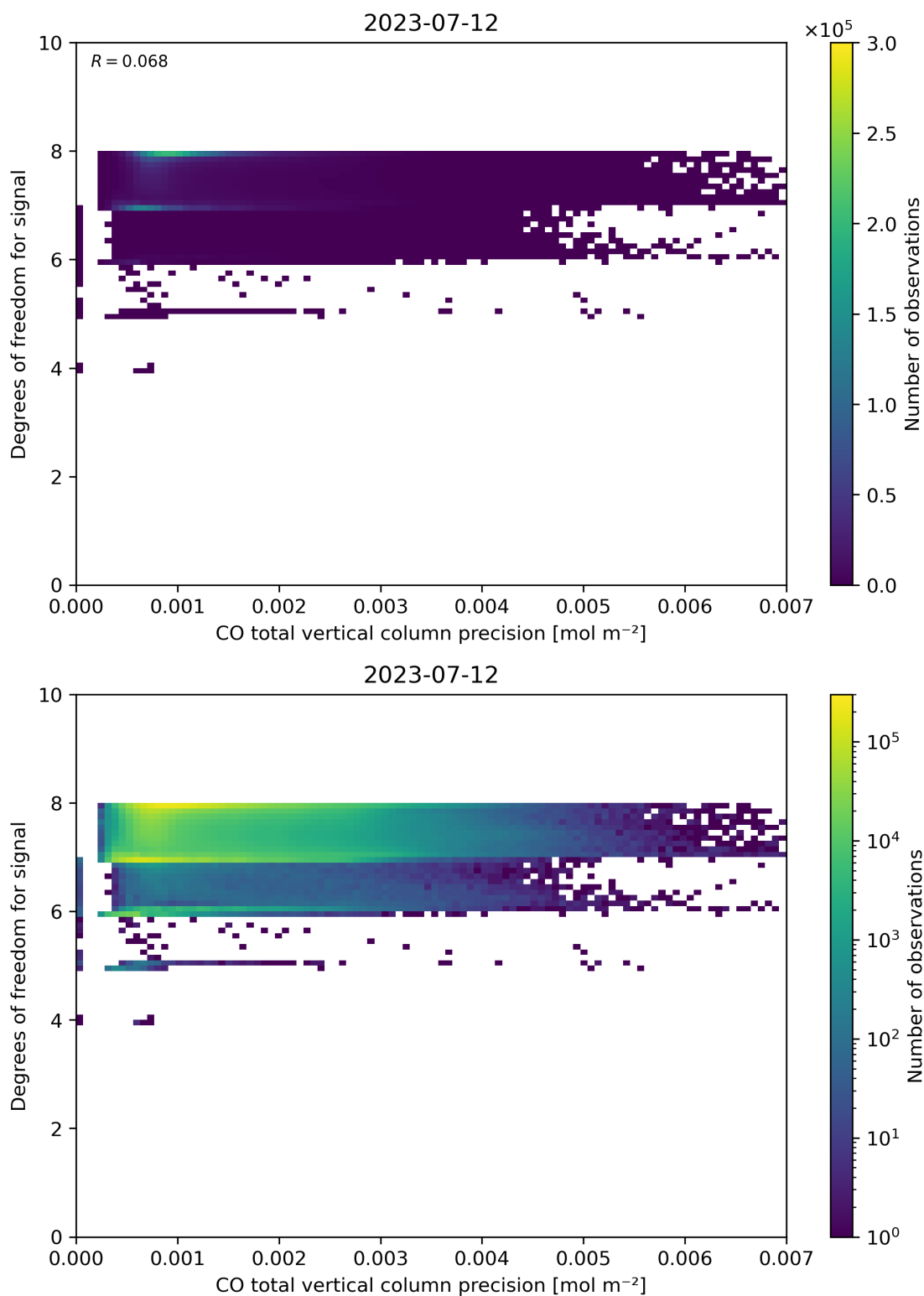
Figure 45: Scatter density plot of “CO total vertical column precision” against “Degrees of freedom for signal” for 2023-07-11 to 2023-07-13.
