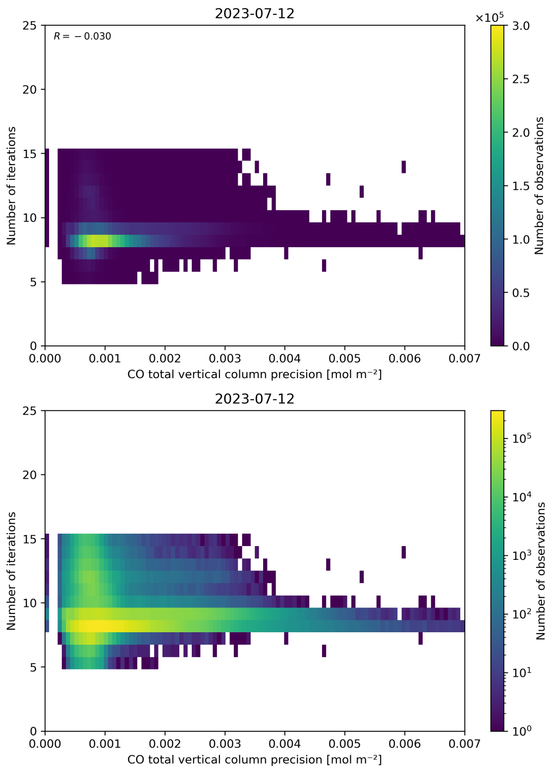
Figure 46: Scatter density plot of “CO total vertical column precision” against “Number of iterations” for 2023-07-11 to 2023-07-13.
