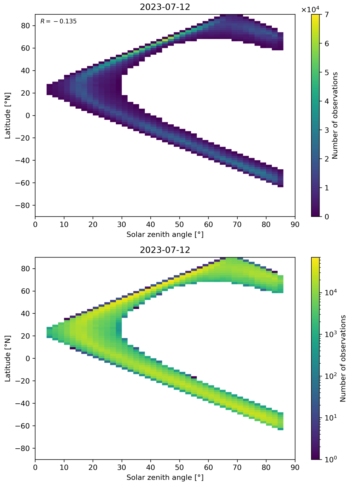
Figure 66: Scatter density plot of “Solar zenith angle” against “Latitude” for 2023-07-11 to 2023-07-13.
