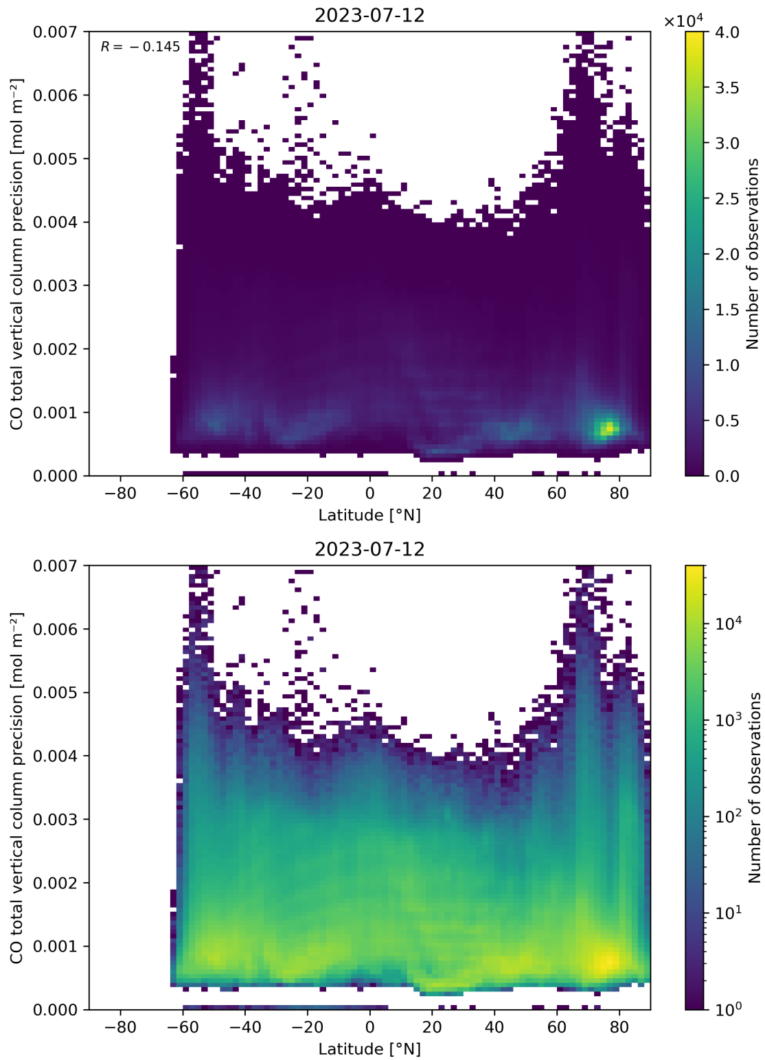
Figure 53: Scatter density plot of “Latitude” against “CO total vertical column precision” for 2023-07-11 to 2023-07-13.
