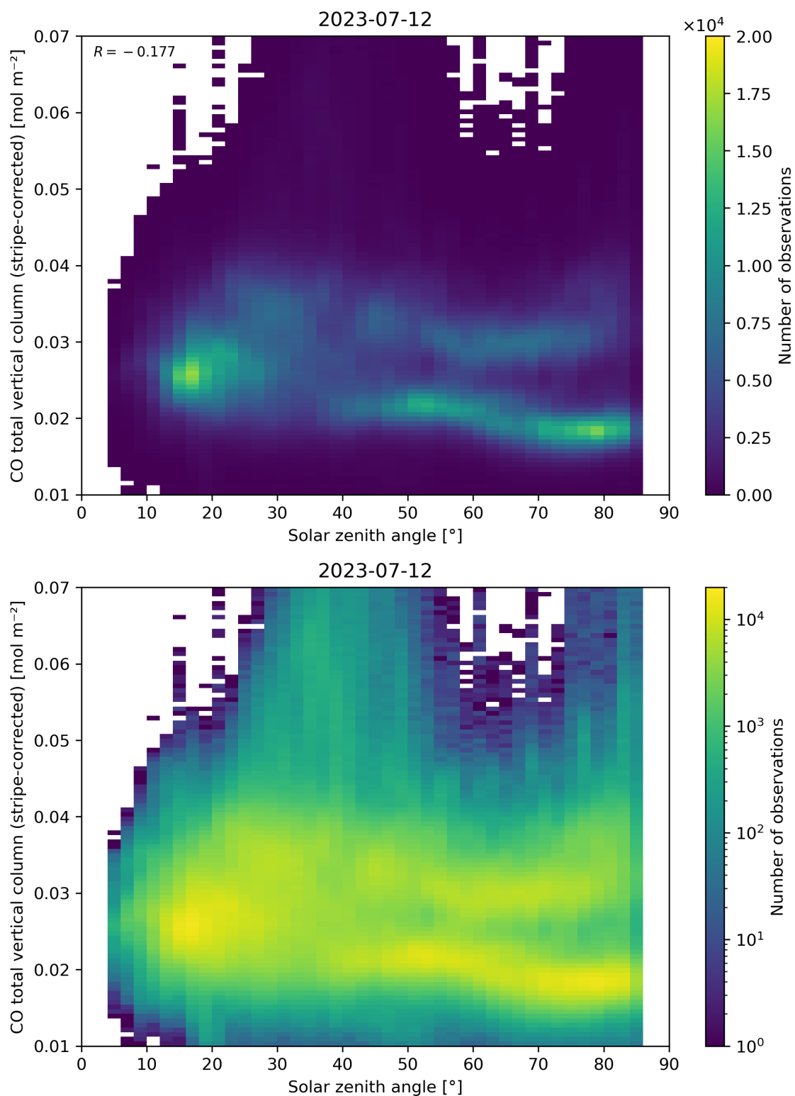
Figure 62: Scatter density plot of “Solar zenith angle” against “CO total vertical column (stripe-corrected)” for 2023-07-11 to 2023-07-13.
