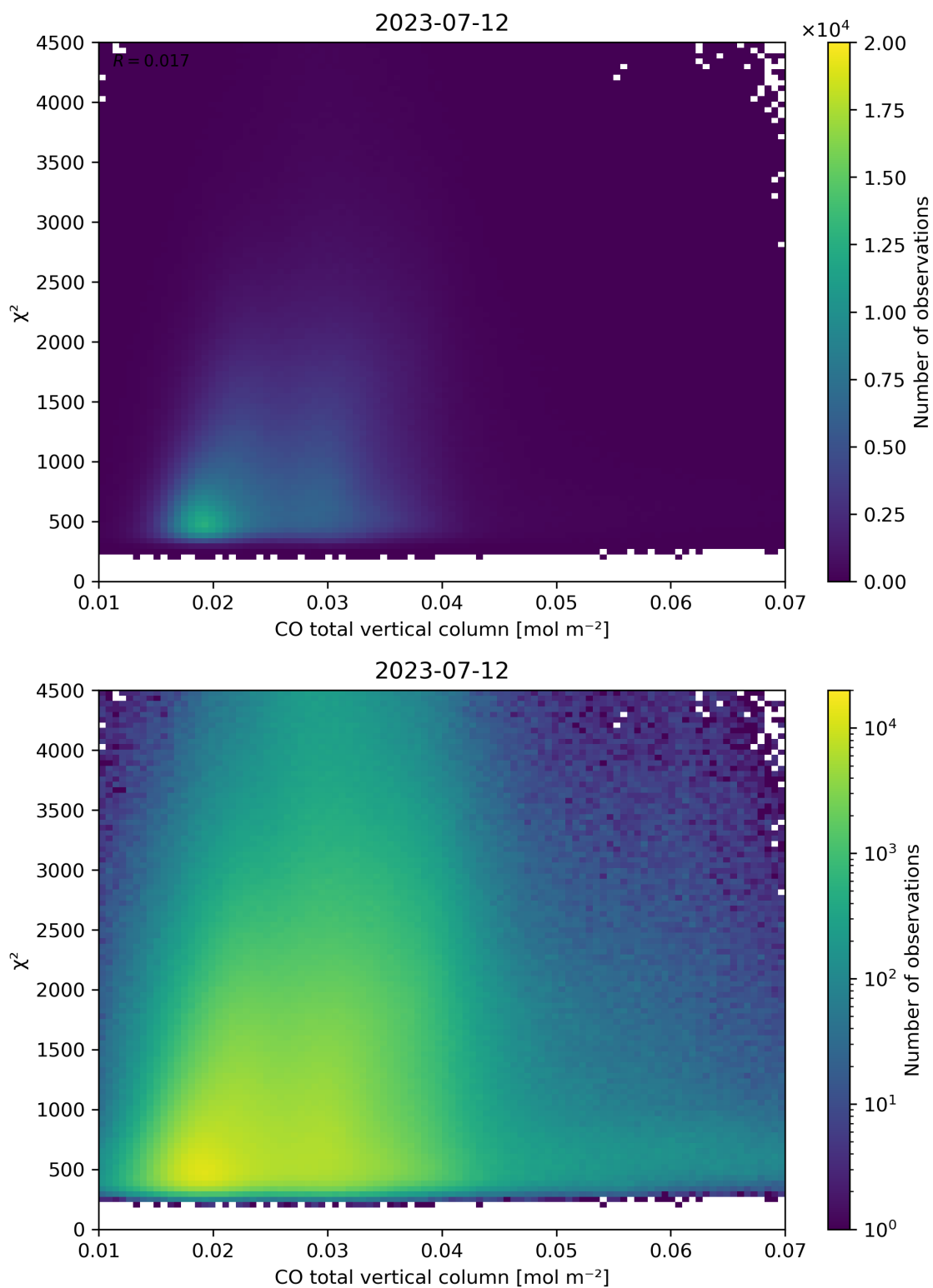
Figure 35: Scatter density plot of “CO total vertical column” against “ \chi^2 ” for 2023-07-11 to 2023-07-13.
