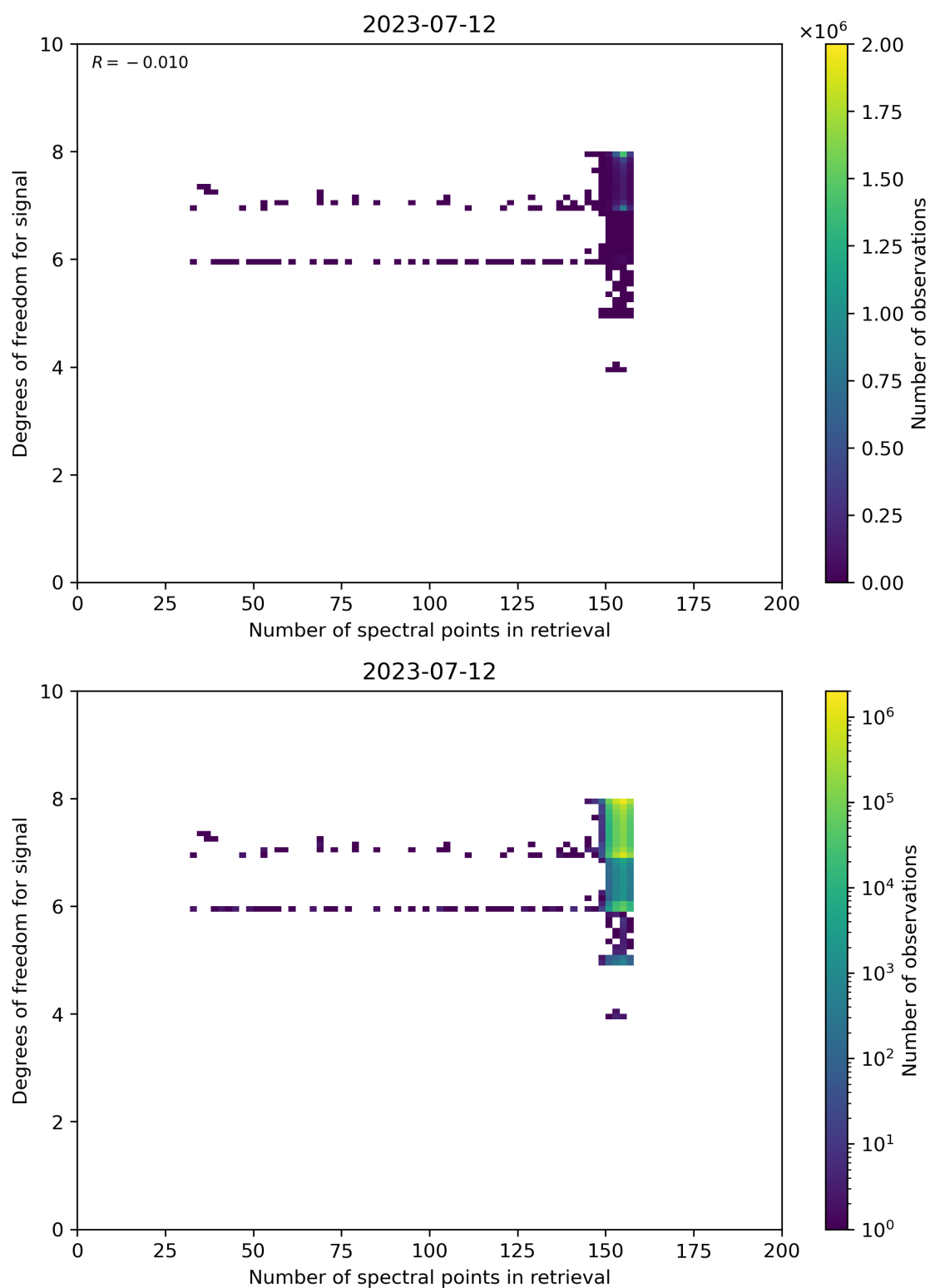
Figure 59: Scatter density plot of “Number of spectral points in retrieval” against “Degrees of freedom for signal” for 2023-07-11 to 2023-07-13.
