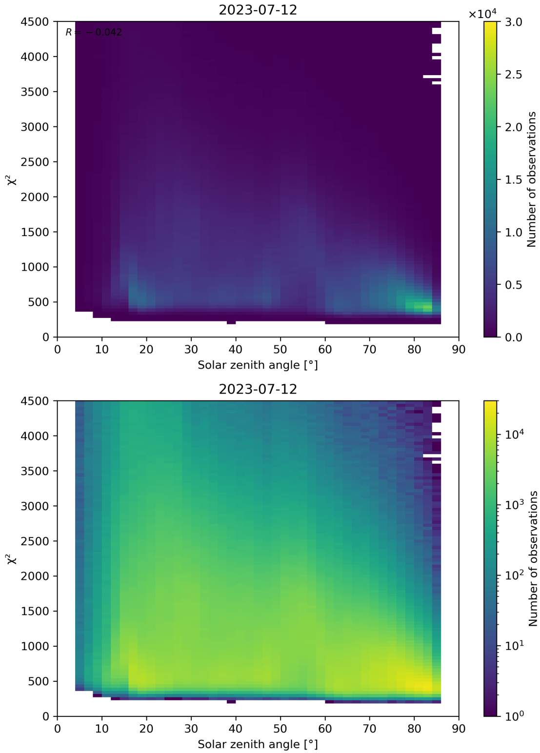
Figure 64: Scatter density plot of “Solar zenith angle” against “ \chi^2 ” for 2023-07-11 to 2023-07-13.
