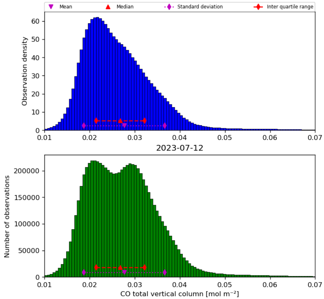
Figure 18: Histogram of “CO total vertical column” for 2023-07-11 to 2023-07-13
