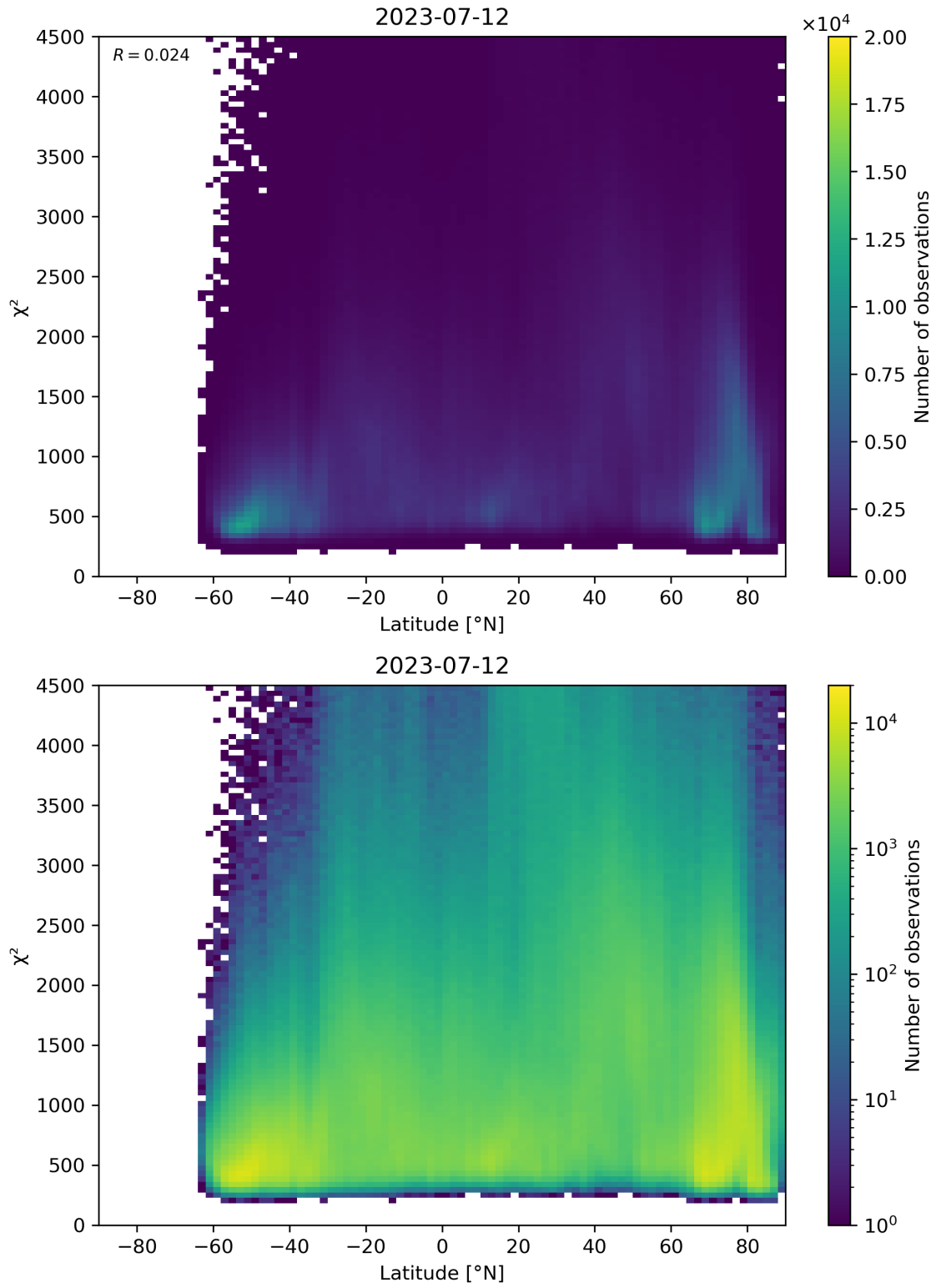
Figure 54: Scatter density plot of “Latitude” against “ \chi^2 ” for 2023-07-11 to 2023-07-13.
