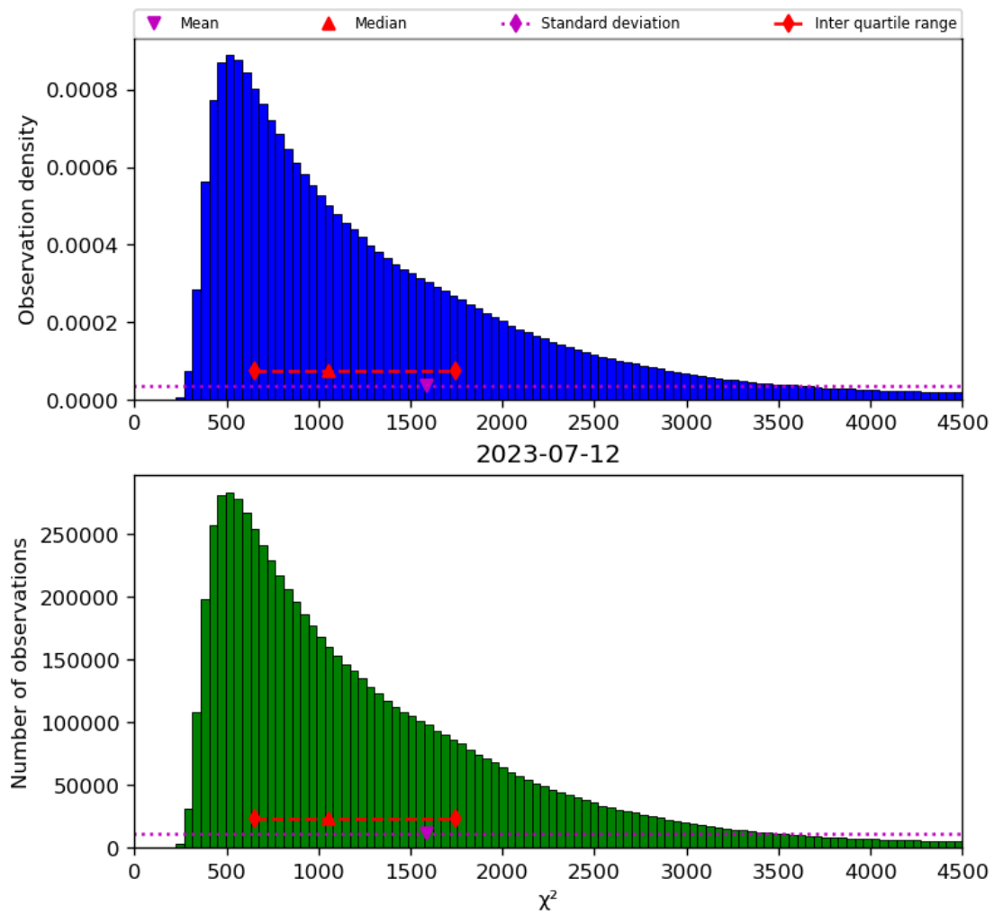
Figure 22: Histogram of “ \chi^2 ” for 2023-07-11 to 2023-07-13
