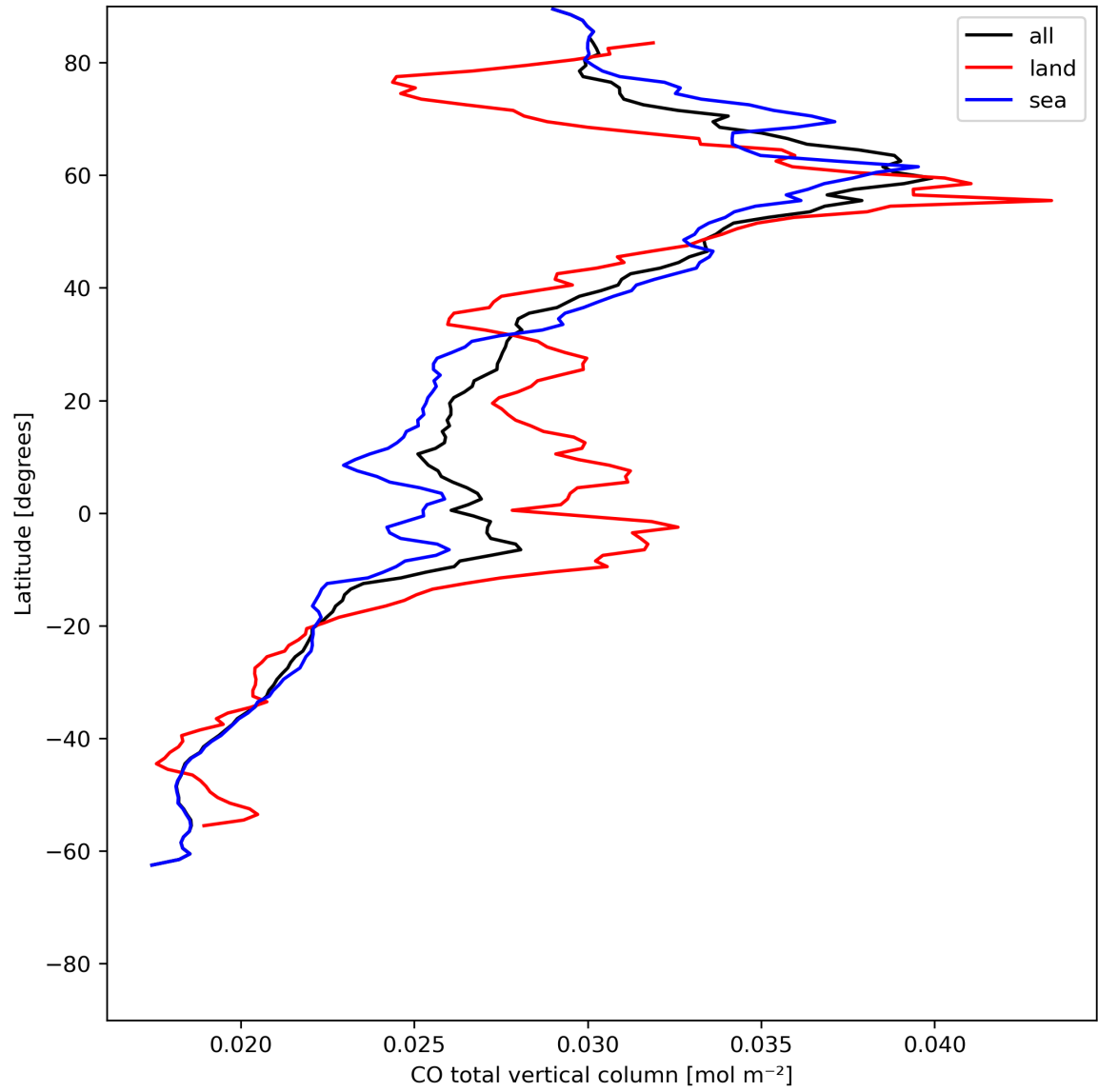
Figure 10: Zonal average of “CO total vertical column” for 2023-07-11 to 2023-07-13.
