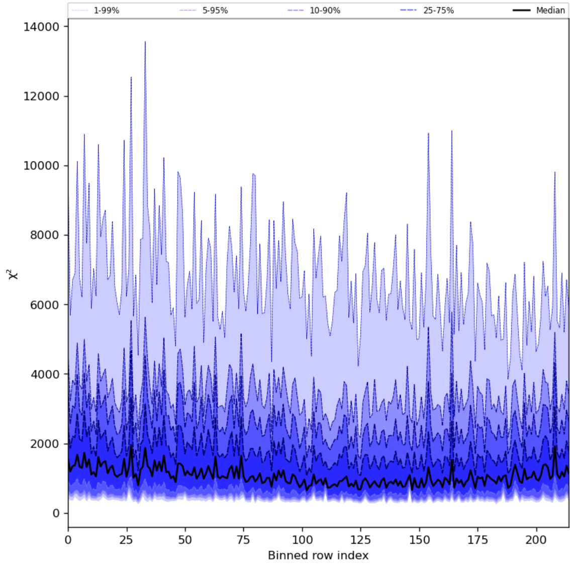
Figure 30: Along track statistics of “ \chi^2 ” for 2023-07-13 to 2023-07-14
