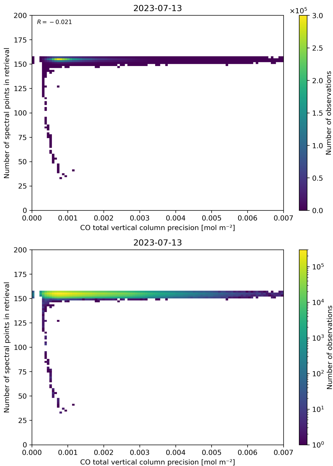
Figure 47: Scatter density plot of “CO total vertical column precision” against “Number of spectral points in retrieval” for 2023-07-13 to 2023-07-14.
