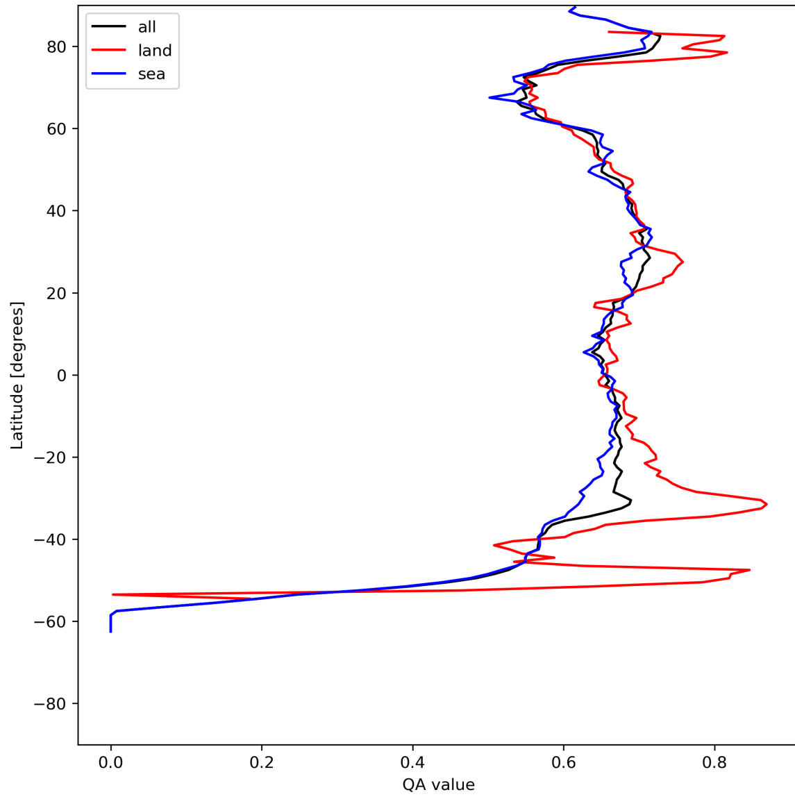
Figure 9: Zonal average of “QA value” for 2023-07-13 to 2023-07-14.
