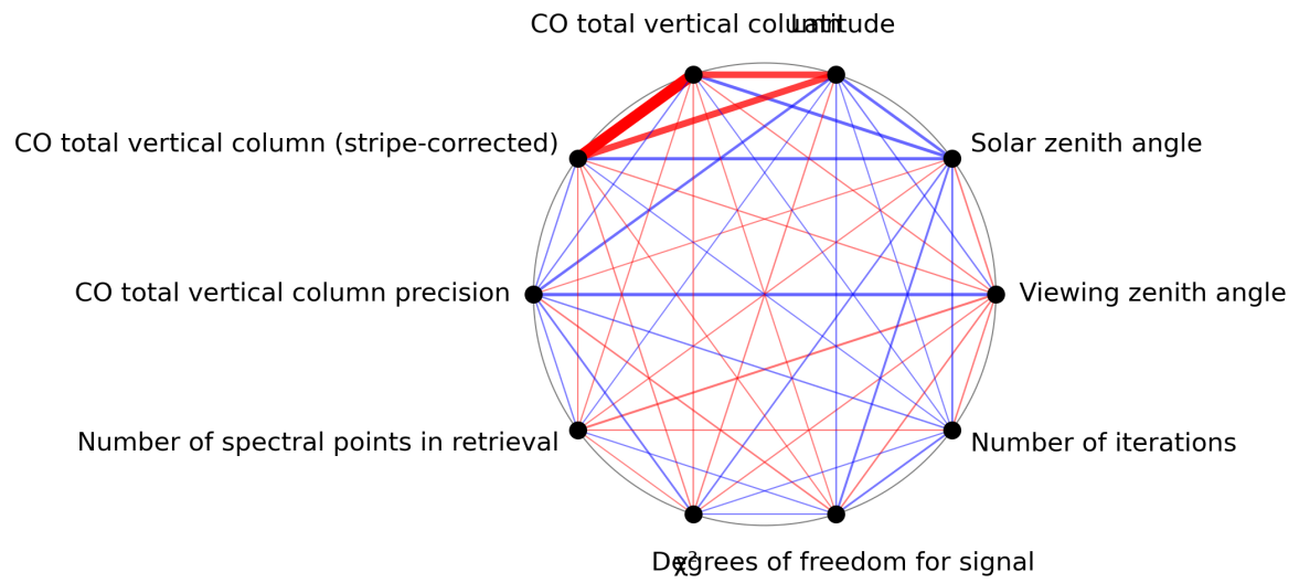
Figure 1: Map of correlation graph for 2023-07-13 to 2023-07-14.
