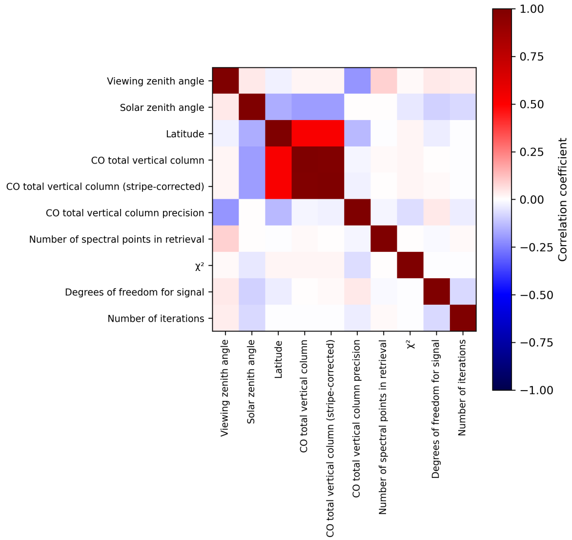
Figure 2: Map of correlation matrix for 2023-07-13 to 2023-07-14.
