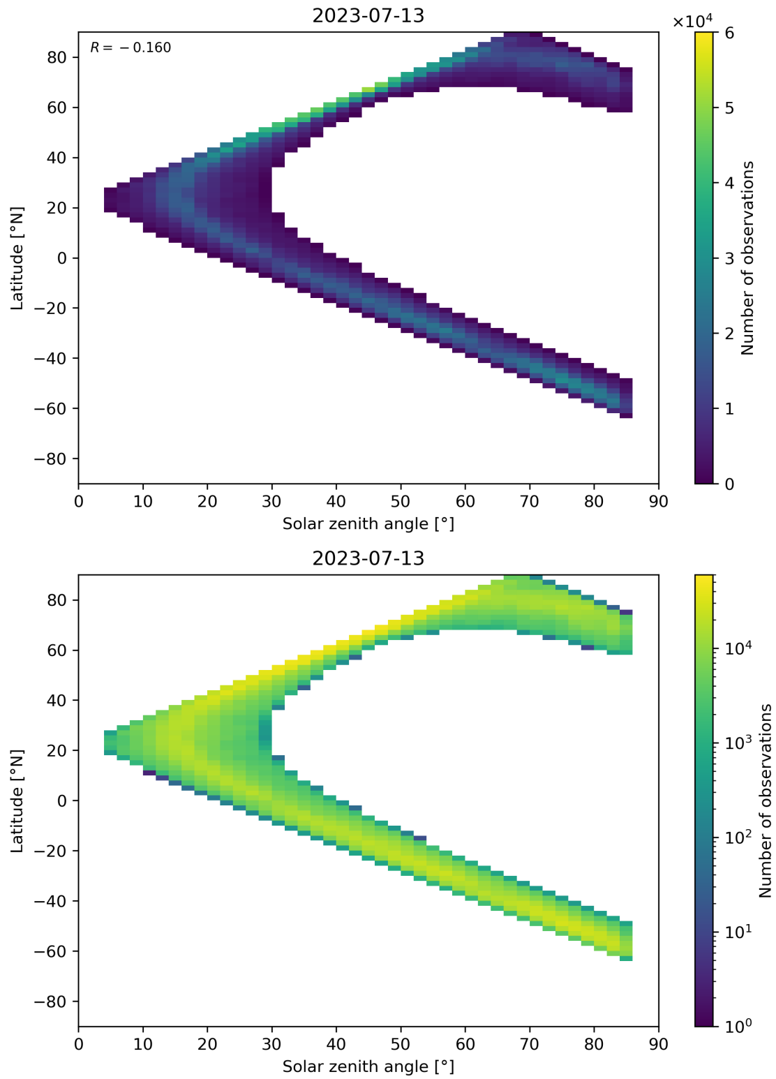
Figure 66: Scatter density plot of “Solar zenith angle” against “Latitude” for 2023-07-13 to 2023-07-14.
