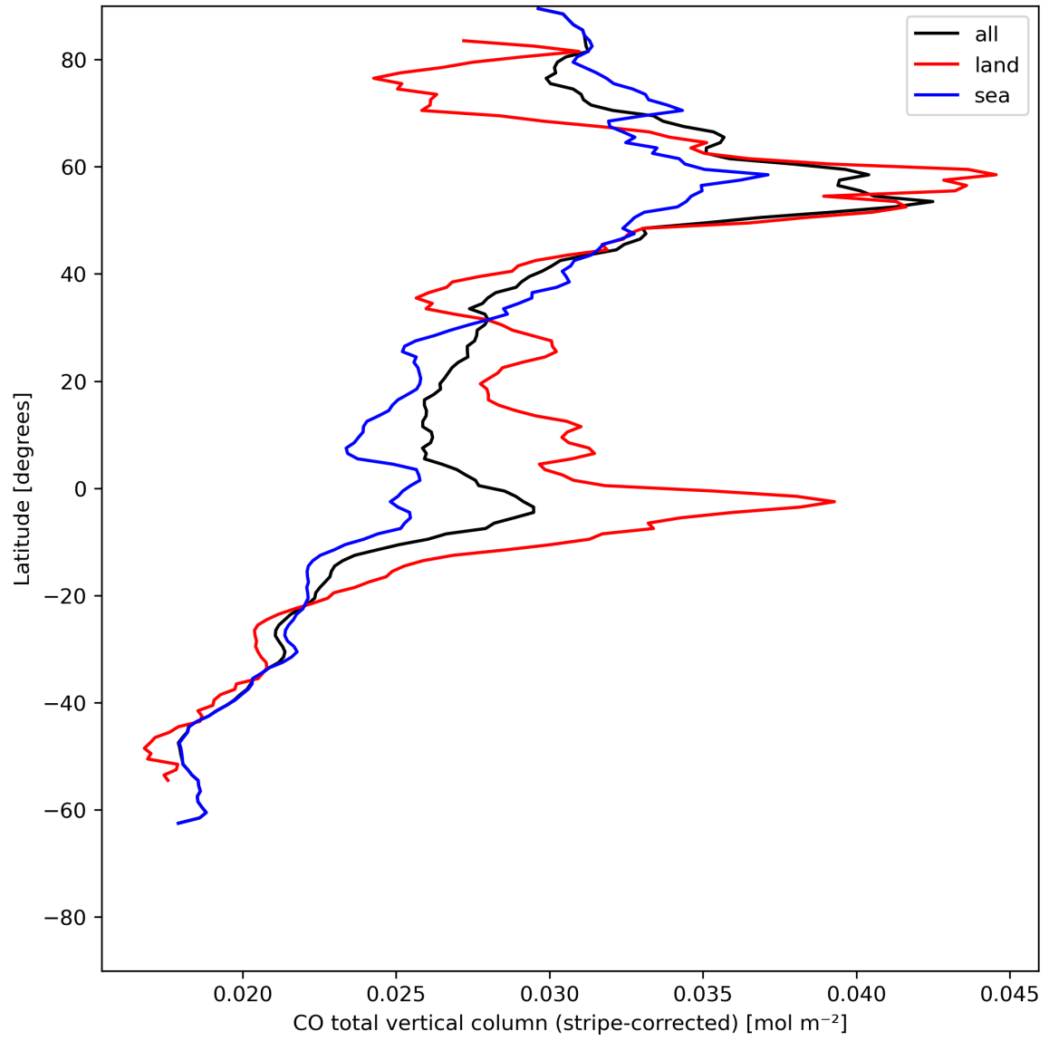
Figure 11: Zonal average of “CO total vertical column (stripe-corrected)” for 2023-07-13 to 2023-07-14.
