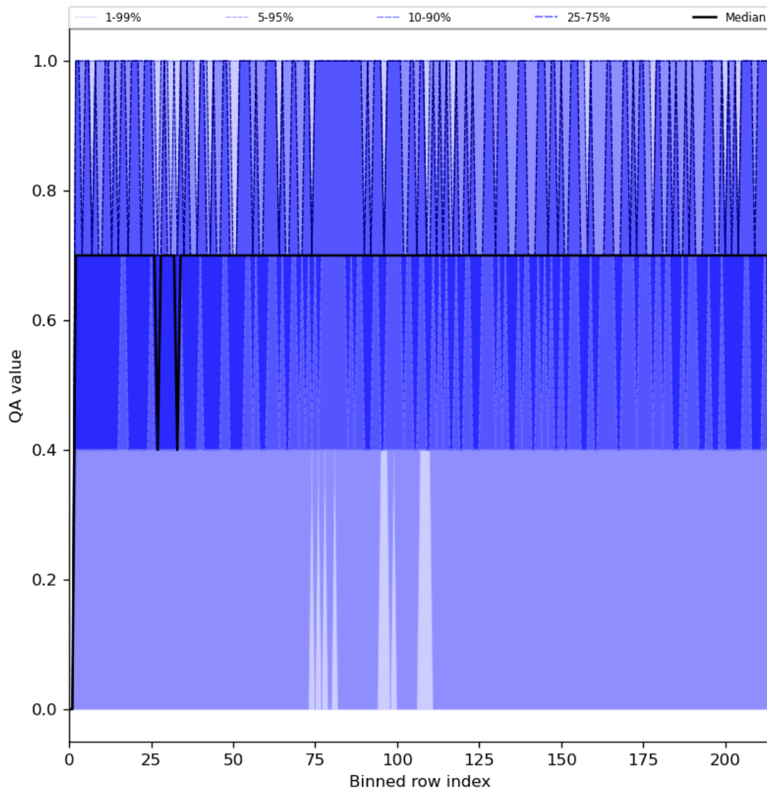
Figure 25: Along track statistics of “QA value” for 2023-07-13 to 2023-07-14
