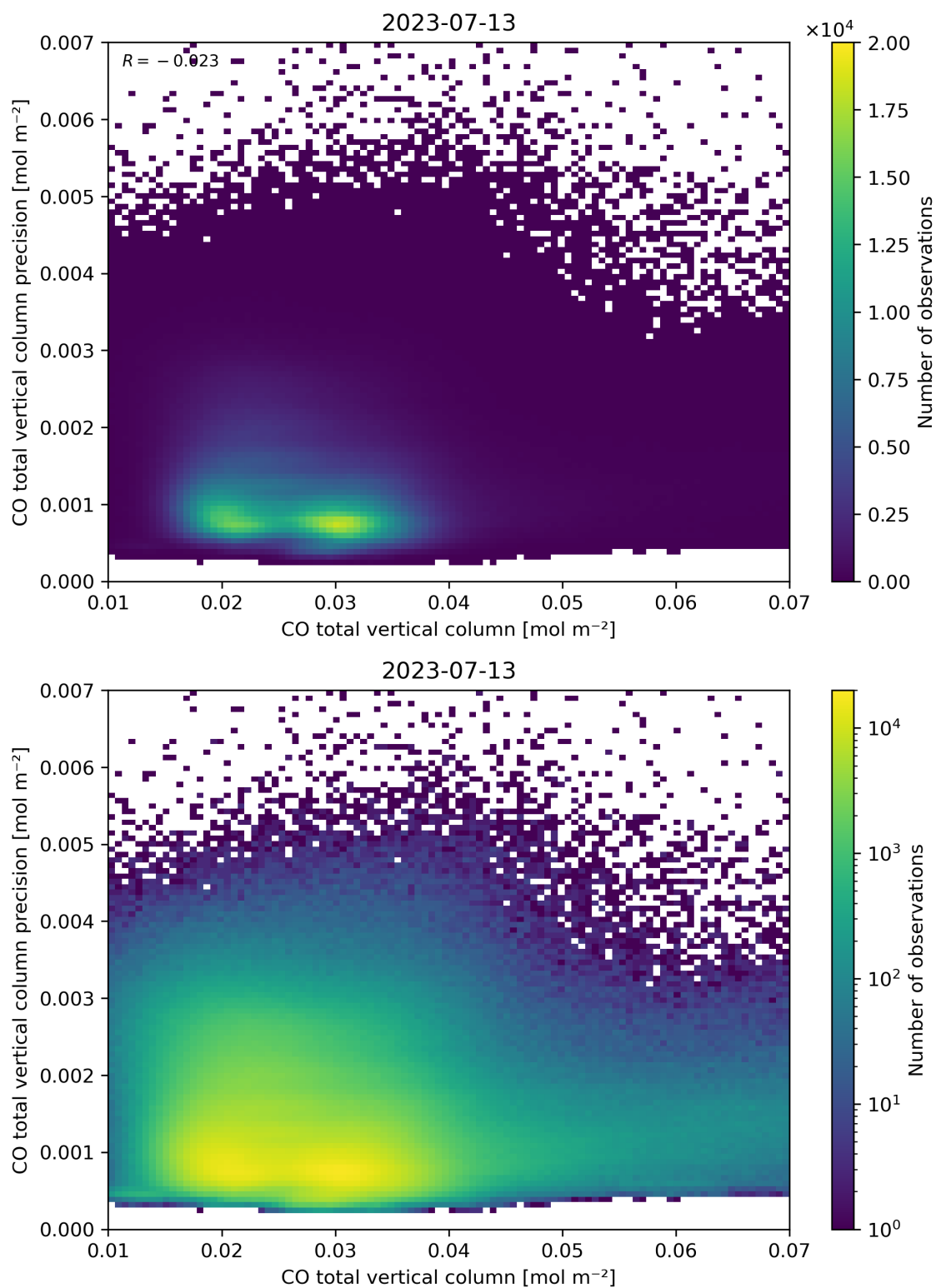
Figure 34: Scatter density plot of “CO total vertical column” against “CO total vertical column precision” for 2023-07-13 to 2023-07-14.
