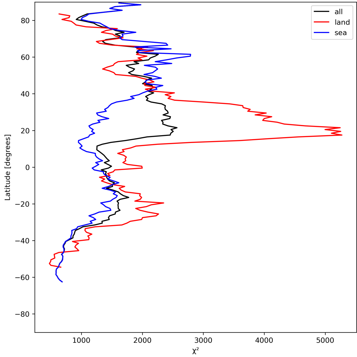
Figure 14: Zonal average of “ \chi^2 ” for 2023-07-13 to 2023-07-14.
