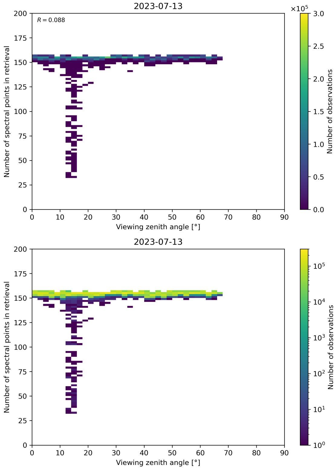
Figure 76: Scatter density plot of “Viewing zenith angle” against “Number of spectral points in retrieval” for 2023-07-13 to 2023-07-14.
