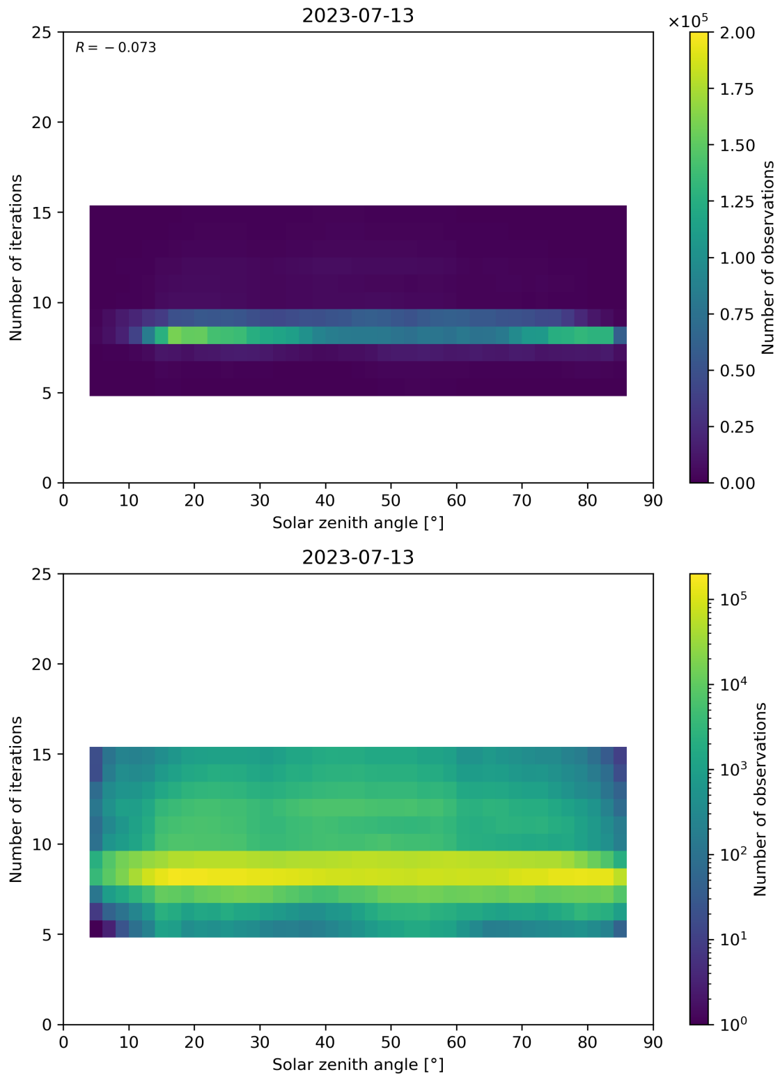
Figure 67: Scatter density plot of “Solar zenith angle” against “Number of iterations” for 2023-07-13 to 2023-07-14.
