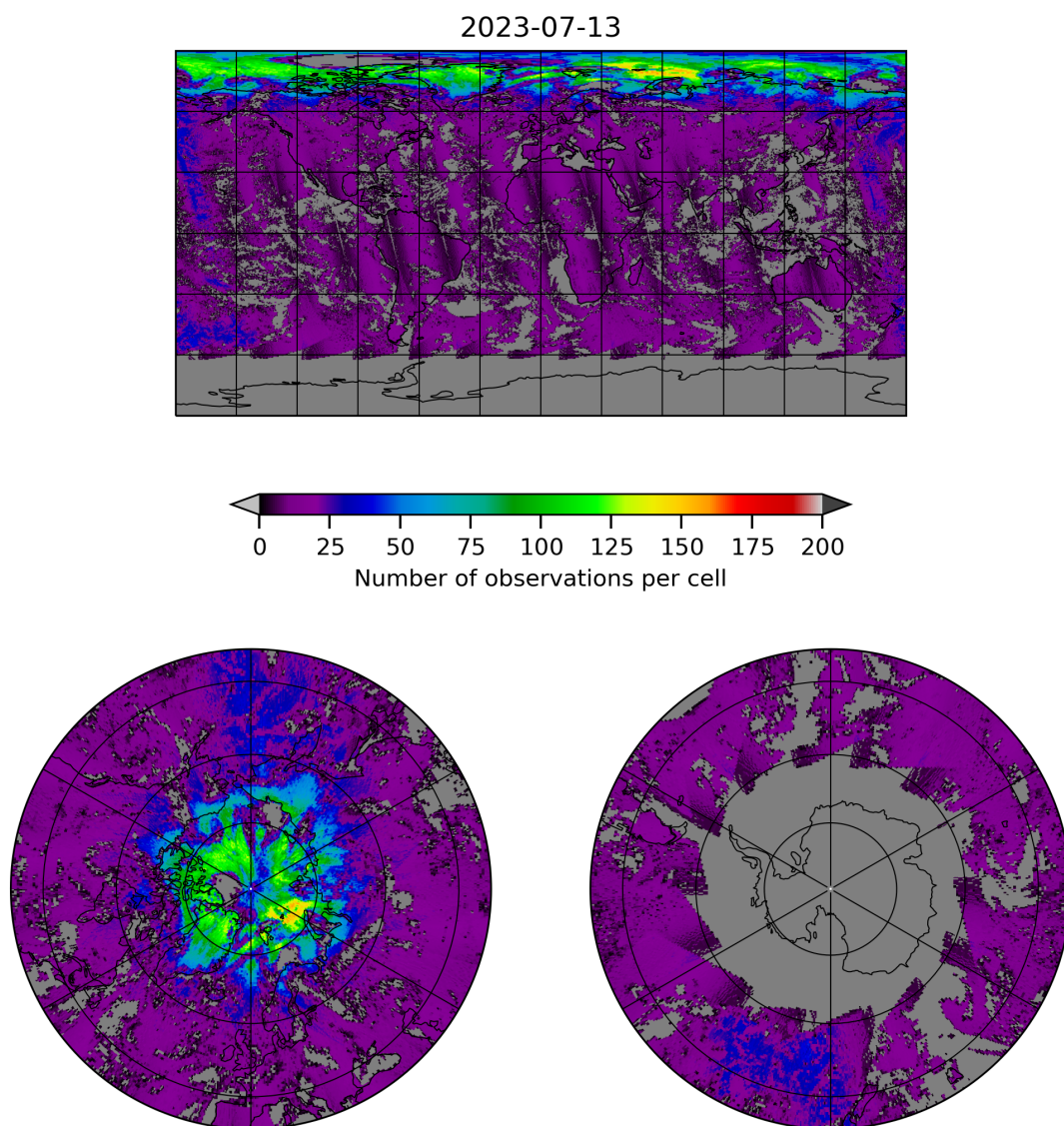
Figure 8: Map of the number of observations for 2023-07-13 to 2023-07-14
