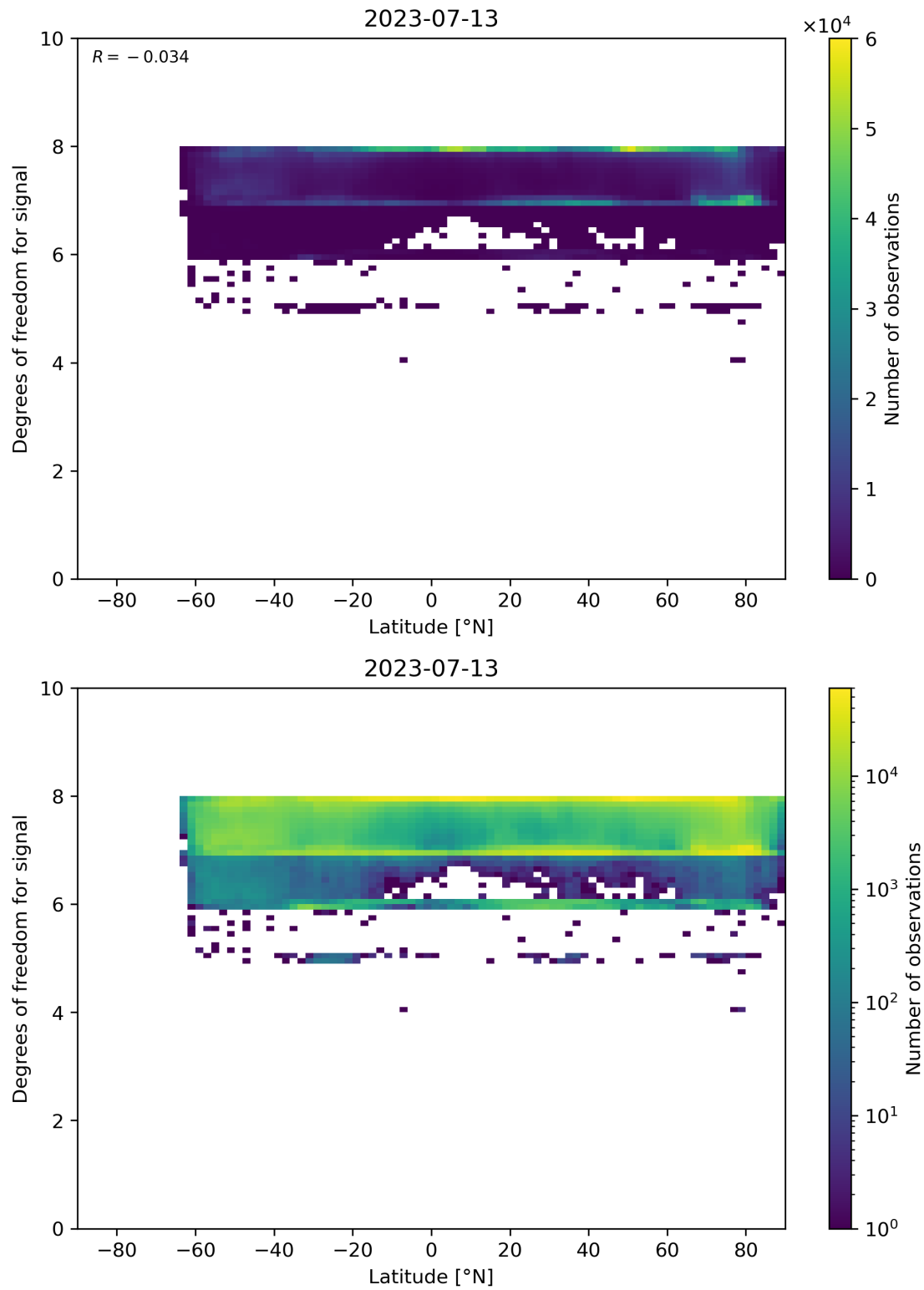
Figure 55: Scatter density plot of “Latitude” against “Degrees of freedom for signal” for 2023-07-13 to 2023-07-14.
