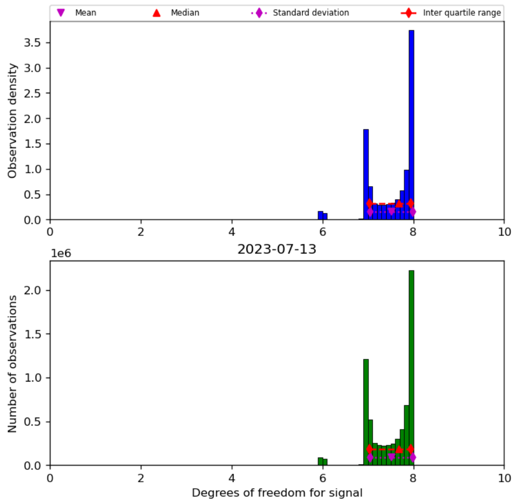
Figure 23: Histogram of “Degrees of freedom for signal” for 2023-07-13 to 2023-07-14
