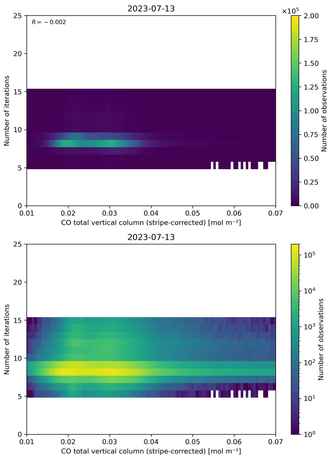
Figure 39: Scatter density plot of “CO total vertical column (stripe-corrected)” against “Number of iterations” for 2023-07-13 to 2023-07-14.
