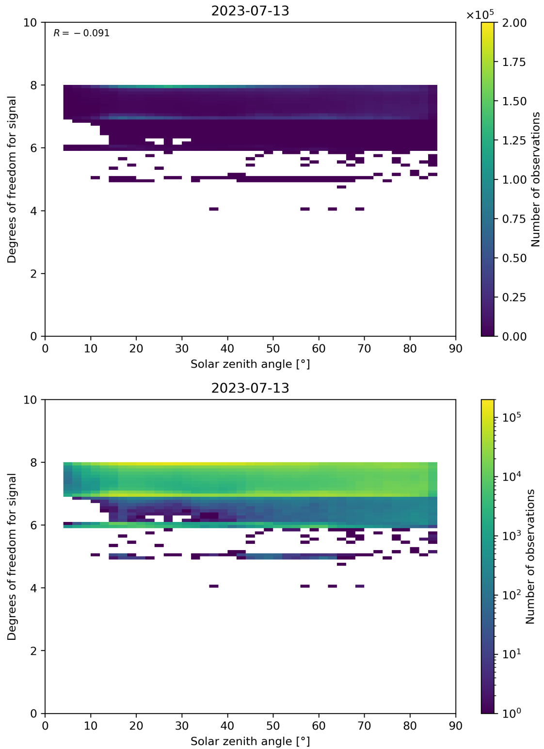
Figure 65: Scatter density plot of “Solar zenith angle” against “Degrees of freedom for signal” for 2023-07-13 to 2023-07-14.
