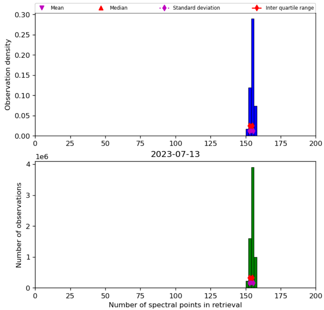
Figure 21: Histogram of “Number of spectral points in retrieval” for 2023-07-13 to 2023-07-14
