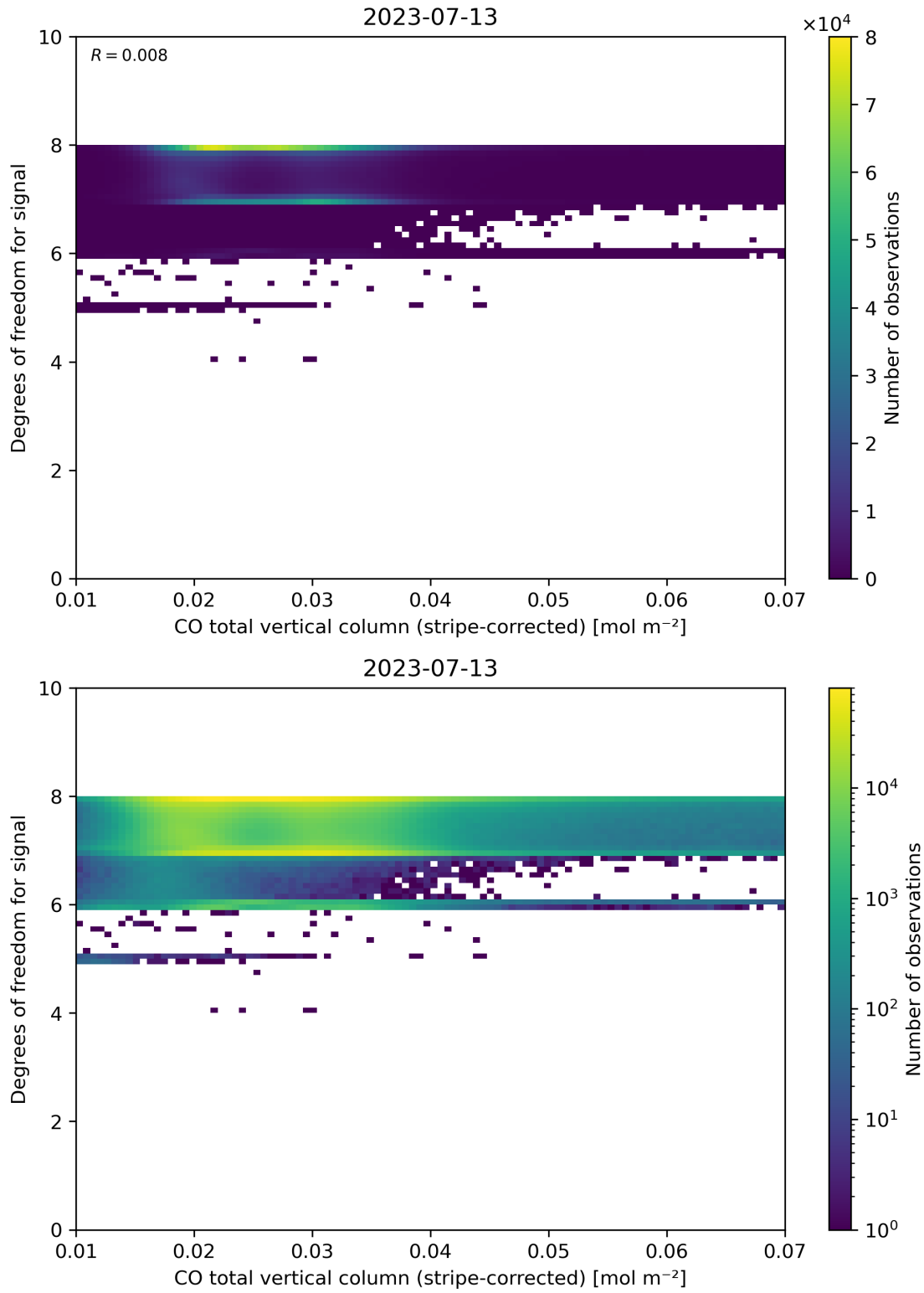
Figure 38: Scatter density plot of “CO total vertical column (stripe-corrected)” against “Degrees of freedom for signal” for 2023-07-13 to 2023-07-14.
