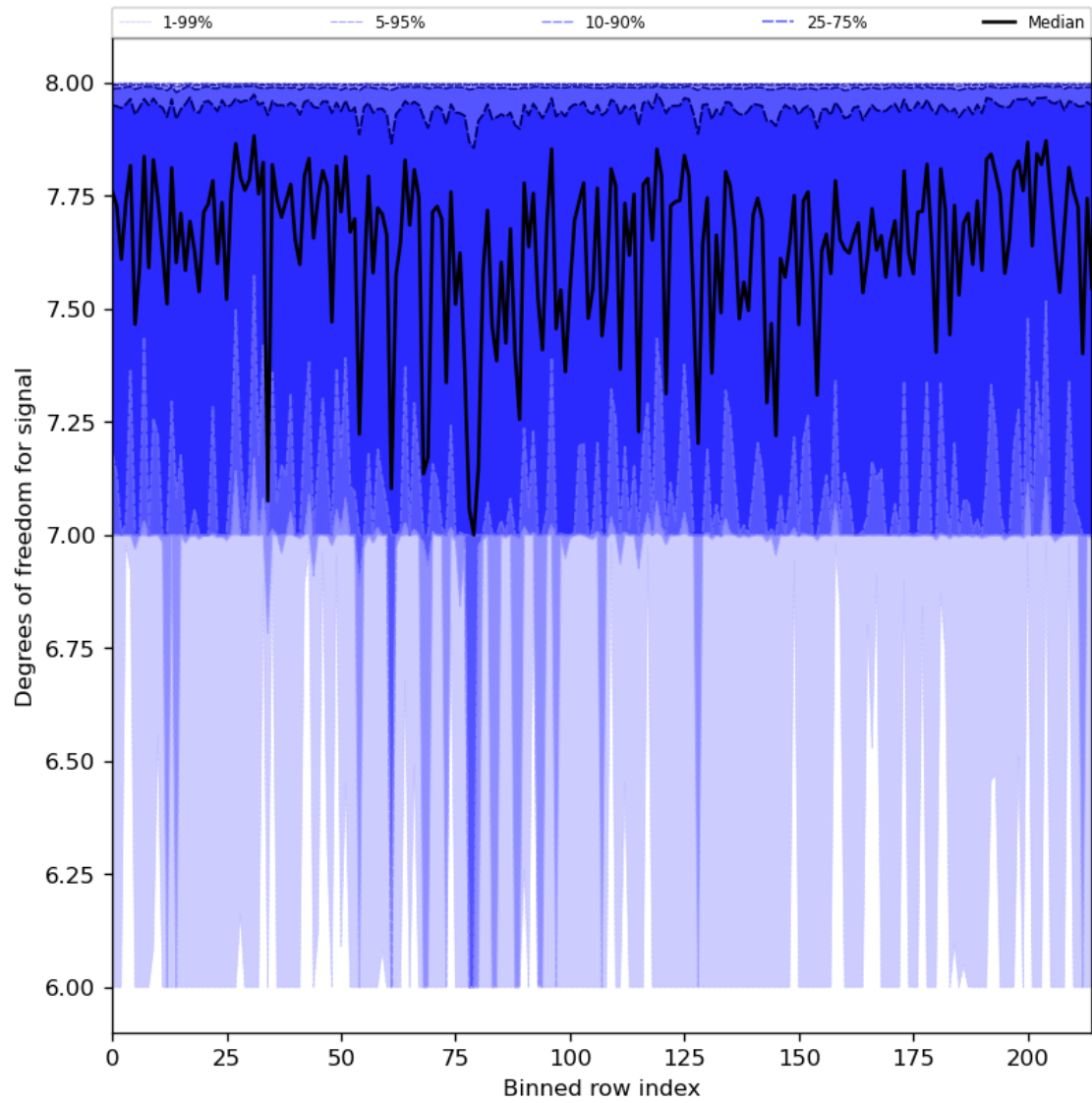
Figure 31: Along track statistics of “Degrees of freedom for signal” for 2023-07-13 to 2023-07-14
