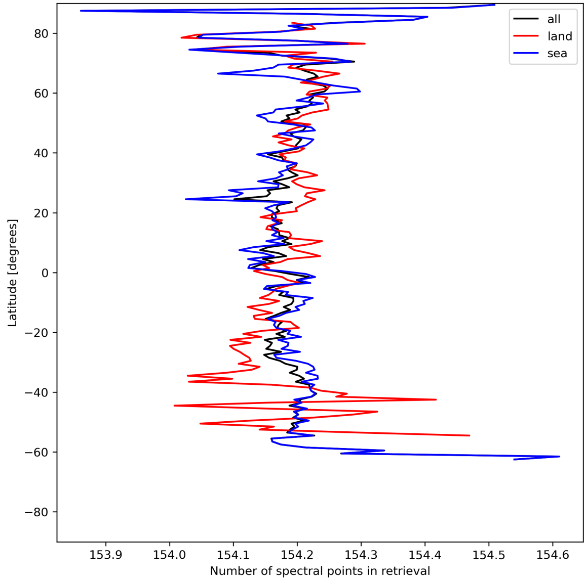
Figure 13: Zonal average of “Number of spectral points in retrieval” for 2023-07-13 to 2023-07-14.
