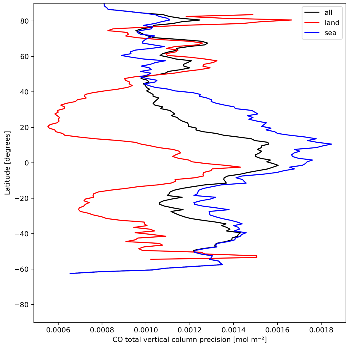
Figure 12: Zonal average of “CO total vertical column precision” for 2023-07-13 to 2023-07-14.
