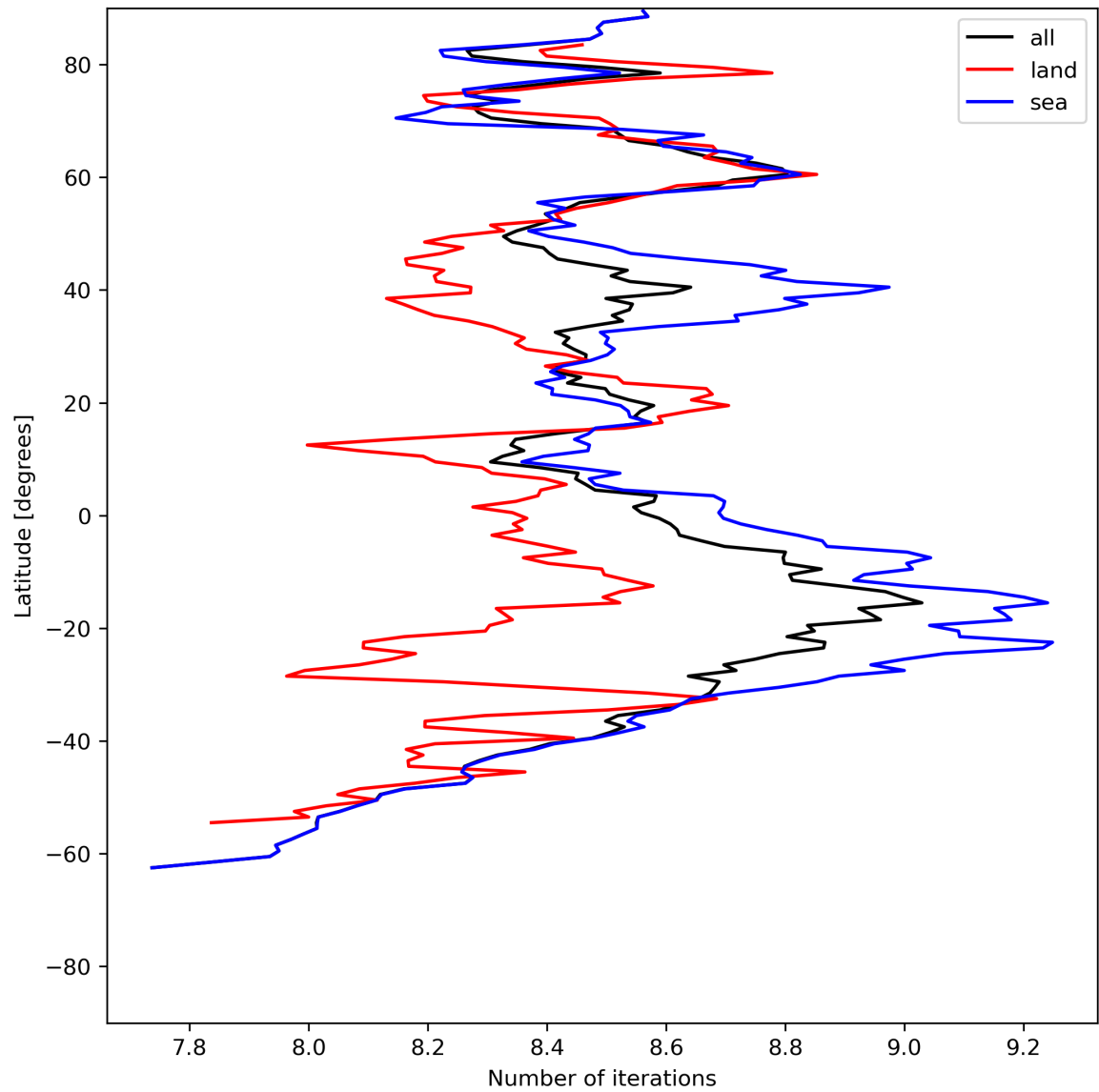
Figure 16: Zonal average of “Number of iterations” for 2023-07-13 to 2023-07-14.
