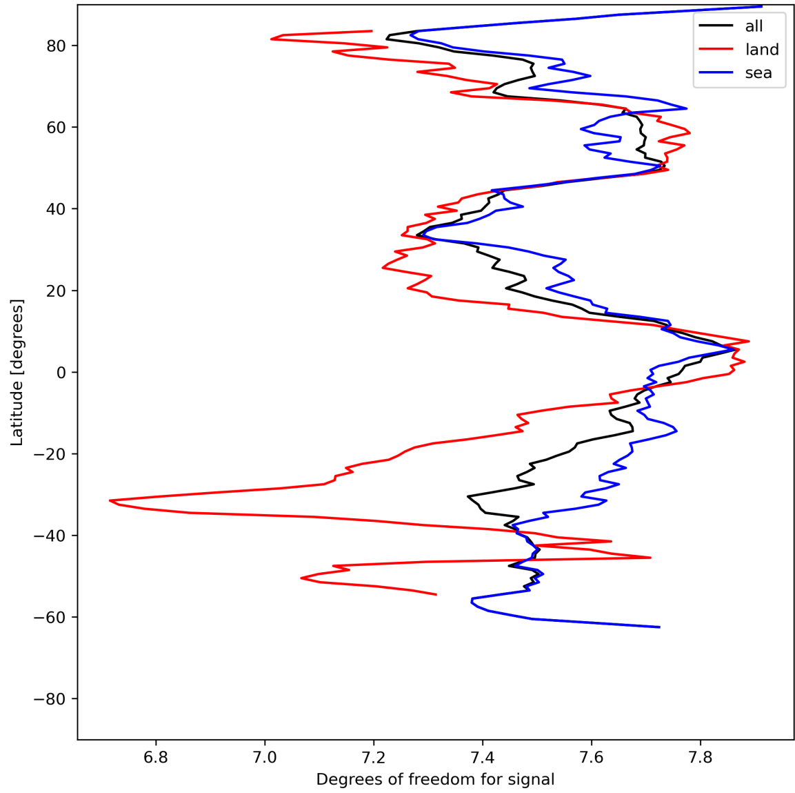
Figure 15: Zonal average of “Degrees of freedom for signal” for 2023-07-13 to 2023-07-14.
