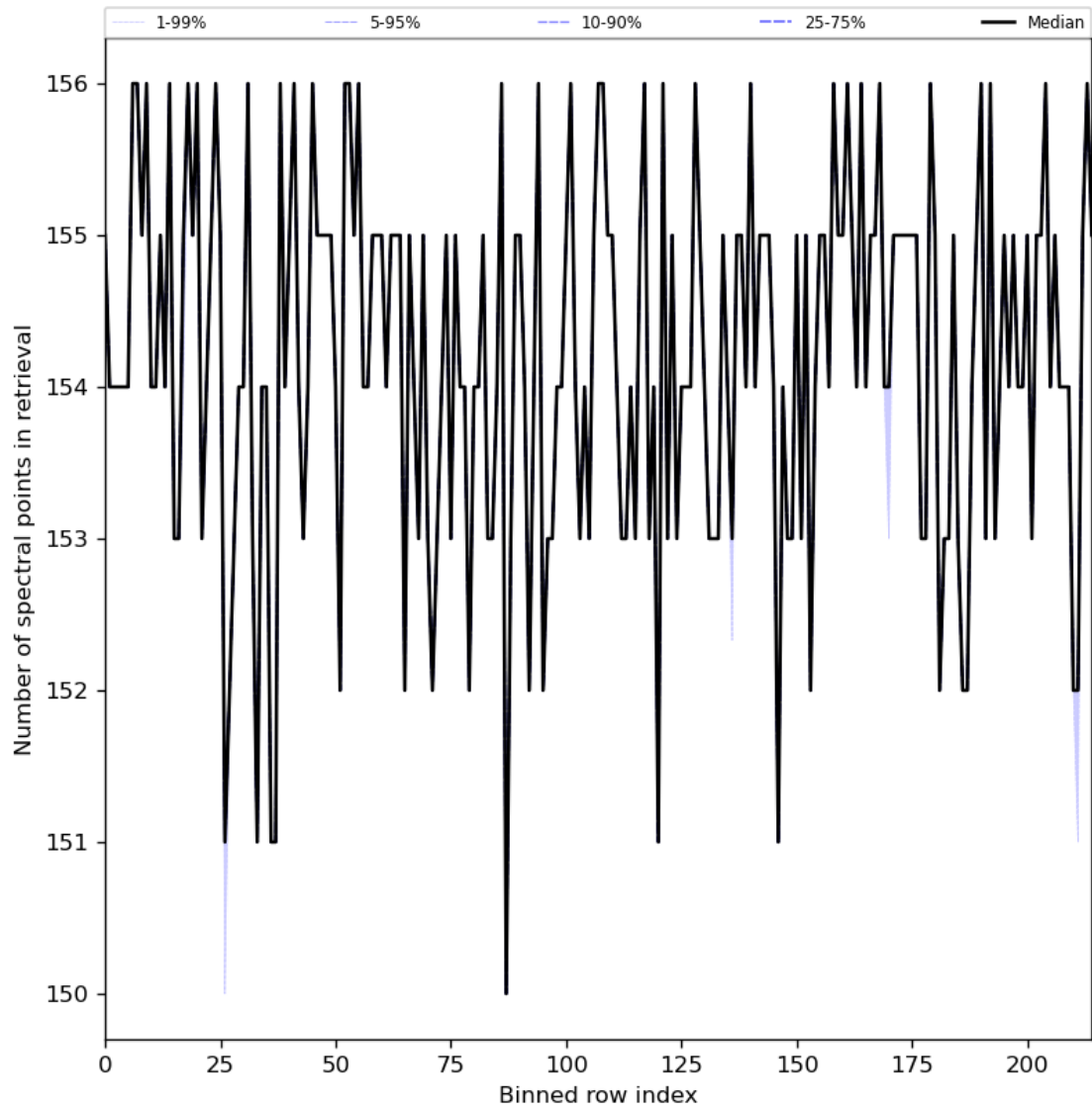
Figure 29: Along track statistics of “Number of spectral points in retrieval” for 2023-07-13 to 2023-07-14
