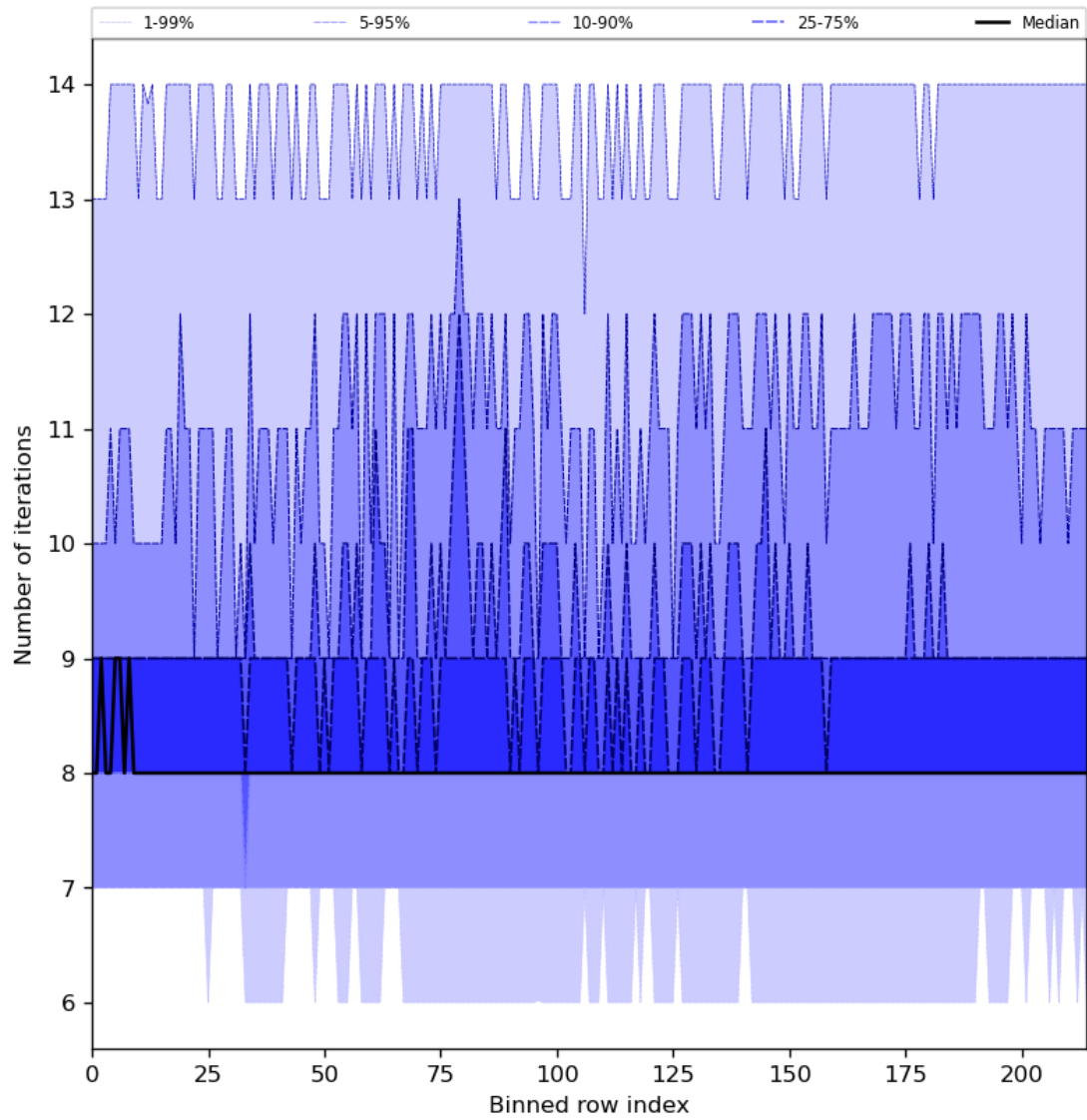
Figure 32: Along track statistics of “Number of iterations” for 2023-07-13 to 2023-07-14
