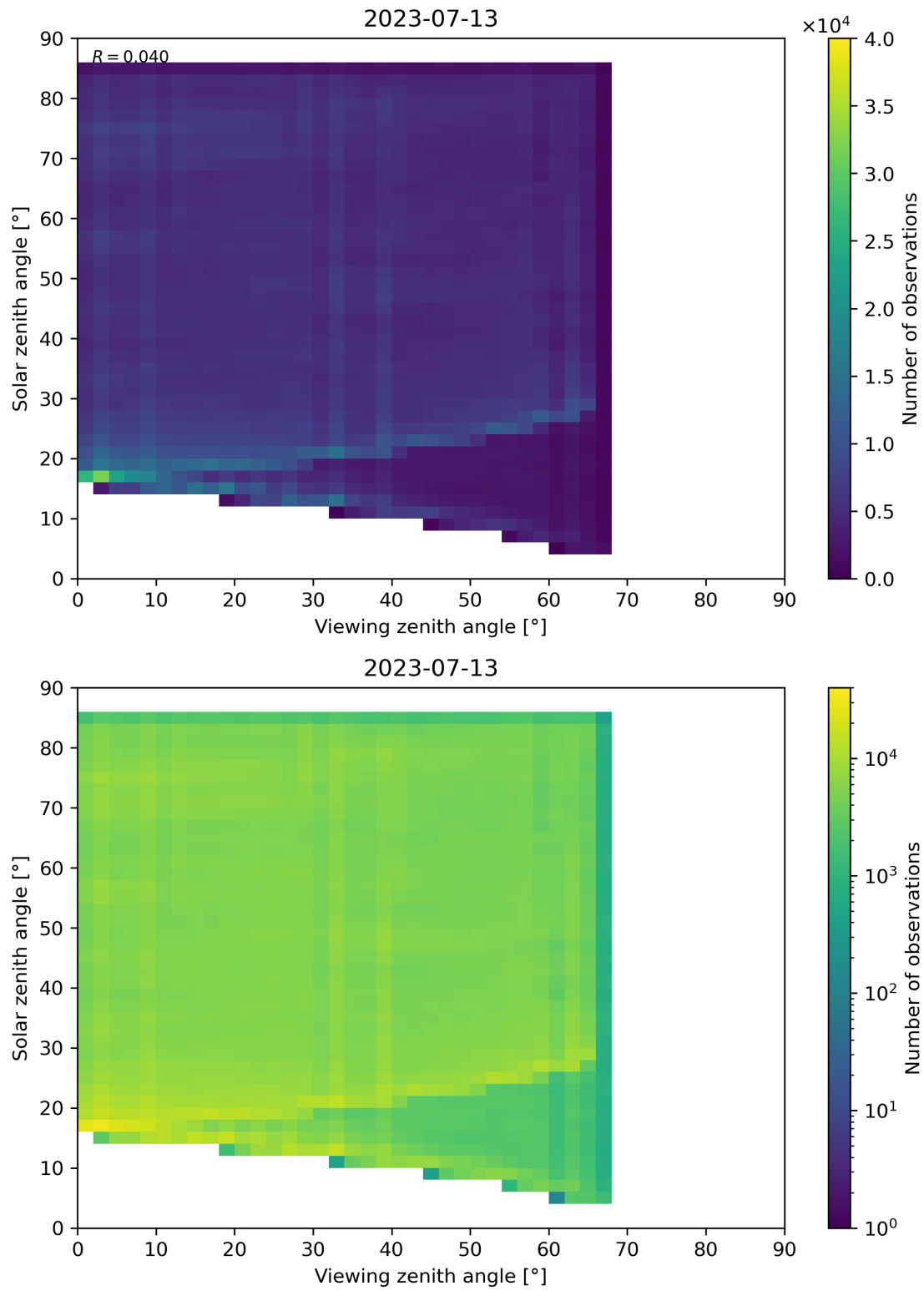
Figure 77: Scatter density plot of “Viewing zenith angle” against “Solar zenith angle” for 2023-07-13 to 2023-07-14.
