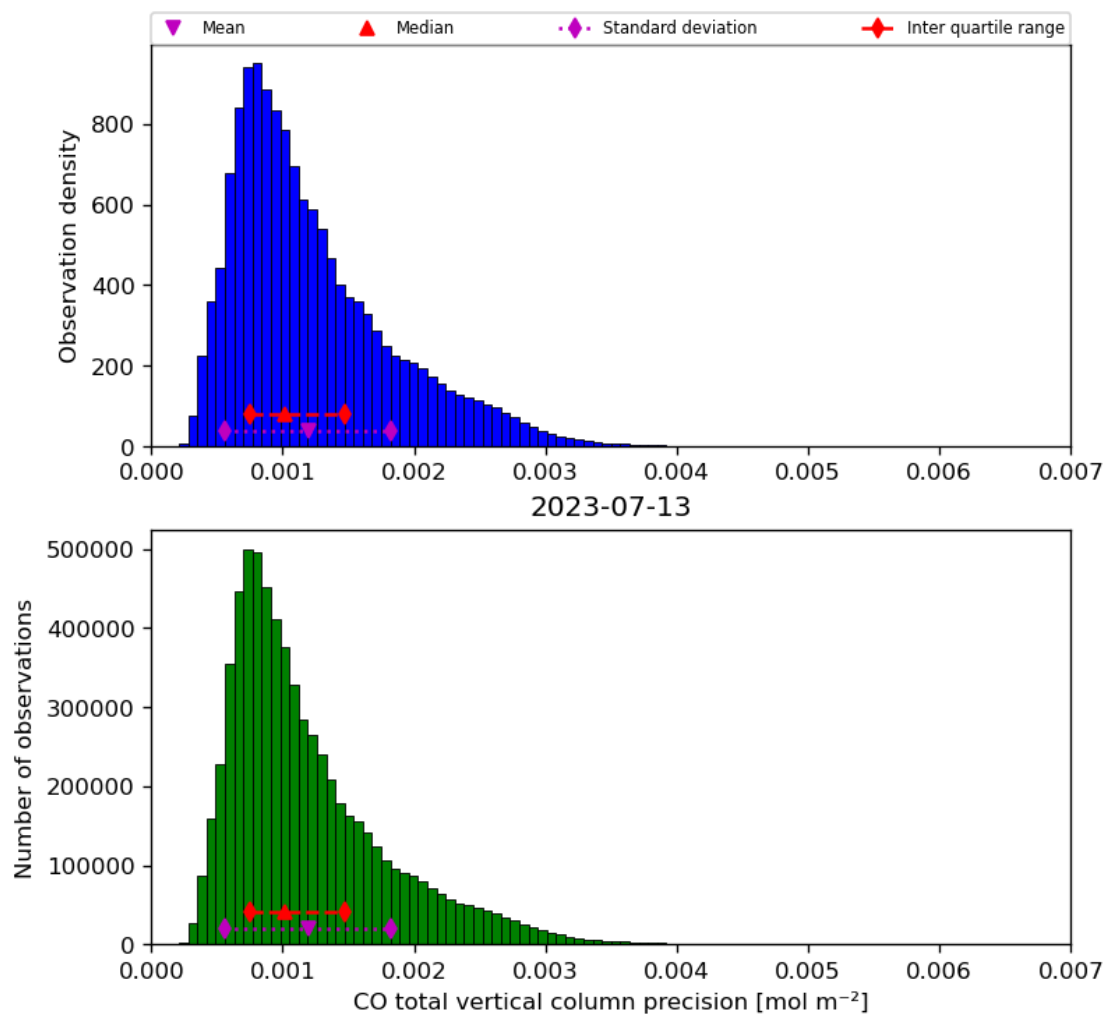
Figure 20: Histogram of “CO total vertical column precision” for 2023-07-13 to 2023-07-14
