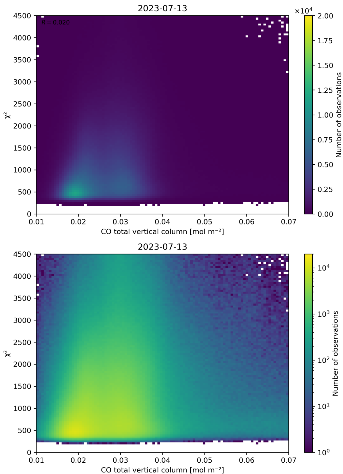
Figure 35: Scatter density plot of “CO total vertical column” against “ \chi^2 ” for 2023-07-13 to 2023-07-14.
