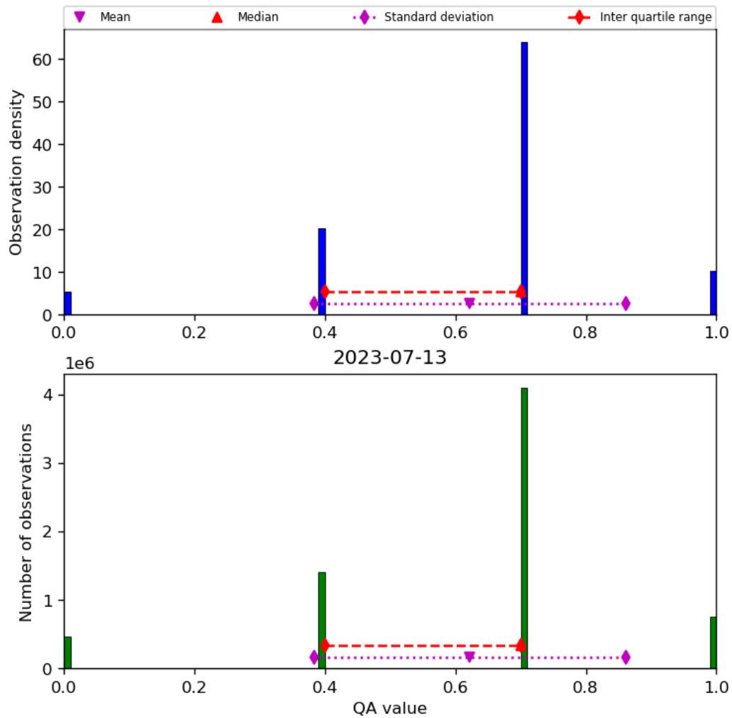
Figure 17: Histogram of “QA value” for 2023-07-13 to 2023-07-14
