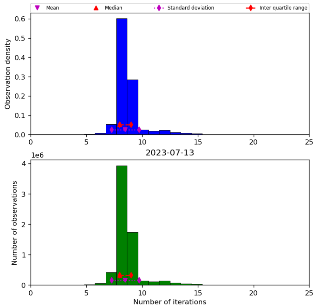
Figure 24: Histogram of “Number of iterations” for 2023-07-13 to 2023-07-14
