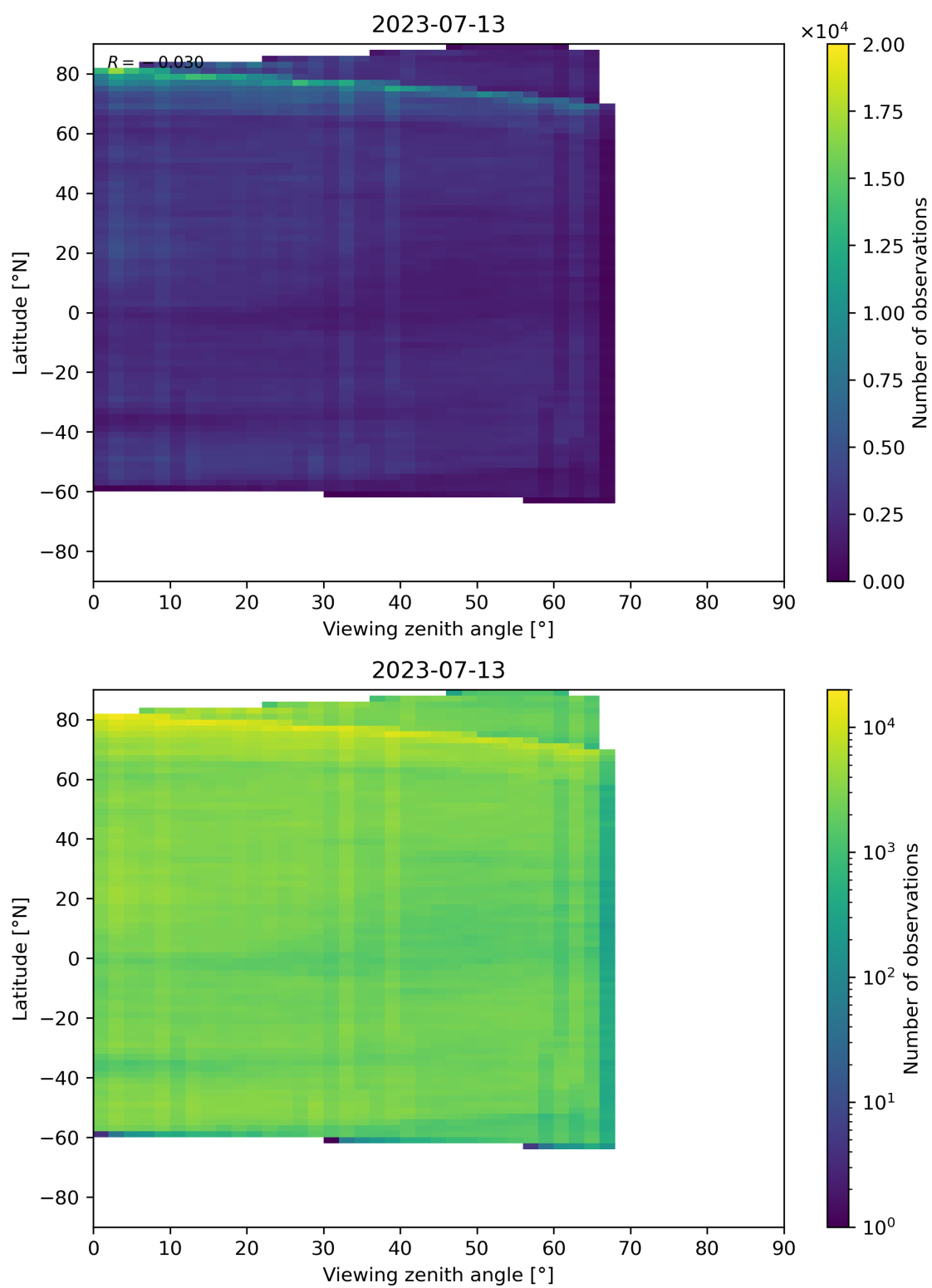
Figure 74: Scatter density plot of “Viewing zenith angle” against “Latitude” for 2023-07-13 to 2023-07-14.
