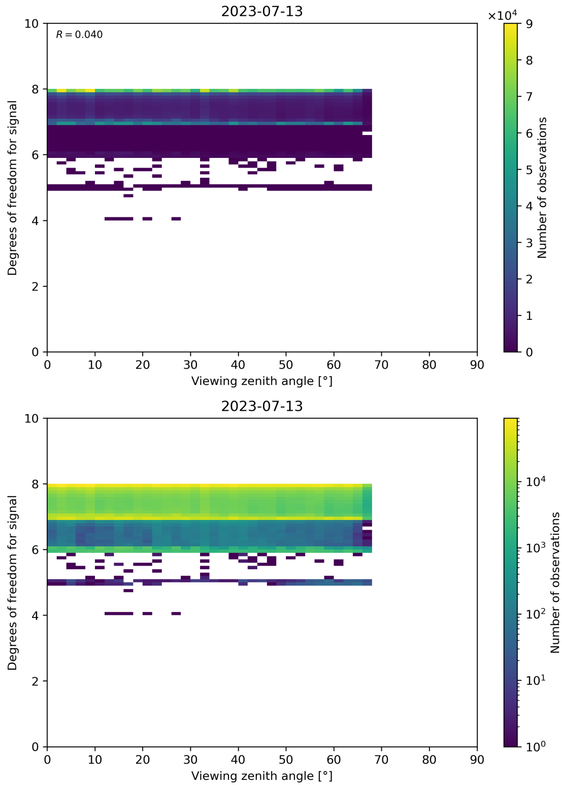
Figure 73: Scatter density plot of “Viewing zenith angle” against “Degrees of freedom for signal” for 2023-07-13 to 2023-07-14.
