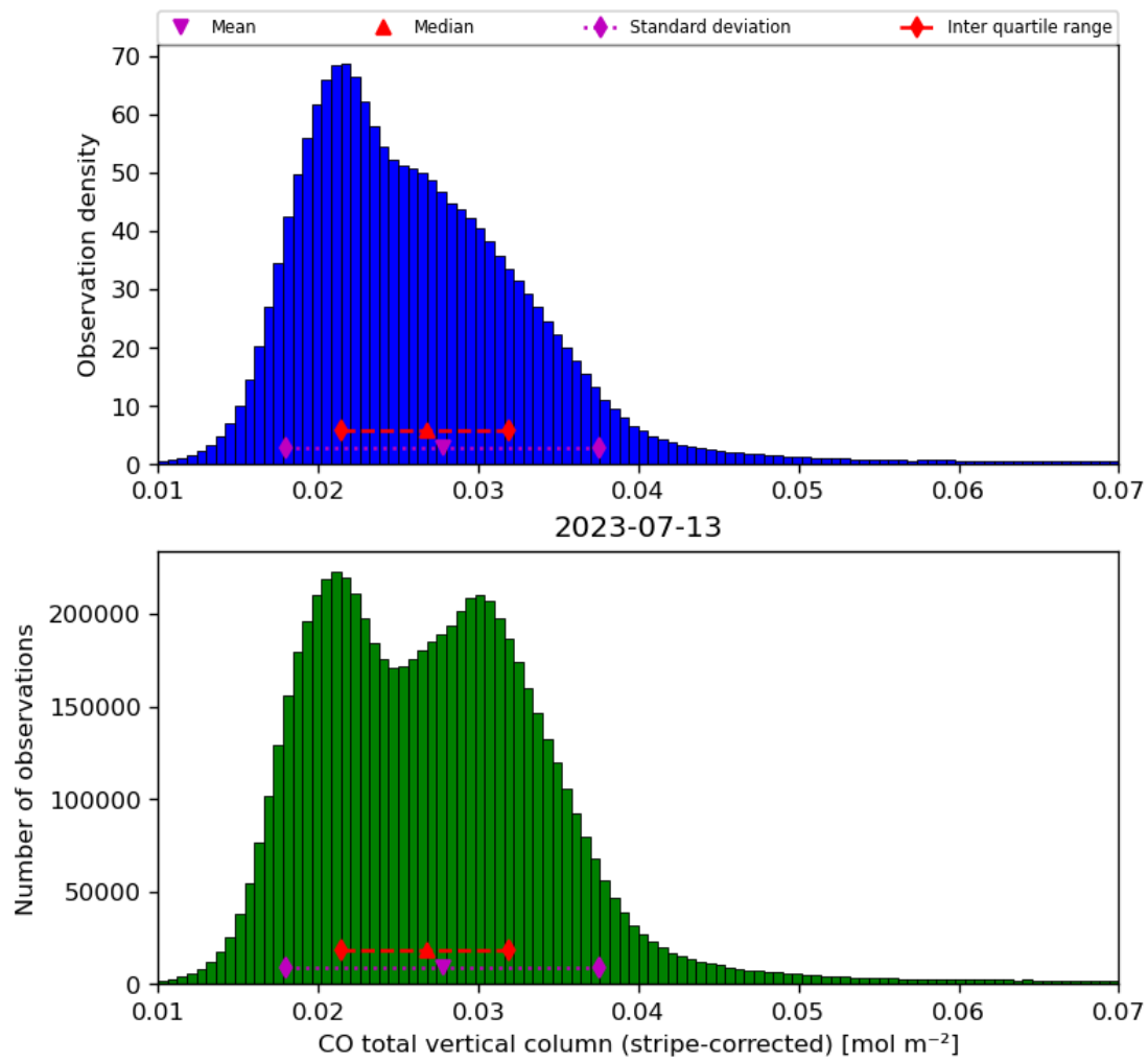
Figure 19: Histogram of “CO total vertical column (stripe-corrected)” for 2023-07-13 to 2023-07-14
