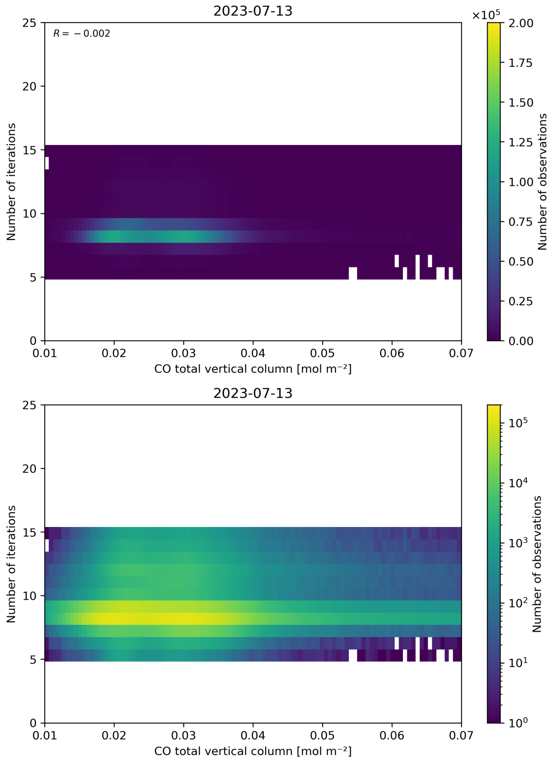
Figure 42: Scatter density plot of “CO total vertical column” against “Number of iterations” for 2023-07-13 to 2023-07-14.
