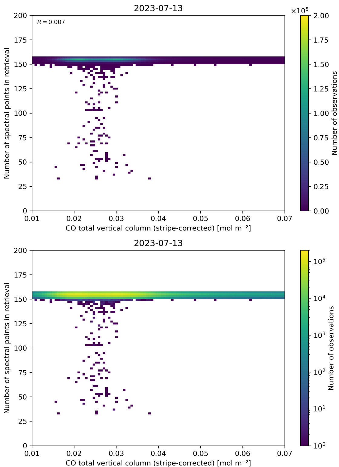
Figure 40: Scatter density plot of “CO total vertical column (stripe-corrected)” against “Number of spectral points in retrieval” for 2023-07-13 to 2023-07-14.
