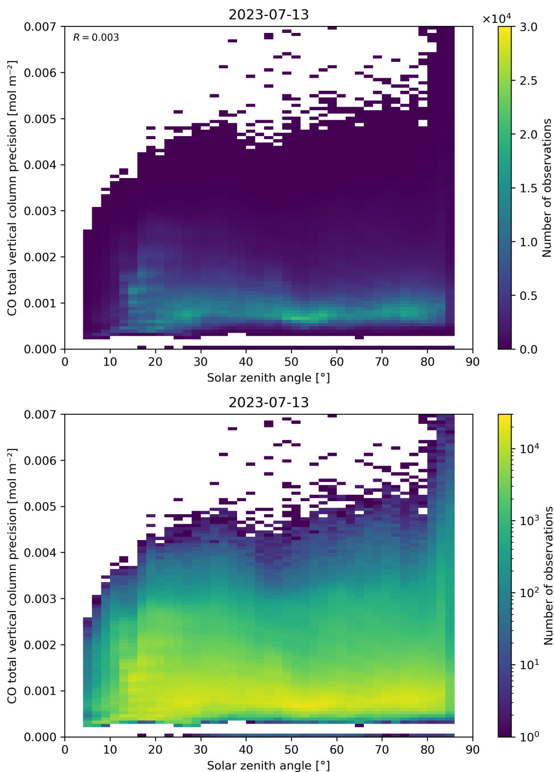
Figure 63: Scatter density plot of “Solar zenith angle” against “CO total vertical column precision” for 2023-07-13 to 2023-07-14.
