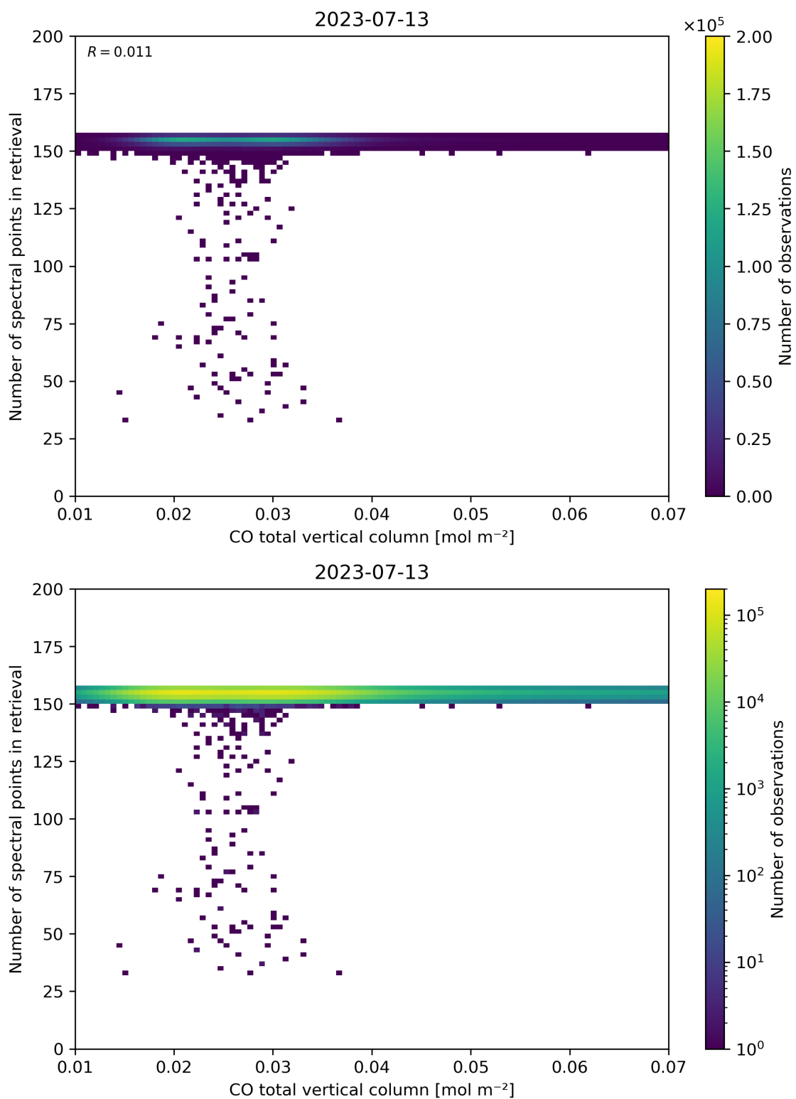
Figure 43: Scatter density plot of “CO total vertical column” against “Number of spectral points in retrieval” for 2023-07-13 to 2023-07-14.
