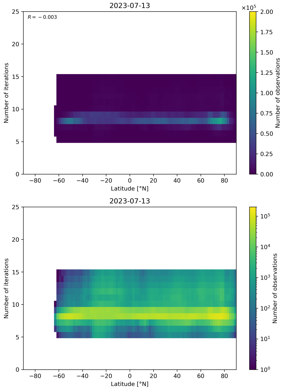
Figure 56: Scatter density plot of “Latitude” against “Number of iterations” for 2023-07-13 to 2023-07-14.
