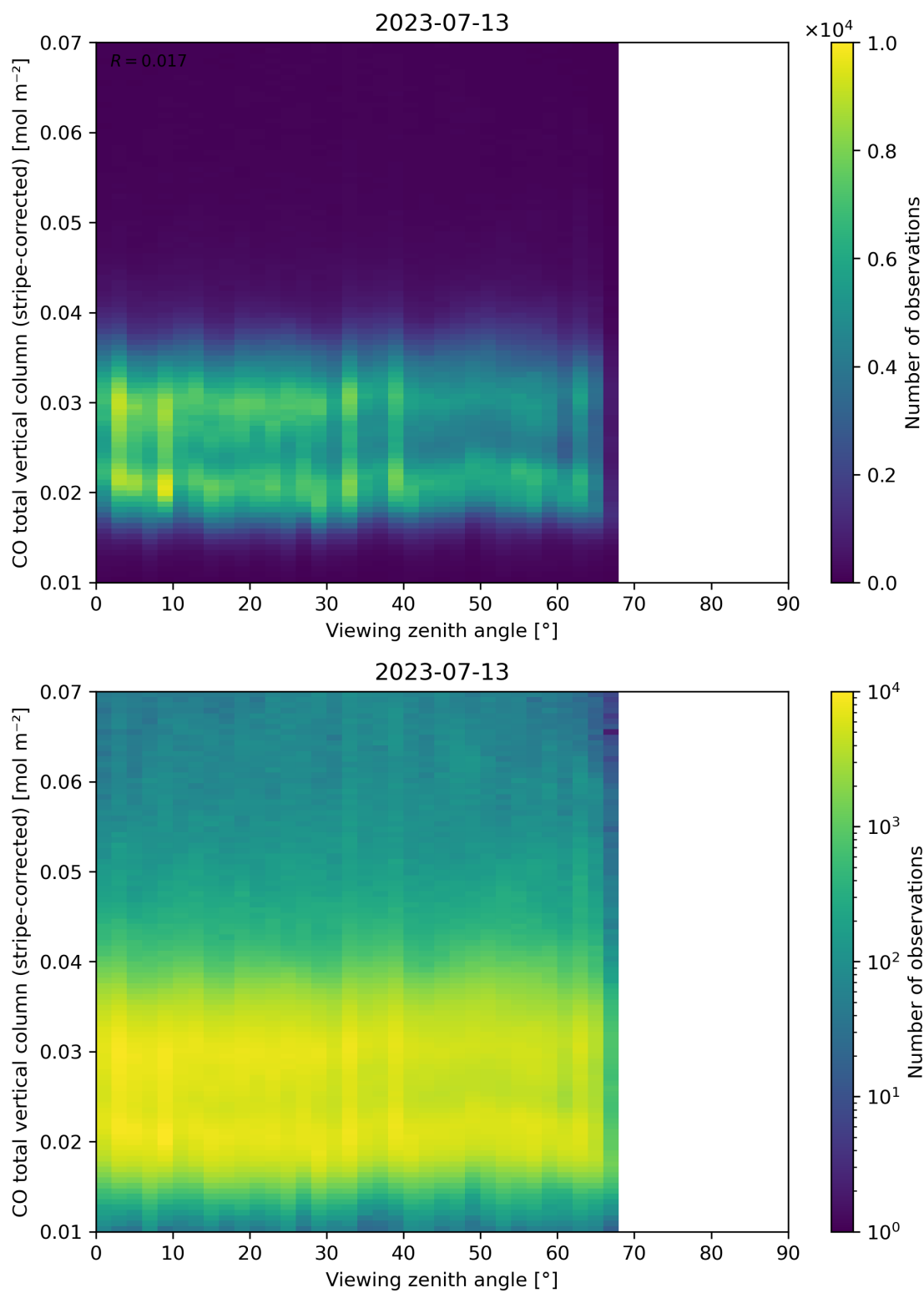
Figure 70: Scatter density plot of “Viewing zenith angle” against “CO total vertical column (stripe-corrected)” for 2023-07-13 to 2023-07-14.
