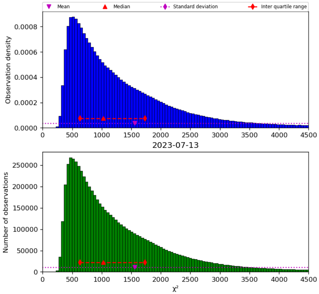
Figure 22: Histogram of “ \chi^2 ” for 2023-07-13 to 2023-07-14
