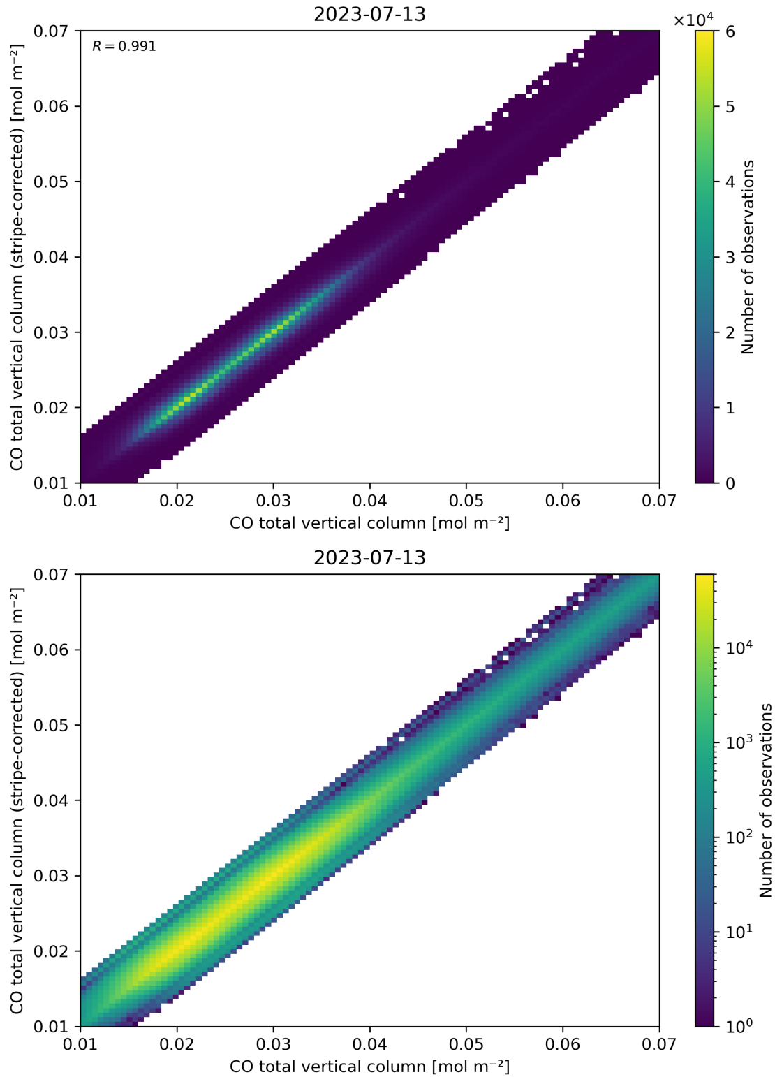
Figure 33: Scatter density plot of “CO total vertical column” against “CO total vertical column (stripe-corrected)” for 2023-07-13 to 2023-07-14.
