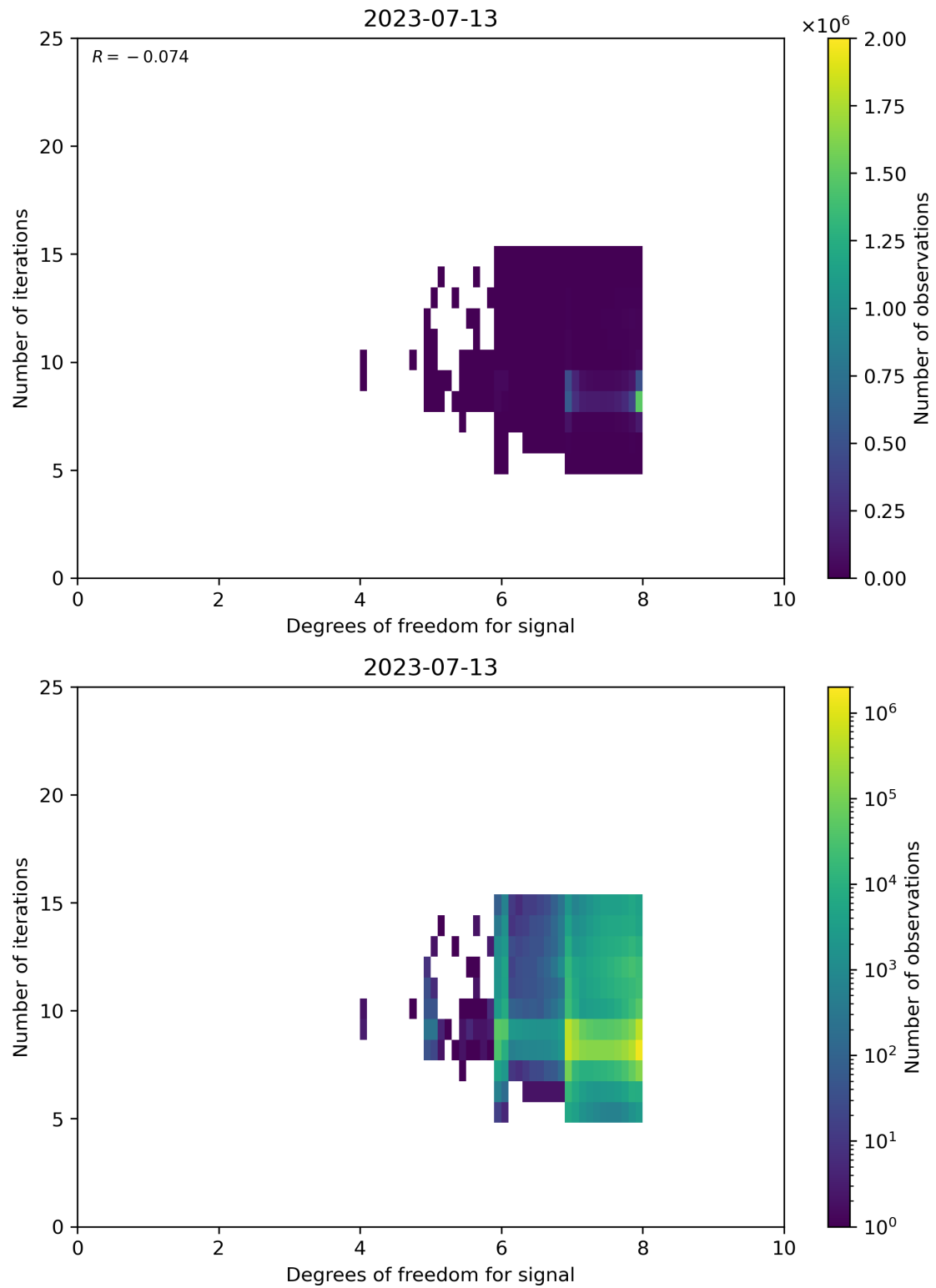
Figure 50: Scatter density plot of “Degrees of freedom for signal” against “Number of iterations” for 2023-07-13 to 2023-07-14.
