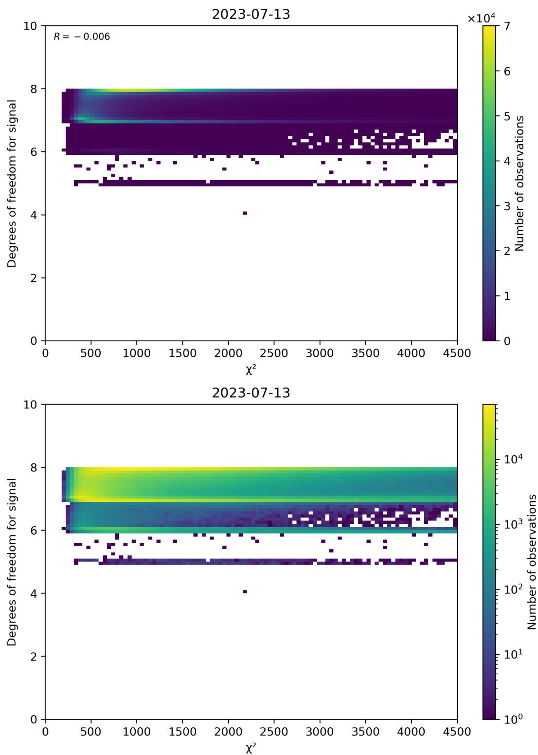
Figure 48: Scatter density plot of " \chi^2 " against "Degrees of freedom for signal" for 2023-07-13 to 2023-07-14.
