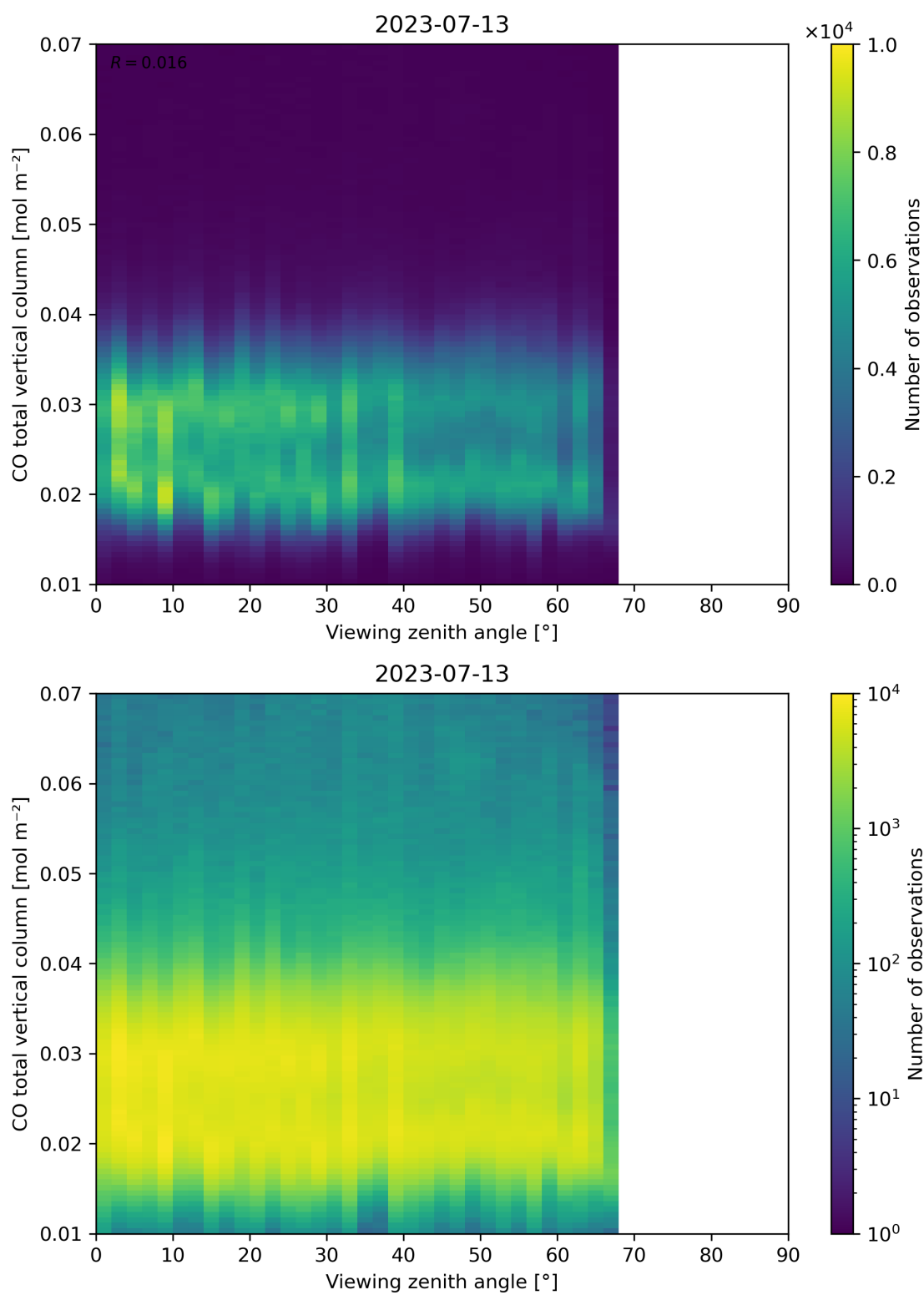
Figure 69: Scatter density plot of “Viewing zenith angle” against “CO total vertical column” for 2023-07-13 to 2023-07-14.
