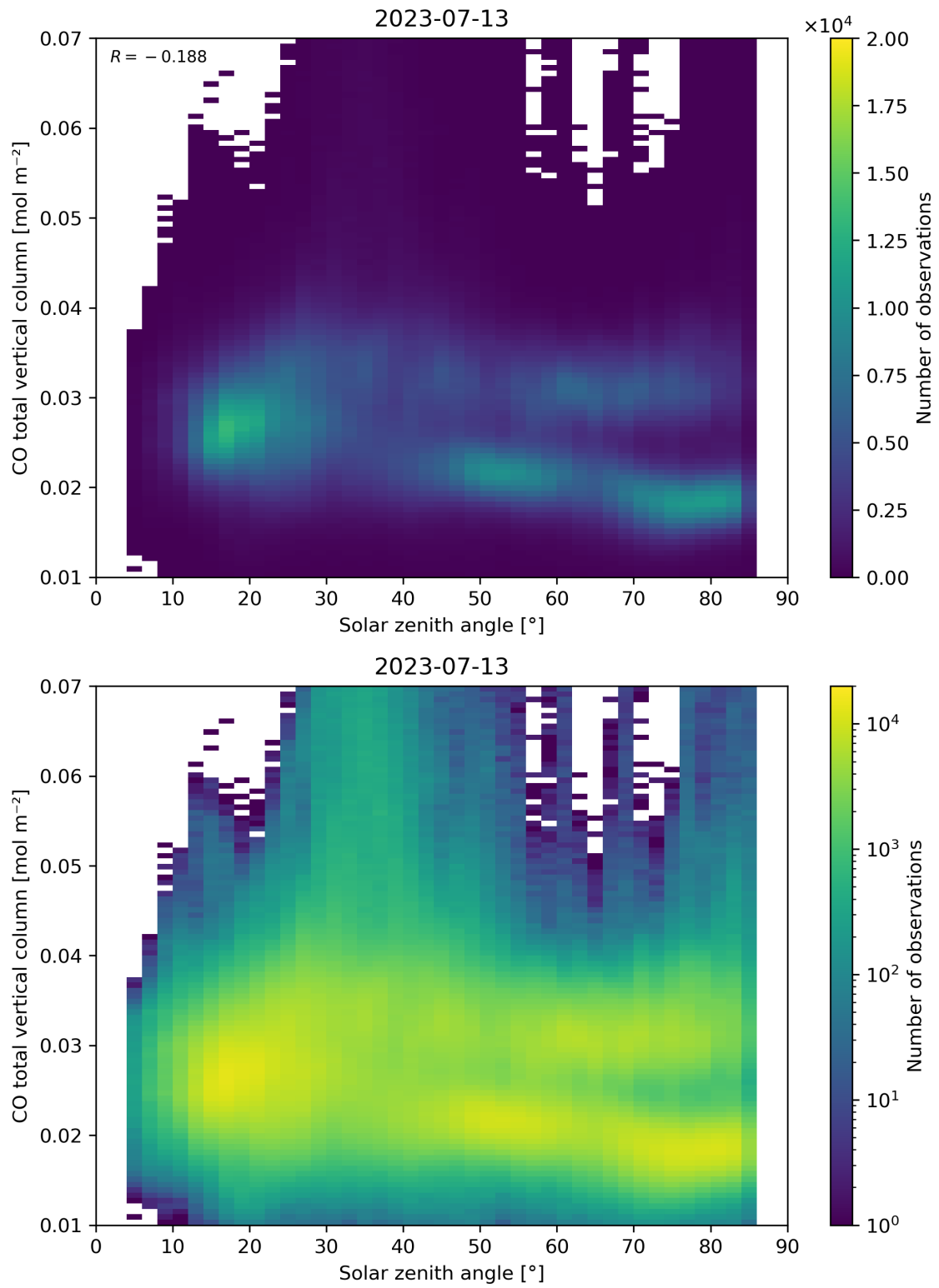
Figure 61: Scatter density plot of “Solar zenith angle” against “CO total vertical column” for 2023-07-13 to 2023-07-14.
