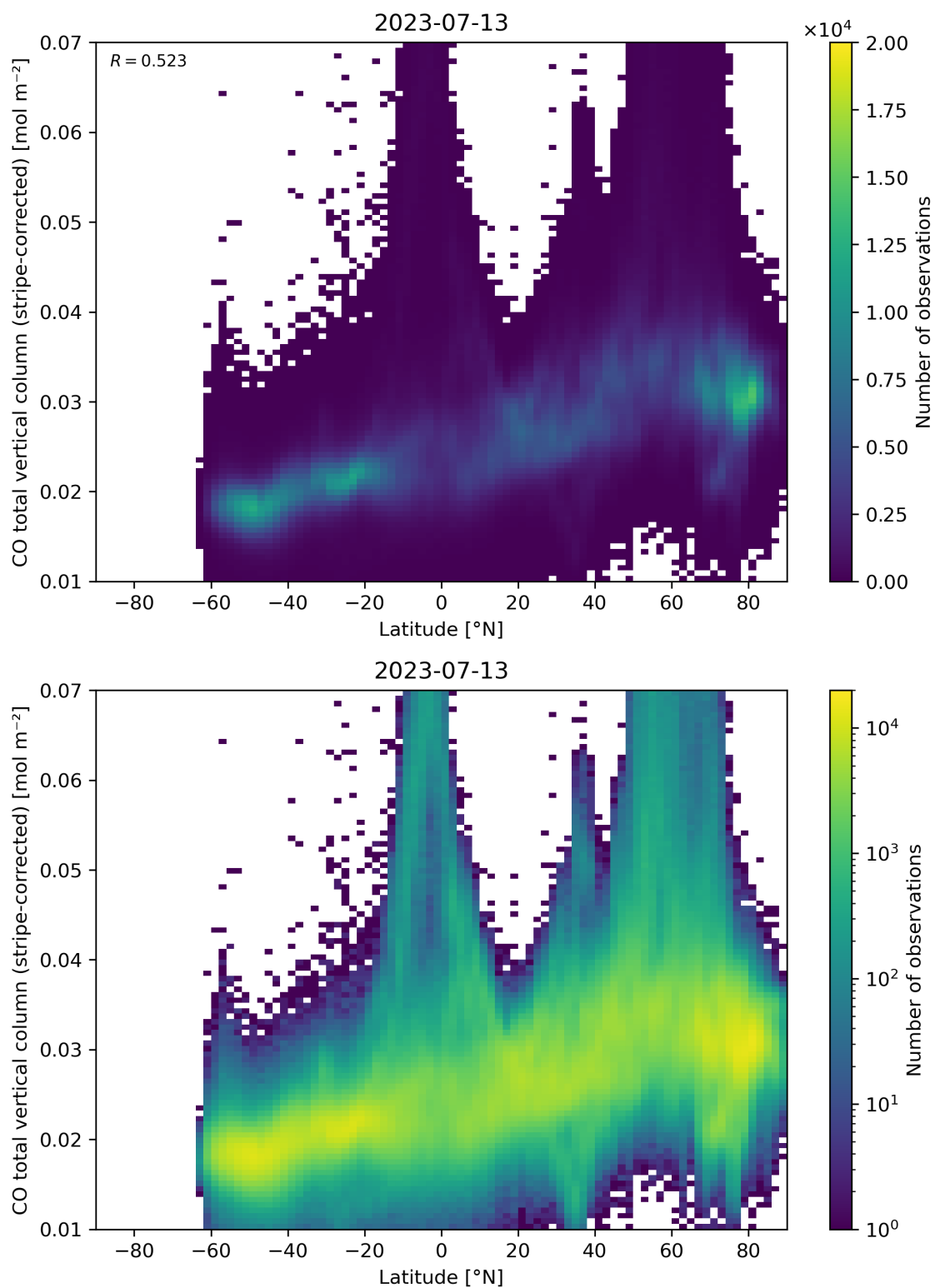
Figure 52: Scatter density plot of “Latitude” against “CO total vertical column (stripe-corrected)” for 2023-07-13 to 2023-07-14.
