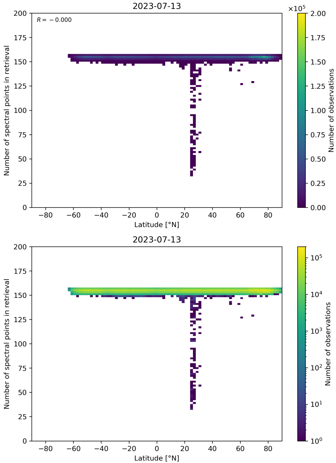
Figure 57: Scatter density plot of “Latitude” against “Number of spectral points in retrieval” for 2023-07-13 to 2023-07-14.
