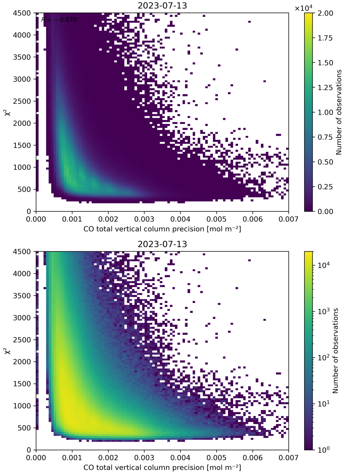
Figure 44: Scatter density plot of “CO total vertical column precision” against “ \chi^2 ” for 2023-07-13 to 2023-07-14.
