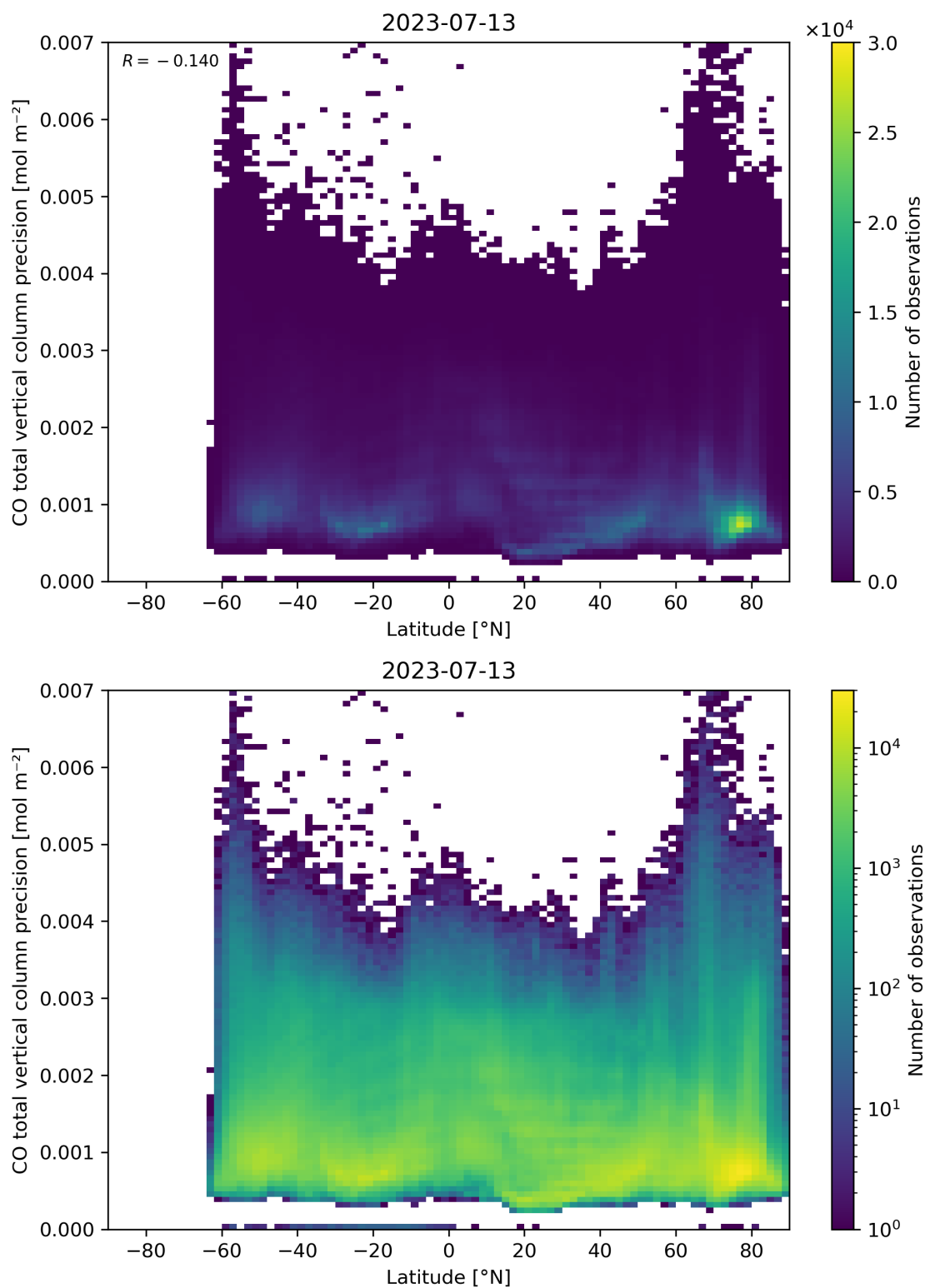
Figure 53: Scatter density plot of “Latitude” against “CO total vertical column precision” for 2023-07-13 to 2023-07-14.
