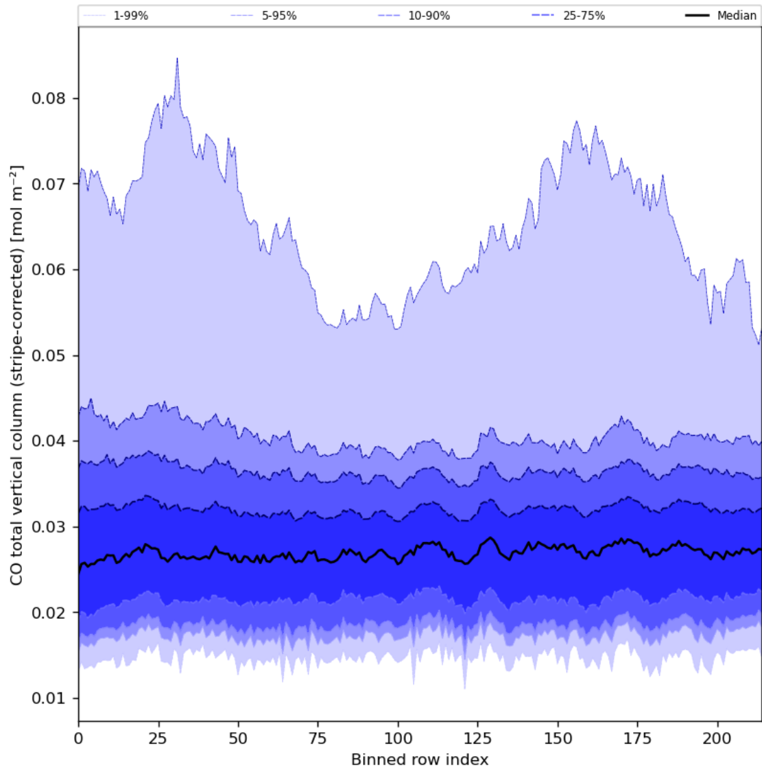
Figure 27: Along track statistics of “CO total vertical column (stripe-corrected)” for 2023-07-13 to 2023-07-14
