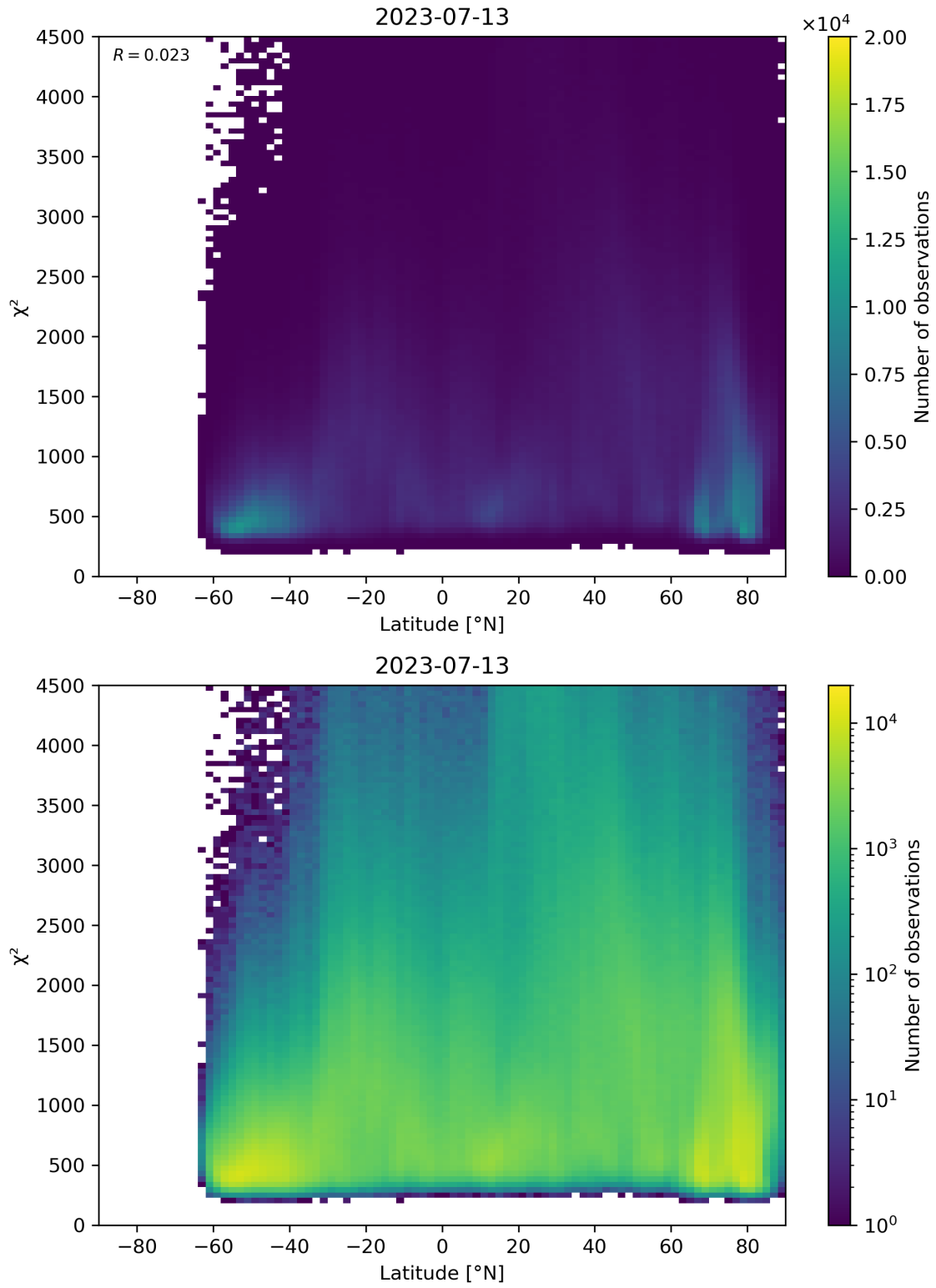
Figure 54: Scatter density plot of “Latitude” against “ \chi^2 ” for 2023-07-13 to 2023-07-14.
