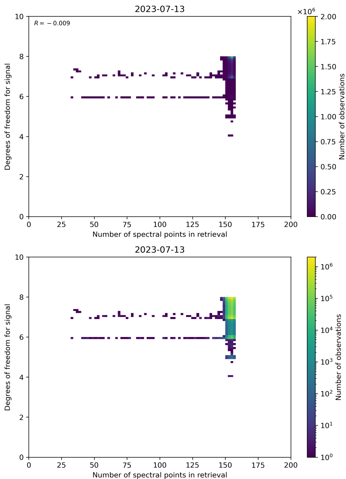
Figure 59: Scatter density plot of “Number of spectral points in retrieval” against “Degrees of freedom for signal” for 2023-07-13 to 2023-07-14.
