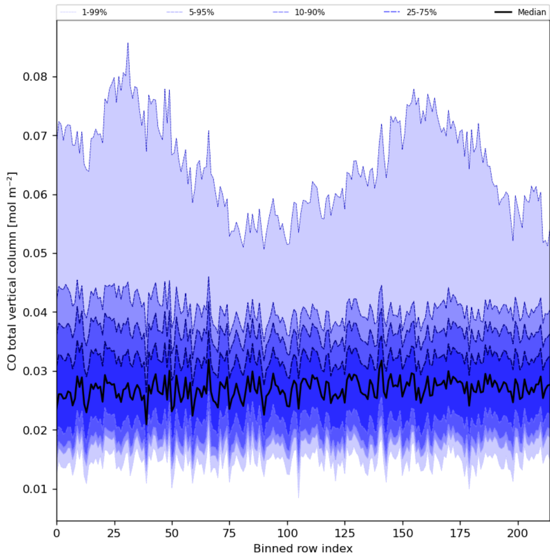
Figure 26: Along track statistics of “CO total vertical column” for 2023-07-13 to 2023-07-14
