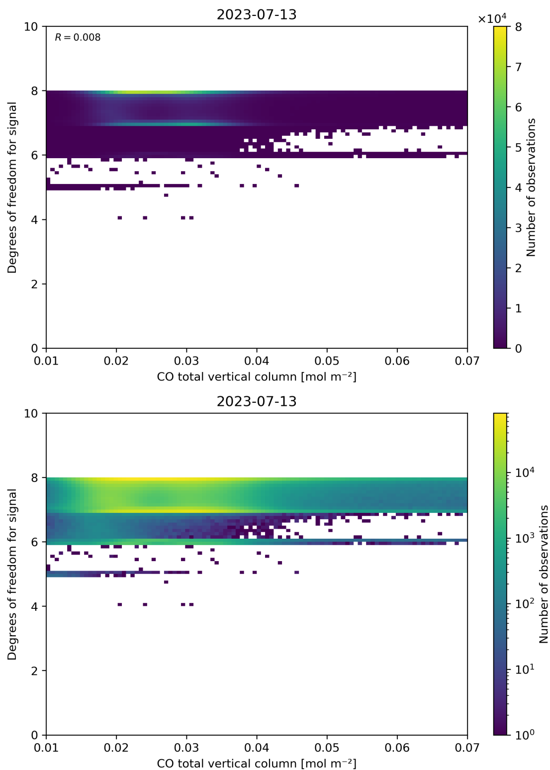
Figure 41: Scatter density plot of “CO total vertical column” against “Degrees of freedom for signal” for 2023-07-13 to 2023-07-14.
