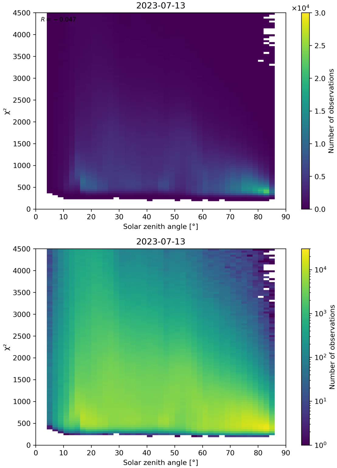
Figure 64: Scatter density plot of “Solar zenith angle” against “ \chi^2 ” for 2023-07-13 to 2023-07-14.
