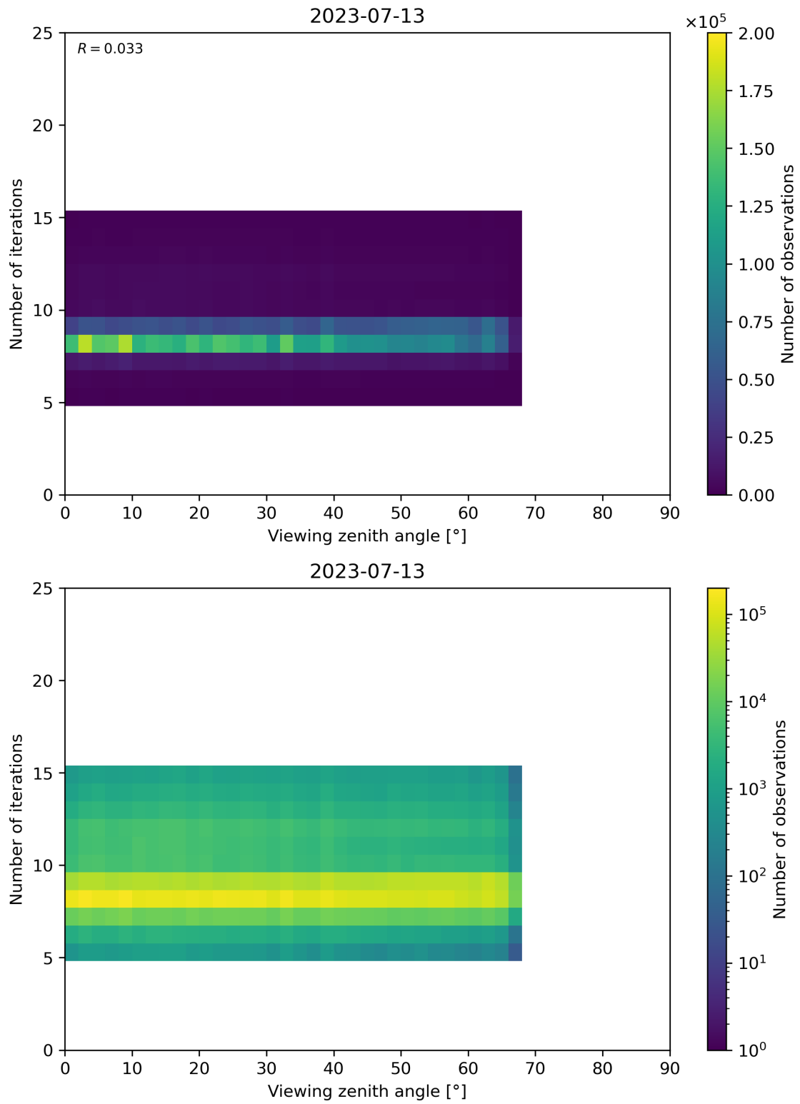
Figure 75: Scatter density plot of “Viewing zenith angle” against “Number of iterations” for 2023-07-13 to 2023-07-14.
