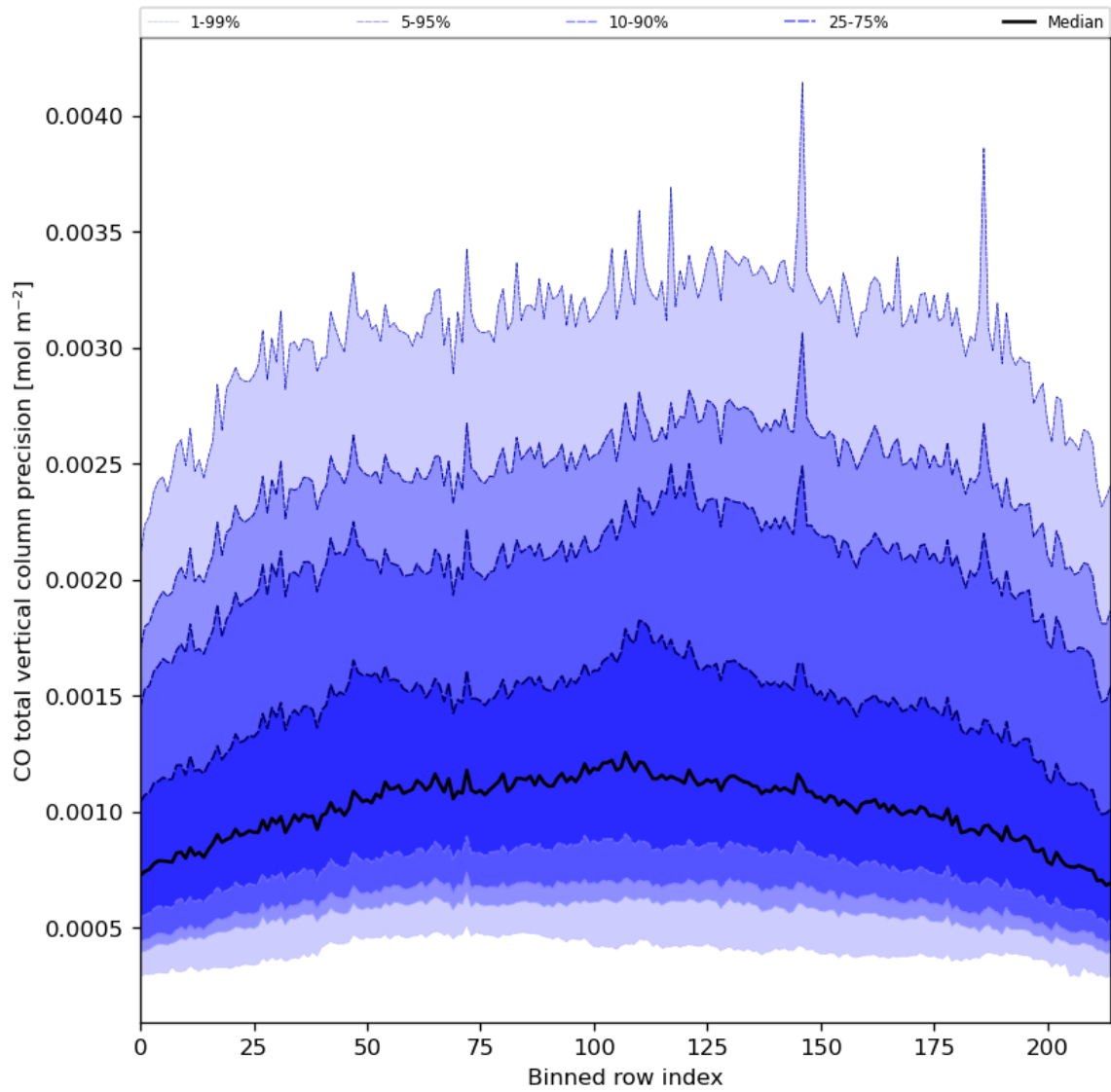
Figure 28: Along track statistics of “CO total vertical column precision” for 2023-07-13 to 2023-07-14
