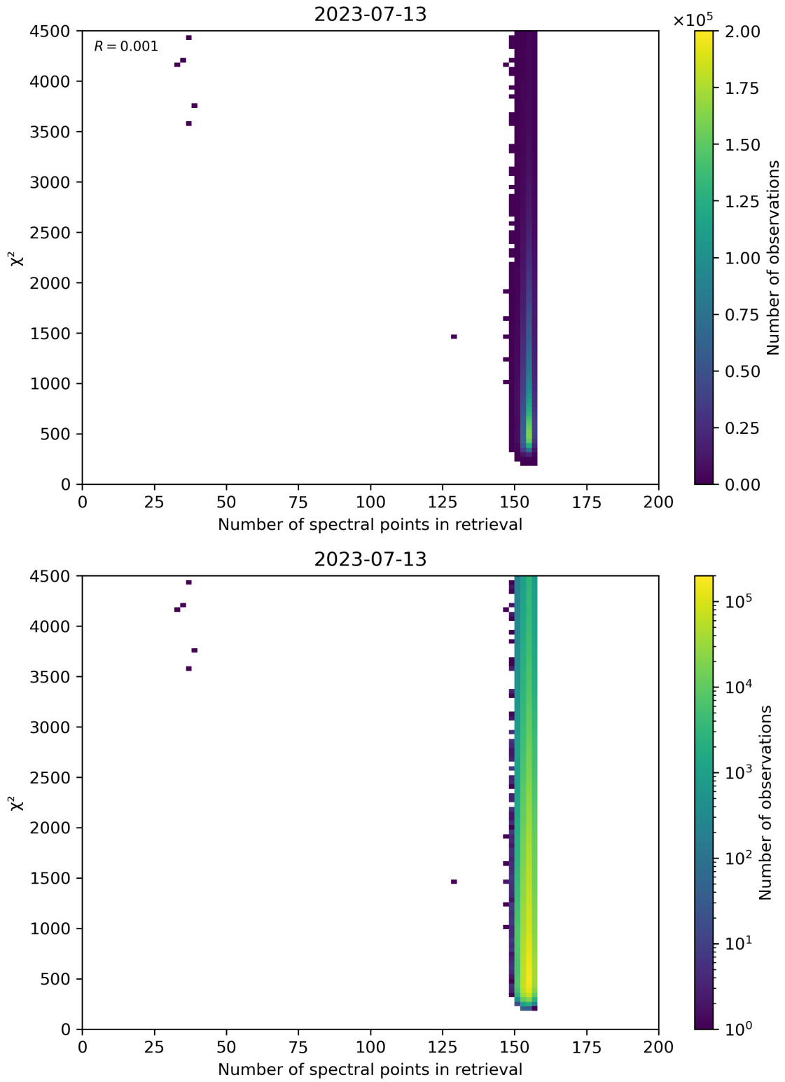
Figure 58: Scatter density plot of “Number of spectral points in retrieval” against “ \chi^2 ” for 2023-07-13 to 2023-07-14.
