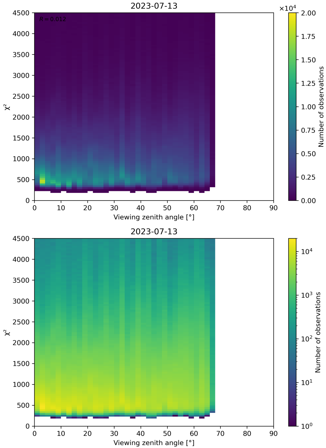
Figure 72: Scatter density plot of “Viewing zenith angle” against “ \chi^2 ” for 2023-07-13 to 2023-07-14.
