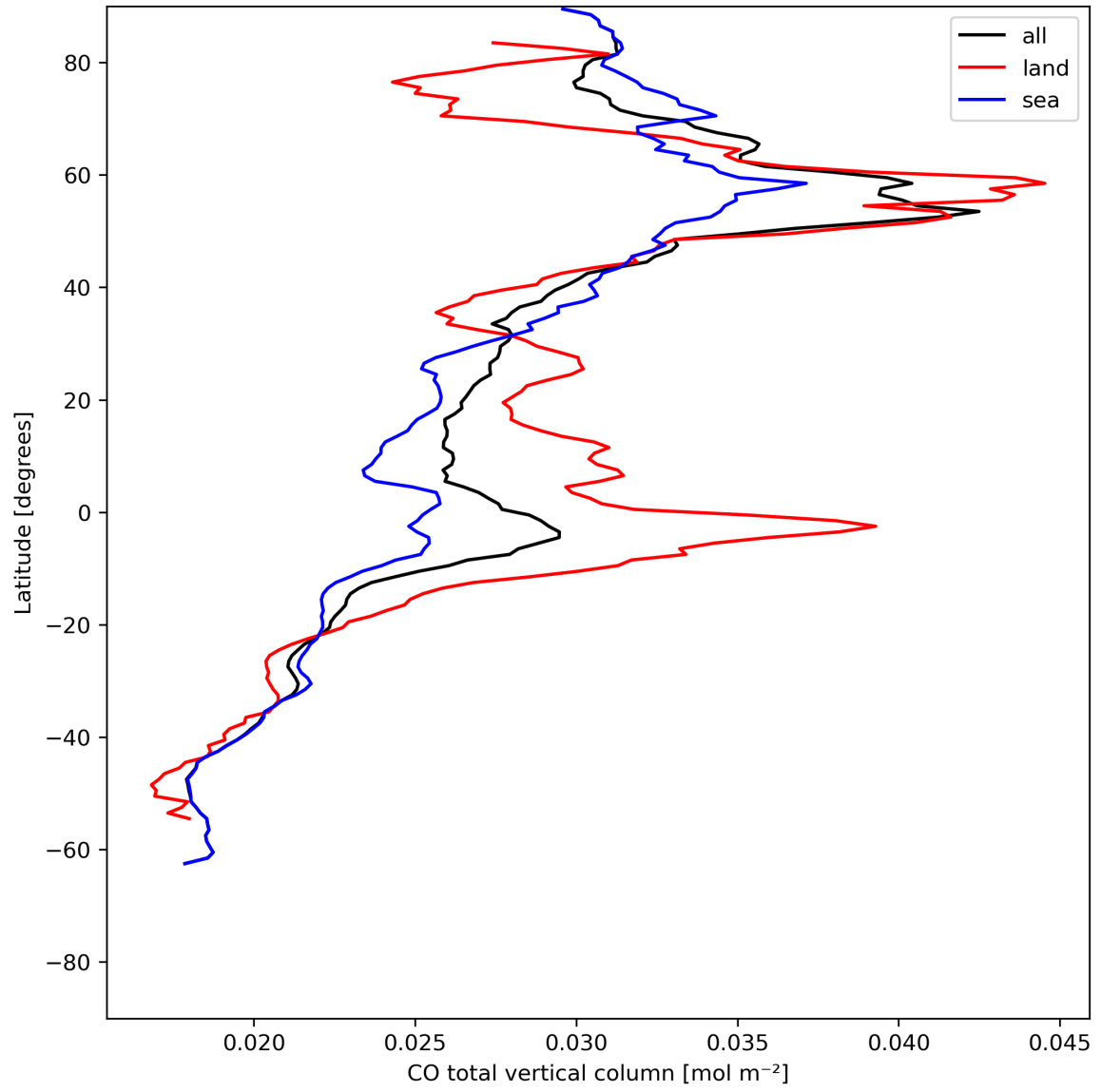
Figure 10: Zonal average of “CO total vertical column” for 2023-07-13 to 2023-07-14.
