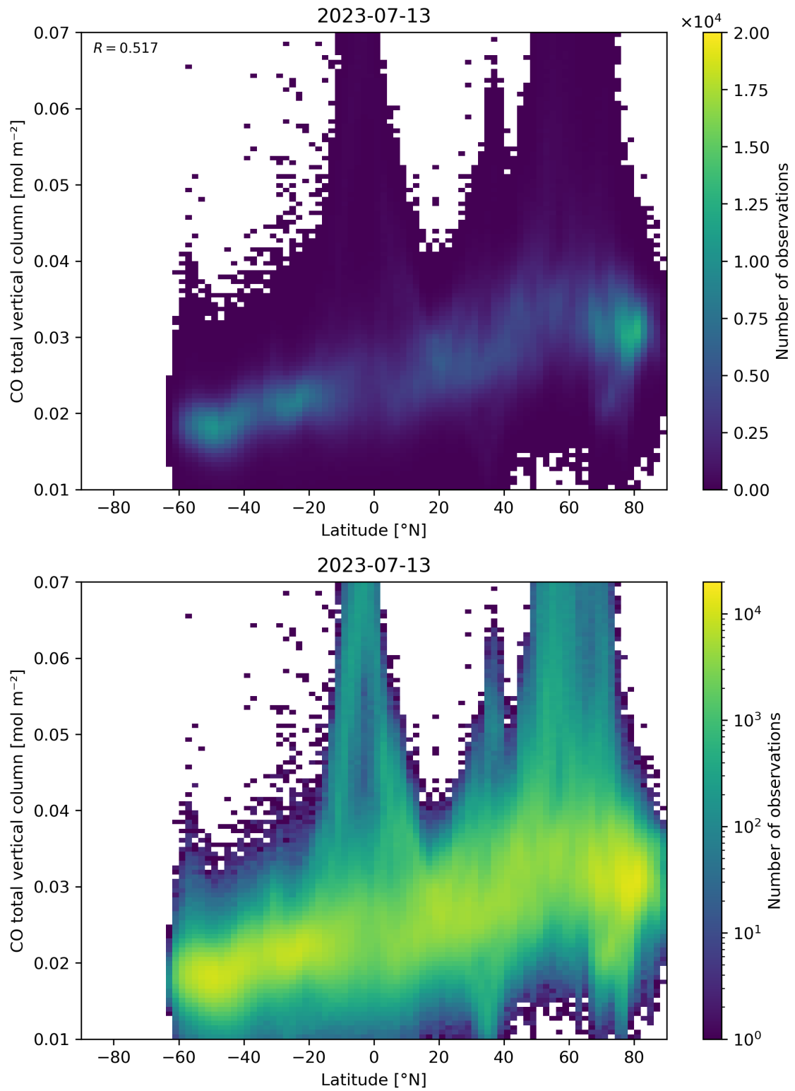
Figure 51: Scatter density plot of “Latitude” against “CO total vertical column” for 2023-07-13 to 2023-07-14.
