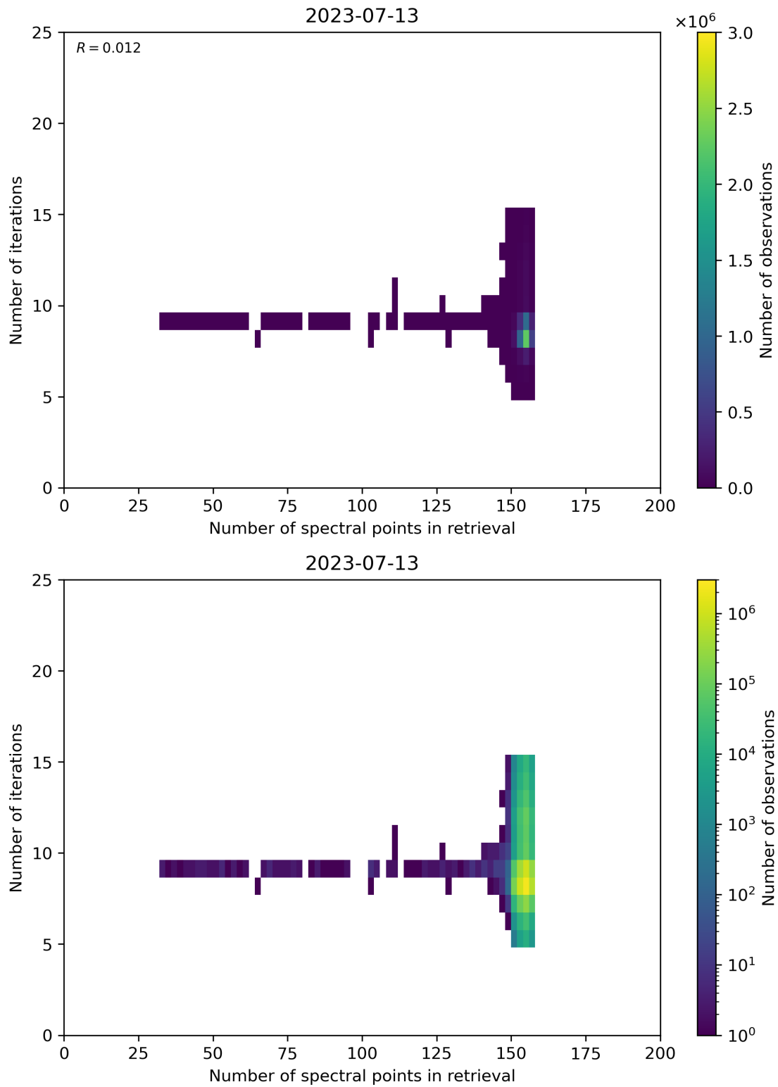
Figure 60: Scatter density plot of “Number of spectral points in retrieval” against “Number of iterations” for 2023-07-13 to 2023-07-14.
