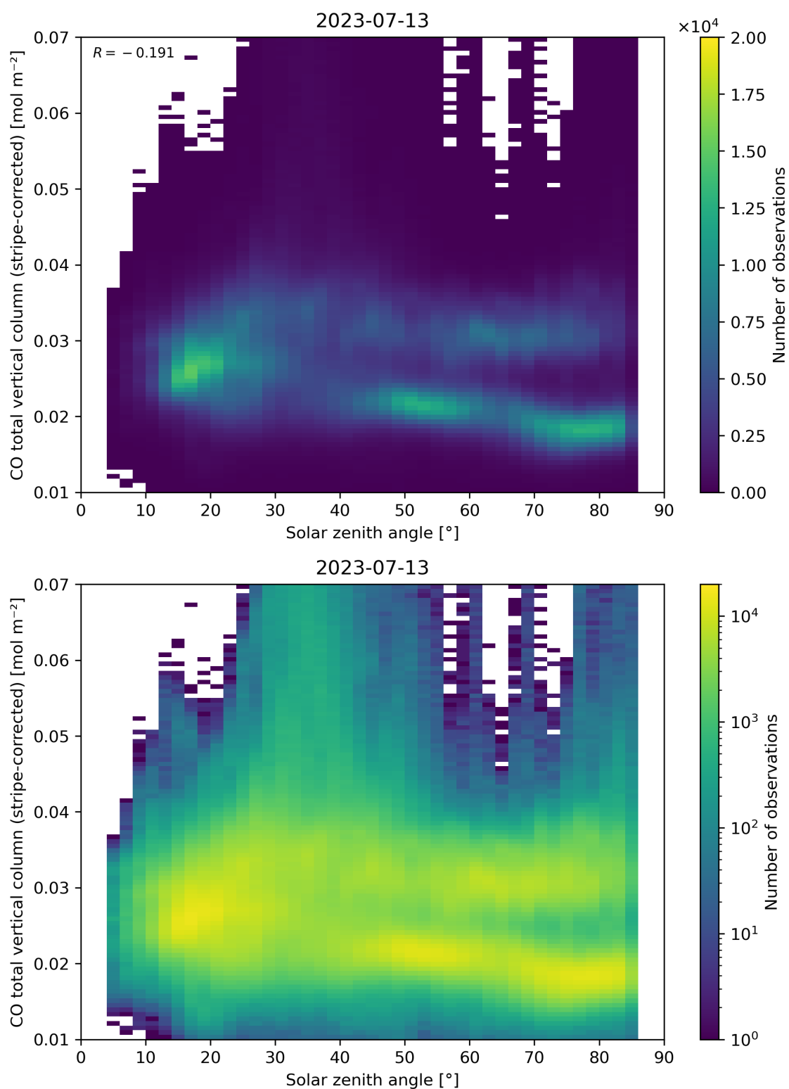
Figure 62: Scatter density plot of “Solar zenith angle” against “CO total vertical column (stripe-corrected)” for 2023-07-13 to 2023-07-14.
