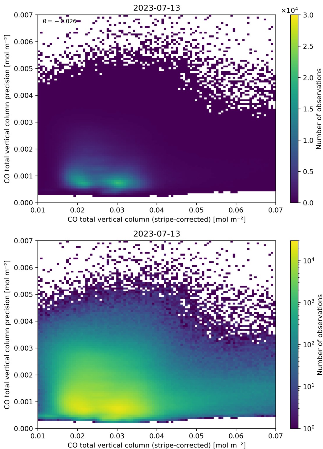
Figure 36: Scatter density plot of “CO total vertical column (stripe-corrected)” against “CO total vertical column precision” for 2023-07-13 to 2023-07-14.
