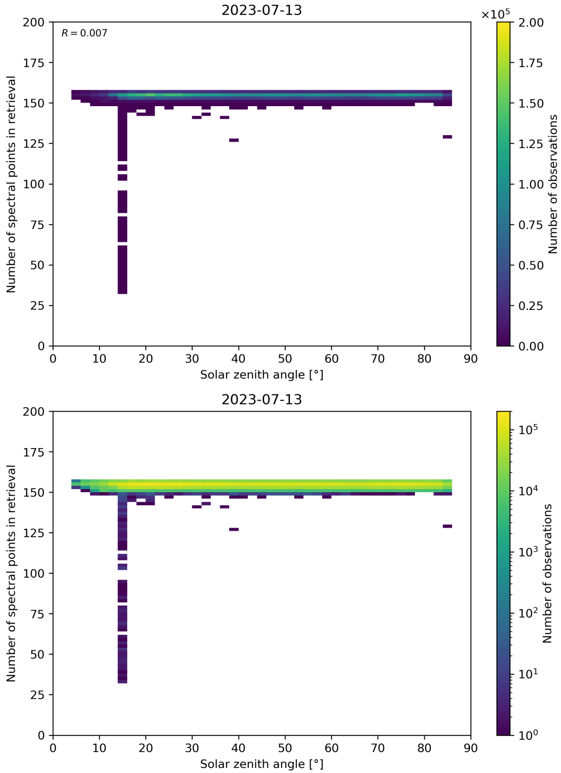
Figure 68: Scatter density plot of “Solar zenith angle” against “Number of spectral points in retrieval” for 2023-07-13 to 2023-07-14.
