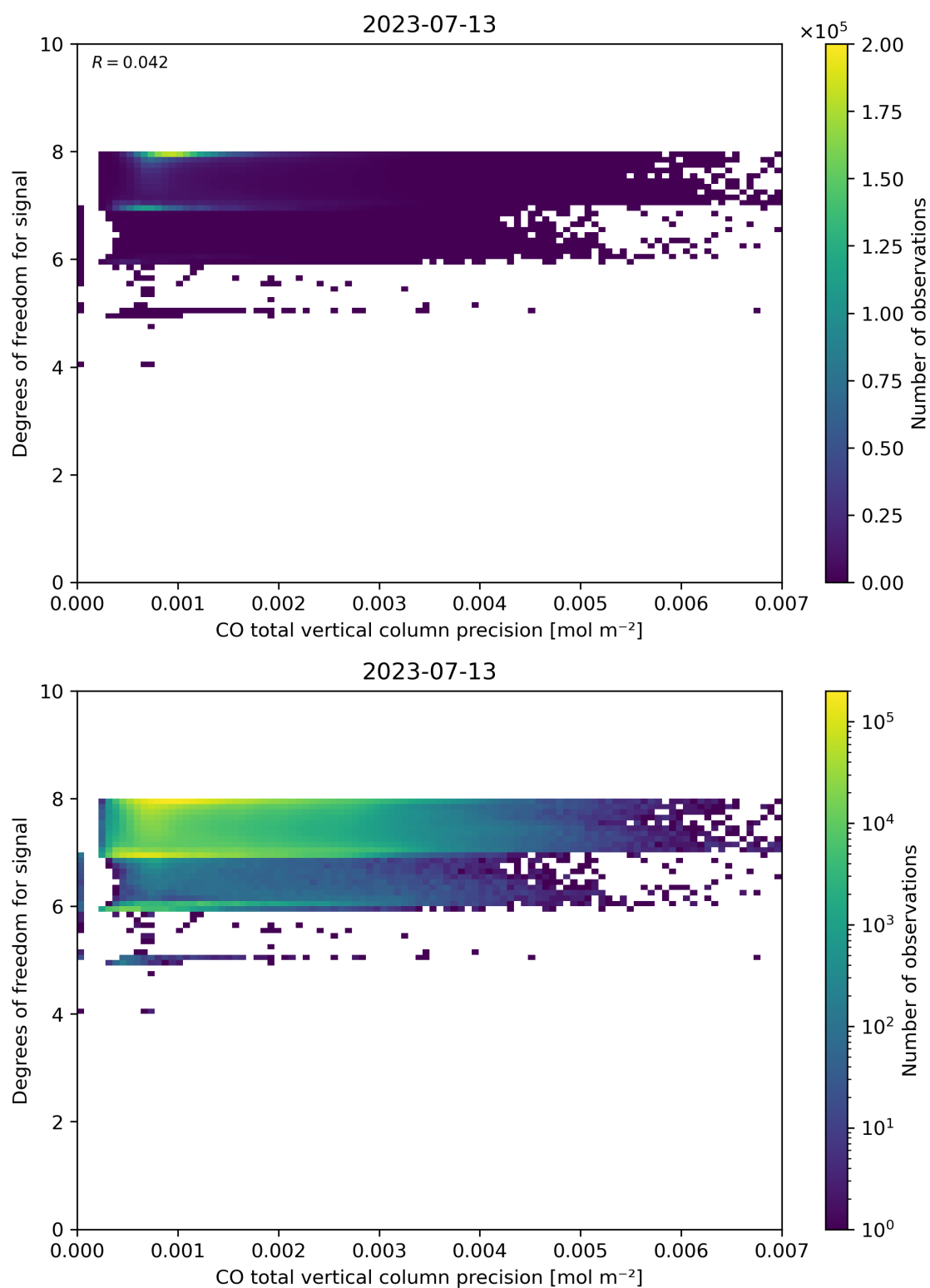
Figure 45: Scatter density plot of “CO total vertical column precision” against “Degrees of freedom for signal” for 2023-07-13 to 2023-07-14.
