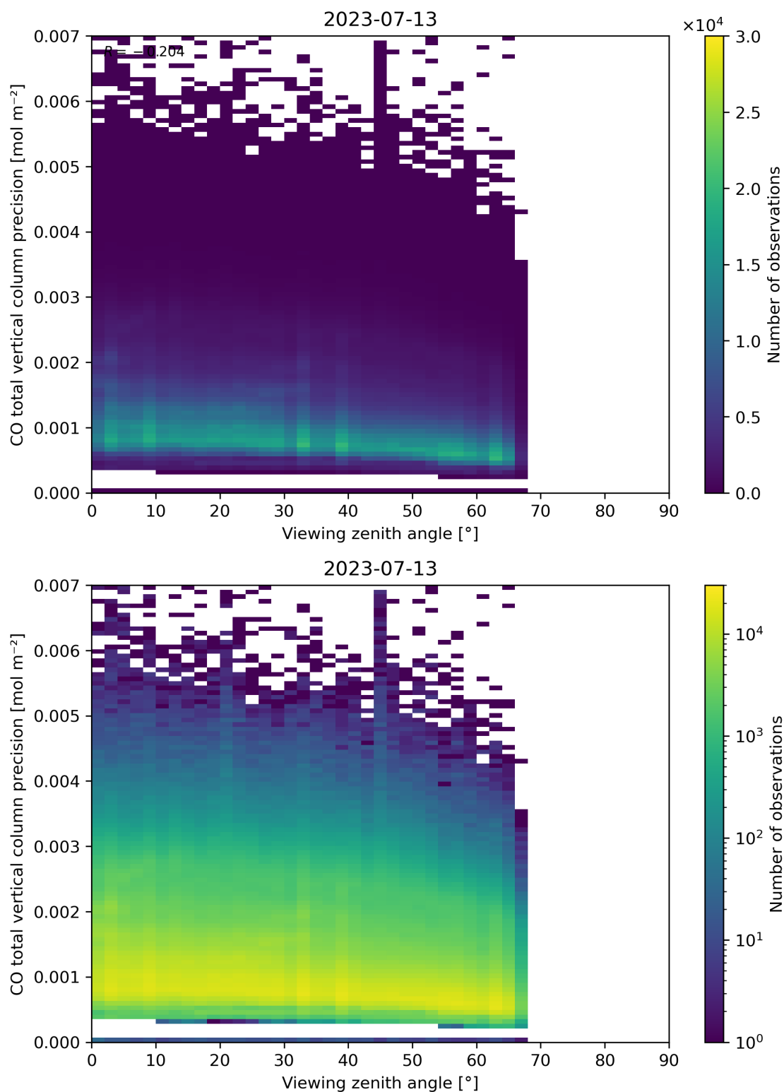
Figure 71: Scatter density plot of “Viewing zenith angle” against “CO total vertical column precision” for 2023-07-13 to 2023-07-14.
