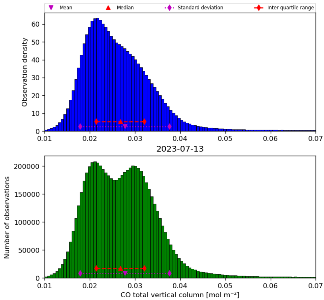
Figure 18: Histogram of “CO total vertical column” for 2023-07-13 to 2023-07-14
