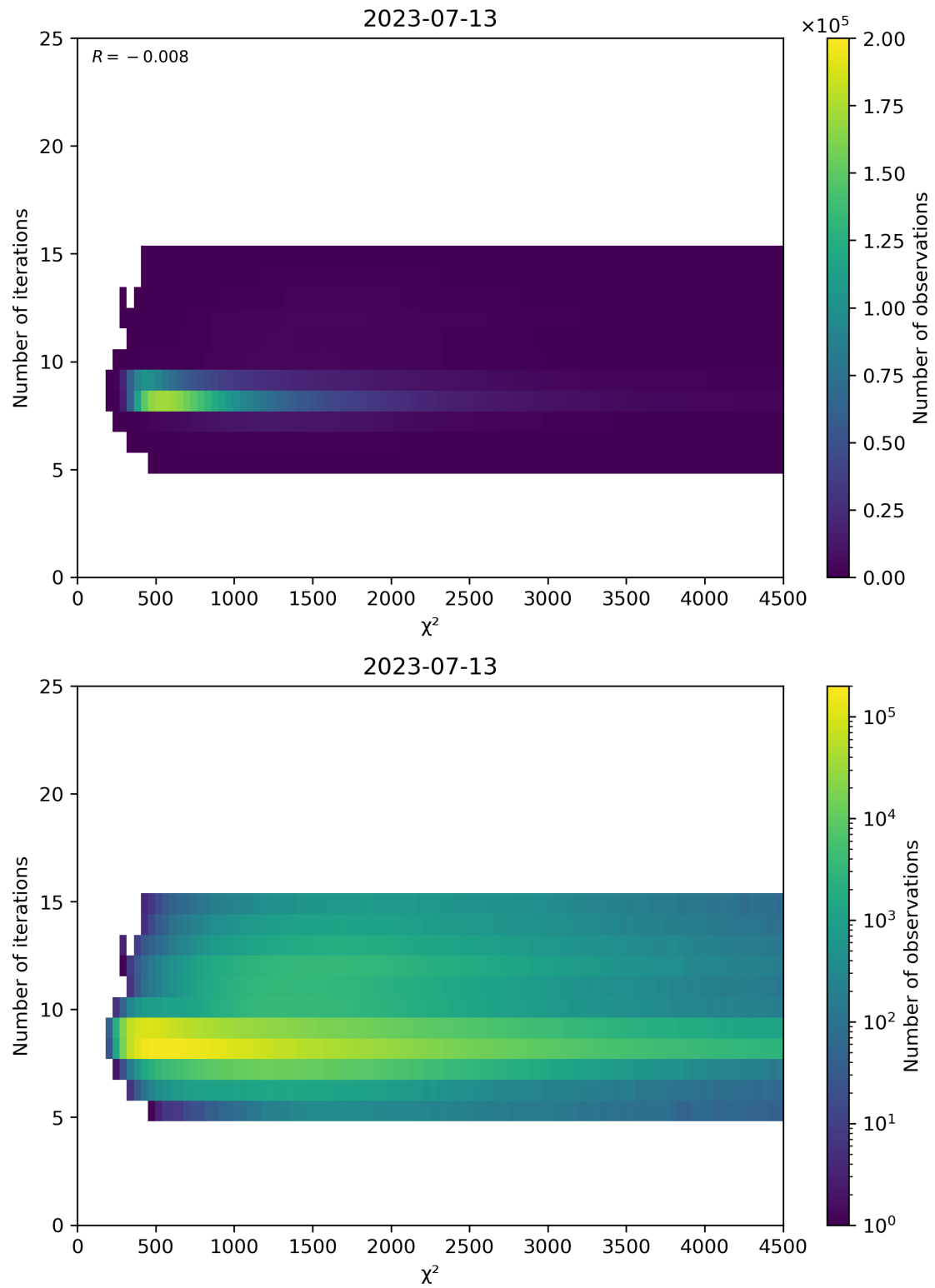
Figure 49: Scatter density plot of “ \chi^2 ” against “Number of iterations” for 2023-07-13 to 2023-07-14.
