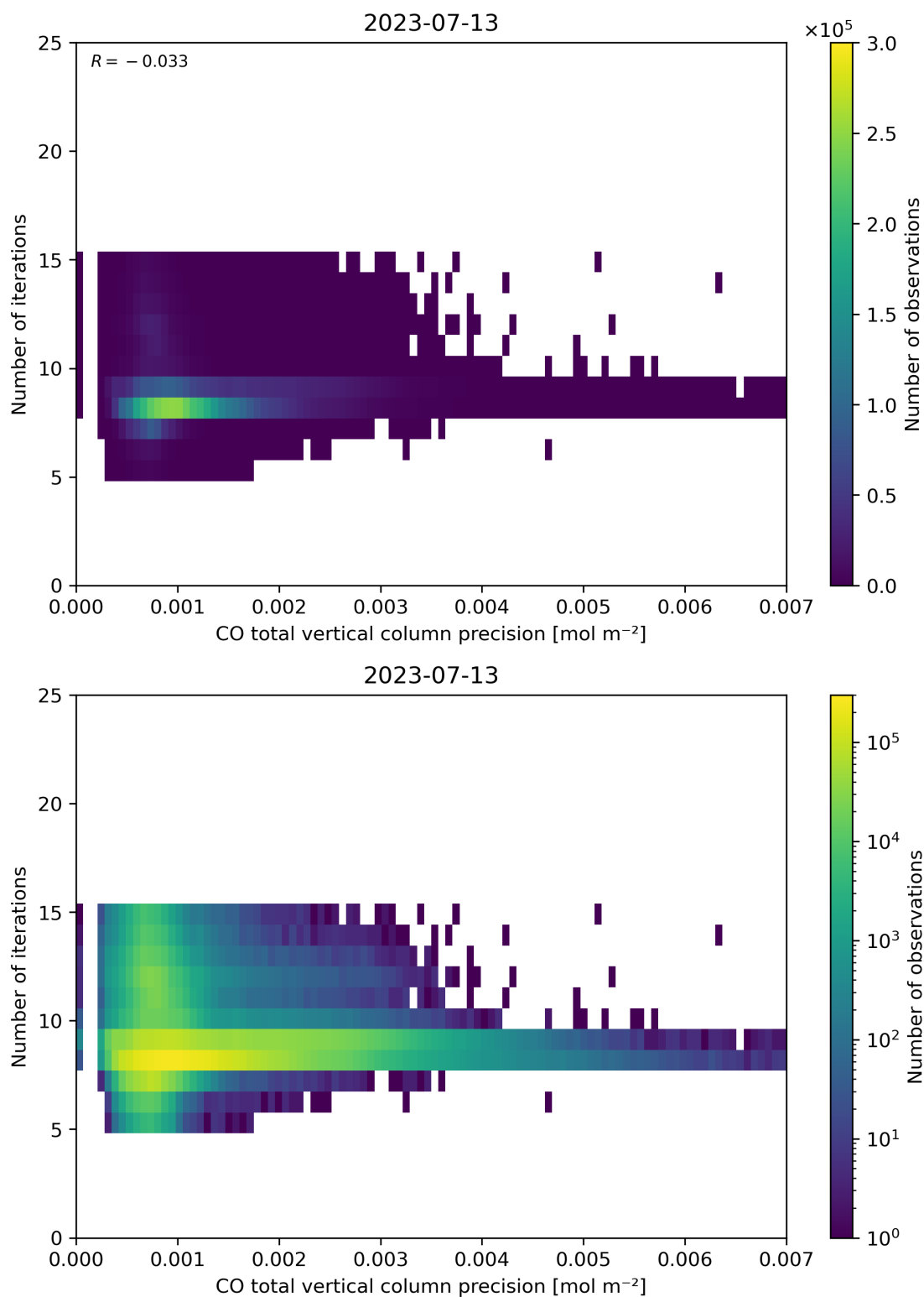
Figure 46: Scatter density plot of “CO total vertical column precision” against “Number of iterations” for 2023-07-13 to 2023-07-14.
