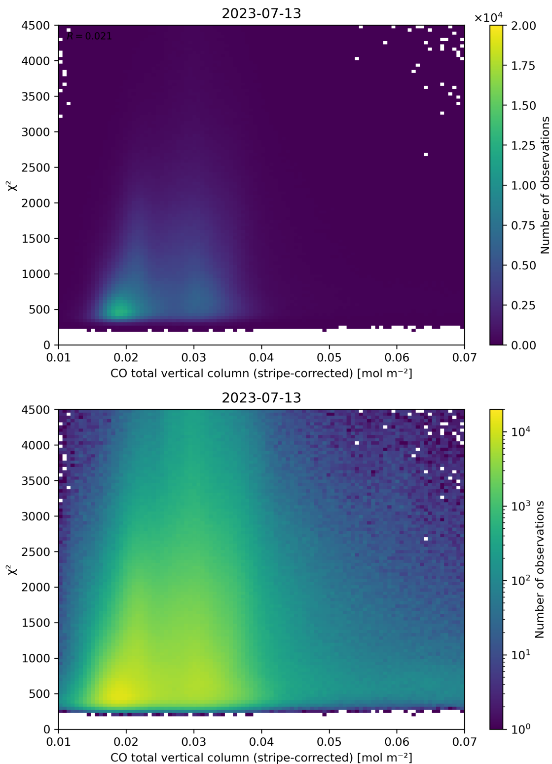
Figure 37: Scatter density plot of “CO total vertical column (stripe-corrected)” against “ \chi^2 ” for 2023-07-13 to 2023-07-14.
