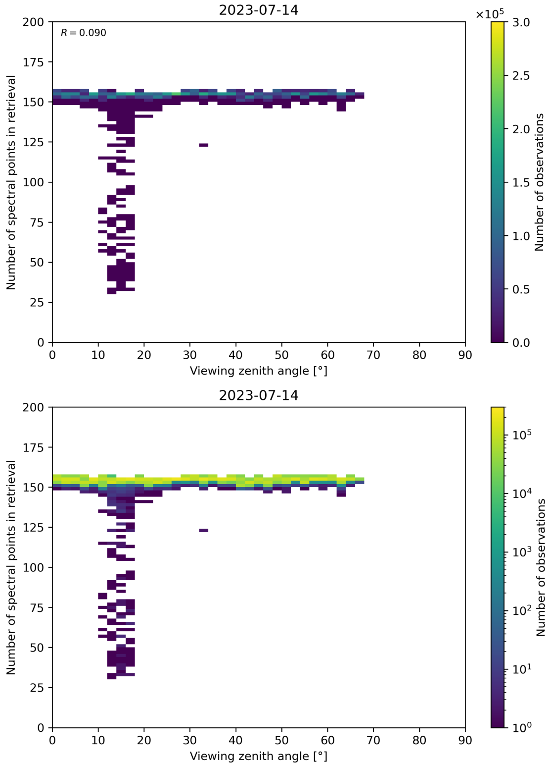
Figure 76: Scatter density plot of “Viewing zenith angle” against “Number of spectral points in retrieval” for 2023-07-14 to 2023-07-15.
