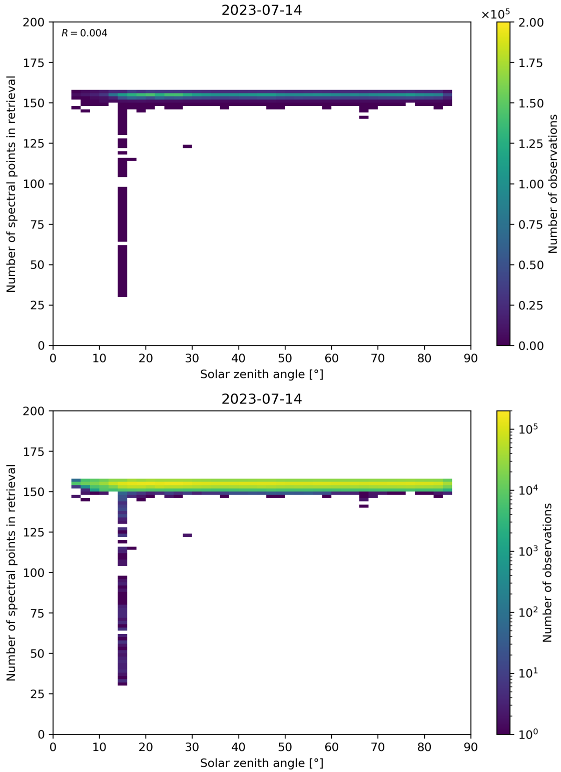
Figure 68: Scatter density plot of “Solar zenith angle” against “Number of spectral points in retrieval” for 2023-07-14 to 2023-07-15.
