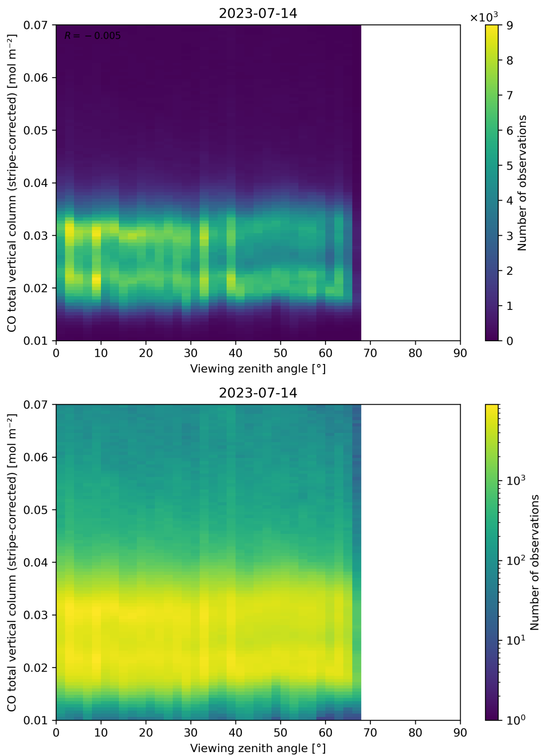
Figure 70: Scatter density plot of “Viewing zenith angle” against “CO total vertical column (stripe-corrected)” for 2023-07-14 to 2023-07-15.
