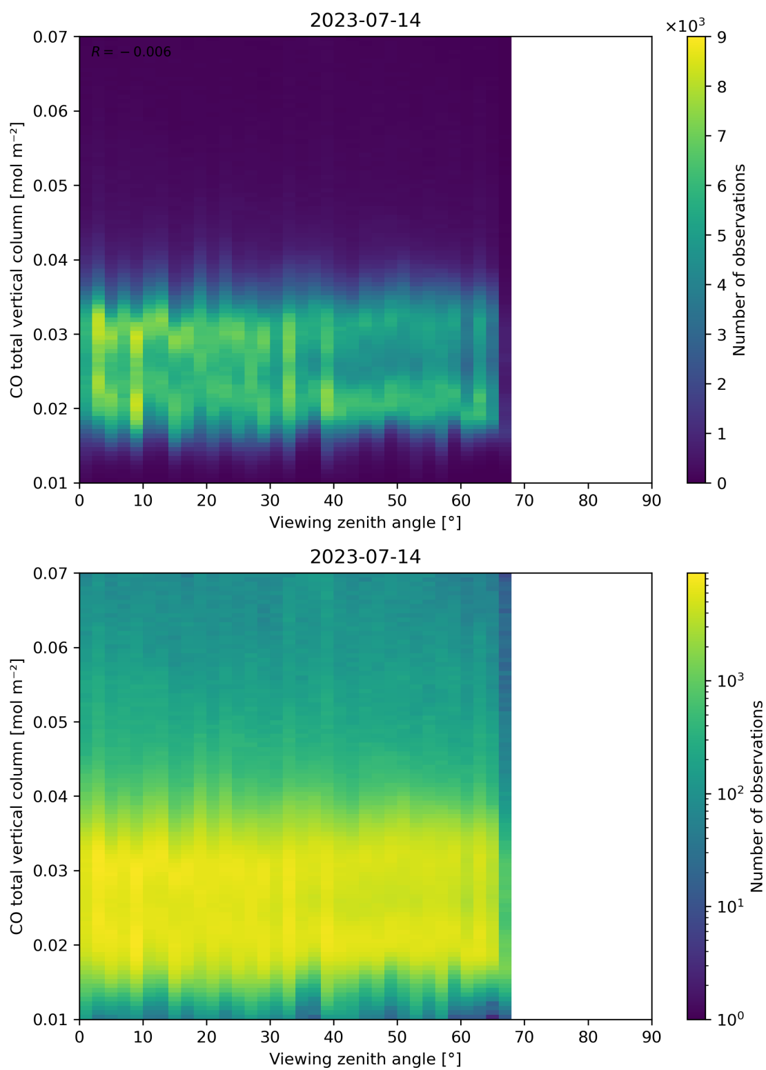
Figure 69: Scatter density plot of “Viewing zenith angle” against “CO total vertical column” for 2023-07-14 to 2023-07-15.
