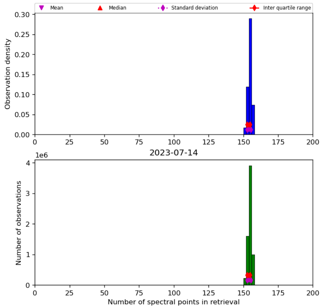
Figure 21: Histogram of “Number of spectral points in retrieval” for 2023-07-14 to 2023-07-15
