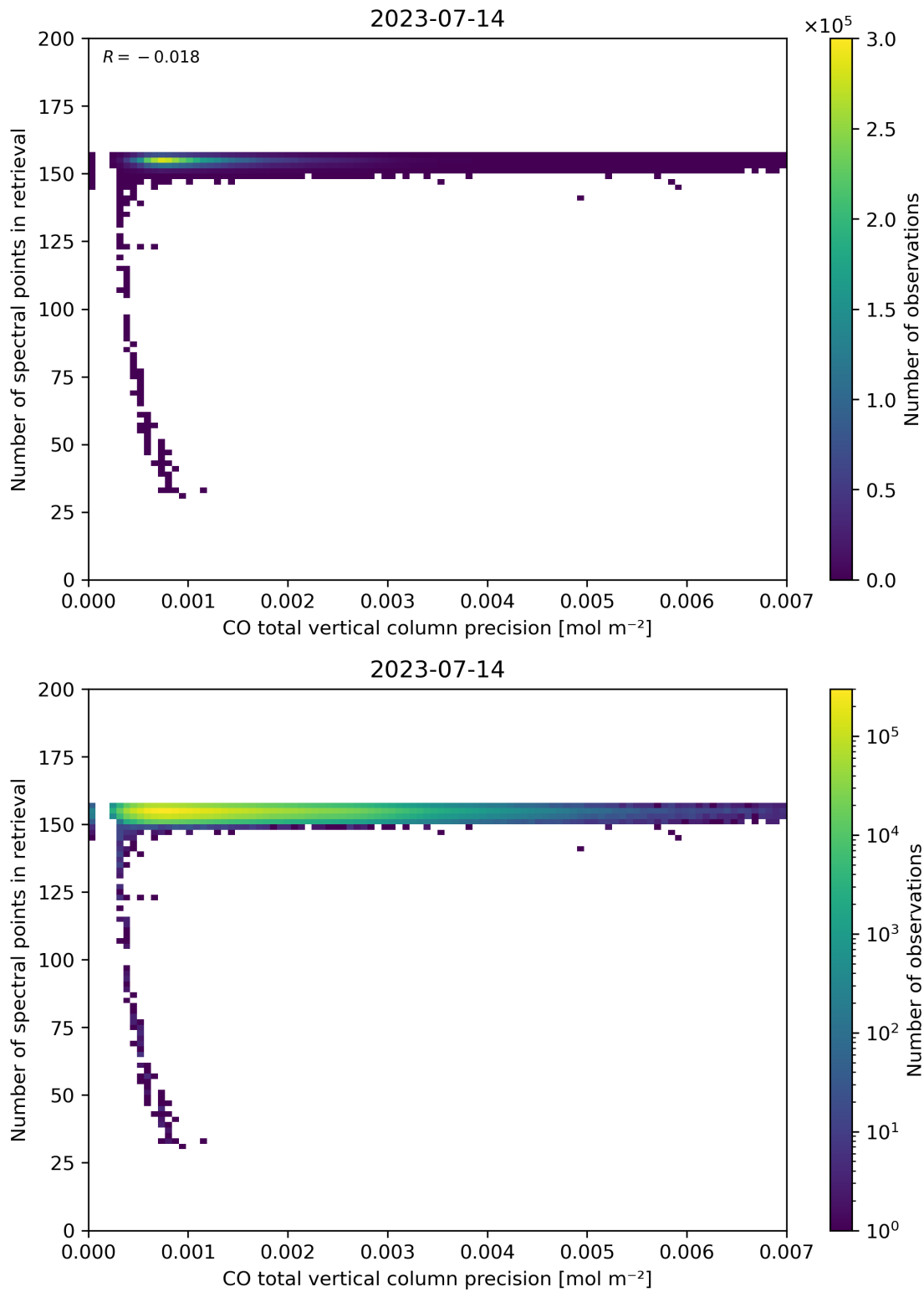
Figure 47: Scatter density plot of “CO total vertical column precision” against “Number of spectral points in retrieval” for 2023-07-14 to 2023-07-15.
