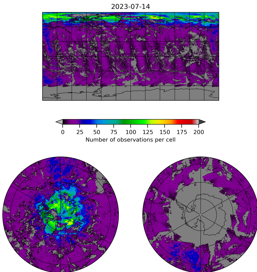
Figure 8: Map of the number of observations for 2023-07-14 to 2023-07-15
