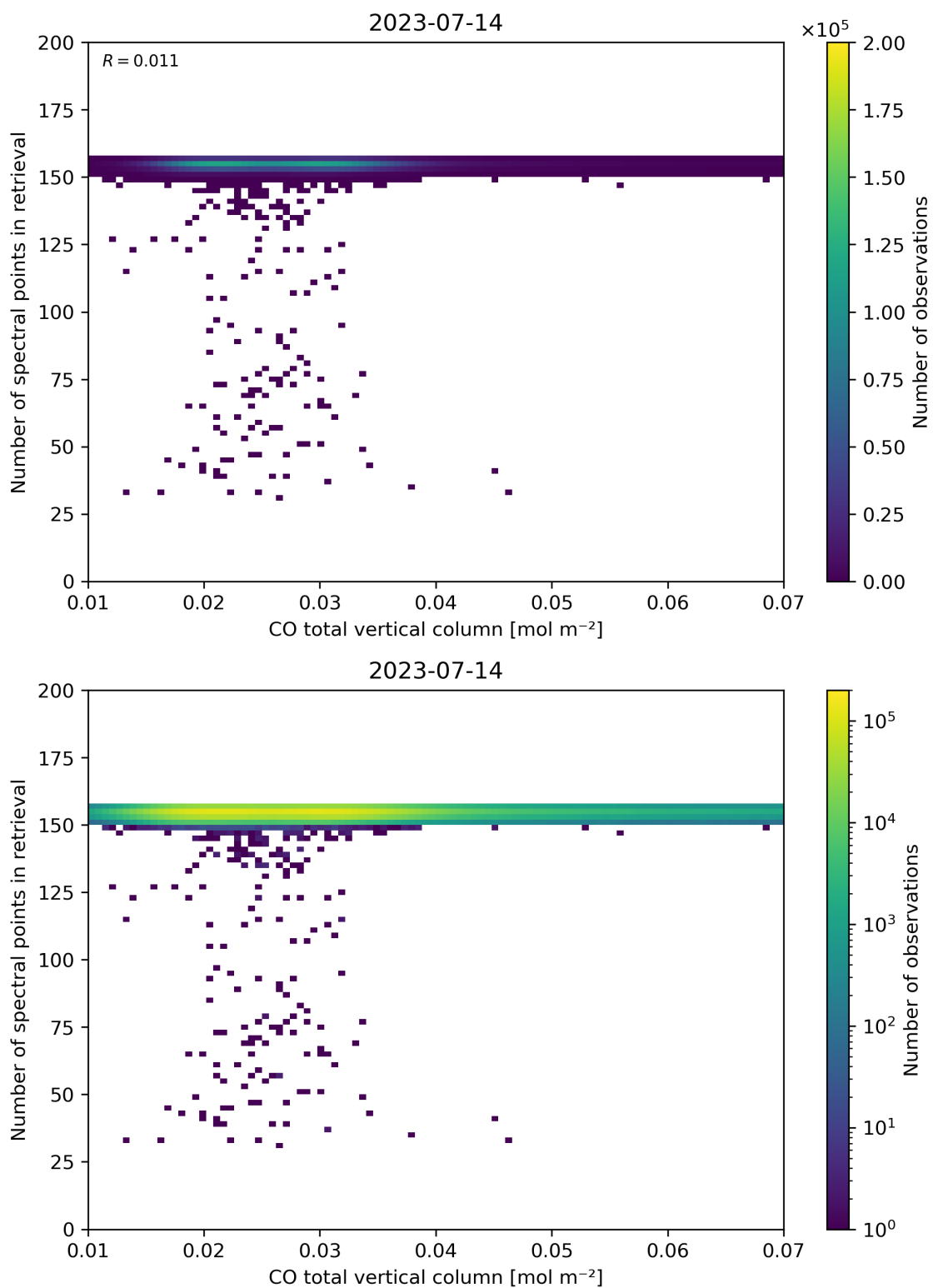
Figure 43: Scatter density plot of “CO total vertical column” against “Number of spectral points in retrieval” for 2023-07-14 to 2023-07-15.
