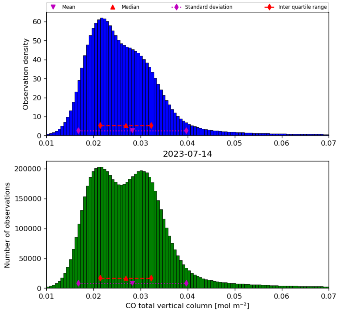
Figure 18: Histogram of “CO total vertical column” for 2023-07-14 to 2023-07-15
