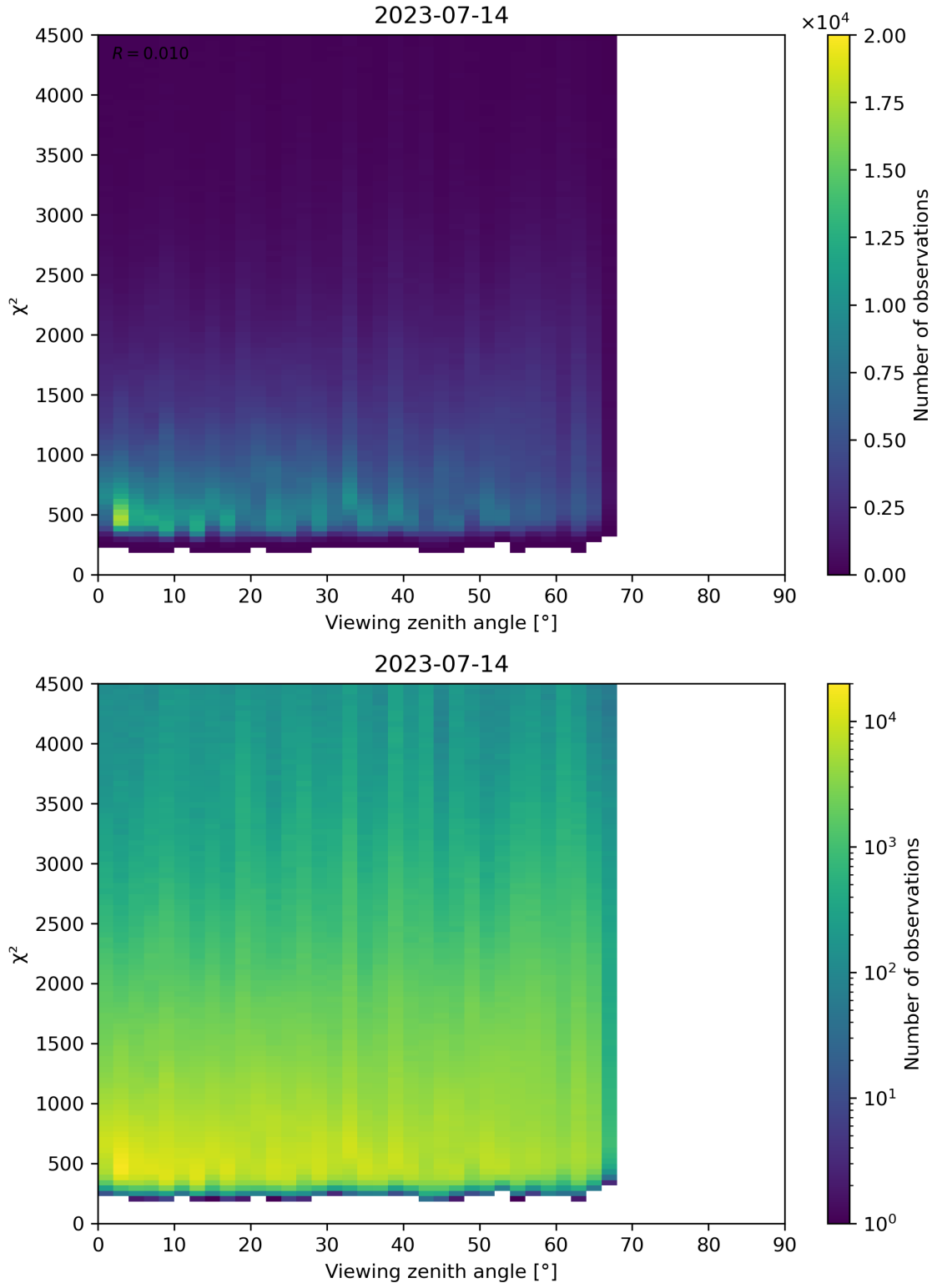
Figure 72: Scatter density plot of “Viewing zenith angle” against “ \chi^2 ” for 2023-07-14 to 2023-07-15.
