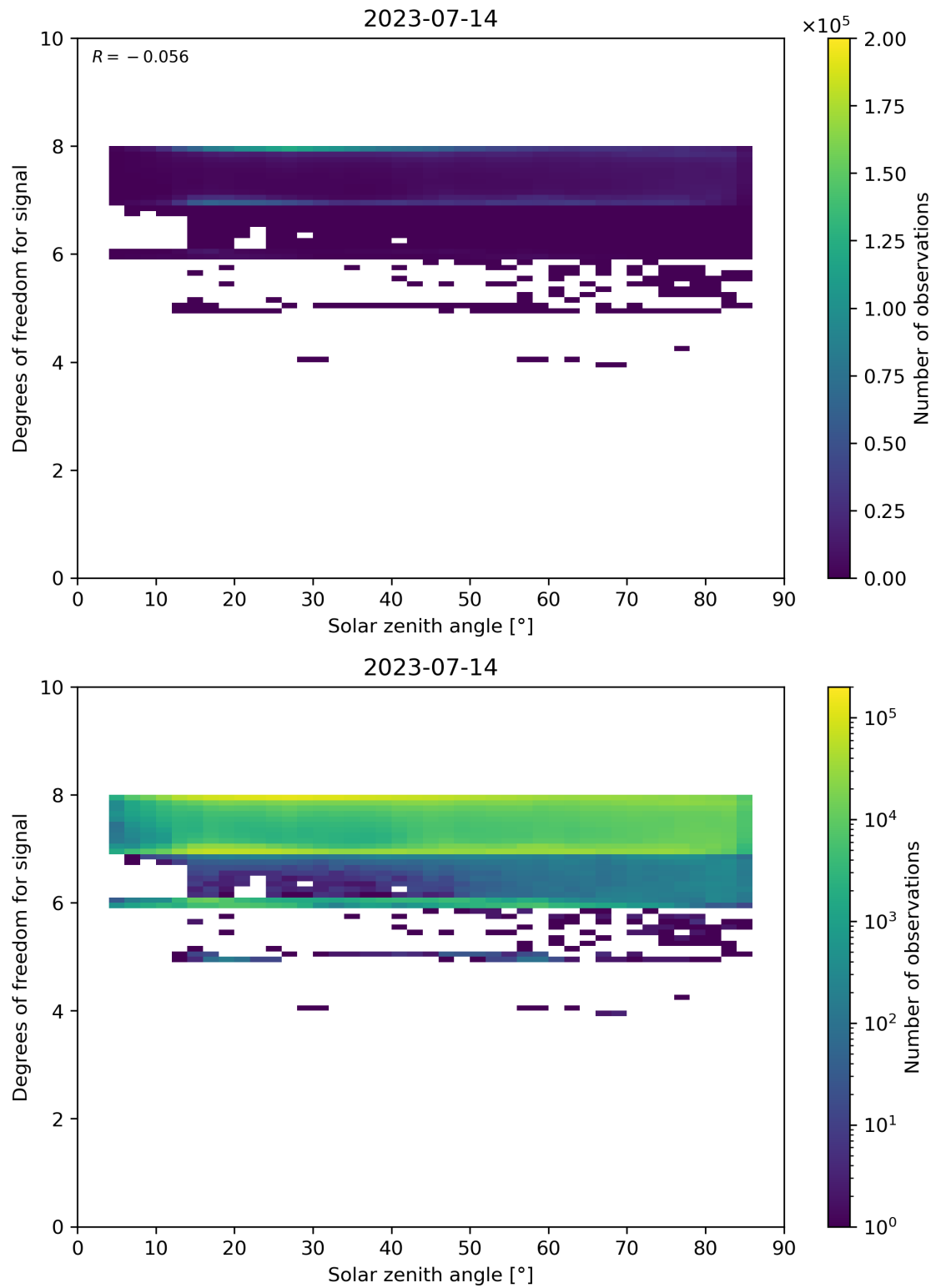
Figure 65: Scatter density plot of “Solar zenith angle” against “Degrees of freedom for signal” for 2023-07-14 to 2023-07-15.
