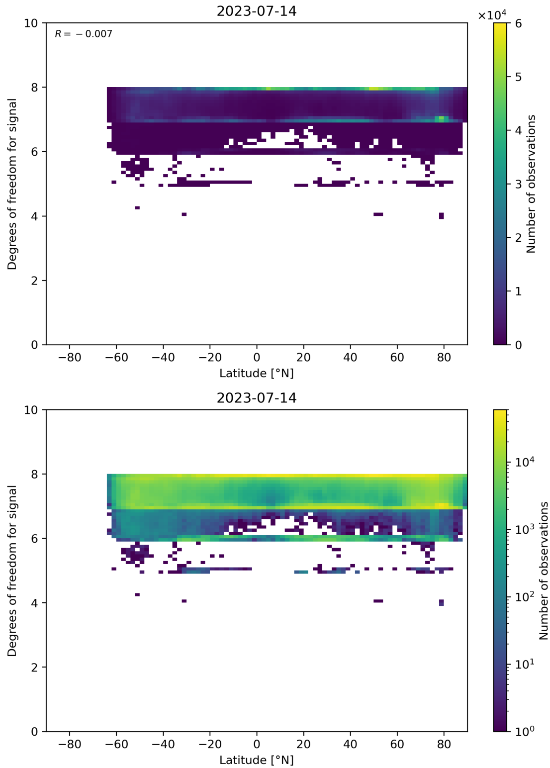
Figure 55: Scatter density plot of “Latitude” against “Degrees of freedom for signal” for 2023-07-14 to 2023-07-15.
