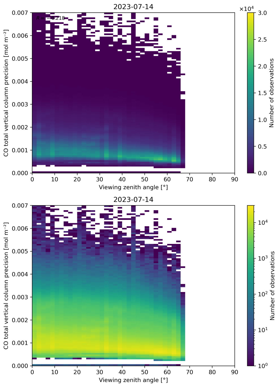
Figure 71: Scatter density plot of “Viewing zenith angle” against “CO total vertical column precision” for 2023-07-14 to 2023-07-15.
