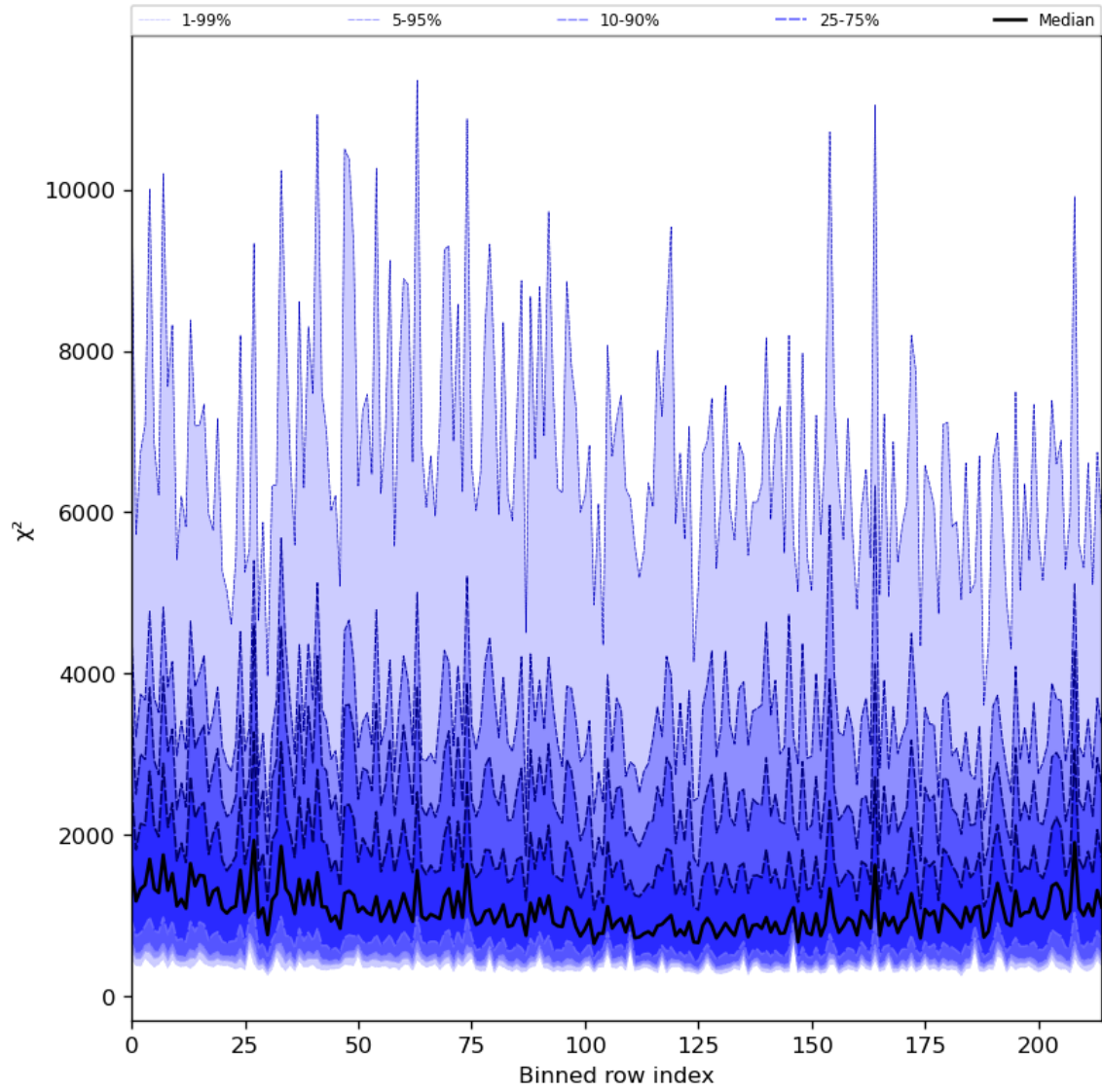
Figure 30: Along track statistics of “ \chi^2 ” for 2023-07-14 to 2023-07-15
