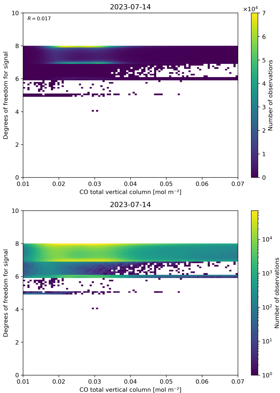
Figure 41: Scatter density plot of “CO total vertical column” against “Degrees of freedom for signal” for 2023-07-14 to 2023-07-15.
