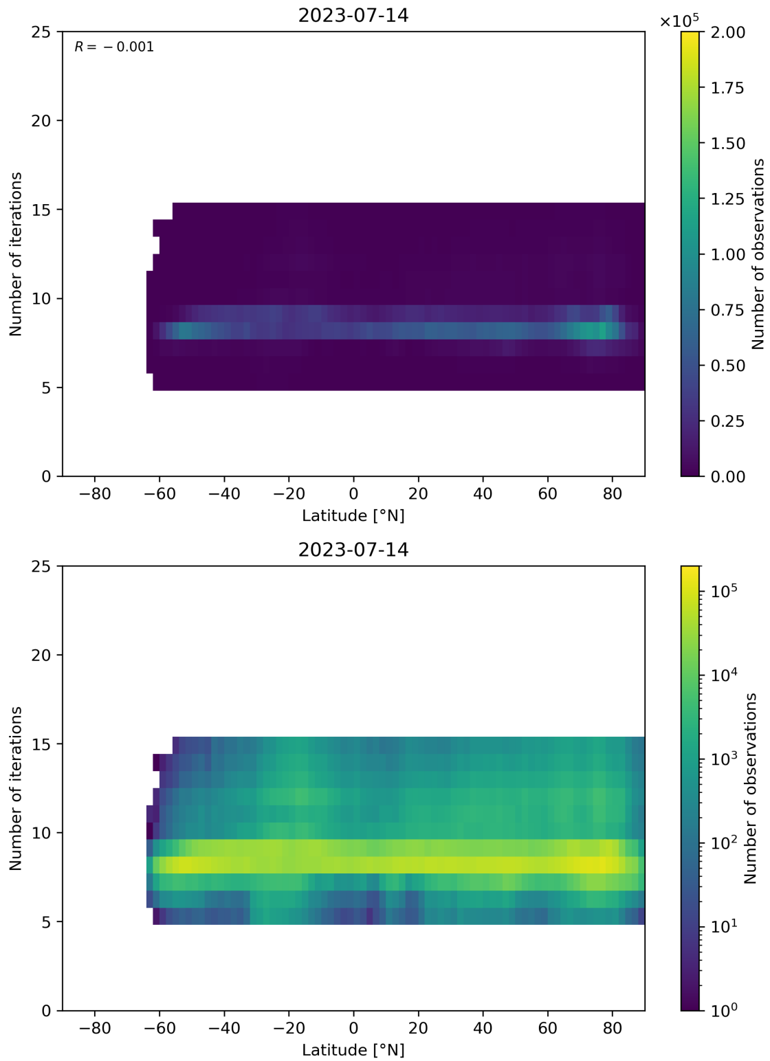
Figure 56: Scatter density plot of “Latitude” against “Number of iterations” for 2023-07-14 to 2023-07-15.
