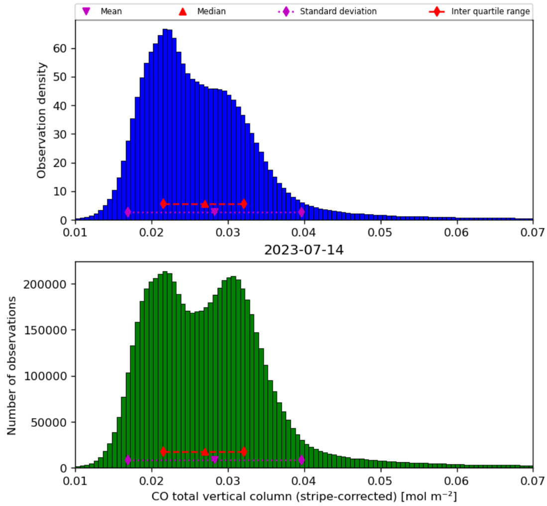
Figure 19: Histogram of “CO total vertical column (stripe-corrected)” for 2023-07-14 to 2023-07-15
