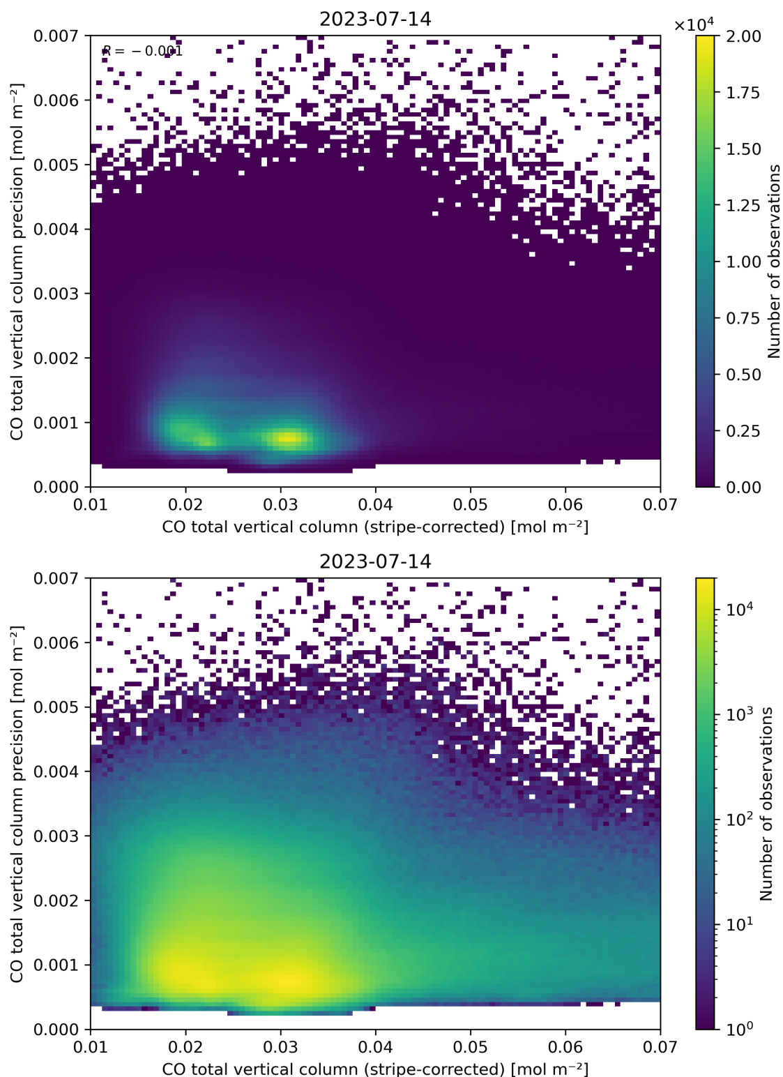
Figure 36: Scatter density plot of “CO total vertical column (stripe-corrected)” against “CO total vertical column precision” for 2023-07-14 to 2023-07-15.
