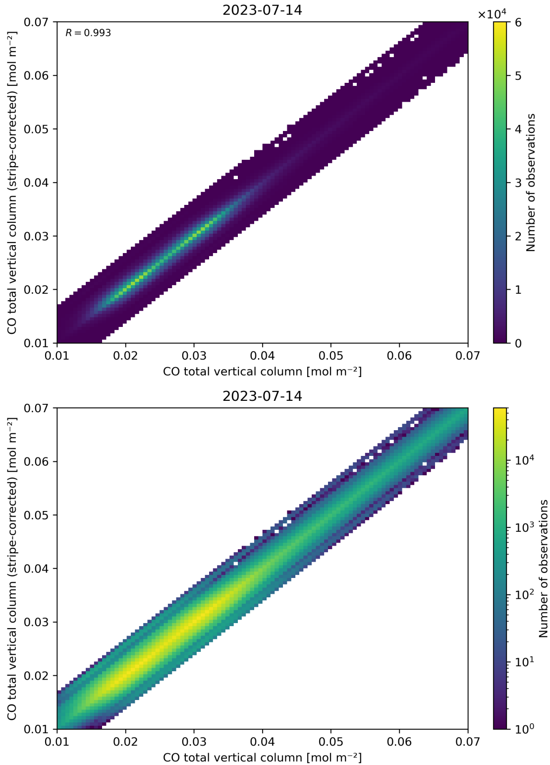
Figure 33: Scatter density plot of “CO total vertical column” against “CO total vertical column (stripe-corrected)” for 2023-07-14 to 2023-07-15.
