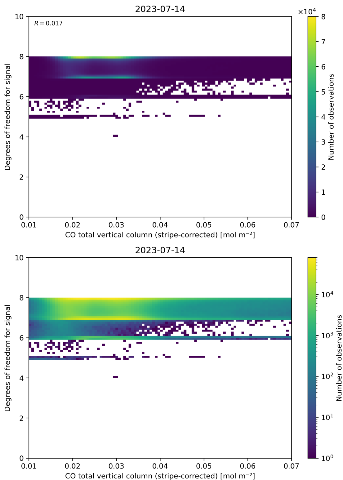
Figure 38: Scatter density plot of “CO total vertical column (stripe-corrected)” against “Degrees of freedom for signal” for 2023-07-14 to 2023-07-15.
