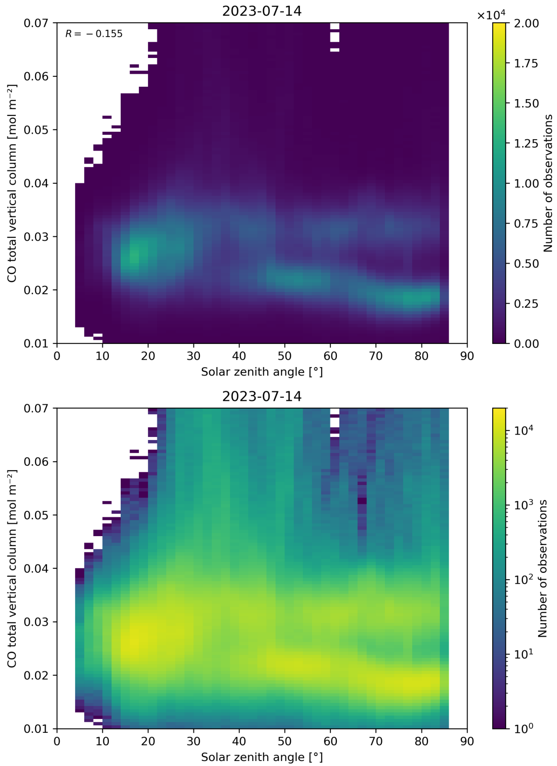
Figure 61: Scatter density plot of “Solar zenith angle” against “CO total vertical column” for 2023-07-14 to 2023-07-15.
