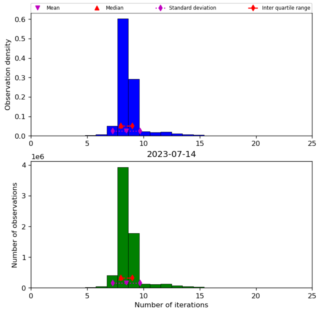
Figure 24: Histogram of “Number of iterations” for 2023-07-14 to 2023-07-15
