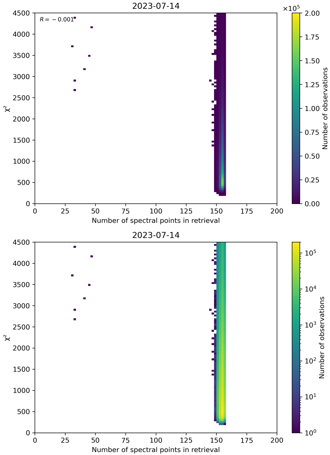
Figure 58: Scatter density plot of “Number of spectral points in retrieval” against “ \chi^2 ” for 2023-07-14 to 2023-07-15.
