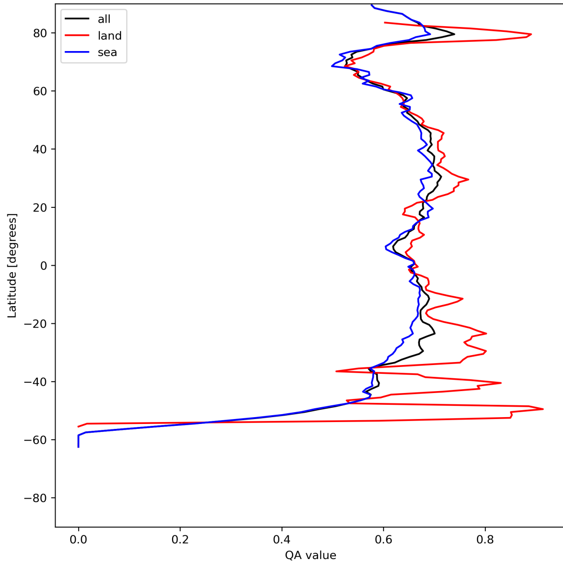
Figure 9: Zonal average of “QA value” for 2023-07-14 to 2023-07-15.
