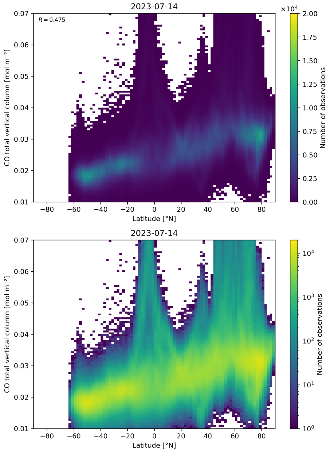
Figure 51: Scatter density plot of “Latitude” against “CO total vertical column” for 2023-07-14 to 2023-07-15.
