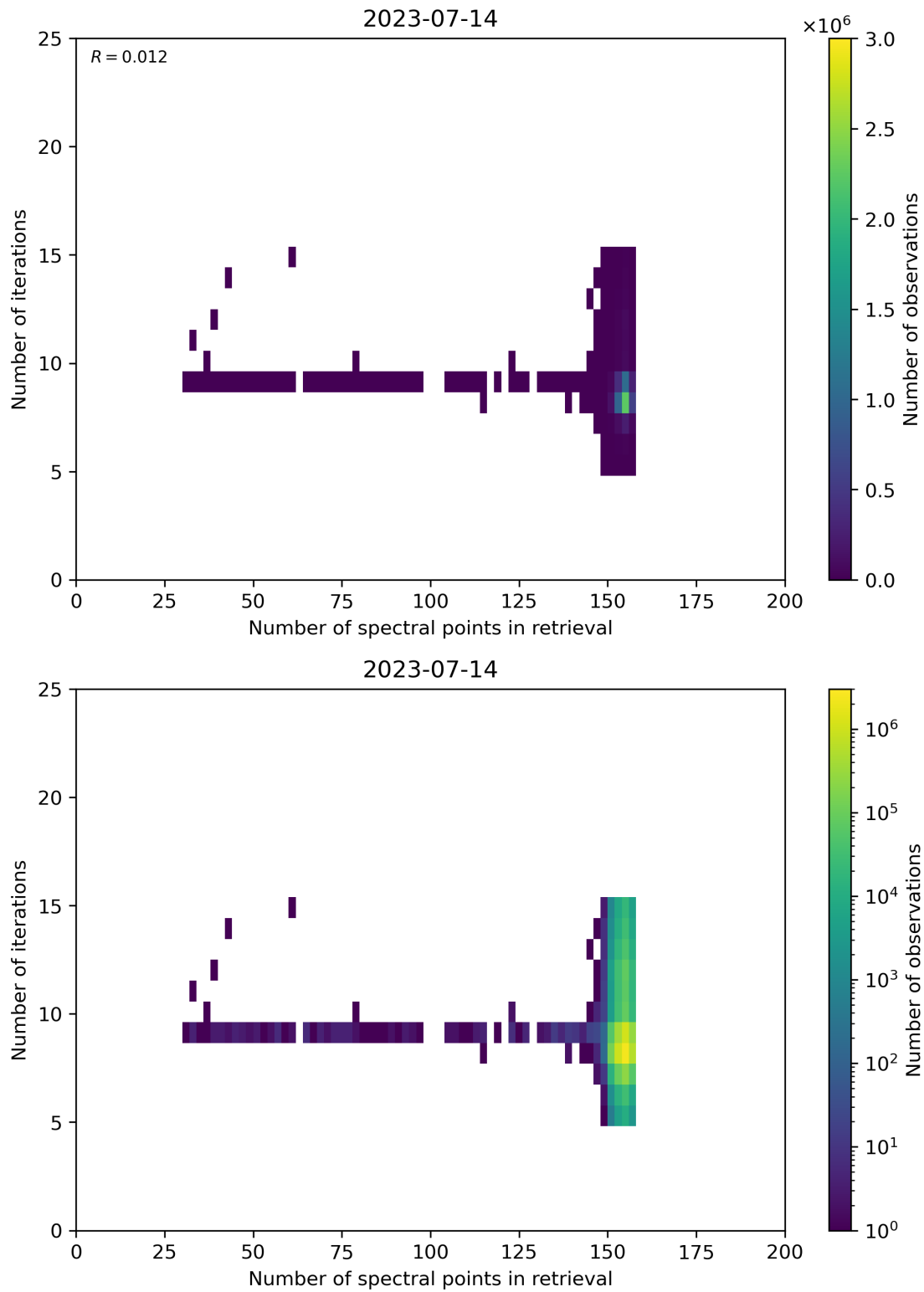
Figure 60: Scatter density plot of “Number of spectral points in retrieval” against “Number of iterations” for 2023-07-14 to 2023-07-15.
