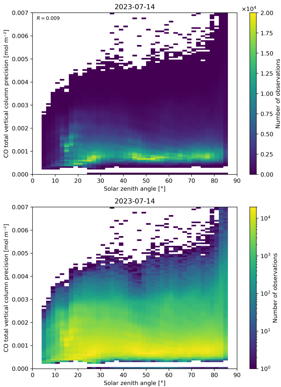
Figure 63: Scatter density plot of “Solar zenith angle” against “CO total vertical column precision” for 2023-07-14 to 2023-07-15.
