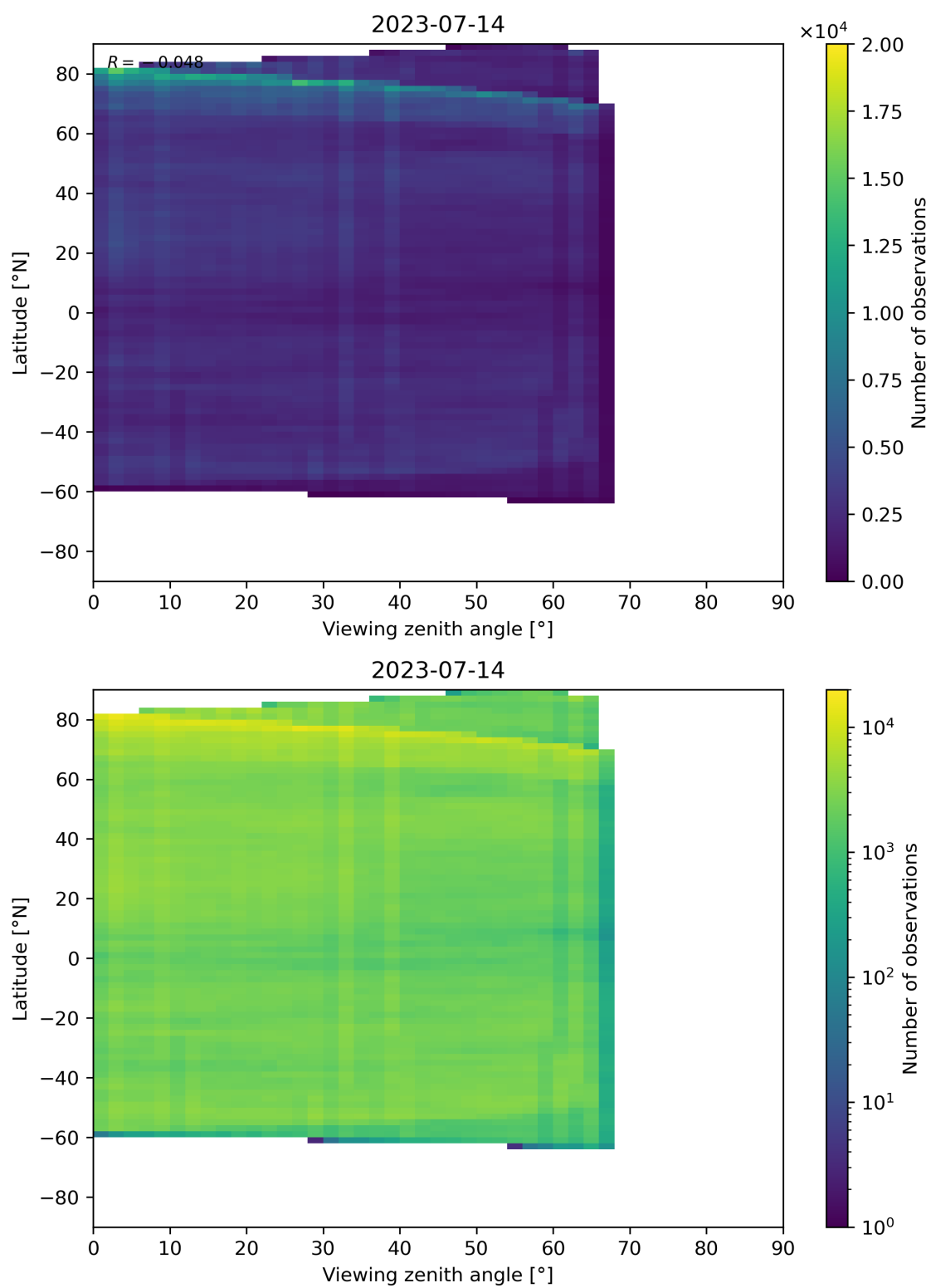
Figure 74: Scatter density plot of “Viewing zenith angle” against “Latitude” for 2023-07-14 to 2023-07-15.
