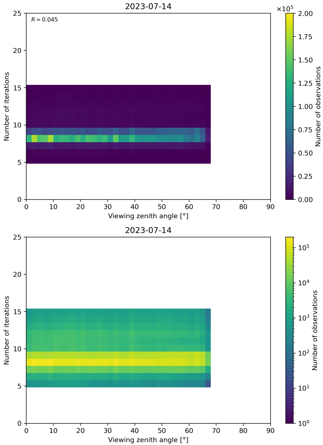
Figure 75: Scatter density plot of “Viewing zenith angle” against “Number of iterations” for 2023-07-14 to 2023-07-15.
