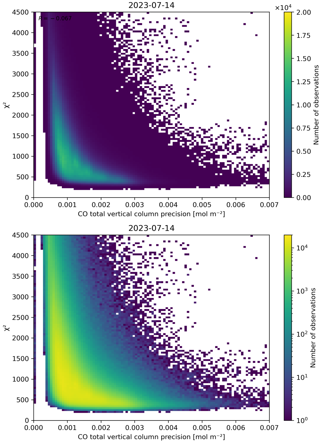
Figure 44: Scatter density plot of “CO total vertical column precision” against “ \chi^2 ” for 2023-07-14 to 2023-07-15.
