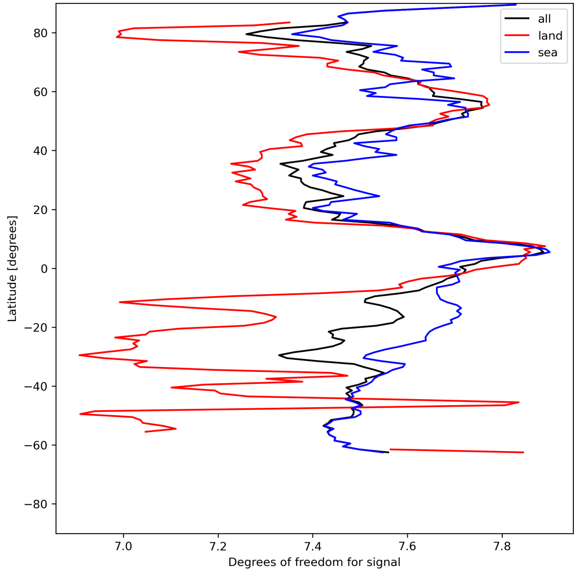
Figure 15: Zonal average of “Degrees of freedom for signal” for 2023-07-14 to 2023-07-15.
