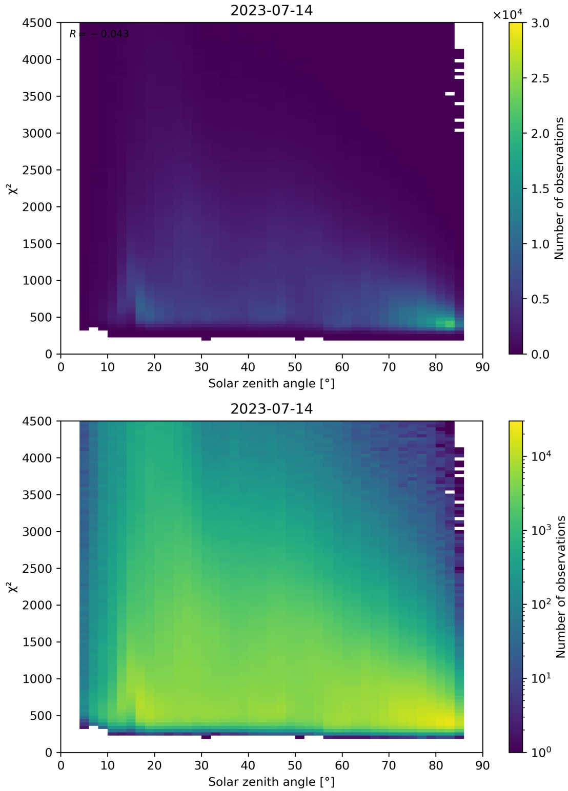
Figure 64: Scatter density plot of “Solar zenith angle” against “ \chi^2 ” for 2023-07-14 to 2023-07-15.
