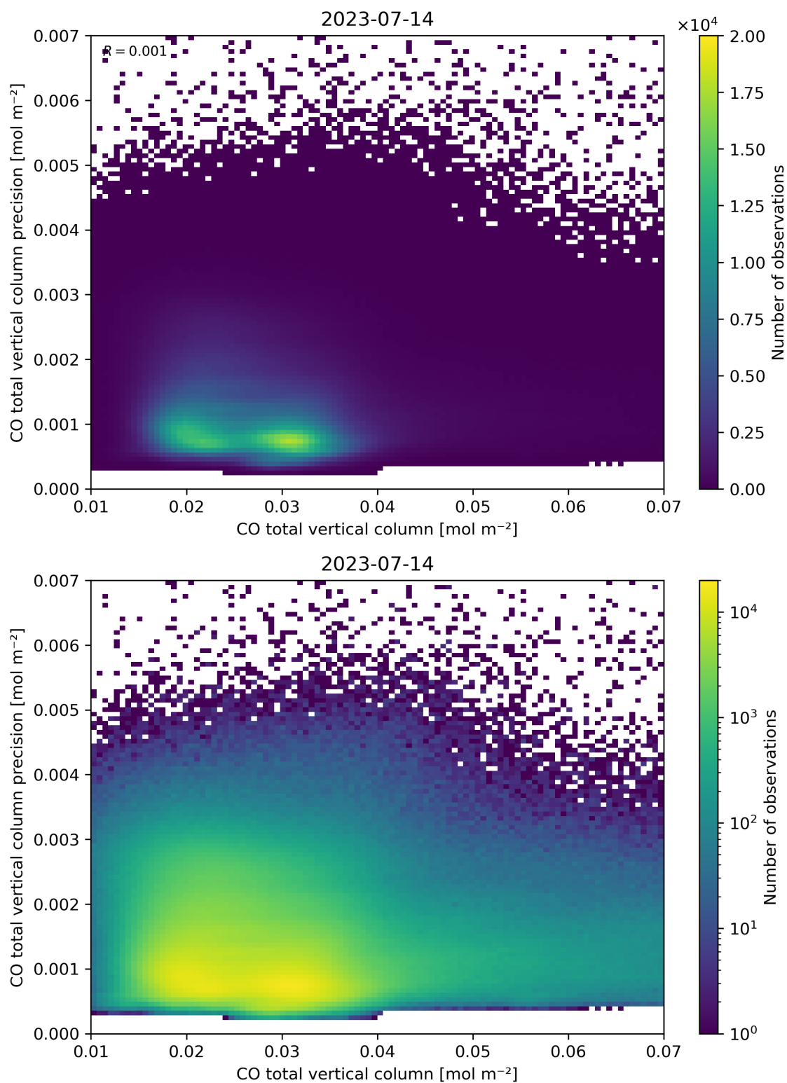
Figure 34: Scatter density plot of “CO total vertical column” against “CO total vertical column precision” for 2023-07-14 to 2023-07-15.
