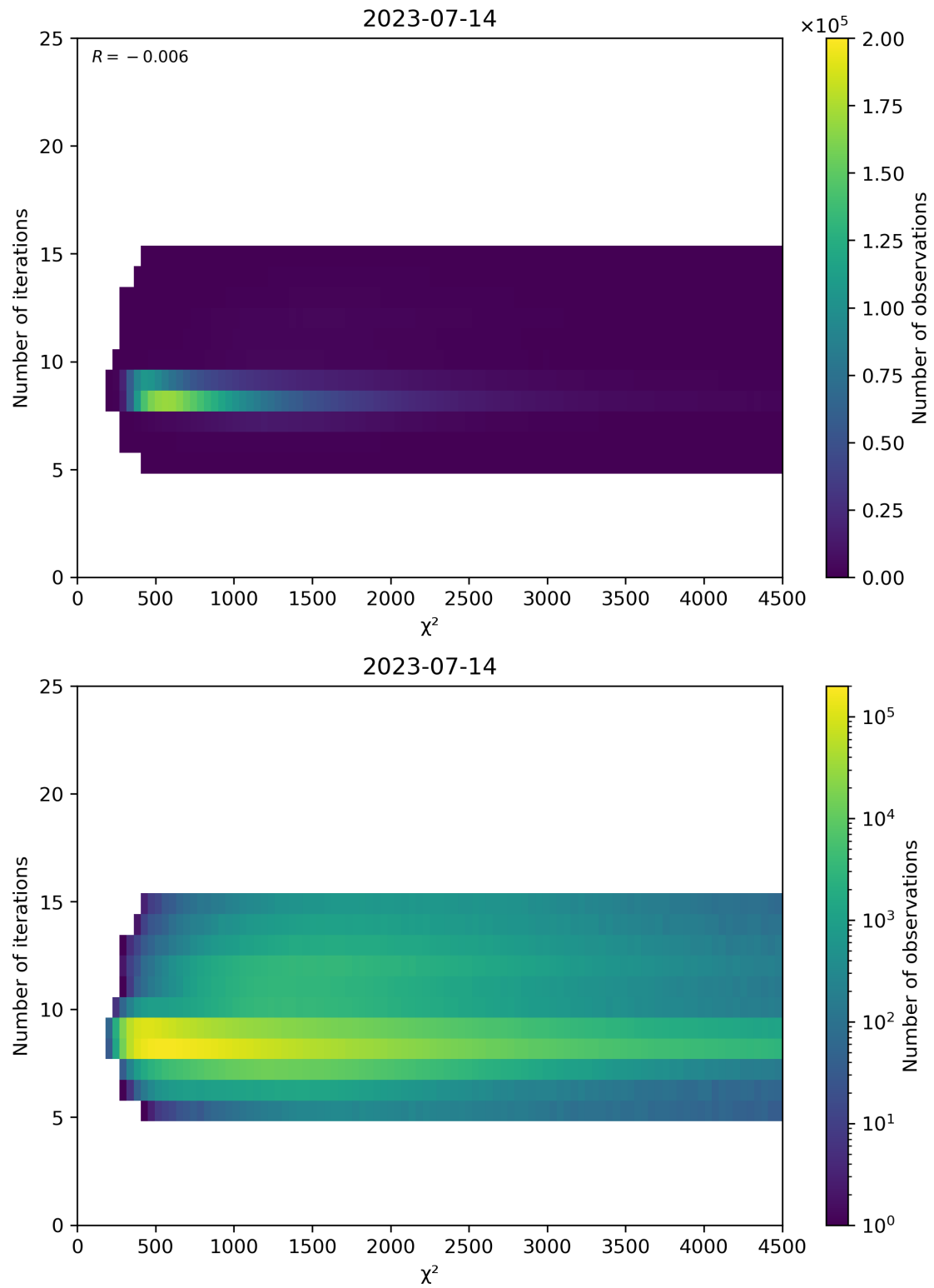
Figure 49: Scatter density plot of “ \chi^2 ” against “Number of iterations” for 2023-07-14 to 2023-07-15.
