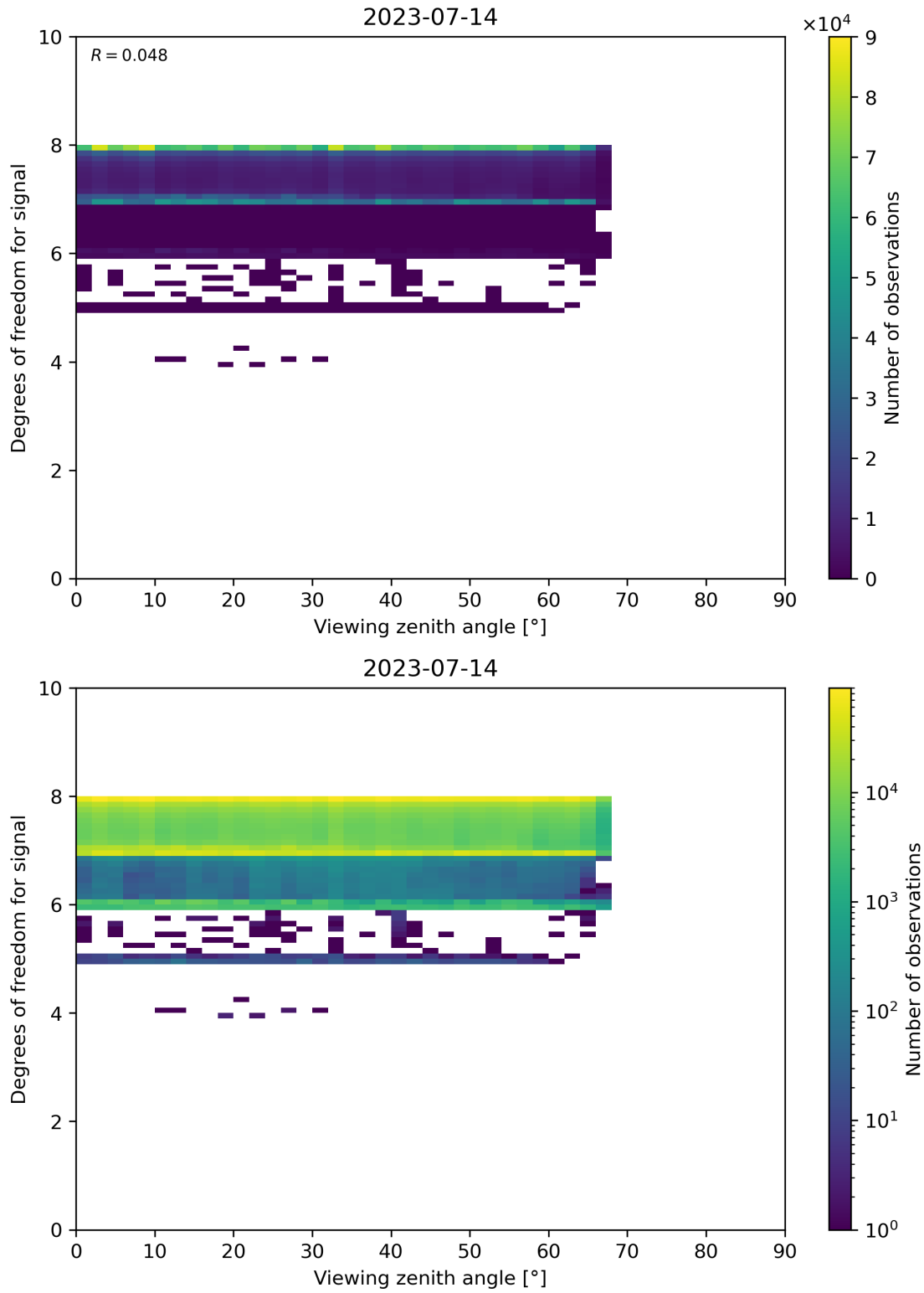
Figure 73: Scatter density plot of “Viewing zenith angle” against “Degrees of freedom for signal” for 2023-07-14 to 2023-07-15.
