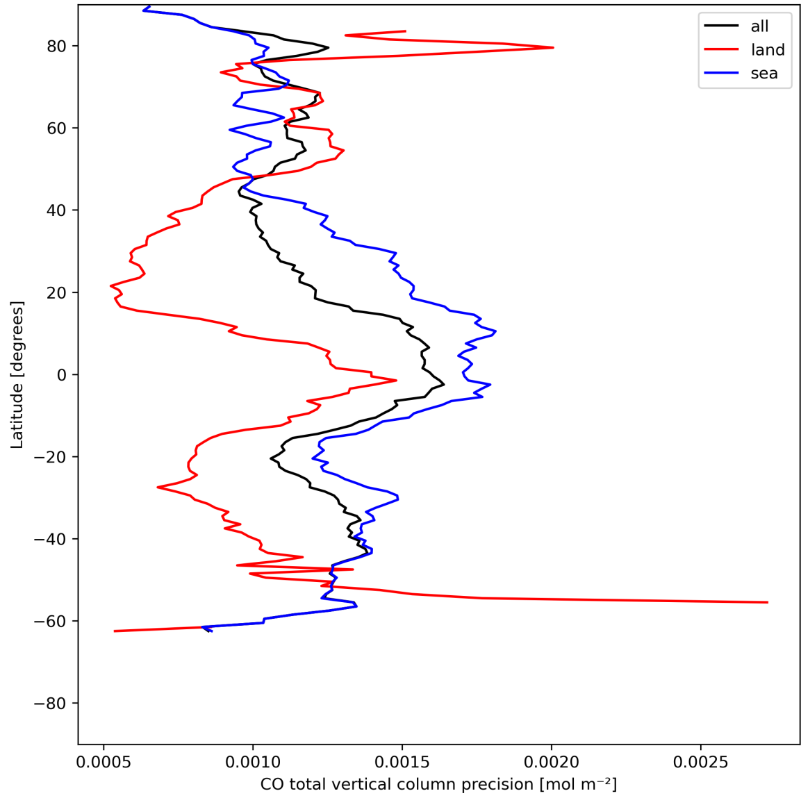
Figure 12: Zonal average of “CO total vertical column precision” for 2023-07-14 to 2023-07-15.
