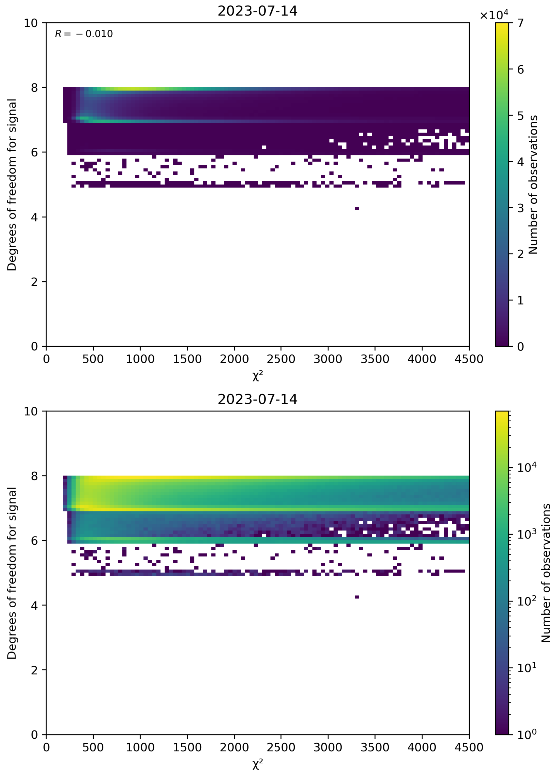
Figure 48: Scatter density plot of " \chi^2 " against "Degrees of freedom for signal" for 2023-07-14 to 2023-07-15.
