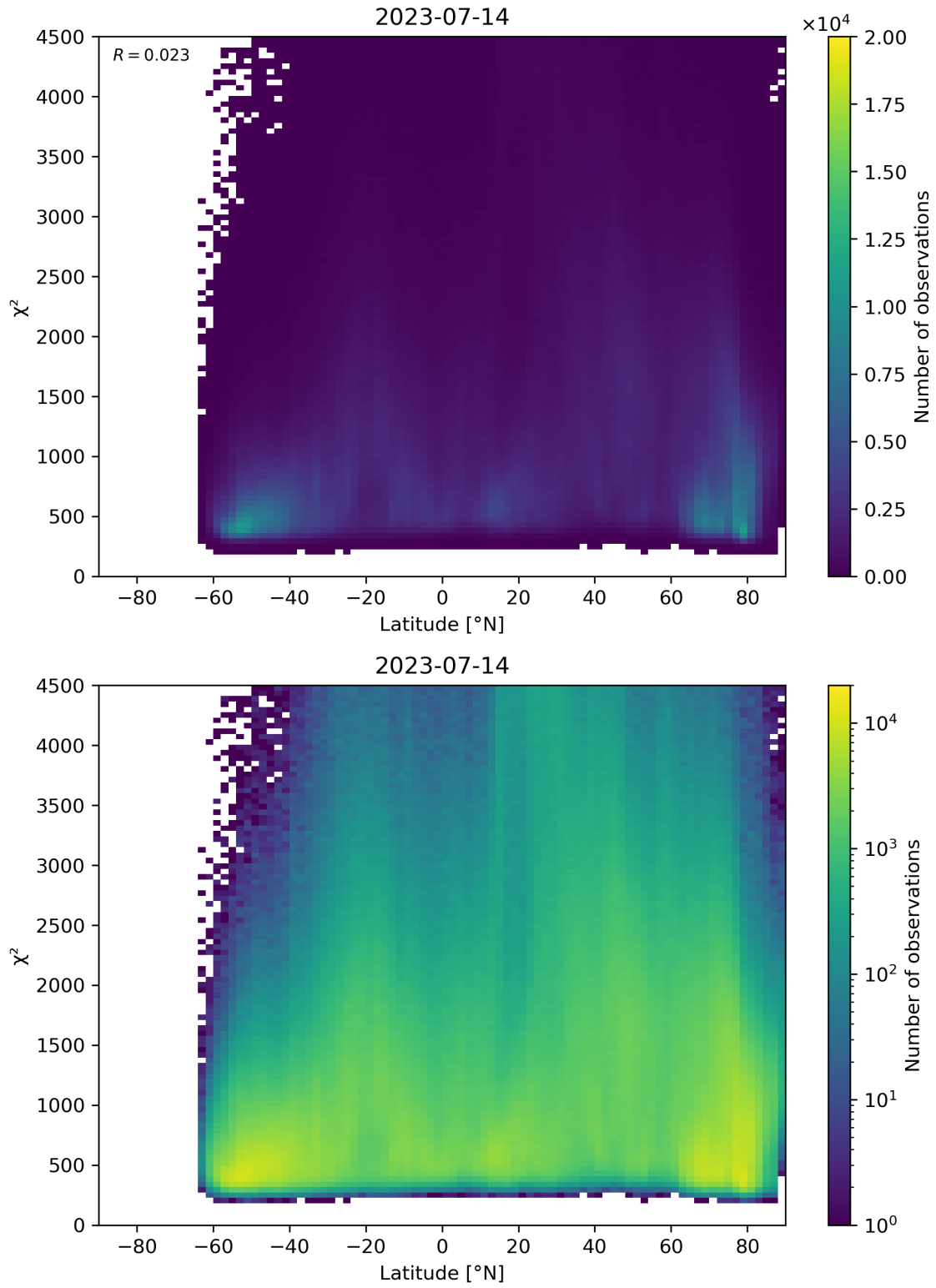
Figure 54: Scatter density plot of “Latitude” against “ \chi^2 ” for 2023-07-14 to 2023-07-15.
