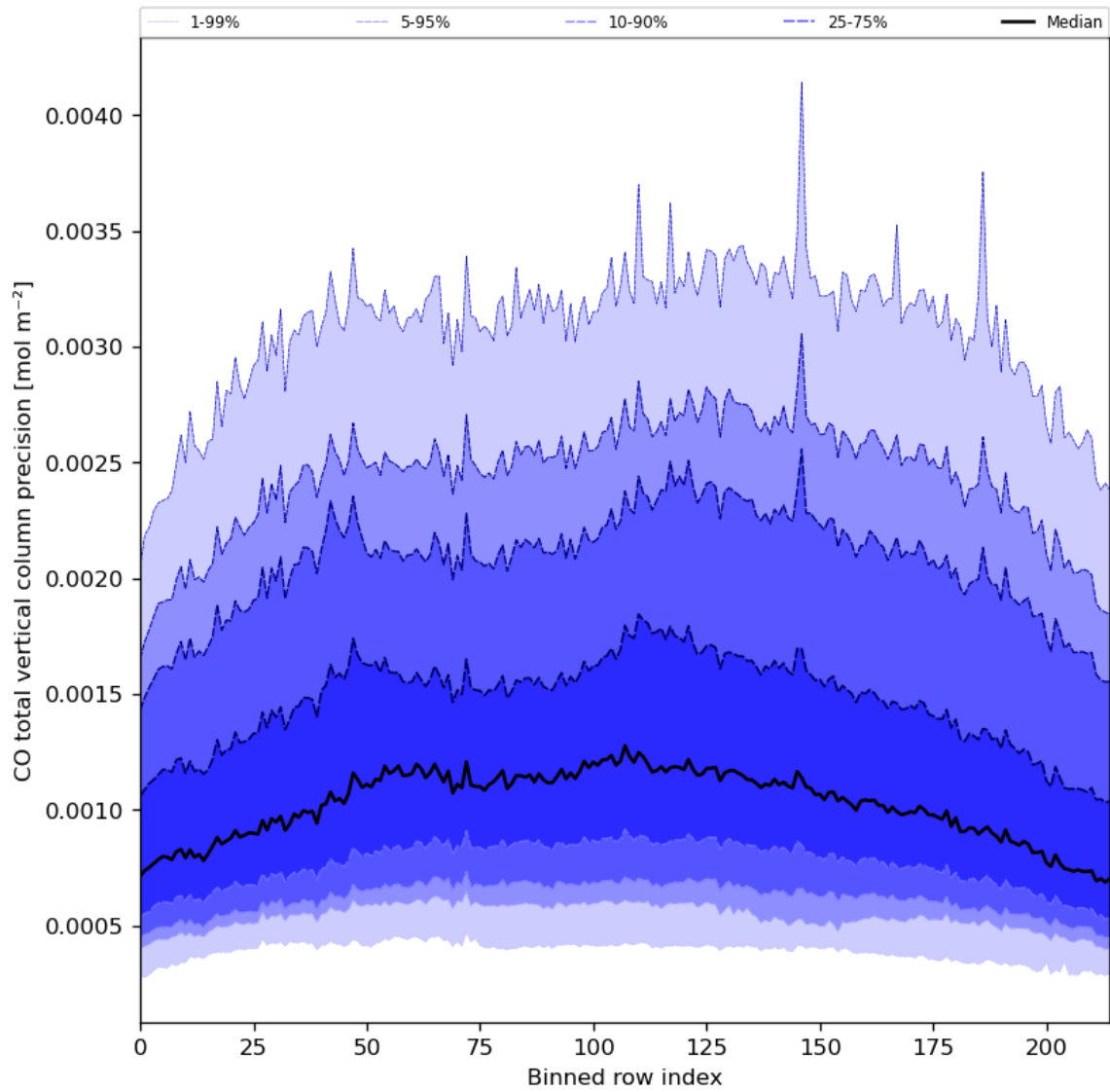
Figure 28: Along track statistics of “CO total vertical column precision” for 2023-07-14 to 2023-07-15
