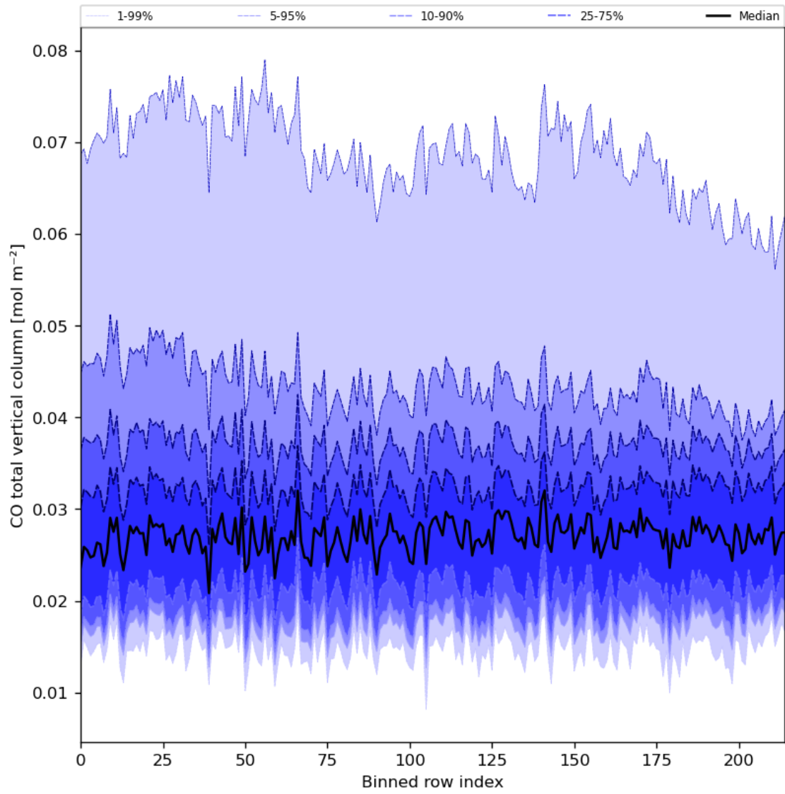
Figure 26: Along track statistics of “CO total vertical column” for 2023-07-14 to 2023-07-15
