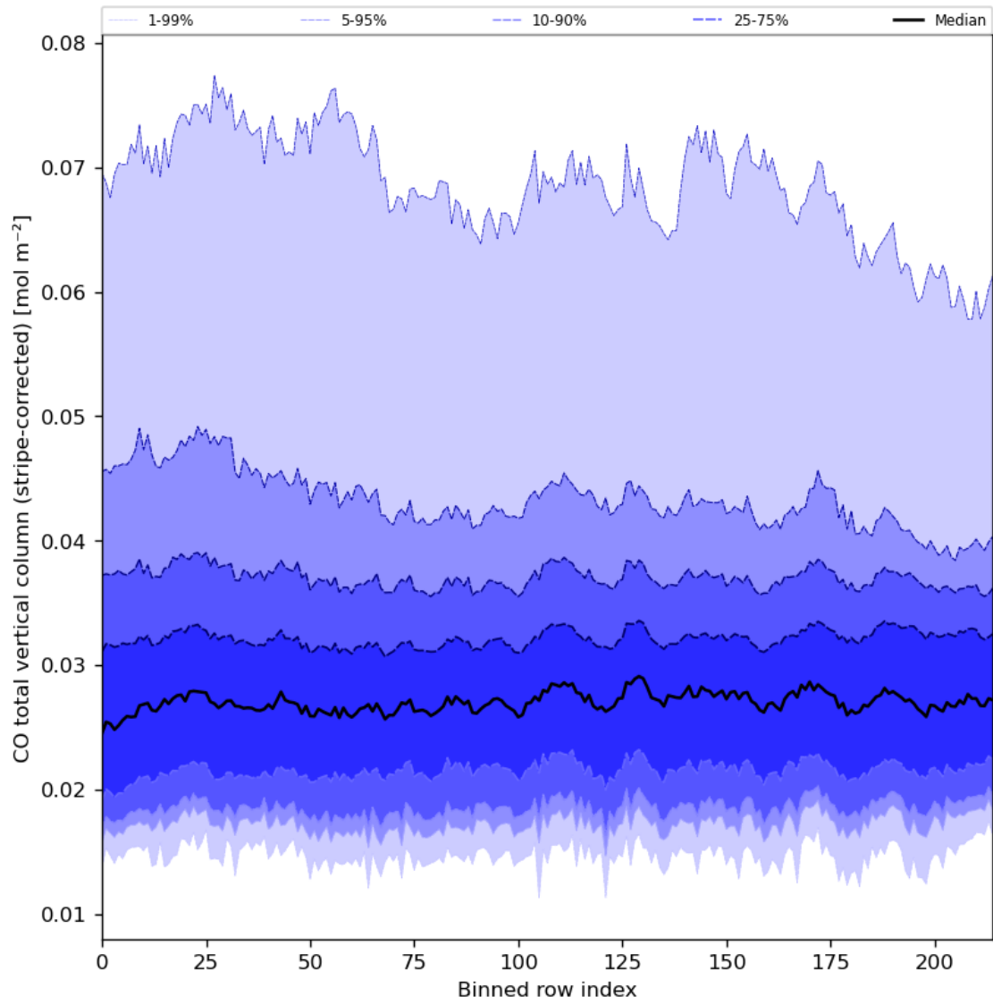
Figure 27: Along track statistics of “CO total vertical column (stripe-corrected)” for 2023-07-14 to 2023-07-15
