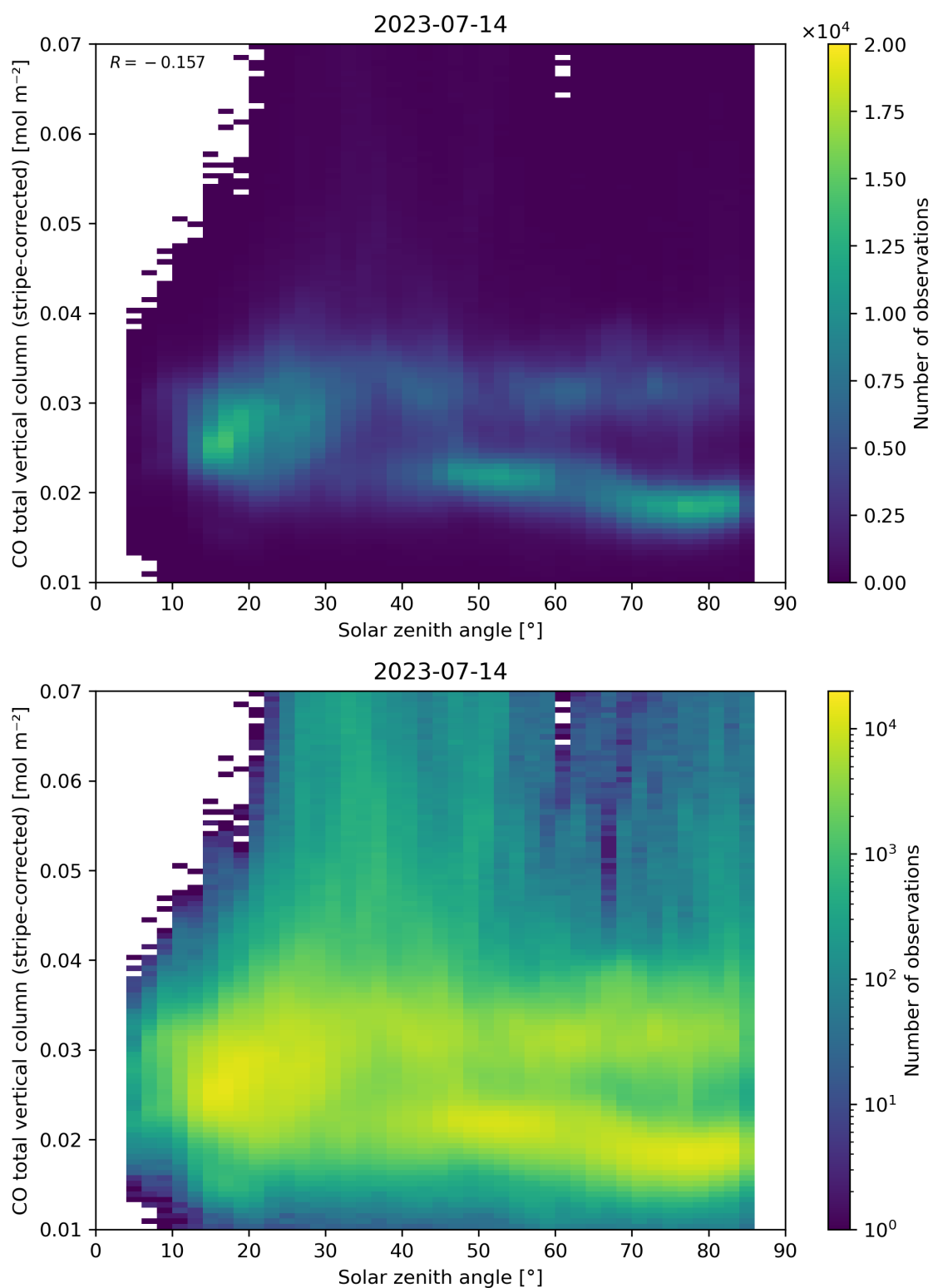
Figure 62: Scatter density plot of “Solar zenith angle” against “CO total vertical column (stripe-corrected)” for 2023-07-14 to 2023-07-15.
