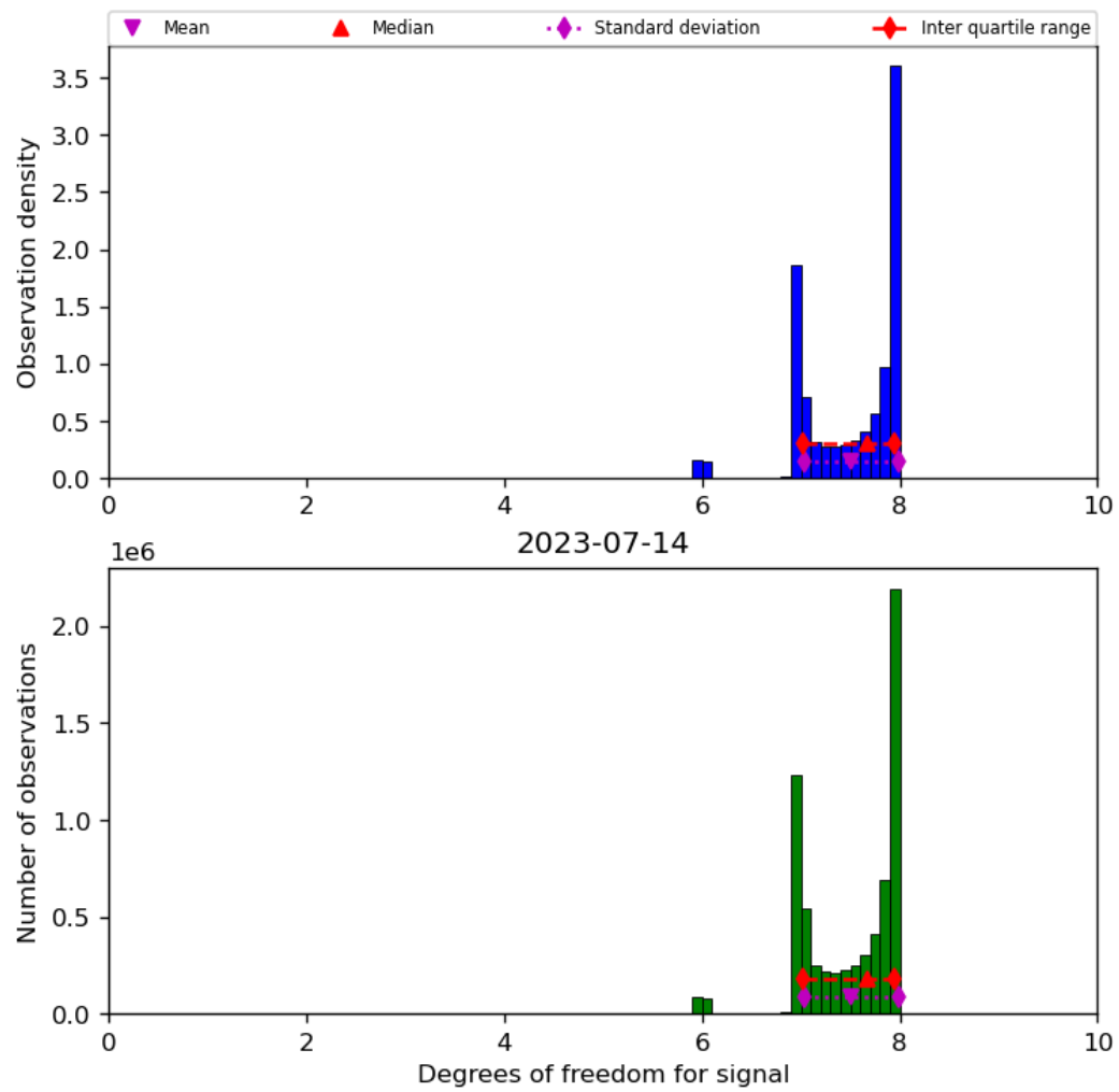
Figure 23: Histogram of “Degrees of freedom for signal” for 2023-07-14 to 2023-07-15
