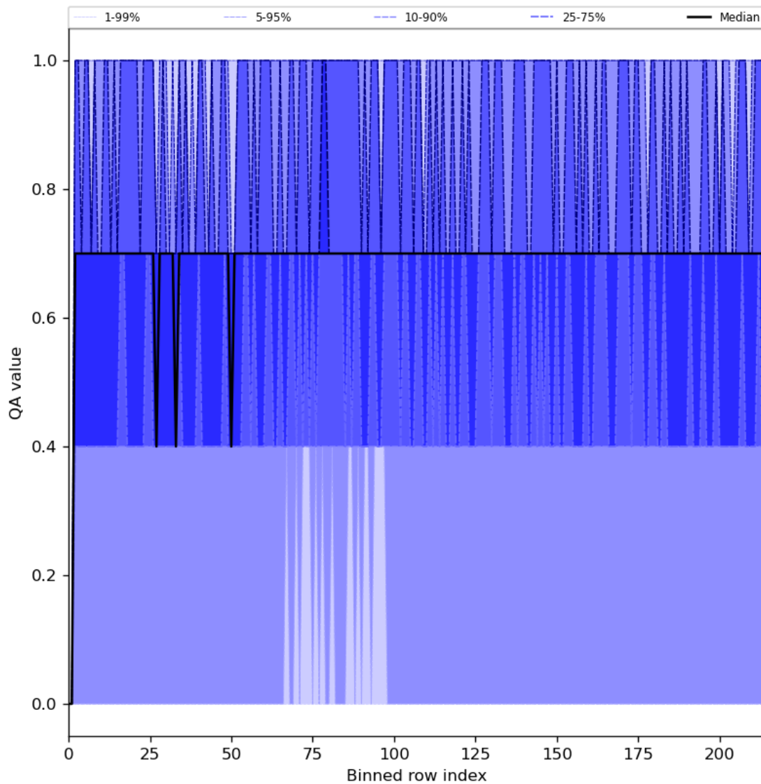
Figure 25: Along track statistics of “QA value” for 2023-07-14 to 2023-07-15
