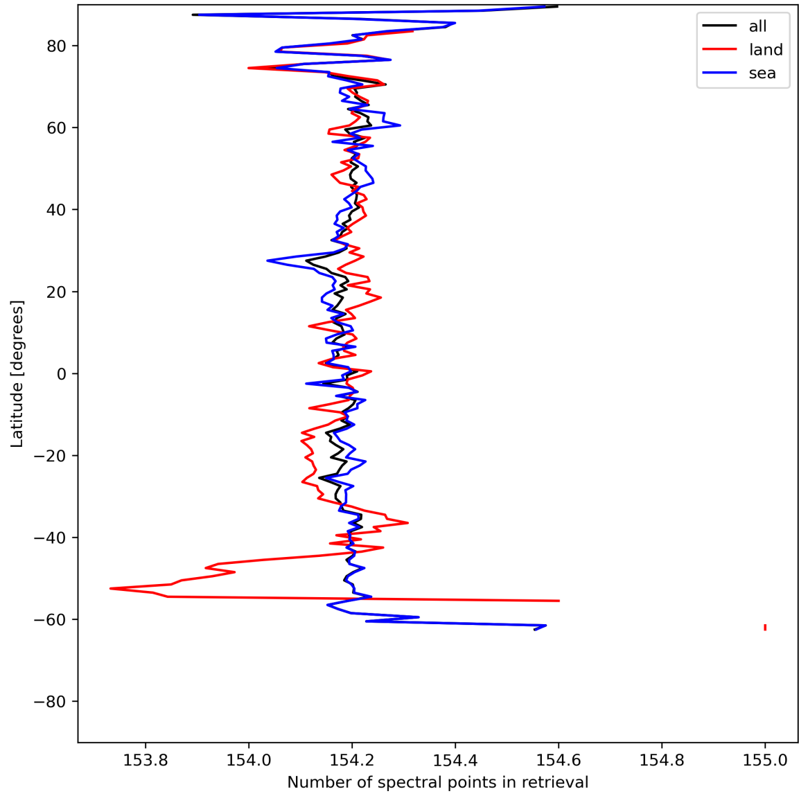
Figure 13: Zonal average of “Number of spectral points in retrieval” for 2023-07-14 to 2023-07-15.
