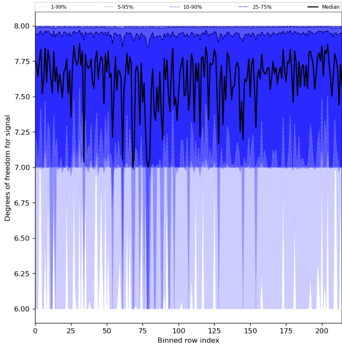
Figure 31: Along track statistics of “Degrees of freedom for signal” for 2023-07-14 to 2023-07-15
