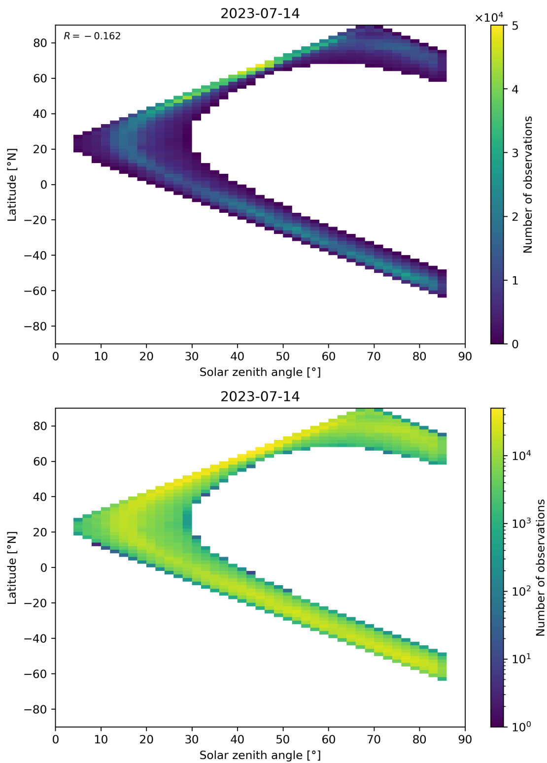
Figure 66: Scatter density plot of “Solar zenith angle” against “Latitude” for 2023-07-14 to 2023-07-15.
