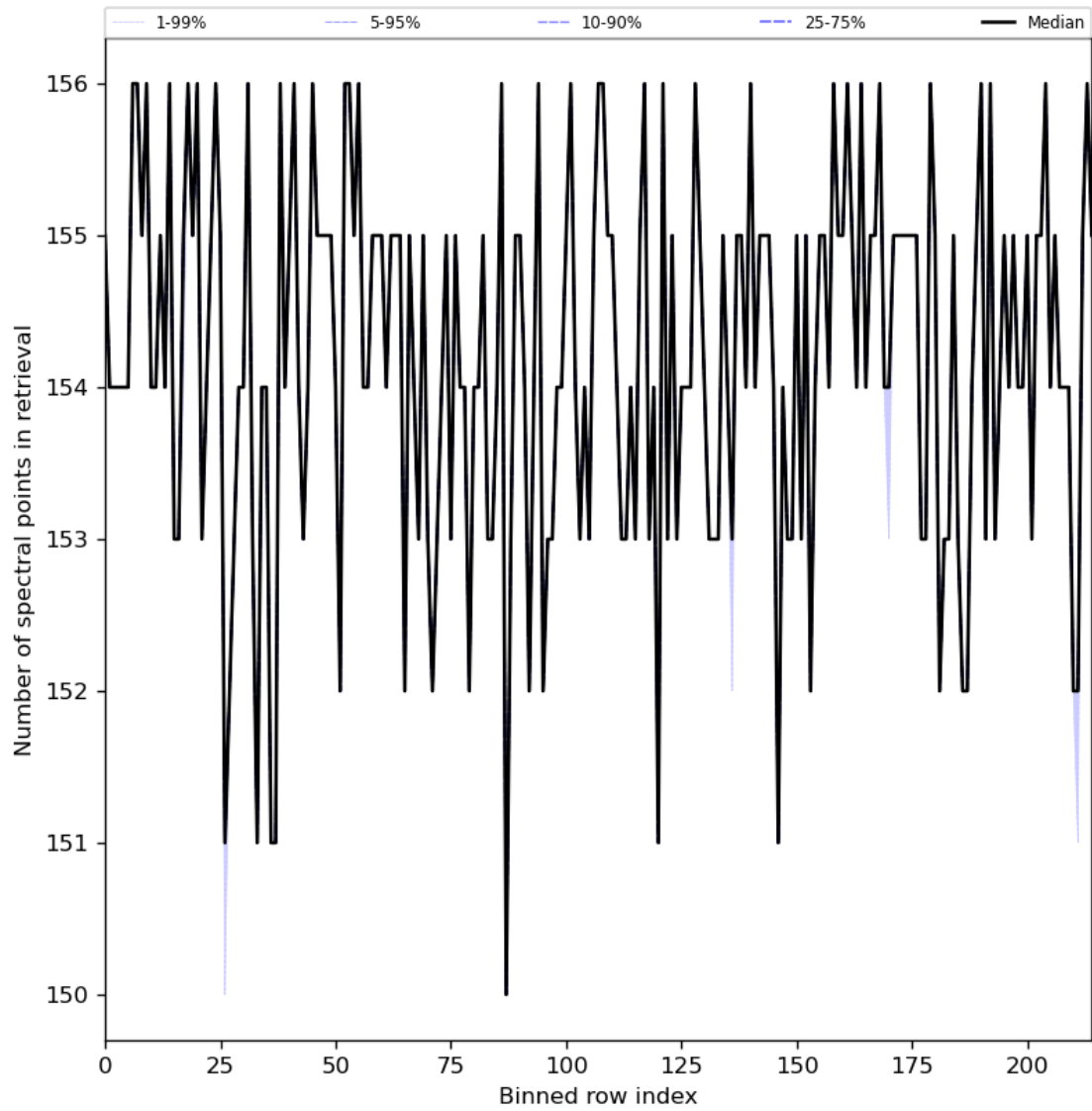
Figure 29: Along track statistics of “Number of spectral points in retrieval” for 2023-07-14 to 2023-07-15
