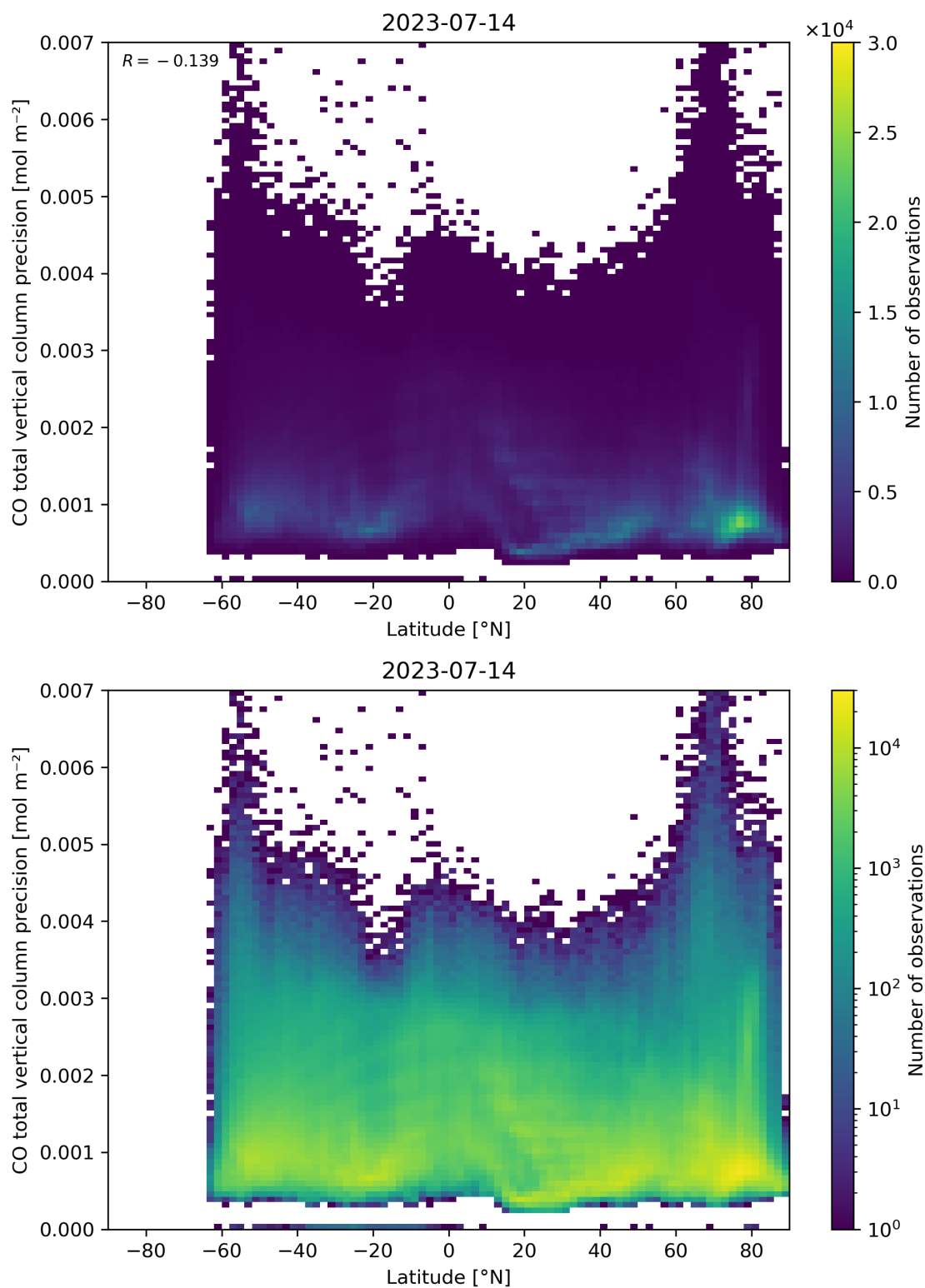
Figure 53: Scatter density plot of “Latitude” against “CO total vertical column precision” for 2023-07-14 to 2023-07-15.
