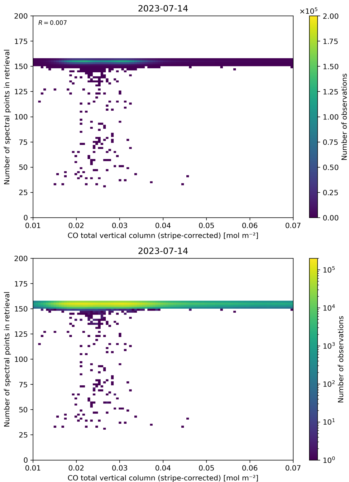
Figure 40: Scatter density plot of “CO total vertical column (stripe-corrected)” against “Number of spectral points in retrieval” for 2023-07-14 to 2023-07-15.
