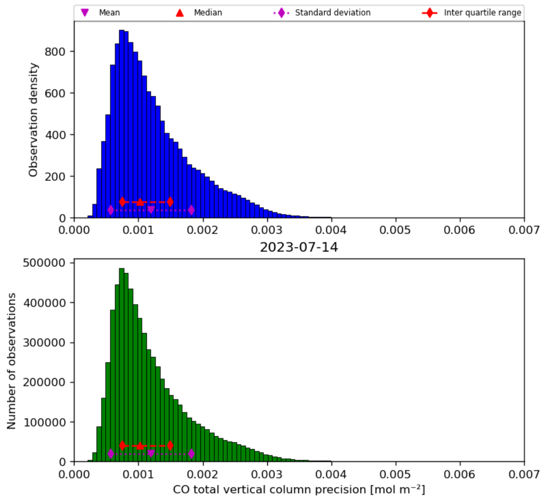
Figure 20: Histogram of “CO total vertical column precision” for 2023-07-14 to 2023-07-15
