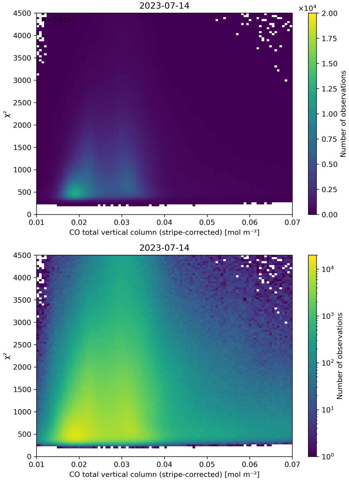
Figure 37: Scatter density plot of “CO total vertical column (stripe-corrected)” against “ \chi^2 ” for 2023-07-14 to 2023-07-15.
