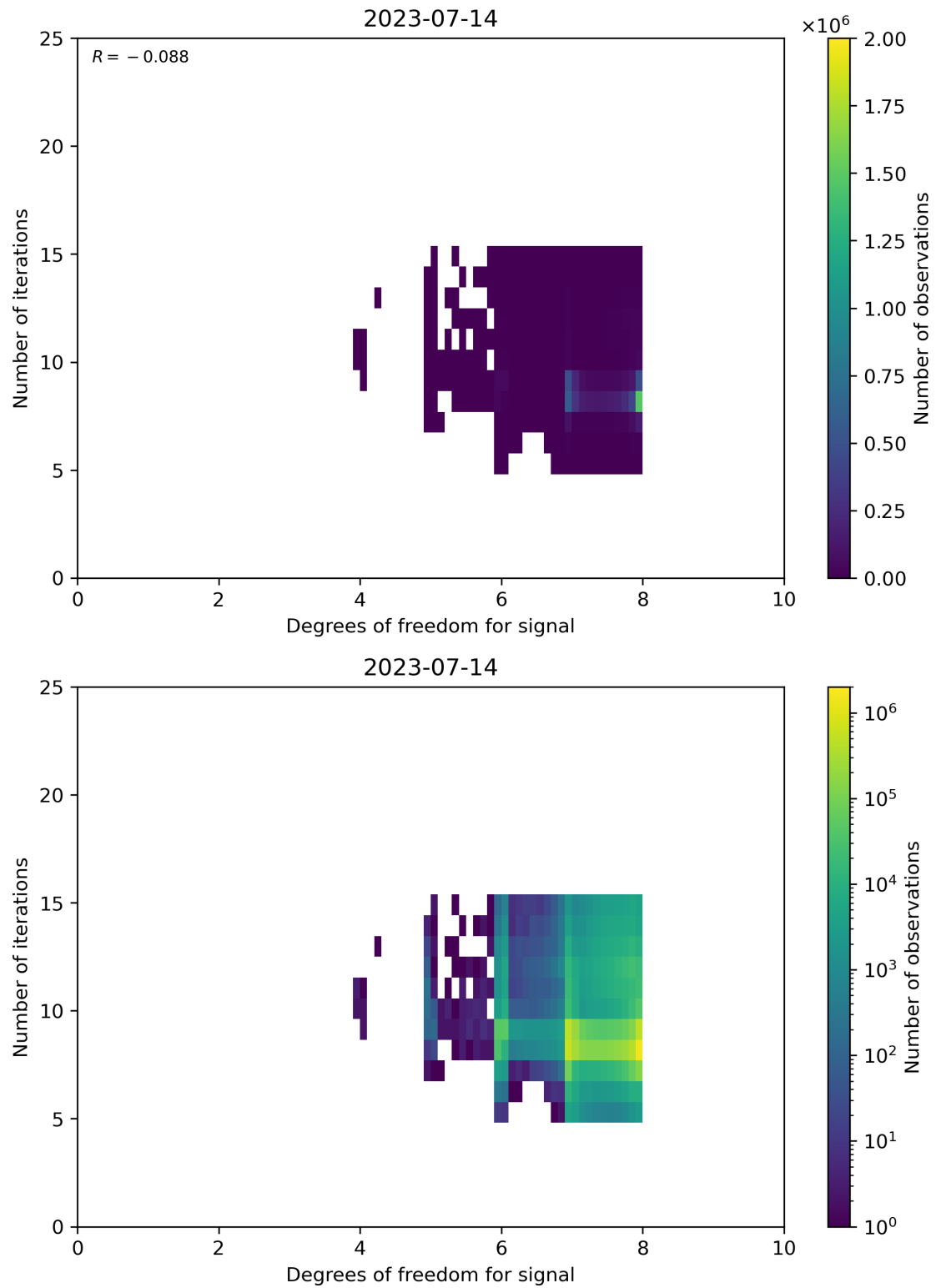
Figure 50: Scatter density plot of “Degrees of freedom for signal” against “Number of iterations” for 2023-07-14 to 2023-07-15.
