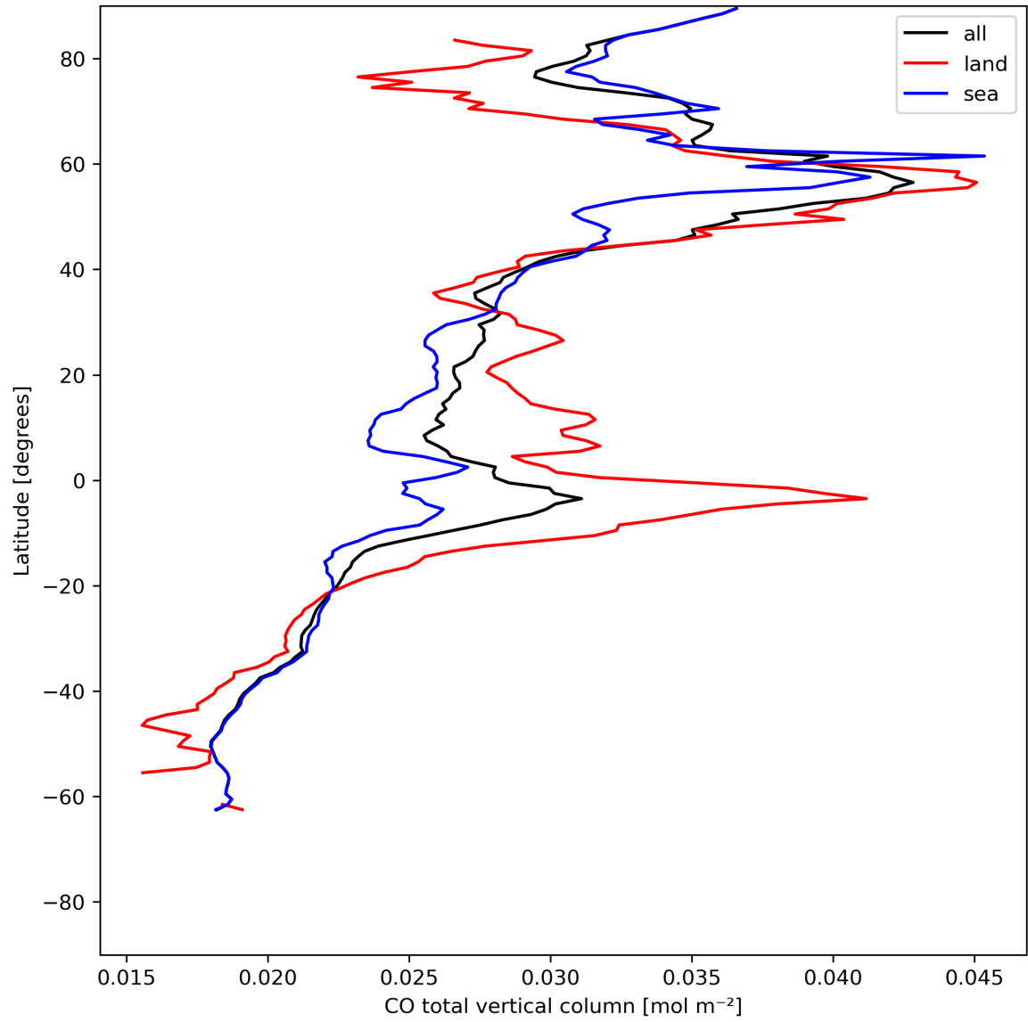
Figure 10: Zonal average of “CO total vertical column” for 2023-07-14 to 2023-07-15.
