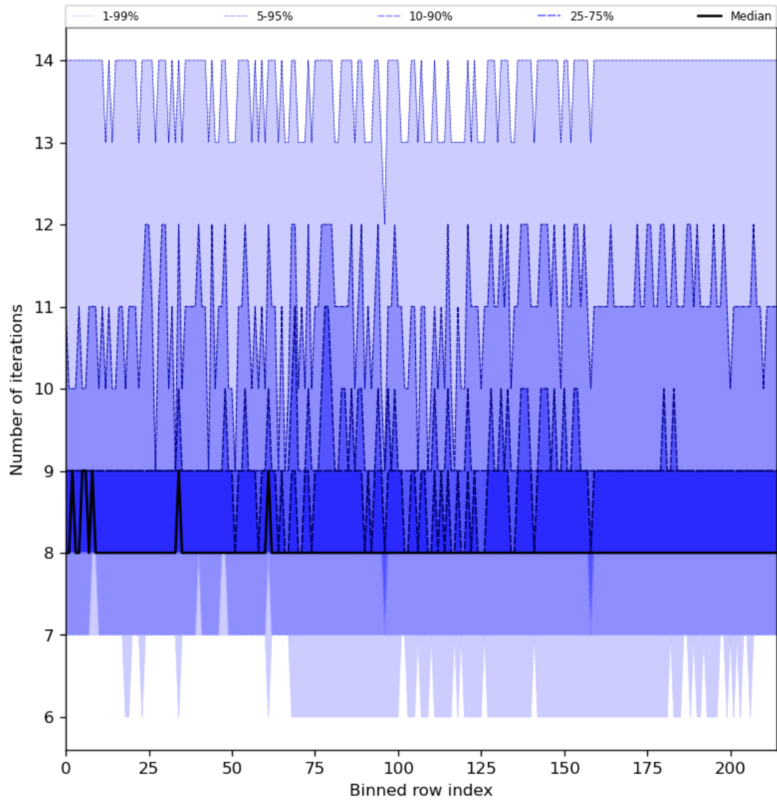
Figure 32: Along track statistics of “Number of iterations” for 2023-07-14 to 2023-07-15
