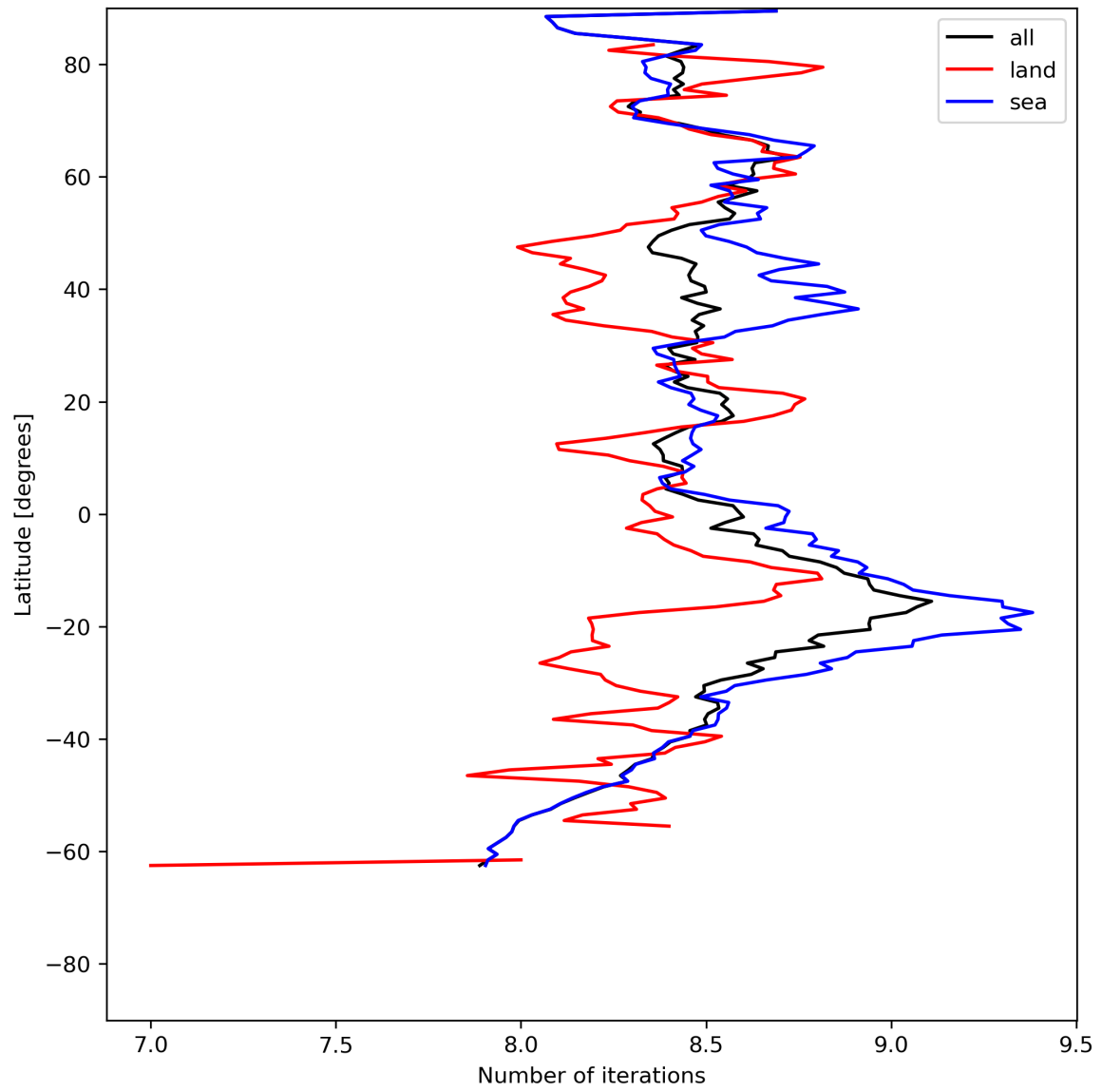
Figure 16: Zonal average of “Number of iterations” for 2023-07-14 to 2023-07-15.
