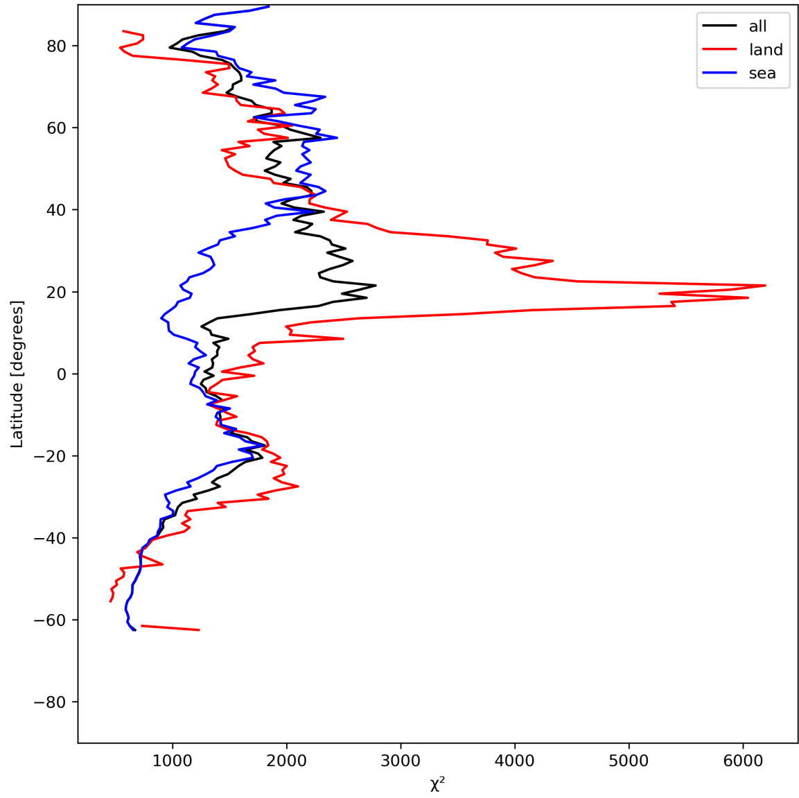
Figure 14: Zonal average of “ \chi^2 ” for 2023-07-14 to 2023-07-15.
