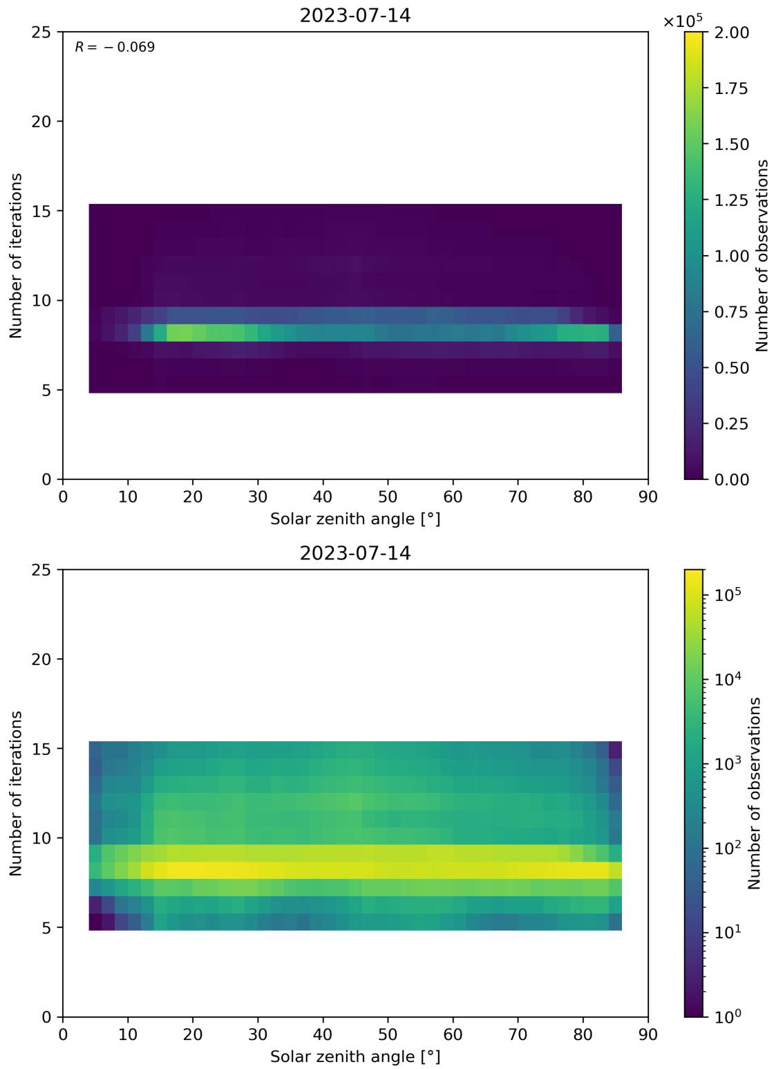
Figure 67: Scatter density plot of “Solar zenith angle” against “Number of iterations” for 2023-07-14 to 2023-07-15.
