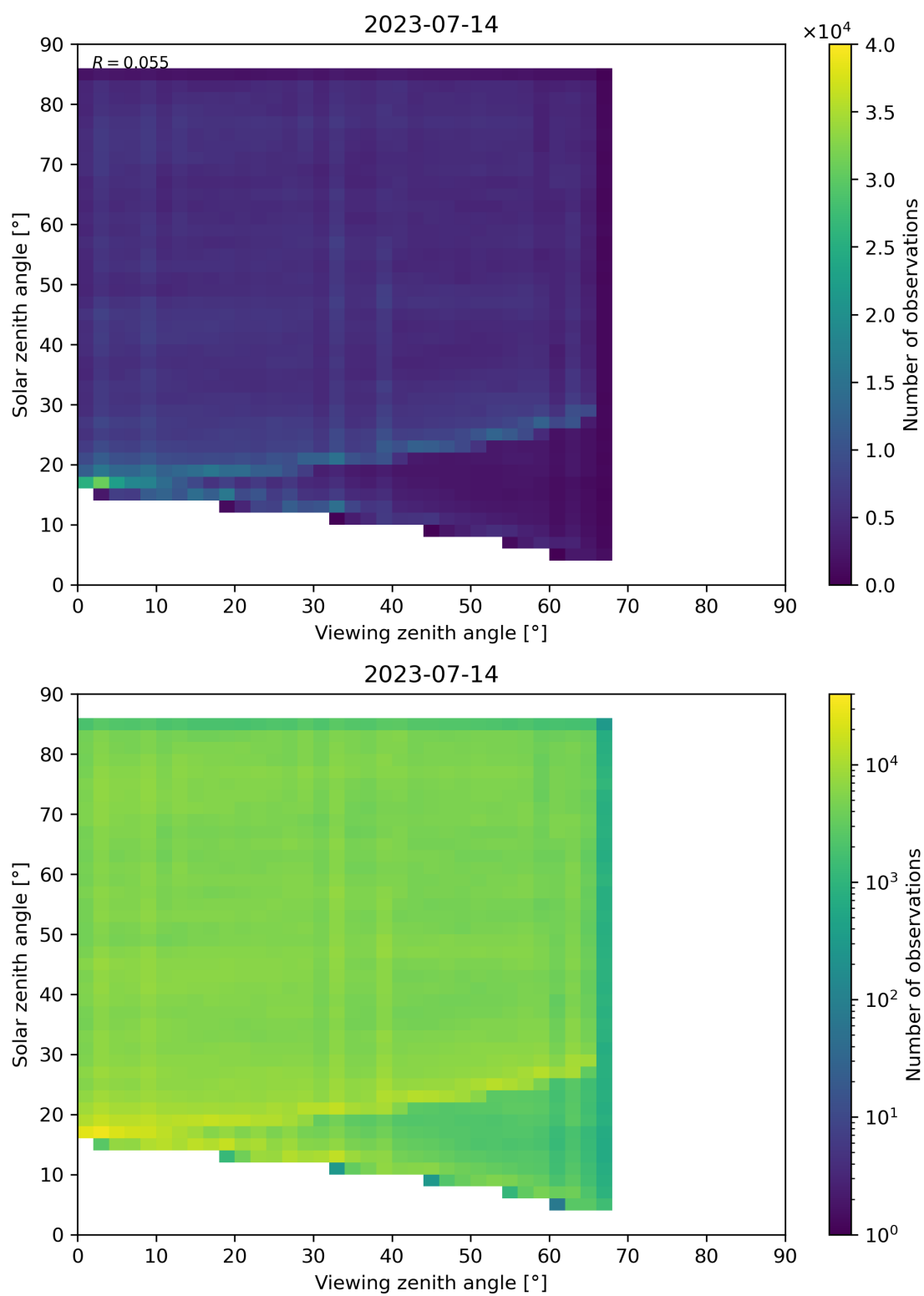
Figure 77: Scatter density plot of “Viewing zenith angle” against “Solar zenith angle” for 2023-07-14 to 2023-07-15.
