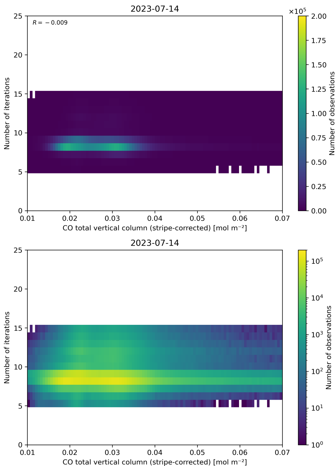
Figure 39: Scatter density plot of “CO total vertical column (stripe-corrected)” against “Number of iterations” for 2023-07-14 to 2023-07-15.
