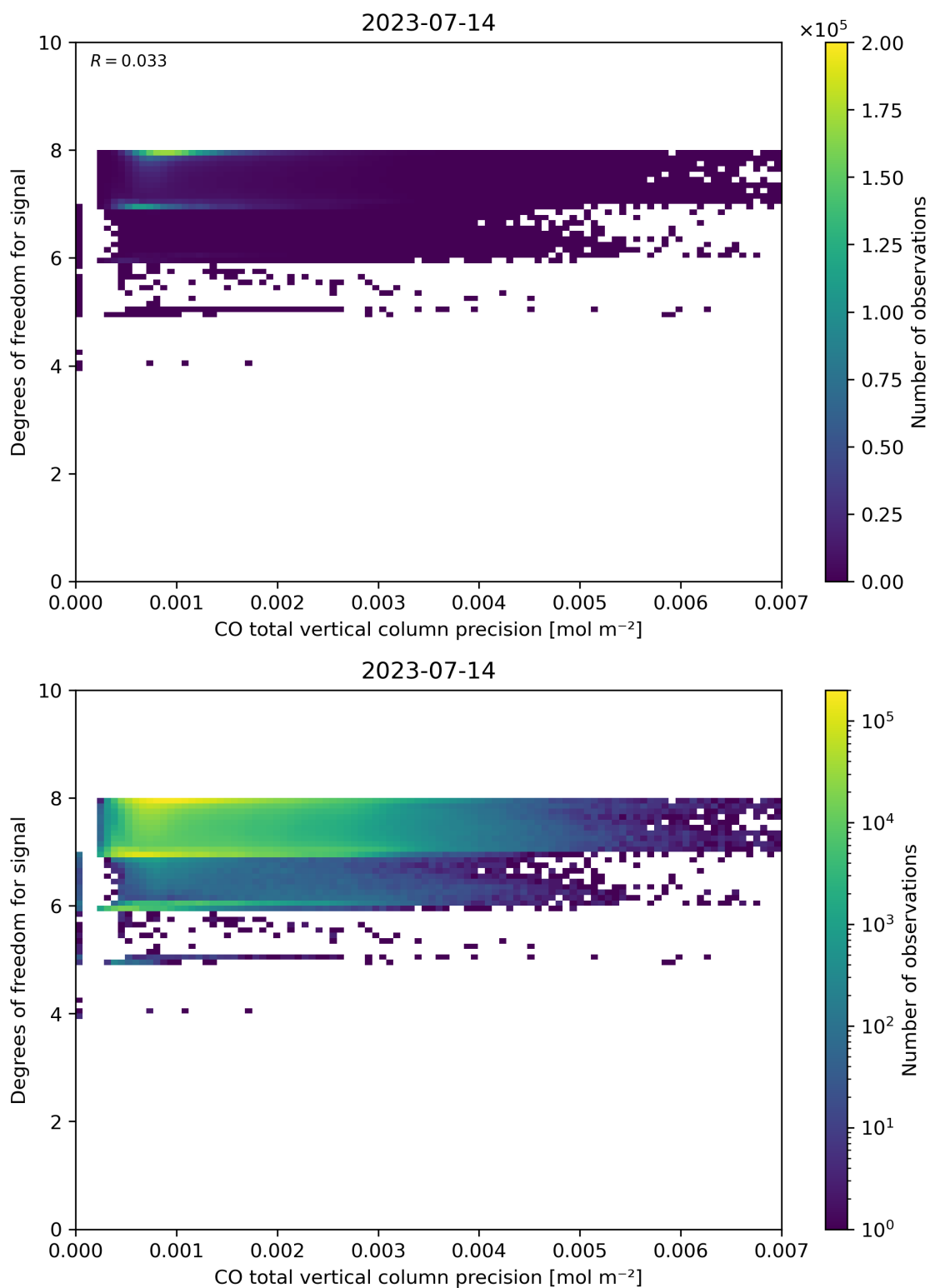
Figure 45: Scatter density plot of “CO total vertical column precision” against “Degrees of freedom for signal” for 2023-07-14 to 2023-07-15.
