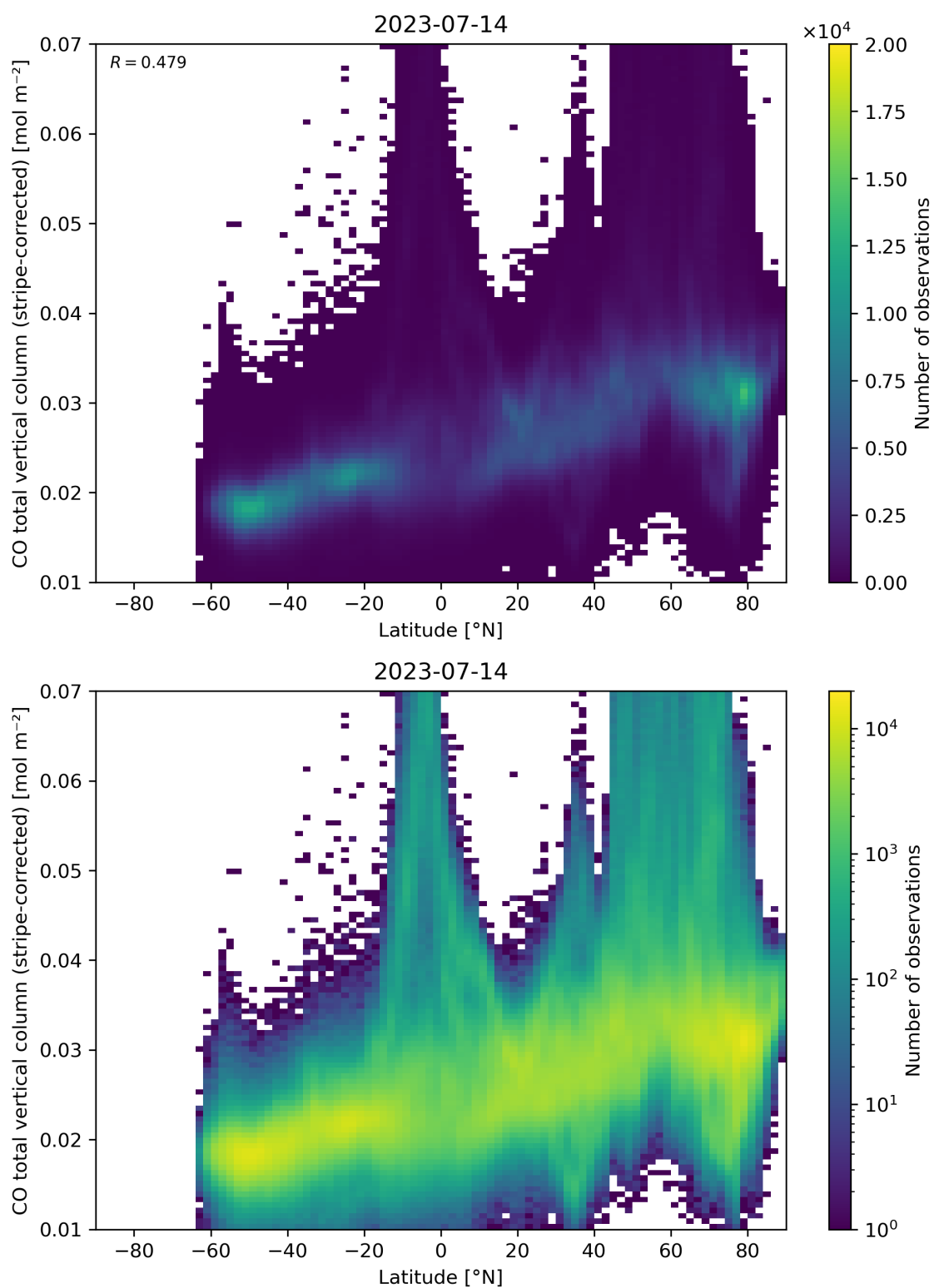
Figure 52: Scatter density plot of “Latitude” against “CO total vertical column (stripe-corrected)” for 2023-07-14 to 2023-07-15.
