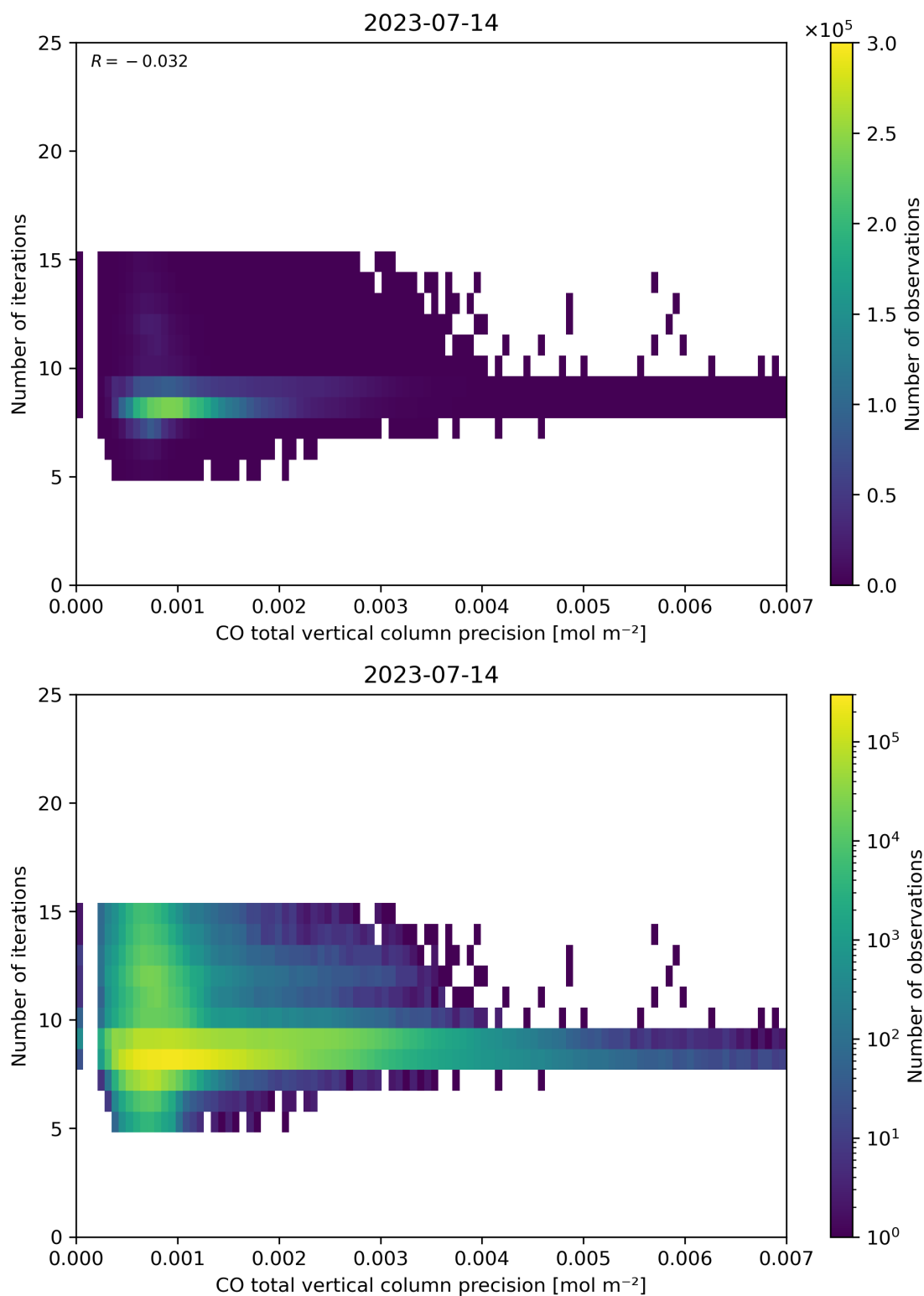
Figure 46: Scatter density plot of “CO total vertical column precision” against “Number of iterations” for 2023-07-14 to 2023-07-15.
