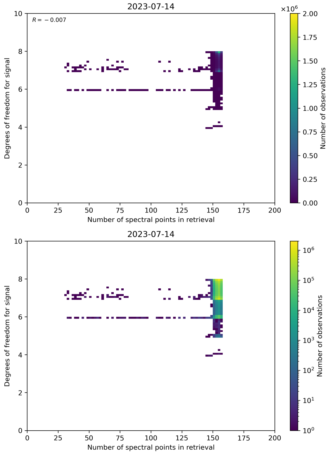
Figure 59: Scatter density plot of “Number of spectral points in retrieval” against “Degrees of freedom for signal” for 2023-07-14 to 2023-07-15.
