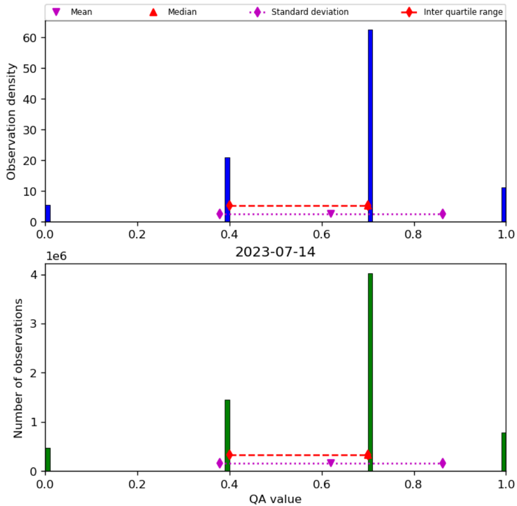
Figure 17: Histogram of “QA value” for 2023-07-14 to 2023-07-15
