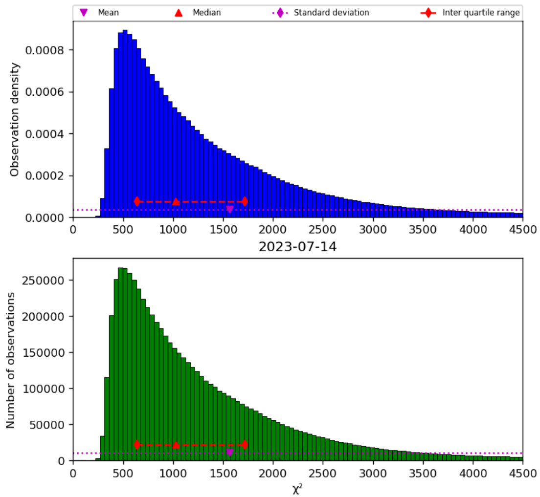
Figure 22: Histogram of " \chi^2 " for 2023-07-14 to 2023-07-15
