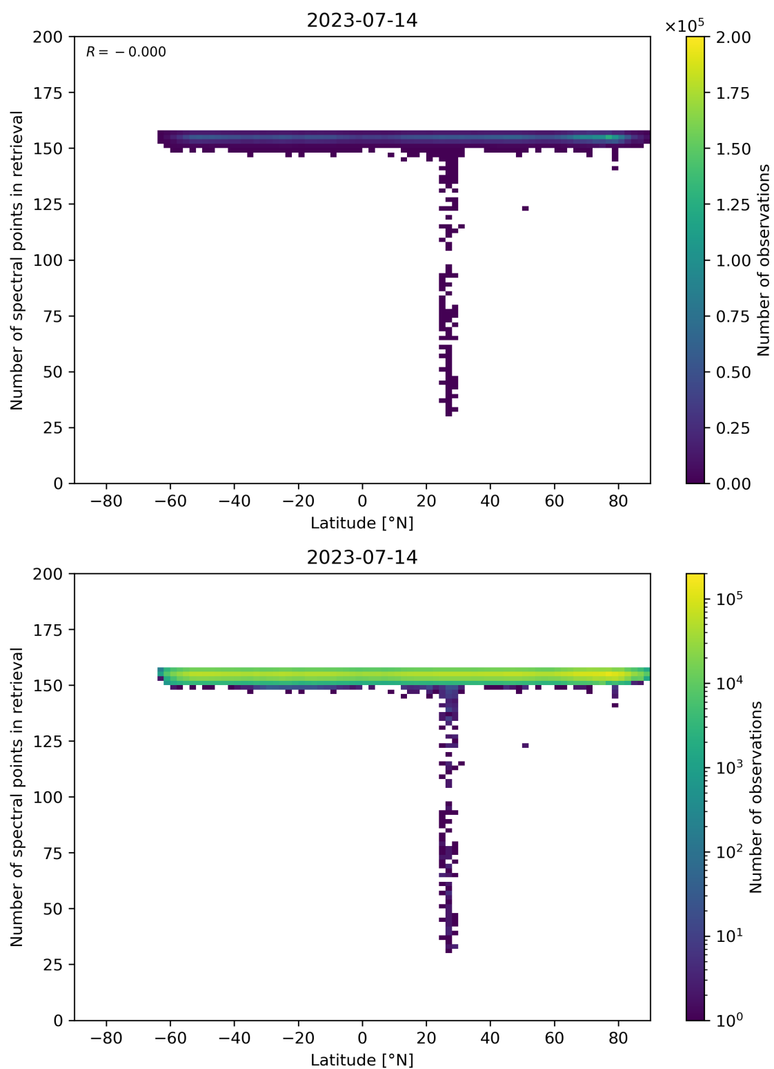
Figure 57: Scatter density plot of “Latitude” against “Number of spectral points in retrieval” for 2023-07-14 to 2023-07-15.
