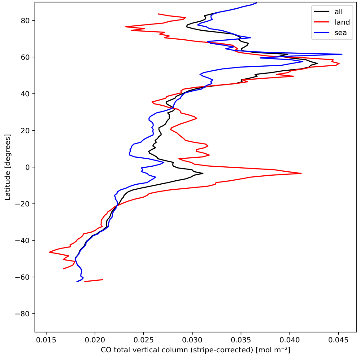
Figure 11: Zonal average of “CO total vertical column (stripe-corrected)” for 2023-07-14 to 2023-07-15.
