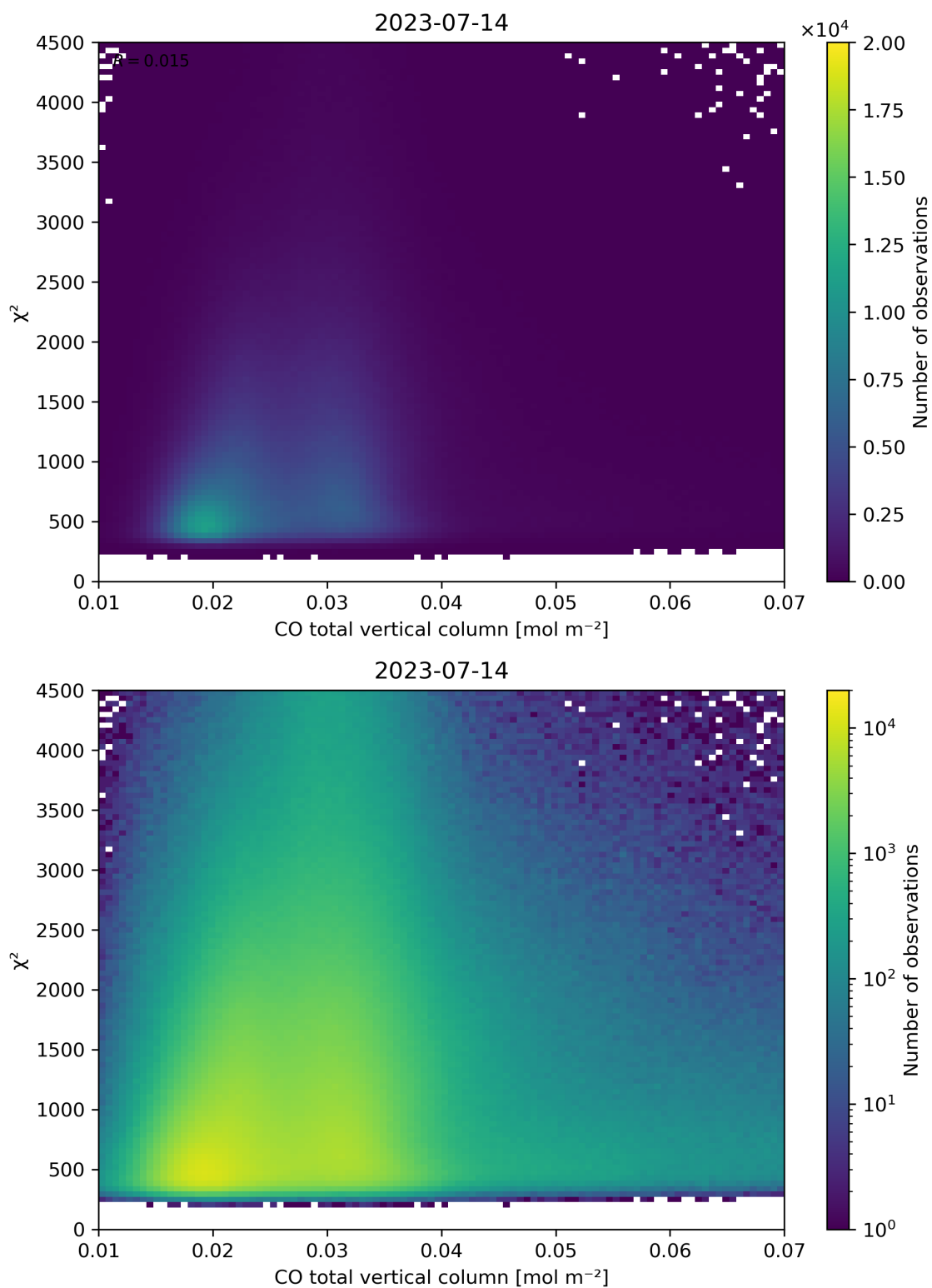
Figure 35: Scatter density plot of “CO total vertical column” against “ \chi^2 ” for 2023-07-14 to 2023-07-15.
