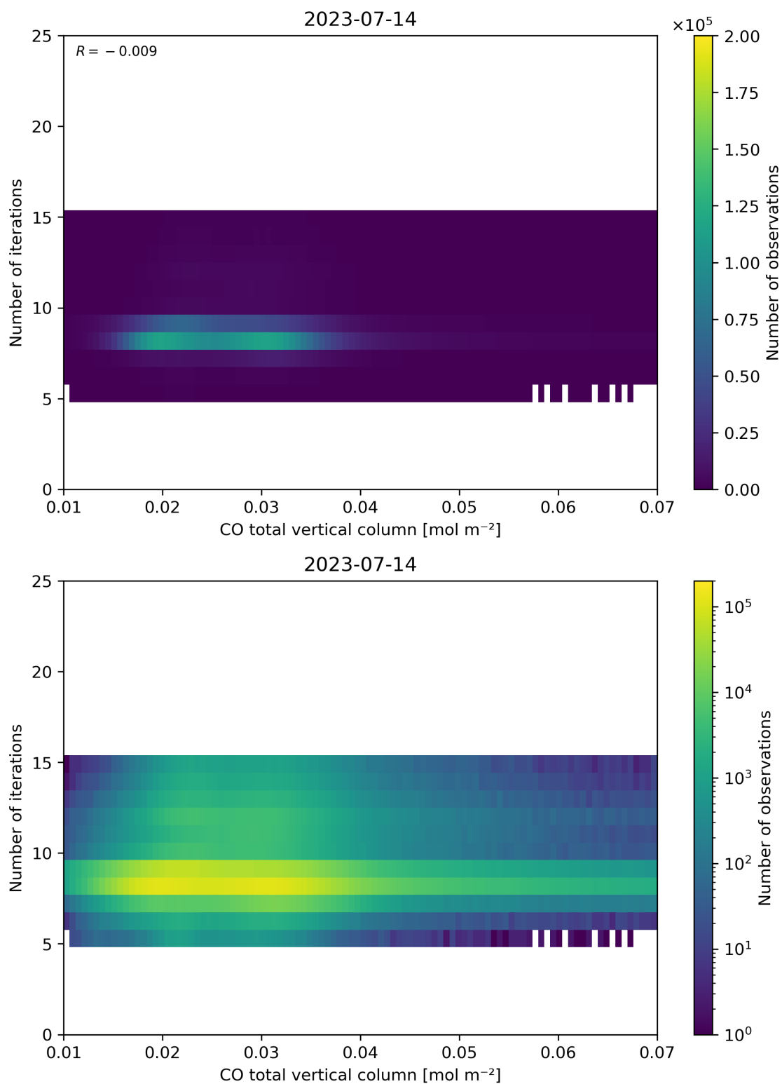
Figure 42: Scatter density plot of “CO total vertical column” against “Number of iterations” for 2023-07-14 to 2023-07-15.
