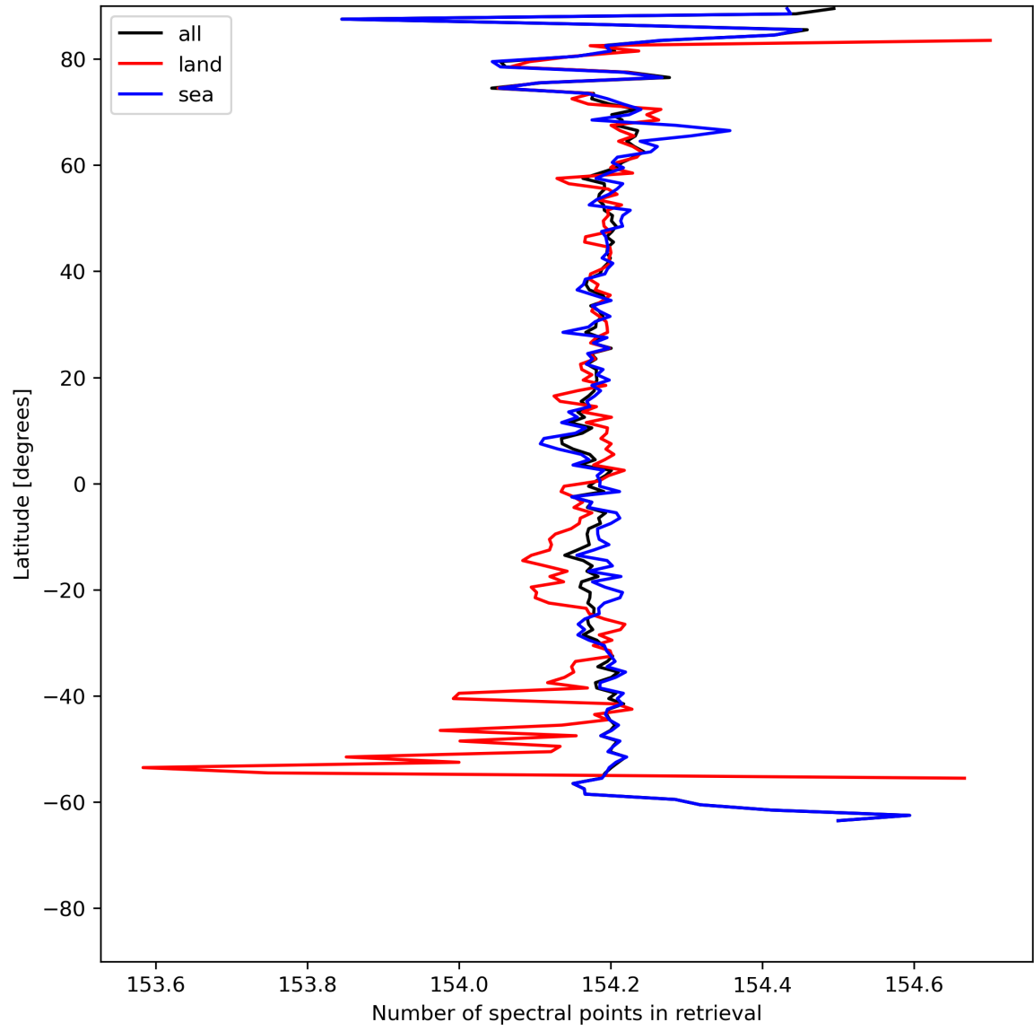
Figure 13: Zonal average of “Number of spectral points in retrieval” for 2023-07-15 to 2023-07-17.
