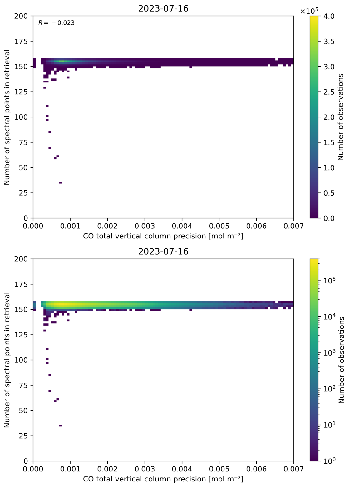
Figure 47: Scatter density plot of “CO total vertical column precision” against “Number of spectral points in retrieval” for 2023-07-15 to 2023-07-17.
