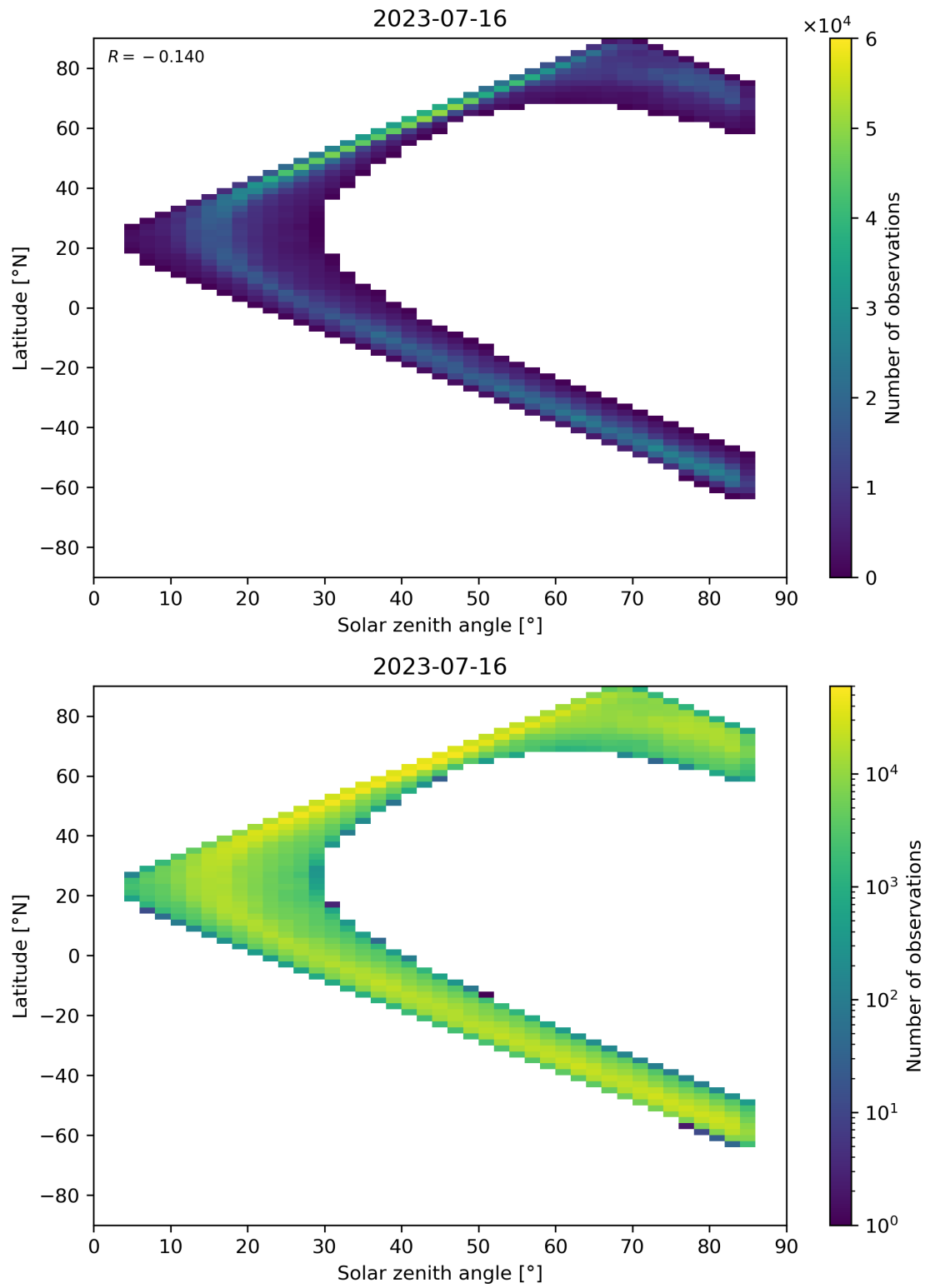
Figure 66: Scatter density plot of “Solar zenith angle” against “Latitude” for 2023-07-15 to 2023-07-17.
