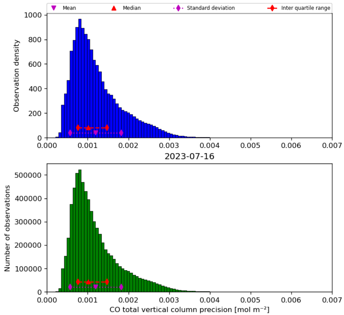
Figure 20: Histogram of “CO total vertical column precision” for 2023-07-15 to 2023-07-17
