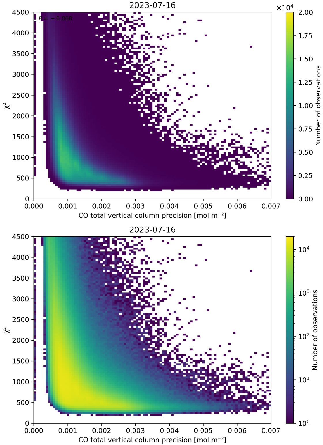
Figure 44: Scatter density plot of “CO total vertical column precision” against “ \chi^2 ” for 2023-07-15 to 2023-07-17.
