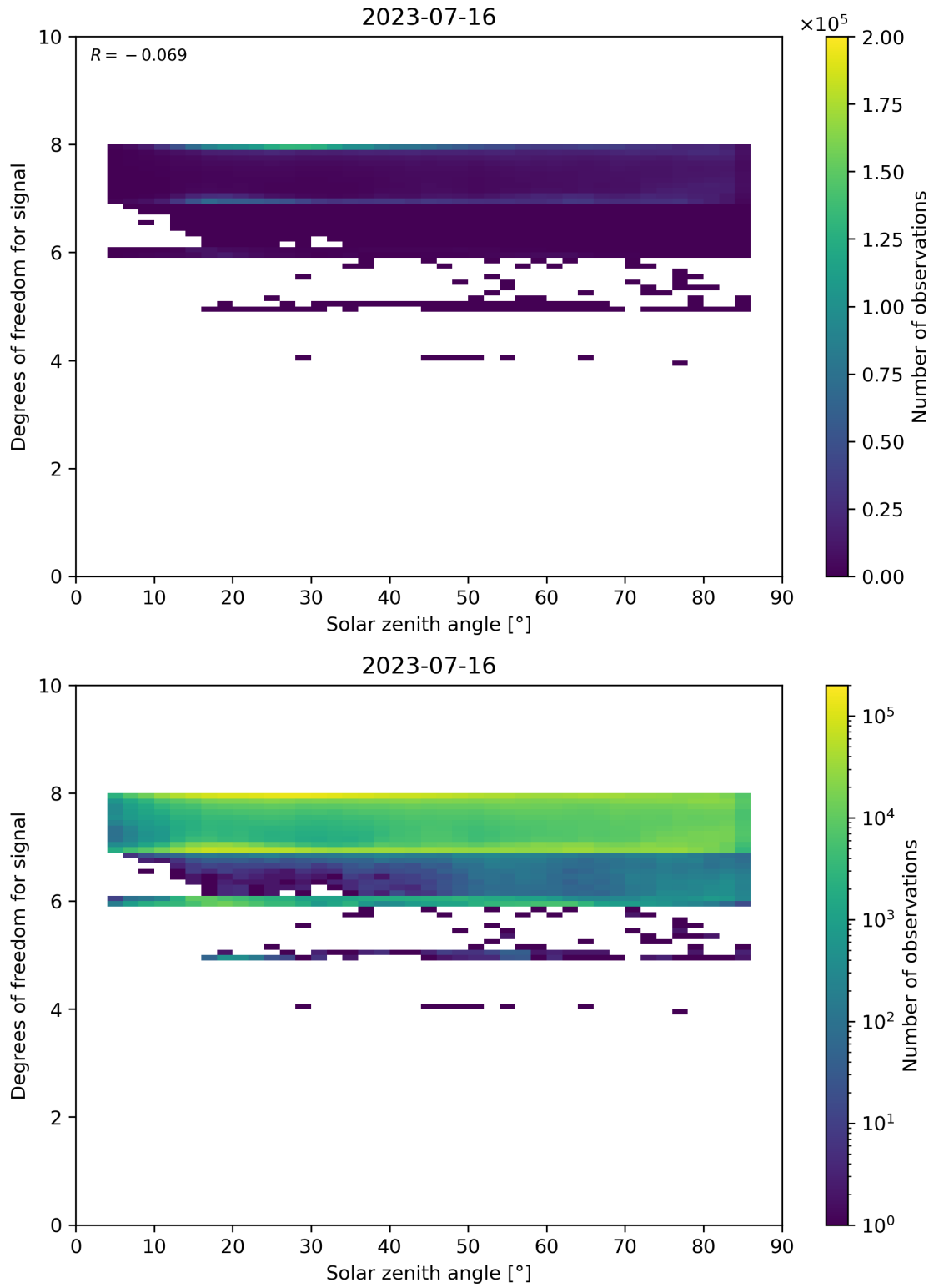
Figure 65: Scatter density plot of “Solar zenith angle” against “Degrees of freedom for signal” for 2023-07-15 to 2023-07-17.
