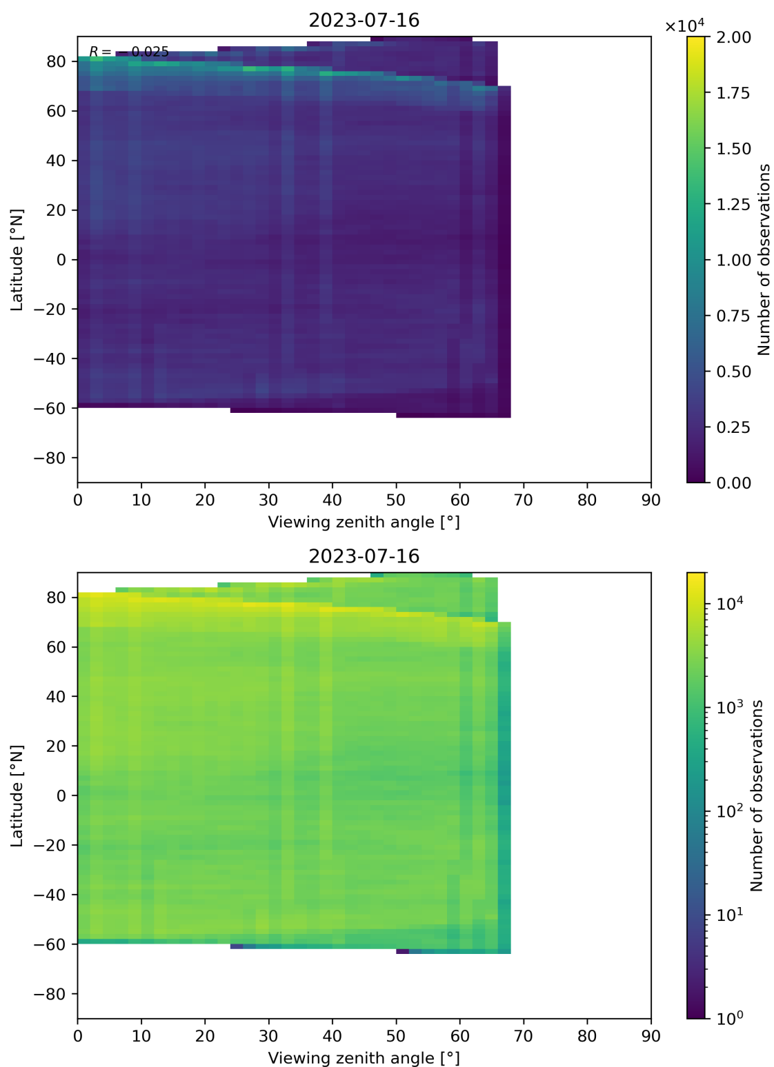
Figure 74: Scatter density plot of “Viewing zenith angle” against “Latitude” for 2023-07-15 to 2023-07-17.
