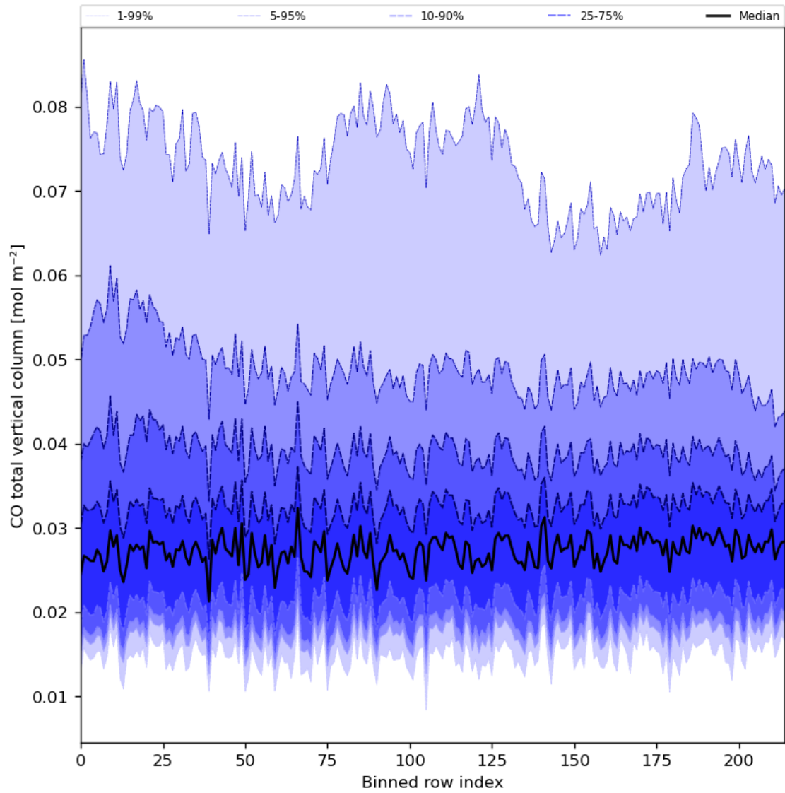
Figure 26: Along track statistics of “CO total vertical column” for 2023-07-15 to 2023-07-17
