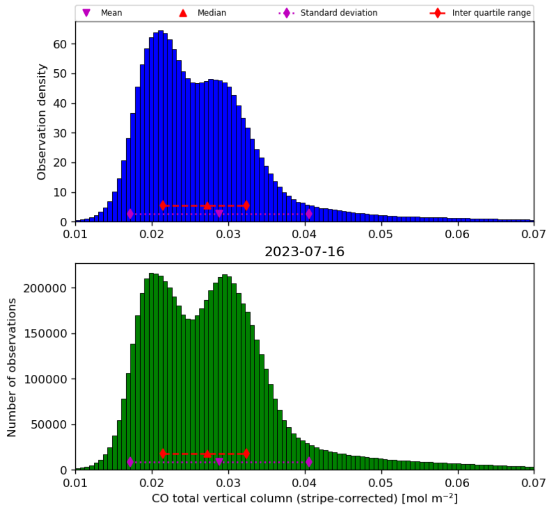
Figure 19: Histogram of “CO total vertical column (stripe-corrected)” for 2023-07-15 to 2023-07-17
