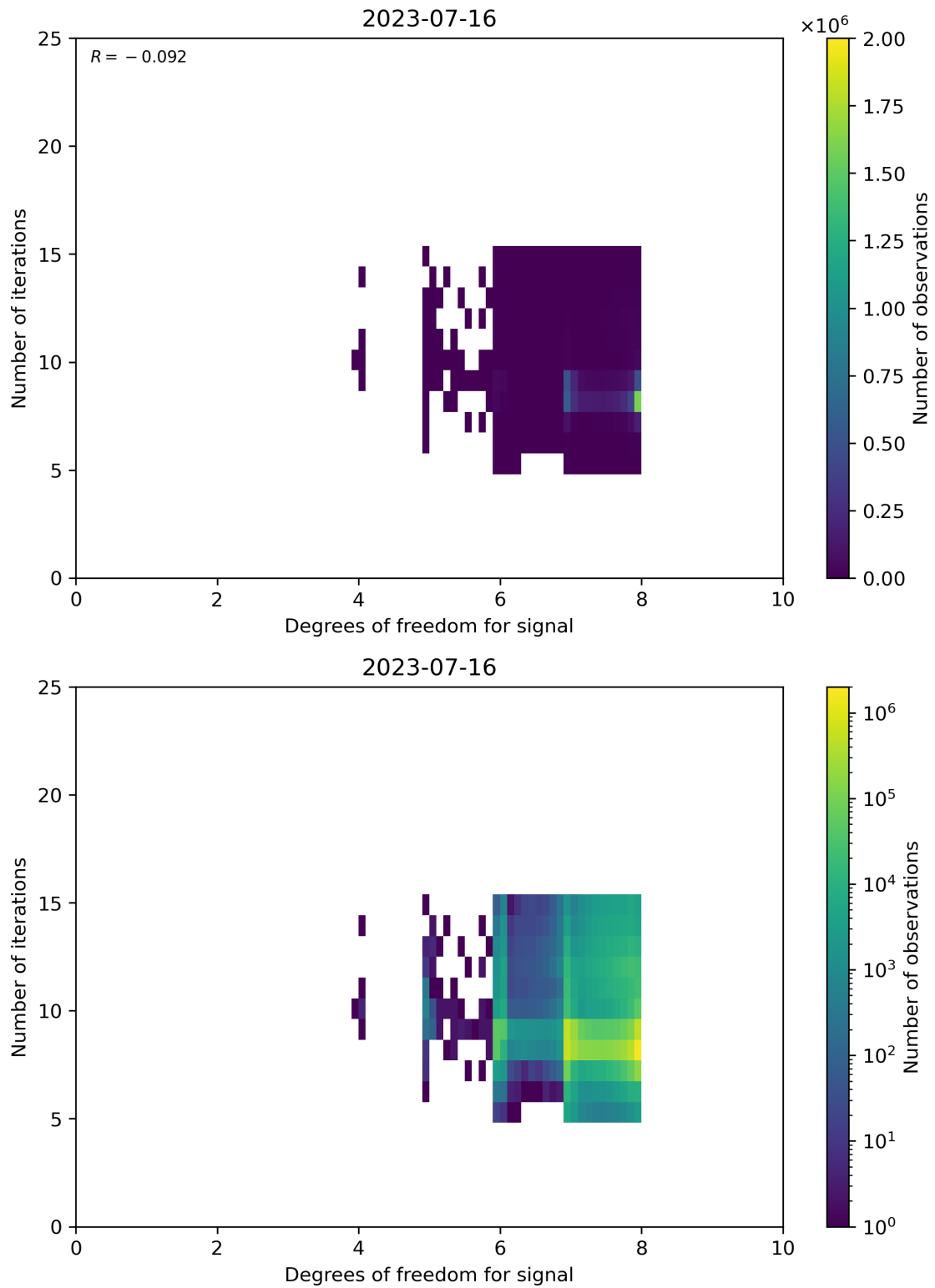
Figure 50: Scatter density plot of “Degrees of freedom for signal” against “Number of iterations” for 2023-07-15 to 2023-07-17.
