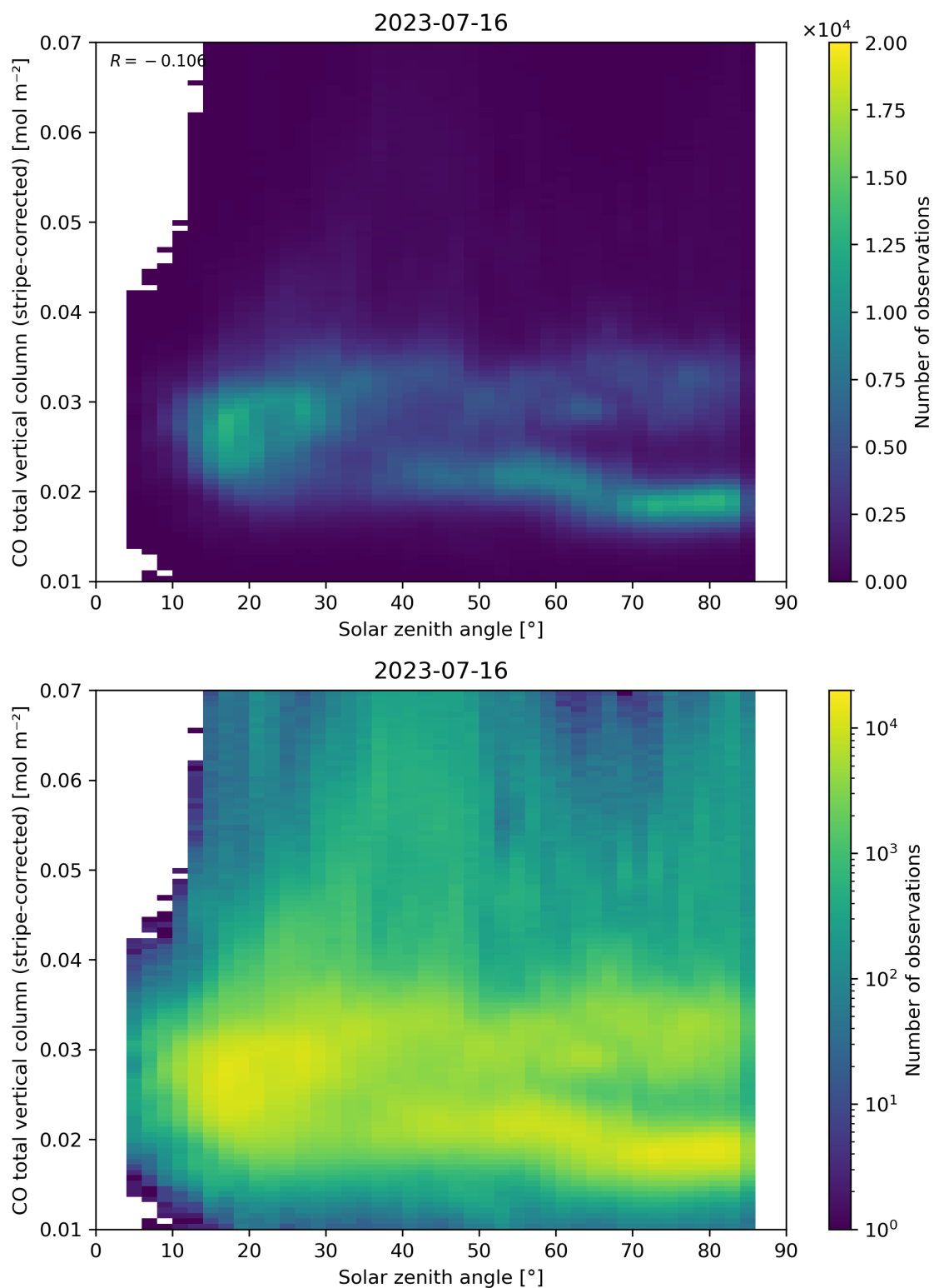
Figure 62: Scatter density plot of “Solar zenith angle” against “CO total vertical column (stripe-corrected)” for 2023-07-15 to 2023-07-17.
