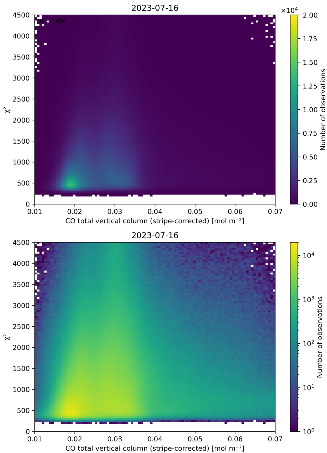
Figure 37: Scatter density plot of “CO total vertical column (stripe-corrected)” against “ \chi^2 ” for 2023-07-15 to 2023-07-17.
