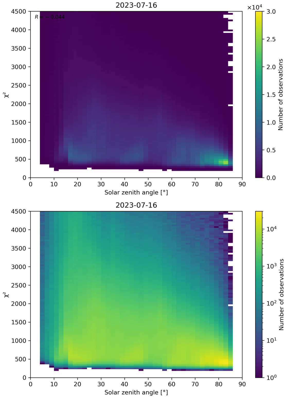
Figure 64: Scatter density plot of “Solar zenith angle” against “ \chi^2 ” for 2023-07-15 to 2023-07-17.
