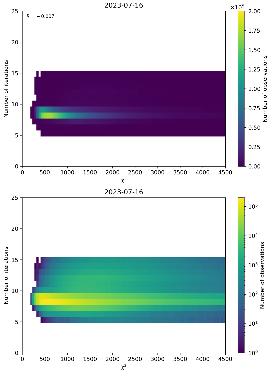
Figure 49: Scatter density plot of “ \chi^2 ” against “Number of iterations” for 2023-07-15 to 2023-07-17.
