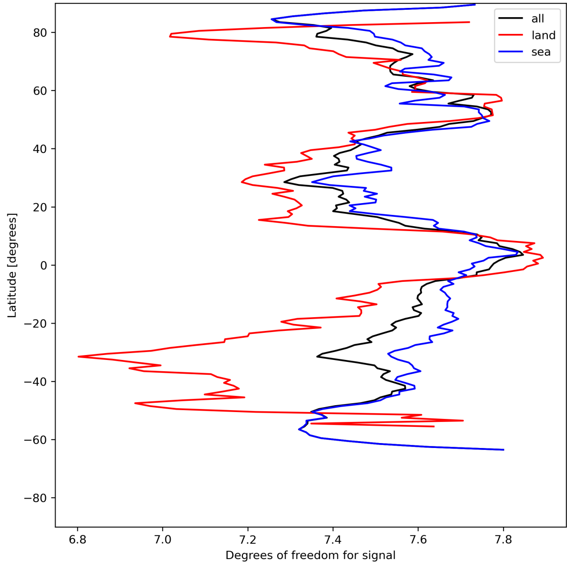
Figure 15: Zonal average of “Degrees of freedom for signal” for 2023-07-15 to 2023-07-17.
