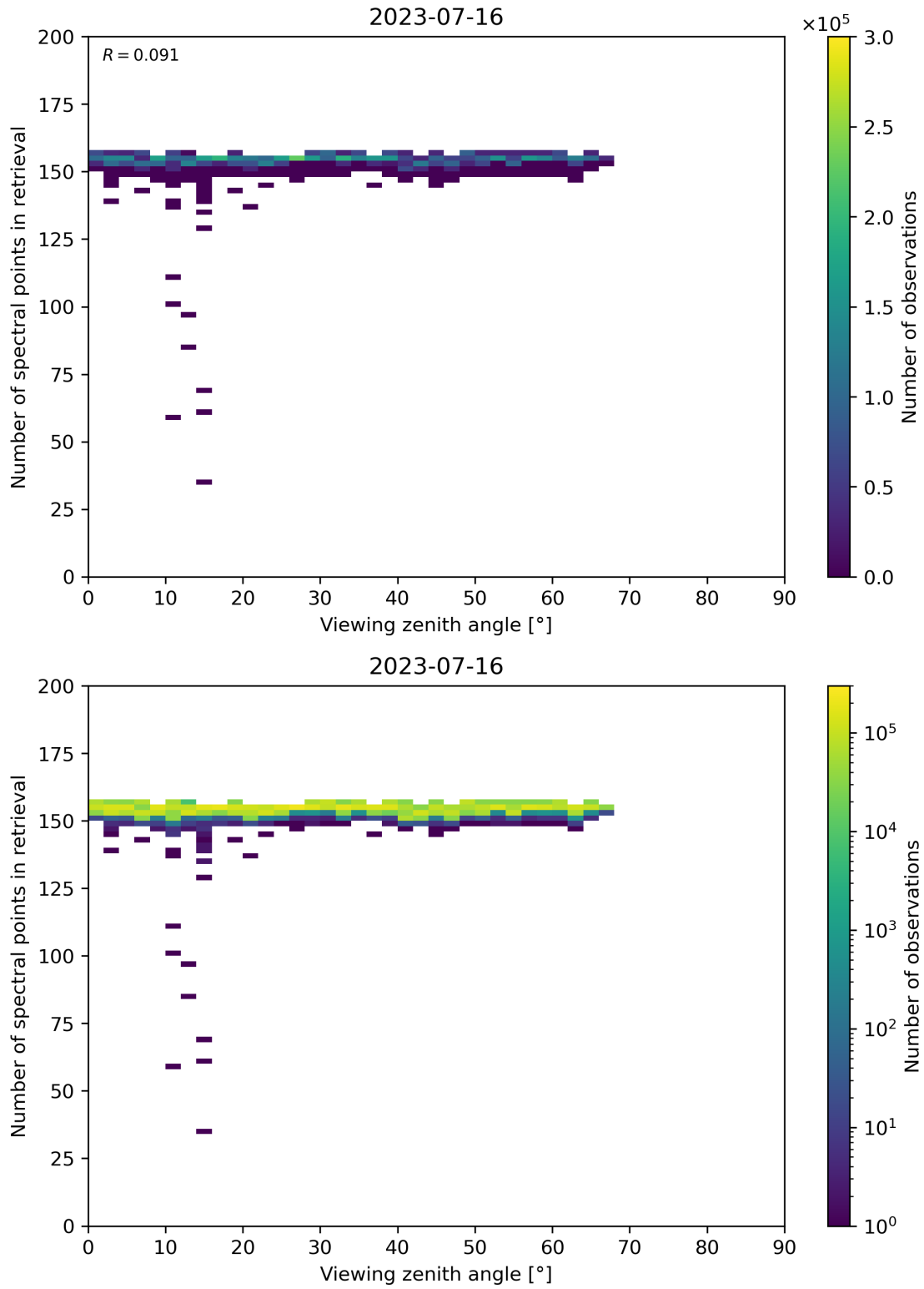
Figure 76: Scatter density plot of “Viewing zenith angle” against “Number of spectral points in retrieval” for 2023-07-15 to 2023-07-17.
