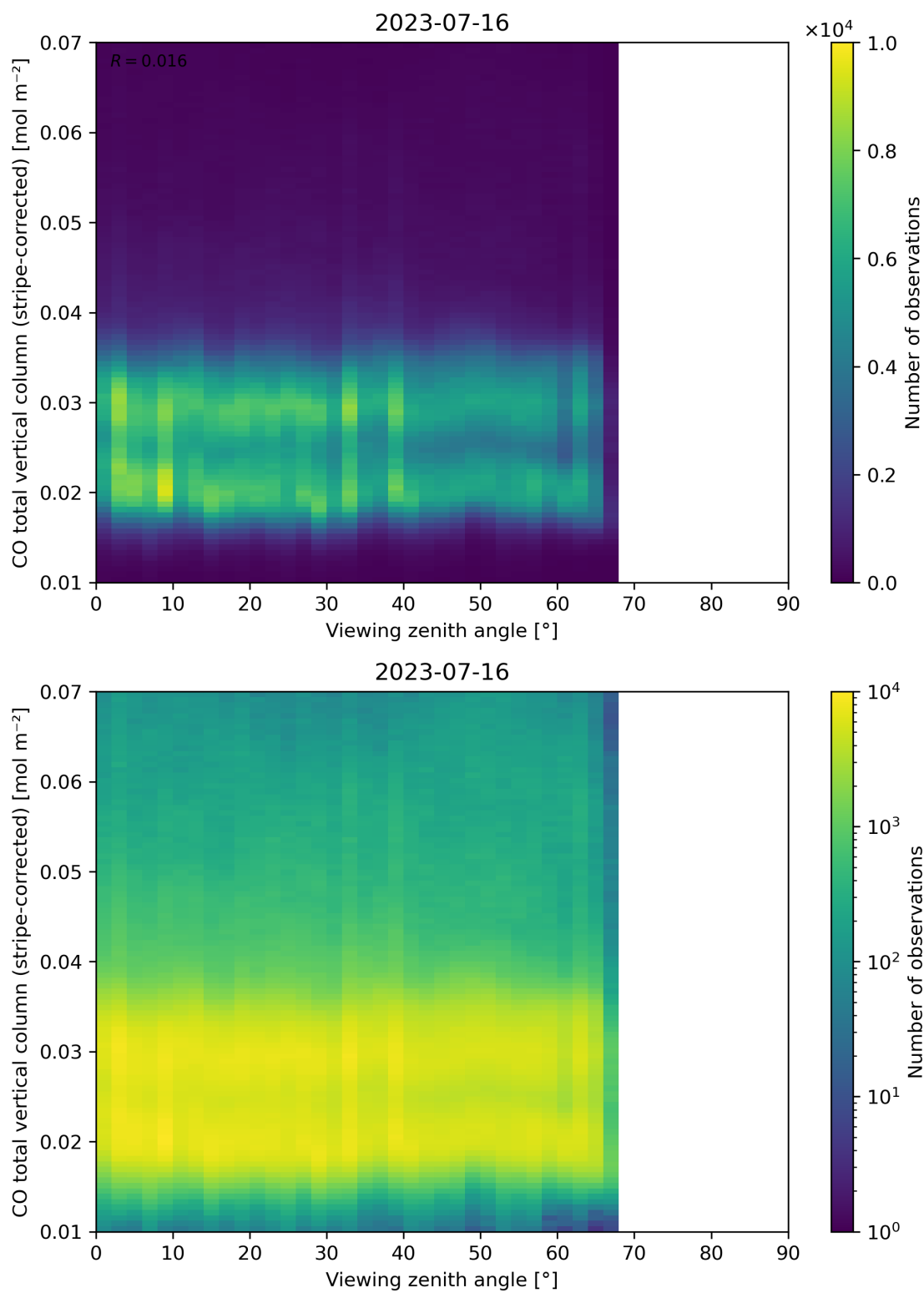
Figure 70: Scatter density plot of “Viewing zenith angle” against “CO total vertical column (stripe-corrected)” for 2023-07-15 to 2023-07-17.
