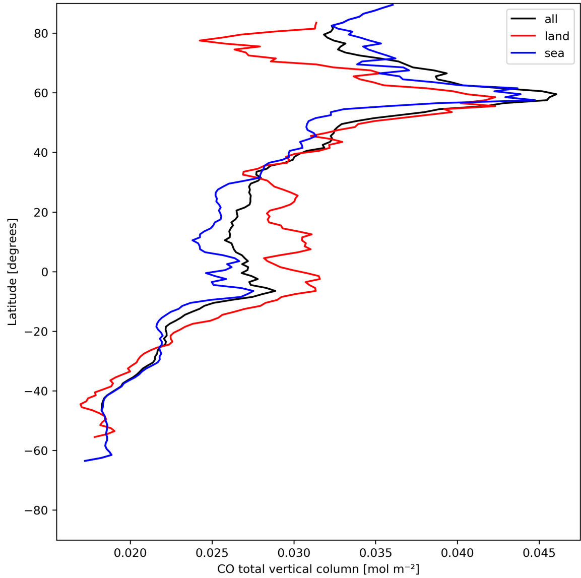
Figure 10: Zonal average of “CO total vertical column” for 2023-07-15 to 2023-07-17.
