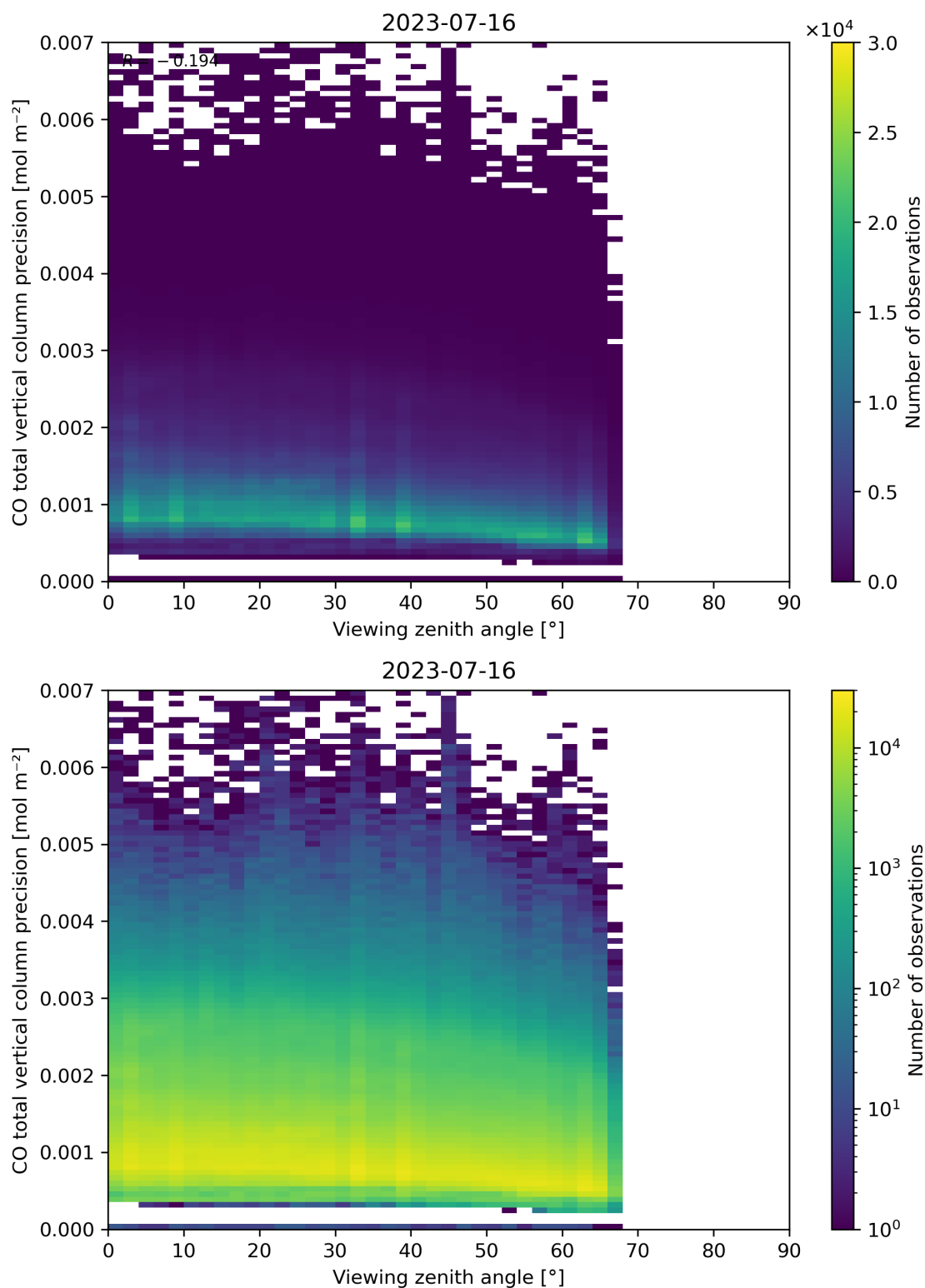
Figure 71: Scatter density plot of “Viewing zenith angle” against “CO total vertical column precision” for 2023-07-15 to 2023-07-17.
