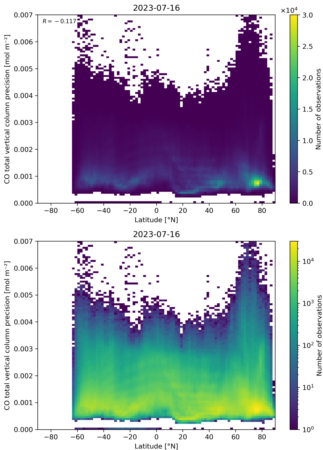
Figure 53: Scatter density plot of “Latitude” against “CO total vertical column precision” for 2023-07-15 to 2023-07-17.
