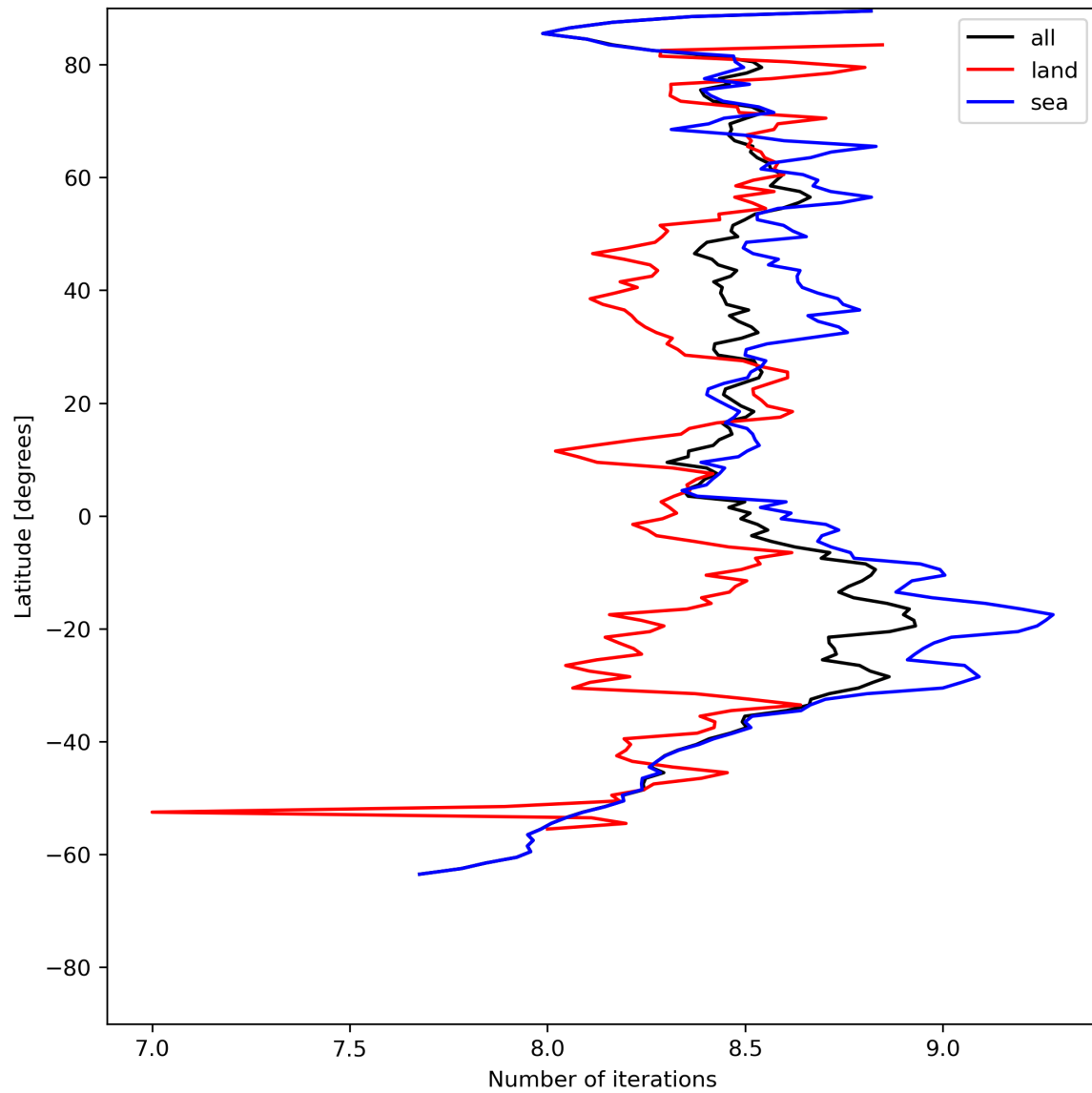
Figure 16: Zonal average of “Number of iterations” for 2023-07-15 to 2023-07-17.
