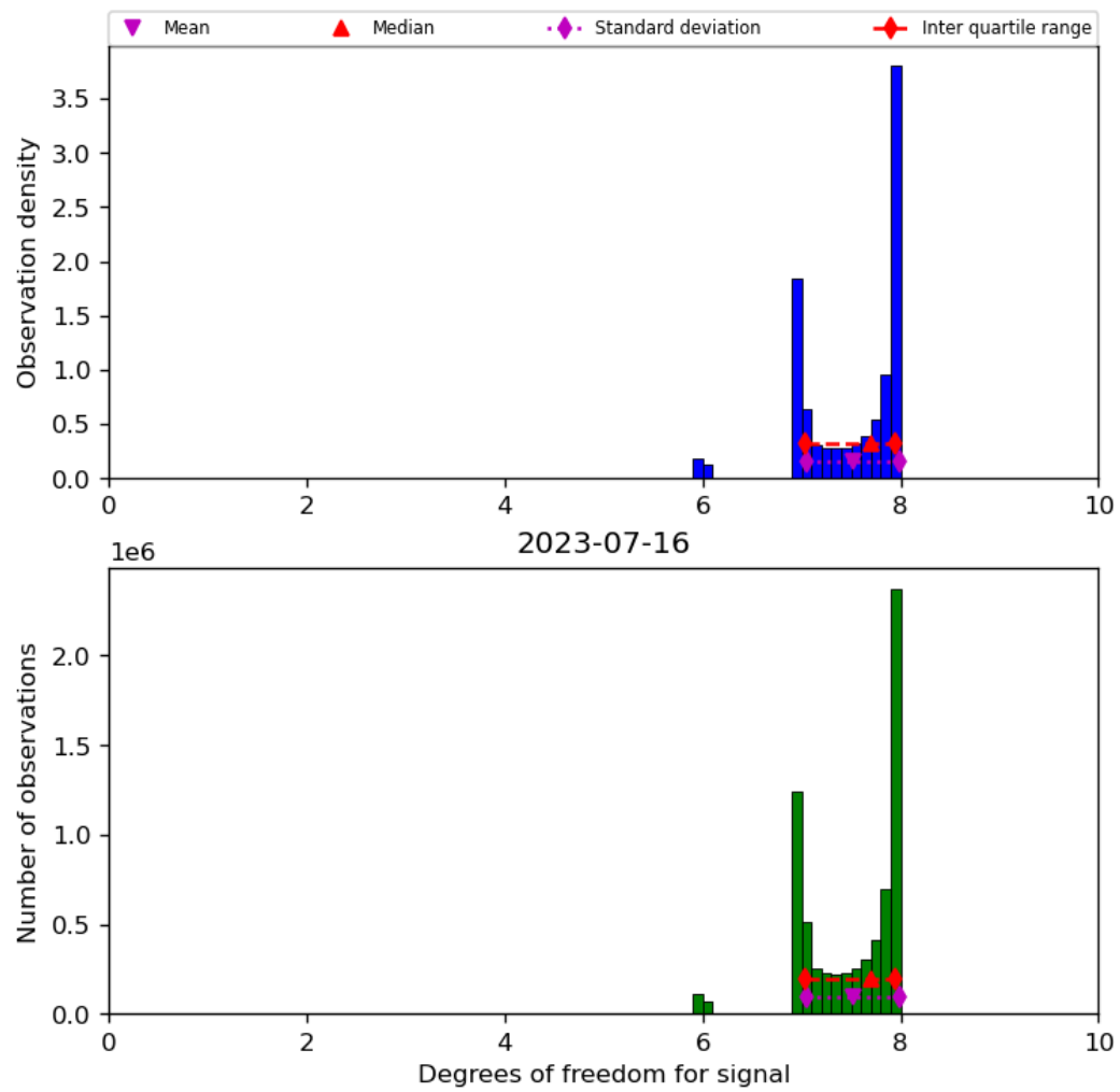
Figure 23: Histogram of “Degrees of freedom for signal” for 2023-07-15 to 2023-07-17
