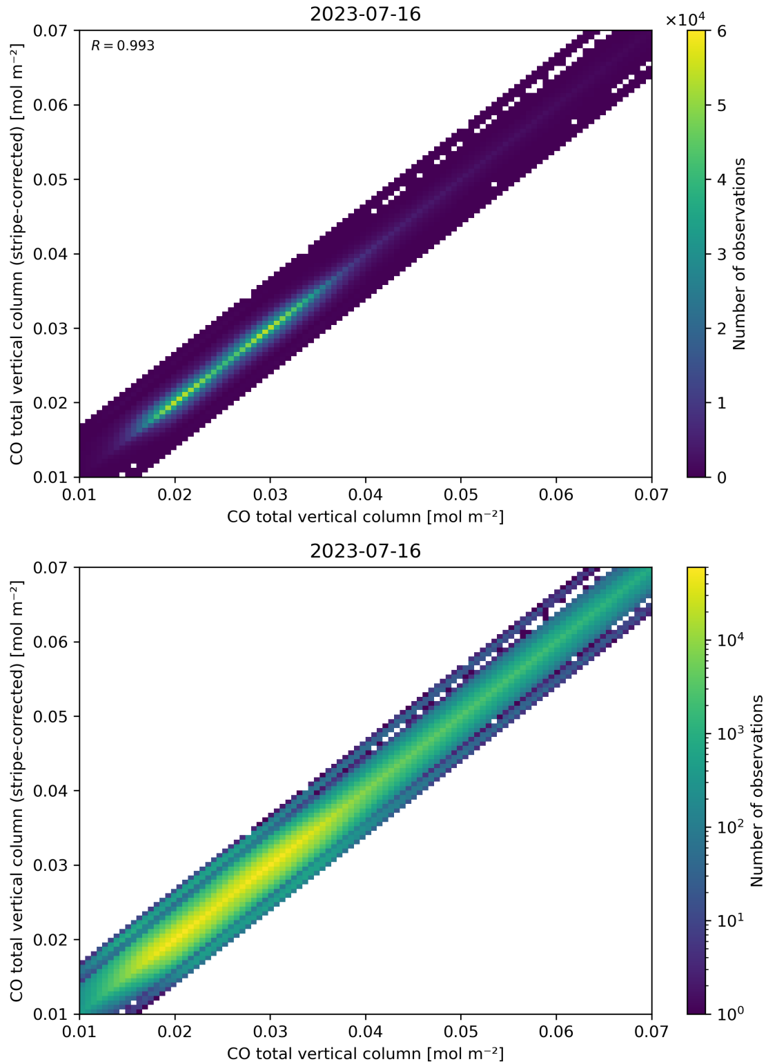
Figure 33: Scatter density plot of “CO total vertical column” against “CO total vertical column (stripe-corrected)” for 2023-07-15 to 2023-07-17.
