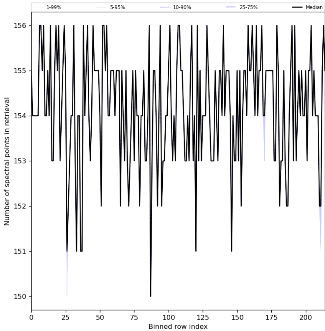
Figure 29: Along track statistics of “Number of spectral points in retrieval” for 2023-07-15 to 2023-07-17
