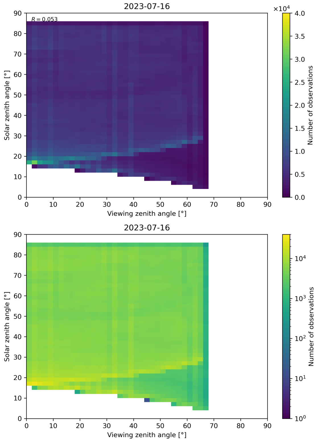
Figure 77: Scatter density plot of “Viewing zenith angle” against “Solar zenith angle” for 2023-07-15 to 2023-07-17.
