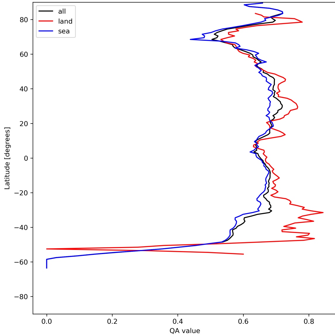
Figure 9: Zonal average of “QA value” for 2023-07-15 to 2023-07-17.
