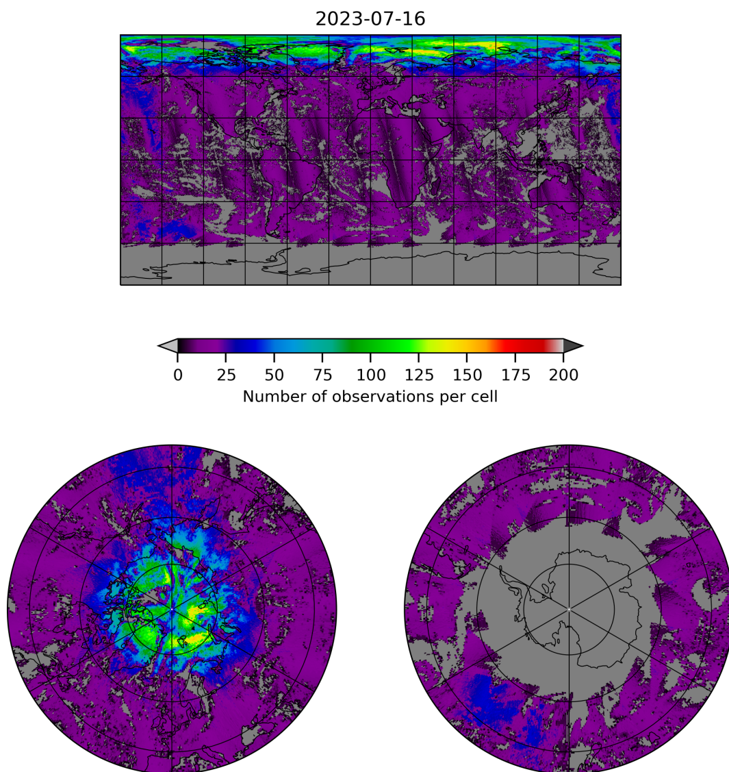
Figure 8: Map of the number of observations for 2023-07-15 to 2023-07-17
