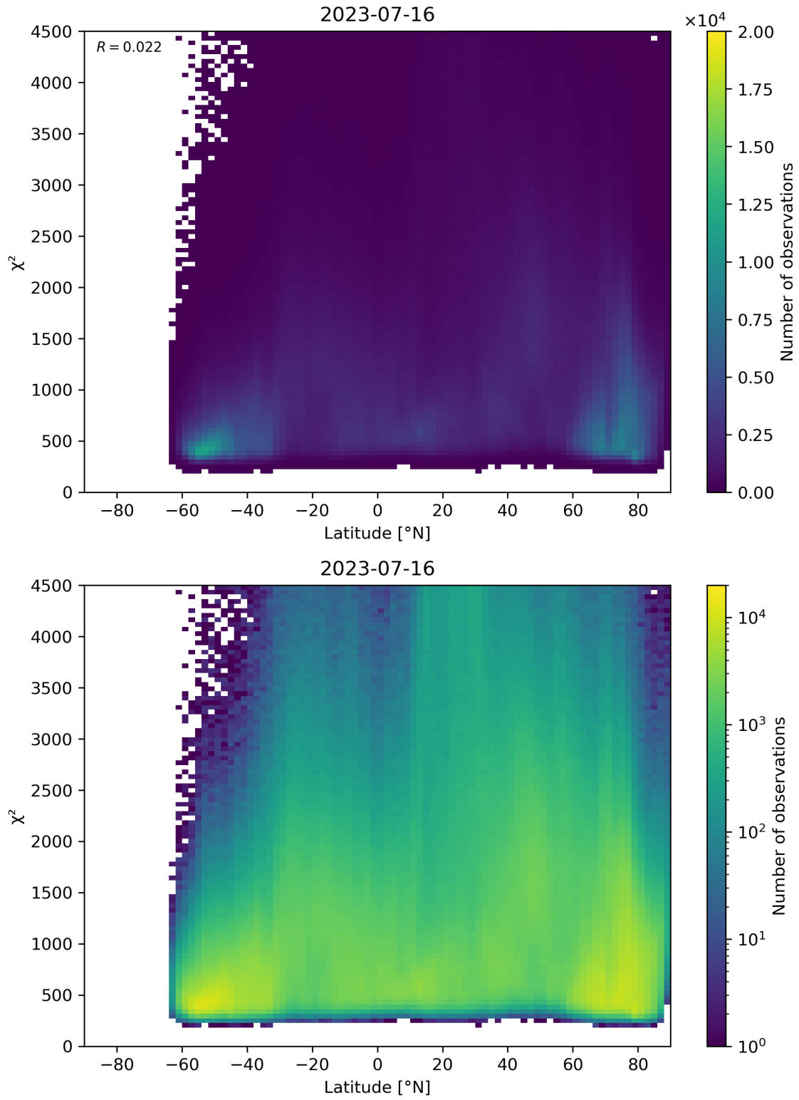
Figure 54: Scatter density plot of “Latitude” against “ \chi^2 ” for 2023-07-15 to 2023-07-17.
