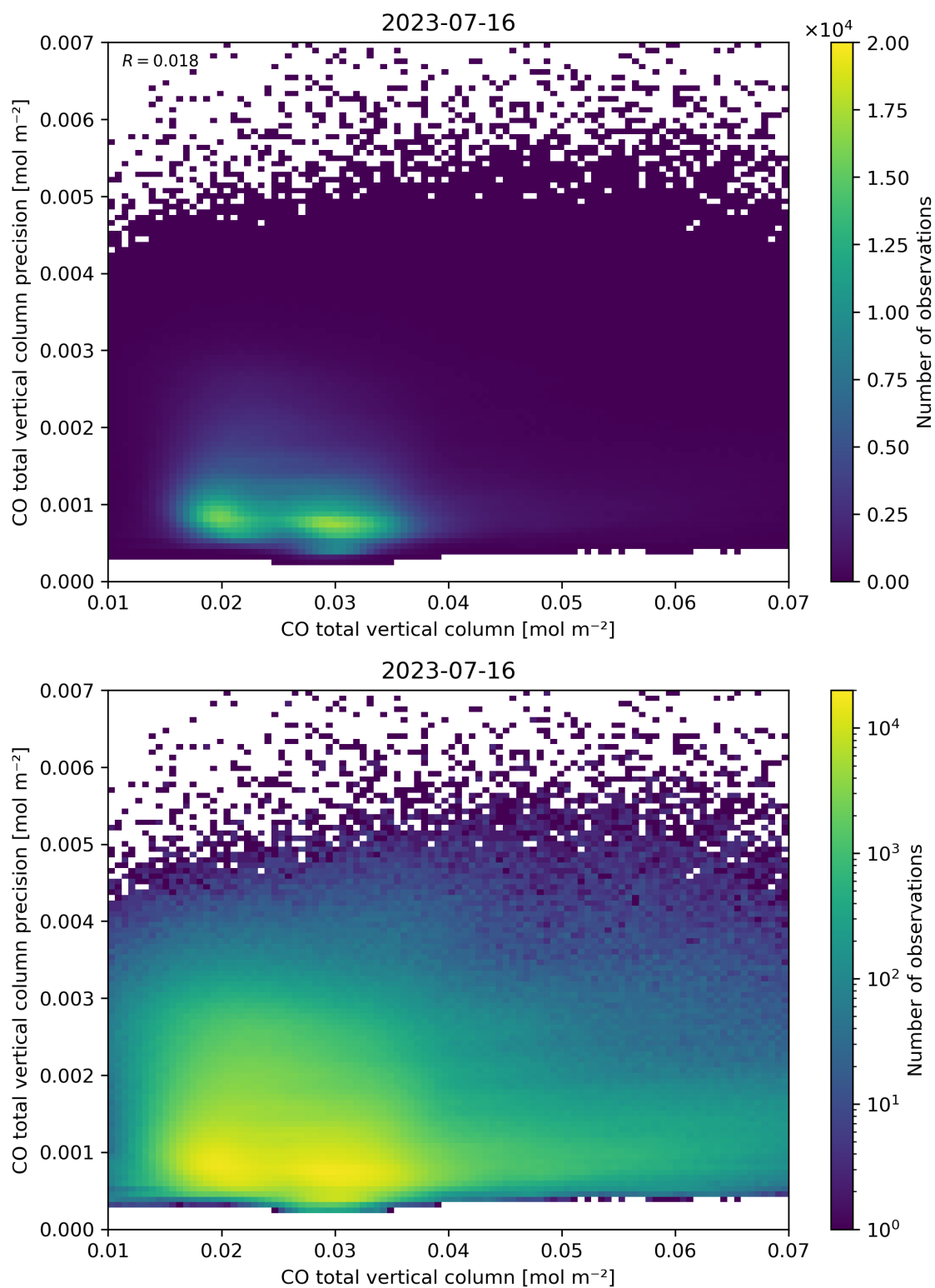
Figure 34: Scatter density plot of “CO total vertical column” against “CO total vertical column precision” for 2023-07-15 to 2023-07-17.
