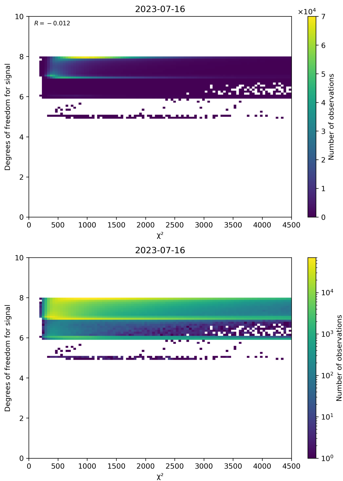
Figure 48: Scatter density plot of “ \chi^2 ” against “Degrees of freedom for signal” for 2023-07-15 to 2023-07-17.
