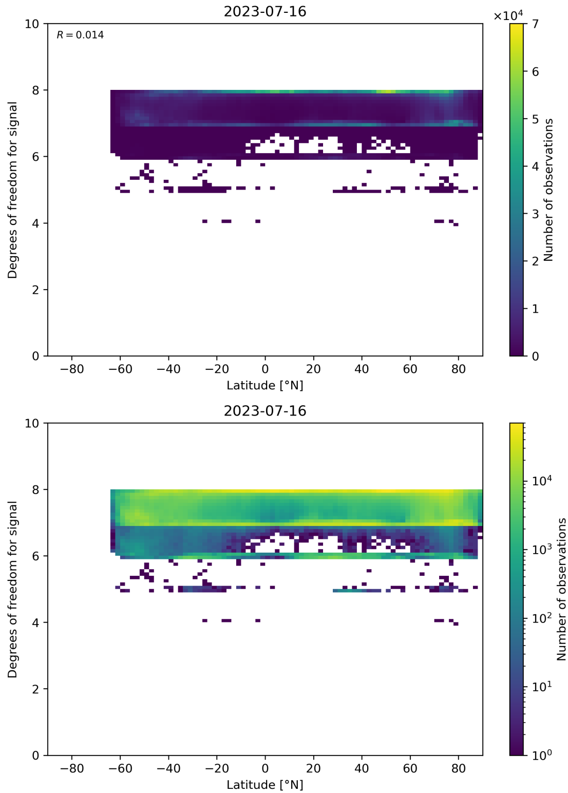
Figure 55: Scatter density plot of “Latitude” against “Degrees of freedom for signal” for 2023-07-15 to 2023-07-17.
