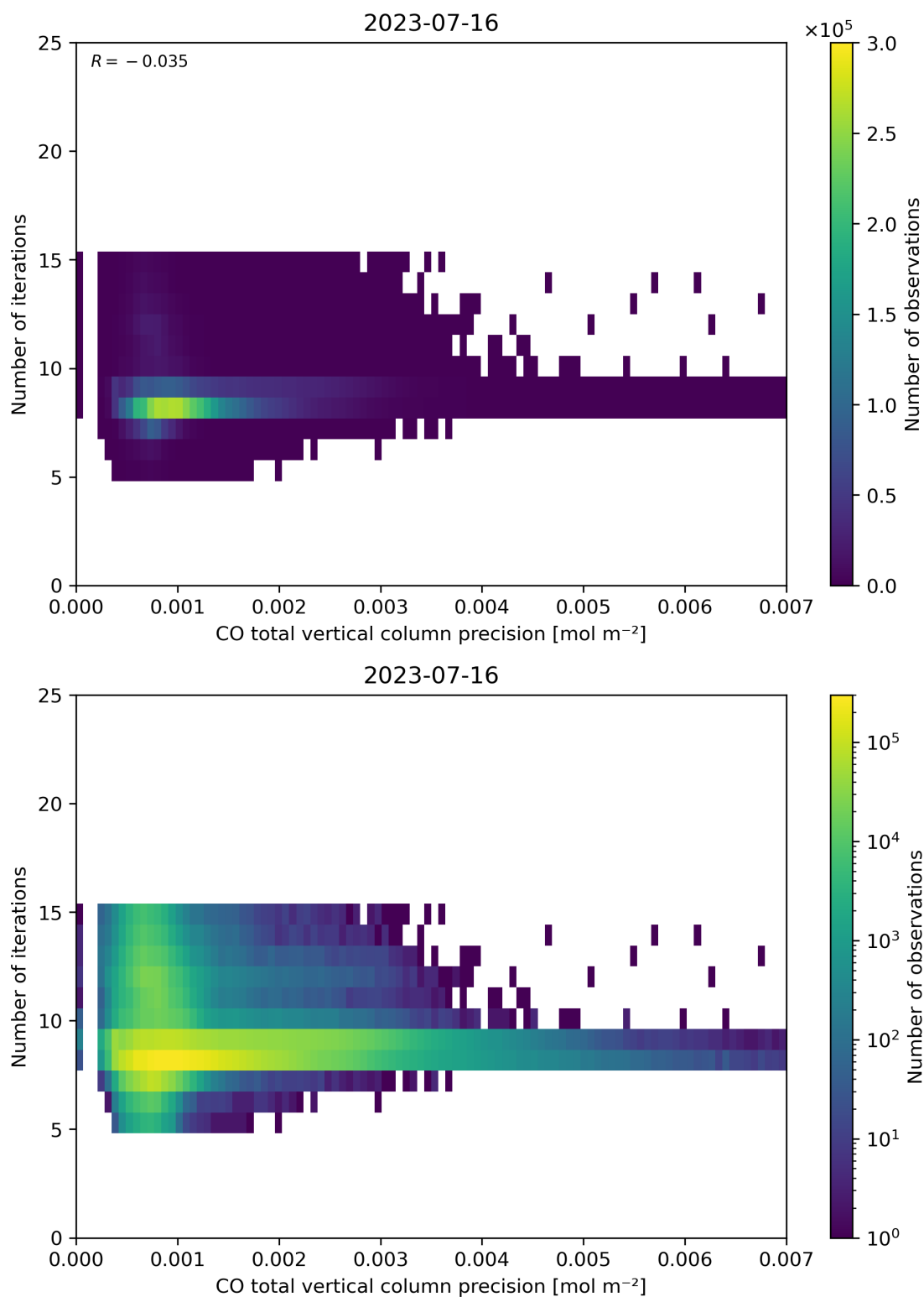
Figure 46: Scatter density plot of “CO total vertical column precision” against “Number of iterations” for 2023-07-15 to 2023-07-17.
