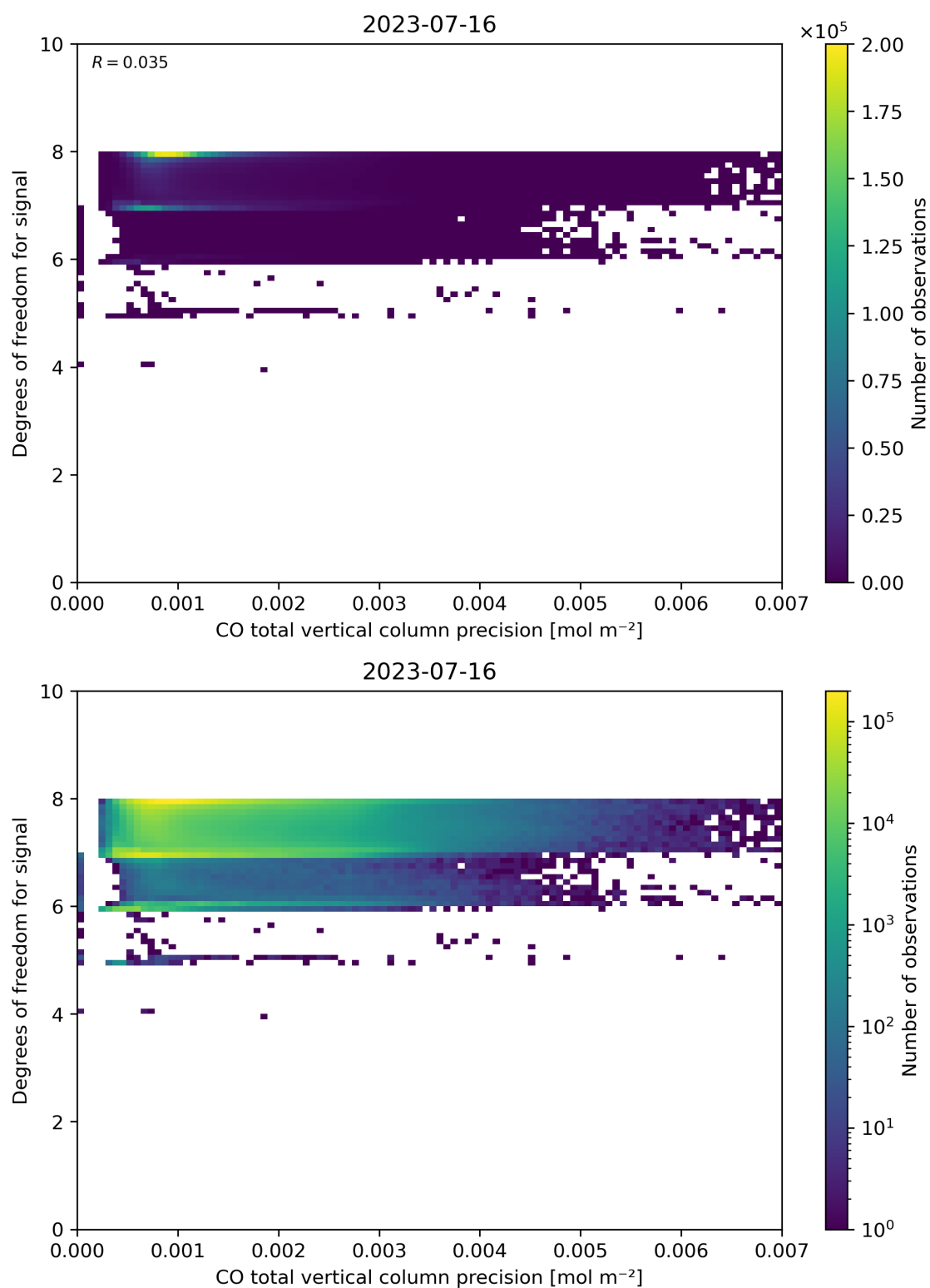
Figure 45: Scatter density plot of “CO total vertical column precision” against “Degrees of freedom for signal” for 2023-07-15 to 2023-07-17.
