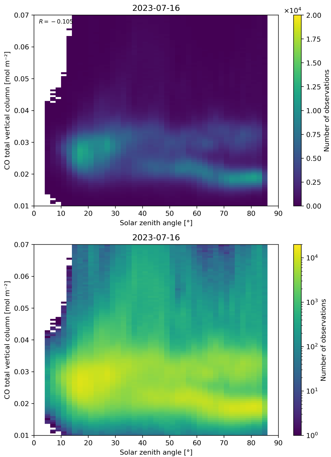
Figure 61: Scatter density plot of “Solar zenith angle” against “CO total vertical column” for 2023-07-15 to 2023-07-17.
