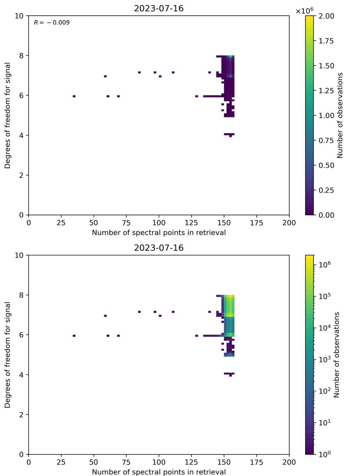
Figure 59: Scatter density plot of “Number of spectral points in retrieval” against “Degrees of freedom for signal” for 2023-07-15 to 2023-07-17.
