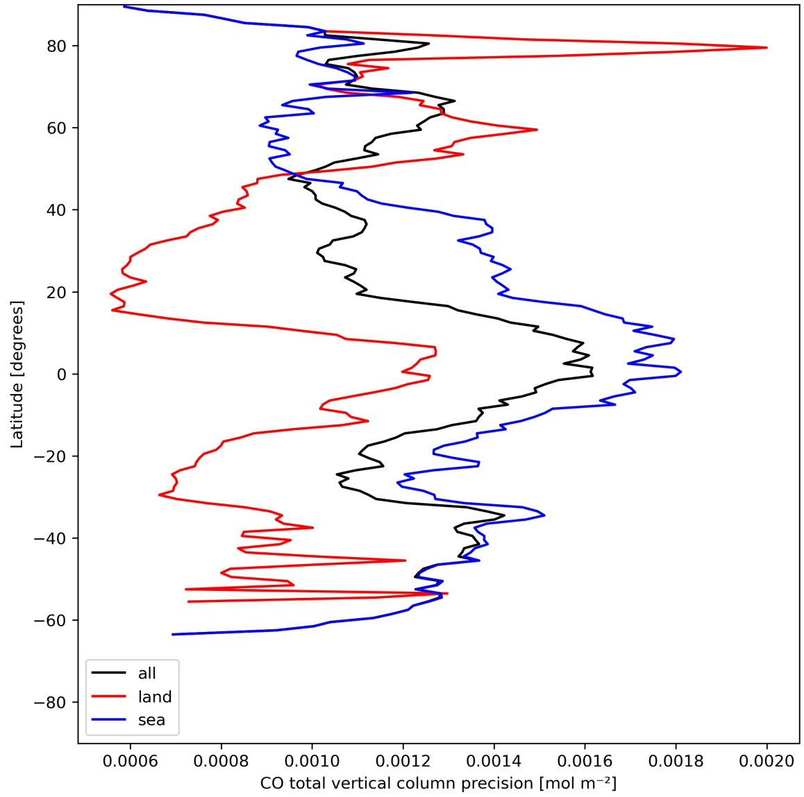
Figure 12: Zonal average of “CO total vertical column precision” for 2023-07-15 to 2023-07-17.
