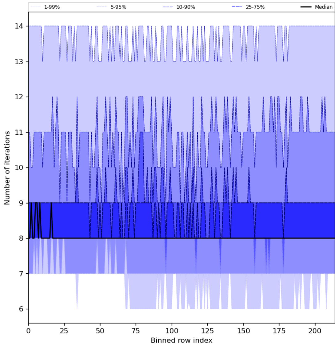
Figure 32: Along track statistics of “Number of iterations” for 2023-07-15 to 2023-07-17
