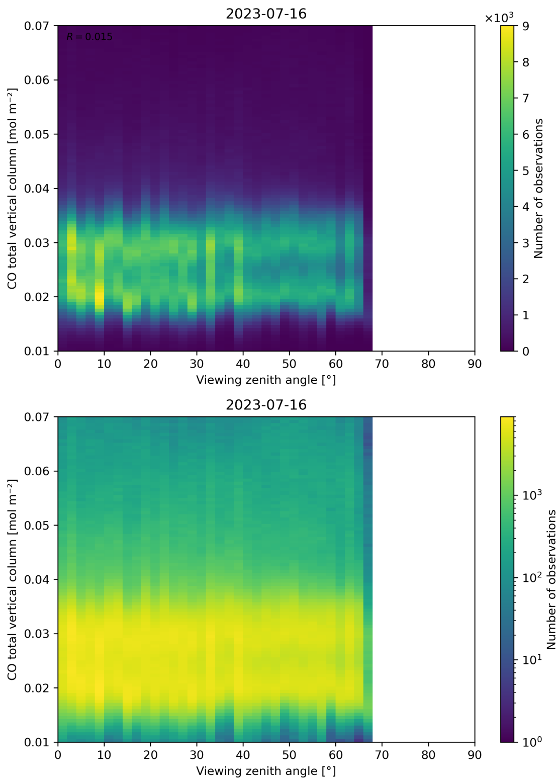
Figure 69: Scatter density plot of “Viewing zenith angle” against “CO total vertical column” for 2023-07-15 to 2023-07-17.
