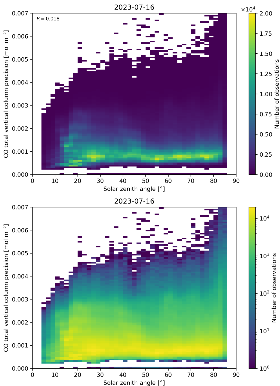
Figure 63: Scatter density plot of “Solar zenith angle” against “CO total vertical column precision” for 2023-07-15 to 2023-07-17.
