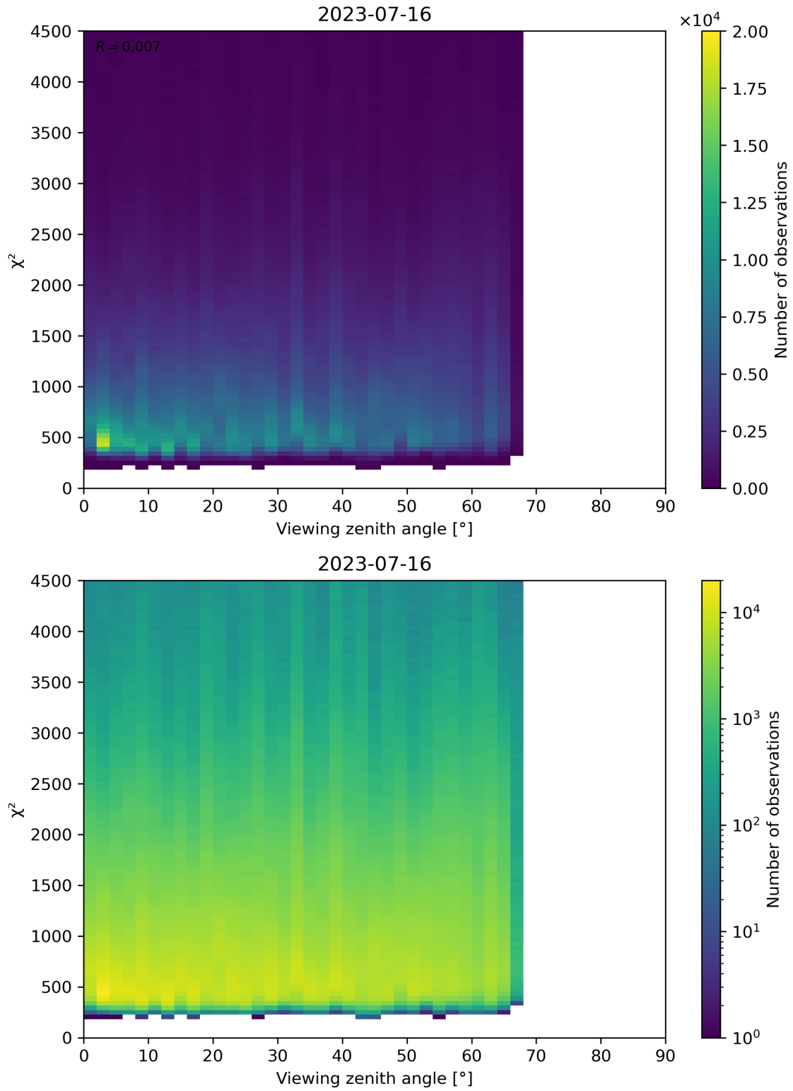
Figure 72: Scatter density plot of “Viewing zenith angle” against “ \chi^2 ” for 2023-07-15 to 2023-07-17.
