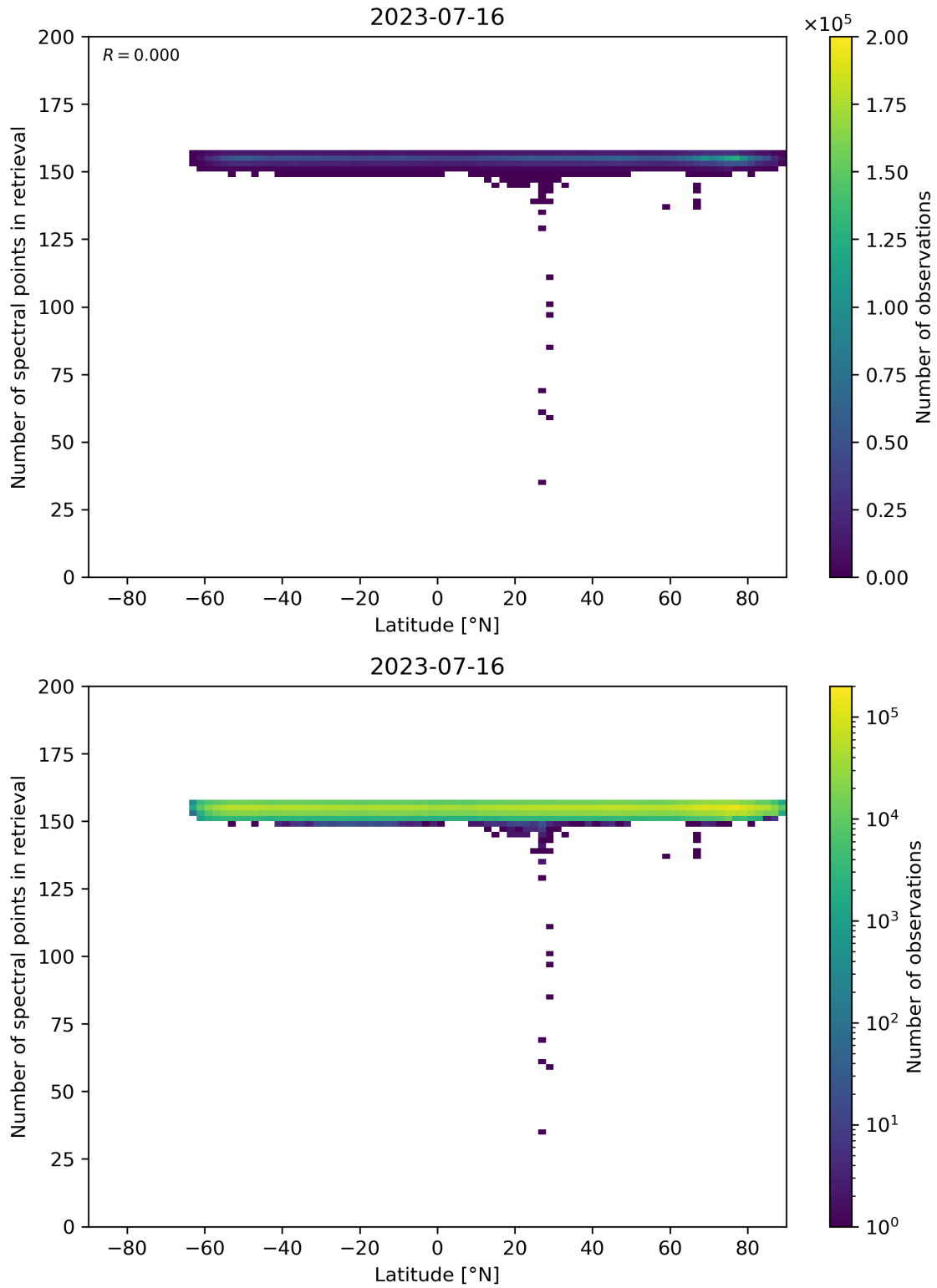
Figure 57: Scatter density plot of “Latitude” against “Number of spectral points in retrieval” for 2023-07-15 to 2023-07-17.
