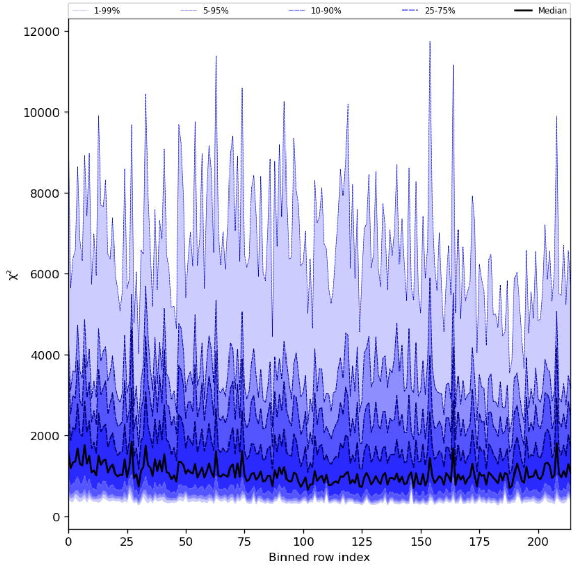
Figure 30: Along track statistics of “ \chi^2 ” for 2023-07-15 to 2023-07-17
