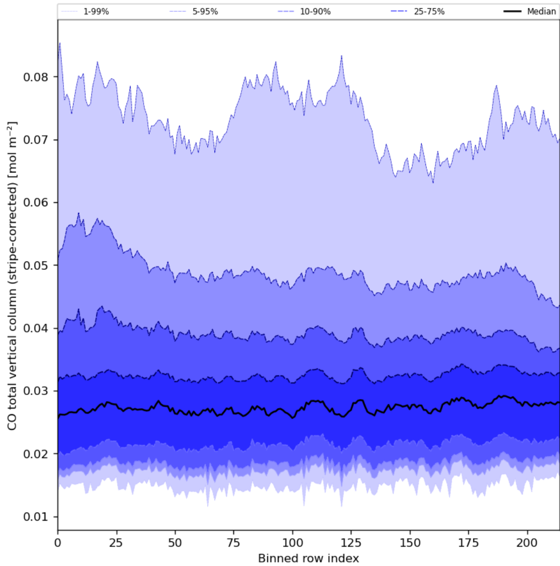
Figure 27: Along track statistics of “CO total vertical column (stripe-corrected)” for 2023-07-15 to 2023-07-17
