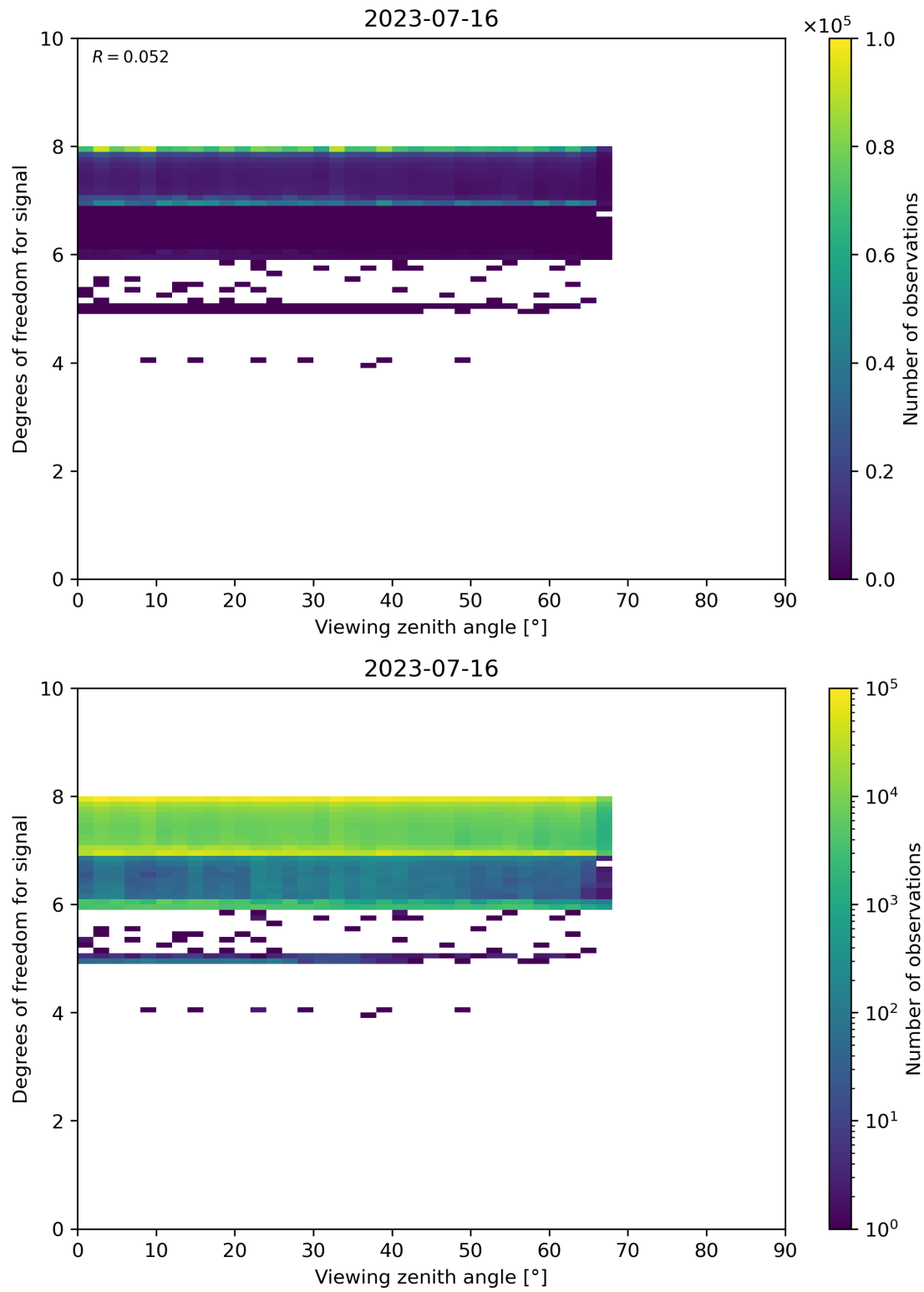
Figure 73: Scatter density plot of “Viewing zenith angle” against “Degrees of freedom for signal” for 2023-07-15 to 2023-07-17.
