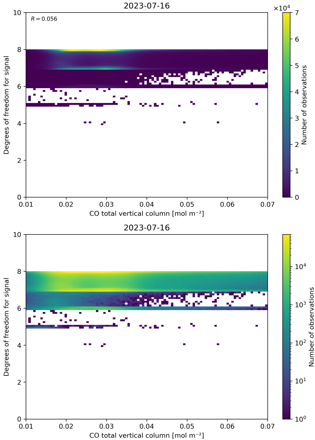
Figure 41: Scatter density plot of “CO total vertical column” against “Degrees of freedom for signal” for 2023-07-15 to 2023-07-17.
