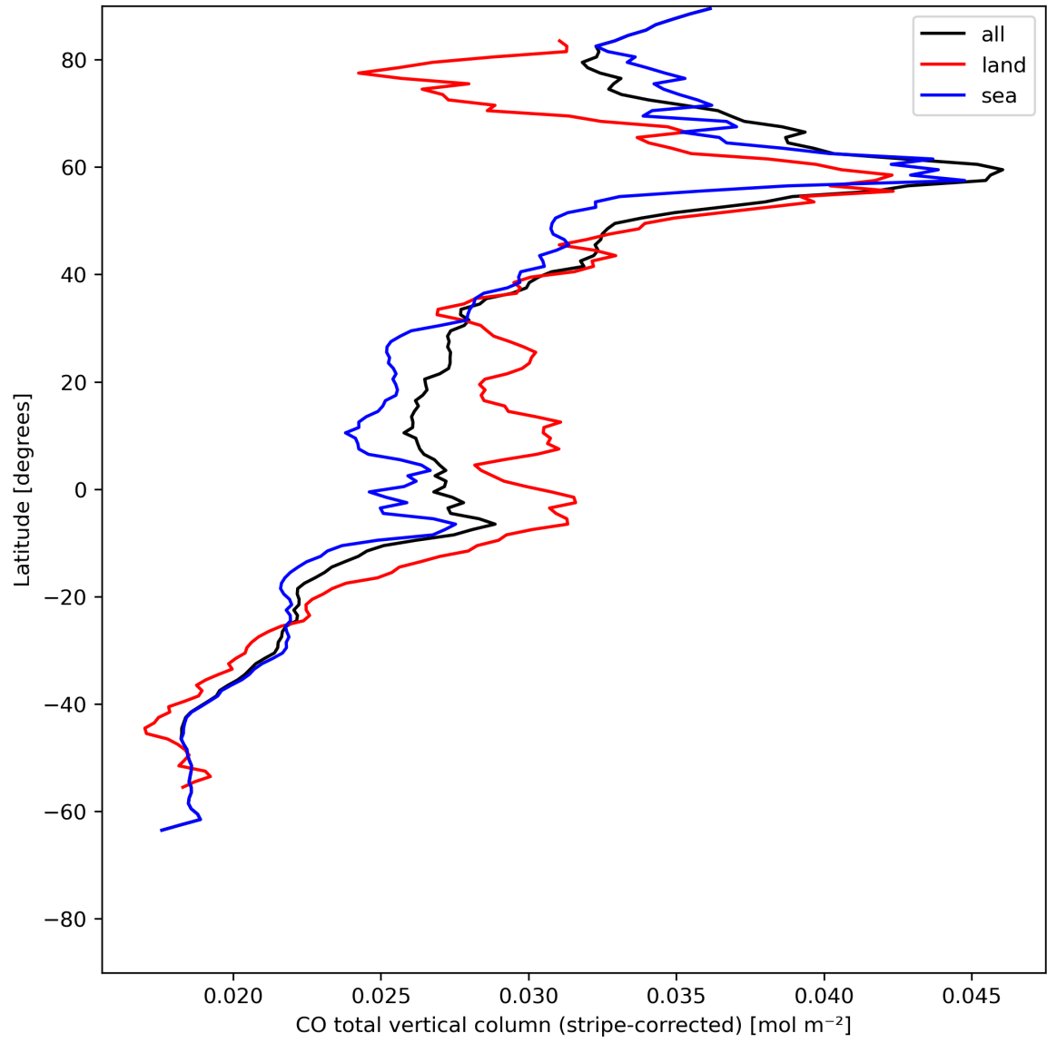
Figure 11: Zonal average of “CO total vertical column (stripe-corrected)” for 2023-07-15 to 2023-07-17.
