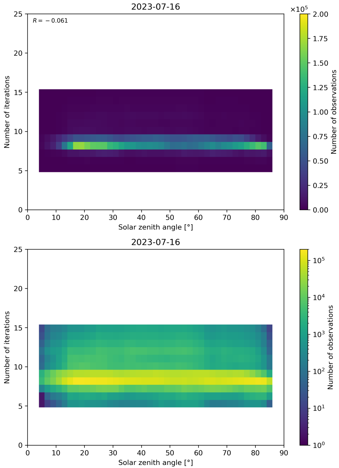
Figure 67: Scatter density plot of “Solar zenith angle” against “Number of iterations” for 2023-07-15 to 2023-07-17.
