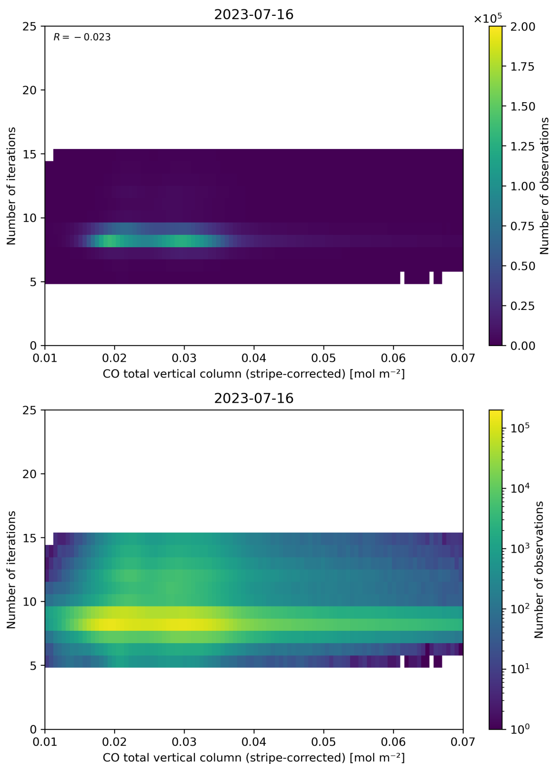
Figure 39: Scatter density plot of “CO total vertical column (stripe-corrected)” against “Number of iterations” for 2023-07-15 to 2023-07-17.
