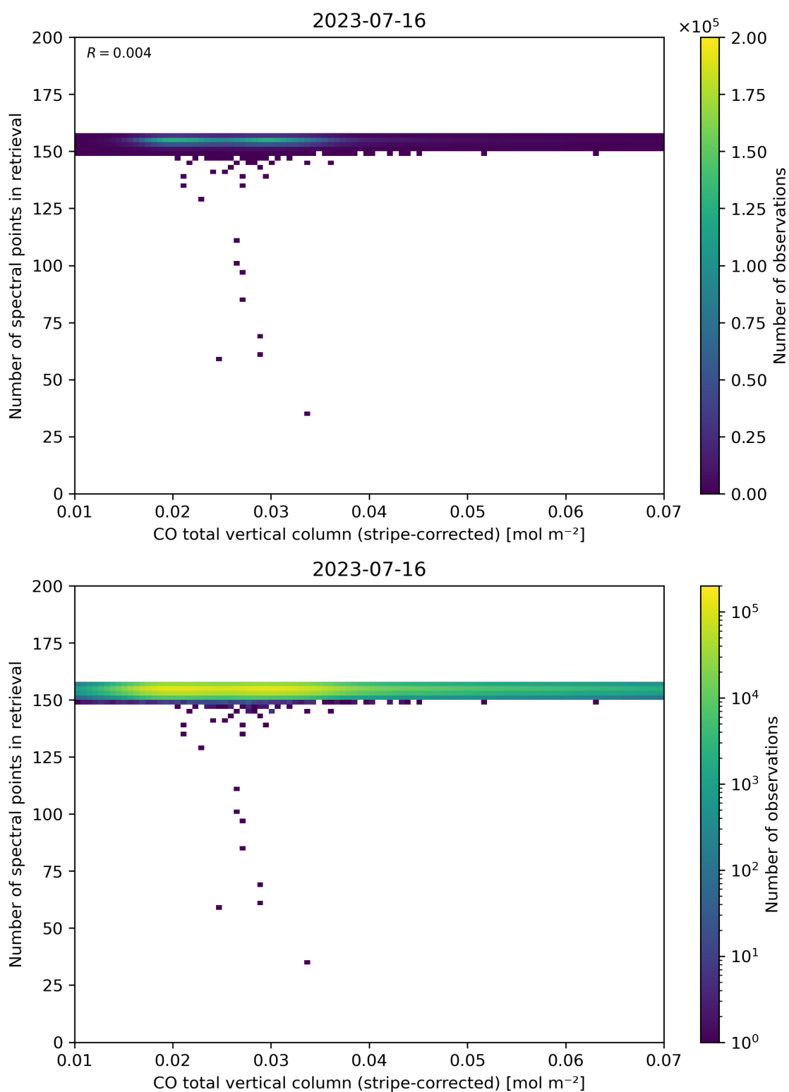
Figure 40: Scatter density plot of “CO total vertical column (stripe-corrected)” against “Number of spectral points in retrieval” for 2023-07-15 to 2023-07-17.
