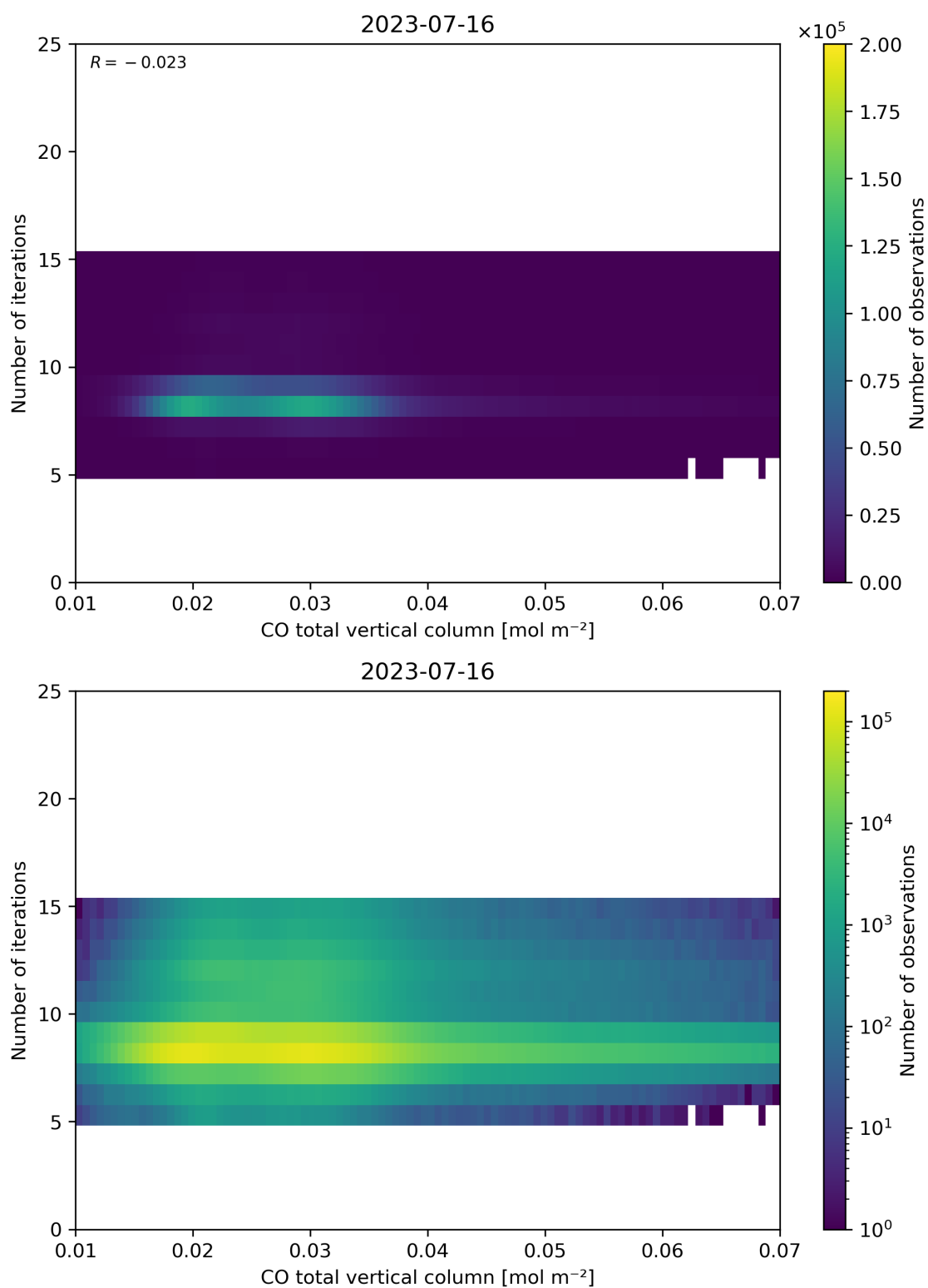
Figure 42: Scatter density plot of “CO total vertical column” against “Number of iterations” for 2023-07-15 to 2023-07-17.
