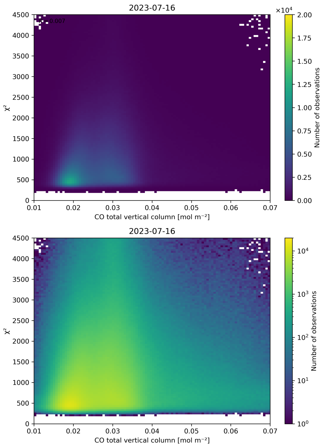
Figure 35: Scatter density plot of “CO total vertical column” against “ \chi^2 ” for 2023-07-15 to 2023-07-17.
