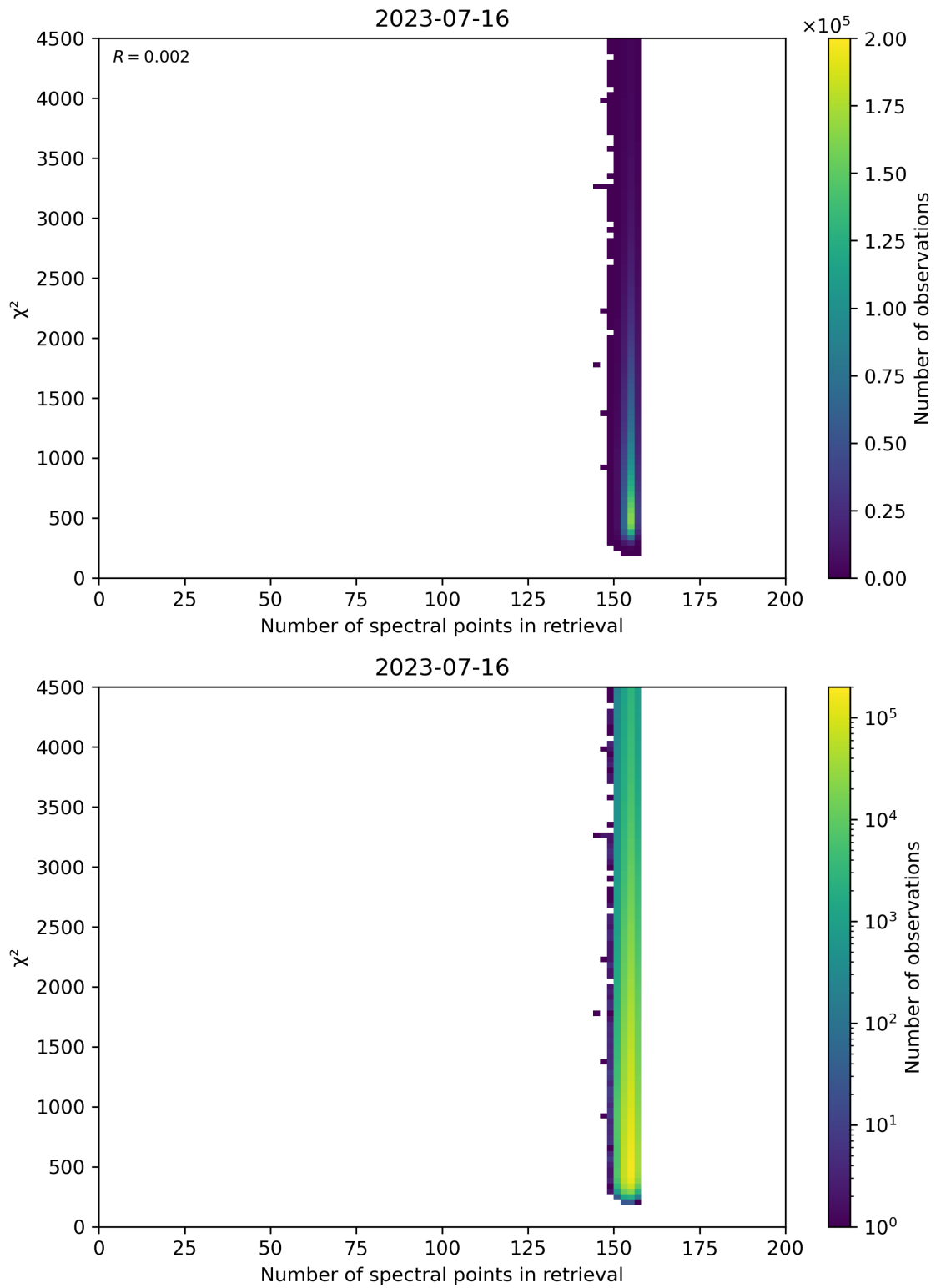
Figure 58: Scatter density plot of “Number of spectral points in retrieval” against “ \chi^2 ” for 2023-07-15 to 2023-07-17.
