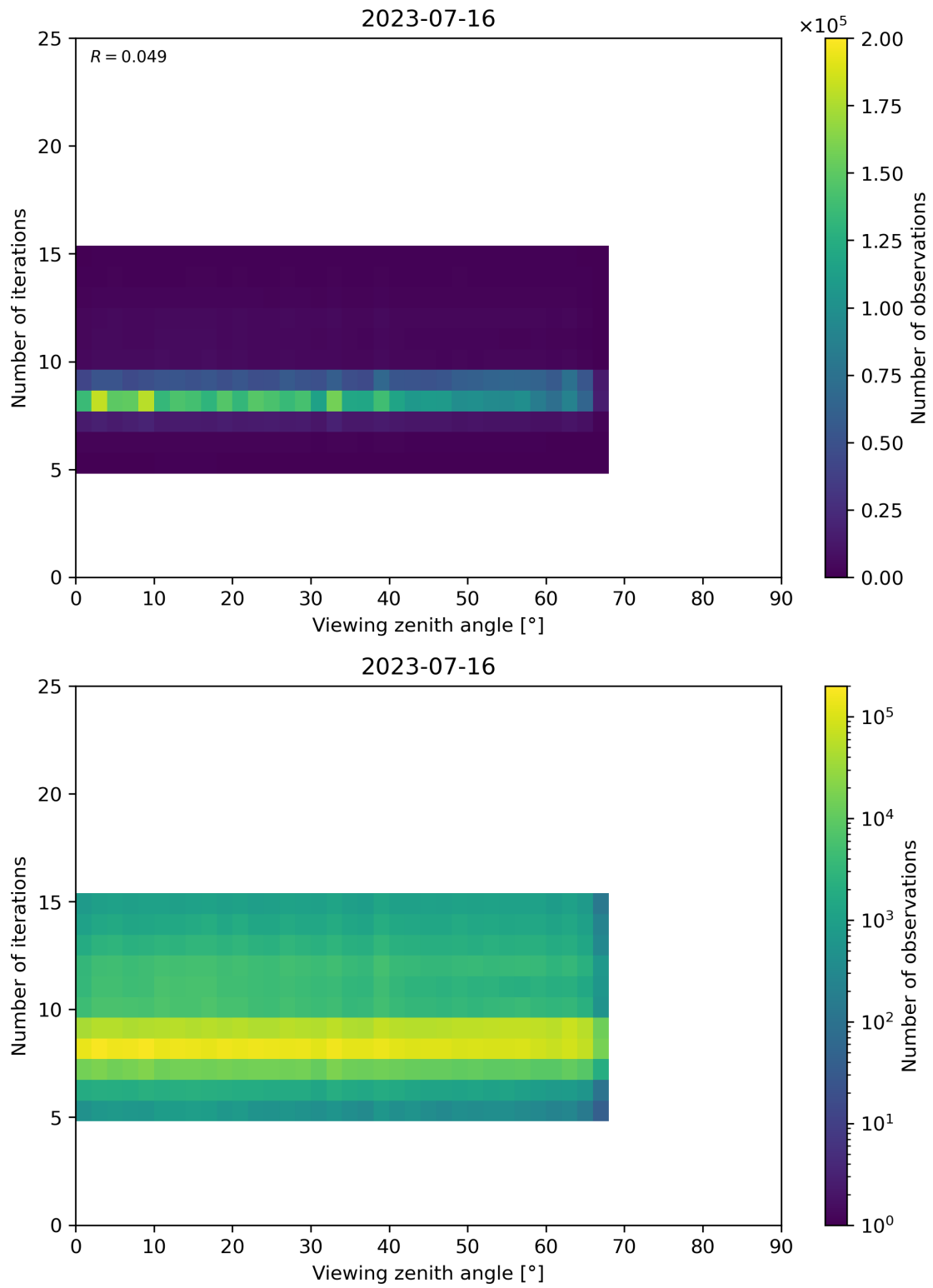
Figure 75: Scatter density plot of “Viewing zenith angle” against “Number of iterations” for 2023-07-15 to 2023-07-17.
