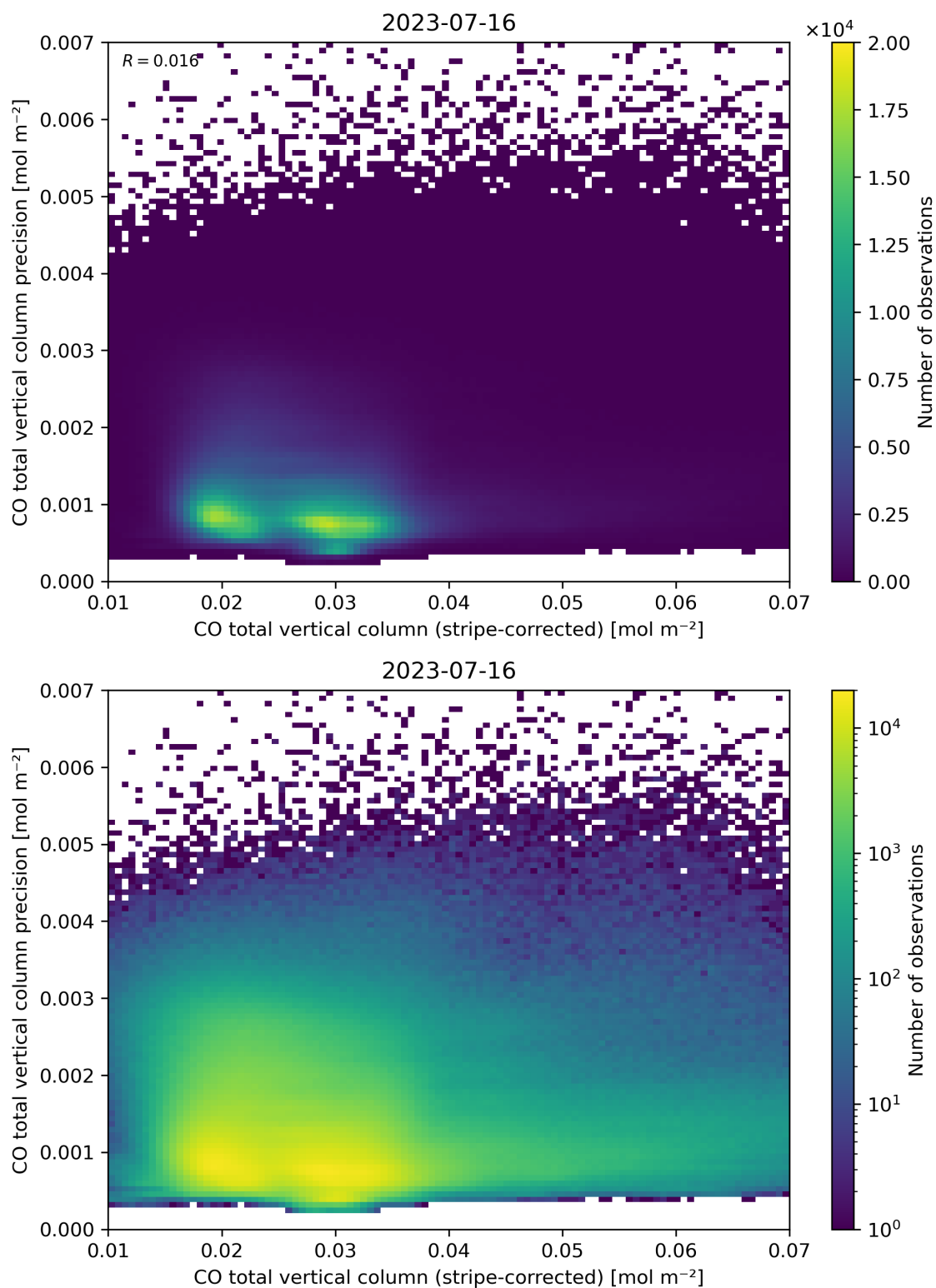
Figure 36: Scatter density plot of “CO total vertical column (stripe-corrected)” against “CO total vertical column precision” for 2023-07-15 to 2023-07-17.
