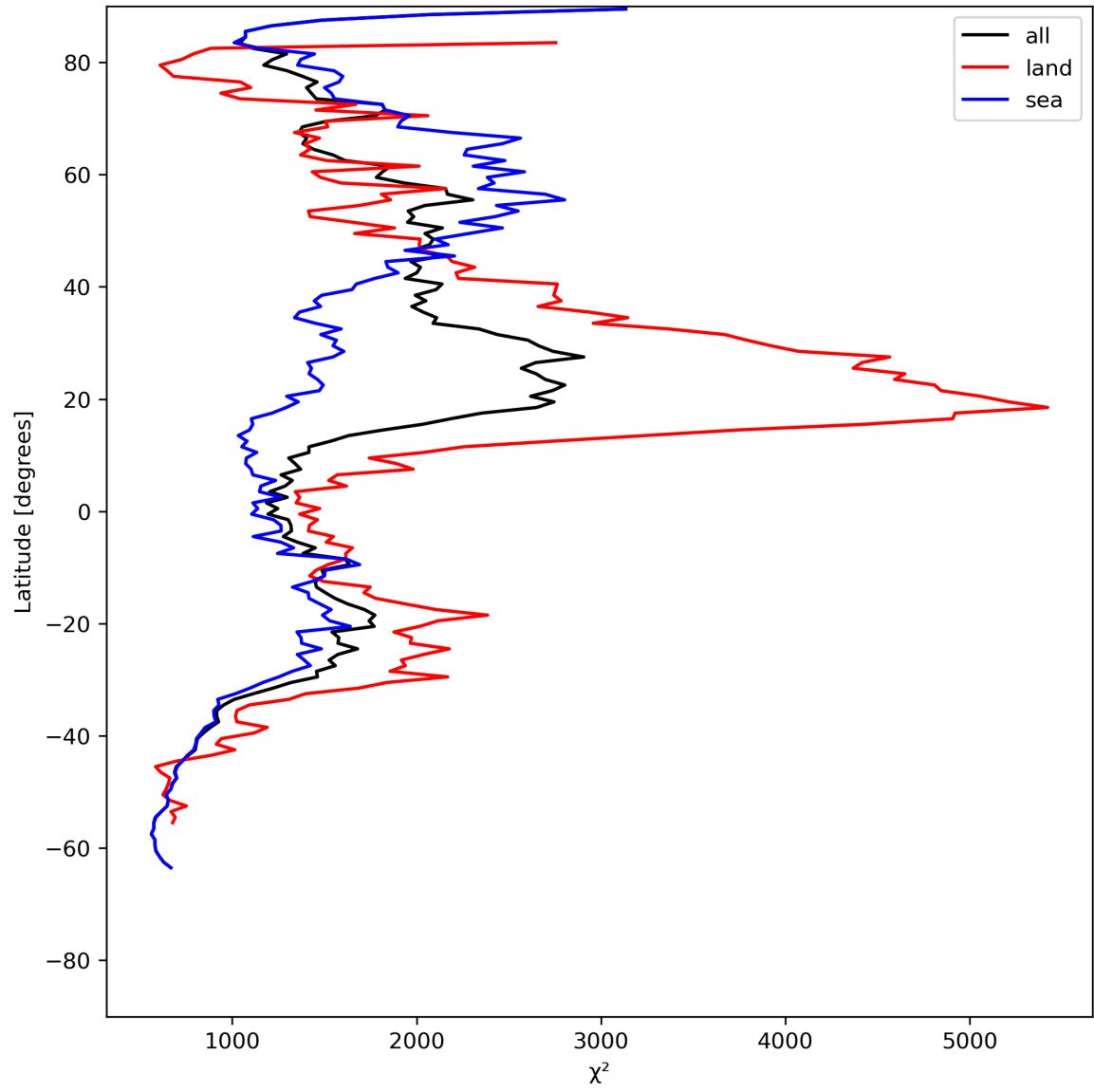
Figure 14: Zonal average of “ \chi^2 ” for 2023-07-15 to 2023-07-17.
