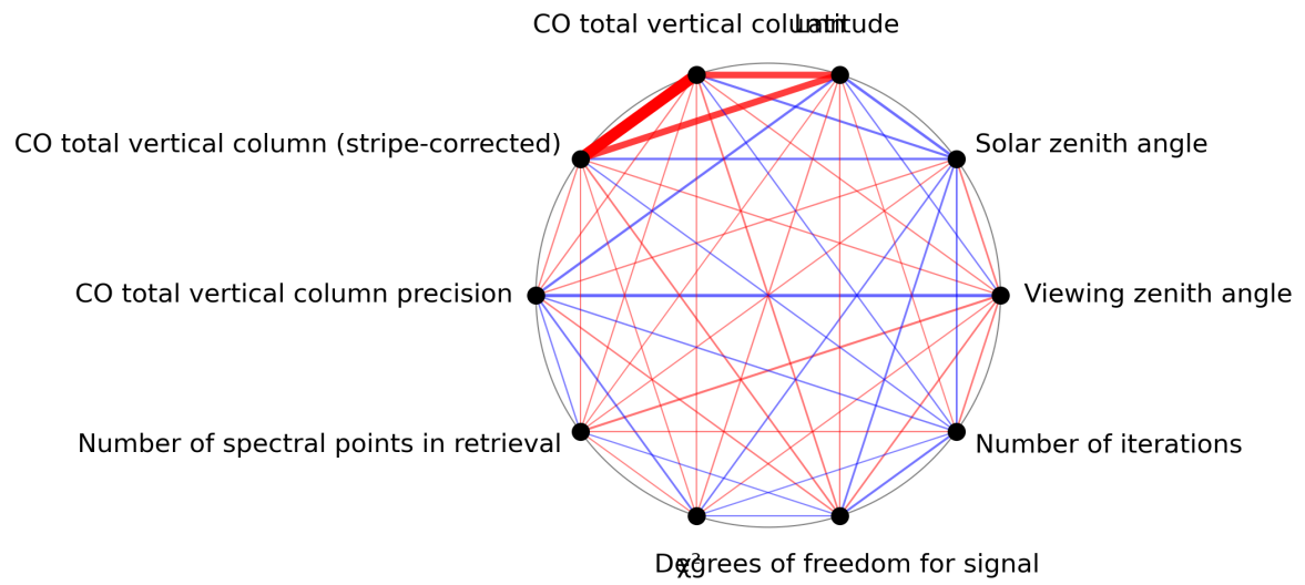
Figure 1: Map of correlation graph for 2023-07-15 to 2023-07-17.
