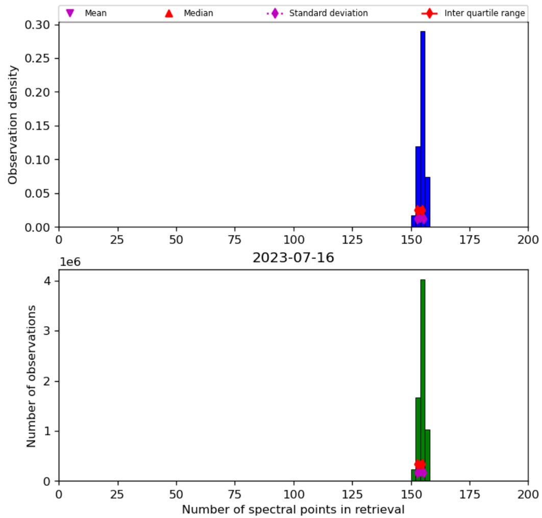
Figure 21: Histogram of “Number of spectral points in retrieval” for 2023-07-15 to 2023-07-17
