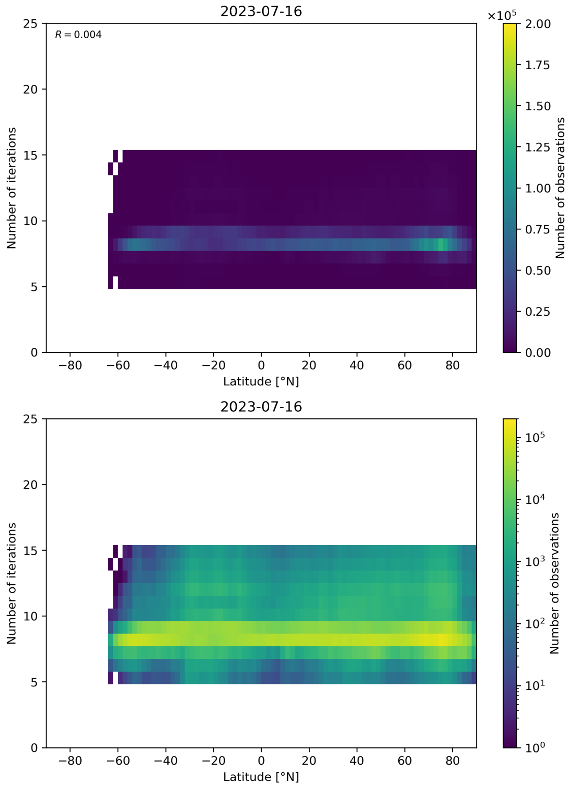
Figure 56: Scatter density plot of “Latitude” against “Number of iterations” for 2023-07-15 to 2023-07-17.
