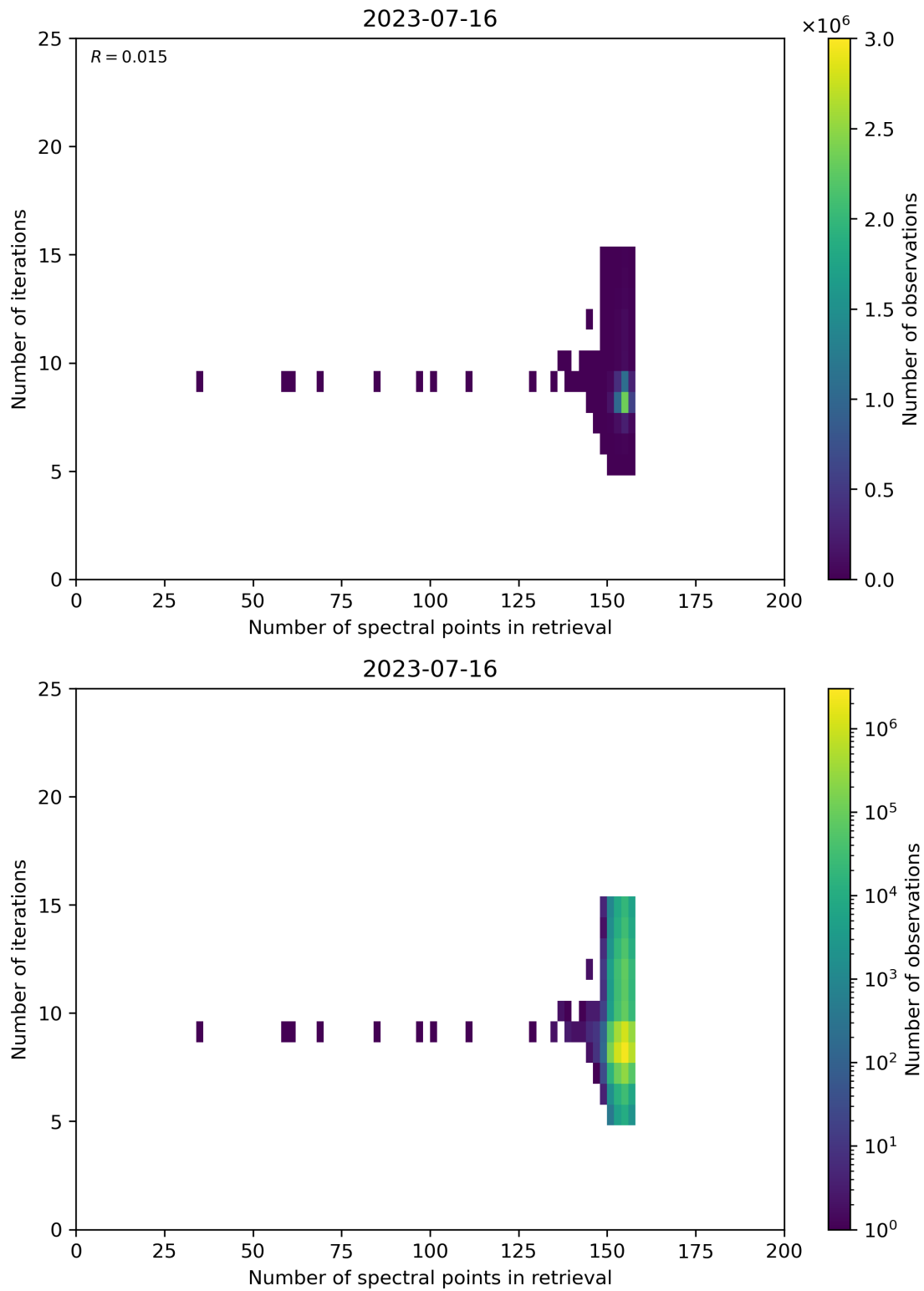
Figure 60: Scatter density plot of “Number of spectral points in retrieval” against “Number of iterations” for 2023-07-15 to 2023-07-17.
