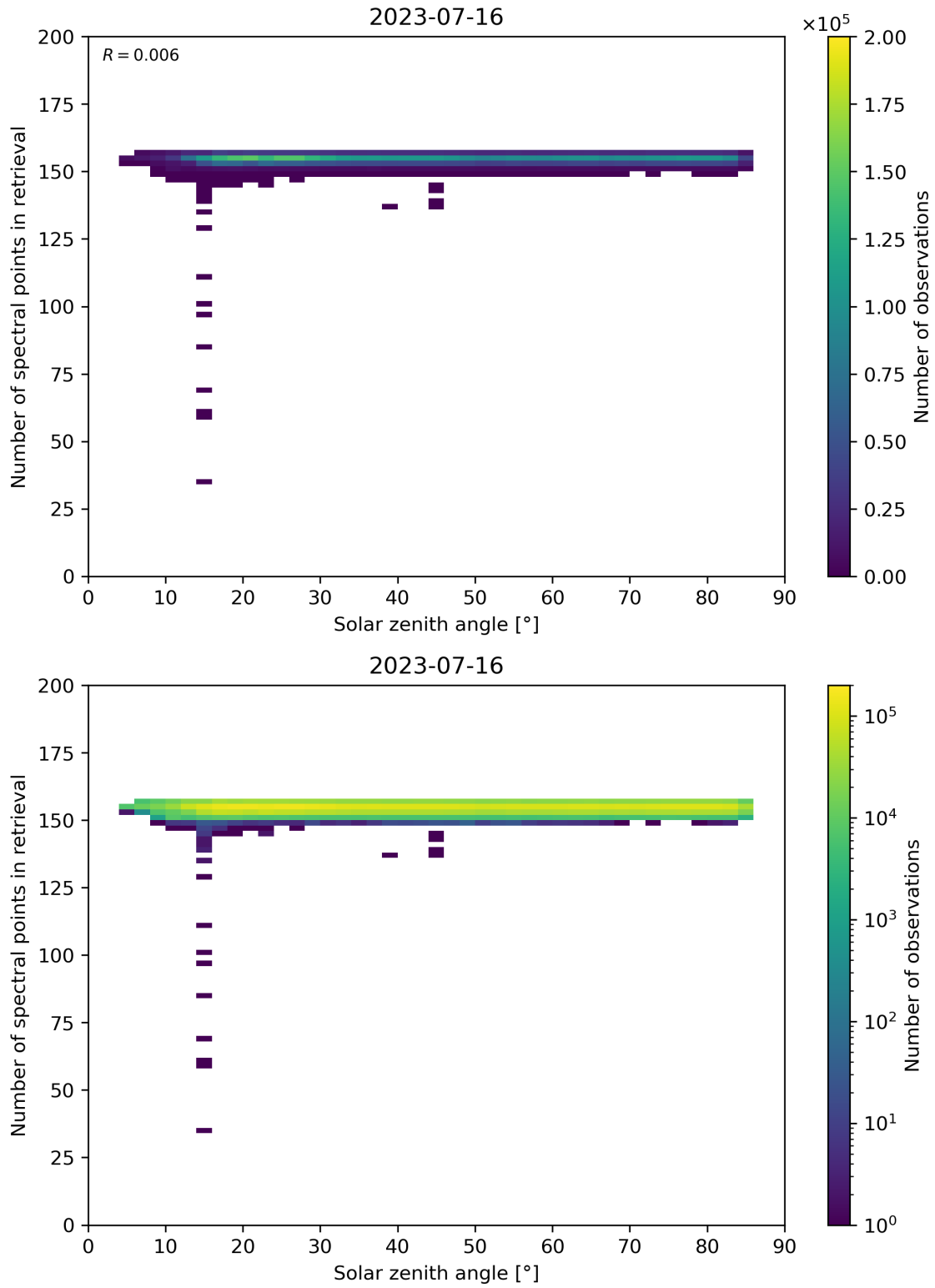
Figure 68: Scatter density plot of “Solar zenith angle” against “Number of spectral points in retrieval” for 2023-07-15 to 2023-07-17.
