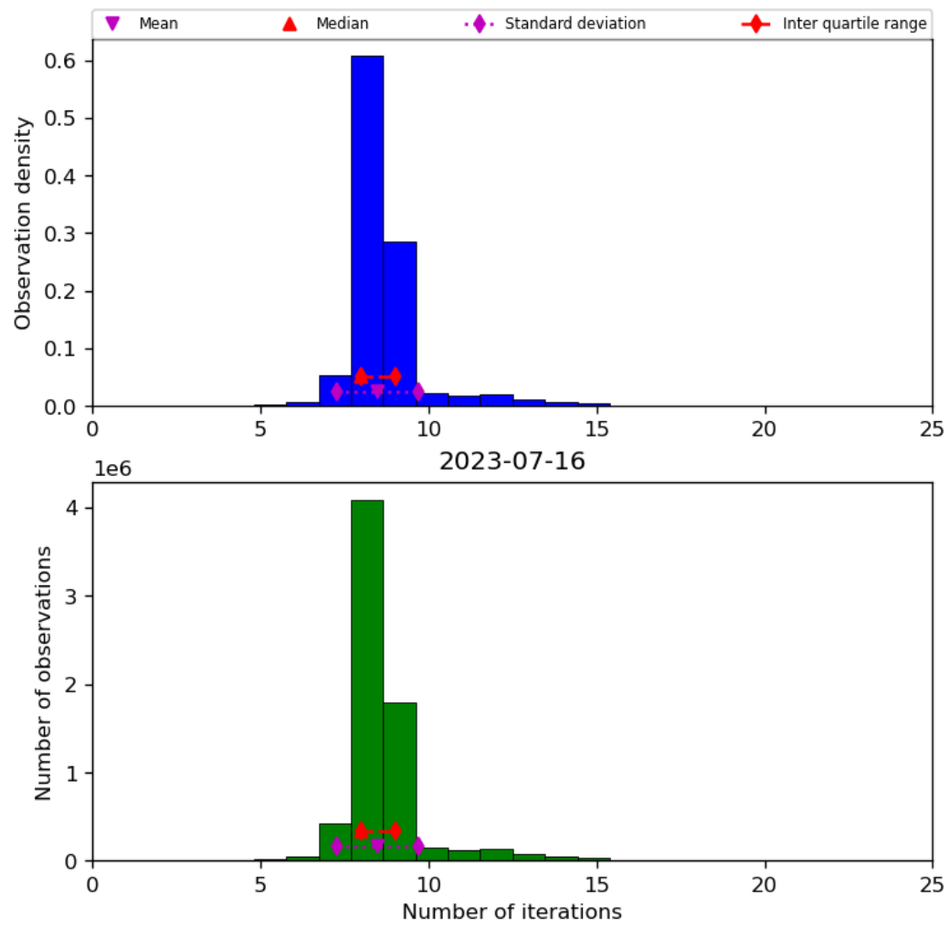
Figure 24: Histogram of “Number of iterations” for 2023-07-15 to 2023-07-17
