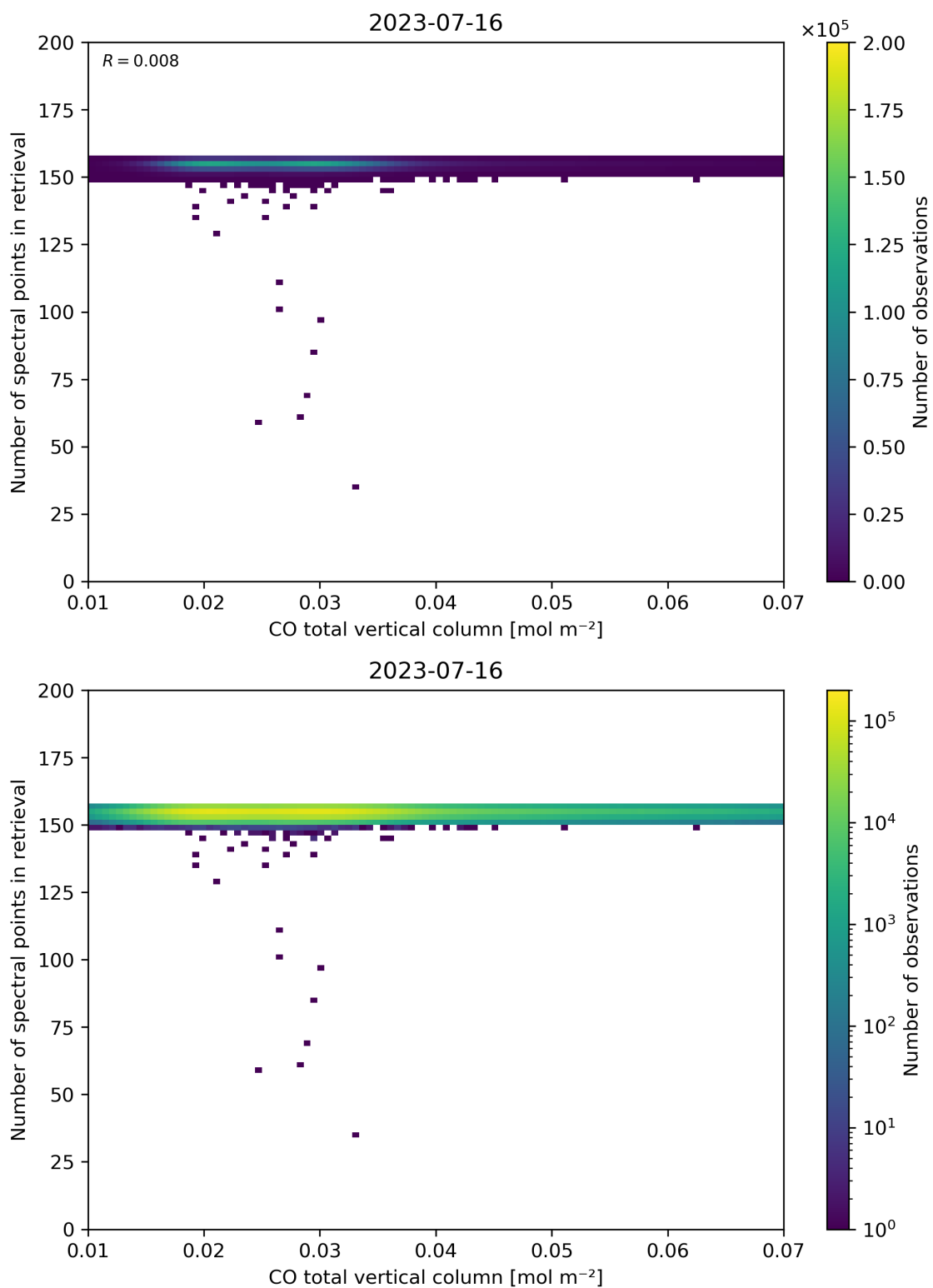
Figure 43: Scatter density plot of “CO total vertical column” against “Number of spectral points in retrieval” for 2023-07-15 to 2023-07-17.
