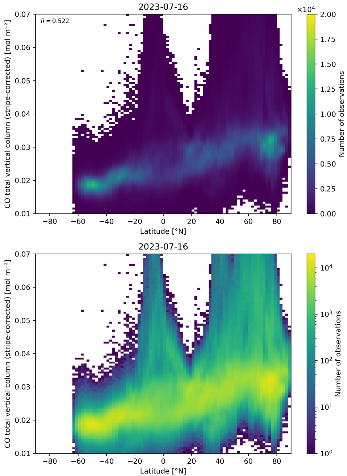
Figure 52: Scatter density plot of “Latitude” against “CO total vertical column (stripe-corrected)” for 2023-07-15 to 2023-07-17.
