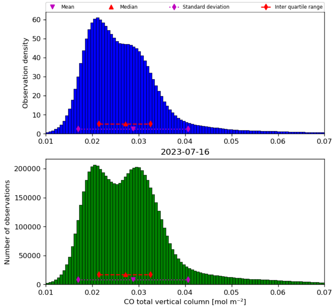
Figure 18: Histogram of “CO total vertical column” for 2023-07-15 to 2023-07-17
