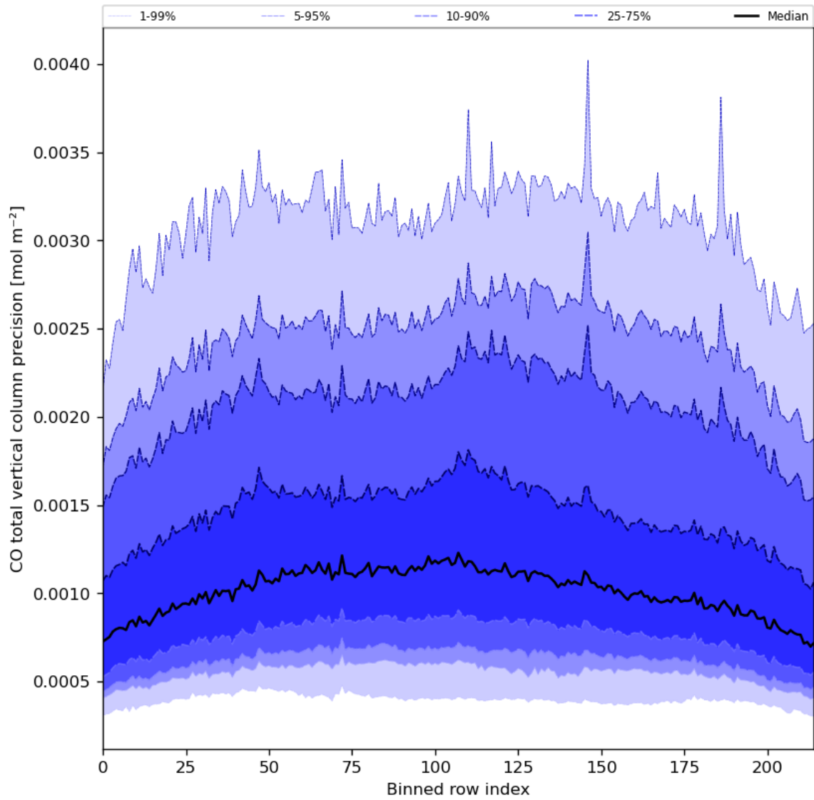
Figure 28: Along track statistics of “CO total vertical column precision” for 2023-07-15 to 2023-07-17
