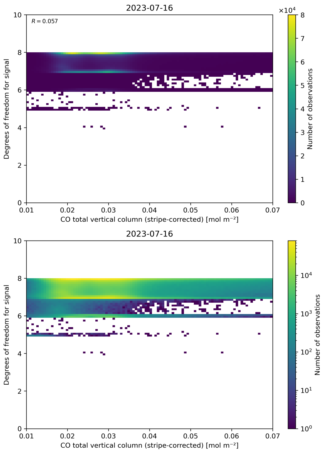
Figure 38: Scatter density plot of “CO total vertical column (stripe-corrected)” against “Degrees of freedom for signal” for 2023-07-15 to 2023-07-17.
