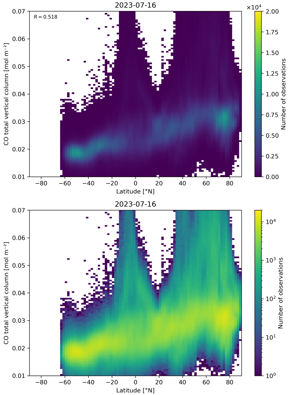
Figure 51: Scatter density plot of “Latitude” against “CO total vertical column” for 2023-07-15 to 2023-07-17.
