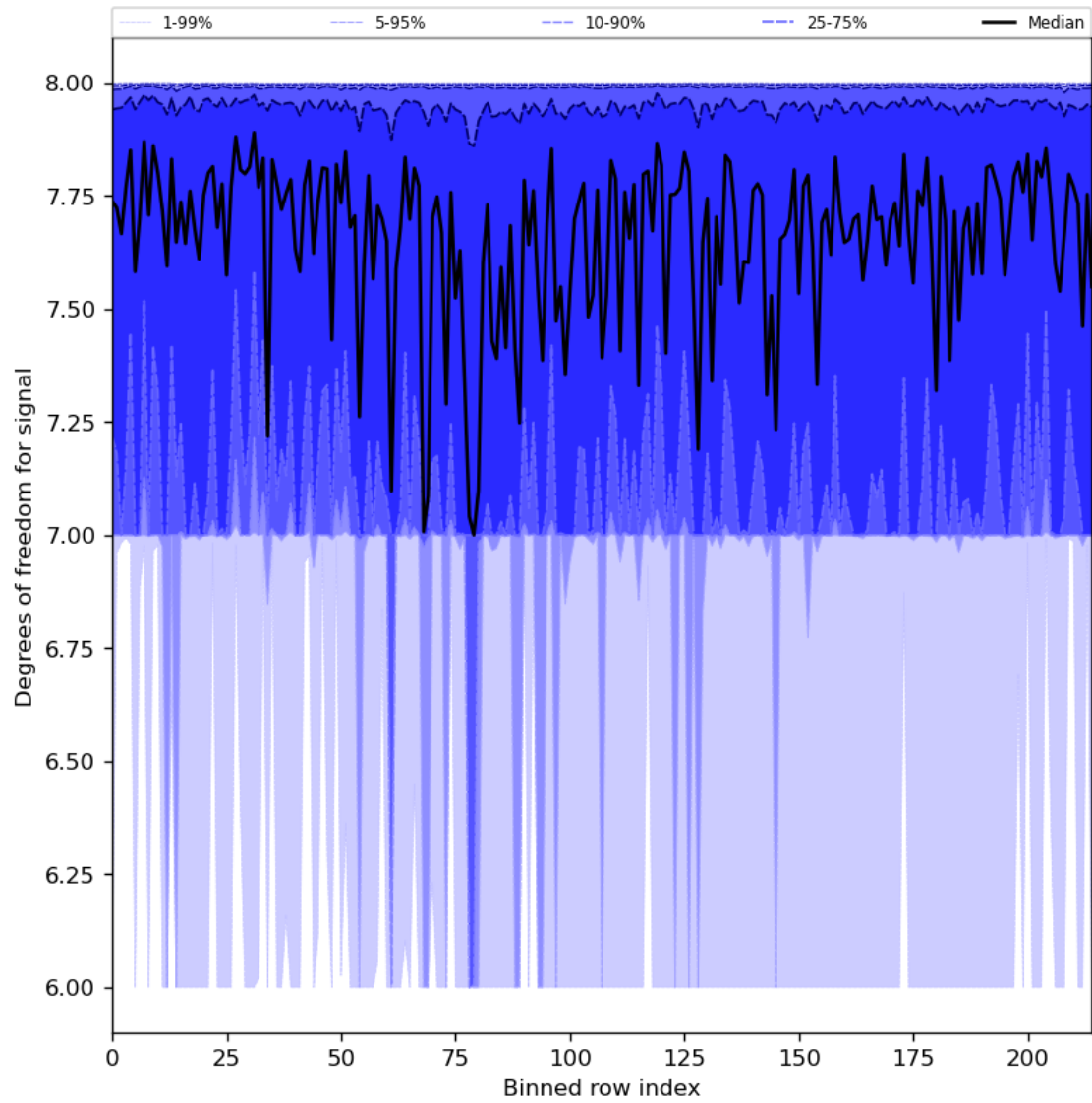
Figure 31: Along track statistics of “Degrees of freedom for signal” for 2023-07-15 to 2023-07-17
