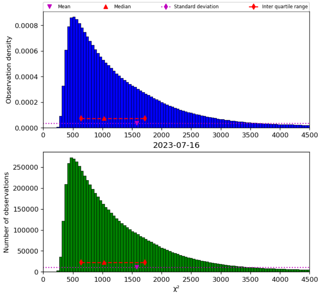
Figure 22: Histogram of “ \chi^2 ” for 2023-07-15 to 2023-07-17
