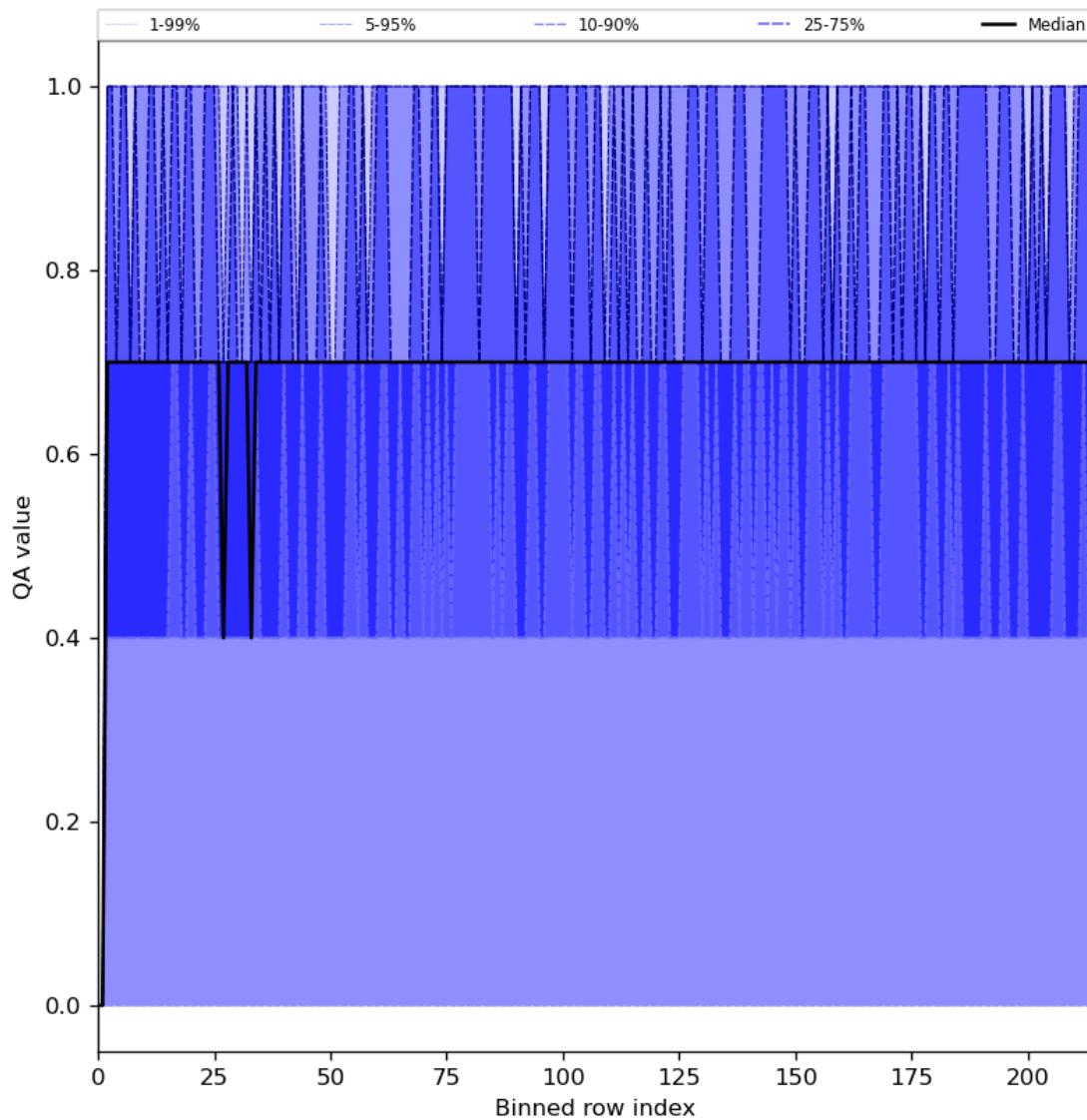
Figure 25: Along track statistics of “QA value” for 2023-07-15 to 2023-07-17
