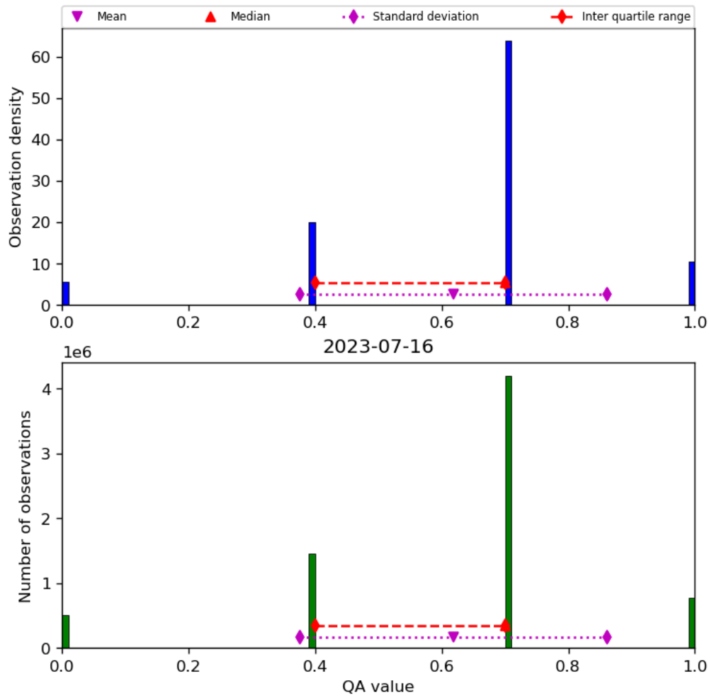
Figure 17: Histogram of “QA value” for 2023-07-15 to 2023-07-17
