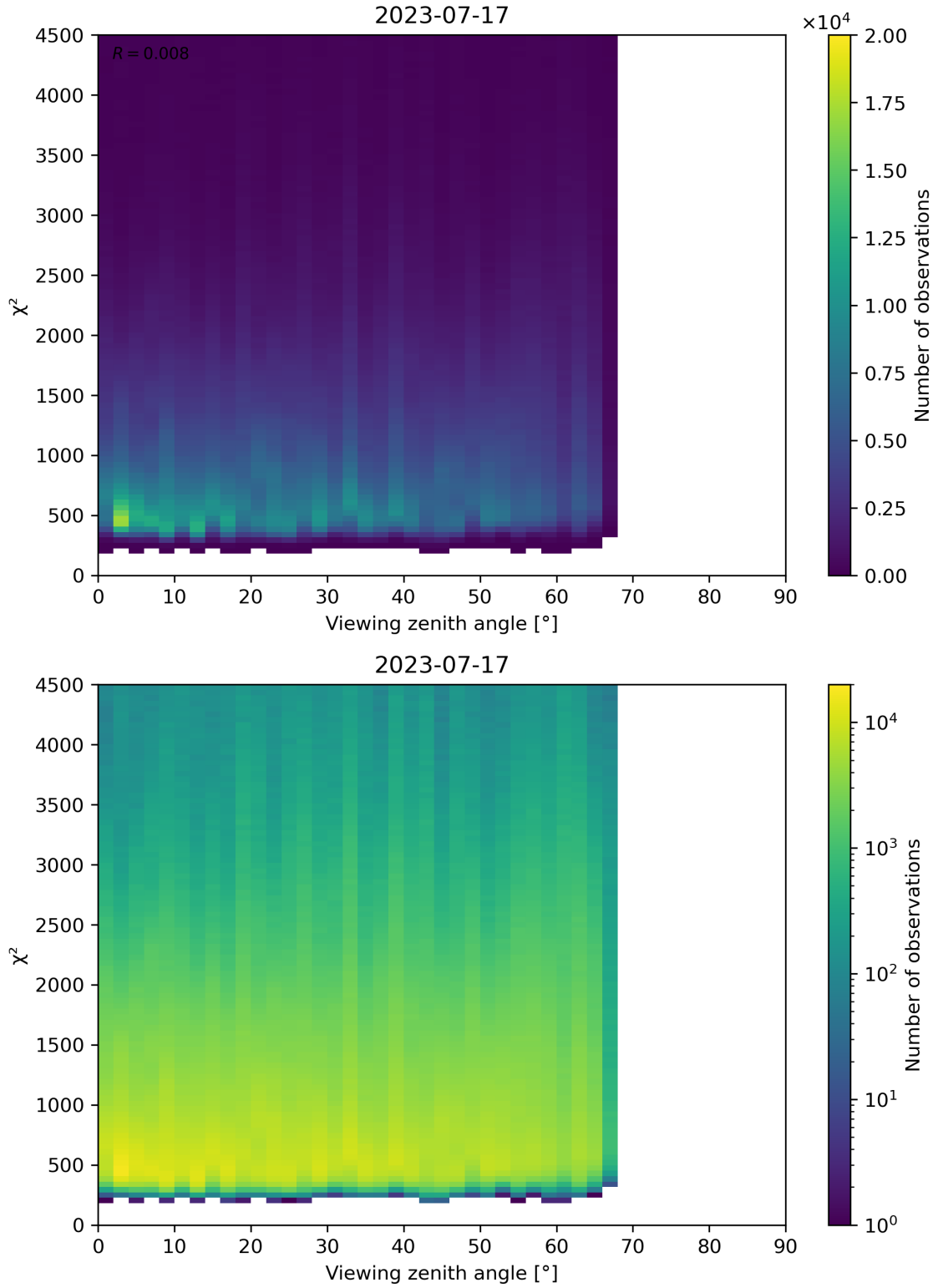
Figure 72: Scatter density plot of “Viewing zenith angle” against “ \chi^2 ” for 2023-07-16 to 2023-07-18.
