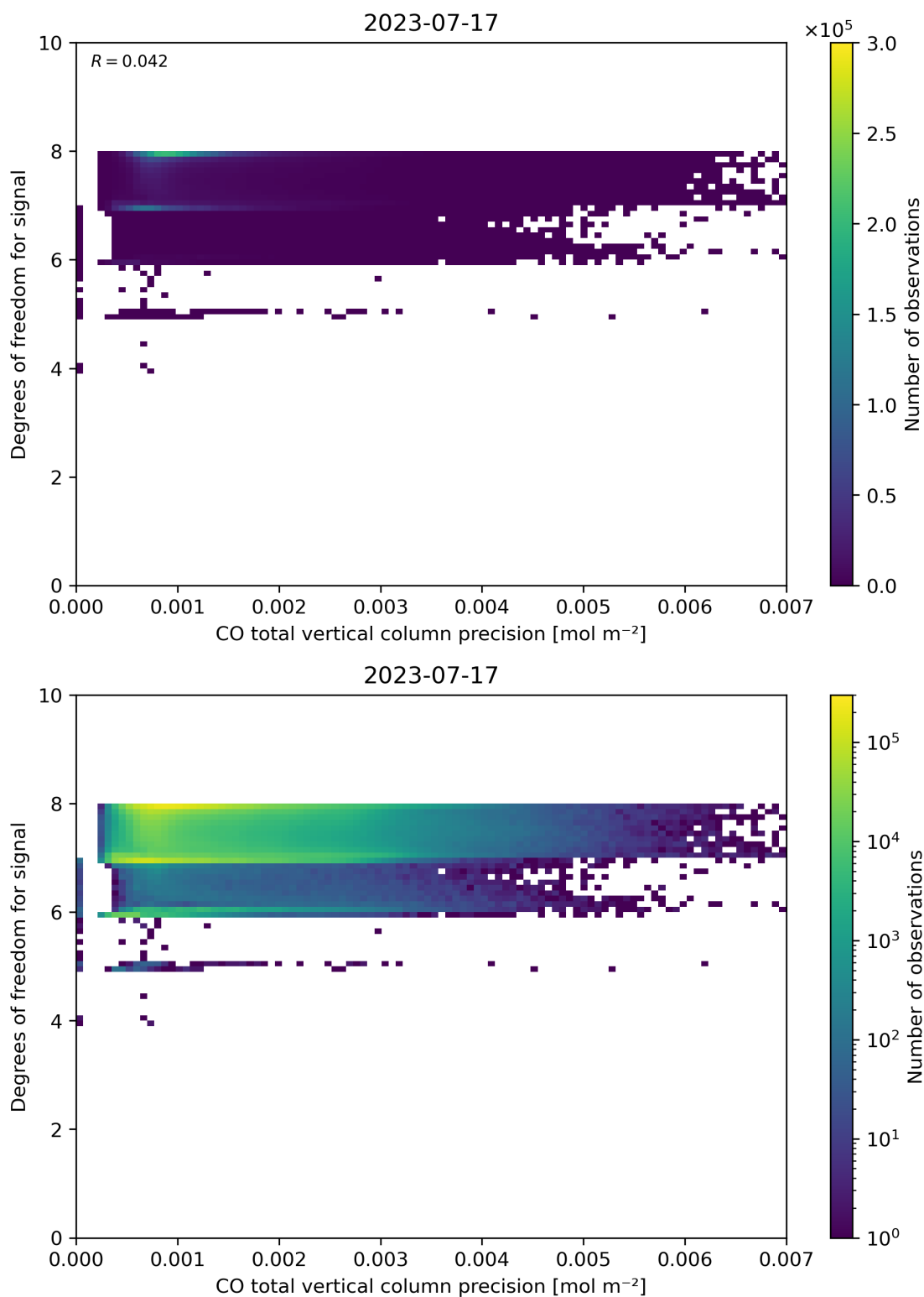
Figure 45: Scatter density plot of “CO total vertical column precision” against “Degrees of freedom for signal” for 2023-07-16 to 2023-07-18.
