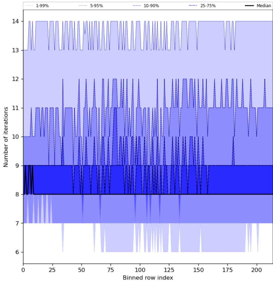
Figure 32: Along track statistics of “Number of iterations” for 2023-07-16 to 2023-07-18
