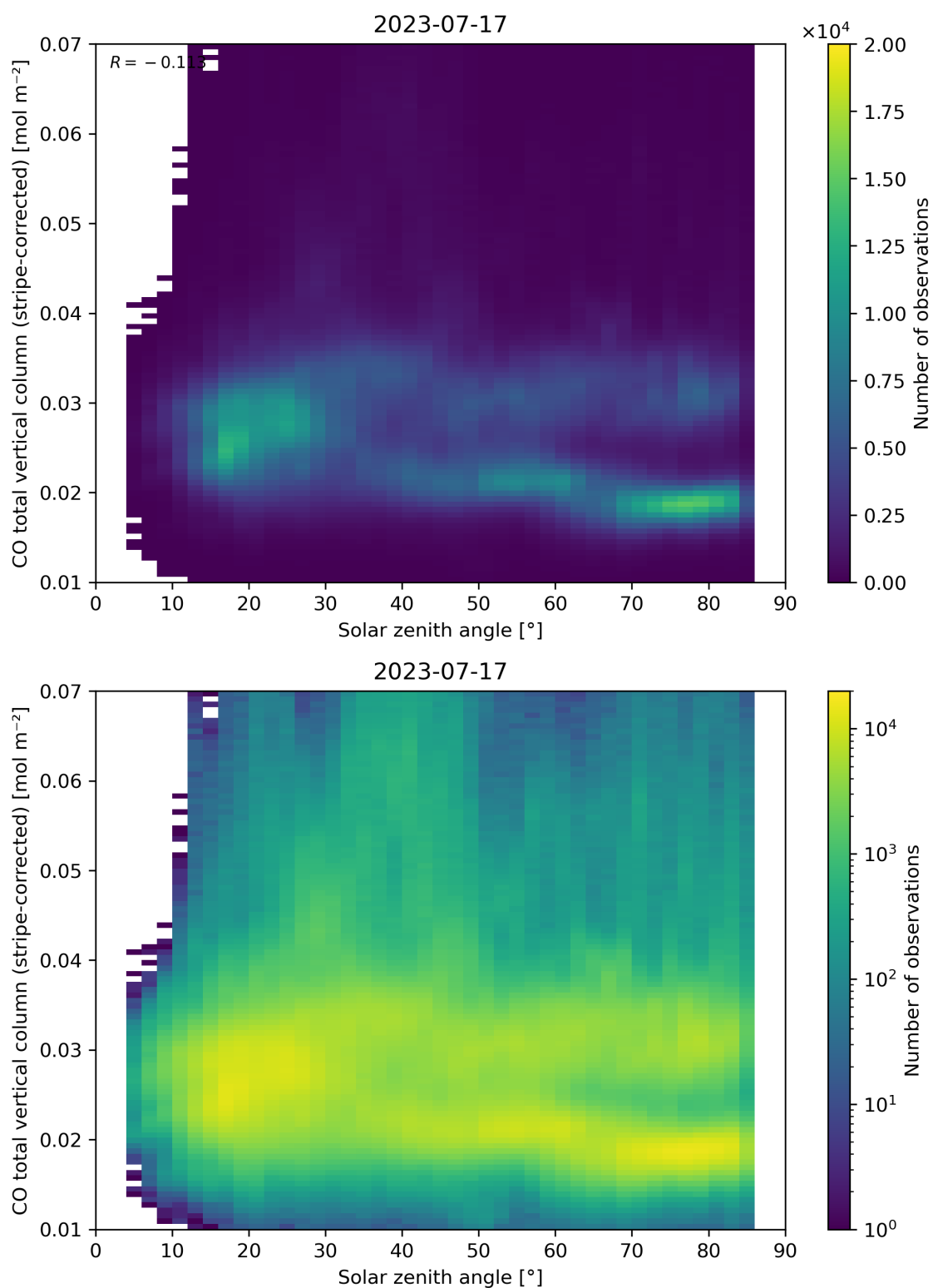
Figure 62: Scatter density plot of “Solar zenith angle” against “CO total vertical column (stripe-corrected)” for 2023-07-16 to 2023-07-18.
