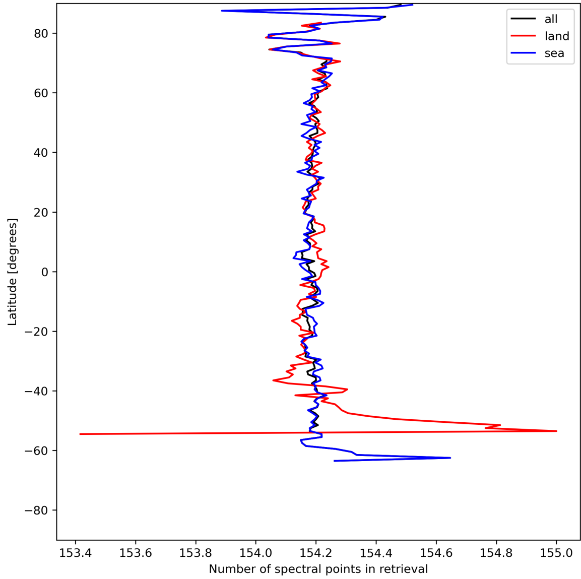
Figure 13: Zonal average of “Number of spectral points in retrieval” for 2023-07-16 to 2023-07-18.
