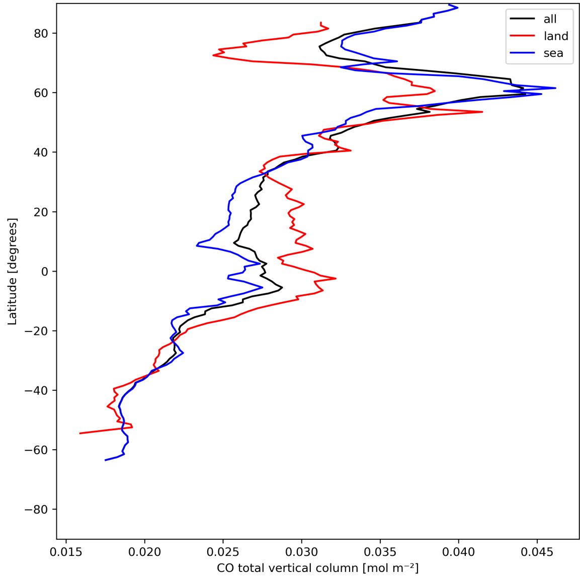
Figure 10: Zonal average of “CO total vertical column” for 2023-07-16 to 2023-07-18.
