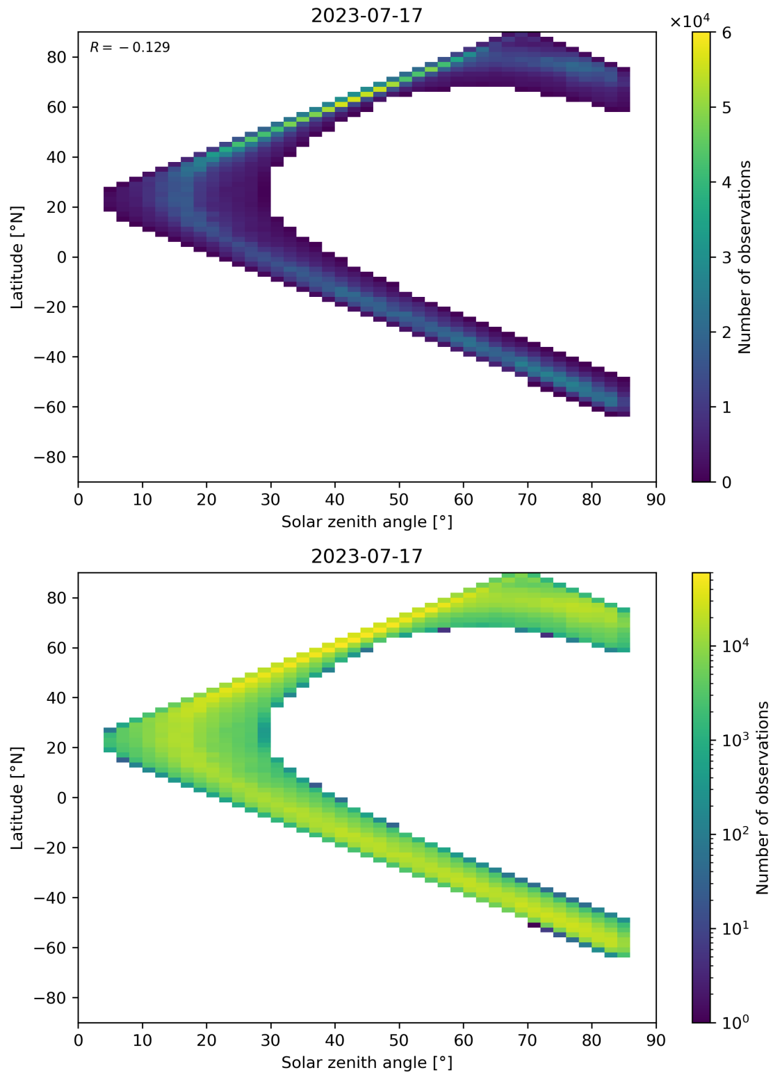
Figure 66: Scatter density plot of “Solar zenith angle” against “Latitude” for 2023-07-16 to 2023-07-18.
