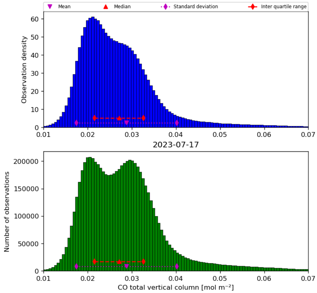
Figure 18: Histogram of “CO total vertical column” for 2023-07-16 to 2023-07-18
