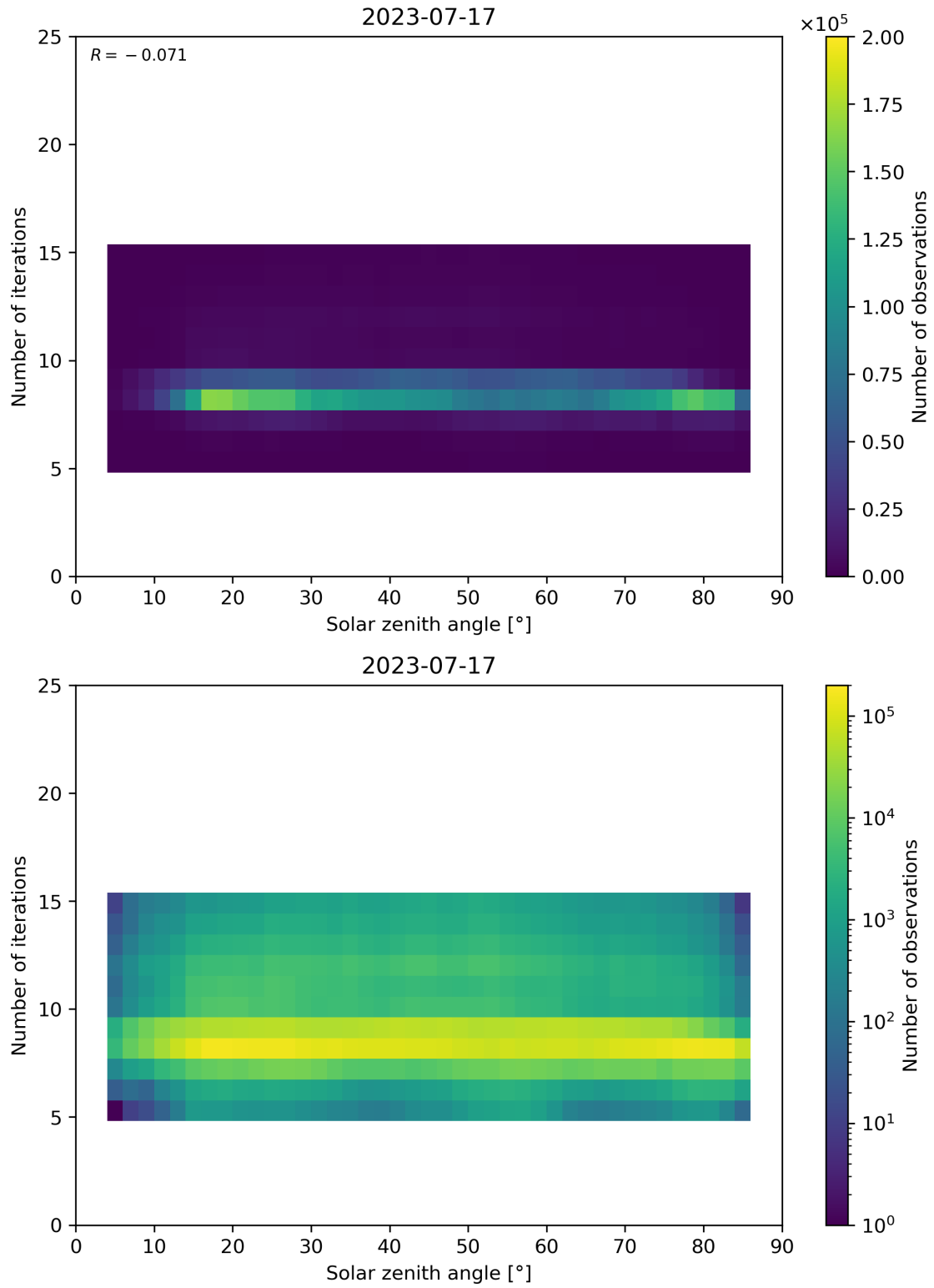
Figure 67: Scatter density plot of “Solar zenith angle” against “Number of iterations” for 2023-07-16 to 2023-07-18.
