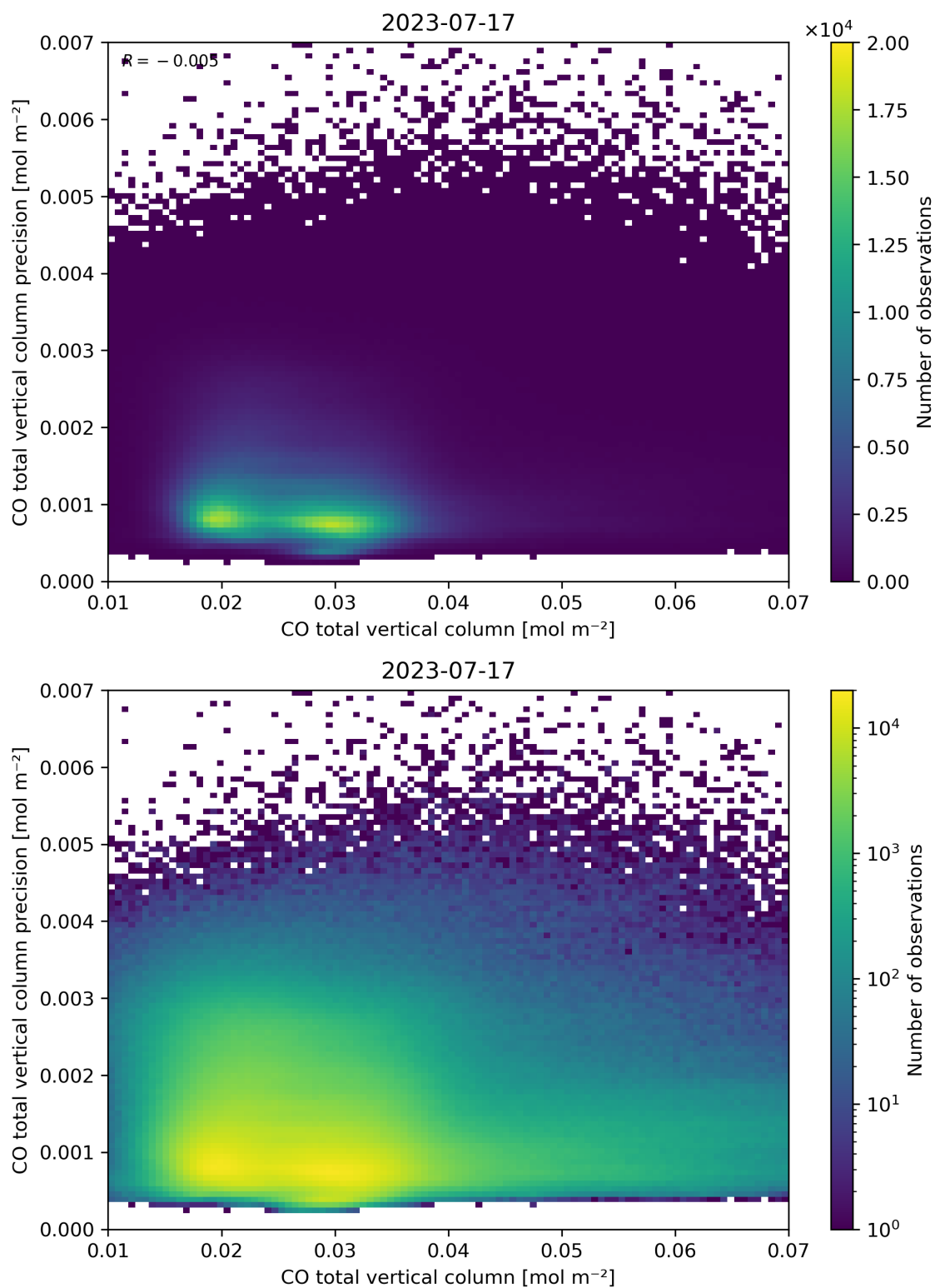
Figure 34: Scatter density plot of “CO total vertical column” against “CO total vertical column precision” for 2023-07-16 to 2023-07-18.
