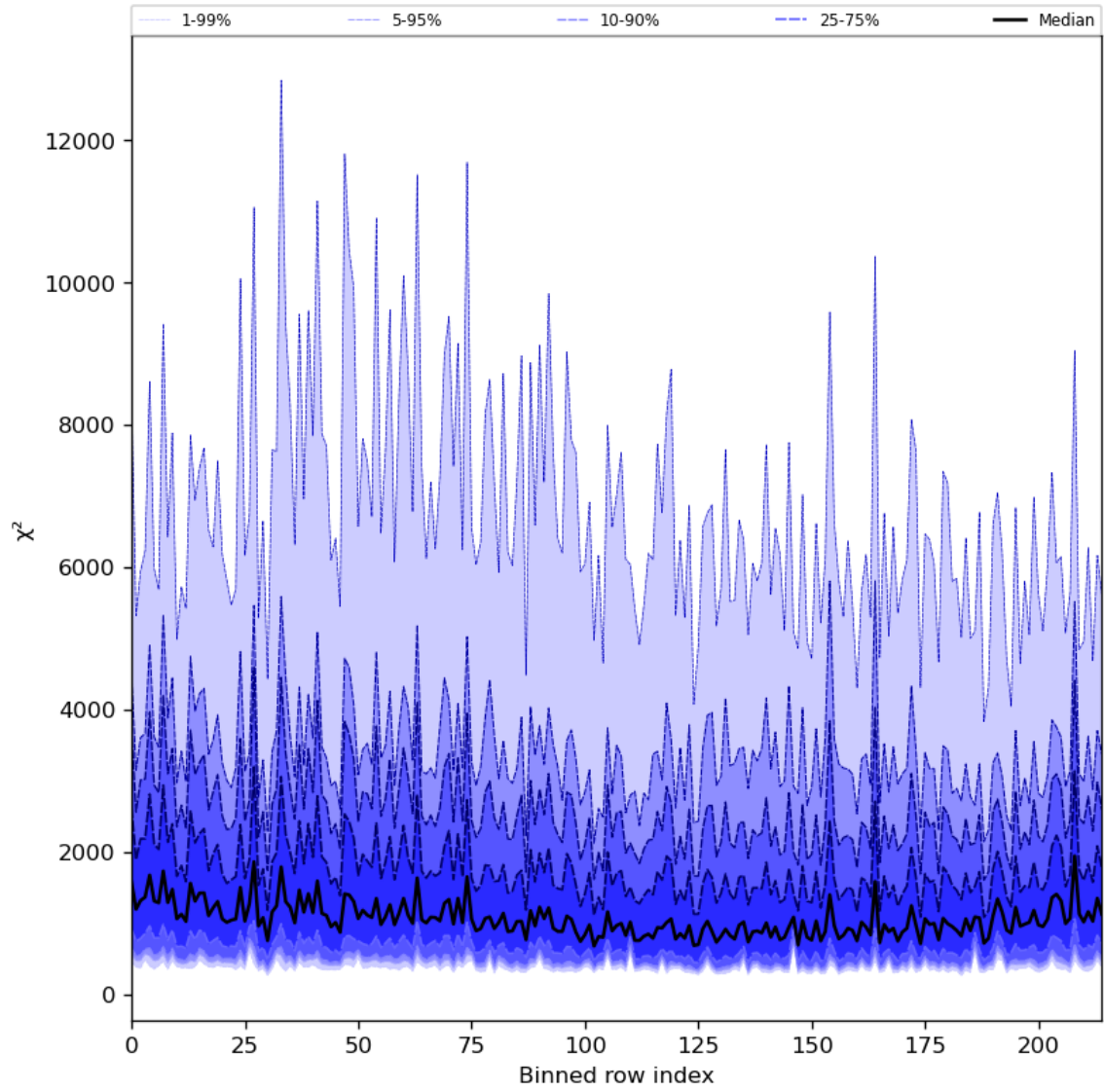
Figure 30: Along track statistics of “ \chi^2 ” for 2023-07-16 to 2023-07-18
