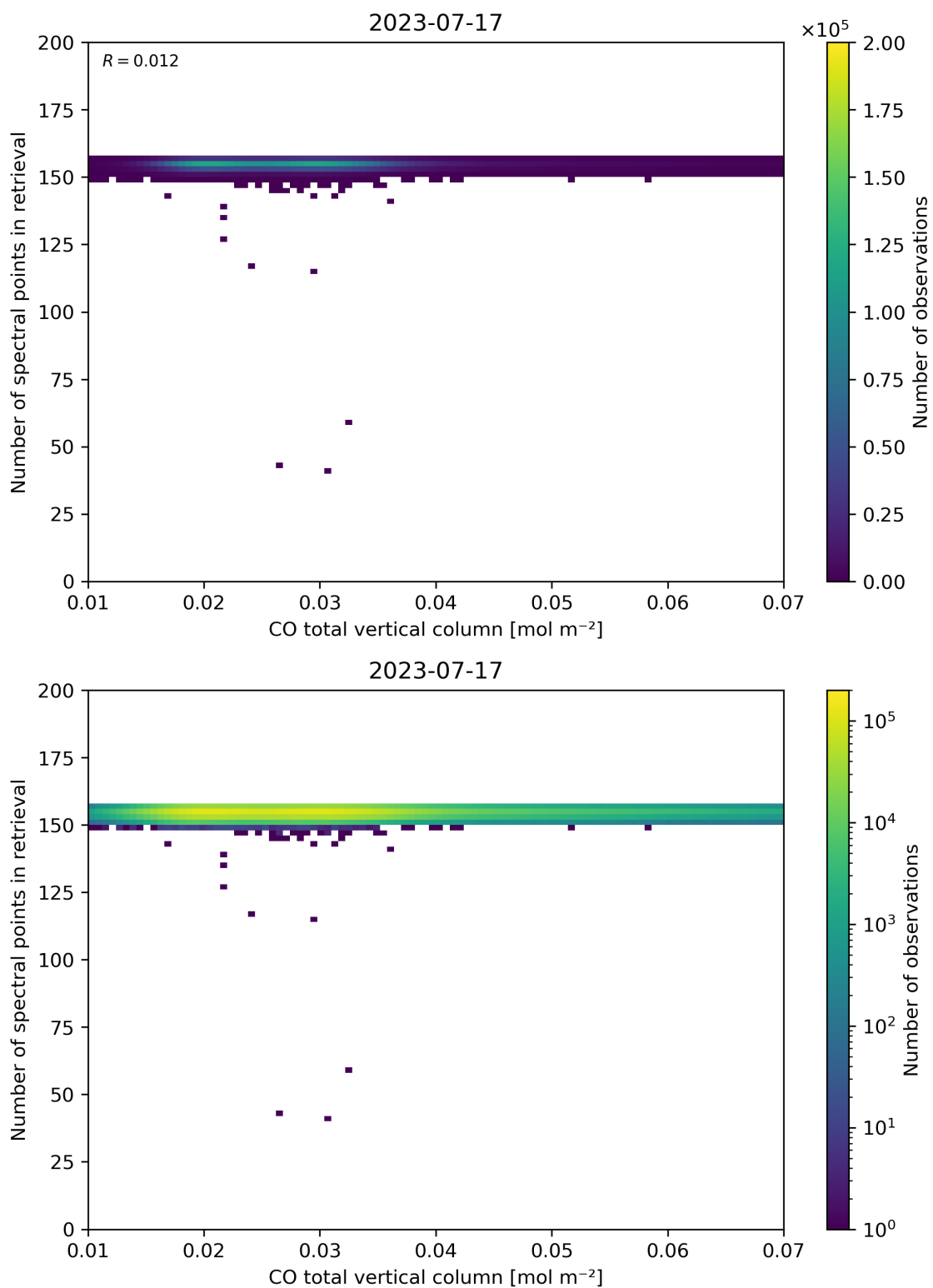
Figure 43: Scatter density plot of “CO total vertical column” against “Number of spectral points in retrieval” for 2023-07-16 to 2023-07-18.
