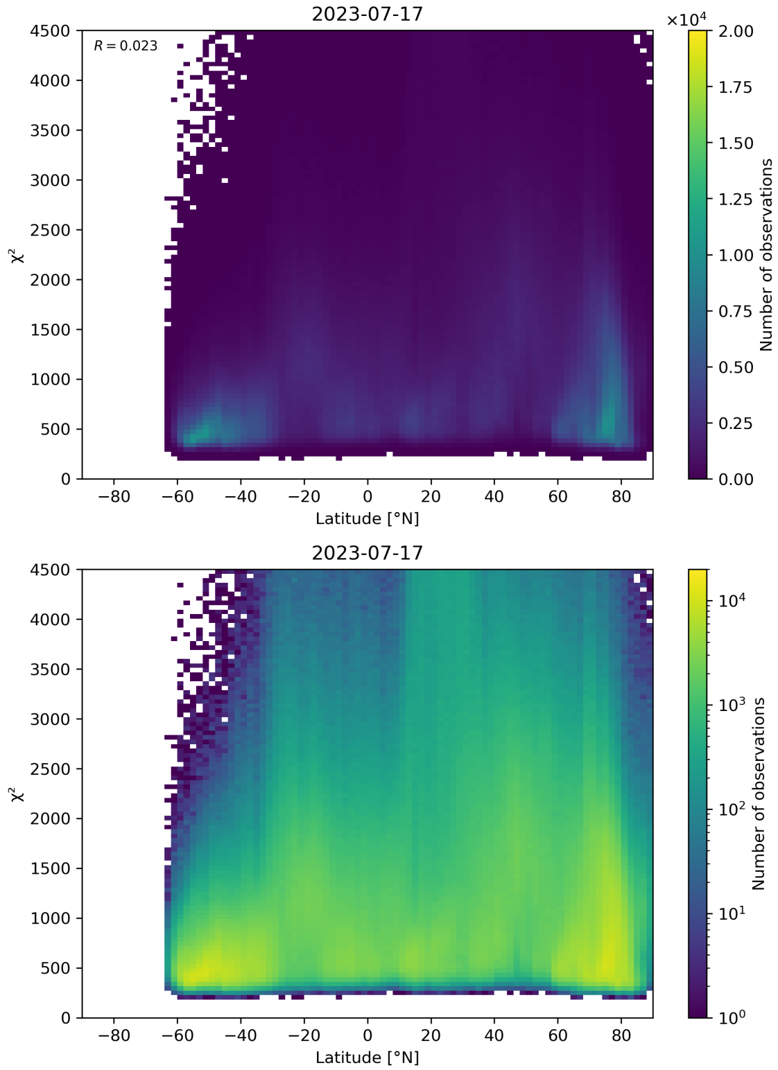
Figure 54: Scatter density plot of “Latitude” against “ \chi^2 ” for 2023-07-16 to 2023-07-18.
