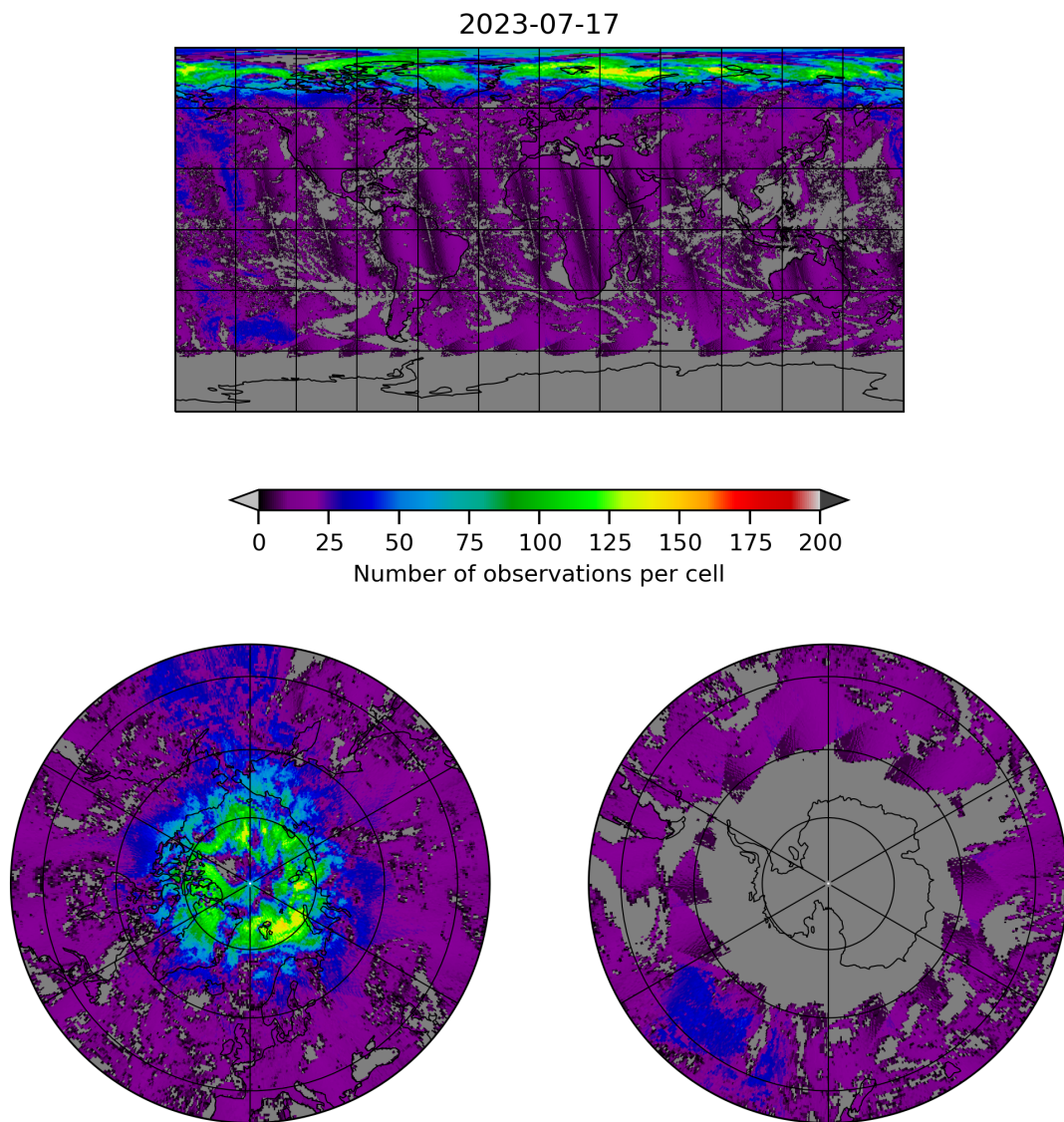
Figure 8: Map of the number of observations for 2023-07-16 to 2023-07-18
