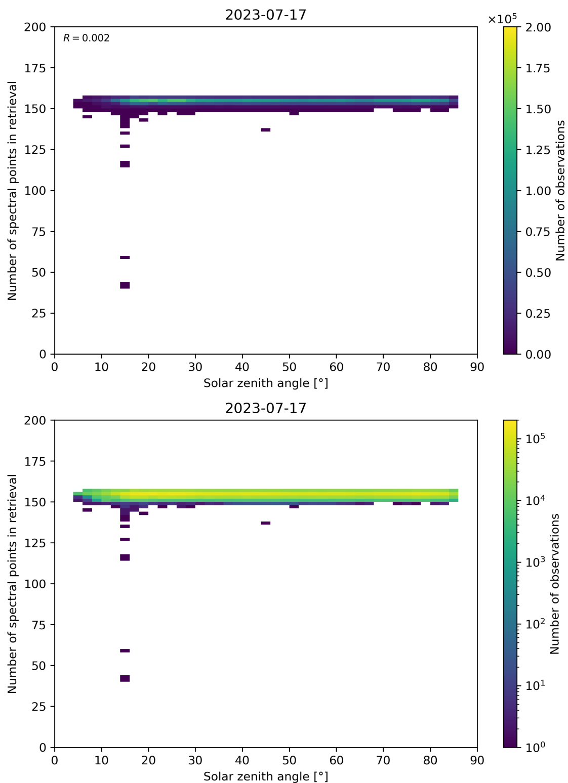
Figure 68: Scatter density plot of “Solar zenith angle” against “Number of spectral points in retrieval” for 2023-07-16 to 2023-07-18.
