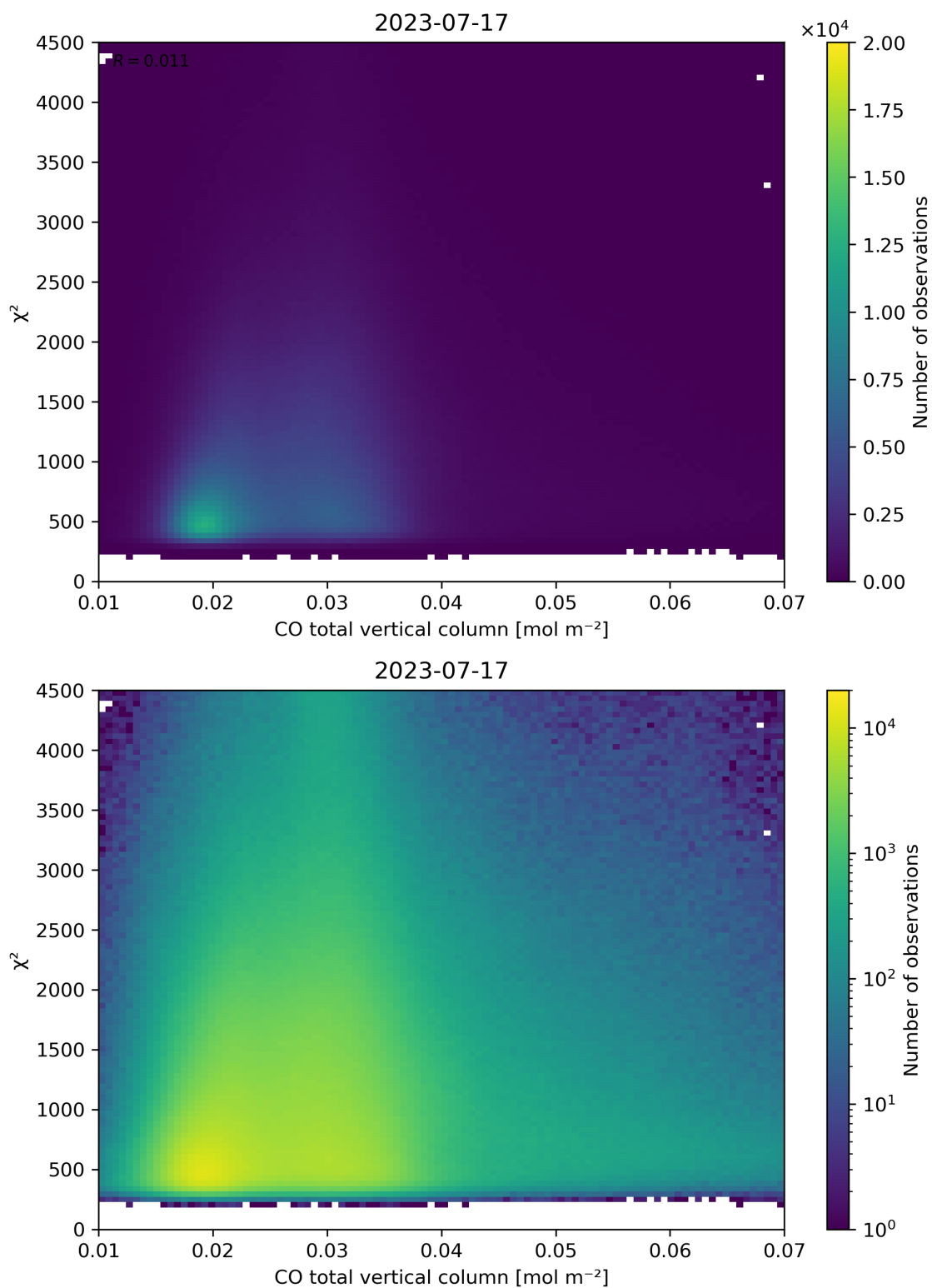
Figure 35: Scatter density plot of “CO total vertical column” against “ \chi^2 ” for 2023-07-16 to 2023-07-18.
