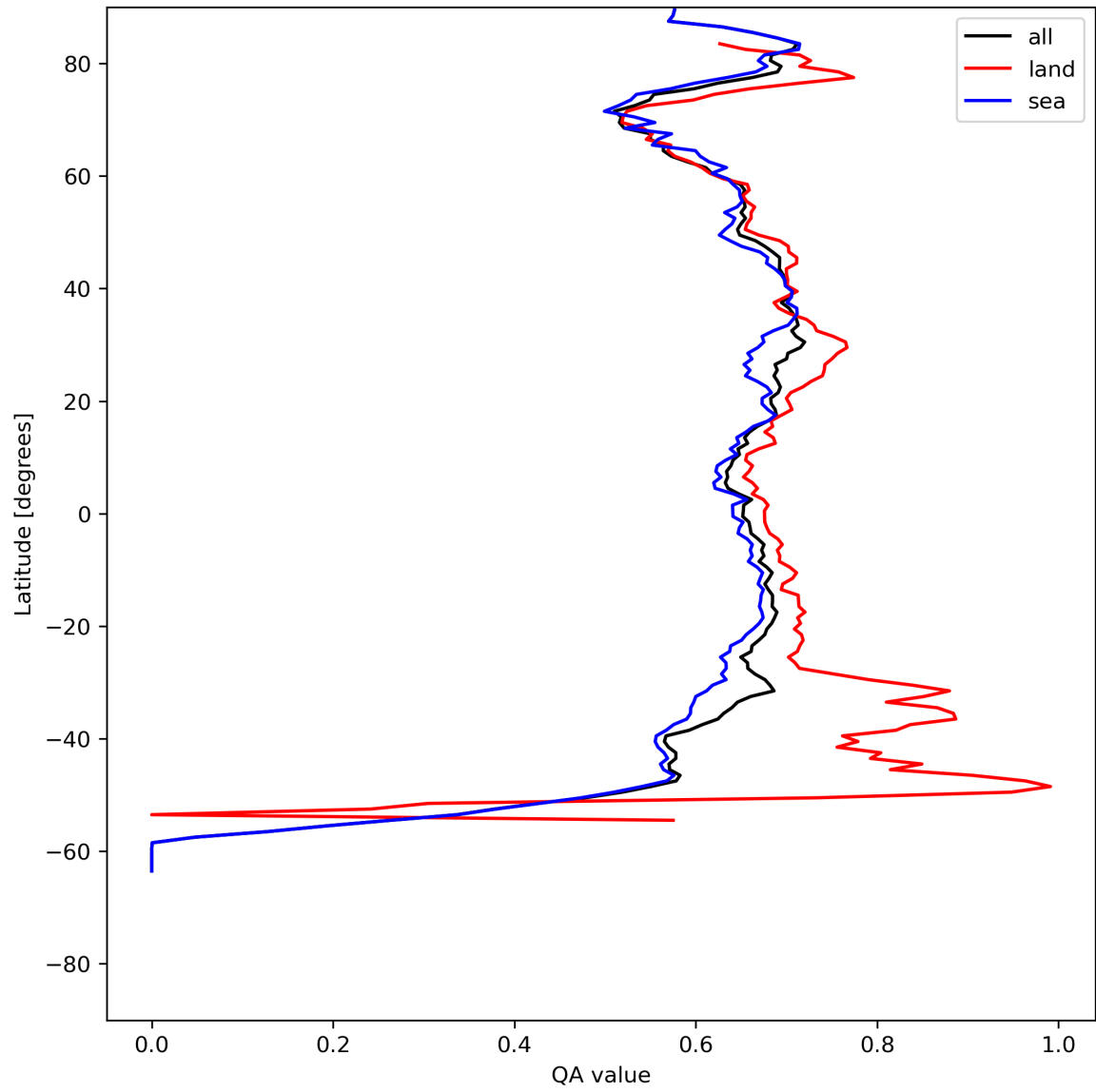
Figure 9: Zonal average of “QA value” for 2023-07-16 to 2023-07-18.
