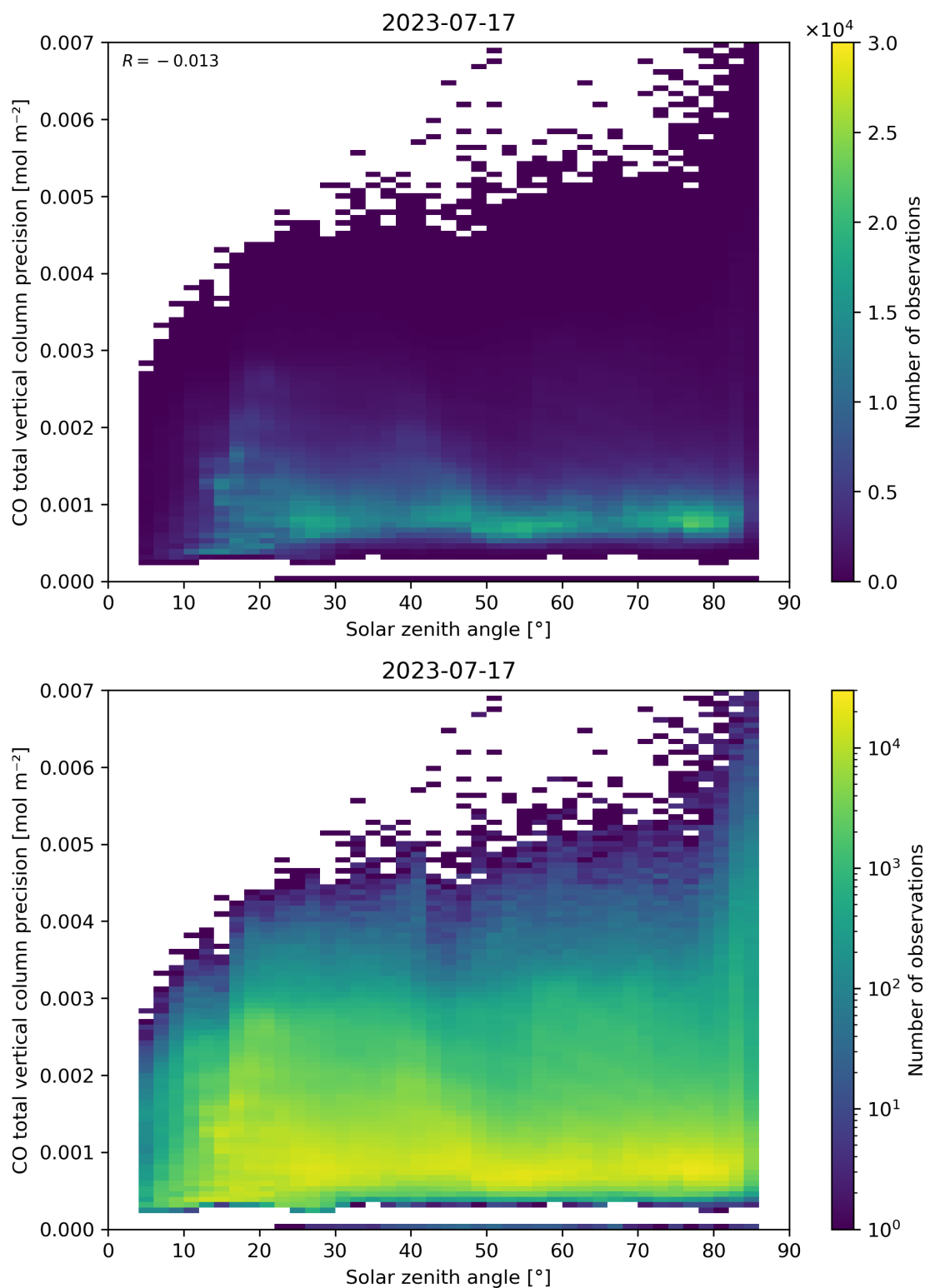
Figure 63: Scatter density plot of “Solar zenith angle” against “CO total vertical column precision” for 2023-07-16 to 2023-07-18.
