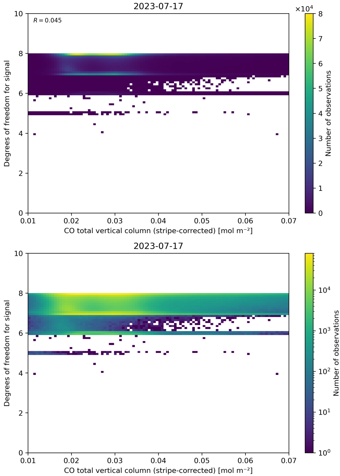
Figure 38: Scatter density plot of “CO total vertical column (stripe-corrected)” against “Degrees of freedom for signal” for 2023-07-16 to 2023-07-18.
