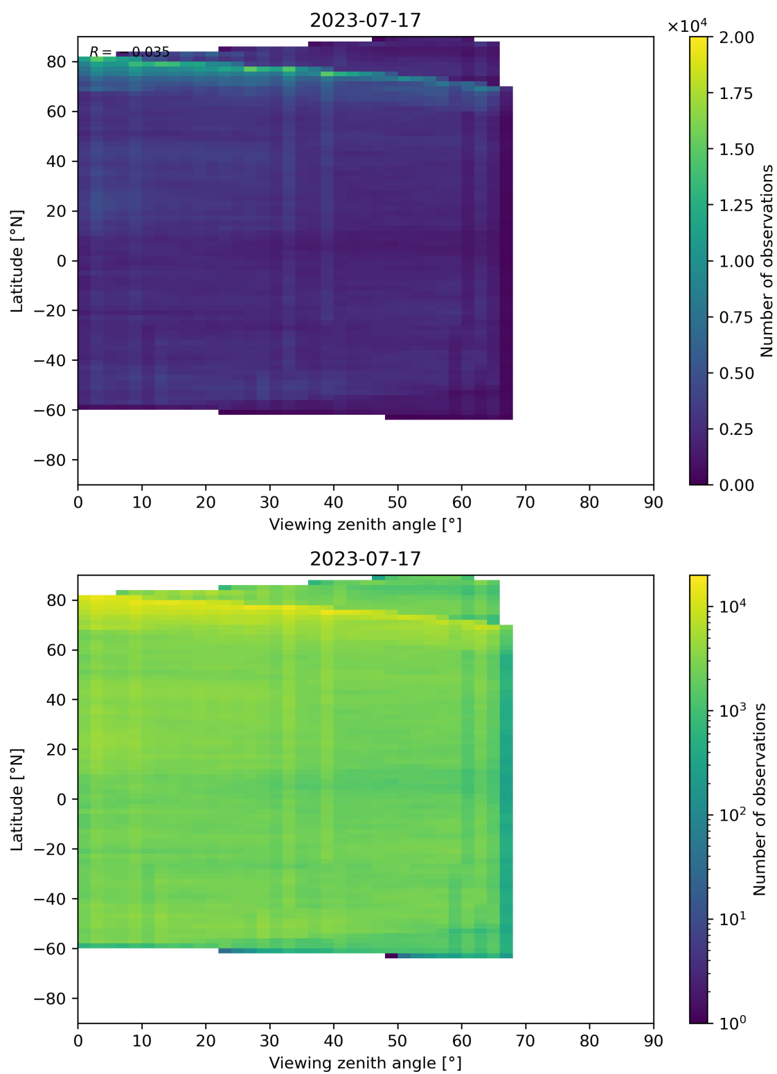
Figure 74: Scatter density plot of “Viewing zenith angle” against “Latitude” for 2023-07-16 to 2023-07-18.
