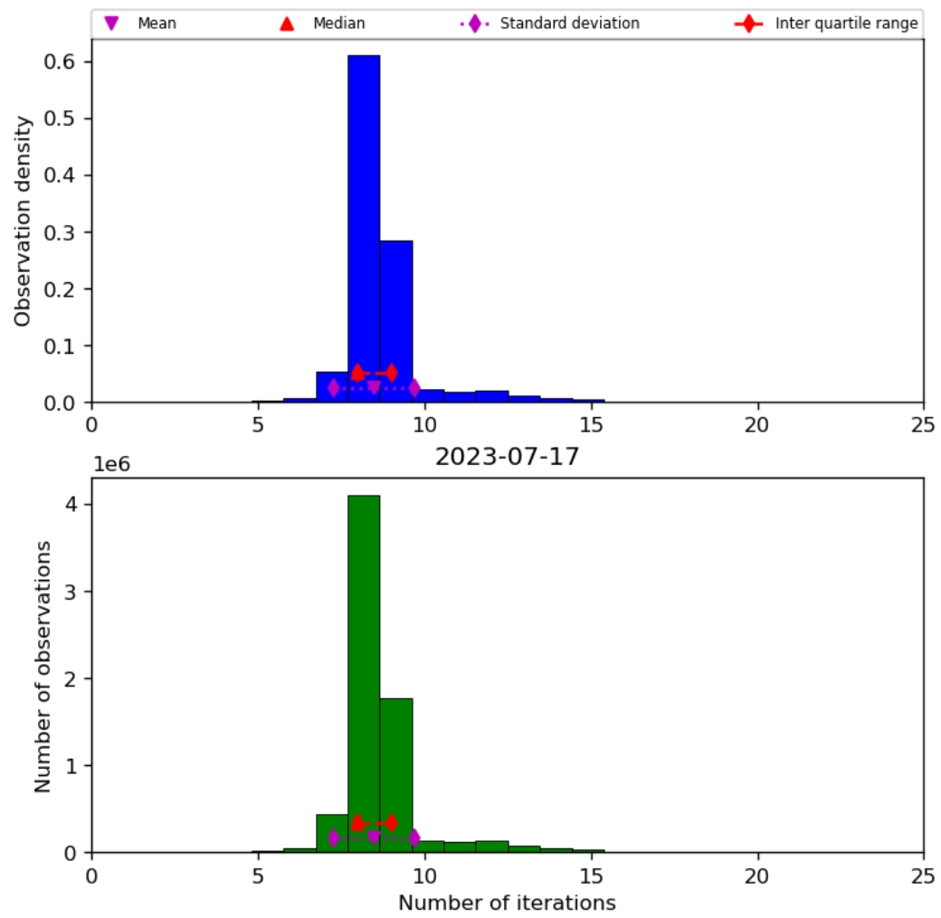
Figure 24: Histogram of “Number of iterations” for 2023-07-16 to 2023-07-18
