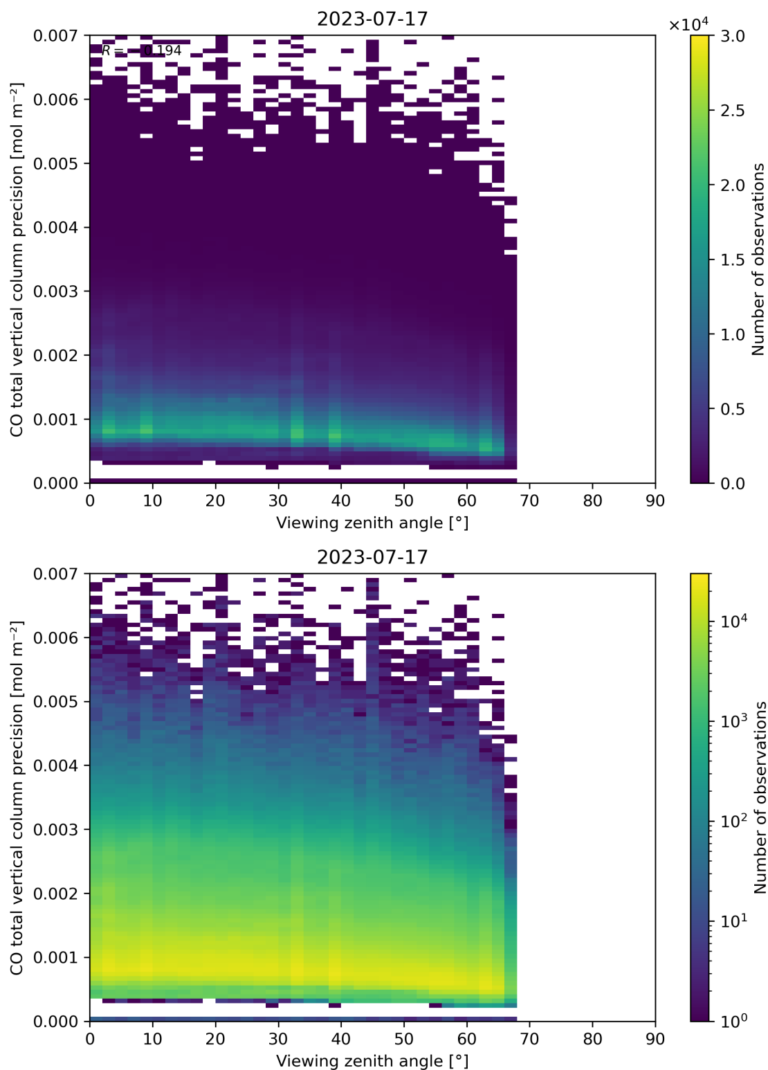
Figure 71: Scatter density plot of “Viewing zenith angle” against “CO total vertical column precision” for 2023-07-16 to 2023-07-18.
