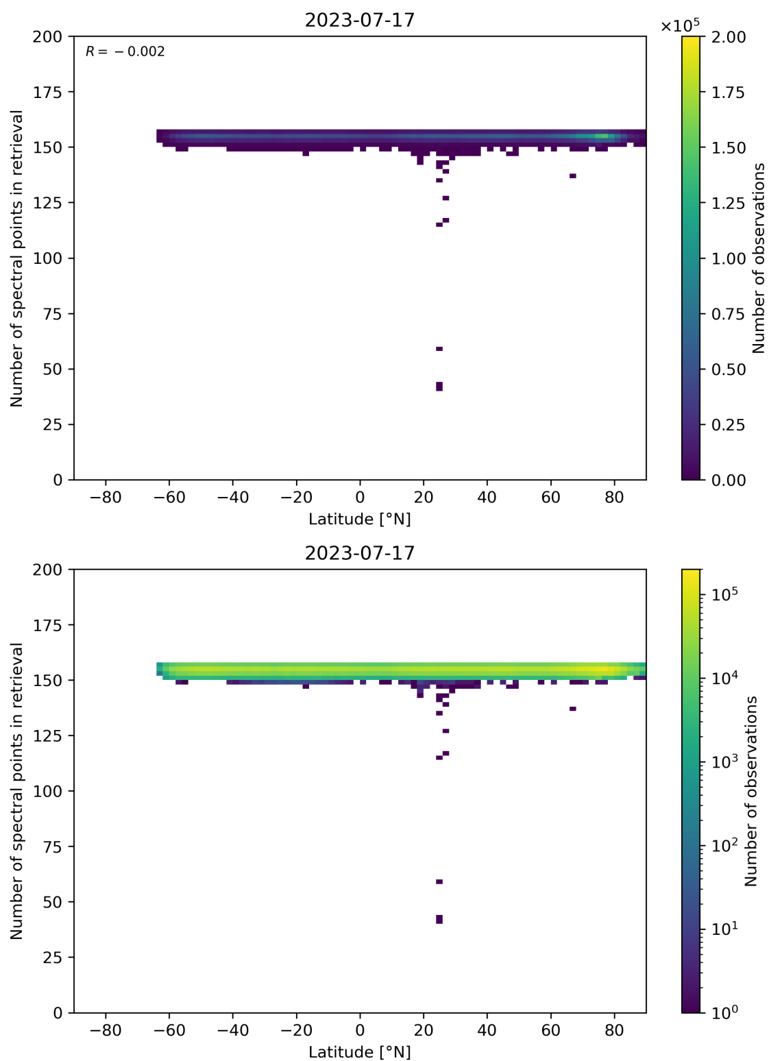
Figure 57: Scatter density plot of “Latitude” against “Number of spectral points in retrieval” for 2023-07-16 to 2023-07-18.
