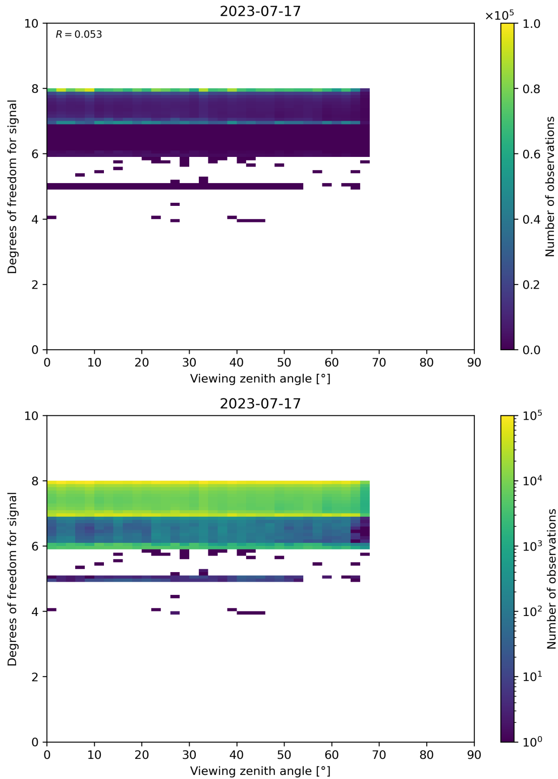
Figure 73: Scatter density plot of “Viewing zenith angle” against “Degrees of freedom for signal” for 2023-07-16 to 2023-07-18.
