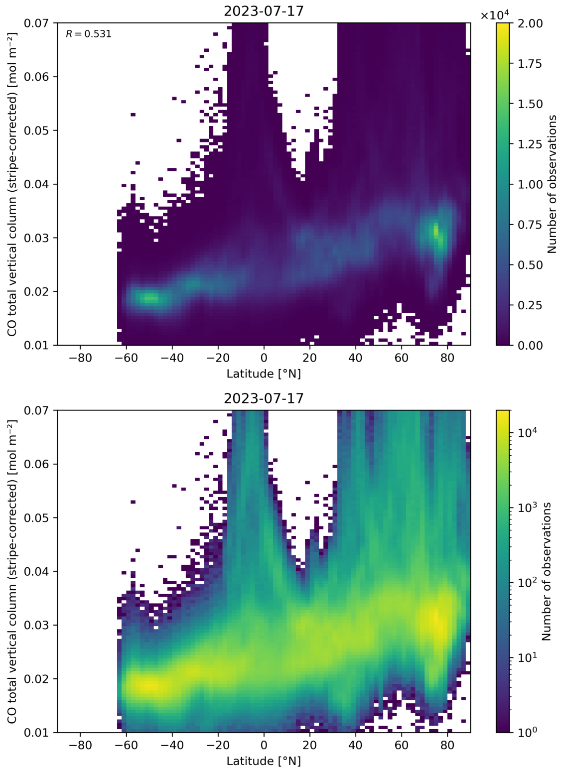
Figure 52: Scatter density plot of “Latitude” against “CO total vertical column (stripe-corrected)” for 2023-07-16 to 2023-07-18.
