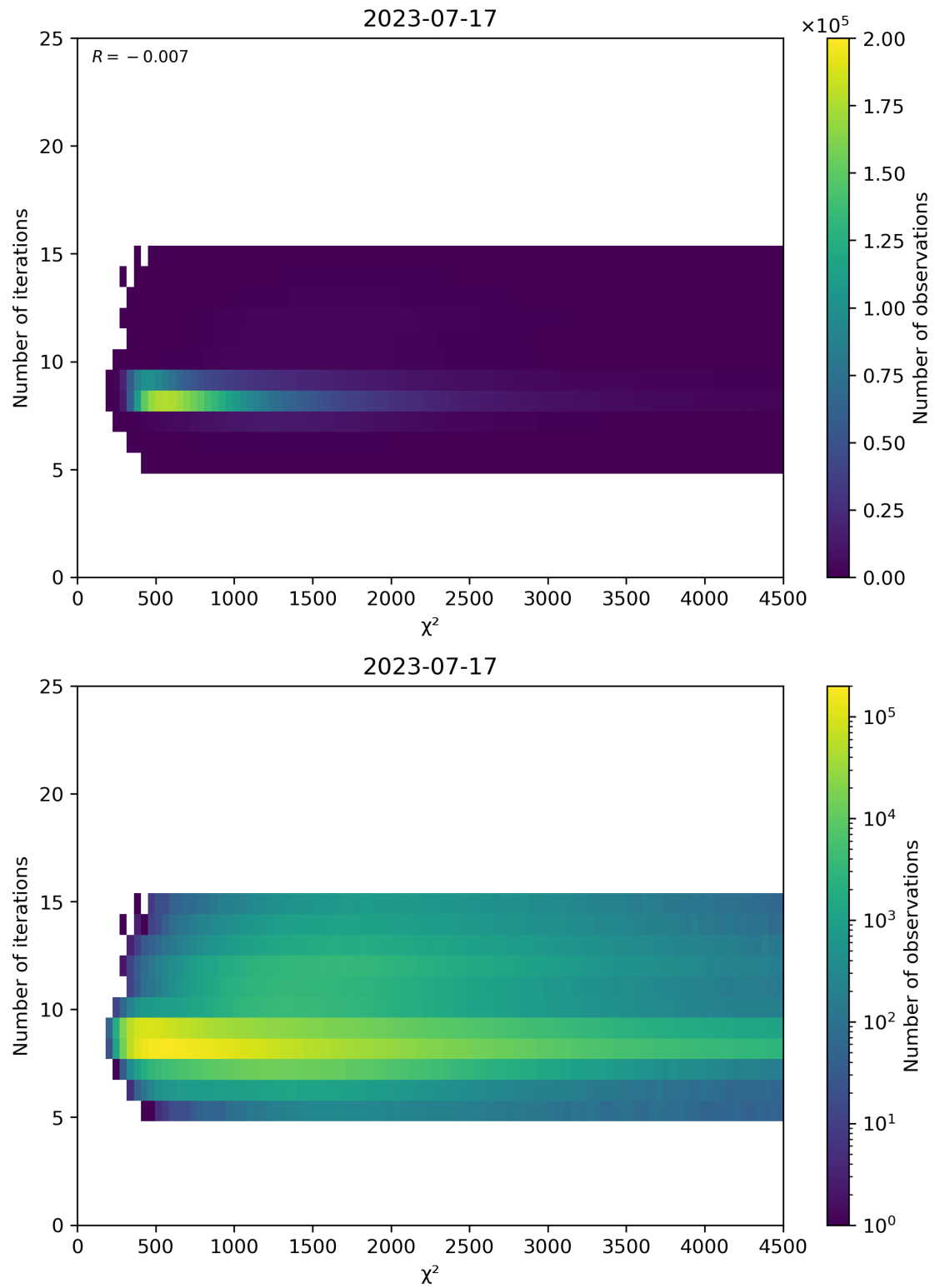
Figure 49: Scatter density plot of “ \chi^2 ” against “Number of iterations” for 2023-07-16 to 2023-07-18.
