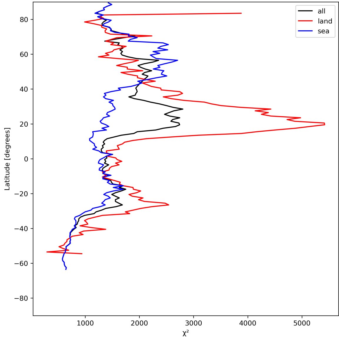
Figure 14: Zonal average of “ \chi^2 ” for 2023-07-16 to 2023-07-18.
