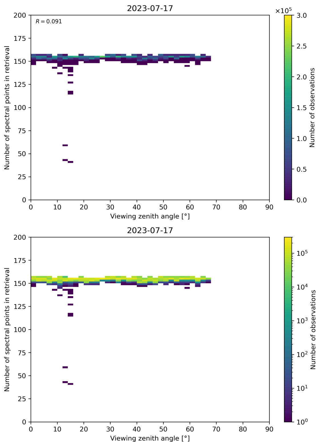
Figure 76: Scatter density plot of “Viewing zenith angle” against “Number of spectral points in retrieval” for 2023-07-16 to 2023-07-18.
