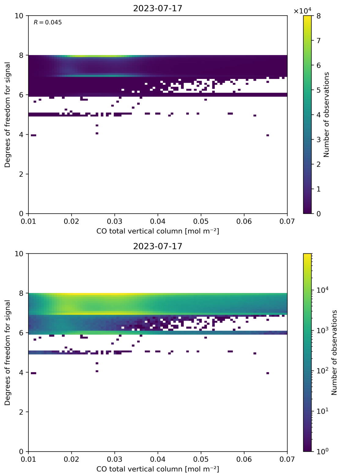
Figure 41: Scatter density plot of “CO total vertical column” against “Degrees of freedom for signal” for 2023-07-16 to 2023-07-18.
