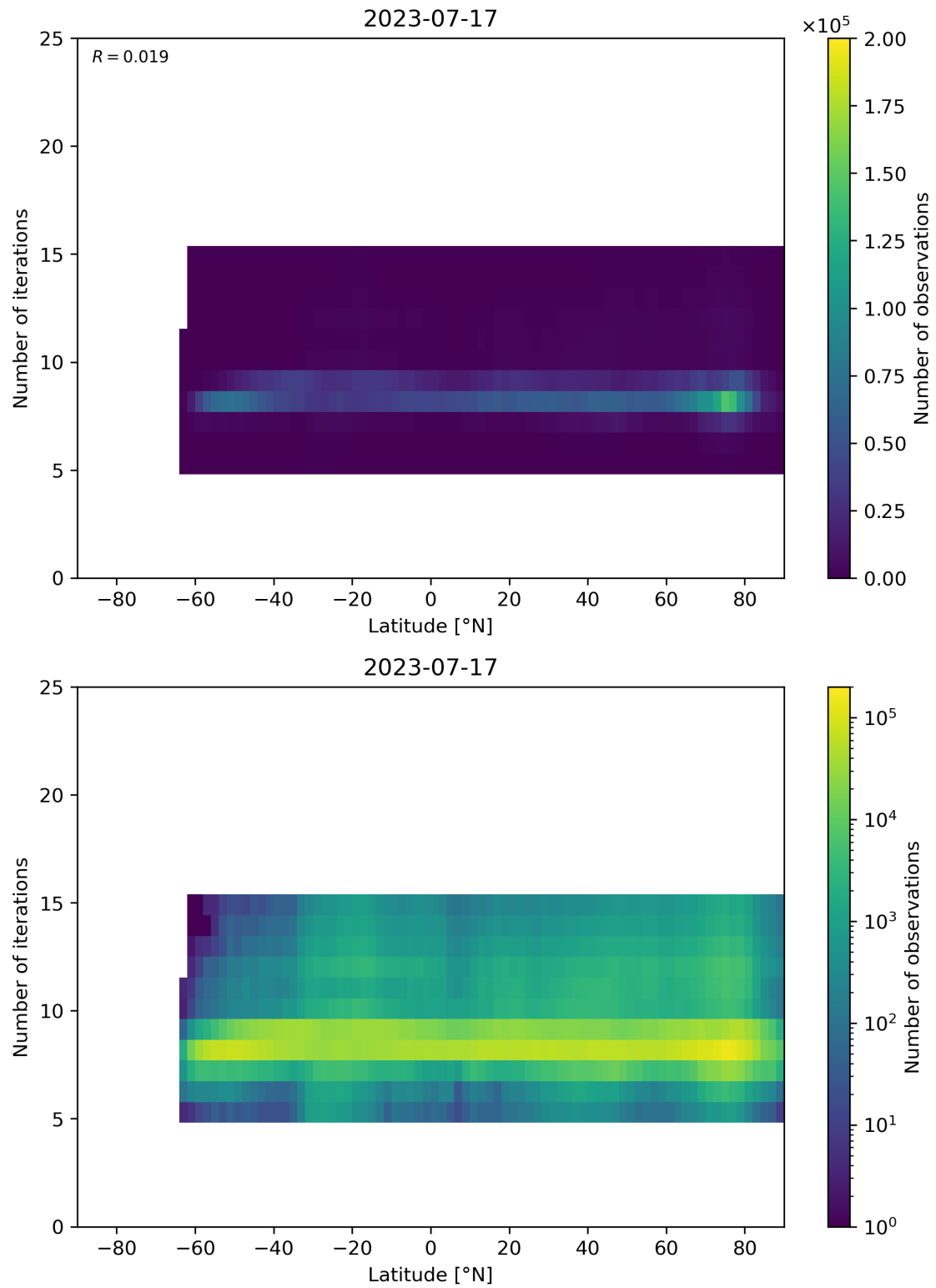
Figure 56: Scatter density plot of “Latitude” against “Number of iterations” for 2023-07-16 to 2023-07-18.
