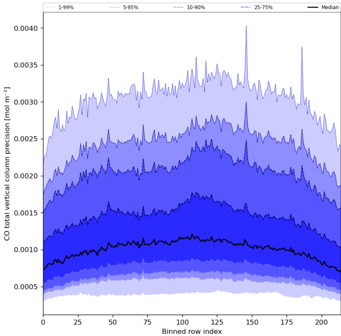
Figure 28: Along track statistics of “CO total vertical column precision” for 2023-07-16 to 2023-07-18
