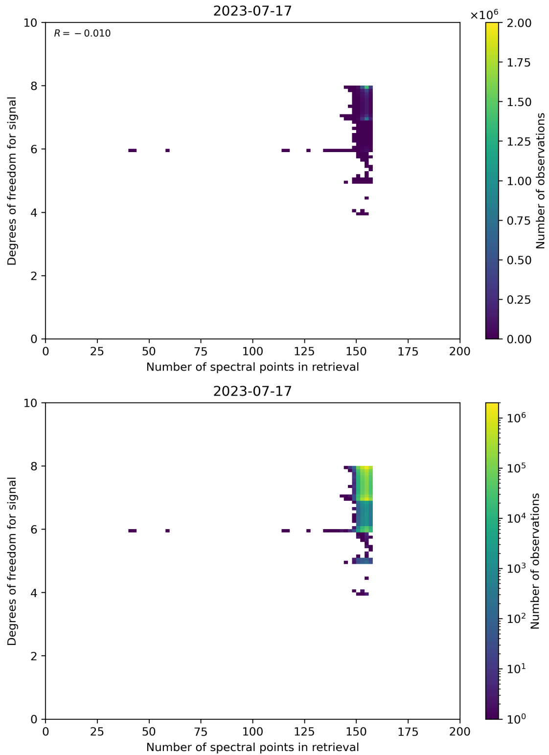
Figure 59: Scatter density plot of “Number of spectral points in retrieval” against “Degrees of freedom for signal” for 2023-07-16 to 2023-07-18.
