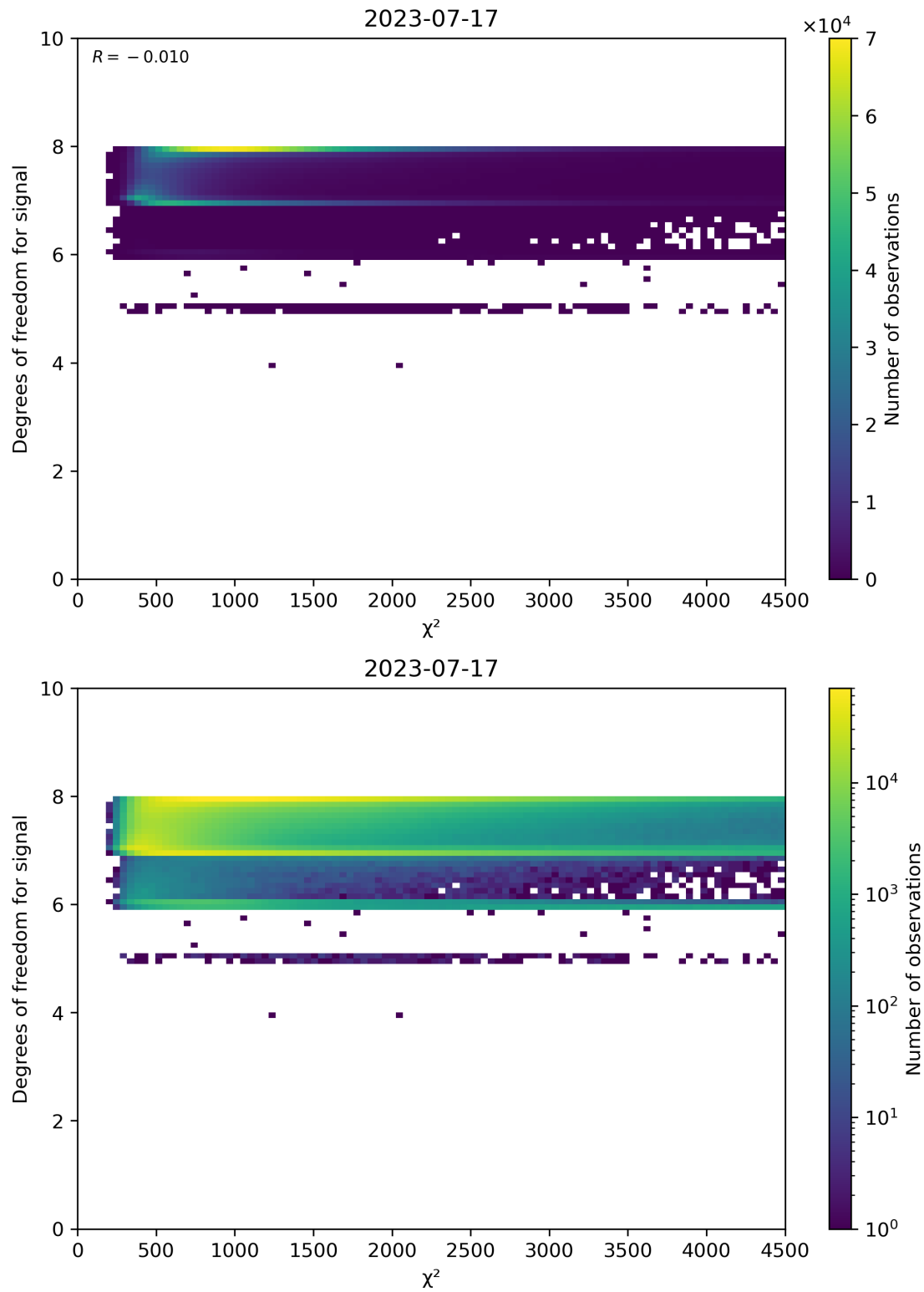
Figure 48: Scatter density plot of “ \chi^2 ” against “Degrees of freedom for signal” for 2023-07-16 to 2023-07-18.
