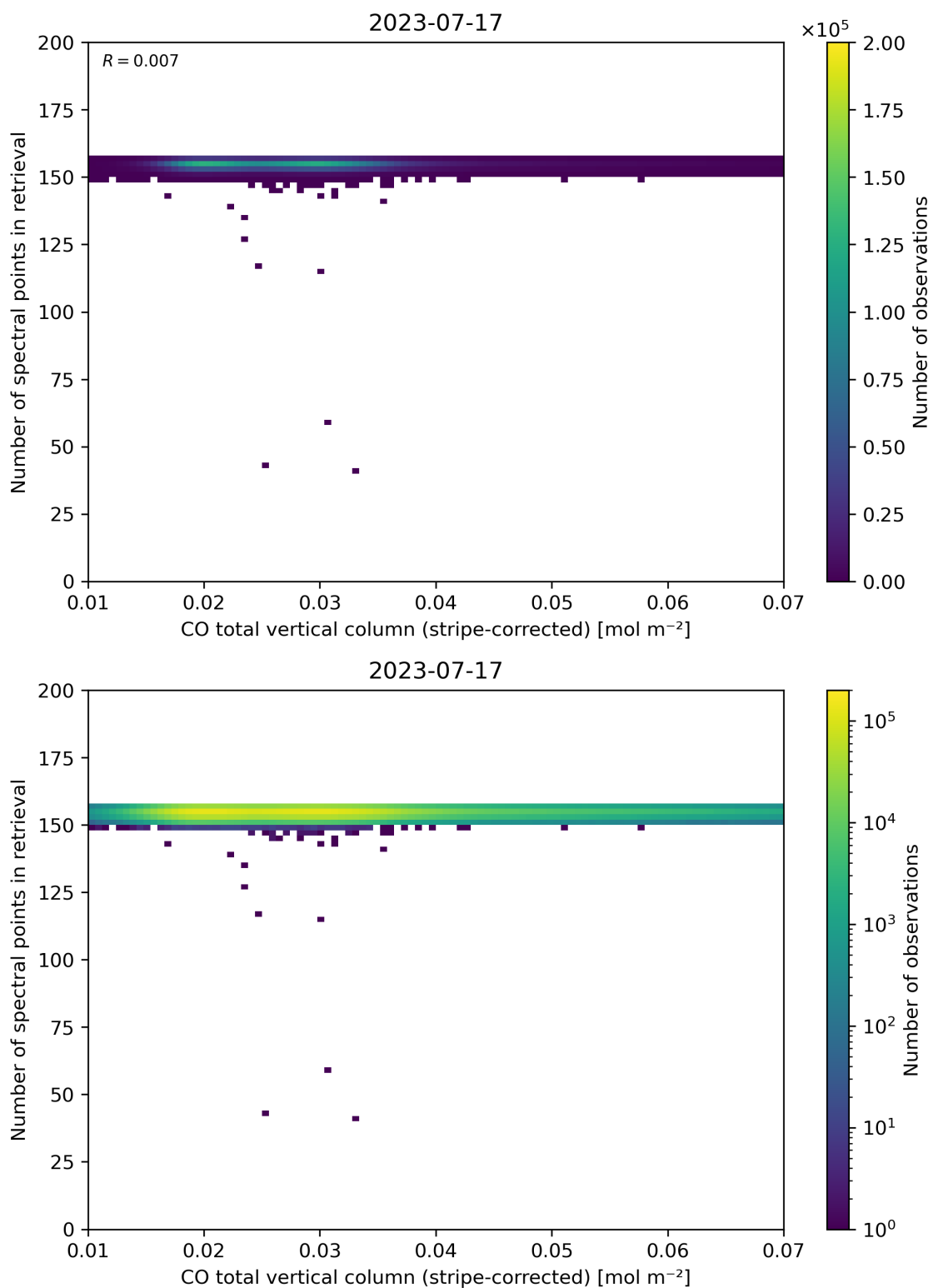
Figure 40: Scatter density plot of “CO total vertical column (stripe-corrected)” against “Number of spectral points in retrieval” for 2023-07-16 to 2023-07-18.
