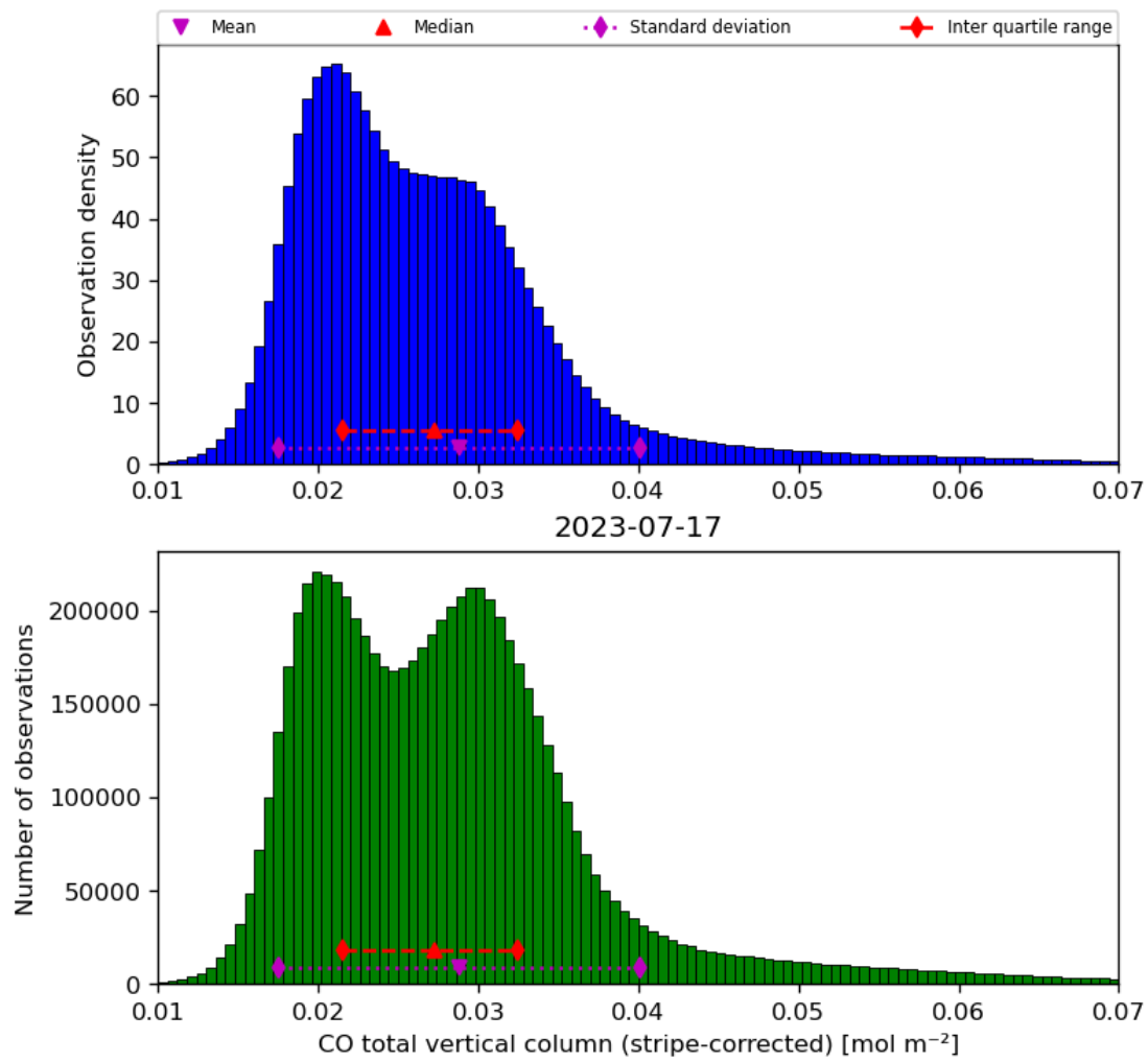
Figure 19: Histogram of “CO total vertical column (stripe-corrected)” for 2023-07-16 to 2023-07-18
