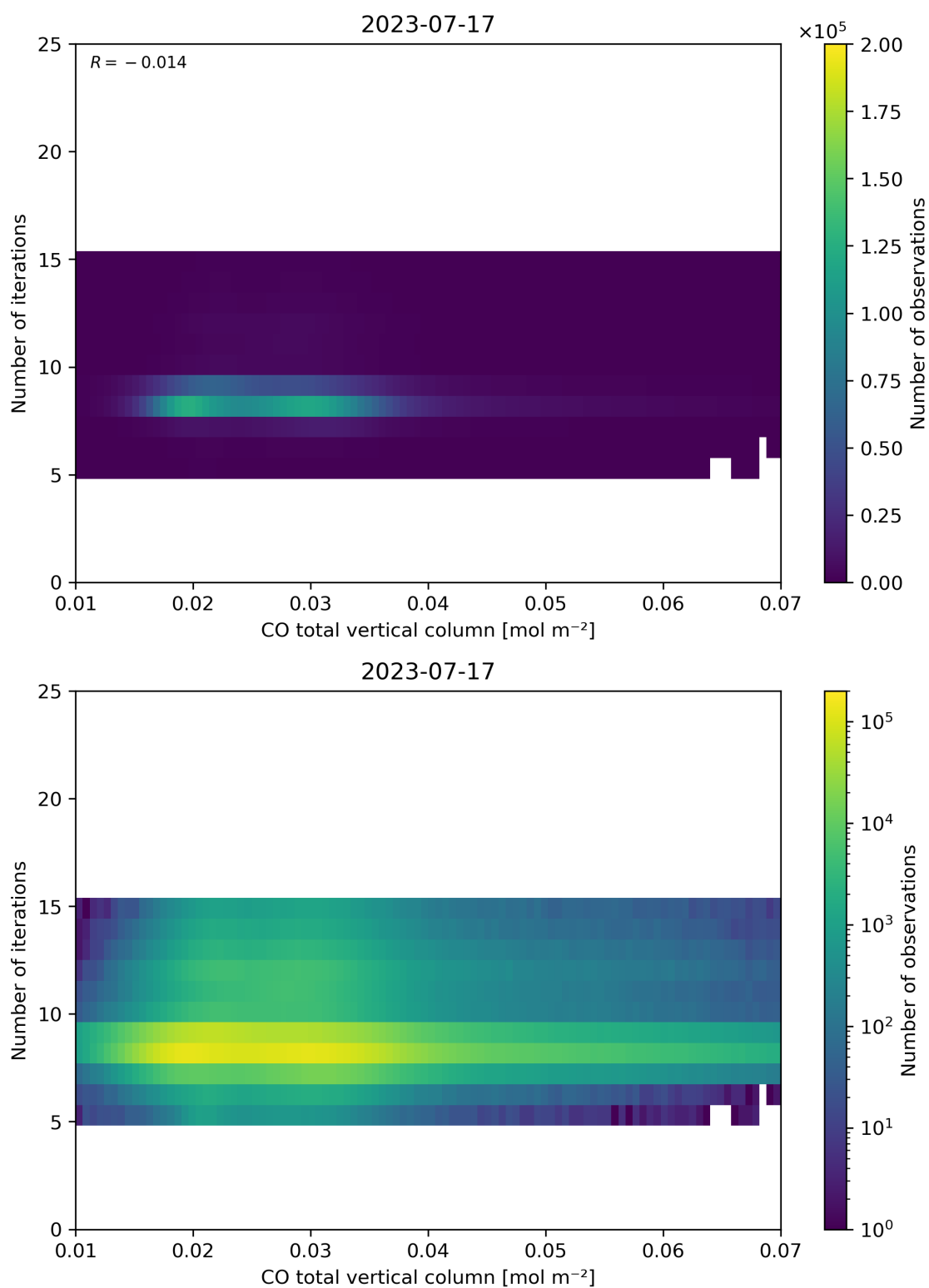
Figure 42: Scatter density plot of “CO total vertical column” against “Number of iterations” for 2023-07-16 to 2023-07-18.
