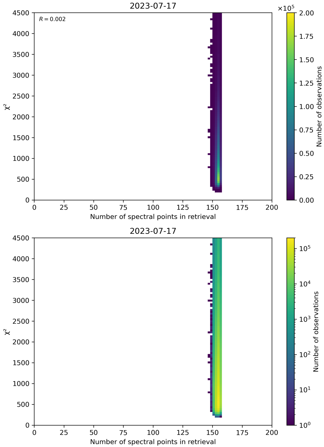
Figure 58: Scatter density plot of “Number of spectral points in retrieval” against “ \chi^2 ” for 2023-07-16 to 2023-07-18.
