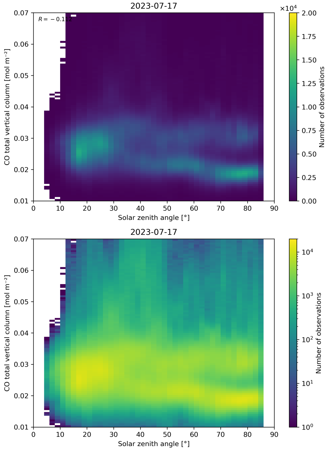
Figure 61: Scatter density plot of “Solar zenith angle” against “CO total vertical column” for 2023-07-16 to 2023-07-18.
