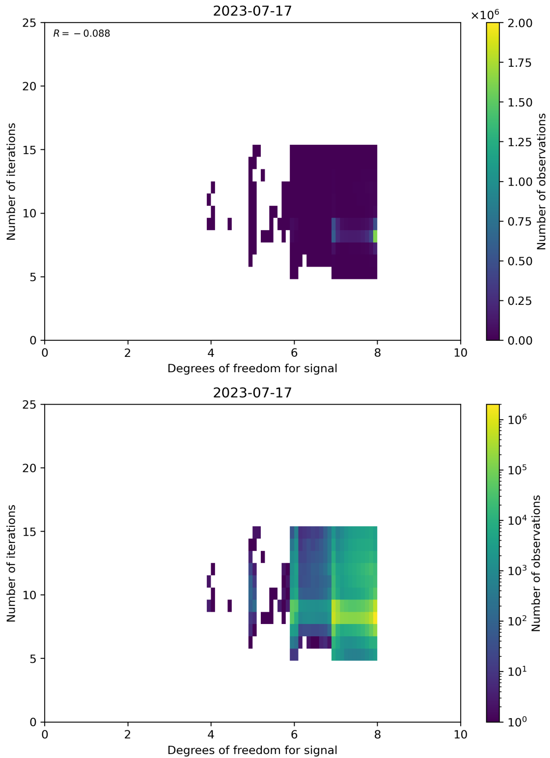
Figure 50: Scatter density plot of “Degrees of freedom for signal” against “Number of iterations” for 2023-07-16 to 2023-07-18.
