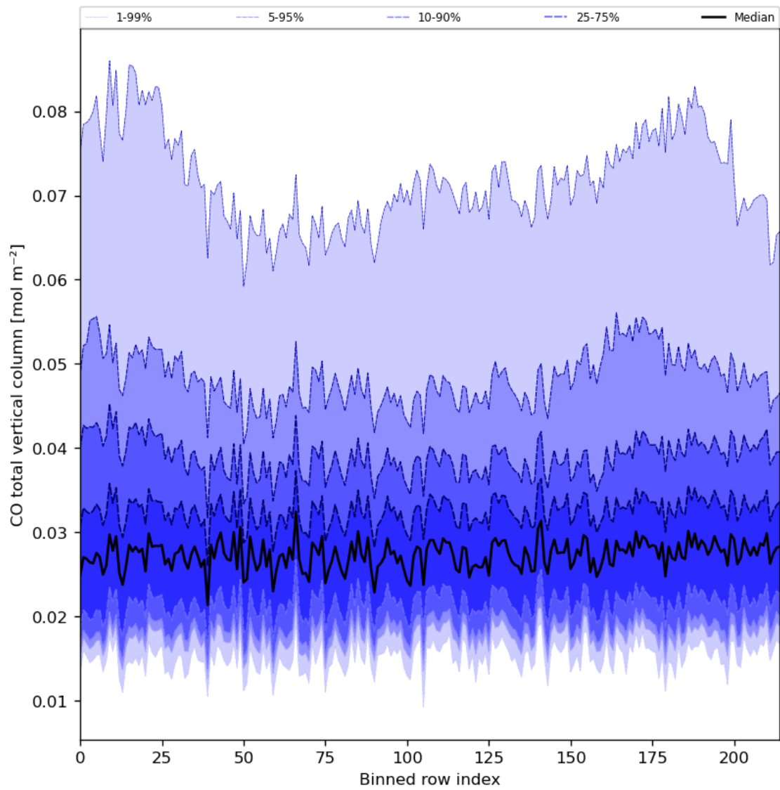
Figure 26: Along track statistics of “CO total vertical column” for 2023-07-16 to 2023-07-18
