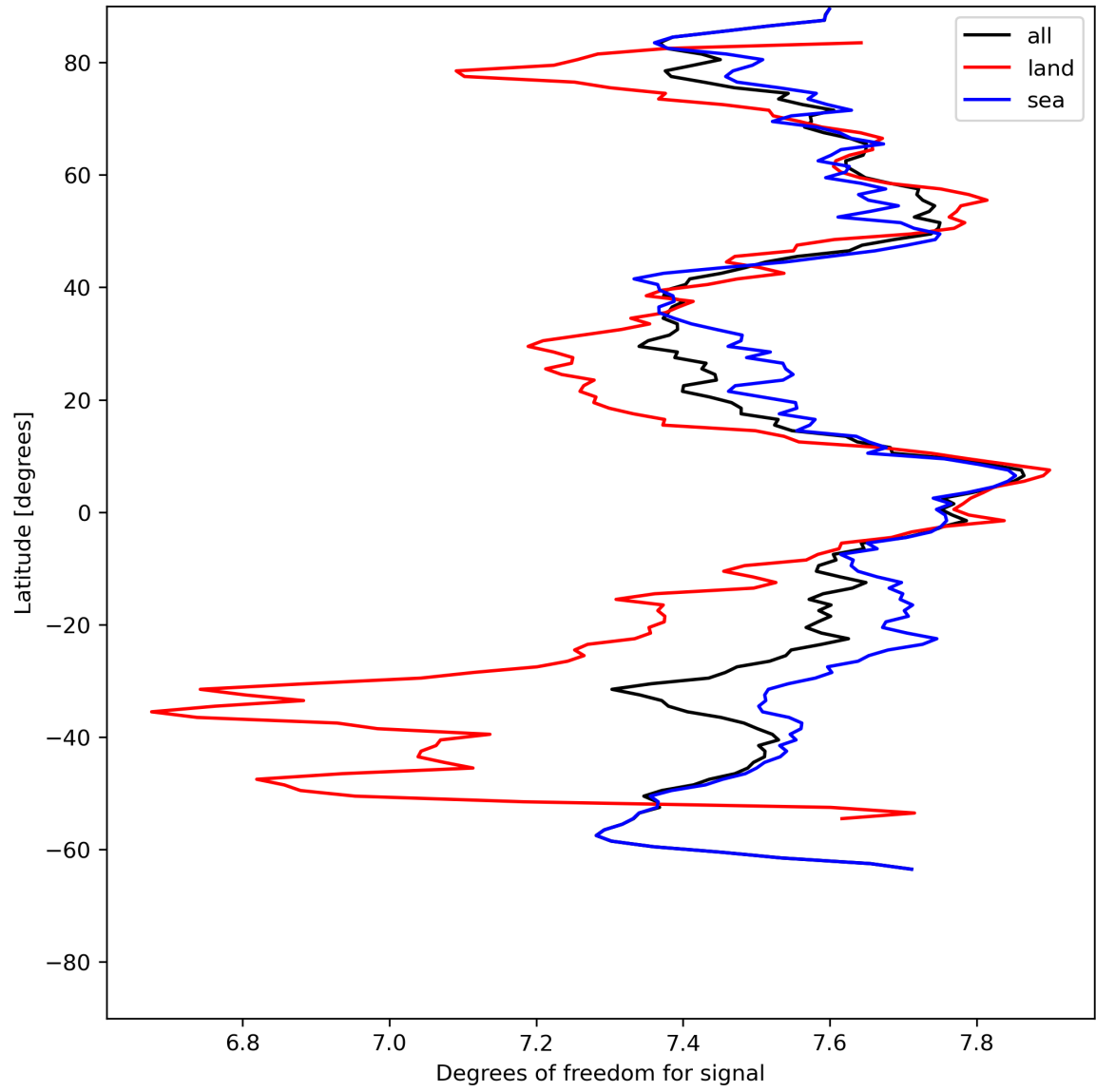
Figure 15: Zonal average of “Degrees of freedom for signal” for 2023-07-16 to 2023-07-18.
