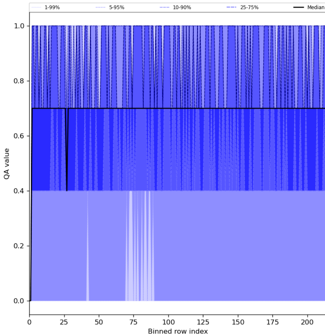
Figure 25: Along track statistics of “QA value” for 2023-07-16 to 2023-07-18
