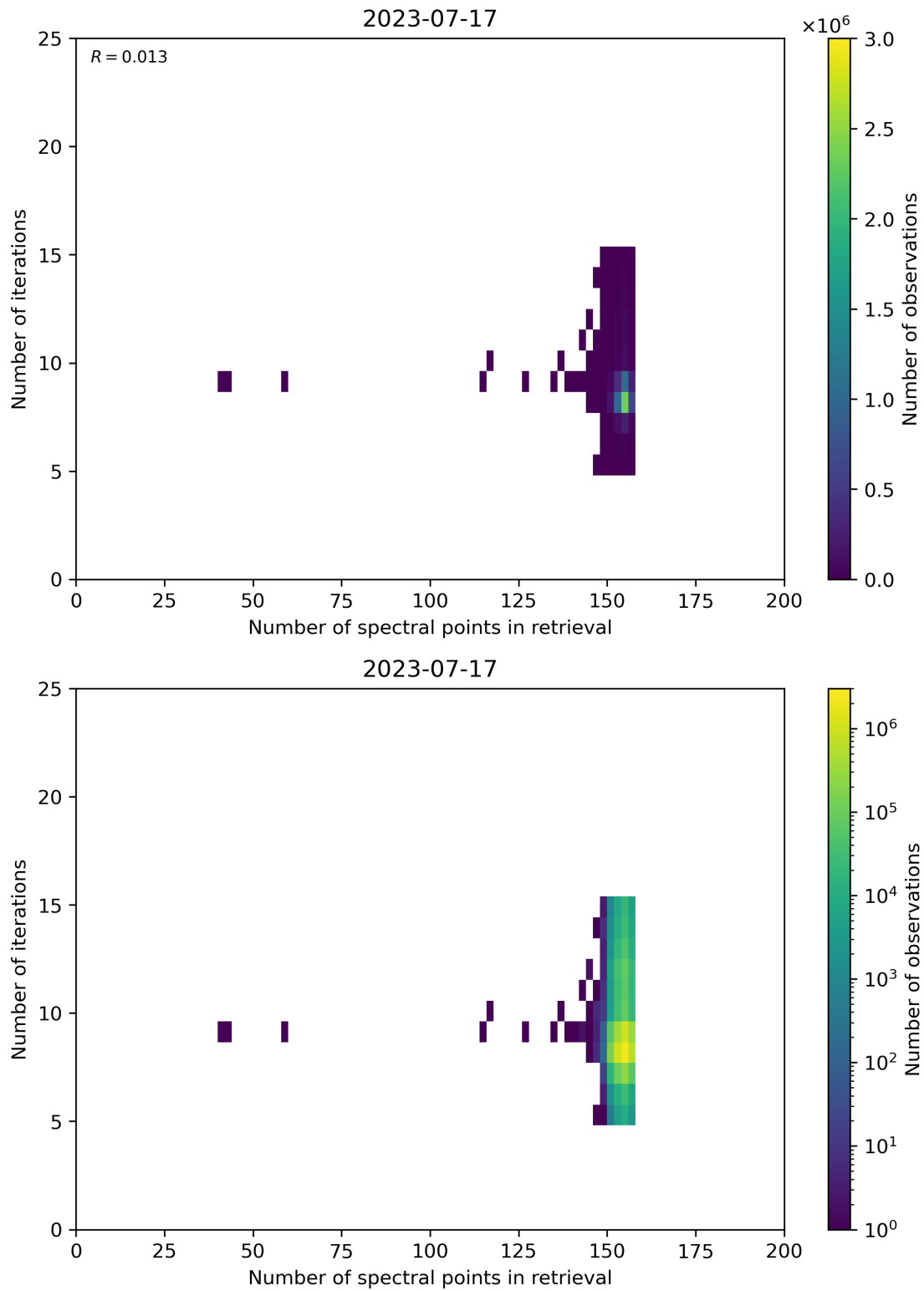
Figure 60: Scatter density plot of “Number of spectral points in retrieval” against “Number of iterations” for 2023-07-16 to 2023-07-18.
