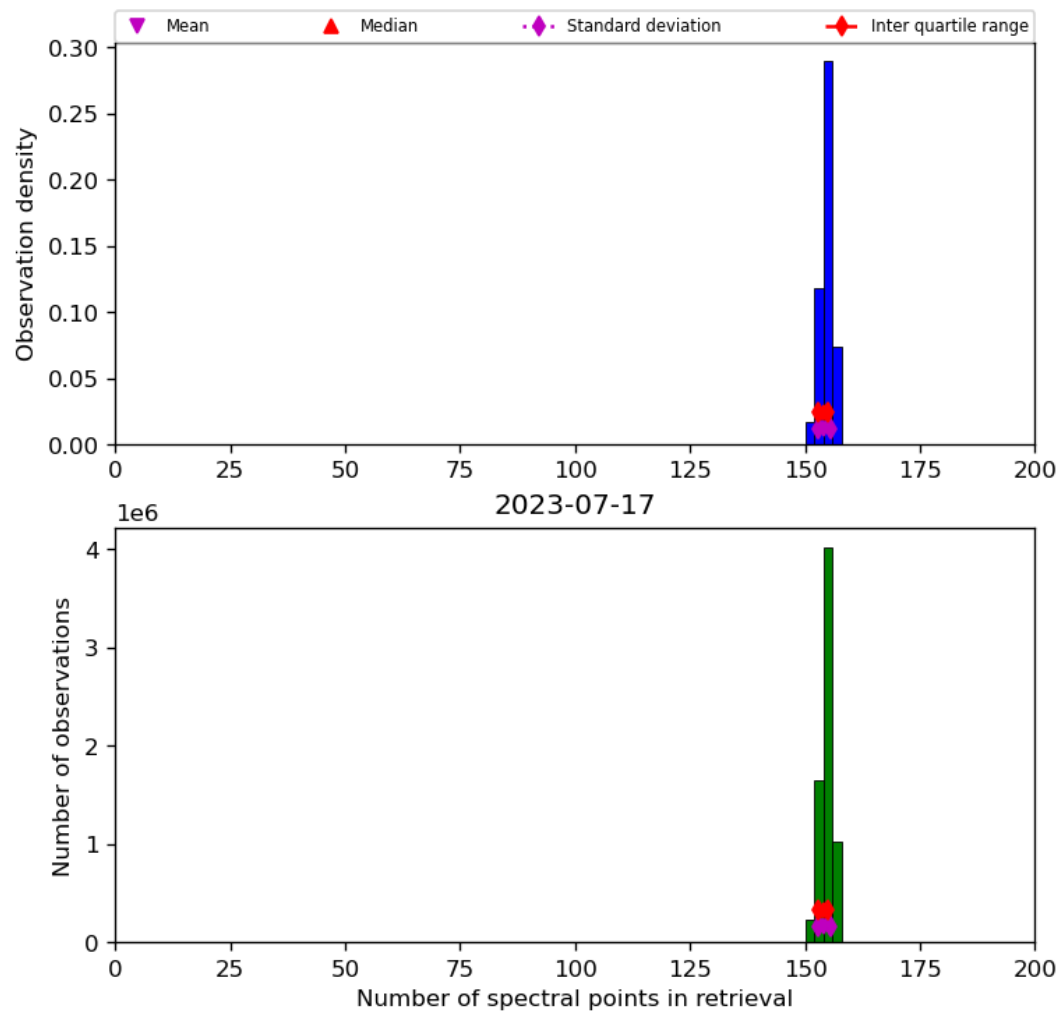
Figure 21: Histogram of “Number of spectral points in retrieval” for 2023-07-16 to 2023-07-18
