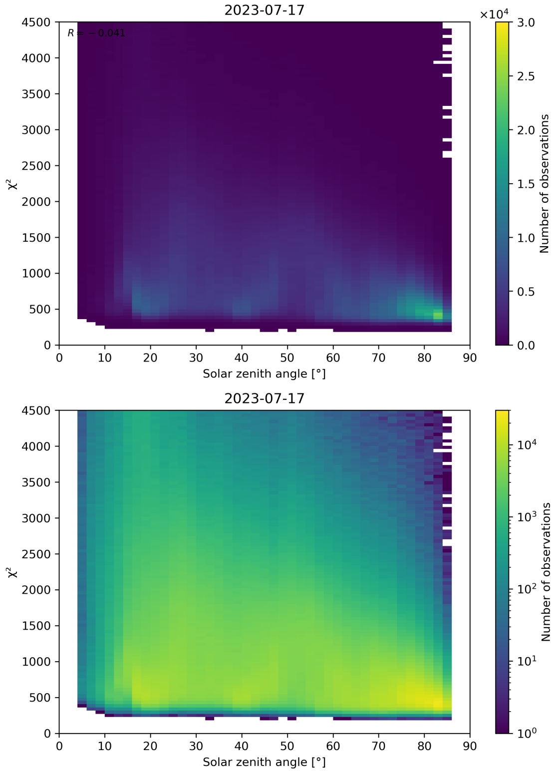
Figure 64: Scatter density plot of “Solar zenith angle” against “ \chi^2 ” for 2023-07-16 to 2023-07-18.
