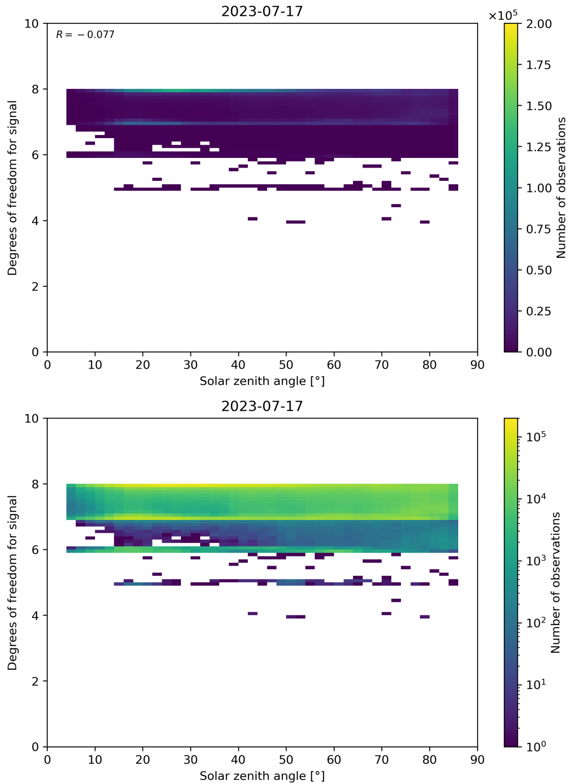
Figure 65: Scatter density plot of “Solar zenith angle” against “Degrees of freedom for signal” for 2023-07-16 to 2023-07-18.
