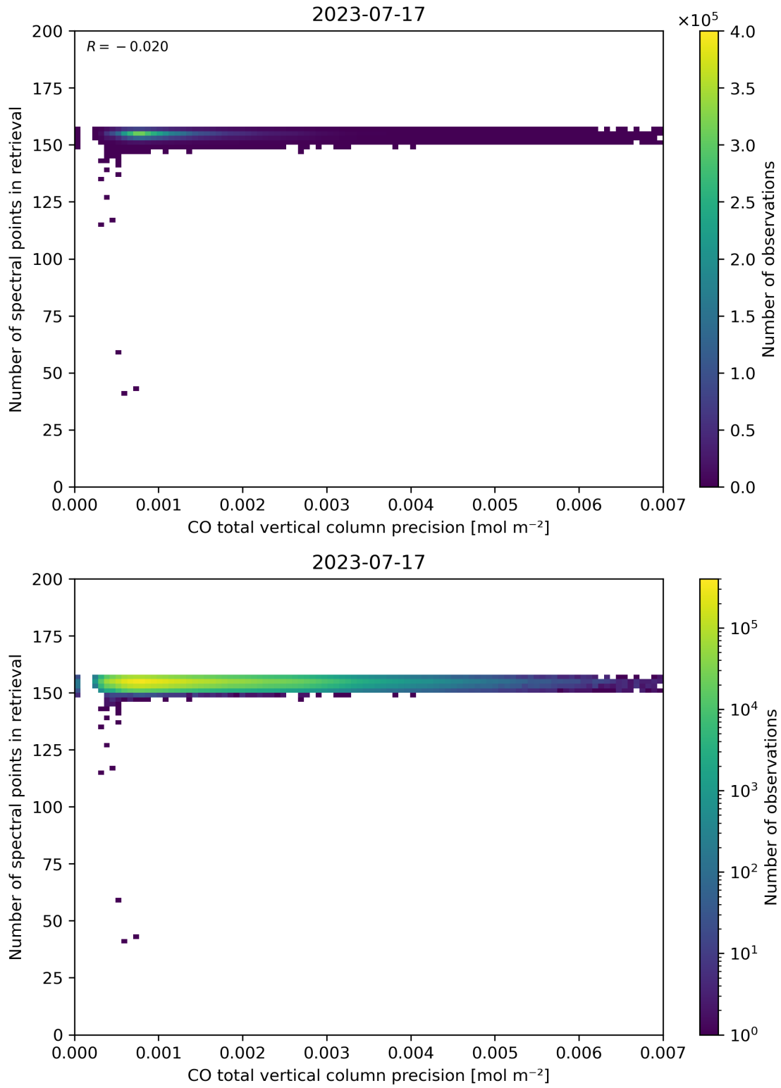
Figure 47: Scatter density plot of “CO total vertical column precision” against “Number of spectral points in retrieval” for 2023-07-16 to 2023-07-18.
