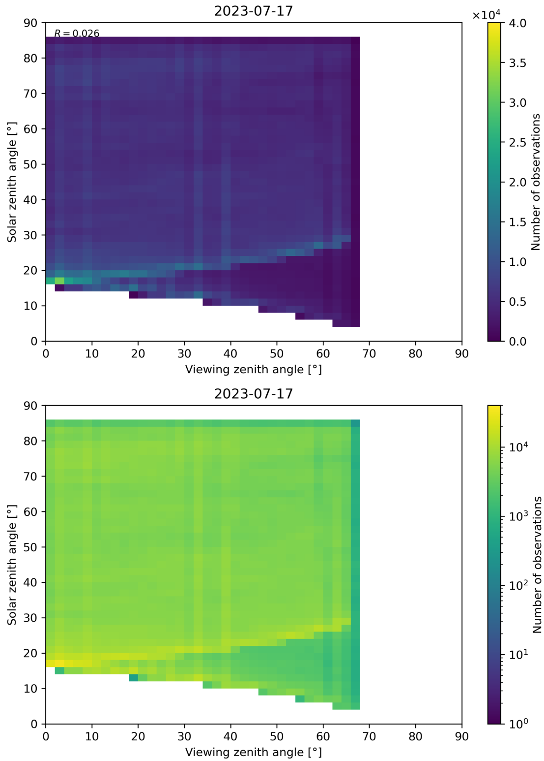
Figure 77: Scatter density plot of “Viewing zenith angle” against “Solar zenith angle” for 2023-07-16 to 2023-07-18.
