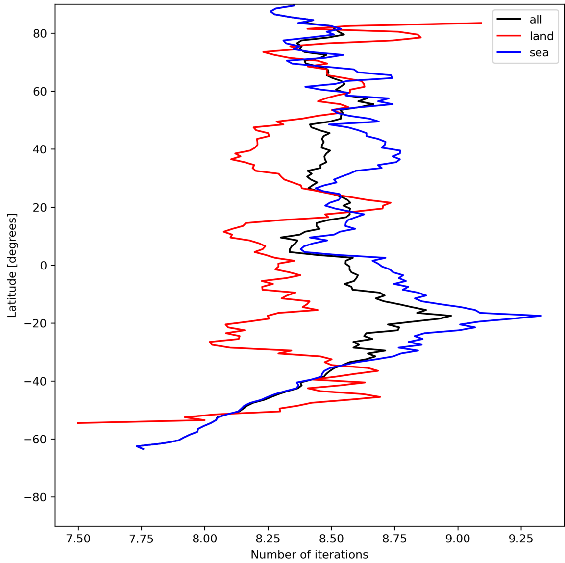
Figure 16: Zonal average of “Number of iterations” for 2023-07-16 to 2023-07-18.
