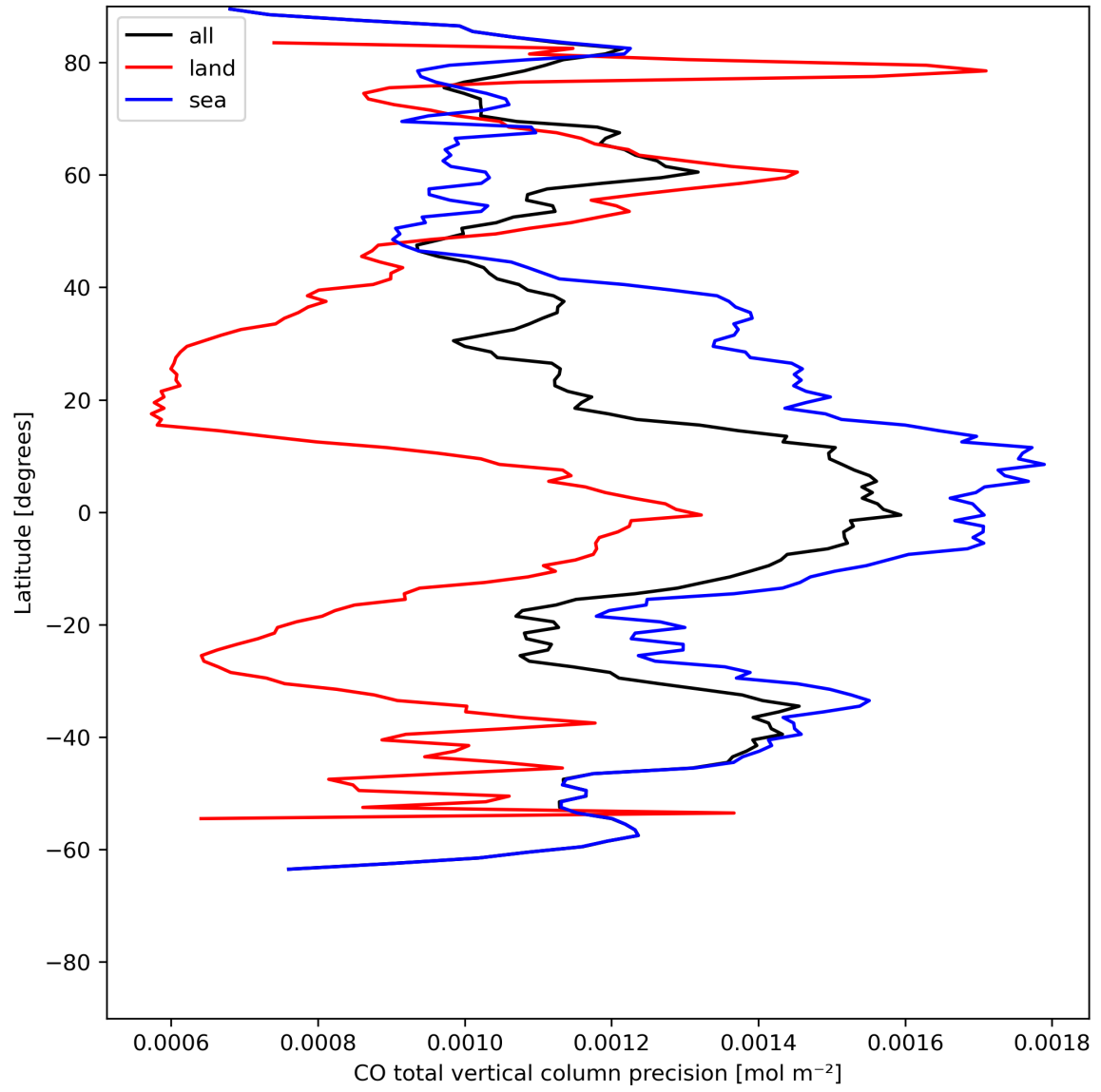
Figure 12: Zonal average of “CO total vertical column precision” for 2023-07-16 to 2023-07-18.
