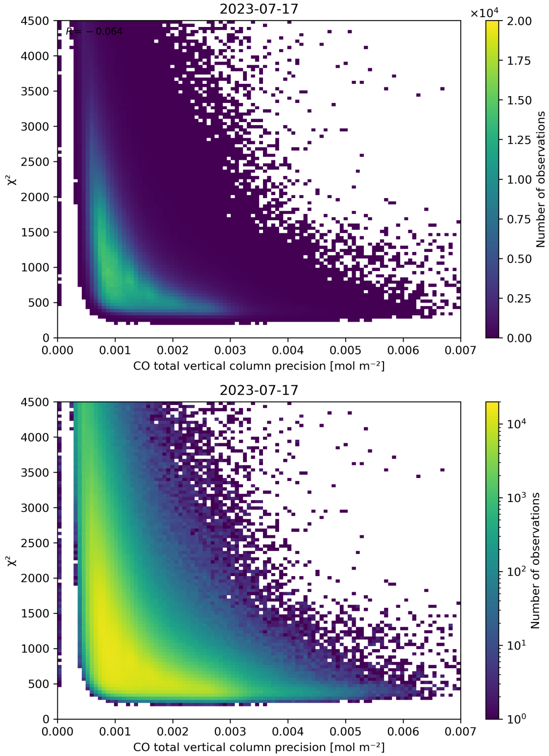
Figure 44: Scatter density plot of “CO total vertical column precision” against “ \chi^2 ” for 2023-07-16 to 2023-07-18.
