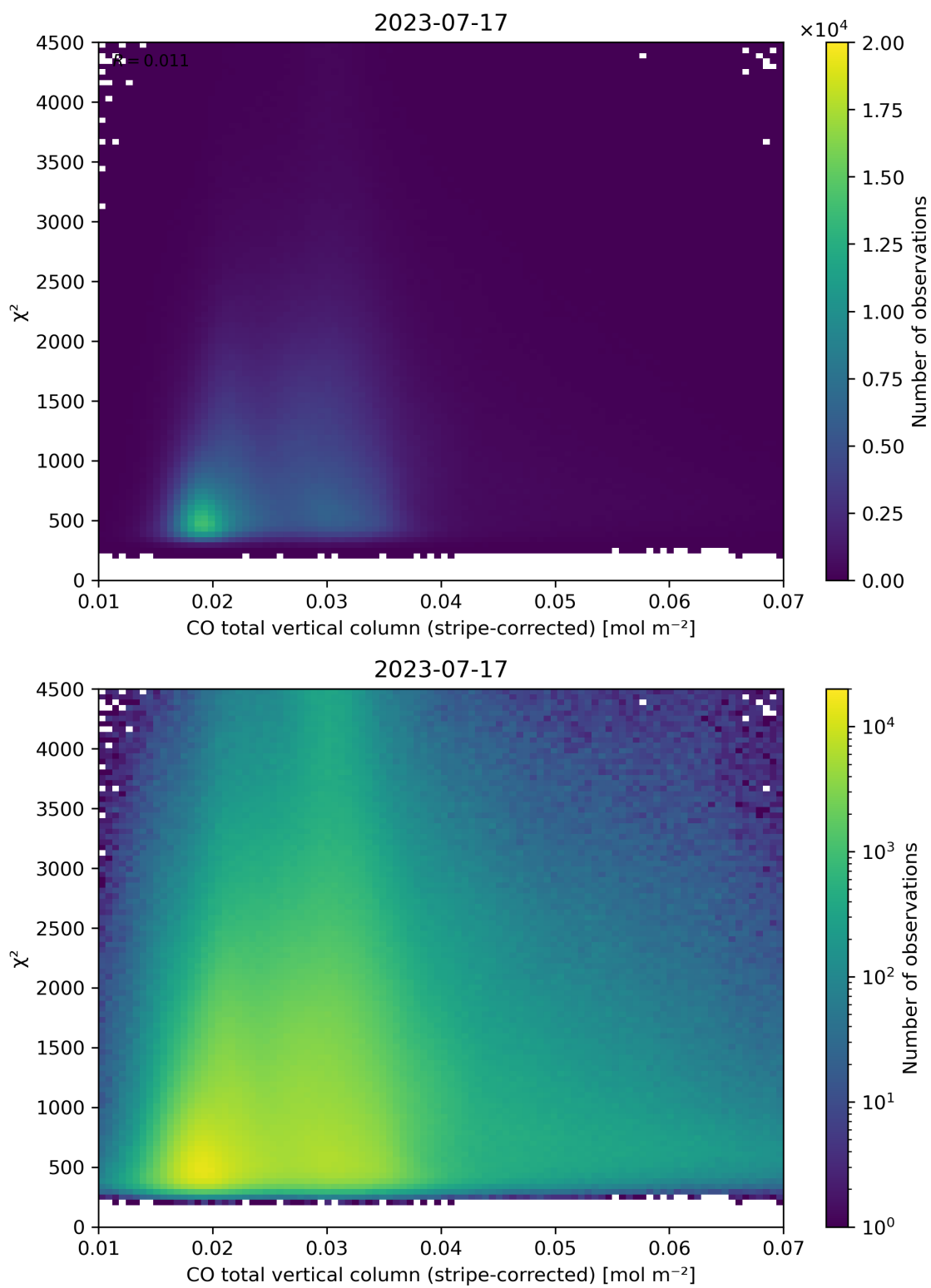
Figure 37: Scatter density plot of “CO total vertical column (stripe-corrected)” against “ \chi^2 ” for 2023-07-16 to 2023-07-18.
