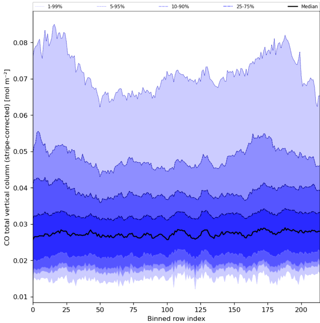
Figure 27: Along track statistics of “CO total vertical column (stripe-corrected)” for 2023-07-16 to 2023-07-18
