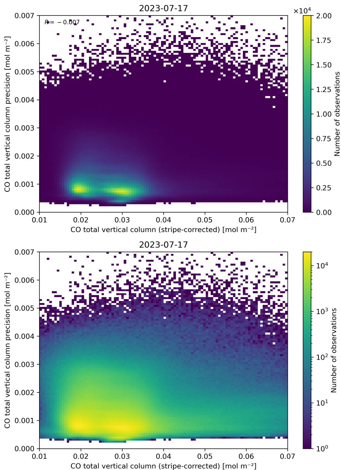
Figure 36: Scatter density plot of “CO total vertical column (stripe-corrected)” against “CO total vertical column precision” for 2023-07-16 to 2023-07-18.
