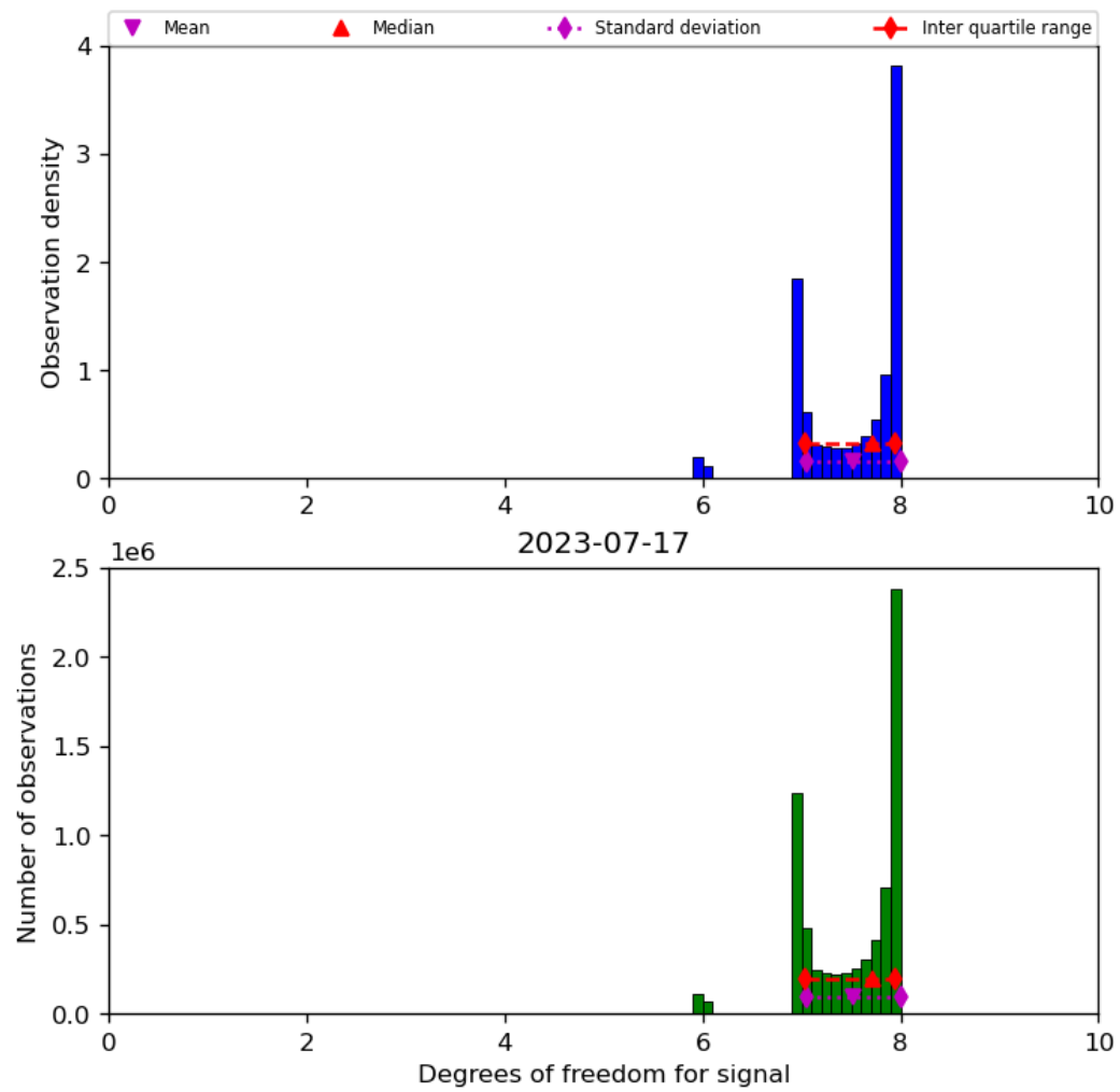
Figure 23: Histogram of “Degrees of freedom for signal” for 2023-07-16 to 2023-07-18
