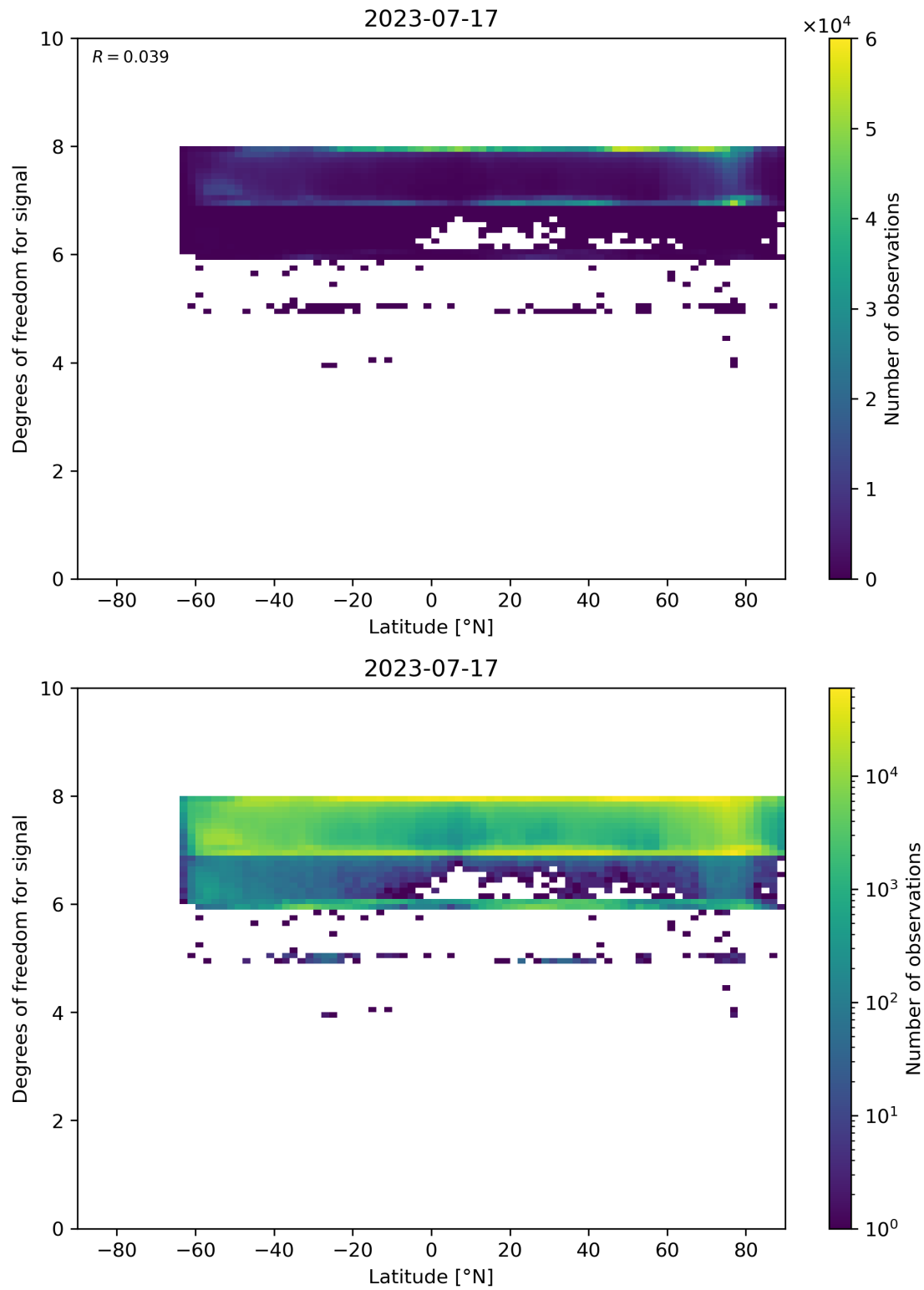
Figure 55: Scatter density plot of “Latitude” against “Degrees of freedom for signal” for 2023-07-16 to 2023-07-18.
