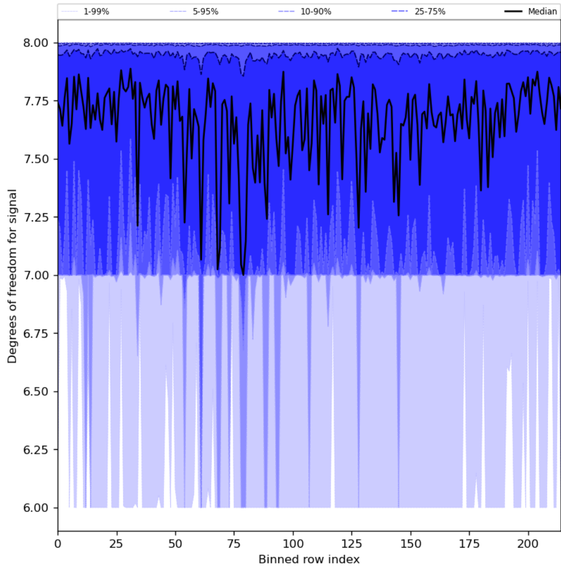
Figure 31: Along track statistics of “Degrees of freedom for signal” for 2023-07-16 to 2023-07-18
