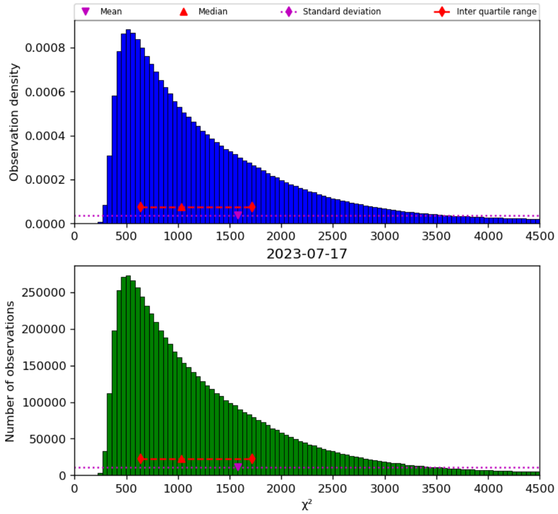
Figure 22: Histogram of “ \chi^2 ” for 2023-07-16 to 2023-07-18
