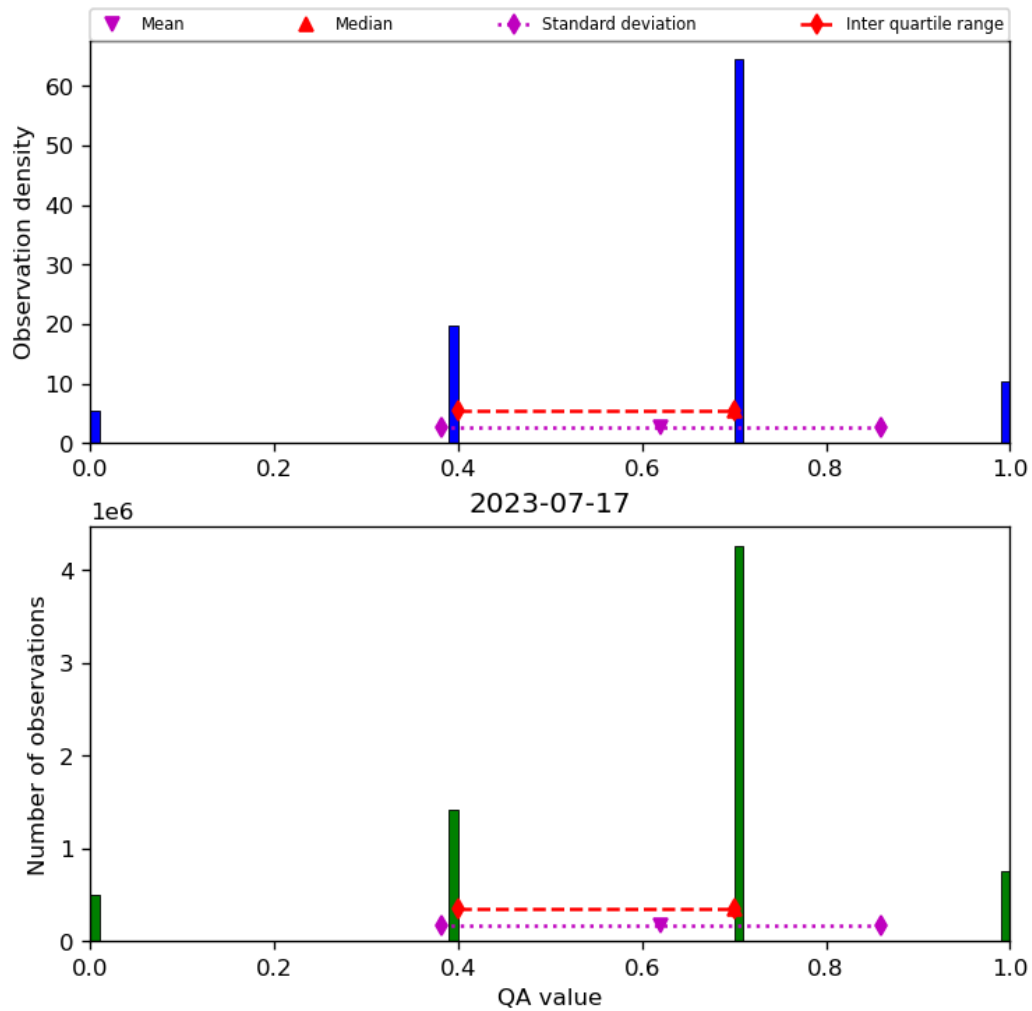
Figure 17: Histogram of “QA value” for 2023-07-16 to 2023-07-18
