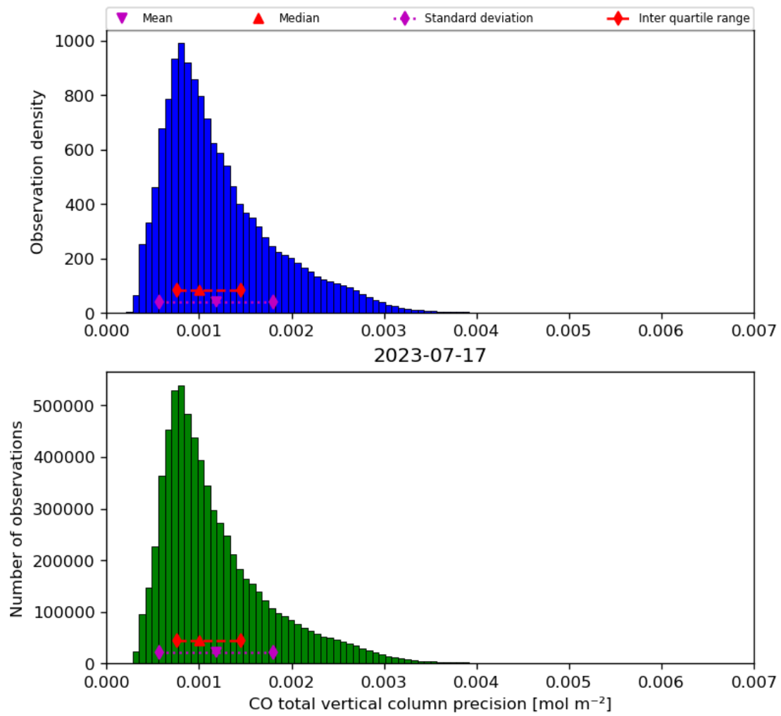
Figure 20: Histogram of “CO total vertical column precision” for 2023-07-16 to 2023-07-18
