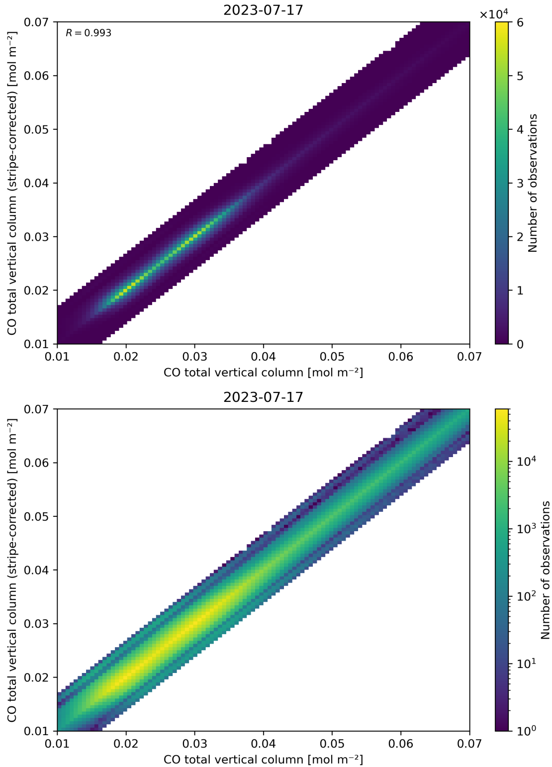
Figure 33: Scatter density plot of “CO total vertical column” against “CO total vertical column (stripe-corrected)” for 2023-07-16 to 2023-07-18.
