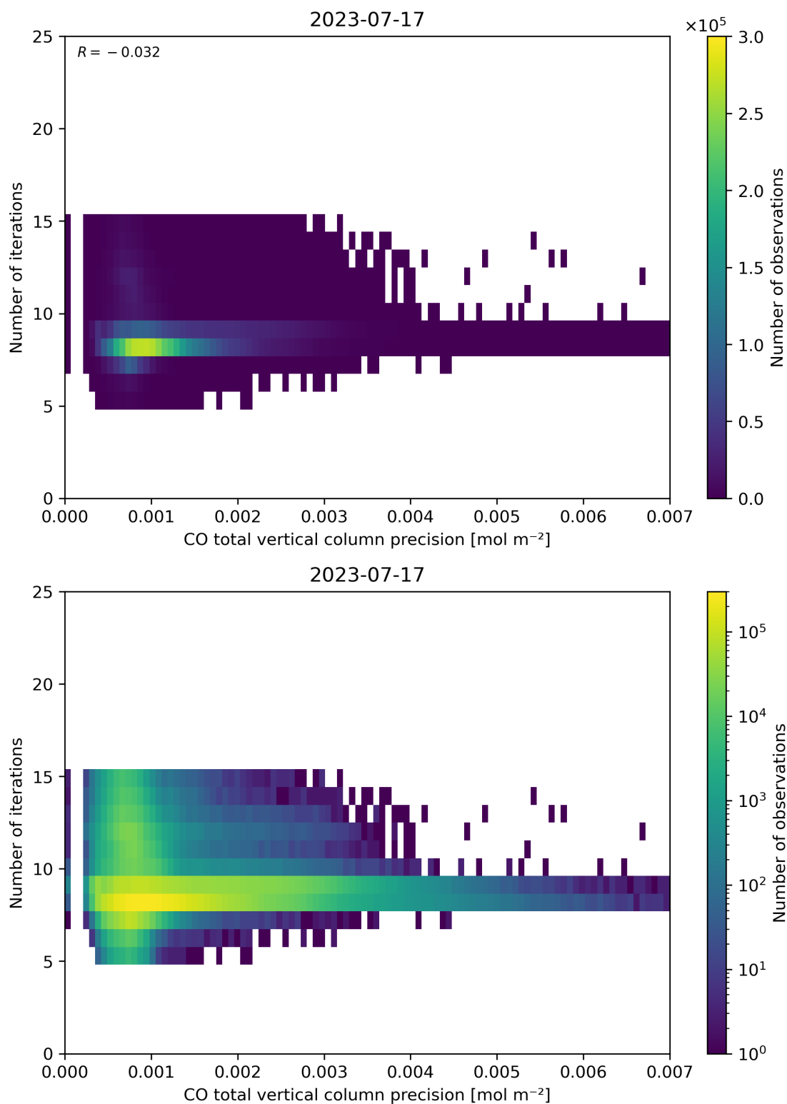
Figure 46: Scatter density plot of “CO total vertical column precision” against “Number of iterations” for 2023-07-16 to 2023-07-18.
