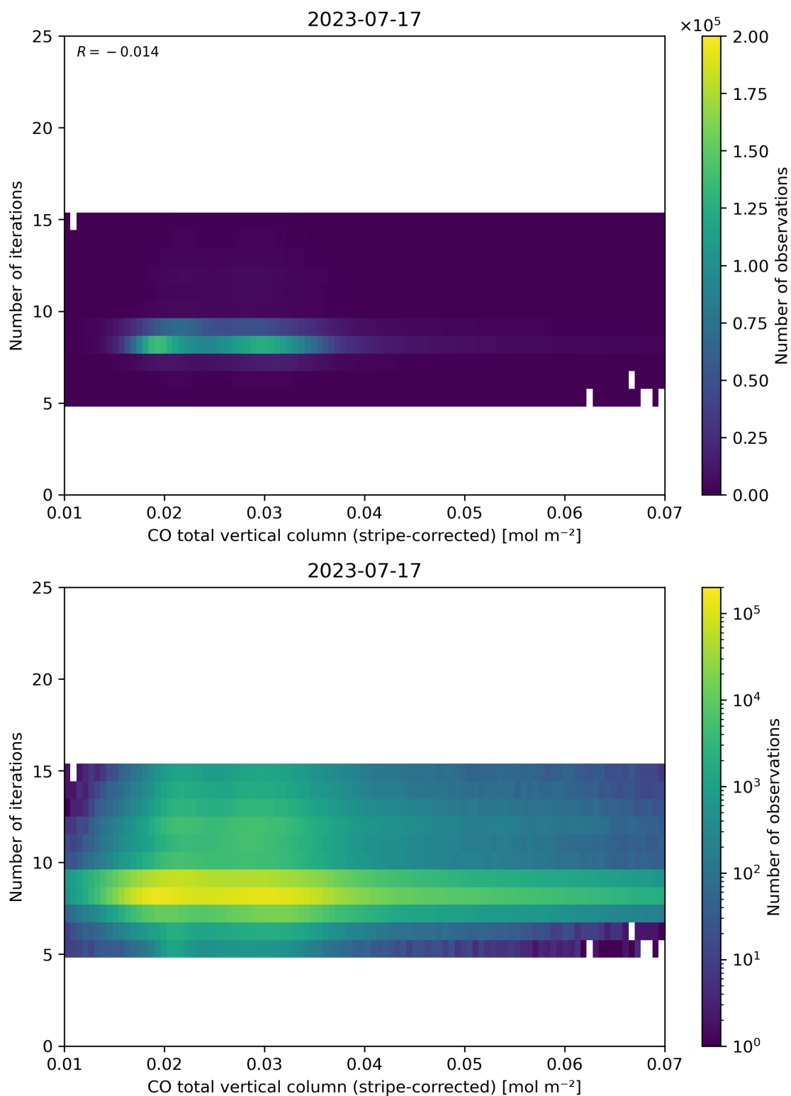
Figure 39: Scatter density plot of “CO total vertical column (stripe-corrected)” against “Number of iterations” for 2023-07-16 to 2023-07-18.
