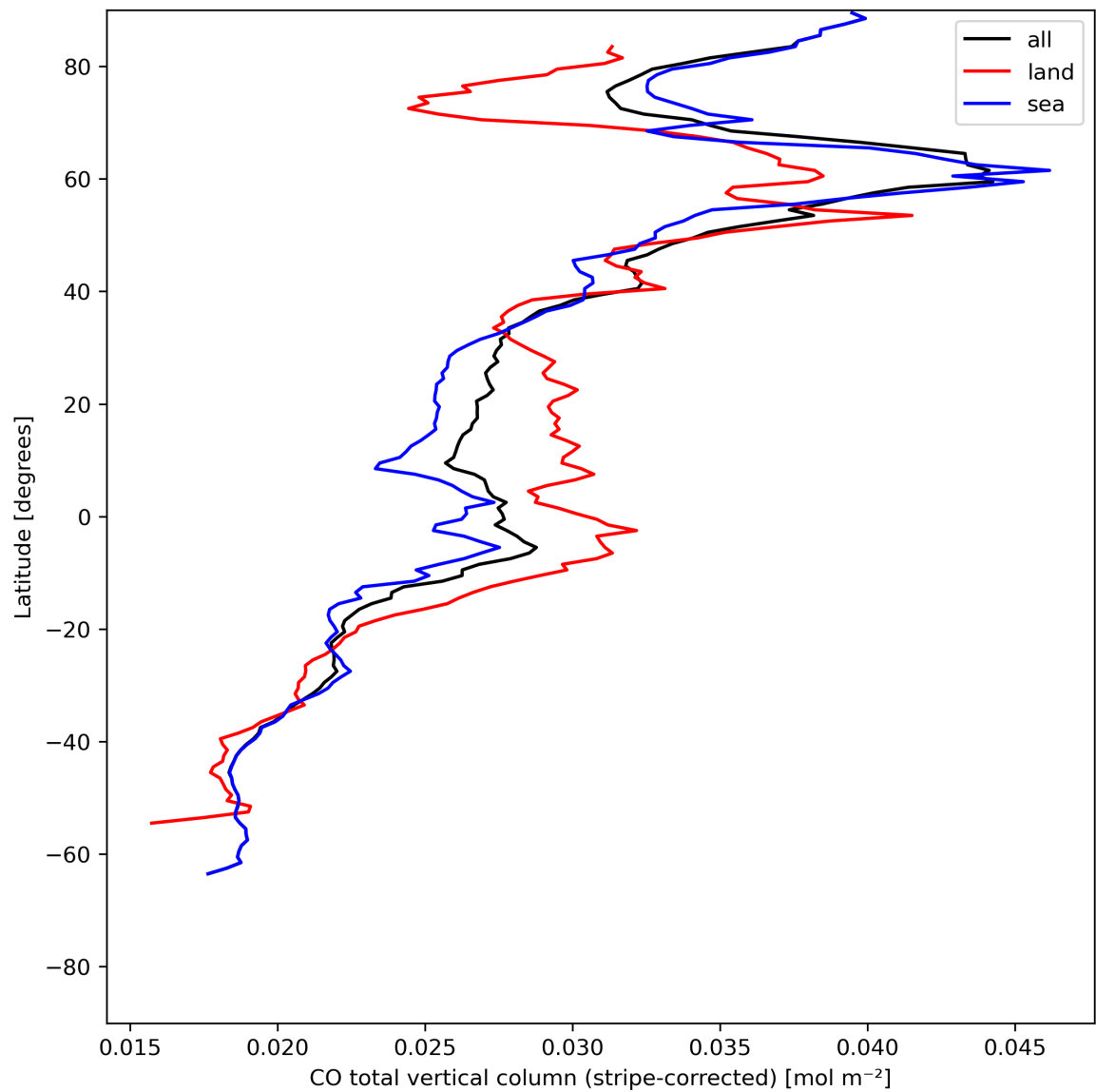
Figure 11: Zonal average of “CO total vertical column (stripe-corrected)” for 2023-07-16 to 2023-07-18.
