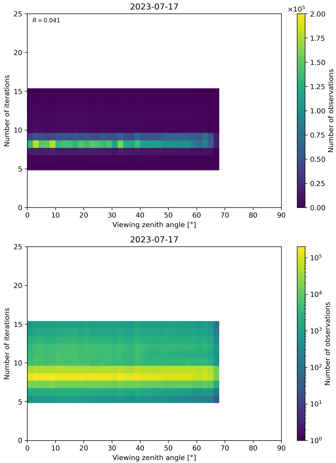
Figure 75: Scatter density plot of “Viewing zenith angle” against “Number of iterations” for 2023-07-16 to 2023-07-18.
