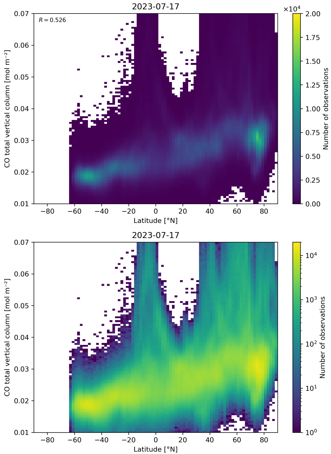
Figure 51: Scatter density plot of “Latitude” against “CO total vertical column” for 2023-07-16 to 2023-07-18.
