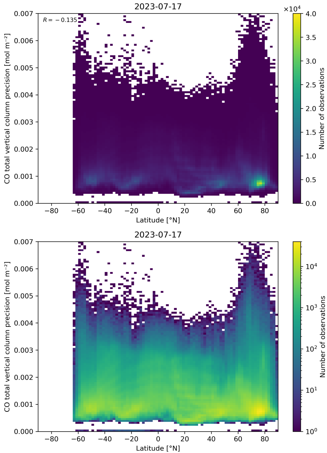
Figure 53: Scatter density plot of “Latitude” against “CO total vertical column precision” for 2023-07-16 to 2023-07-18.
