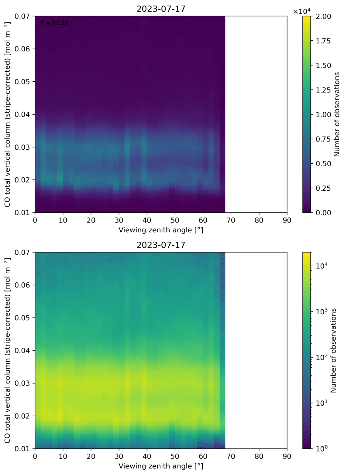
Figure 70: Scatter density plot of “Viewing zenith angle” against “CO total vertical column (stripe-corrected)” for 2023-07-16 to 2023-07-18.
