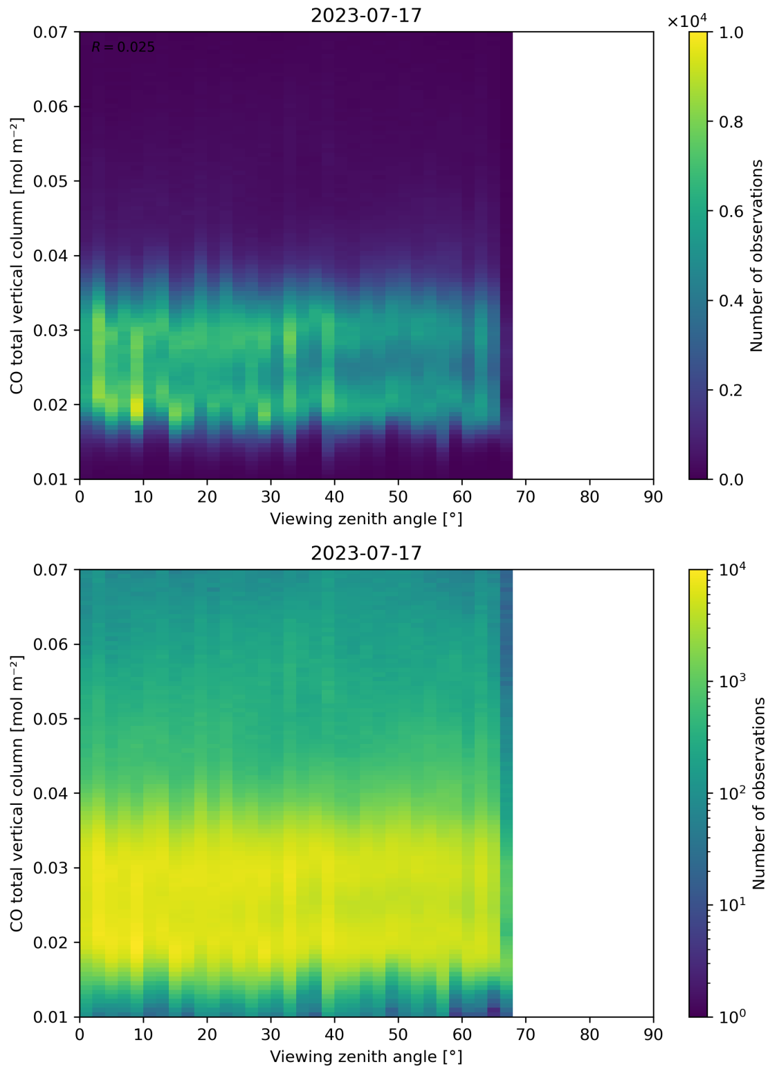
Figure 69: Scatter density plot of “Viewing zenith angle” against “CO total vertical column” for 2023-07-16 to 2023-07-18.
