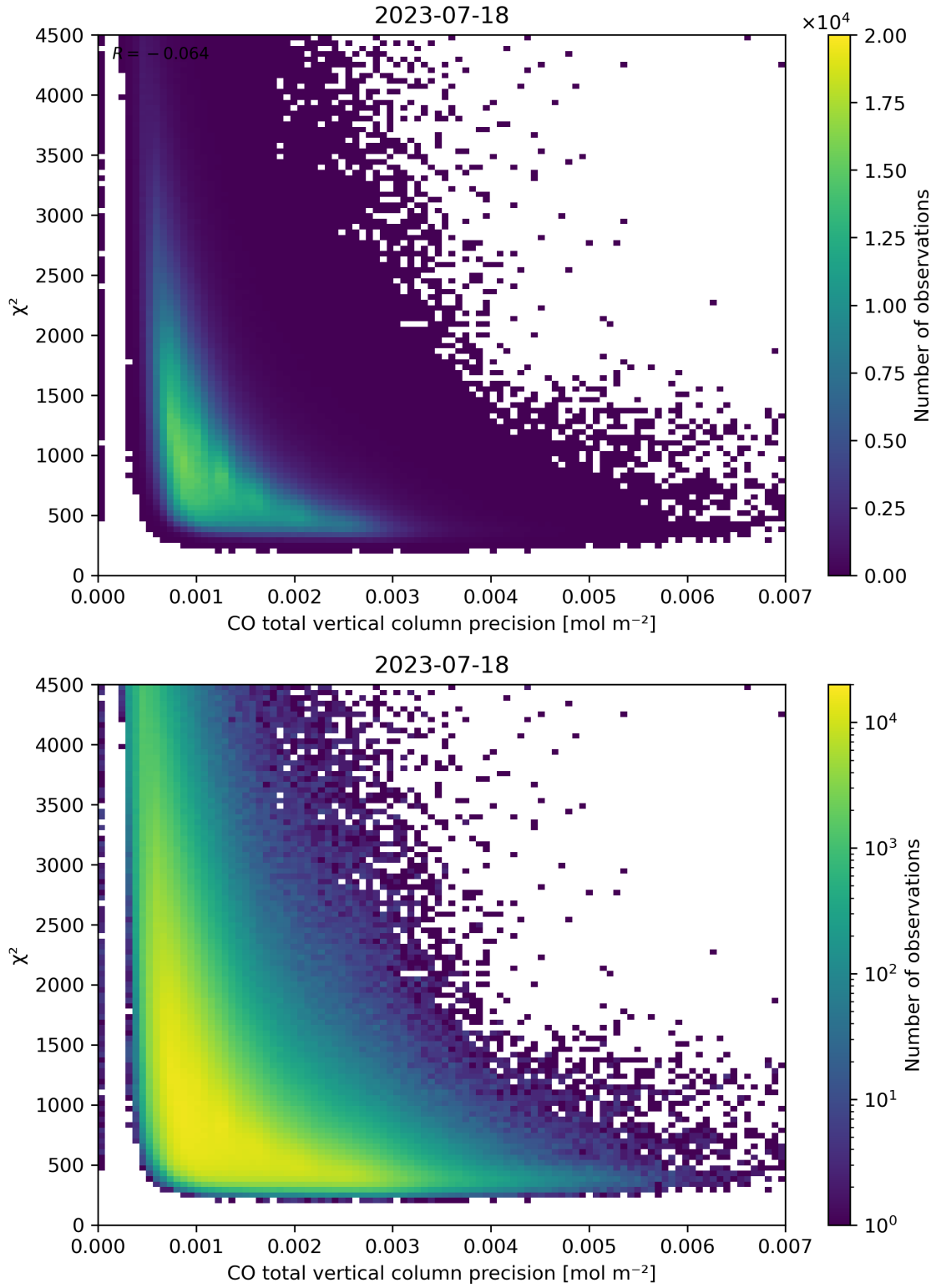
Figure 44: Scatter density plot of “CO total vertical column precision” against “ \chi^2 ” for 2023-07-17 to 2023-07-19.
