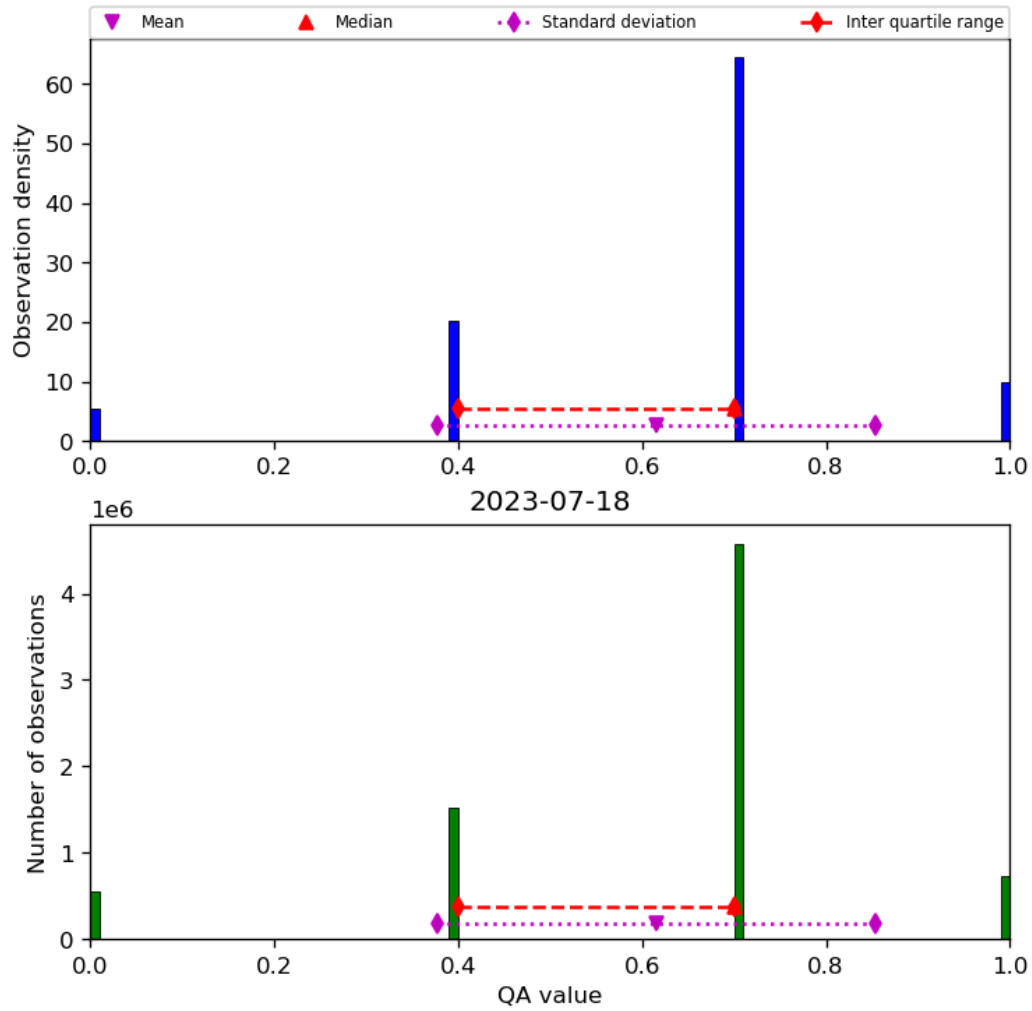
Figure 17: Histogram of “QA value” for 2023-07-17 to 2023-07-19
