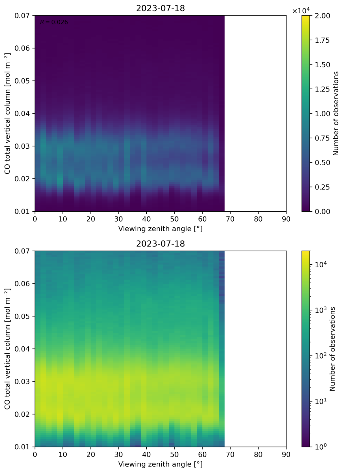
Figure 69: Scatter density plot of “Viewing zenith angle” against “CO total vertical column” for 2023-07-17 to 2023-07-19.
