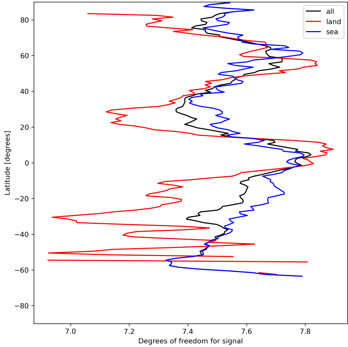
Figure 15: Zonal average of “Degrees of freedom for signal” for 2023-07-17 to 2023-07-19.
