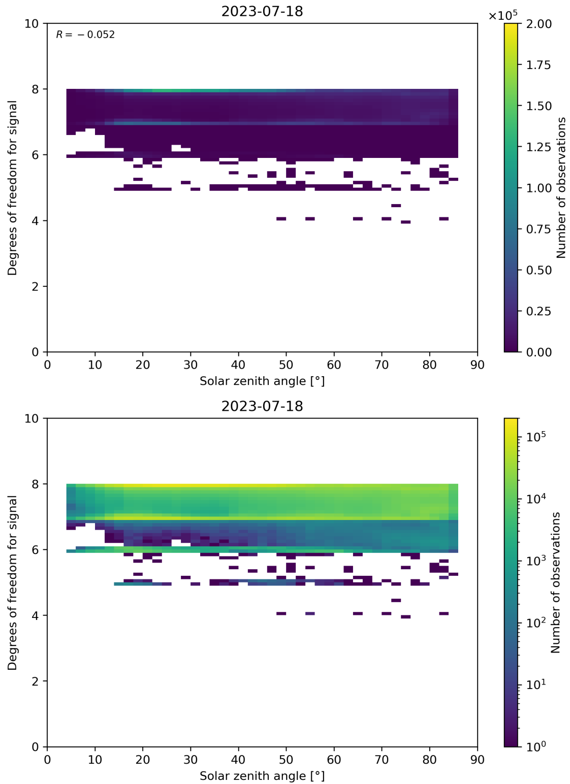
Figure 65: Scatter density plot of “Solar zenith angle” against “Degrees of freedom for signal” for 2023-07-17 to 2023-07-19.
