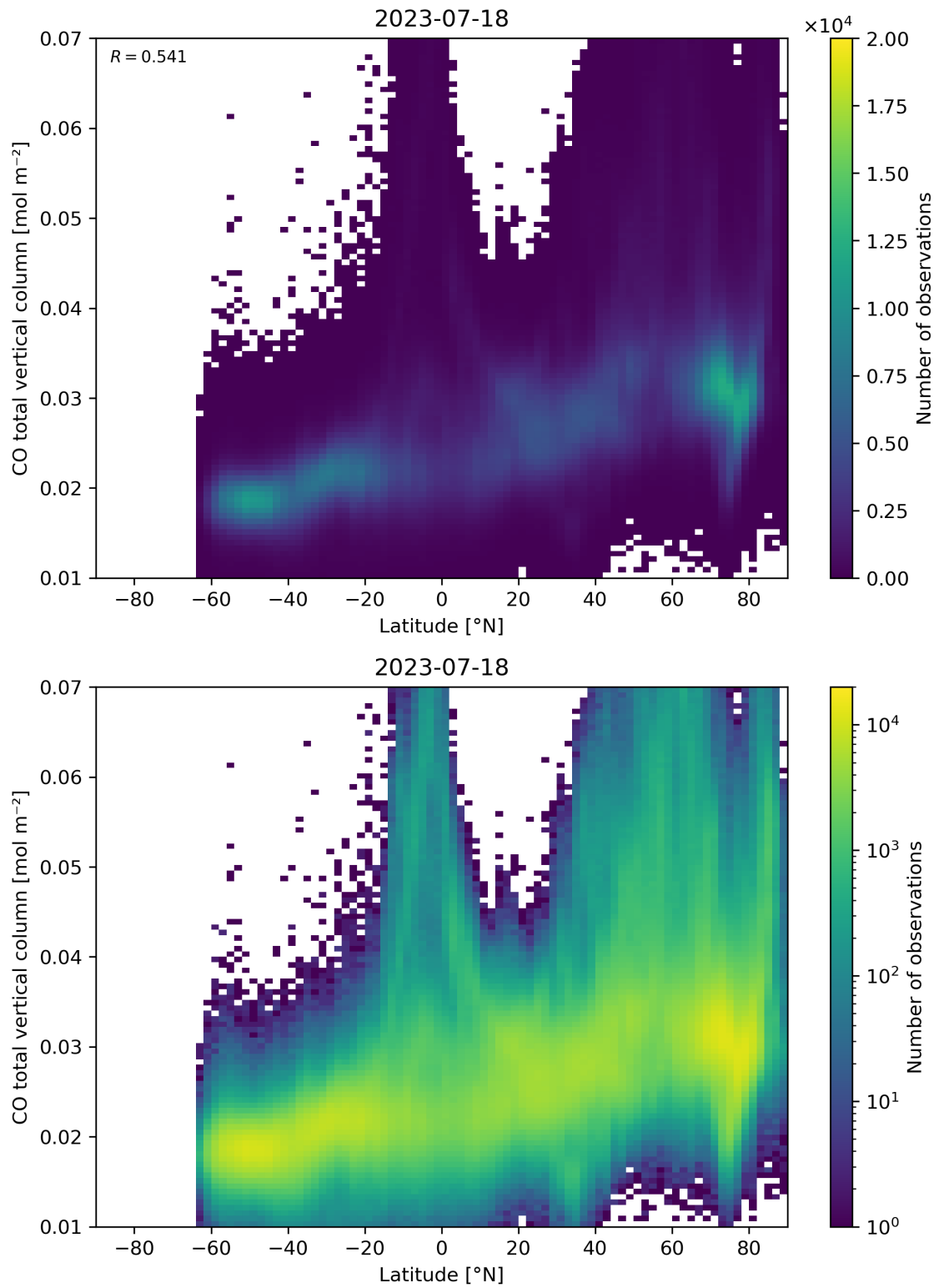
Figure 51: Scatter density plot of “Latitude” against “CO total vertical column” for 2023-07-17 to 2023-07-19.
