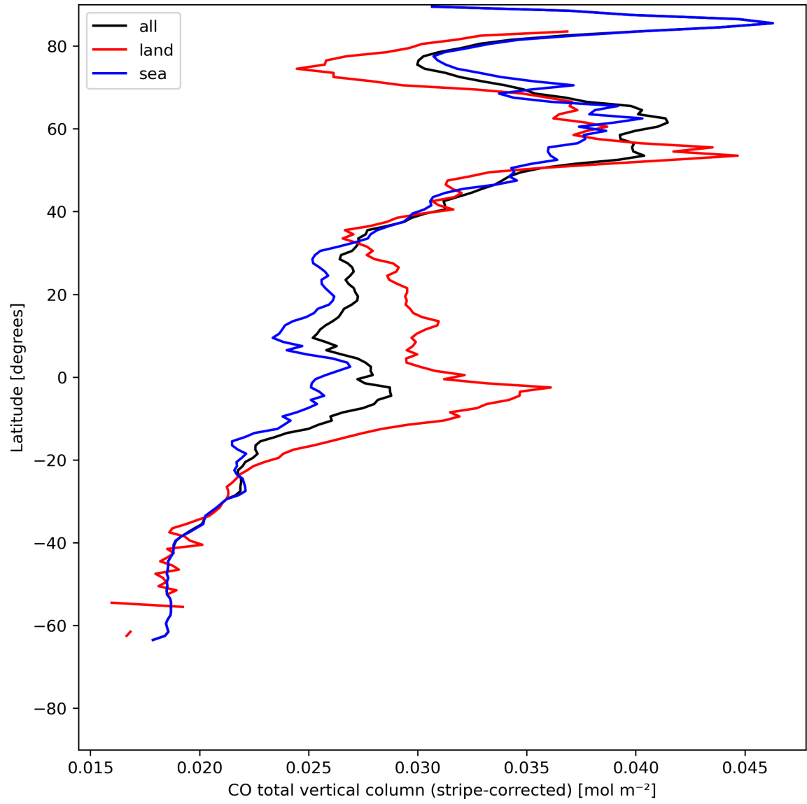
Figure 11: Zonal average of “CO total vertical column (stripe-corrected)” for 2023-07-17 to 2023-07-19.
