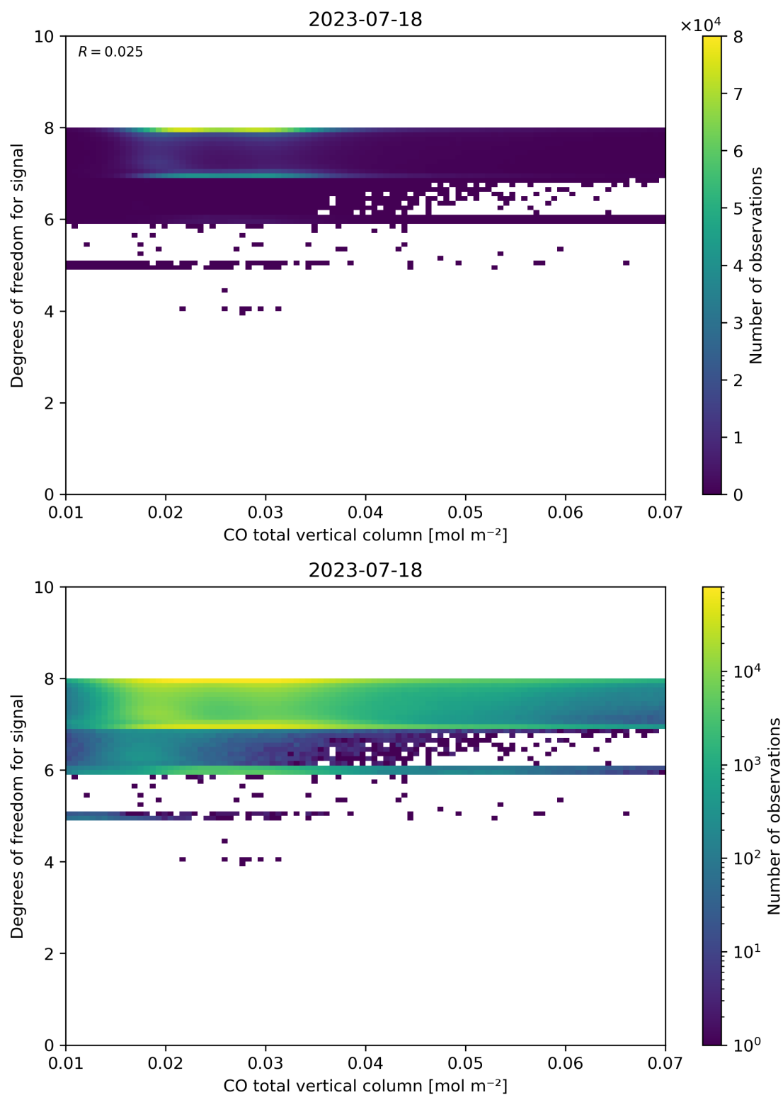
Figure 41: Scatter density plot of “CO total vertical column” against “Degrees of freedom for signal” for 2023-07-17 to 2023-07-19.
