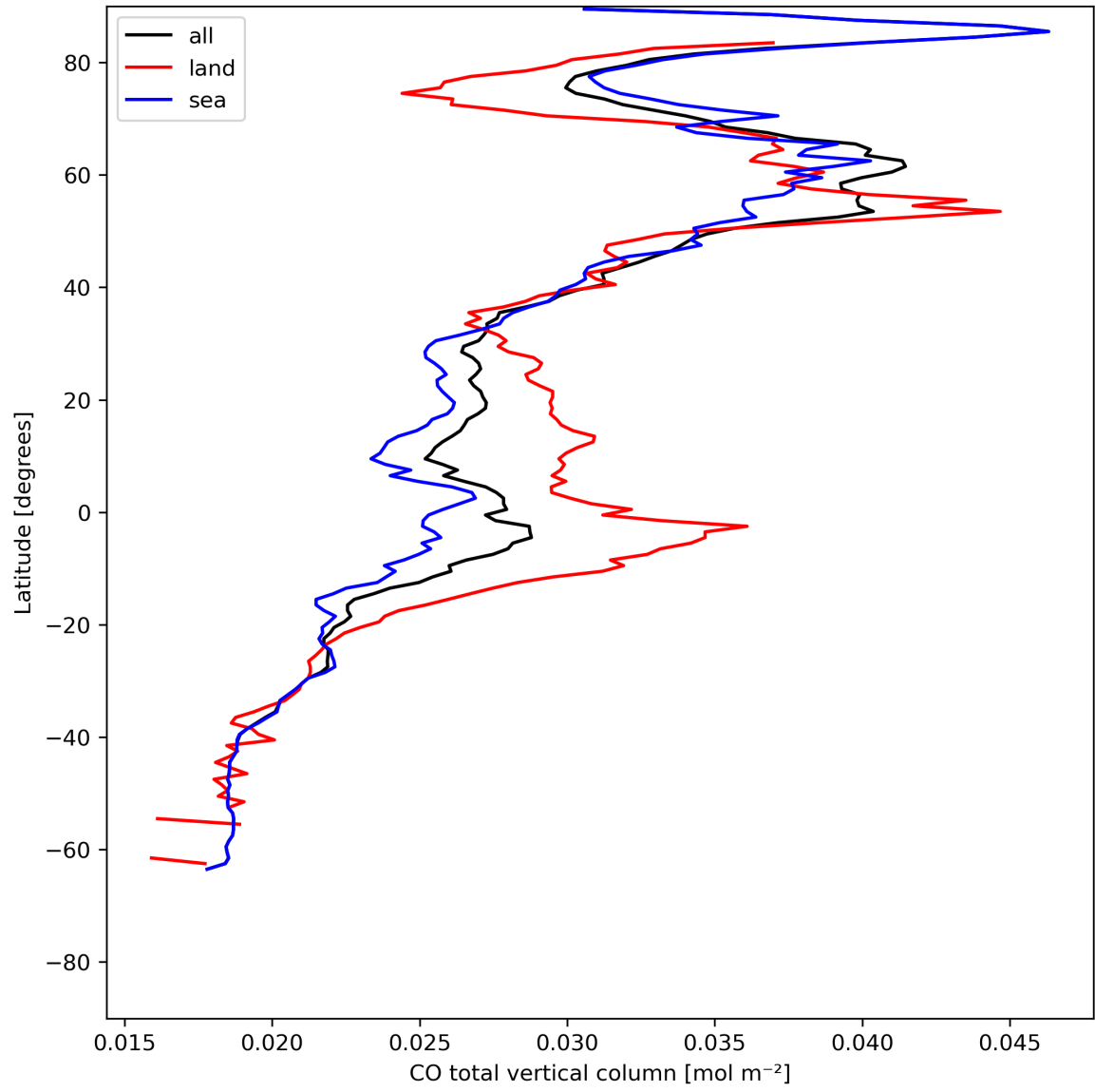
Figure 10: Zonal average of “CO total vertical column” for 2023-07-17 to 2023-07-19.
