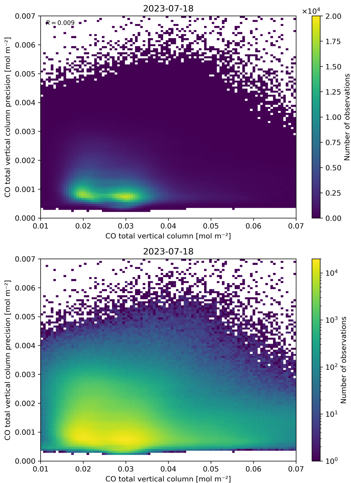
Figure 34: Scatter density plot of “CO total vertical column” against “CO total vertical column precision” for 2023-07-17 to 2023-07-19.
