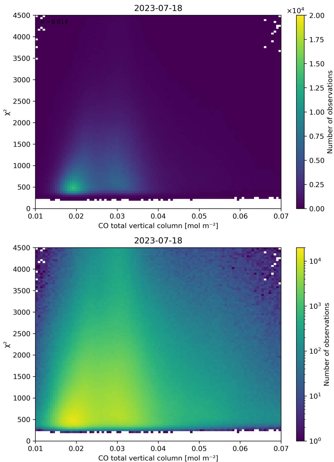
Figure 35: Scatter density plot of “CO total vertical column” against “ \chi^2 ” for 2023-07-17 to 2023-07-19.
