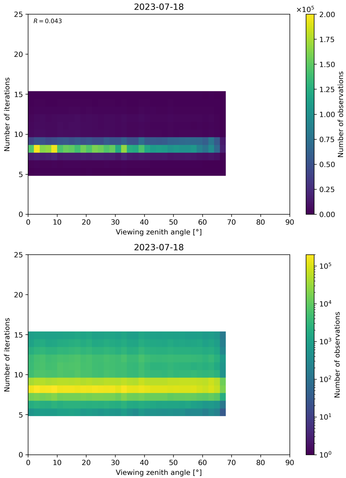
Figure 75: Scatter density plot of “Viewing zenith angle” against “Number of iterations” for 2023-07-17 to 2023-07-19.
