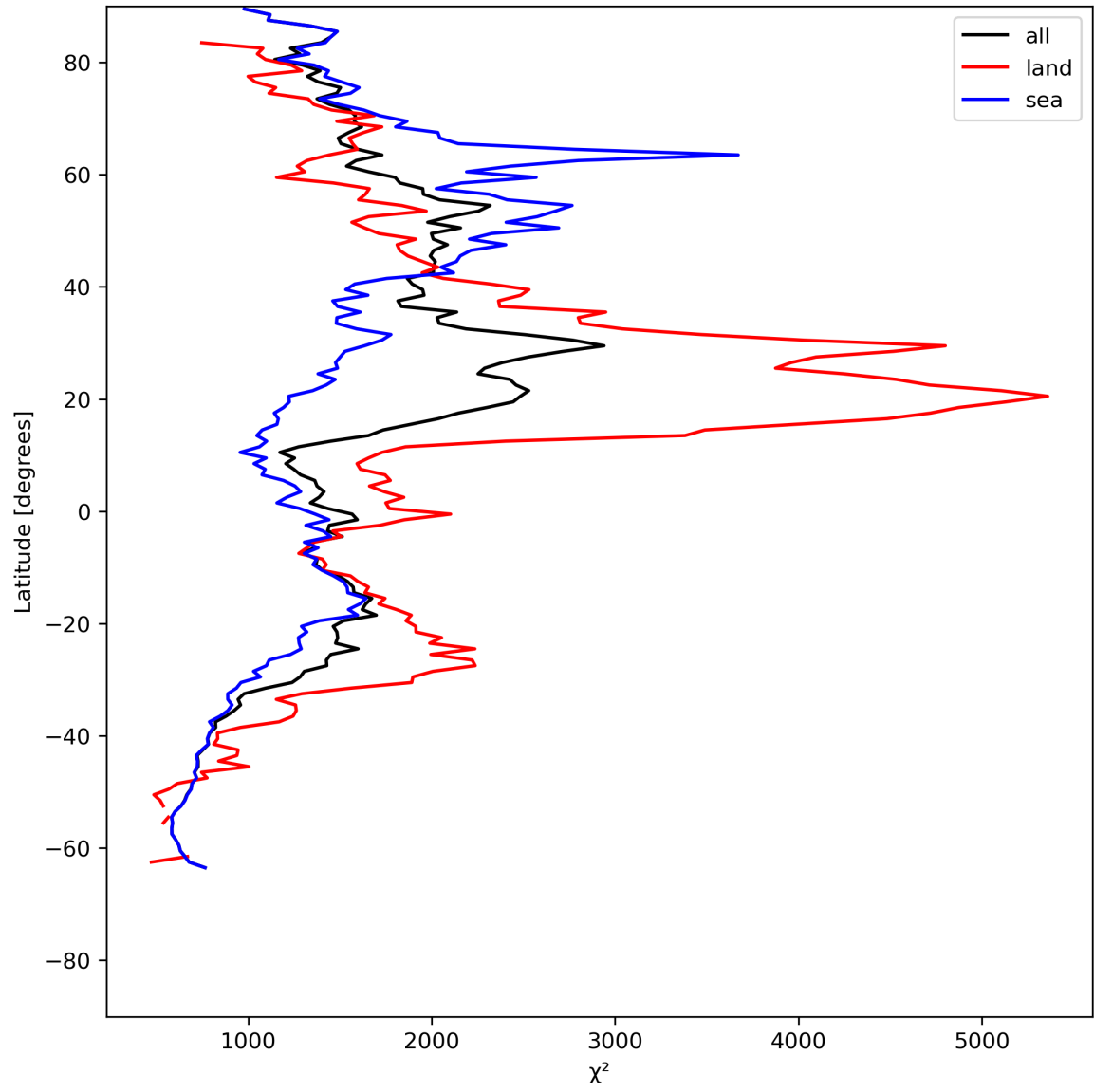
Figure 14: Zonal average of “ \chi^2 ” for 2023-07-17 to 2023-07-19.
