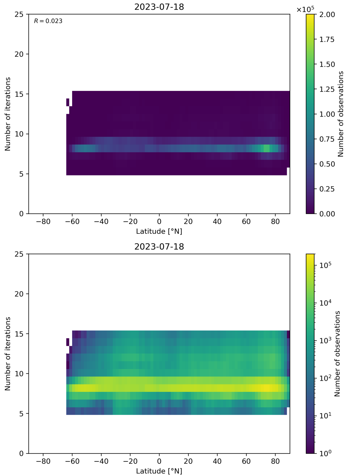
Figure 56: Scatter density plot of “Latitude” against “Number of iterations” for 2023-07-17 to 2023-07-19.
