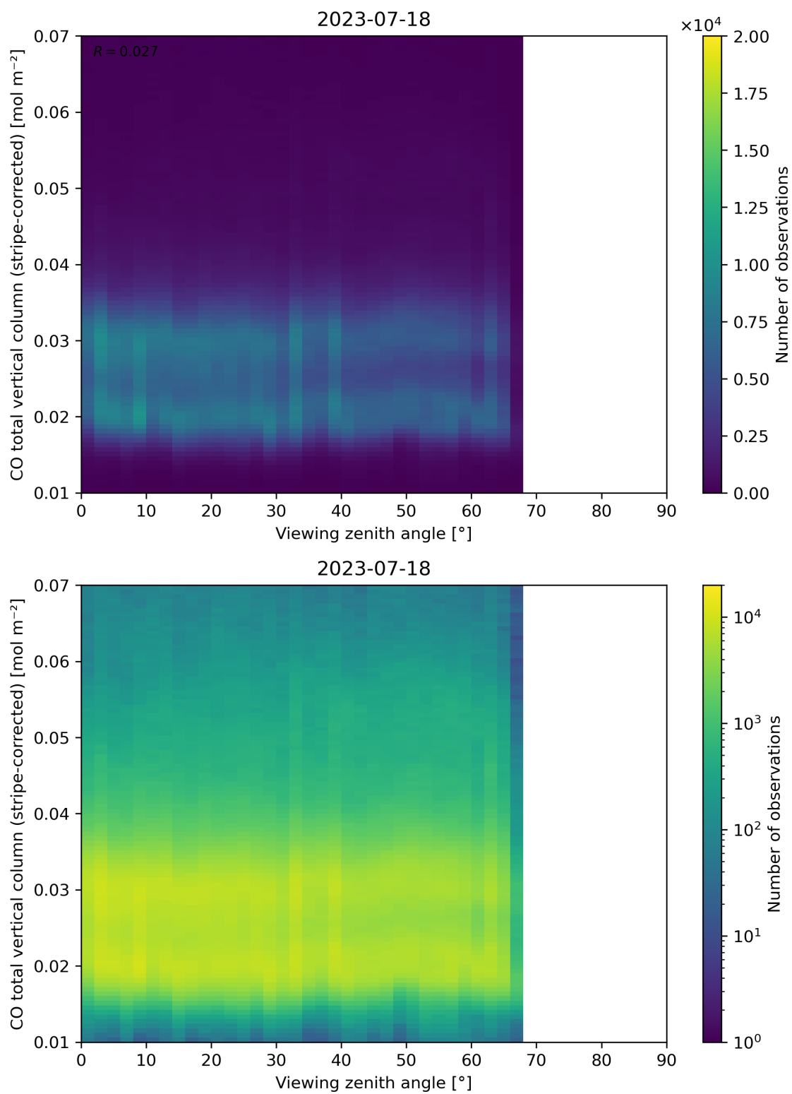
Figure 70: Scatter density plot of “Viewing zenith angle” against “CO total vertical column (stripe-corrected)” for 2023-07-17 to 2023-07-19.
