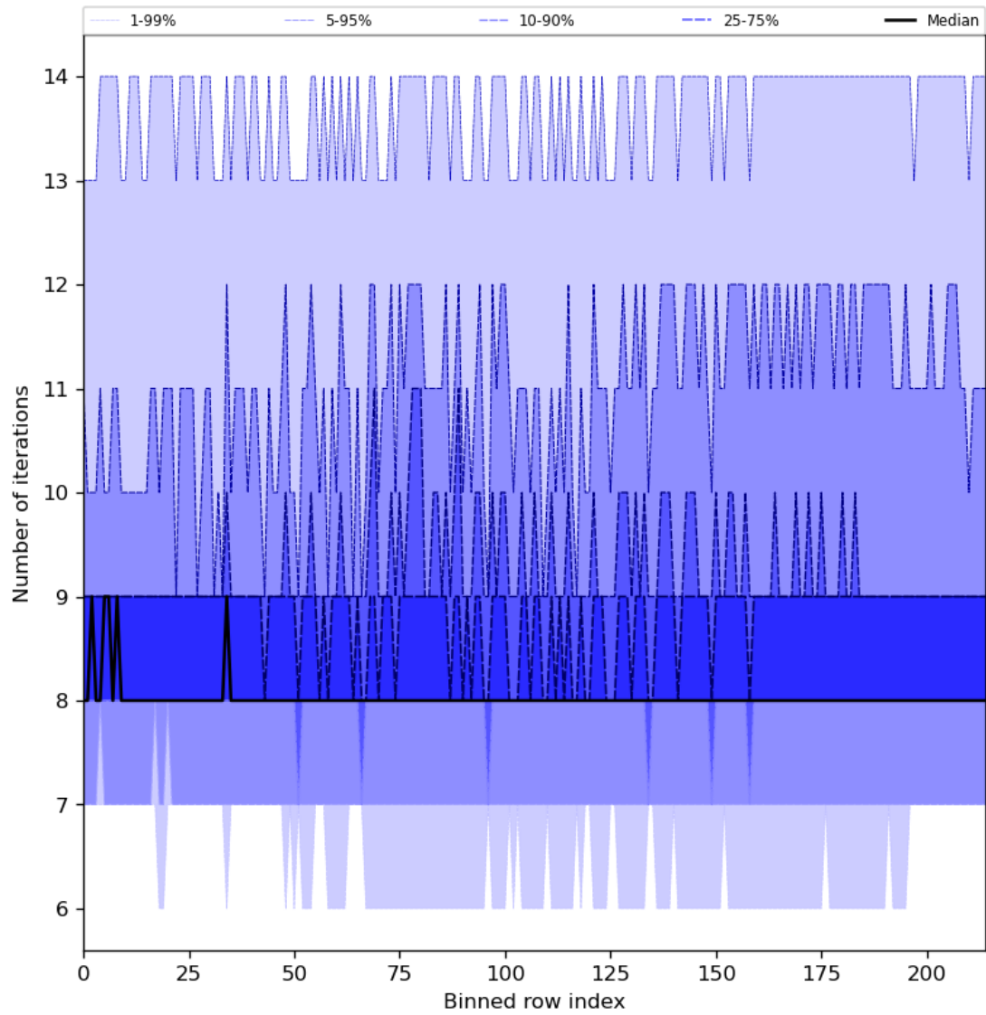
Figure 32: Along track statistics of “Number of iterations” for 2023-07-17 to 2023-07-19
