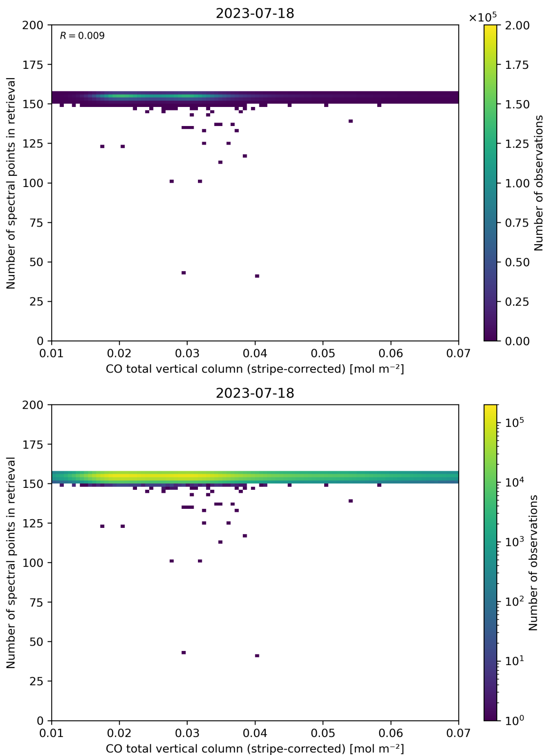
Figure 40: Scatter density plot of “CO total vertical column (stripe-corrected)” against “Number of spectral points in retrieval” for 2023-07-17 to 2023-07-19.
