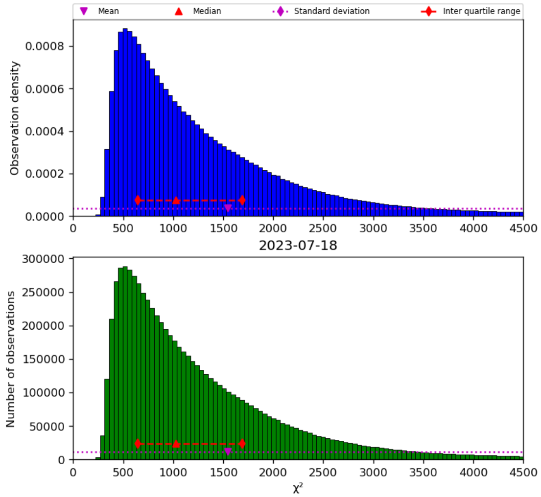
Figure 22: Histogram of “ \chi^2 ” for 2023-07-17 to 2023-07-19
