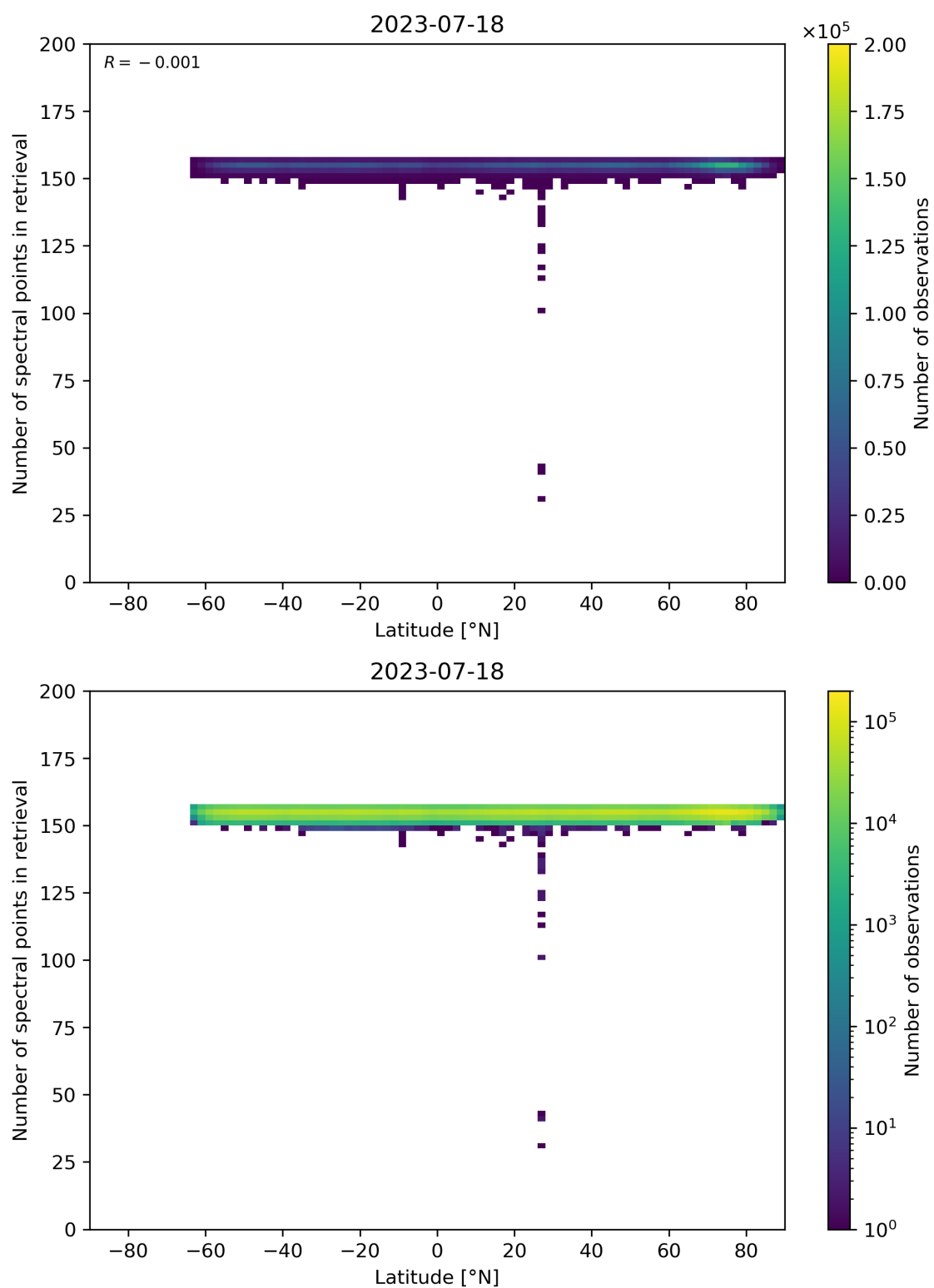
Figure 57: Scatter density plot of “Latitude” against “Number of spectral points in retrieval” for 2023-07-17 to 2023-07-19.
