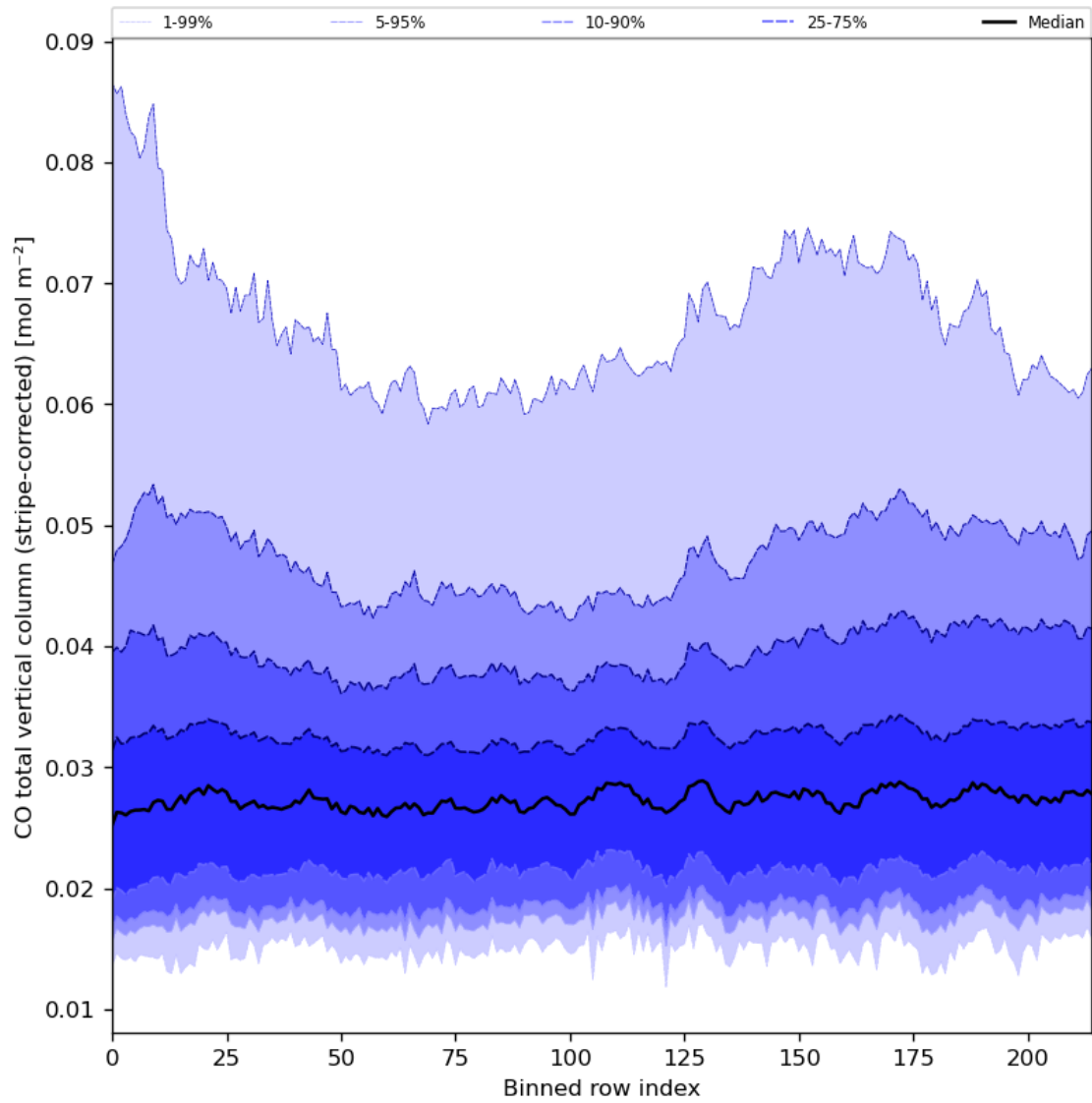
Figure 27: Along track statistics of “CO total vertical column (stripe-corrected)” for 2023-07-17 to 2023-07-19
