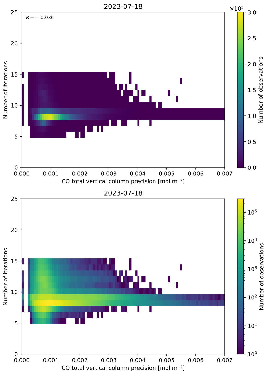
Figure 46: Scatter density plot of “CO total vertical column precision” against “Number of iterations” for 2023-07-17 to 2023-07-19.
