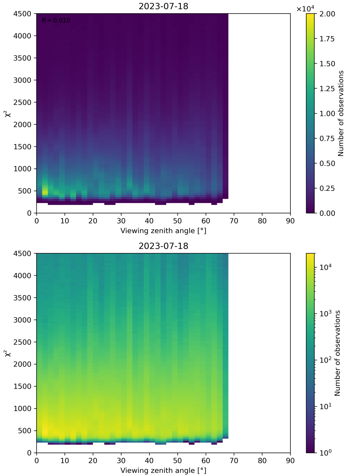
Figure 72: Scatter density plot of “Viewing zenith angle” against “ \chi^2 ” for 2023-07-17 to 2023-07-19.
