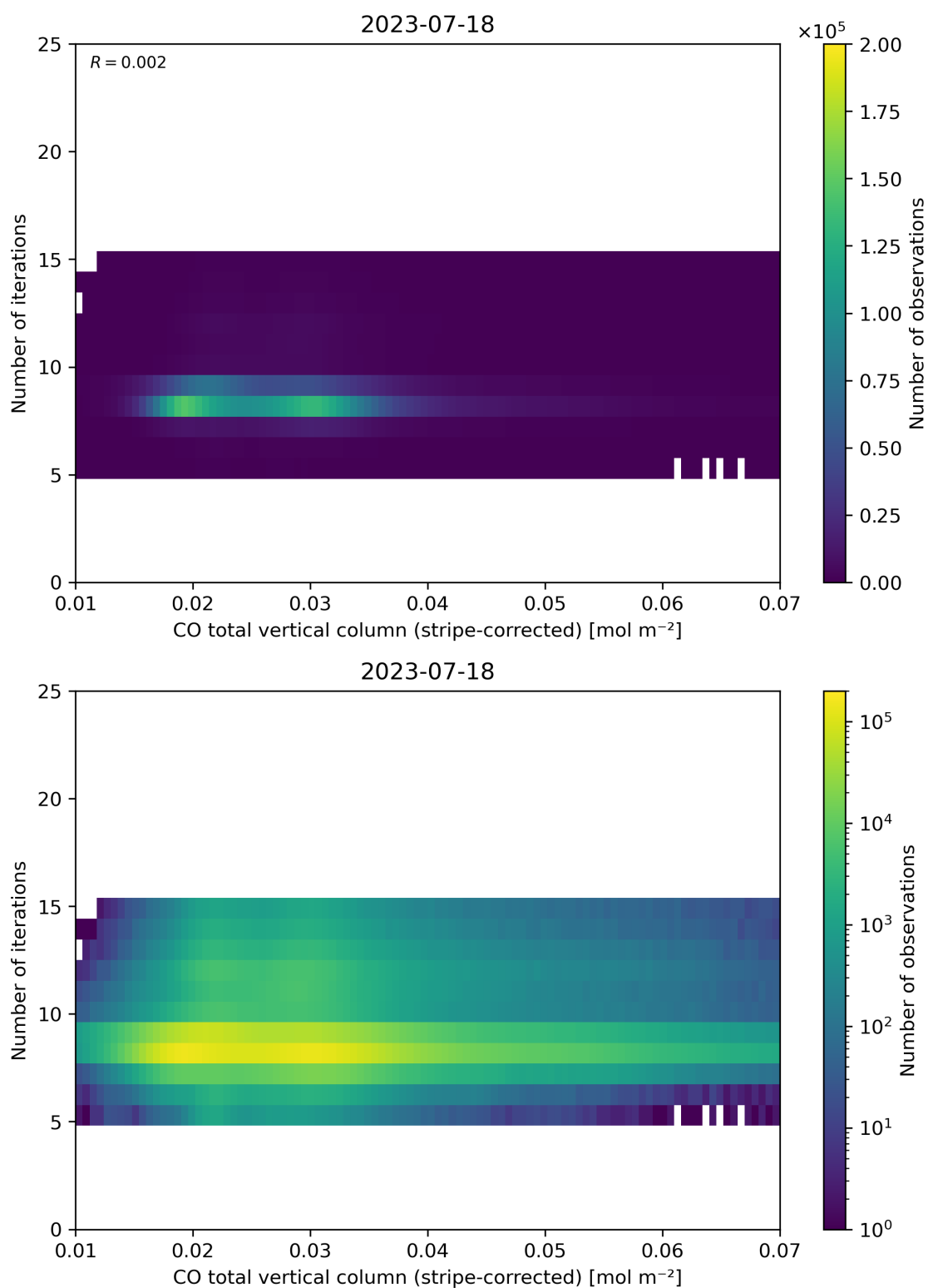
Figure 39: Scatter density plot of “CO total vertical column (stripe-corrected)” against “Number of iterations” for 2023-07-17 to 2023-07-19.
