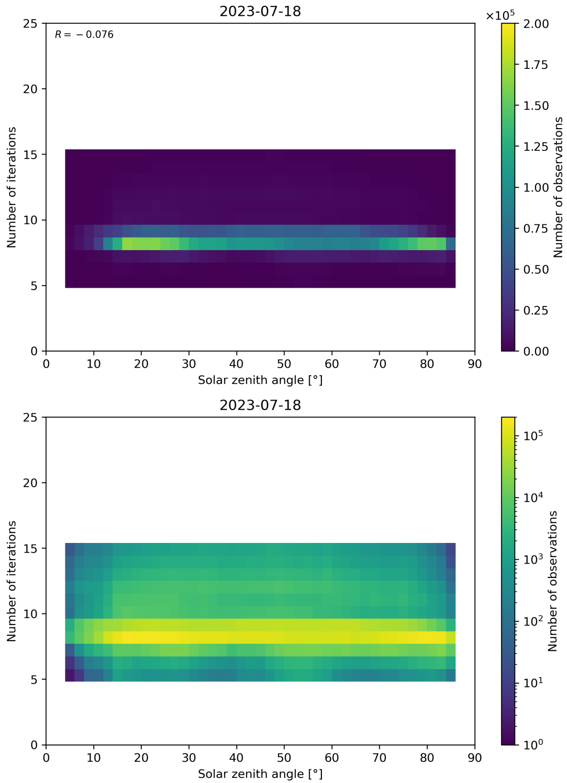
Figure 67: Scatter density plot of “Solar zenith angle” against “Number of iterations” for 2023-07-17 to 2023-07-19.
