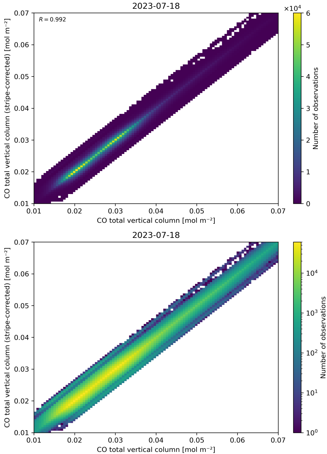
Figure 33: Scatter density plot of “CO total vertical column” against “CO total vertical column (stripe-corrected)” for 2023-07-17 to 2023-07-19.
