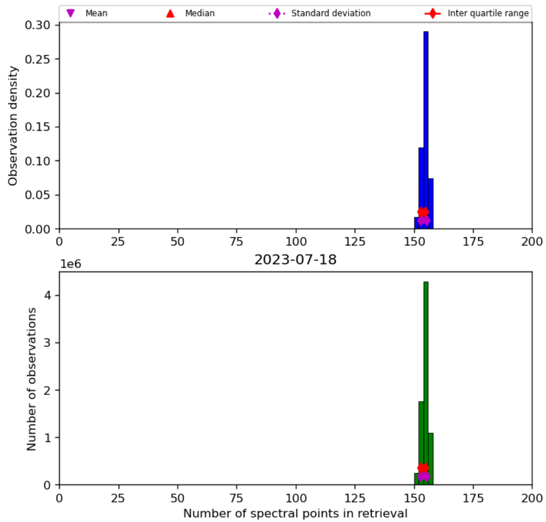
Figure 21: Histogram of “Number of spectral points in retrieval” for 2023-07-17 to 2023-07-19
