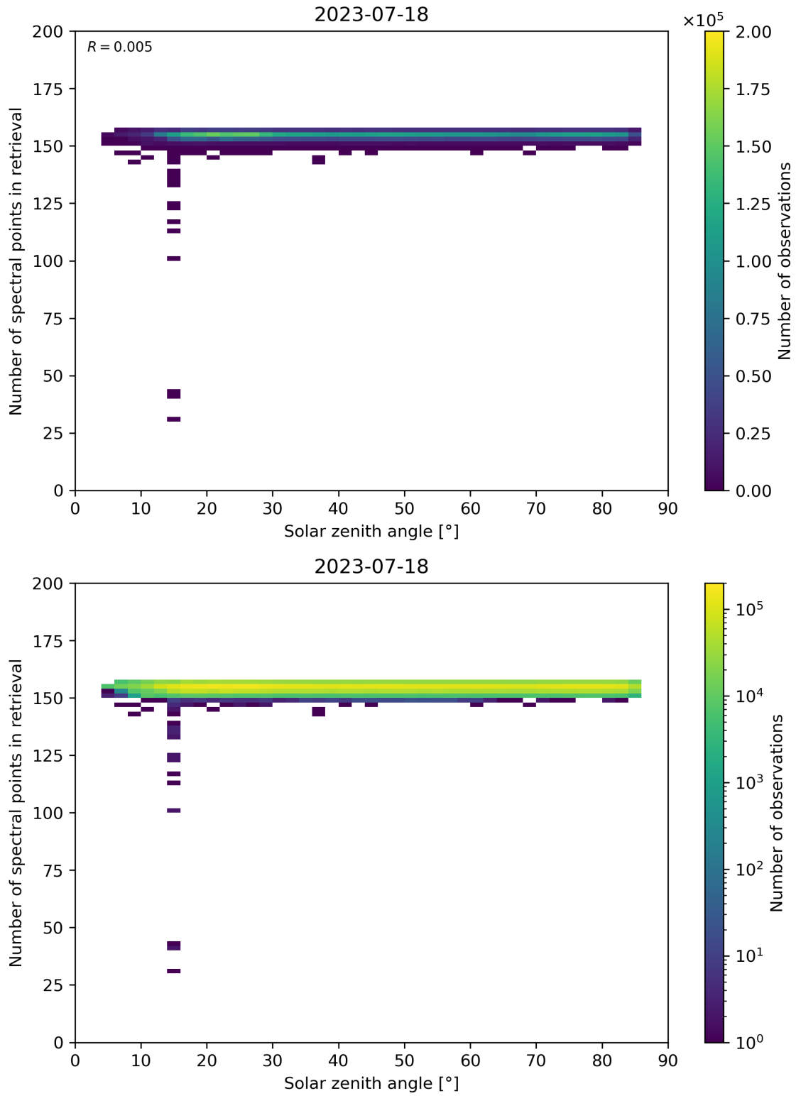
Figure 68: Scatter density plot of “Solar zenith angle” against “Number of spectral points in retrieval” for 2023-07-17 to 2023-07-19.
