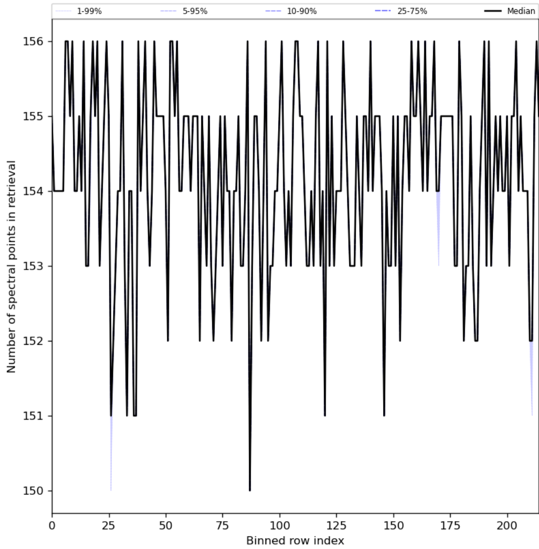
Figure 29: Along track statistics of “Number of spectral points in retrieval” for 2023-07-17 to 2023-07-19
