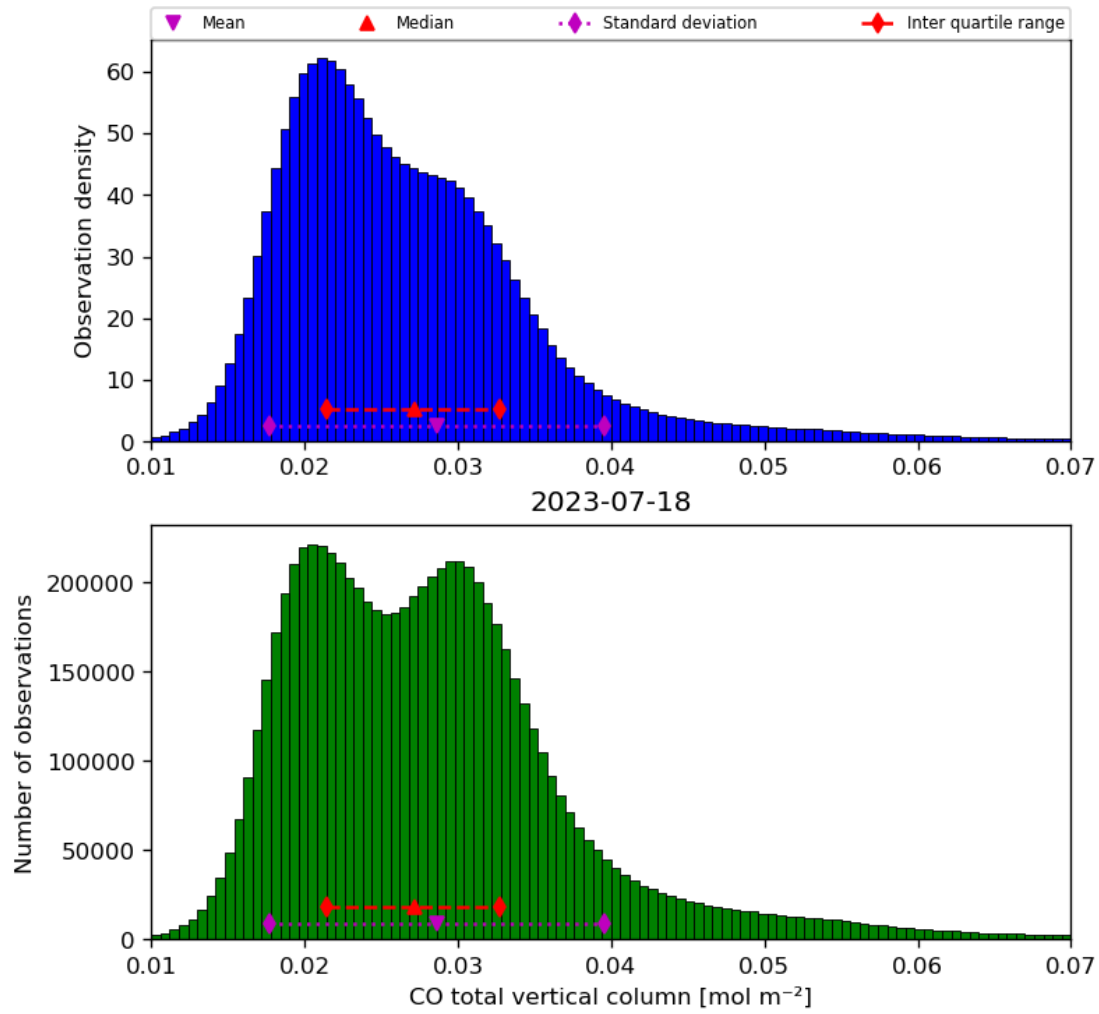
Figure 18: Histogram of “CO total vertical column” for 2023-07-17 to 2023-07-19
