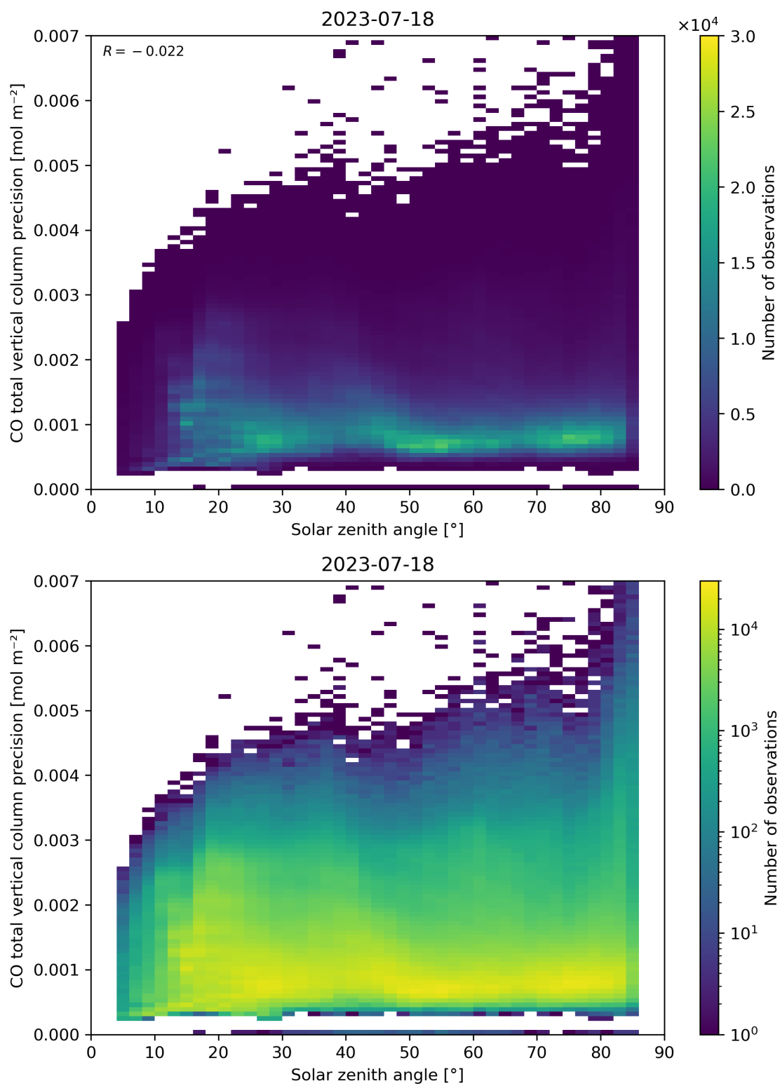
Figure 63: Scatter density plot of “Solar zenith angle” against “CO total vertical column precision” for 2023-07-17 to 2023-07-19.
