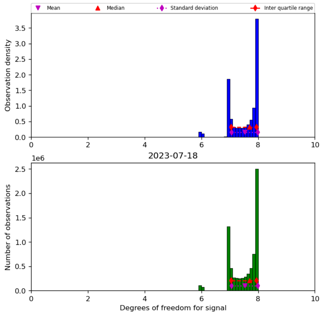
Figure 23: Histogram of “Degrees of freedom for signal” for 2023-07-17 to 2023-07-19
