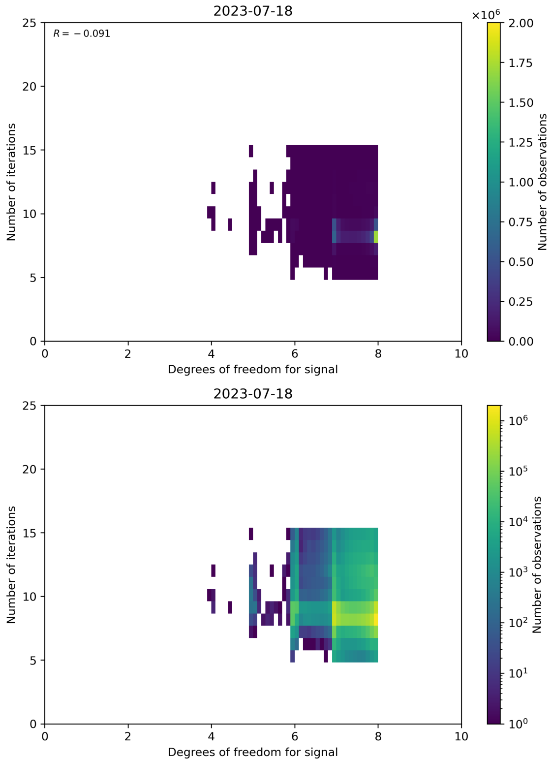
Figure 50: Scatter density plot of “Degrees of freedom for signal” against “Number of iterations” for 2023-07-17 to 2023-07-19.
