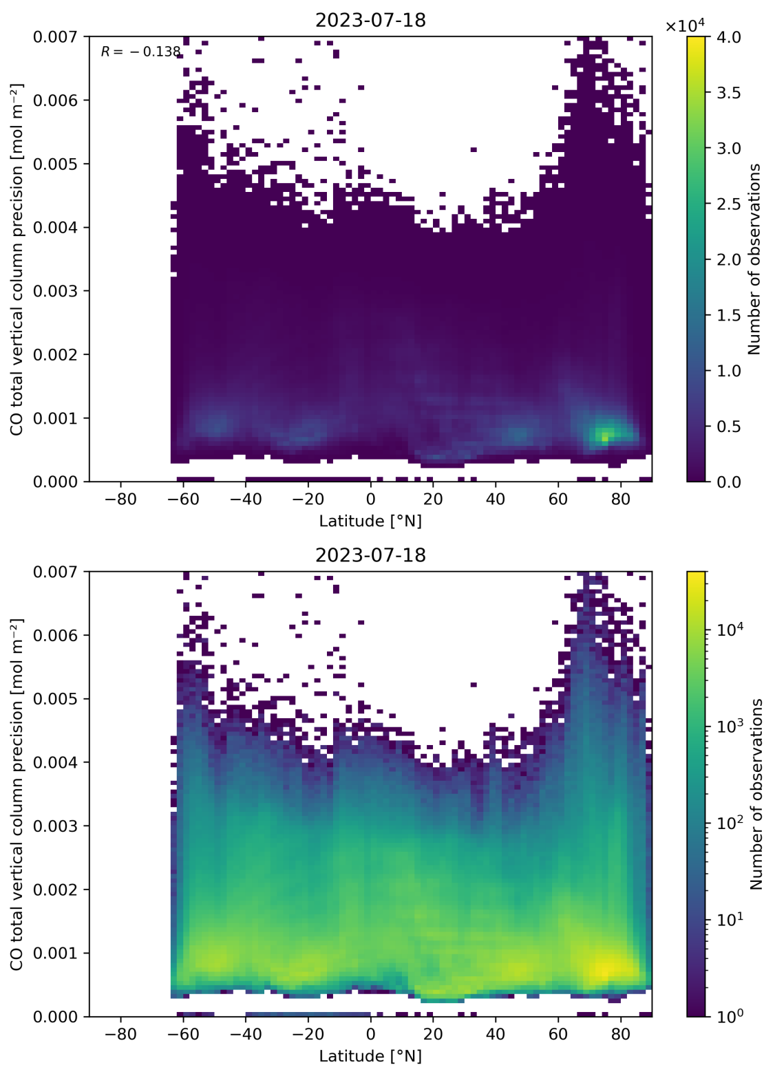
Figure 53: Scatter density plot of “Latitude” against “CO total vertical column precision” for 2023-07-17 to 2023-07-19.
