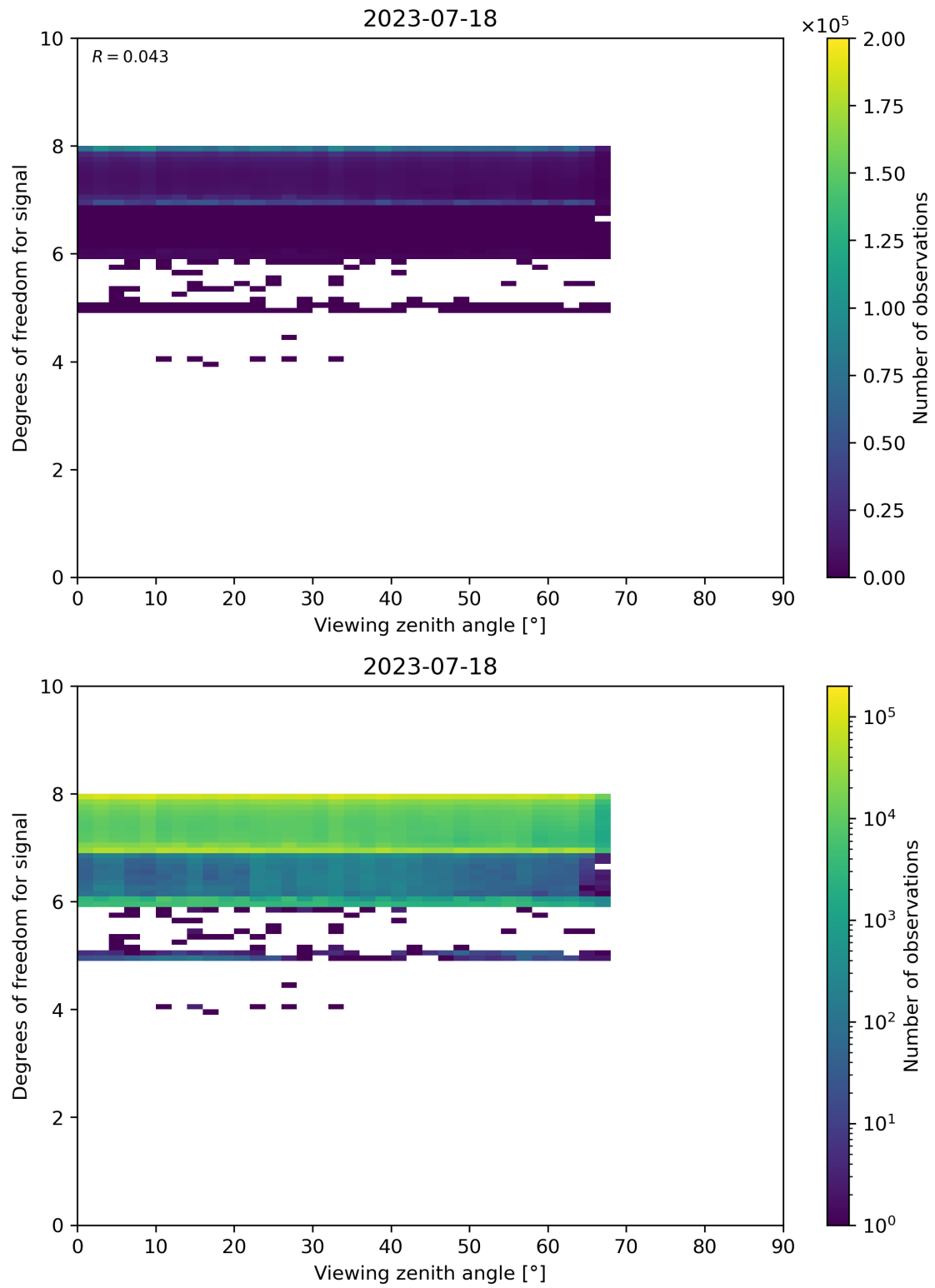
Figure 73: Scatter density plot of “Viewing zenith angle” against “Degrees of freedom for signal” for 2023-07-17 to 2023-07-19.
