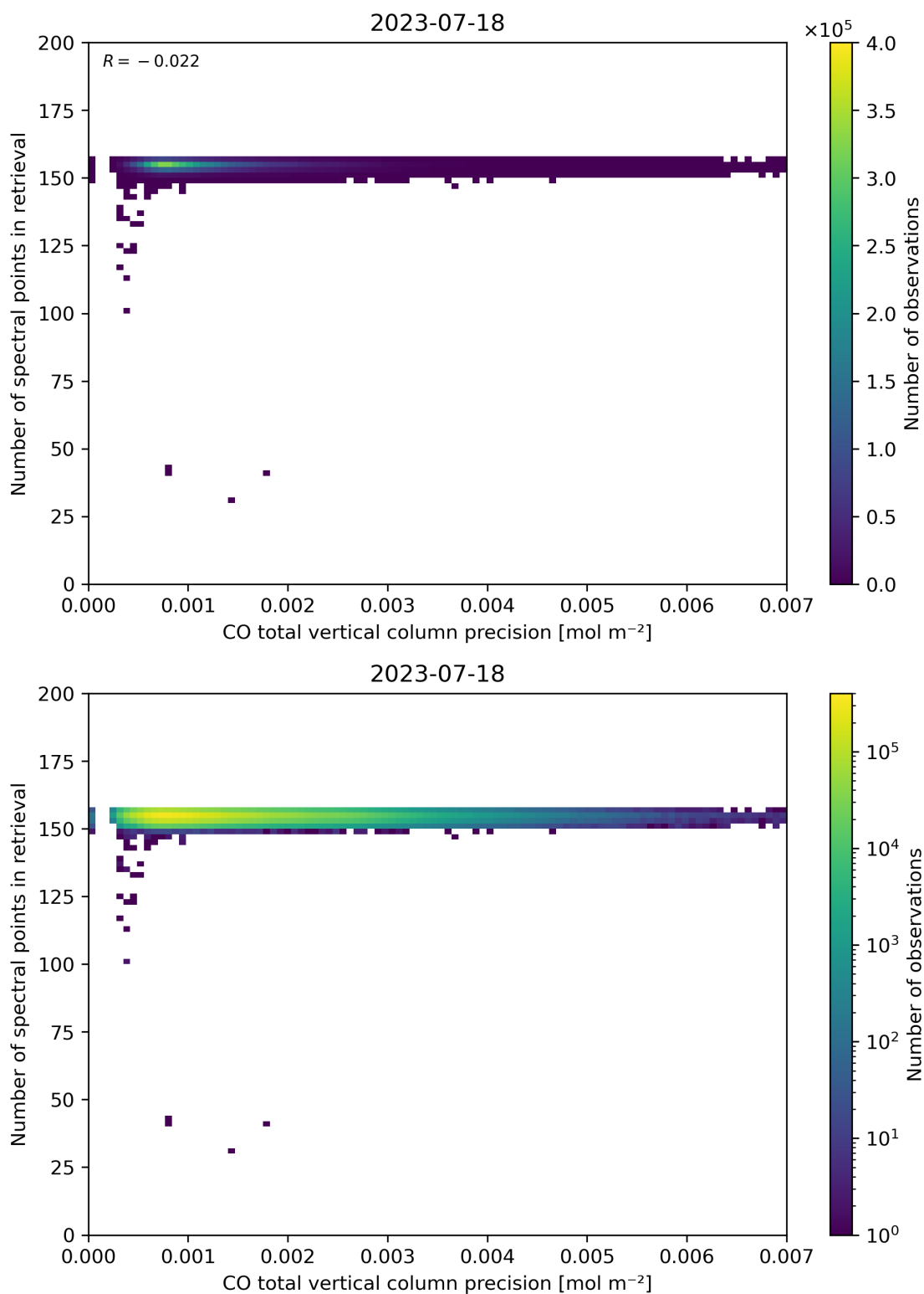
Figure 47: Scatter density plot of “CO total vertical column precision” against “Number of spectral points in retrieval” for 2023-07-17 to 2023-07-19.
