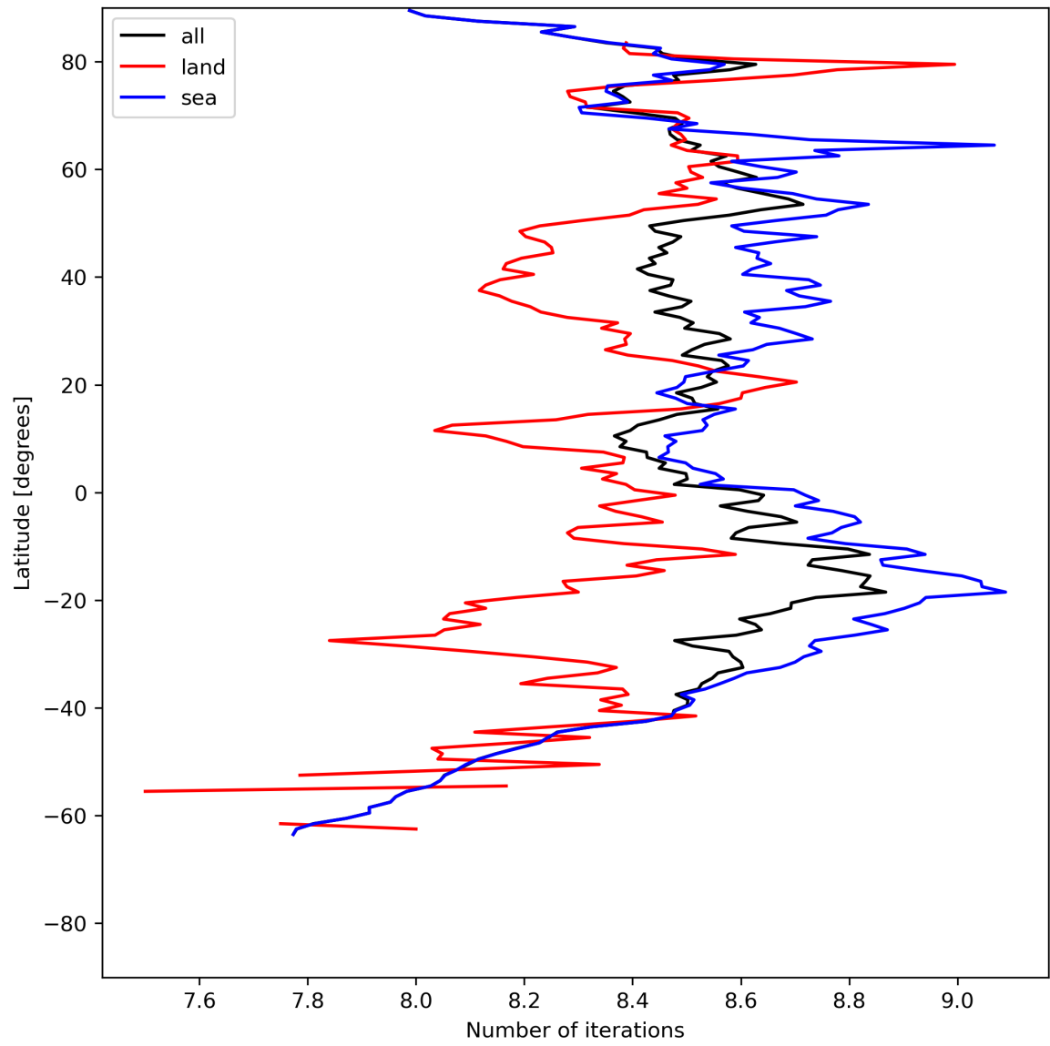
Figure 16: Zonal average of “Number of iterations” for 2023-07-17 to 2023-07-19.
