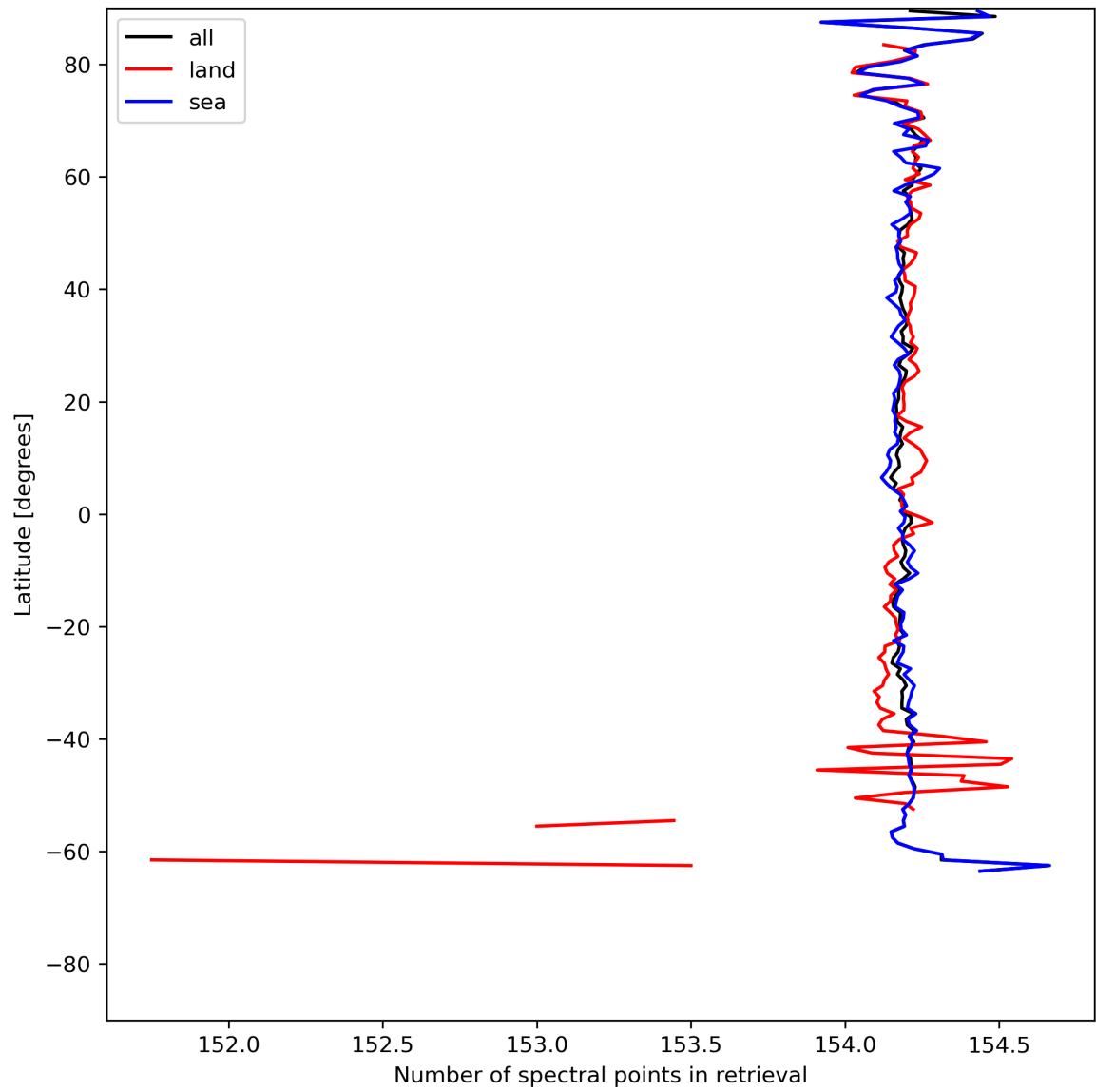
Figure 13: Zonal average of “Number of spectral points in retrieval” for 2023-07-17 to 2023-07-19.
