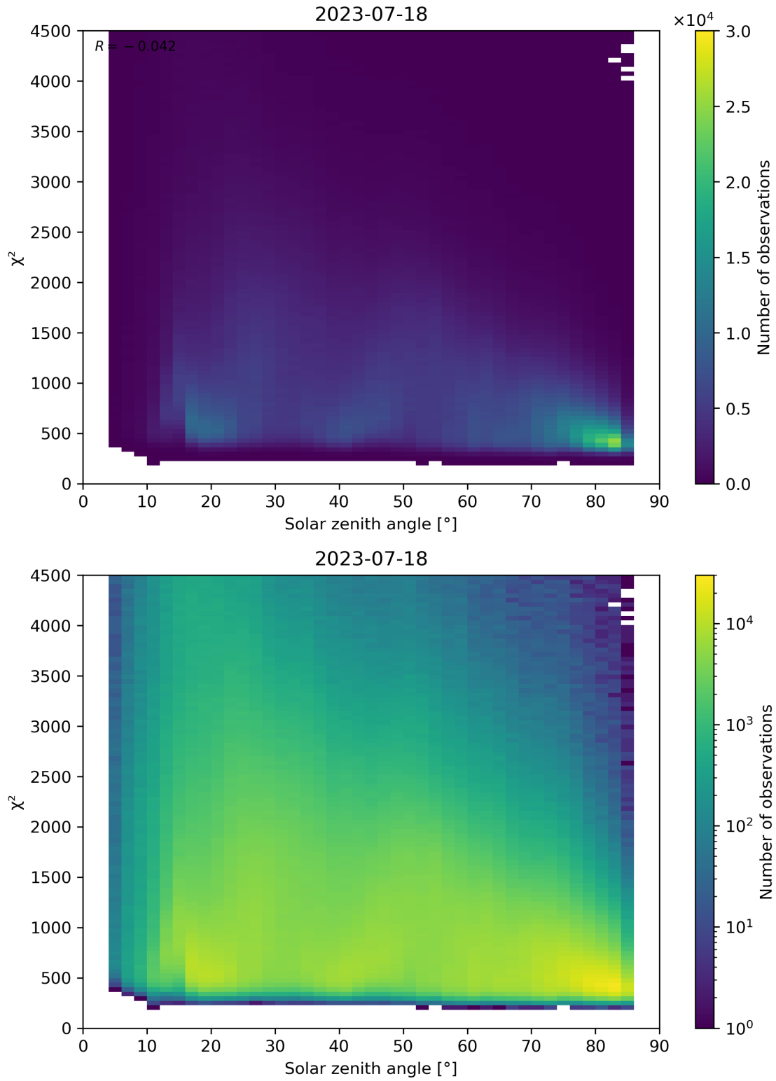
Figure 64: Scatter density plot of “Solar zenith angle” against “ \chi^2 ” for 2023-07-17 to 2023-07-19.
