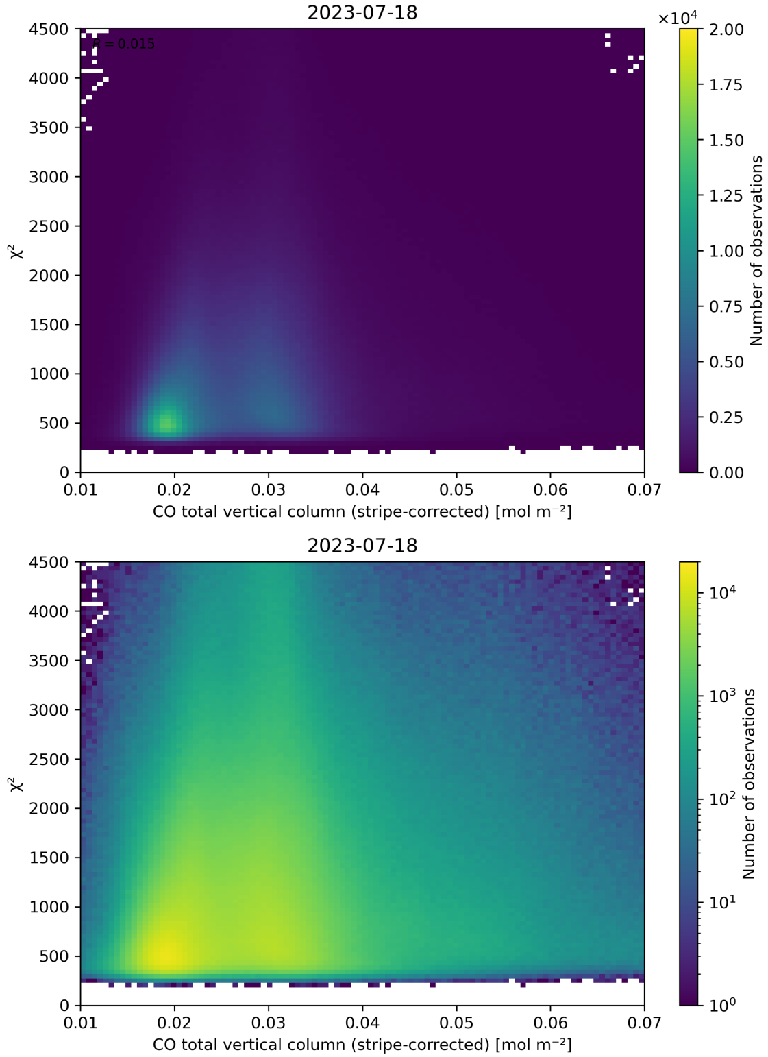
Figure 37: Scatter density plot of “CO total vertical column (stripe-corrected)” against “ \chi^2 ” for 2023-07-17 to 2023-07-19.
