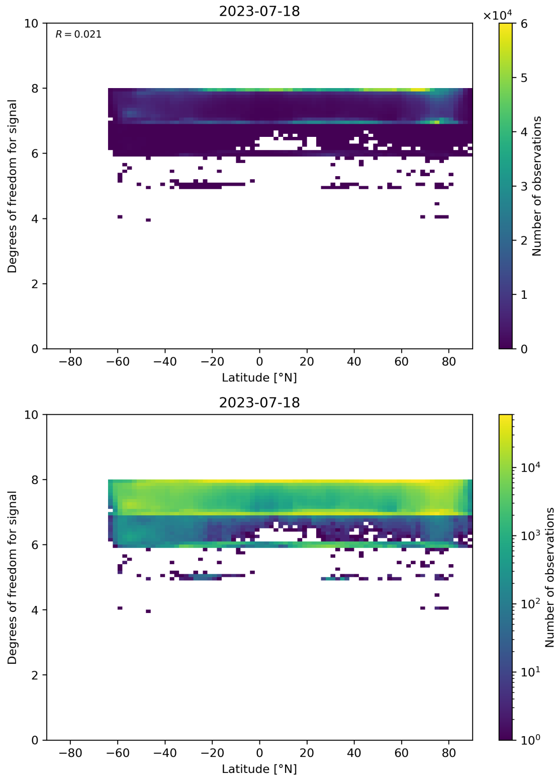
Figure 55: Scatter density plot of “Latitude” against “Degrees of freedom for signal” for 2023-07-17 to 2023-07-19.
