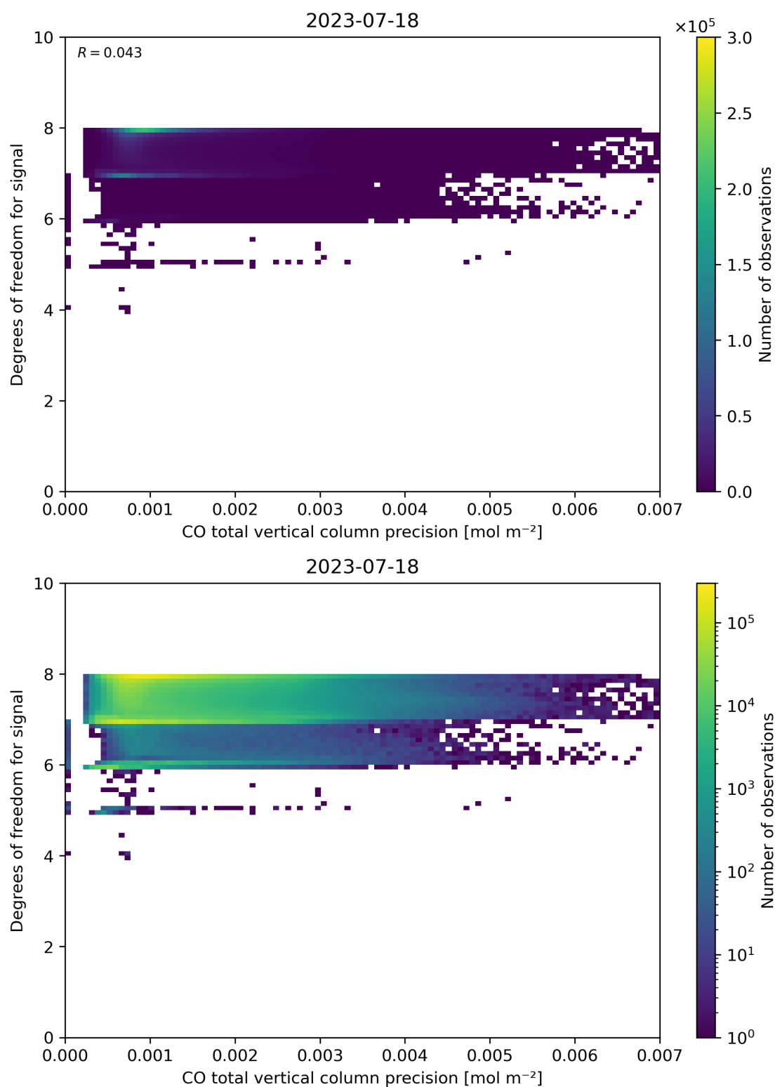
Figure 45: Scatter density plot of “CO total vertical column precision” against “Degrees of freedom for signal” for 2023-07-17 to 2023-07-19.
