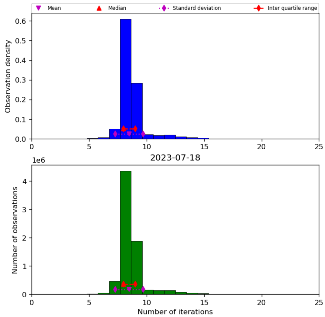
Figure 24: Histogram of “Number of iterations” for 2023-07-17 to 2023-07-19
