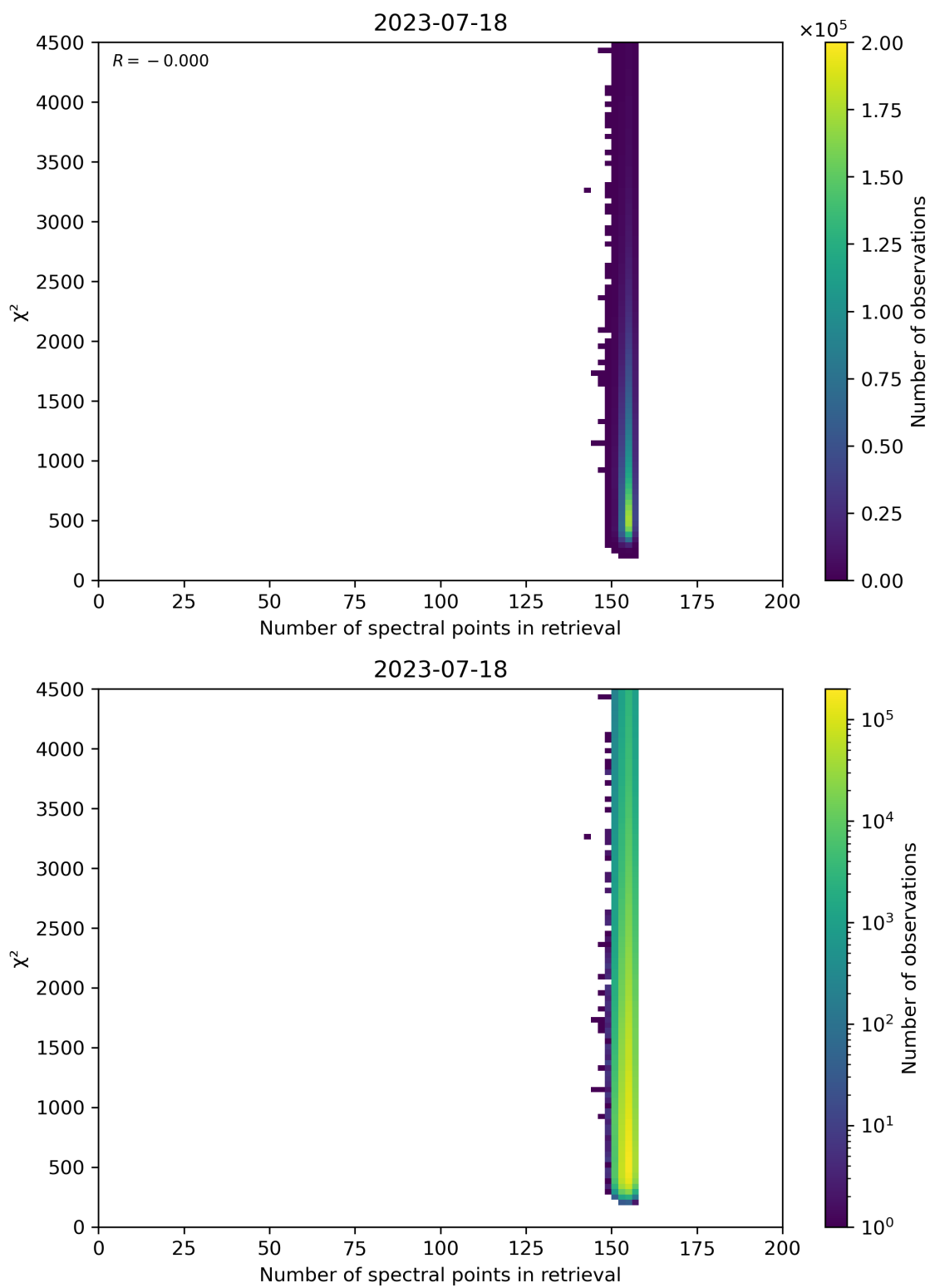
Figure 58: Scatter density plot of “Number of spectral points in retrieval” against “ \chi^2 ” for 2023-07-17 to 2023-07-19.
