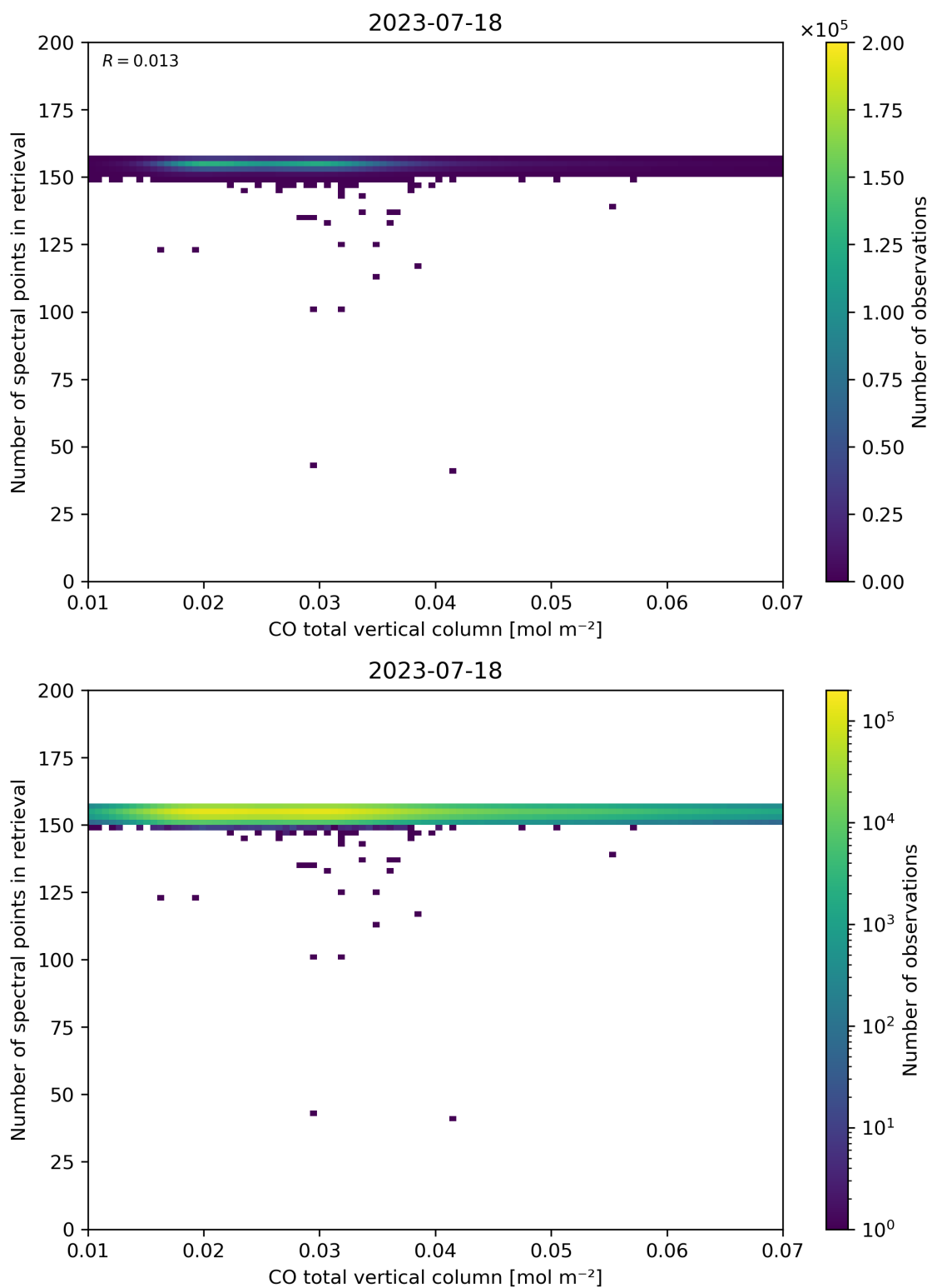
Figure 43: Scatter density plot of “CO total vertical column” against “Number of spectral points in retrieval” for 2023-07-17 to 2023-07-19.
