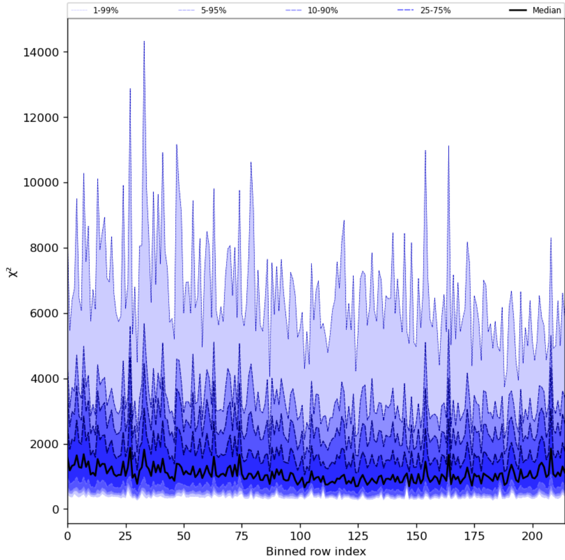
Figure 30: Along track statistics of “ \chi^2 ” for 2023-07-17 to 2023-07-19
