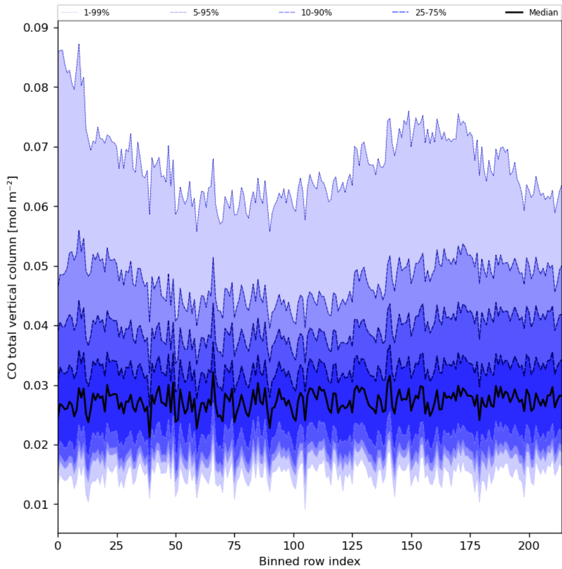
Figure 26: Along track statistics of “CO total vertical column” for 2023-07-17 to 2023-07-19
