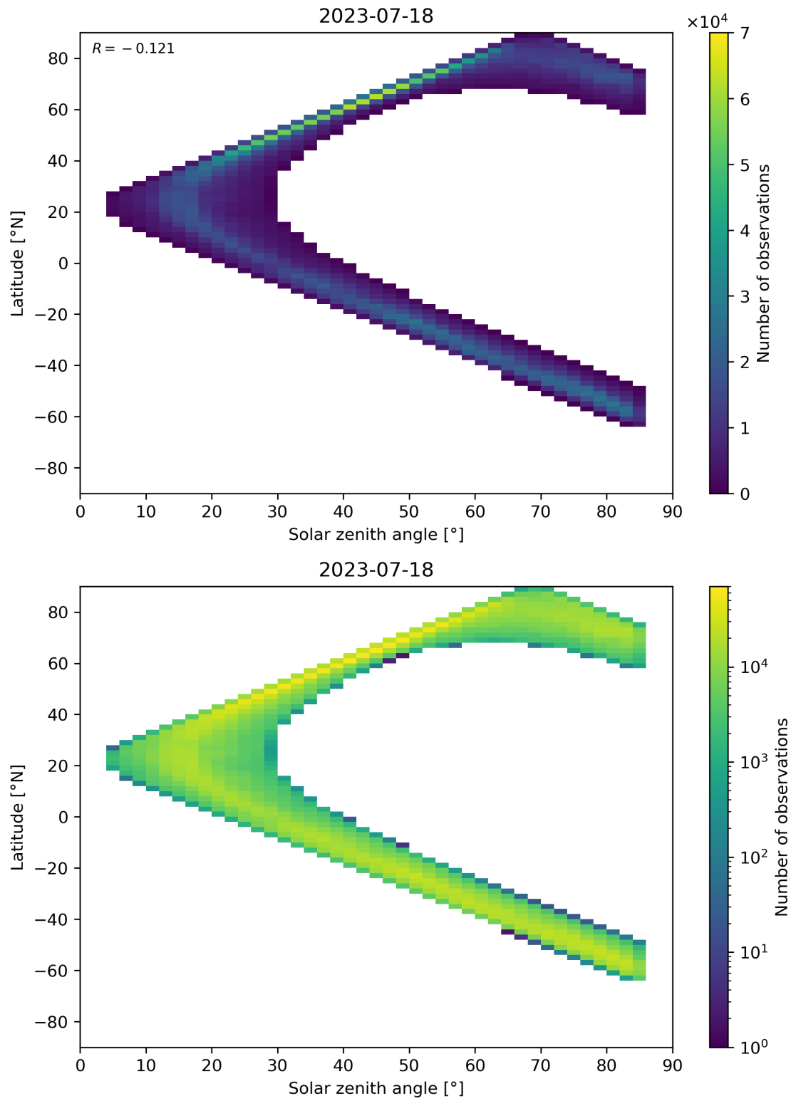
Figure 66: Scatter density plot of “Solar zenith angle” against “Latitude” for 2023-07-17 to 2023-07-19.
