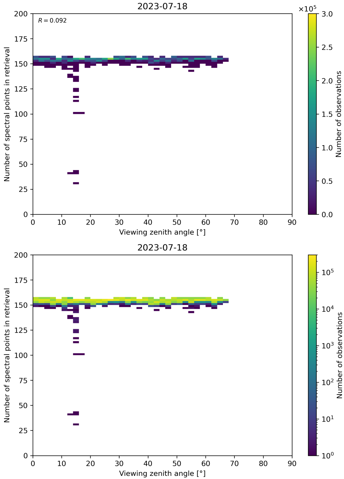
Figure 76: Scatter density plot of “Viewing zenith angle” against “Number of spectral points in retrieval” for 2023-07-17 to 2023-07-19.
