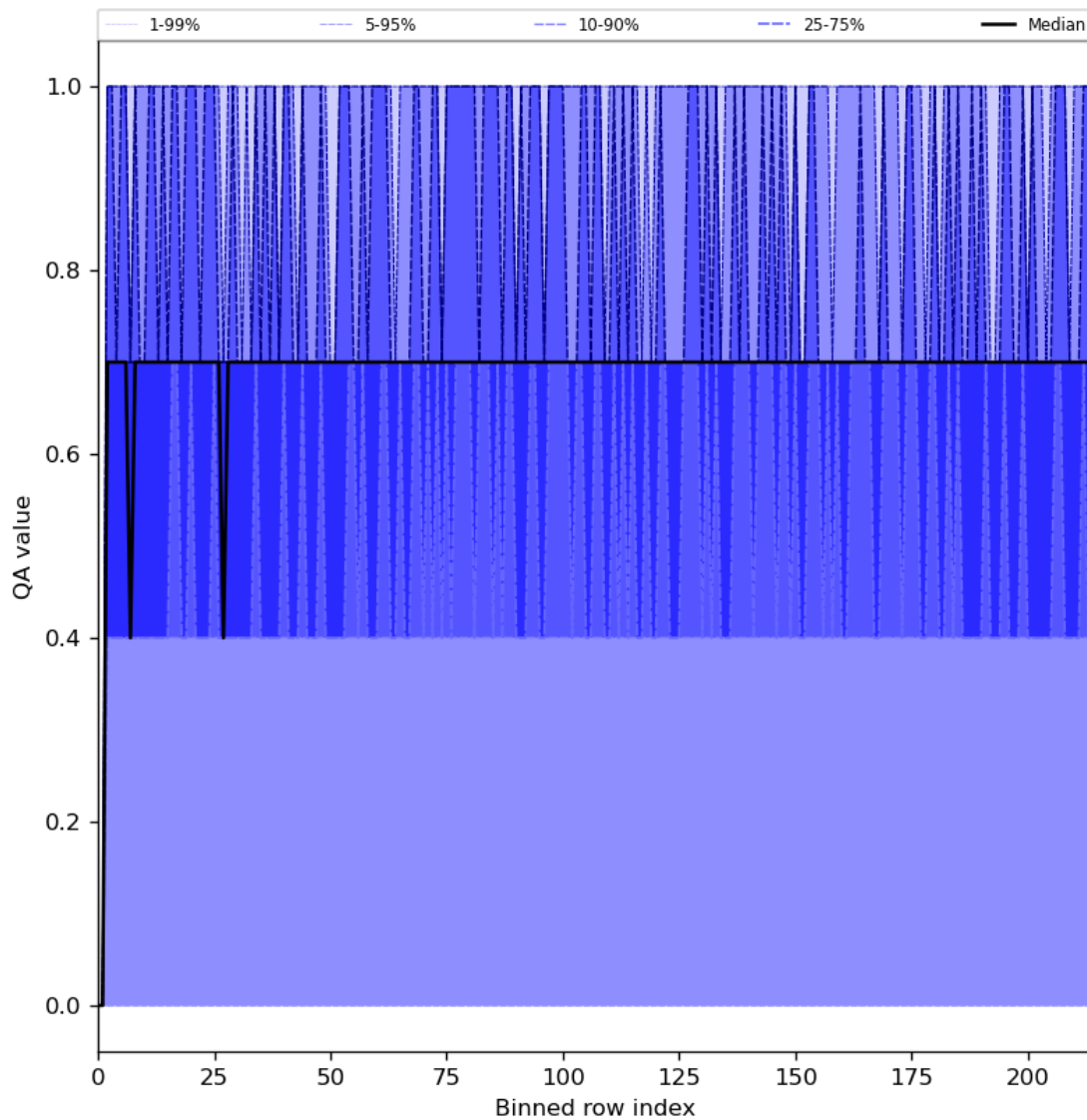
Figure 25: Along track statistics of “QA value” for 2023-07-17 to 2023-07-19
