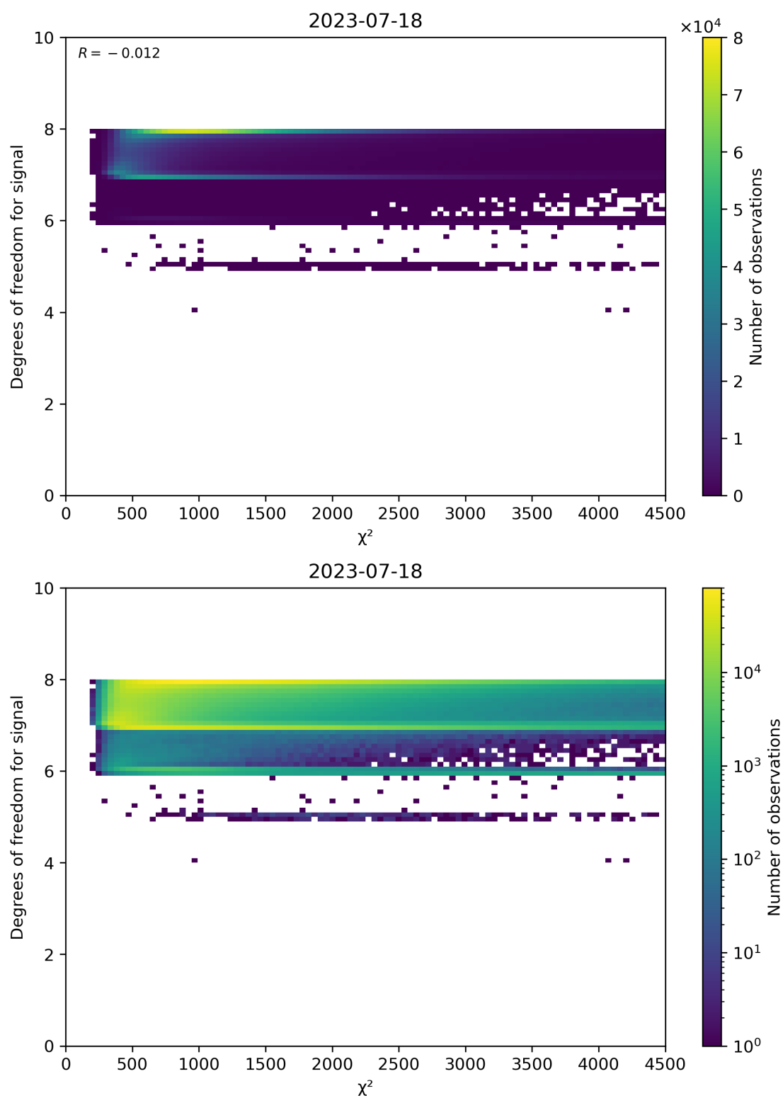
Figure 48: Scatter density plot of " \chi^2 " against "Degrees of freedom for signal" for 2023-07-17 to 2023-07-19.
