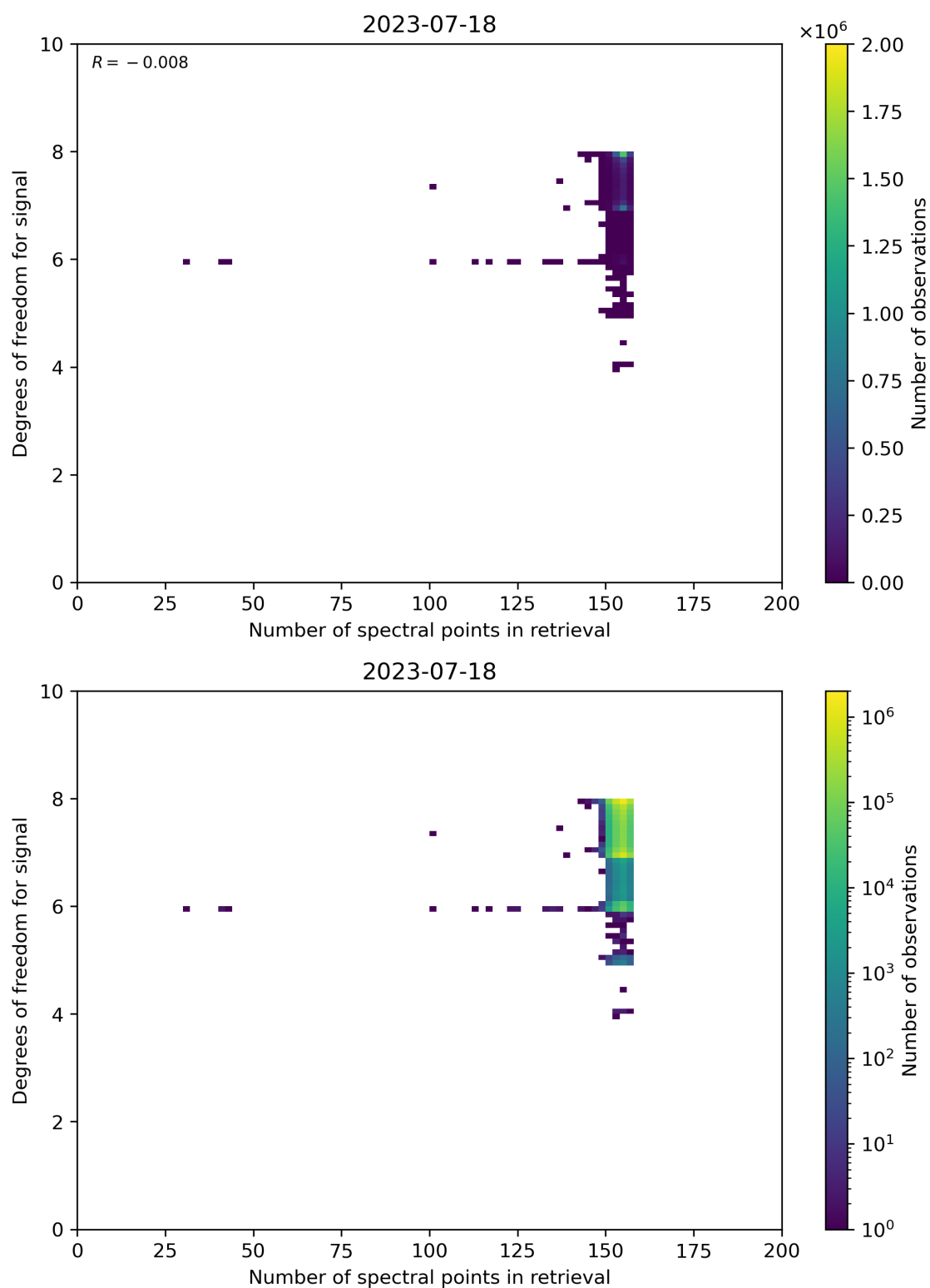
Figure 59: Scatter density plot of “Number of spectral points in retrieval” against “Degrees of freedom for signal” for 2023-07-17 to 2023-07-19.
