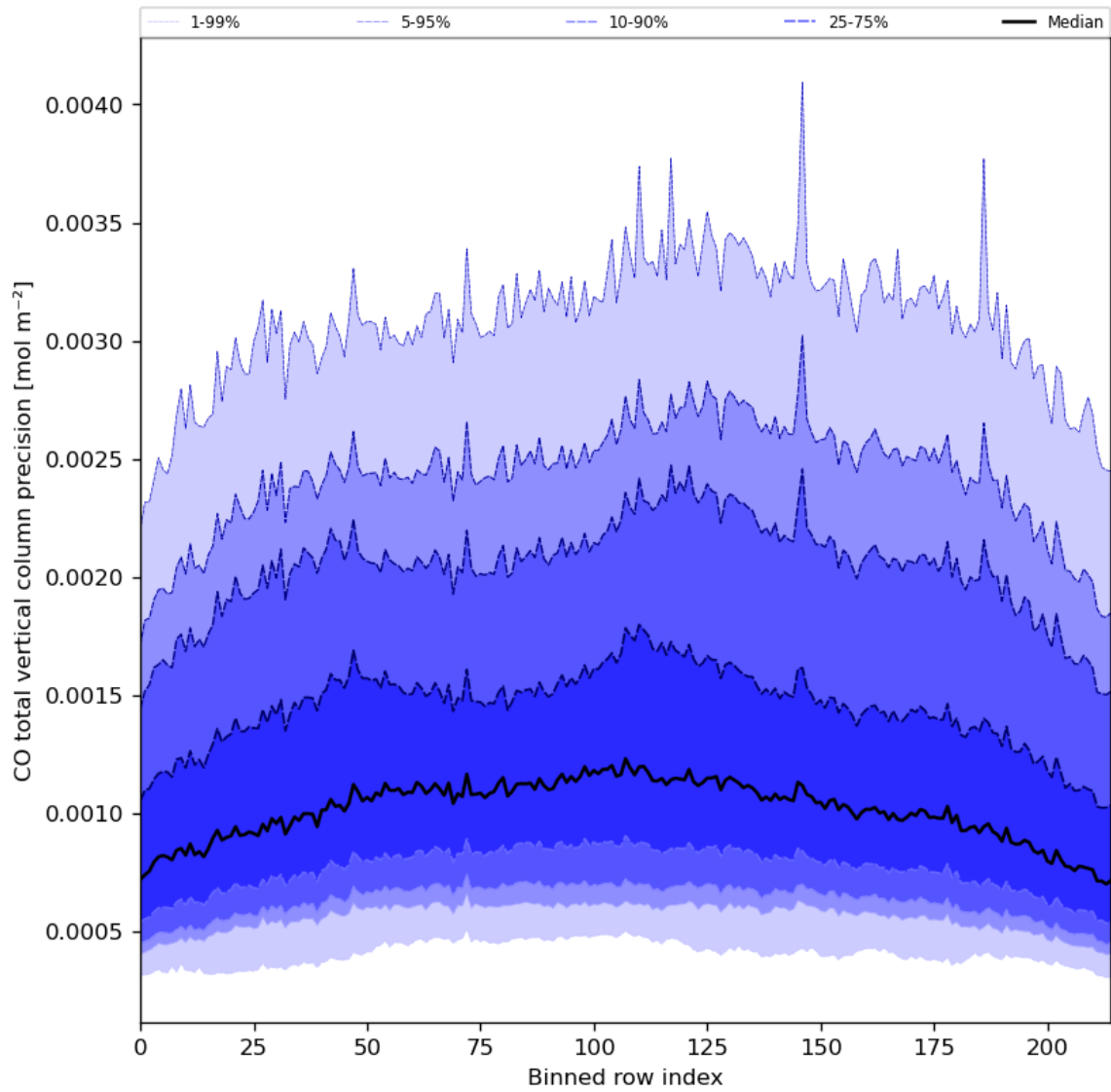
Figure 28: Along track statistics of “CO total vertical column precision” for 2023-07-17 to 2023-07-19
