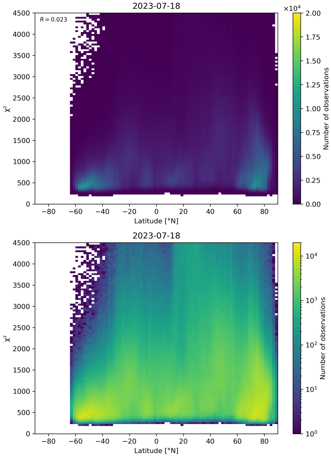
Figure 54: Scatter density plot of “Latitude” against “ \chi^2 ” for 2023-07-17 to 2023-07-19.
