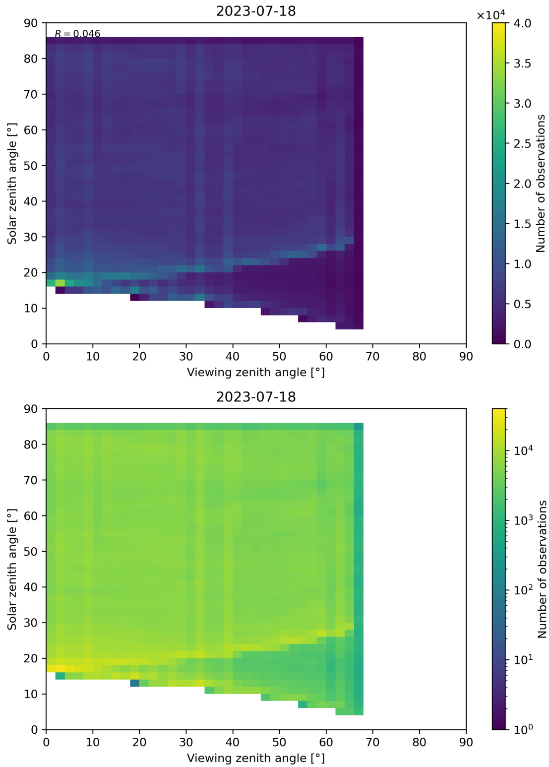
Figure 77: Scatter density plot of “Viewing zenith angle” against “Solar zenith angle” for 2023-07-17 to 2023-07-19.
