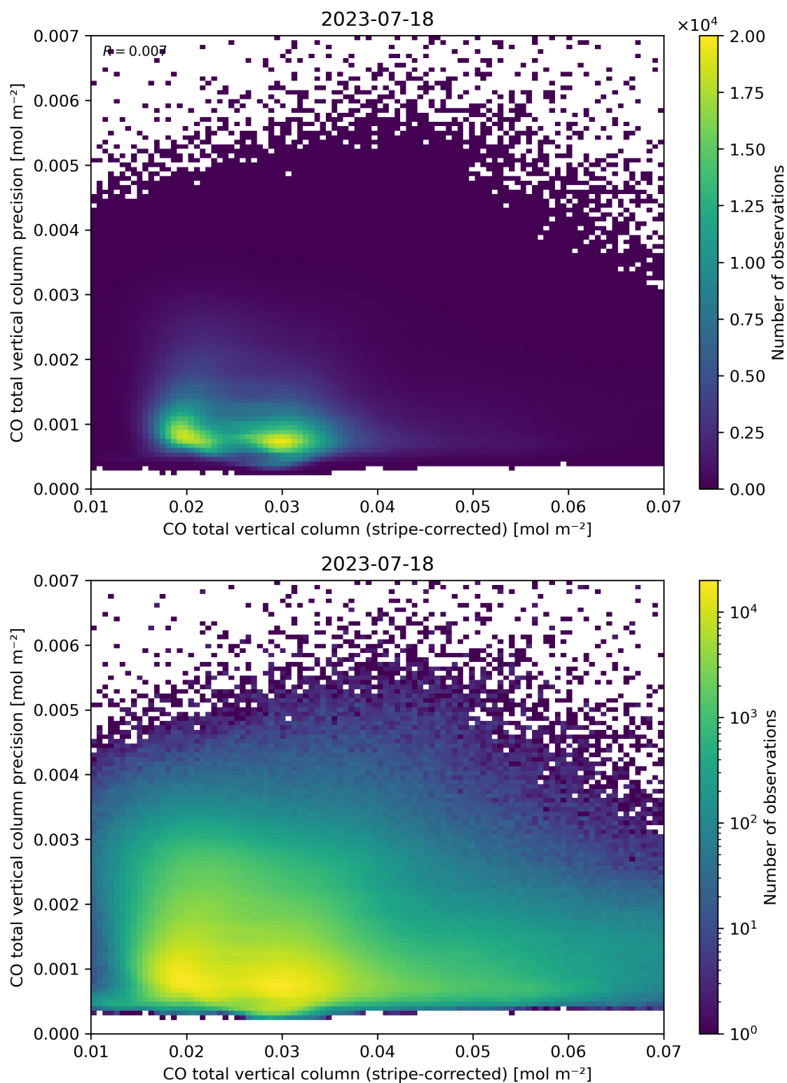
Figure 36: Scatter density plot of “CO total vertical column (stripe-corrected)” against “CO total vertical column precision” for 2023-07-17 to 2023-07-19.
