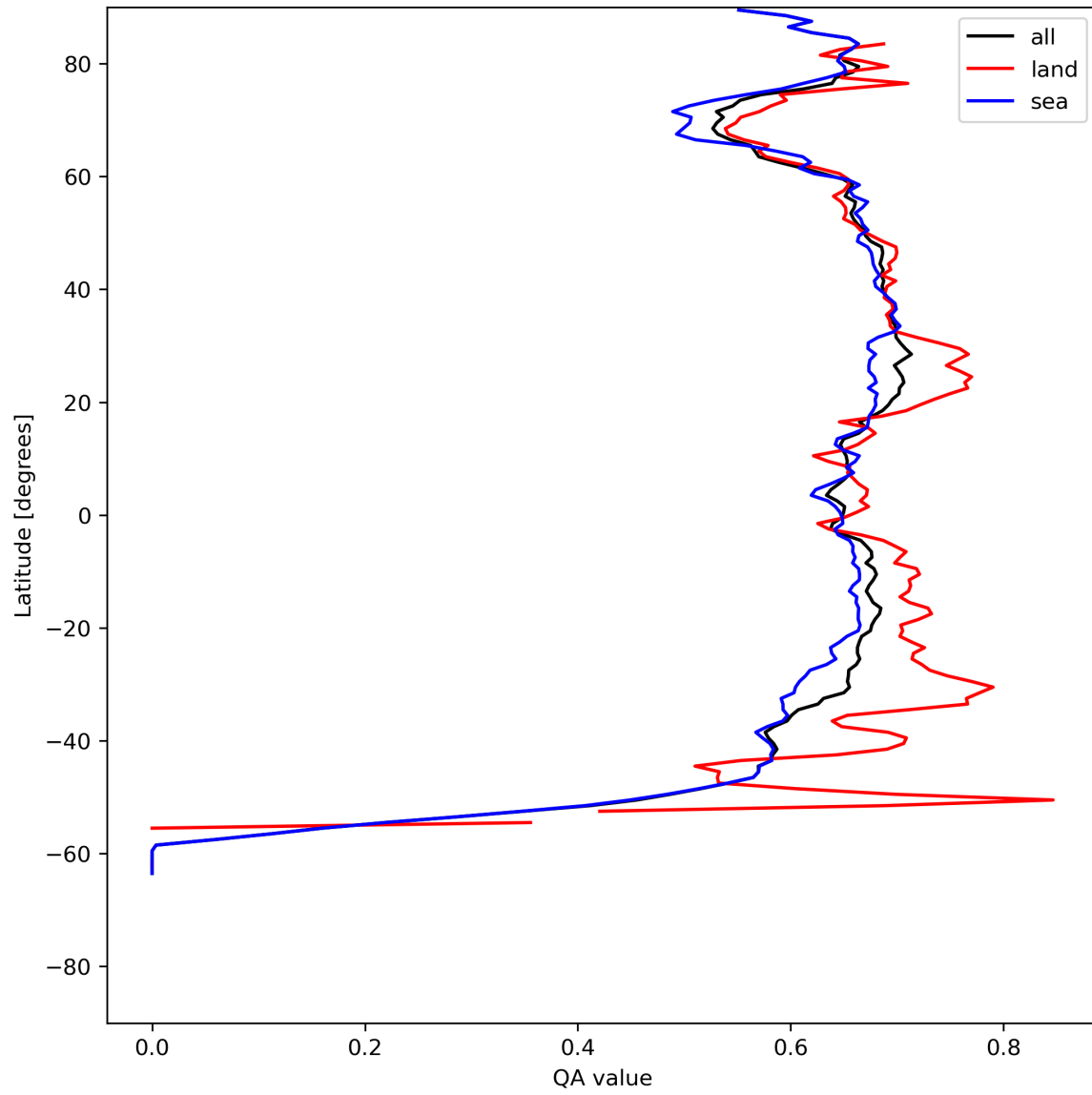
Figure 9: Zonal average of “QA value” for 2023-07-17 to 2023-07-19.
