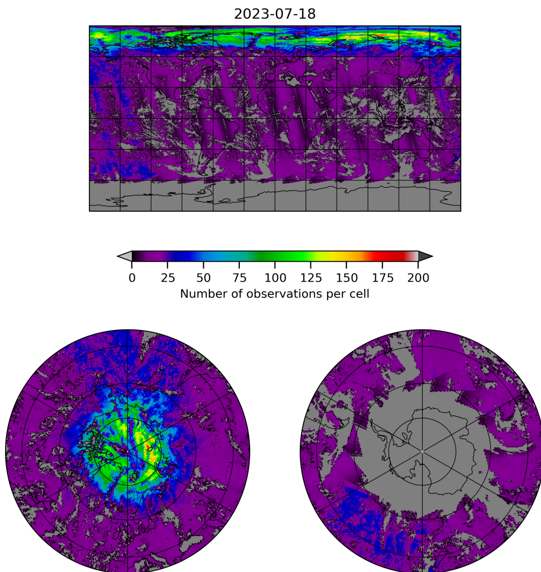
Figure 8: Map of the number of observations for 2023-07-17 to 2023-07-19
