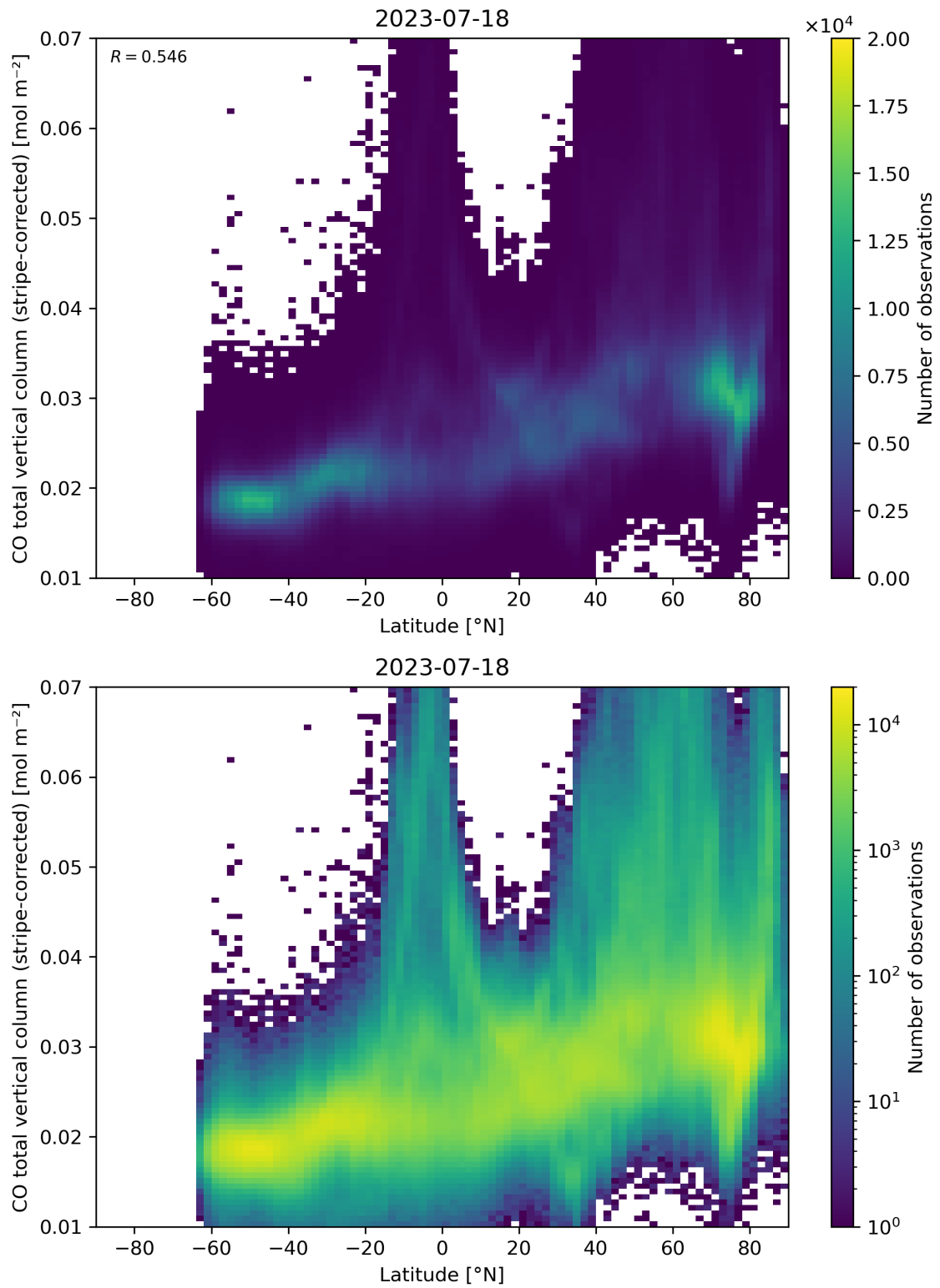
Figure 52: Scatter density plot of “Latitude” against “CO total vertical column (stripe-corrected)” for 2023-07-17 to 2023-07-19.
