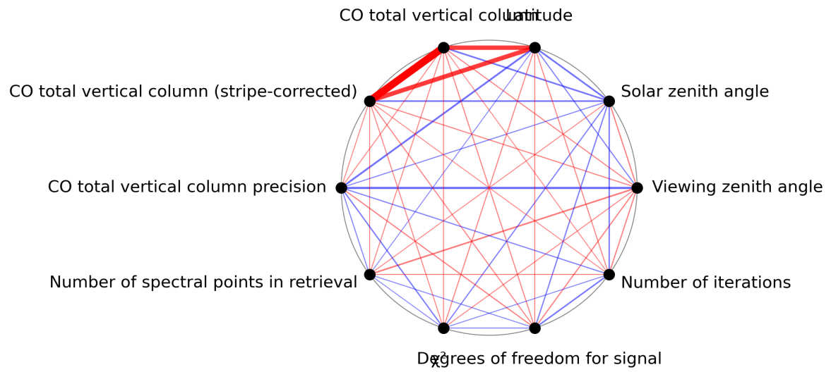
Figure 1: Map of correlation graph for 2023-07-17 to 2023-07-19.
