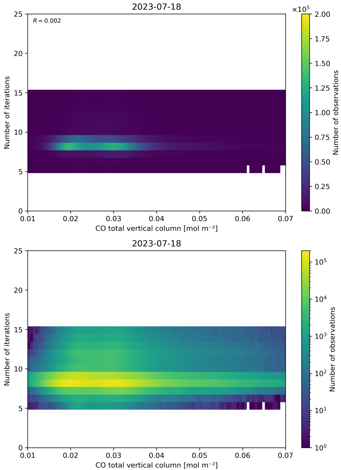
Figure 42: Scatter density plot of “CO total vertical column” against “Number of iterations” for 2023-07-17 to 2023-07-19.
