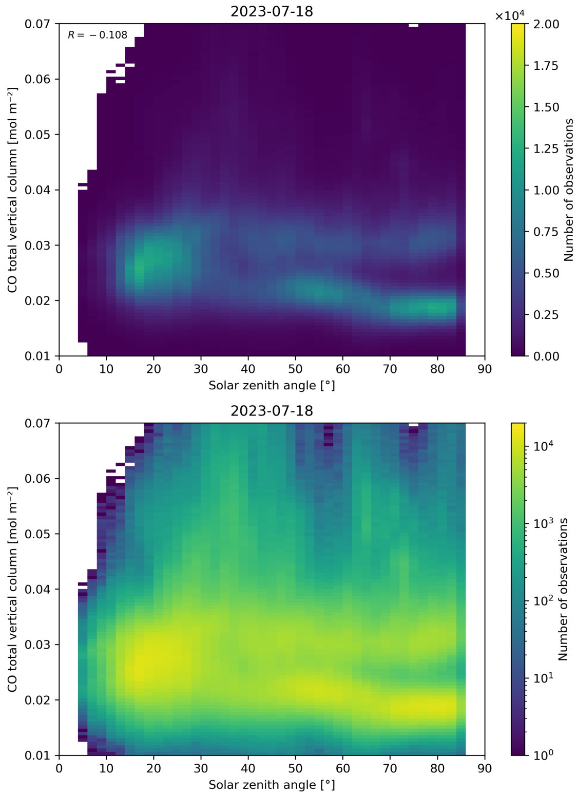
Figure 61: Scatter density plot of “Solar zenith angle” against “CO total vertical column” for 2023-07-17 to 2023-07-19.
