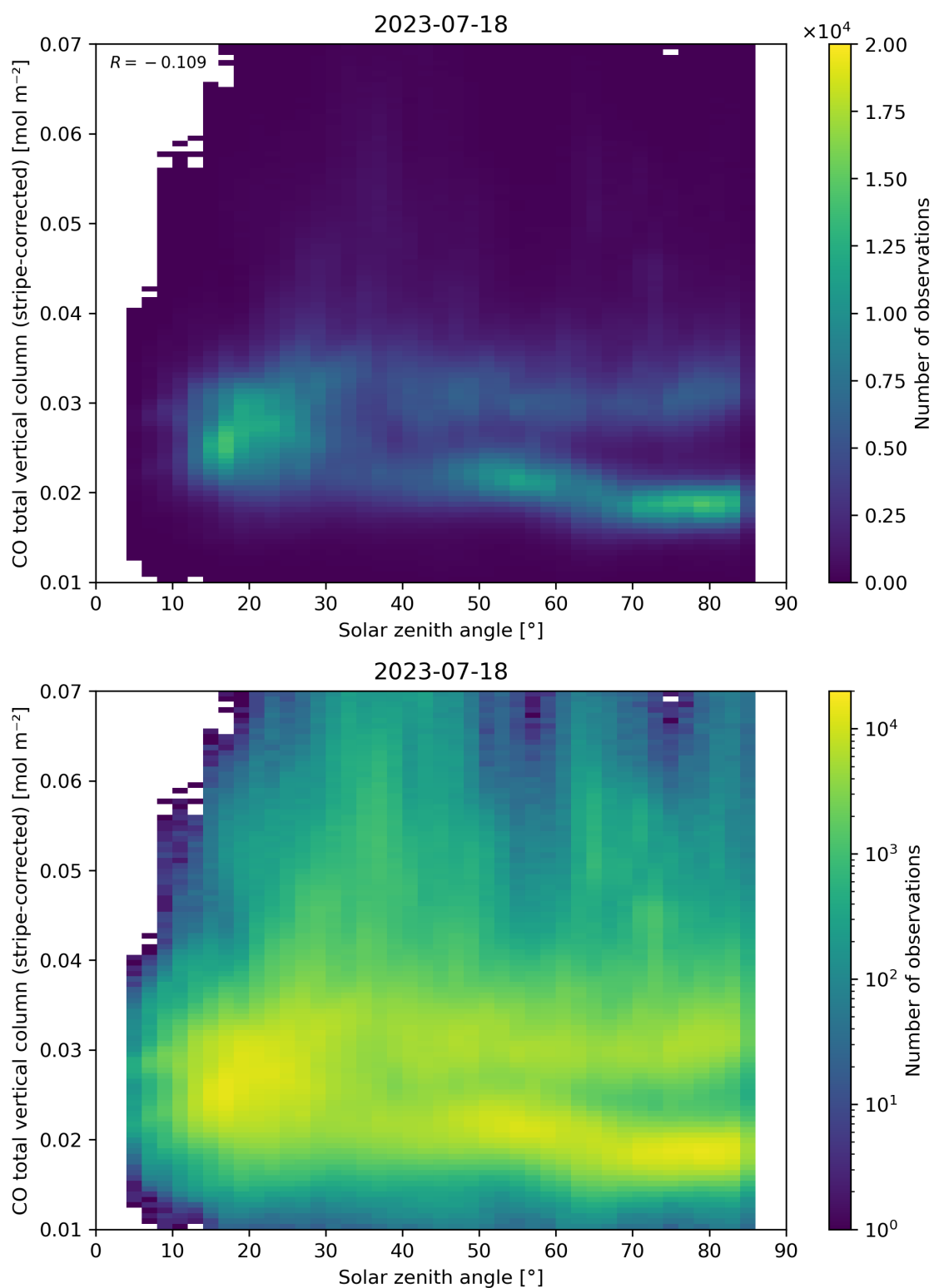
Figure 62: Scatter density plot of “Solar zenith angle” against “CO total vertical column (stripe-corrected)” for 2023-07-17 to 2023-07-19.
