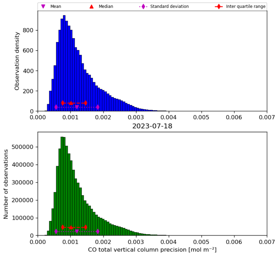
Figure 20: Histogram of “CO total vertical column precision” for 2023-07-17 to 2023-07-19
