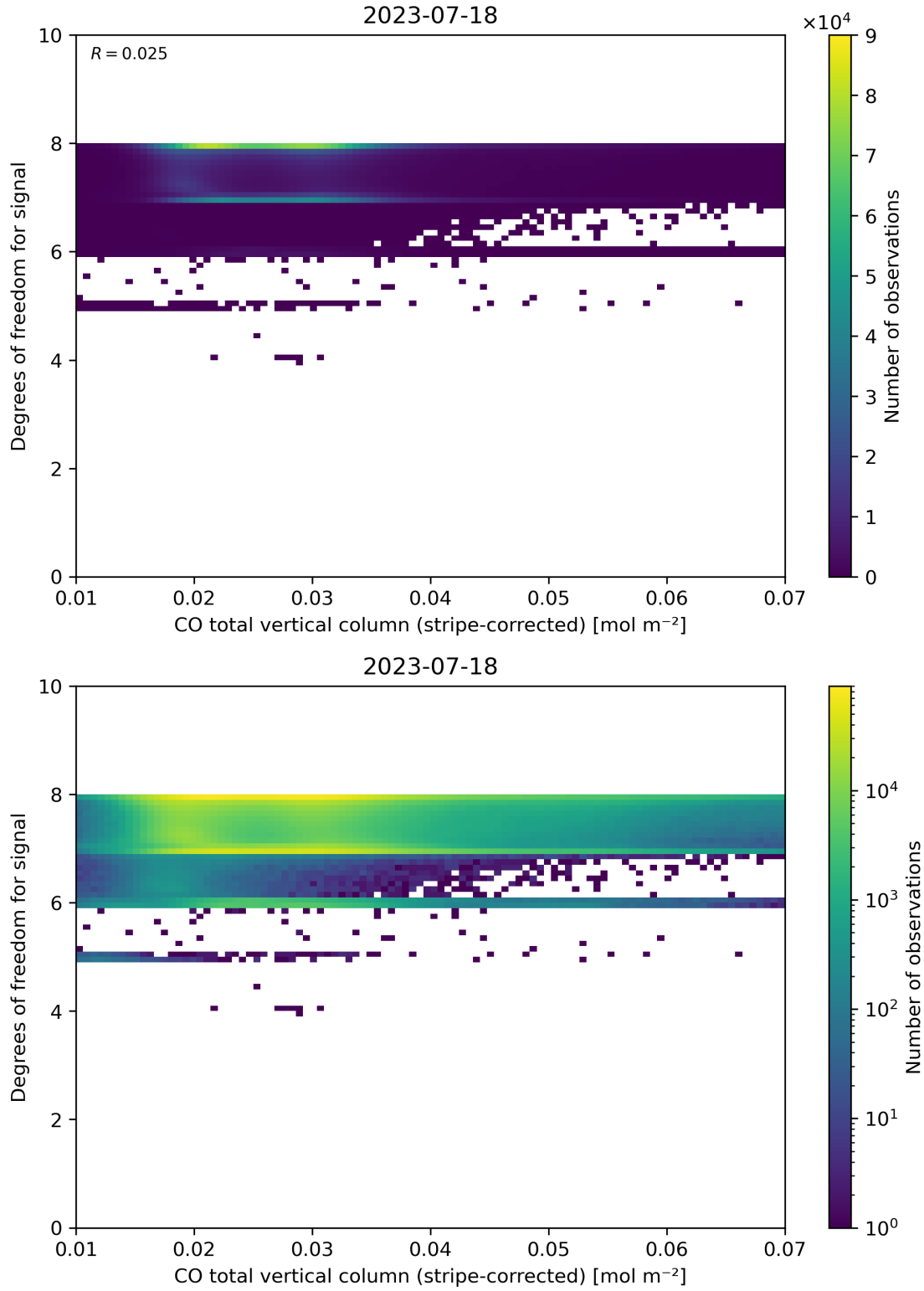
Figure 38: Scatter density plot of “CO total vertical column (stripe-corrected)” against “Degrees of freedom for signal” for 2023-07-17 to 2023-07-19.
