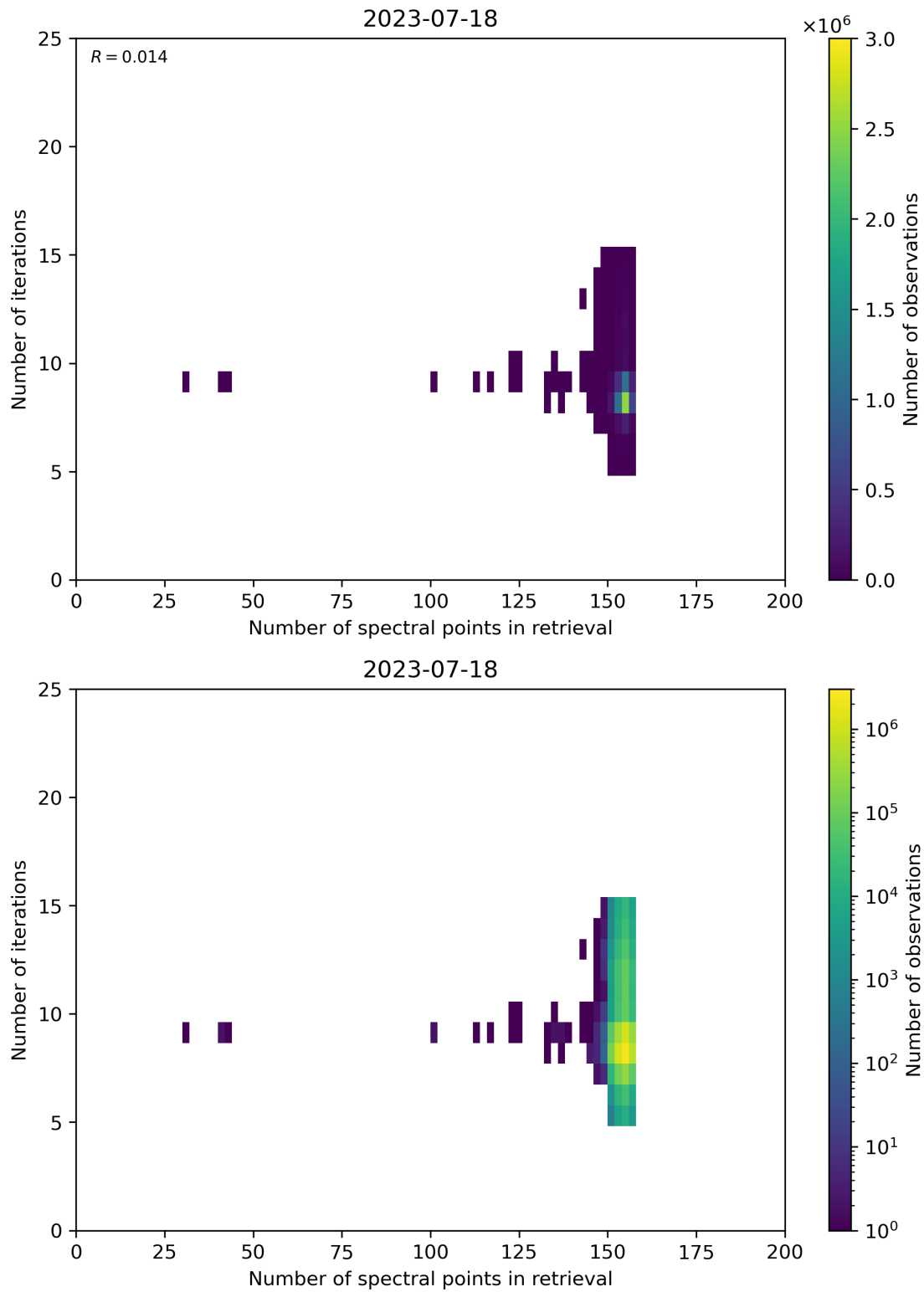
Figure 60: Scatter density plot of “Number of spectral points in retrieval” against “Number of iterations” for 2023-07-17 to 2023-07-19.
