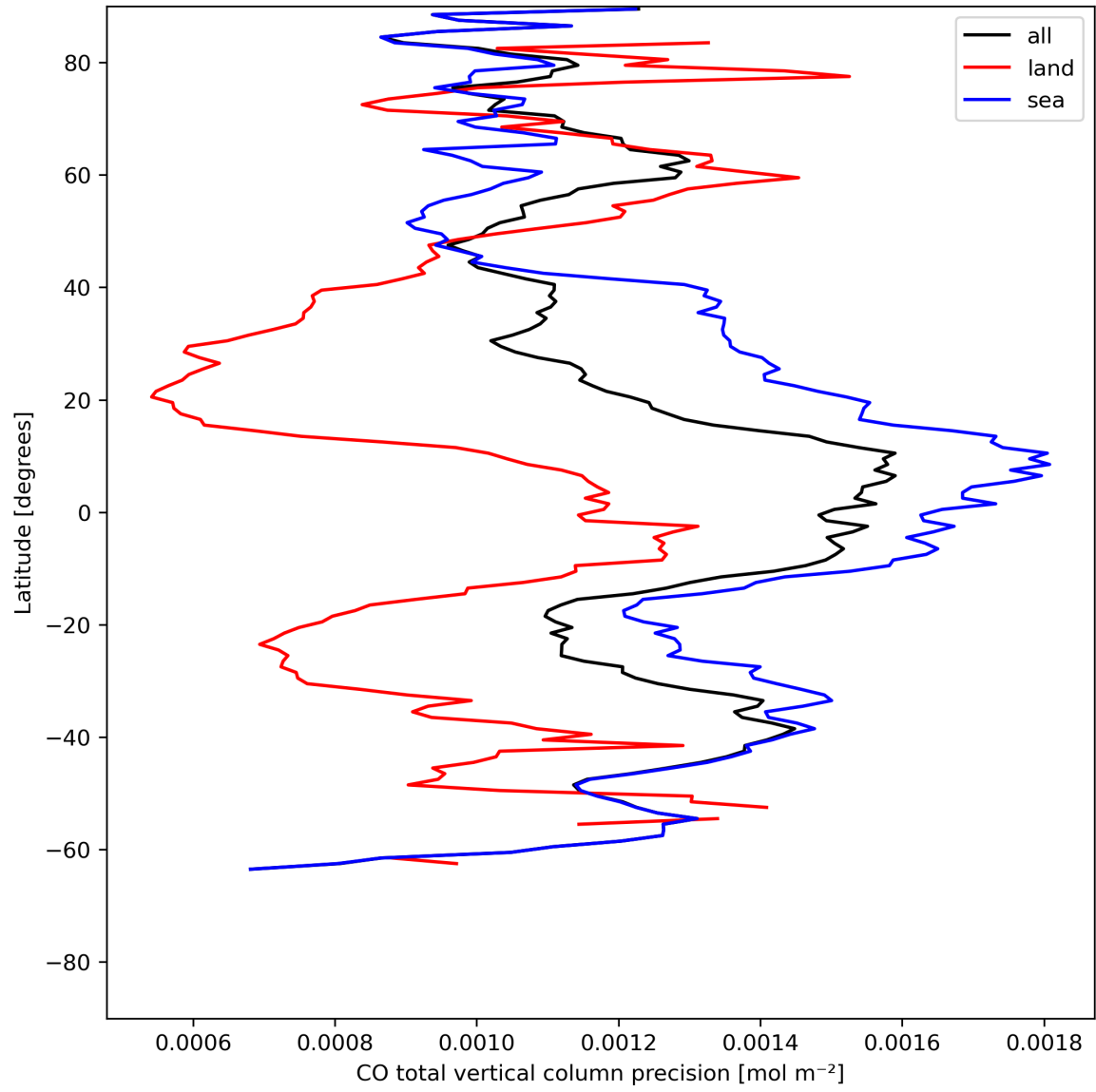
Figure 12: Zonal average of “CO total vertical column precision” for 2023-07-17 to 2023-07-19.
