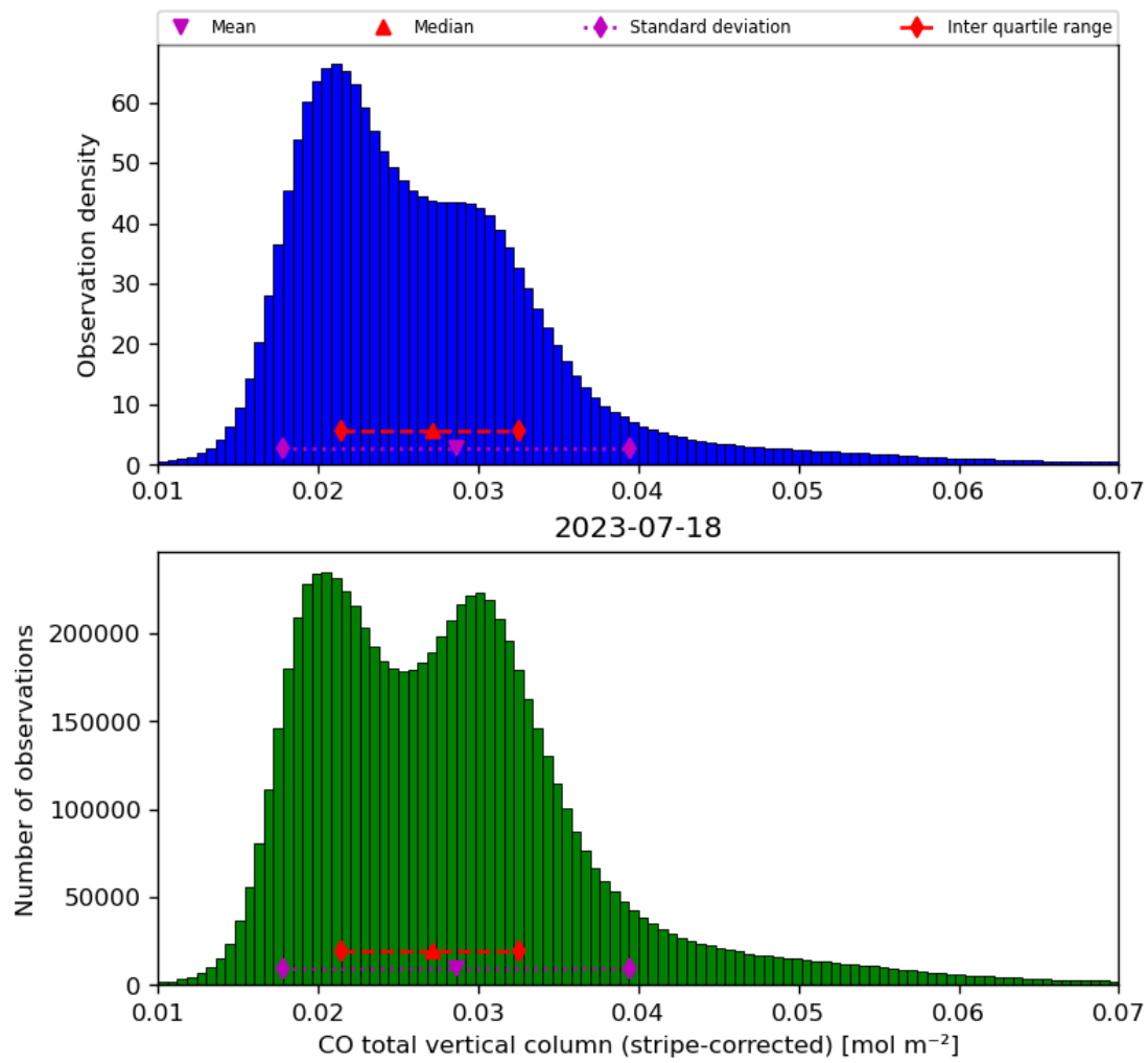
Figure 19: Histogram of “CO total vertical column (stripe-corrected)” for 2023-07-17 to 2023-07-19
