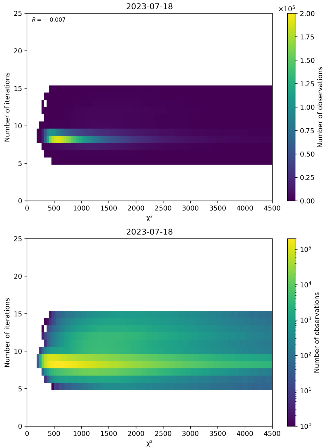
Figure 49: Scatter density plot of “ \chi^2 ” against “Number of iterations” for 2023-07-17 to 2023-07-19.
