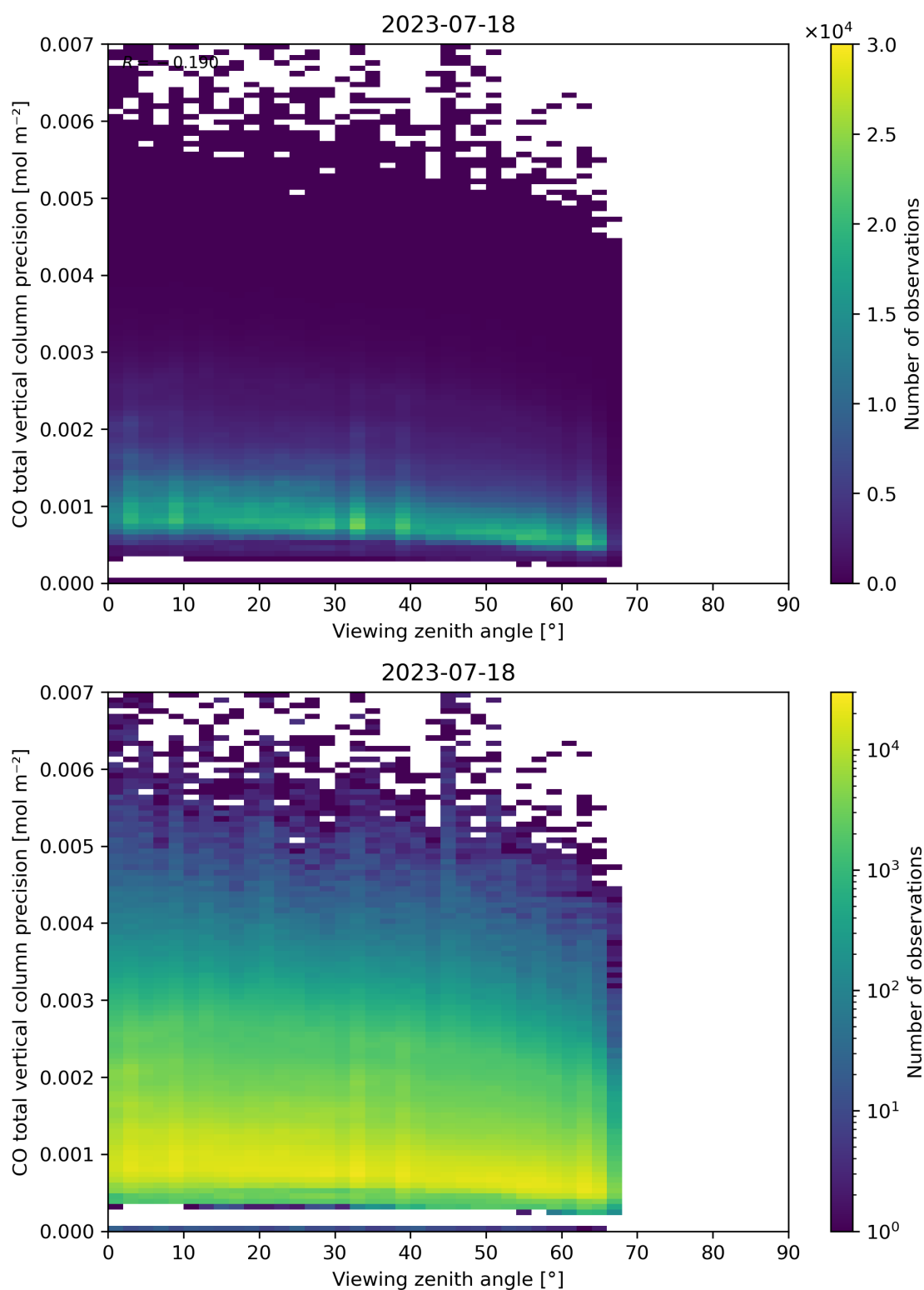
Figure 71: Scatter density plot of “Viewing zenith angle” against “CO total vertical column precision” for 2023-07-17 to 2023-07-19.
