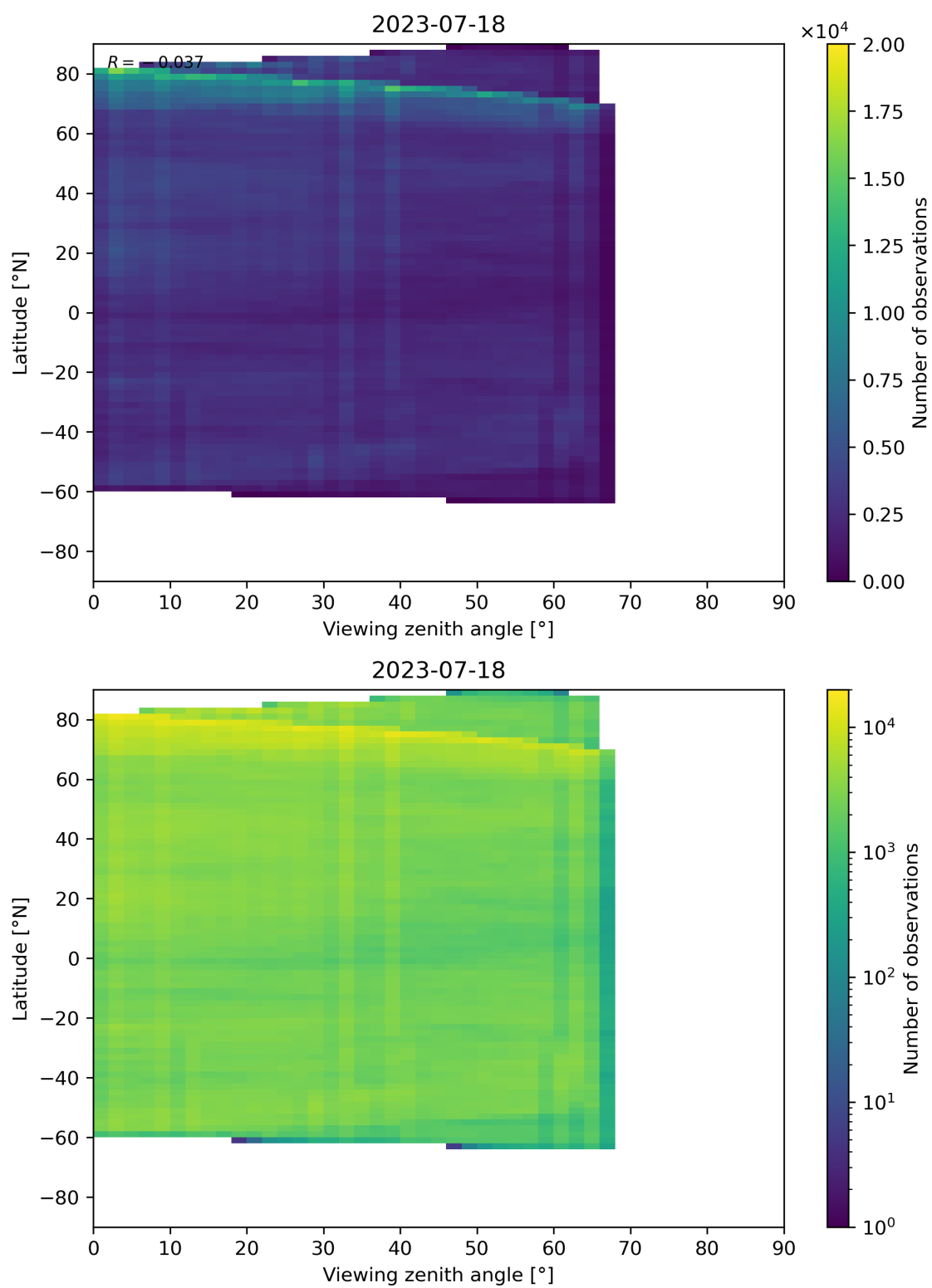
Figure 74: Scatter density plot of “Viewing zenith angle” against “Latitude” for 2023-07-17 to 2023-07-19.
