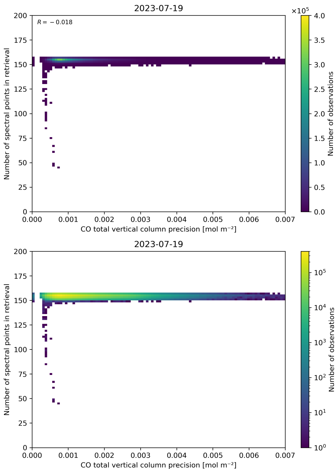
Figure 47: Scatter density plot of “CO total vertical column precision” against “Number of spectral points in retrieval” for 2023-07-19 to 2023-07-20.
