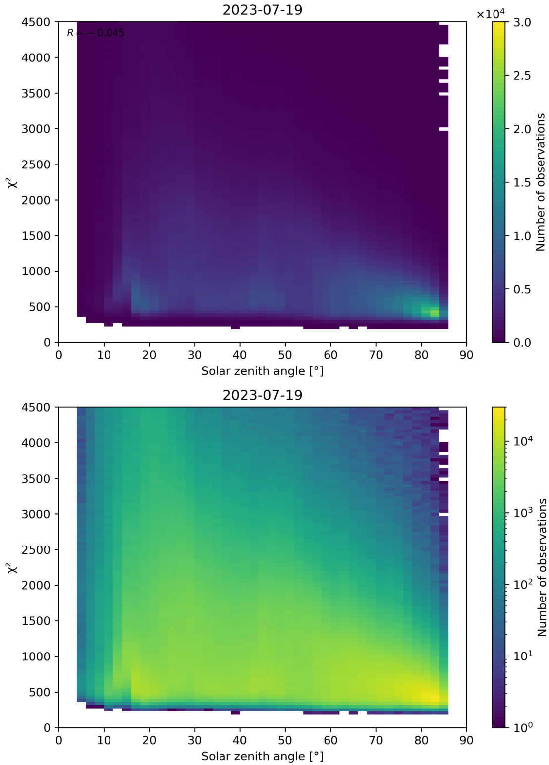
Figure 64: Scatter density plot of “Solar zenith angle” against “ \chi^2 ” for 2023-07-19 to 2023-07-20.
