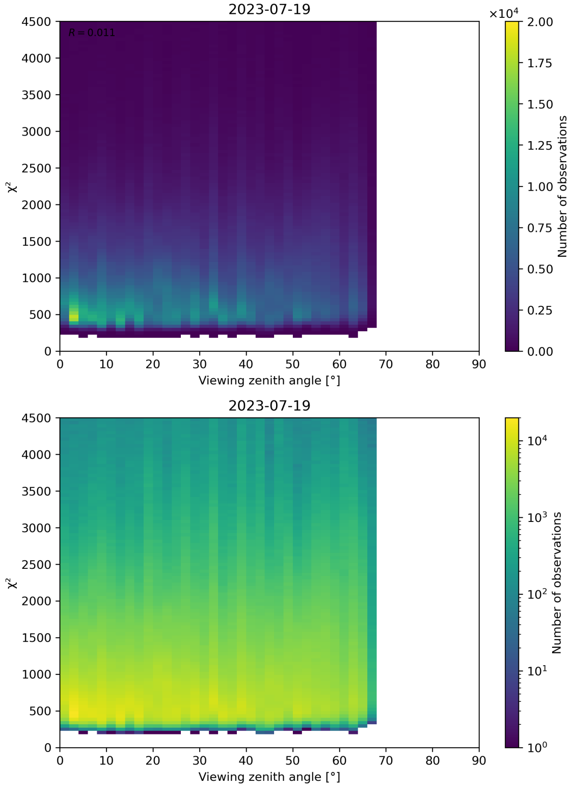
Figure 72: Scatter density plot of “Viewing zenith angle” against “ \chi^2 ” for 2023-07-19 to 2023-07-20.
