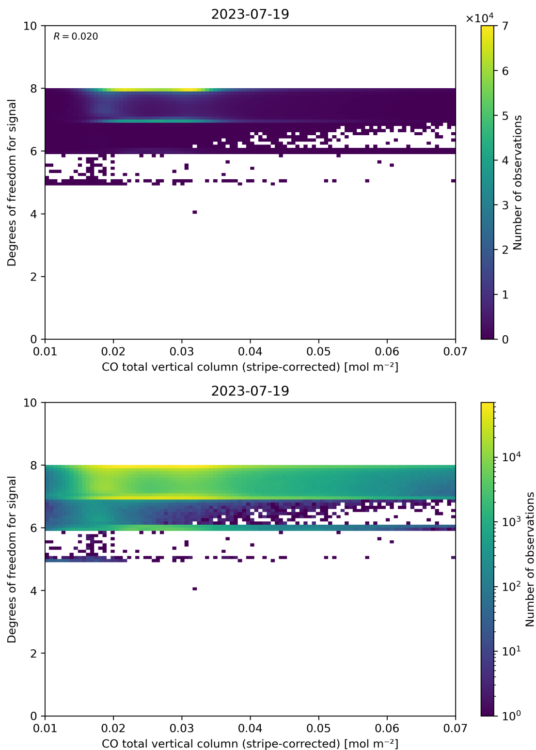
Figure 38: Scatter density plot of “CO total vertical column (stripe-corrected)” against “Degrees of freedom for signal” for 2023-07-19 to 2023-07-20.
