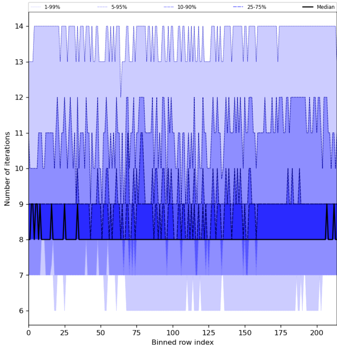
Figure 32: Along track statistics of “Number of iterations” for 2023-07-19 to 2023-07-20
