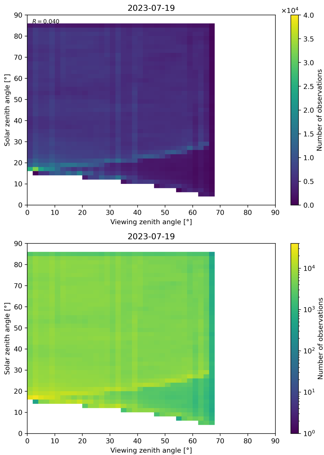
Figure 77: Scatter density plot of “Viewing zenith angle” against “Solar zenith angle” for 2023-07-19 to 2023-07-20.
