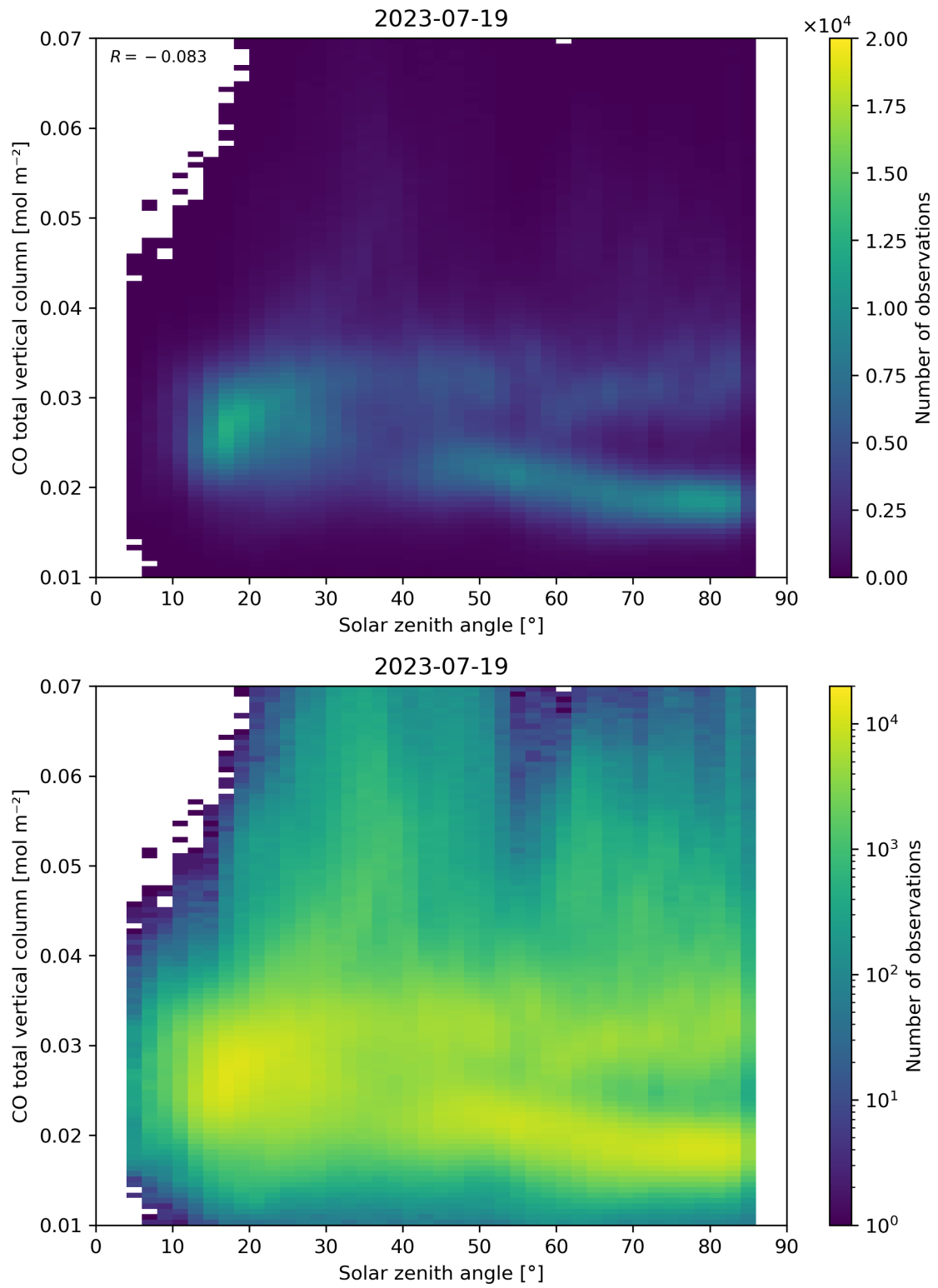
Figure 61: Scatter density plot of “Solar zenith angle” against “CO total vertical column” for 2023-07-19 to 2023-07-20.
