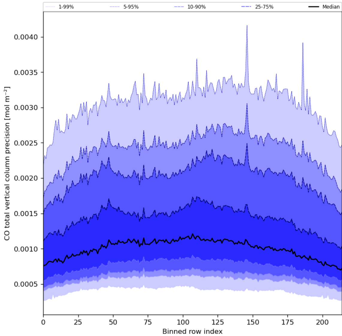
Figure 28: Along track statistics of “CO total vertical column precision” for 2023-07-19 to 2023-07-20
