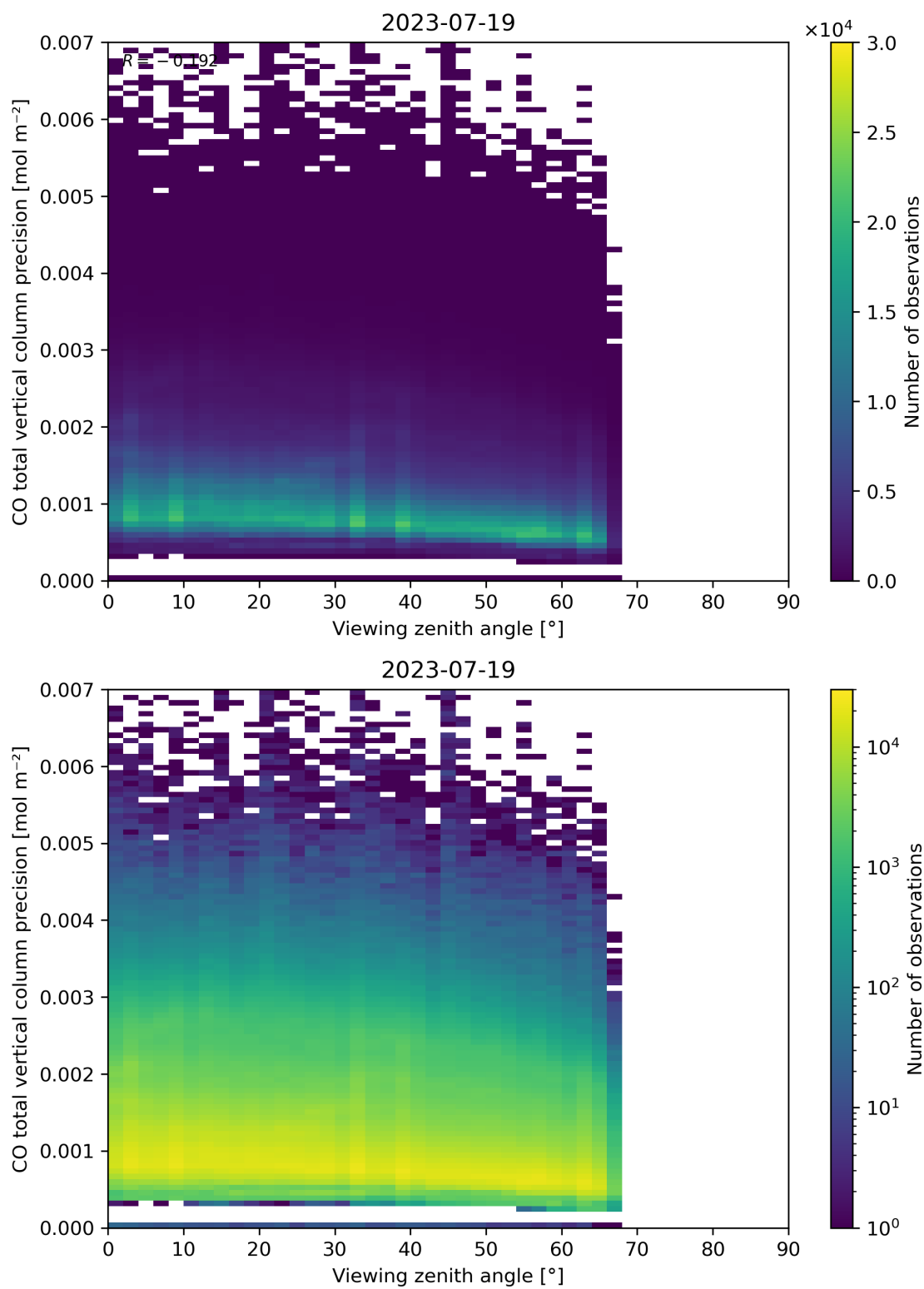
Figure 71: Scatter density plot of “Viewing zenith angle” against “CO total vertical column precision” for 2023-07-19 to 2023-07-20.
