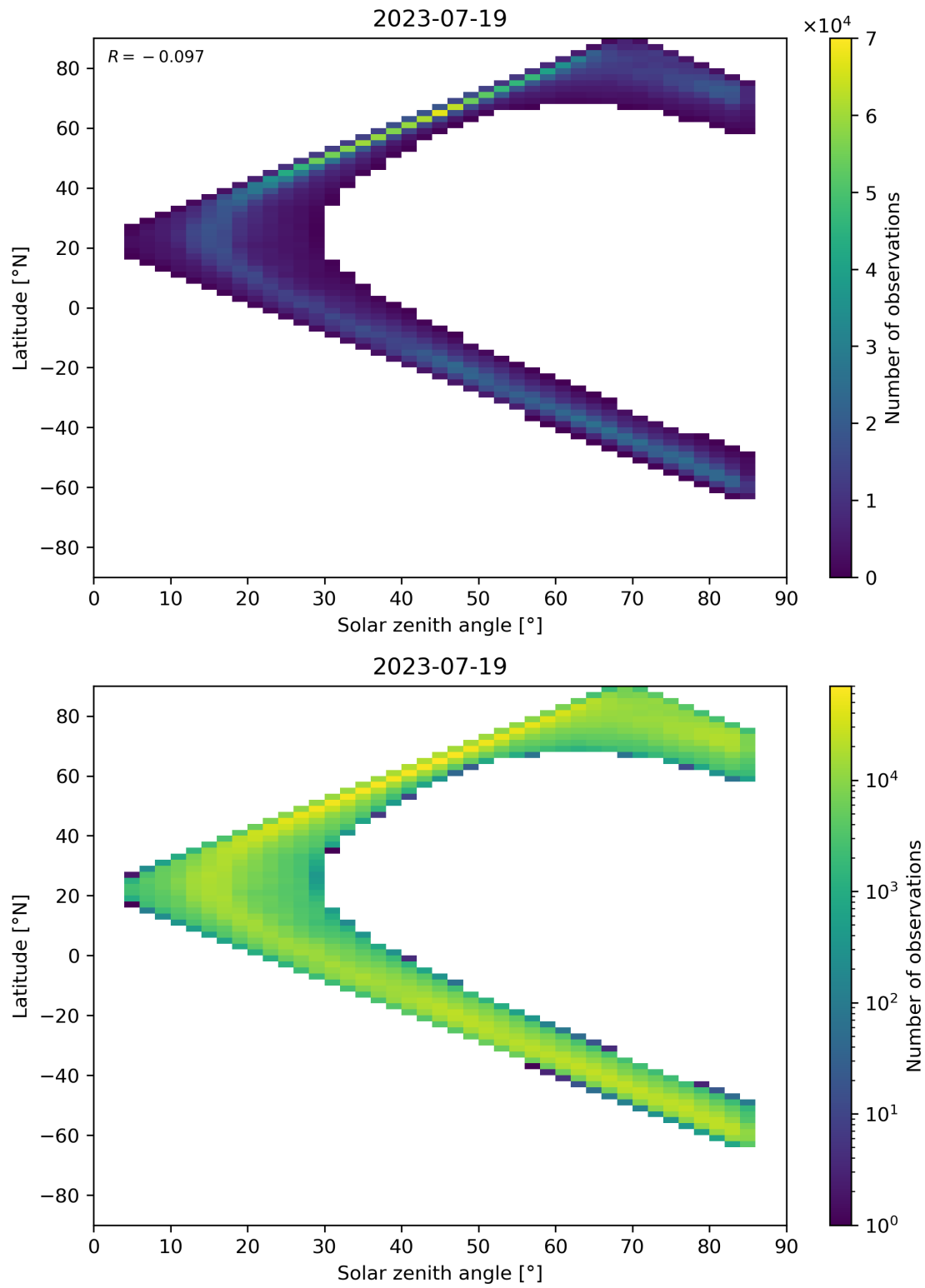
Figure 66: Scatter density plot of “Solar zenith angle” against “Latitude” for 2023-07-19 to 2023-07-20.
