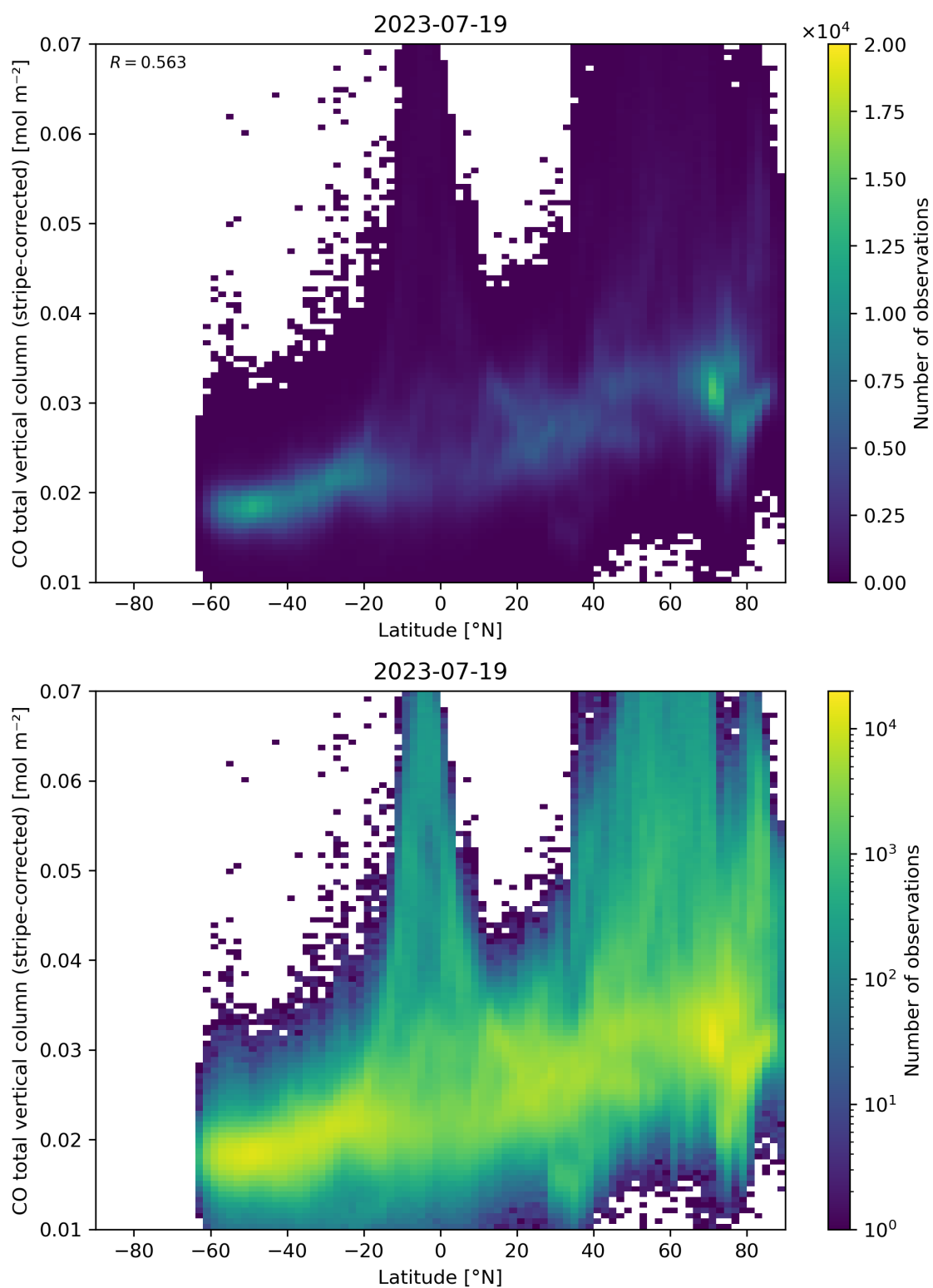
Figure 52: Scatter density plot of “Latitude” against “CO total vertical column (stripe-corrected)” for 2023-07-19 to 2023-07-20.
