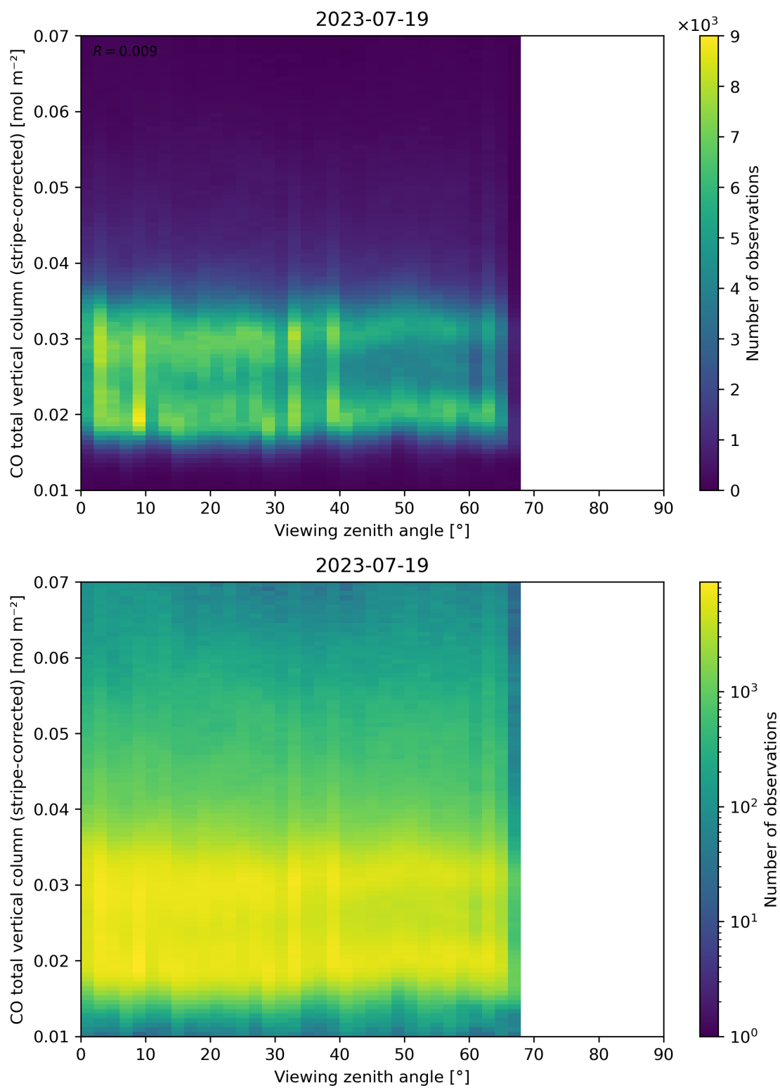
Figure 70: Scatter density plot of “Viewing zenith angle” against “CO total vertical column (stripe-corrected)” for 2023-07-19 to 2023-07-20.
