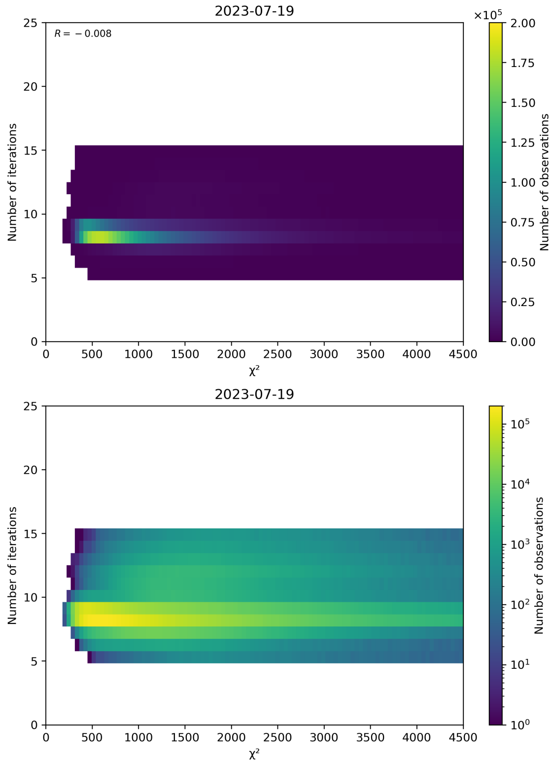
Figure 49: Scatter density plot of “ \chi^2 ” against “Number of iterations” for 2023-07-19 to 2023-07-20.
