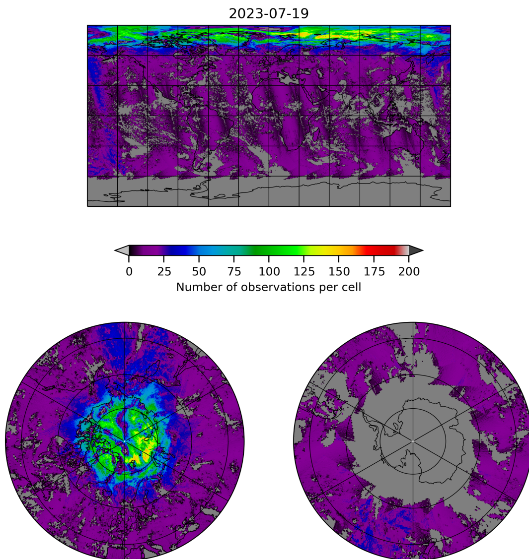
Figure 8: Map of the number of observations for 2023-07-19 to 2023-07-20
