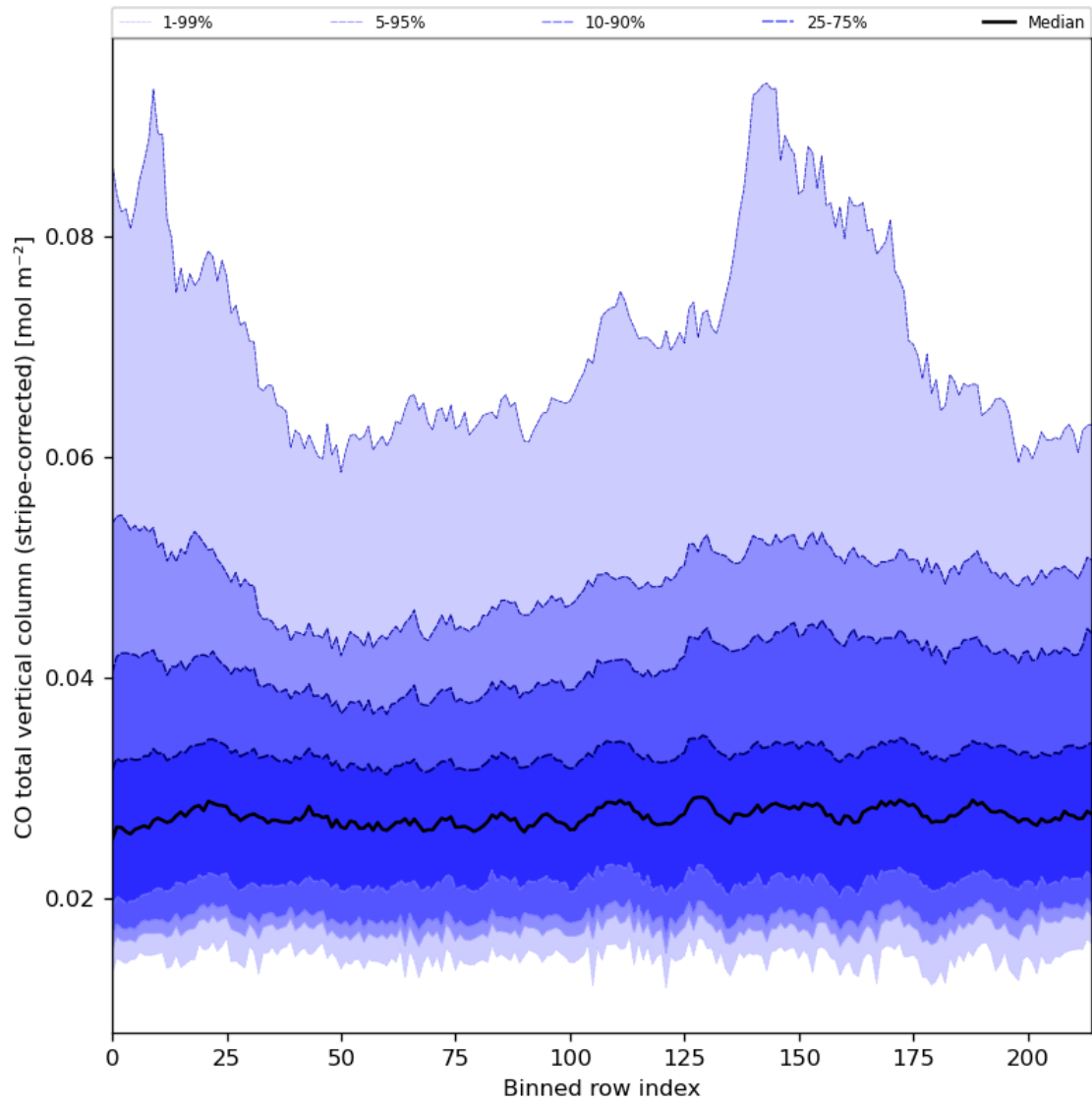
Figure 27: Along track statistics of “CO total vertical column (stripe-corrected)” for 2023-07-19 to 2023-07-20
