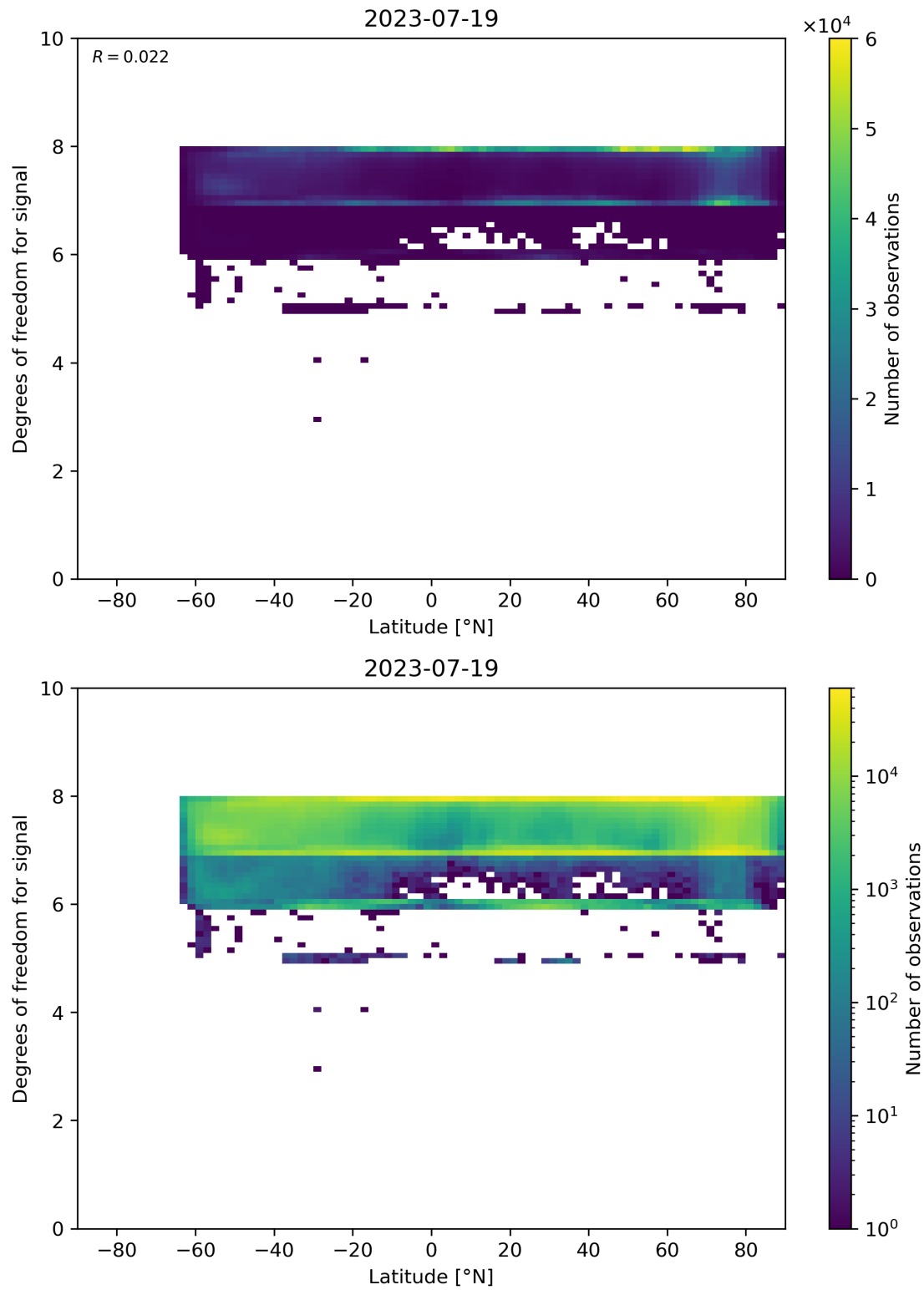
Figure 55: Scatter density plot of “Latitude” against “Degrees of freedom for signal” for 2023-07-19 to 2023-07-20.
