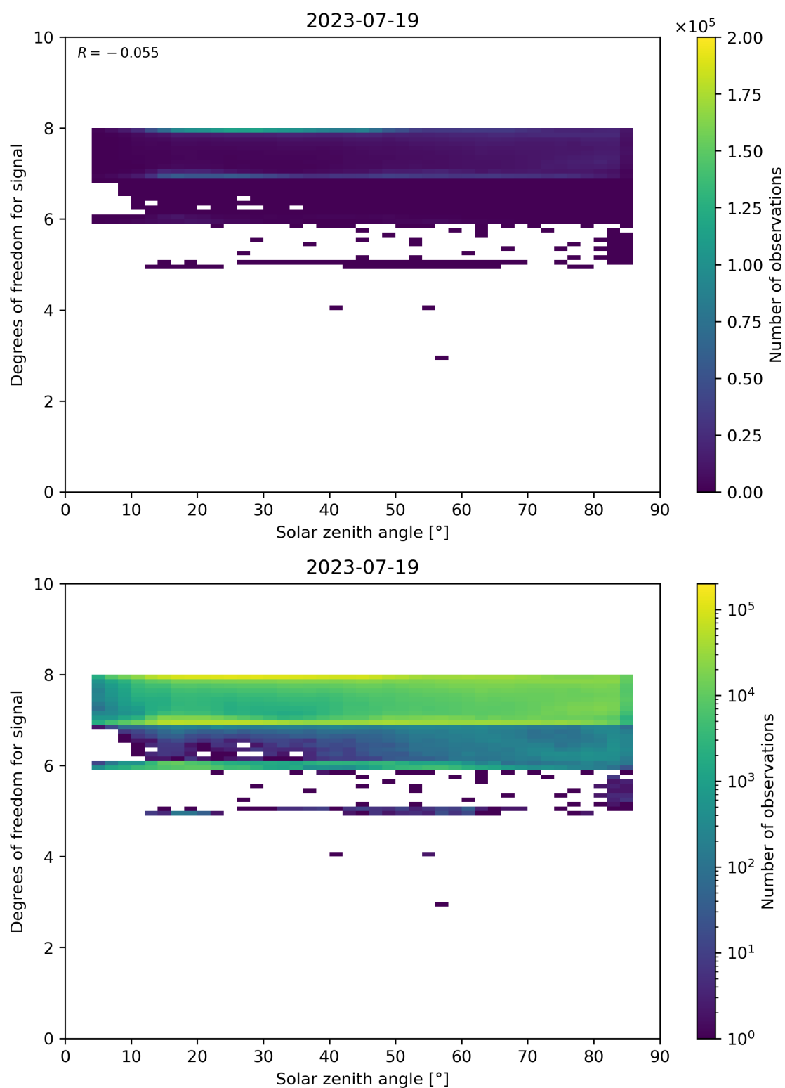
Figure 65: Scatter density plot of “Solar zenith angle” against “Degrees of freedom for signal” for 2023-07-19 to 2023-07-20.
