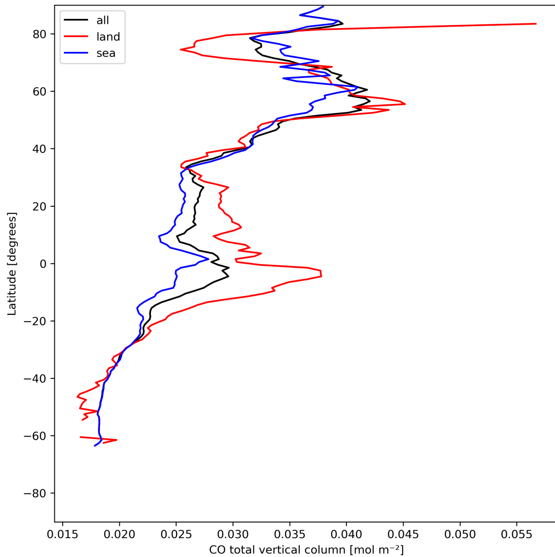
Figure 10: Zonal average of “CO total vertical column” for 2023-07-19 to 2023-07-20.
