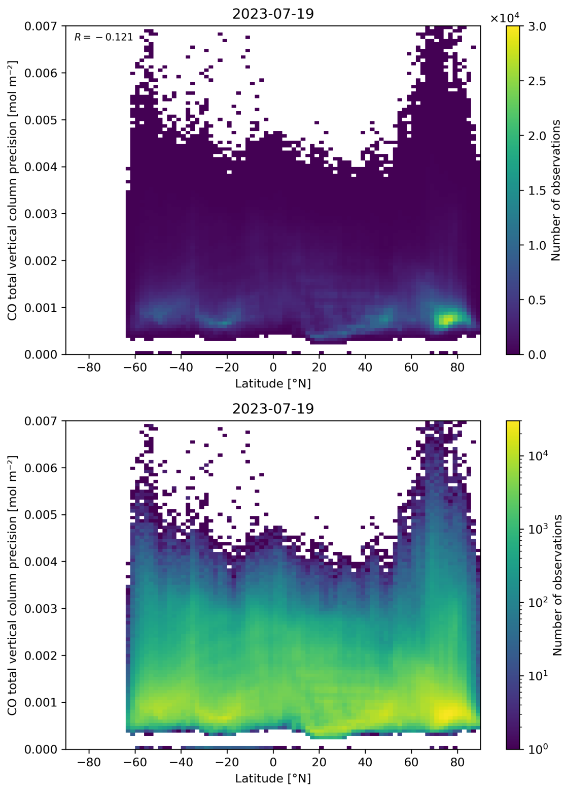
Figure 53: Scatter density plot of “Latitude” against “CO total vertical column precision” for 2023-07-19 to 2023-07-20.
