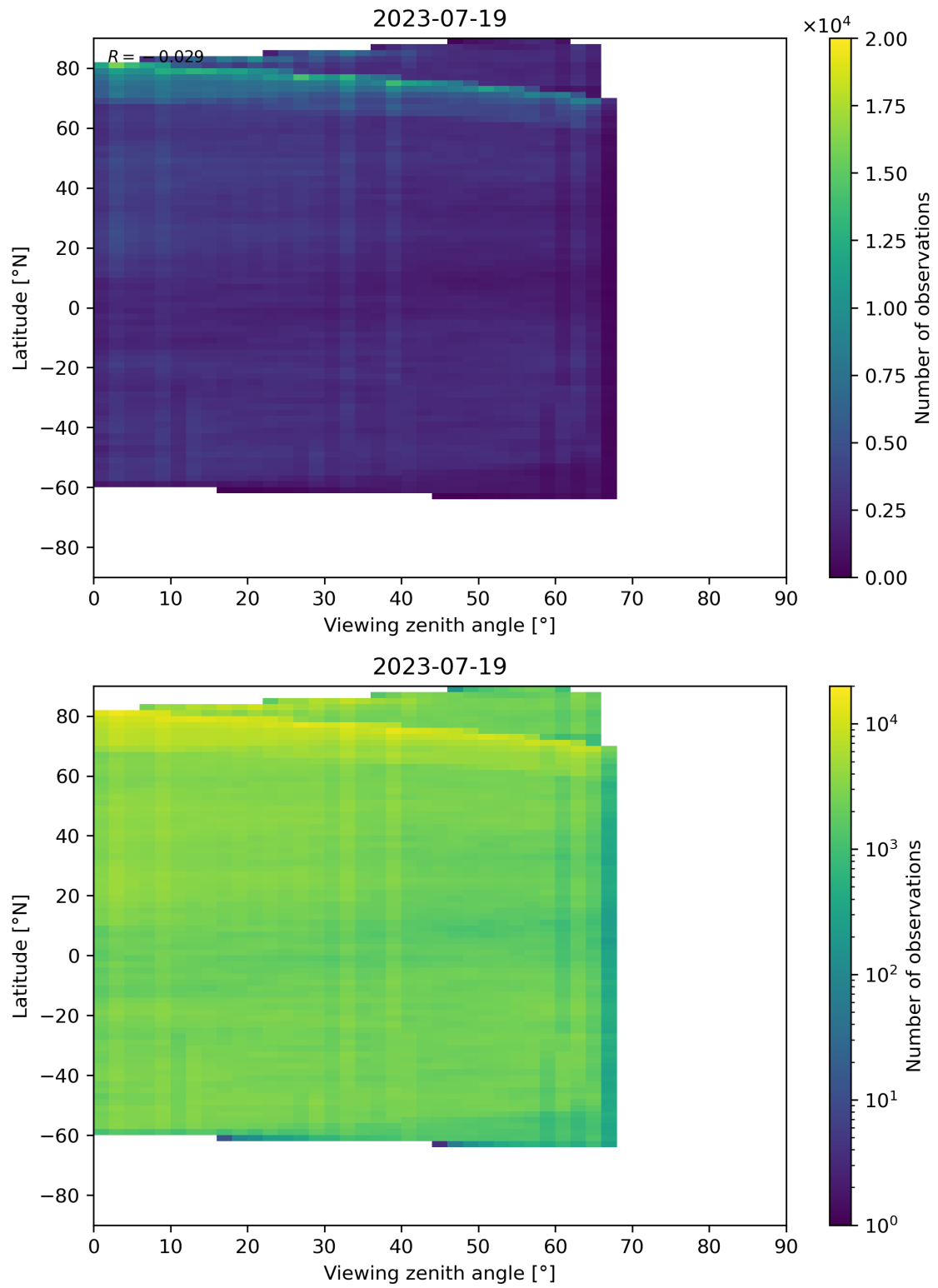
Figure 74: Scatter density plot of “Viewing zenith angle” against “Latitude” for 2023-07-19 to 2023-07-20.
