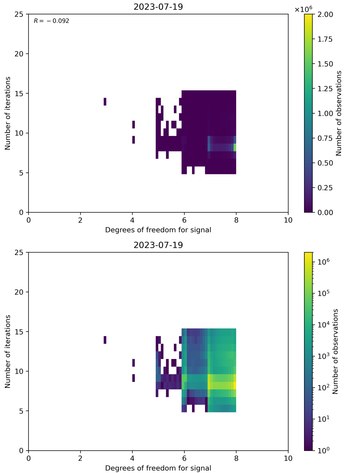
Figure 50: Scatter density plot of “Degrees of freedom for signal” against “Number of iterations” for 2023-07-19 to 2023-07-20.
