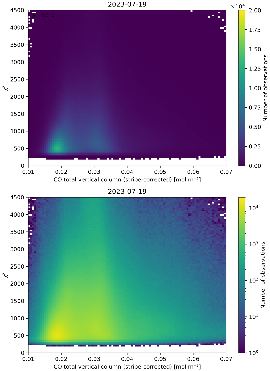
Figure 37: Scatter density plot of “CO total vertical column (stripe-corrected)” against “ \chi^2 ” for 2023-07-19 to 2023-07-20.
