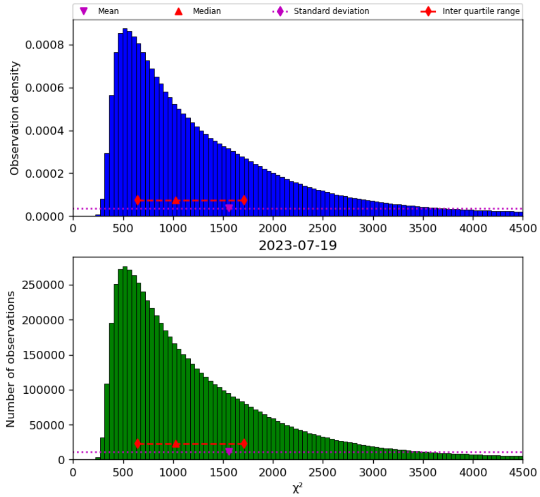
Figure 22: Histogram of “ \chi^2 ” for 2023-07-19 to 2023-07-20
