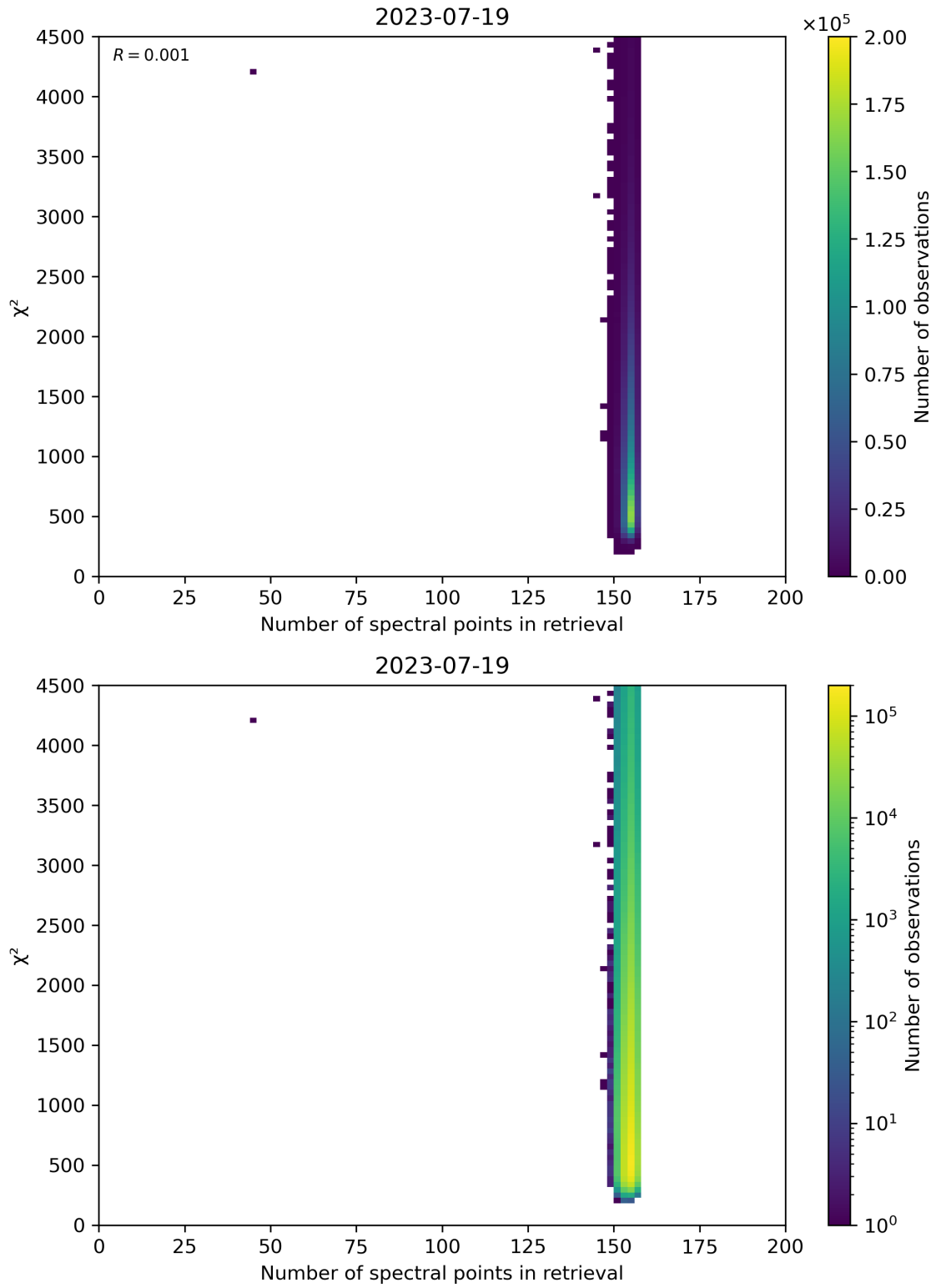
Figure 58: Scatter density plot of “Number of spectral points in retrieval” against “ \chi^2 ” for 2023-07-19 to 2023-07-20.
