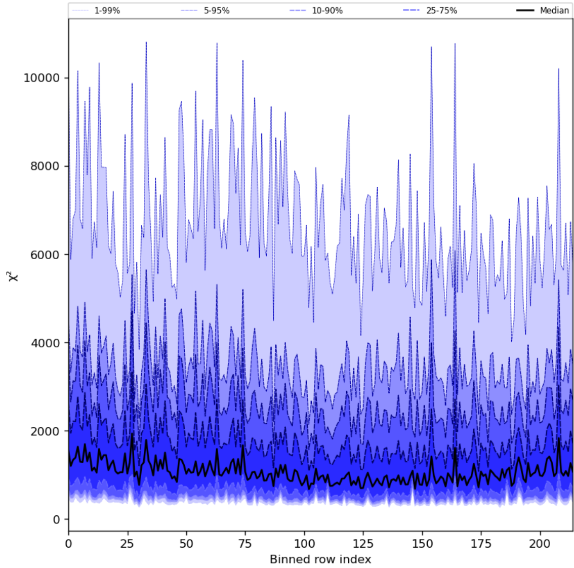
Figure 30: Along track statistics of “ \chi^2 ” for 2023-07-19 to 2023-07-20
