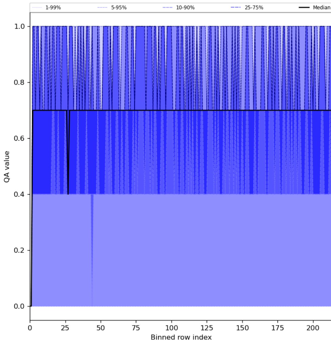
Figure 25: Along track statistics of “QA value” for 2023-07-19 to 2023-07-20
