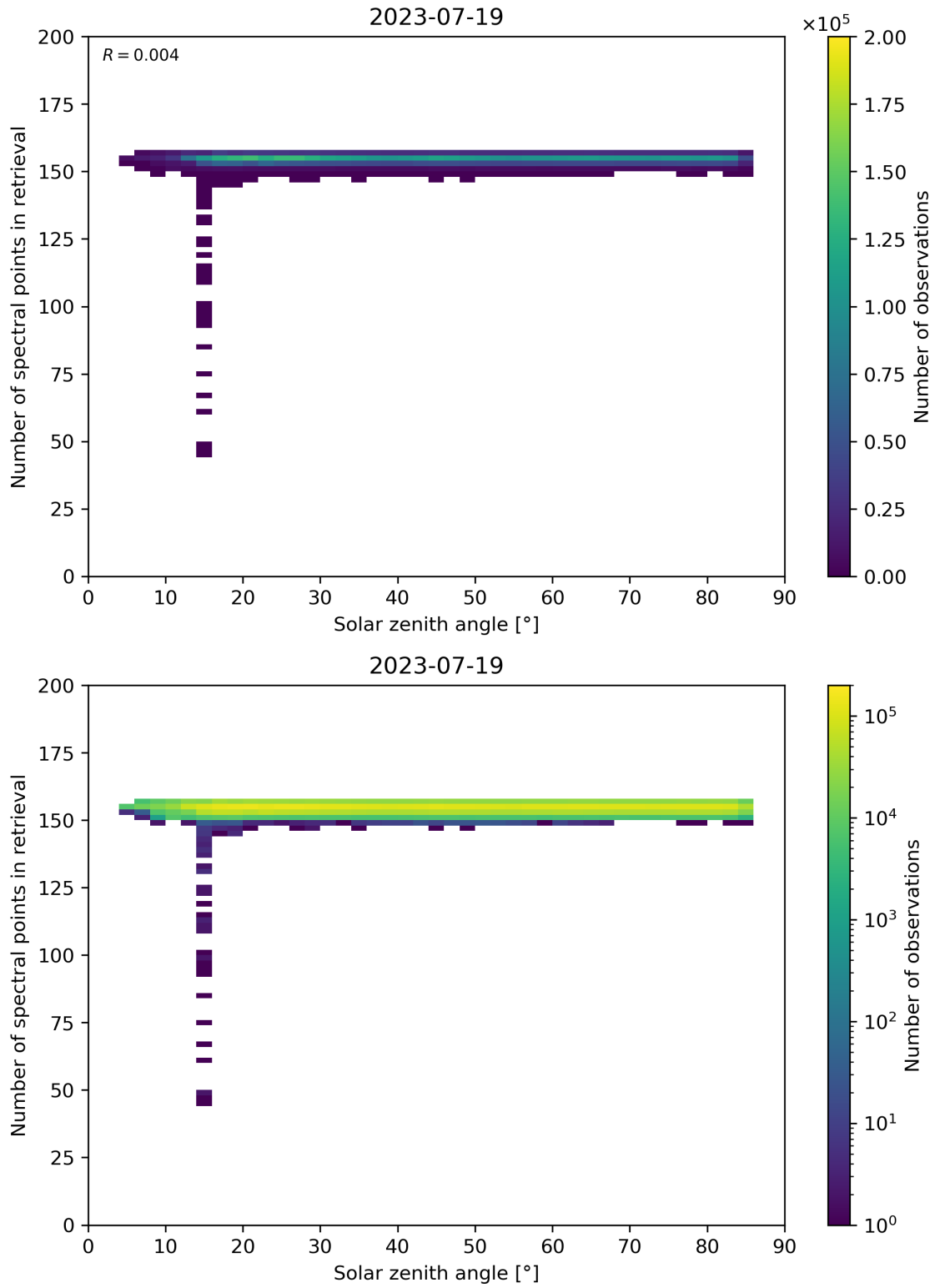
Figure 68: Scatter density plot of “Solar zenith angle” against “Number of spectral points in retrieval” for 2023-07-19 to 2023-07-20.
