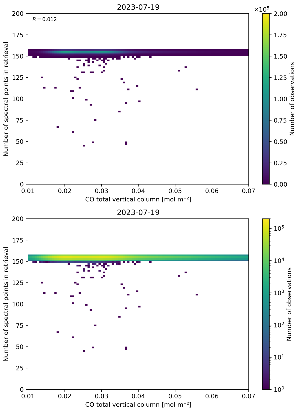
Figure 43: Scatter density plot of “CO total vertical column” against “Number of spectral points in retrieval” for 2023-07-19 to 2023-07-20.
