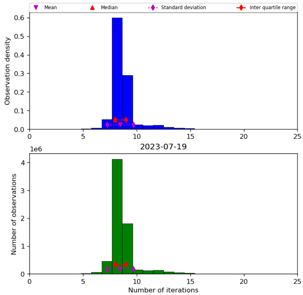
Figure 24: Histogram of “Number of iterations” for 2023-07-19 to 2023-07-20
