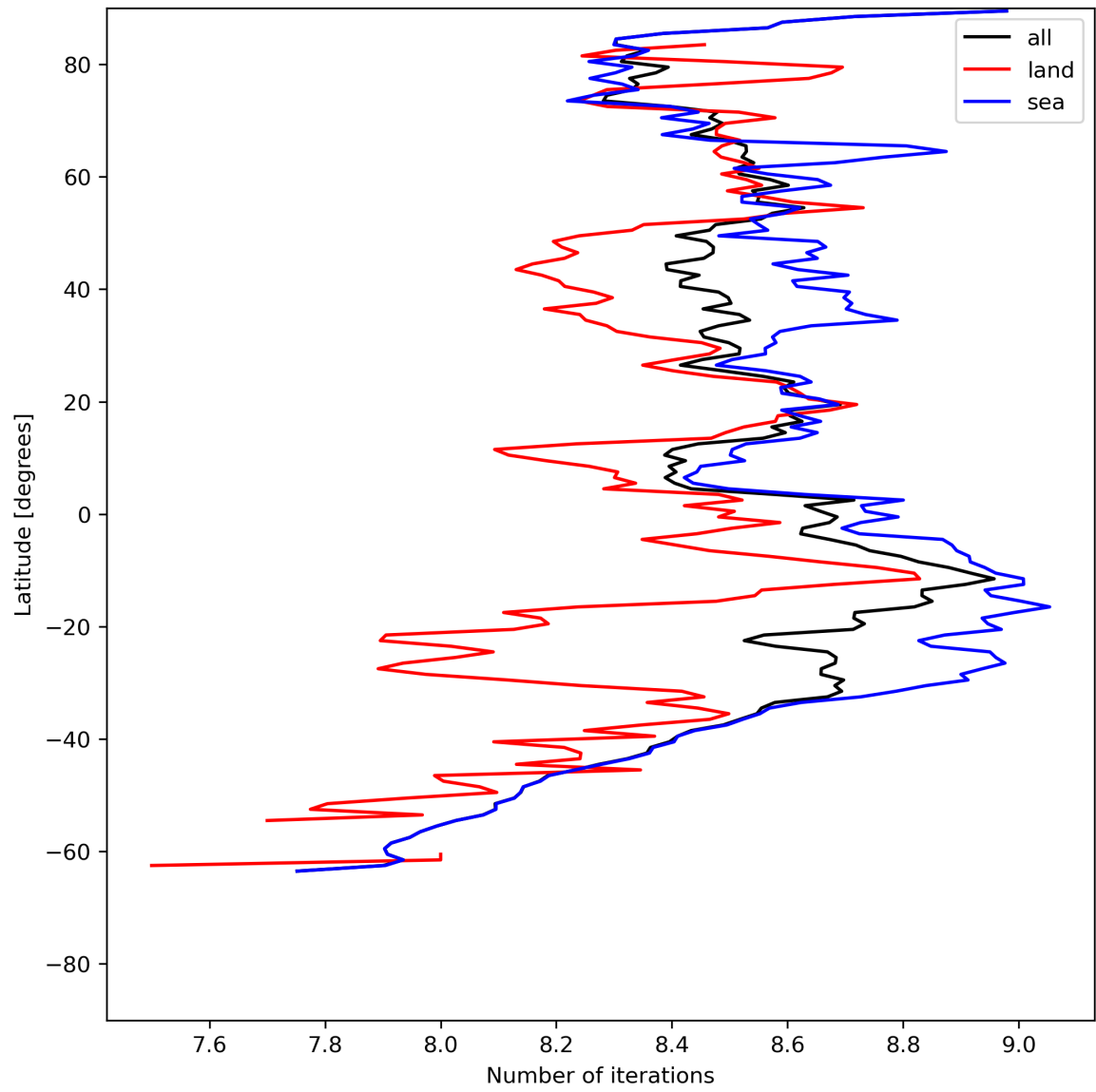
Figure 16: Zonal average of “Number of iterations” for 2023-07-19 to 2023-07-20.
