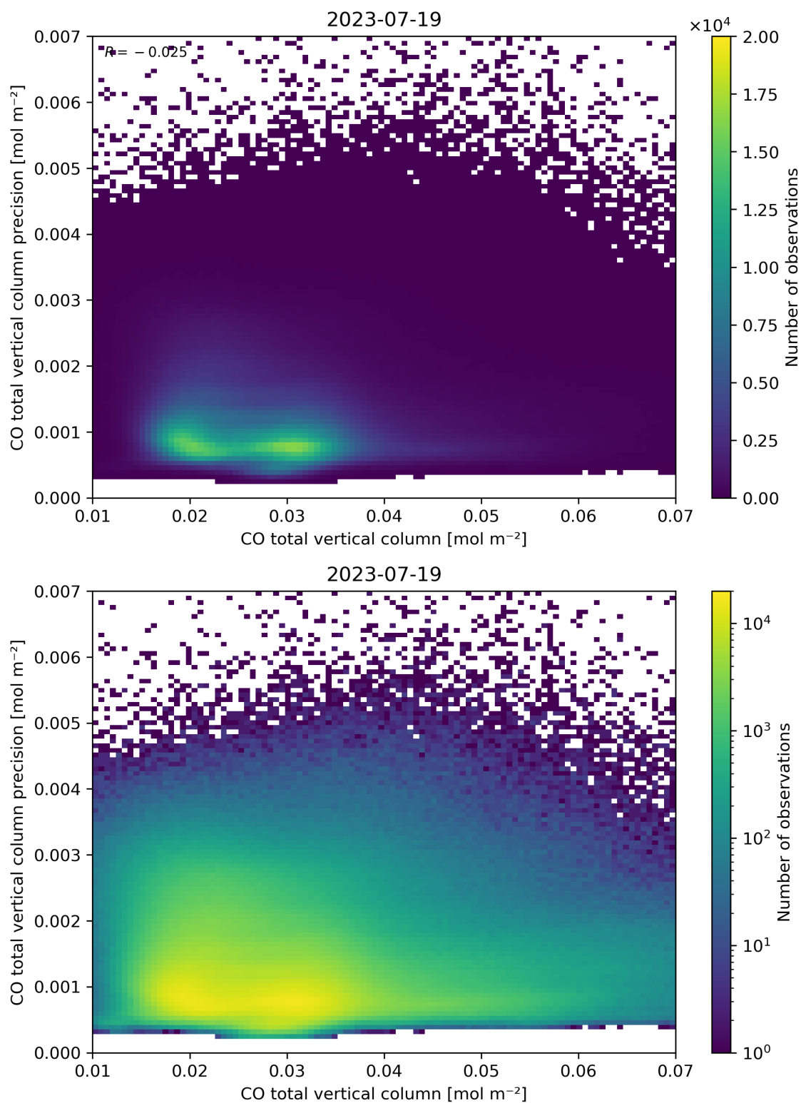
Figure 34: Scatter density plot of “CO total vertical column” against “CO total vertical column precision” for 2023-07-19 to 2023-07-20.
