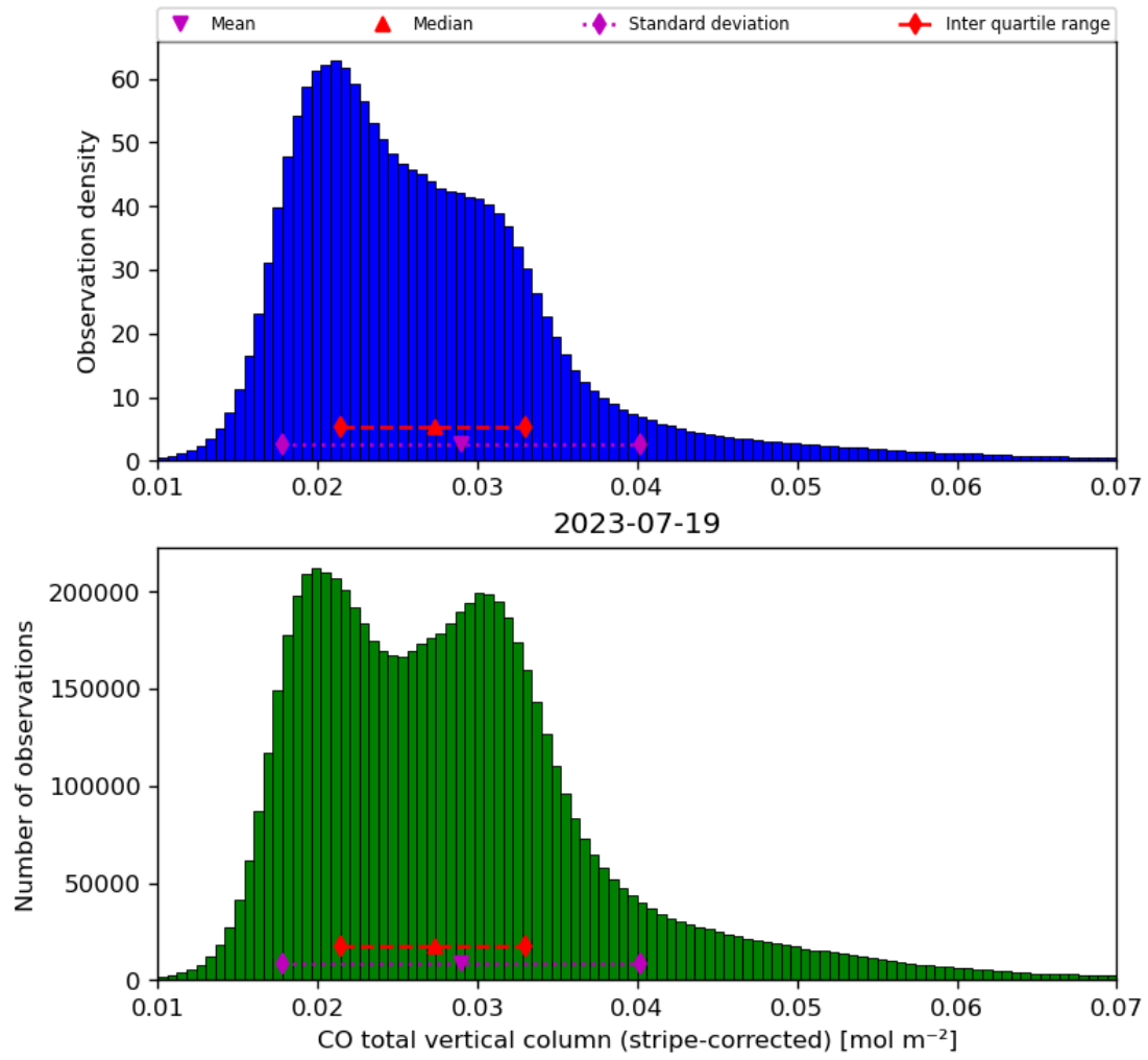
Figure 19: Histogram of “CO total vertical column (stripe-corrected)” for 2023-07-19 to 2023-07-20
