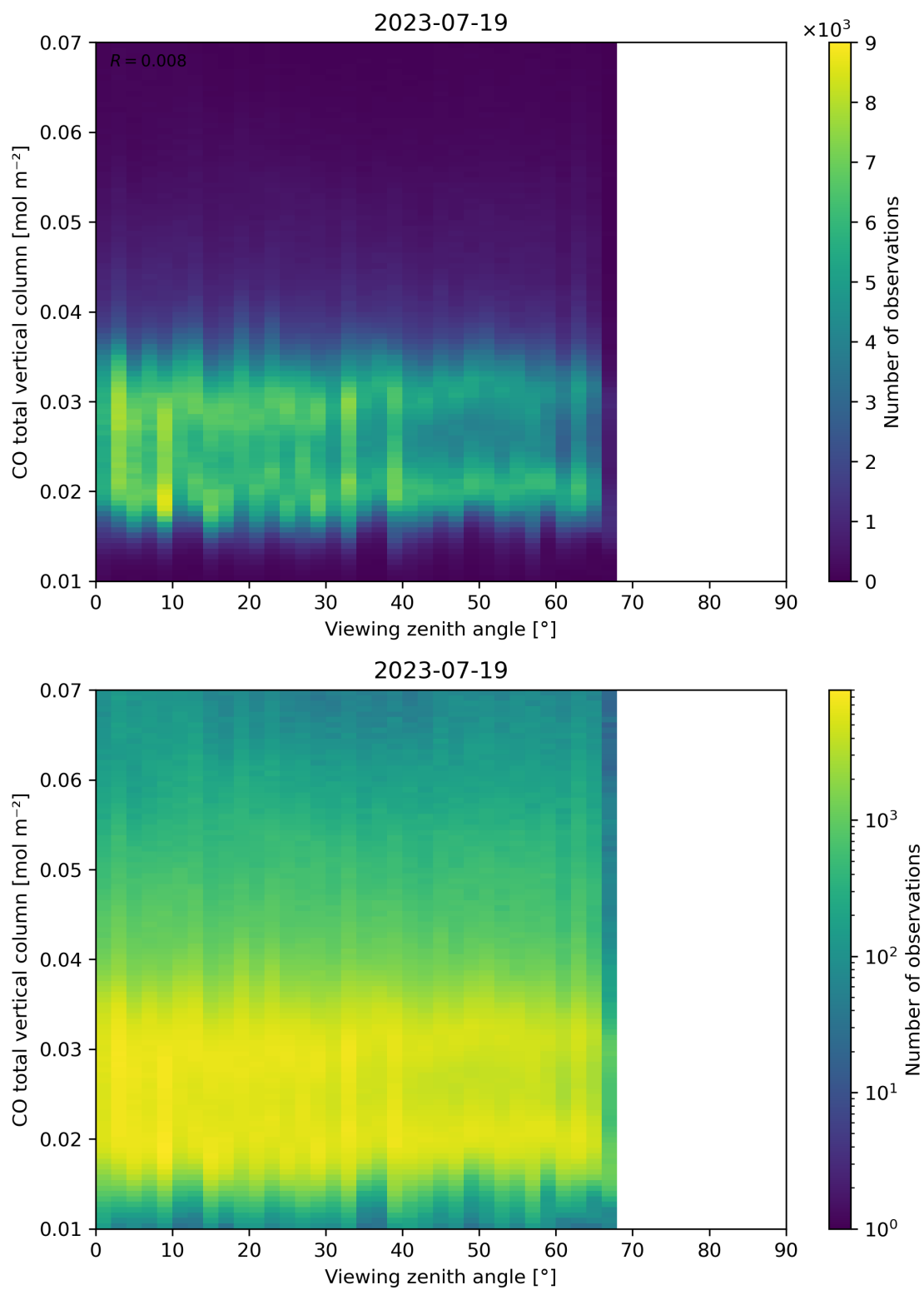
Figure 69: Scatter density plot of “Viewing zenith angle” against “CO total vertical column” for 2023-07-19 to 2023-07-20.
