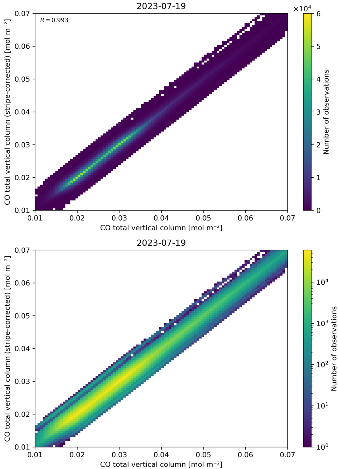
Figure 33: Scatter density plot of “CO total vertical column” against “CO total vertical column (stripe-corrected)” for 2023-07-19 to 2023-07-20.
