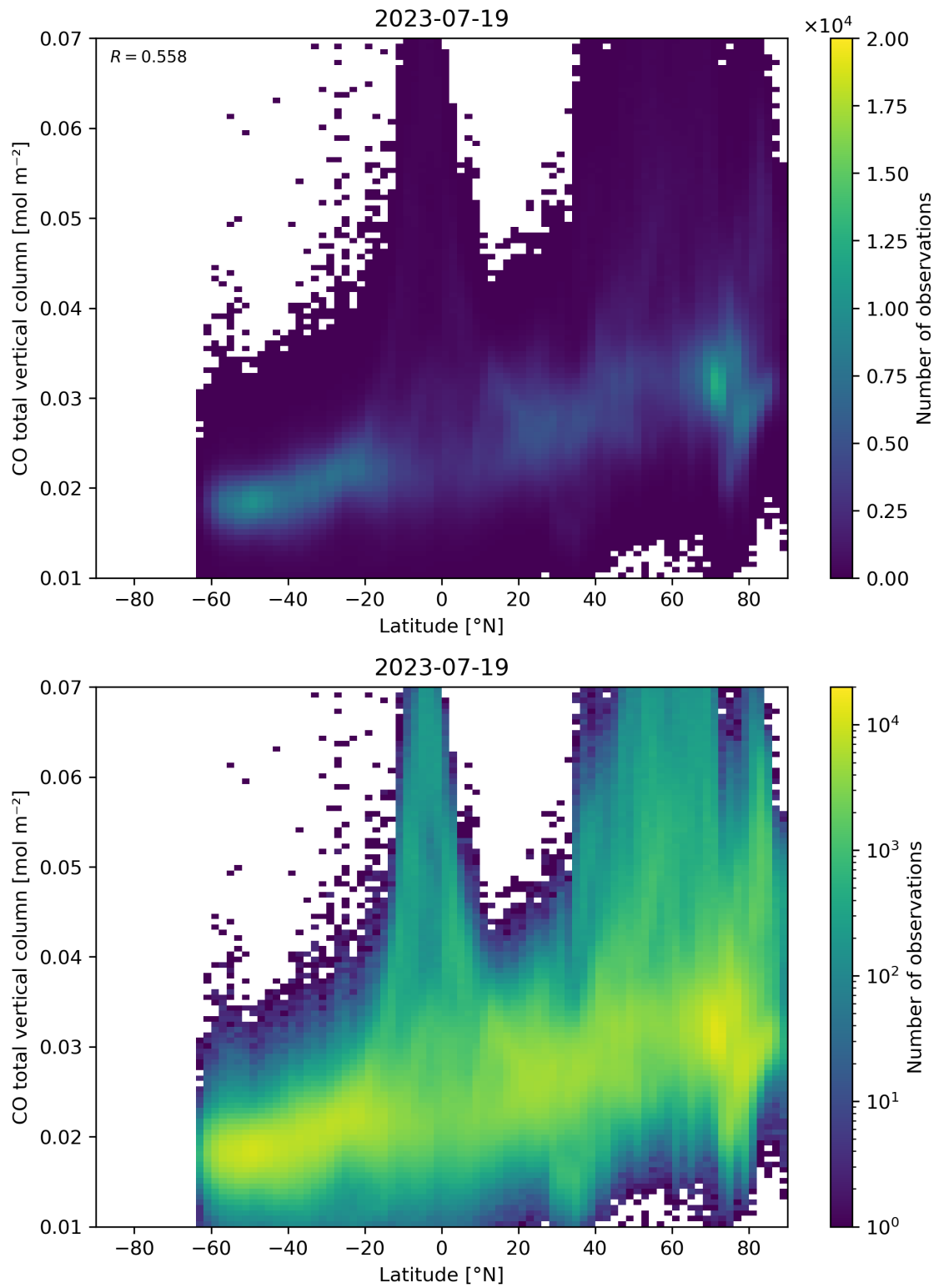
Figure 51: Scatter density plot of “Latitude” against “CO total vertical column” for 2023-07-19 to 2023-07-20.
