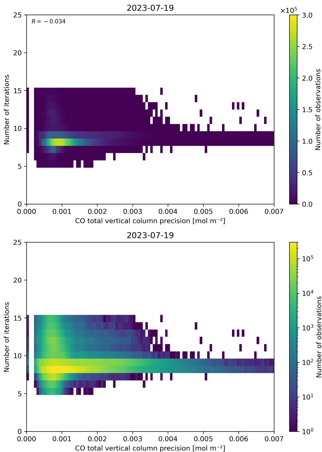
Figure 46: Scatter density plot of “CO total vertical column precision” against “Number of iterations” for 2023-07-19 to 2023-07-20.
