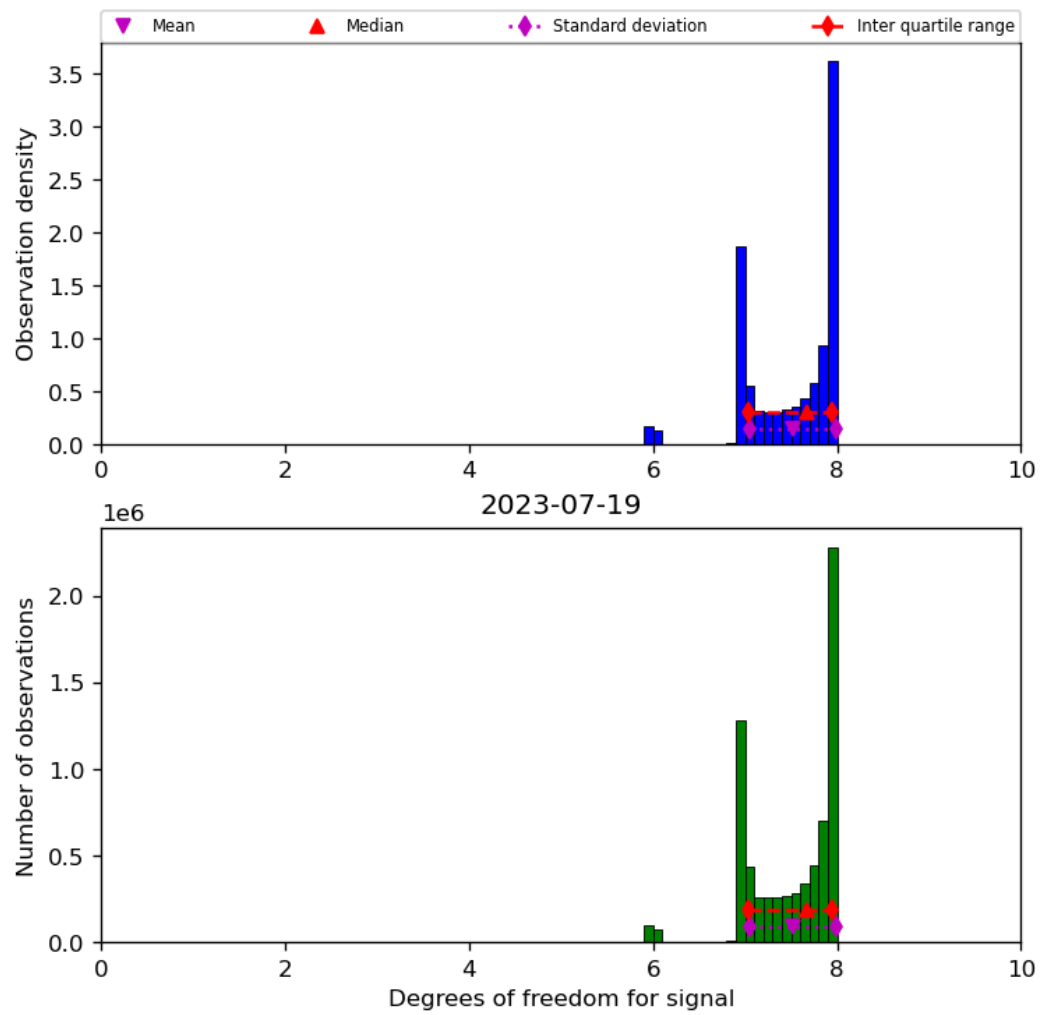
Figure 23: Histogram of “Degrees of freedom for signal” for 2023-07-19 to 2023-07-20
