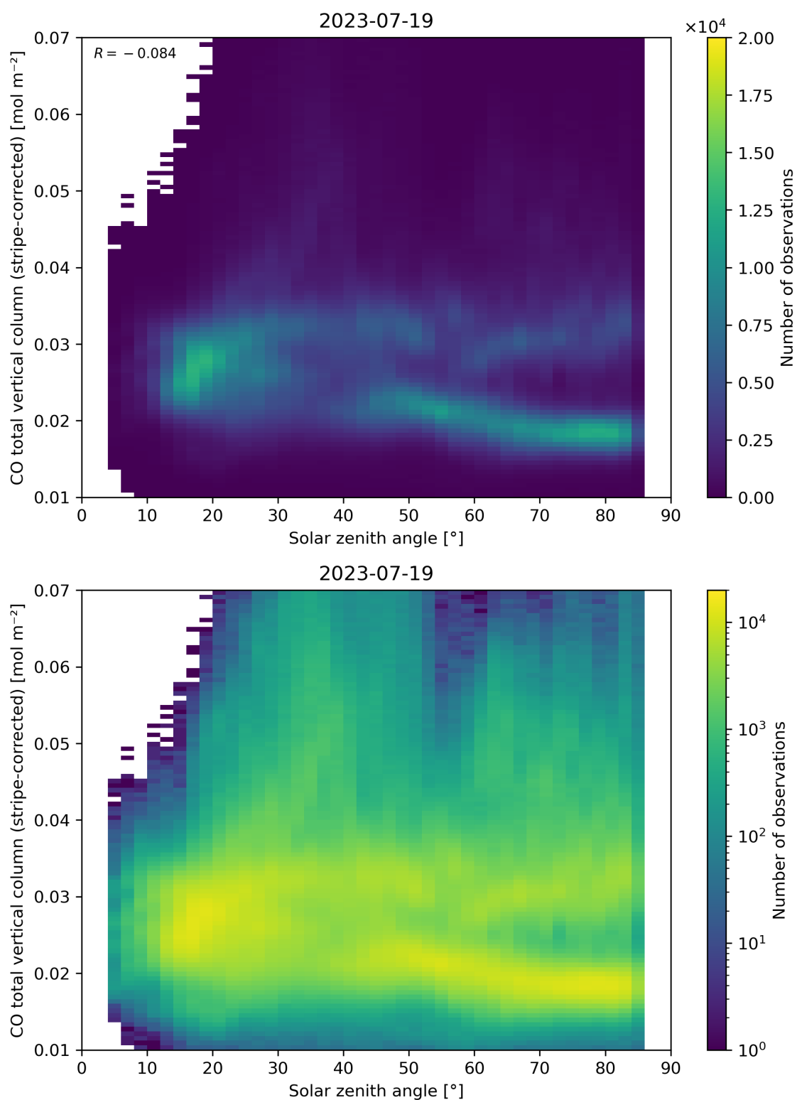
Figure 62: Scatter density plot of “Solar zenith angle” against “CO total vertical column (stripe-corrected)” for 2023-07-19 to 2023-07-20.
