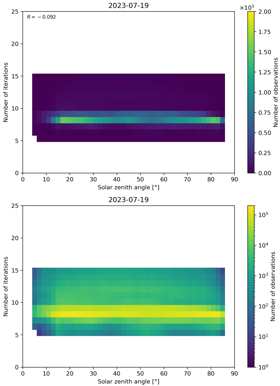
Figure 67: Scatter density plot of “Solar zenith angle” against “Number of iterations” for 2023-07-19 to 2023-07-20.
