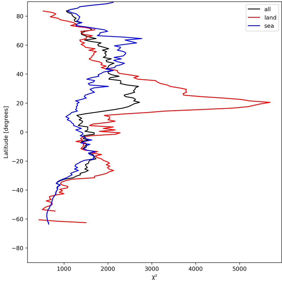
Figure 14: Zonal average of “ \chi^2 ” for 2023-07-19 to 2023-07-20.
