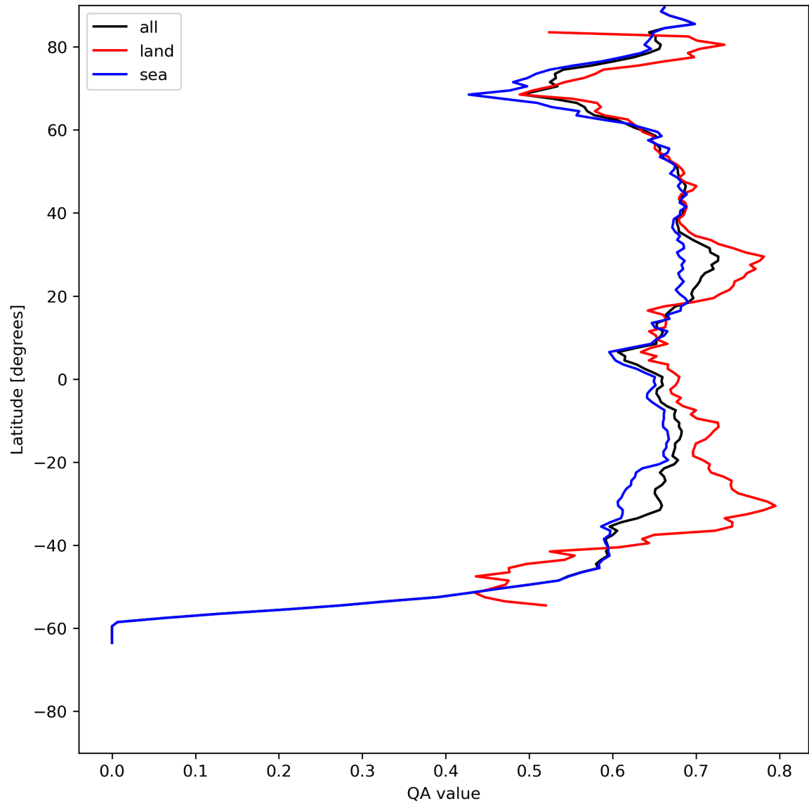
Figure 9: Zonal average of “QA value” for 2023-07-19 to 2023-07-20.
