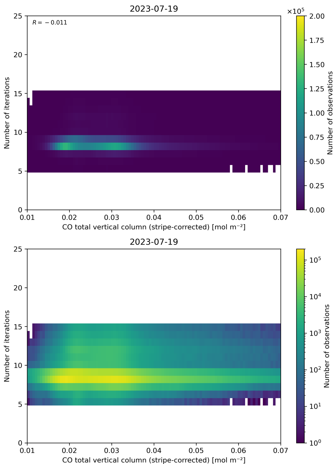
Figure 39: Scatter density plot of “CO total vertical column (stripe-corrected)” against “Number of iterations” for 2023-07-19 to 2023-07-20.
