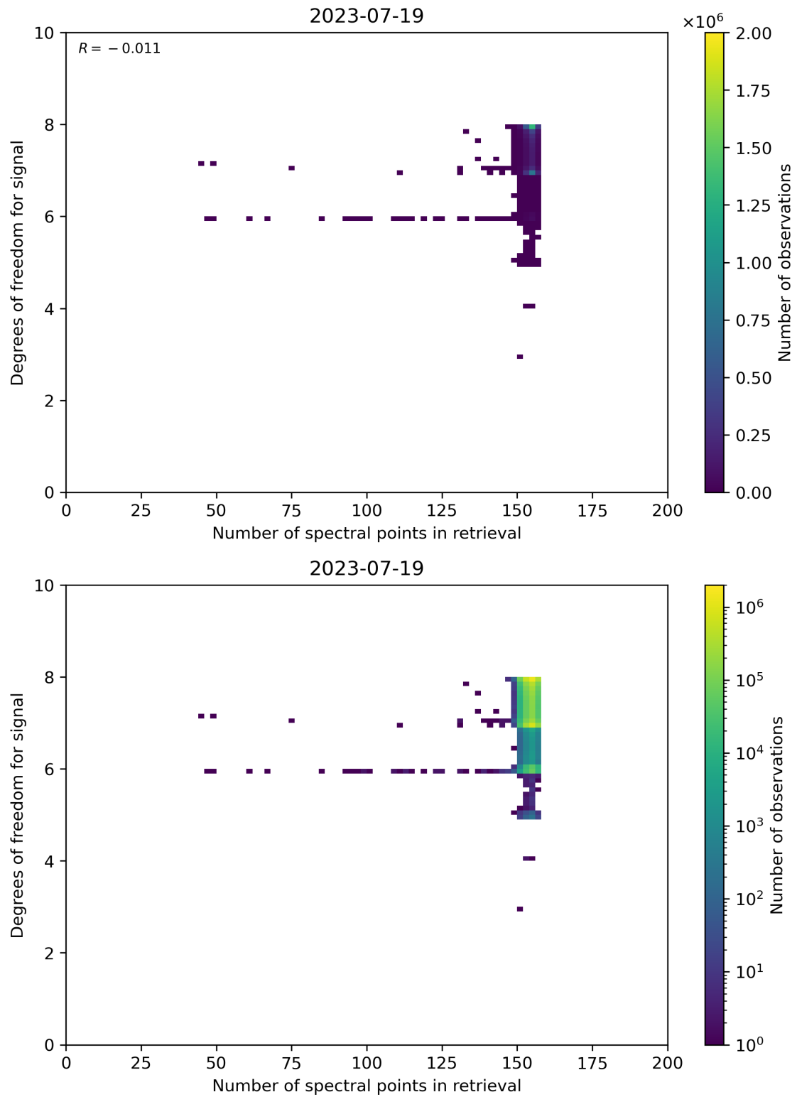
Figure 59: Scatter density plot of “Number of spectral points in retrieval” against “Degrees of freedom for signal” for 2023-07-19 to 2023-07-20.
