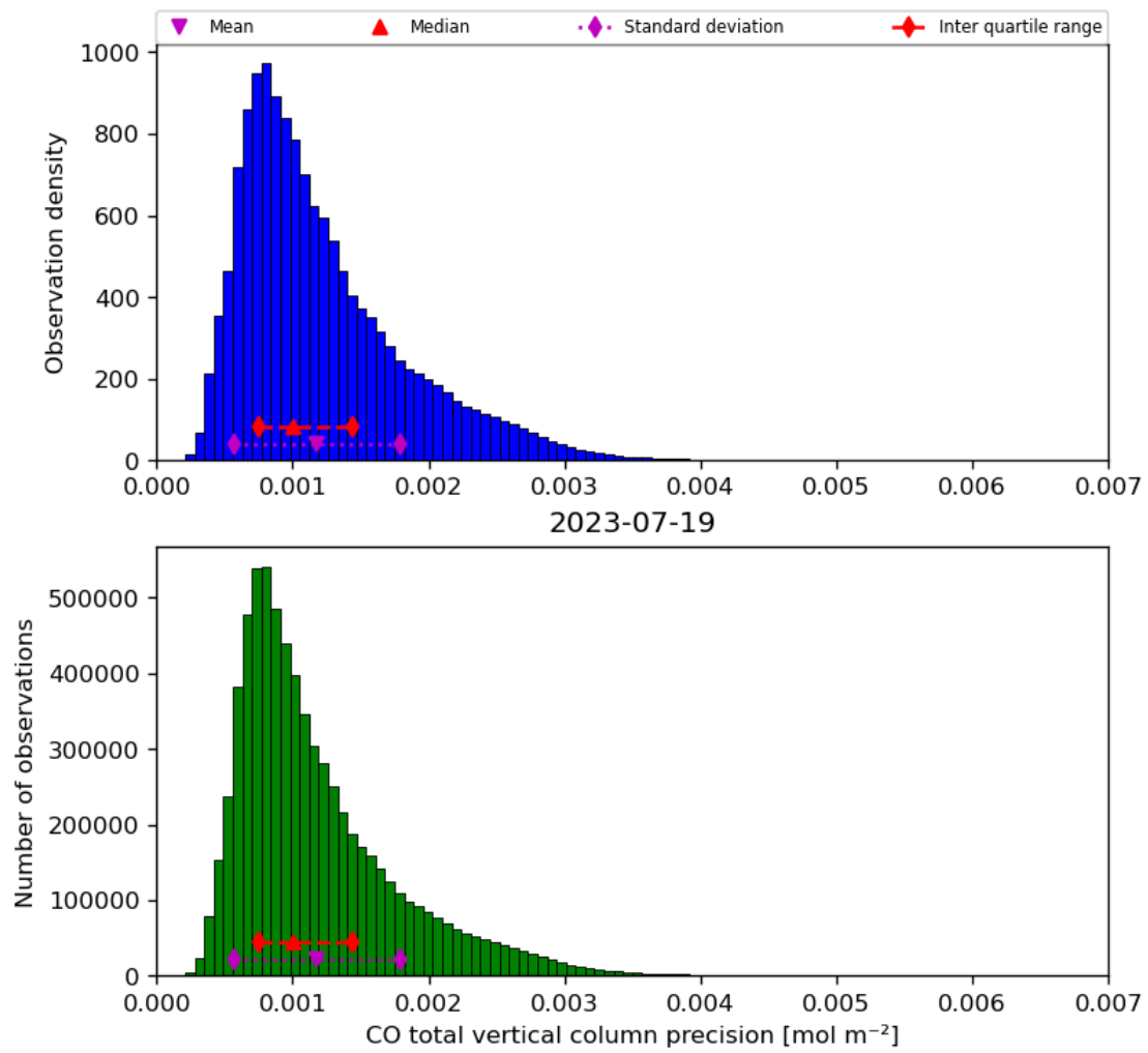
Figure 20: Histogram of “CO total vertical column precision” for 2023-07-19 to 2023-07-20
