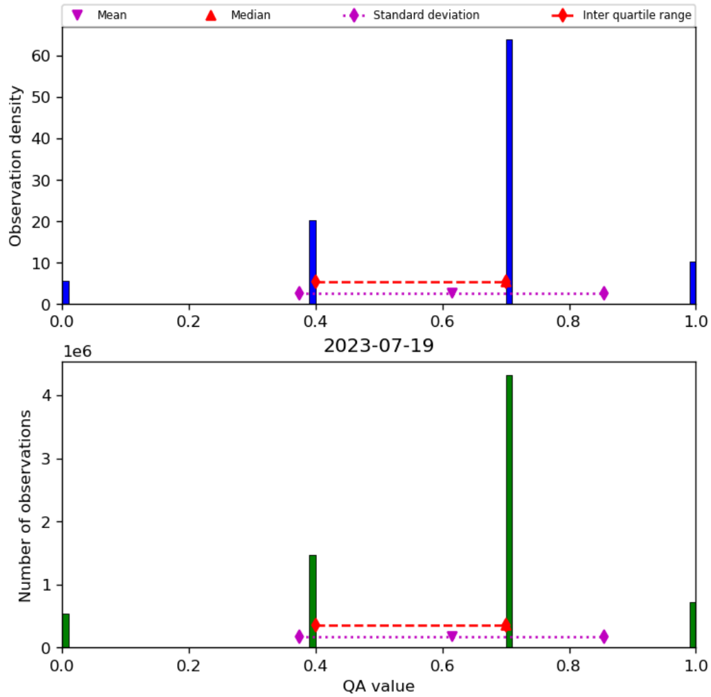
Figure 17: Histogram of “QA value” for 2023-07-19 to 2023-07-20
