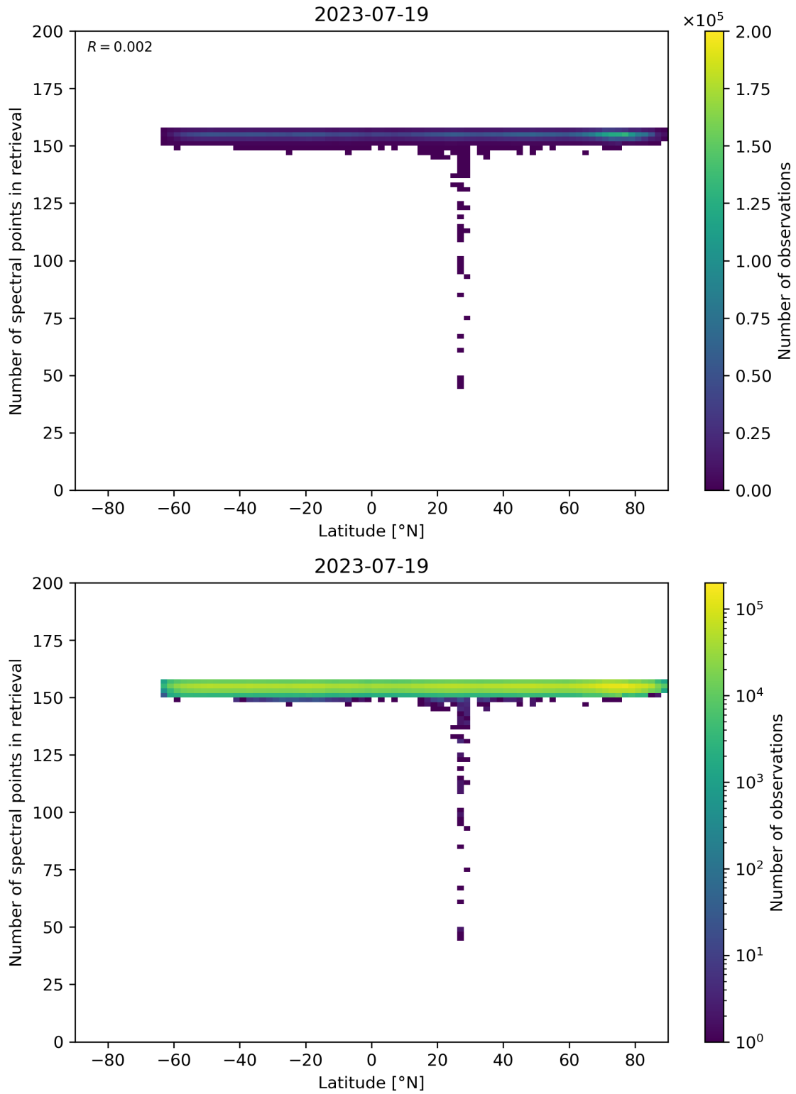
Figure 57: Scatter density plot of “Latitude” against “Number of spectral points in retrieval” for 2023-07-19 to 2023-07-20.
