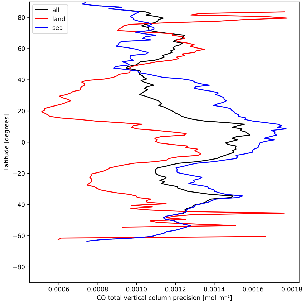
Figure 12: Zonal average of "CO total vertical column precision" for 2023-07-19 to 2023-07-20.
