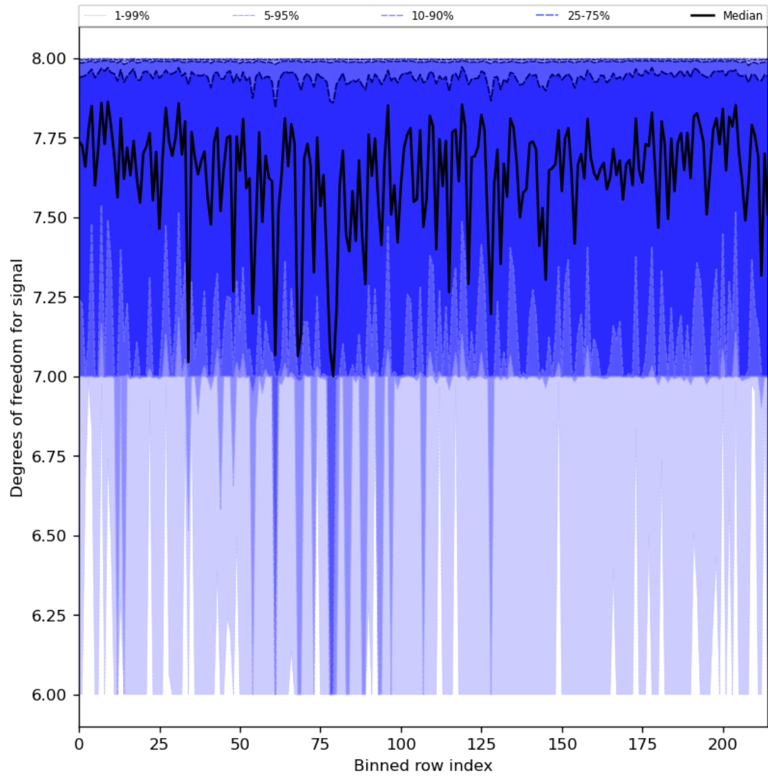
Figure 31: Along track statistics of “Degrees of freedom for signal” for 2023-07-19 to 2023-07-20
