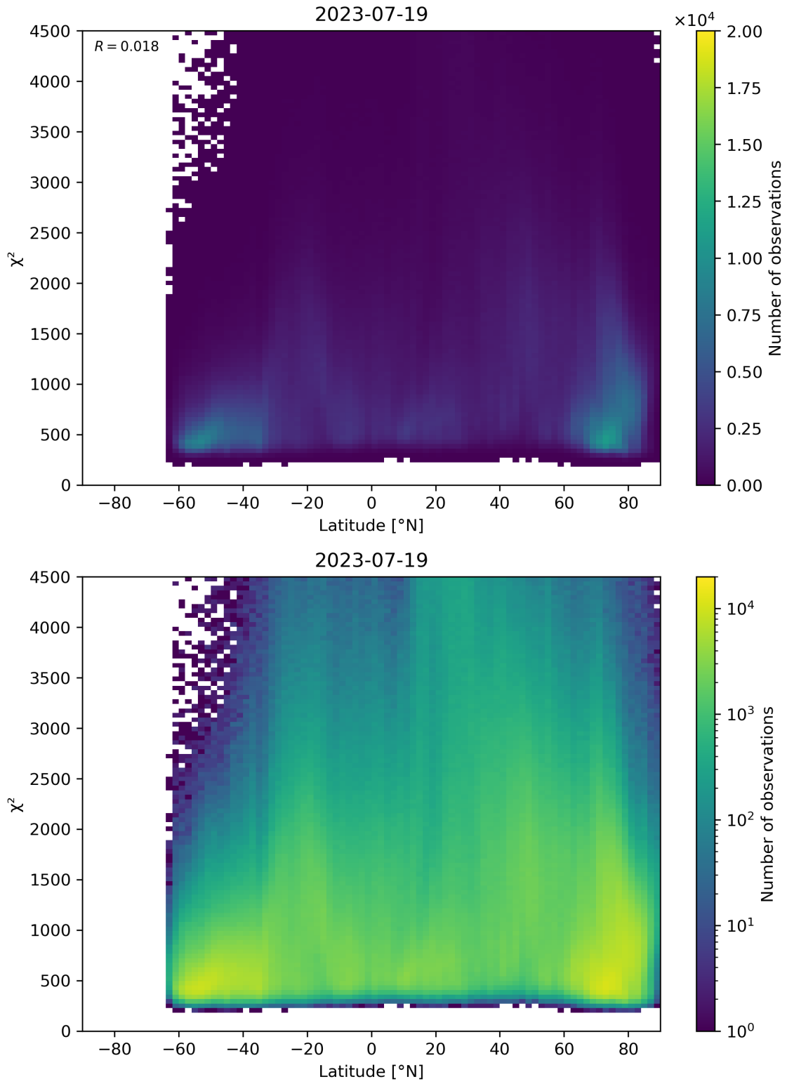
Figure 54: Scatter density plot of “Latitude” against “ \chi^2 ” for 2023-07-19 to 2023-07-20.
