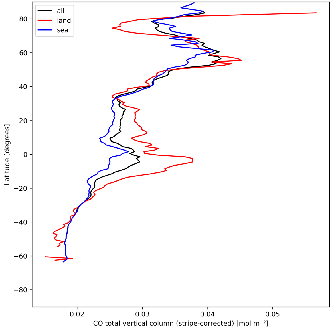
Figure 11: Zonal average of “CO total vertical column (stripe-corrected)” for 2023-07-19 to 2023-07-20.
