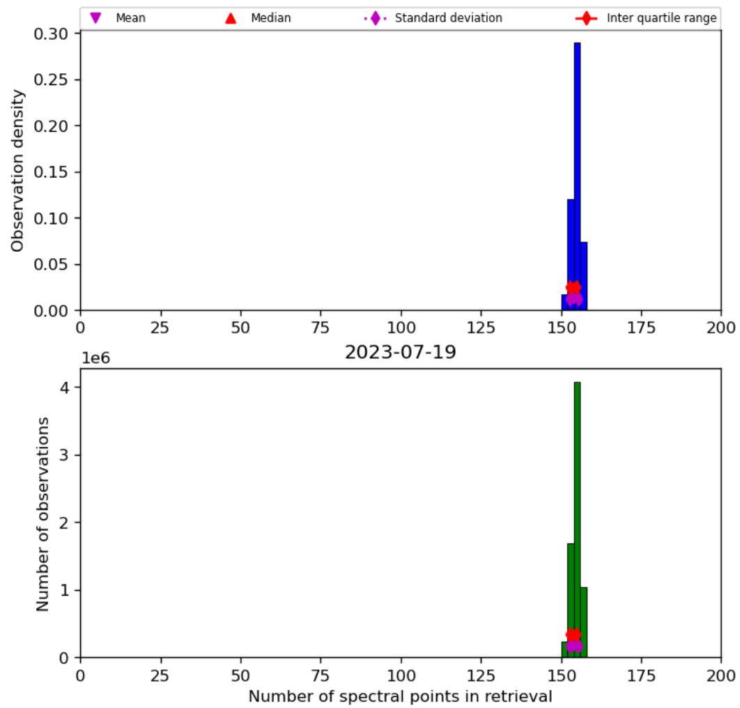
Figure 21: Histogram of “Number of spectral points in retrieval” for 2023-07-19 to 2023-07-20
