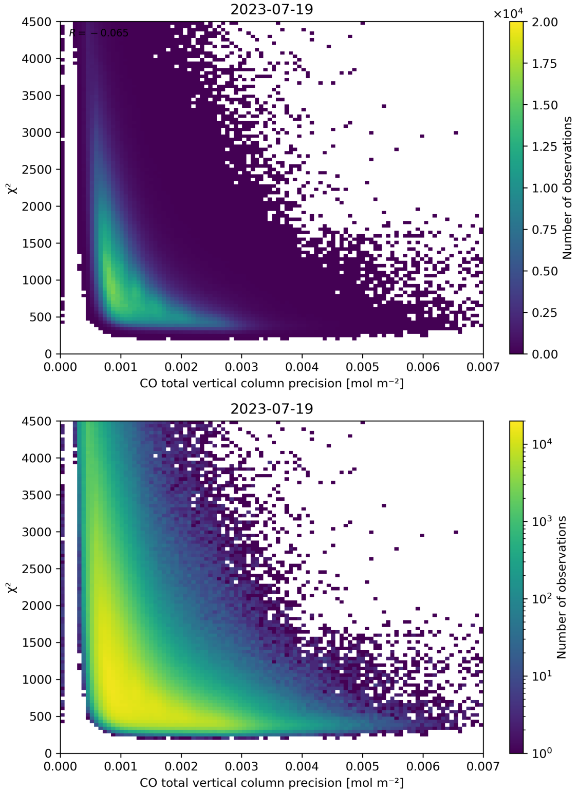
Figure 44: Scatter density plot of “CO total vertical column precision” against “ \chi^2 ” for 2023-07-19 to 2023-07-20.
