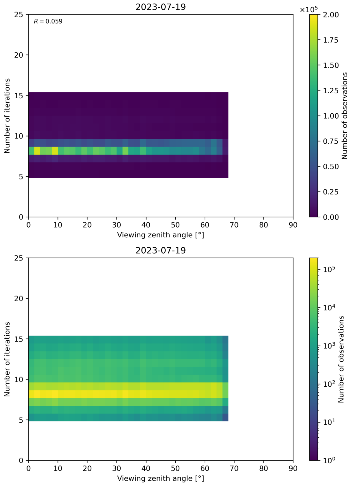
Figure 75: Scatter density plot of “Viewing zenith angle” against “Number of iterations” for 2023-07-19 to 2023-07-20.
