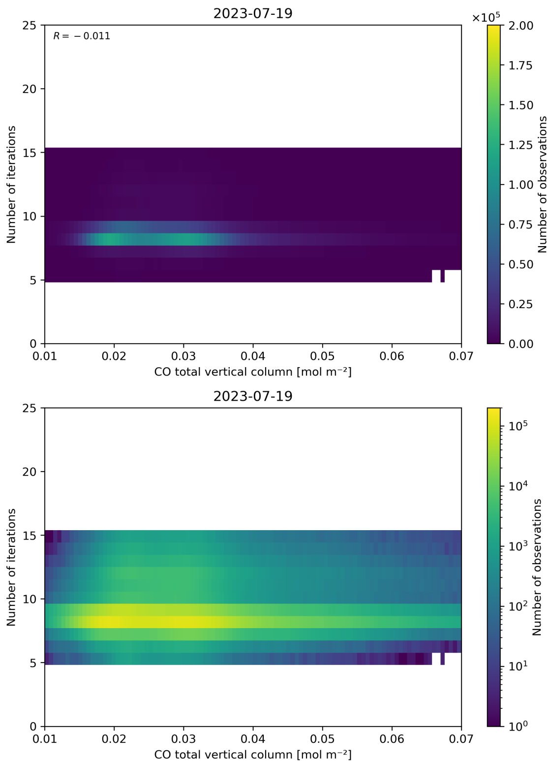
Figure 42: Scatter density plot of “CO total vertical column” against “Number of iterations” for 2023-07-19 to 2023-07-20.
