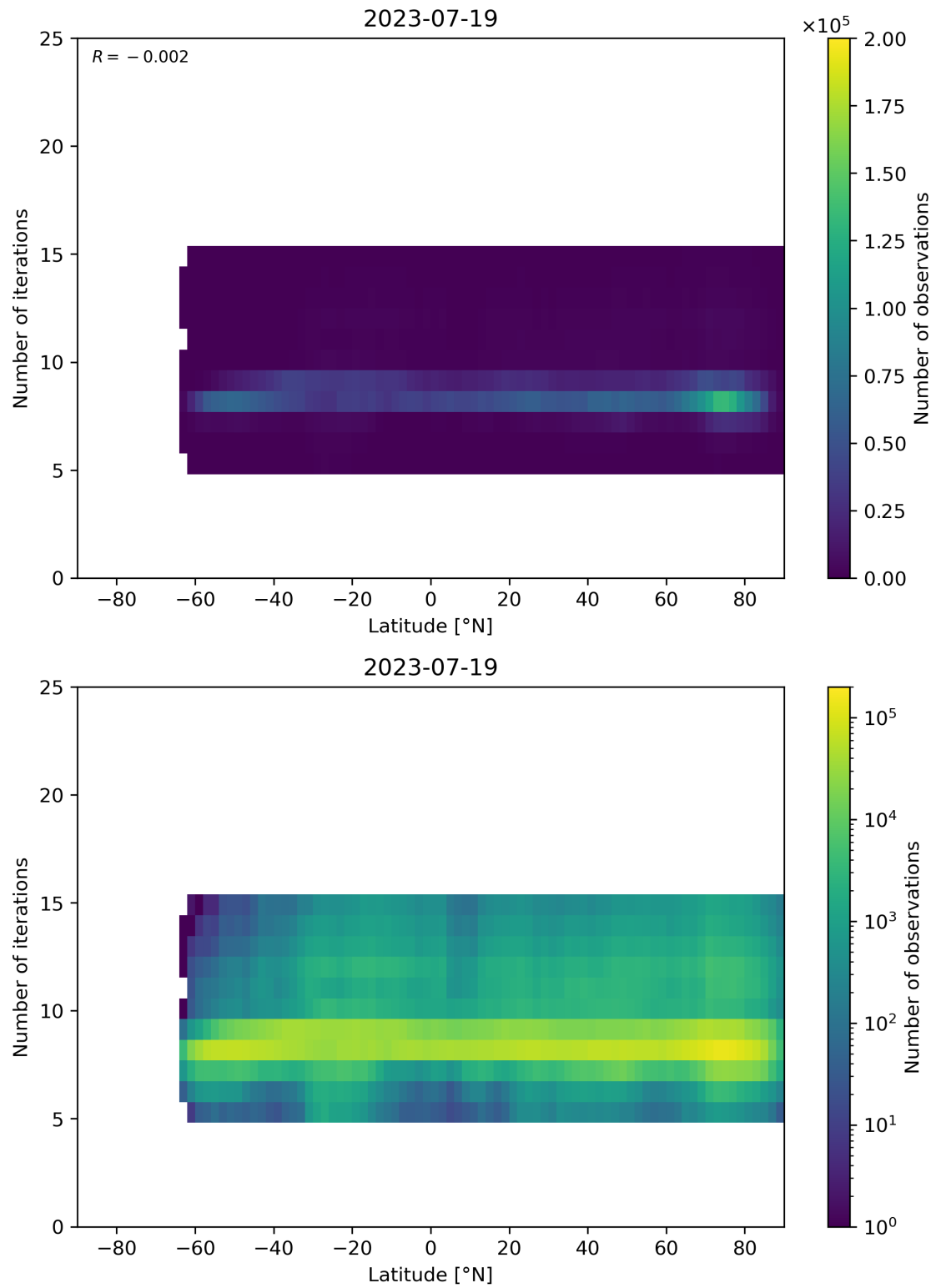
Figure 56: Scatter density plot of “Latitude” against “Number of iterations” for 2023-07-19 to 2023-07-20.
