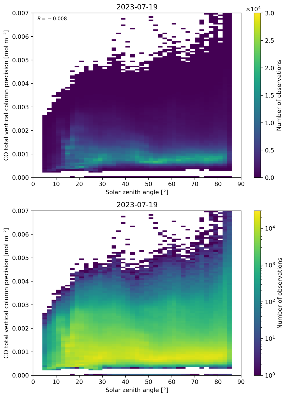
Figure 63: Scatter density plot of “Solar zenith angle” against “CO total vertical column precision” for 2023-07-19 to 2023-07-20.
