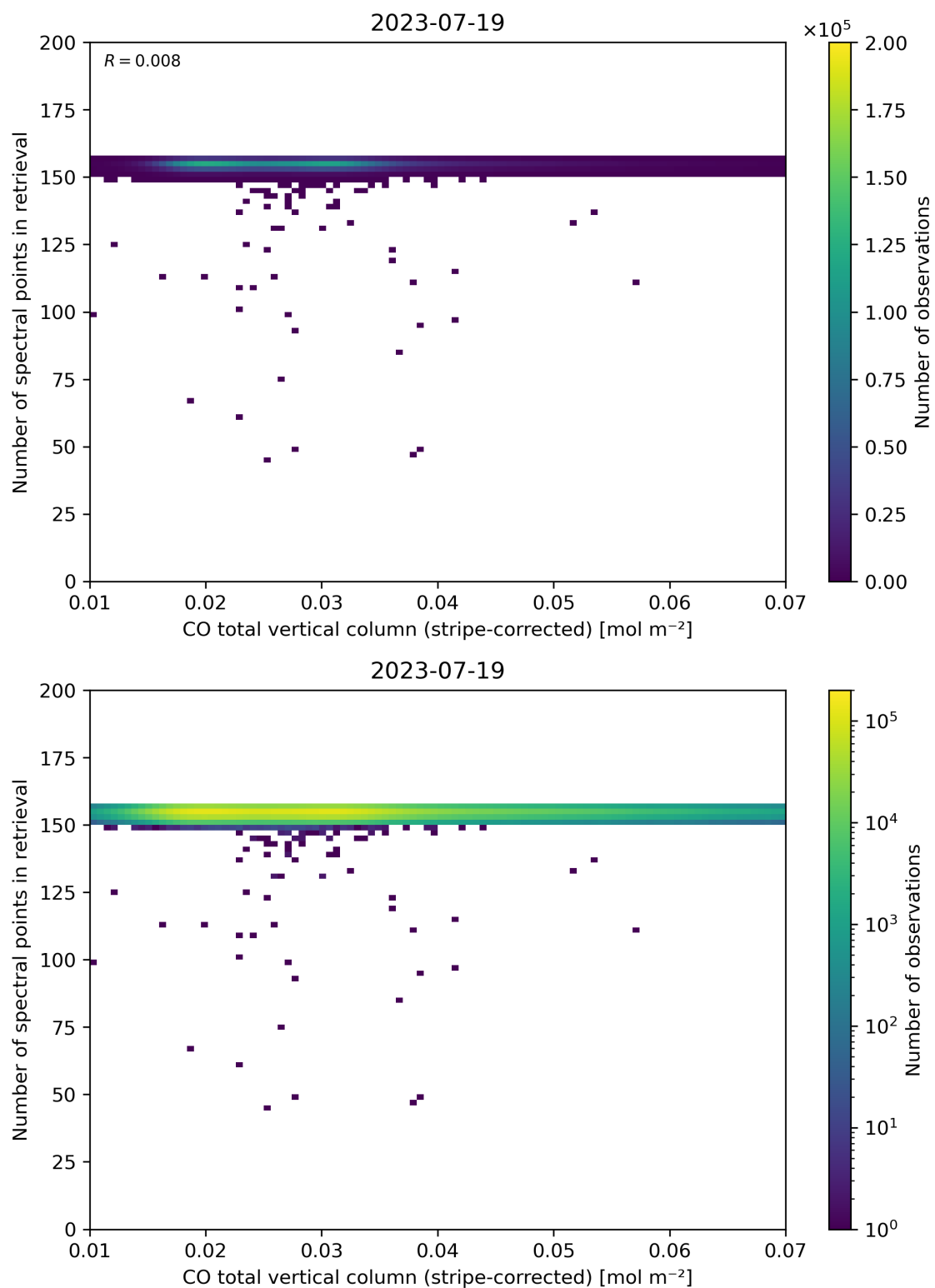
Figure 40: Scatter density plot of “CO total vertical column (stripe-corrected)” against “Number of spectral points in retrieval” for 2023-07-19 to 2023-07-20.
