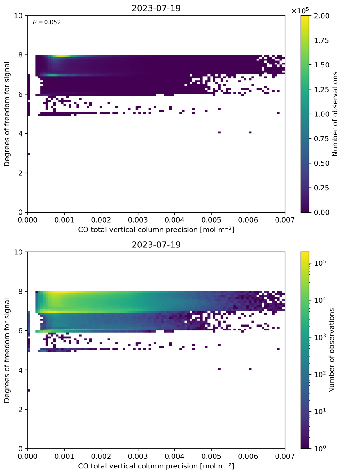
Figure 45: Scatter density plot of “CO total vertical column precision” against “Degrees of freedom for signal” for 2023-07-19 to 2023-07-20.
