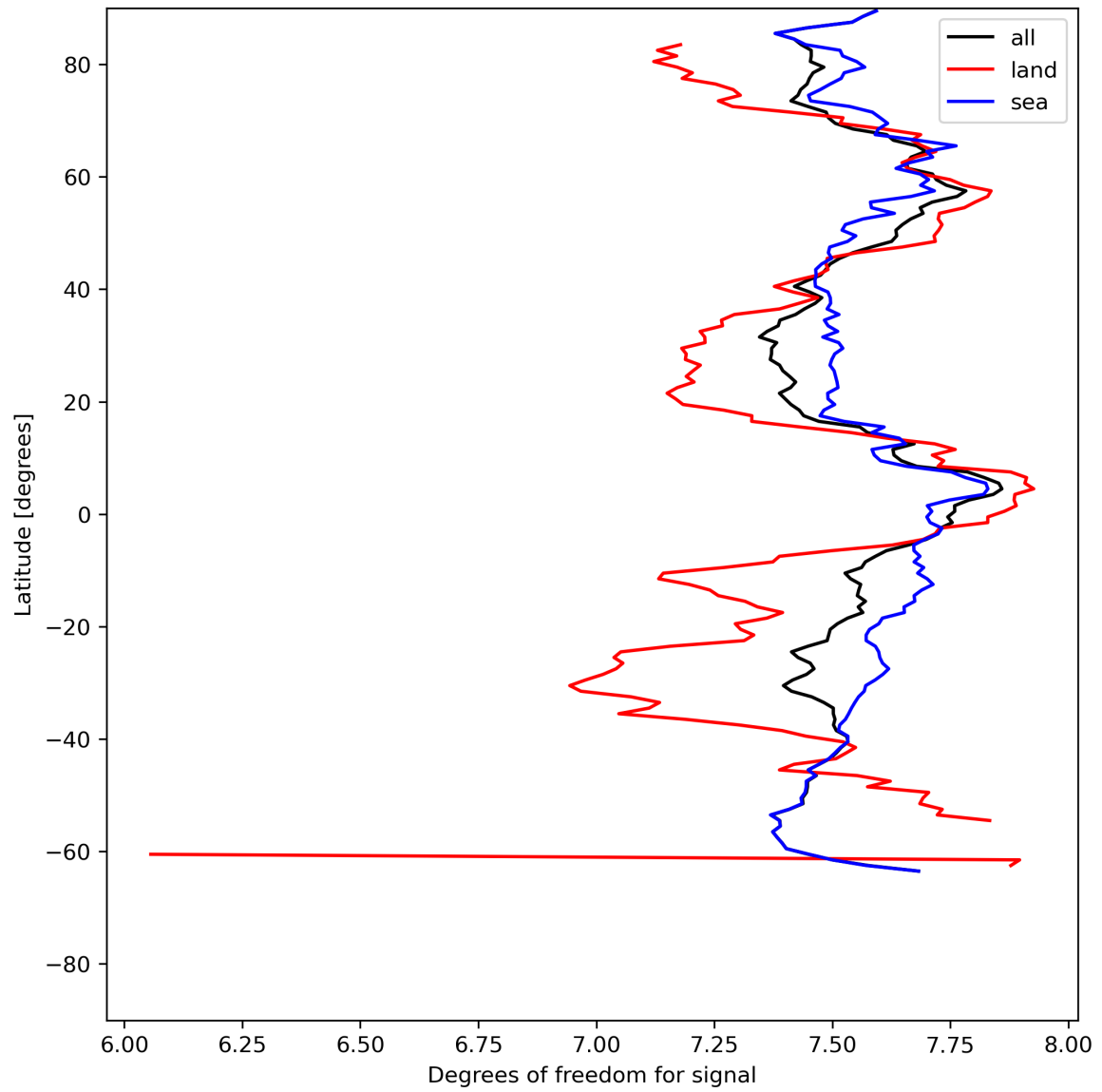
Figure 15: Zonal average of “Degrees of freedom for signal” for 2023-07-19 to 2023-07-20.
