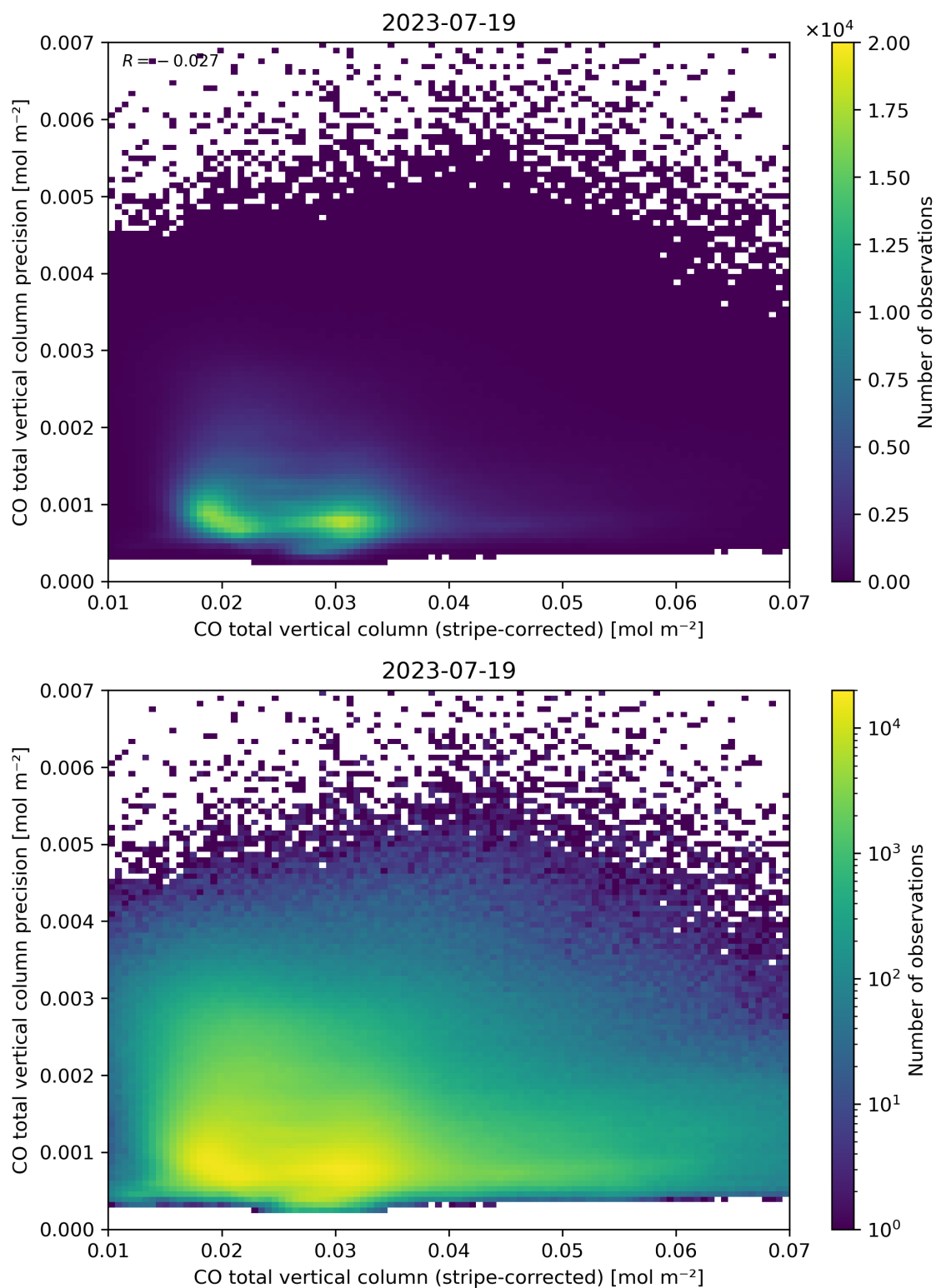
Figure 36: Scatter density plot of “CO total vertical column (stripe-corrected)” against “CO total vertical column precision” for 2023-07-19 to 2023-07-20.
