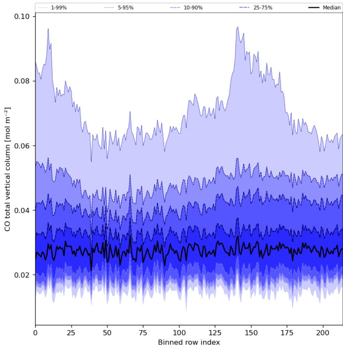
Figure 26: Along track statistics of “CO total vertical column” for 2023-07-19 to 2023-07-20
