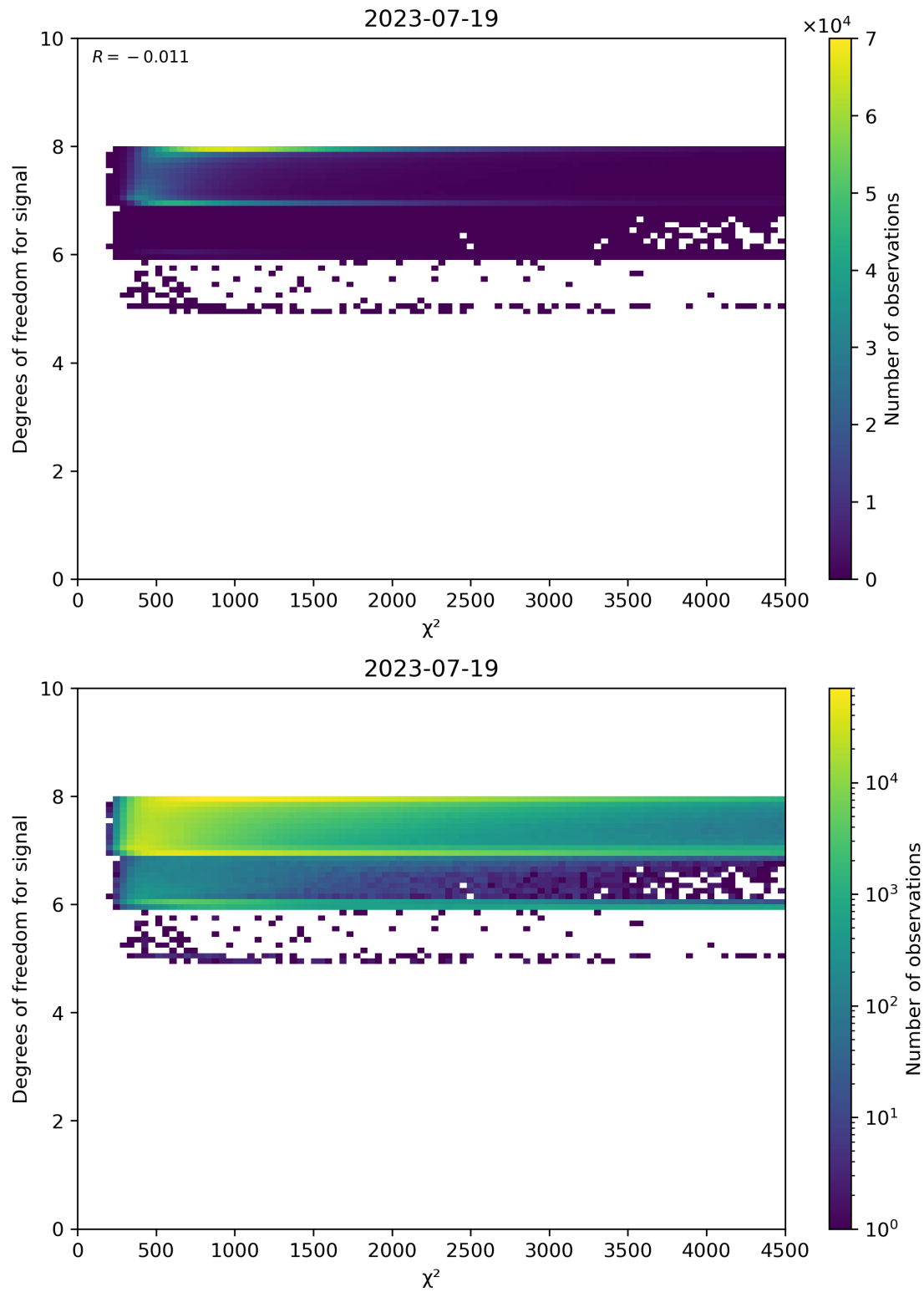
Figure 48: Scatter density plot of “ \chi^2 ” against “Degrees of freedom for signal” for 2023-07-19 to 2023-07-20.
