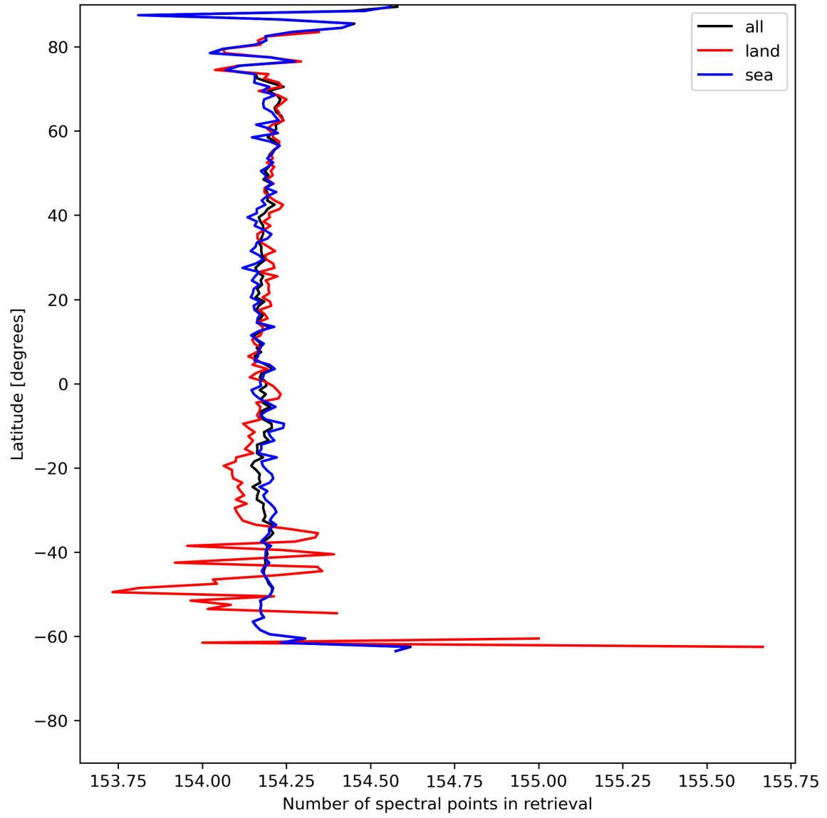
Figure 13: Zonal average of “Number of spectral points in retrieval” for 2023-07-19 to 2023-07-20.
