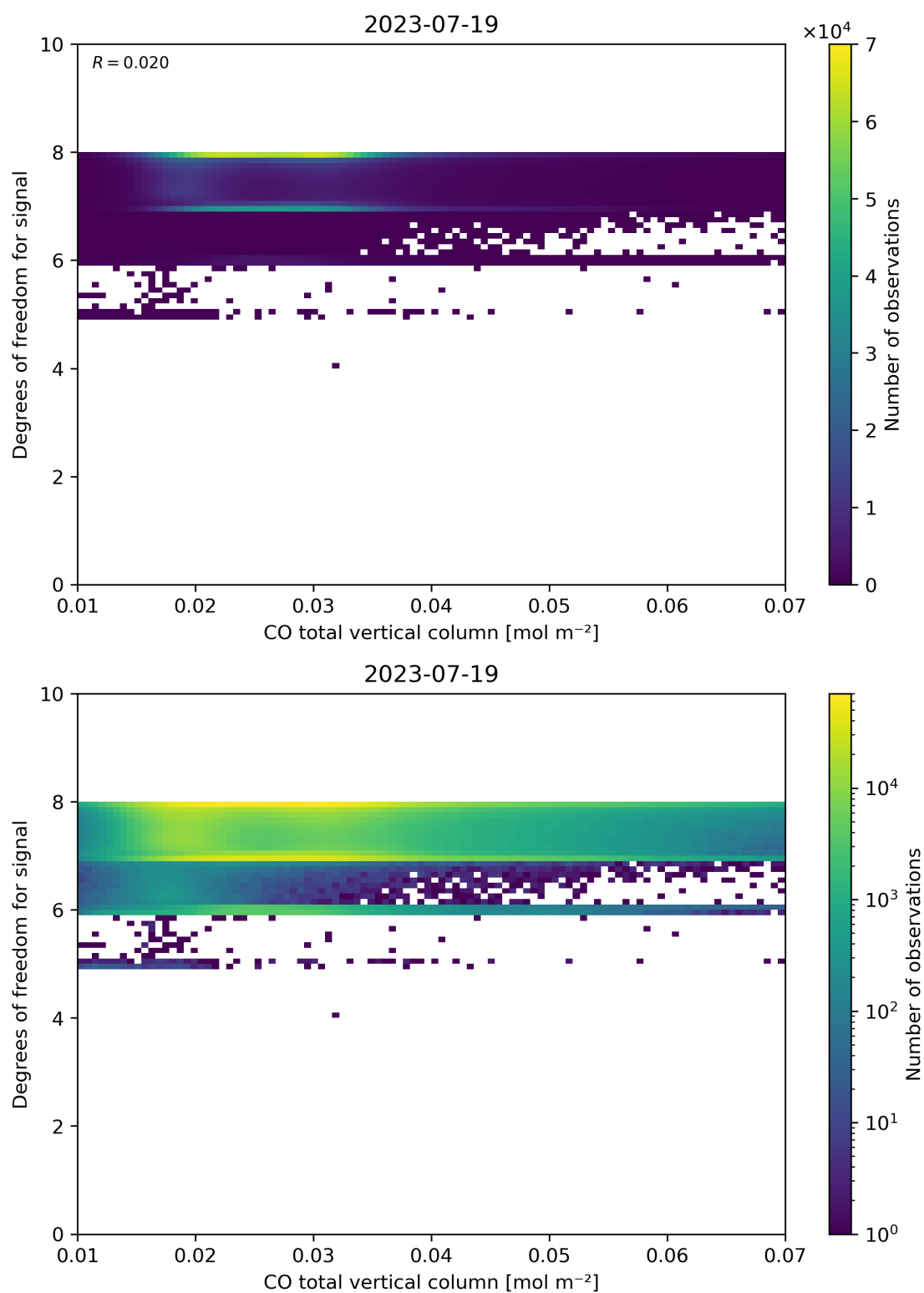
Figure 41: Scatter density plot of “CO total vertical column” against “Degrees of freedom for signal” for 2023-07-19 to 2023-07-20.
