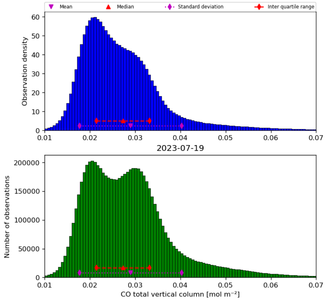
Figure 18: Histogram of “CO total vertical column” for 2023-07-19 to 2023-07-20
