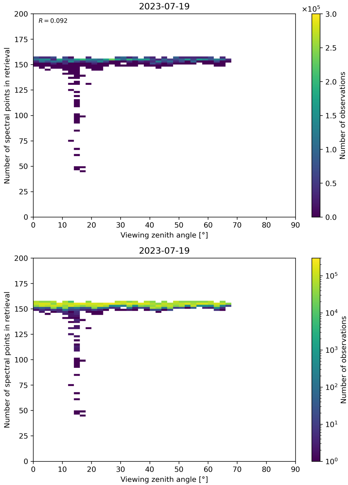
Figure 76: Scatter density plot of “Viewing zenith angle” against “Number of spectral points in retrieval” for 2023-07-19 to 2023-07-20.
