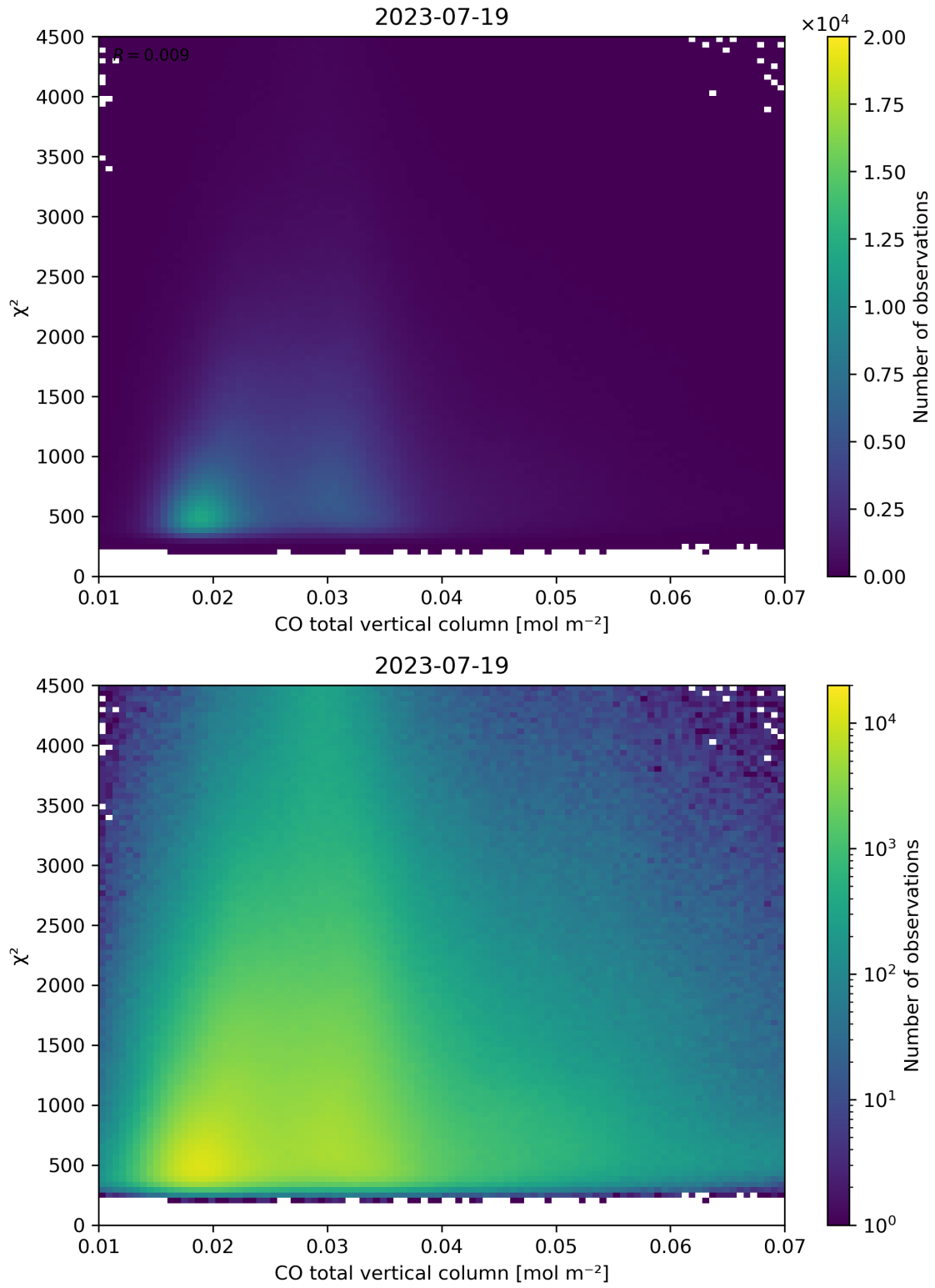
Figure 35: Scatter density plot of “CO total vertical column” against “ \chi^2 ” for 2023-07-19 to 2023-07-20.
