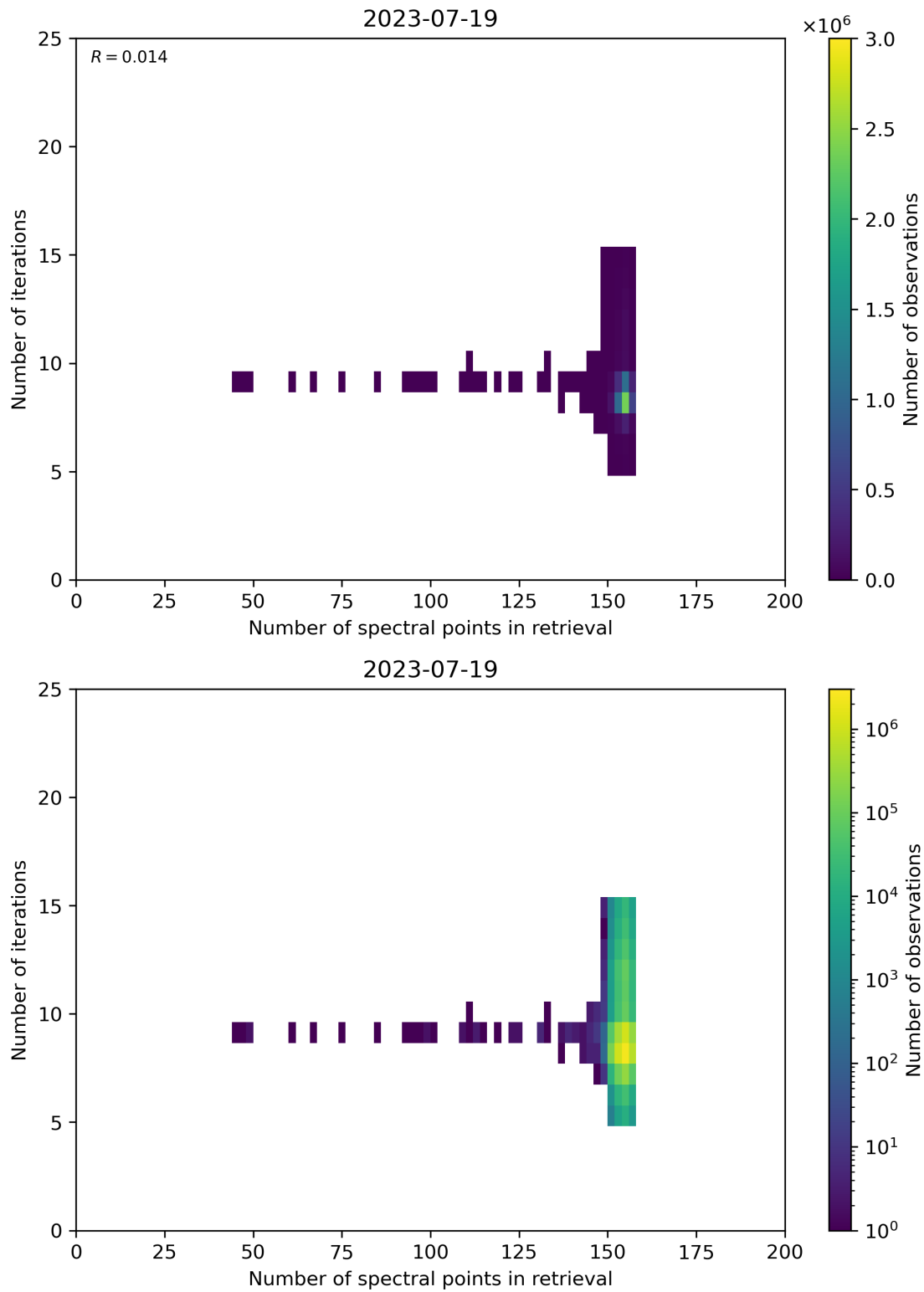
Figure 60: Scatter density plot of “Number of spectral points in retrieval” against “Number of iterations” for 2023-07-19 to 2023-07-20.
