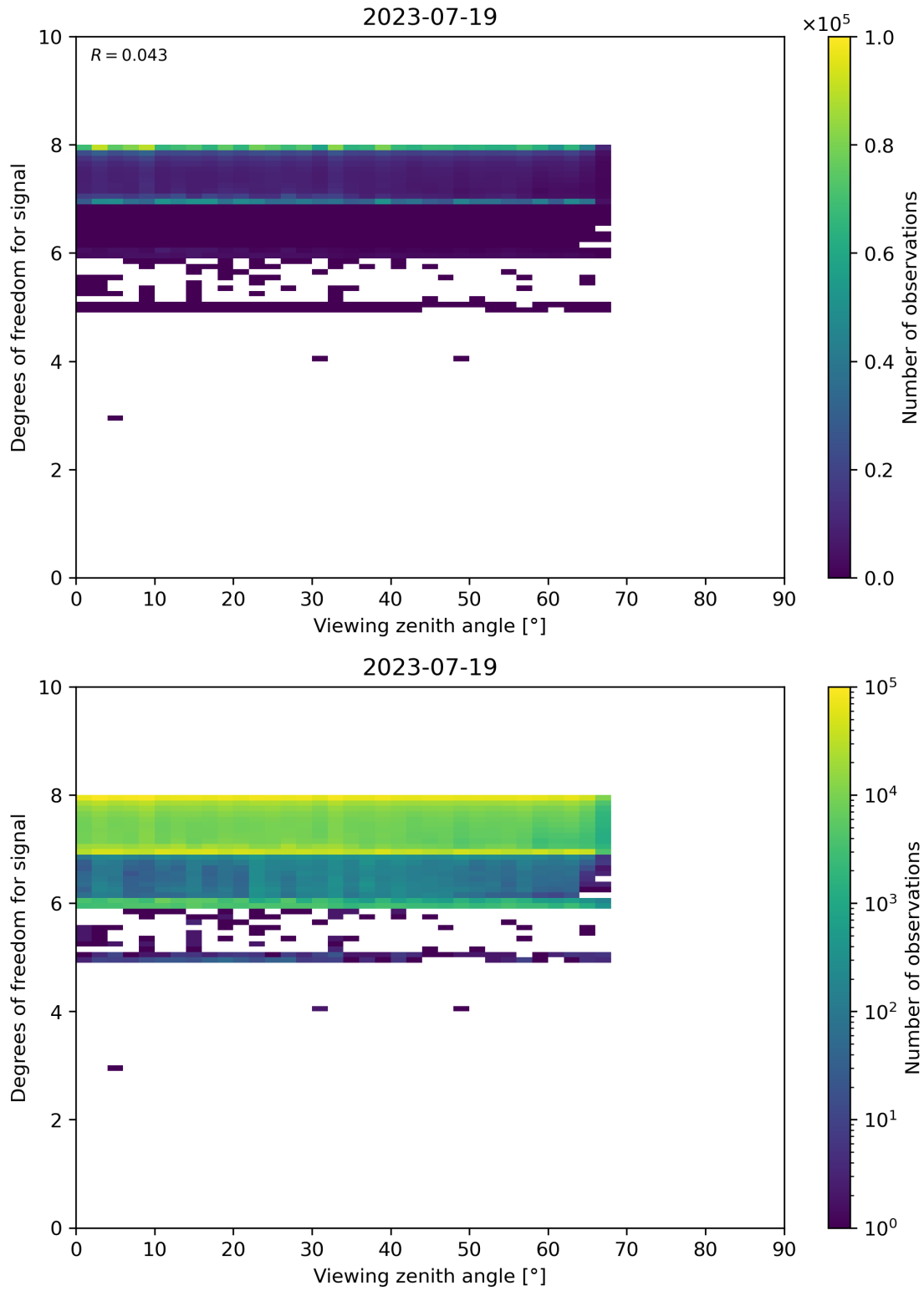
Figure 73: Scatter density plot of “Viewing zenith angle” against “Degrees of freedom for signal” for 2023-07-19 to 2023-07-20.
