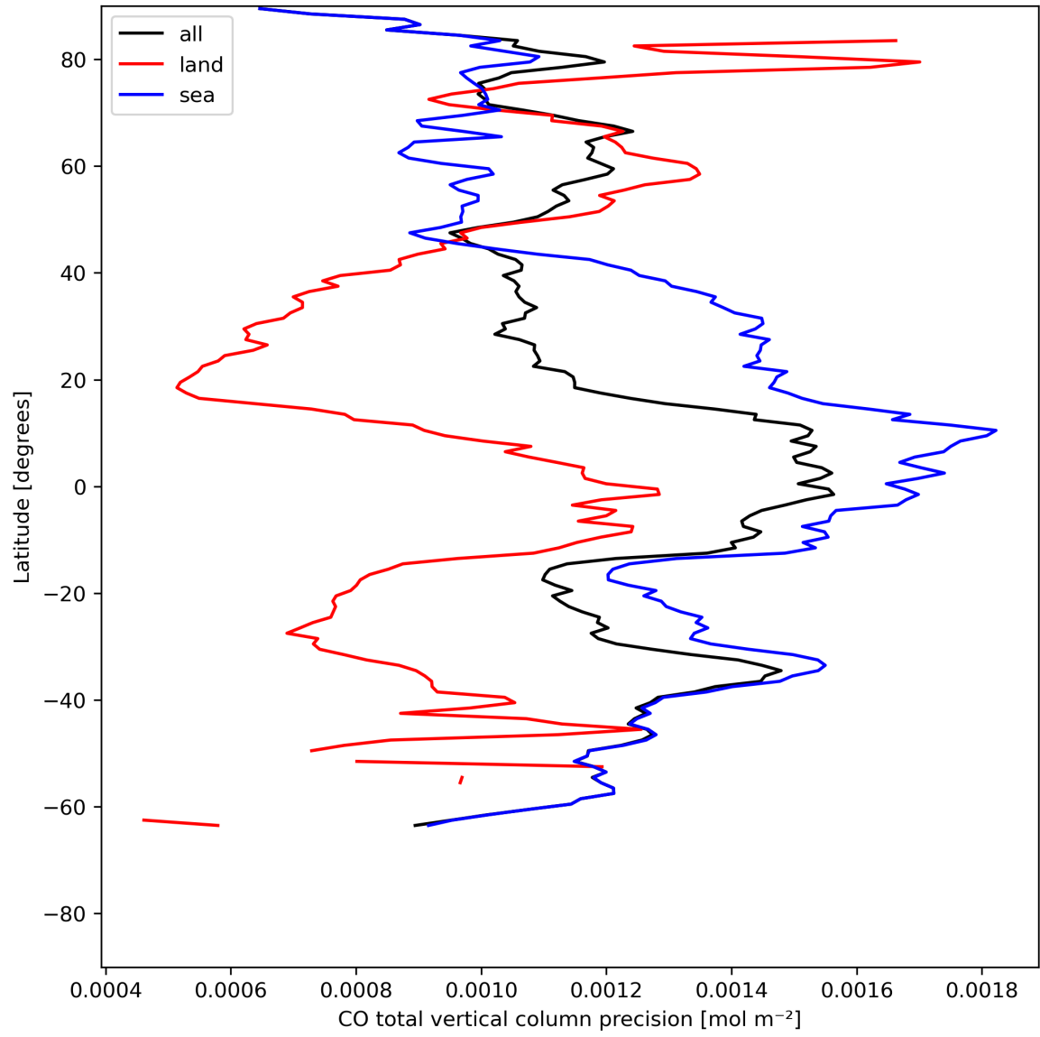
Figure 12: Zonal average of “CO total vertical column precision” for 2023-07-19 to 2023-07-21.
