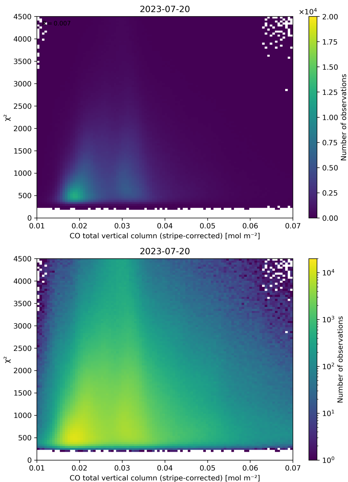
Figure 37: Scatter density plot of “CO total vertical column (stripe-corrected)” against “ \chi^2 ” for 2023-07-19 to 2023-07-21.
