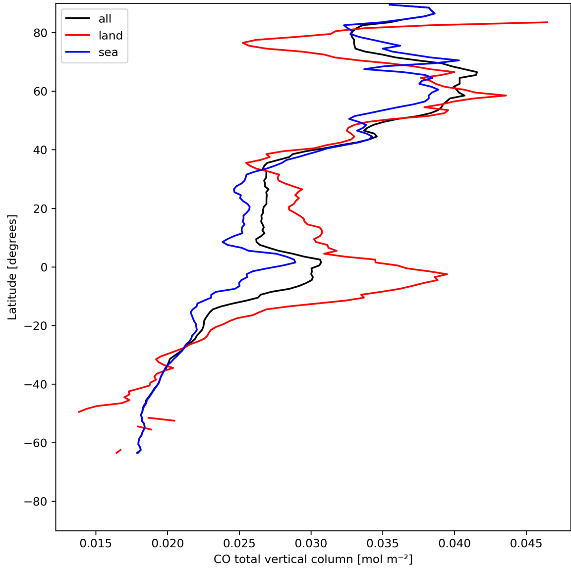
Figure 10: Zonal average of “CO total vertical column” for 2023-07-19 to 2023-07-21.
