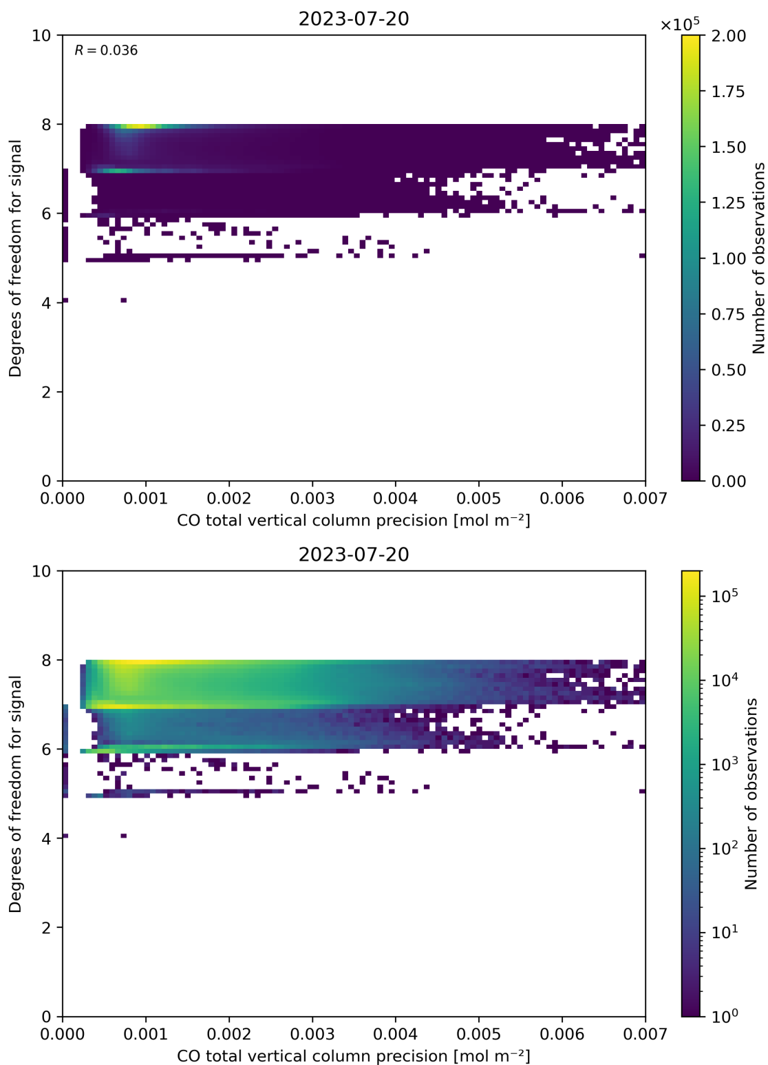
Figure 45: Scatter density plot of “CO total vertical column precision” against “Degrees of freedom for signal” for 2023-07-19 to 2023-07-21.
