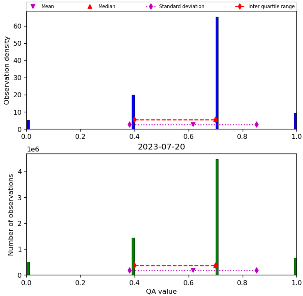
Figure 17: Histogram of “QA value” for 2023-07-19 to 2023-07-21
