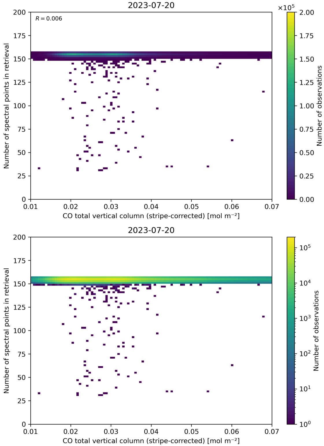
Figure 40: Scatter density plot of “CO total vertical column (stripe-corrected)” against “Number of spectral points in retrieval” for 2023-07-19 to 2023-07-21.
