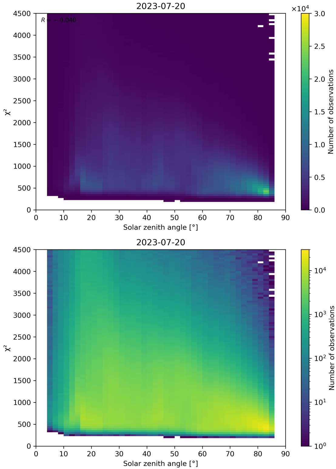
Figure 64: Scatter density plot of “Solar zenith angle” against “ \chi^2 ” for 2023-07-19 to 2023-07-21.
