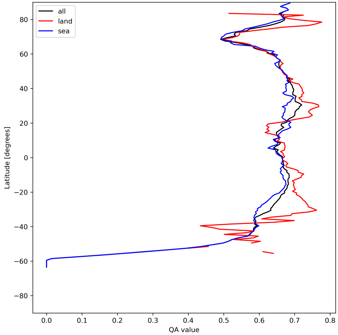
Figure 9: Zonal average of “QA value” for 2023-07-19 to 2023-07-21.
