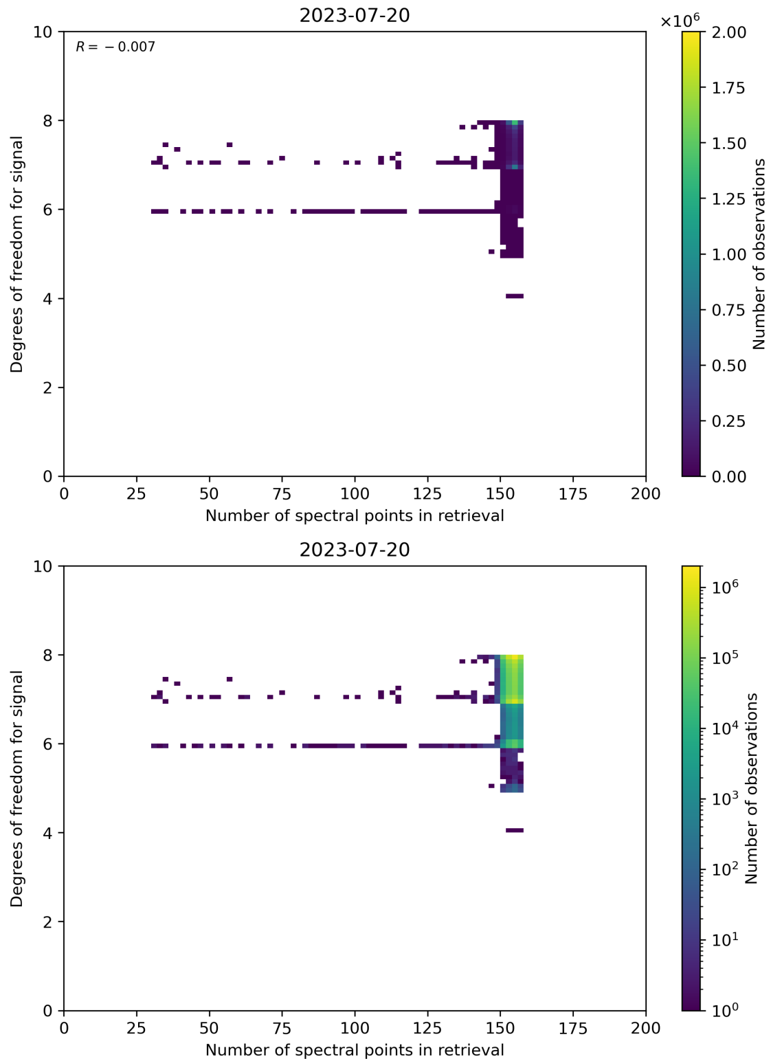
Figure 59: Scatter density plot of “Number of spectral points in retrieval” against “Degrees of freedom for signal” for 2023-07-19 to 2023-07-21.
