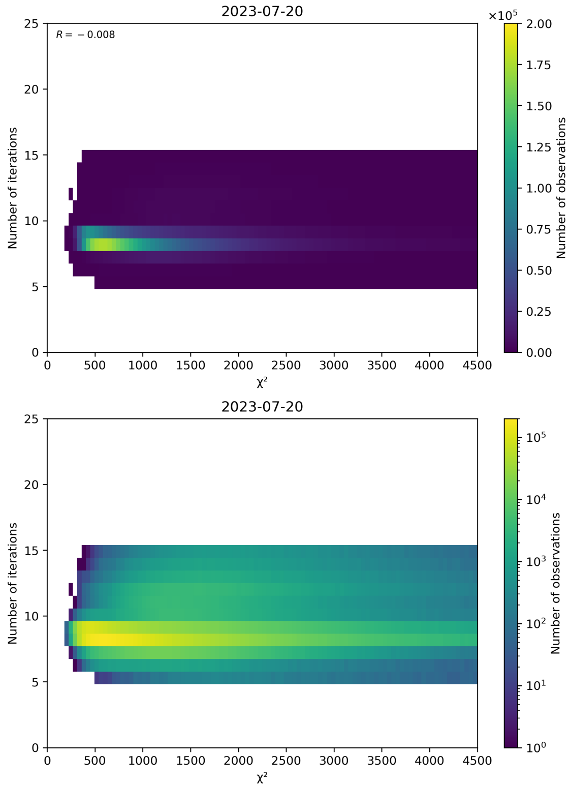
Figure 49: Scatter density plot of “ \chi^2 ” against “Number of iterations” for 2023-07-19 to 2023-07-21.
