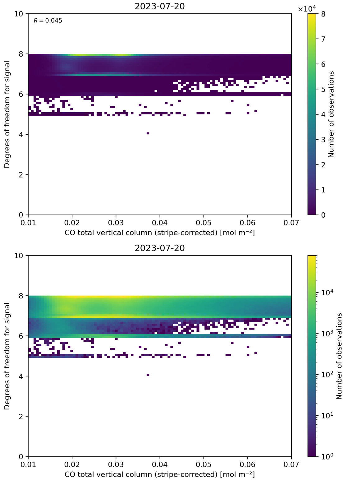
Figure 38: Scatter density plot of “CO total vertical column (stripe-corrected)” against “Degrees of freedom for signal” for 2023-07-19 to 2023-07-21.
