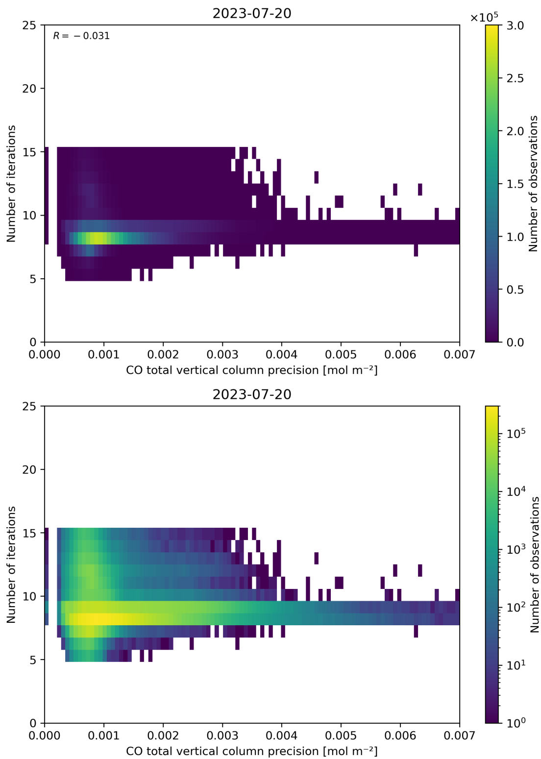
Figure 46: Scatter density plot of “CO total vertical column precision” against “Number of iterations” for 2023-07-19 to 2023-07-21.
