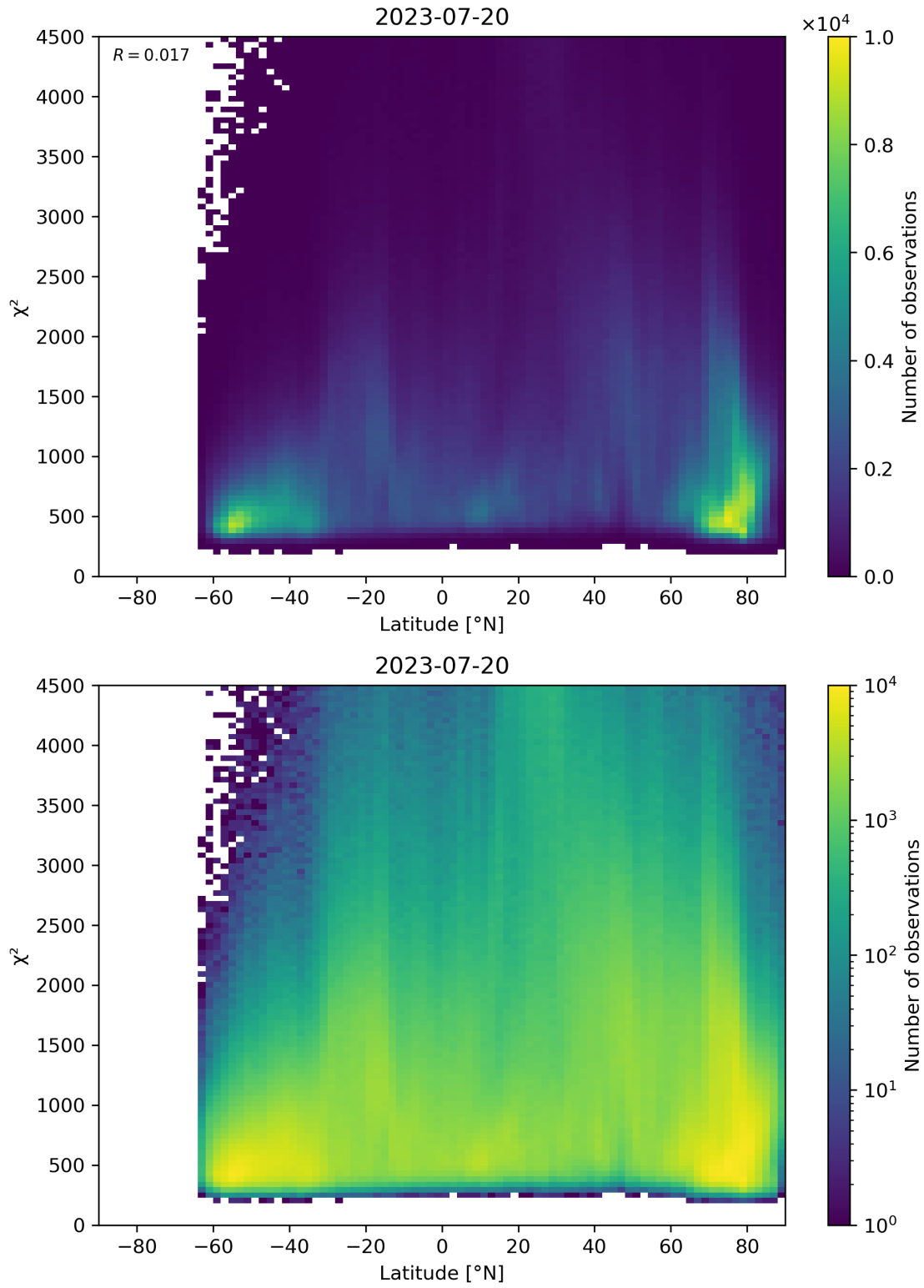
Figure 54: Scatter density plot of “Latitude” against “ \chi^2 ” for 2023-07-19 to 2023-07-21.
