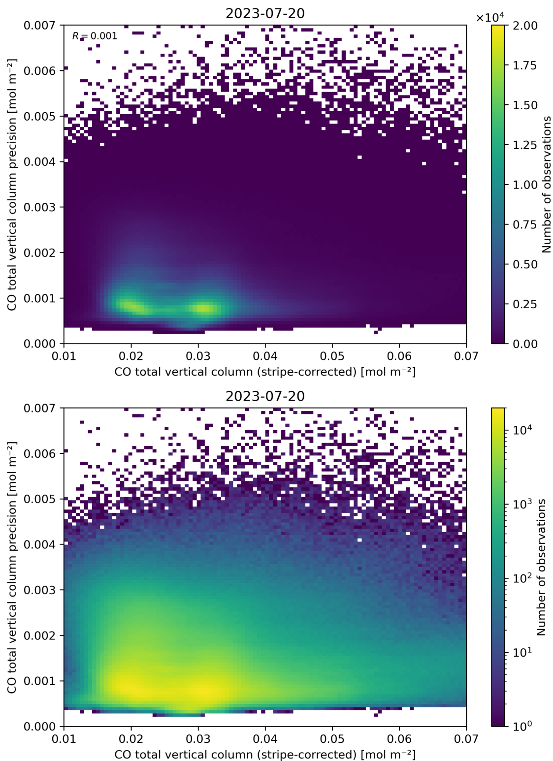
Figure 36: Scatter density plot of “CO total vertical column (stripe-corrected)” against “CO total vertical column precision” for 2023-07-19 to 2023-07-21.
