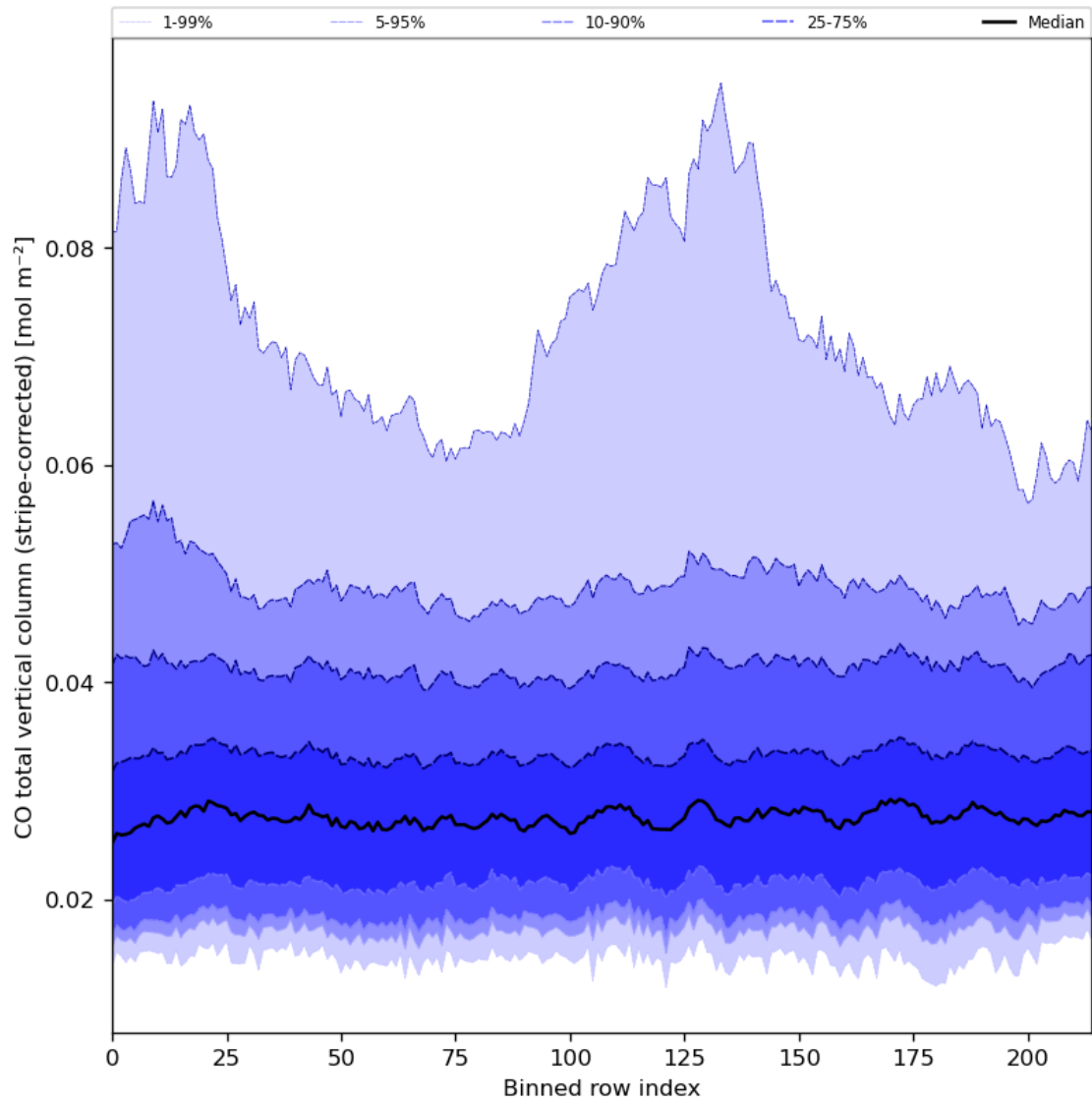
Figure 27: Along track statistics of “CO total vertical column (stripe-corrected)” for 2023-07-19 to 2023-07-21
