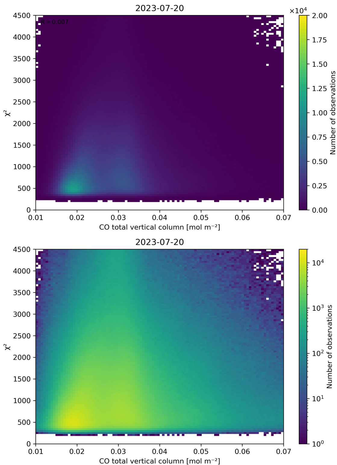
Figure 35: Scatter density plot of “CO total vertical column” against “ \chi^2 ” for 2023-07-19 to 2023-07-21.
