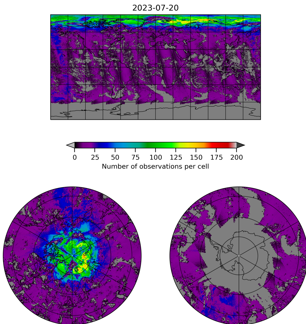
Figure 8: Map of the number of observations for 2023-07-19 to 2023-07-21
