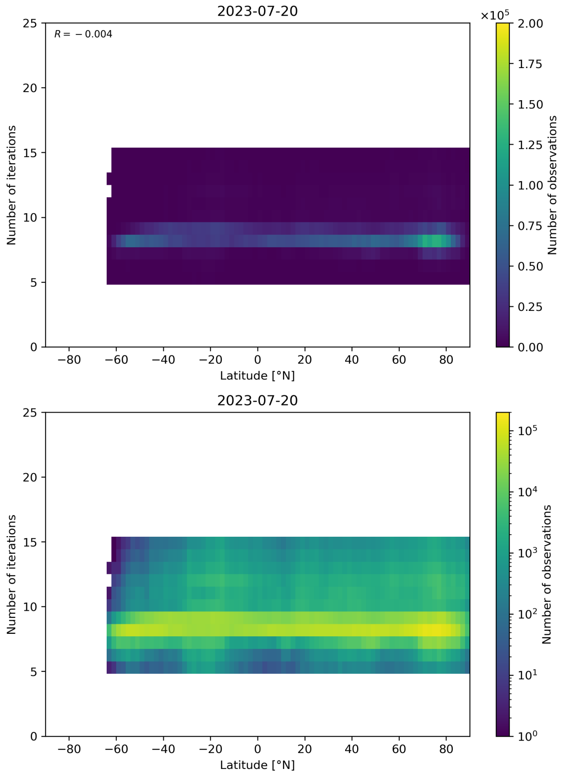
Figure 56: Scatter density plot of “Latitude” against “Number of iterations” for 2023-07-19 to 2023-07-21.
