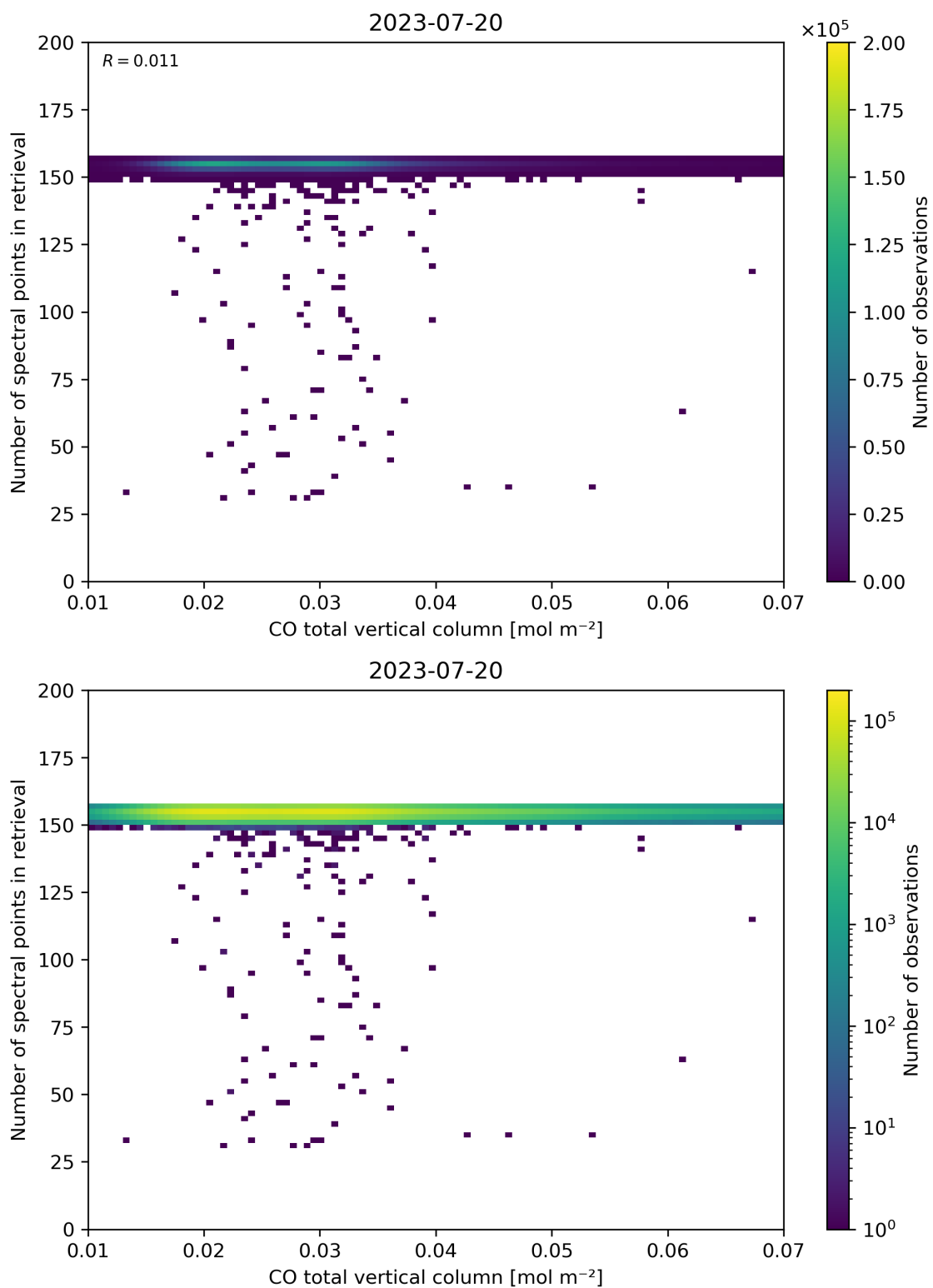
Figure 43: Scatter density plot of “CO total vertical column” against “Number of spectral points in retrieval” for 2023-07-19 to 2023-07-21.
