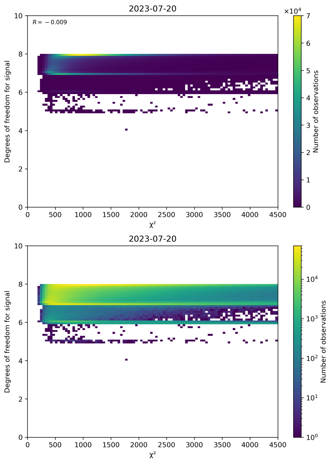
Figure 48: Scatter density plot of “ \chi^2 ” against “Degrees of freedom for signal” for 2023-07-19 to 2023-07-21.
