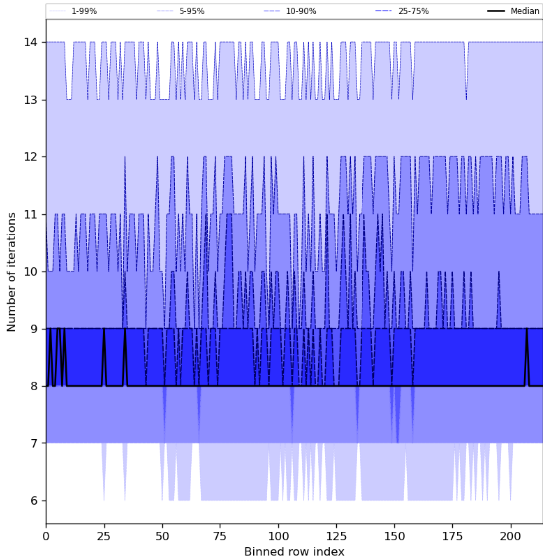
Figure 32: Along track statistics of “Number of iterations” for 2023-07-19 to 2023-07-21
