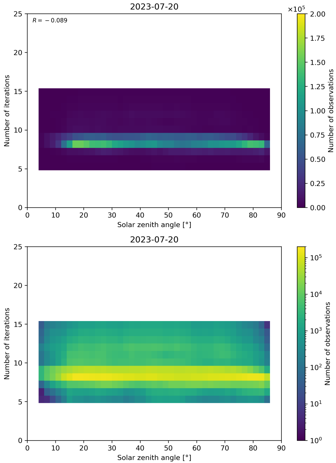
Figure 67: Scatter density plot of “Solar zenith angle” against “Number of iterations” for 2023-07-19 to 2023-07-21.
