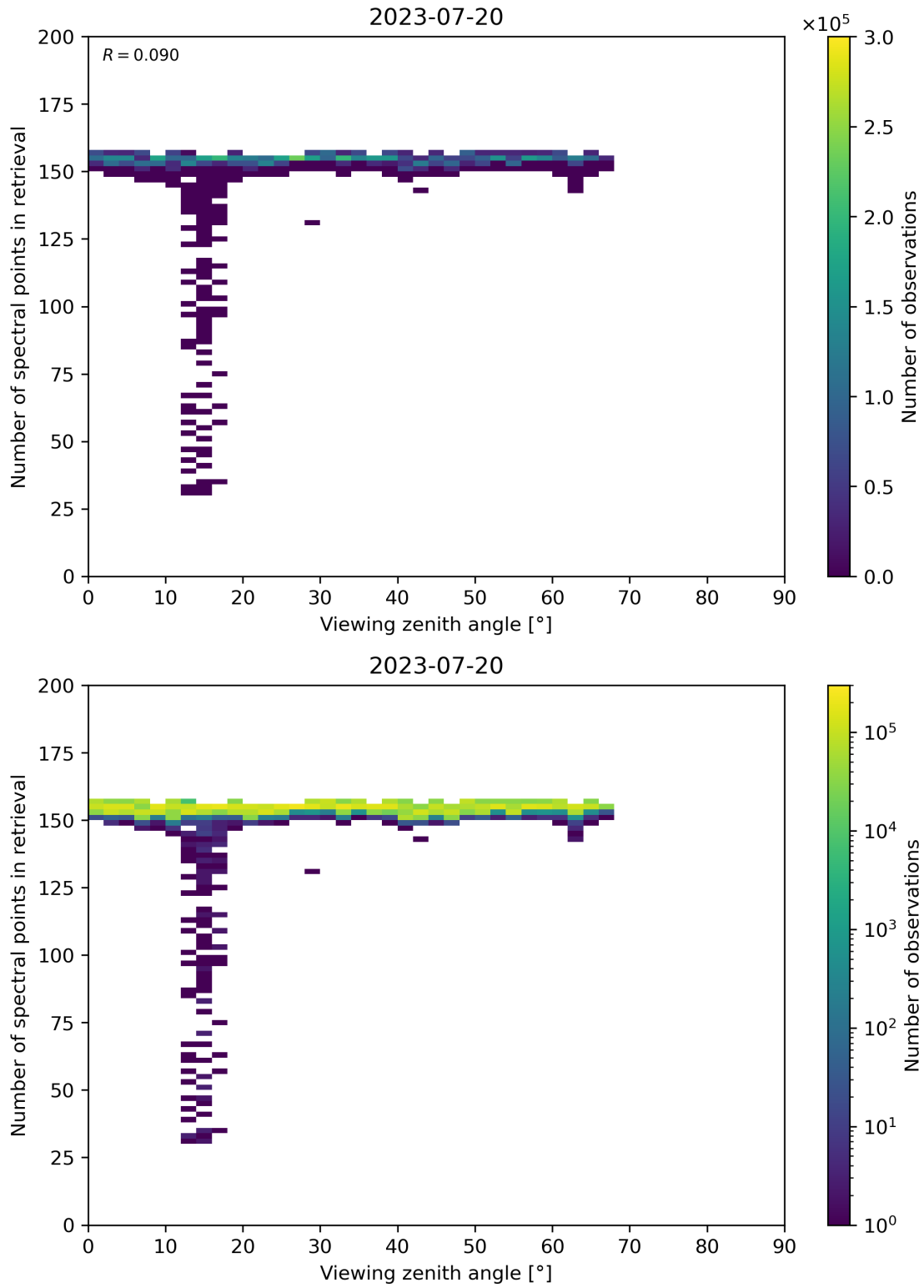
Figure 76: Scatter density plot of “Viewing zenith angle” against “Number of spectral points in retrieval” for 2023-07-19 to 2023-07-21.
