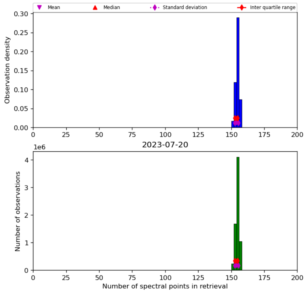
Figure 21: Histogram of “Number of spectral points in retrieval” for 2023-07-19 to 2023-07-21
