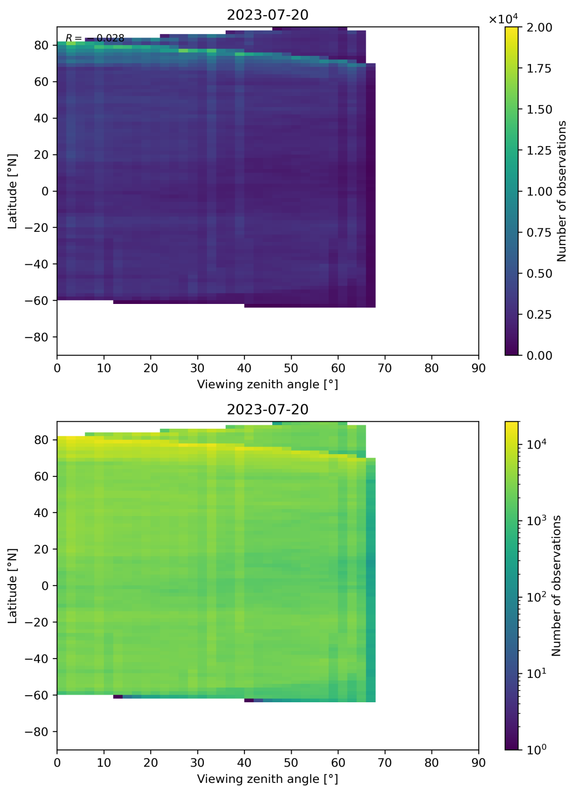
Figure 74: Scatter density plot of “Viewing zenith angle” against “Latitude” for 2023-07-19 to 2023-07-21.
