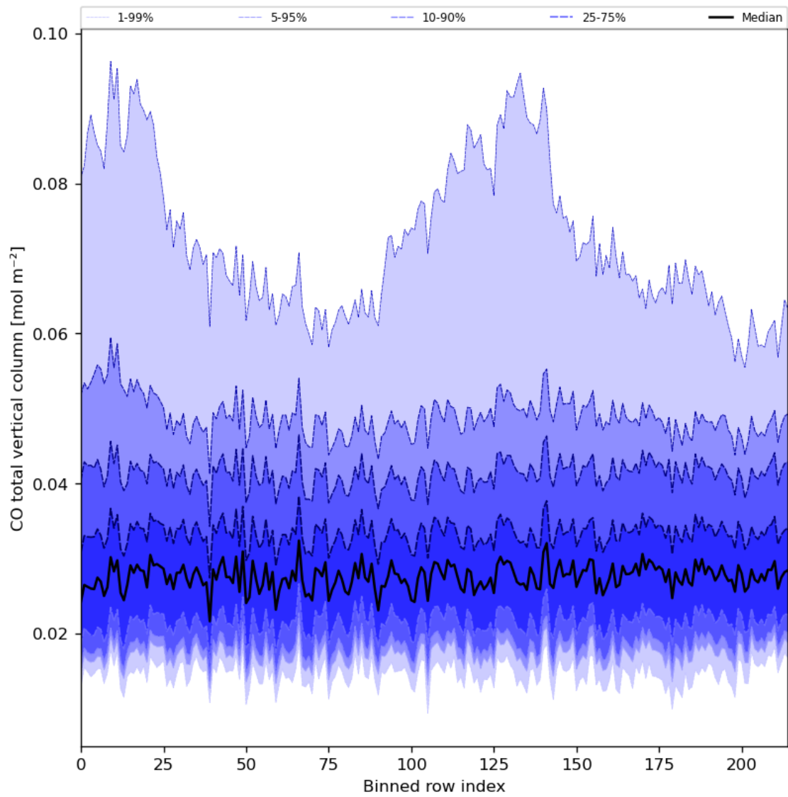
Figure 26: Along track statistics of “CO total vertical column” for 2023-07-19 to 2023-07-21
