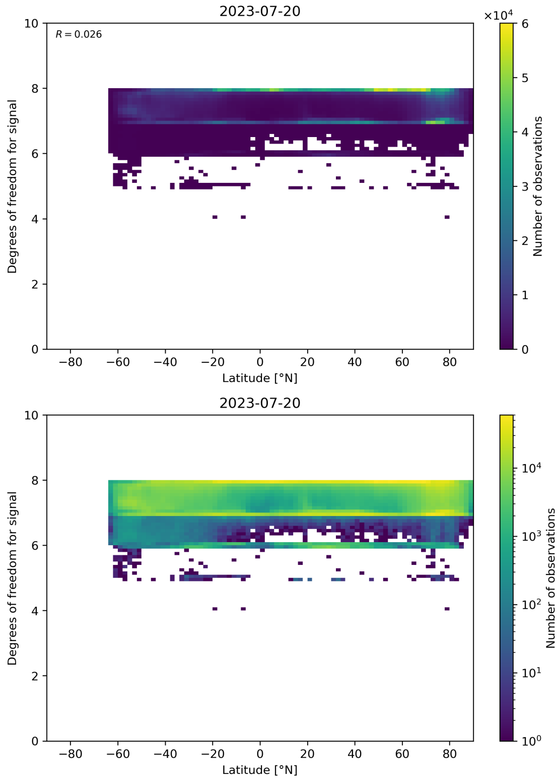
Figure 55: Scatter density plot of “Latitude” against “Degrees of freedom for signal” for 2023-07-19 to 2023-07-21.
