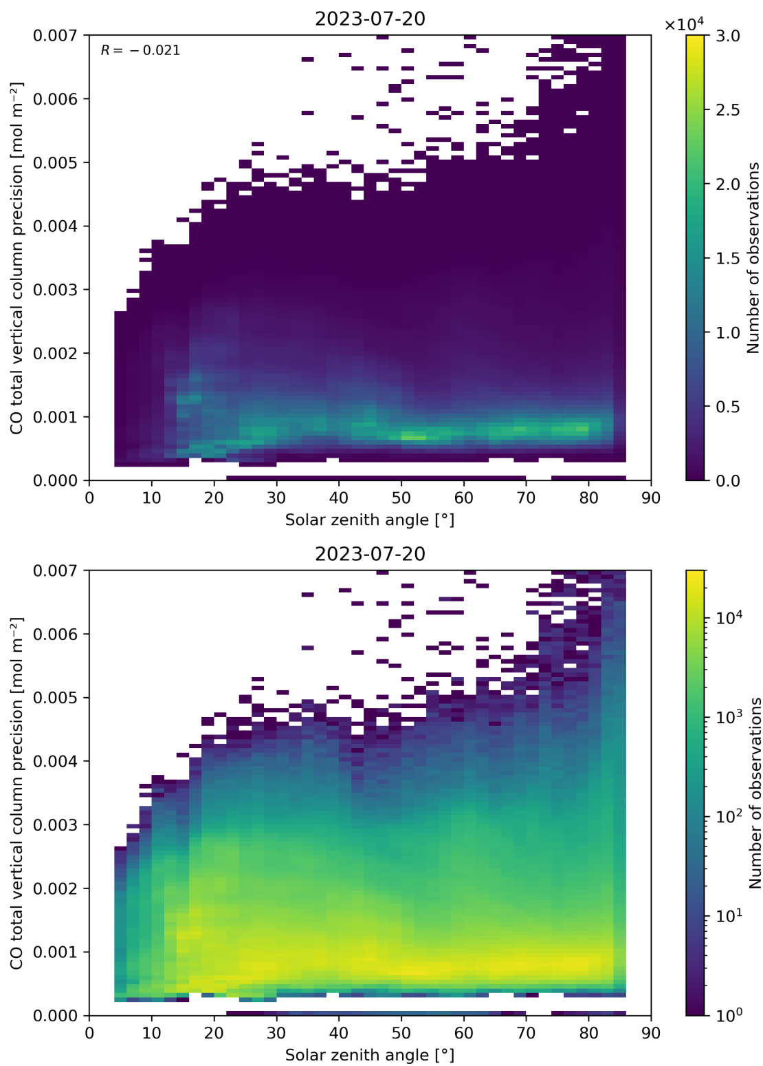
Figure 63: Scatter density plot of “Solar zenith angle” against “CO total vertical column precision” for 2023-07-19 to 2023-07-21.
