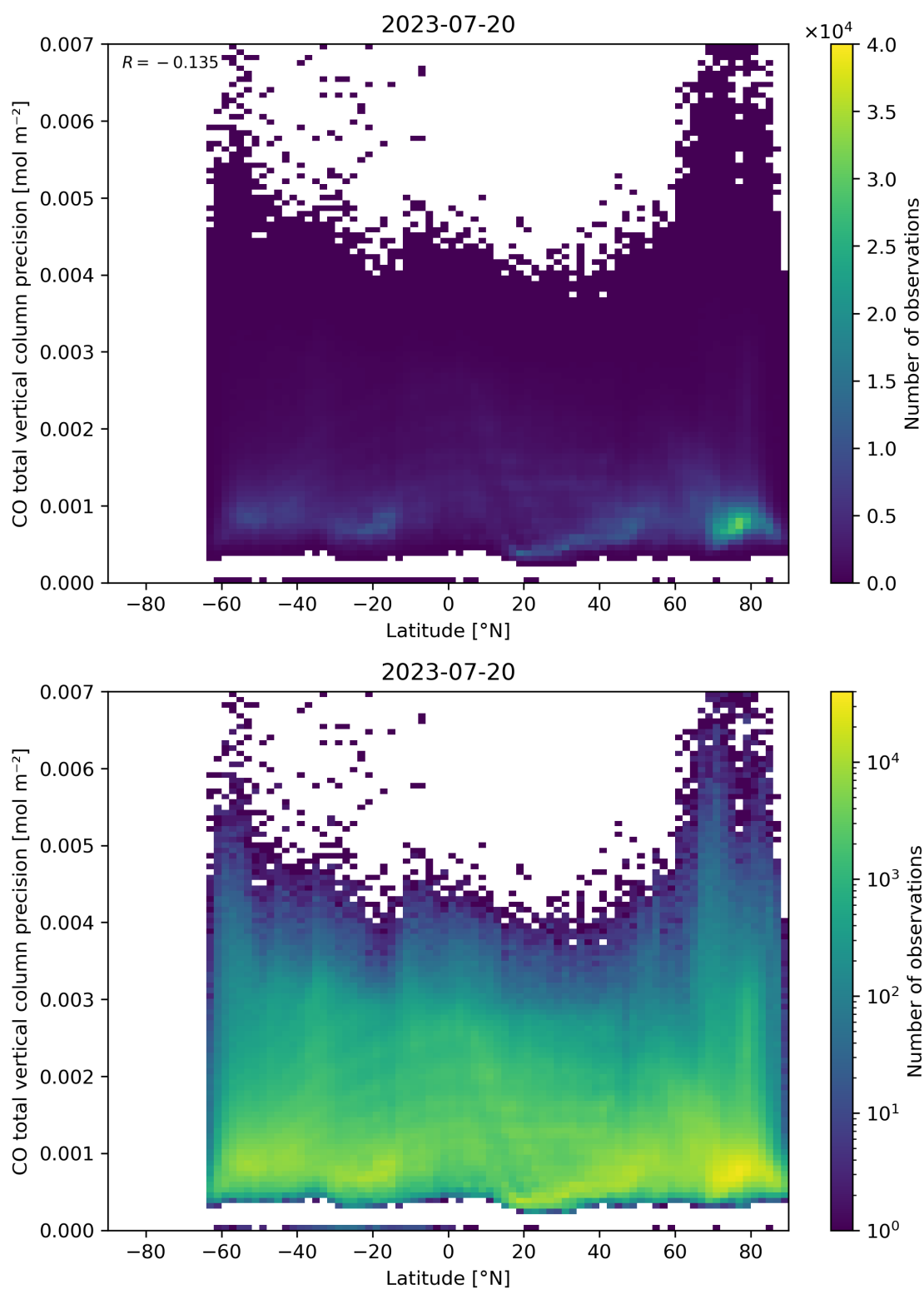
Figure 53: Scatter density plot of “Latitude” against “CO total vertical column precision” for 2023-07-19 to 2023-07-21.
