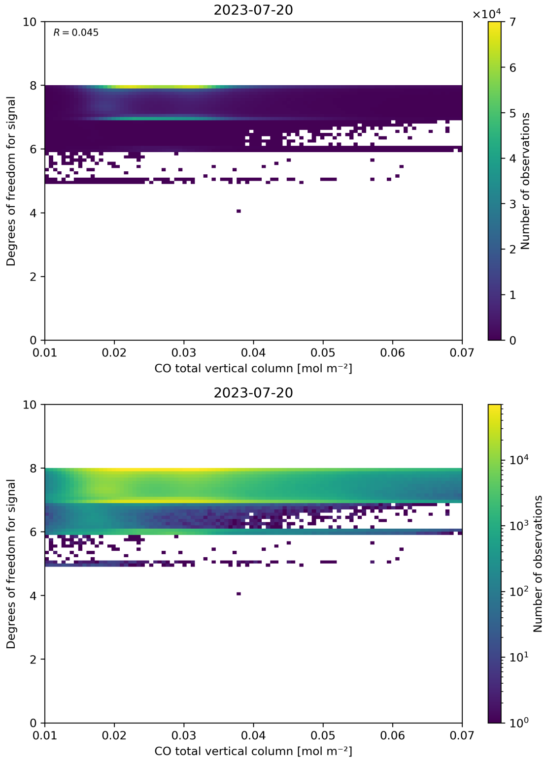
Figure 41: Scatter density plot of “CO total vertical column” against “Degrees of freedom for signal” for 2023-07-19 to 2023-07-21.
