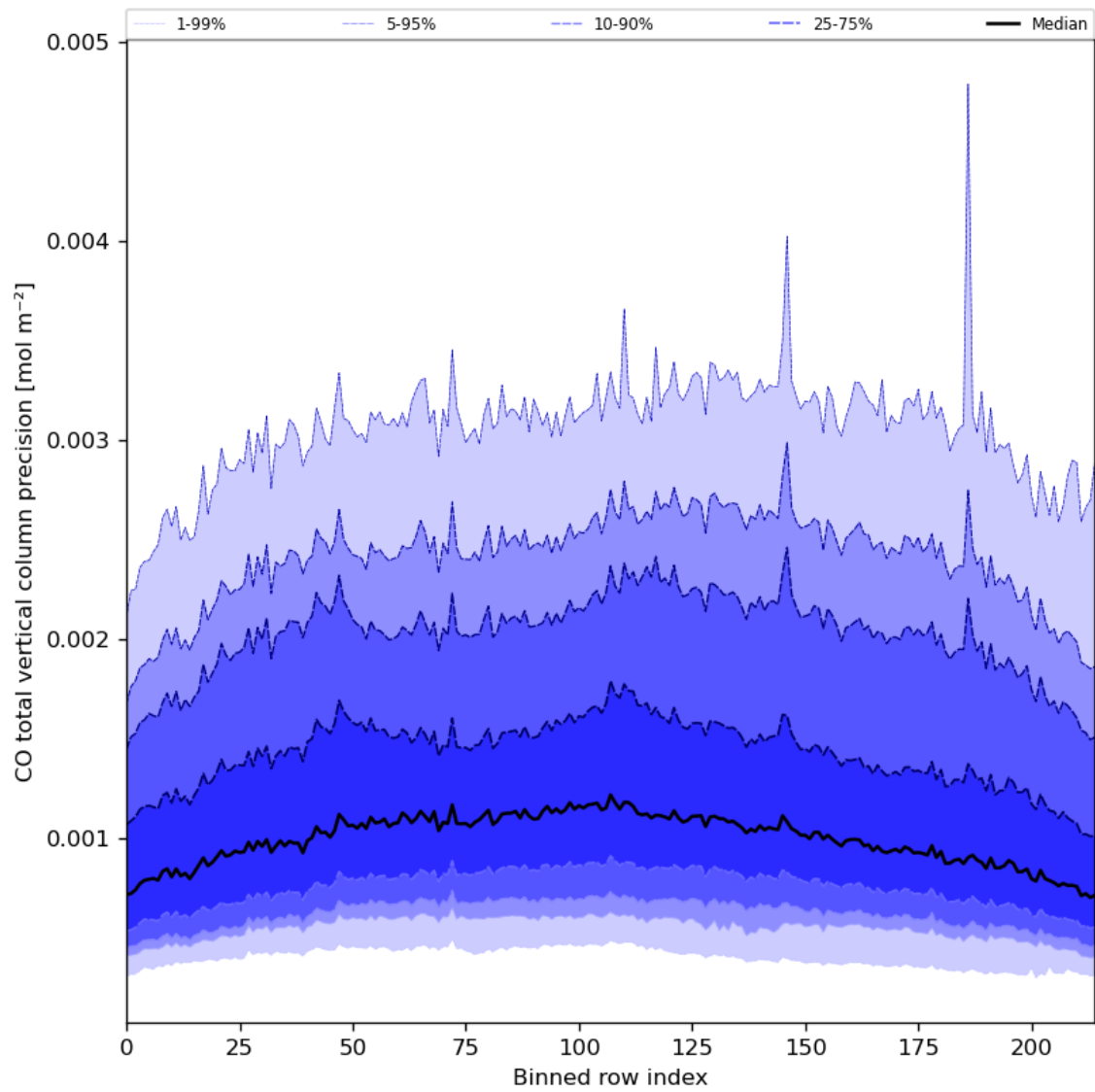
Figure 28: Along track statistics of “CO total vertical column precision” for 2023-07-19 to 2023-07-21
