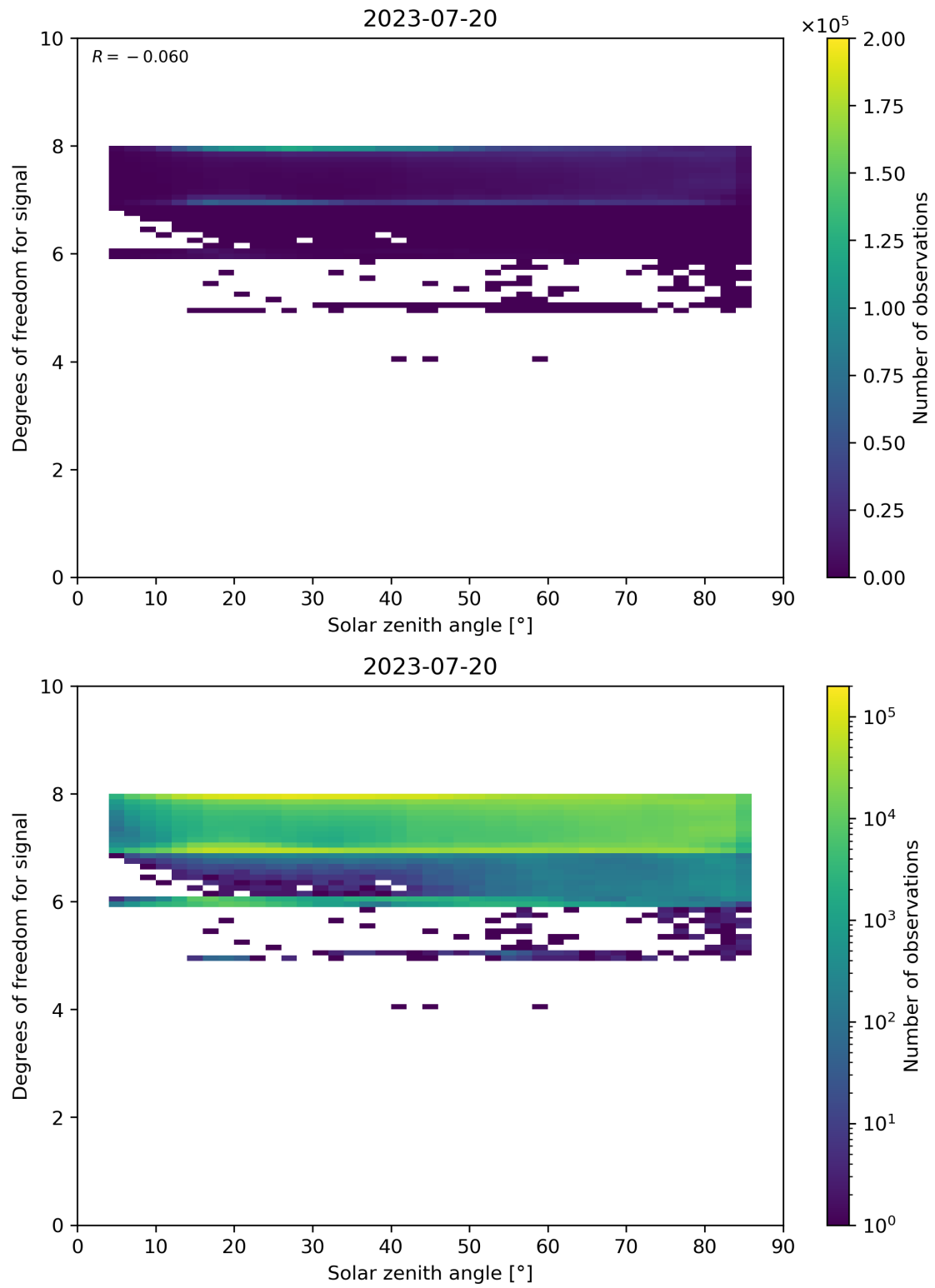
Figure 65: Scatter density plot of “Solar zenith angle” against “Degrees of freedom for signal” for 2023-07-19 to 2023-07-21.
