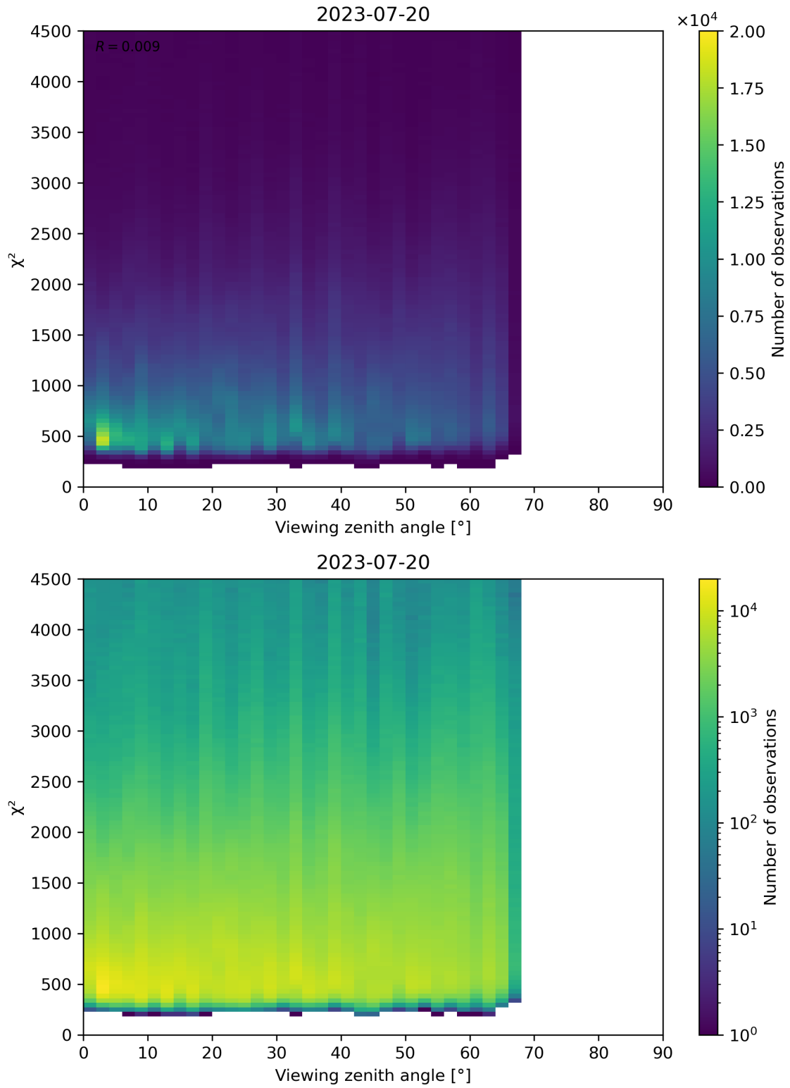
Figure 72: Scatter density plot of “Viewing zenith angle” against “ \chi^2 ” for 2023-07-19 to 2023-07-21.
