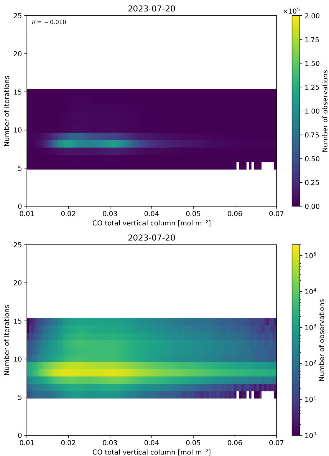
Figure 42: Scatter density plot of “CO total vertical column” against “Number of iterations” for 2023-07-19 to 2023-07-21.
