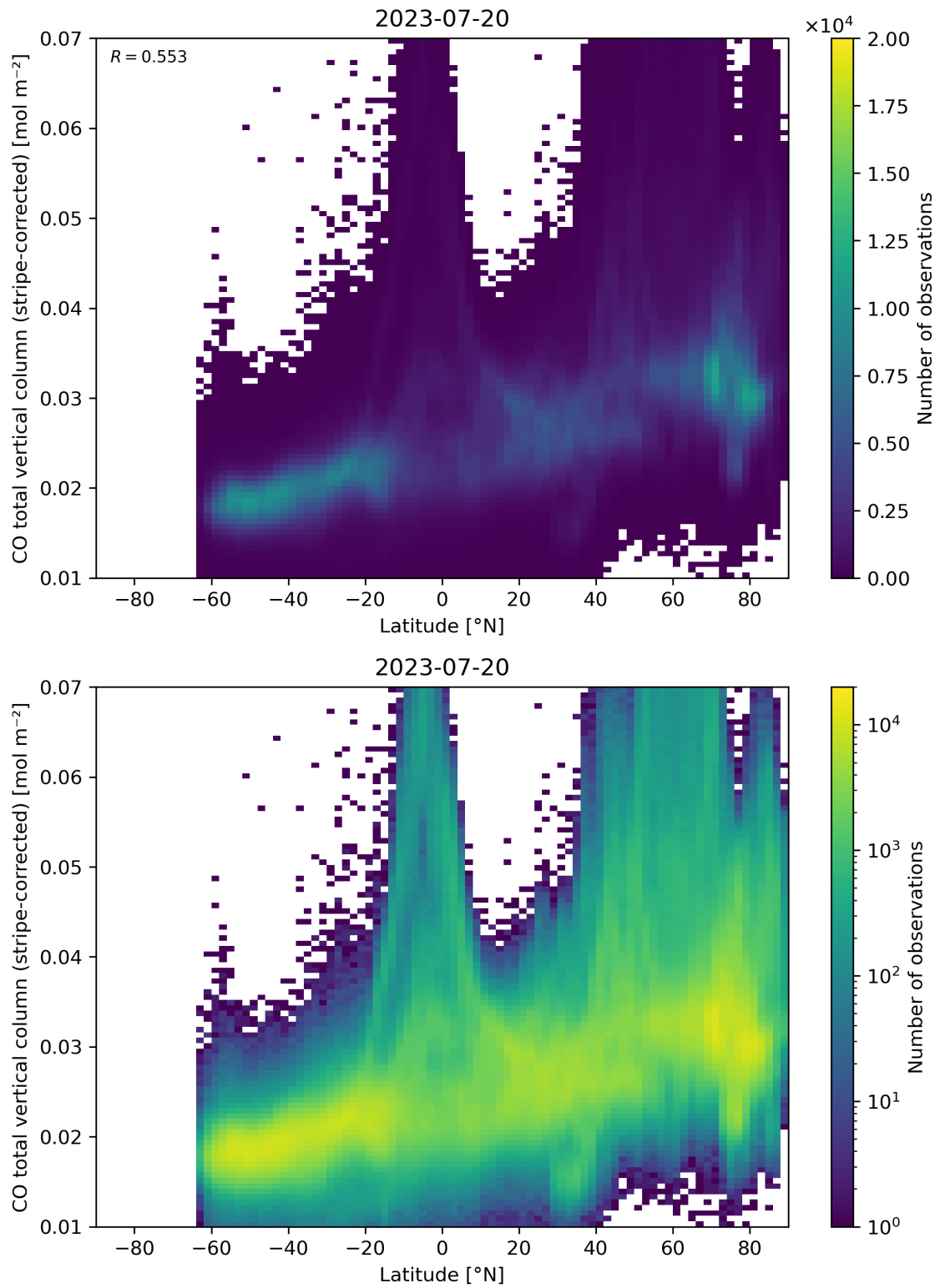
Figure 52: Scatter density plot of “Latitude” against “CO total vertical column (stripe-corrected)” for 2023-07-19 to 2023-07-21.
