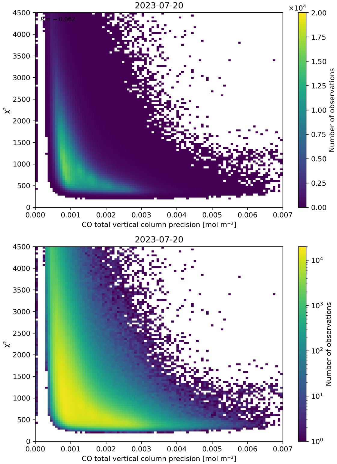
Figure 44: Scatter density plot of “CO total vertical column precision” against “ \chi^2 ” for 2023-07-19 to 2023-07-21.
