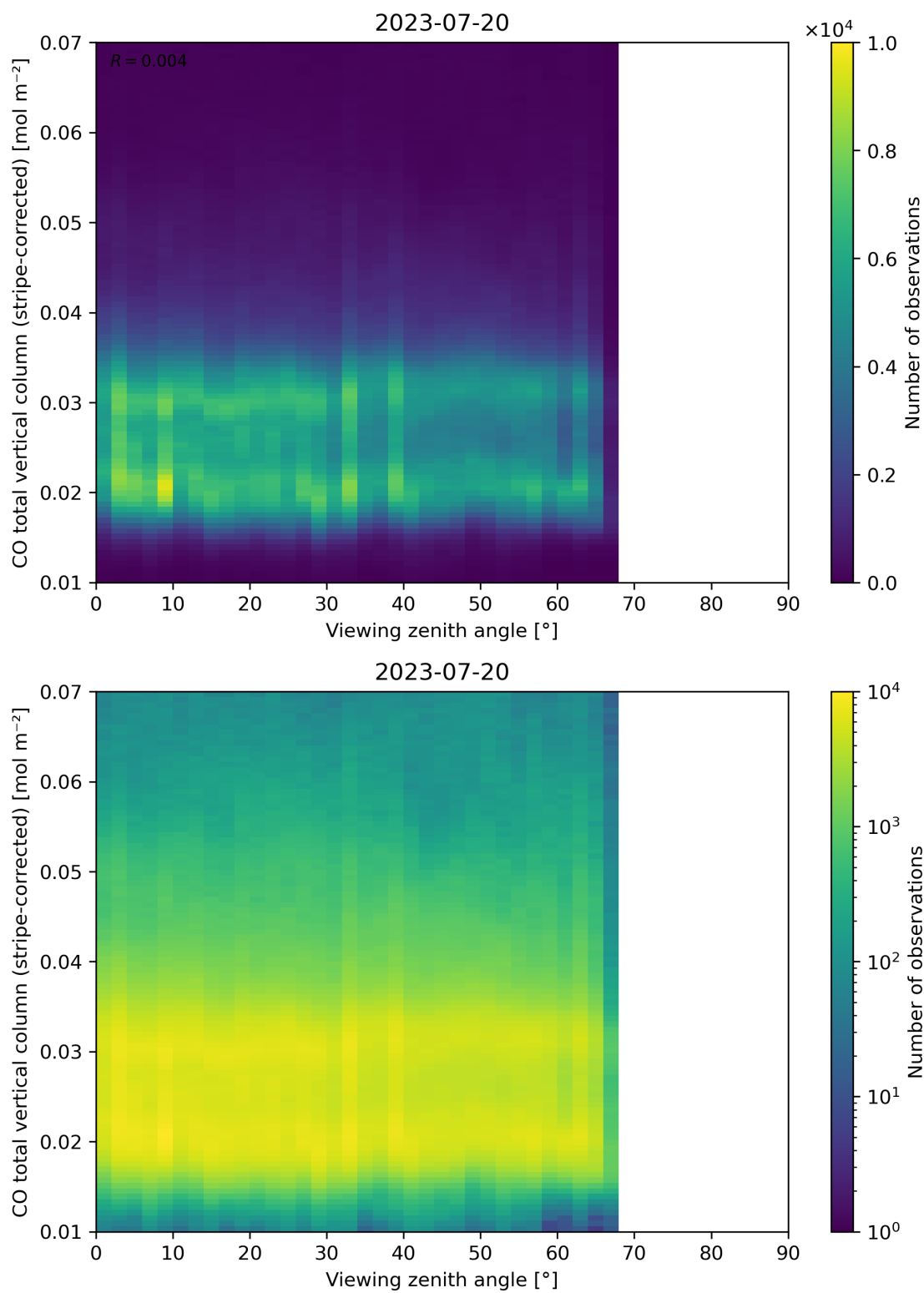
Figure 70: Scatter density plot of “Viewing zenith angle” against “CO total vertical column (stripe-corrected)” for 2023-07-19 to 2023-07-21.
