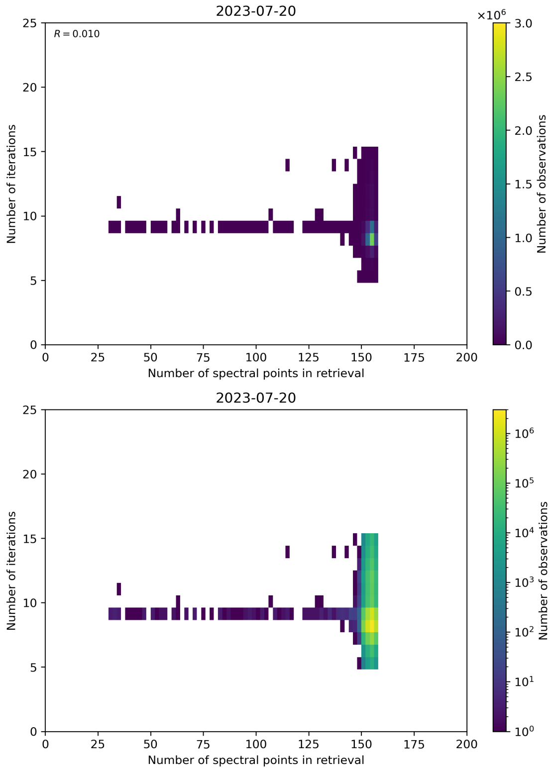
Figure 60: Scatter density plot of “Number of spectral points in retrieval” against “Number of iterations” for 2023-07-19 to 2023-07-21.
