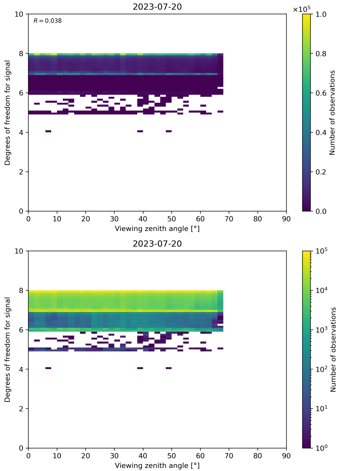
Figure 73: Scatter density plot of “Viewing zenith angle” against “Degrees of freedom for signal” for 2023-07-19 to 2023-07-21.
