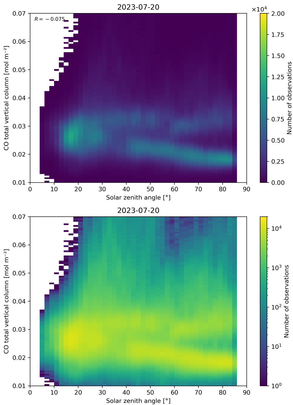
Figure 61: Scatter density plot of “Solar zenith angle” against “CO total vertical column” for 2023-07-19 to 2023-07-21.
