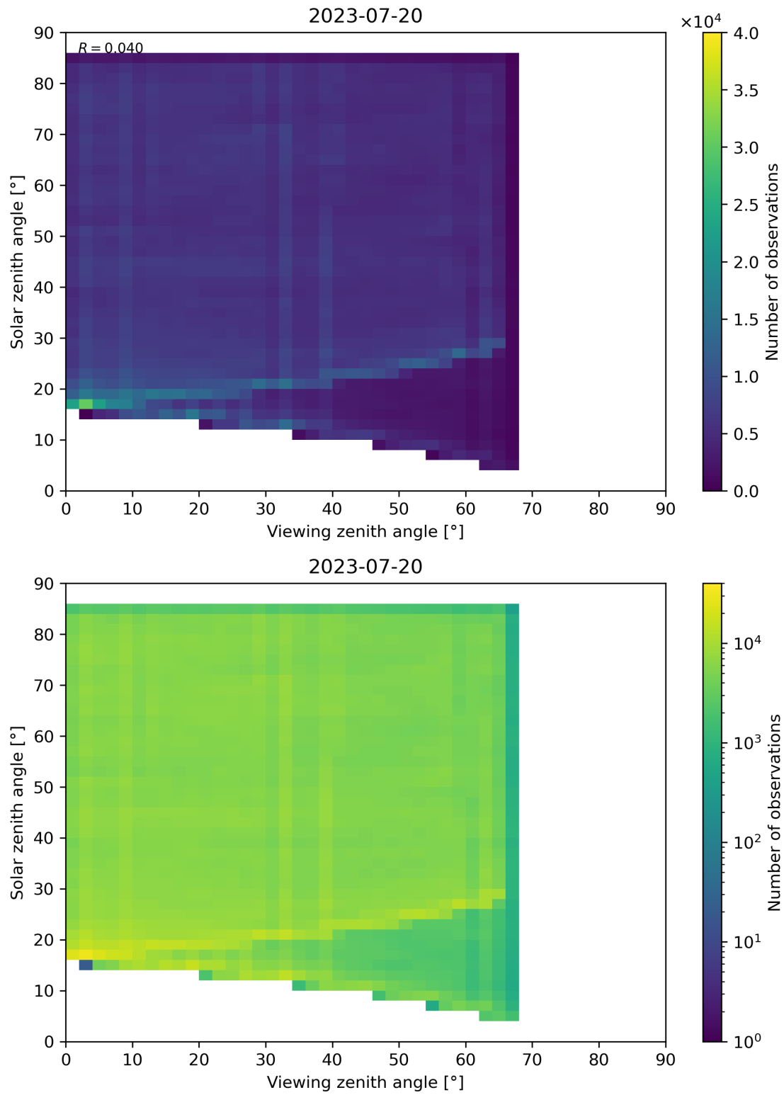
Figure 77: Scatter density plot of “Viewing zenith angle” against “Solar zenith angle” for 2023-07-19 to 2023-07-21.
