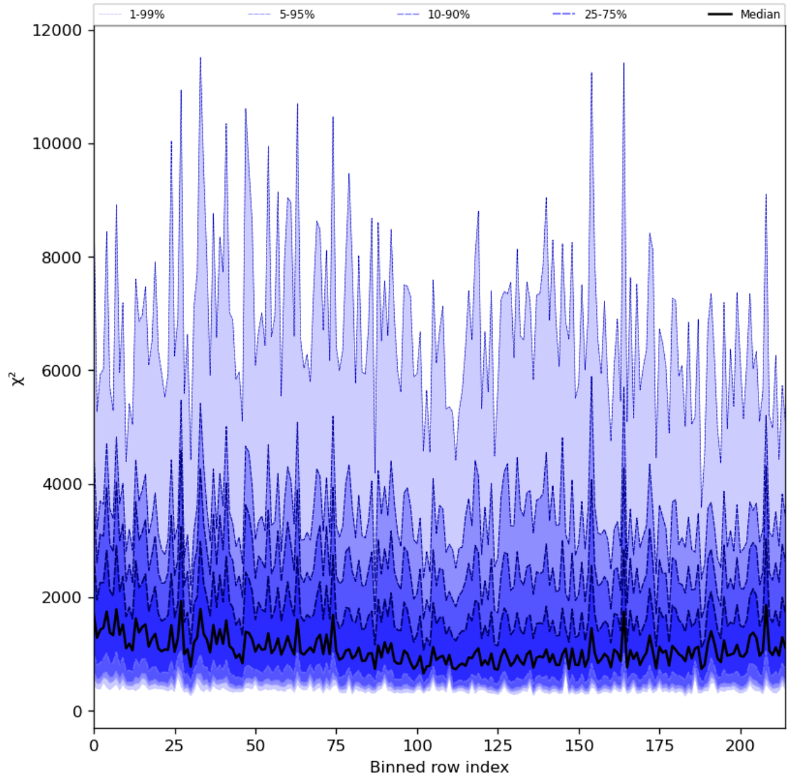
Figure 30: Along track statistics of “ \chi^2 ” for 2023-07-19 to 2023-07-21
