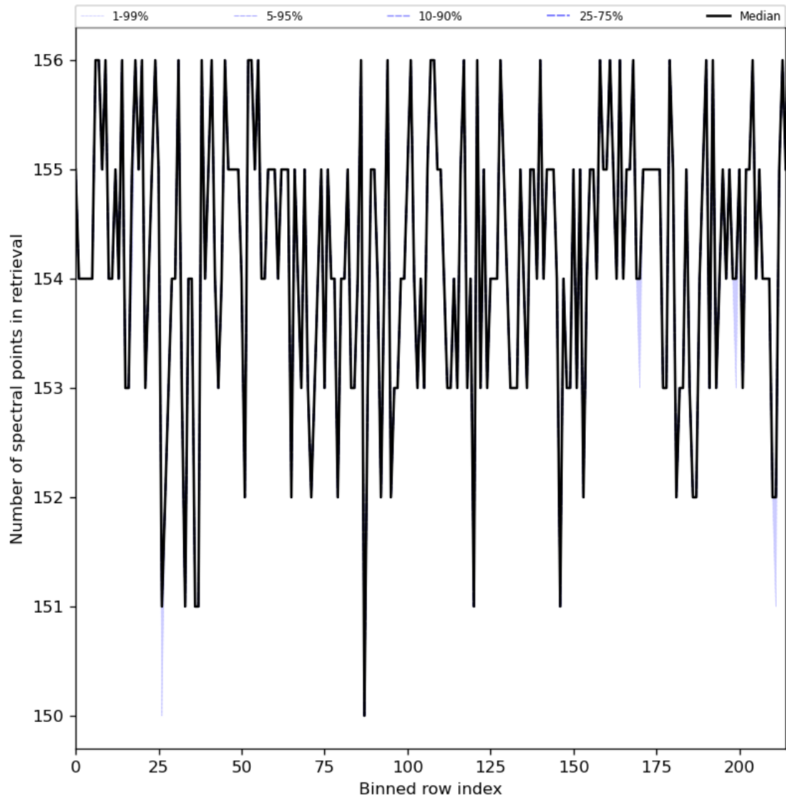
Figure 29: Along track statistics of “Number of spectral points in retrieval” for 2023-07-19 to 2023-07-21
