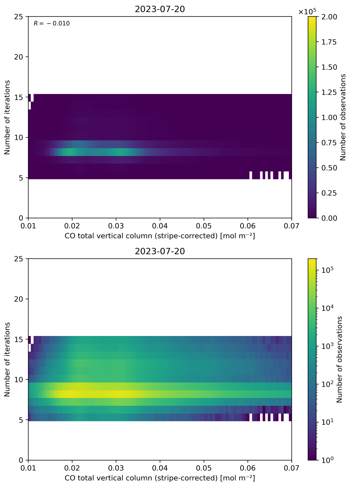
Figure 39: Scatter density plot of “CO total vertical column (stripe-corrected)” against “Number of iterations” for 2023-07-19 to 2023-07-21.
