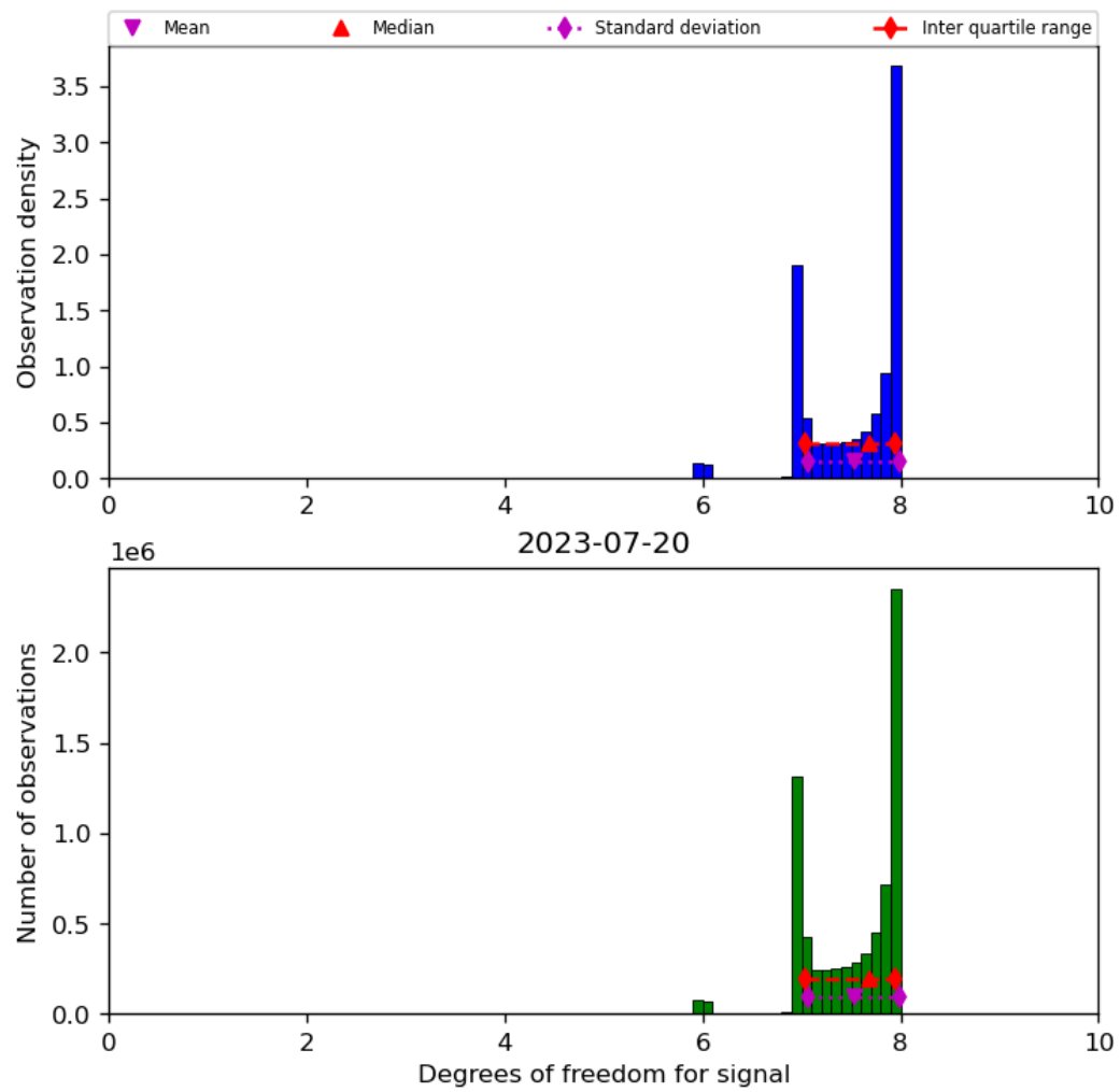
Figure 23: Histogram of “Degrees of freedom for signal” for 2023-07-19 to 2023-07-21
