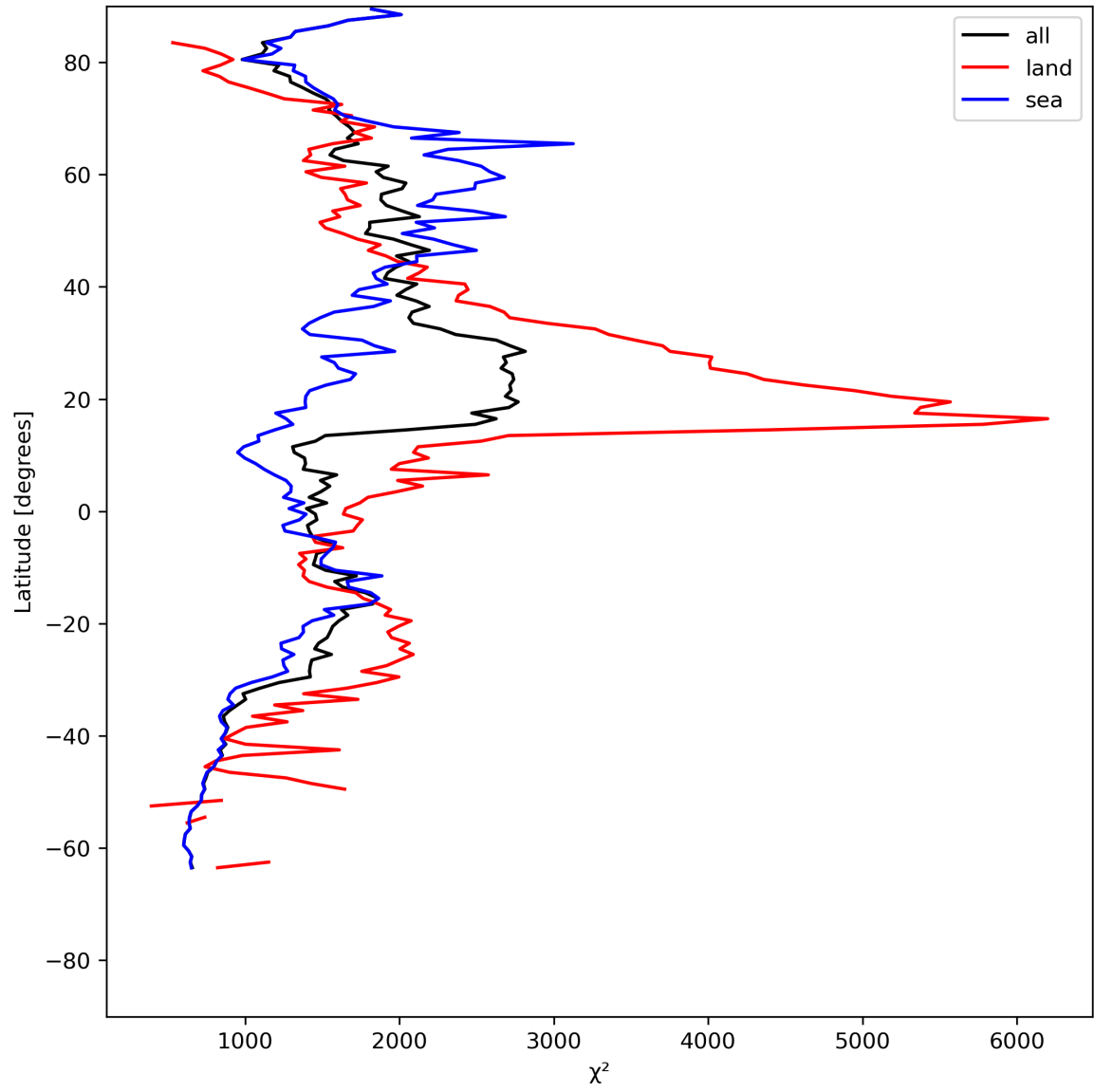
Figure 14: Zonal average of “ \chi^2 ” for 2023-07-19 to 2023-07-21.
