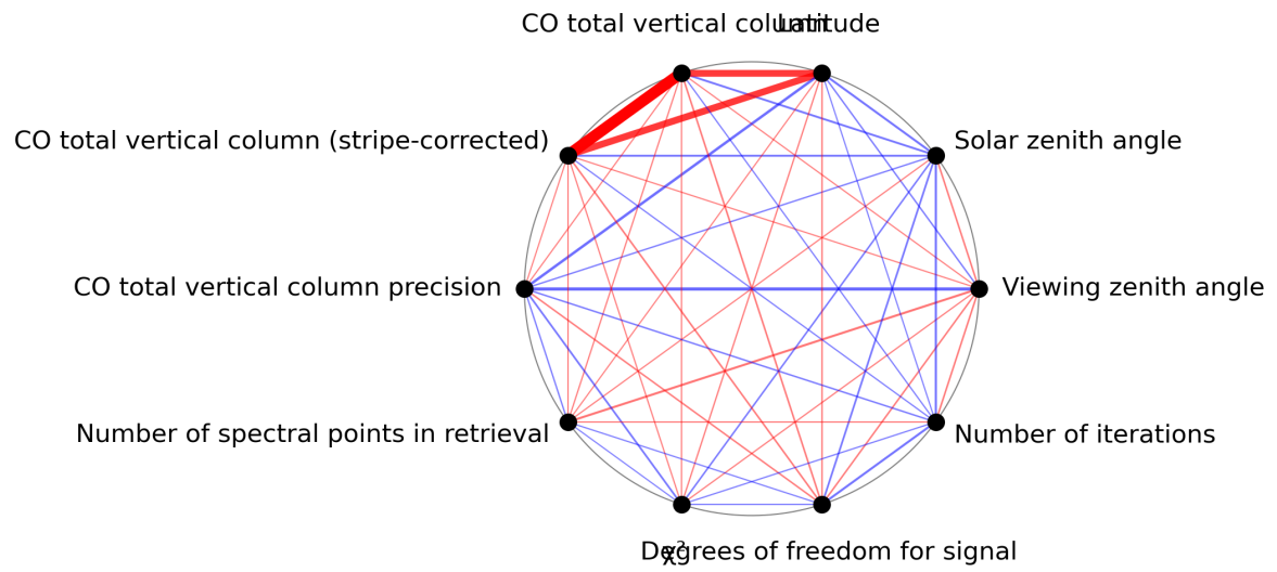
Figure 1: Map of correlation graph for 2023-07-19 to 2023-07-21.
