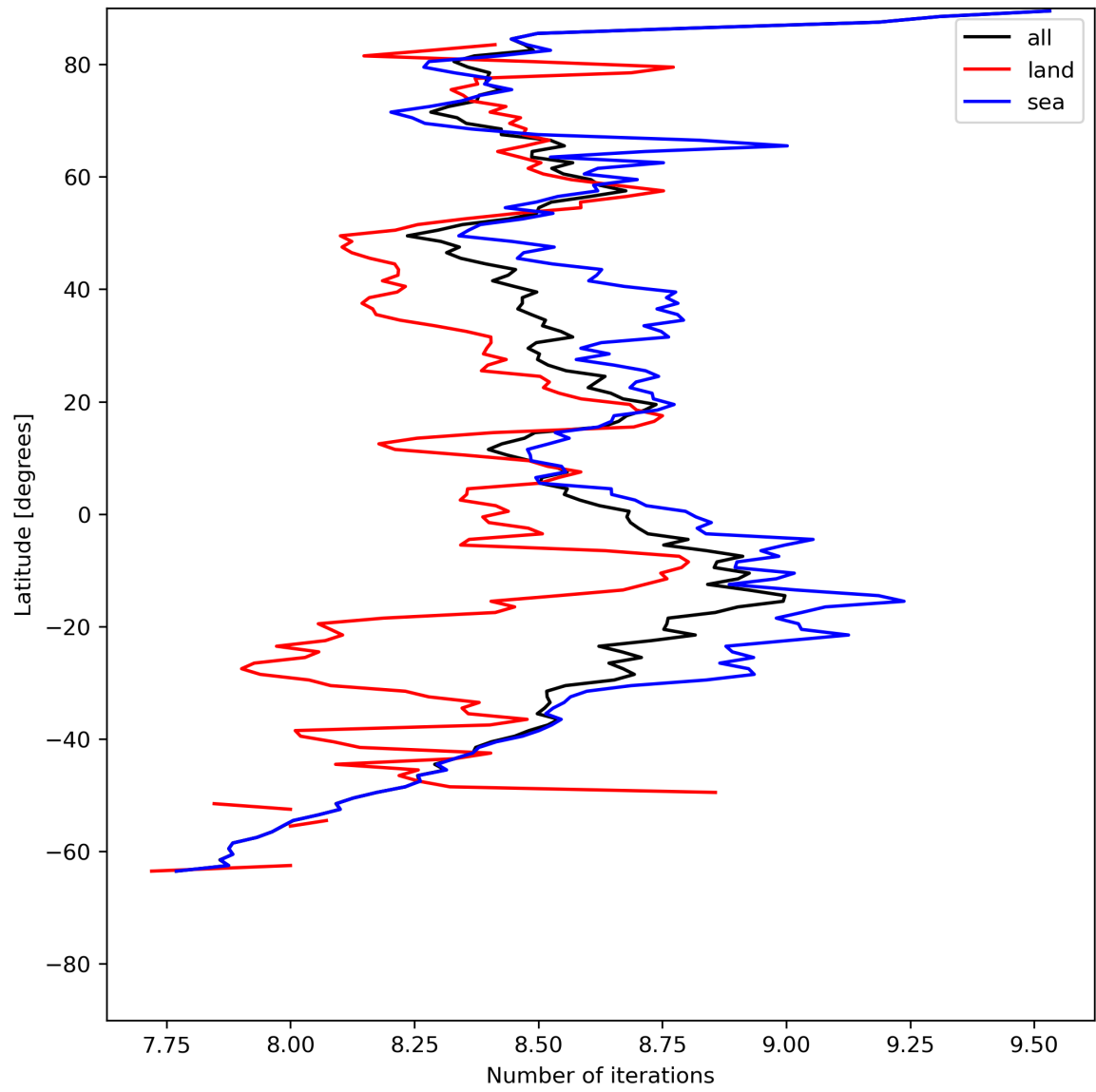
Figure 16: Zonal average of “Number of iterations” for 2023-07-19 to 2023-07-21.
