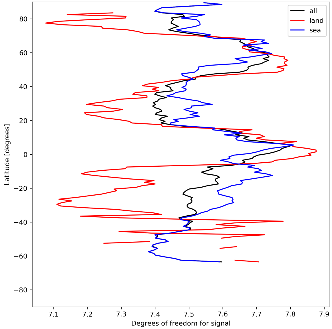
Figure 15: Zonal average of “Degrees of freedom for signal” for 2023-07-19 to 2023-07-21.
