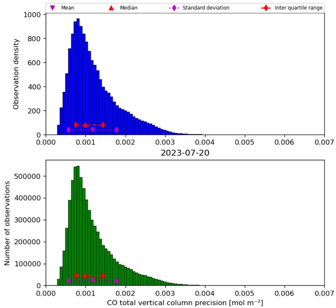
Figure 20: Histogram of “CO total vertical column precision” for 2023-07-19 to 2023-07-21
