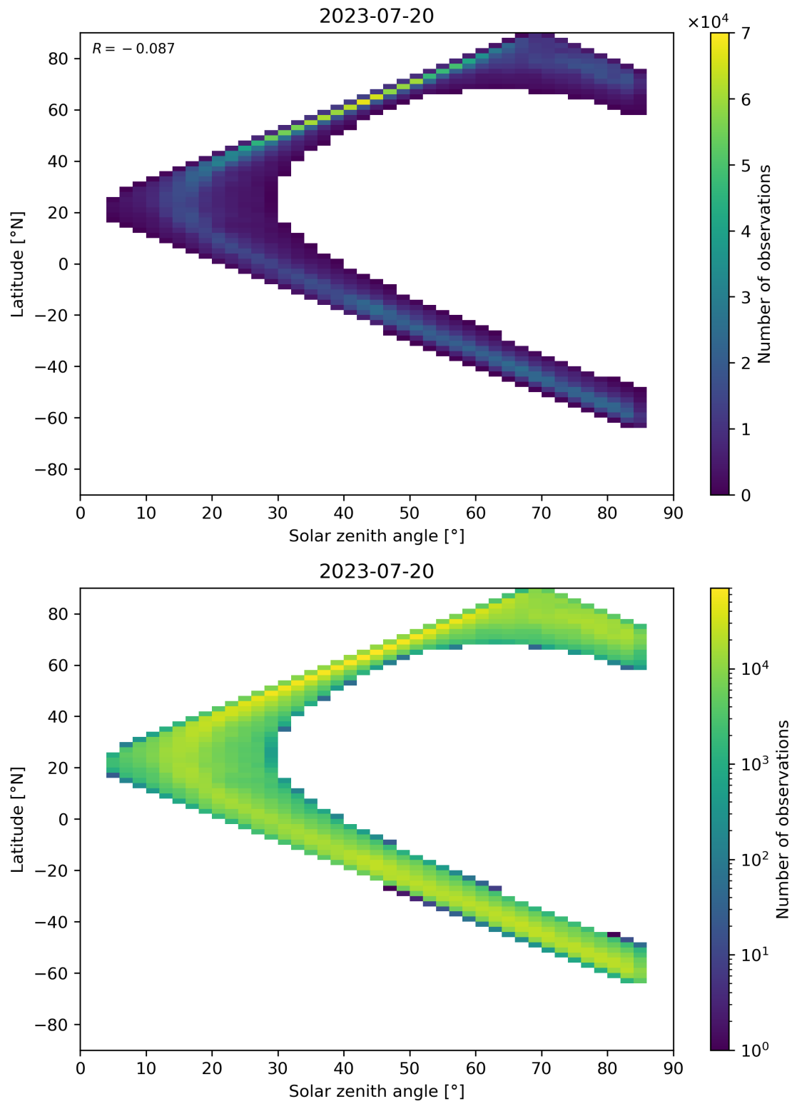
Figure 66: Scatter density plot of “Solar zenith angle” against “Latitude” for 2023-07-19 to 2023-07-21.
