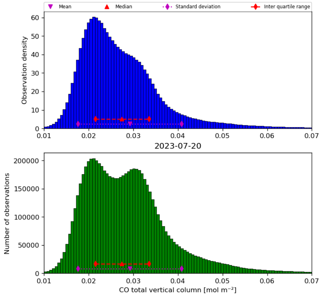
Figure 18: Histogram of “CO total vertical column” for 2023-07-19 to 2023-07-21
