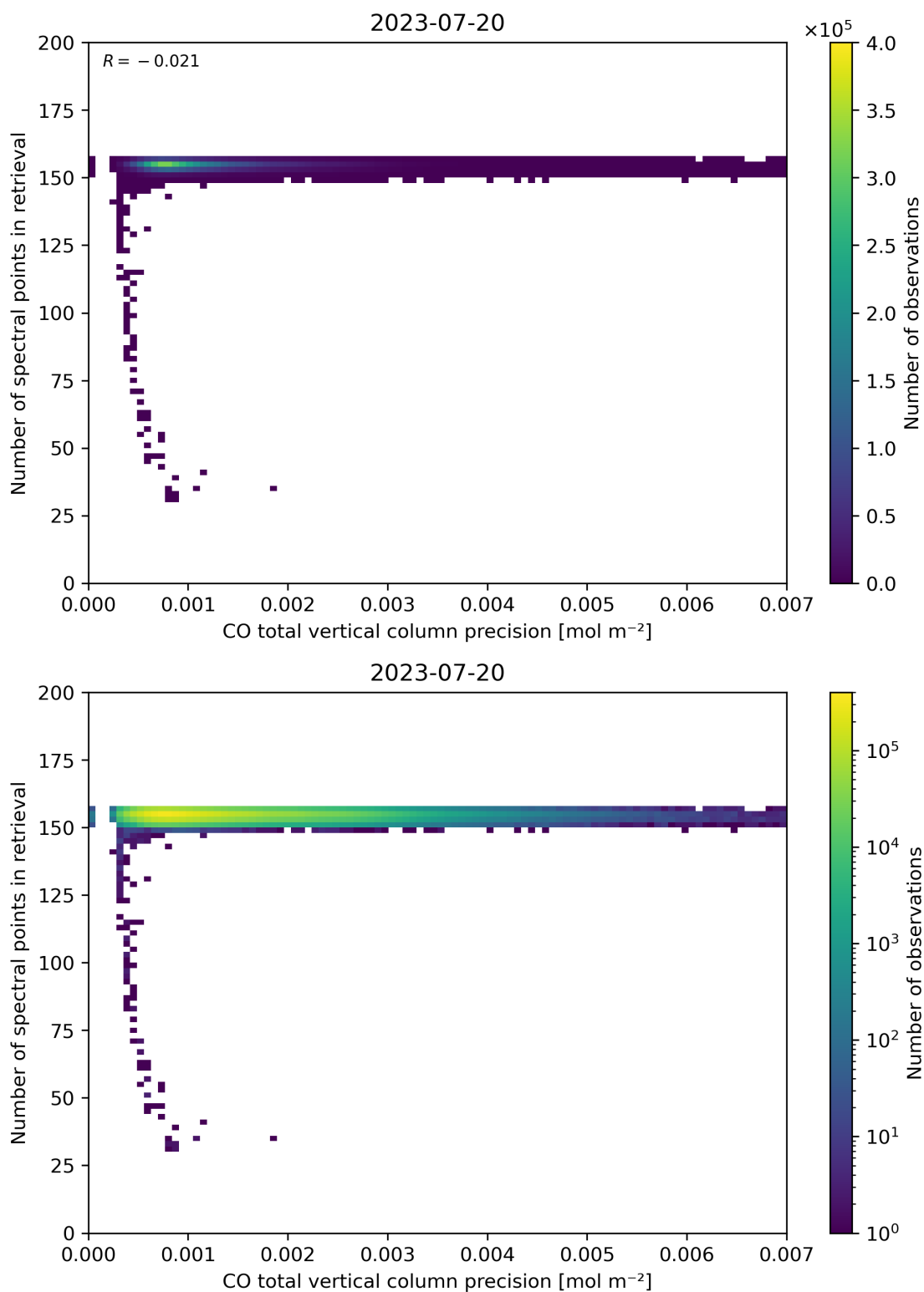
Figure 47: Scatter density plot of “CO total vertical column precision” against “Number of spectral points in retrieval” for 2023-07-19 to 2023-07-21.
