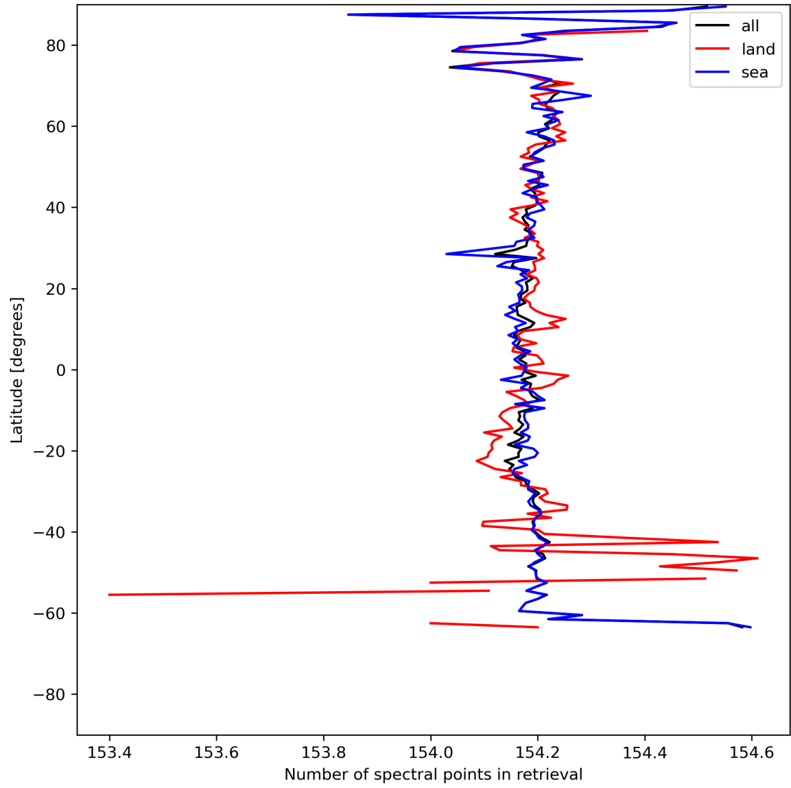
Figure 13: Zonal average of “Number of spectral points in retrieval” for 2023-07-19 to 2023-07-21.
