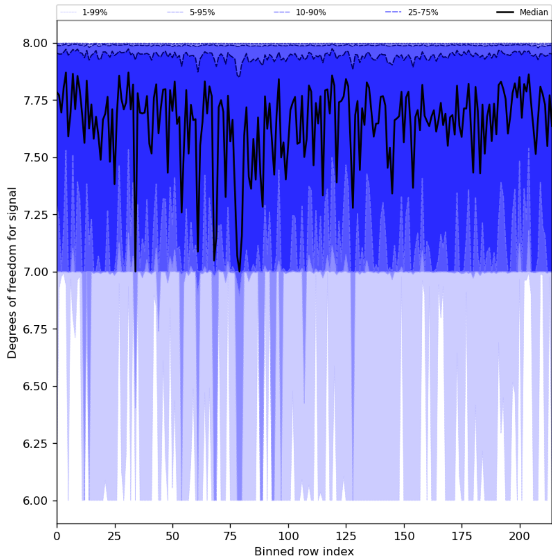
Figure 31: Along track statistics of “Degrees of freedom for signal” for 2023-07-19 to 2023-07-21
