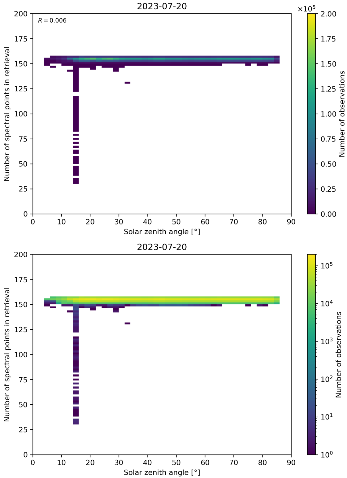
Figure 68: Scatter density plot of “Solar zenith angle” against “Number of spectral points in retrieval” for 2023-07-19 to 2023-07-21.
