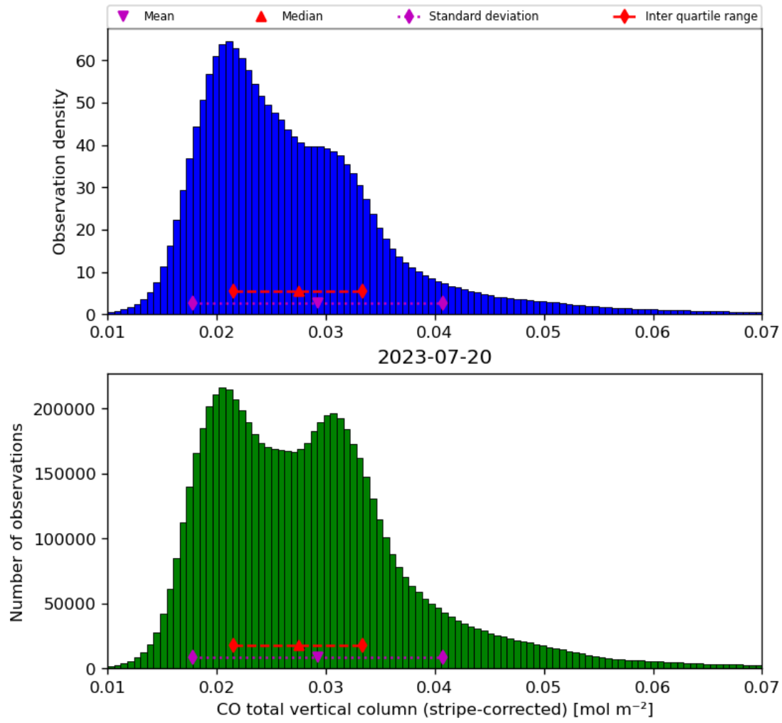
Figure 19: Histogram of “CO total vertical column (stripe-corrected)” for 2023-07-19 to 2023-07-21
