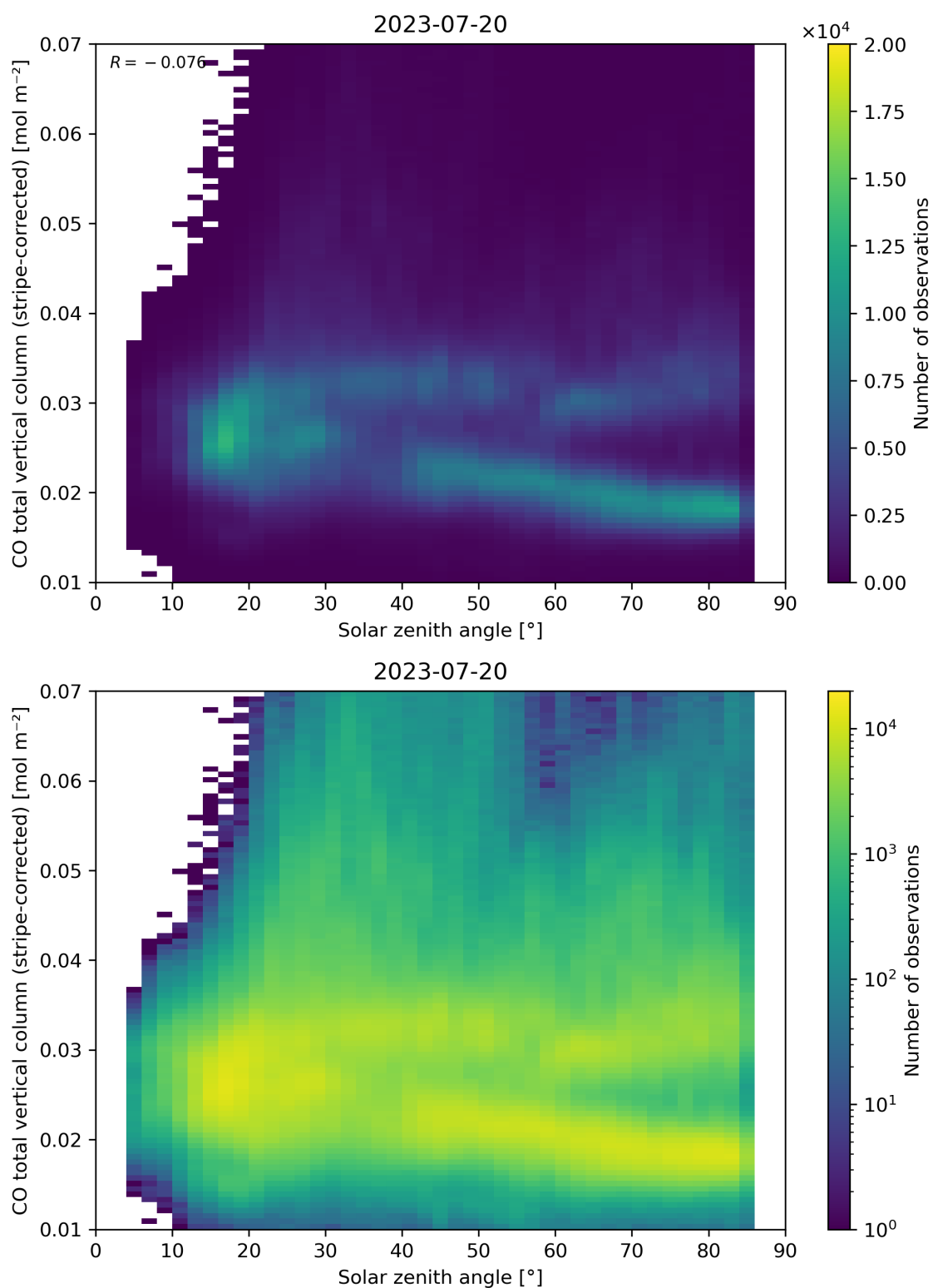
Figure 62: Scatter density plot of “Solar zenith angle” against “CO total vertical column (stripe-corrected)” for 2023-07-19 to 2023-07-21.
