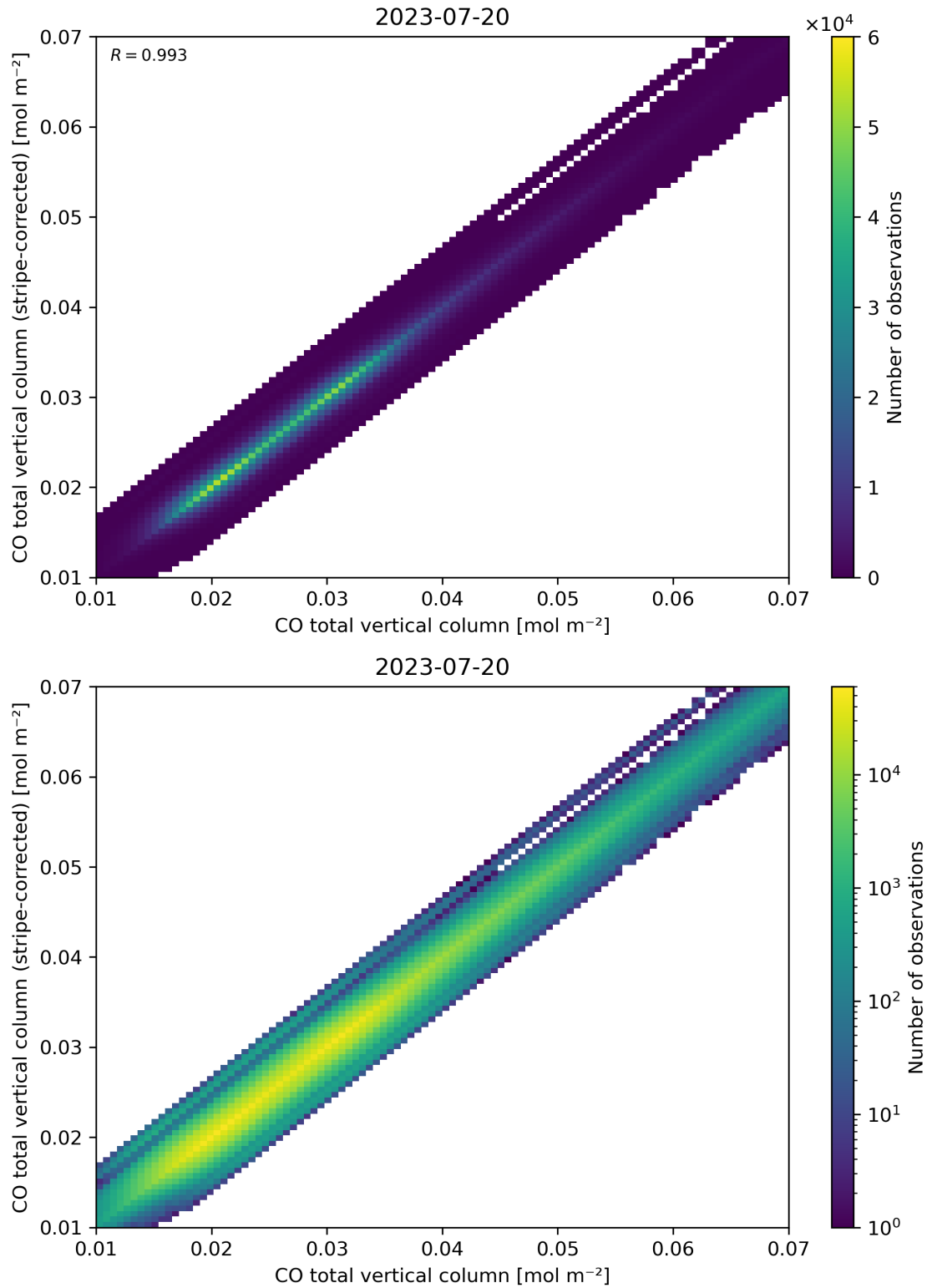
Figure 33: Scatter density plot of “CO total vertical column” against “CO total vertical column (stripe-corrected)” for 2023-07-19 to 2023-07-21.
