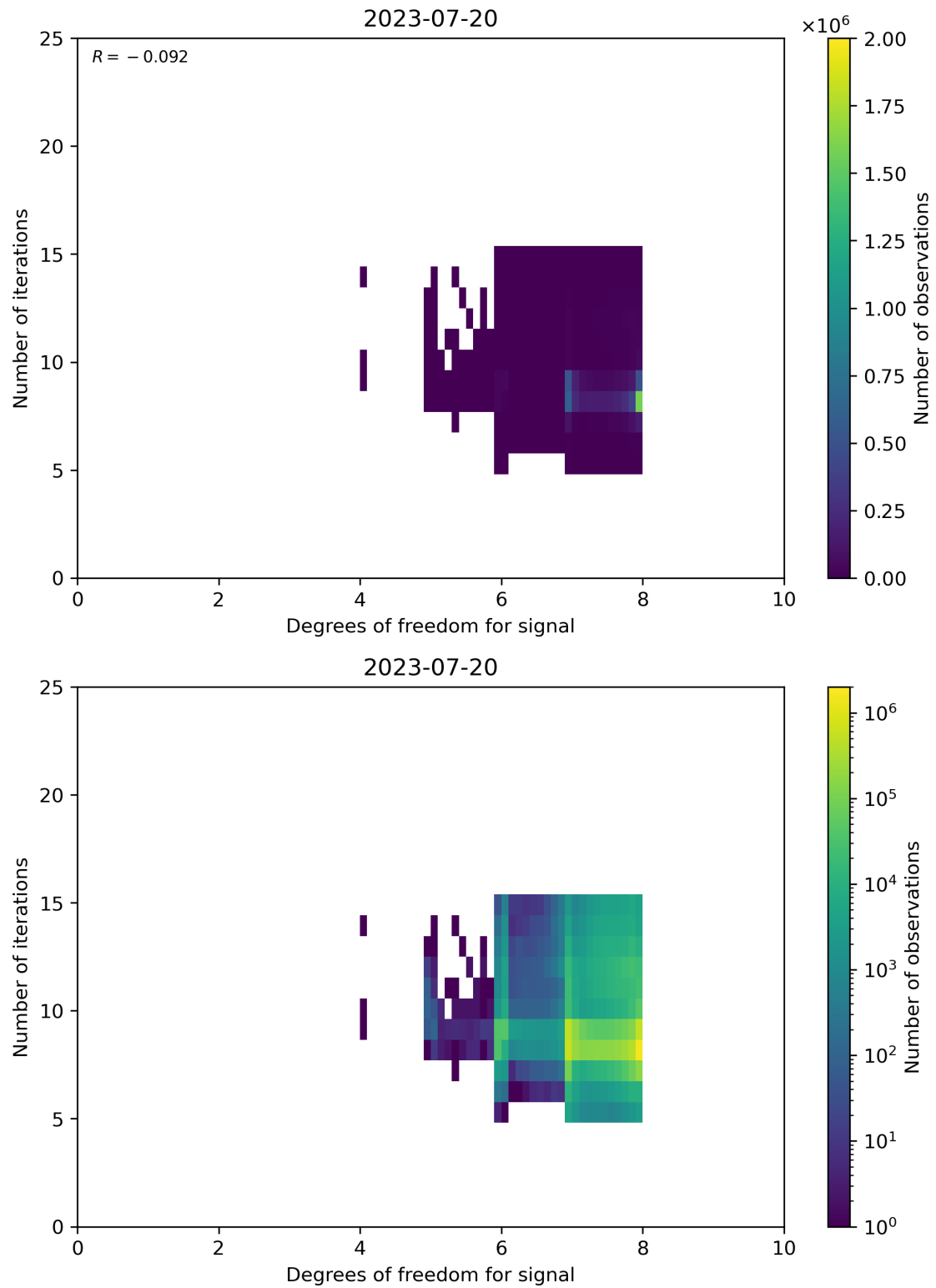
Figure 50: Scatter density plot of “Degrees of freedom for signal” against “Number of iterations” for 2023-07-19 to 2023-07-21.
