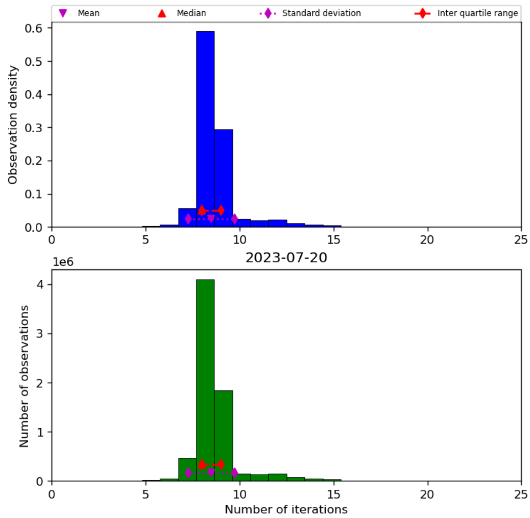
Figure 24: Histogram of “Number of iterations” for 2023-07-19 to 2023-07-21
