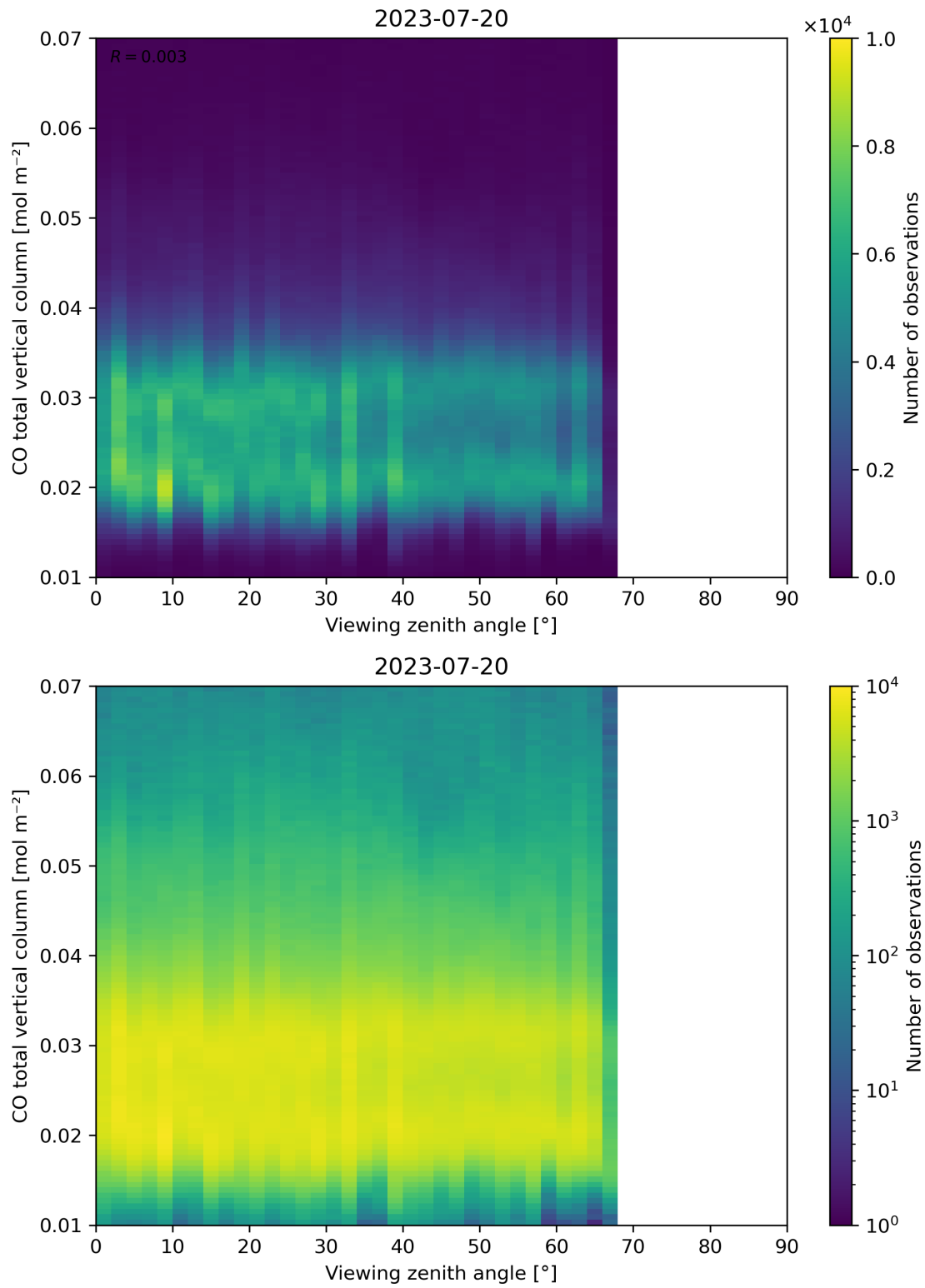
Figure 69: Scatter density plot of “Viewing zenith angle” against “CO total vertical column” for 2023-07-19 to 2023-07-21.
