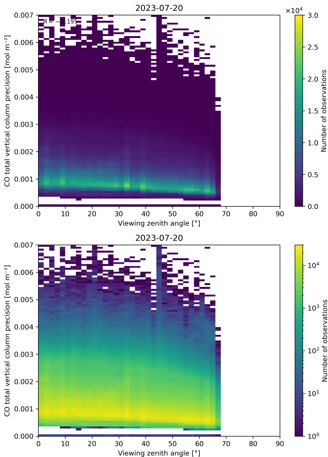
Figure 71: Scatter density plot of “Viewing zenith angle” against “CO total vertical column precision” for 2023-07-19 to 2023-07-21.
