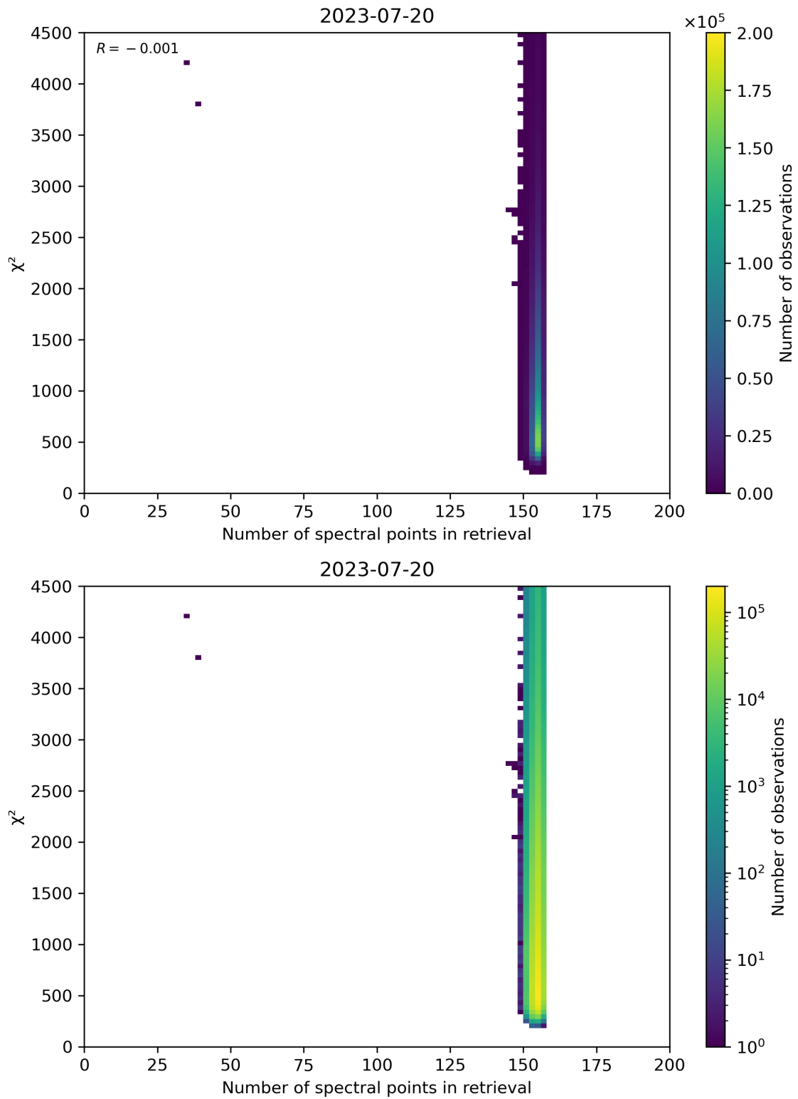
Figure 58: Scatter density plot of “Number of spectral points in retrieval” against “ \chi^2 ” for 2023-07-19 to 2023-07-21.
