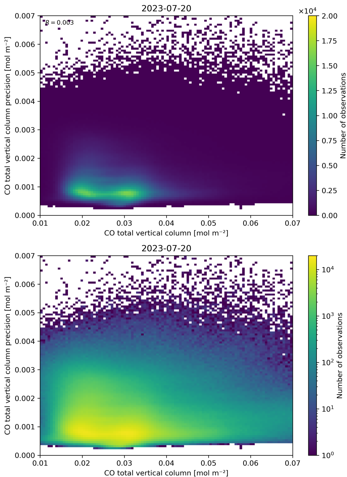
Figure 34: Scatter density plot of “CO total vertical column” against “CO total vertical column precision” for 2023-07-19 to 2023-07-21.
