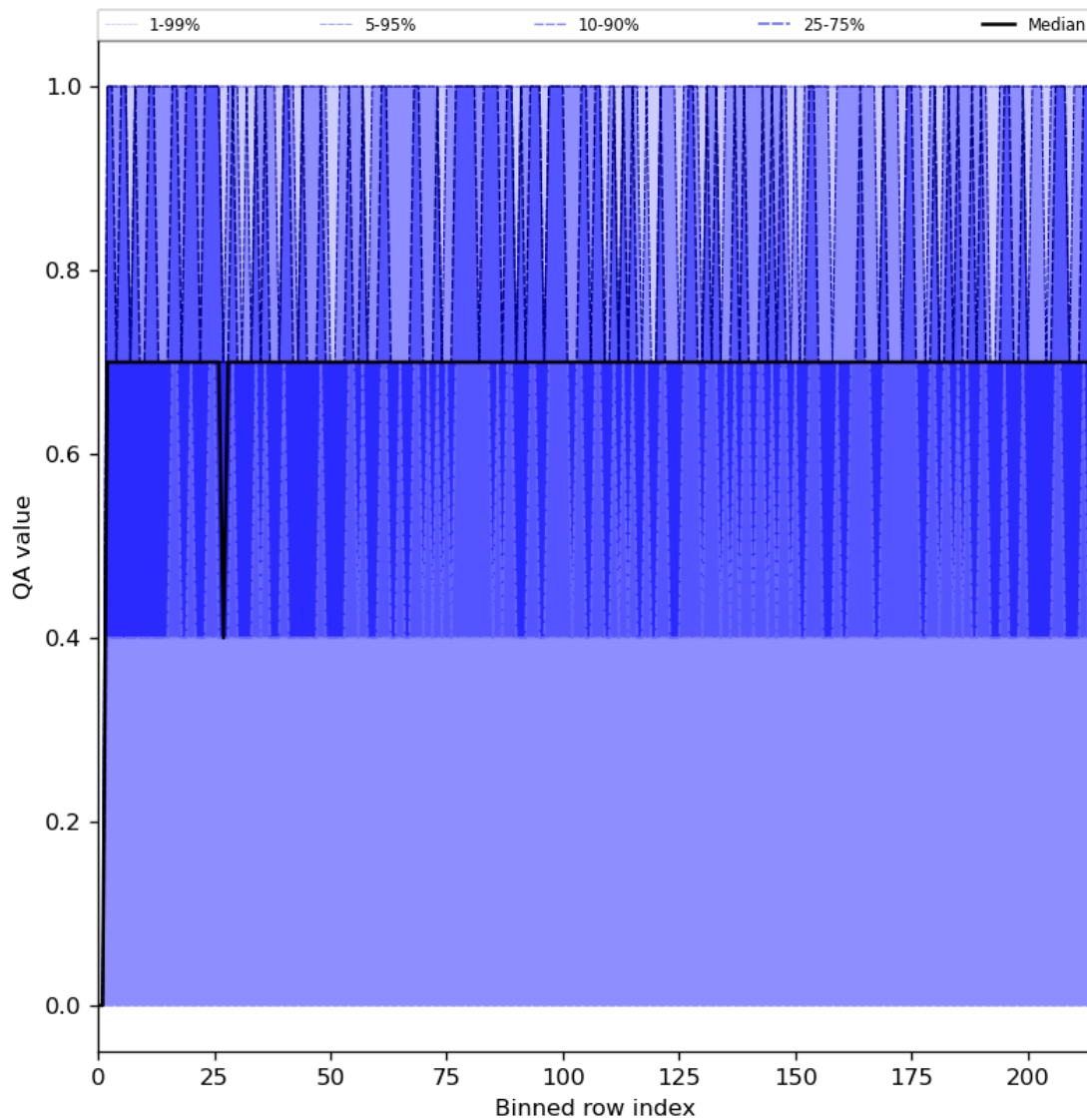
Figure 25: Along track statistics of “QA value” for 2023-07-19 to 2023-07-21
