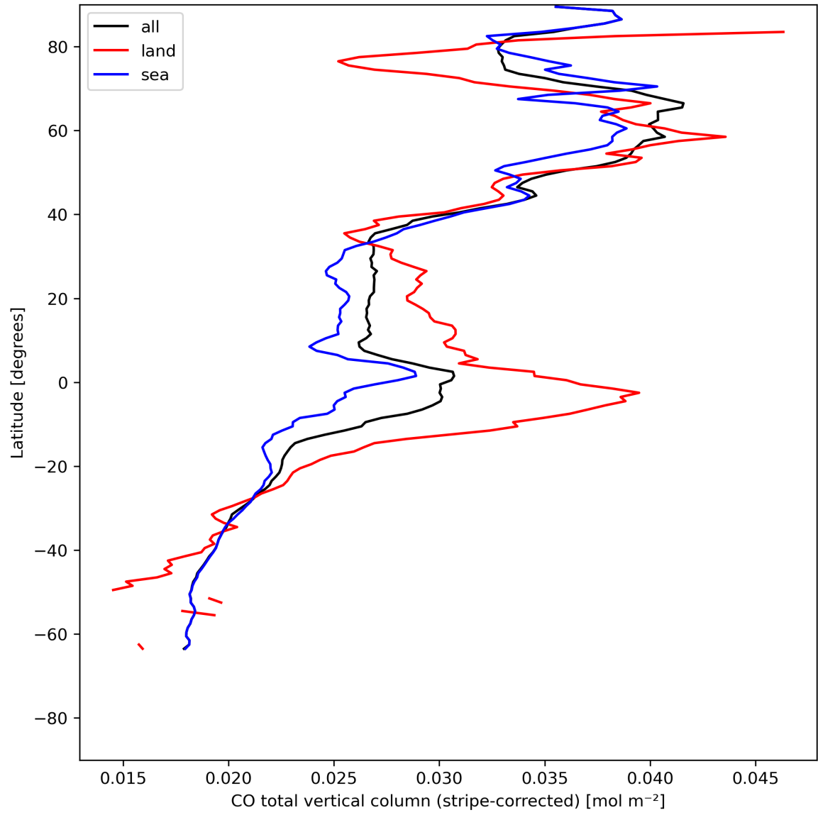
Figure 11: Zonal average of “CO total vertical column (stripe-corrected)” for 2023-07-19 to 2023-07-21.
