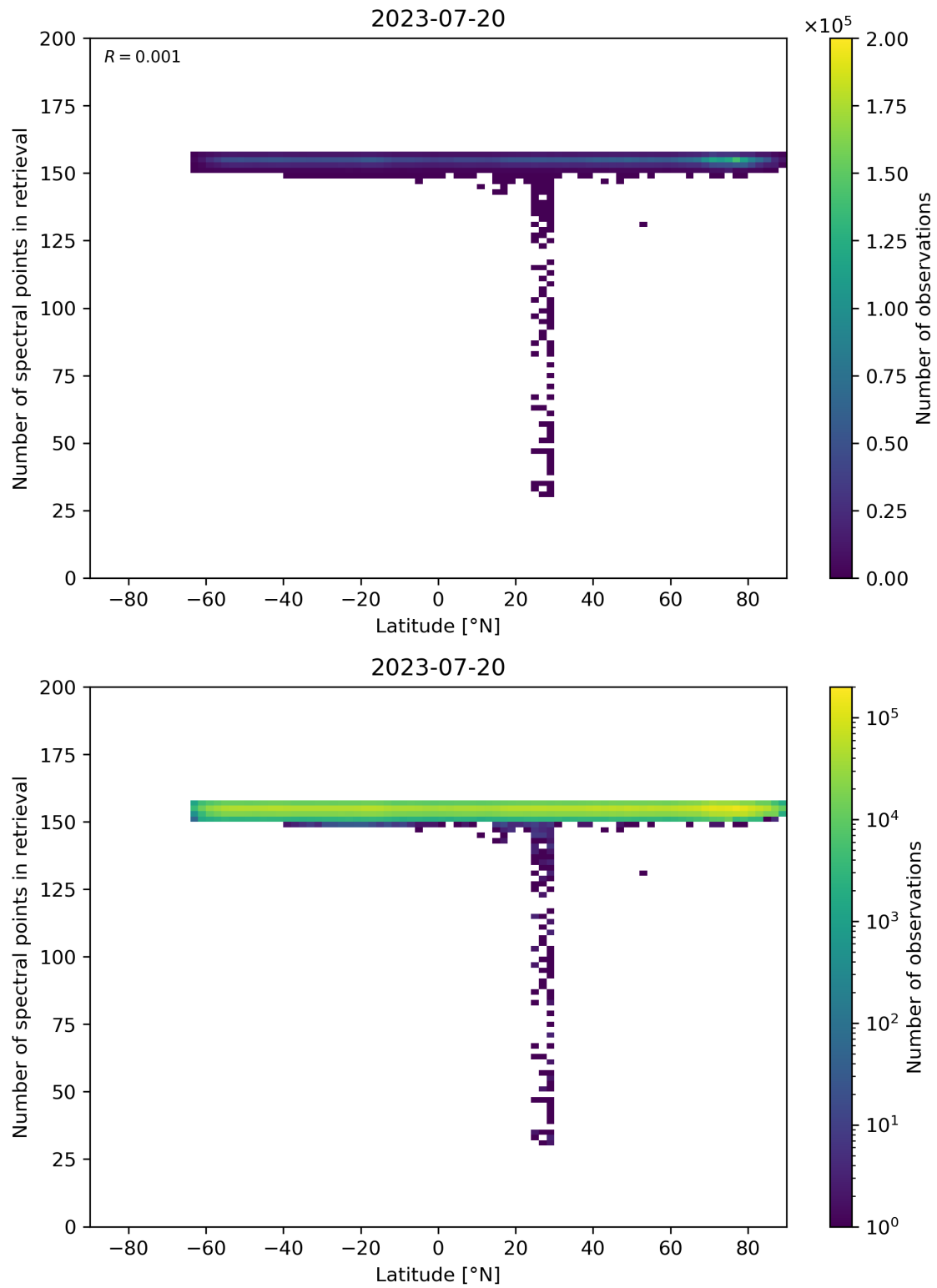
Figure 57: Scatter density plot of “Latitude” against “Number of spectral points in retrieval” for 2023-07-19 to 2023-07-21.
