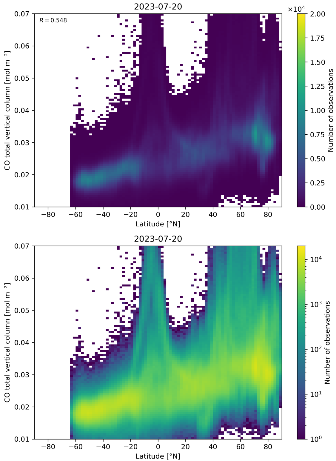
Figure 51: Scatter density plot of “Latitude” against “CO total vertical column” for 2023-07-19 to 2023-07-21.
