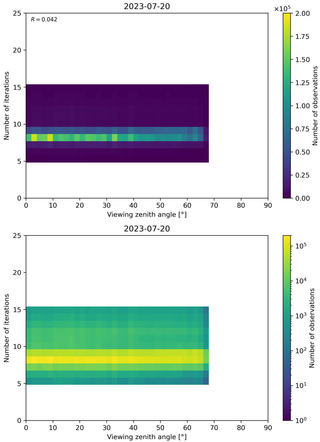
Figure 75: Scatter density plot of “Viewing zenith angle” against “Number of iterations” for 2023-07-19 to 2023-07-21.
