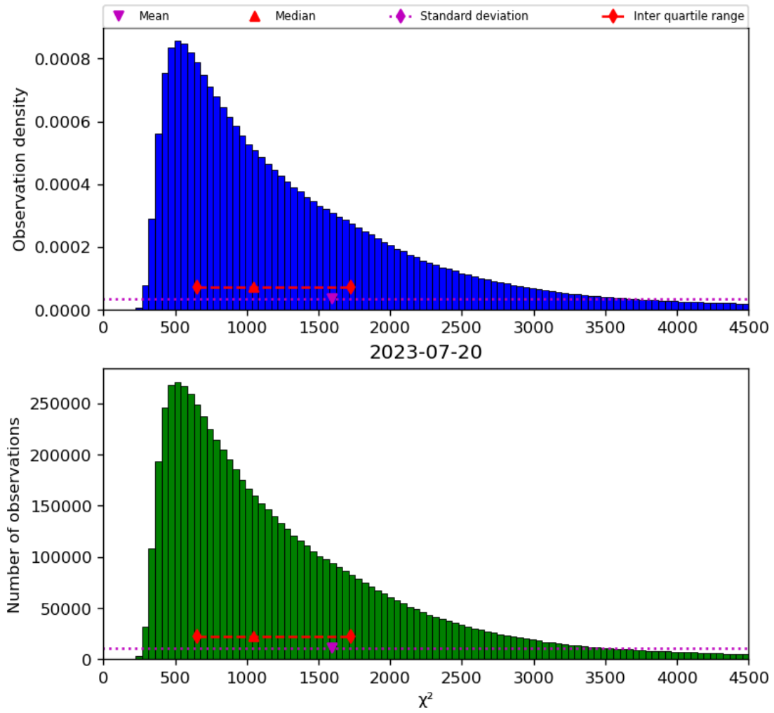
Figure 22: Histogram of " \chi^2 " for 2023-07-19 to 2023-07-21
