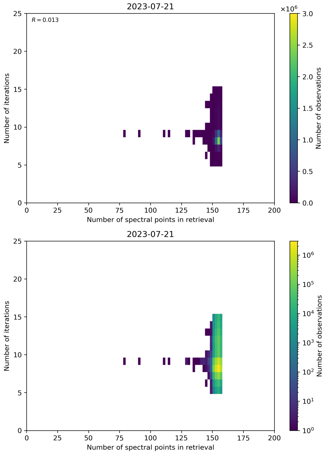
Figure 60: Scatter density plot of “Number of spectral points in retrieval” against “Number of iterations” for 2023-07-20 to 2023-07-22.
