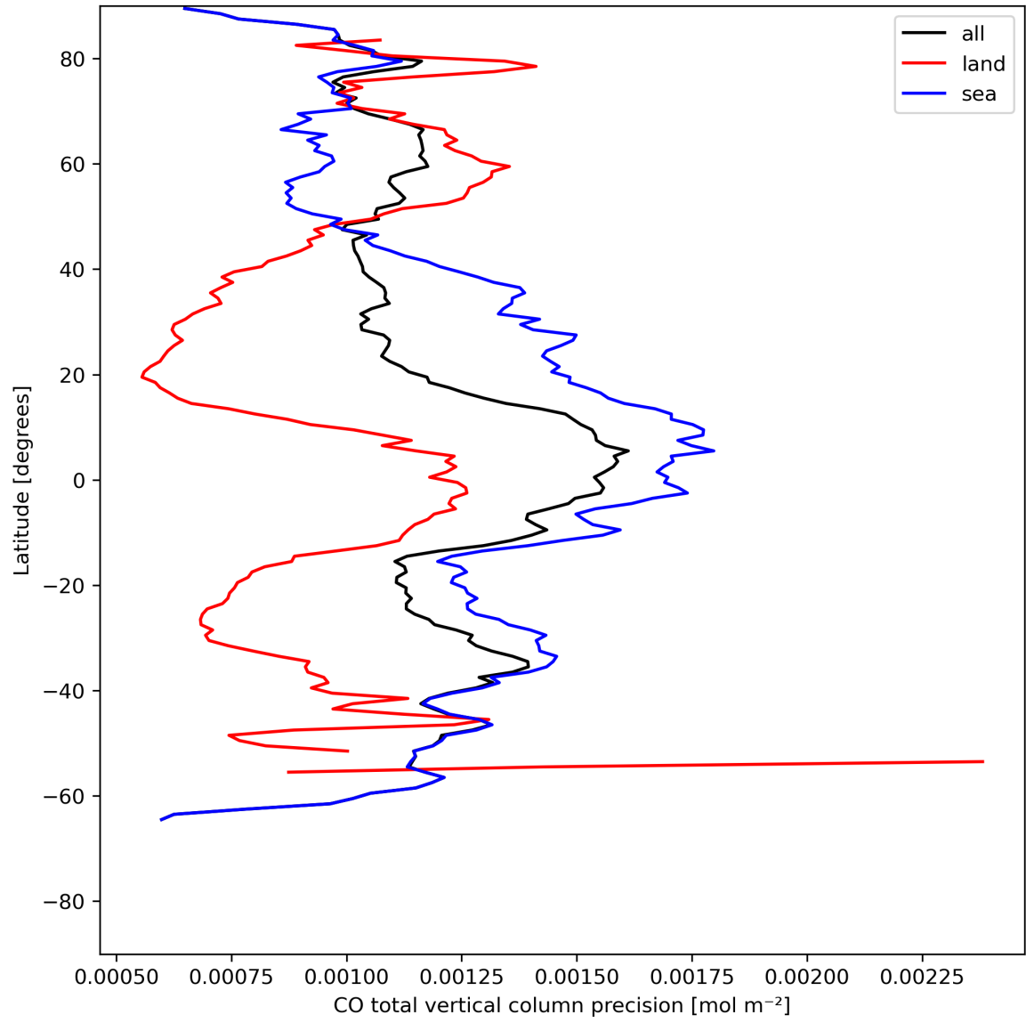
Figure 12: Zonal average of “CO total vertical column precision” for 2023-07-20 to 2023-07-22.
