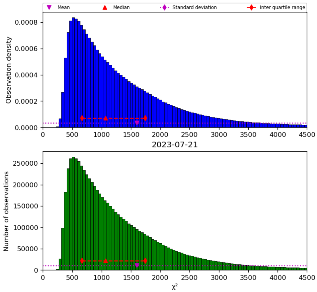
Figure 22: Histogram of “ \chi^2 ” for 2023-07-20 to 2023-07-22
