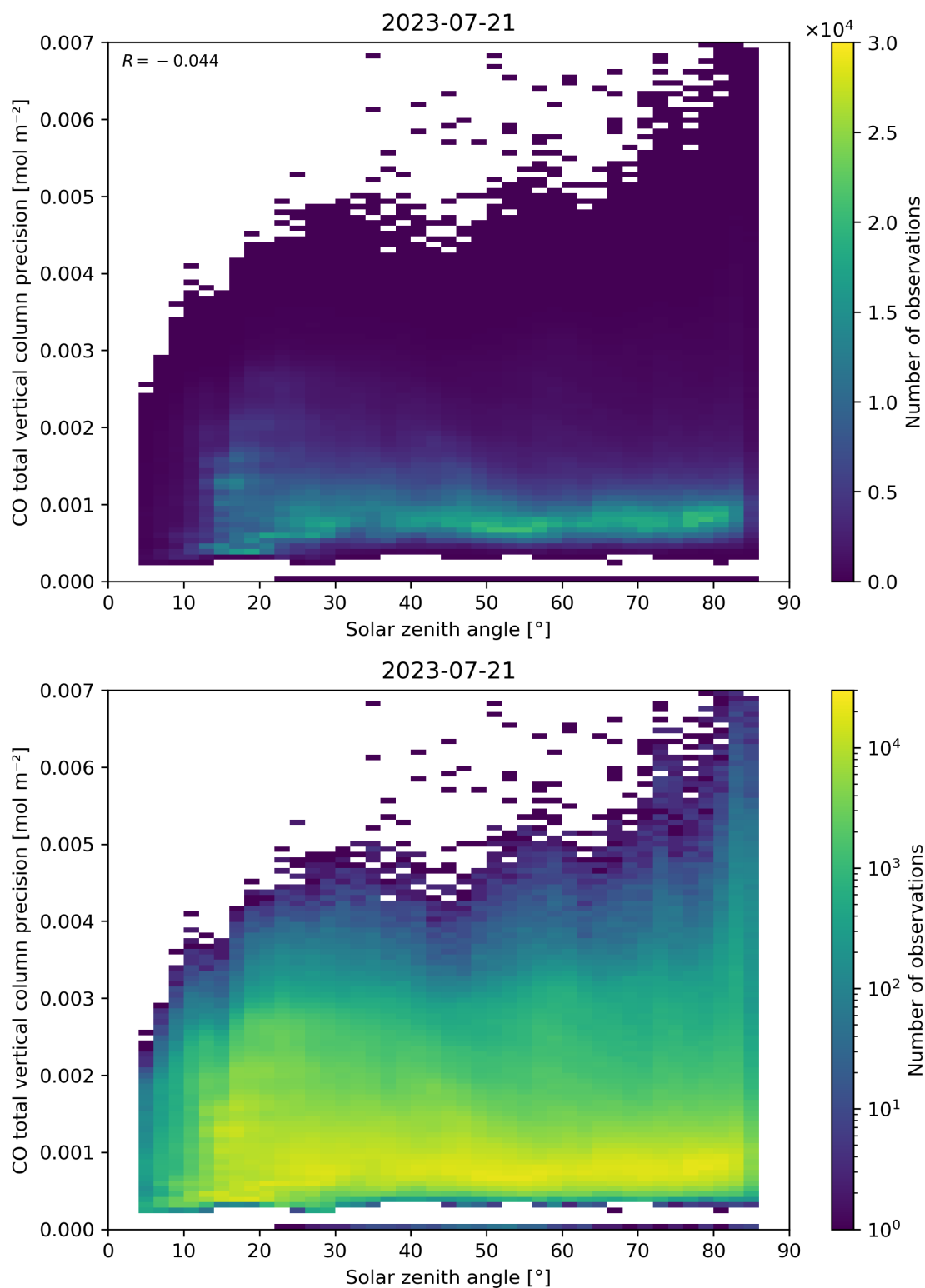
Figure 63: Scatter density plot of “Solar zenith angle” against “CO total vertical column precision” for 2023-07-20 to 2023-07-22.
