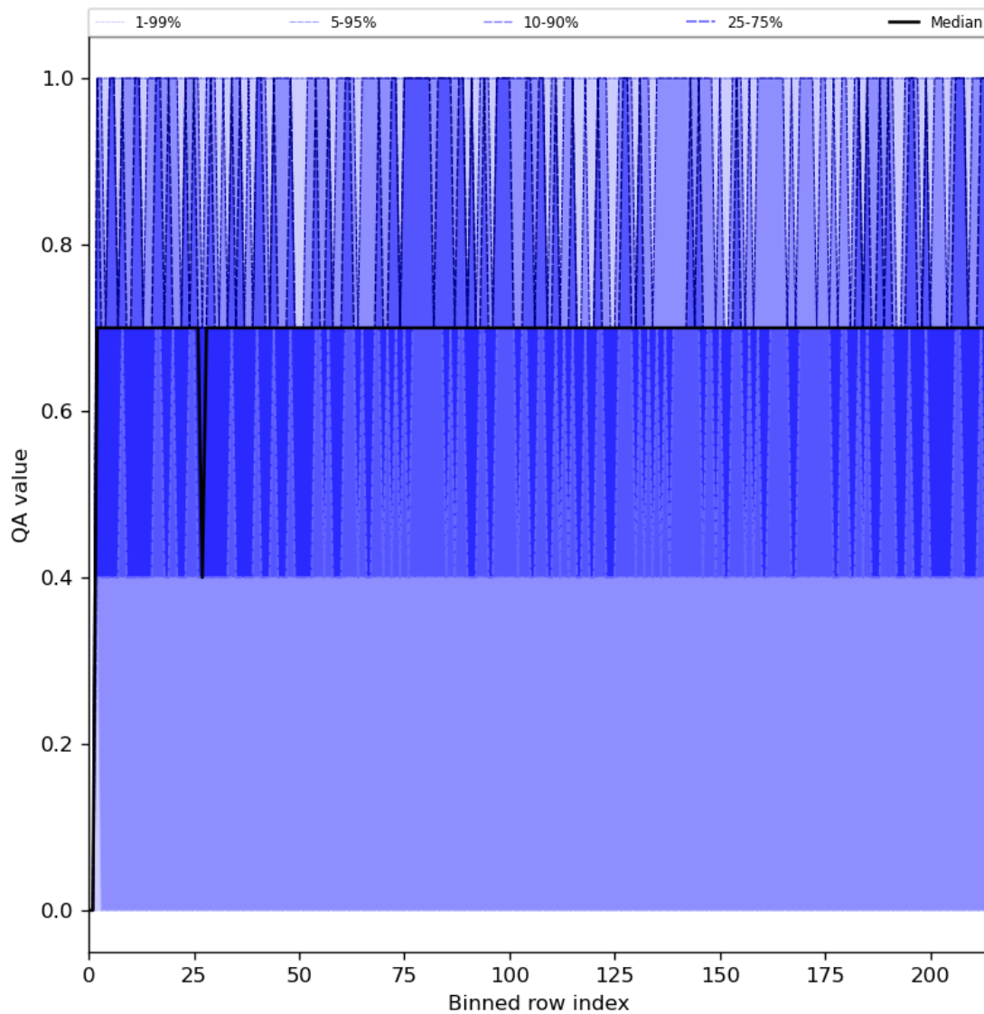
Figure 25: Along track statistics of “QA value” for 2023-07-20 to 2023-07-22
