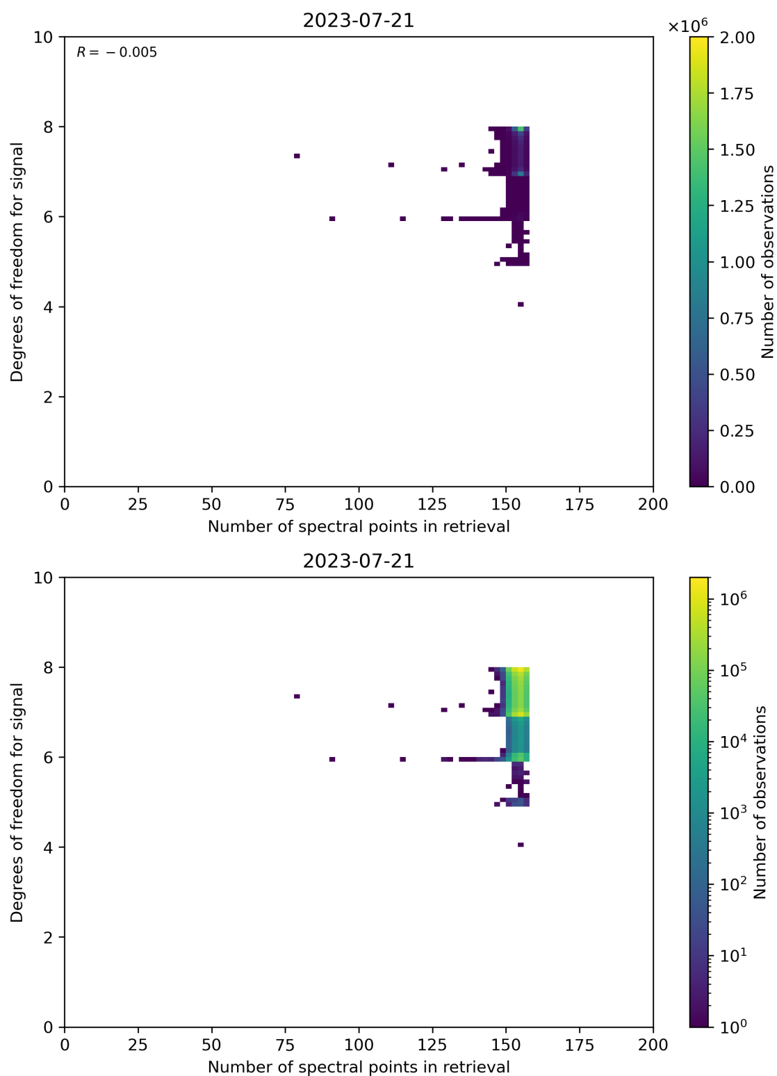
Figure 59: Scatter density plot of “Number of spectral points in retrieval” against “Degrees of freedom for signal” for 2023-07-20 to 2023-07-22.
