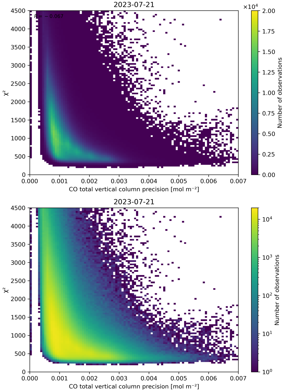
Figure 44: Scatter density plot of “CO total vertical column precision” against “ \chi^2 ” for 2023-07-20 to 2023-07-22.
