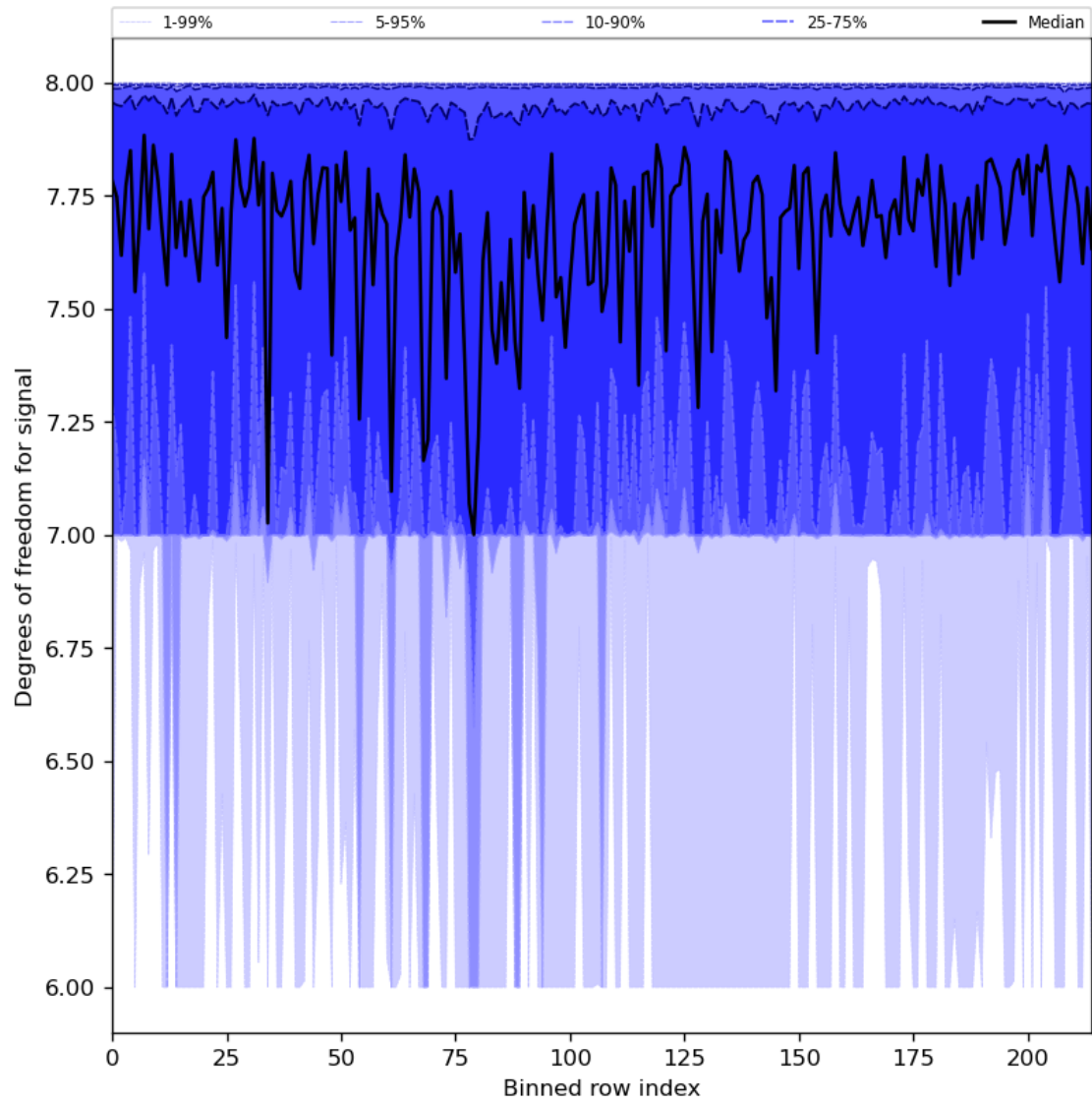
Figure 31: Along track statistics of “Degrees of freedom for signal” for 2023-07-20 to 2023-07-22
