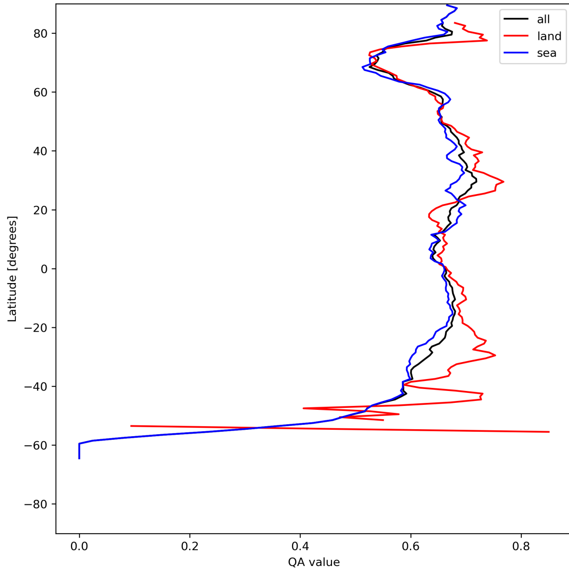
Figure 9: Zonal average of “QA value” for 2023-07-20 to 2023-07-22.
