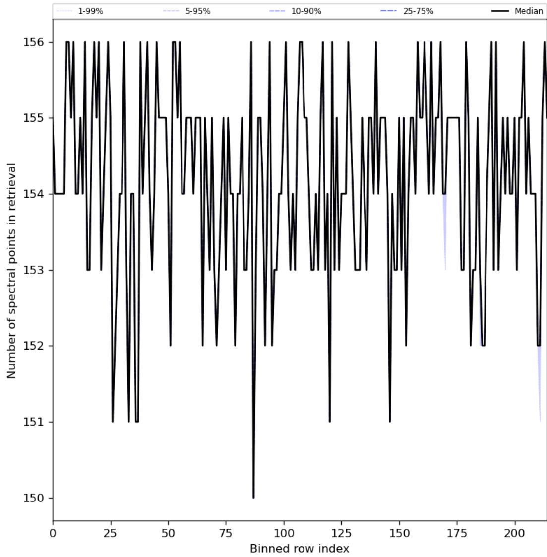
Figure 29: Along track statistics of “Number of spectral points in retrieval” for 2023-07-20 to 2023-07-22
