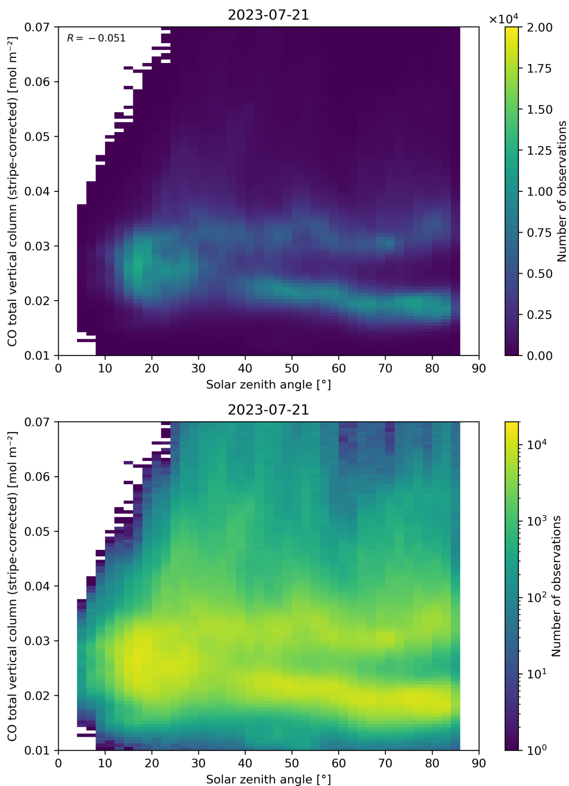
Figure 62: Scatter density plot of “Solar zenith angle” against “CO total vertical column (stripe-corrected)” for 2023-07-20 to 2023-07-22.
