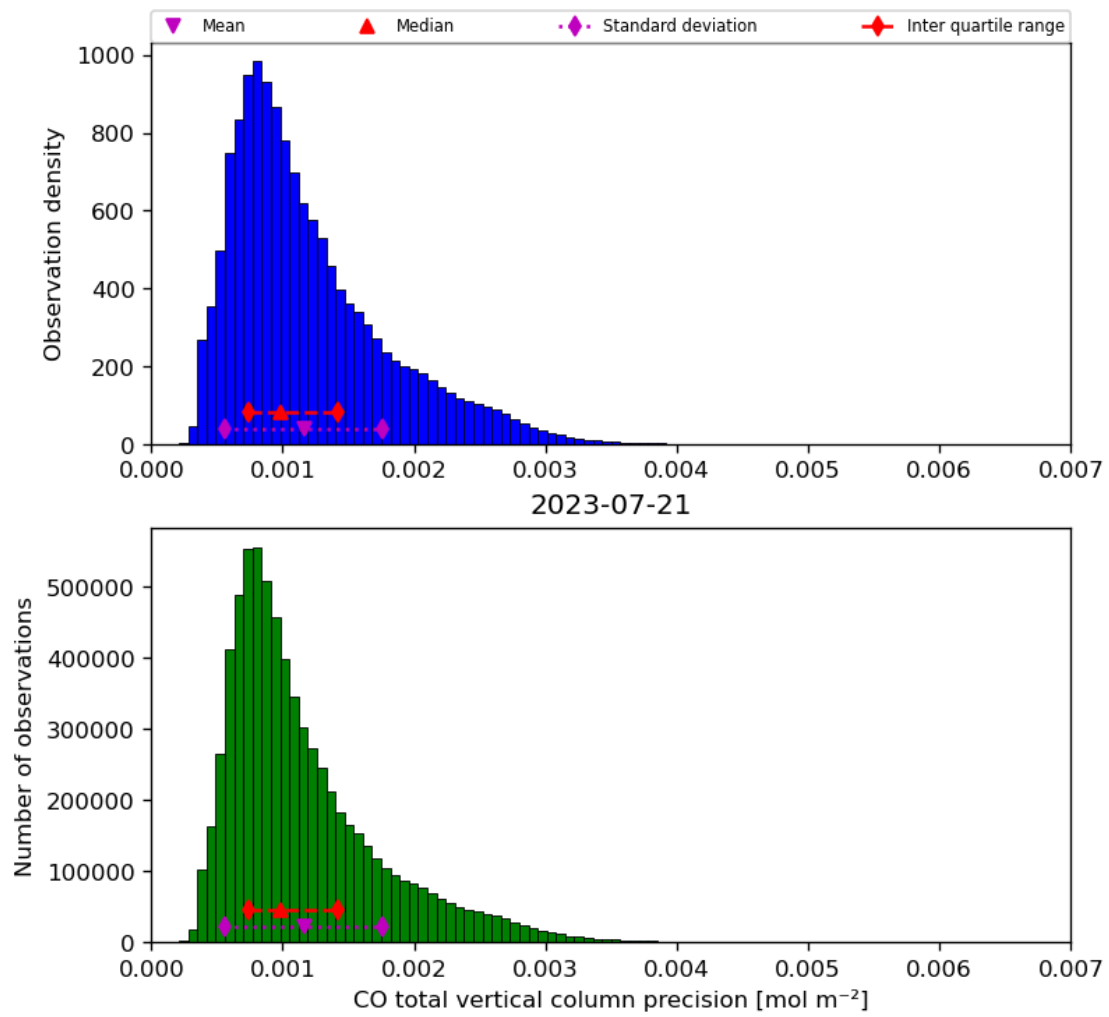
Figure 20: Histogram of “CO total vertical column precision” for 2023-07-20 to 2023-07-22
