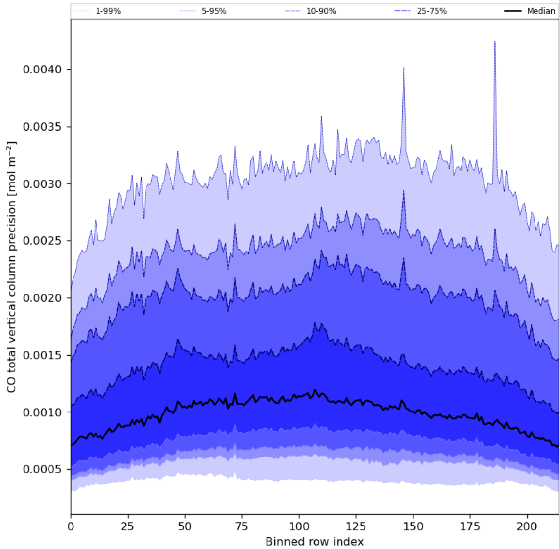
Figure 28: Along track statistics of “CO total vertical column precision” for 2023-07-20 to 2023-07-22
