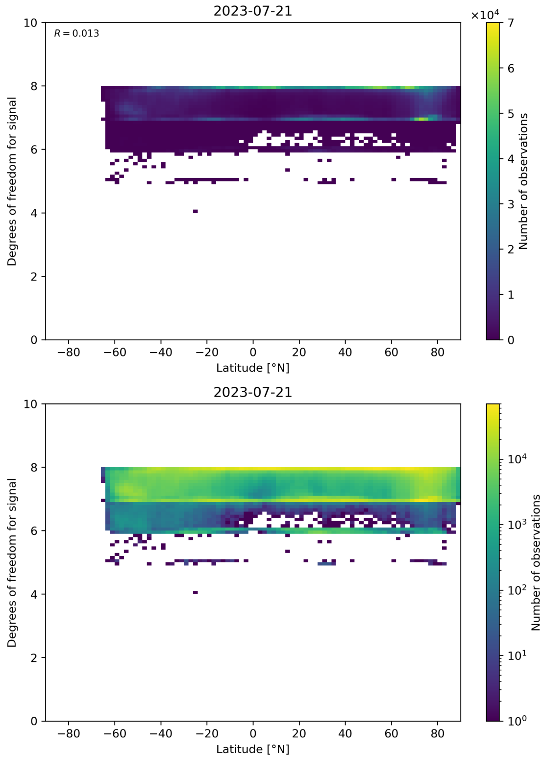
Figure 55: Scatter density plot of “Latitude” against “Degrees of freedom for signal” for 2023-07-20 to 2023-07-22.
