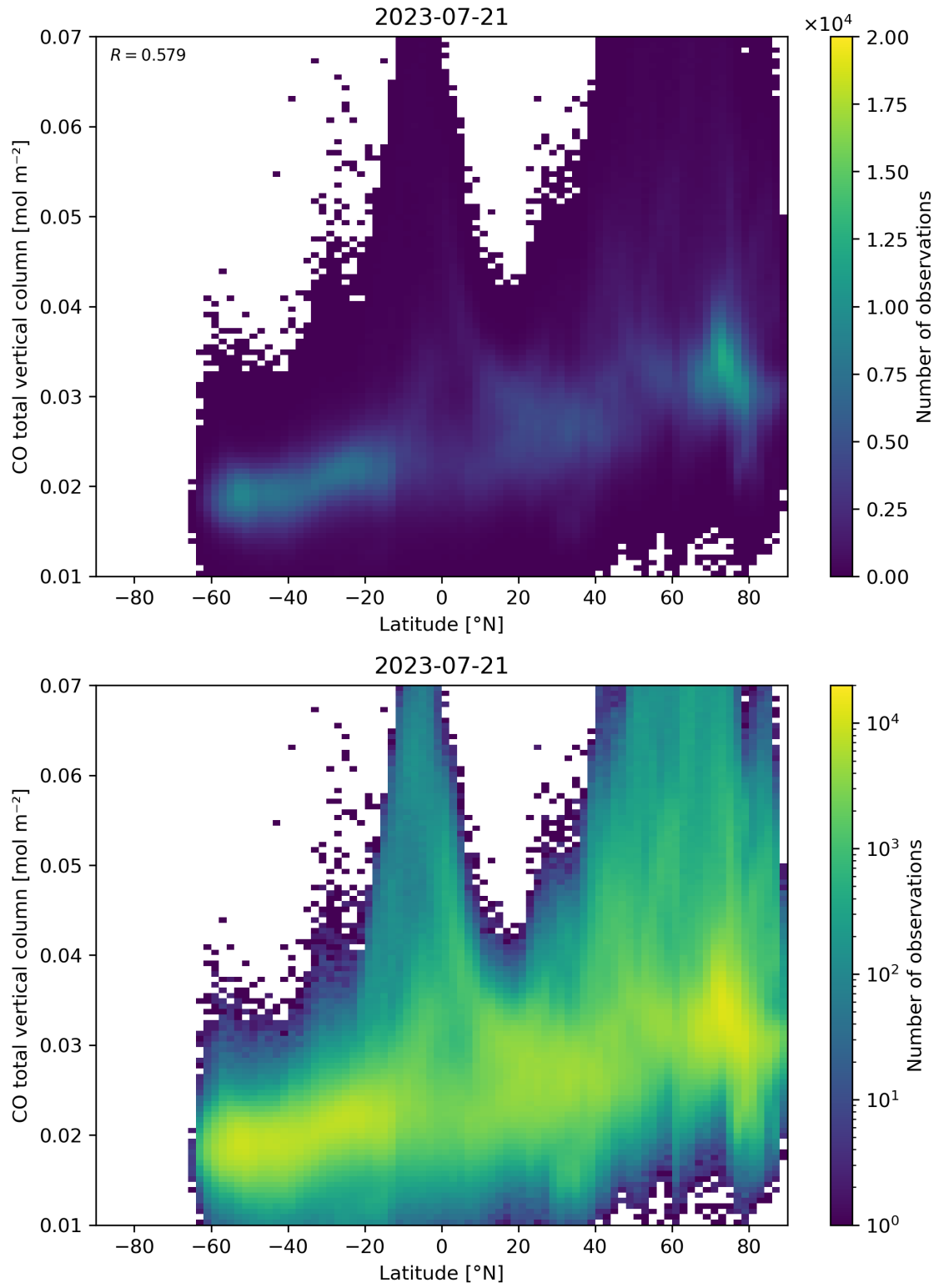
Figure 51: Scatter density plot of “Latitude” against “CO total vertical column” for 2023-07-20 to 2023-07-22.
