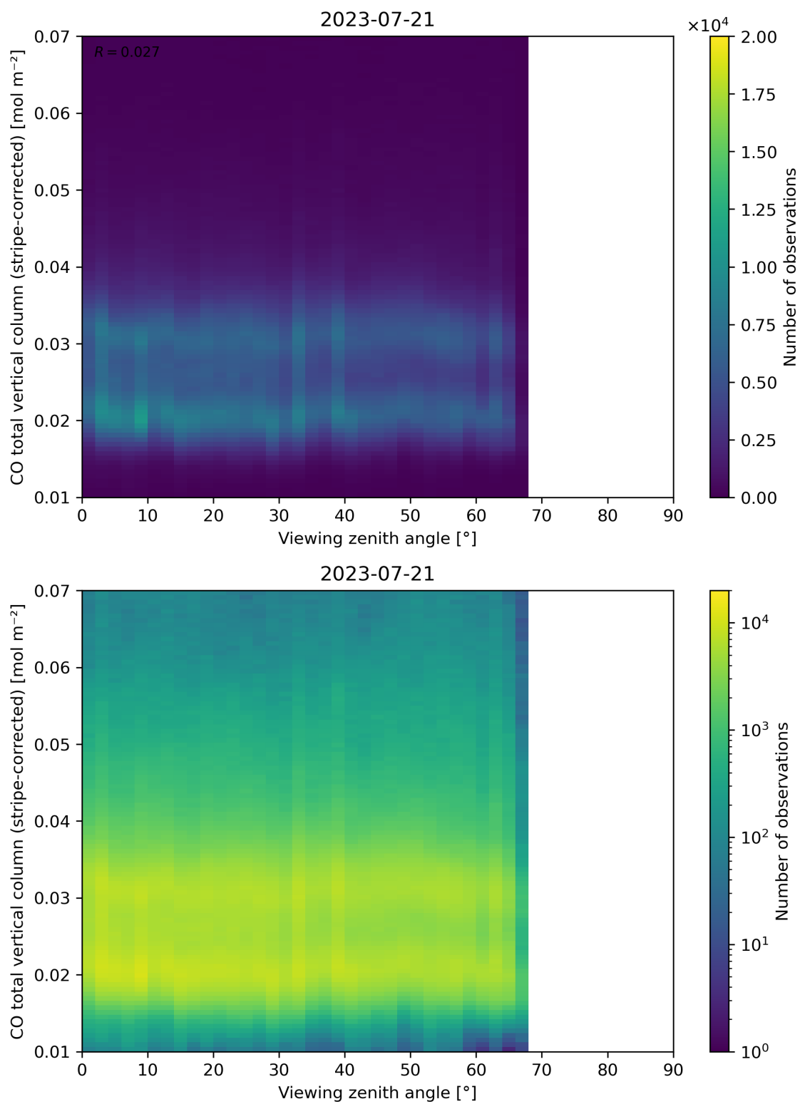
Figure 70: Scatter density plot of “Viewing zenith angle” against “CO total vertical column (stripe-corrected)” for 2023-07-20 to 2023-07-22.
