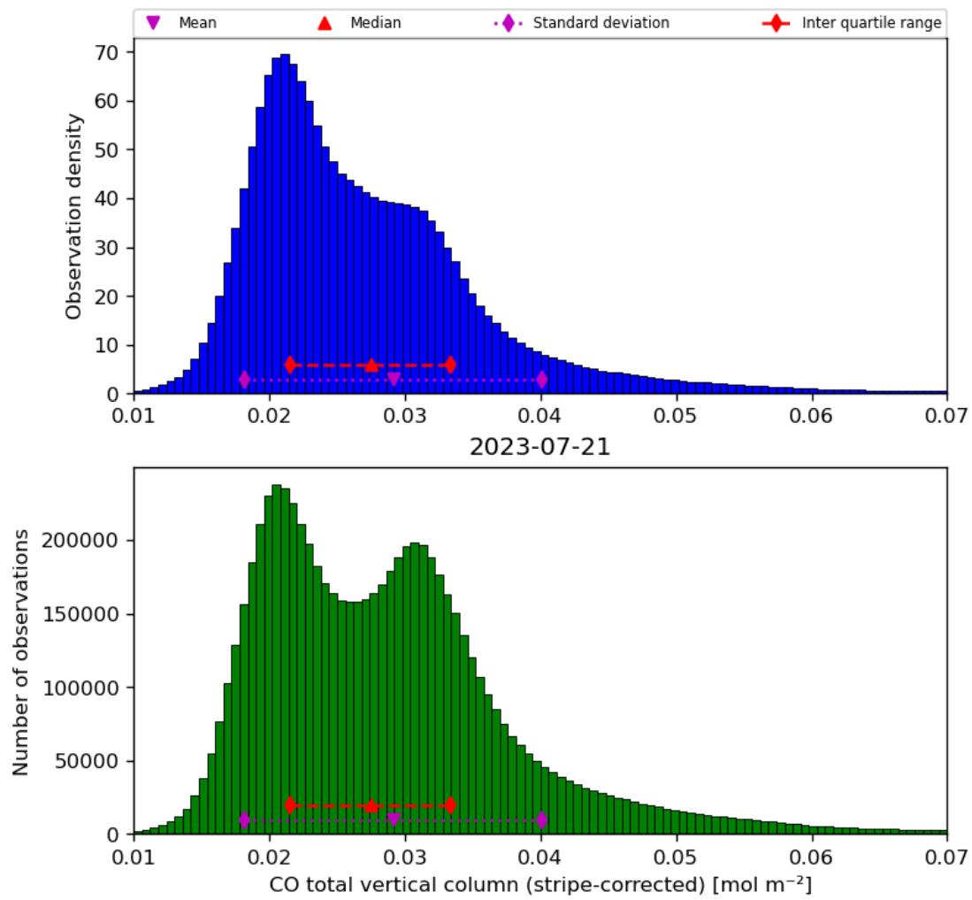
Figure 19: Histogram of “CO total vertical column (stripe-corrected)” for 2023-07-20 to 2023-07-22
