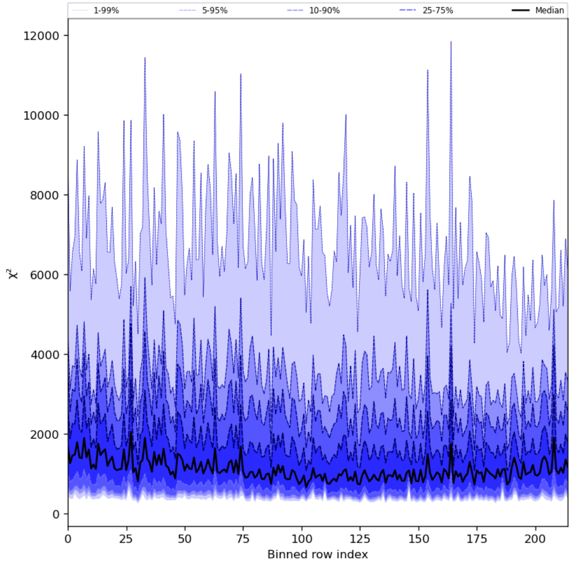
Figure 30: Along track statistics of “ \chi^2 ” for 2023-07-20 to 2023-07-22
