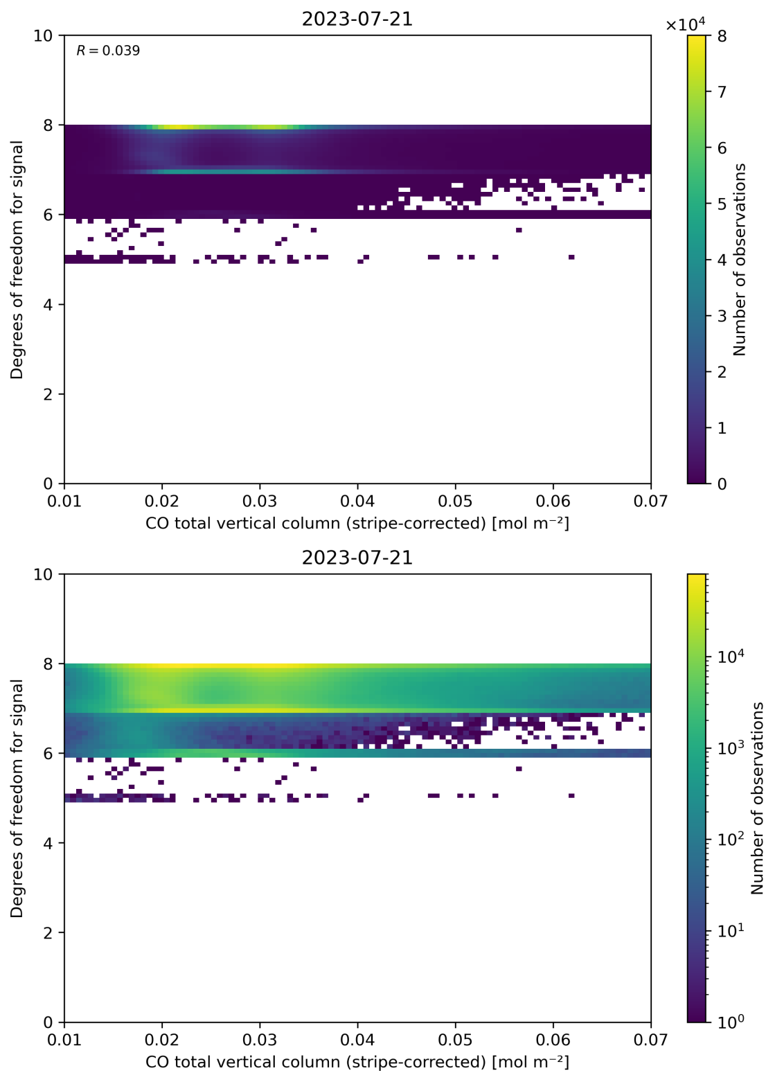
Figure 38: Scatter density plot of “CO total vertical column (stripe-corrected)” against “Degrees of freedom for signal” for 2023-07-20 to 2023-07-22.
