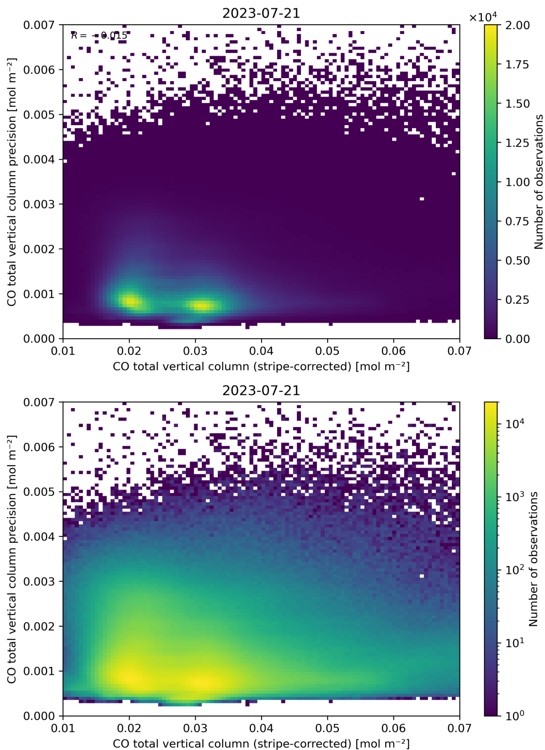
Figure 36: Scatter density plot of “CO total vertical column (stripe-corrected)” against “CO total vertical column precision” for 2023-07-20 to 2023-07-22.
