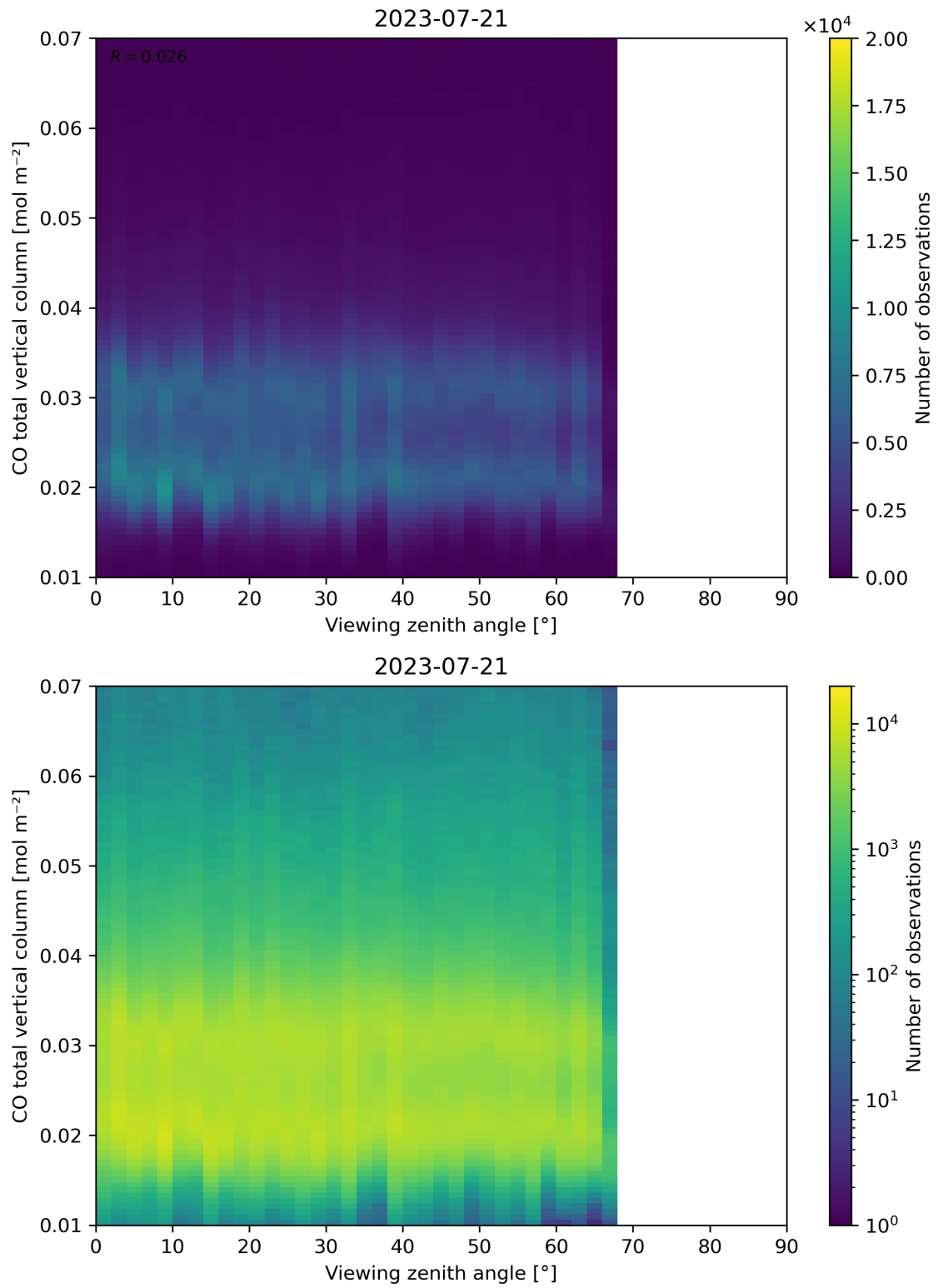
Figure 69: Scatter density plot of “Viewing zenith angle” against “CO total vertical column” for 2023-07-20 to 2023-07-22.
