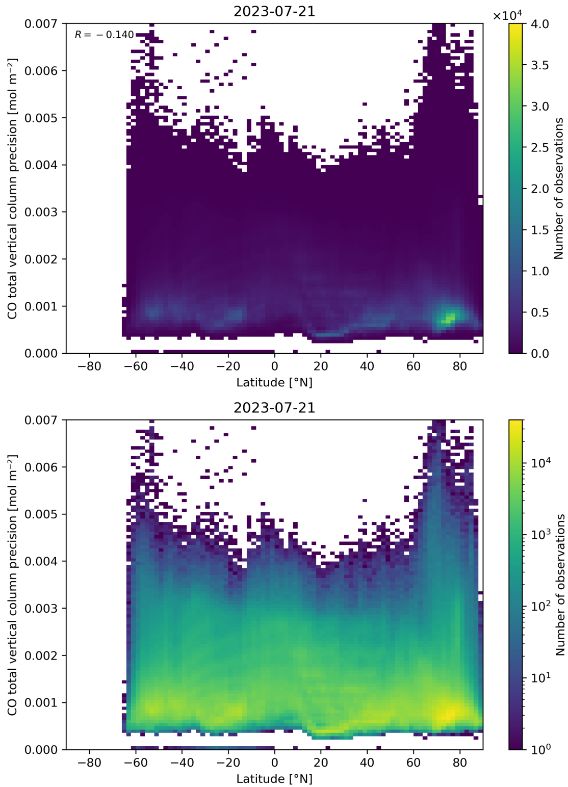
Figure 53: Scatter density plot of “Latitude” against “CO total vertical column precision” for 2023-07-20 to 2023-07-22.
