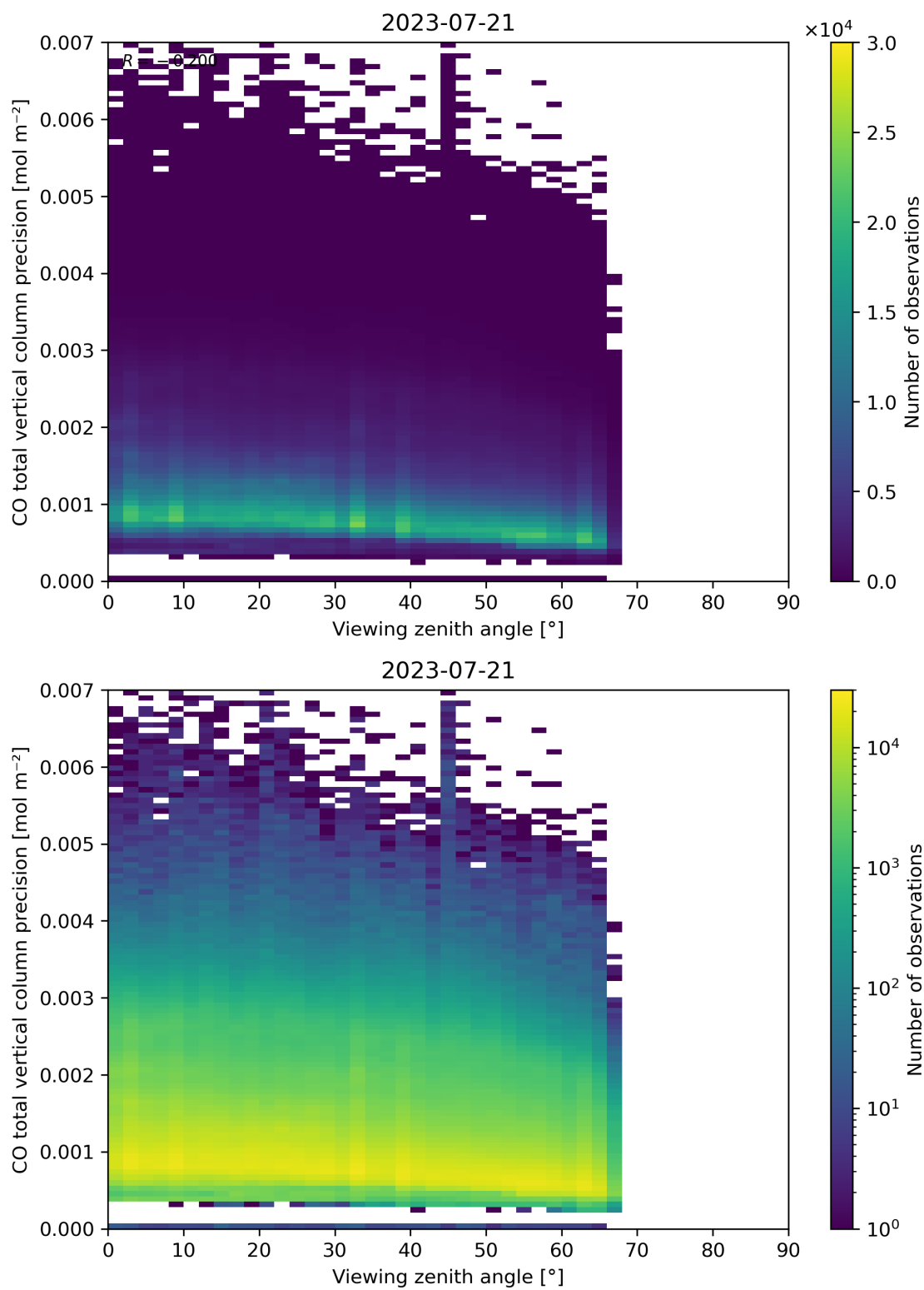
Figure 71: Scatter density plot of “Viewing zenith angle” against “CO total vertical column precision” for 2023-07-20 to 2023-07-22.
