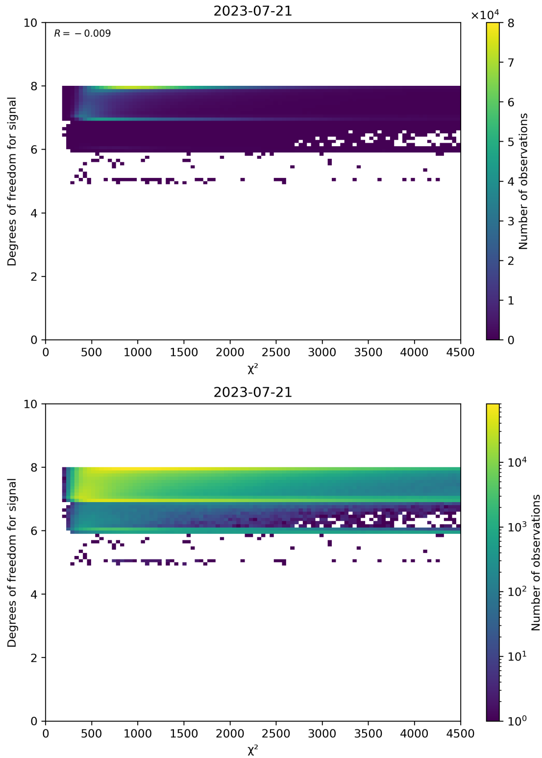
Figure 48: Scatter density plot of “ \chi^2 ” against “Degrees of freedom for signal” for 2023-07-20 to 2023-07-22.
