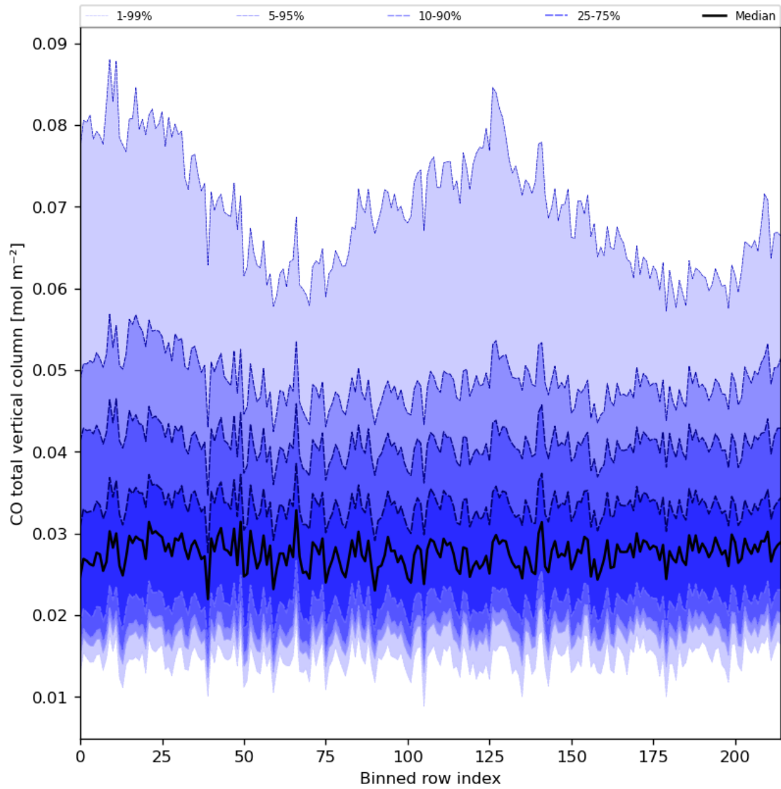
Figure 26: Along track statistics of “CO total vertical column” for 2023-07-20 to 2023-07-22
