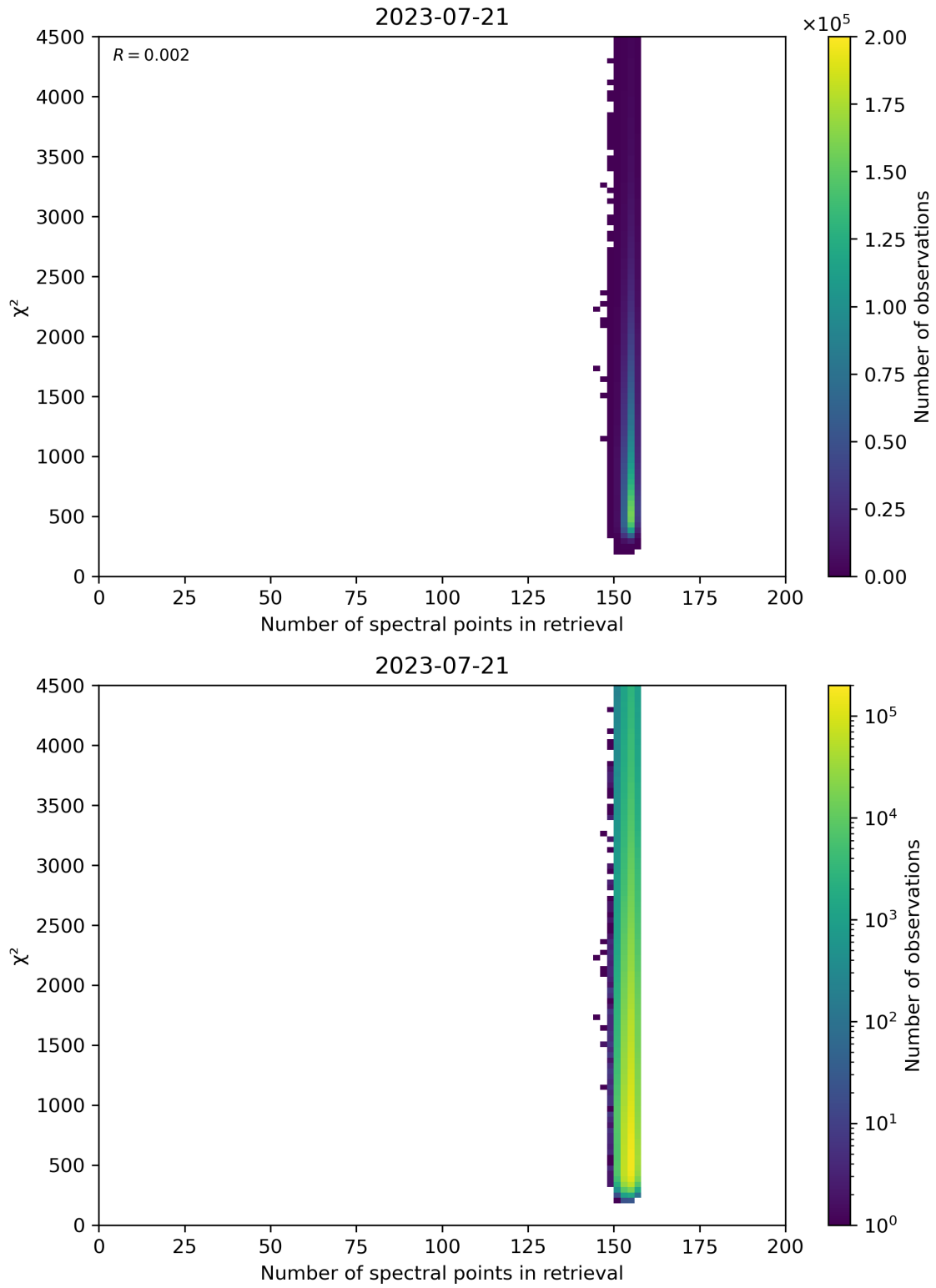
Figure 58: Scatter density plot of “Number of spectral points in retrieval” against “ \chi^2 ” for 2023-07-20 to 2023-07-22.
