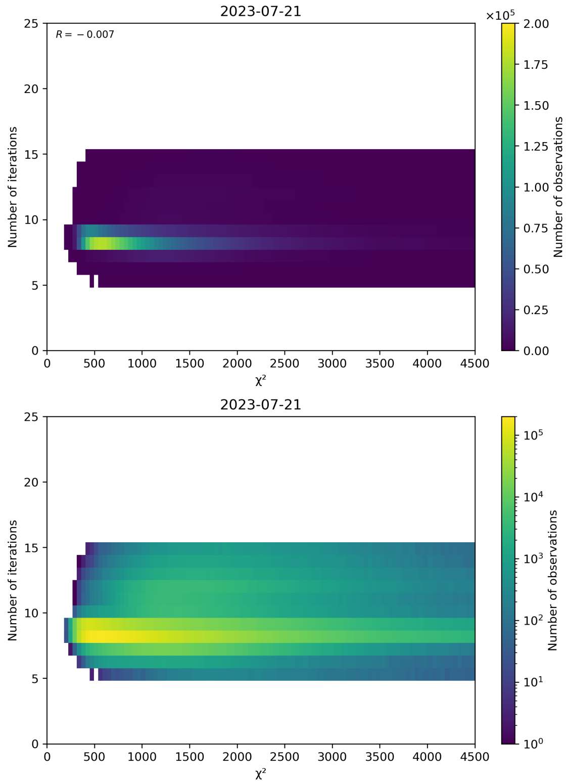
Figure 49: Scatter density plot of “ \chi^2 ” against “Number of iterations” for 2023-07-20 to 2023-07-22.
