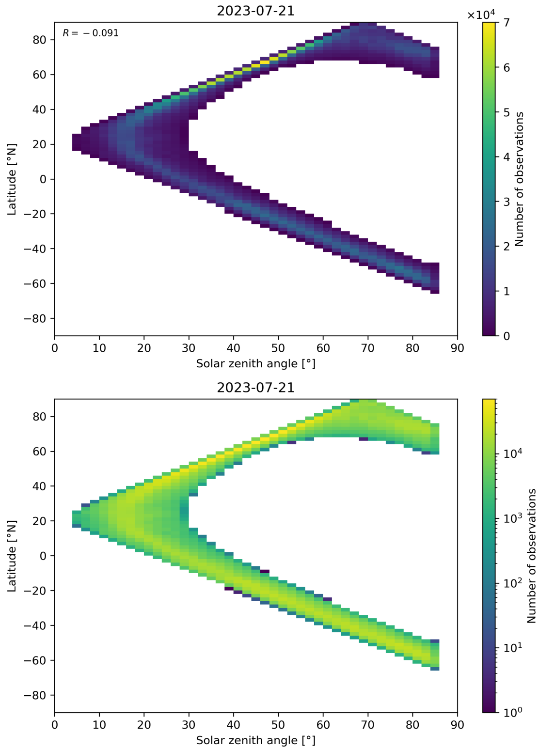
Figure 66: Scatter density plot of “Solar zenith angle” against “Latitude” for 2023-07-20 to 2023-07-22.
