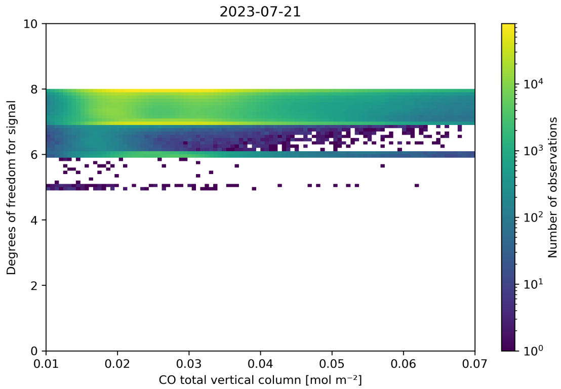
Figure 41: Scatter density plot of “CO total vertical column” against “Degrees of freedom for signal” for 2023-07-20 to 2023-07-22.
