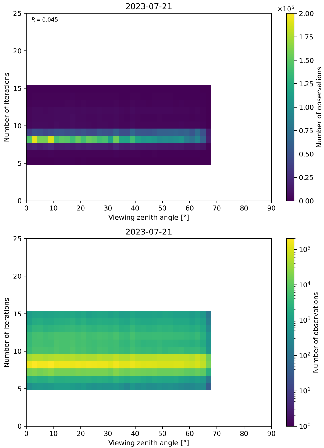
Figure 75: Scatter density plot of “Viewing zenith angle” against “Number of iterations” for 2023-07-20 to 2023-07-22.
