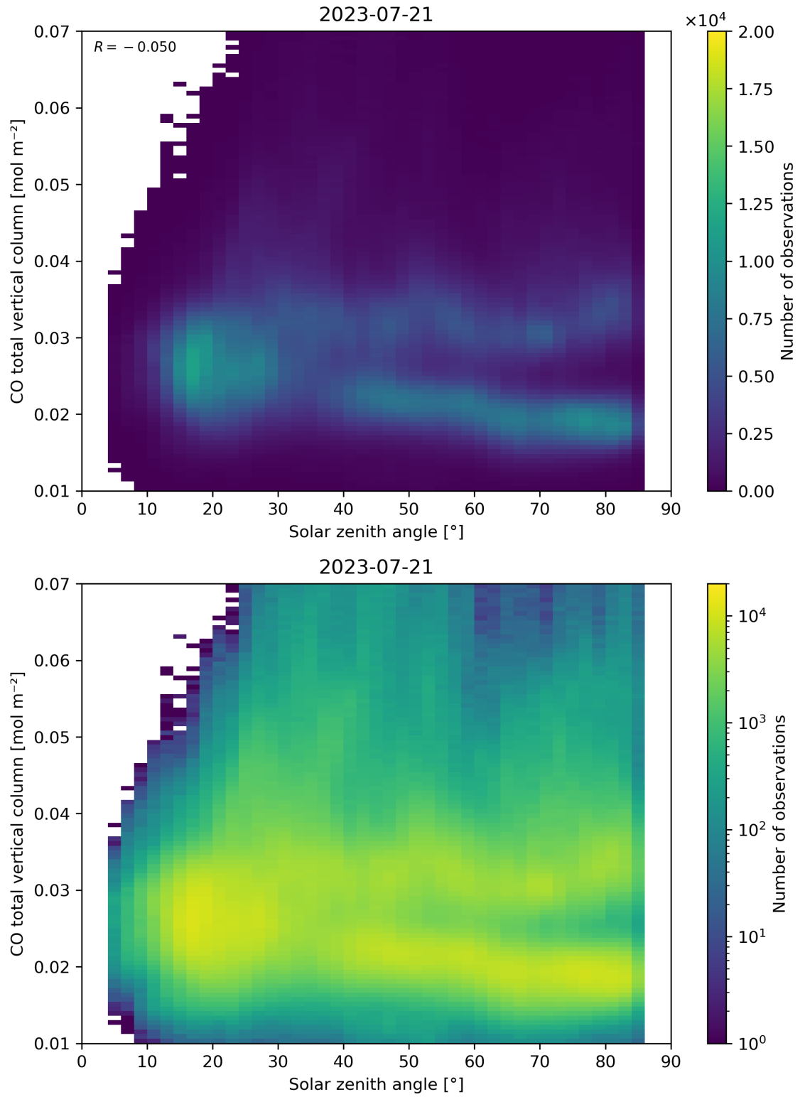
Figure 61: Scatter density plot of “Solar zenith angle” against “CO total vertical column” for 2023-07-20 to 2023-07-22.
