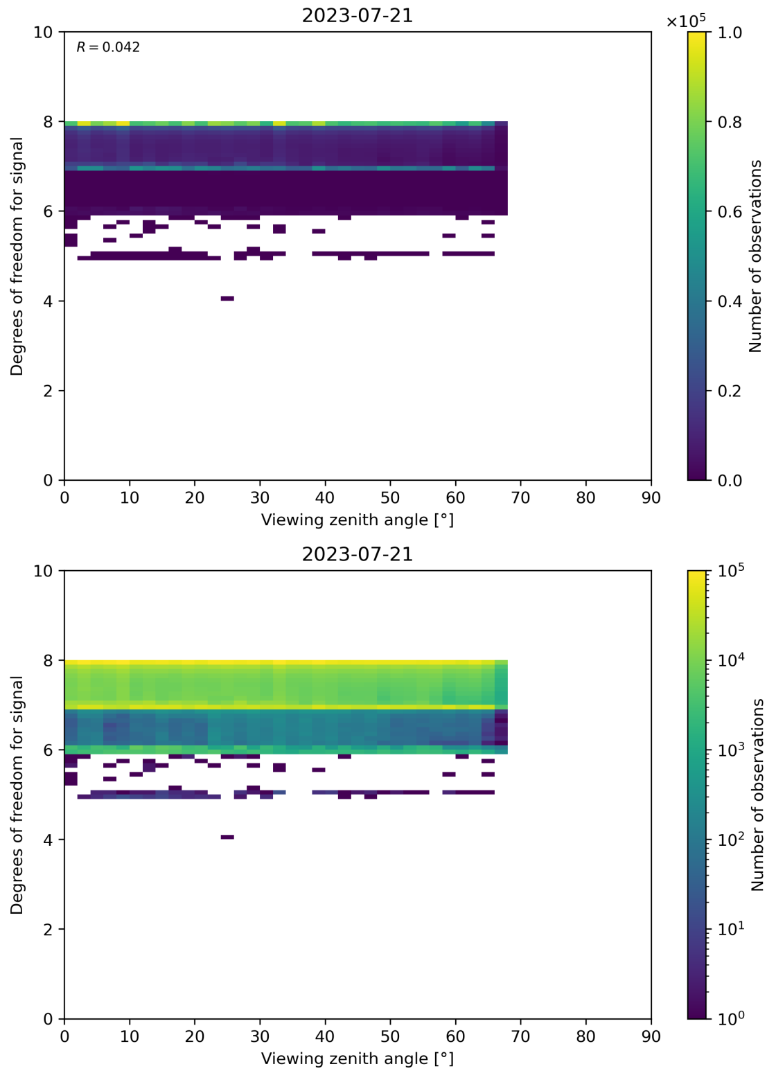
Figure 73: Scatter density plot of “Viewing zenith angle” against “Degrees of freedom for signal” for 2023-07-20 to 2023-07-22.
