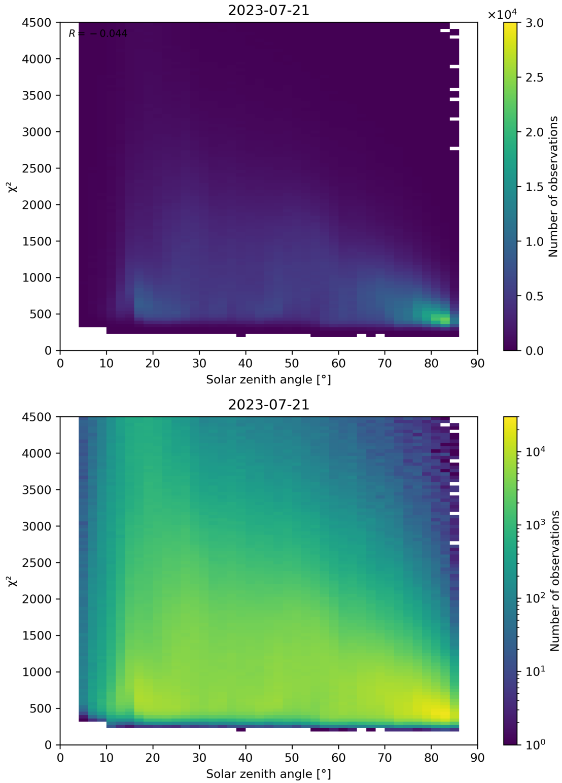
Figure 64: Scatter density plot of “Solar zenith angle” against “ \chi^2 ” for 2023-07-20 to 2023-07-22.
