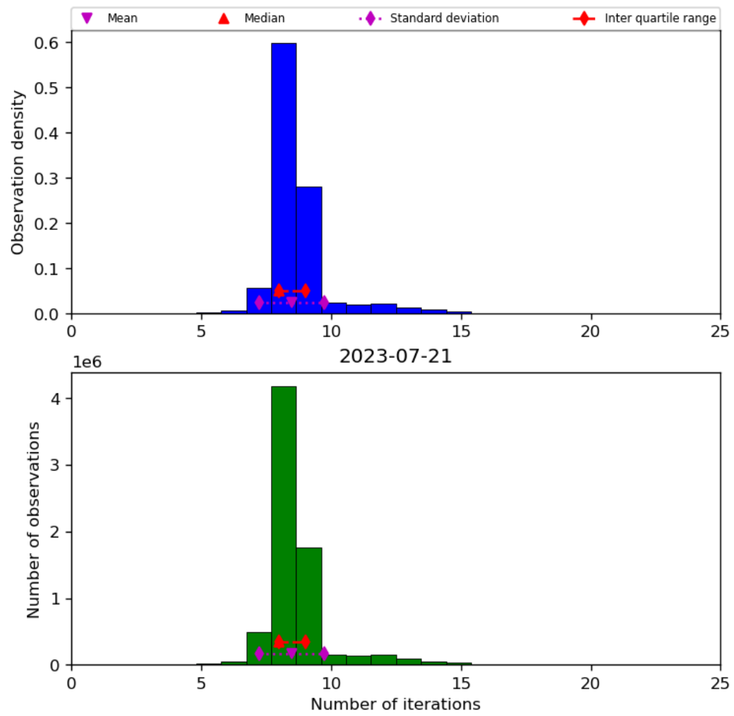
Figure 24: Histogram of “Number of iterations” for 2023-07-20 to 2023-07-22
