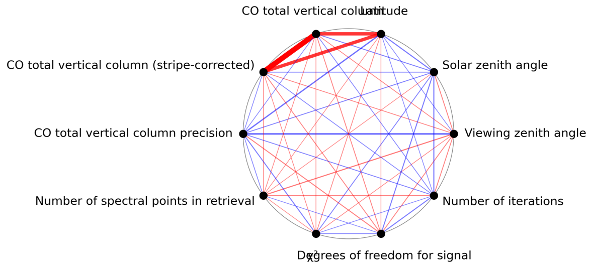
Figure 1: Map of correlation graph for 2023-07-20 to 2023-07-22.
