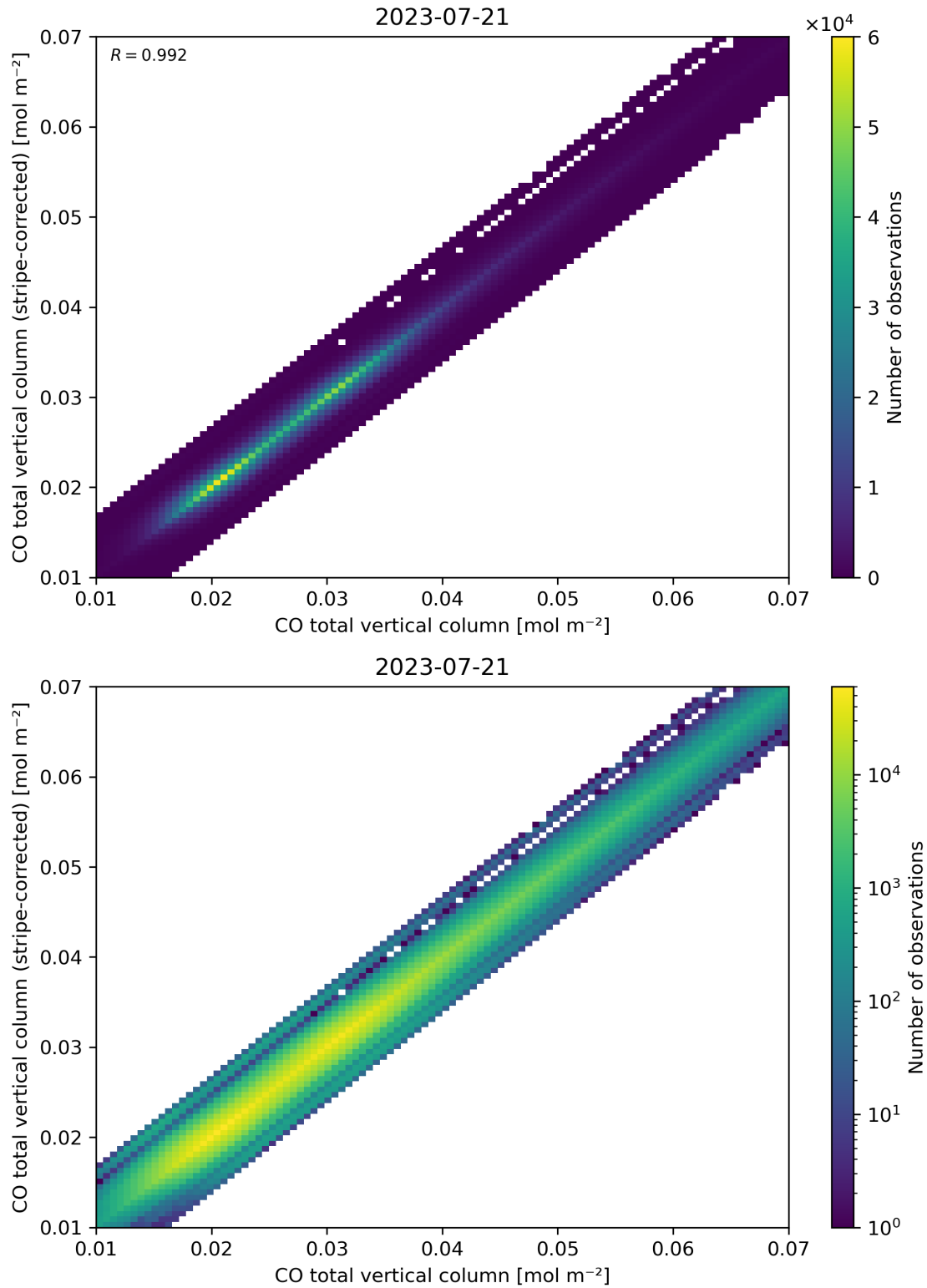
Figure 33: Scatter density plot of “CO total vertical column” against “CO total vertical column (stripe-corrected)” for 2023-07-20 to 2023-07-22.
