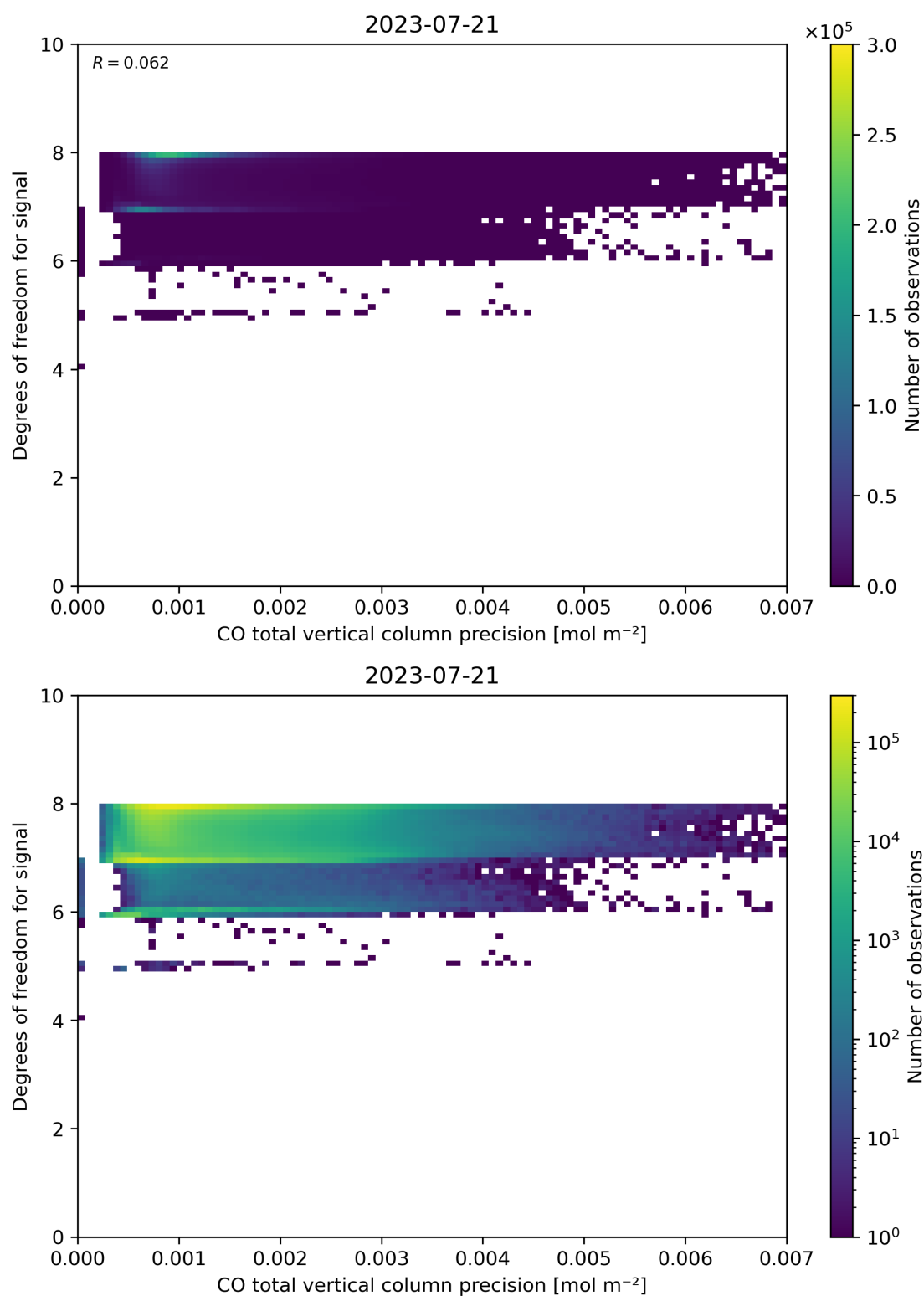
Figure 45: Scatter density plot of “CO total vertical column precision” against “Degrees of freedom for signal” for 2023-07-20 to 2023-07-22.
