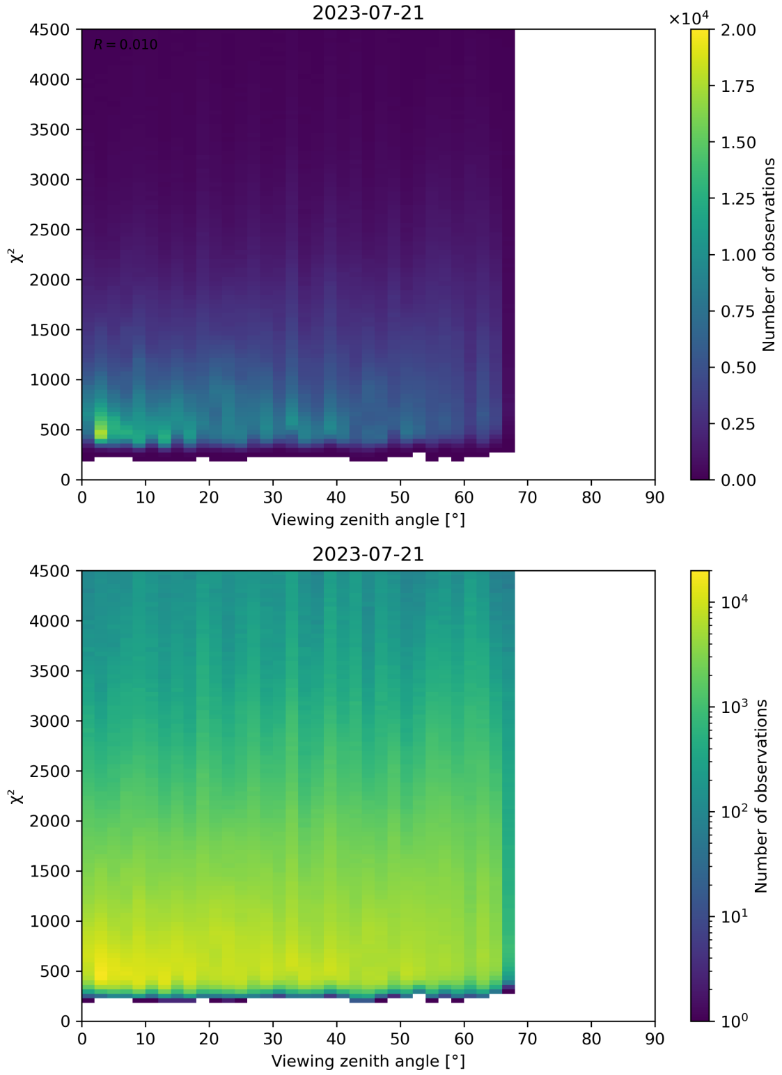
Figure 72: Scatter density plot of “Viewing zenith angle” against “ \chi^2 ” for 2023-07-20 to 2023-07-22.
