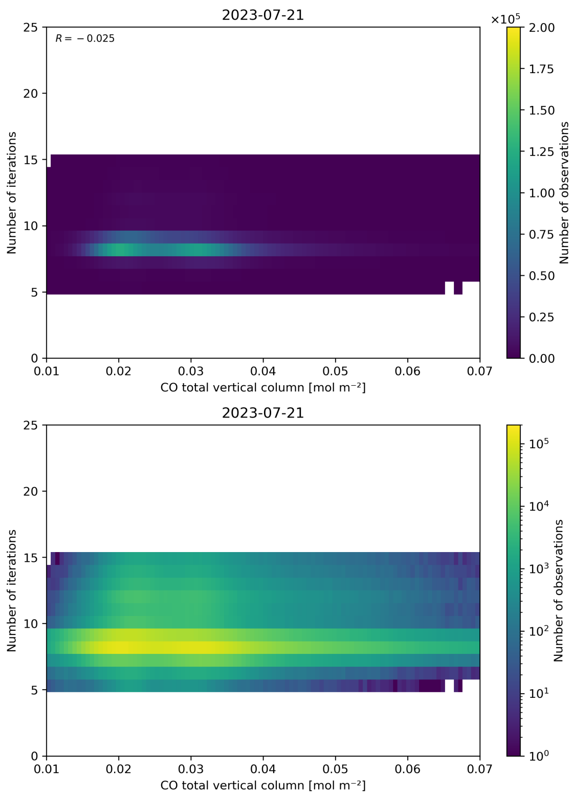
Figure 42: Scatter density plot of “CO total vertical column” against “Number of iterations” for 2023-07-20 to 2023-07-22.
