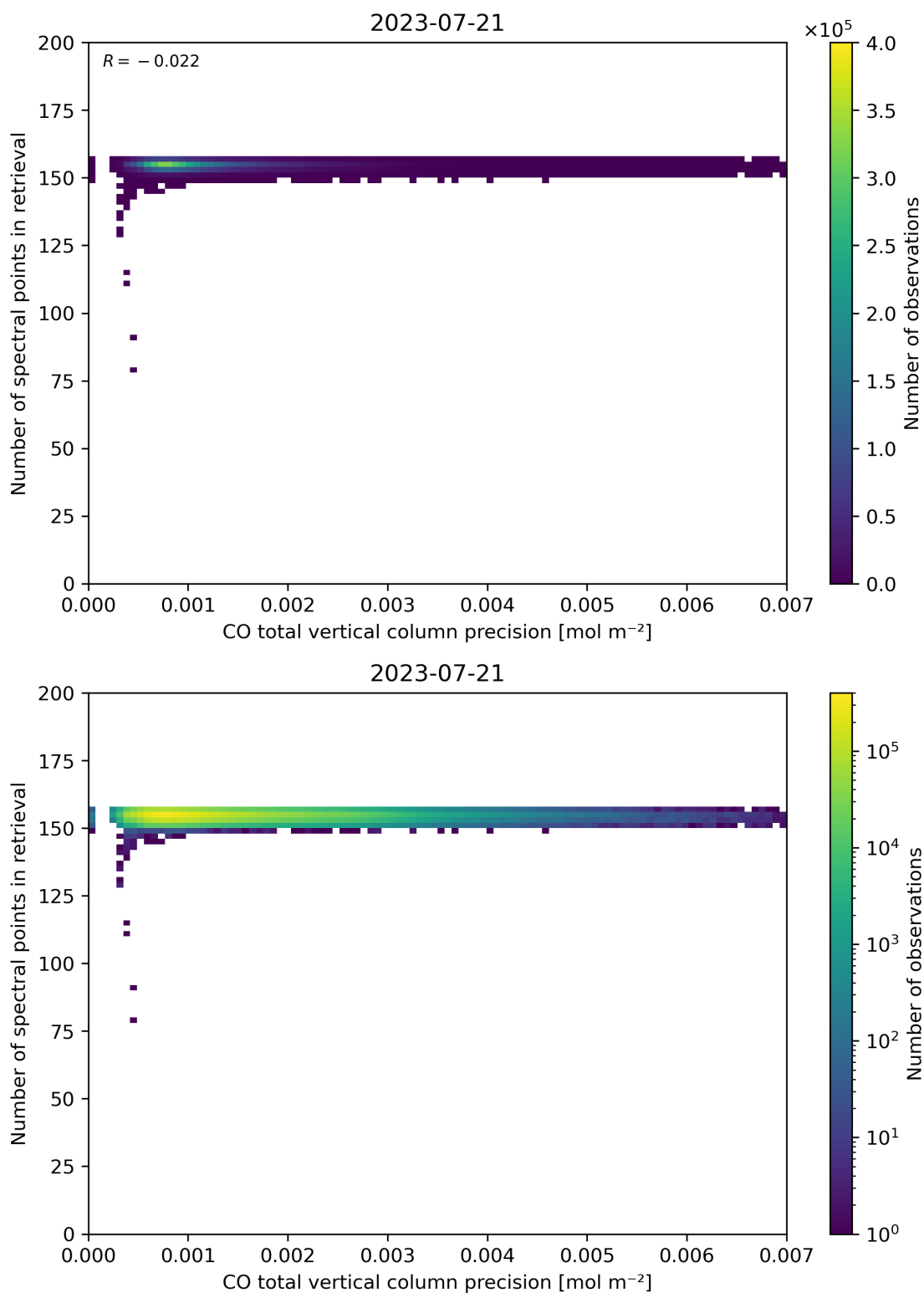
Figure 47: Scatter density plot of “CO total vertical column precision” against “Number of spectral points in retrieval” for 2023-07-20 to 2023-07-22.
