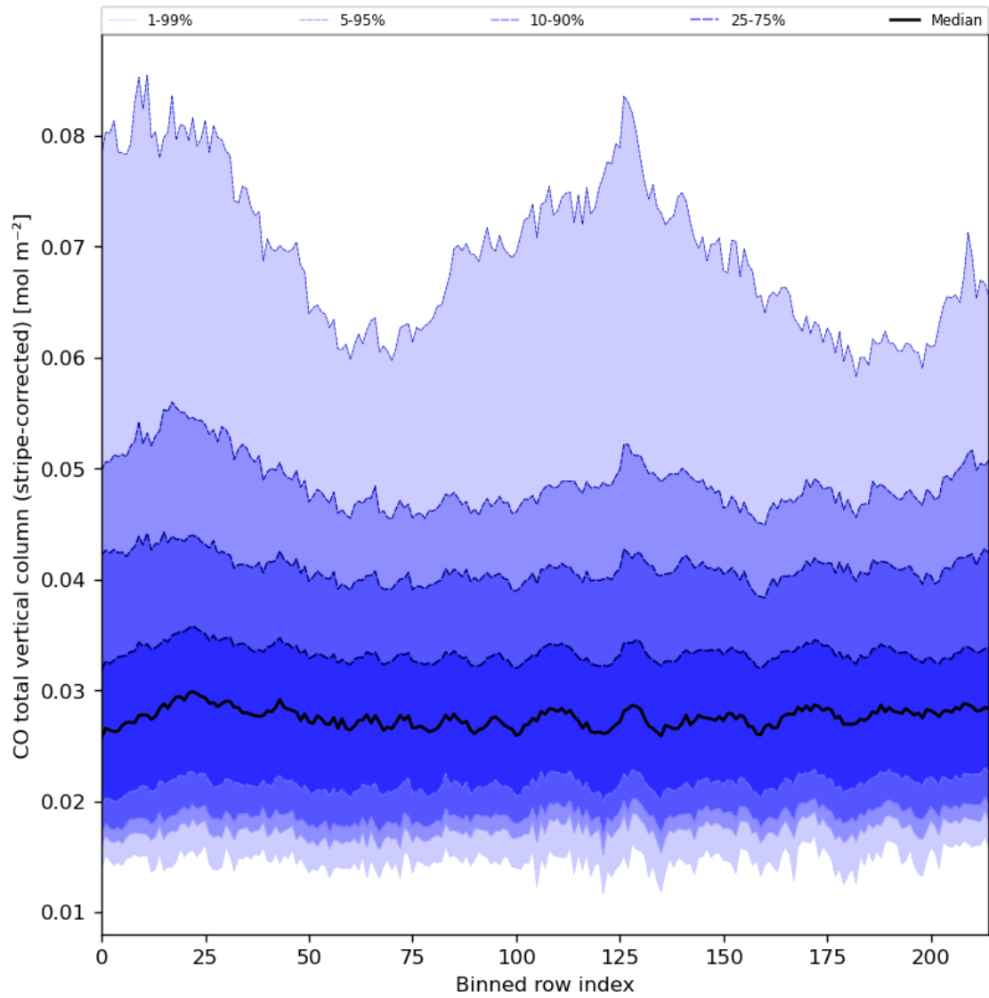
Figure 27: Along track statistics of “CO total vertical column (stripe-corrected)” for 2023-07-20 to 2023-07-22
