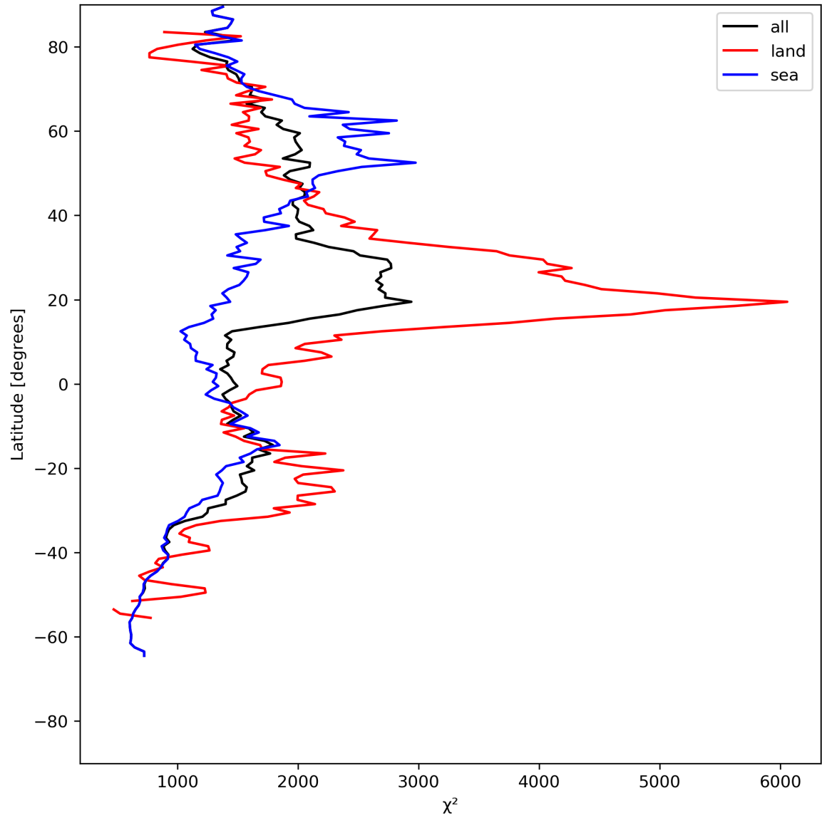
Figure 14: Zonal average of “ \chi^2 ” for 2023-07-20 to 2023-07-22.
