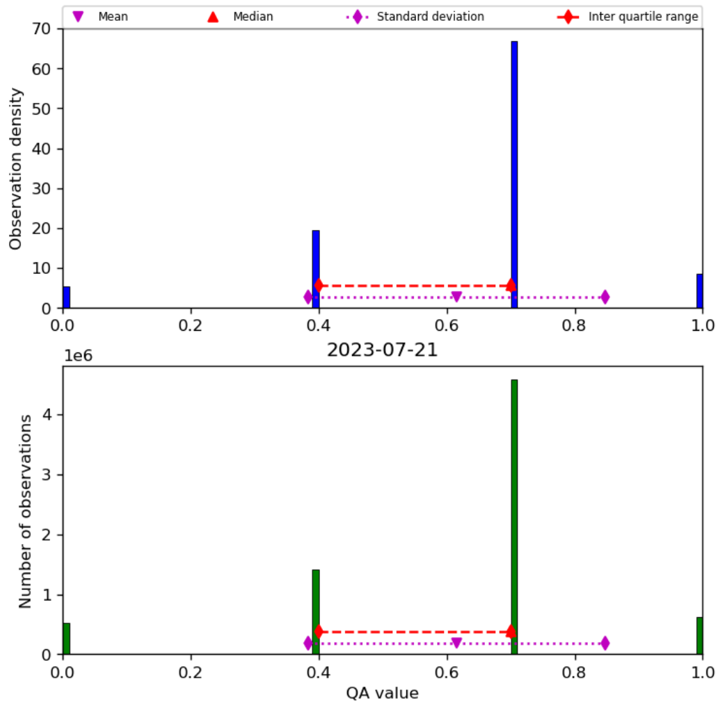
Figure 17: Histogram of “QA value” for 2023-07-20 to 2023-07-22
