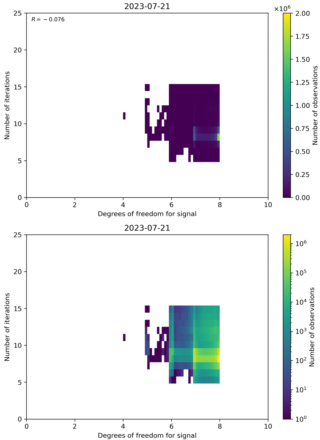
Figure 50: Scatter density plot of “Degrees of freedom for signal” against “Number of iterations” for 2023-07-20 to 2023-07-22.
