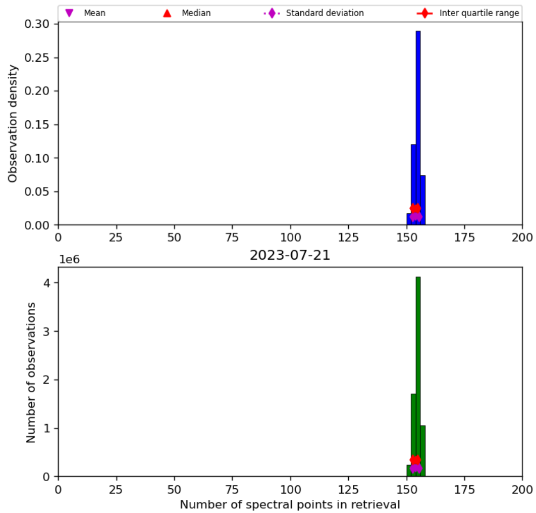
Figure 21: Histogram of “Number of spectral points in retrieval” for 2023-07-20 to 2023-07-22
