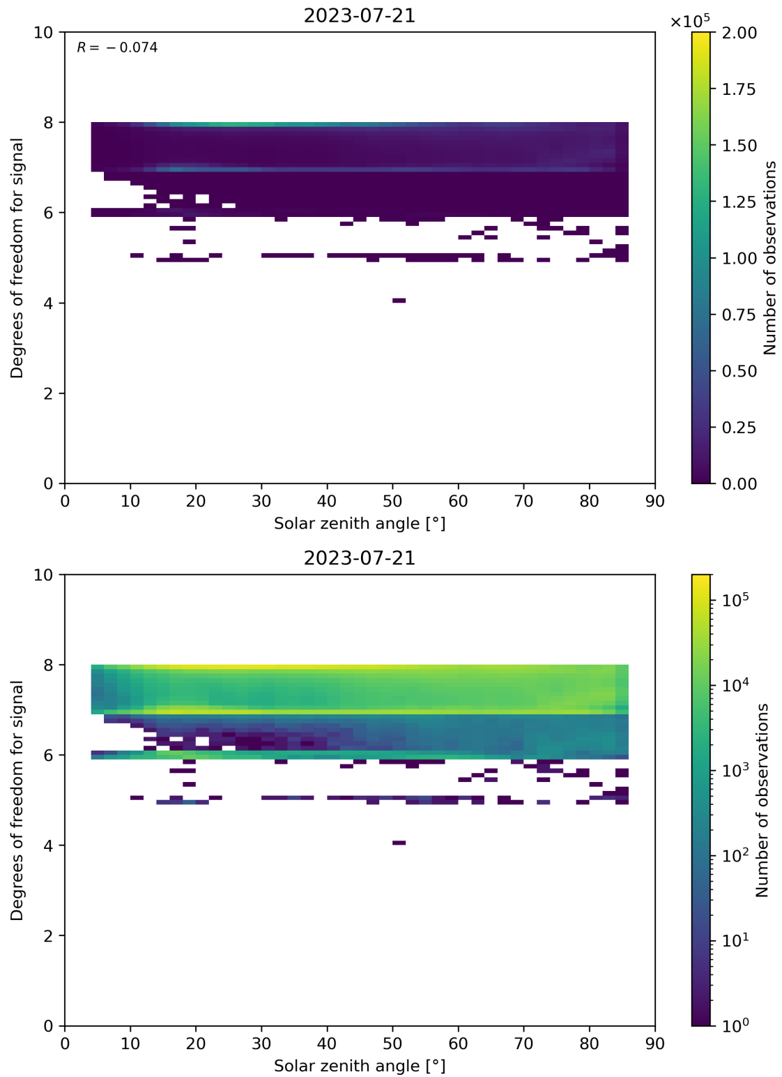
Figure 65: Scatter density plot of “Solar zenith angle” against “Degrees of freedom for signal” for 2023-07-20 to 2023-07-22.
