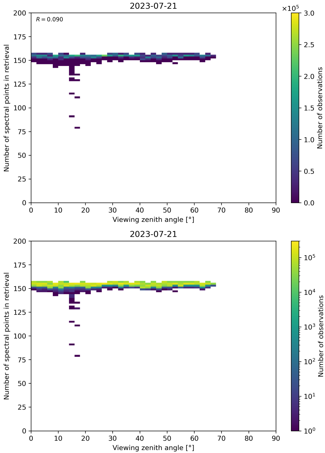
Figure 76: Scatter density plot of “Viewing zenith angle” against “Number of spectral points in retrieval” for 2023-07-20 to 2023-07-22.
