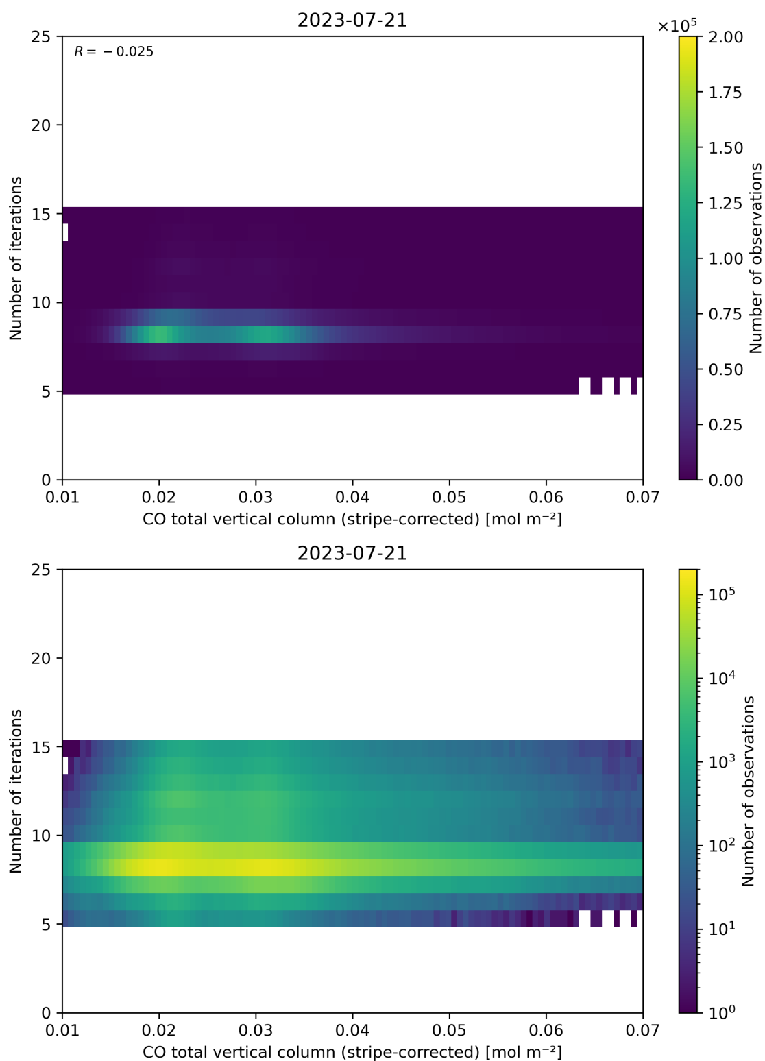
Figure 39: Scatter density plot of “CO total vertical column (stripe-corrected)” against “Number of iterations” for 2023-07-20 to 2023-07-22.
