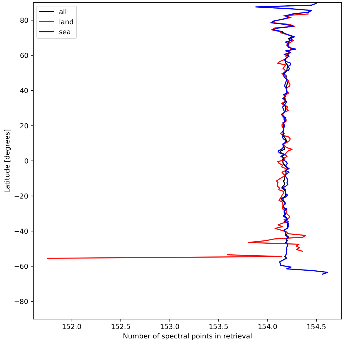
Figure 13: Zonal average of “Number of spectral points in retrieval” for 2023-07-20 to 2023-07-22.
