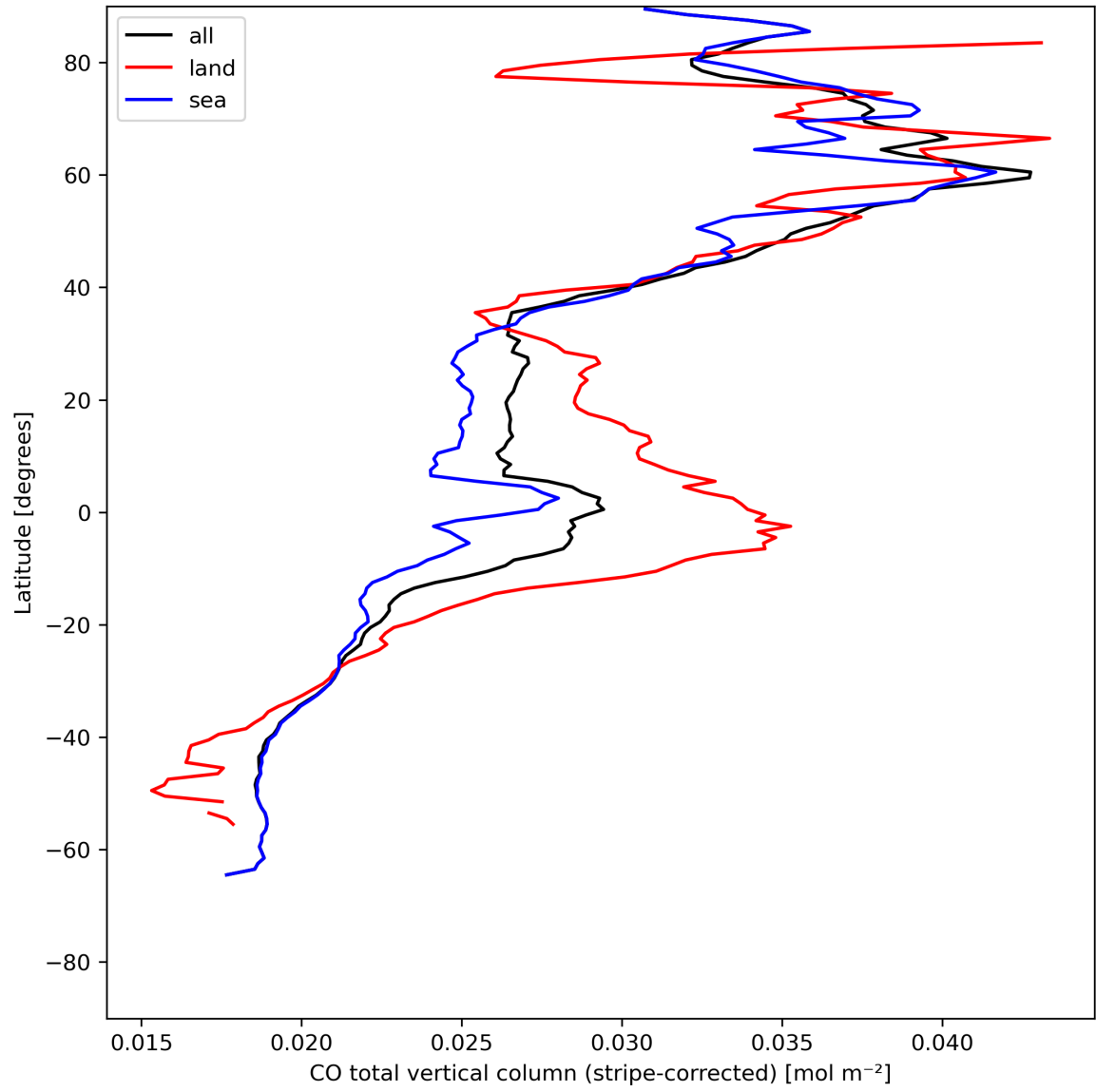
Figure 11: Zonal average of “CO total vertical column (stripe-corrected)” for 2023-07-20 to 2023-07-22.
