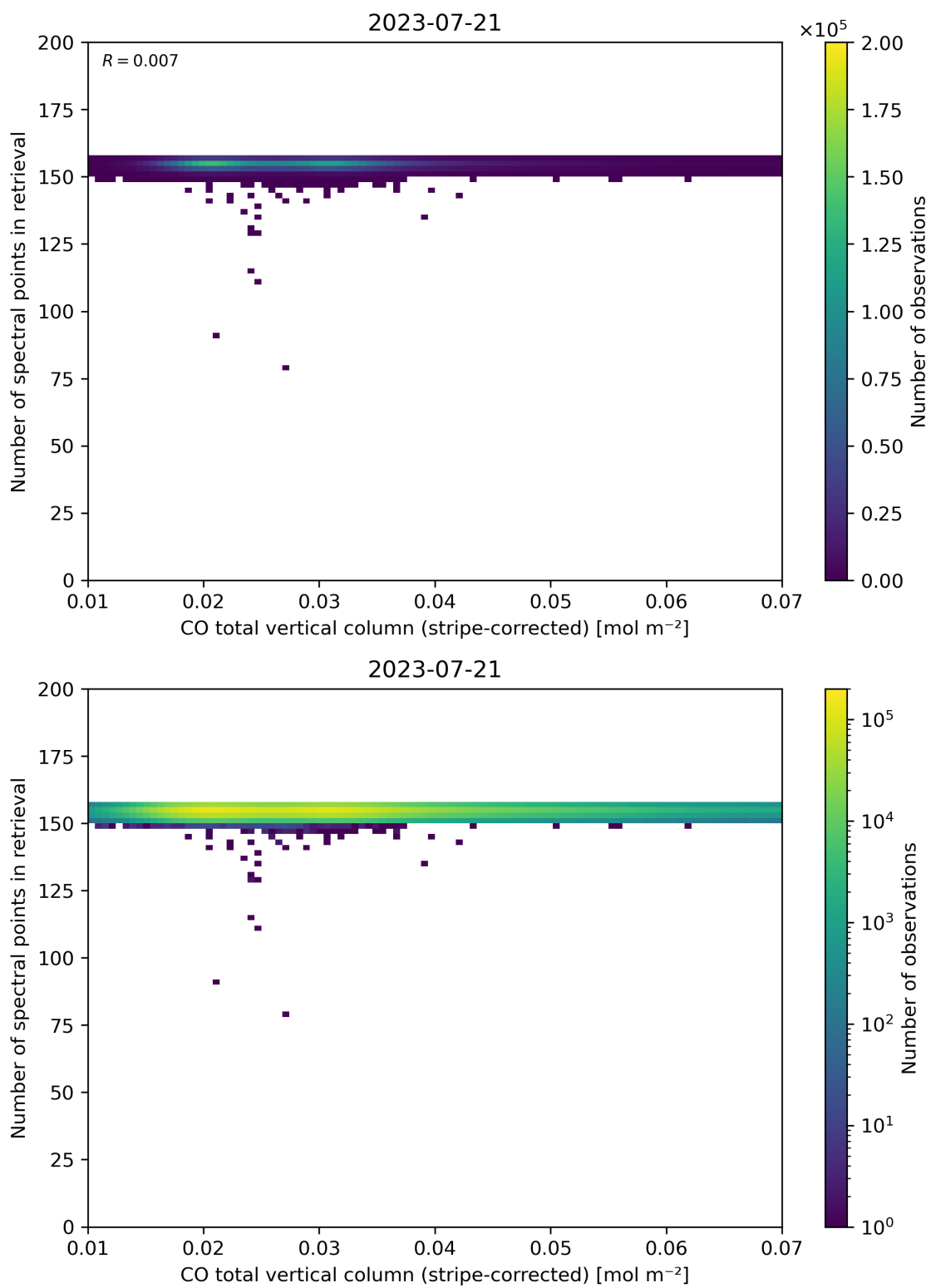
Figure 40: Scatter density plot of “CO total vertical column (stripe-corrected)” against “Number of spectral points in retrieval” for 2023-07-20 to 2023-07-22.
