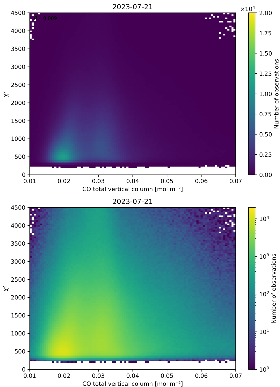
Figure 35: Scatter density plot of “CO total vertical column” against “ \chi^2 ” for 2023-07-20 to 2023-07-22.
