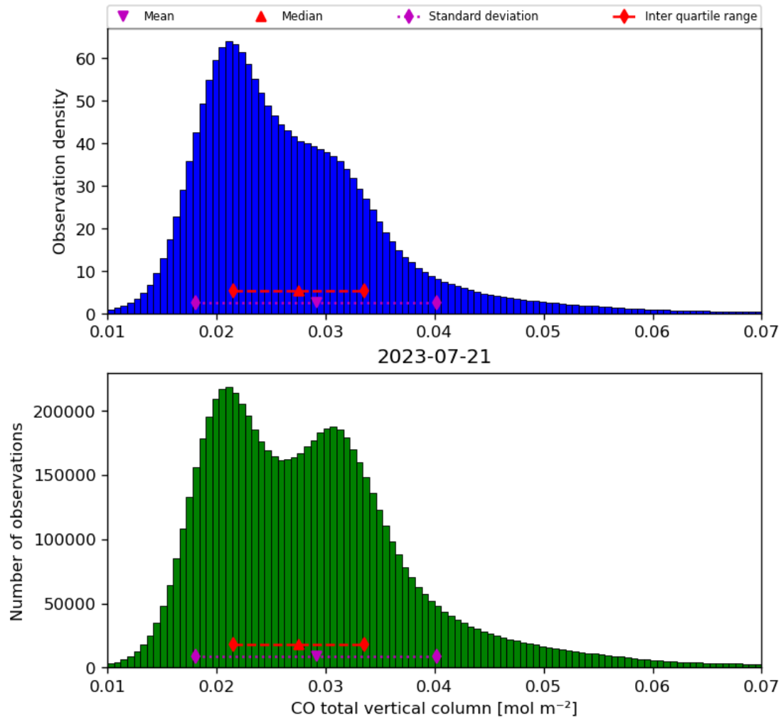
Figure 18: Histogram of “CO total vertical column” for 2023-07-20 to 2023-07-22
