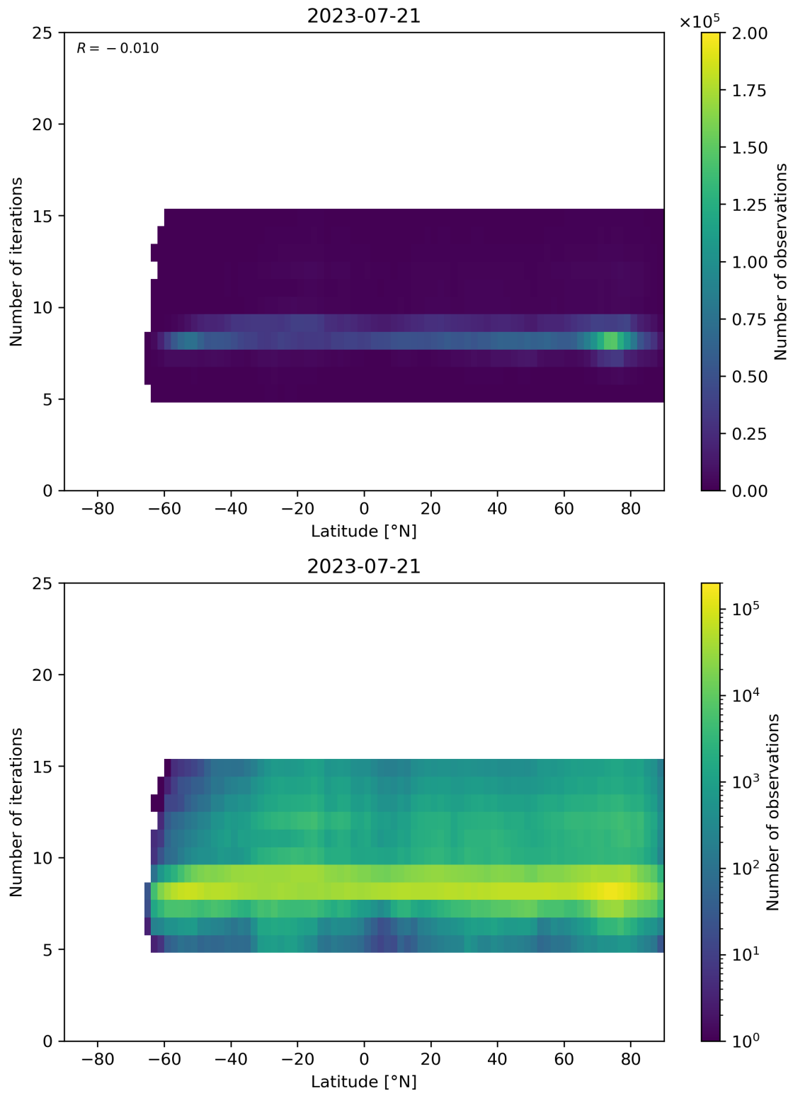
Figure 56: Scatter density plot of “Latitude” against “Number of iterations” for 2023-07-20 to 2023-07-22.
