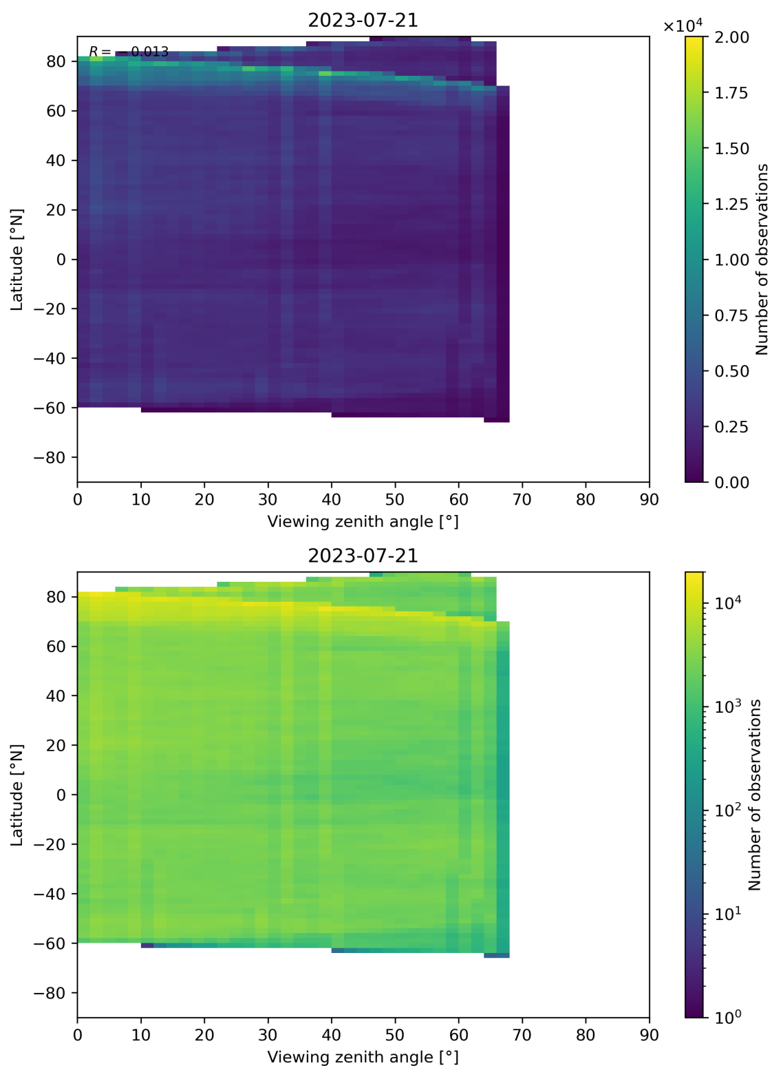
Figure 74: Scatter density plot of “Viewing zenith angle” against “Latitude” for 2023-07-20 to 2023-07-22.
