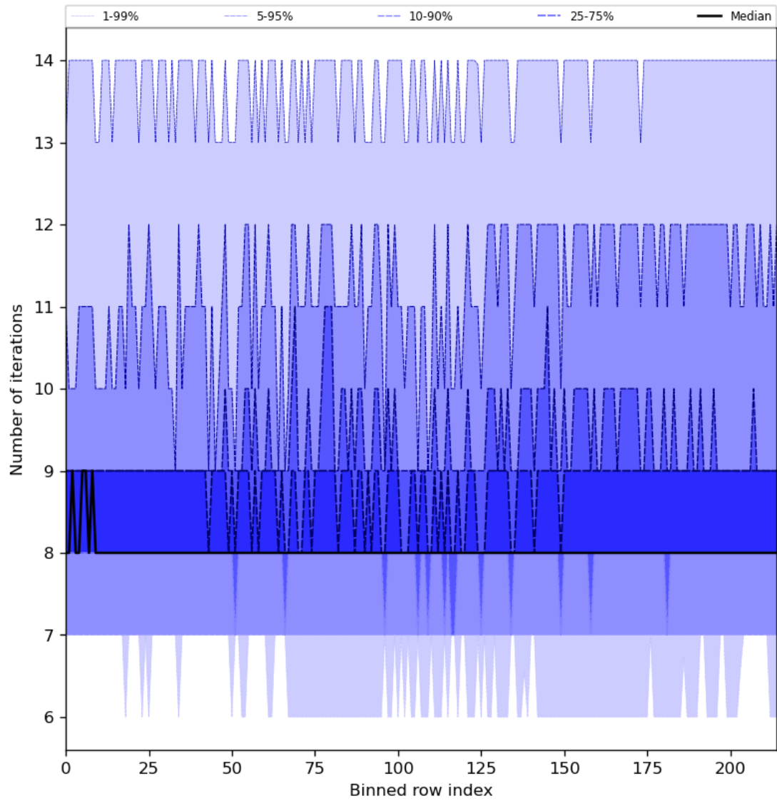
Figure 32: Along track statistics of “Number of iterations” for 2023-07-20 to 2023-07-22
