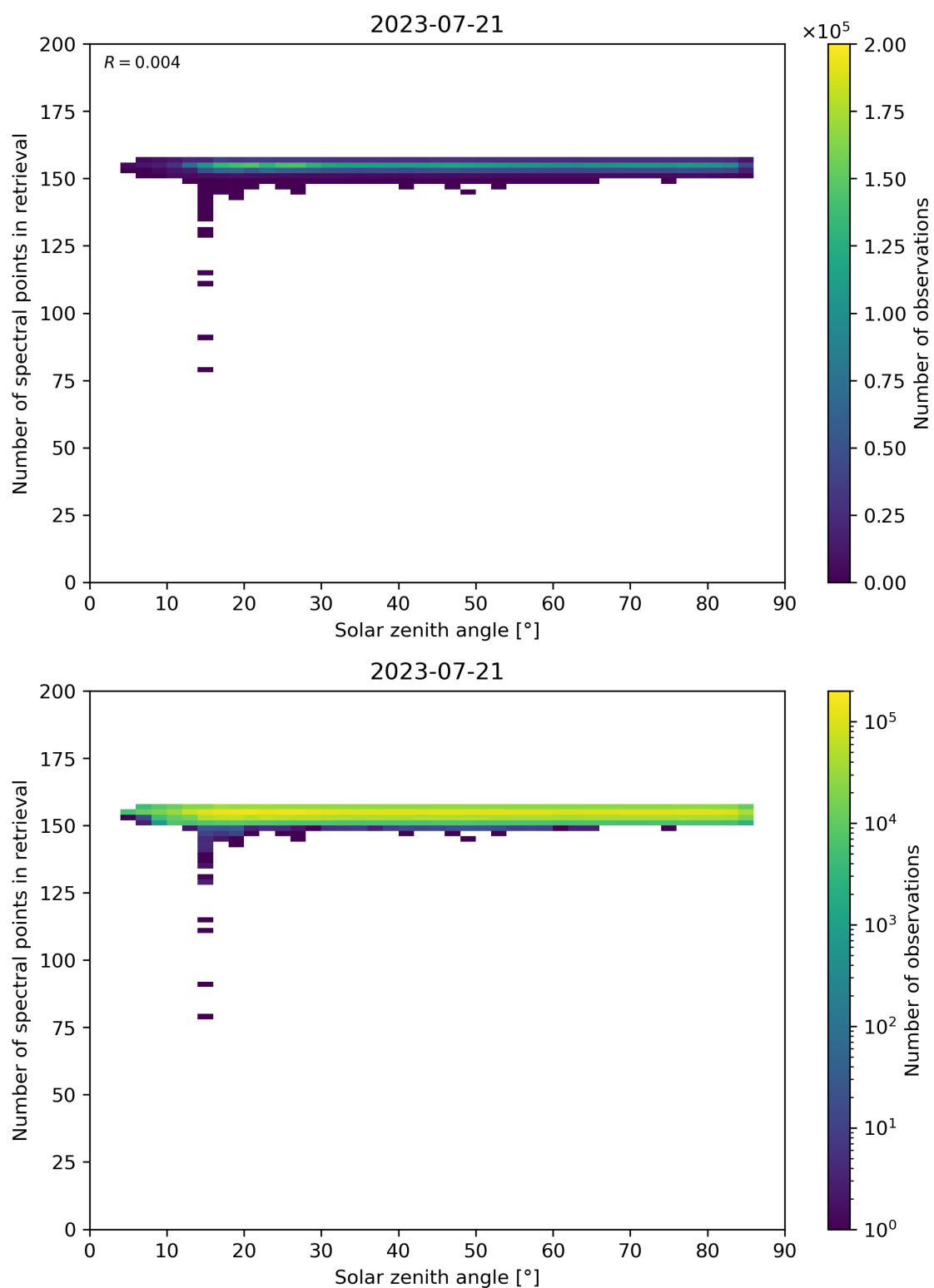
Figure 68: Scatter density plot of “Solar zenith angle” against “Number of spectral points in retrieval” for 2023-07-20 to 2023-07-22.
