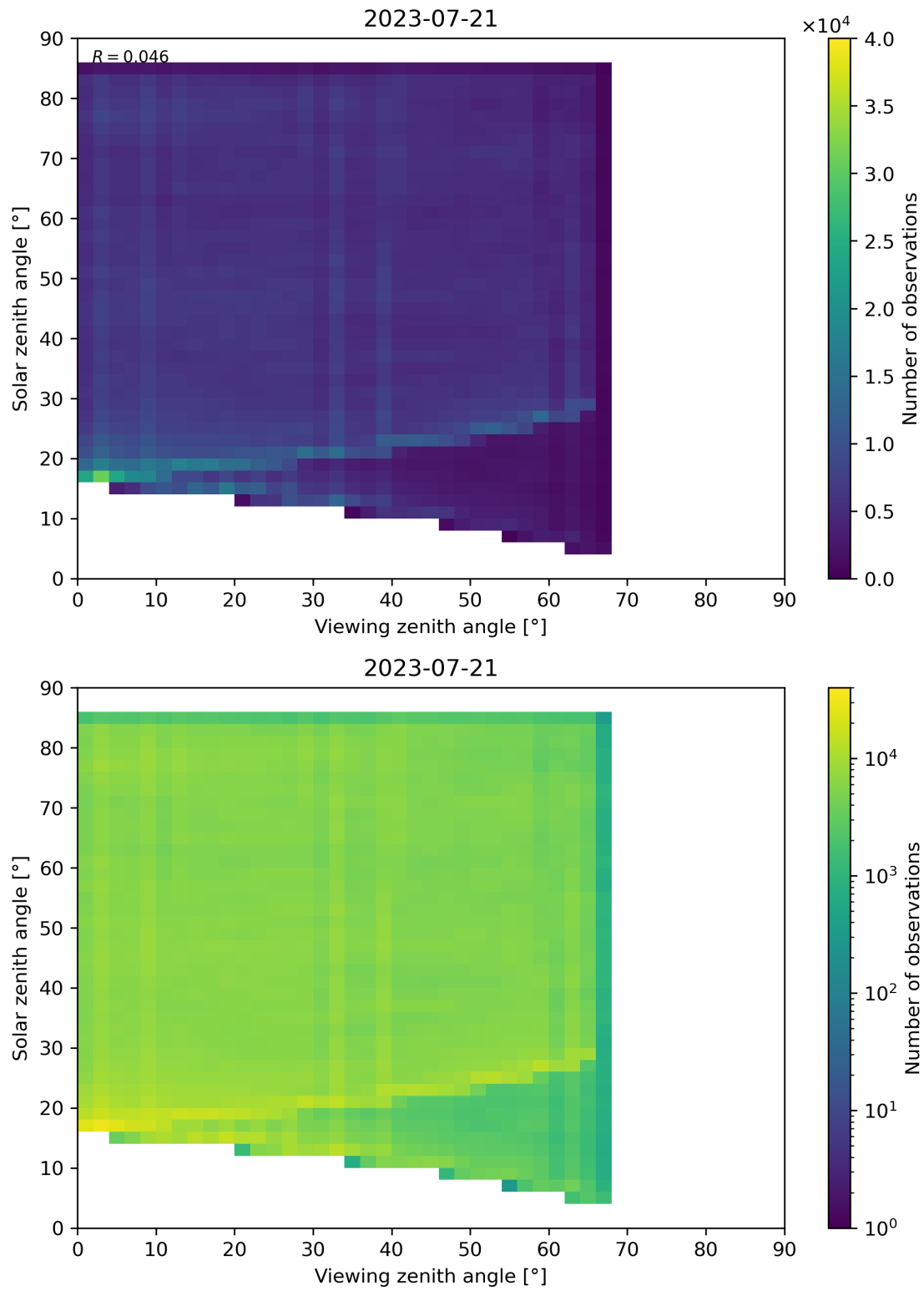
Figure 77: Scatter density plot of “Viewing zenith angle” against “Solar zenith angle” for 2023-07-20 to 2023-07-22.
