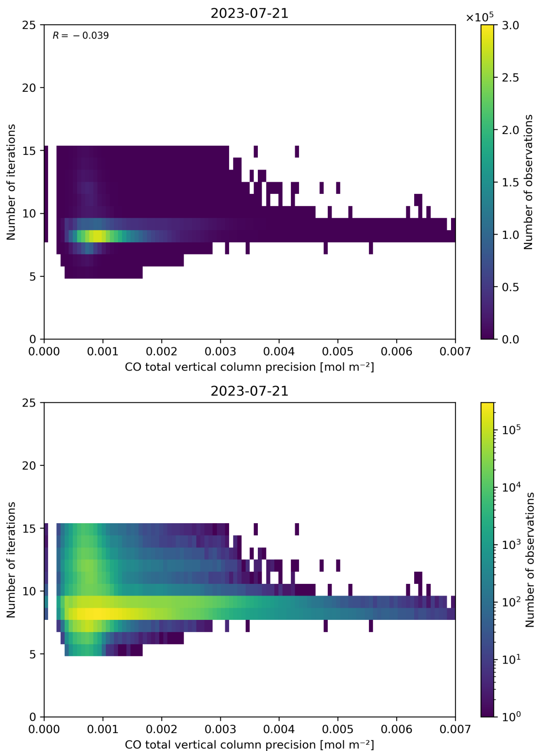
Figure 46: Scatter density plot of “CO total vertical column precision” against “Number of iterations” for 2023-07-20 to 2023-07-22.
