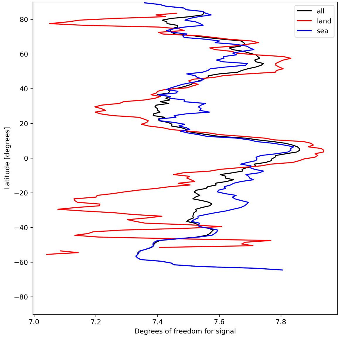
Figure 15: Zonal average of “Degrees of freedom for signal” for 2023-07-20 to 2023-07-22.
