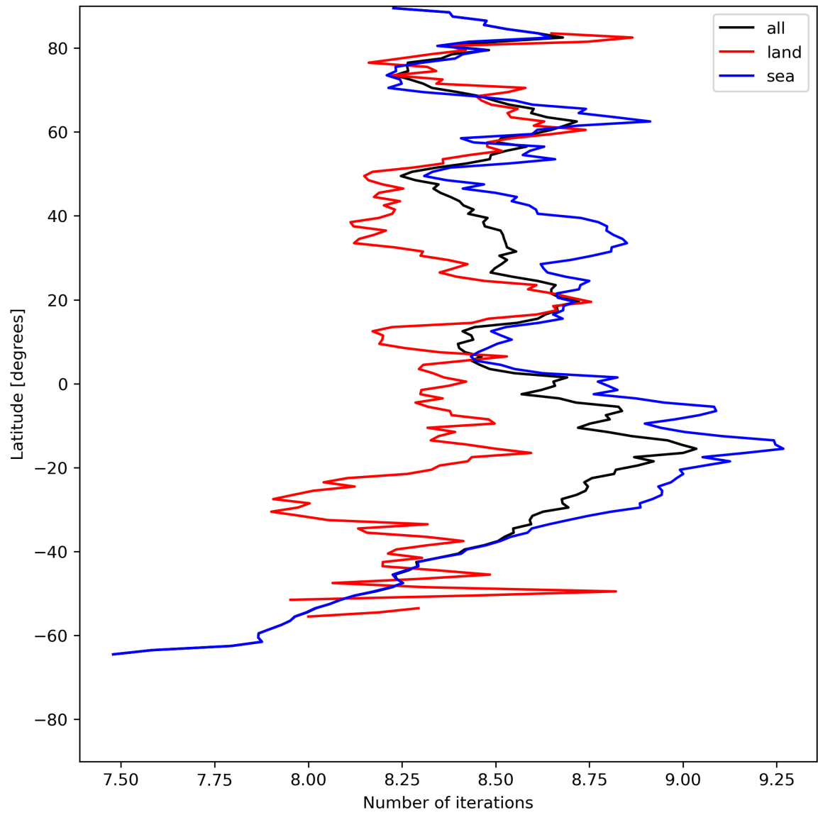
Figure 16: Zonal average of “Number of iterations” for 2023-07-20 to 2023-07-22.
