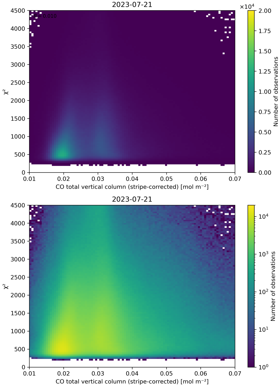
Figure 37: Scatter density plot of “CO total vertical column (stripe-corrected)” against “ \chi^2 ” for 2023-07-20 to 2023-07-22.
