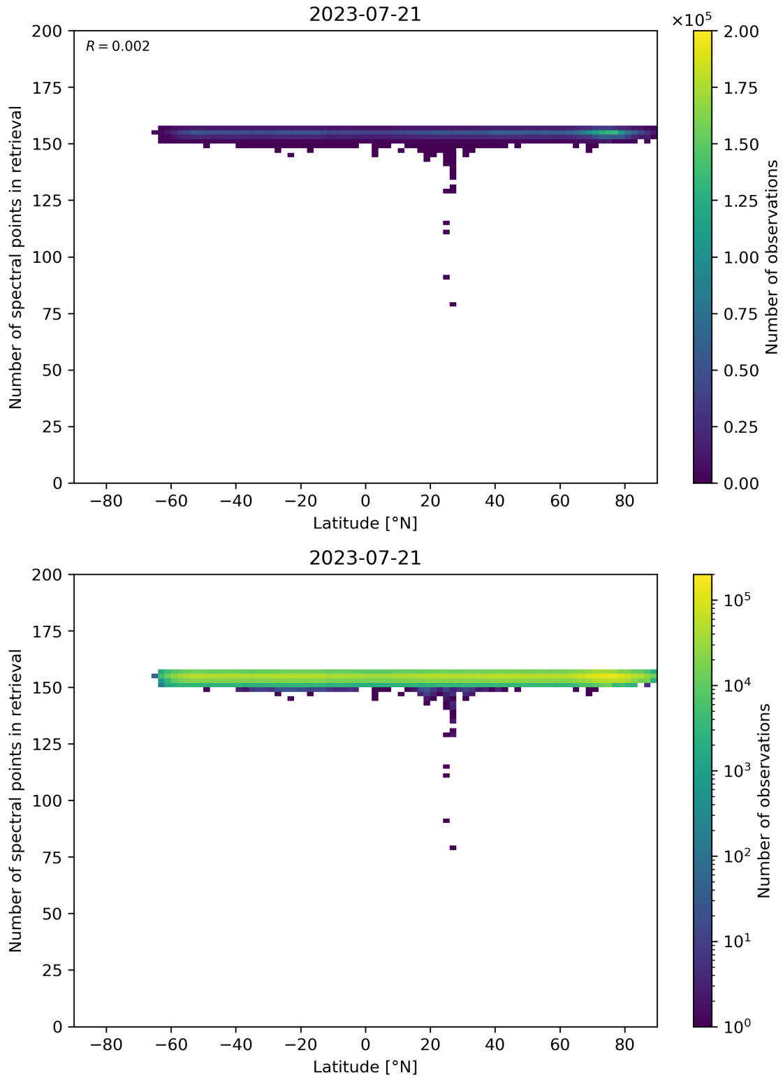
Figure 57: Scatter density plot of “Latitude” against “Number of spectral points in retrieval” for 2023-07-20 to 2023-07-22.
