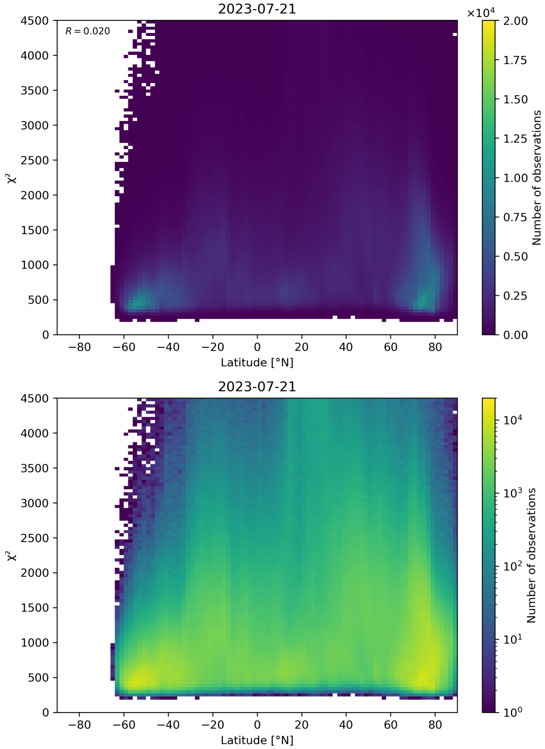
Figure 54: Scatter density plot of “Latitude” against “ \chi^2 ” for 2023-07-20 to 2023-07-22.
