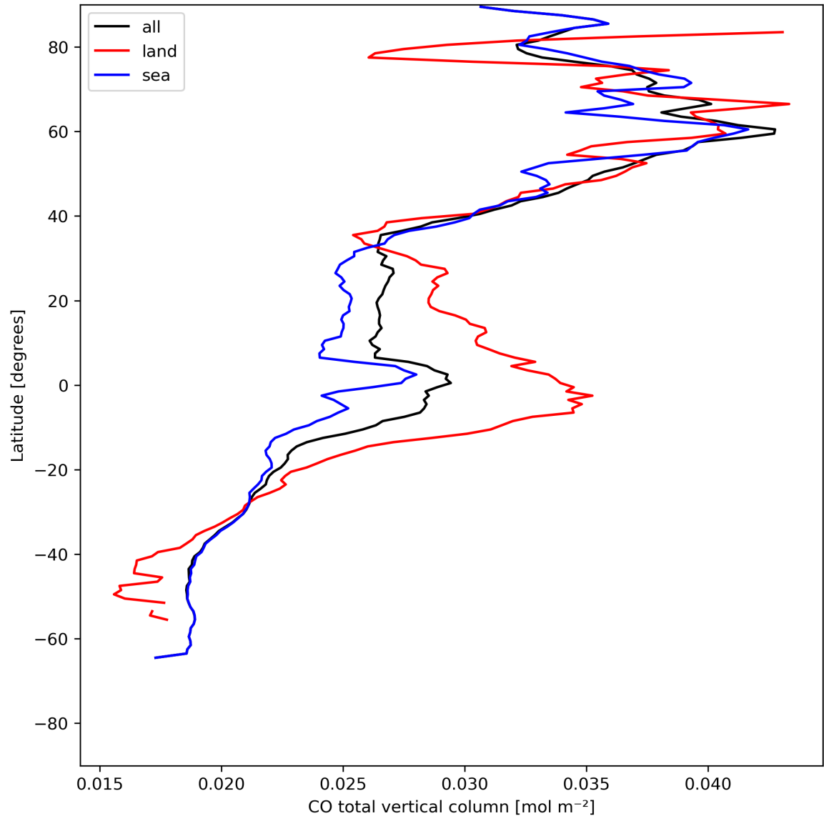
Figure 10: Zonal average of “CO total vertical column” for 2023-07-20 to 2023-07-22.
