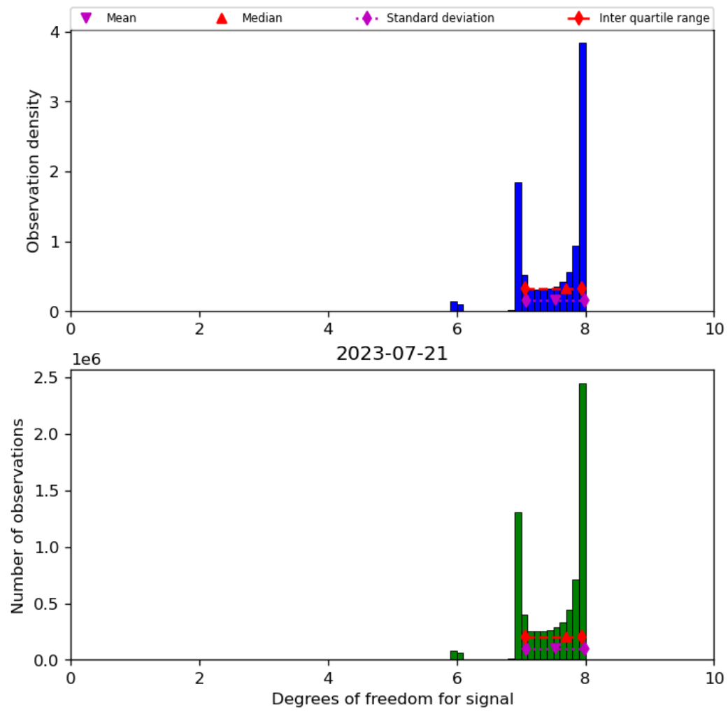
Figure 23: Histogram of “Degrees of freedom for signal” for 2023-07-20 to 2023-07-22
