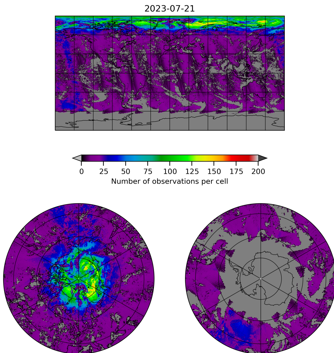
Figure 8: Map of the number of observations for 2023-07-20 to 2023-07-22
