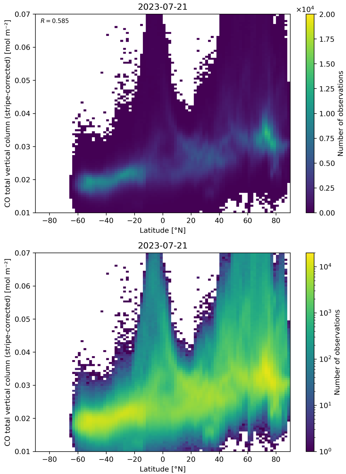
Figure 52: Scatter density plot of “Latitude” against “CO total vertical column (stripe-corrected)” for 2023-07-20 to 2023-07-22.
