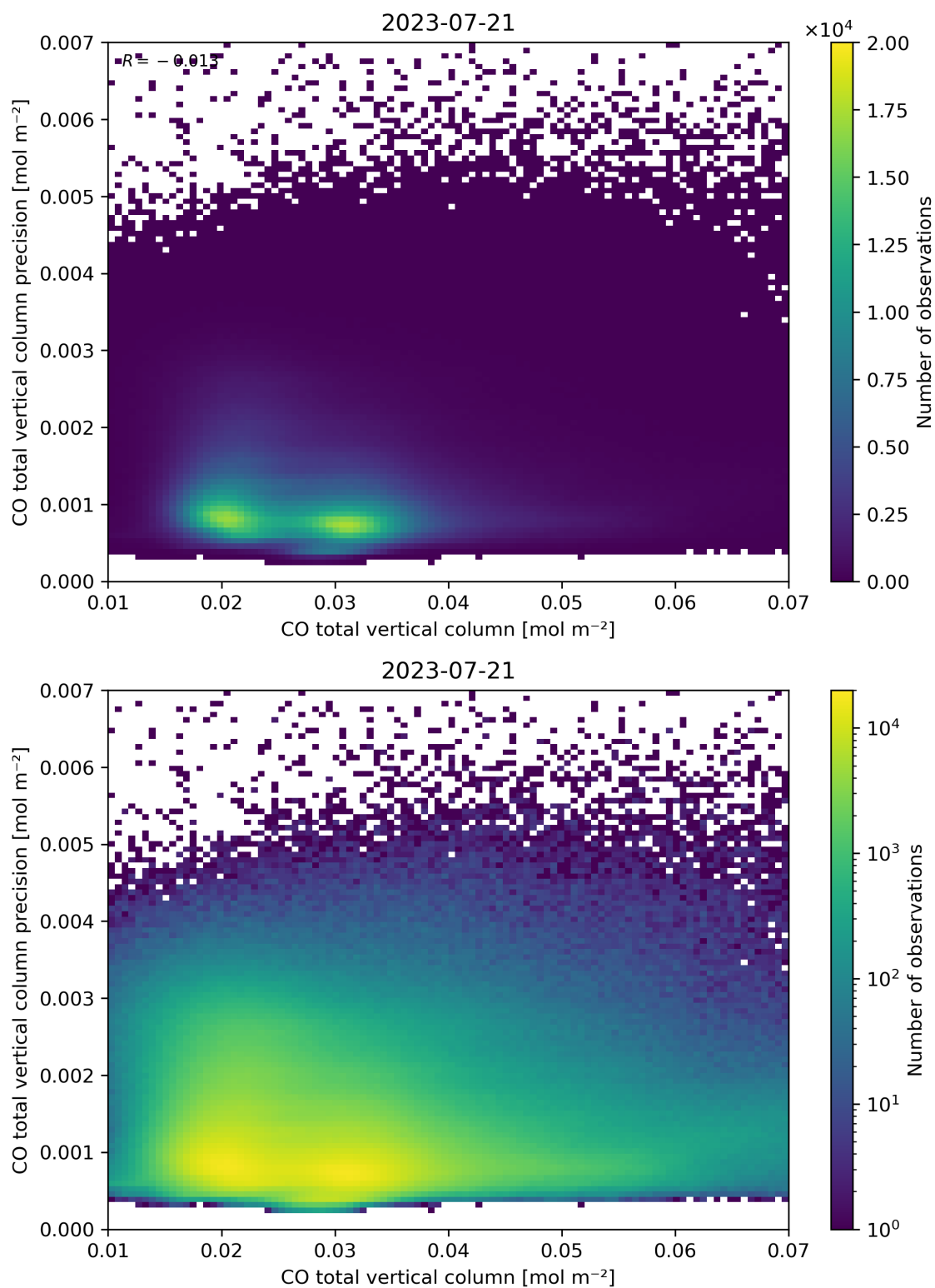
Figure 34: Scatter density plot of “CO total vertical column” against “CO total vertical column precision” for 2023-07-20 to 2023-07-22.
