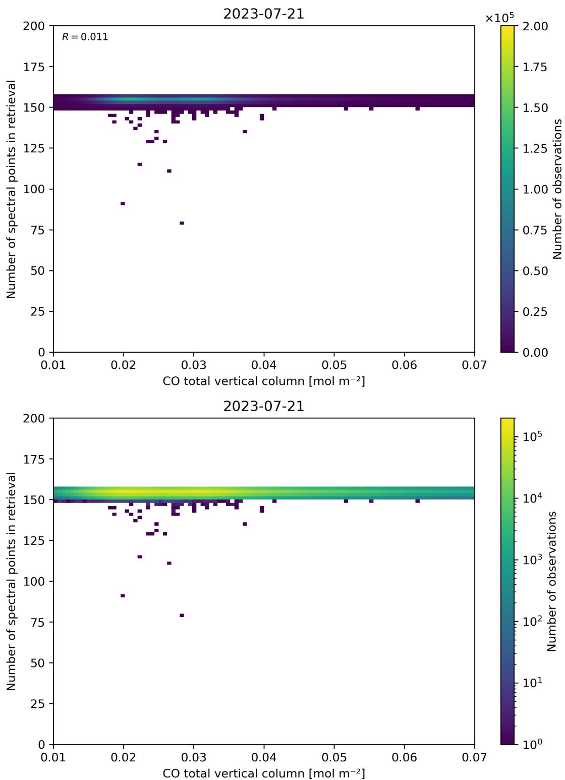
Figure 43: Scatter density plot of “CO total vertical column” against “Number of spectral points in retrieval” for 2023-07-20 to 2023-07-22.
