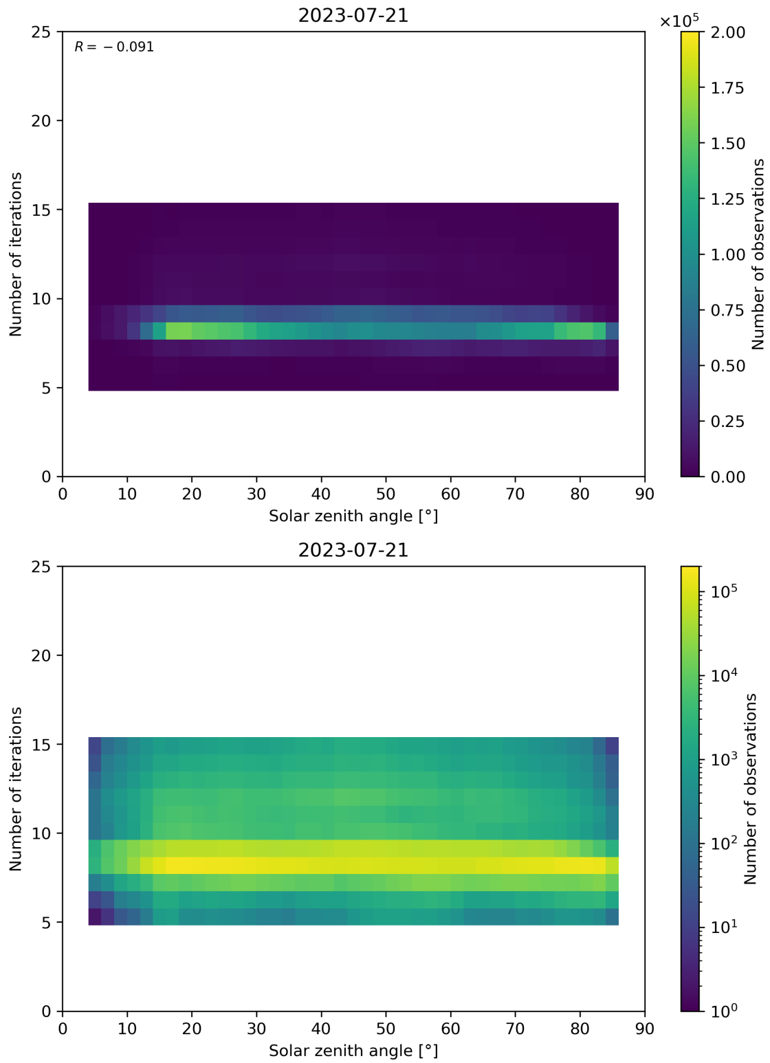
Figure 67: Scatter density plot of “Solar zenith angle” against “Number of iterations” for 2023-07-20 to 2023-07-22.
