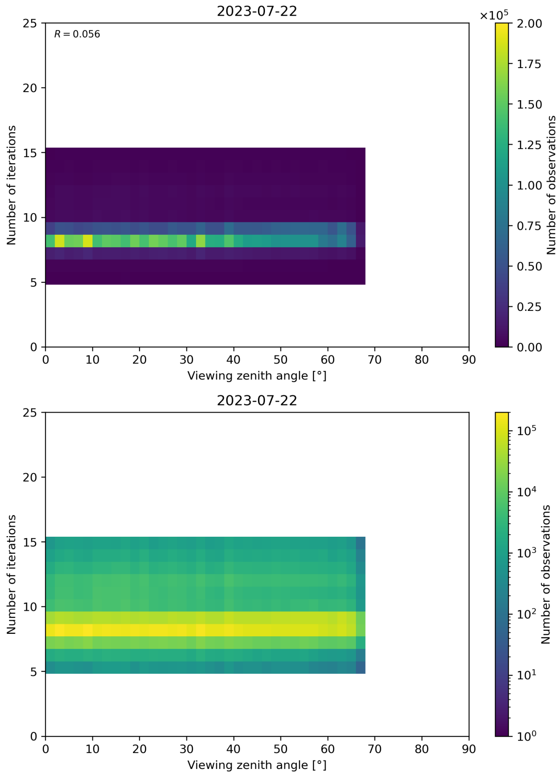
Figure 75: Scatter density plot of “Viewing zenith angle” against “Number of iterations” for 2023-07-21 to 2023-07-23.
