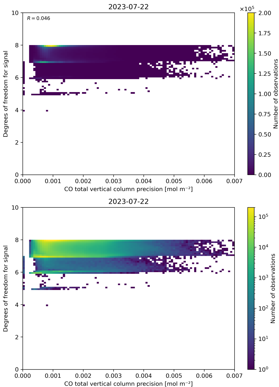
Figure 45: Scatter density plot of “CO total vertical column precision” against “Degrees of freedom for signal” for 2023-07-21 to 2023-07-23.
