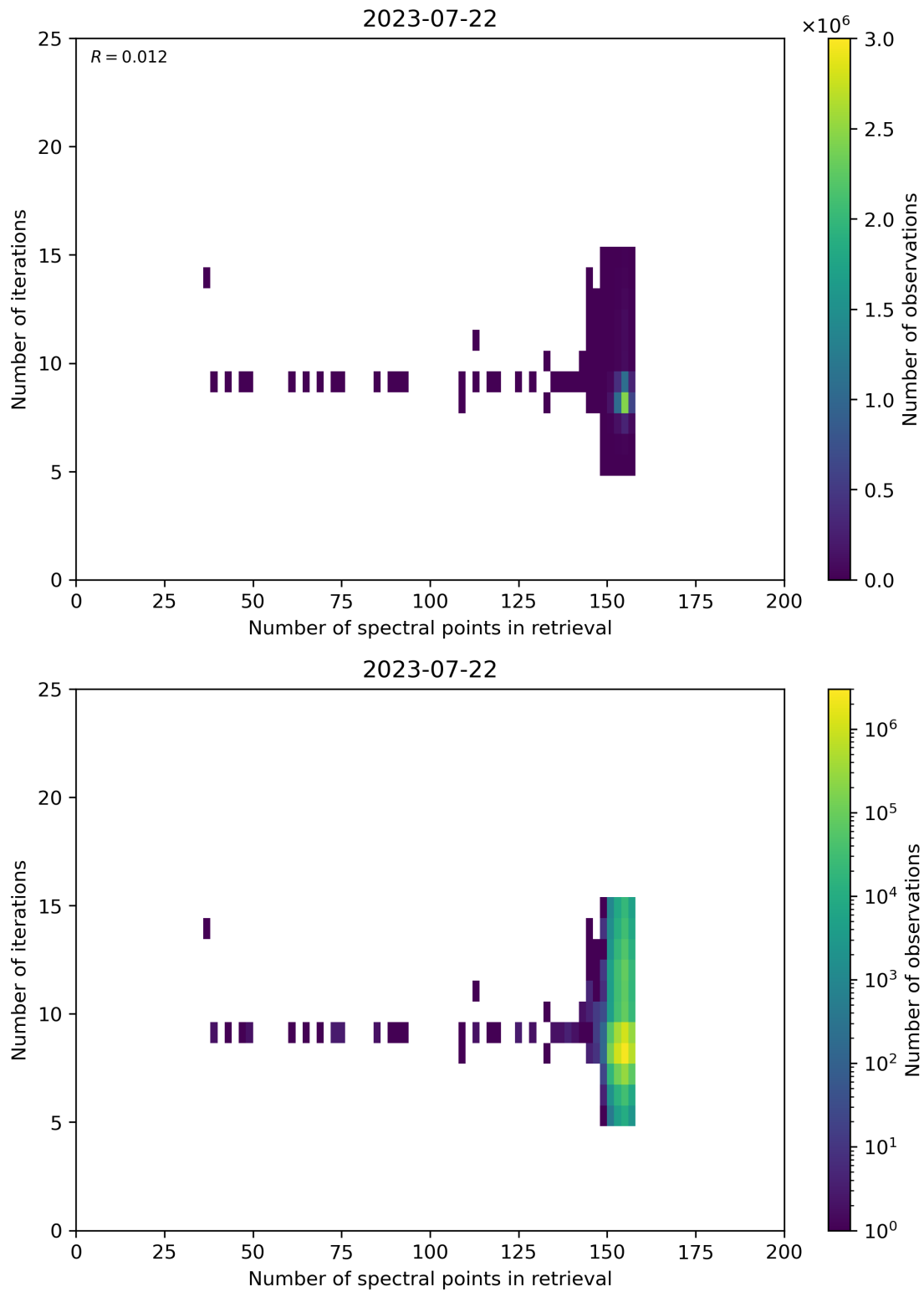
Figure 60: Scatter density plot of “Number of spectral points in retrieval” against “Number of iterations” for 2023-07-21 to 2023-07-23.
