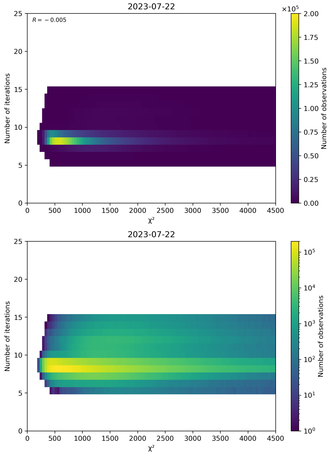
Figure 49: Scatter density plot of “ \chi^2 ” against “Number of iterations” for 2023-07-21 to 2023-07-23.
