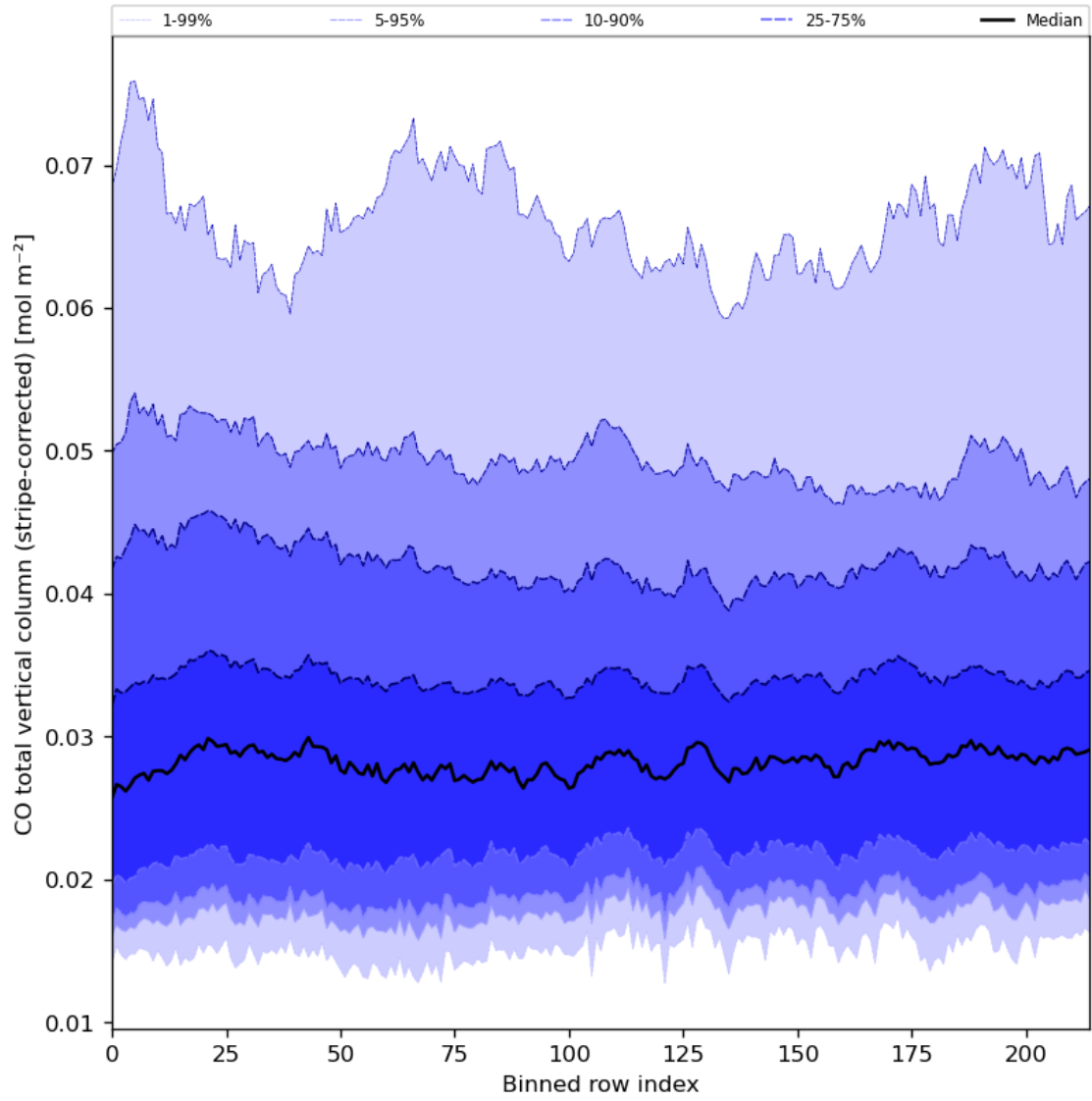
Figure 27: Along track statistics of “CO total vertical column (stripe-corrected)” for 2023-07-21 to 2023-07-23
