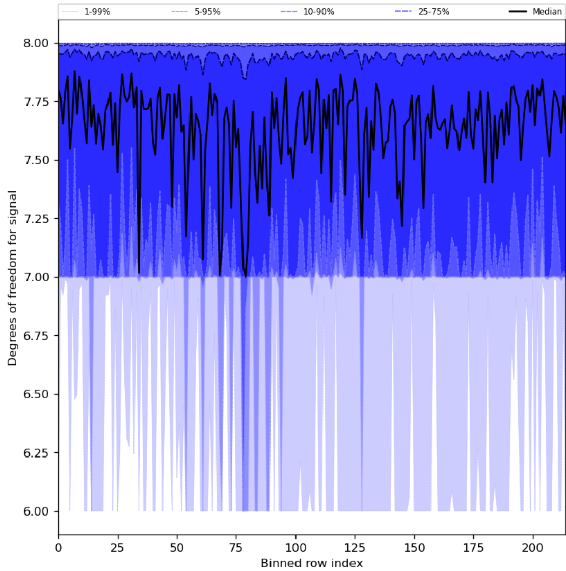
Figure 31: Along track statistics of “Degrees of freedom for signal” for 2023-07-21 to 2023-07-23
