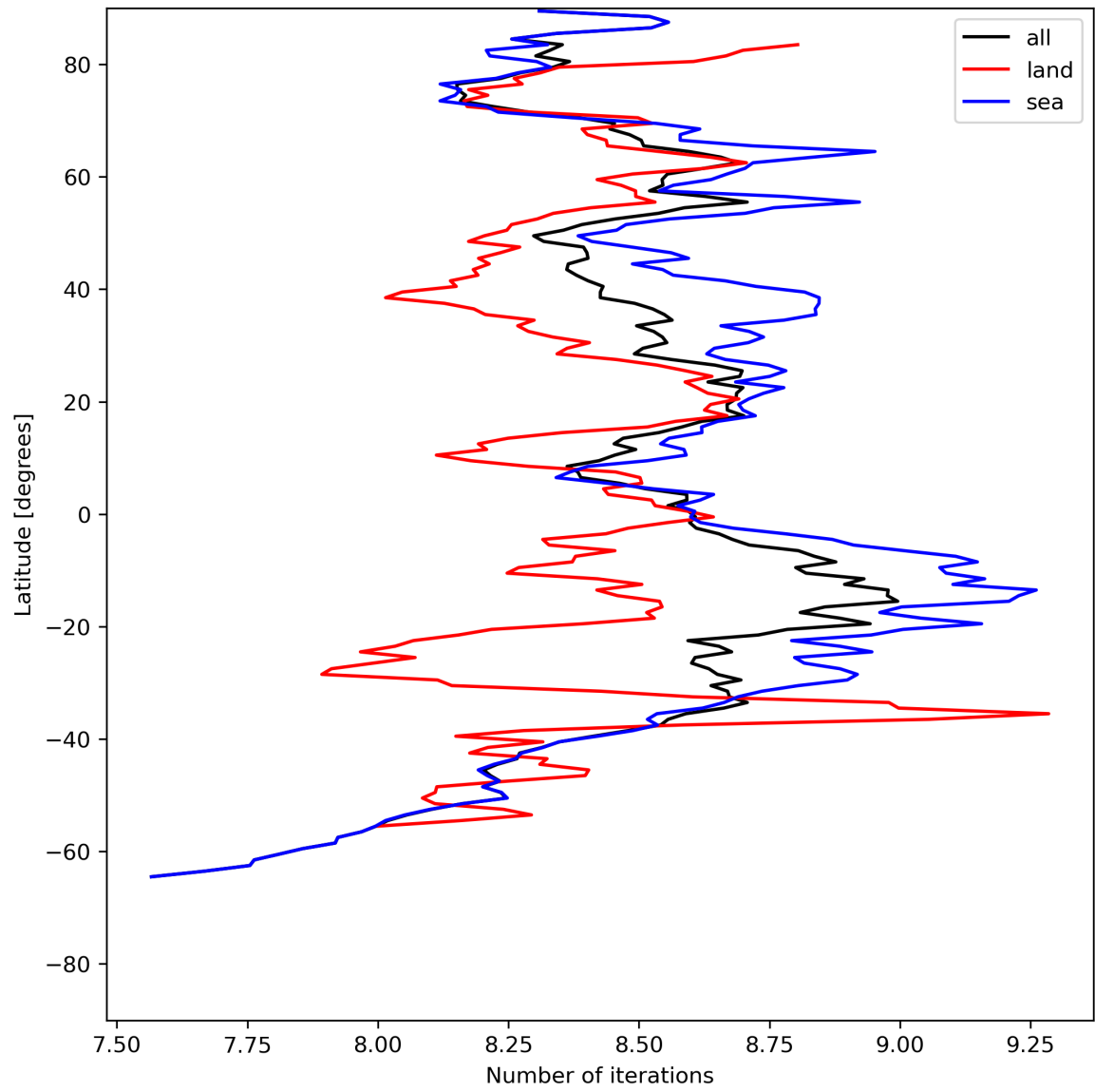
Figure 16: Zonal average of “Number of iterations” for 2023-07-21 to 2023-07-23.
