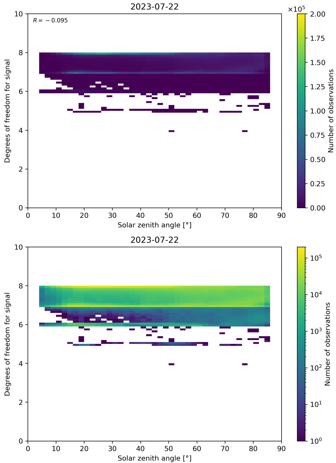
Figure 65: Scatter density plot of “Solar zenith angle” against “Degrees of freedom for signal” for 2023-07-21 to 2023-07-23.
