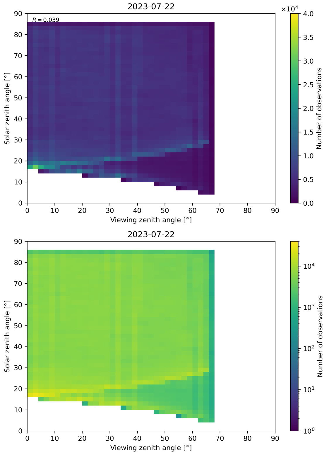
Figure 77: Scatter density plot of “Viewing zenith angle” against “Solar zenith angle” for 2023-07-21 to 2023-07-23.
