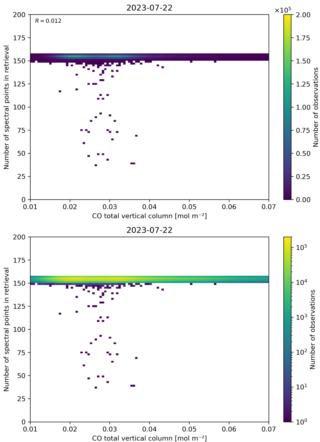
Figure 43: Scatter density plot of “CO total vertical column” against “Number of spectral points in retrieval” for 2023-07-21 to 2023-07-23.
