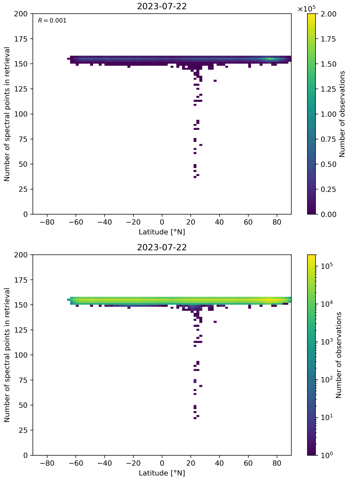
Figure 57: Scatter density plot of “Latitude” against “Number of spectral points in retrieval” for 2023-07-21 to 2023-07-23.
