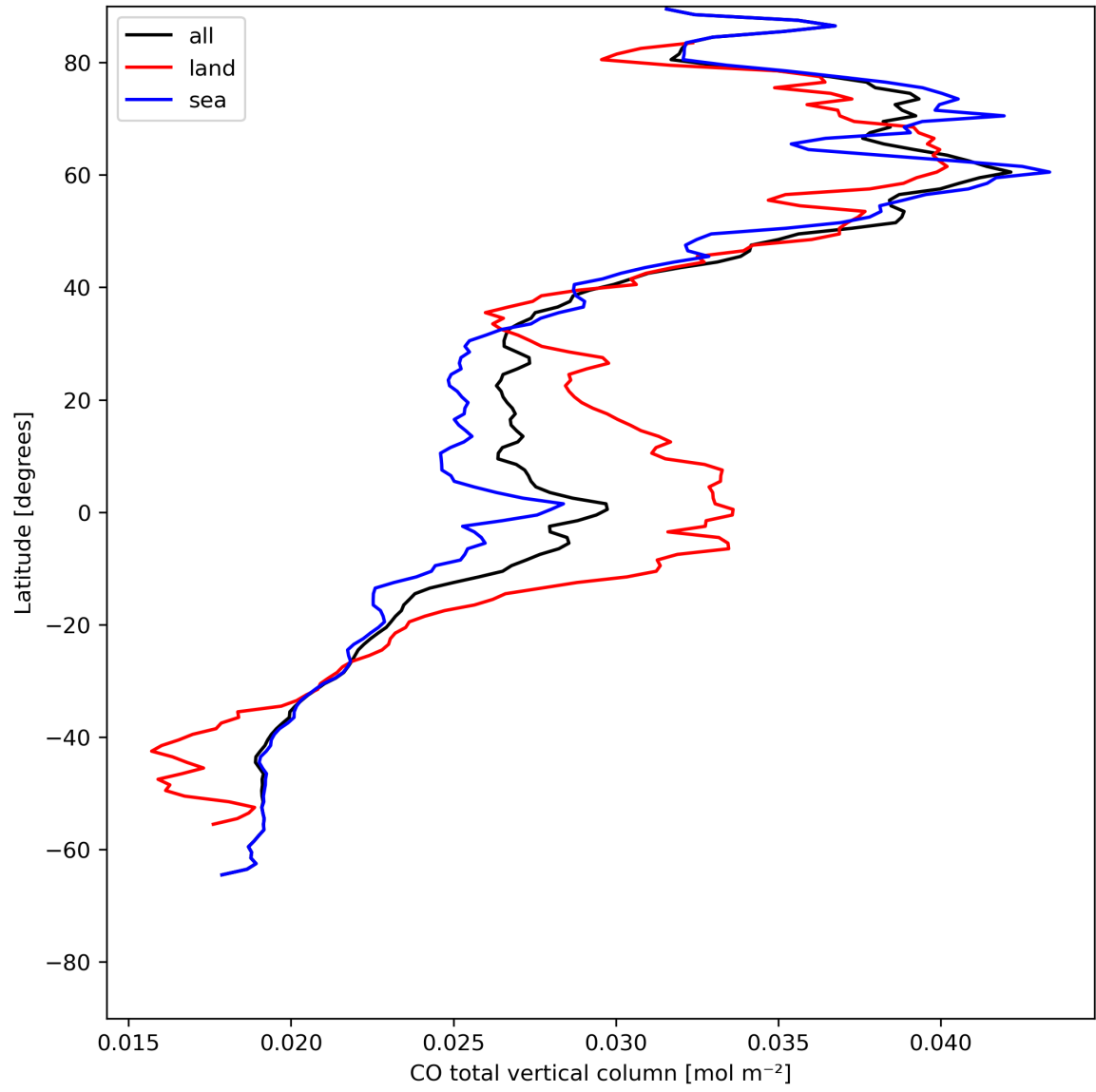
Figure 10: Zonal average of “CO total vertical column” for 2023-07-21 to 2023-07-23.
