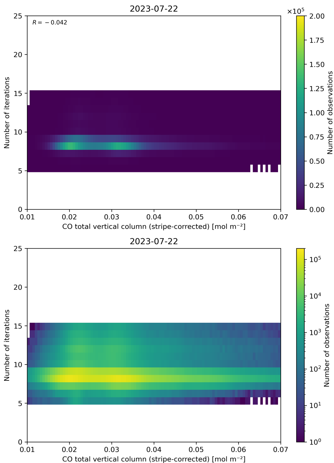
Figure 39: Scatter density plot of “CO total vertical column (stripe-corrected)” against “Number of iterations” for 2023-07-21 to 2023-07-23.
