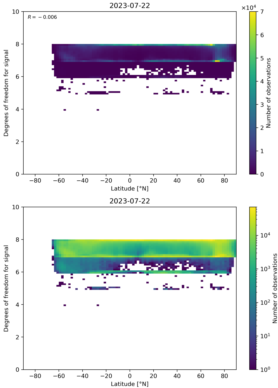
Figure 55: Scatter density plot of “Latitude” against “Degrees of freedom for signal” for 2023-07-21 to 2023-07-23.
