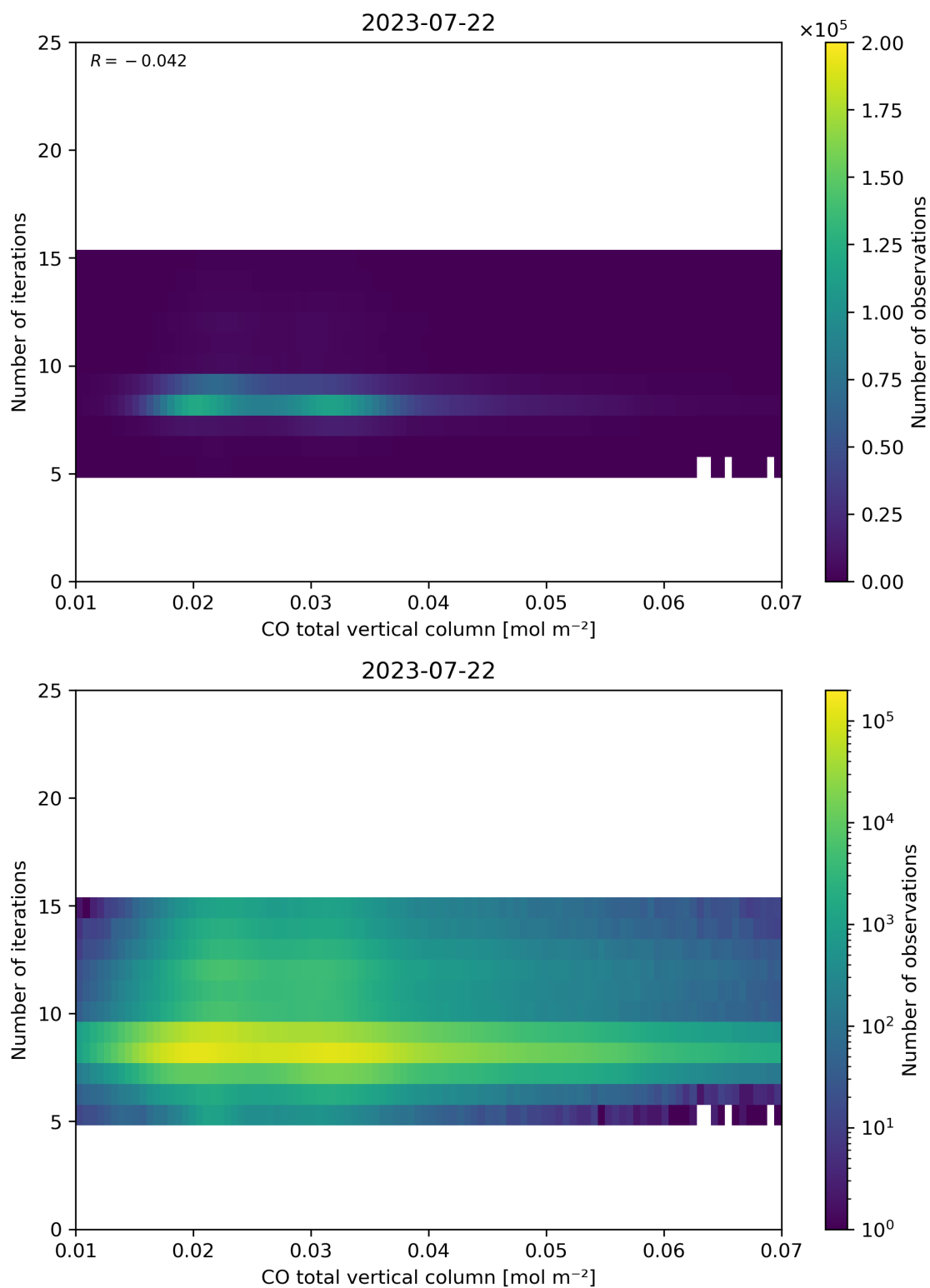
Figure 42: Scatter density plot of “CO total vertical column” against “Number of iterations” for 2023-07-21 to 2023-07-23.
