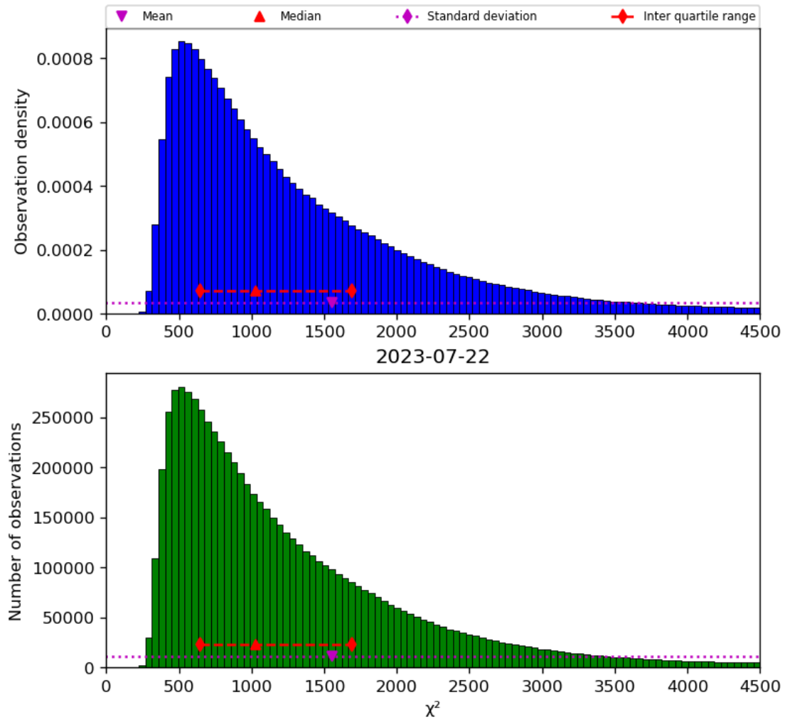
Figure 22: Histogram of “ \chi^2 ” for 2023-07-21 to 2023-07-23
