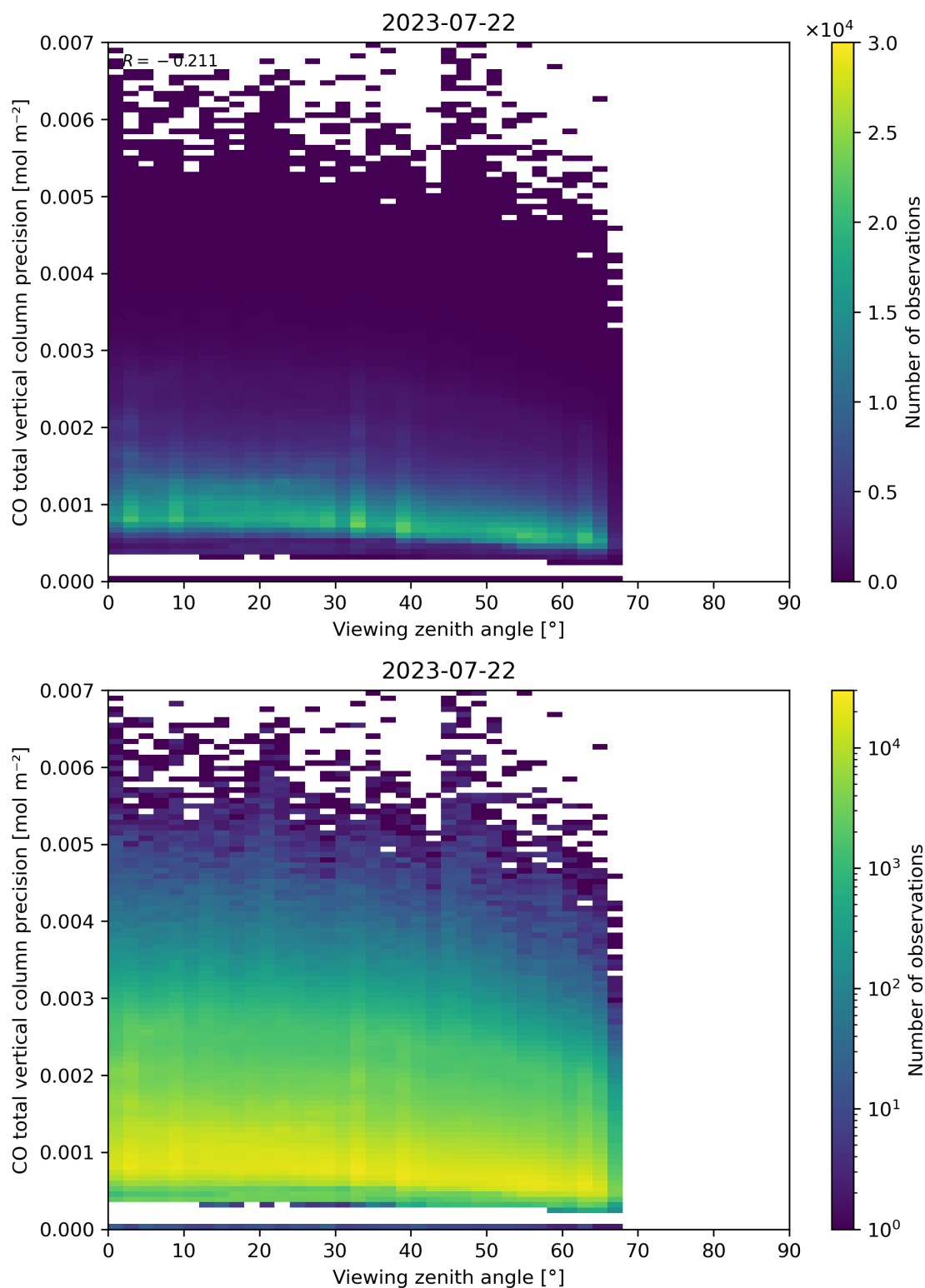
Figure 71: Scatter density plot of “Viewing zenith angle” against “CO total vertical column precision” for 2023-07-21 to 2023-07-23.
