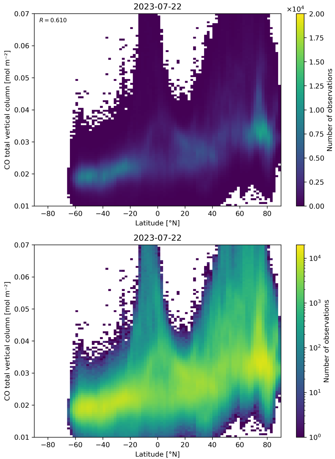
Figure 51: Scatter density plot of “Latitude” against “CO total vertical column” for 2023-07-21 to 2023-07-23.
