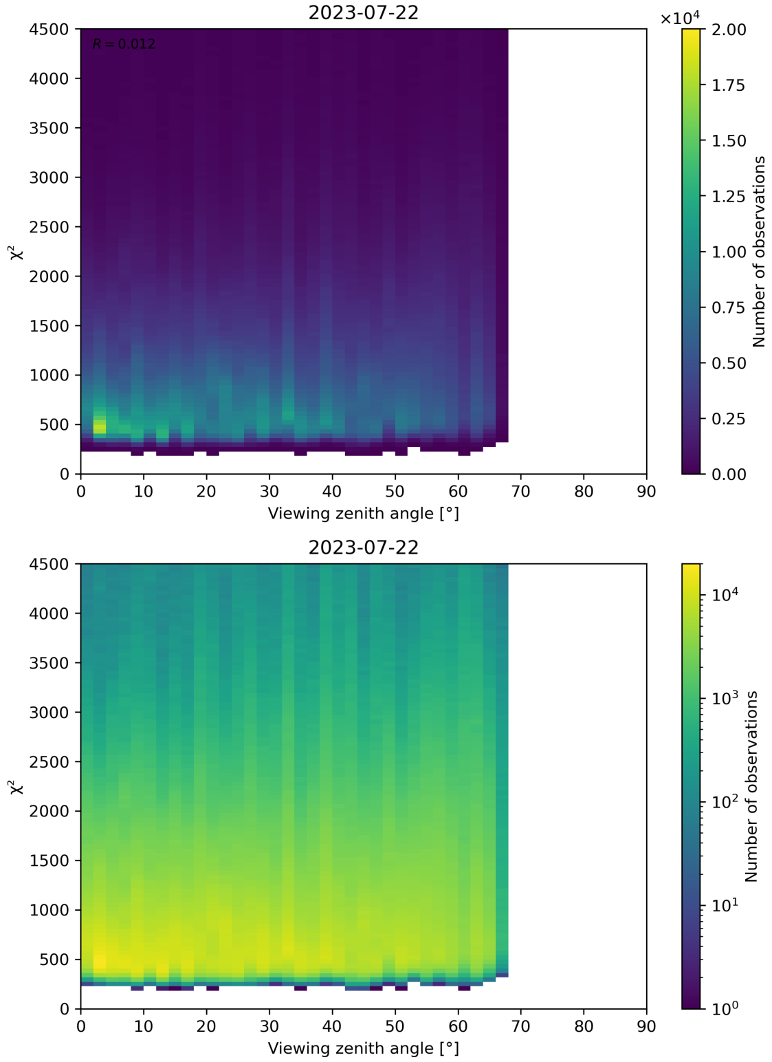
Figure 72: Scatter density plot of “Viewing zenith angle” against “ \chi^2 ” for 2023-07-21 to 2023-07-23.
