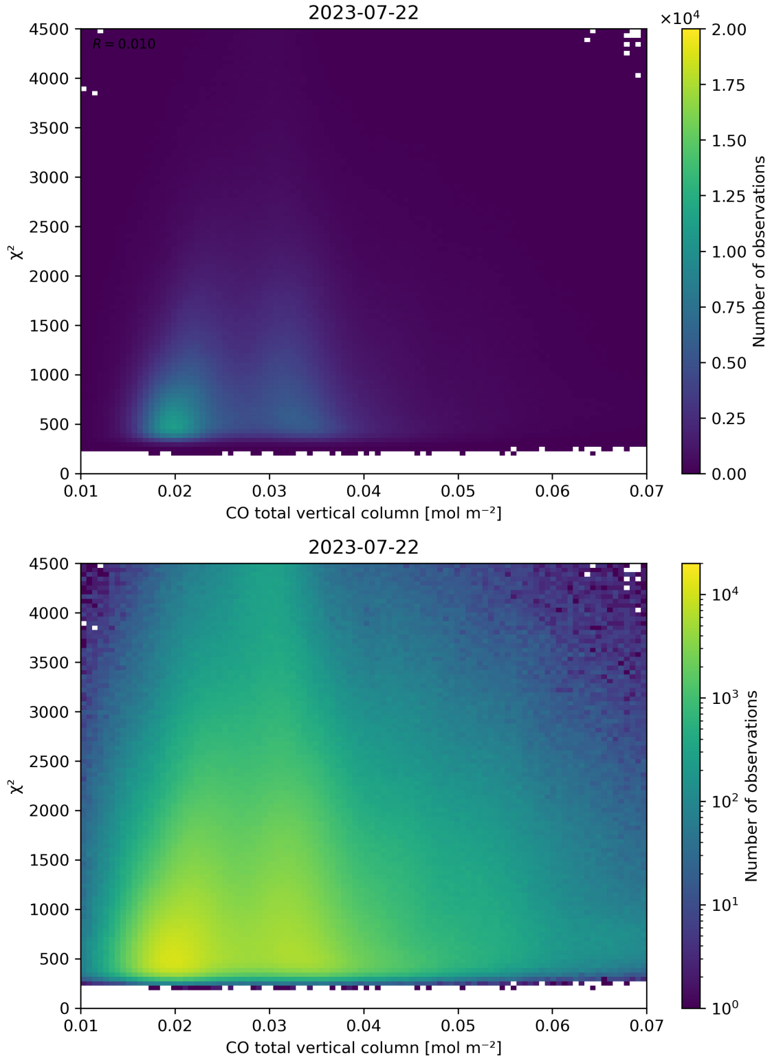
Figure 35: Scatter density plot of “CO total vertical column” against “ \chi^2 ” for 2023-07-21 to 2023-07-23.
