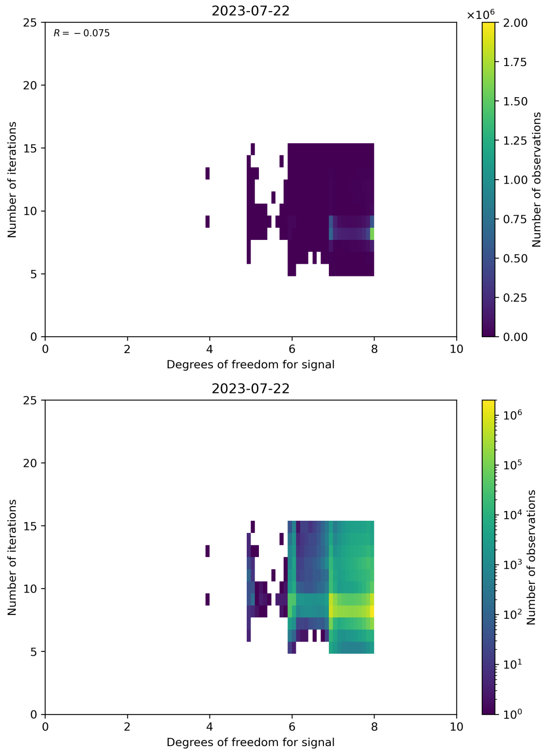
Figure 50: Scatter density plot of “Degrees of freedom for signal” against “Number of iterations” for 2023-07-21 to 2023-07-23.
