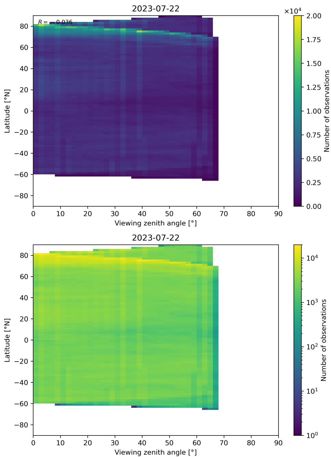
Figure 74: Scatter density plot of “Viewing zenith angle” against “Latitude” for 2023-07-21 to 2023-07-23.
