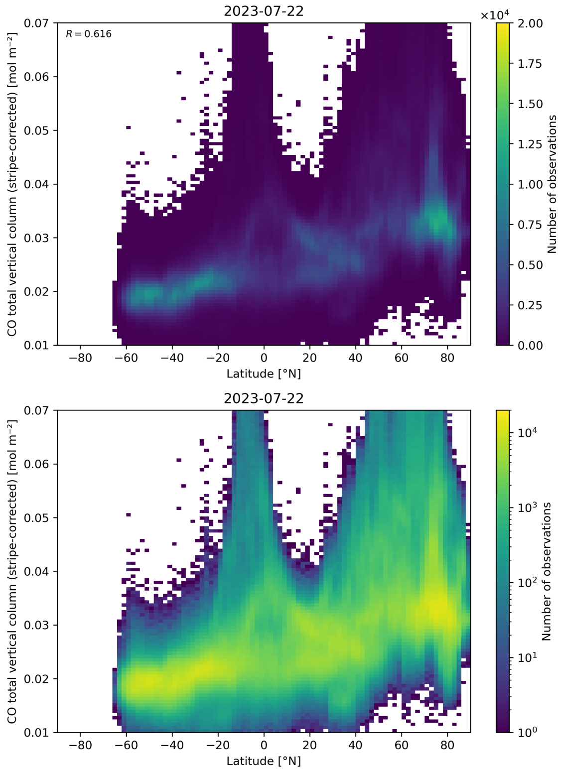
Figure 52: Scatter density plot of “Latitude” against “CO total vertical column (stripe-corrected)” for 2023-07-21 to 2023-07-23.
