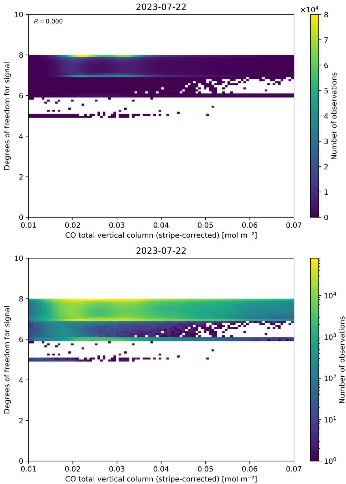
Figure 38: Scatter density plot of “CO total vertical column (stripe-corrected)” against “Degrees of freedom for signal” for 2023-07-21 to 2023-07-23.
