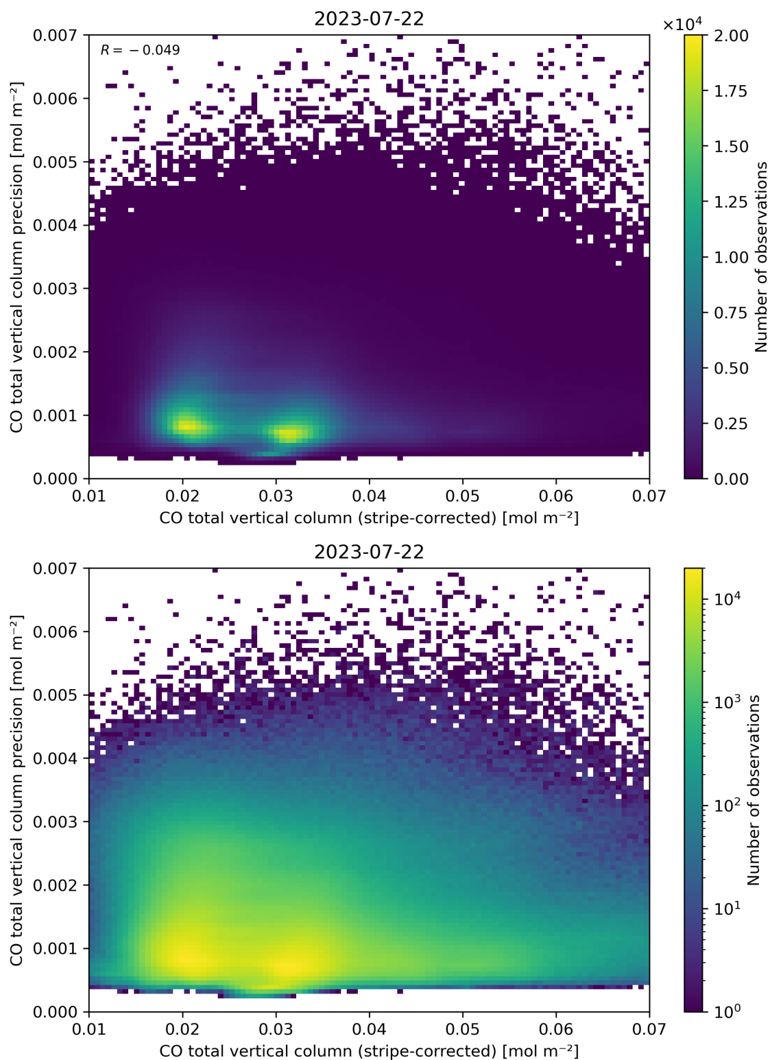
Figure 36: Scatter density plot of “CO total vertical column (stripe-corrected)” against “CO total vertical column precision” for 2023-07-21 to 2023-07-23.
