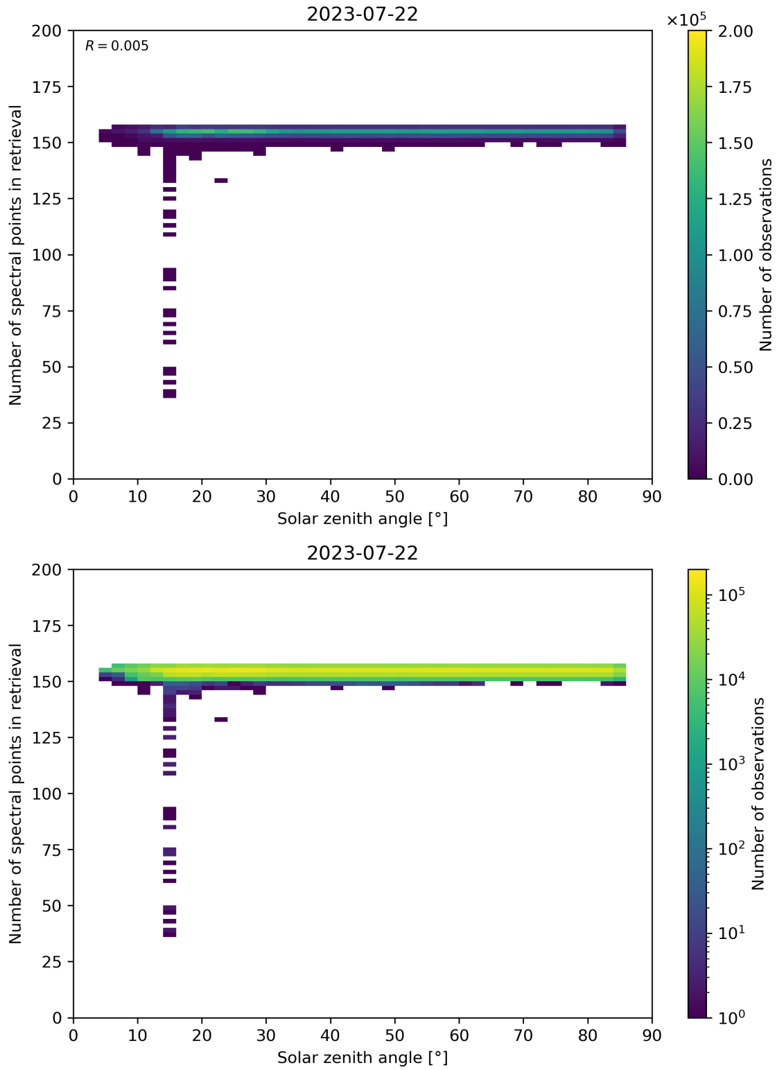
Figure 68: Scatter density plot of “Solar zenith angle” against “Number of spectral points in retrieval” for 2023-07-21 to 2023-07-23.
