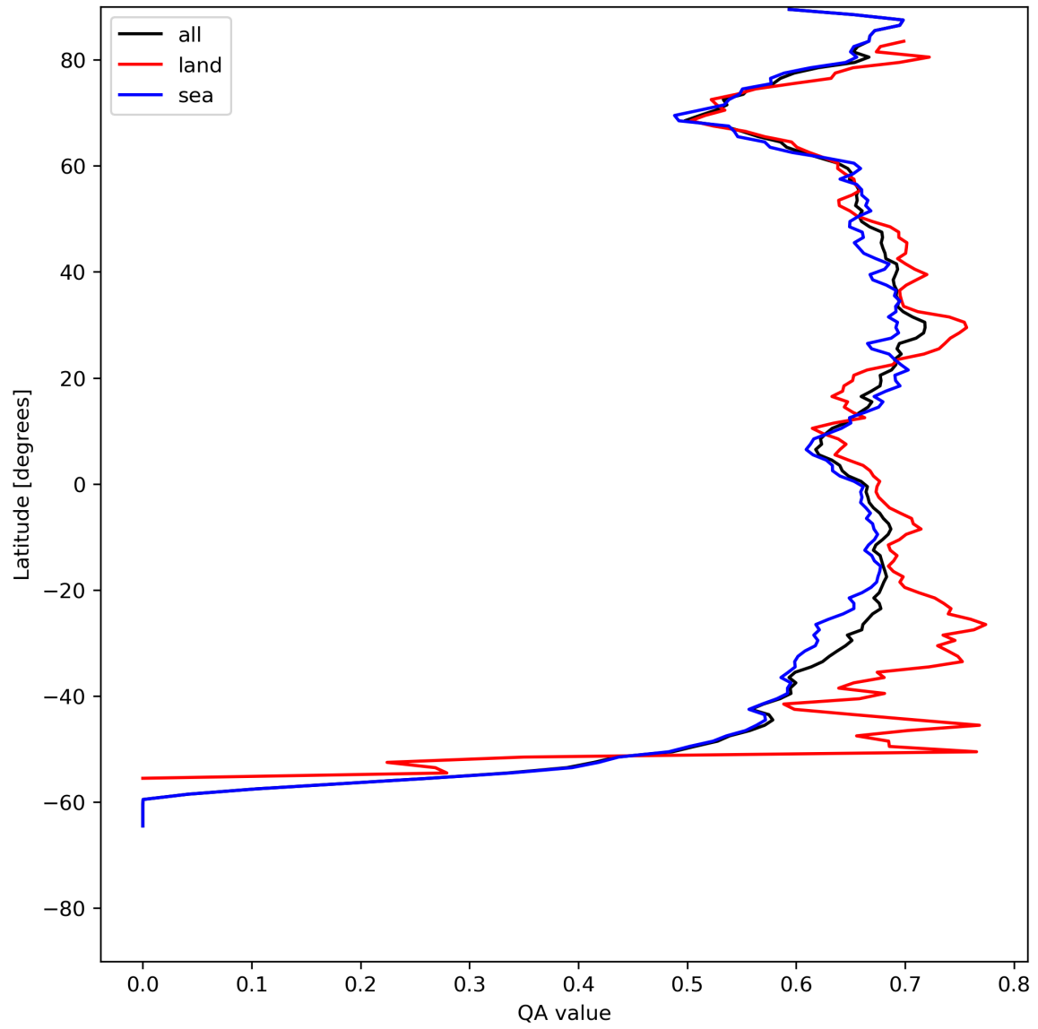
Figure 9: Zonal average of “QA value” for 2023-07-21 to 2023-07-23.
