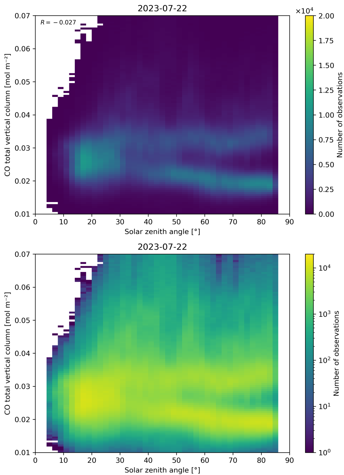
Figure 61: Scatter density plot of “Solar zenith angle” against “CO total vertical column” for 2023-07-21 to 2023-07-23.
