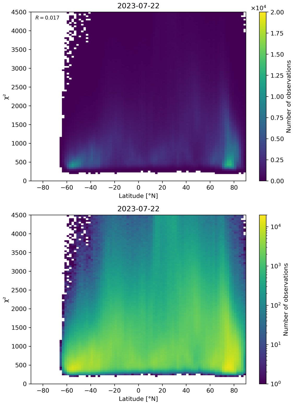
Figure 54: Scatter density plot of “Latitude” against “ \chi^2 ” for 2023-07-21 to 2023-07-23.
