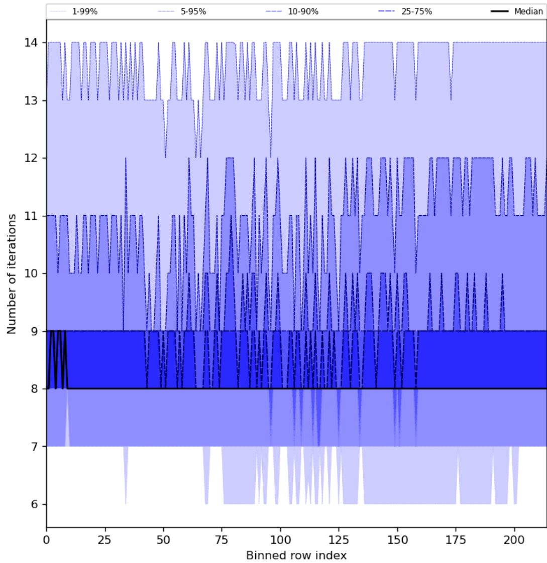
Figure 32: Along track statistics of “Number of iterations” for 2023-07-21 to 2023-07-23
