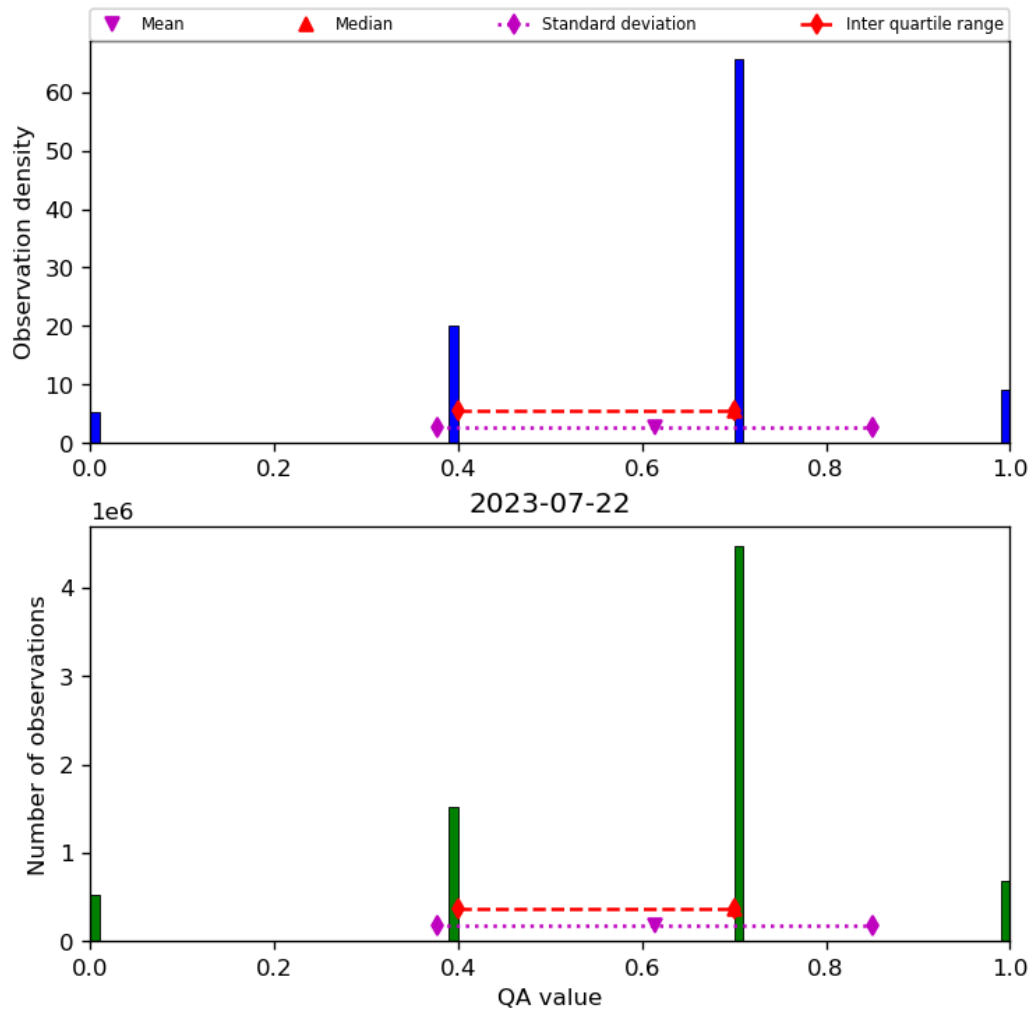
Figure 17: Histogram of “QA value” for 2023-07-21 to 2023-07-23
