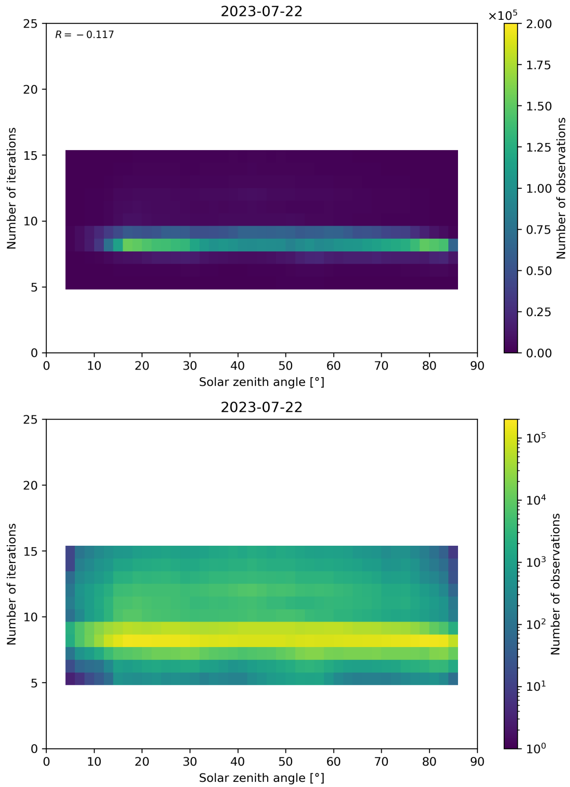
Figure 67: Scatter density plot of “Solar zenith angle” against “Number of iterations” for 2023-07-21 to 2023-07-23.
