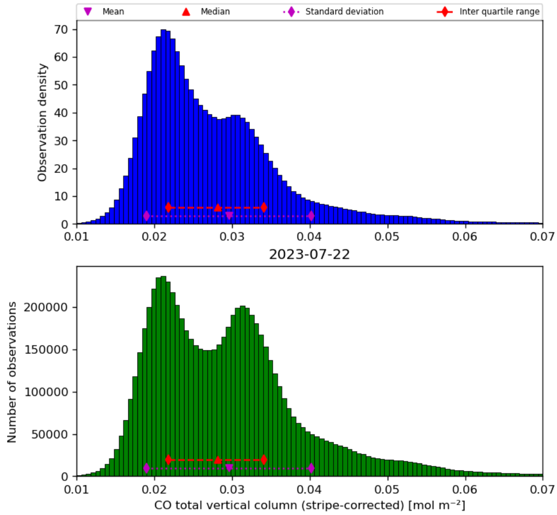
Figure 19: Histogram of “CO total vertical column (stripe-corrected)” for 2023-07-21 to 2023-07-23
