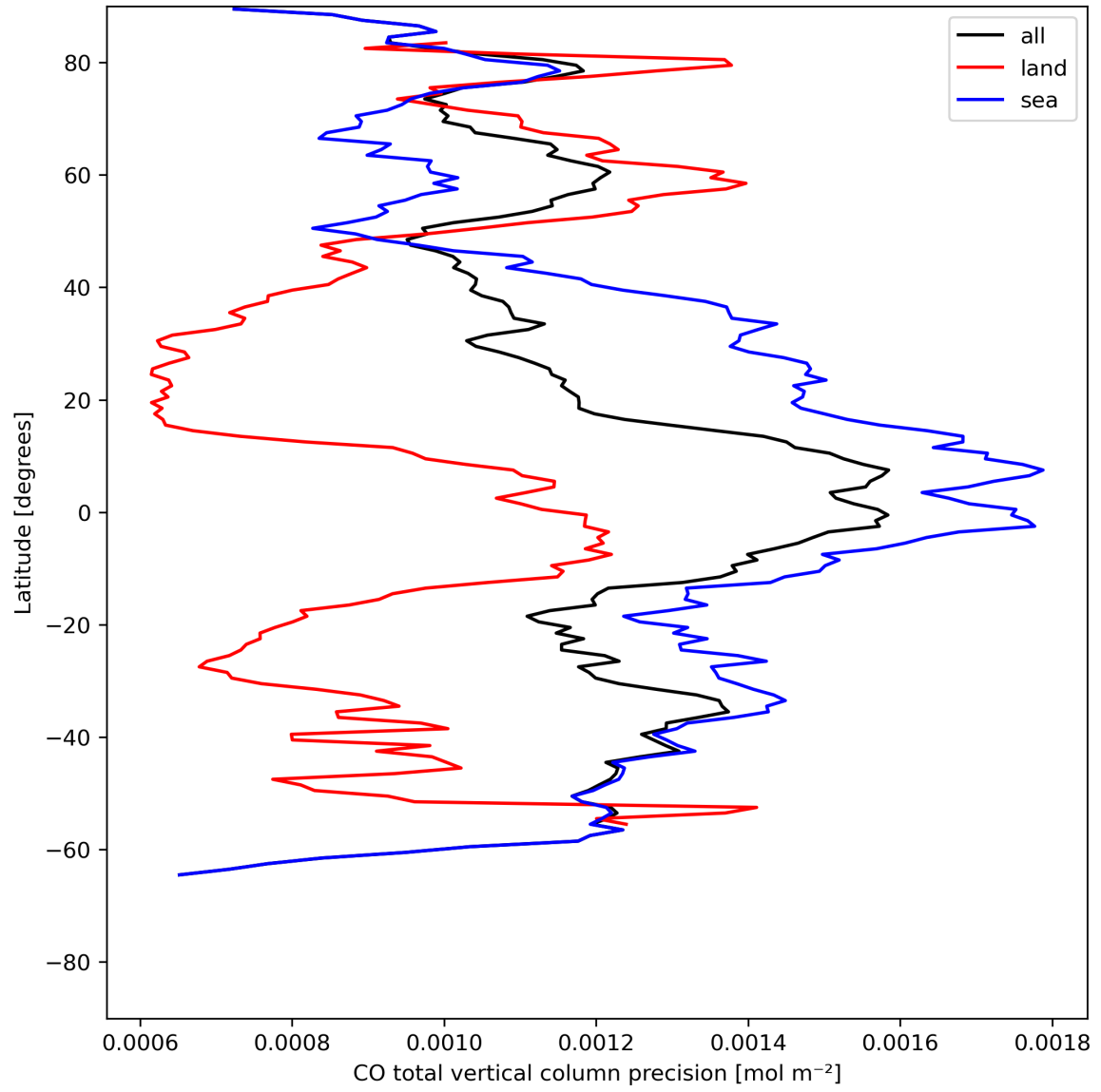
Figure 12: Zonal average of "CO total vertical column precision" for 2023-07-21 to 2023-07-23.
