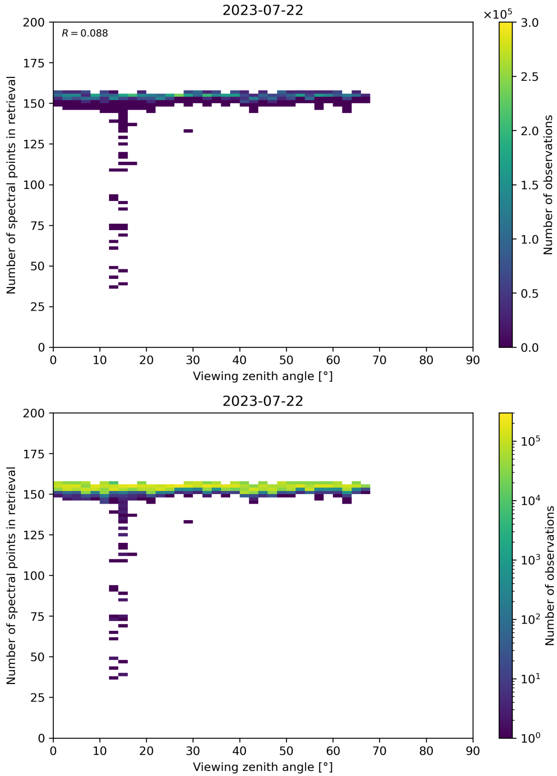
Figure 76: Scatter density plot of “Viewing zenith angle” against “Number of spectral points in retrieval” for 2023-07-21 to 2023-07-23.
