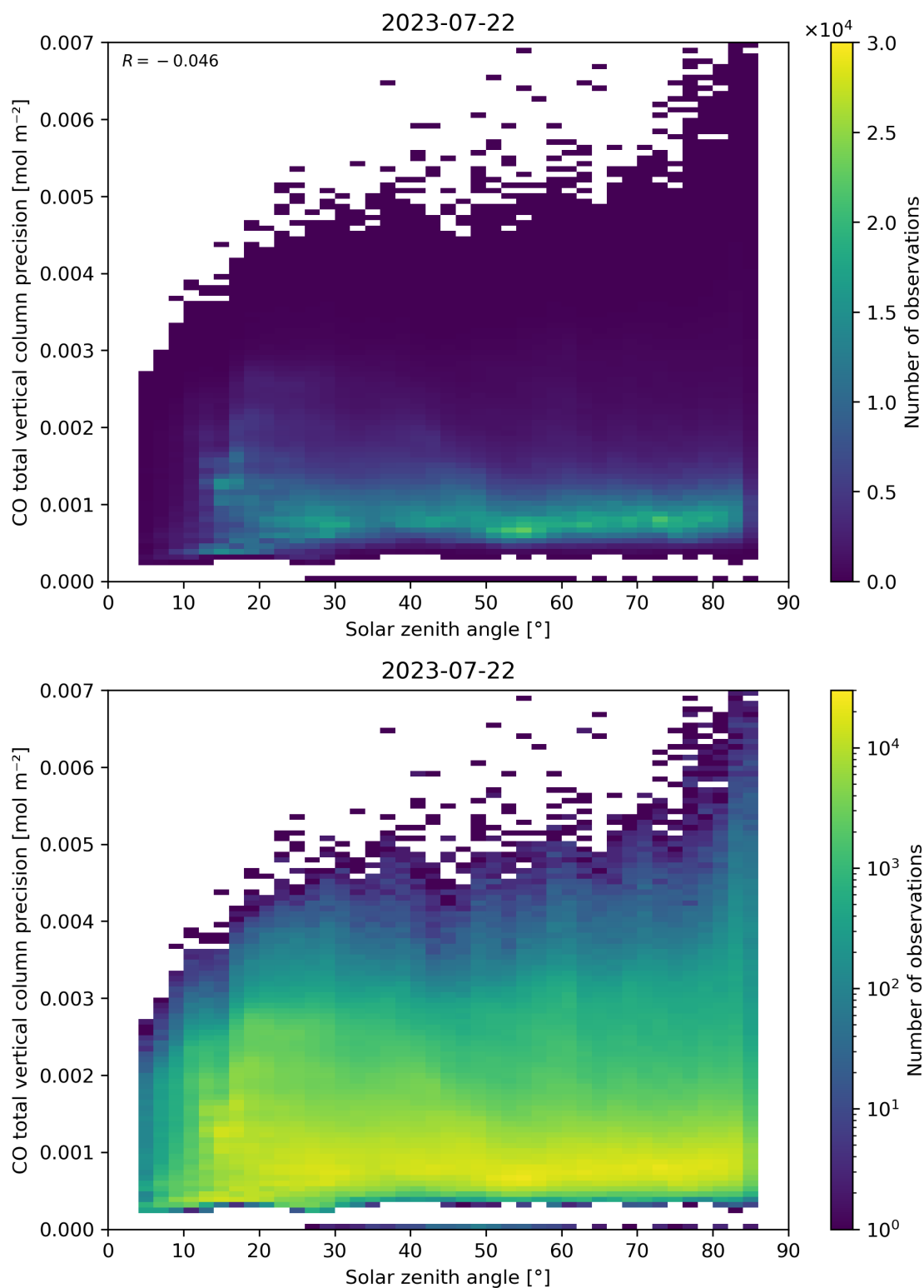
Figure 63: Scatter density plot of “Solar zenith angle” against “CO total vertical column precision” for 2023-07-21 to 2023-07-23.
