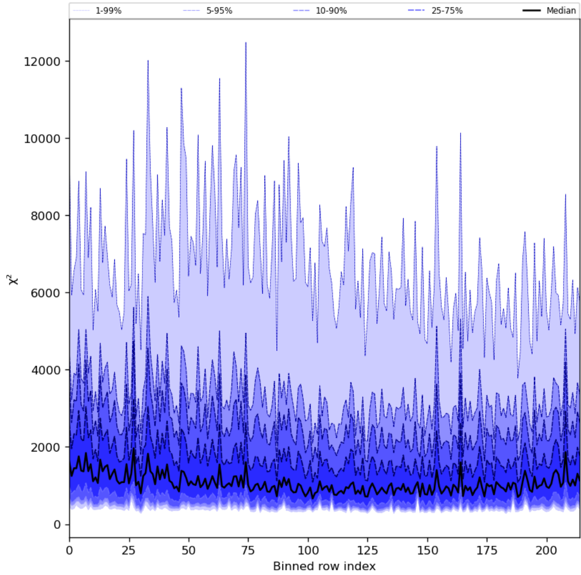
Figure 30: Along track statistics of “ \chi^2 ” for 2023-07-21 to 2023-07-23
