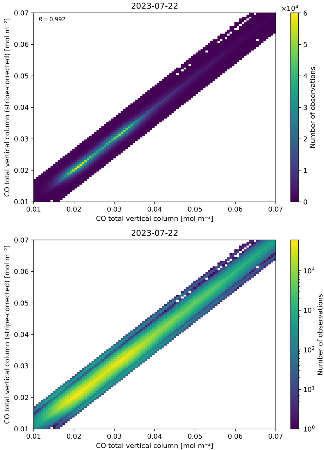
Figure 33: Scatter density plot of “CO total vertical column” against “CO total vertical column (stripe-corrected)” for 2023-07-21 to 2023-07-23.
