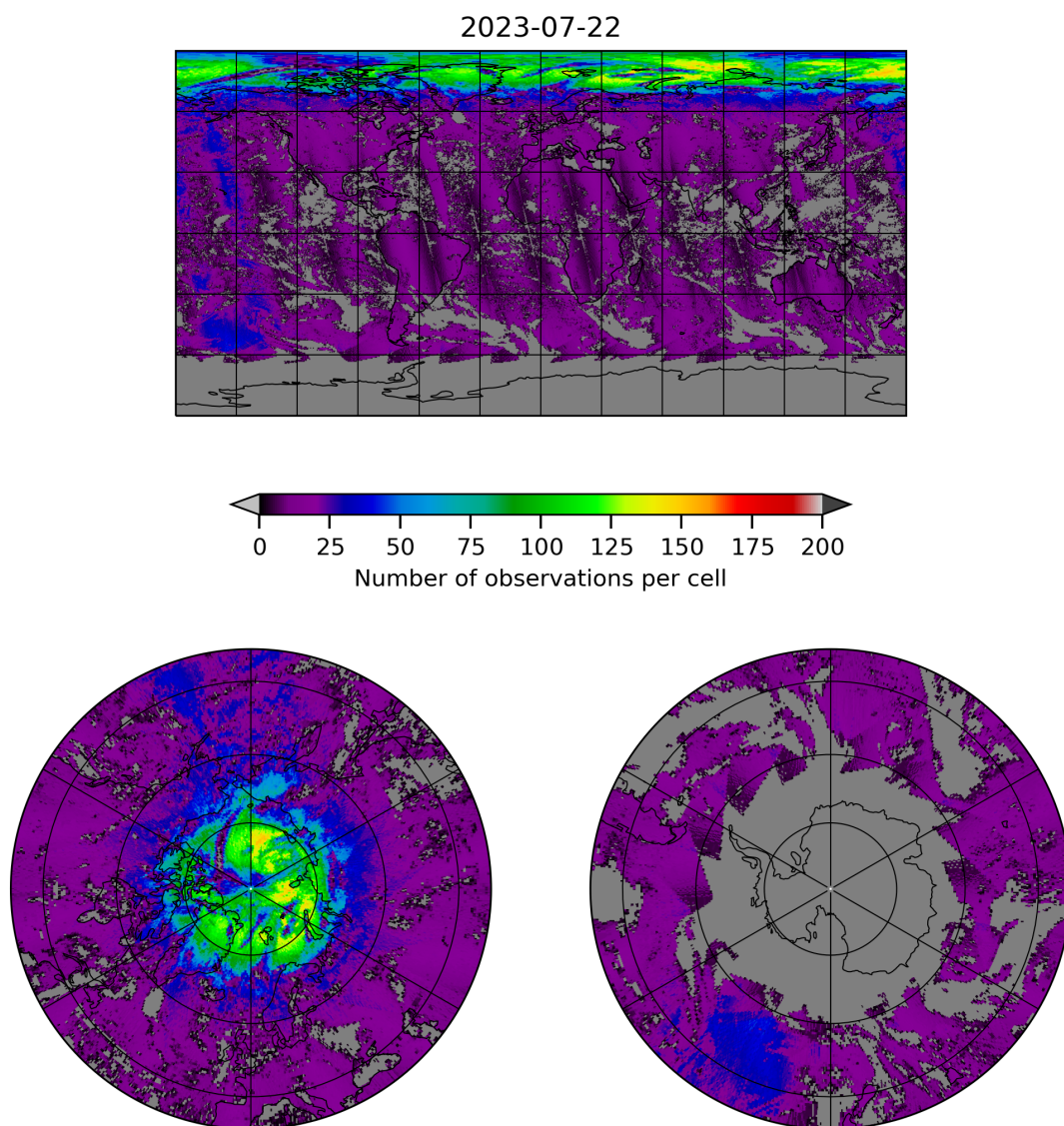
Figure 8: Map of the number of observations for 2023-07-21 to 2023-07-23
