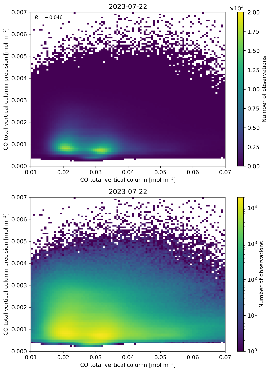
Figure 34: Scatter density plot of “CO total vertical column” against “CO total vertical column precision” for 2023-07-21 to 2023-07-23.
