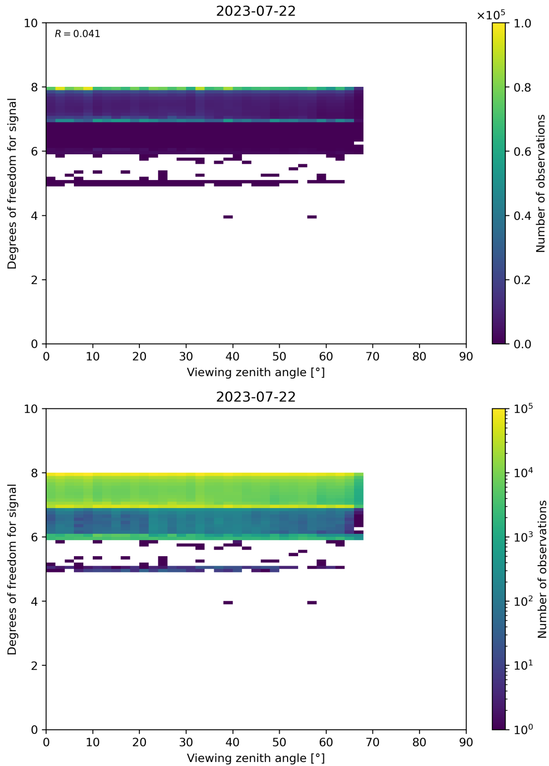
Figure 73: Scatter density plot of “Viewing zenith angle” against “Degrees of freedom for signal” for 2023-07-21 to 2023-07-23.
