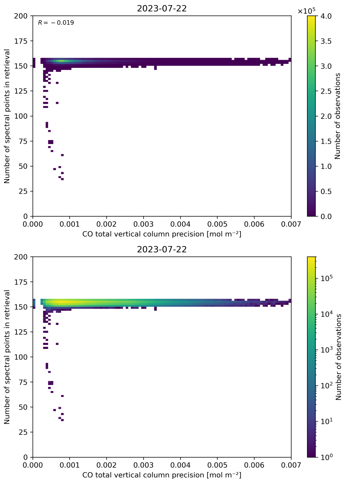
Figure 47: Scatter density plot of “CO total vertical column precision” against “Number of spectral points in retrieval” for 2023-07-21 to 2023-07-23.
