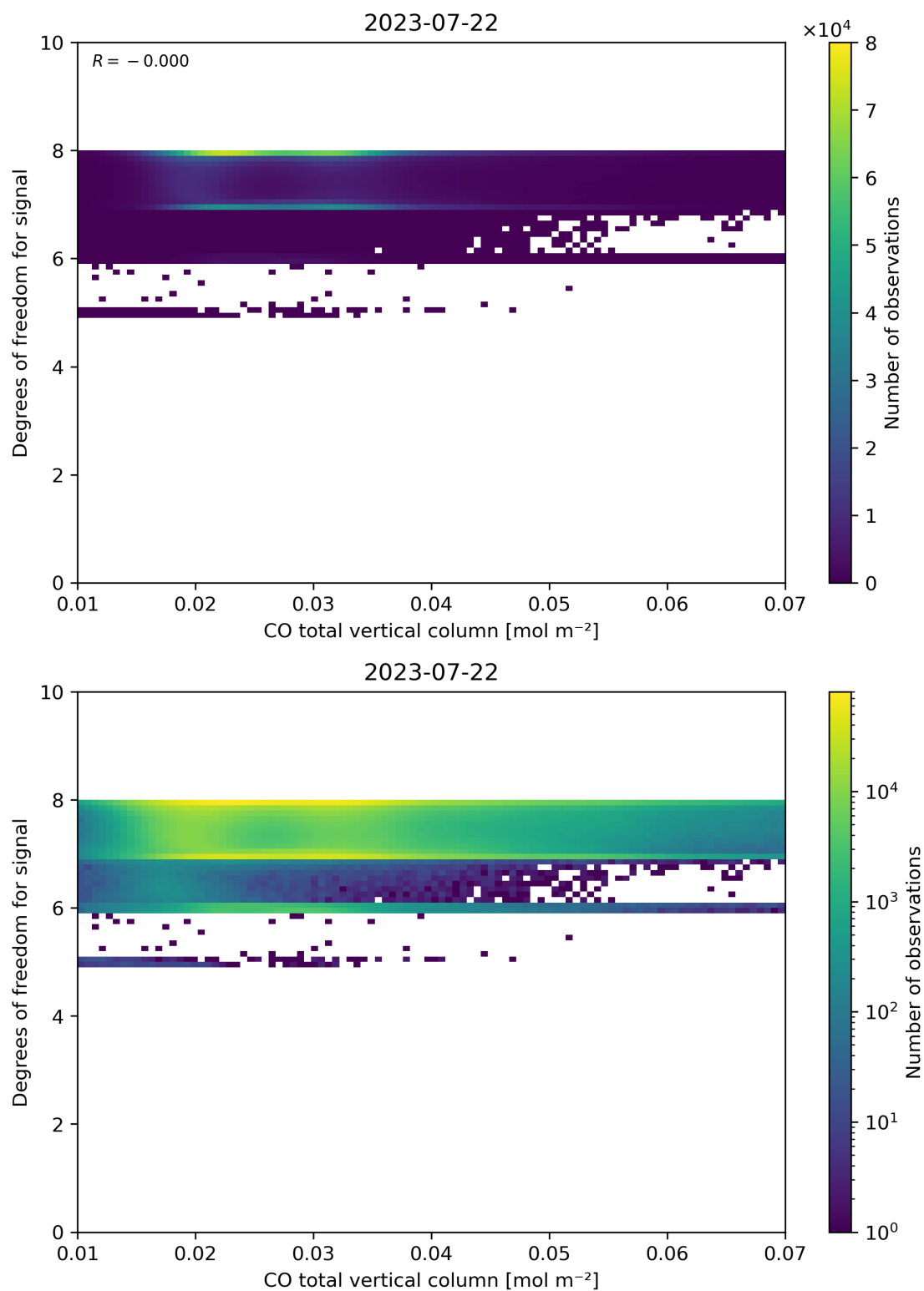
Figure 41: Scatter density plot of “CO total vertical column” against “Degrees of freedom for signal” for 2023-07-21 to 2023-07-23.
