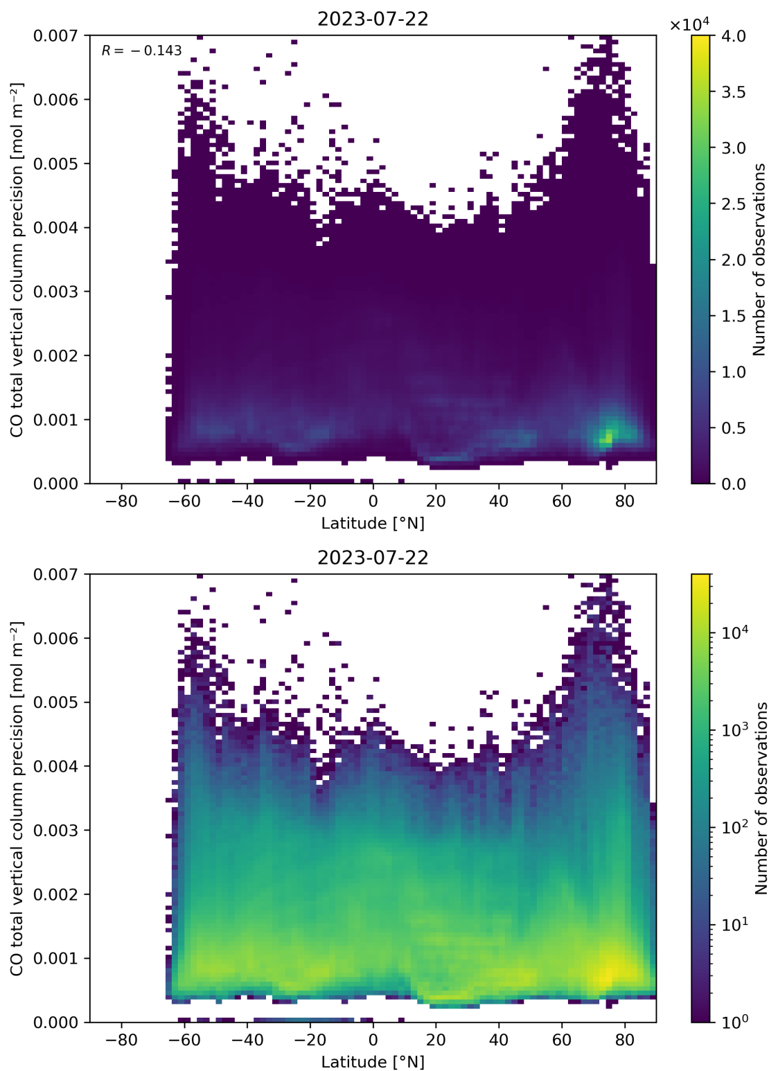
Figure 53: Scatter density plot of “Latitude” against “CO total vertical column precision” for 2023-07-21 to 2023-07-23.
