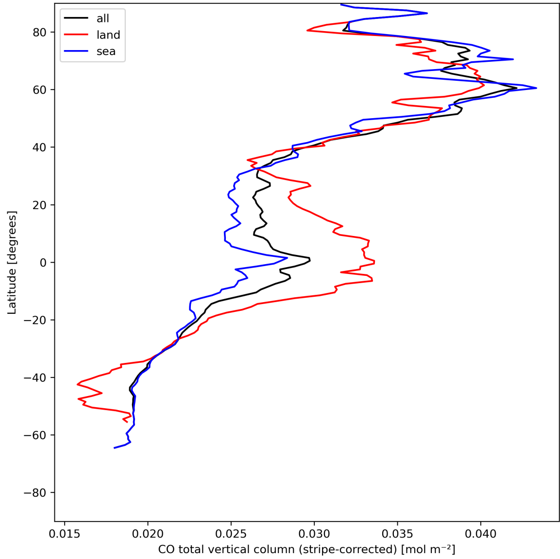
Figure 11: Zonal average of “CO total vertical column (stripe-corrected)” for 2023-07-21 to 2023-07-23.
