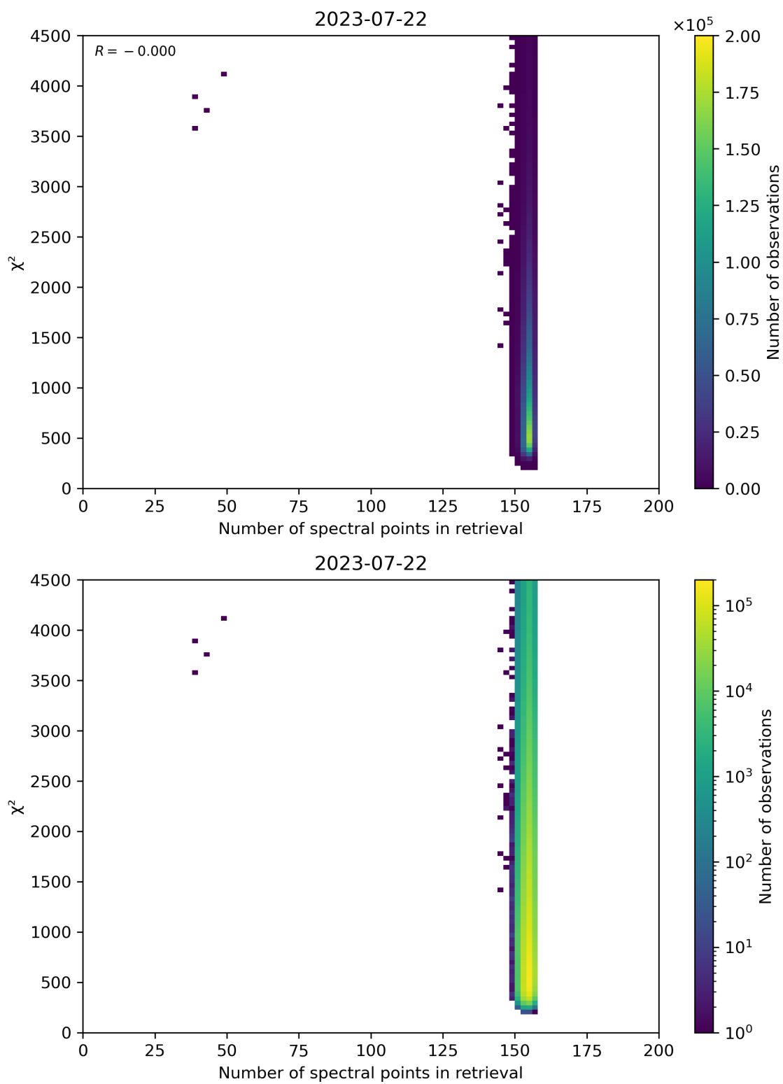
Figure 58: Scatter density plot of “Number of spectral points in retrieval” against “ \chi^2 ” for 2023-07-21 to 2023-07-23.
