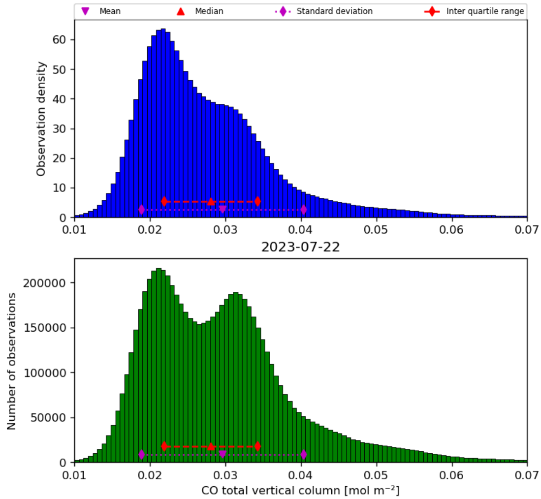
Figure 18: Histogram of “CO total vertical column” for 2023-07-21 to 2023-07-23
