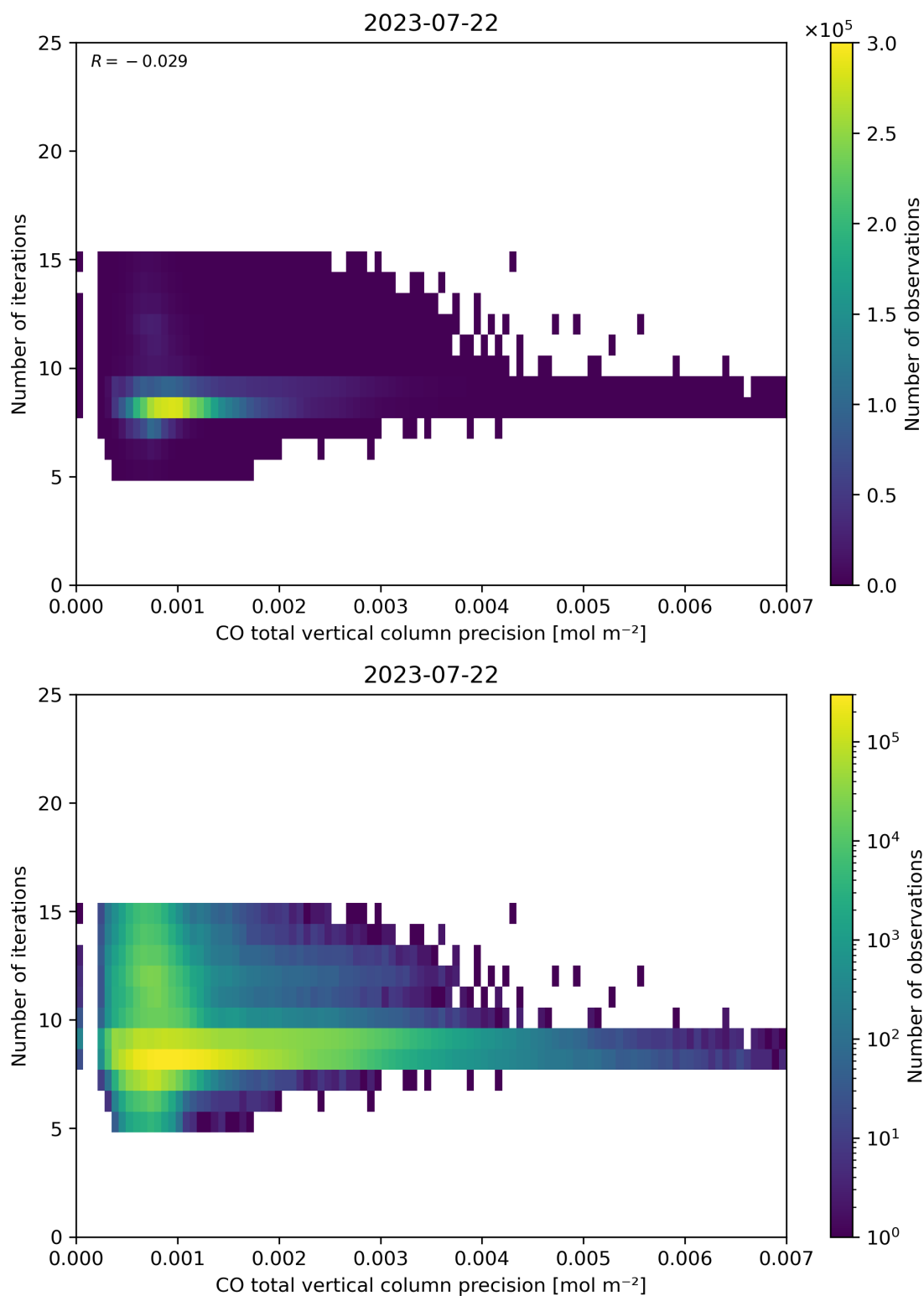
Figure 46: Scatter density plot of “CO total vertical column precision” against “Number of iterations” for 2023-07-21 to 2023-07-23.
