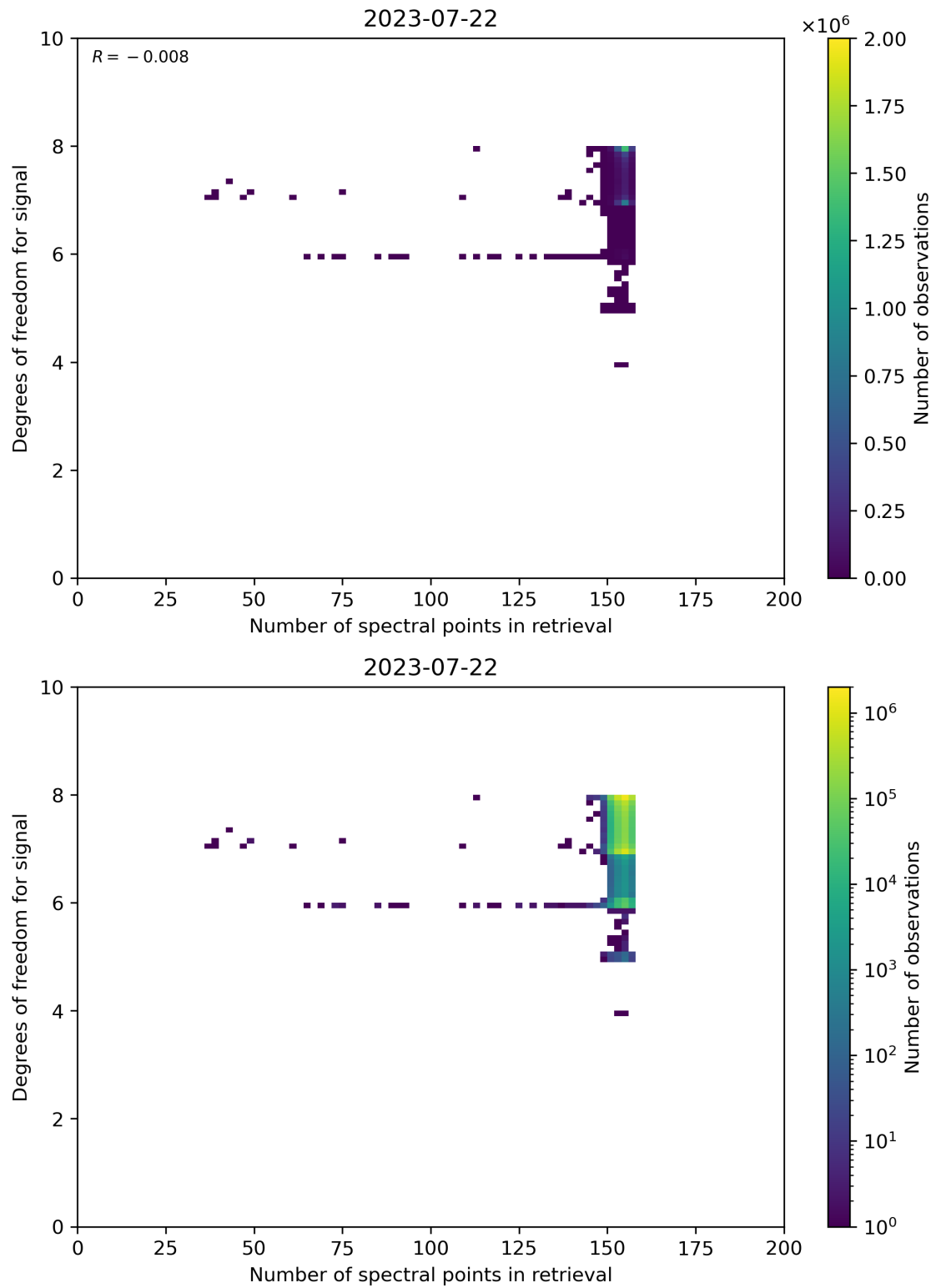
Figure 59: Scatter density plot of “Number of spectral points in retrieval” against “Degrees of freedom for signal” for 2023-07-21 to 2023-07-23.
