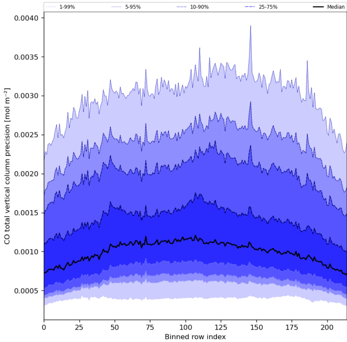
Figure 28: Along track statistics of “CO total vertical column precision” for 2023-07-21 to 2023-07-23
