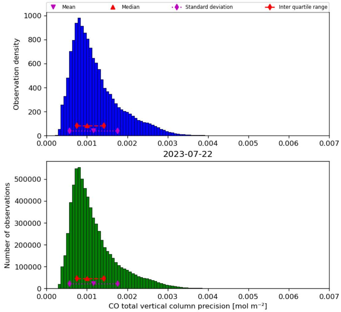
Figure 20: Histogram of “CO total vertical column precision” for 2023-07-21 to 2023-07-23
