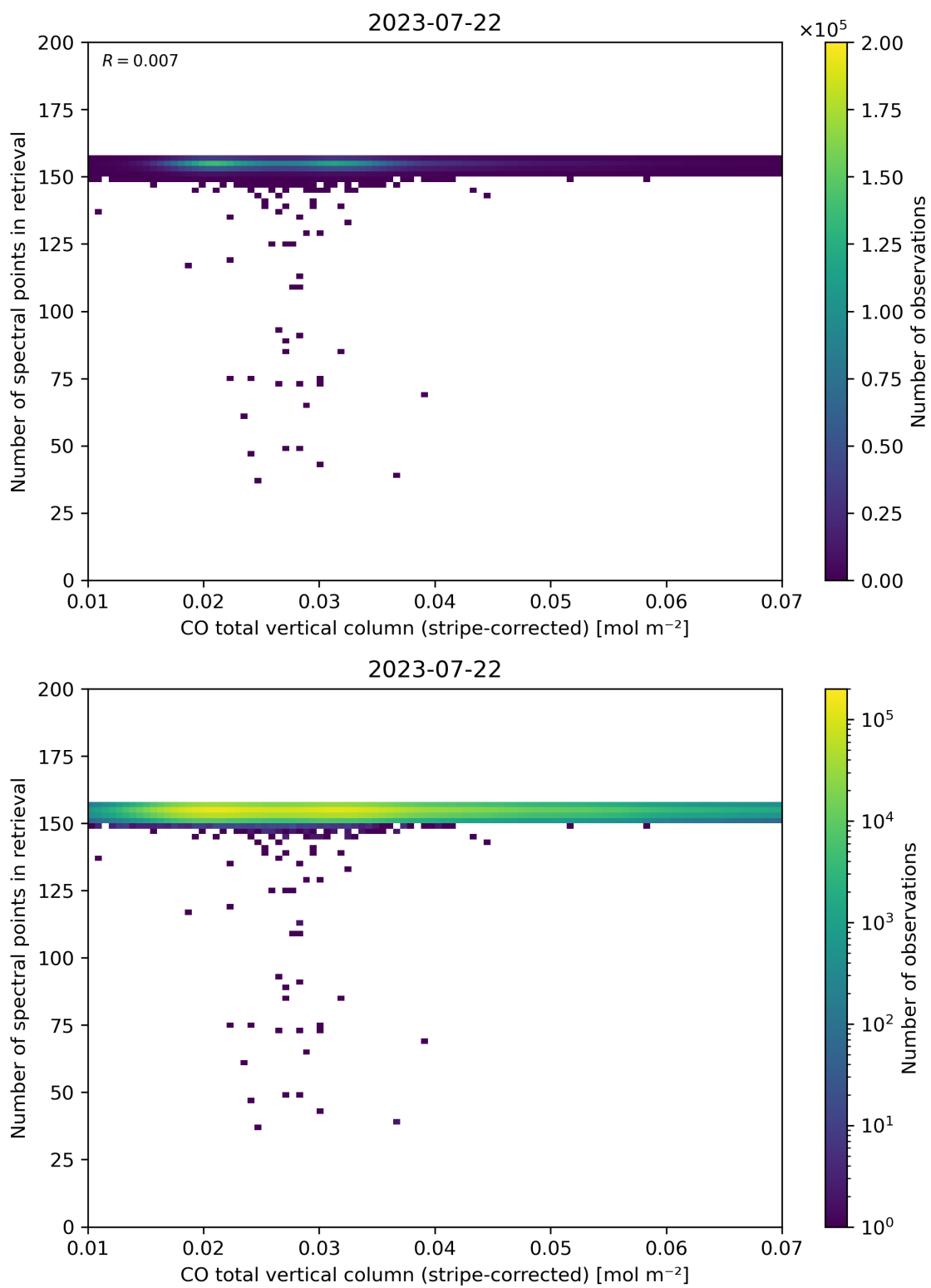
Figure 40: Scatter density plot of “CO total vertical column (stripe-corrected)” against “Number of spectral points in retrieval” for 2023-07-21 to 2023-07-23.
