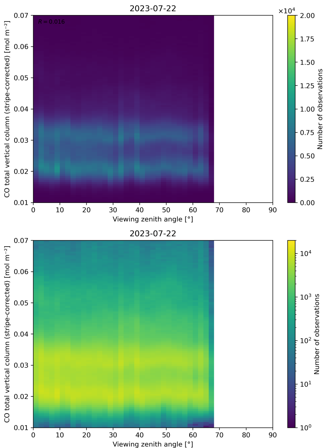
Figure 70: Scatter density plot of “Viewing zenith angle” against “CO total vertical column (stripe-corrected)” for 2023-07-21 to 2023-07-23.
