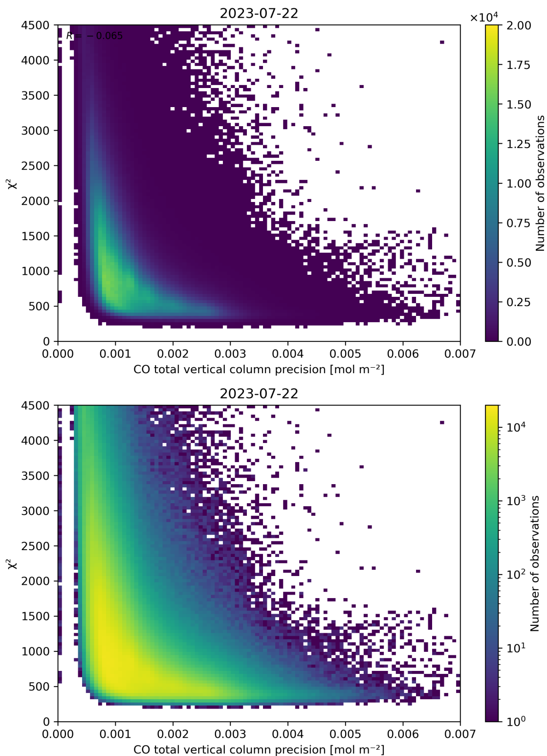
Figure 44: Scatter density plot of “CO total vertical column precision” against “ \chi^2 ” for 2023-07-21 to 2023-07-23.
