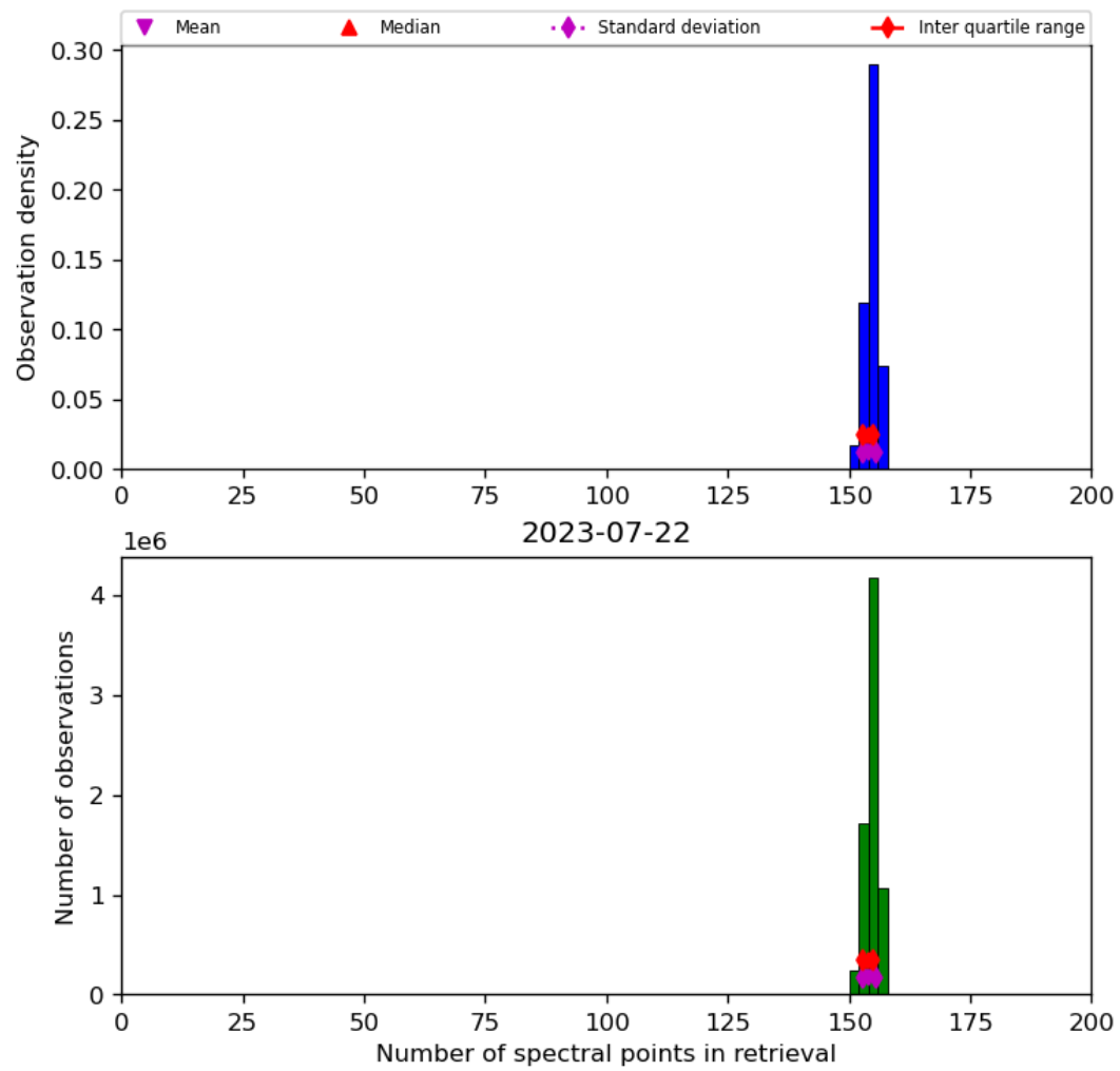
Figure 21: Histogram of “Number of spectral points in retrieval” for 2023-07-21 to 2023-07-23
