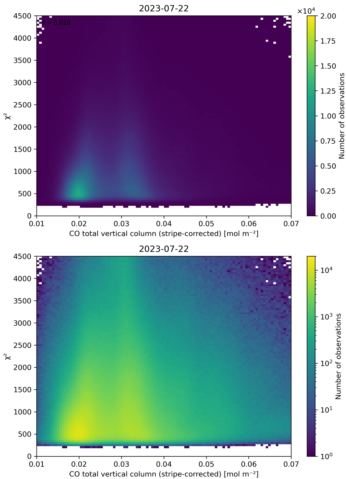
Figure 37: Scatter density plot of “CO total vertical column (stripe-corrected)” against “ \chi^2 ” for 2023-07-21 to 2023-07-23.
