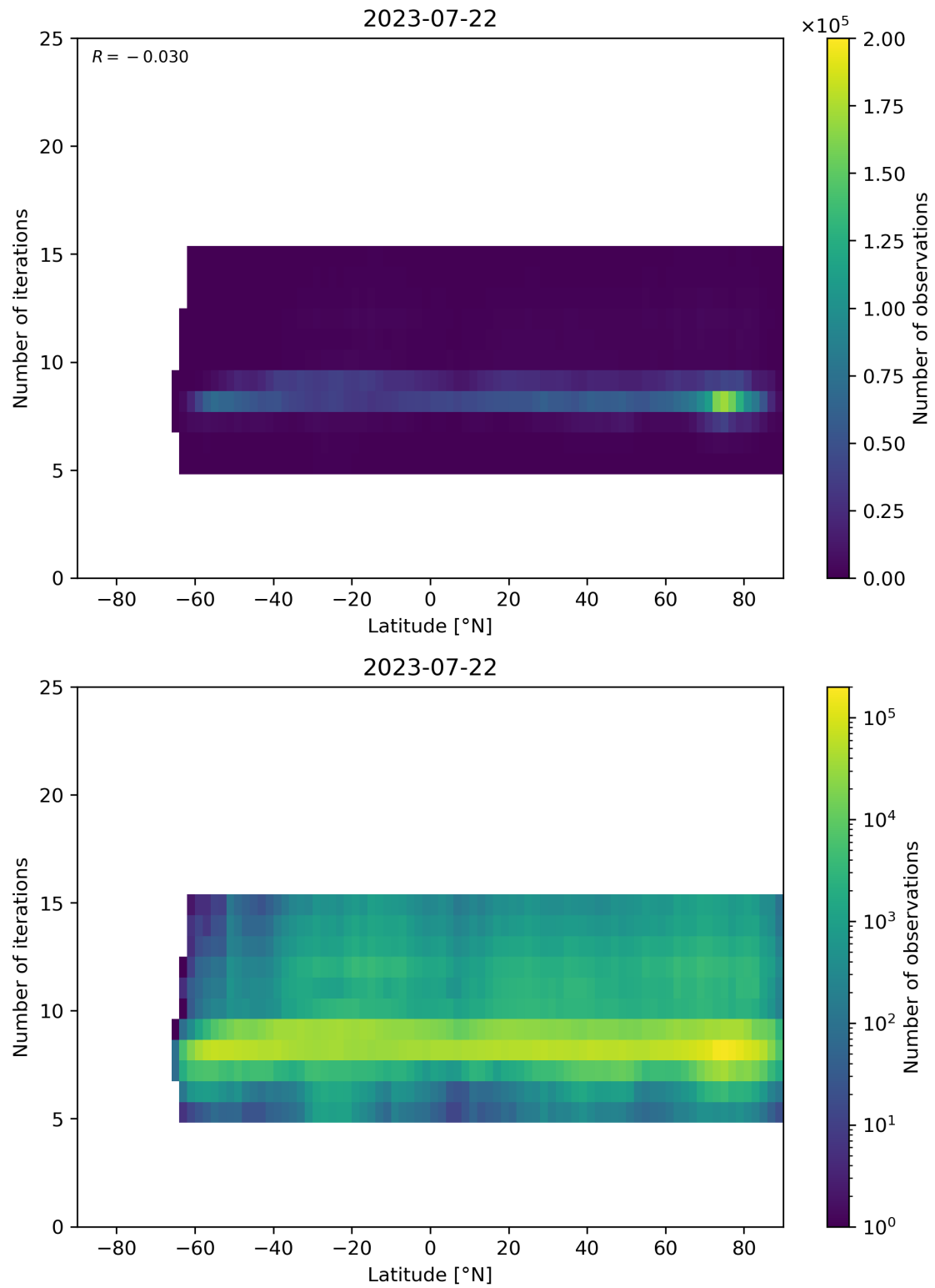
Figure 56: Scatter density plot of “Latitude” against “Number of iterations” for 2023-07-21 to 2023-07-23.
