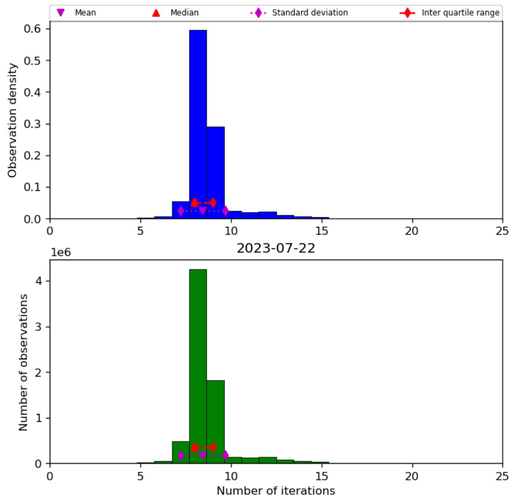
Figure 24: Histogram of “Number of iterations” for 2023-07-21 to 2023-07-23
