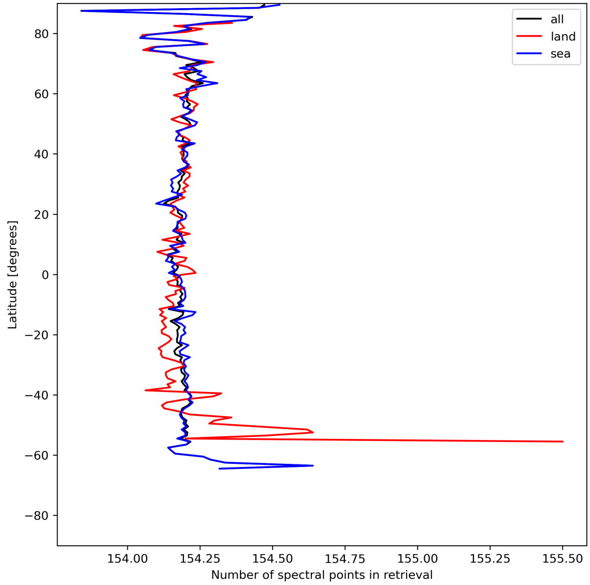
Figure 13: Zonal average of “Number of spectral points in retrieval” for 2023-07-21 to 2023-07-23.
