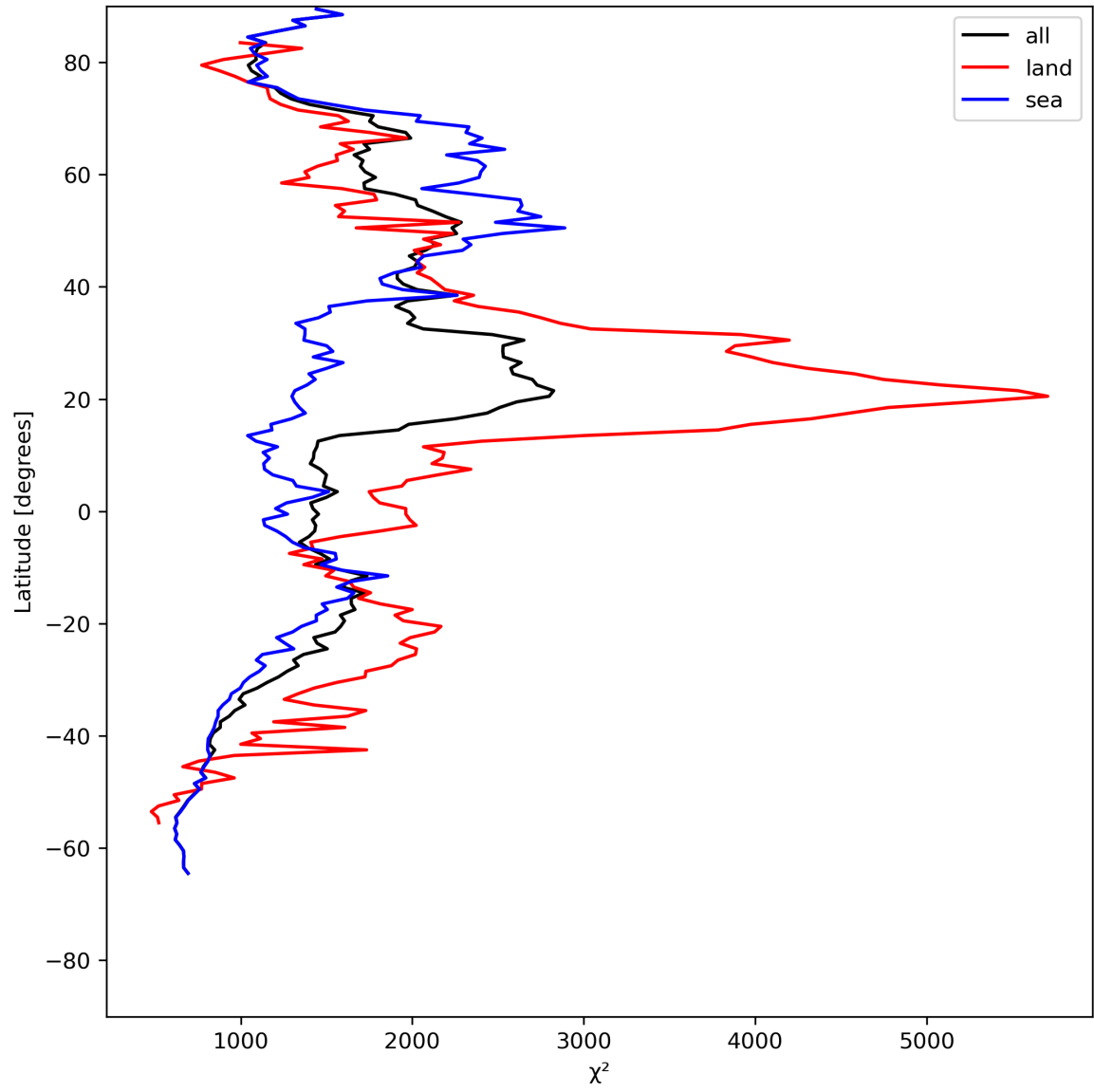
Figure 14: Zonal average of “ \chi^2 ” for 2023-07-21 to 2023-07-23.
