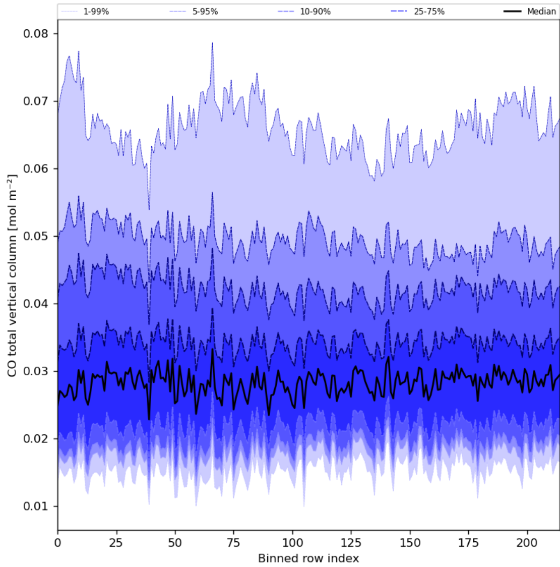
Figure 26: Along track statistics of “CO total vertical column” for 2023-07-21 to 2023-07-23
