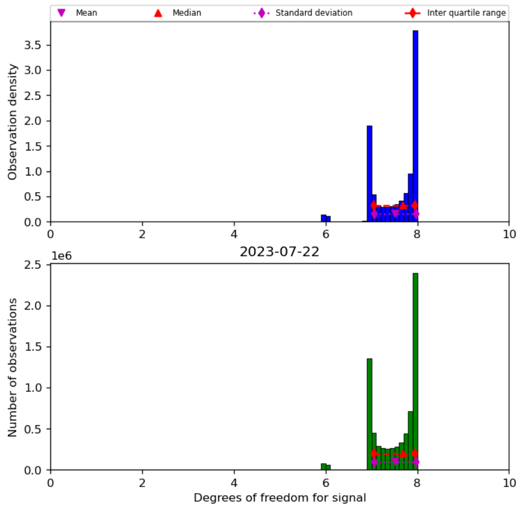
Figure 23: Histogram of “Degrees of freedom for signal” for 2023-07-21 to 2023-07-23
