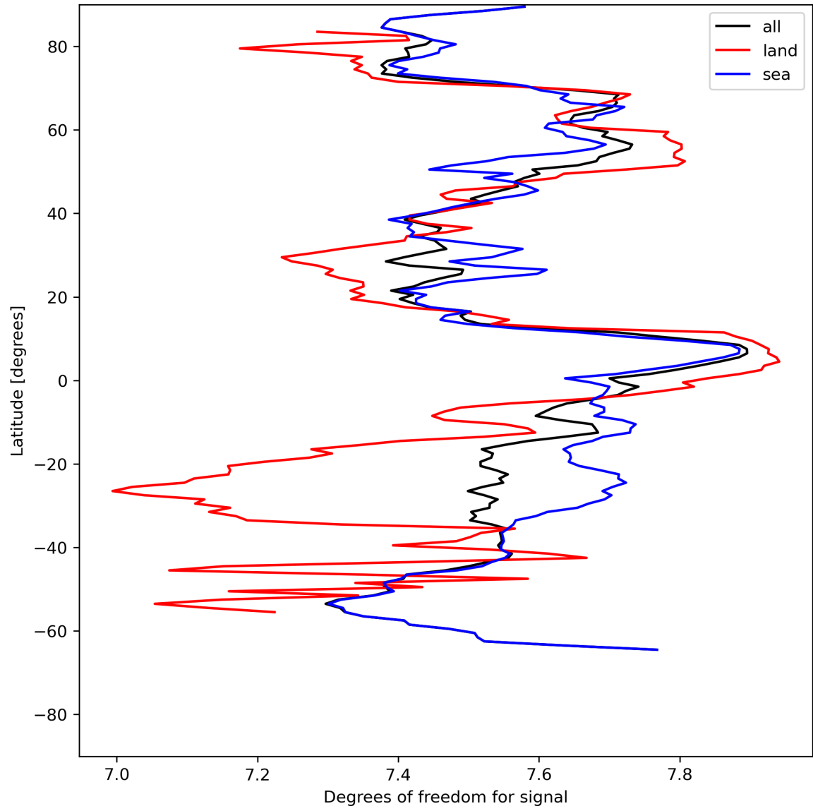
Figure 15: Zonal average of “Degrees of freedom for signal” for 2023-07-21 to 2023-07-23.
