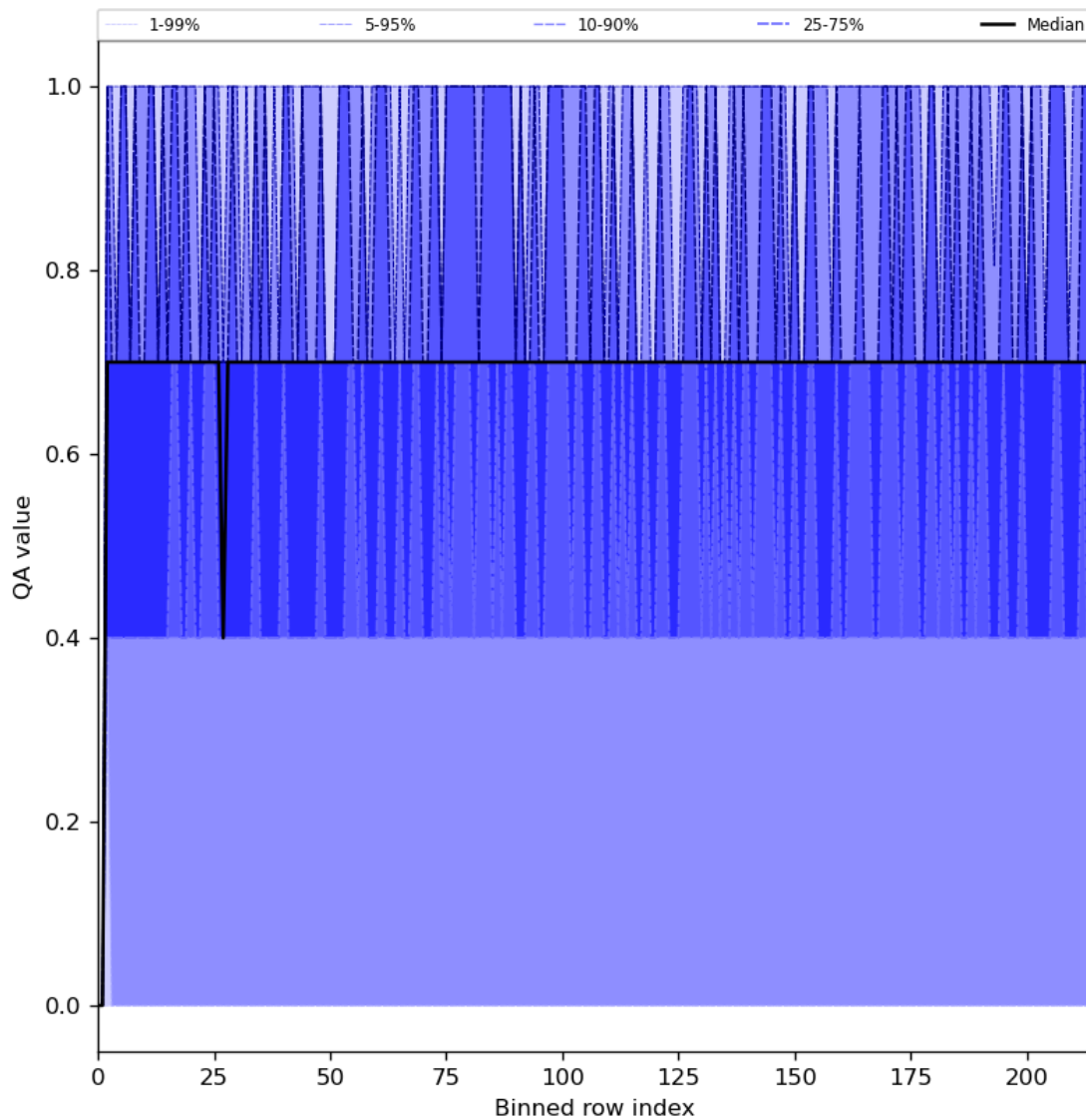
Figure 25: Along track statistics of “QA value” for 2023-07-21 to 2023-07-23
