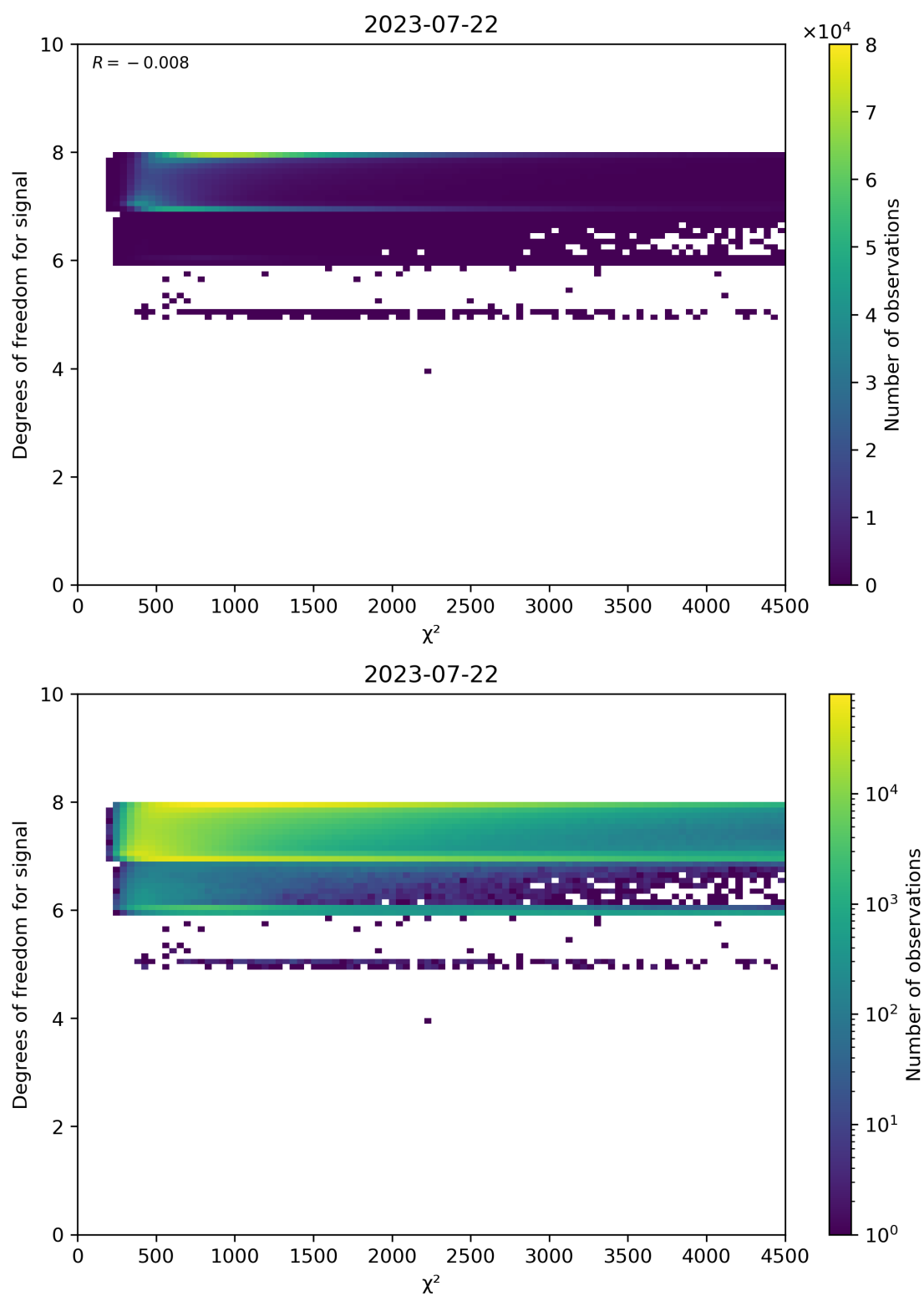
Figure 48: Scatter density plot of “ \chi^2 ” against “Degrees of freedom for signal” for 2023-07-21 to 2023-07-23.
