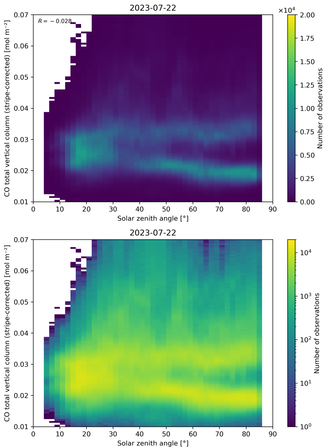
Figure 62: Scatter density plot of “Solar zenith angle” against “CO total vertical column (stripe-corrected)” for 2023-07-21 to 2023-07-23.
