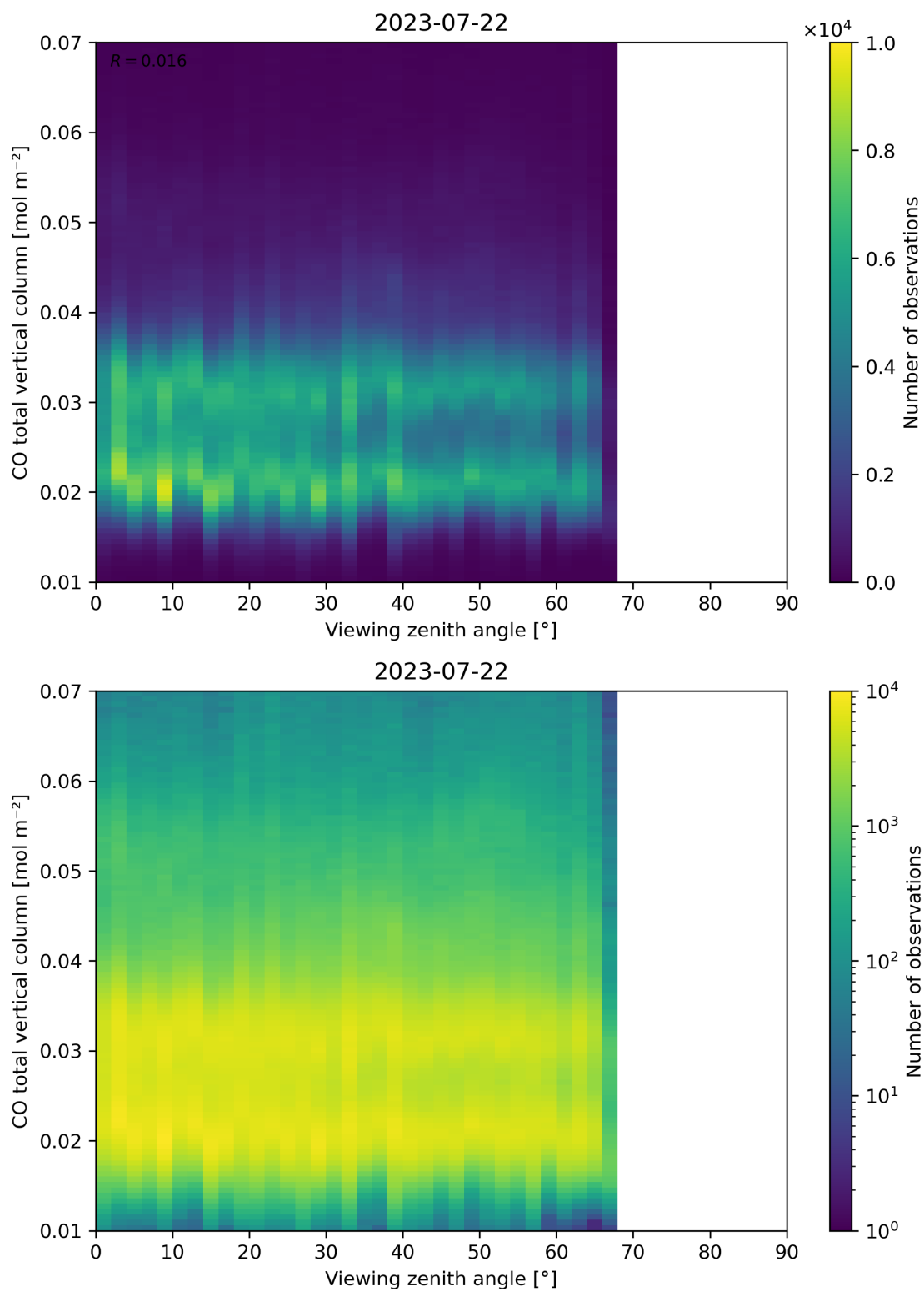
Figure 69: Scatter density plot of “Viewing zenith angle” against “CO total vertical column” for 2023-07-21 to 2023-07-23.
