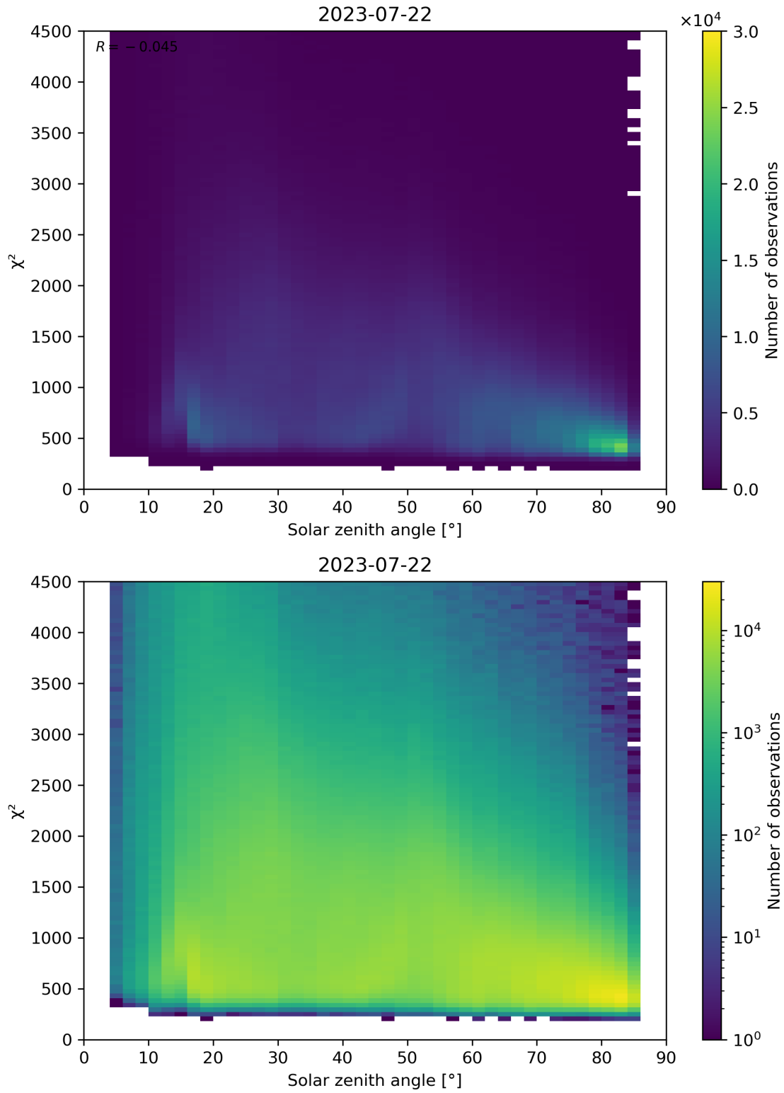
Figure 64: Scatter density plot of “Solar zenith angle” against “ \chi^2 ” for 2023-07-21 to 2023-07-23.
