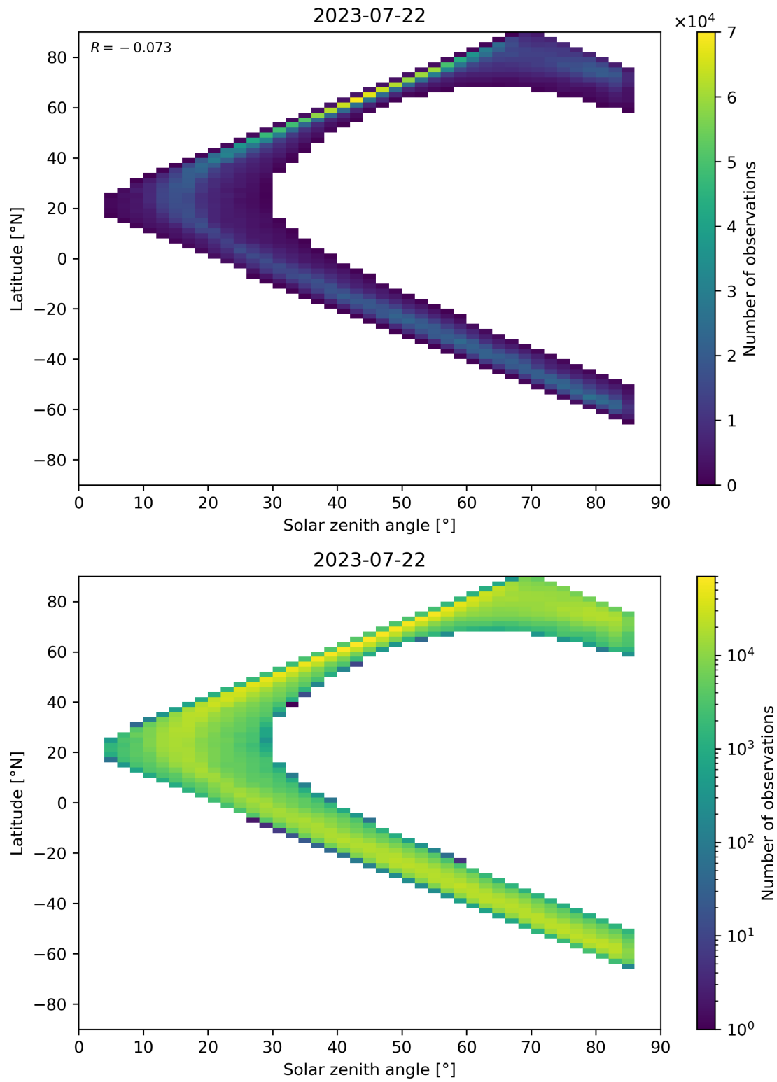
Figure 66: Scatter density plot of “Solar zenith angle” against “Latitude” for 2023-07-21 to 2023-07-23.
