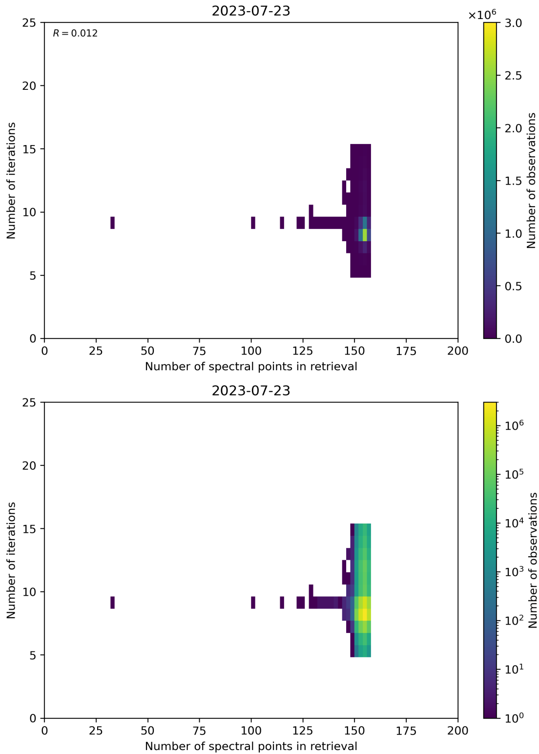
Figure 60: Scatter density plot of “Number of spectral points in retrieval” against “Number of iterations” for 2023-07-22 to 2023-07-24.
