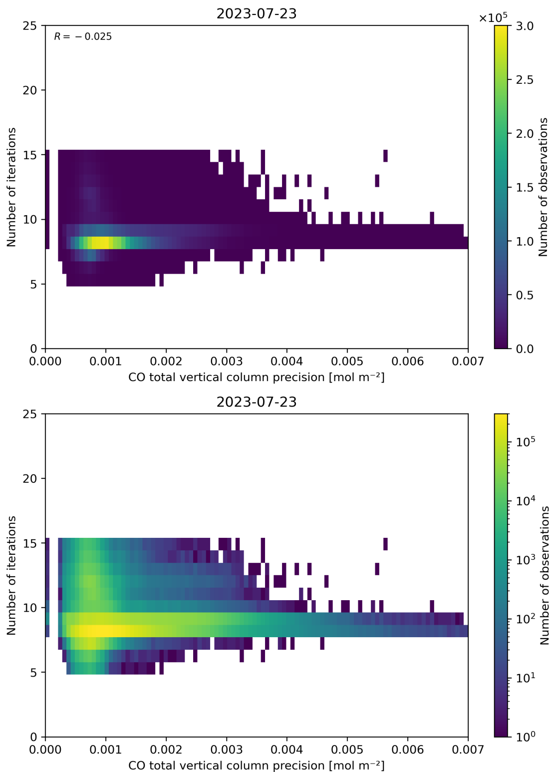
Figure 46: Scatter density plot of “CO total vertical column precision” against “Number of iterations” for 2023-07-22 to 2023-07-24.
