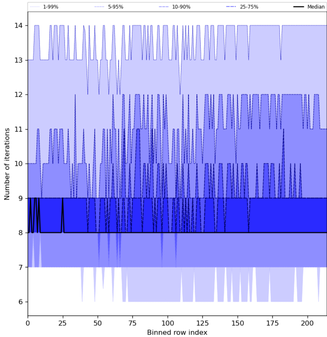
Figure 32: Along track statistics of “Number of iterations” for 2023-07-22 to 2023-07-24
