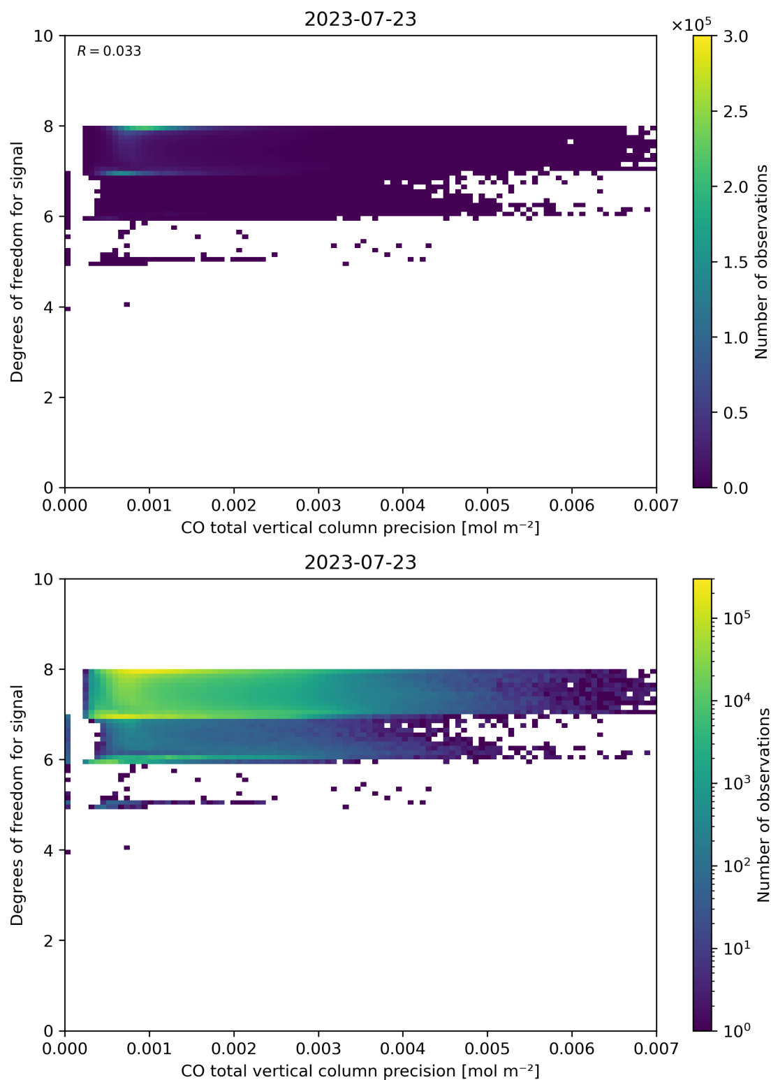
Figure 45: Scatter density plot of “CO total vertical column precision” against “Degrees of freedom for signal” for 2023-07-22 to 2023-07-24.
