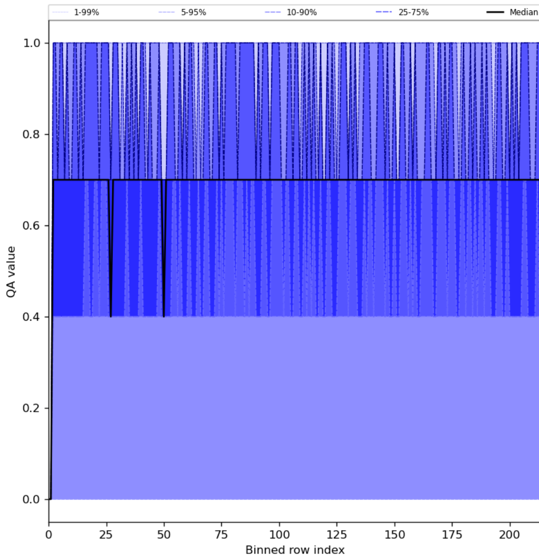
Figure 25: Along track statistics of “QA value” for 2023-07-22 to 2023-07-24
