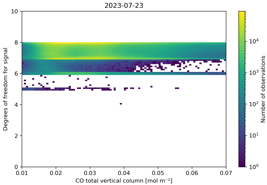
Figure 41: Scatter density plot of “CO total vertical column” against “Degrees of freedom for signal” for 2023-07-22 to 2023-07-24.
