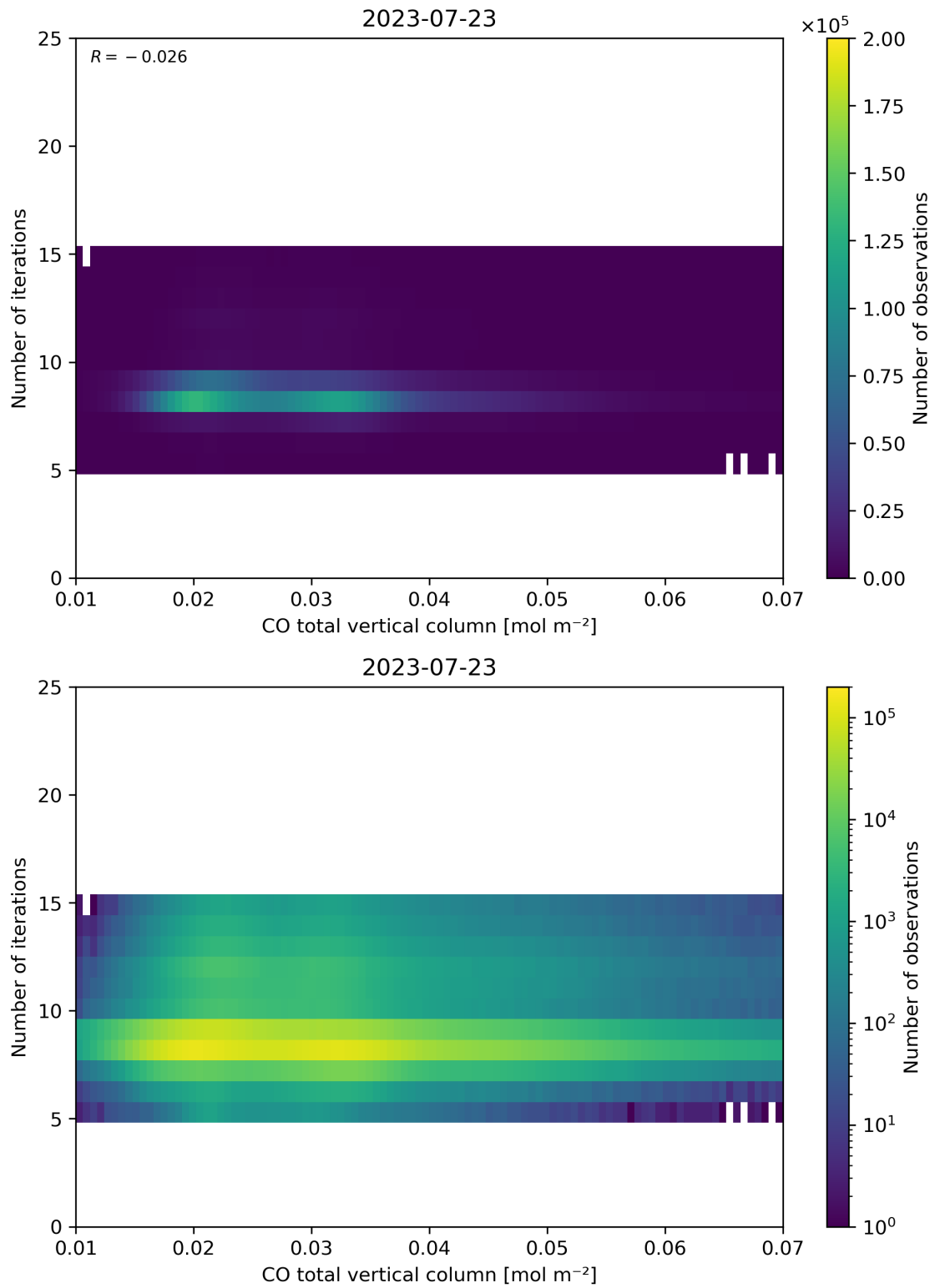
Figure 42: Scatter density plot of “CO total vertical column” against “Number of iterations” for 2023-07-22 to 2023-07-24.
