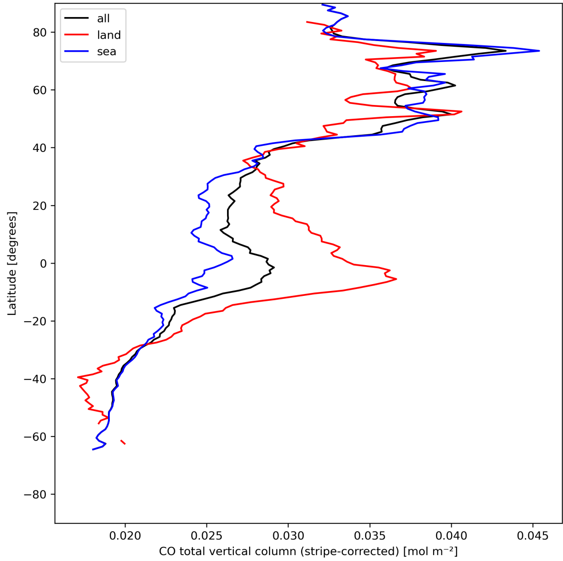
Figure 11: Zonal average of “CO total vertical column (stripe-corrected)” for 2023-07-22 to 2023-07-24.
