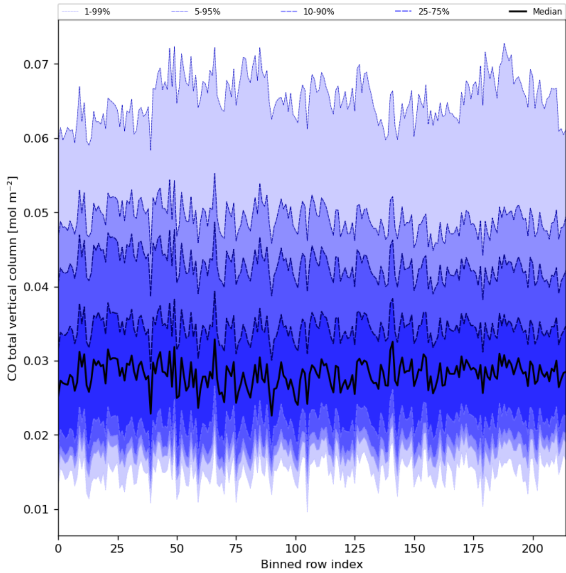
Figure 26: Along track statistics of “CO total vertical column” for 2023-07-22 to 2023-07-24
