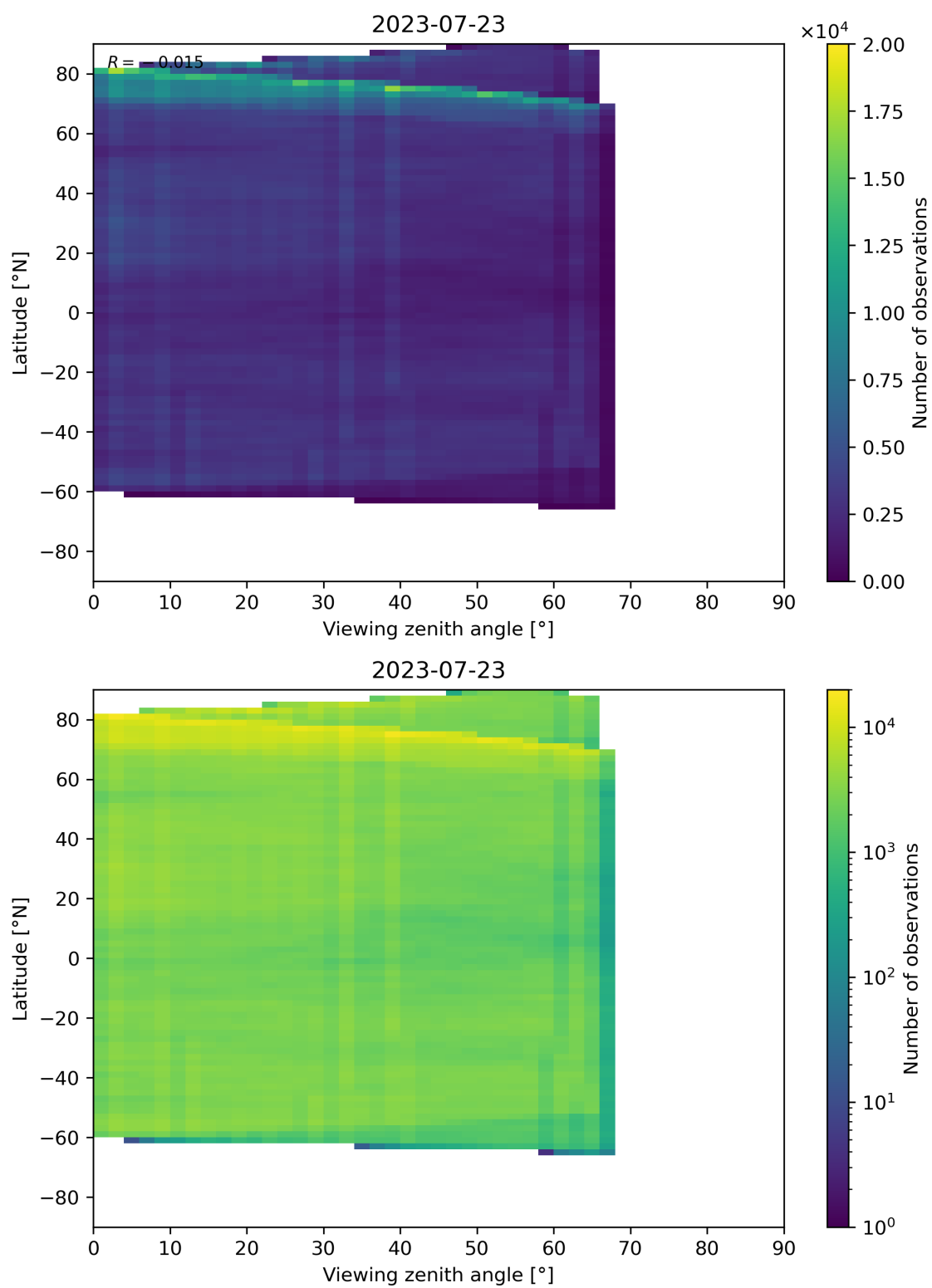
Figure 74: Scatter density plot of “Viewing zenith angle” against “Latitude” for 2023-07-22 to 2023-07-24.
