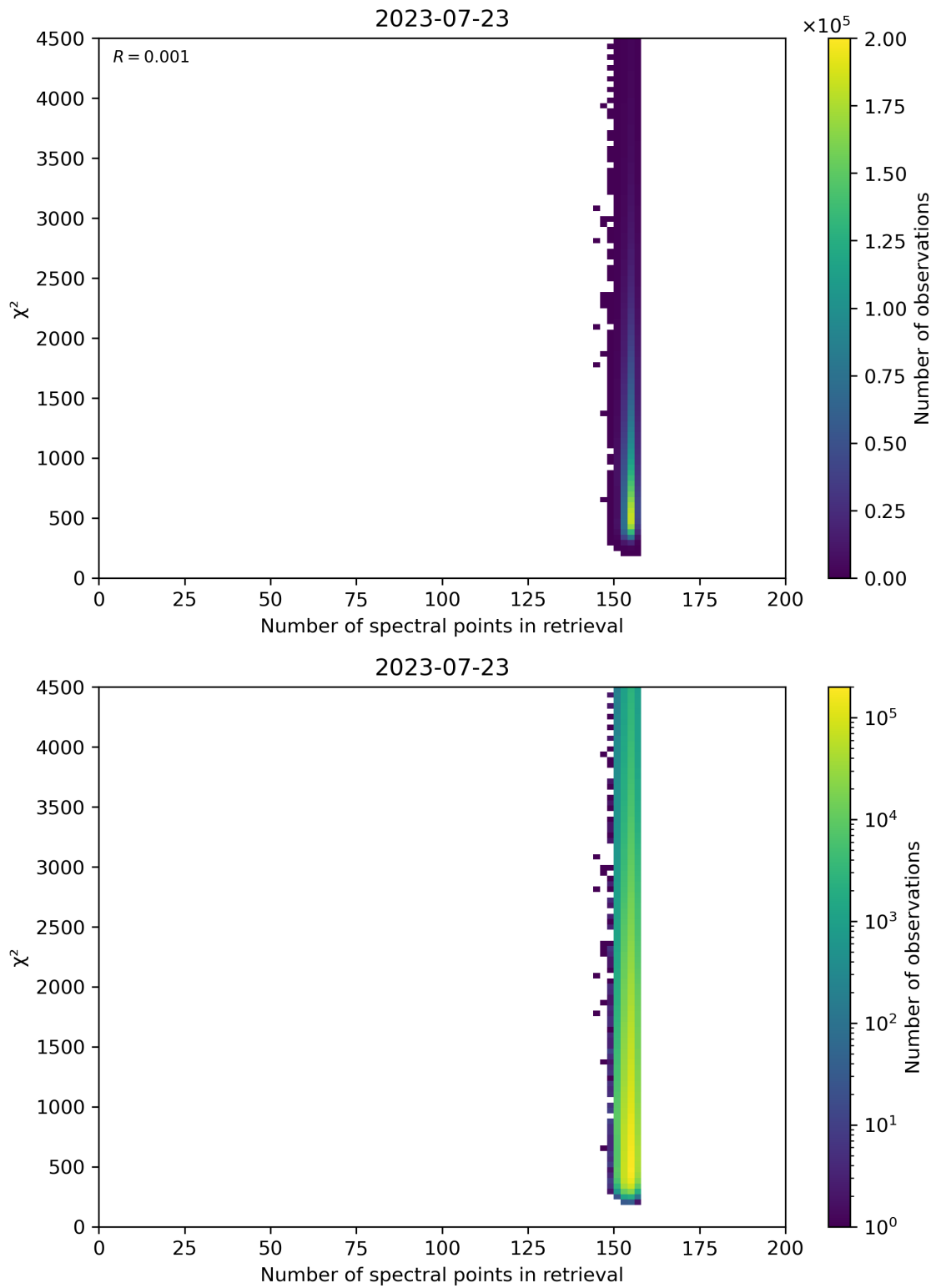
Figure 58: Scatter density plot of “Number of spectral points in retrieval” against “ \chi^2 ” for 2023-07-22 to 2023-07-24.
