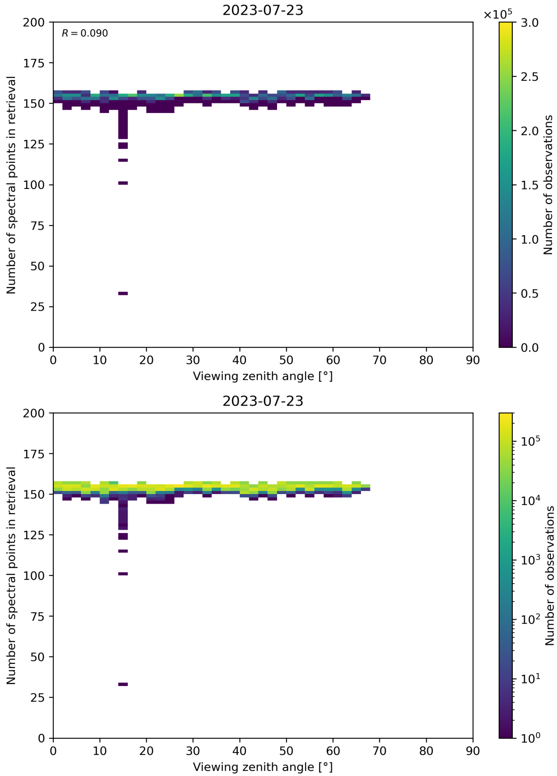
Figure 76: Scatter density plot of “Viewing zenith angle” against “Number of spectral points in retrieval” for 2023-07-22 to 2023-07-24.
