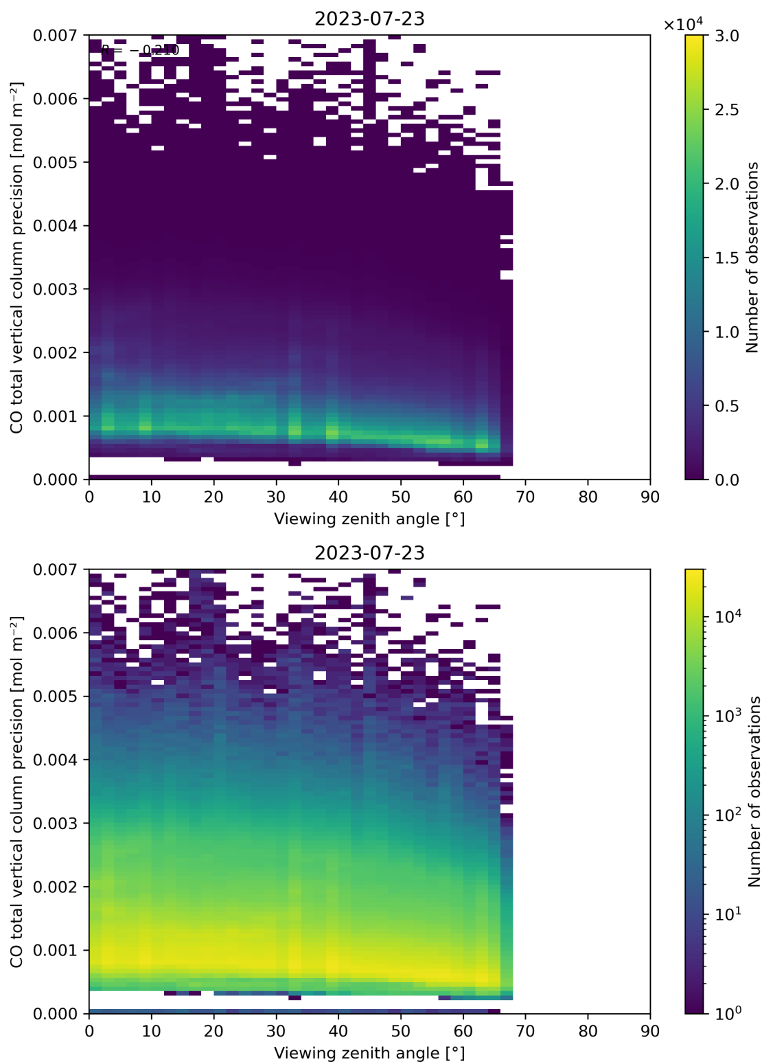
Figure 71: Scatter density plot of “Viewing zenith angle” against “CO total vertical column precision” for 2023-07-22 to 2023-07-24.
