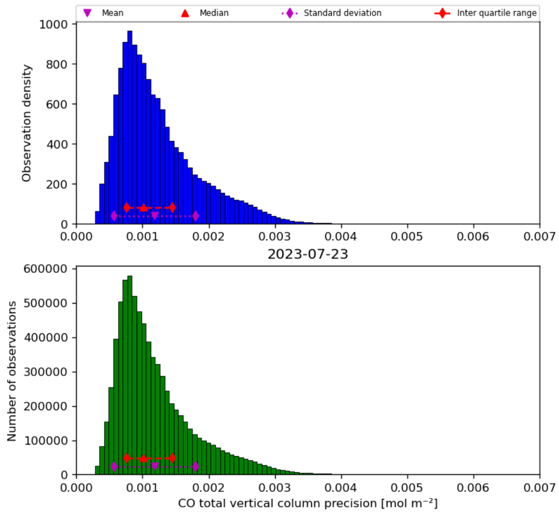
Figure 20: Histogram of “CO total vertical column precision” for 2023-07-22 to 2023-07-24
