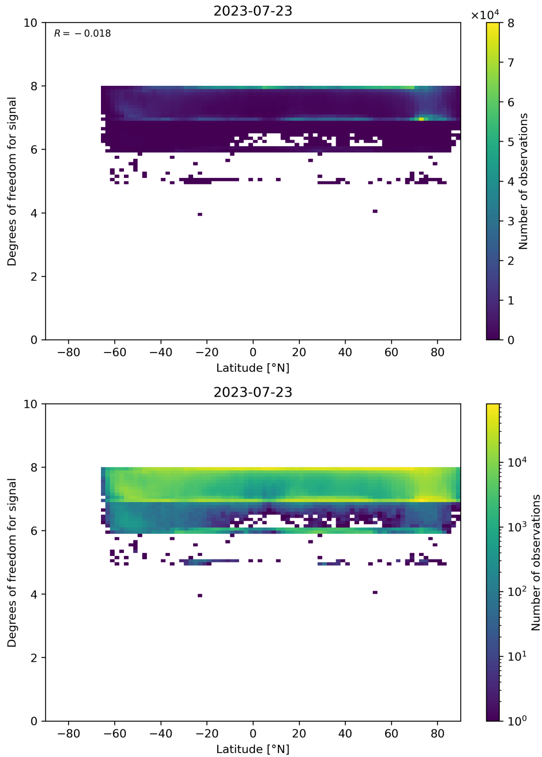
Figure 55: Scatter density plot of “Latitude” against “Degrees of freedom for signal” for 2023-07-22 to 2023-07-24.
