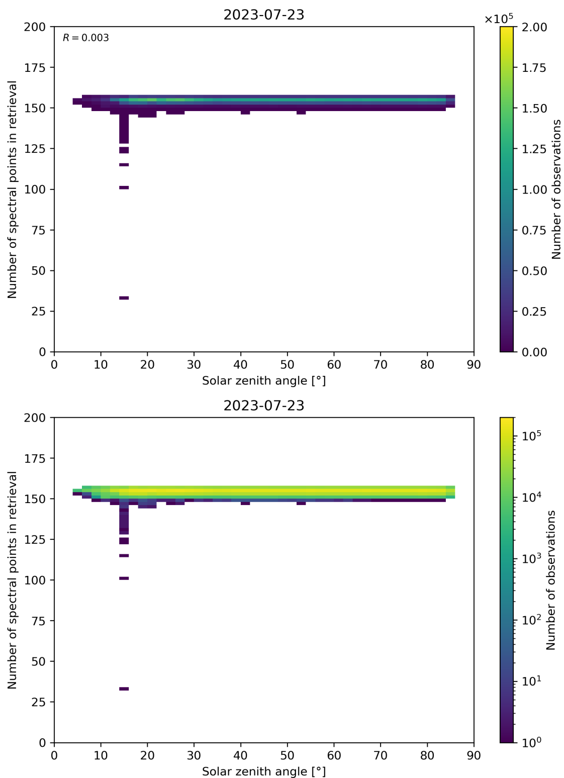
Figure 68: Scatter density plot of “Solar zenith angle” against “Number of spectral points in retrieval” for 2023-07-22 to 2023-07-24.
