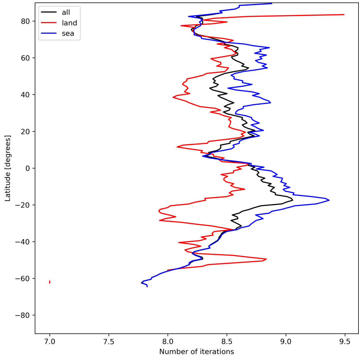
Figure 16: Zonal average of “Number of iterations” for 2023-07-22 to 2023-07-24.
