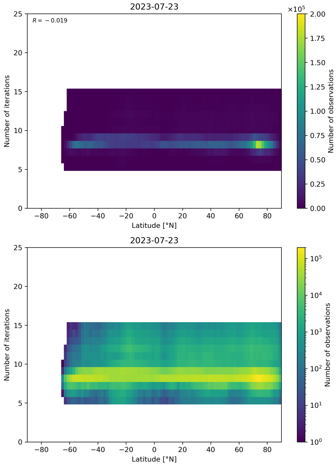
Figure 56: Scatter density plot of “Latitude” against “Number of iterations” for 2023-07-22 to 2023-07-24.
