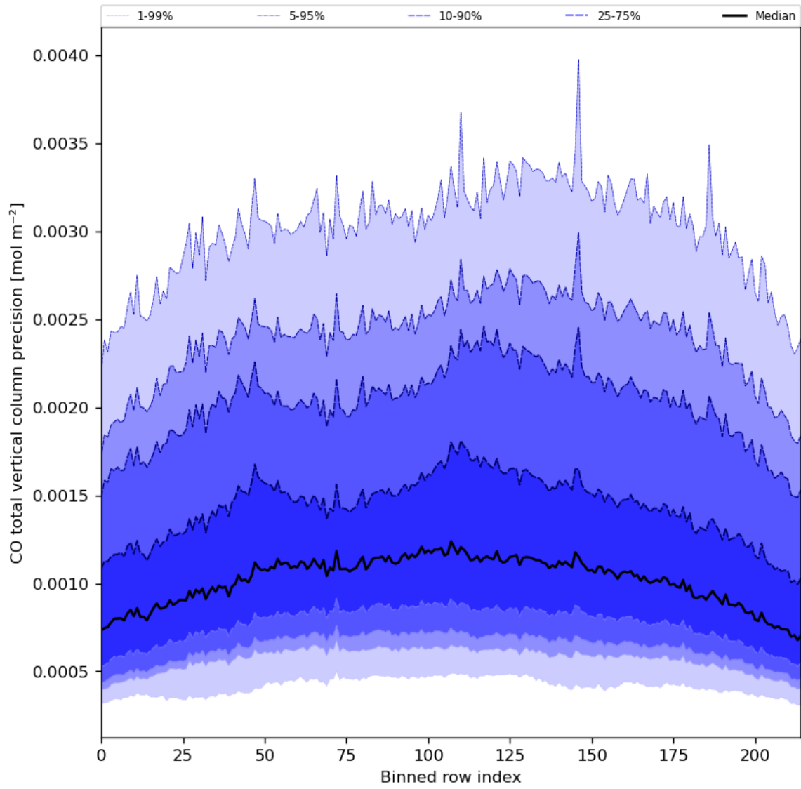
Figure 28: Along track statistics of “CO total vertical column precision” for 2023-07-22 to 2023-07-24
