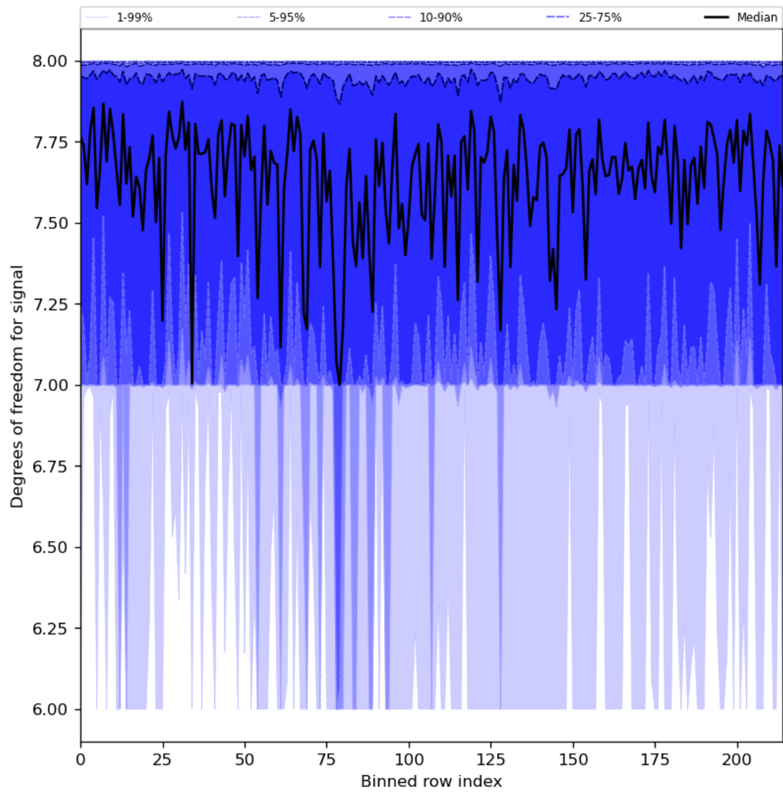
Figure 31: Along track statistics of “Degrees of freedom for signal” for 2023-07-22 to 2023-07-24
