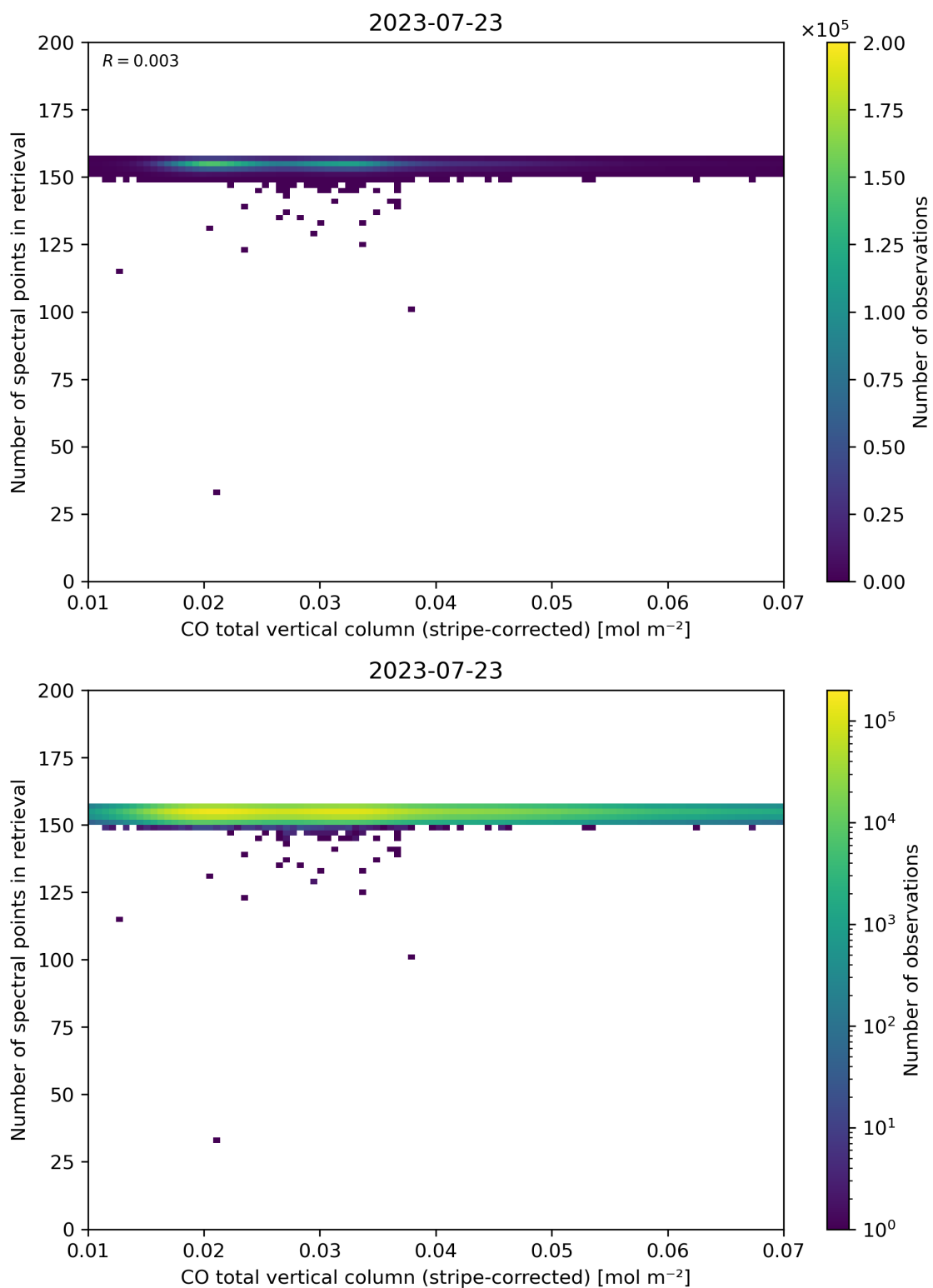
Figure 40: Scatter density plot of “CO total vertical column (stripe-corrected)” against “Number of spectral points in retrieval” for 2023-07-22 to 2023-07-24.
