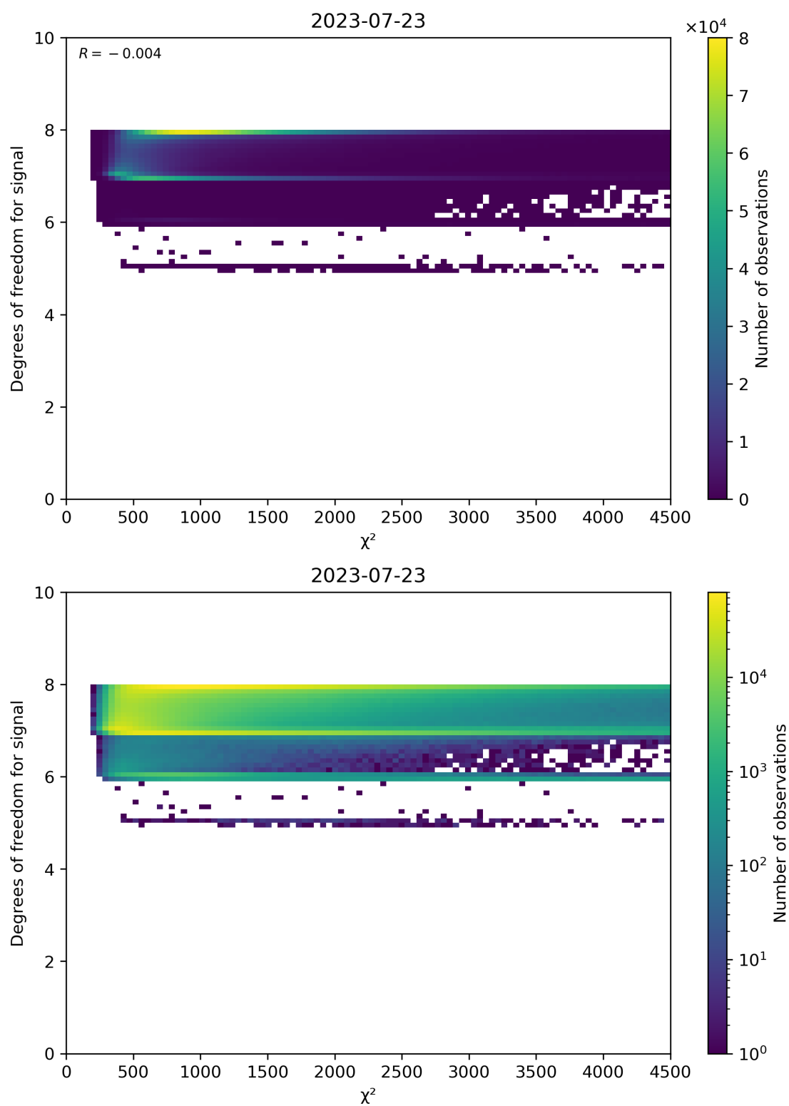
Figure 48: Scatter density plot of “ \chi^2 ” against “Degrees of freedom for signal” for 2023-07-22 to 2023-07-24.
