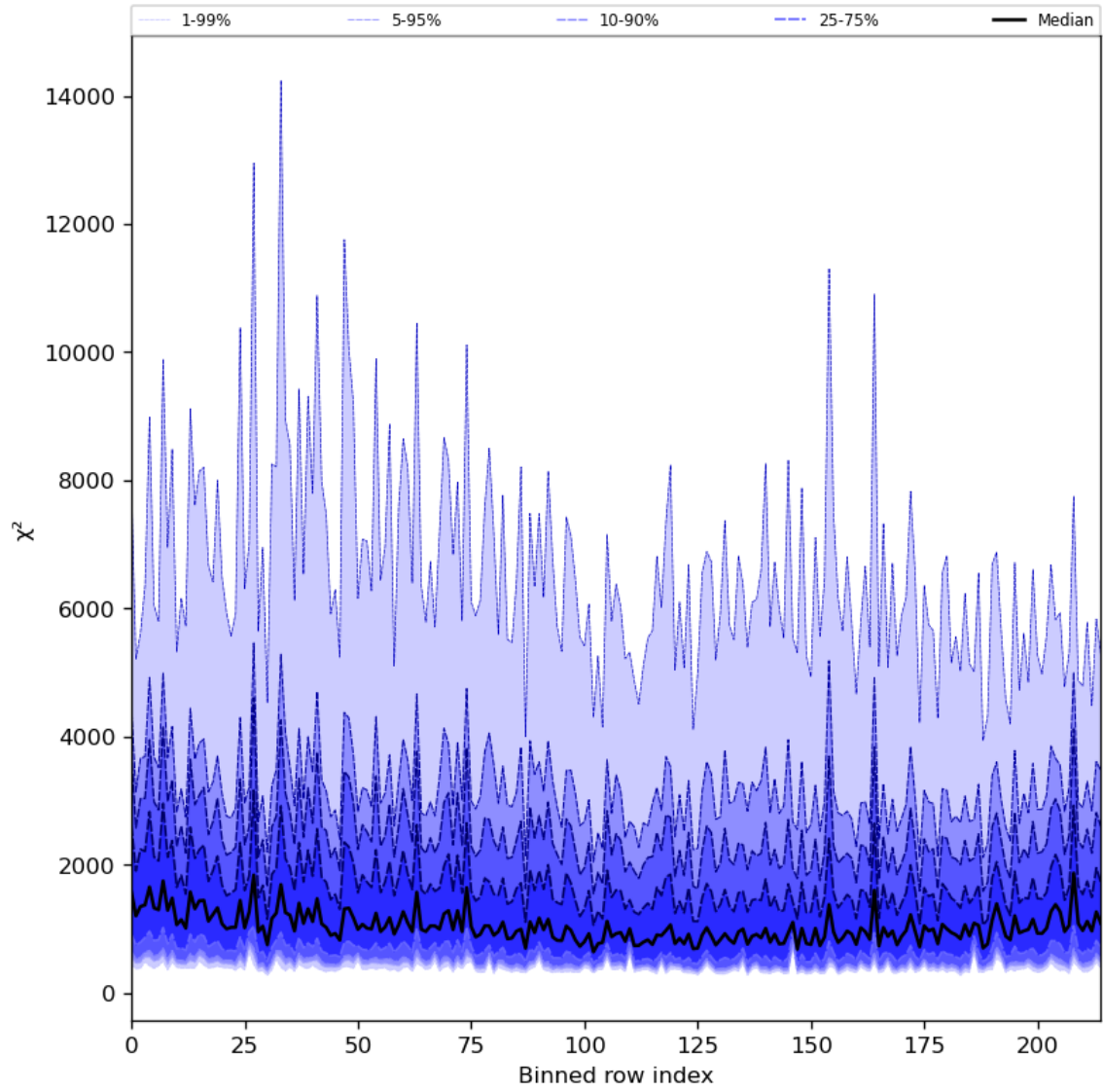
Figure 30: Along track statistics of “ \chi^2 ” for 2023-07-22 to 2023-07-24
