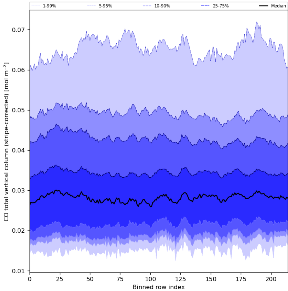
Figure 27: Along track statistics of “CO total vertical column (stripe-corrected)” for 2023-07-22 to 2023-07-24
