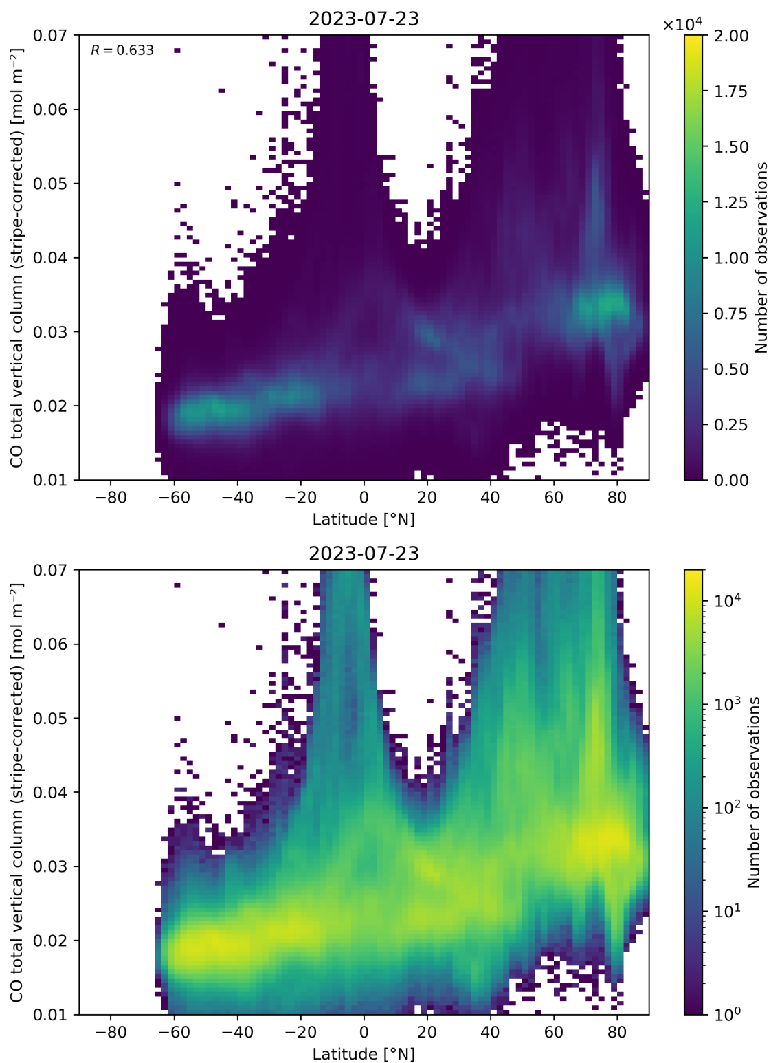
Figure 52: Scatter density plot of “Latitude” against “CO total vertical column (stripe-corrected)” for 2023-07-22 to 2023-07-24.
