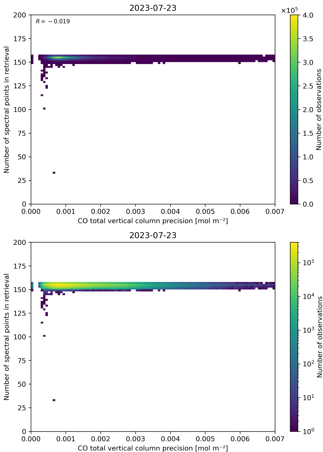
Figure 47: Scatter density plot of “CO total vertical column precision” against “Number of spectral points in retrieval” for 2023-07-22 to 2023-07-24.
