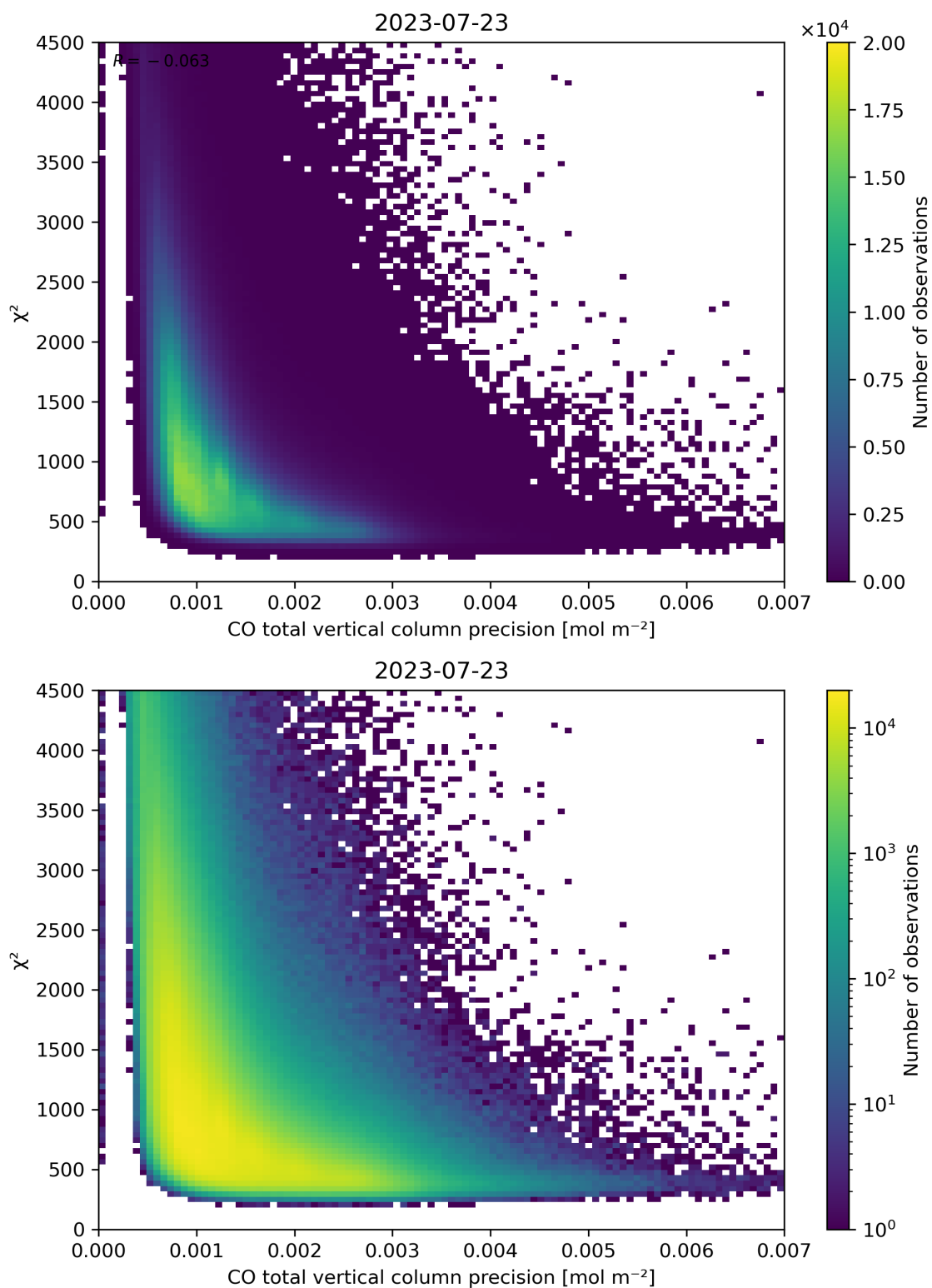
Figure 44: Scatter density plot of “CO total vertical column precision” against “ \chi^2 ” for 2023-07-22 to 2023-07-24.
