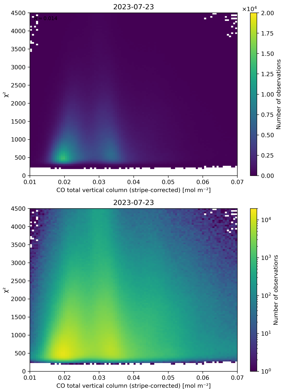
Figure 37: Scatter density plot of “CO total vertical column (stripe-corrected)” against “ \chi^2 ” for 2023-07-22 to 2023-07-24.
