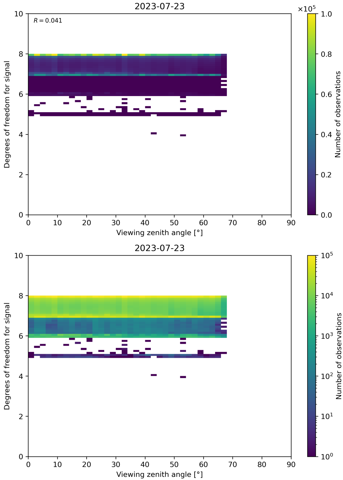
Figure 73: Scatter density plot of “Viewing zenith angle” against “Degrees of freedom for signal” for 2023-07-22 to 2023-07-24.
