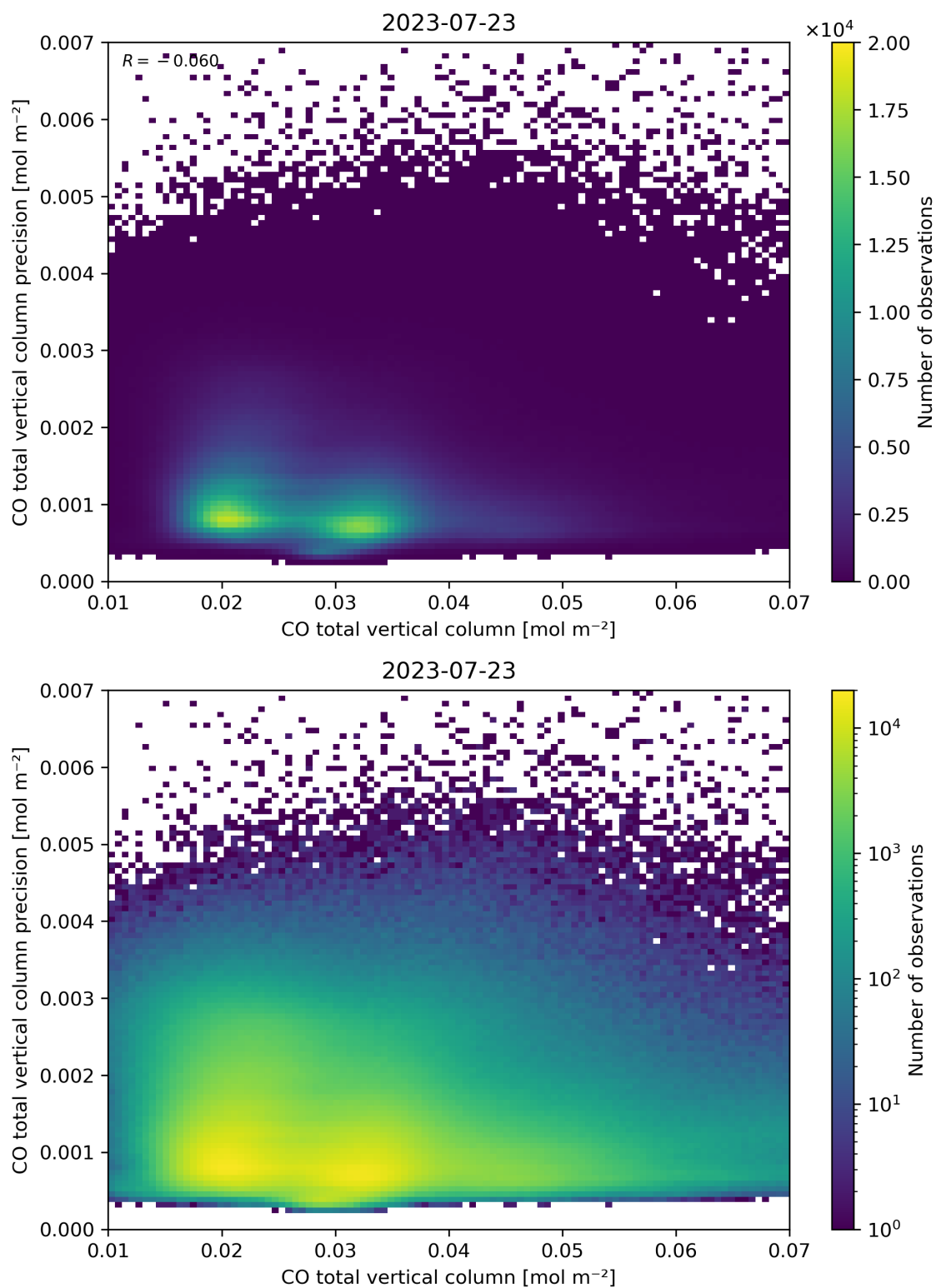
Figure 34: Scatter density plot of “CO total vertical column” against “CO total vertical column precision” for 2023-07-22 to 2023-07-24.
