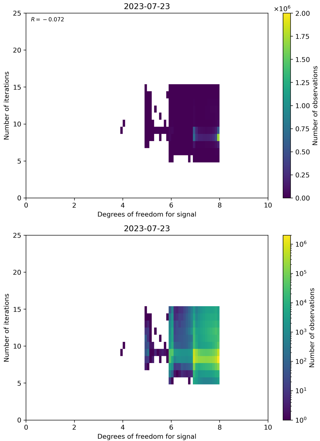
Figure 50: Scatter density plot of “Degrees of freedom for signal” against “Number of iterations” for 2023-07-22 to 2023-07-24.
