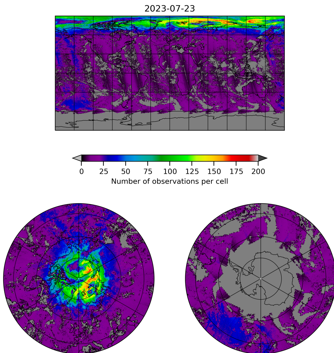
Figure 8: Map of the number of observations for 2023-07-22 to 2023-07-24
