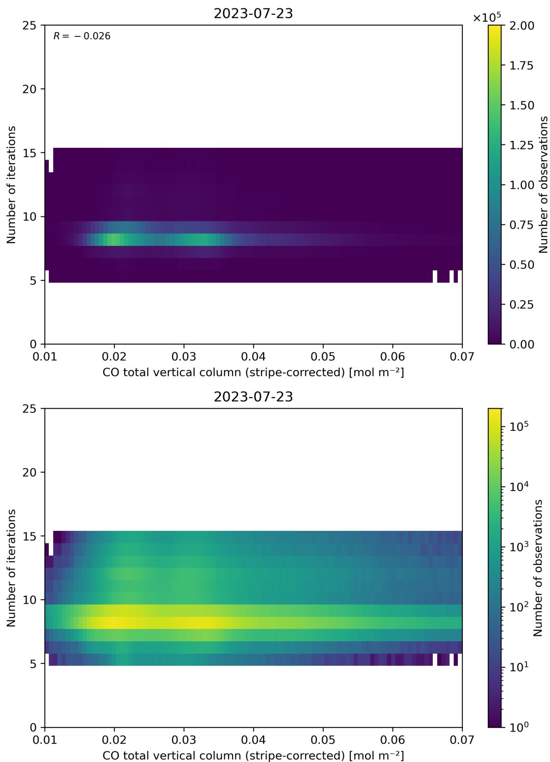
Figure 39: Scatter density plot of “CO total vertical column (stripe-corrected)” against “Number of iterations” for 2023-07-22 to 2023-07-24.
