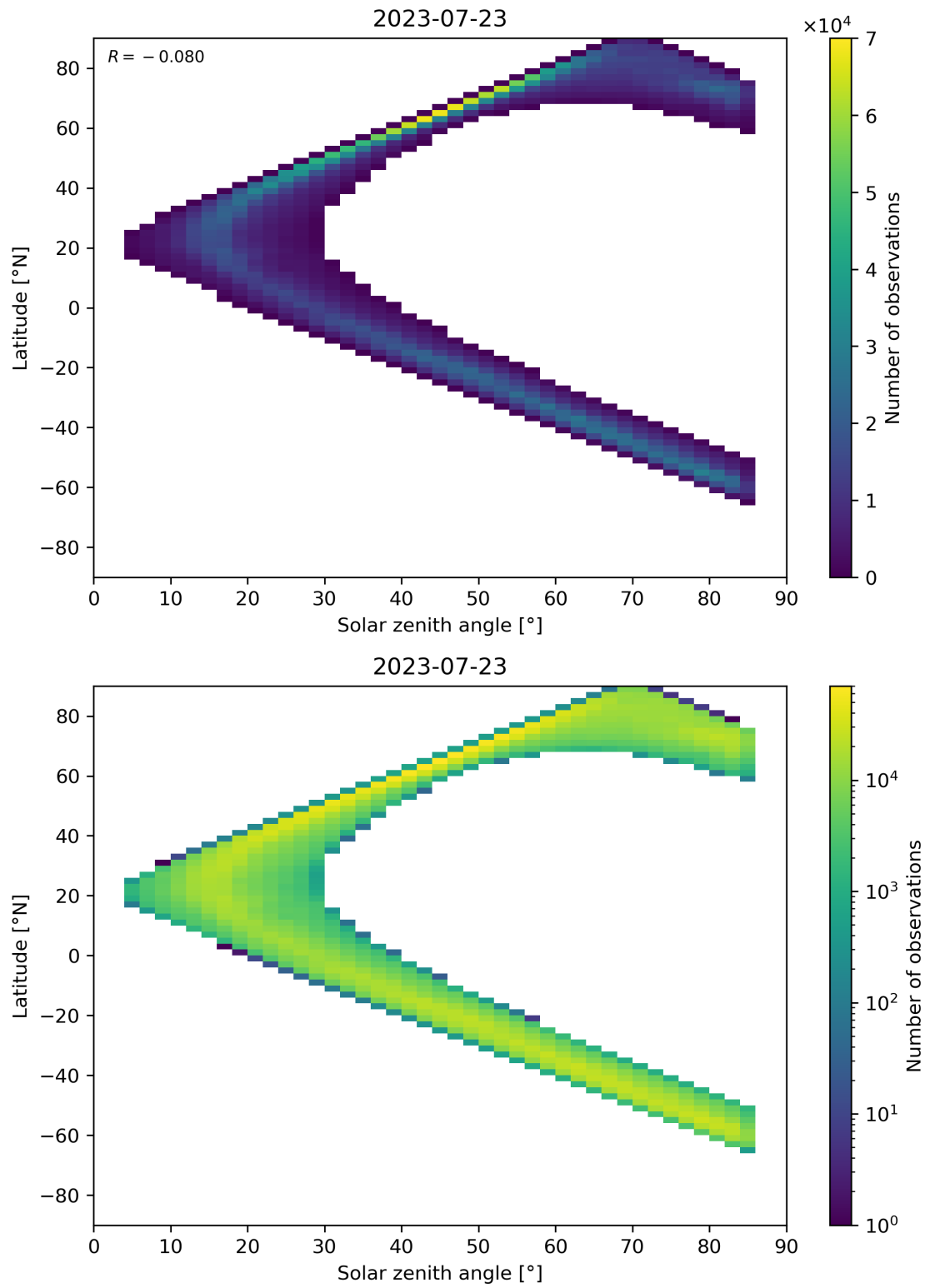
Figure 66: Scatter density plot of “Solar zenith angle” against “Latitude” for 2023-07-22 to 2023-07-24.
