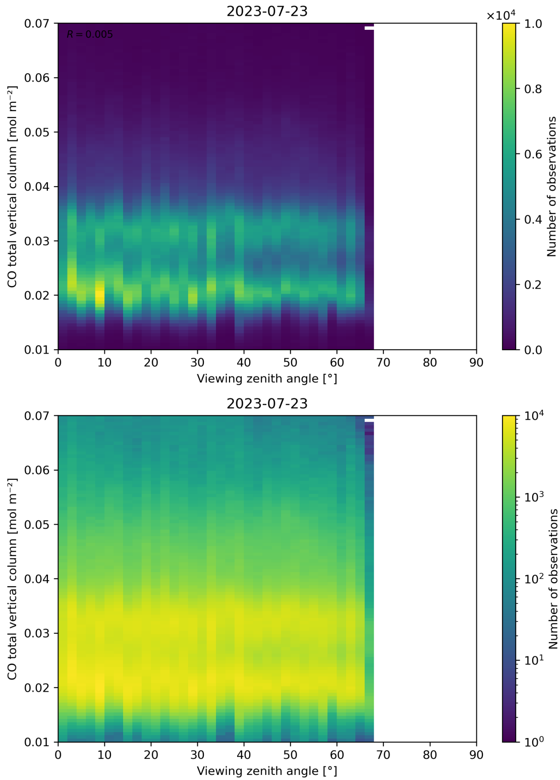
Figure 69: Scatter density plot of “Viewing zenith angle” against “CO total vertical column” for 2023-07-22 to 2023-07-24.
