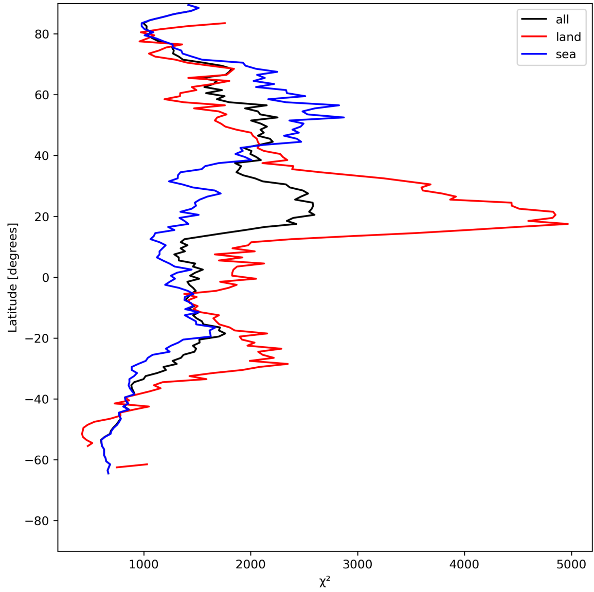
Figure 14: Zonal average of “ \chi^2 ” for 2023-07-22 to 2023-07-24.
