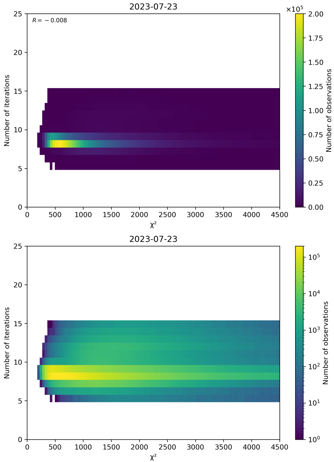
Figure 49: Scatter density plot of “ \chi^2 ” against “Number of iterations” for 2023-07-22 to 2023-07-24.
