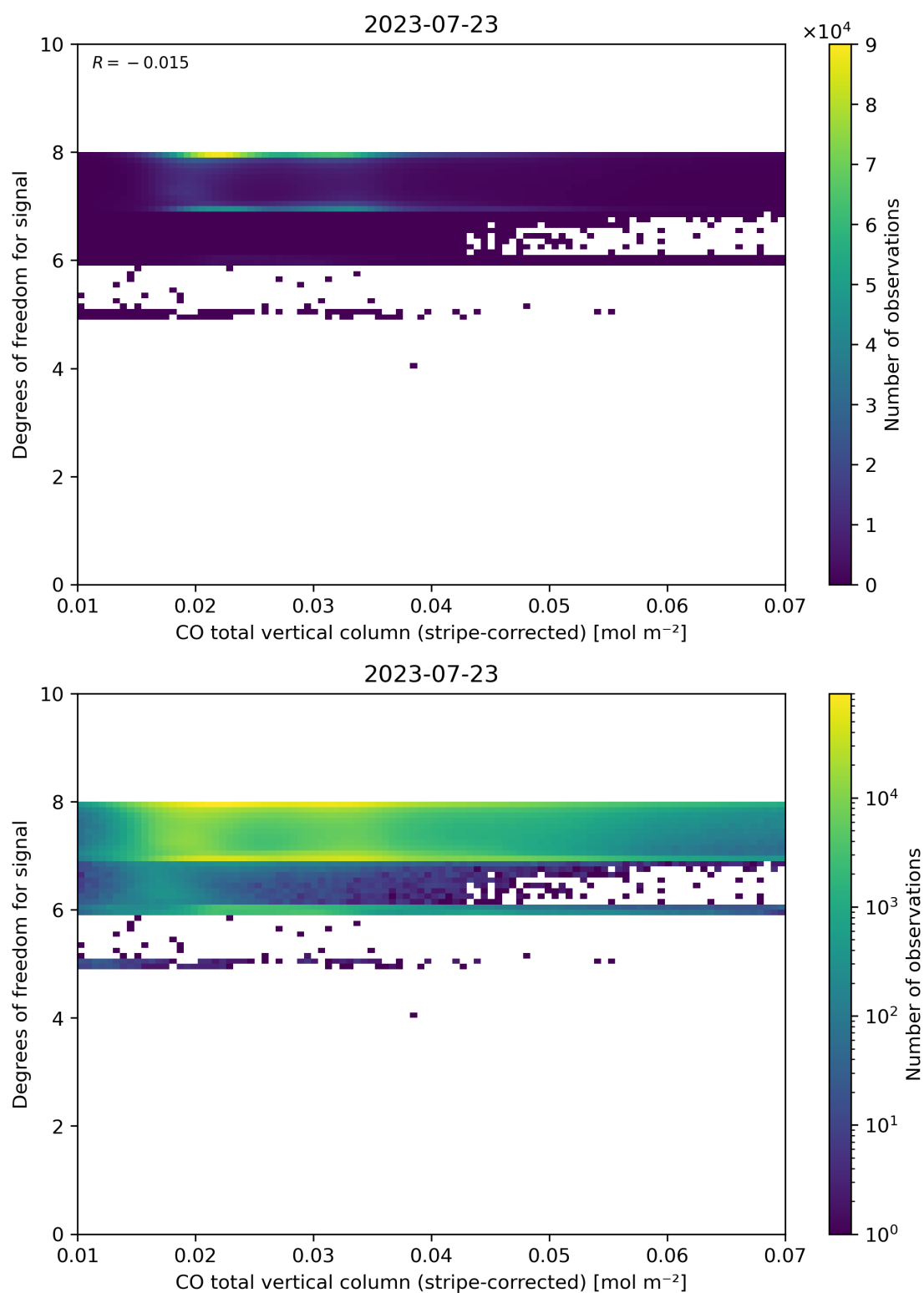
Figure 38: Scatter density plot of “CO total vertical column (stripe-corrected)” against “Degrees of freedom for signal” for 2023-07-22 to 2023-07-24.
