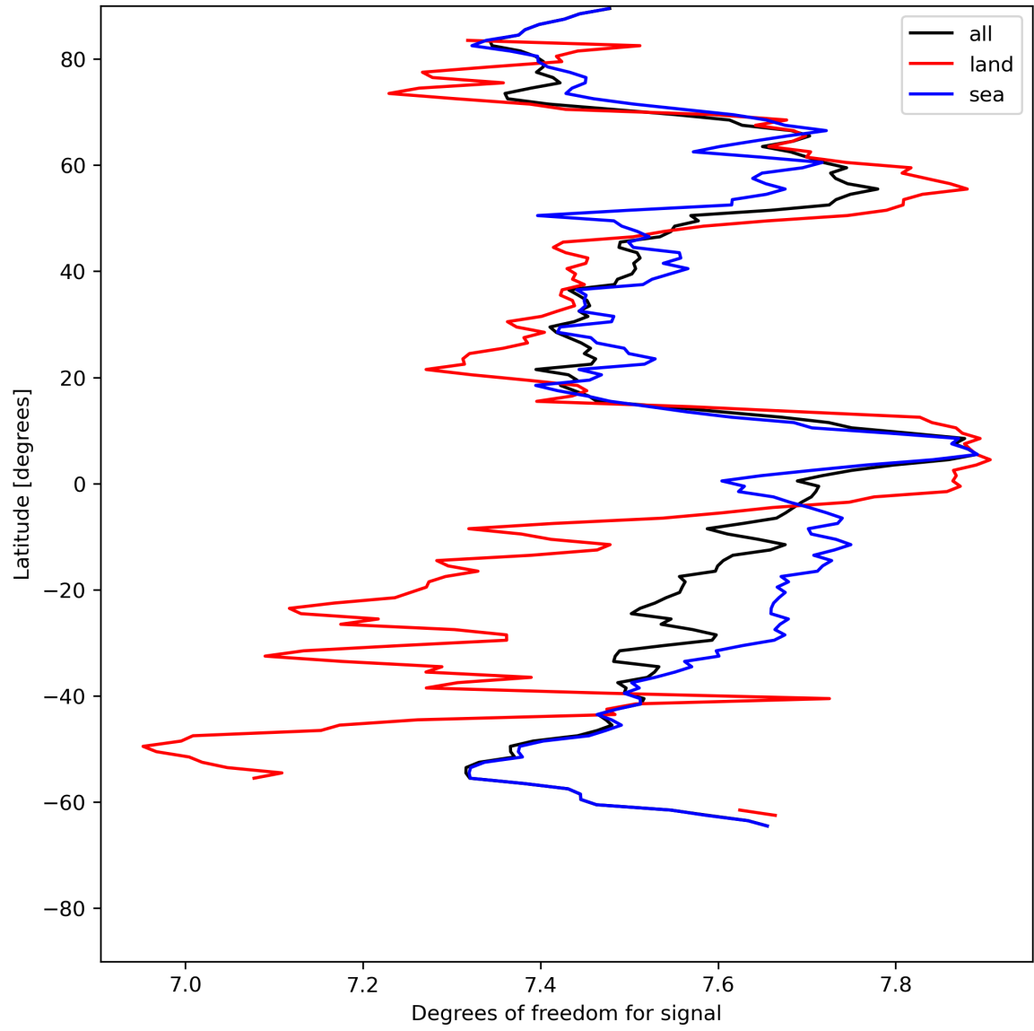
Figure 15: Zonal average of “Degrees of freedom for signal” for 2023-07-22 to 2023-07-24.
