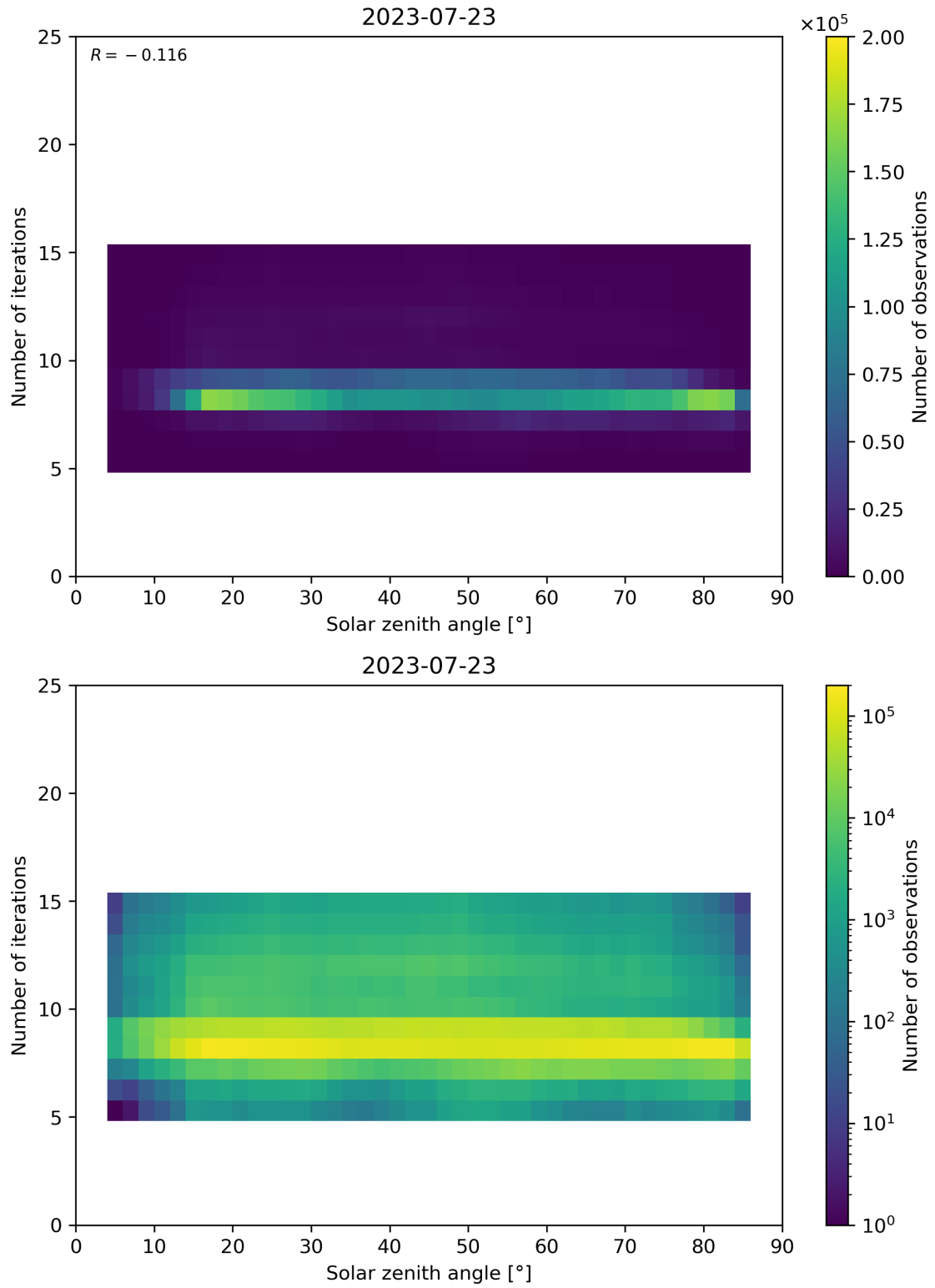
Figure 67: Scatter density plot of “Solar zenith angle” against “Number of iterations” for 2023-07-22 to 2023-07-24.
