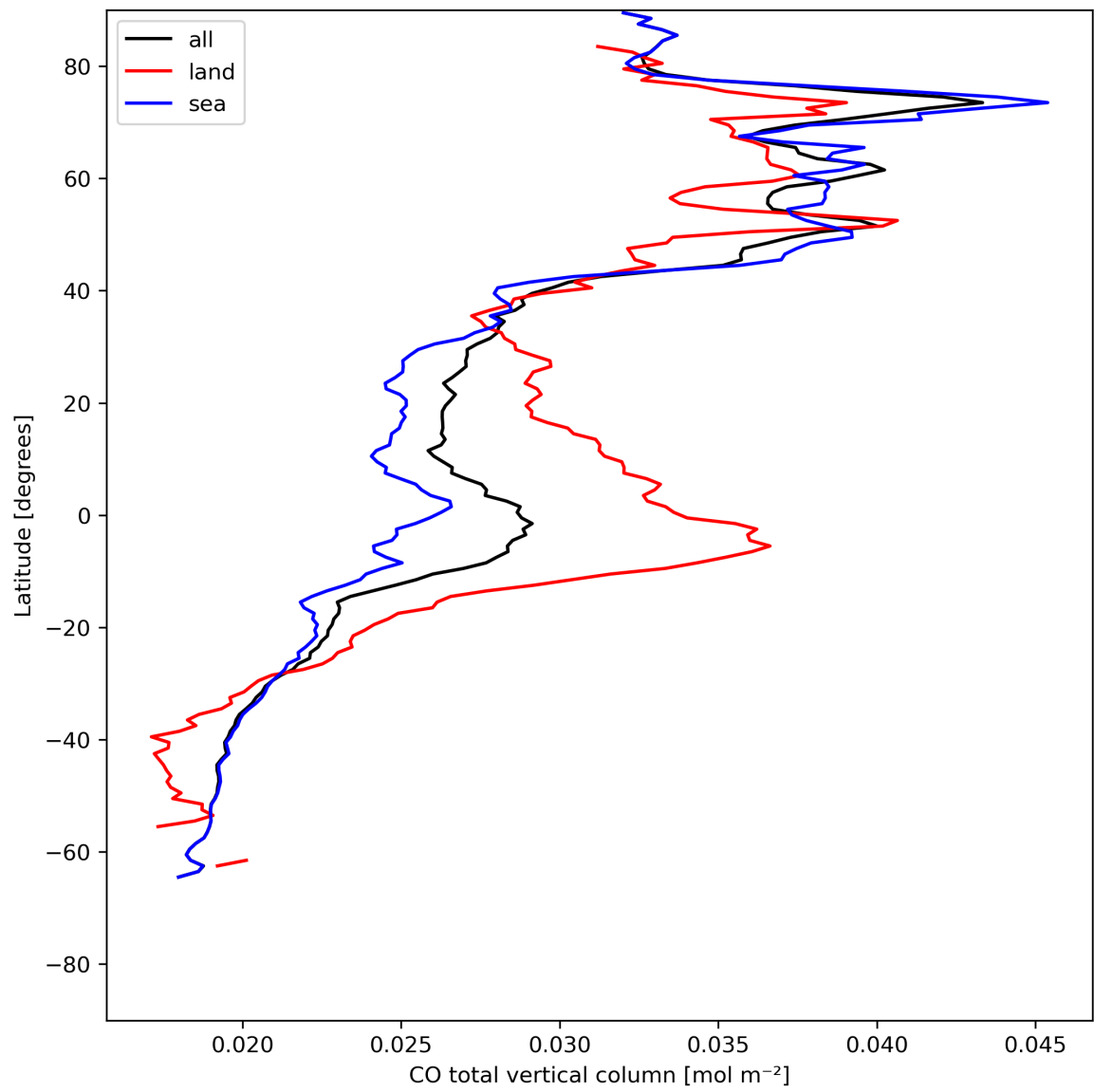
Figure 10: Zonal average of “CO total vertical column” for 2023-07-22 to 2023-07-24.
