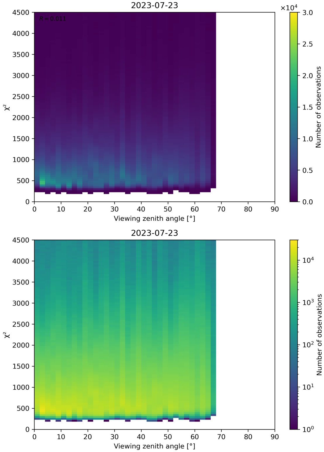
Figure 72: Scatter density plot of “Viewing zenith angle” against “ \chi^2 ” for 2023-07-22 to 2023-07-24.
