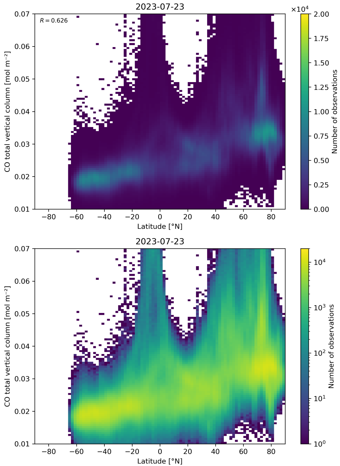
Figure 51: Scatter density plot of “Latitude” against “CO total vertical column” for 2023-07-22 to 2023-07-24.
