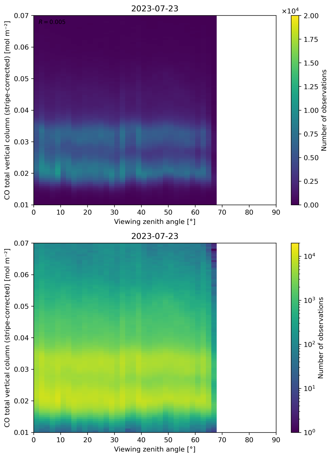
Figure 70: Scatter density plot of “Viewing zenith angle” against “CO total vertical column (stripe-corrected)” for 2023-07-22 to 2023-07-24.
