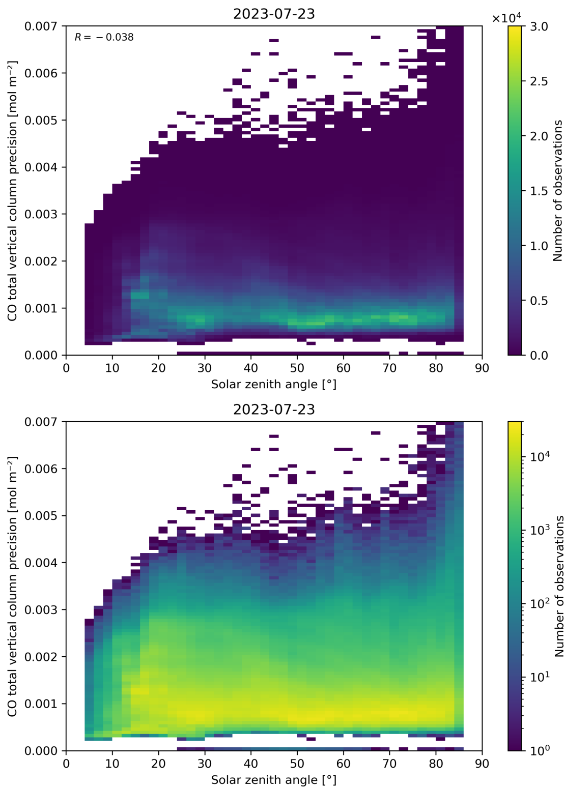
Figure 63: Scatter density plot of “Solar zenith angle” against “CO total vertical column precision” for 2023-07-22 to 2023-07-24.
