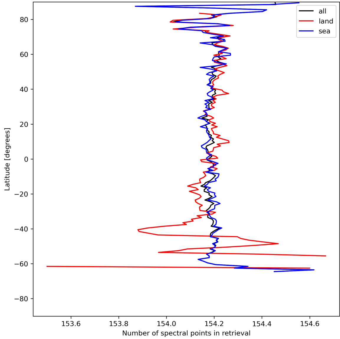
Figure 13: Zonal average of “Number of spectral points in retrieval” for 2023-07-22 to 2023-07-24.
