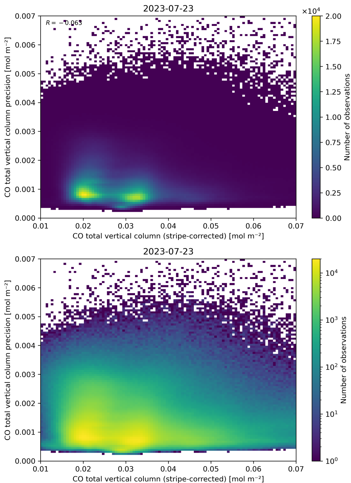
Figure 36: Scatter density plot of “CO total vertical column (stripe-corrected)” against “CO total vertical column precision” for 2023-07-22 to 2023-07-24.
