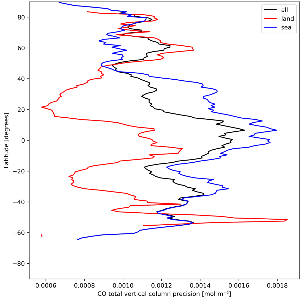
Figure 12: Zonal average of “CO total vertical column precision” for 2023-07-22 to 2023-07-24.
