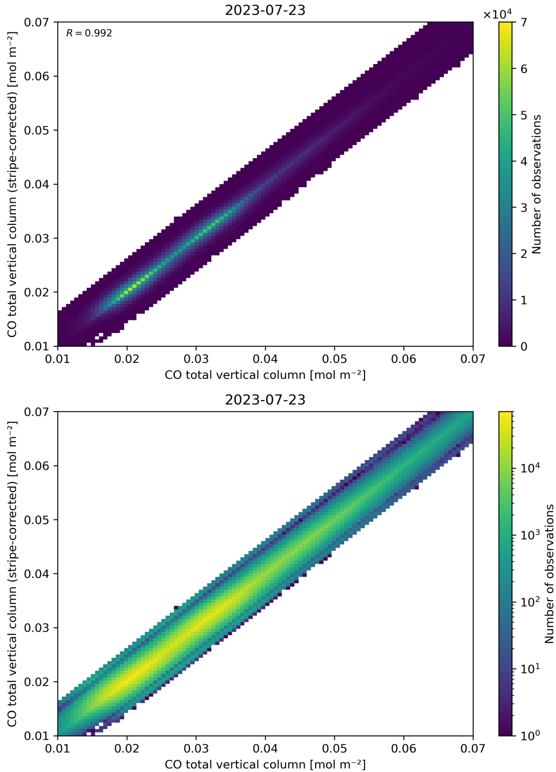
Figure 33: Scatter density plot of “CO total vertical column” against “CO total vertical column (stripe-corrected)” for 2023-07-22 to 2023-07-24.
