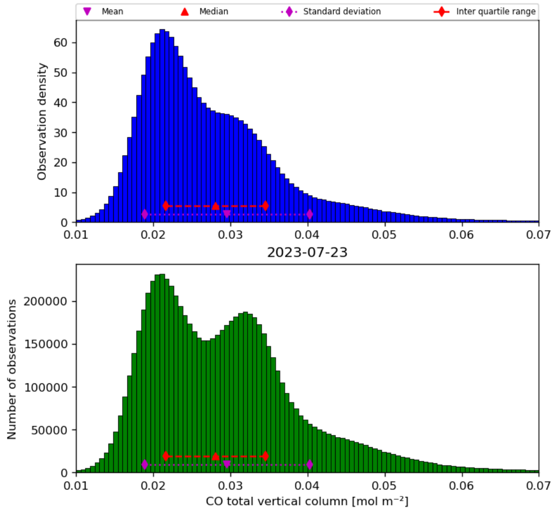
Figure 18: Histogram of “CO total vertical column” for 2023-07-22 to 2023-07-24
