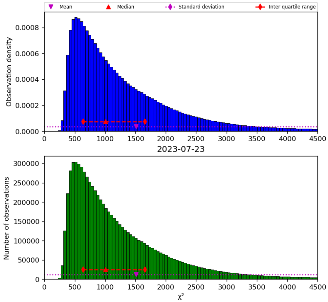
Figure 22: Histogram of “ \chi^2 ” for 2023-07-22 to 2023-07-24
