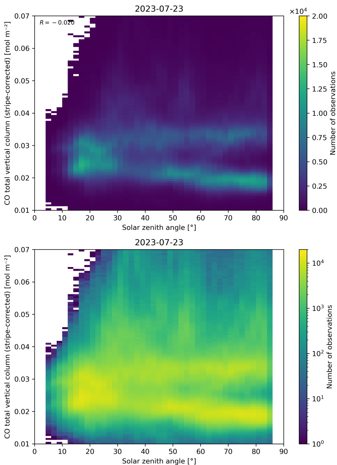
Figure 62: Scatter density plot of “Solar zenith angle” against “CO total vertical column (stripe-corrected)” for 2023-07-22 to 2023-07-24.
