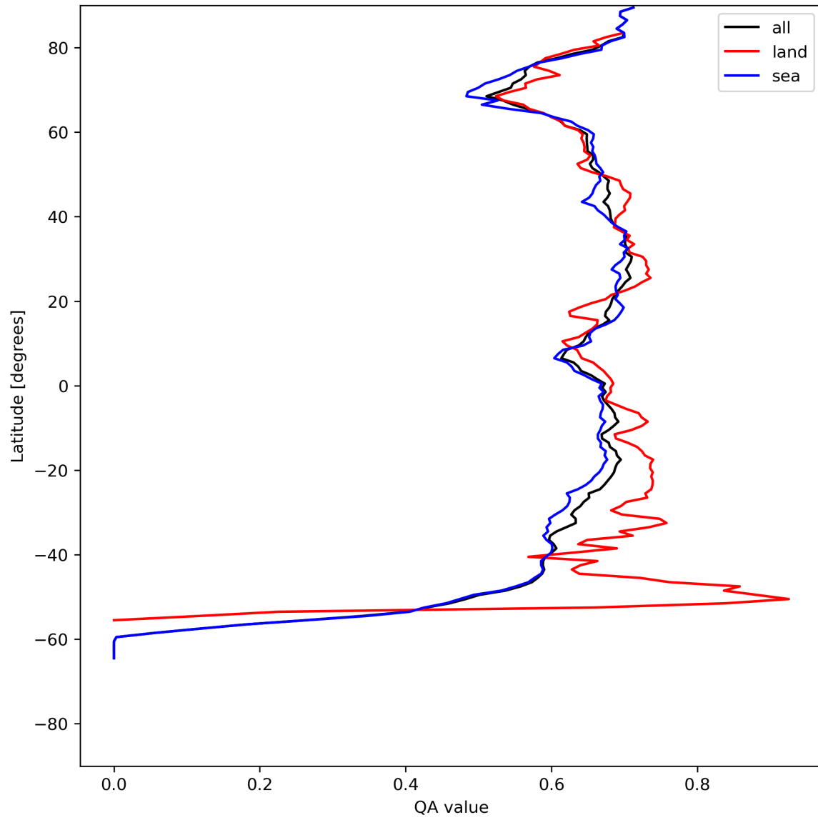
Figure 9: Zonal average of “QA value” for 2023-07-22 to 2023-07-24.
