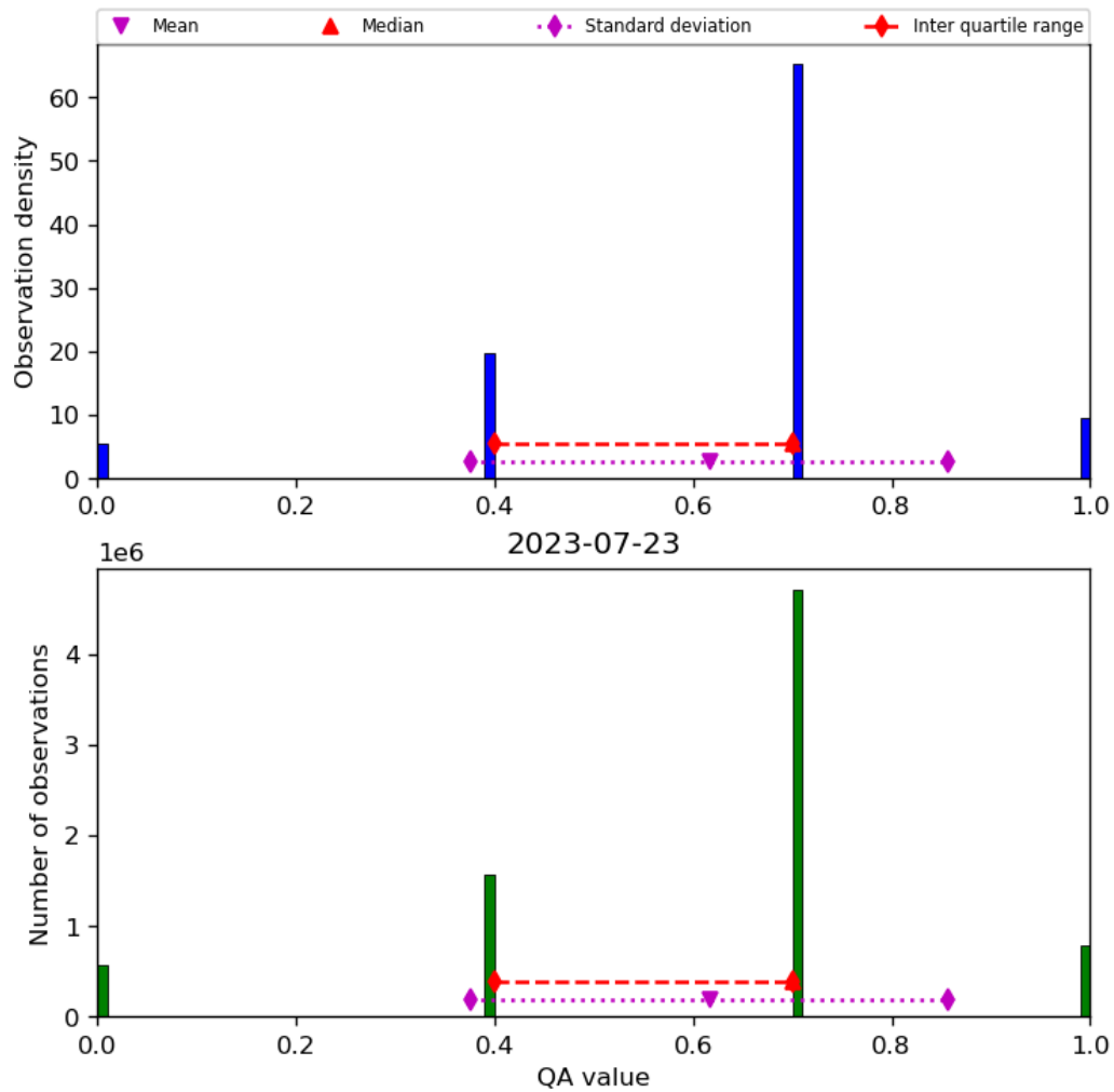
Figure 17: Histogram of “QA value” for 2023-07-22 to 2023-07-24
