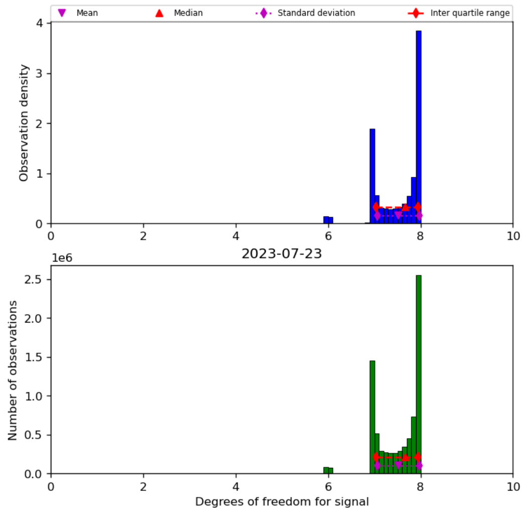
Figure 23: Histogram of “Degrees of freedom for signal” for 2023-07-22 to 2023-07-24
