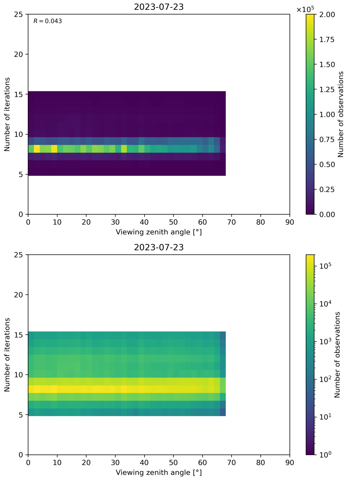
Figure 75: Scatter density plot of “Viewing zenith angle” against “Number of iterations” for 2023-07-22 to 2023-07-24.
