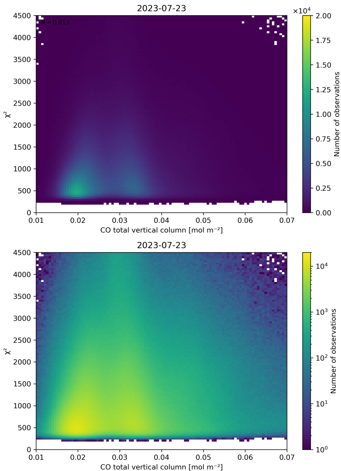
Figure 35: Scatter density plot of “CO total vertical column” against “ \chi^2 ” for 2023-07-22 to 2023-07-24.
