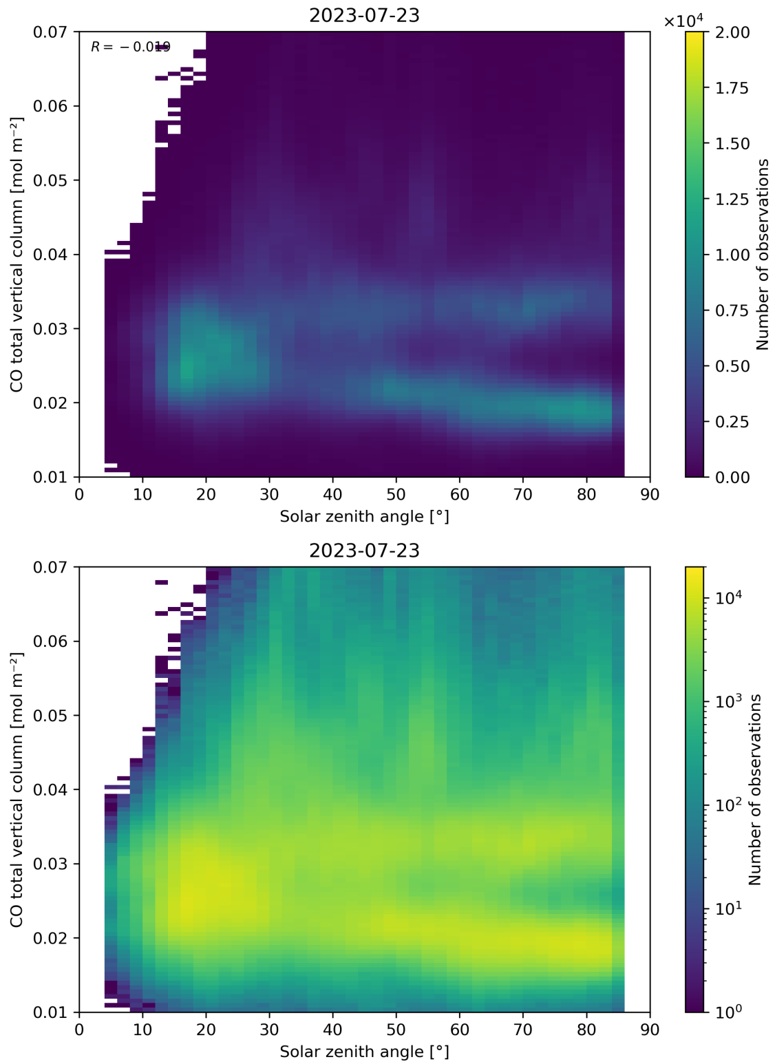
Figure 61: Scatter density plot of “Solar zenith angle” against “CO total vertical column” for 2023-07-22 to 2023-07-24.
