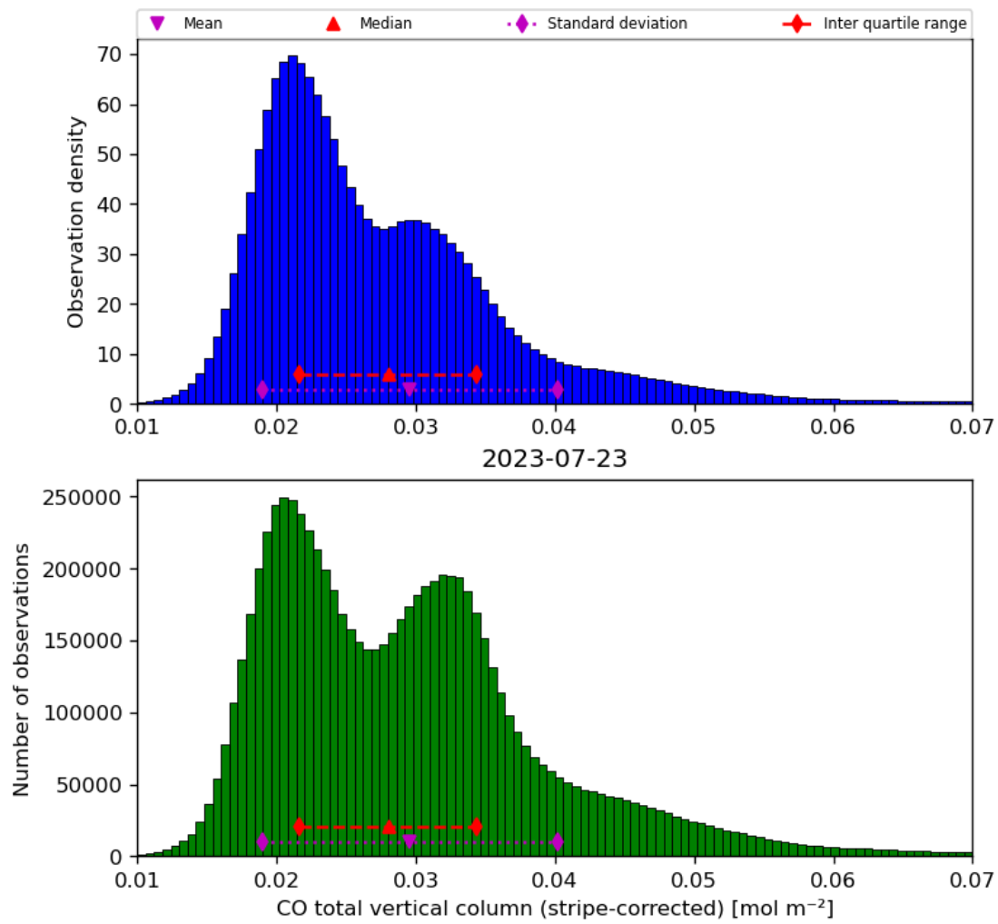
Figure 19: Histogram of “CO total vertical column (stripe-corrected)” for 2023-07-22 to 2023-07-24
