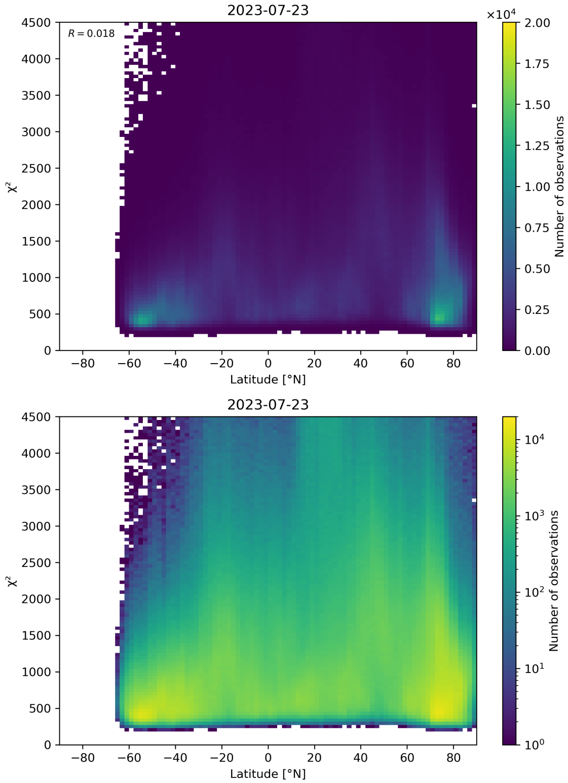
Figure 54: Scatter density plot of “Latitude” against “ \chi^2 ” for 2023-07-22 to 2023-07-24.
