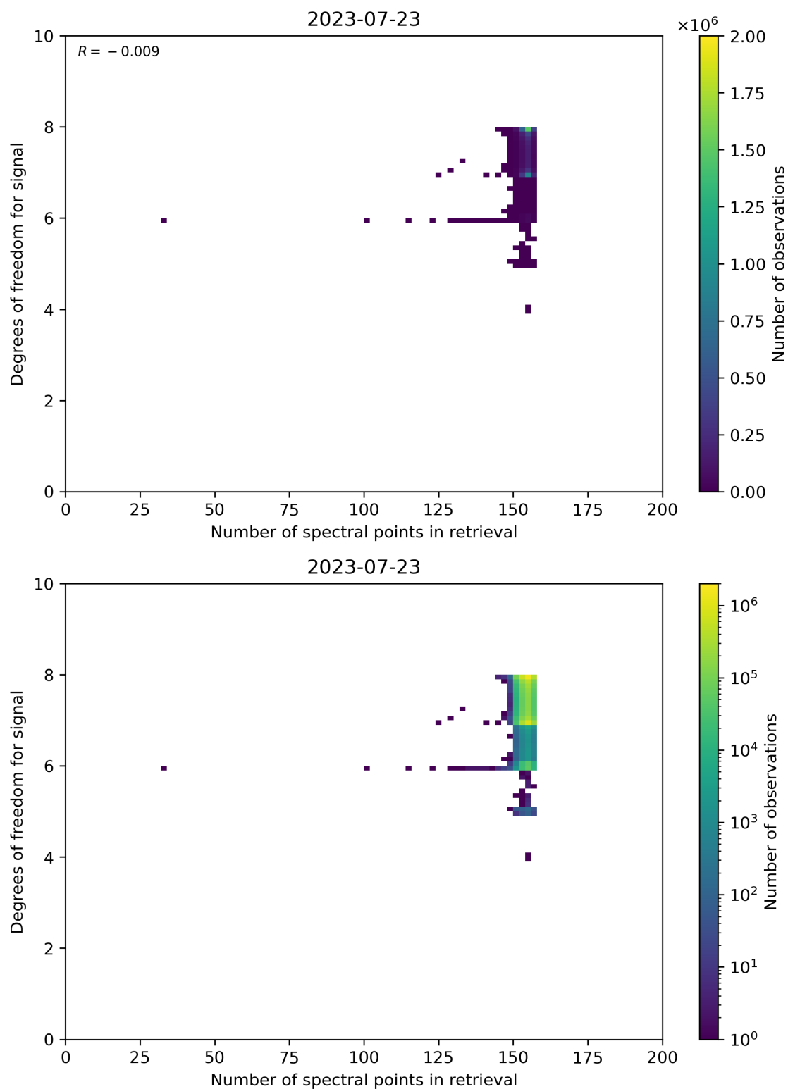
Figure 59: Scatter density plot of “Number of spectral points in retrieval” against “Degrees of freedom for signal” for 2023-07-22 to 2023-07-24.
