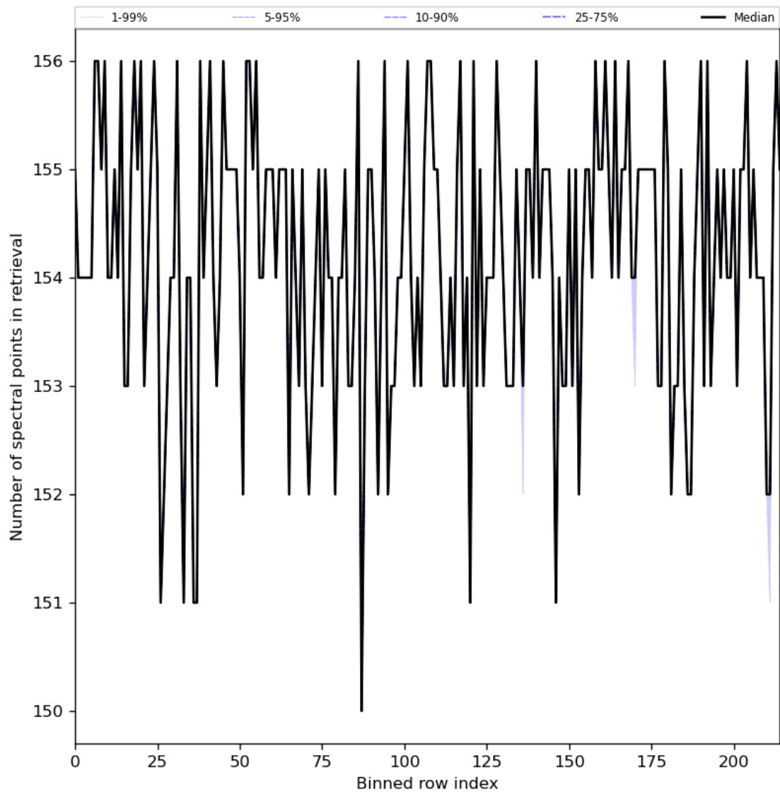
Figure 29: Along track statistics of “Number of spectral points in retrieval” for 2023-07-22 to 2023-07-24
