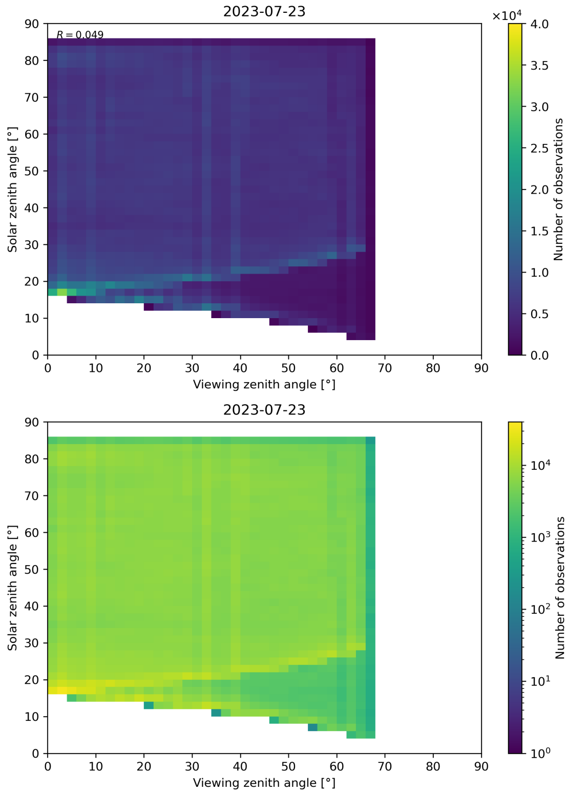
Figure 77: Scatter density plot of “Viewing zenith angle” against “Solar zenith angle” for 2023-07-22 to 2023-07-24.
