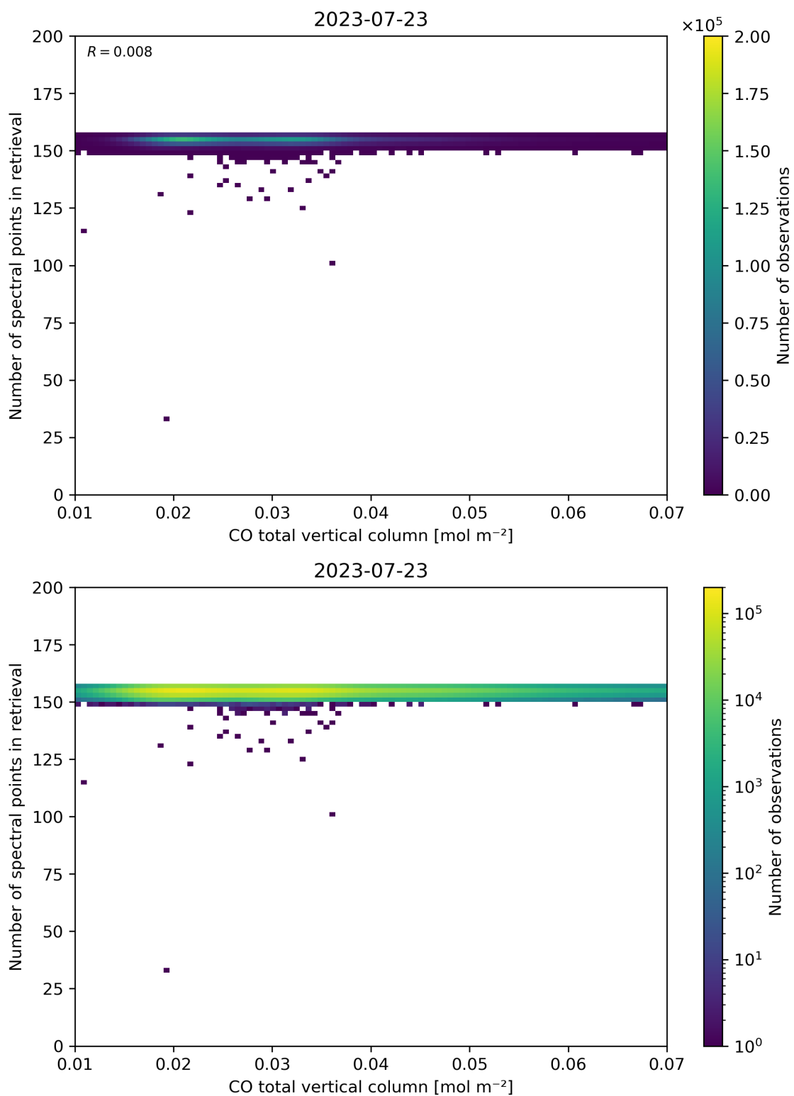
Figure 43: Scatter density plot of “CO total vertical column” against “Number of spectral points in retrieval” for 2023-07-22 to 2023-07-24.
