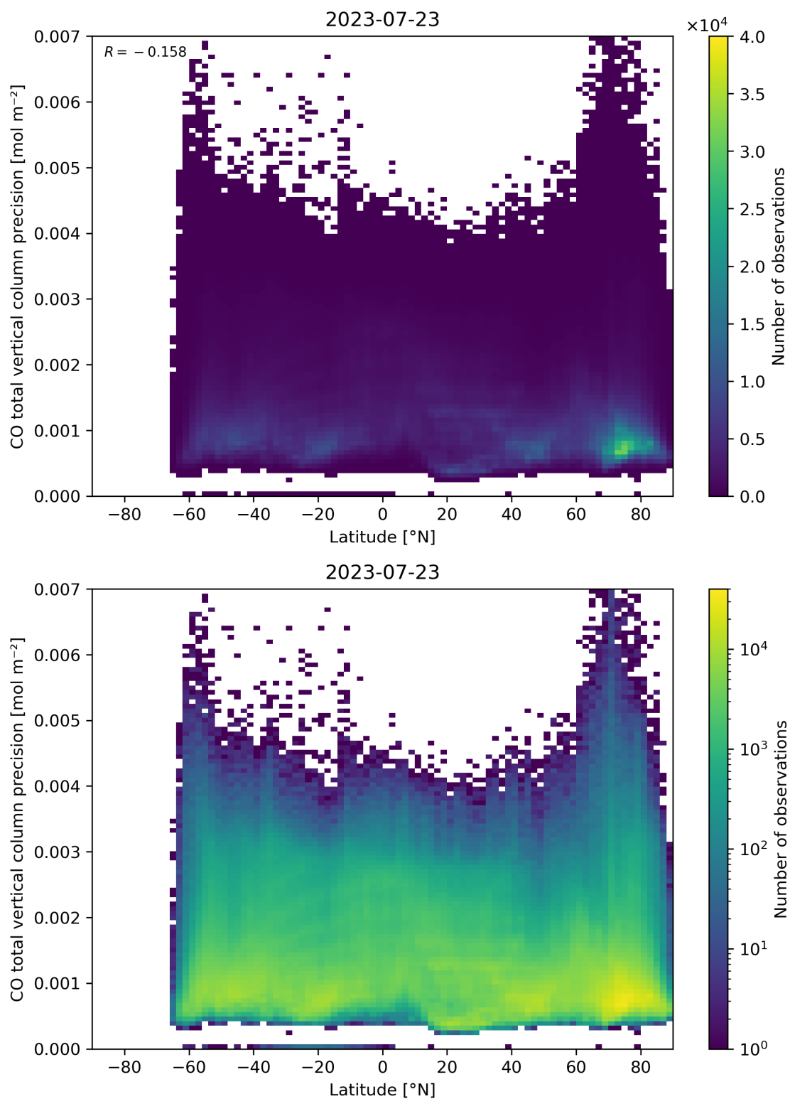
Figure 53: Scatter density plot of “Latitude” against “CO total vertical column precision” for 2023-07-22 to 2023-07-24.
