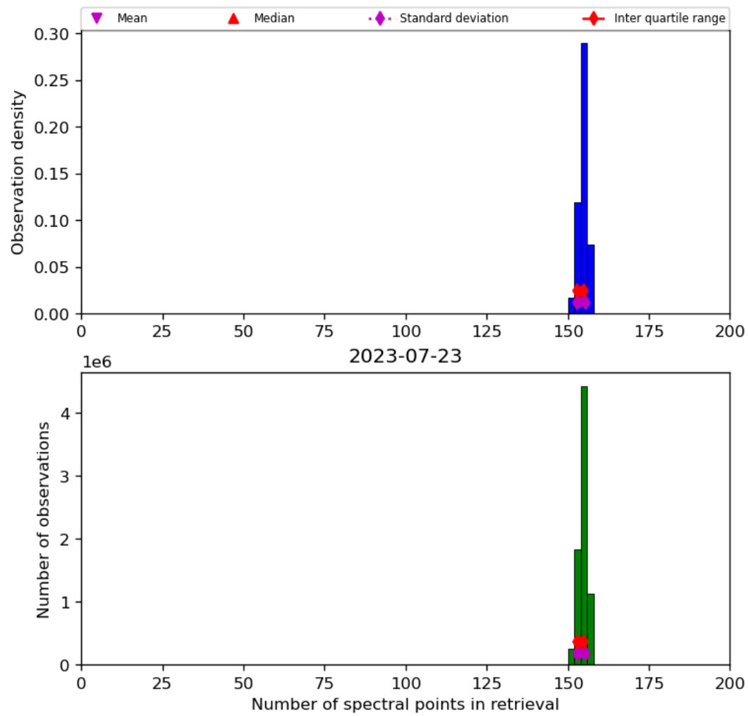
Figure 21: Histogram of “Number of spectral points in retrieval” for 2023-07-22 to 2023-07-24
