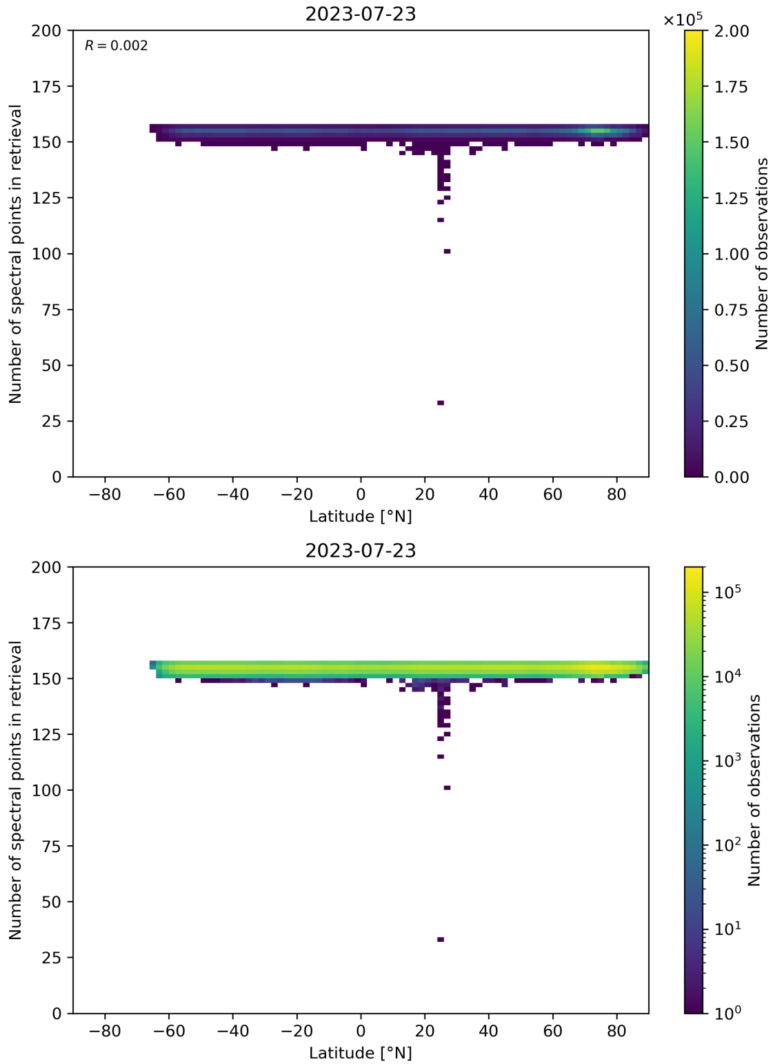
Figure 57: Scatter density plot of “Latitude” against “Number of spectral points in retrieval” for 2023-07-22 to 2023-07-24.
