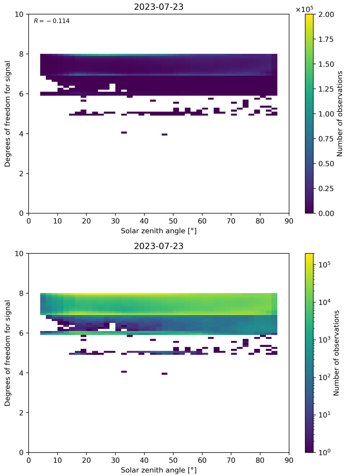
Figure 65: Scatter density plot of “Solar zenith angle” against “Degrees of freedom for signal” for 2023-07-22 to 2023-07-24.
