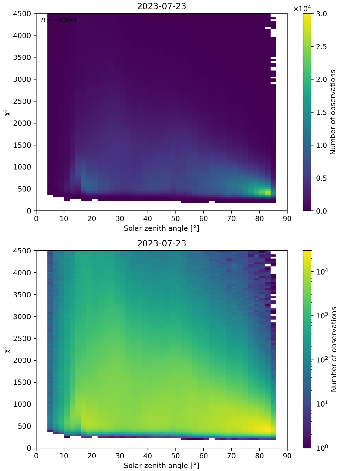
Figure 64: Scatter density plot of “Solar zenith angle” against “ \chi^2 ” for 2023-07-22 to 2023-07-24.
