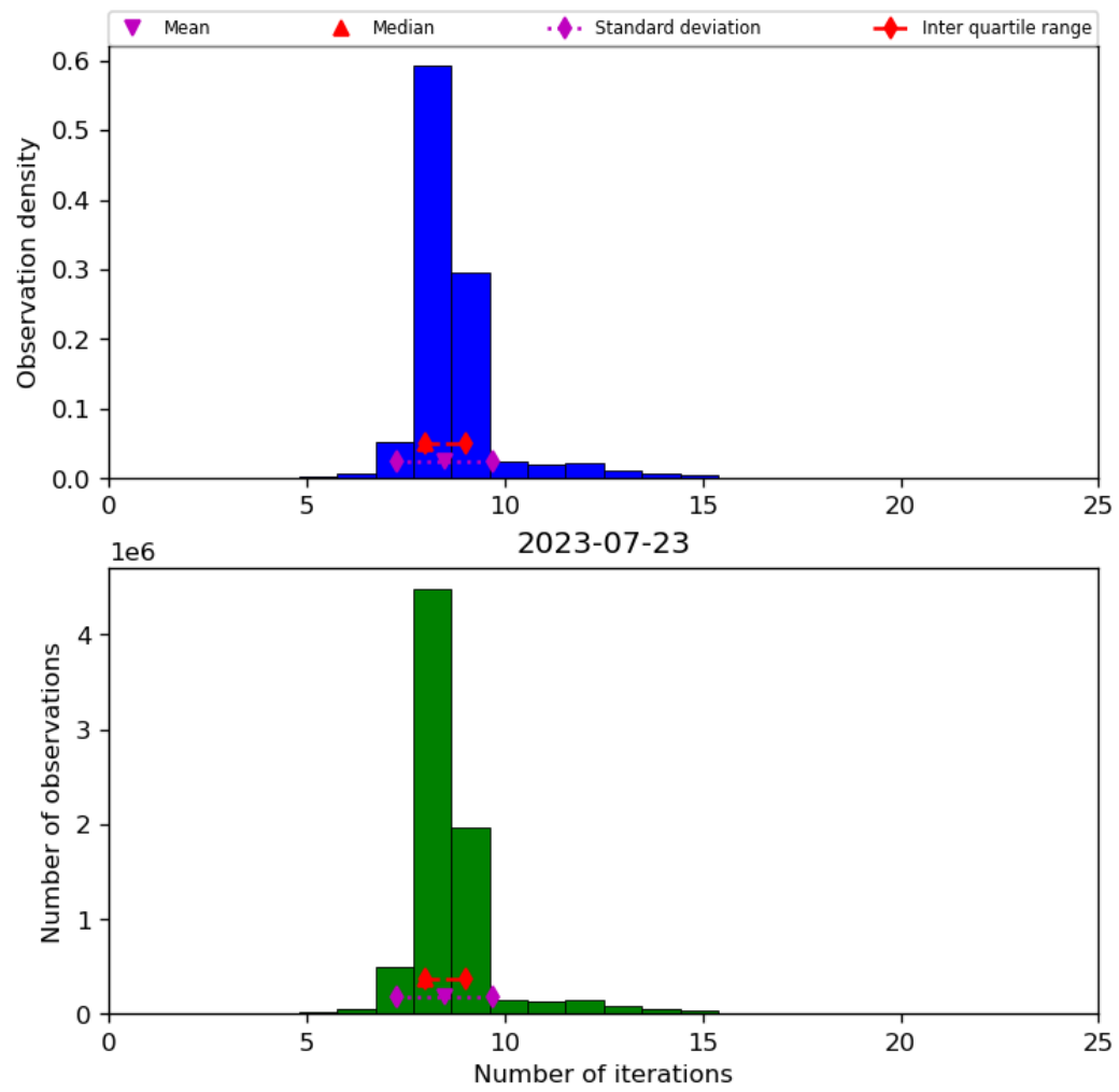
Figure 24: Histogram of “Number of iterations” for 2023-07-22 to 2023-07-24
