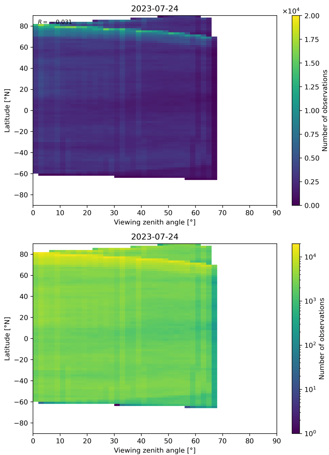
Figure 74: Scatter density plot of “Viewing zenith angle” against “Latitude” for 2023-07-24 to 2023-07-25.
