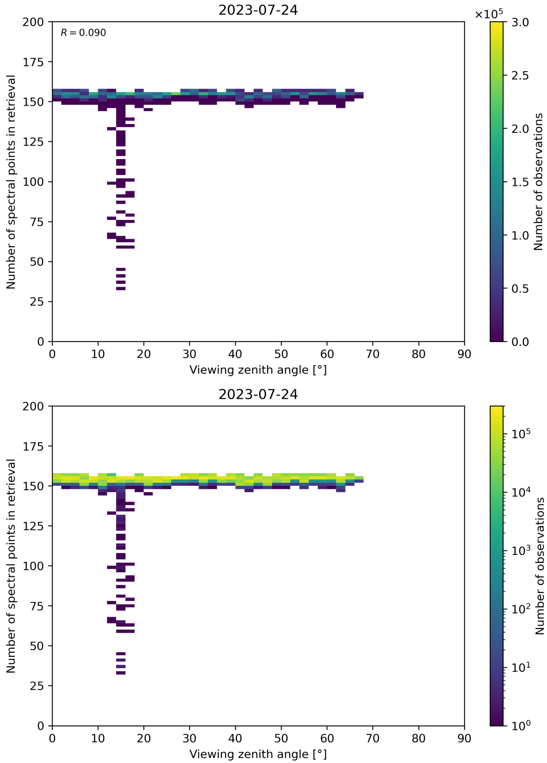
Figure 76: Scatter density plot of “Viewing zenith angle” against “Number of spectral points in retrieval” for 2023-07-24 to 2023-07-25.
