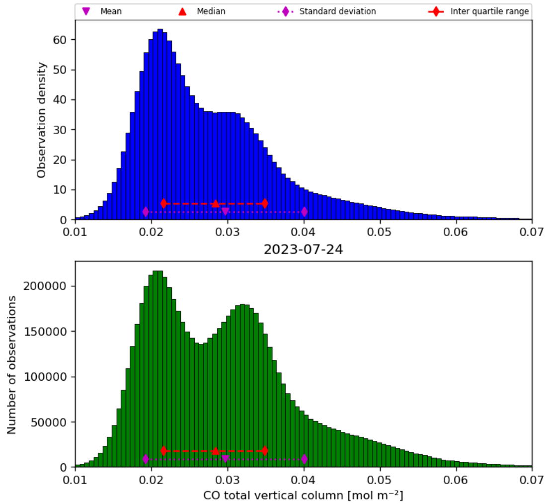
Figure 18: Histogram of “CO total vertical column” for 2023-07-24 to 2023-07-25
