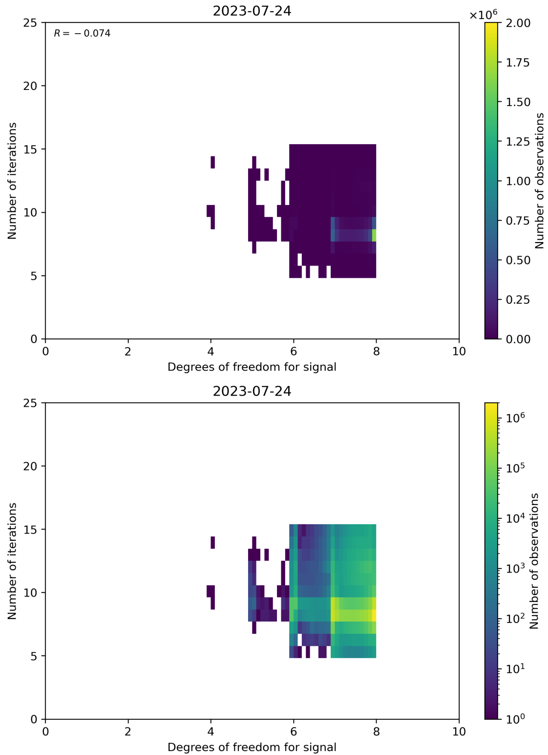
Figure 50: Scatter density plot of “Degrees of freedom for signal” against “Number of iterations” for 2023-07-24 to 2023-07-25.
