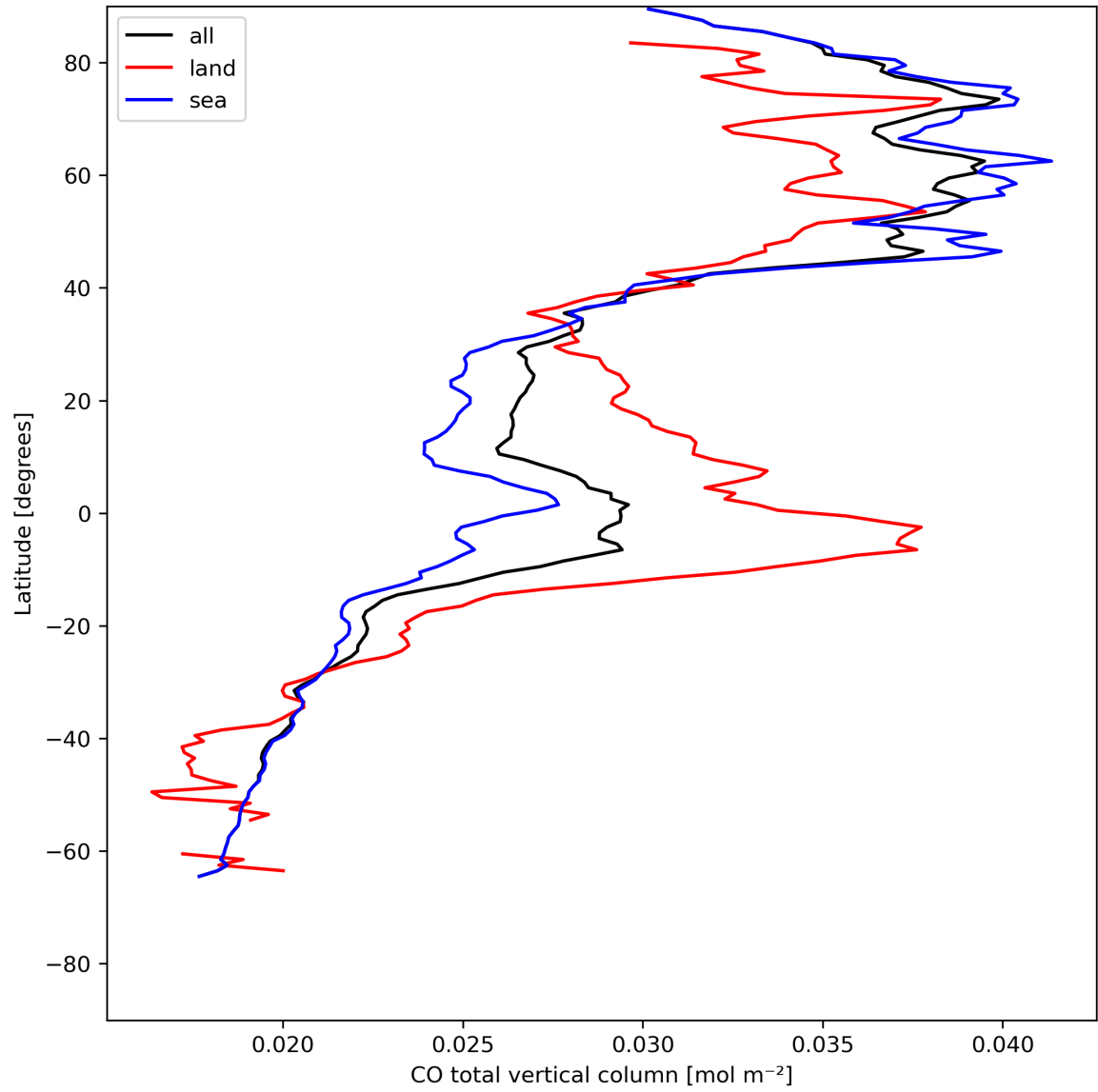
Figure 10: Zonal average of “CO total vertical column” for 2023-07-24 to 2023-07-25.
