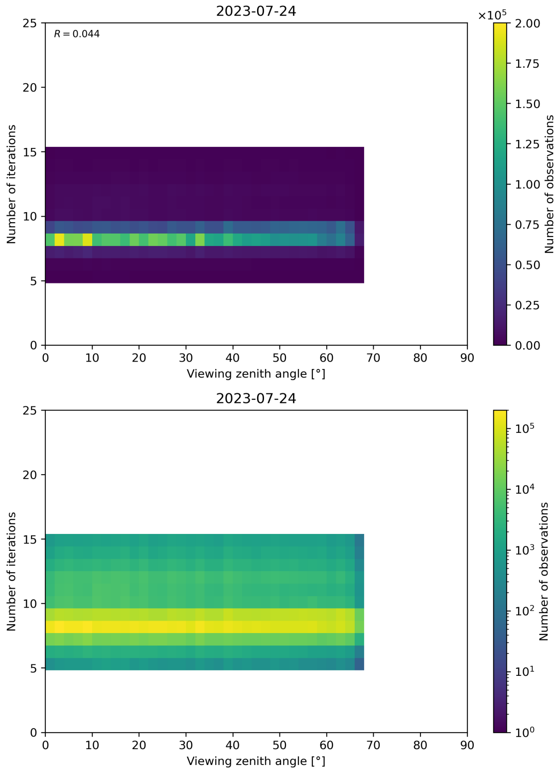
Figure 75: Scatter density plot of “Viewing zenith angle” against “Number of iterations” for 2023-07-24 to 2023-07-25.
