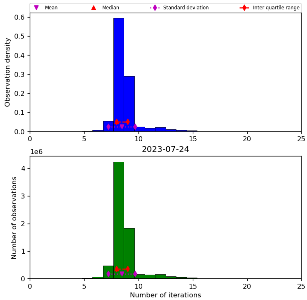
Figure 24: Histogram of “Number of iterations” for 2023-07-24 to 2023-07-25
