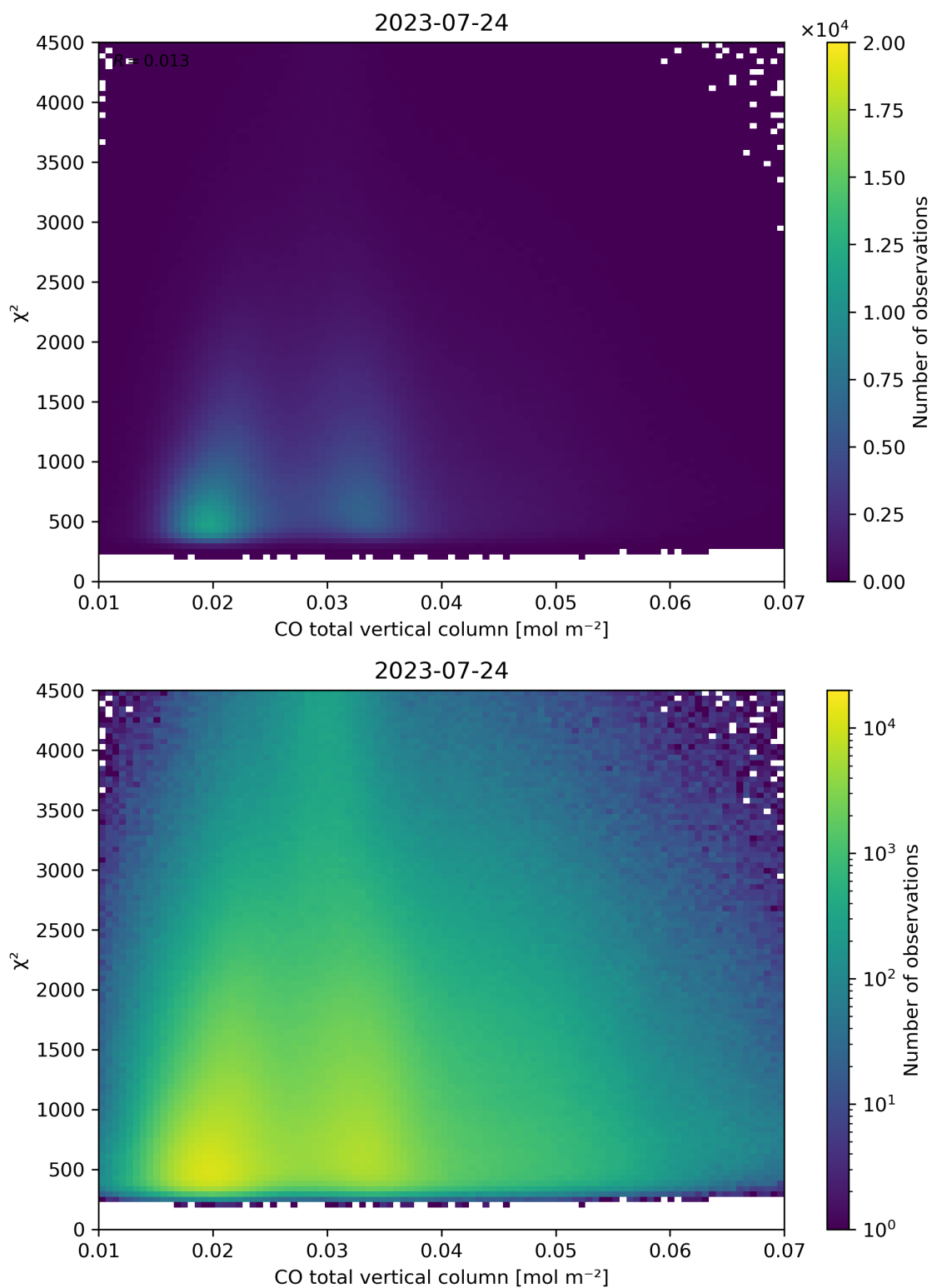
Figure 35: Scatter density plot of “CO total vertical column” against “ \chi^2 ” for 2023-07-24 to 2023-07-25.
