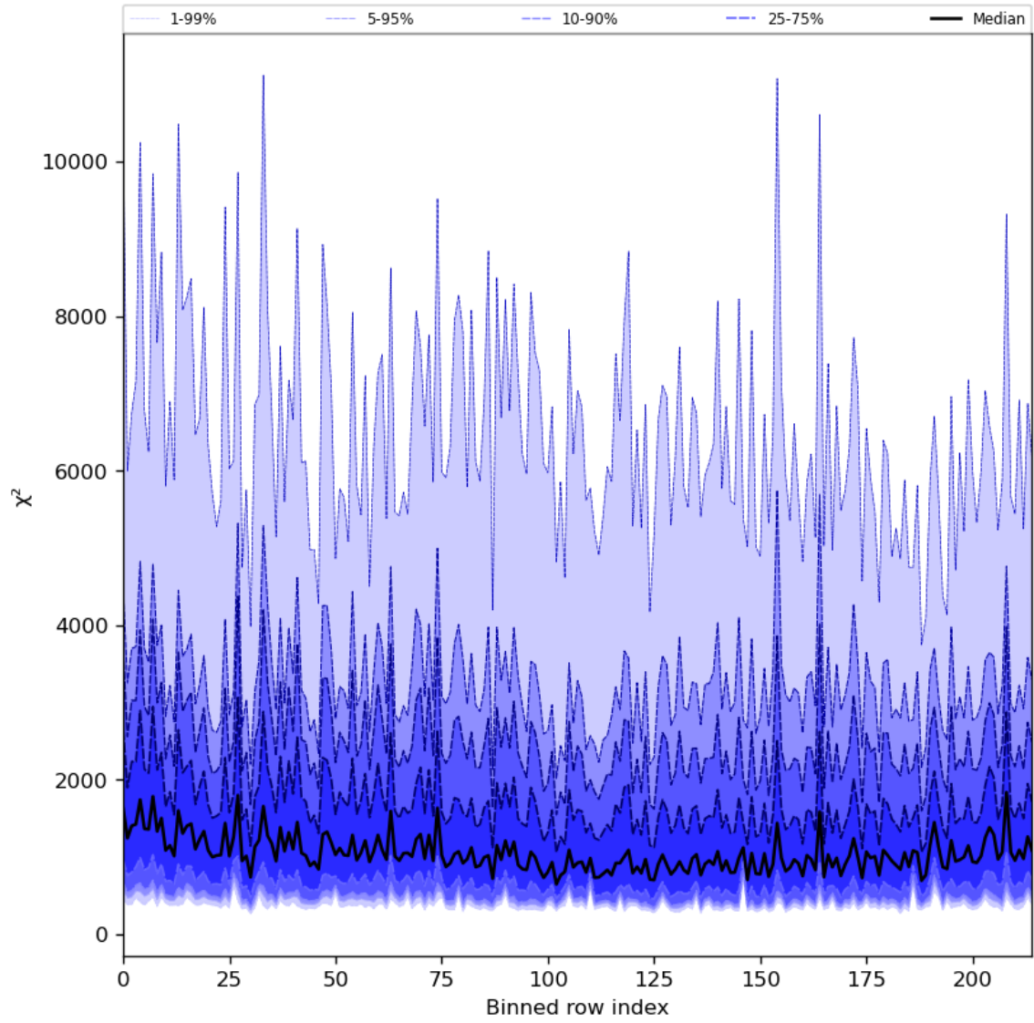
Figure 30: Along track statistics of “ \chi^2 ” for 2023-07-24 to 2023-07-25
