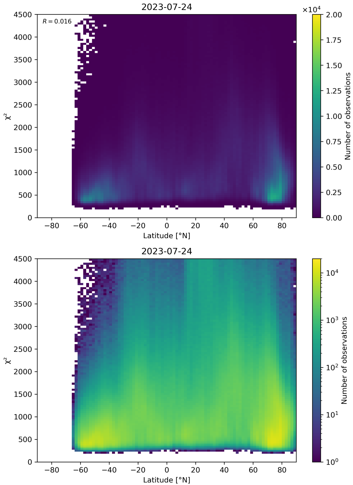
Figure 54: Scatter density plot of “Latitude” against “ \chi^2 ” for 2023-07-24 to 2023-07-25.
