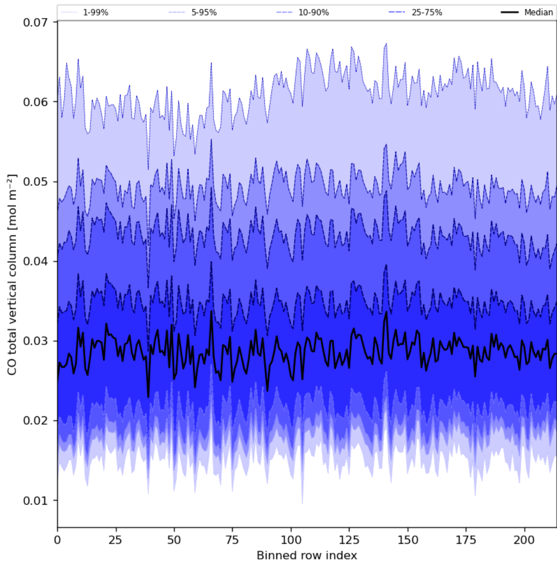
Figure 26: Along track statistics of “CO total vertical column” for 2023-07-24 to 2023-07-25
