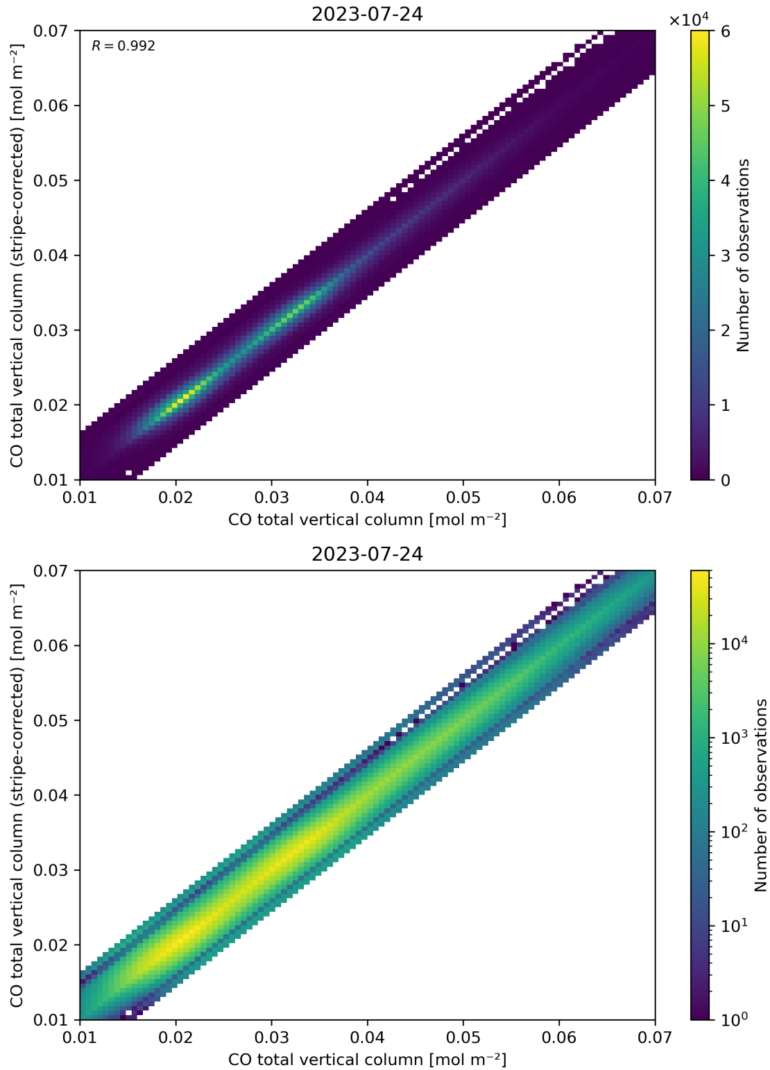
Figure 33: Scatter density plot of “CO total vertical column” against “CO total vertical column (stripe-corrected)” for 2023-07-24 to 2023-07-25.
