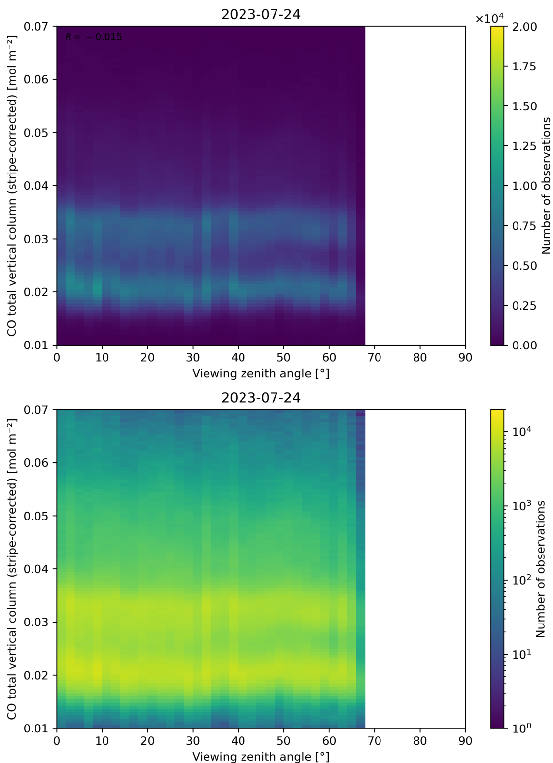
Figure 70: Scatter density plot of “Viewing zenith angle” against “CO total vertical column (stripe-corrected)” for 2023-07-24 to 2023-07-25.
