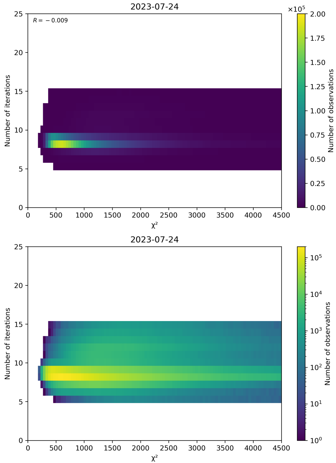
Figure 49: Scatter density plot of “ \chi^2 ” against “Number of iterations” for 2023-07-24 to 2023-07-25.
