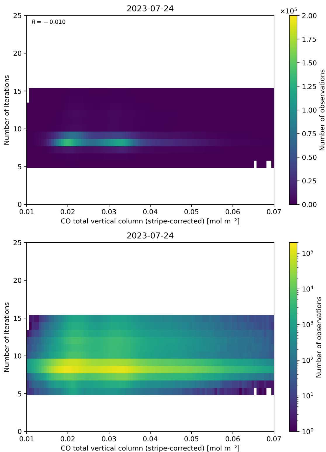
Figure 39: Scatter density plot of “CO total vertical column (stripe-corrected)” against “Number of iterations” for 2023-07-24 to 2023-07-25.
