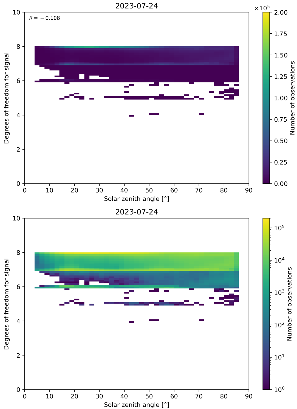
Figure 65: Scatter density plot of “Solar zenith angle” against “Degrees of freedom for signal” for 2023-07-24 to 2023-07-25.
