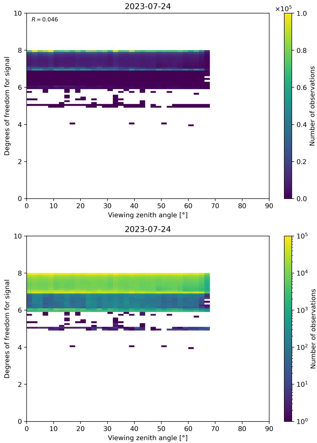
Figure 73: Scatter density plot of “Viewing zenith angle” against “Degrees of freedom for signal” for 2023-07-24 to 2023-07-25.
