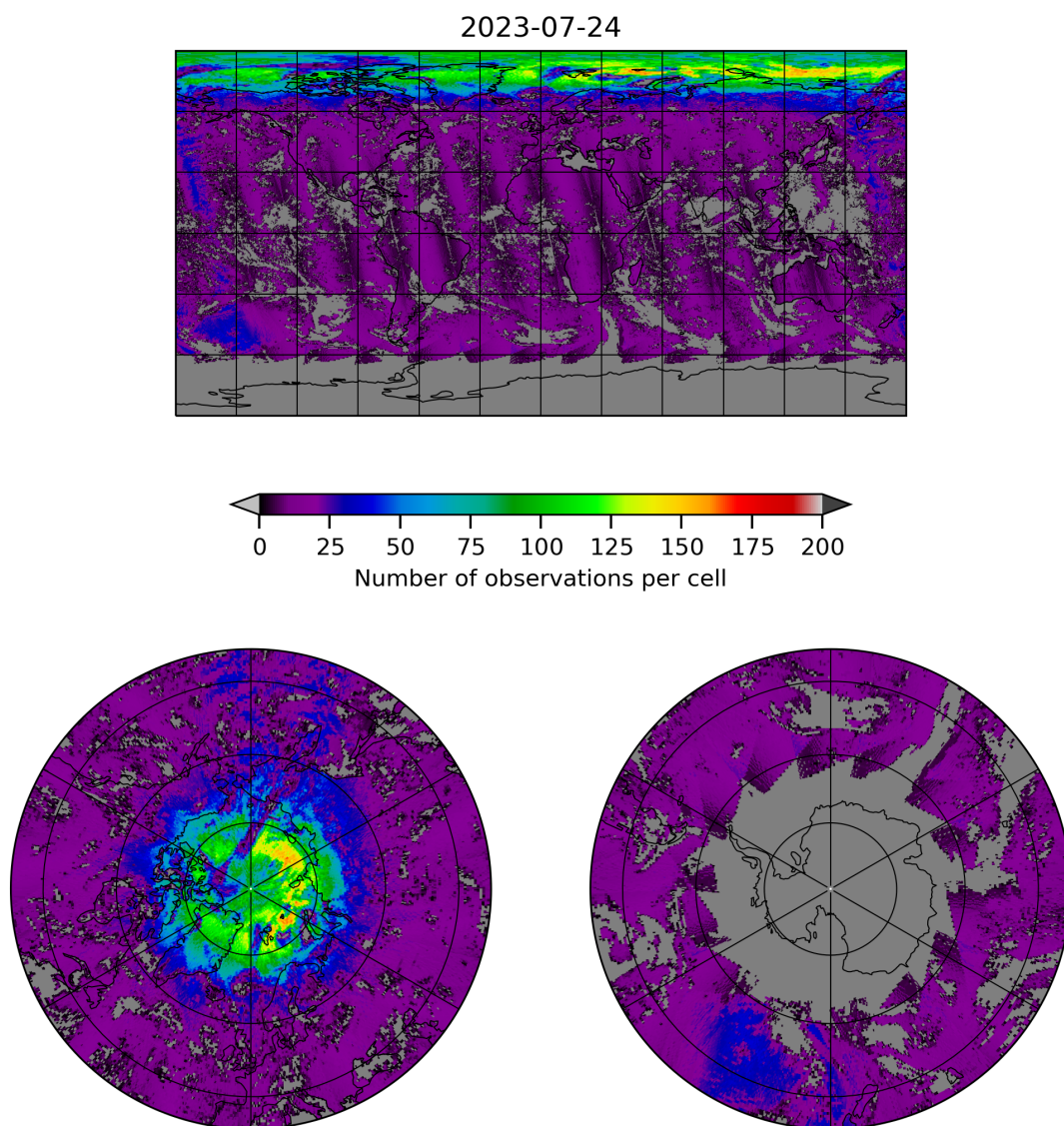
Figure 8: Map of the number of observations for 2023-07-24 to 2023-07-25
