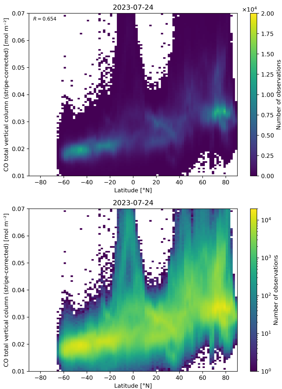
Figure 52: Scatter density plot of “Latitude” against “CO total vertical column (stripe-corrected)” for 2023-07-24 to 2023-07-25.
