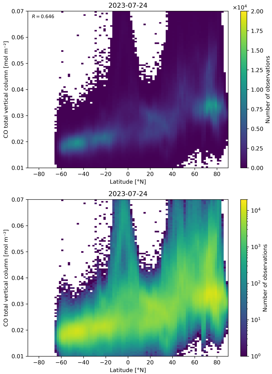
Figure 51: Scatter density plot of “Latitude” against “CO total vertical column” for 2023-07-24 to 2023-07-25.
