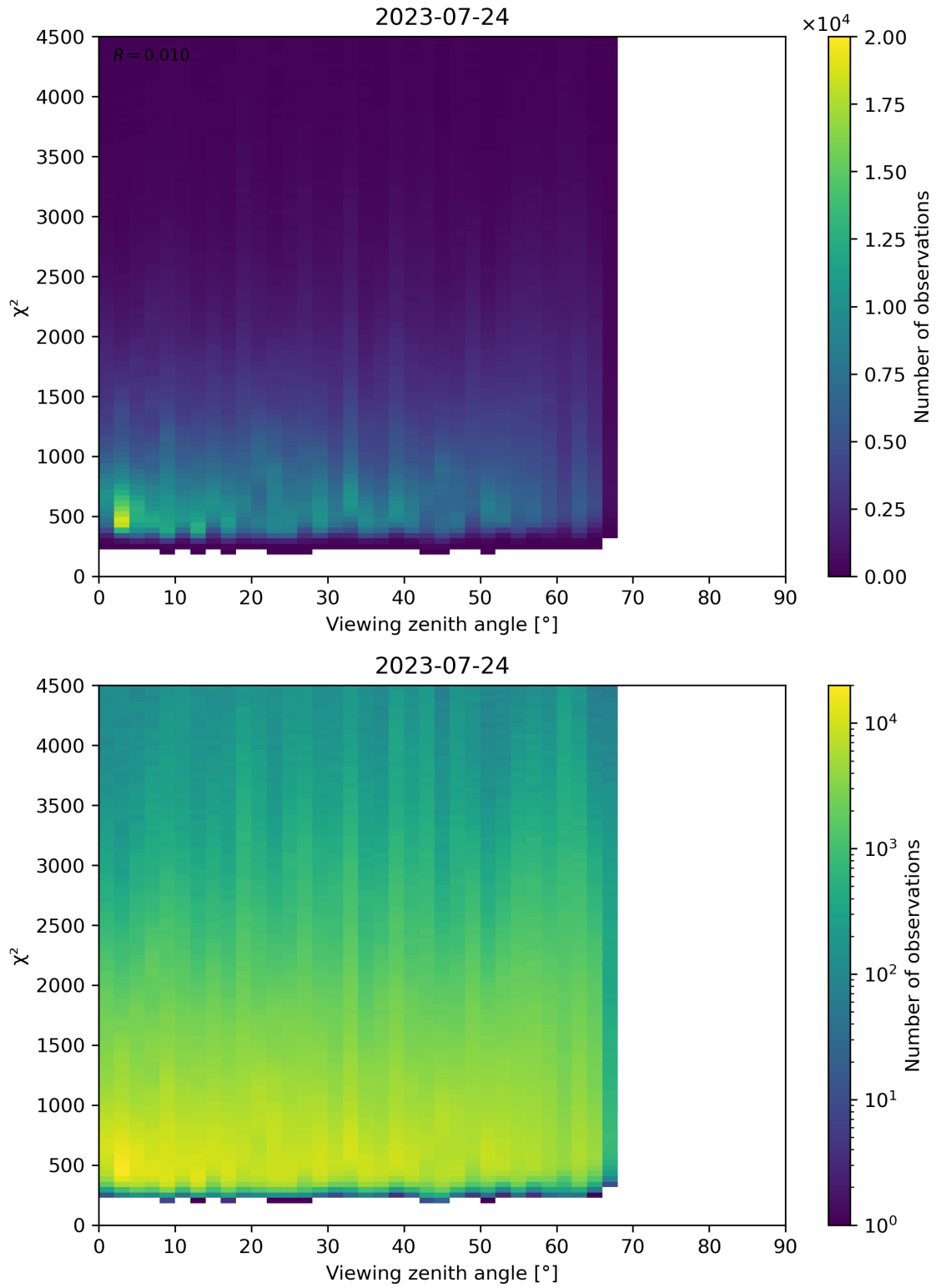
Figure 72: Scatter density plot of “Viewing zenith angle” against “ \chi^2 ” for 2023-07-24 to 2023-07-25.
