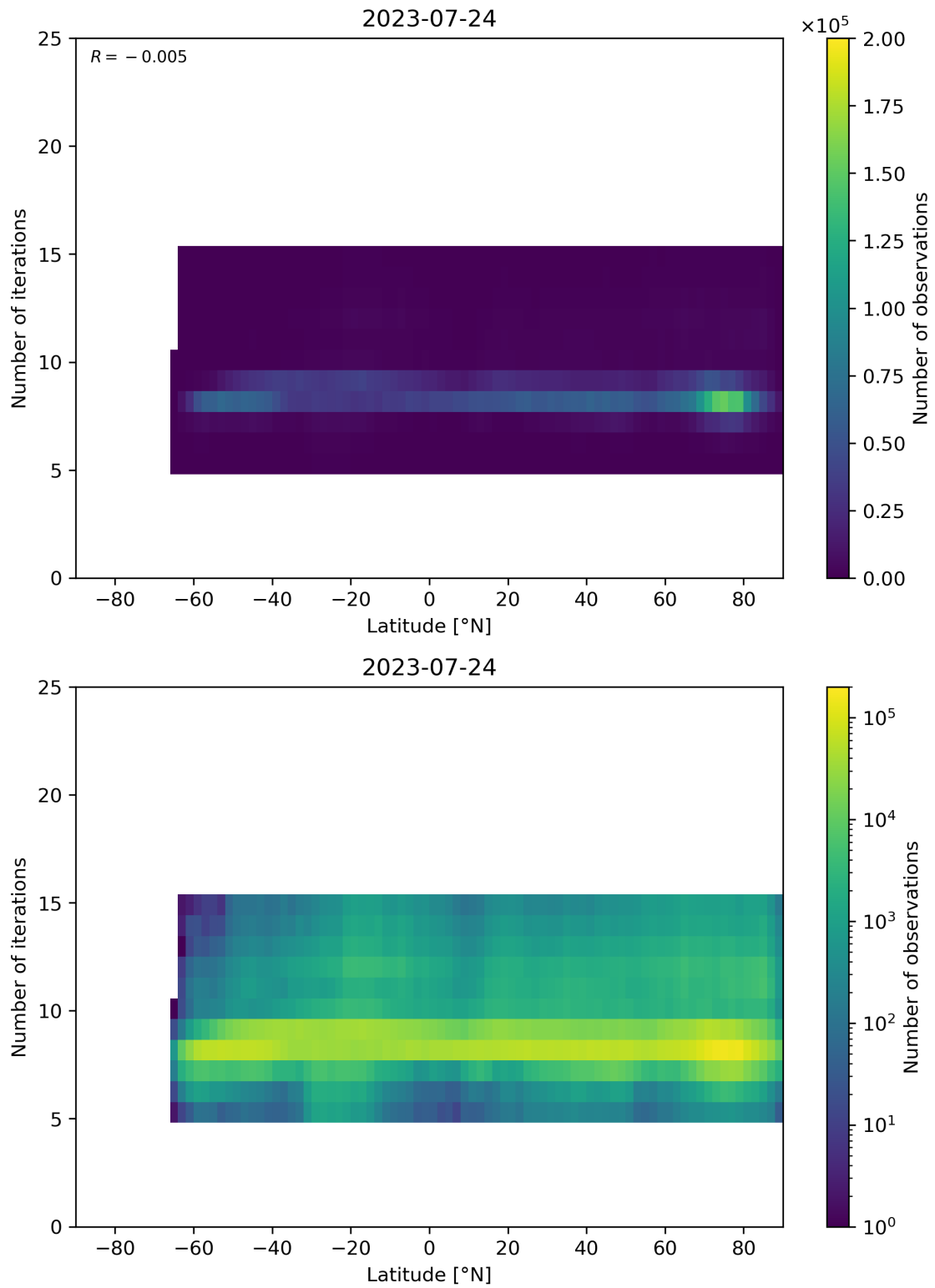
Figure 56: Scatter density plot of “Latitude” against “Number of iterations” for 2023-07-24 to 2023-07-25.
