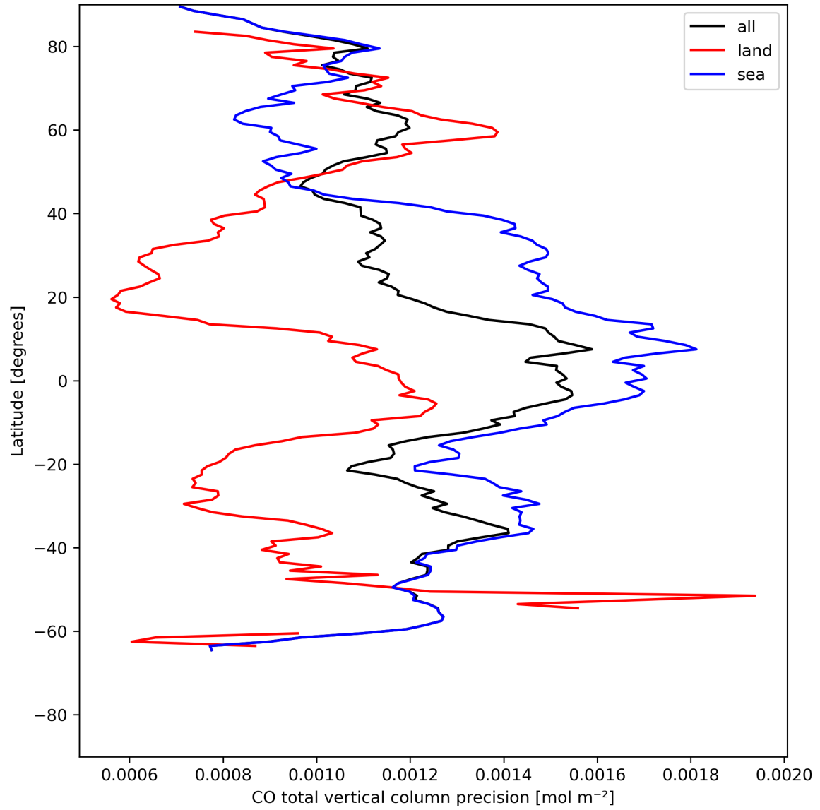
Figure 12: Zonal average of “CO total vertical column precision” for 2023-07-24 to 2023-07-25.
