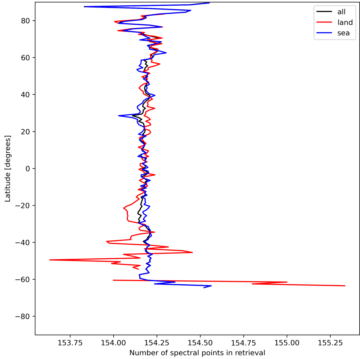
Figure 13: Zonal average of “Number of spectral points in retrieval” for 2023-07-24 to 2023-07-25.
