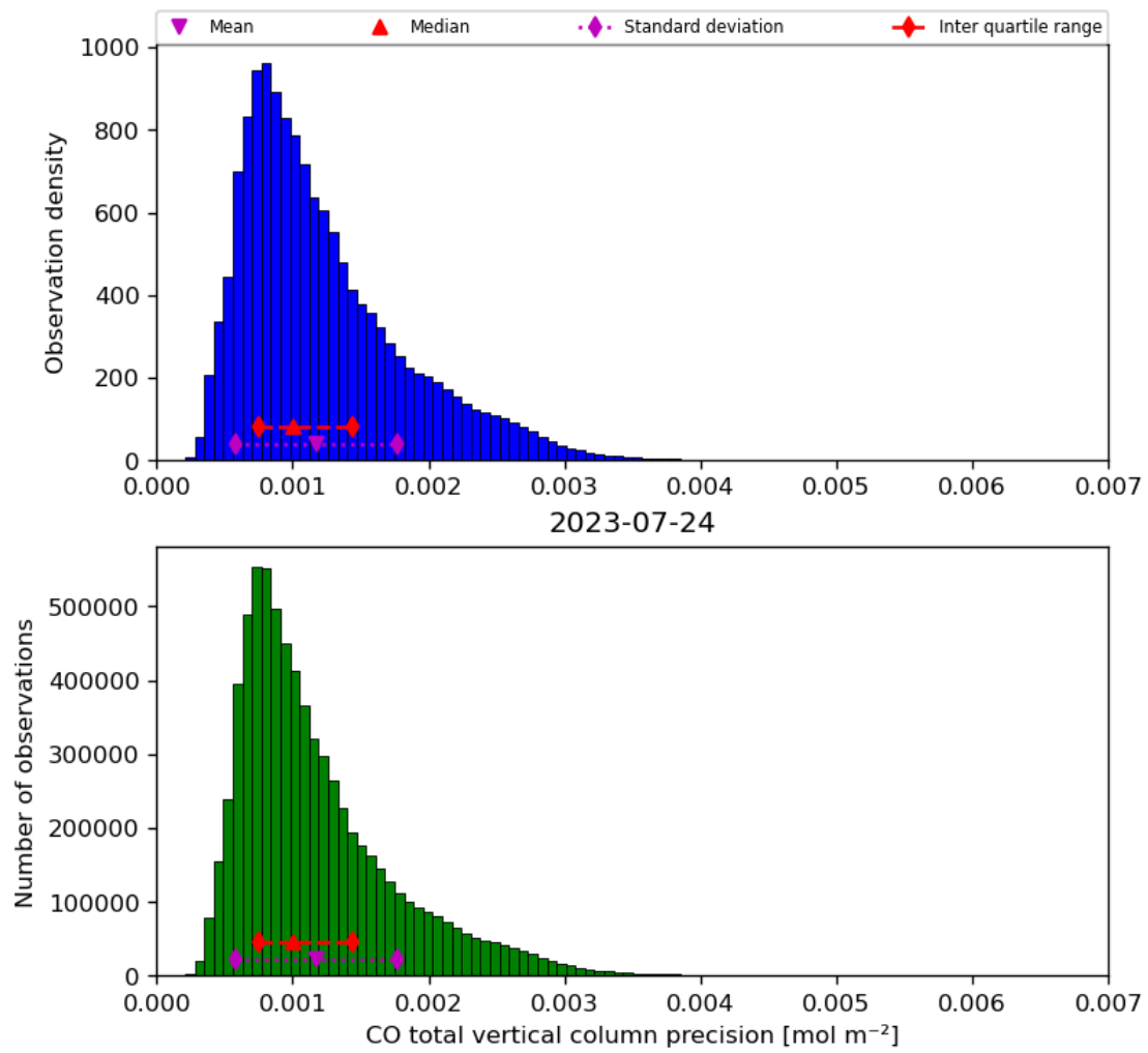
Figure 20: Histogram of “CO total vertical column precision” for 2023-07-24 to 2023-07-25
