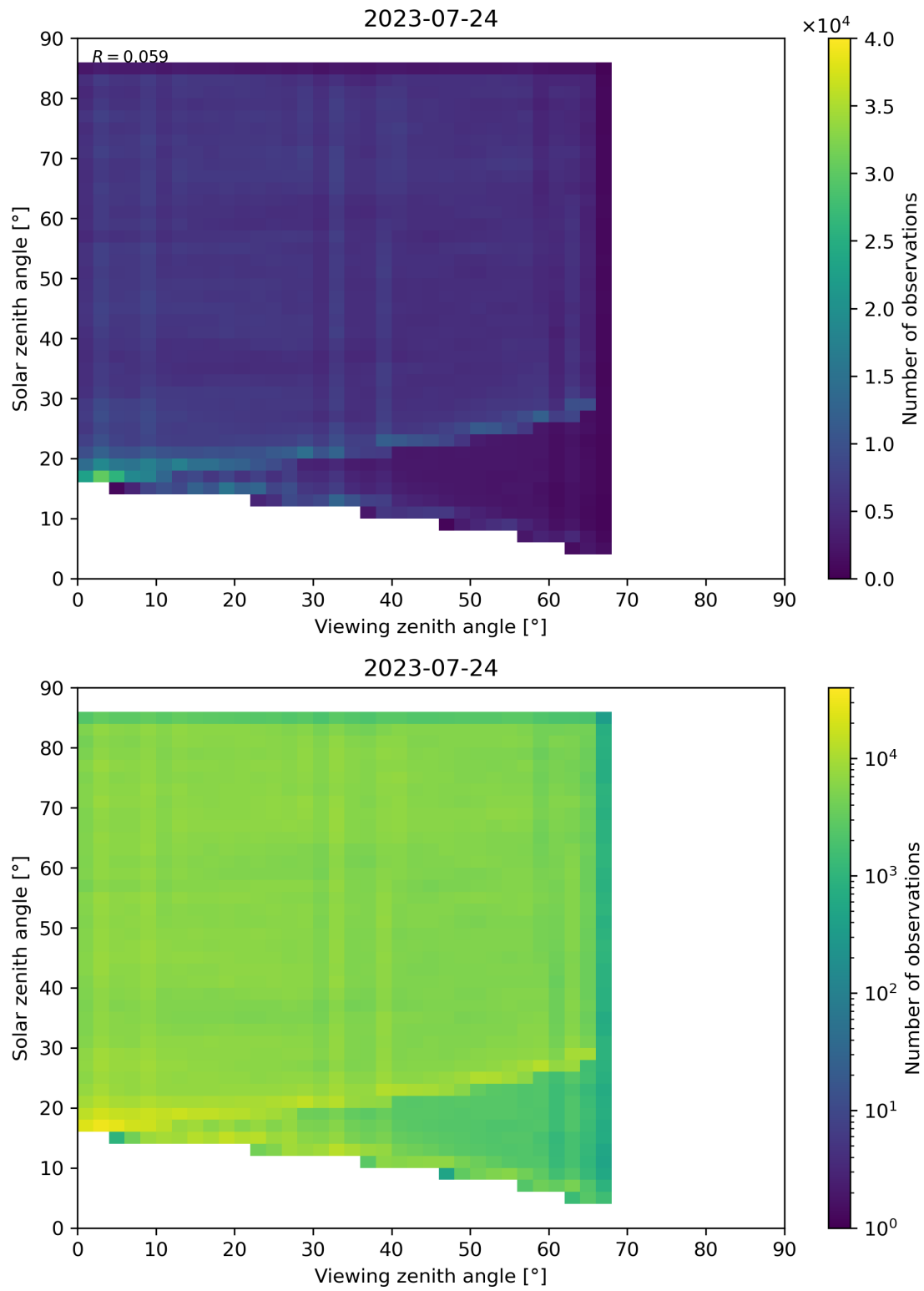
Figure 77: Scatter density plot of “Viewing zenith angle” against “Solar zenith angle” for 2023-07-24 to 2023-07-25.
