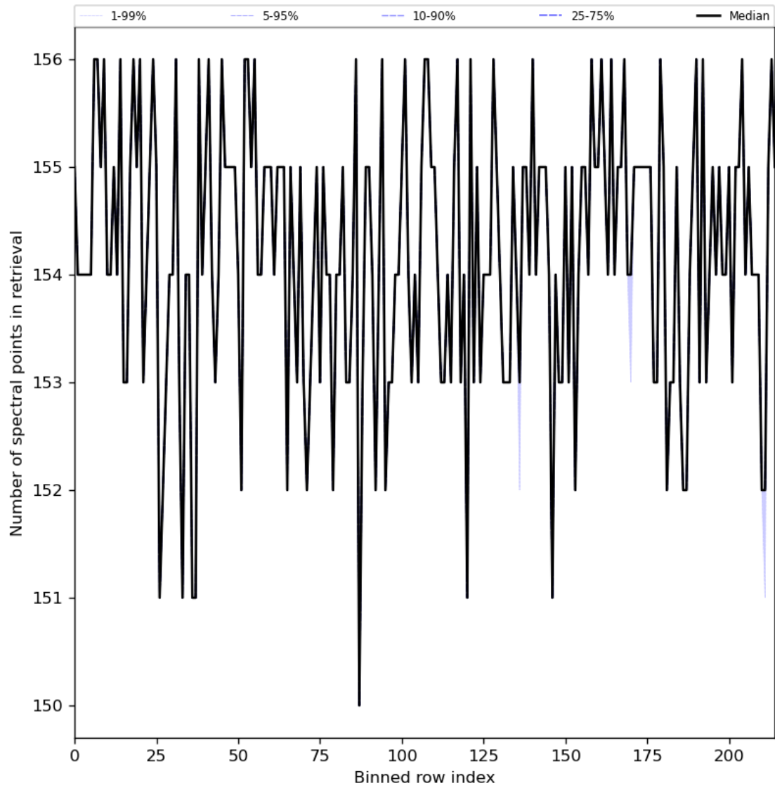
Figure 29: Along track statistics of “Number of spectral points in retrieval” for 2023-07-24 to 2023-07-25
