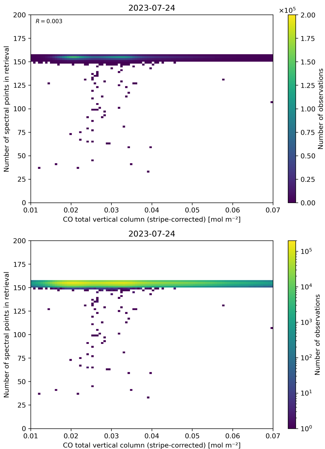
Figure 40: Scatter density plot of “CO total vertical column (stripe-corrected)” against “Number of spectral points in retrieval” for 2023-07-24 to 2023-07-25.
