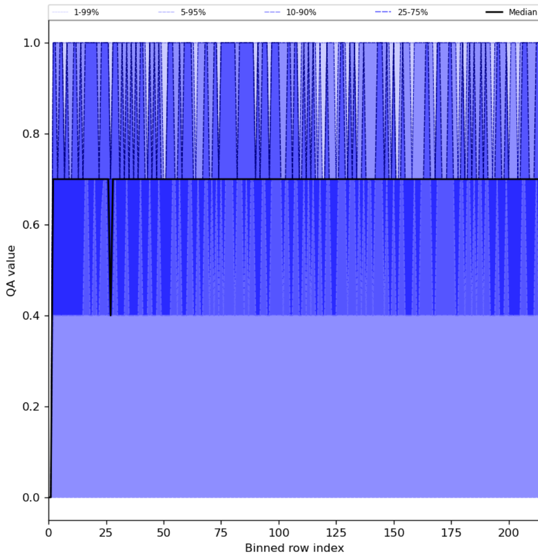
Figure 25: Along track statistics of “QA value” for 2023-07-24 to 2023-07-25
