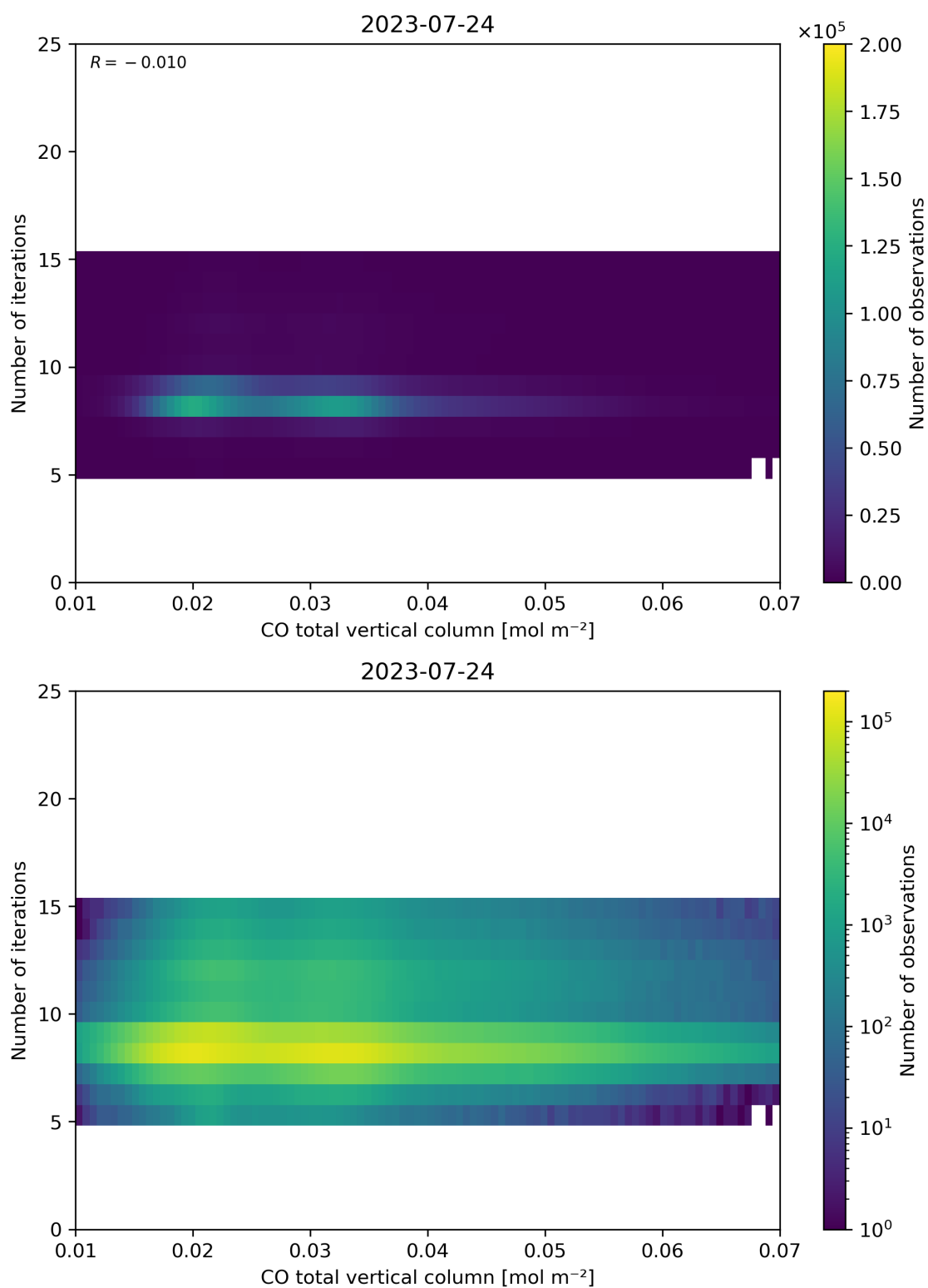
Figure 42: Scatter density plot of “CO total vertical column” against “Number of iterations” for 2023-07-24 to 2023-07-25.
