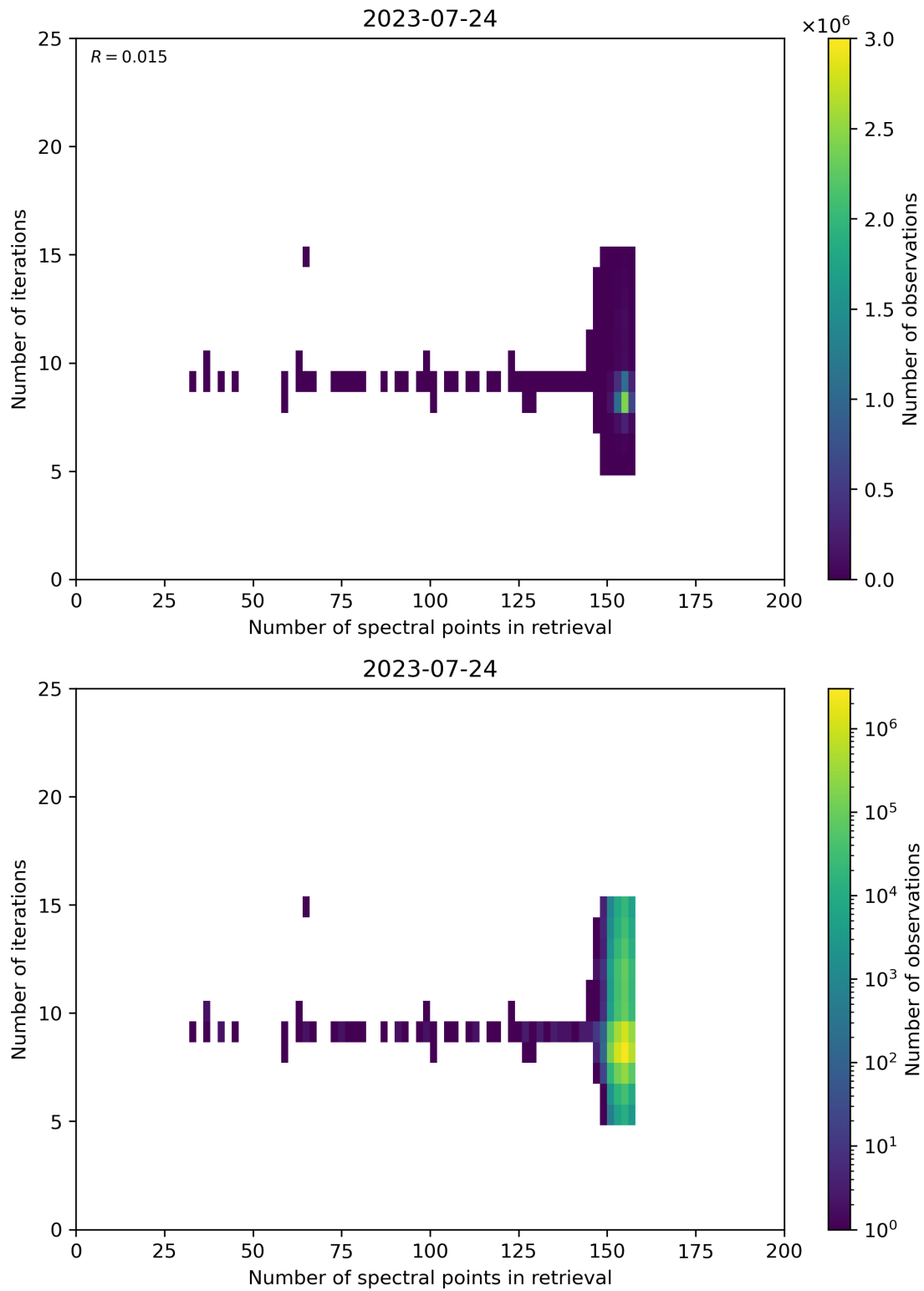
Figure 60: Scatter density plot of “Number of spectral points in retrieval” against “Number of iterations” for 2023-07-24 to 2023-07-25.
