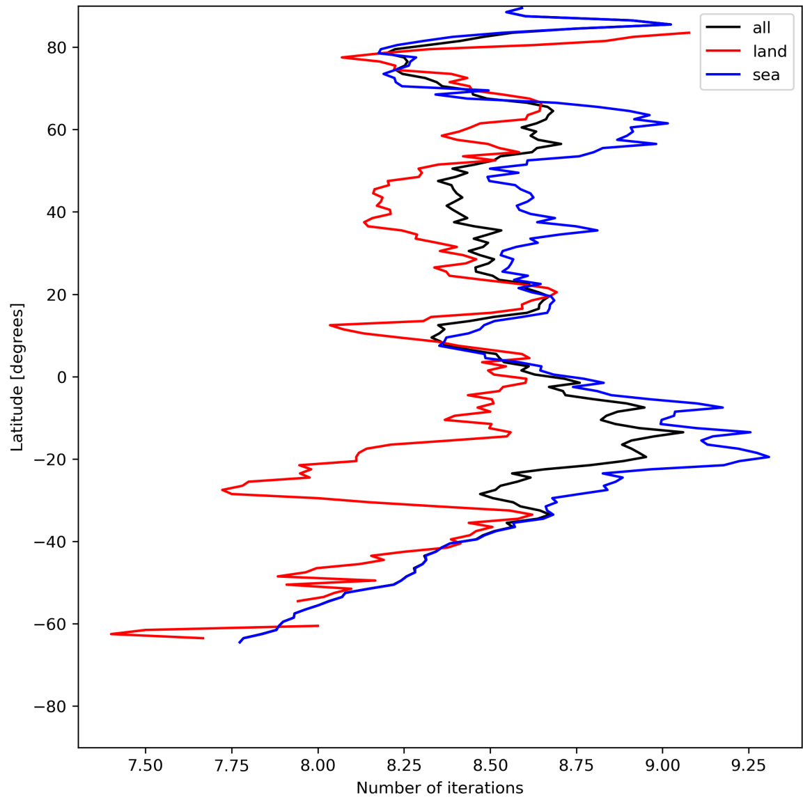
Figure 16: Zonal average of “Number of iterations” for 2023-07-24 to 2023-07-25.
