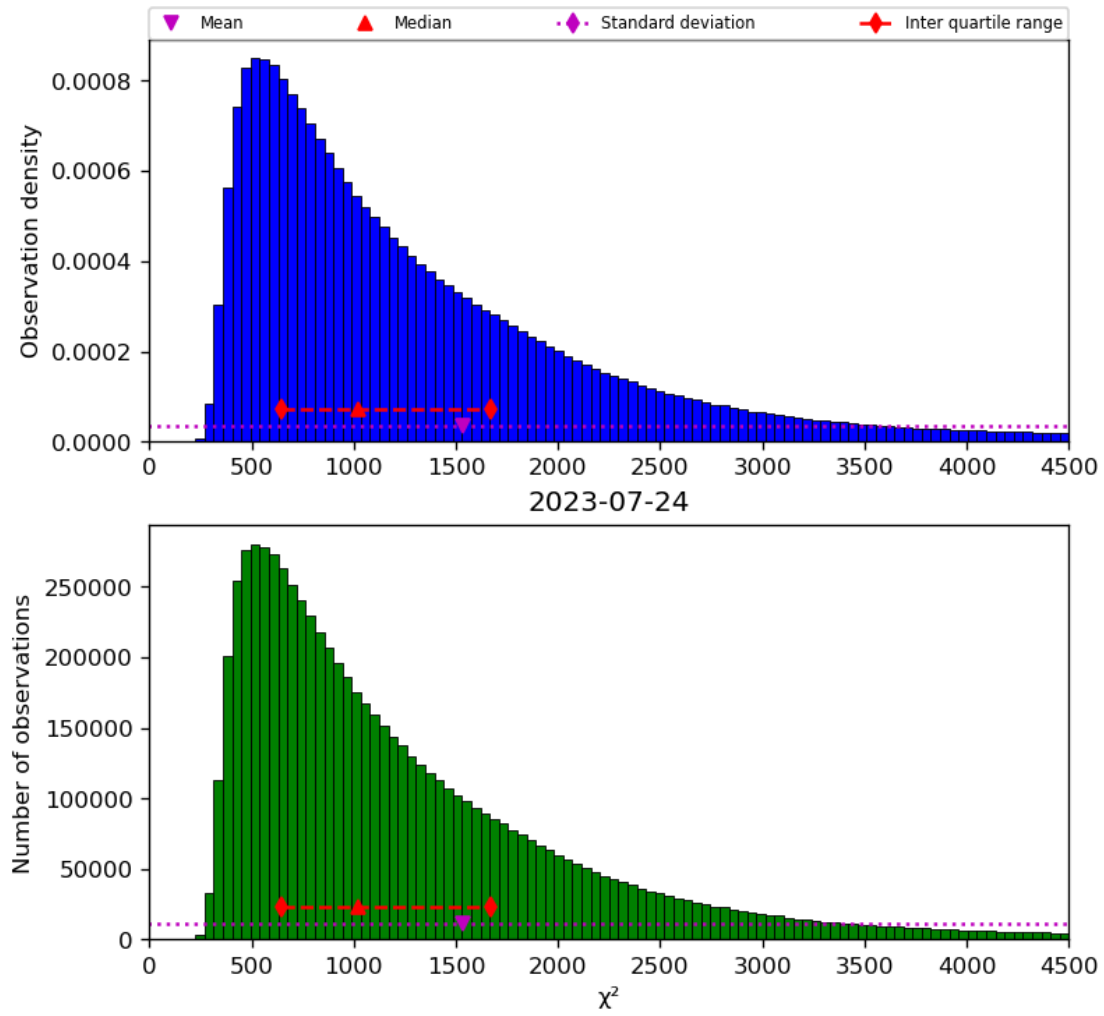
Figure 22: Histogram of “ \chi^2 ” for 2023-07-24 to 2023-07-25
