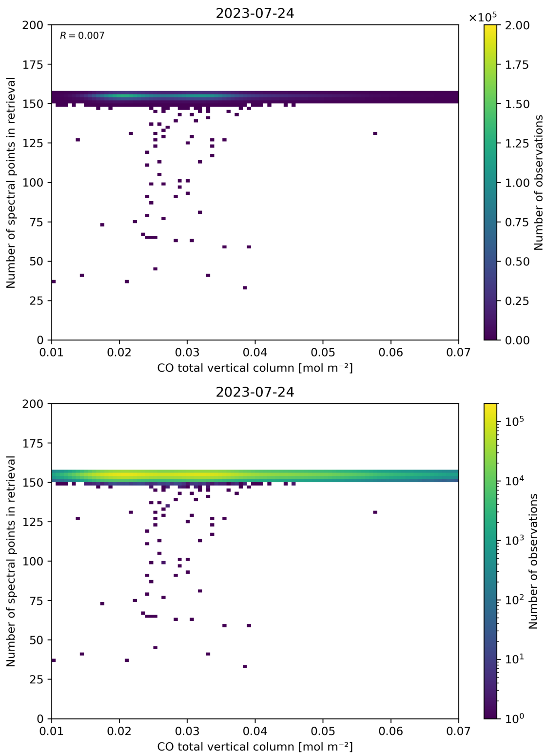
Figure 43: Scatter density plot of “CO total vertical column” against “Number of spectral points in retrieval” for 2023-07-24 to 2023-07-25.
