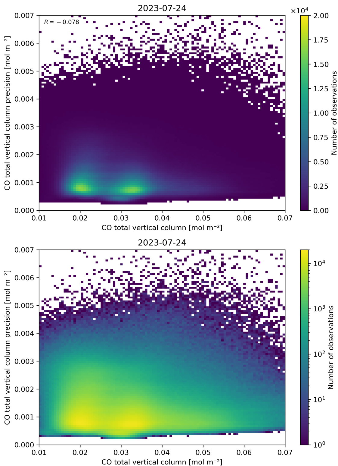
Figure 34: Scatter density plot of “CO total vertical column” against “CO total vertical column precision” for 2023-07-24 to 2023-07-25.
