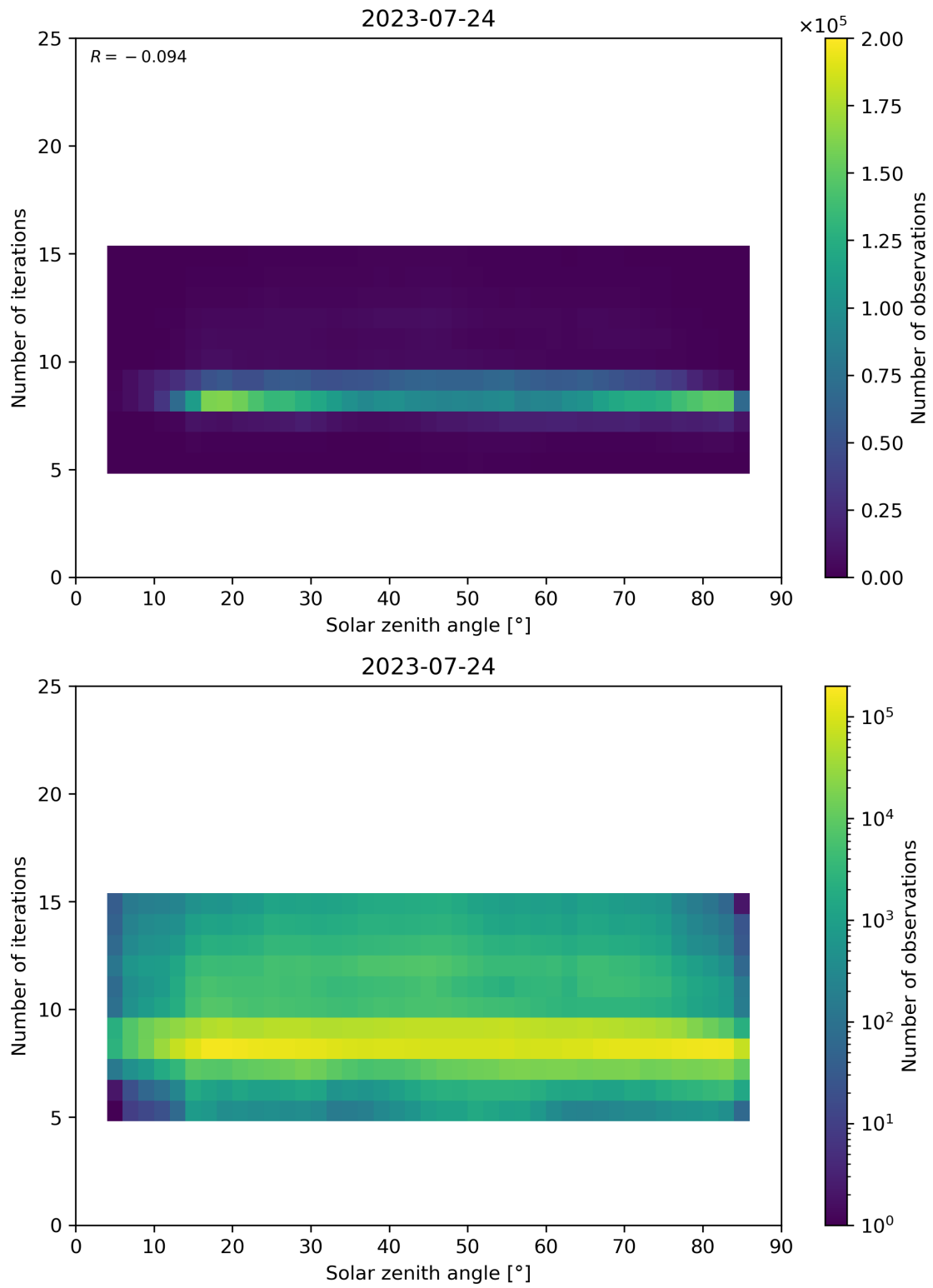
Figure 67: Scatter density plot of “Solar zenith angle” against “Number of iterations” for 2023-07-24 to 2023-07-25.
