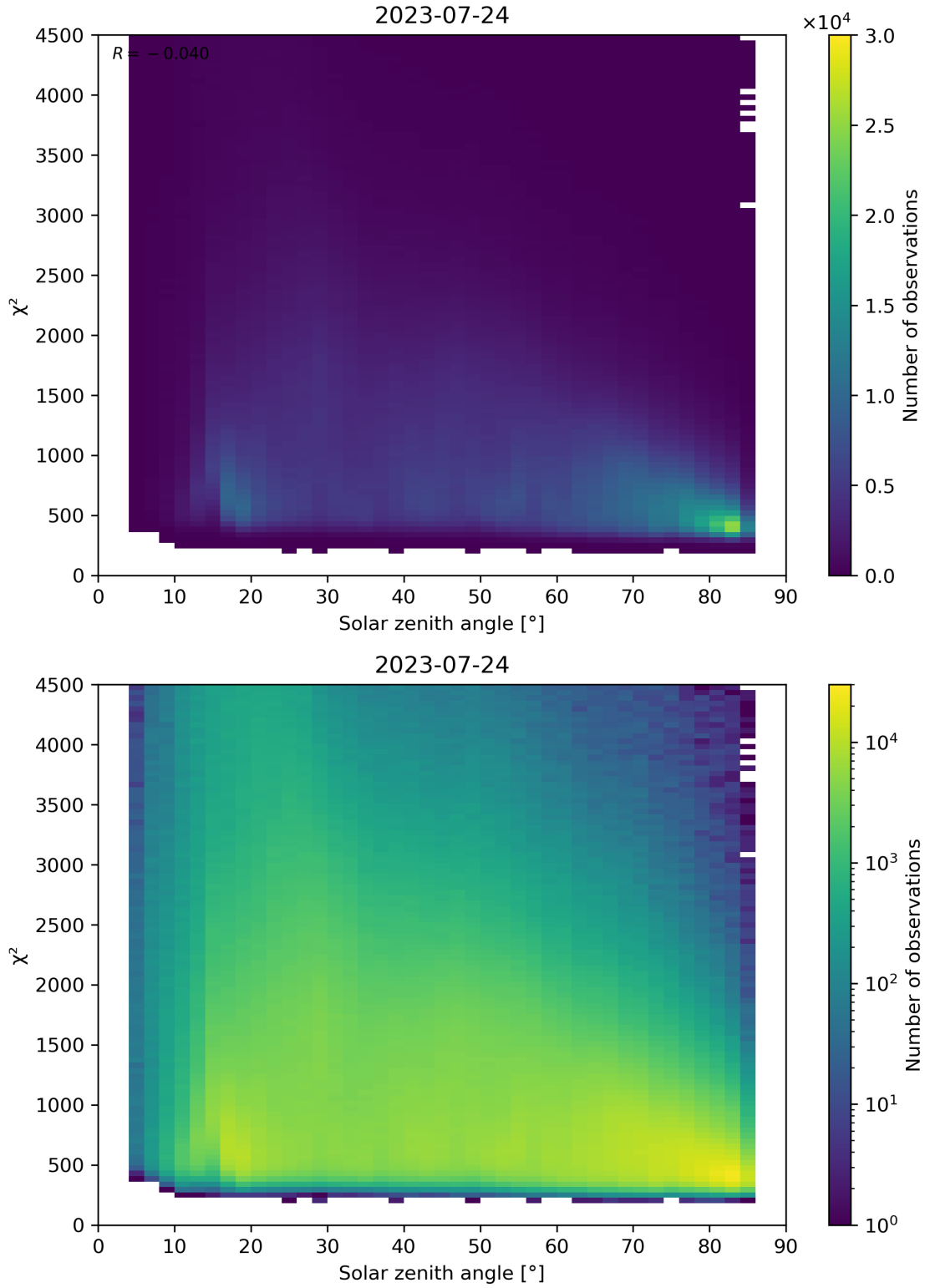
Figure 64: Scatter density plot of “Solar zenith angle” against “ \chi^2 ” for 2023-07-24 to 2023-07-25.
