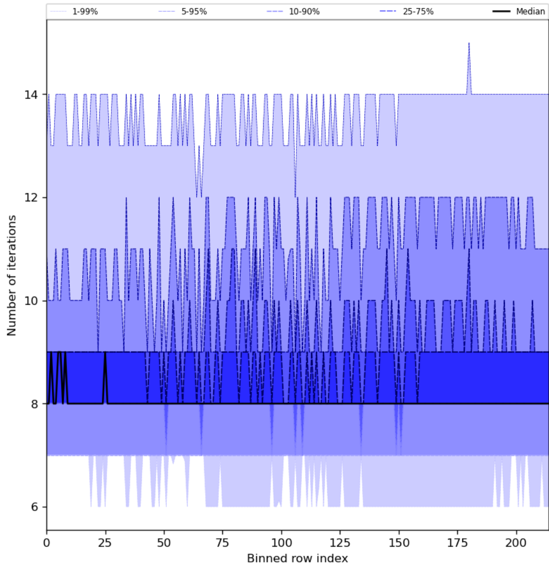
Figure 32: Along track statistics of “Number of iterations” for 2023-07-24 to 2023-07-25
