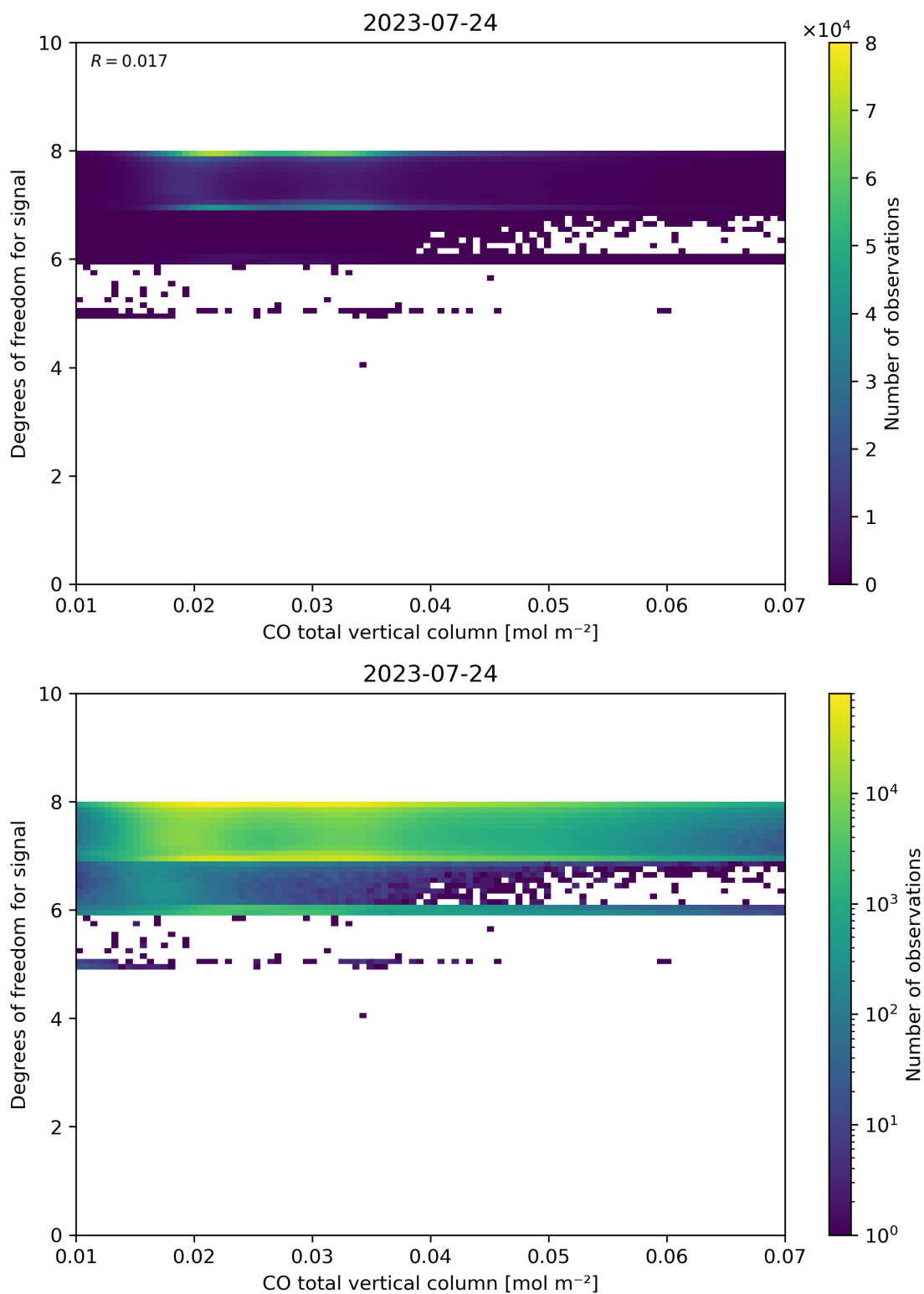
Figure 41: Scatter density plot of “CO total vertical column” against “Degrees of freedom for signal” for 2023-07-24 to 2023-07-25.
