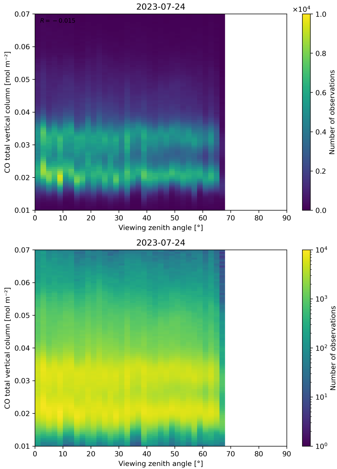
Figure 69: Scatter density plot of “Viewing zenith angle” against “CO total vertical column” for 2023-07-24 to 2023-07-25.
