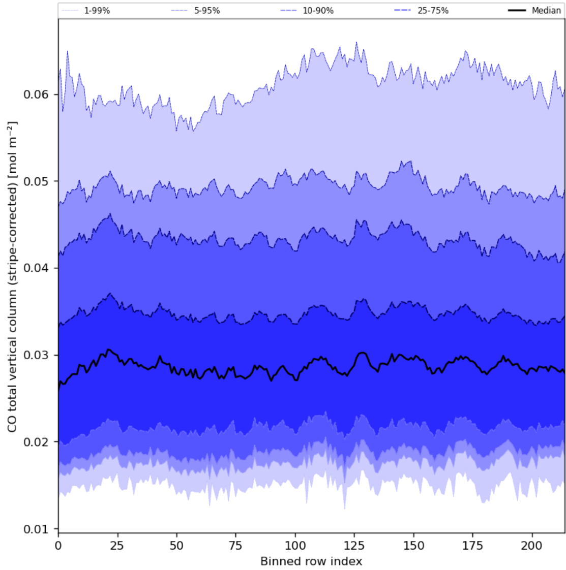
Figure 27: Along track statistics of “CO total vertical column (stripe-corrected)” for 2023-07-24 to 2023-07-25
