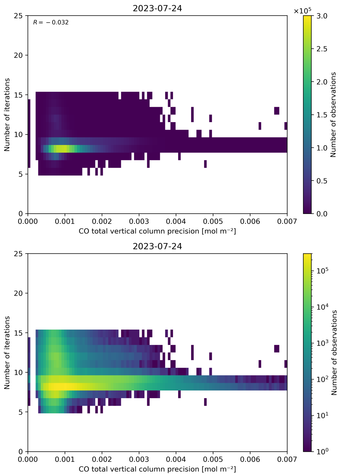
Figure 46: Scatter density plot of “CO total vertical column precision” against “Number of iterations” for 2023-07-24 to 2023-07-25.
