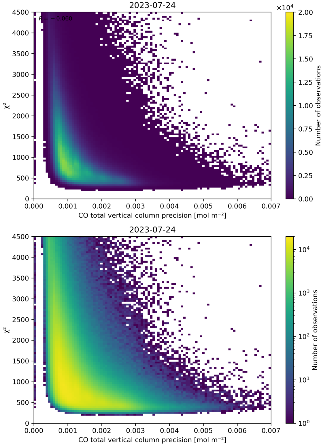
Figure 44: Scatter density plot of “CO total vertical column precision” against “ \chi^2 ” for 2023-07-24 to 2023-07-25.
