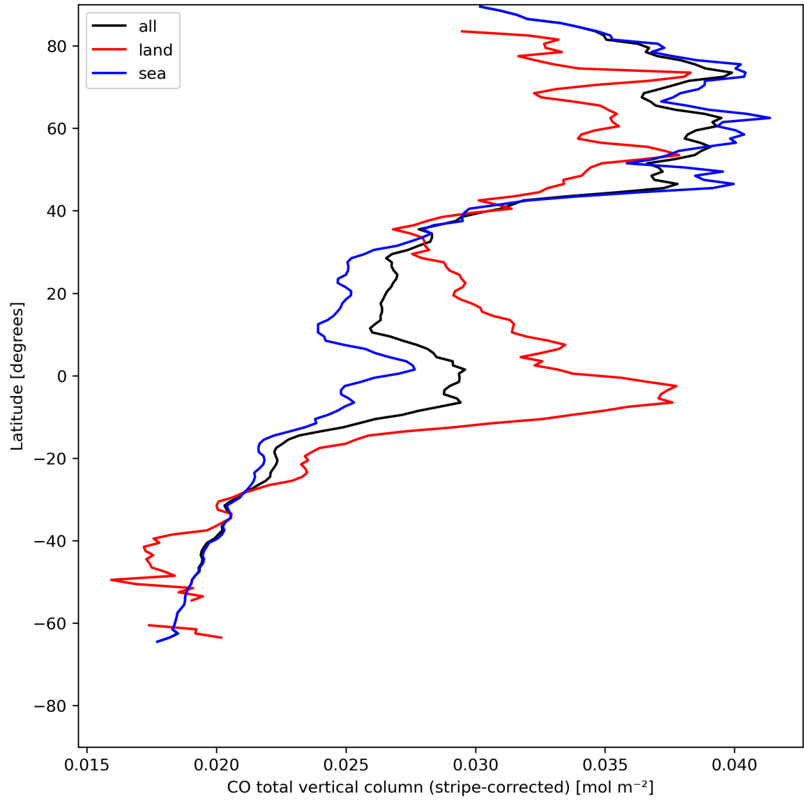
Figure 11: Zonal average of “CO total vertical column (stripe-corrected)” for 2023-07-24 to 2023-07-25.
