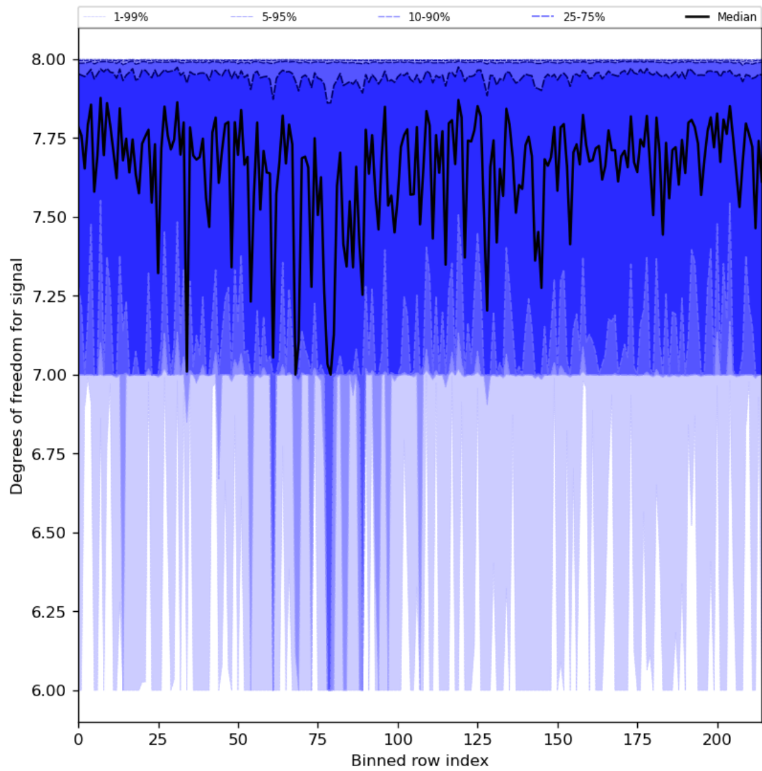
Figure 31: Along track statistics of “Degrees of freedom for signal” for 2023-07-24 to 2023-07-25
