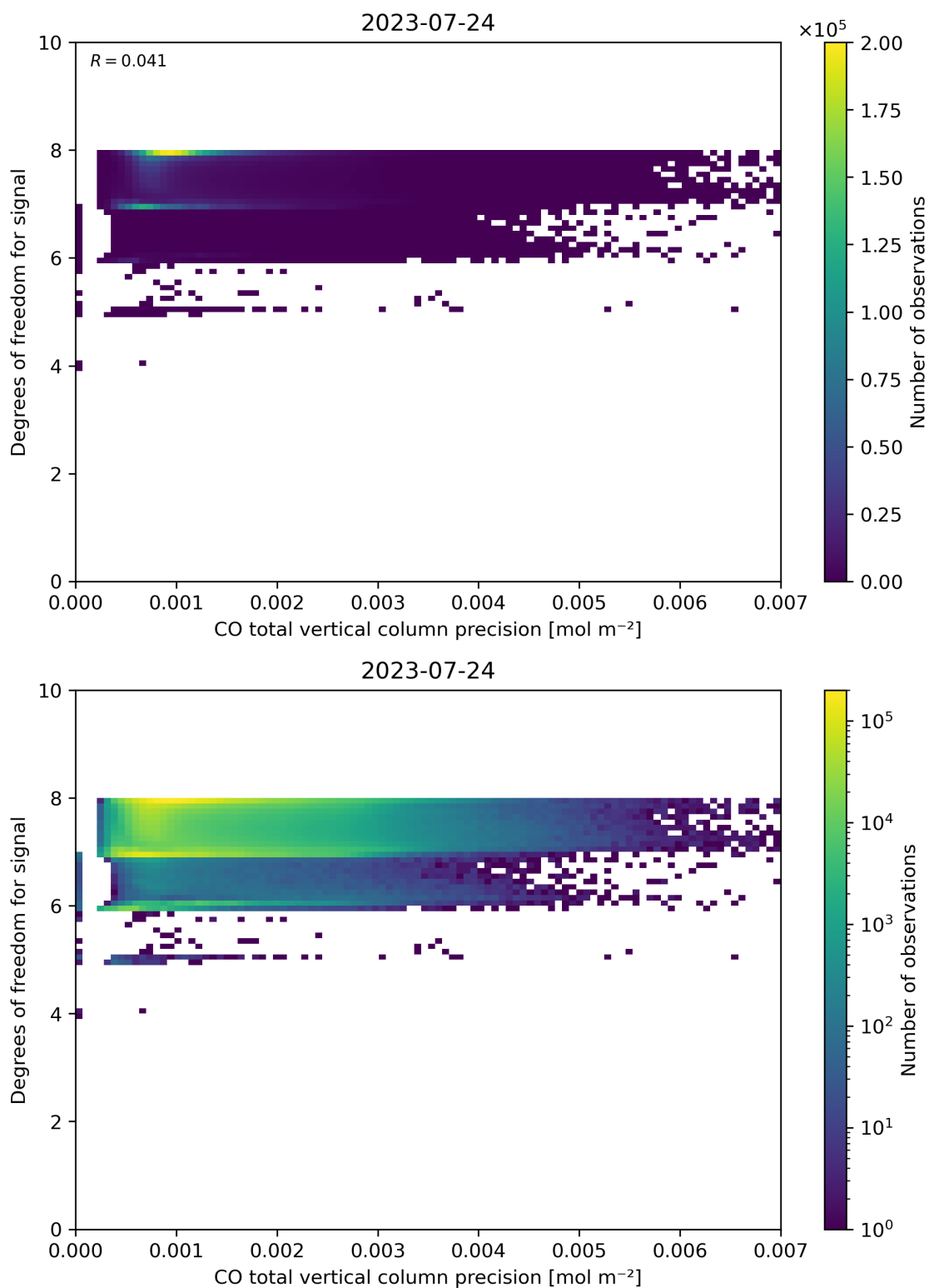
Figure 45: Scatter density plot of “CO total vertical column precision” against “Degrees of freedom for signal” for 2023-07-24 to 2023-07-25.
