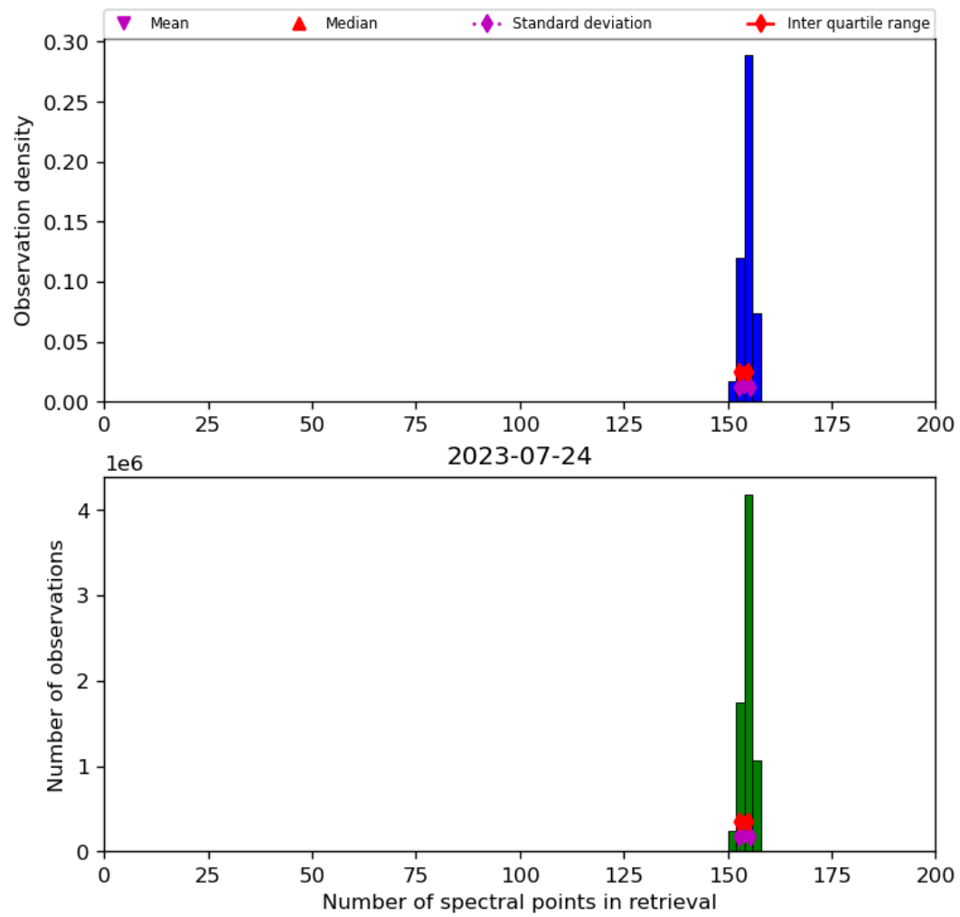
Figure 21: Histogram of “Number of spectral points in retrieval” for 2023-07-24 to 2023-07-25
