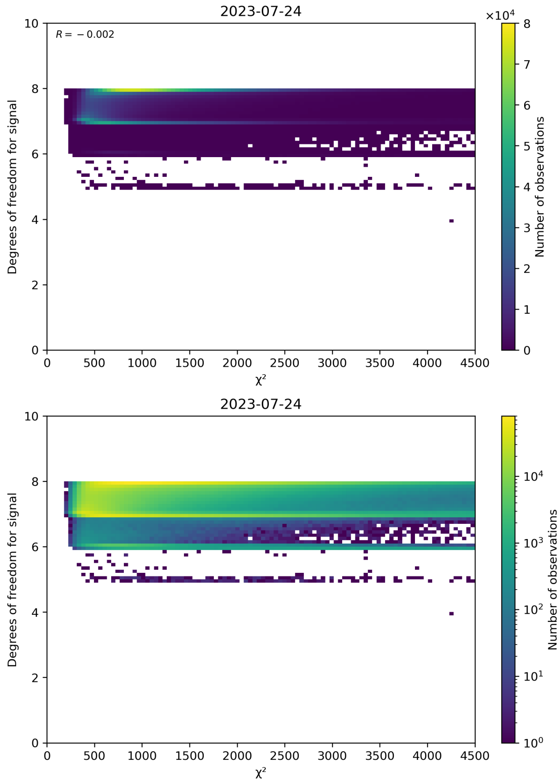
Figure 48: Scatter density plot of " \chi^2 " against "Degrees of freedom for signal" for 2023-07-24 to 2023-07-25.
