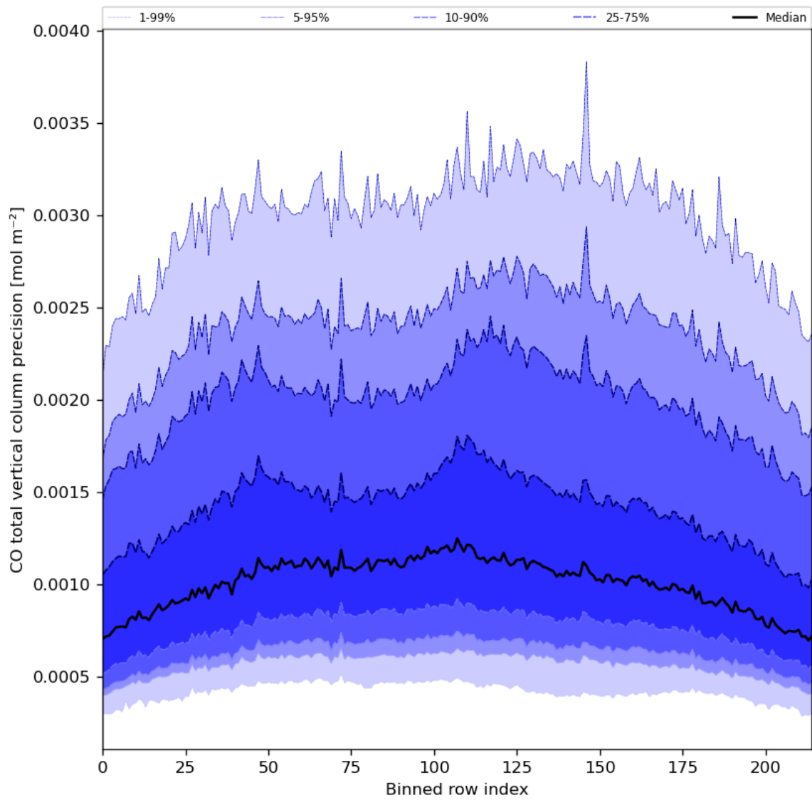
Figure 28: Along track statistics of “CO total vertical column precision” for 2023-07-24 to 2023-07-25
