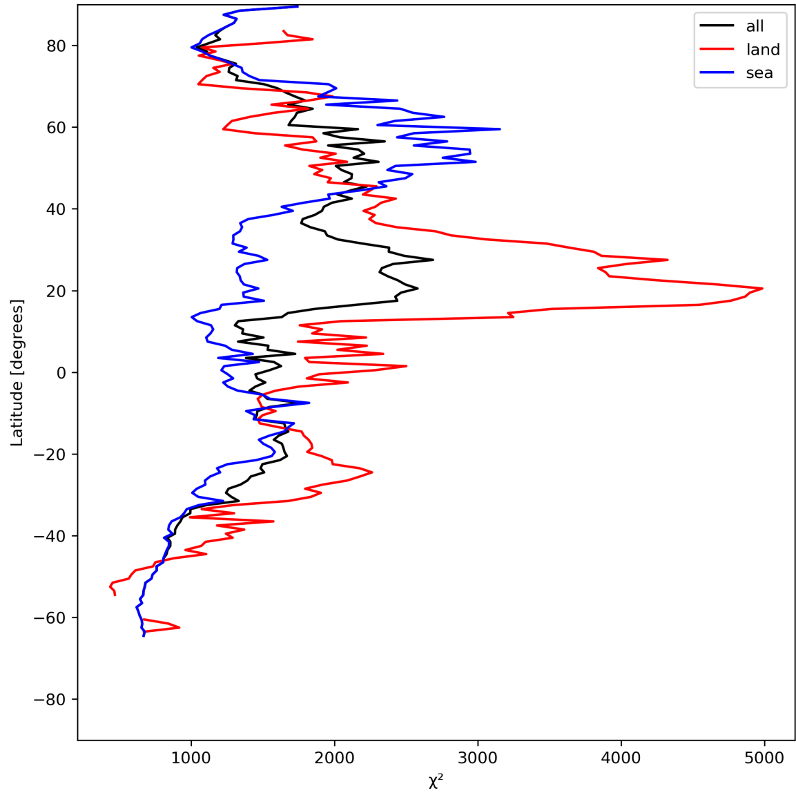
Figure 14: Zonal average of “ \chi^2 ” for 2023-07-24 to 2023-07-25.
