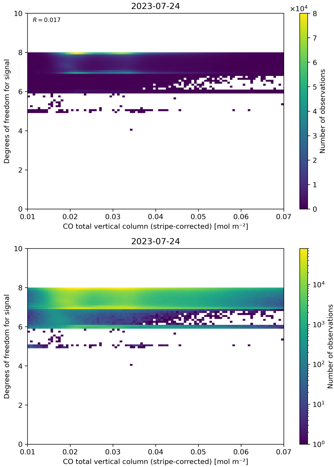
Figure 38: Scatter density plot of “CO total vertical column (stripe-corrected)” against “Degrees of freedom for signal” for 2023-07-24 to 2023-07-25.
