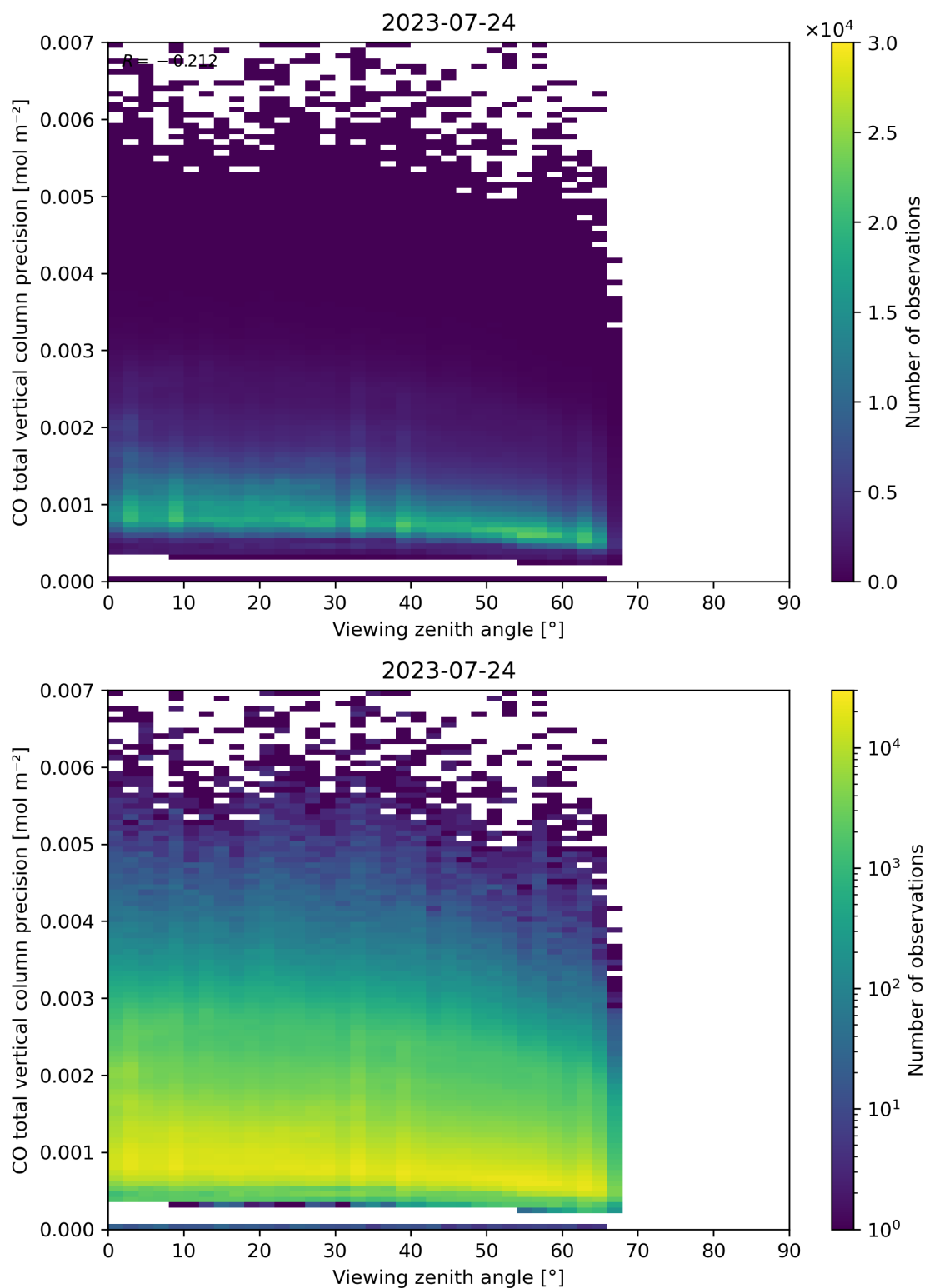
Figure 71: Scatter density plot of “Viewing zenith angle” against “CO total vertical column precision” for 2023-07-24 to 2023-07-25.
