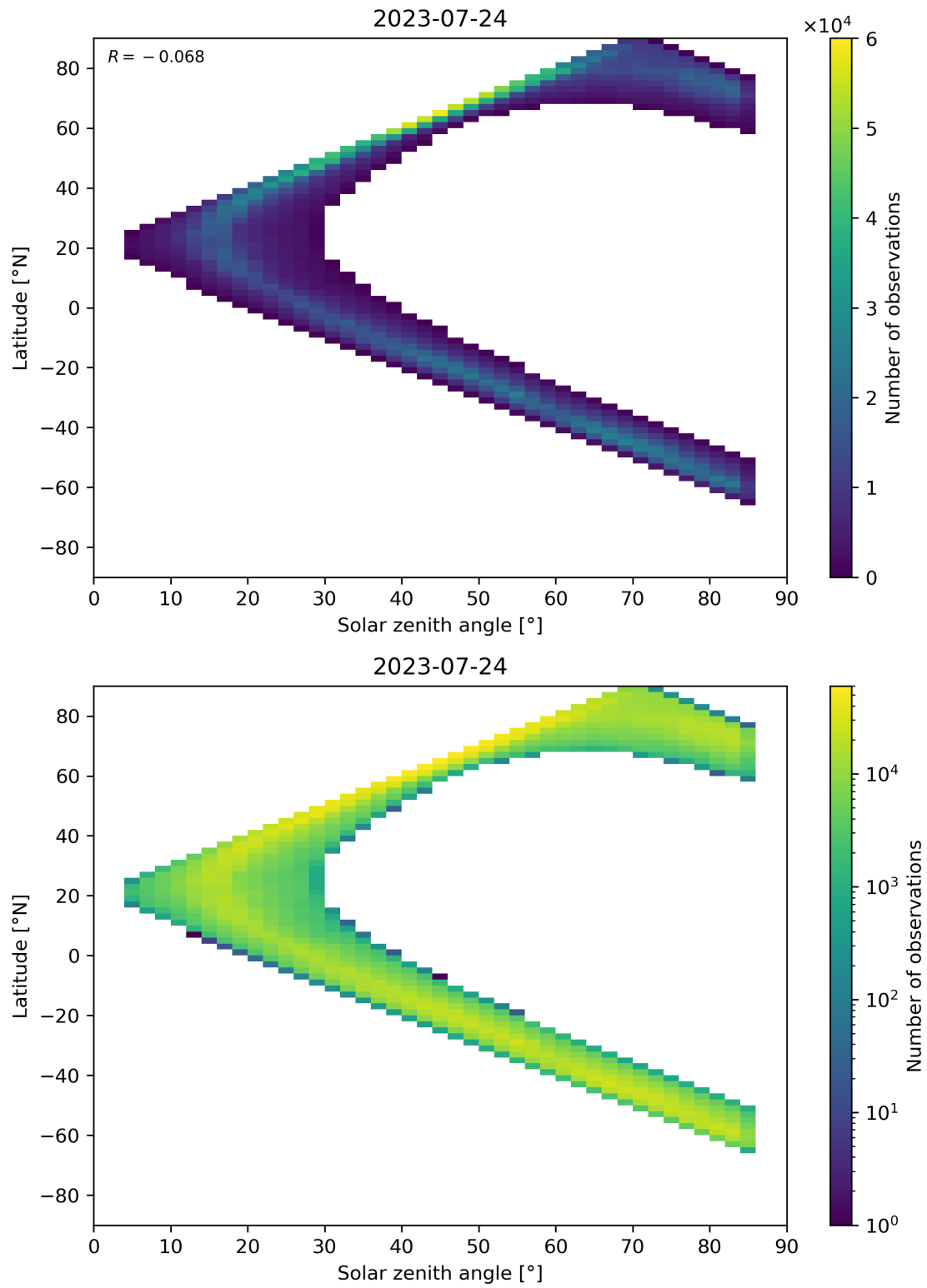
Figure 66: Scatter density plot of “Solar zenith angle” against “Latitude” for 2023-07-24 to 2023-07-25.
