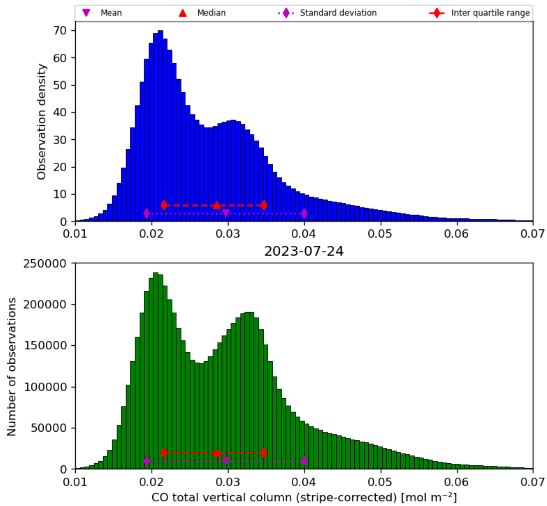
Figure 19: Histogram of “CO total vertical column (stripe-corrected)” for 2023-07-24 to 2023-07-25
