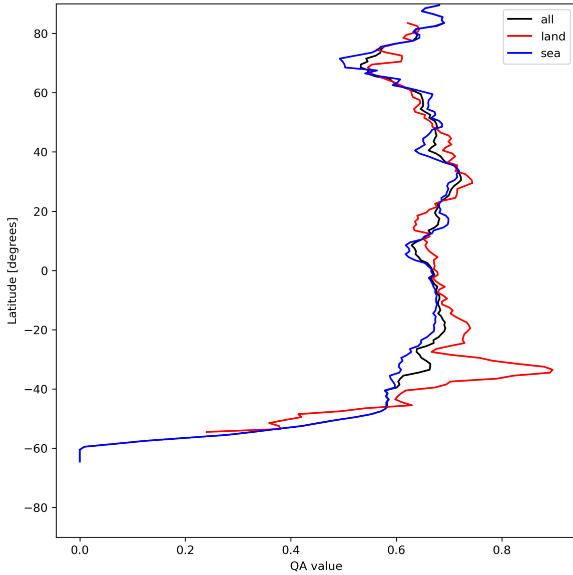
Figure 9: Zonal average of “QA value” for 2023-07-24 to 2023-07-25.
