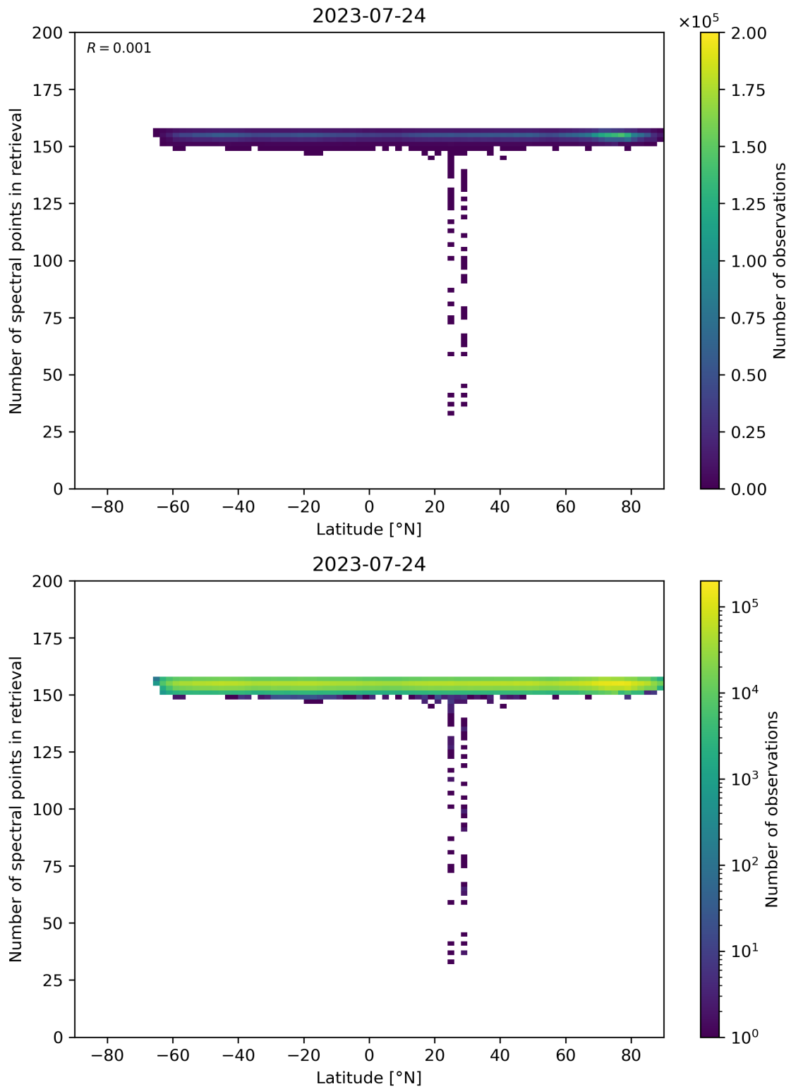
Figure 57: Scatter density plot of “Latitude” against “Number of spectral points in retrieval” for 2023-07-24 to 2023-07-25.
