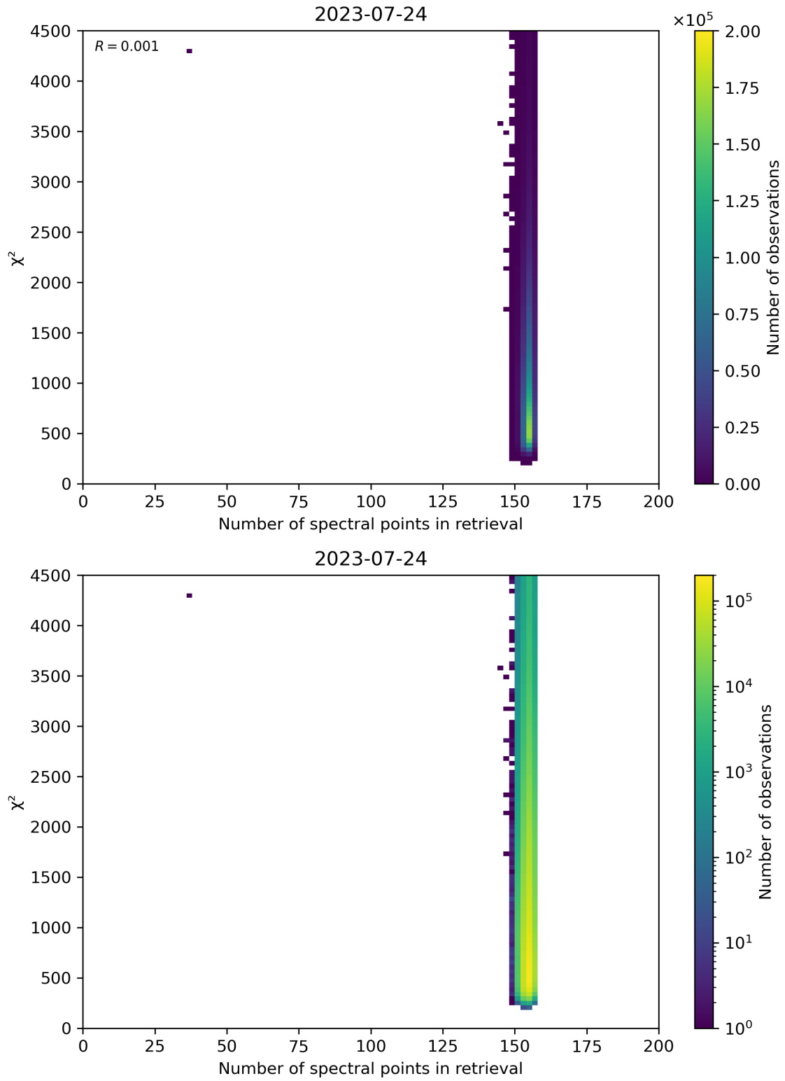
Figure 58: Scatter density plot of “Number of spectral points in retrieval” against “ \chi^2 ” for 2023-07-24 to 2023-07-25.
