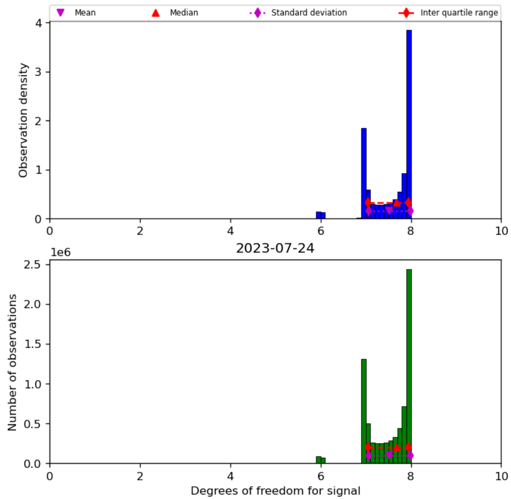
Figure 23: Histogram of “Degrees of freedom for signal” for 2023-07-24 to 2023-07-25
