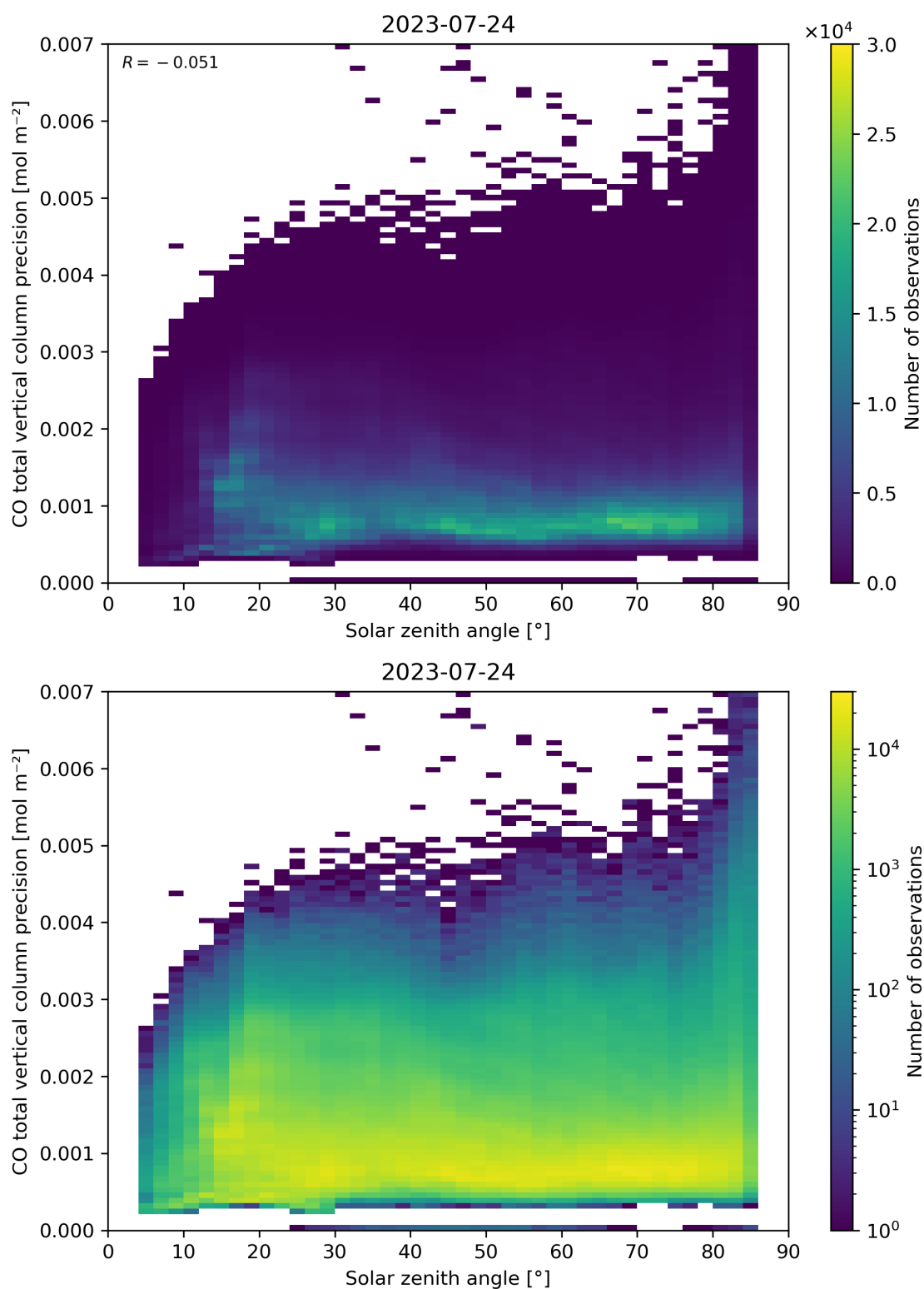
Figure 63: Scatter density plot of “Solar zenith angle” against “CO total vertical column precision” for 2023-07-24 to 2023-07-25.
