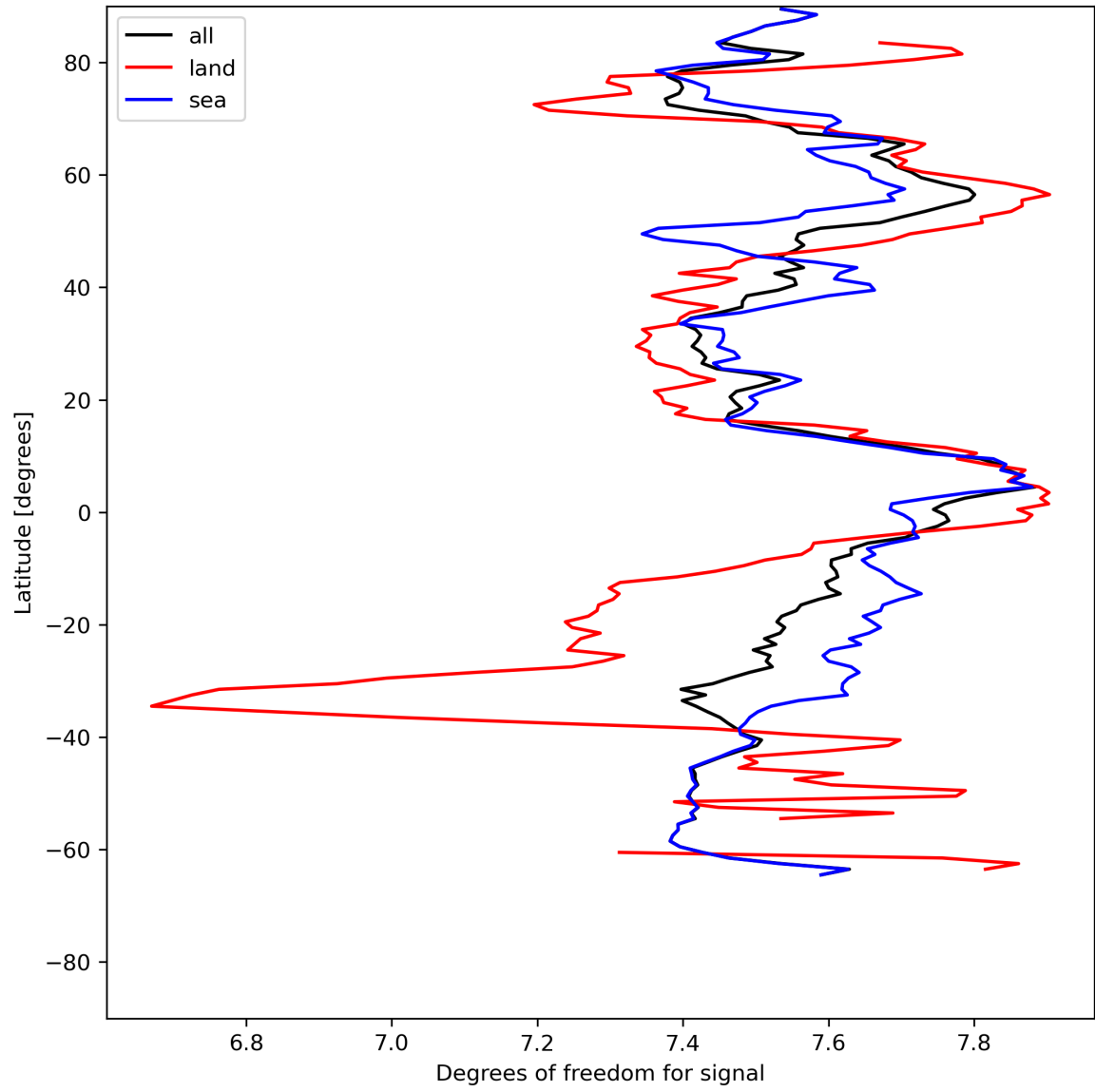
Figure 15: Zonal average of “Degrees of freedom for signal” for 2023-07-24 to 2023-07-25.
