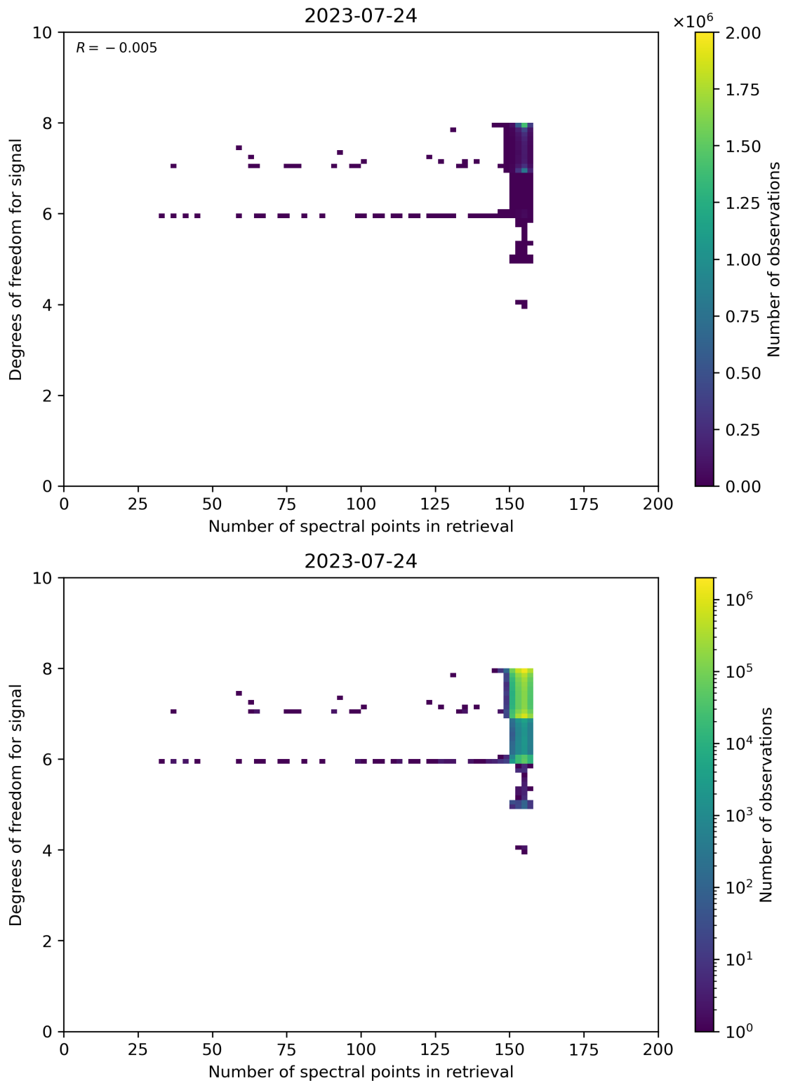
Figure 59: Scatter density plot of “Number of spectral points in retrieval” against “Degrees of freedom for signal” for 2023-07-24 to 2023-07-25.
