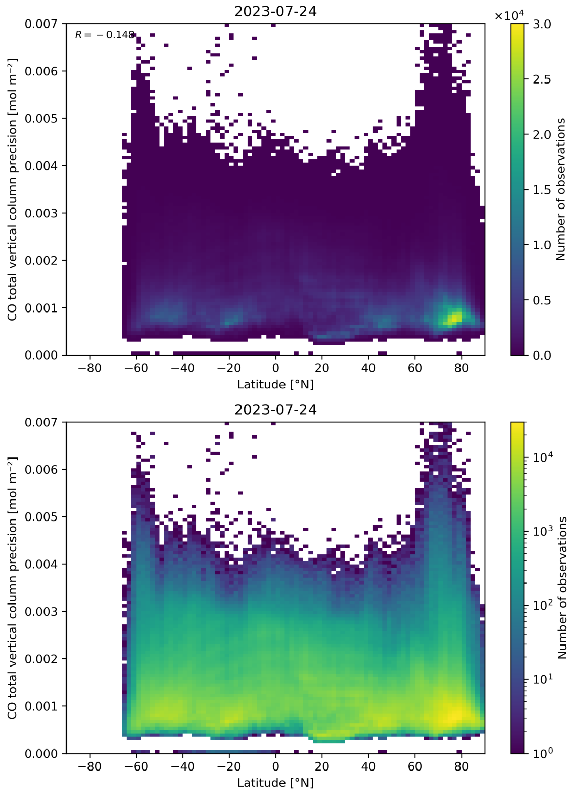
Figure 53: Scatter density plot of “Latitude” against “CO total vertical column precision” for 2023-07-24 to 2023-07-25.
