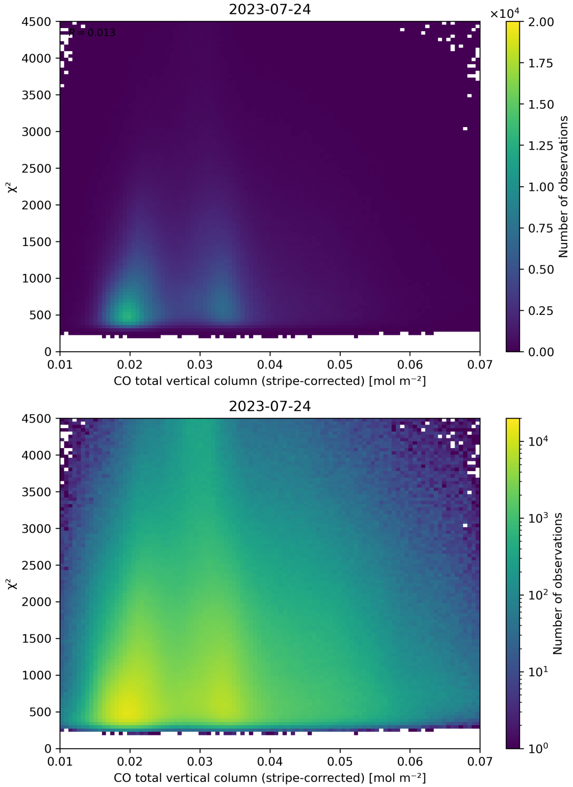
Figure 37: Scatter density plot of “CO total vertical column (stripe-corrected)” against “ \chi^2 ” for 2023-07-24 to 2023-07-25.
