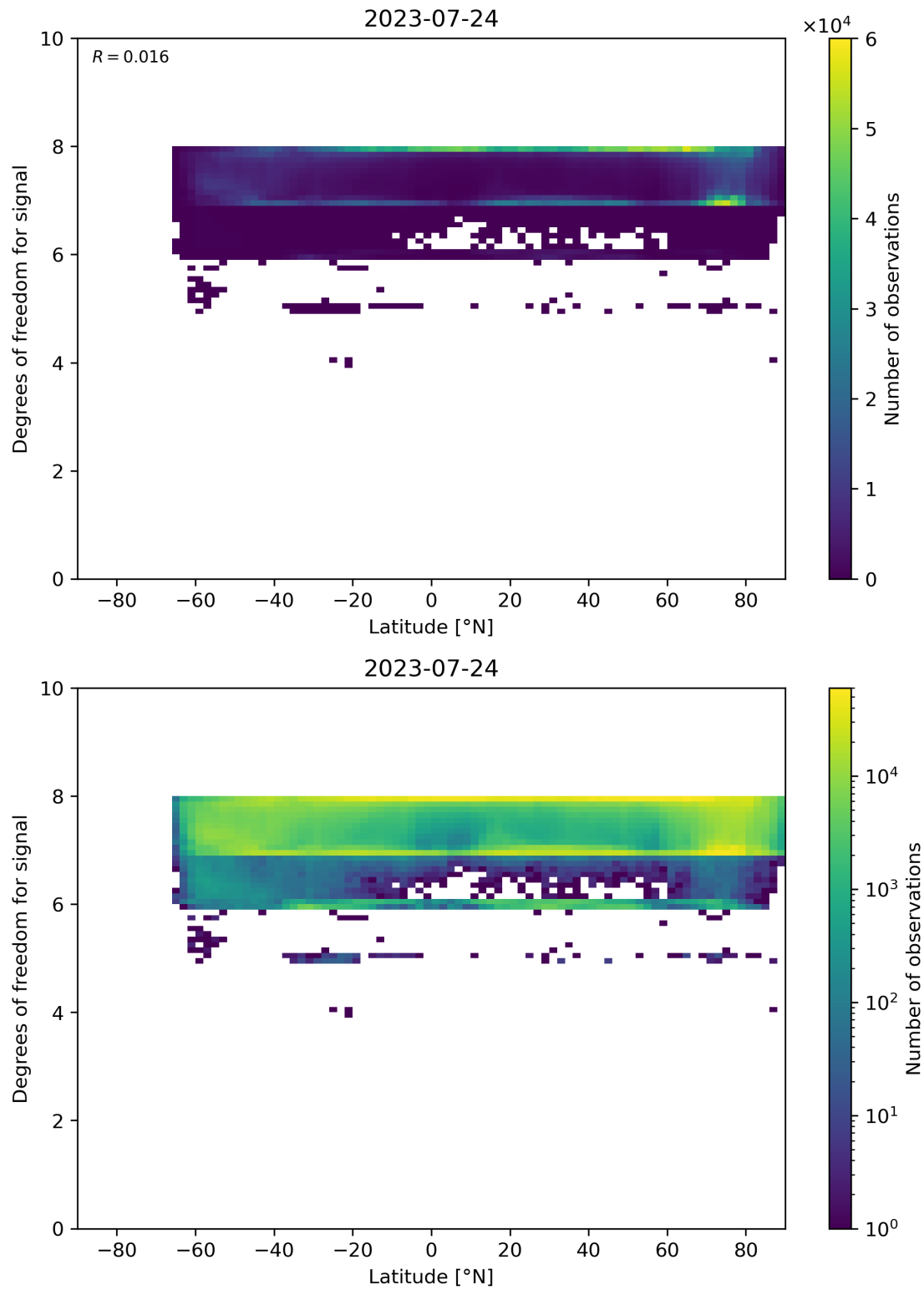
Figure 55: Scatter density plot of “Latitude” against “Degrees of freedom for signal” for 2023-07-24 to 2023-07-25.
