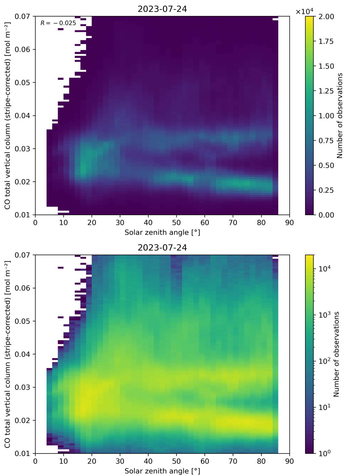
Figure 62: Scatter density plot of “Solar zenith angle” against “CO total vertical column (stripe-corrected)” for 2023-07-24 to 2023-07-25.
