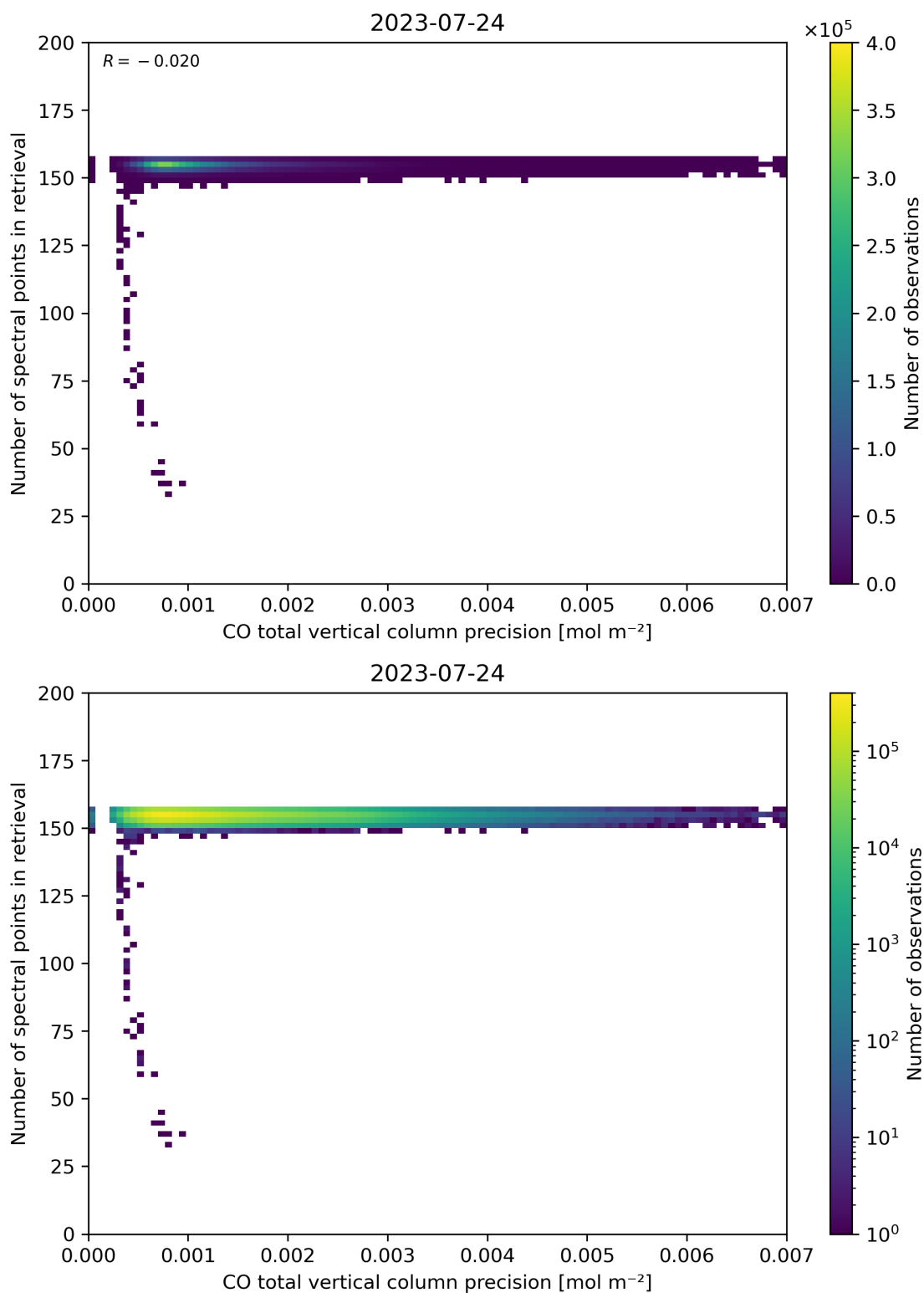
Figure 47: Scatter density plot of “CO total vertical column precision” against “Number of spectral points in retrieval” for 2023-07-24 to 2023-07-25.
