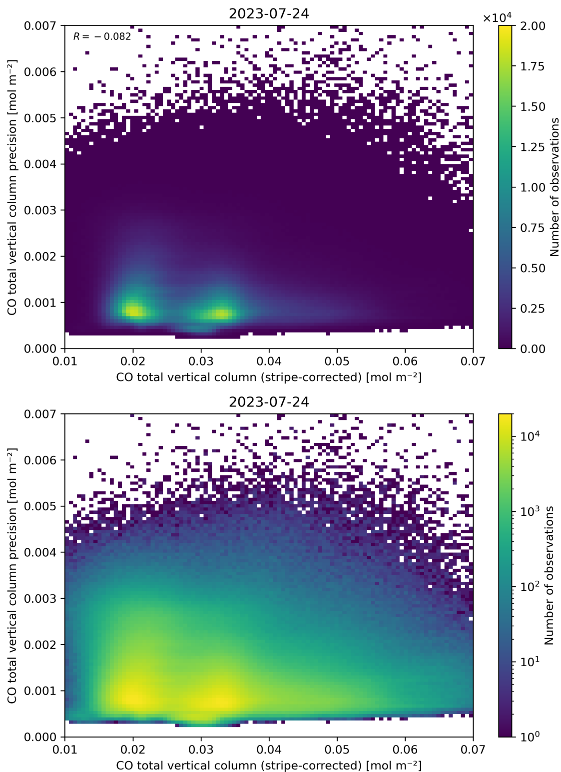
Figure 36: Scatter density plot of “CO total vertical column (stripe-corrected)” against “CO total vertical column precision” for 2023-07-24 to 2023-07-25.
