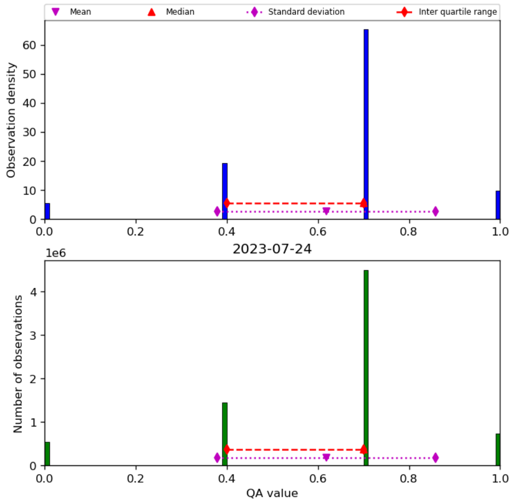
Figure 17: Histogram of “QA value” for 2023-07-24 to 2023-07-25
