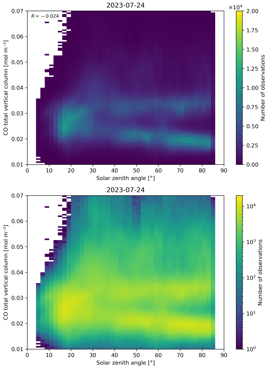
Figure 61: Scatter density plot of “Solar zenith angle” against “CO total vertical column” for 2023-07-24 to 2023-07-25.
