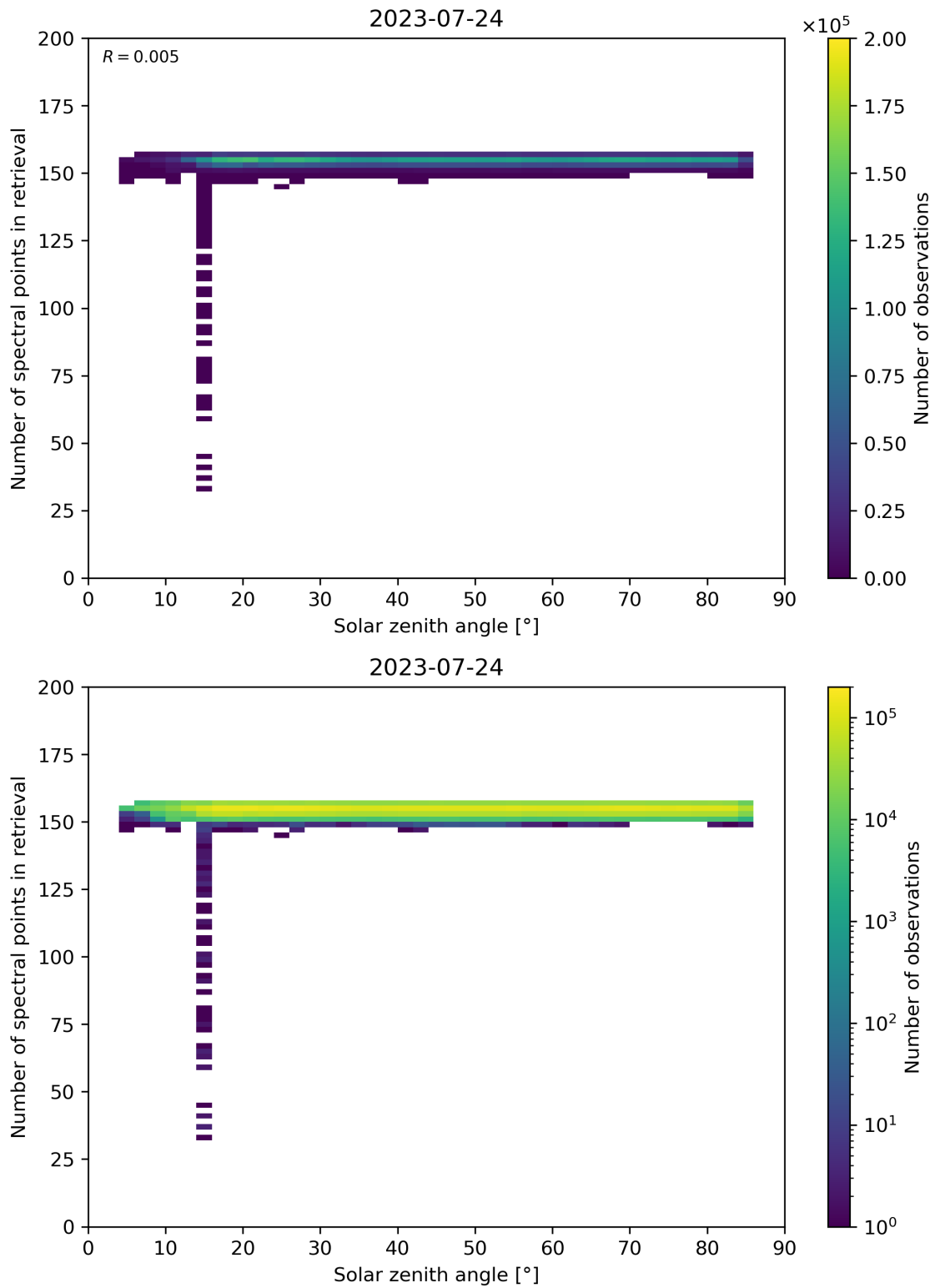
Figure 68: Scatter density plot of “Solar zenith angle” against “Number of spectral points in retrieval” for 2023-07-24 to 2023-07-25.
