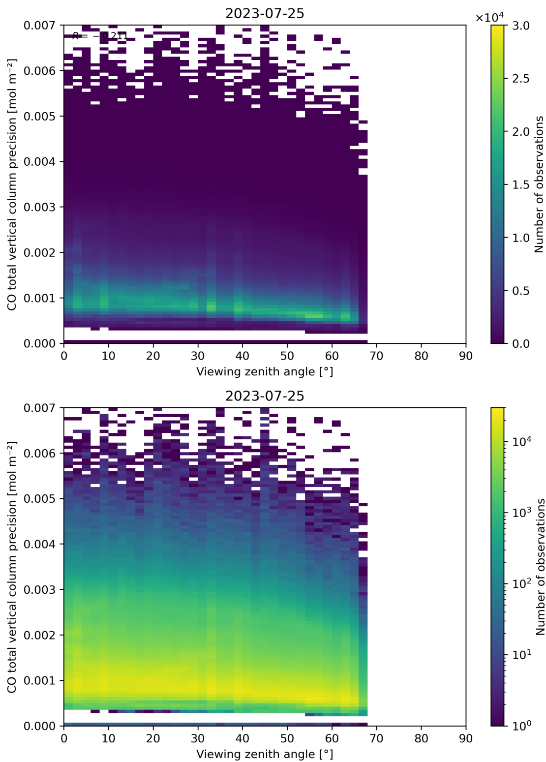
Figure 71: Scatter density plot of “Viewing zenith angle” against “CO total vertical column precision” for 2023-07-24 to 2023-07-26.
