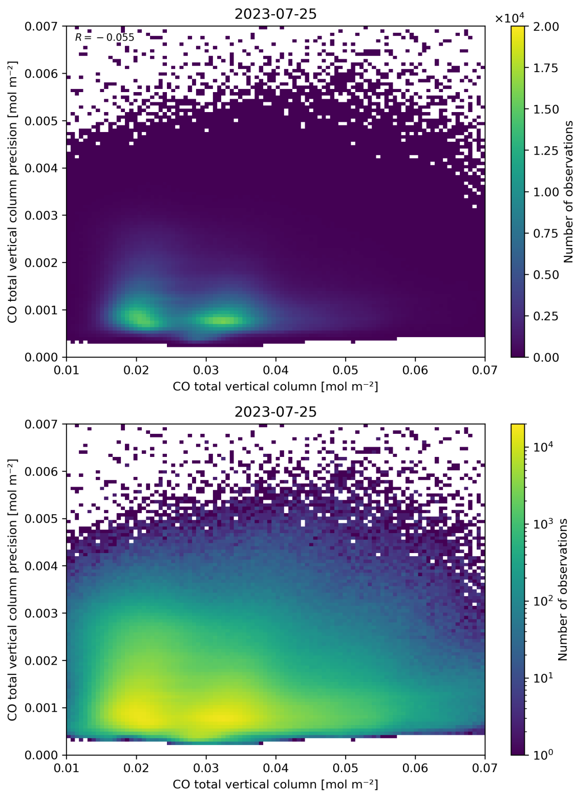
Figure 34: Scatter density plot of “CO total vertical column” against “CO total vertical column precision” for 2023-07-24 to 2023-07-26.
