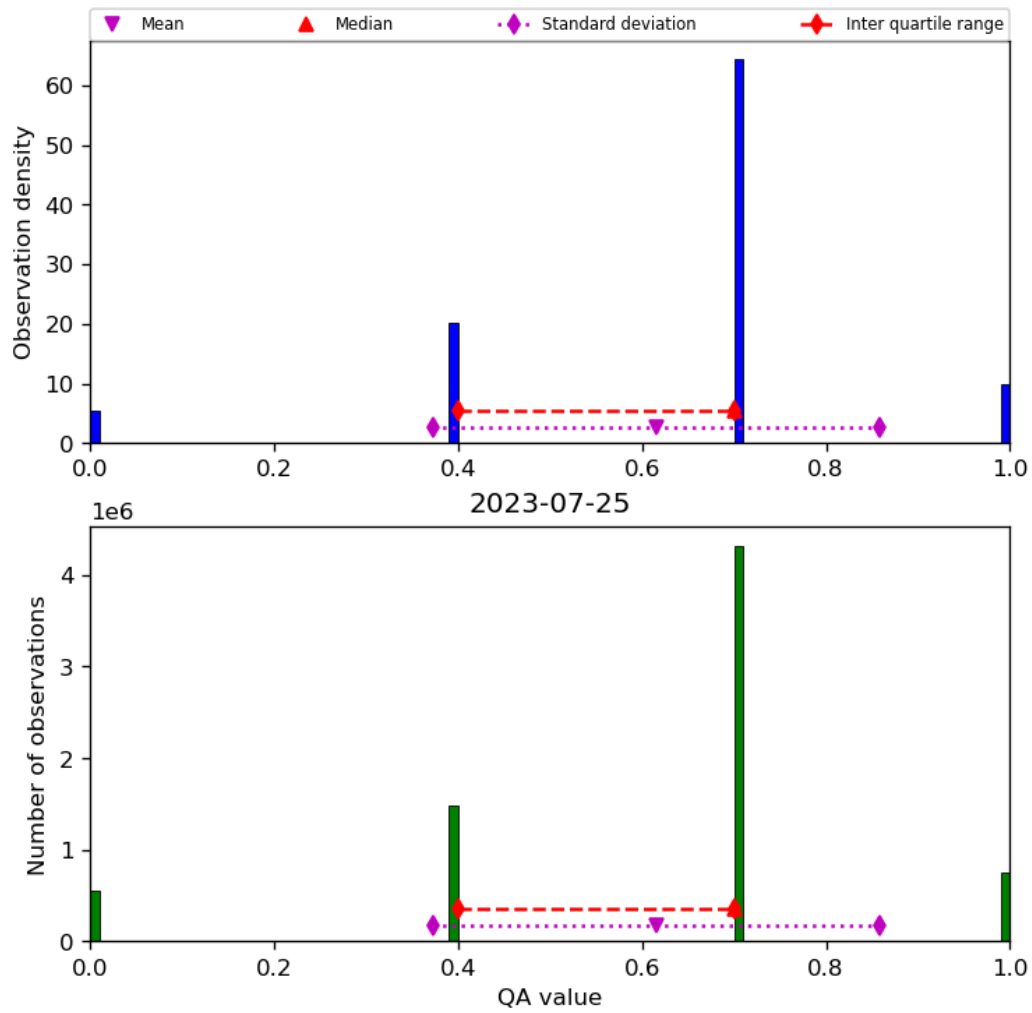
Figure 17: Histogram of “QA value” for 2023-07-24 to 2023-07-26
