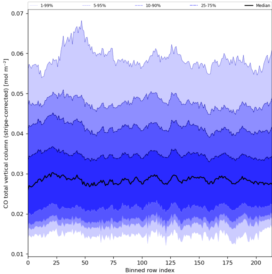
Figure 27: Along track statistics of “CO total vertical column (stripe-corrected)” for 2023-07-24 to 2023-07-26
