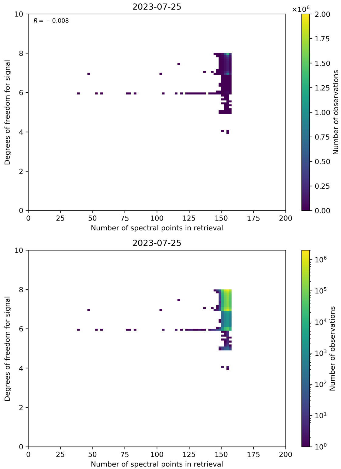
Figure 59: Scatter density plot of “Number of spectral points in retrieval” against “Degrees of freedom for signal” for 2023-07-24 to 2023-07-26.
