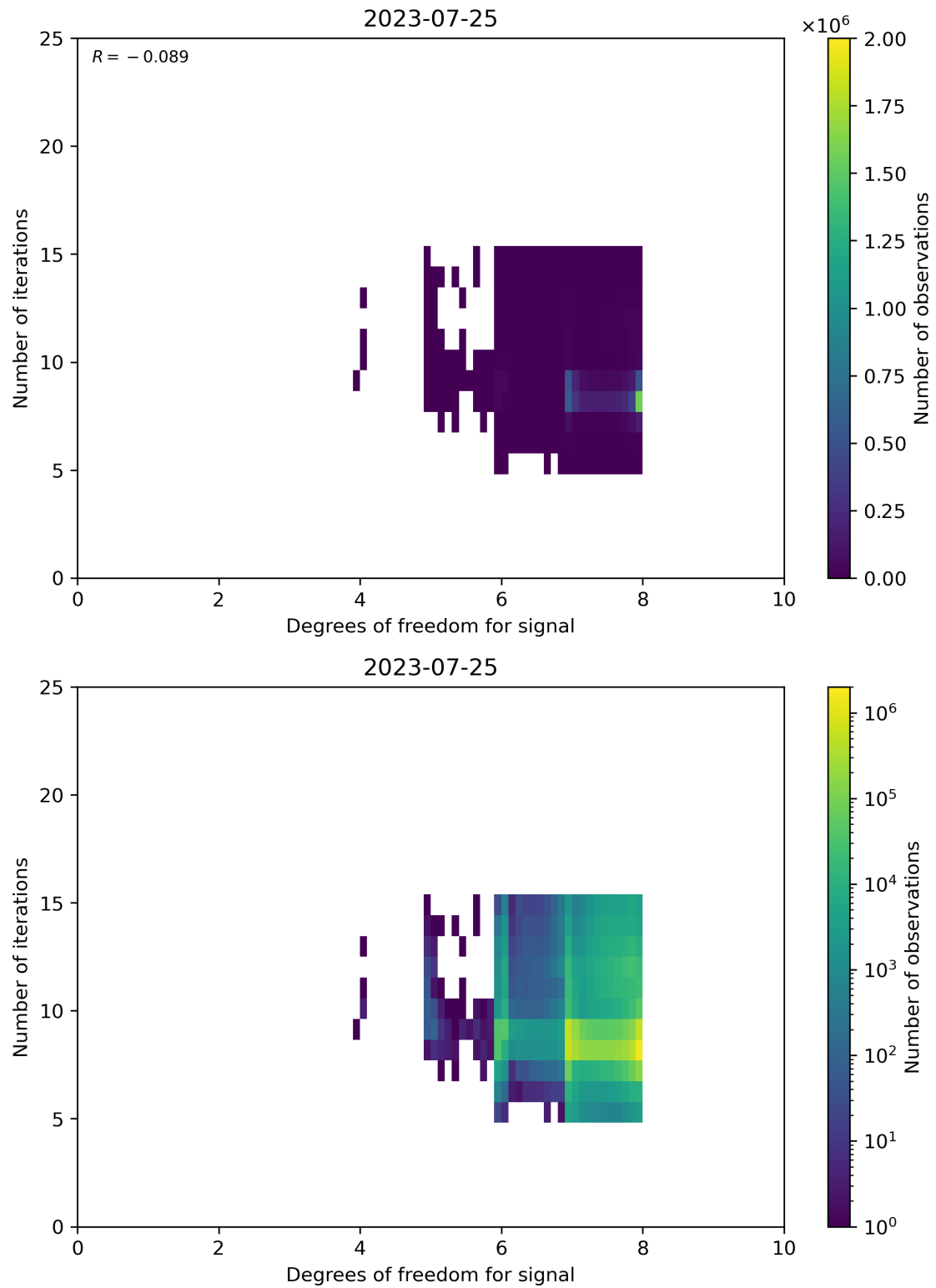
Figure 50: Scatter density plot of “Degrees of freedom for signal” against “Number of iterations” for 2023-07-24 to 2023-07-26.
