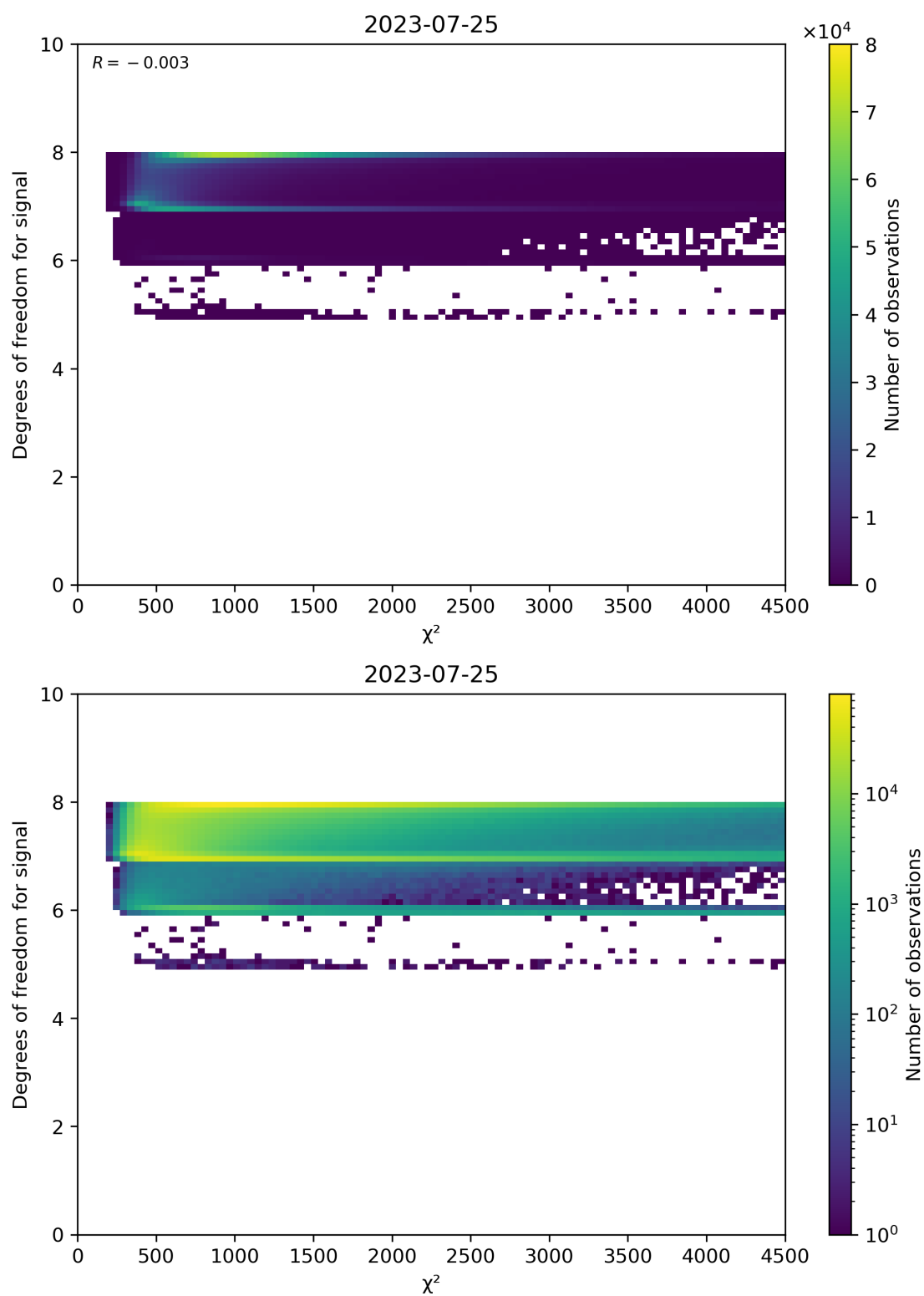
Figure 48: Scatter density plot of “ \chi^2 ” against “Degrees of freedom for signal” for 2023-07-24 to 2023-07-26.
