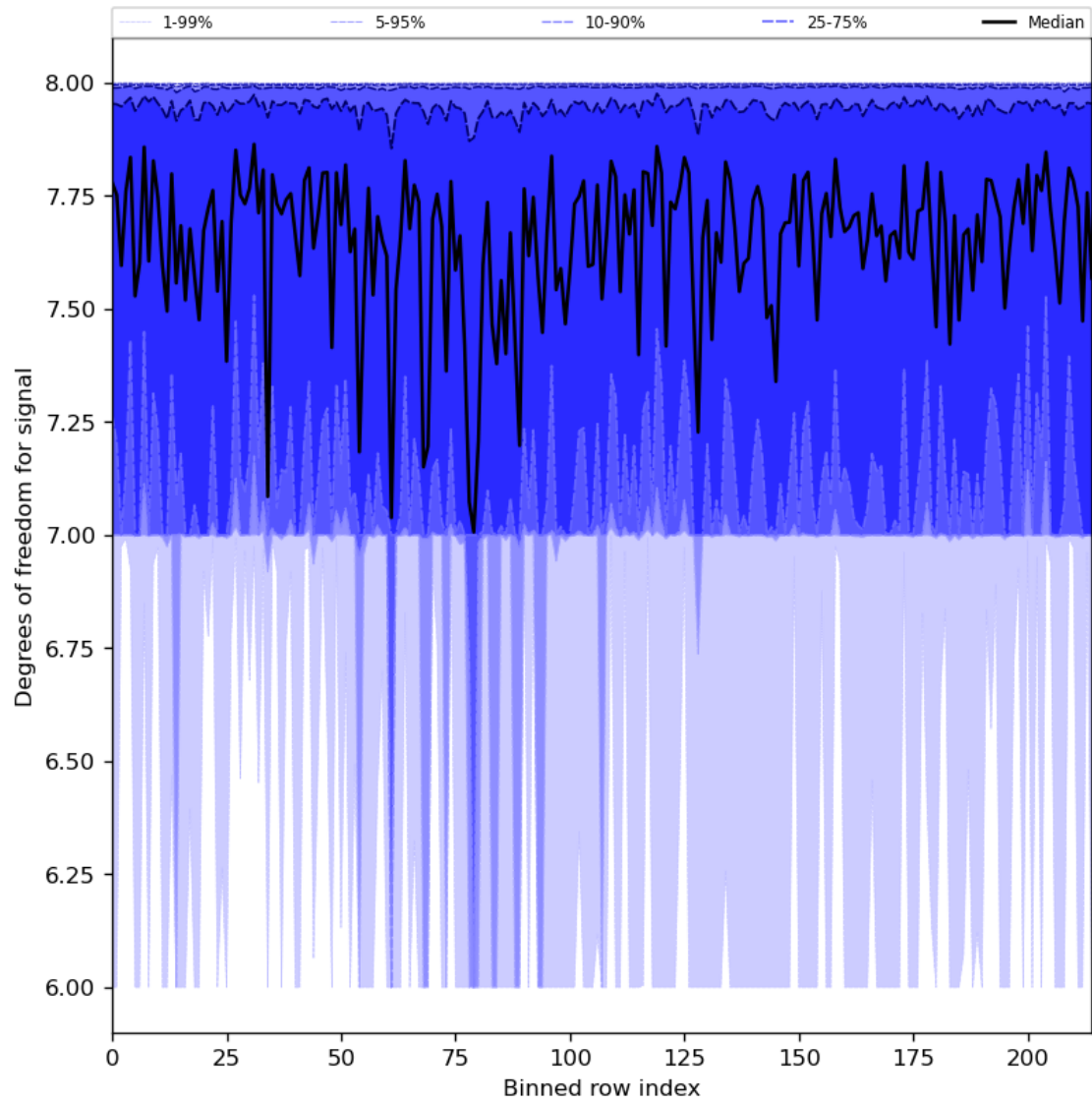
Figure 31: Along track statistics of “Degrees of freedom for signal” for 2023-07-25 to 2023-07-27
