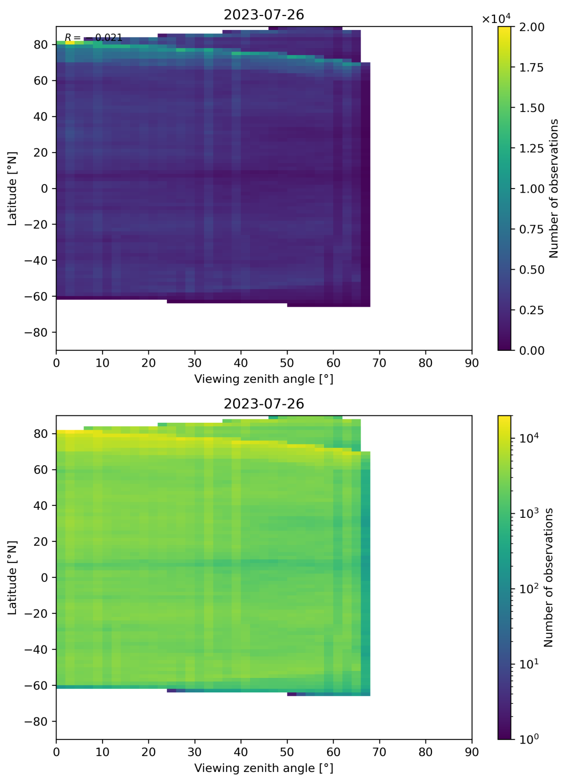
Figure 74: Scatter density plot of “Viewing zenith angle” against “Latitude” for 2023-07-25 to 2023-07-27.
