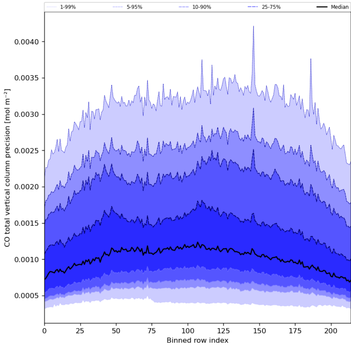
Figure 28: Along track statistics of “CO total vertical column precision” for 2023-07-25 to 2023-07-27
