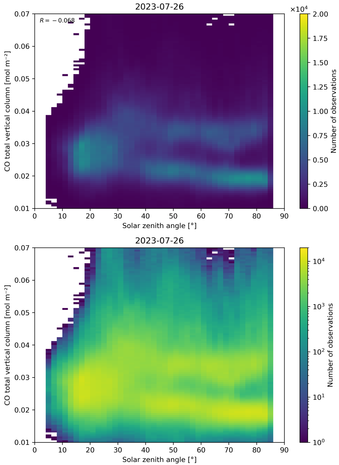
Figure 61: Scatter density plot of “Solar zenith angle” against “CO total vertical column” for 2023-07-25 to 2023-07-27.
