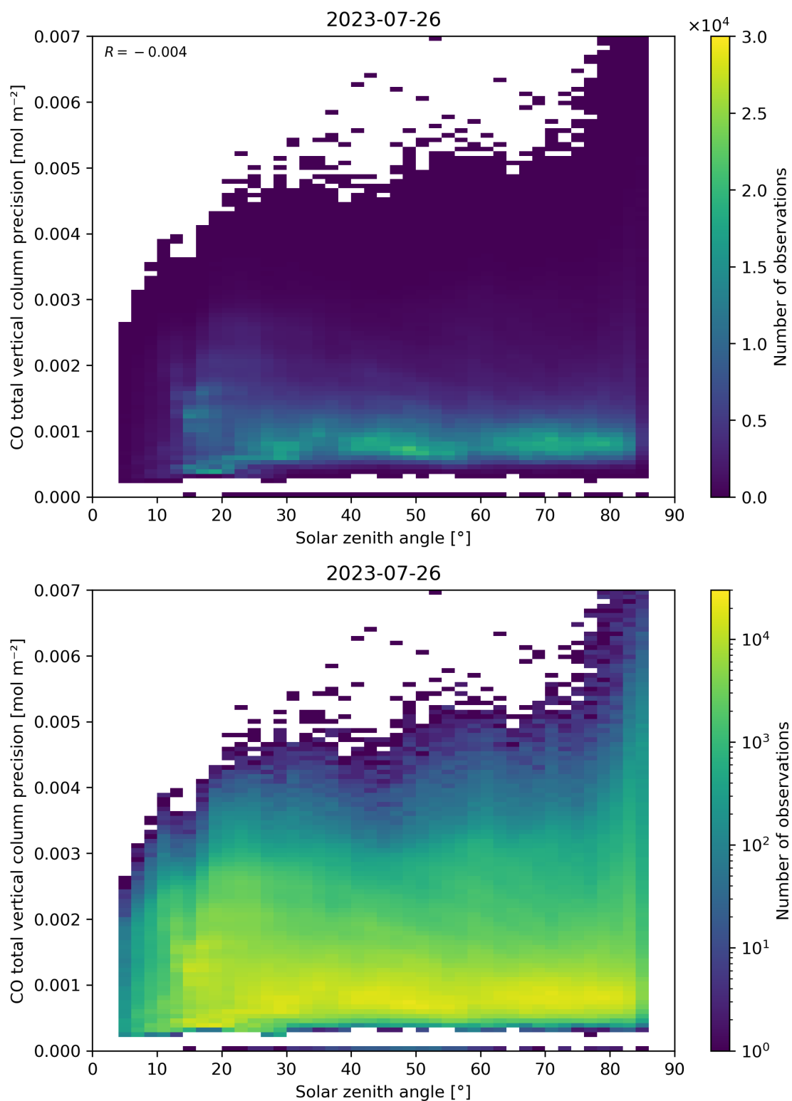
Figure 63: Scatter density plot of “Solar zenith angle” against “CO total vertical column precision” for 2023-07-25 to 2023-07-27.
