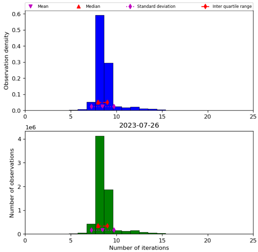
Figure 24: Histogram of “Number of iterations” for 2023-07-25 to 2023-07-27
