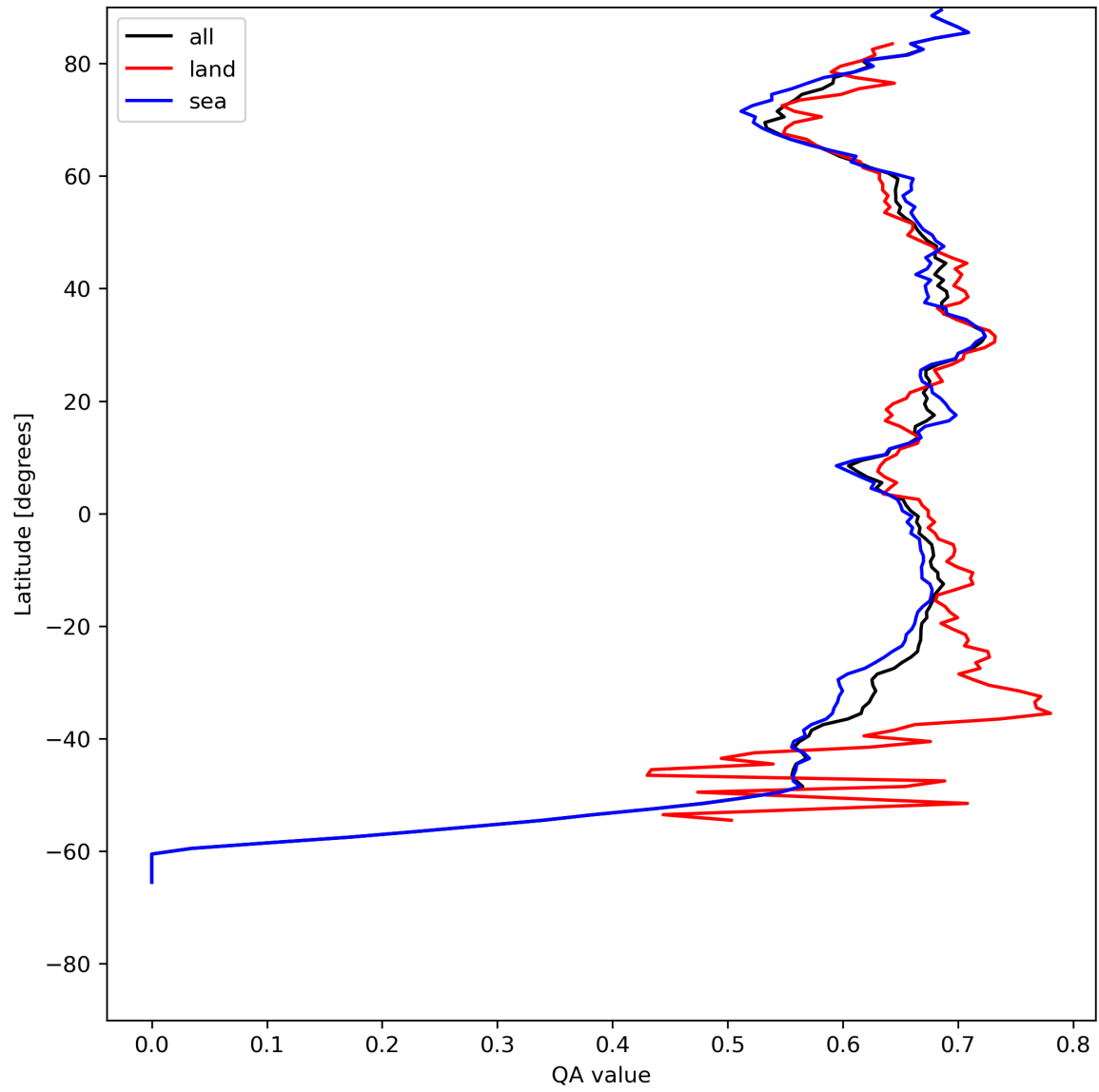
Figure 9: Zonal average of “QA value” for 2023-07-25 to 2023-07-27.
