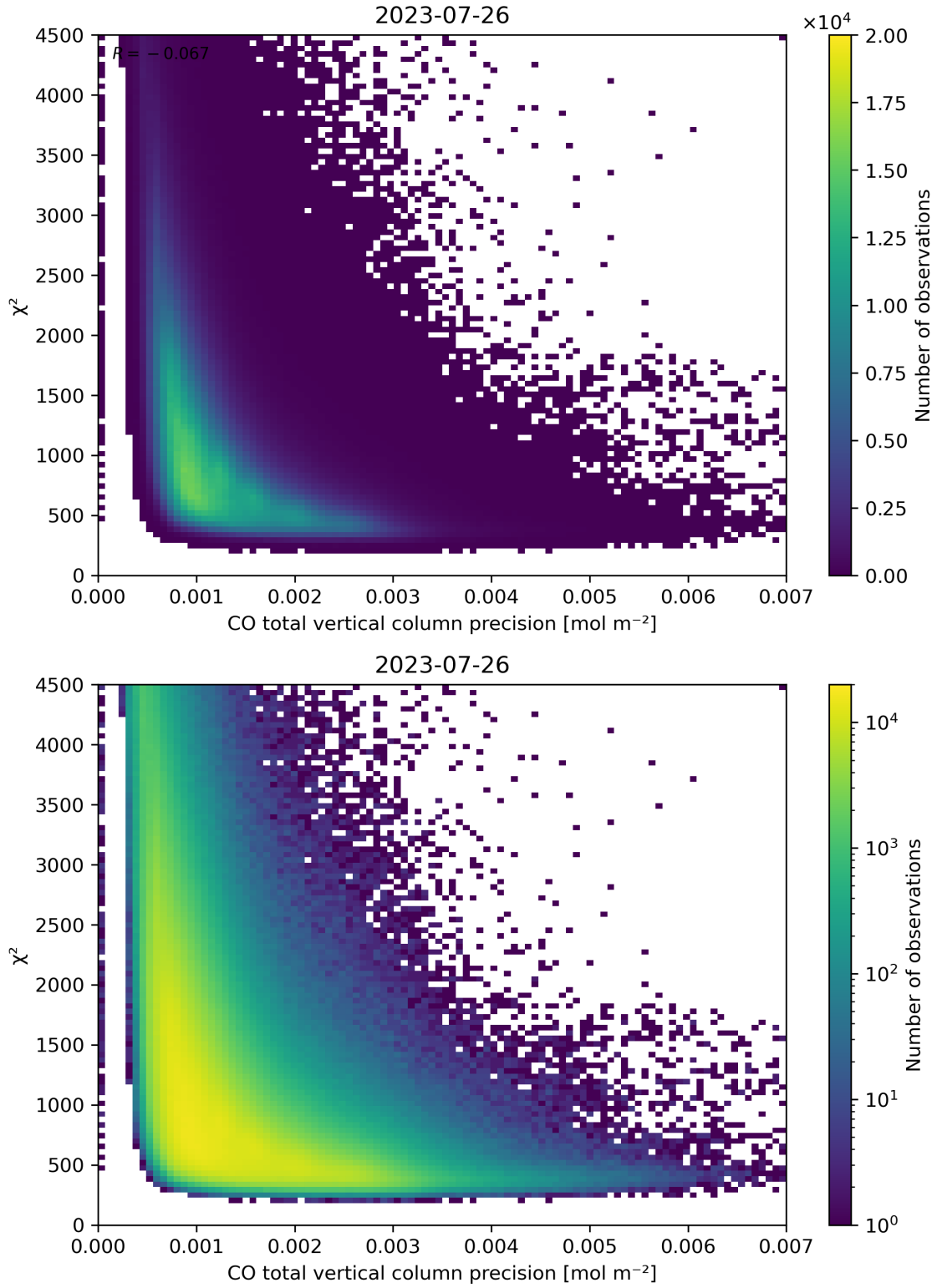
Figure 44: Scatter density plot of “CO total vertical column precision” against “ \chi^2 ” for 2023-07-25 to 2023-07-27.
