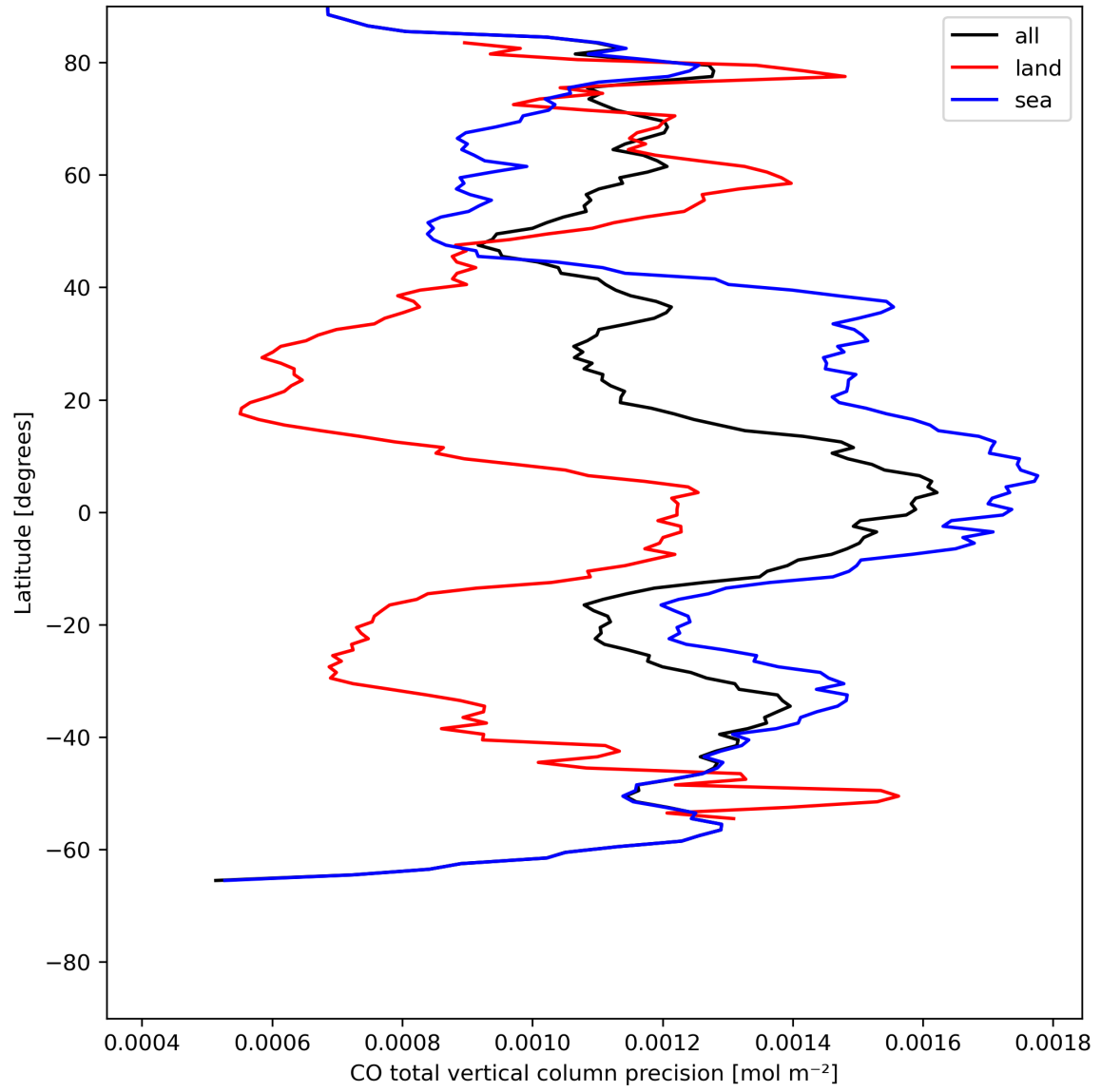
Figure 12: Zonal average of "CO total vertical column precision" for 2023-07-25 to 2023-07-27.
