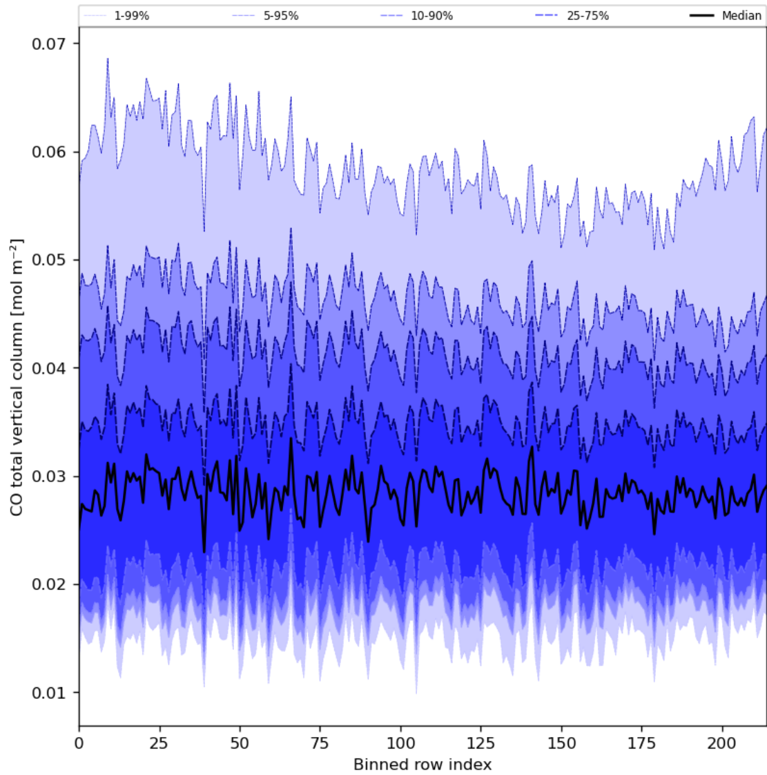
Figure 26: Along track statistics of “CO total vertical column” for 2023-07-25 to 2023-07-27
