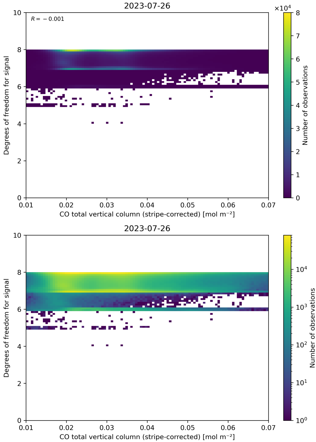
Figure 38: Scatter density plot of “CO total vertical column (stripe-corrected)” against “Degrees of freedom for signal” for 2023-07-25 to 2023-07-27.
