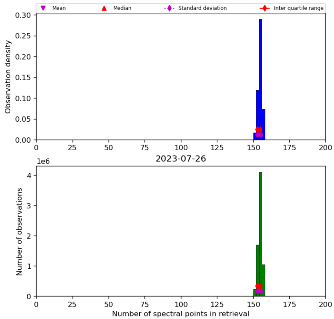
Figure 21: Histogram of “Number of spectral points in retrieval” for 2023-07-25 to 2023-07-27
