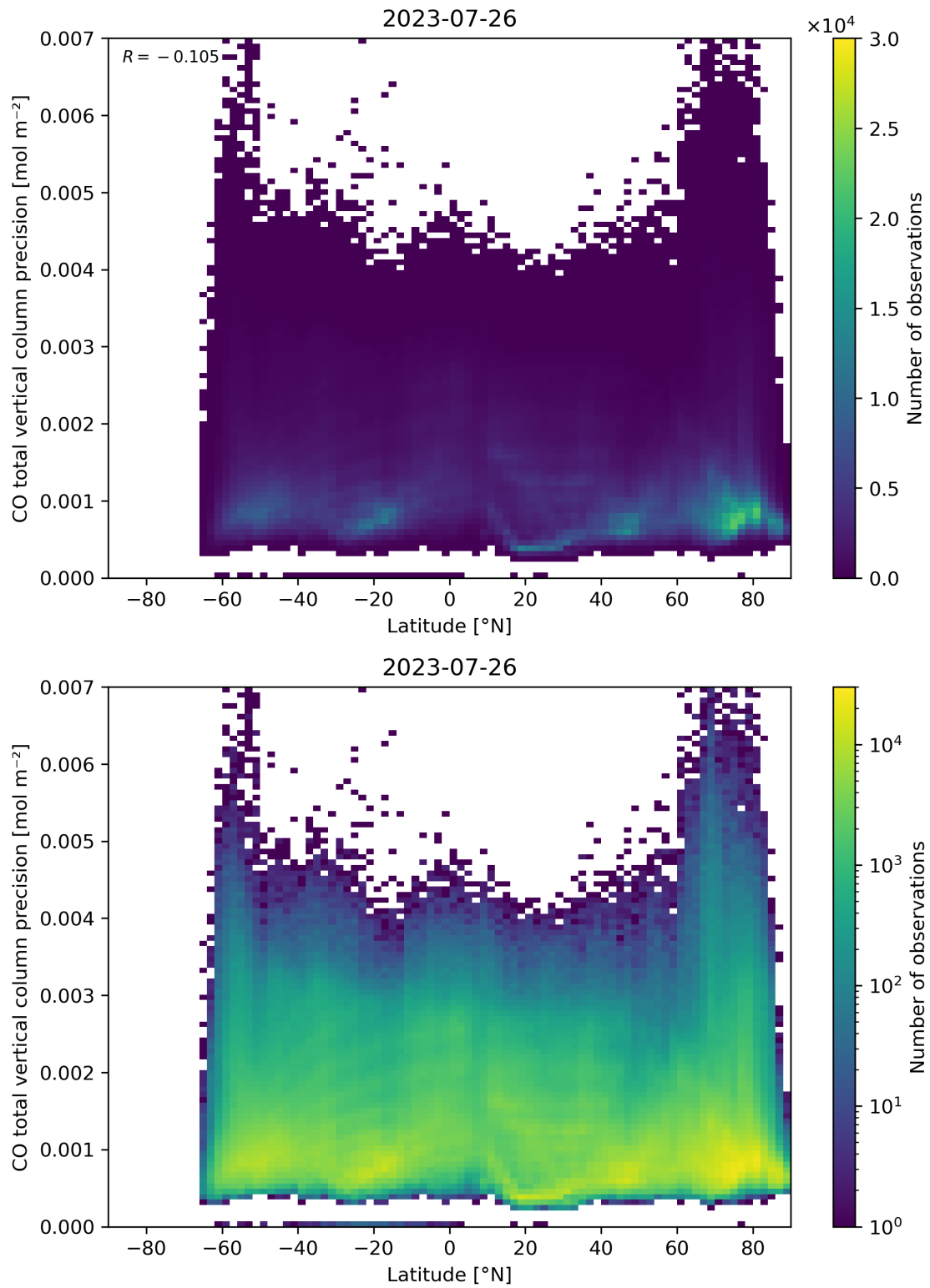
Figure 53: Scatter density plot of “Latitude” against “CO total vertical column precision” for 2023-07-25 to 2023-07-27.
