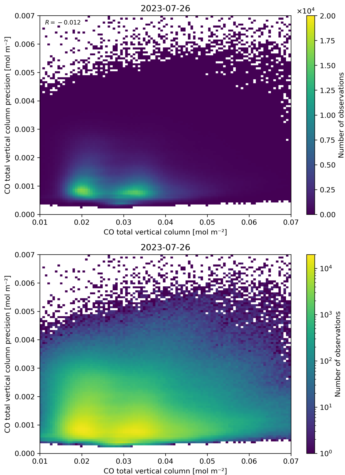
Figure 34: Scatter density plot of “CO total vertical column” against “CO total vertical column precision” for 2023-07-25 to 2023-07-27.
