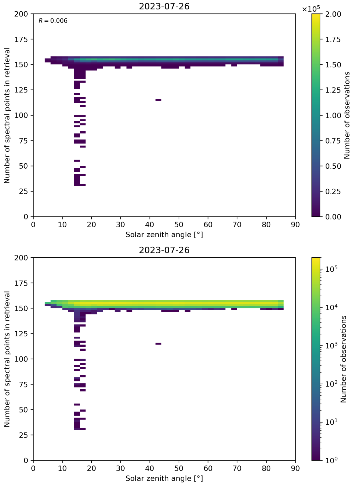
Figure 68: Scatter density plot of “Solar zenith angle” against “Number of spectral points in retrieval” for 2023-07-25 to 2023-07-27.
