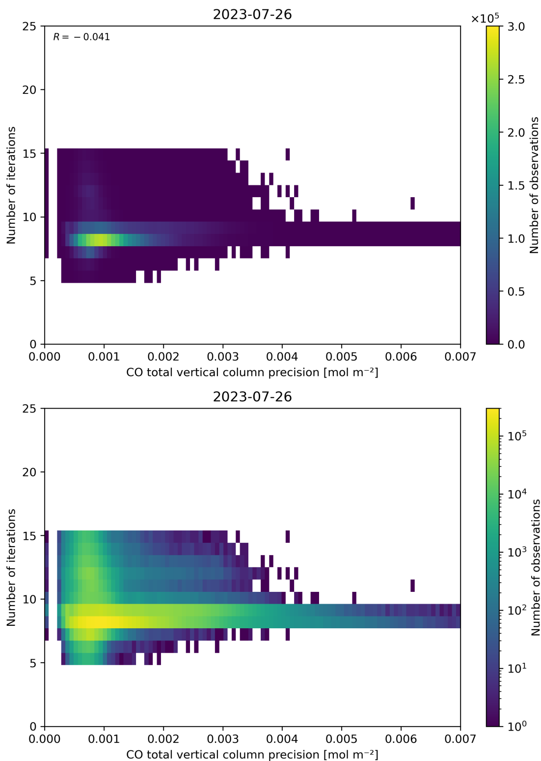
Figure 46: Scatter density plot of “CO total vertical column precision” against “Number of iterations” for 2023-07-25 to 2023-07-27.
