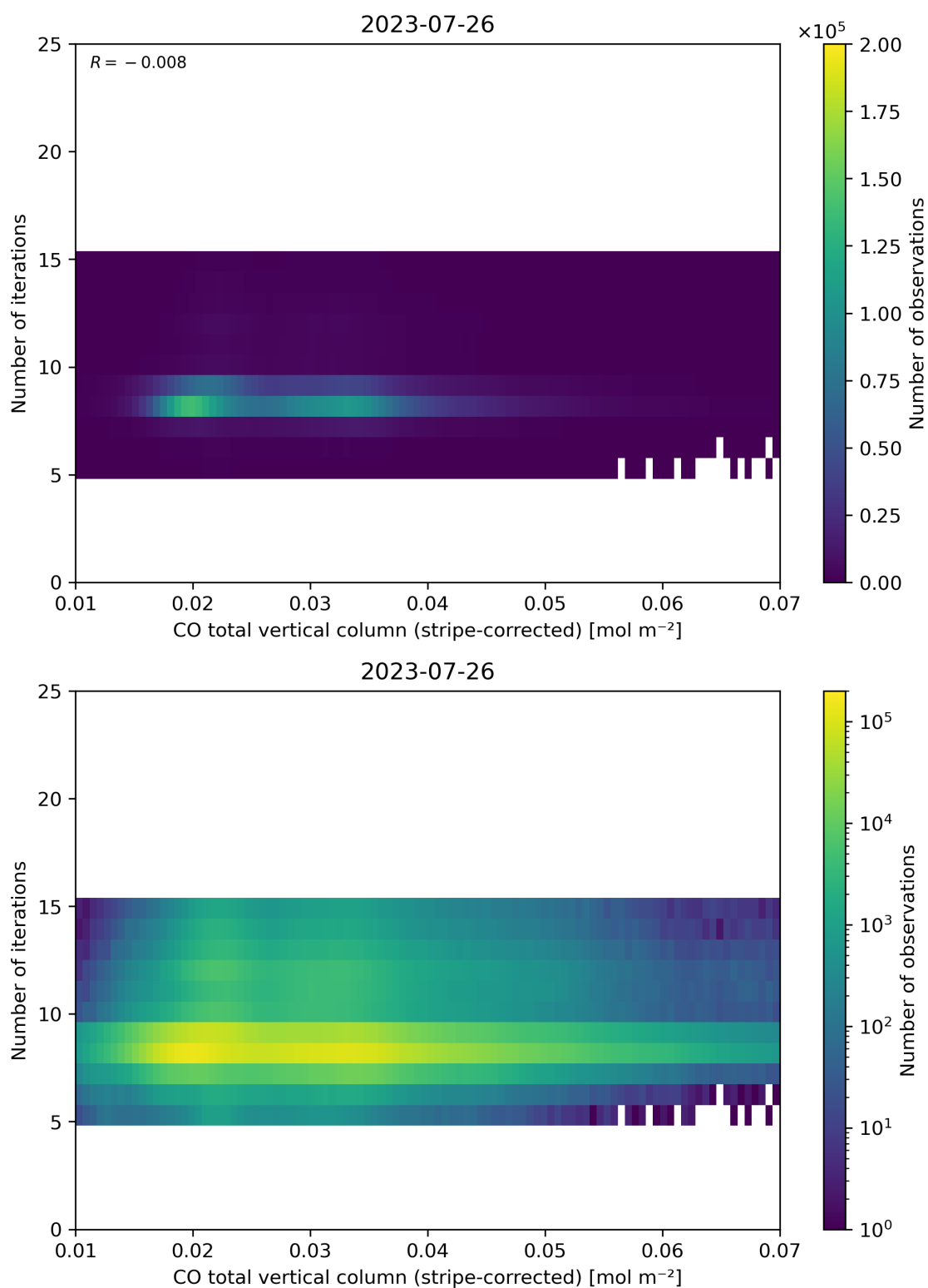
Figure 39: Scatter density plot of “CO total vertical column (stripe-corrected)” against “Number of iterations” for 2023-07-25 to 2023-07-27.
