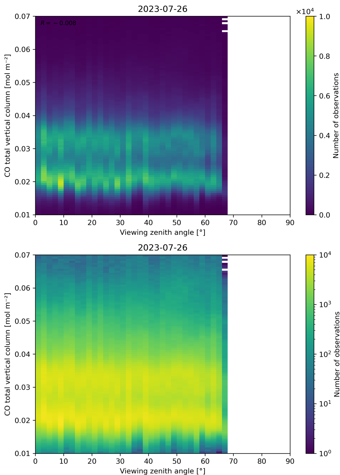
Figure 69: Scatter density plot of “Viewing zenith angle” against “CO total vertical column” for 2023-07-25 to 2023-07-27.
