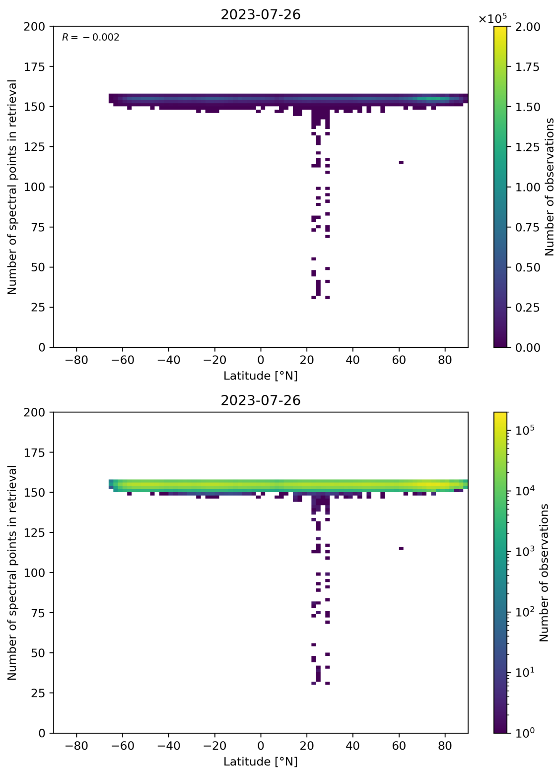
Figure 57: Scatter density plot of “Latitude” against “Number of spectral points in retrieval” for 2023-07-25 to 2023-07-27.
