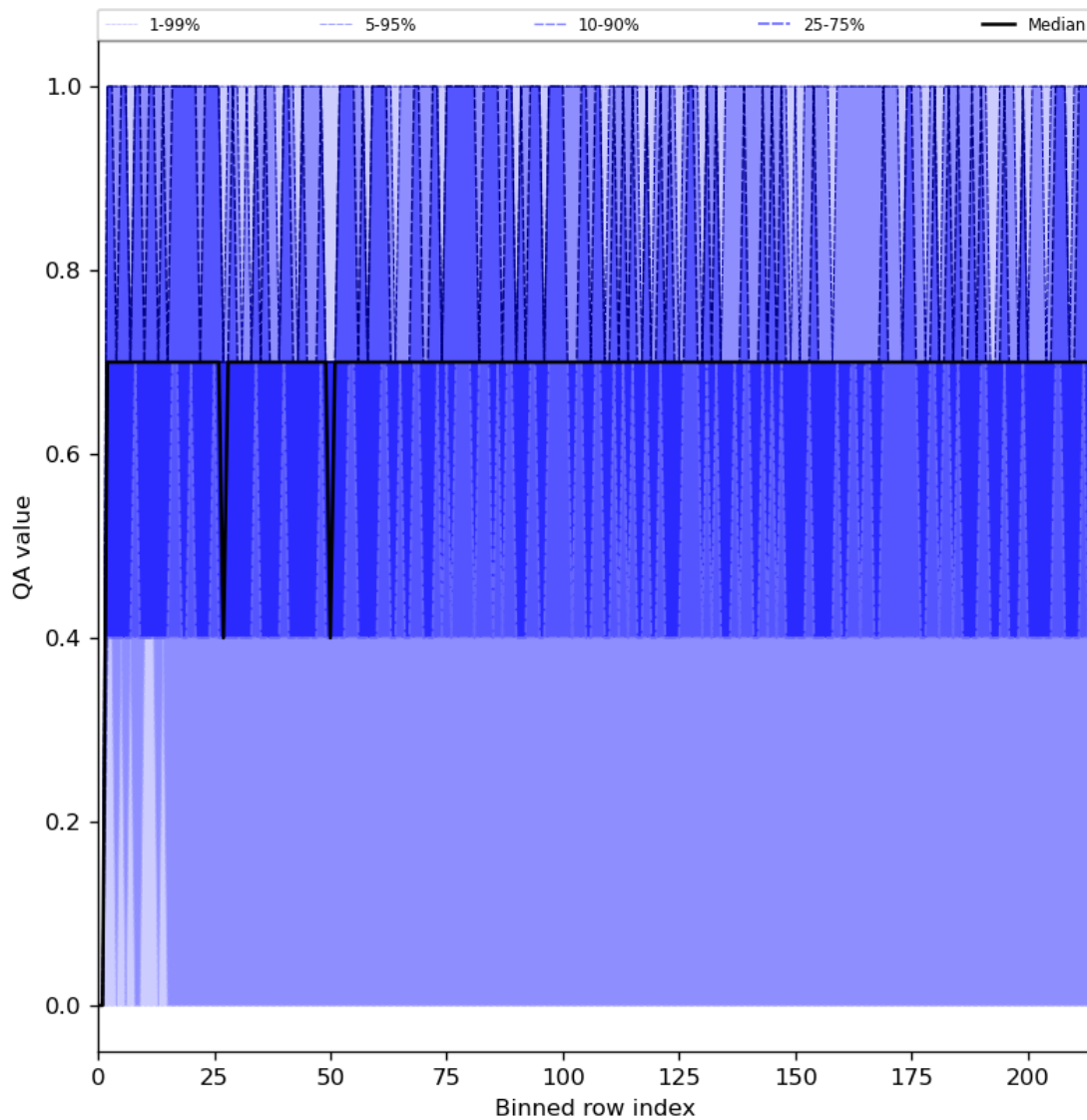
Figure 25: Along track statistics of “QA value” for 2023-07-25 to 2023-07-27
