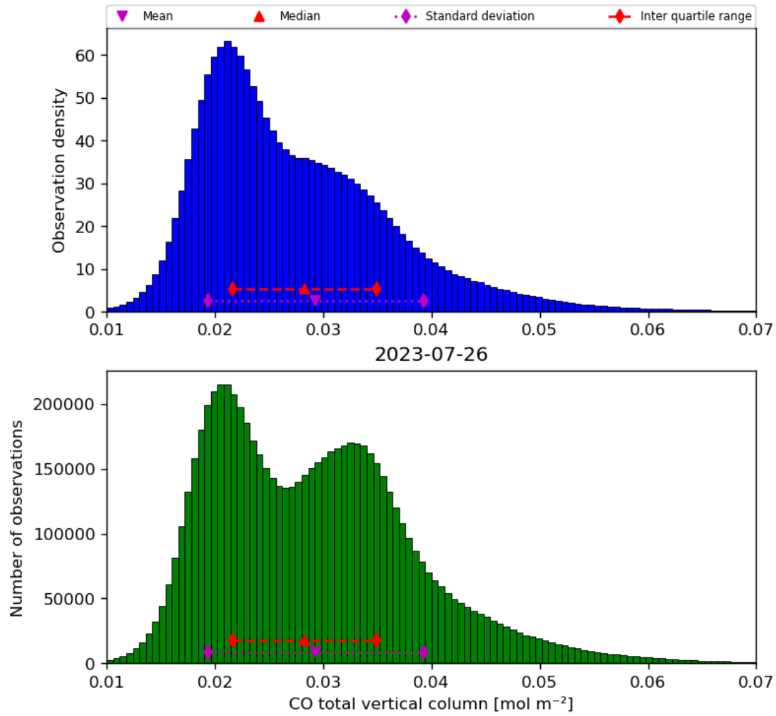
Figure 18: Histogram of “CO total vertical column” for 2023-07-25 to 2023-07-27
