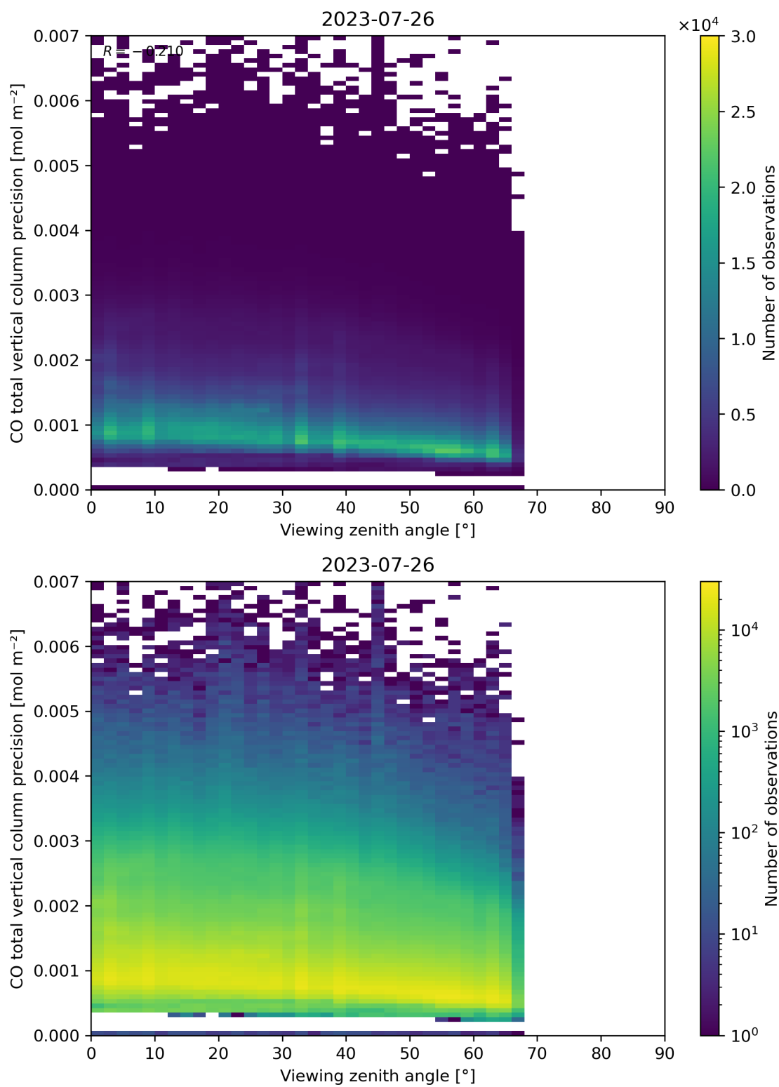
Figure 71: Scatter density plot of “Viewing zenith angle” against “CO total vertical column precision” for 2023-07-25 to 2023-07-27.
