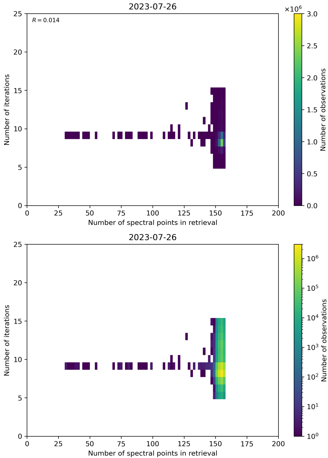
Figure 60: Scatter density plot of “Number of spectral points in retrieval” against “Number of iterations” for 2023-07-25 to 2023-07-27.
