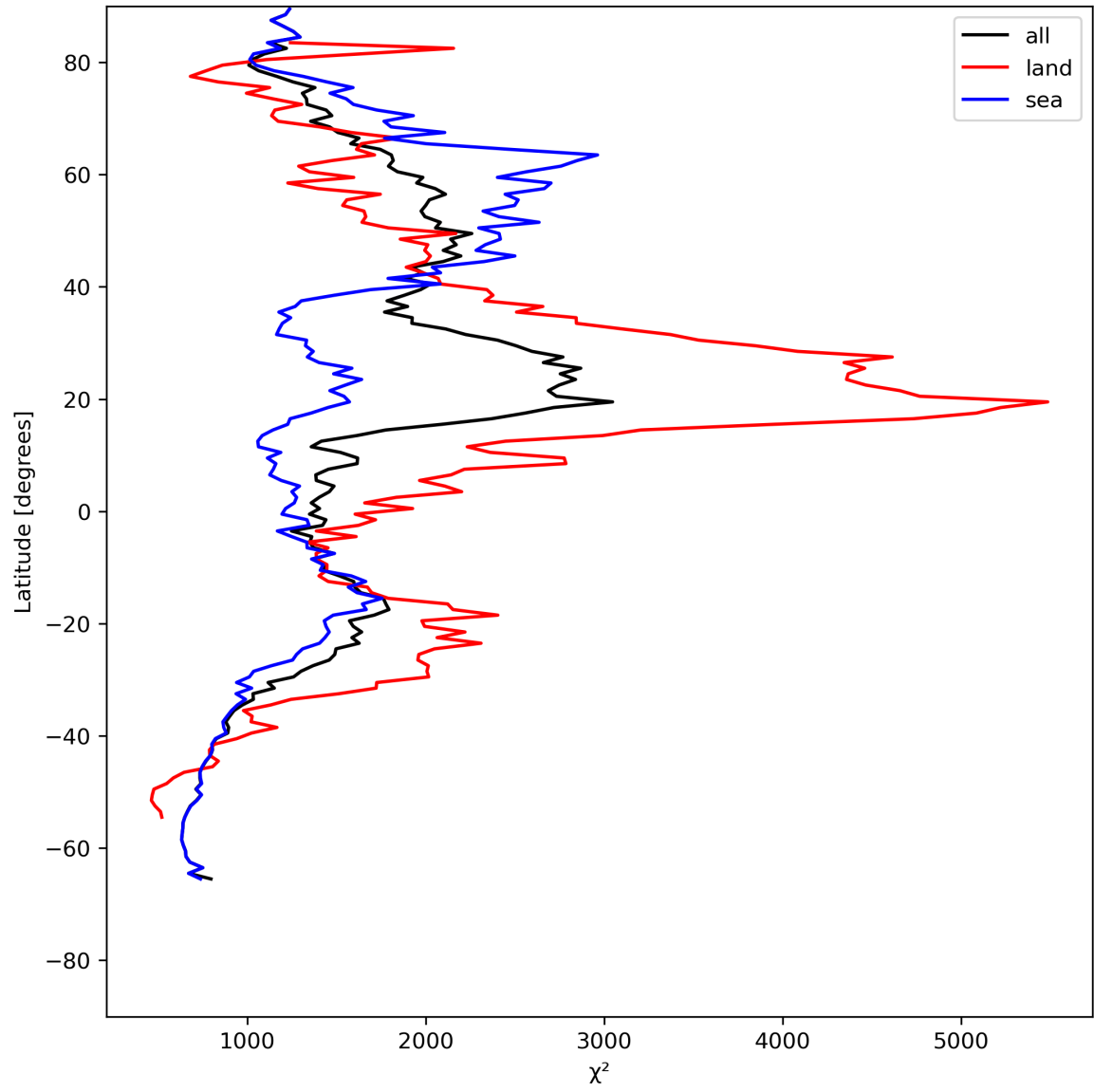
Figure 14: Zonal average of “ \chi^2 ” for 2023-07-25 to 2023-07-27.
