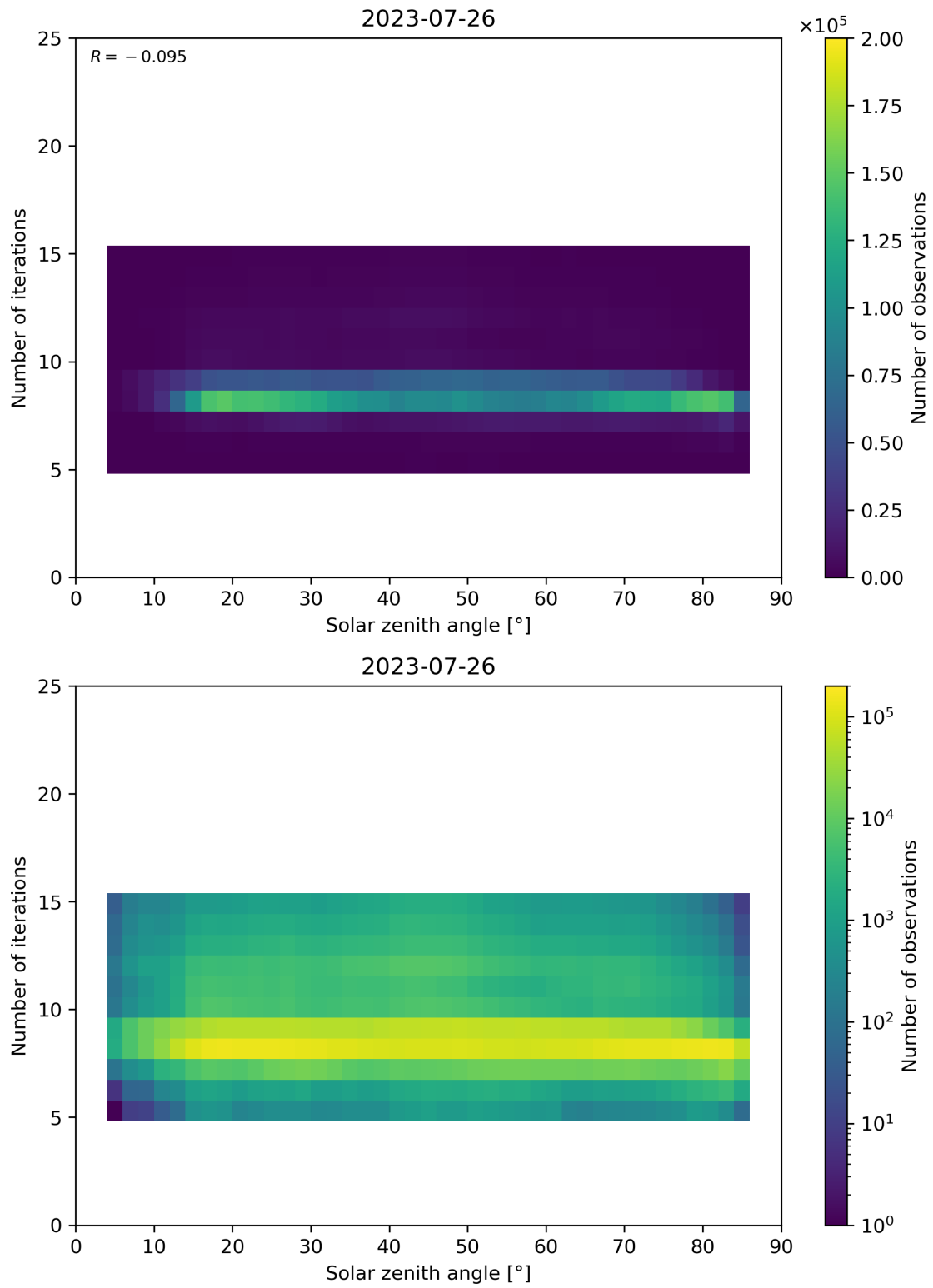
Figure 67: Scatter density plot of “Solar zenith angle” against “Number of iterations” for 2023-07-25 to 2023-07-27.
