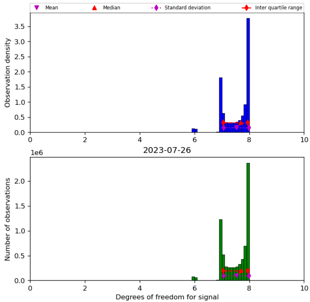
Figure 23: Histogram of “Degrees of freedom for signal” for 2023-07-25 to 2023-07-27
