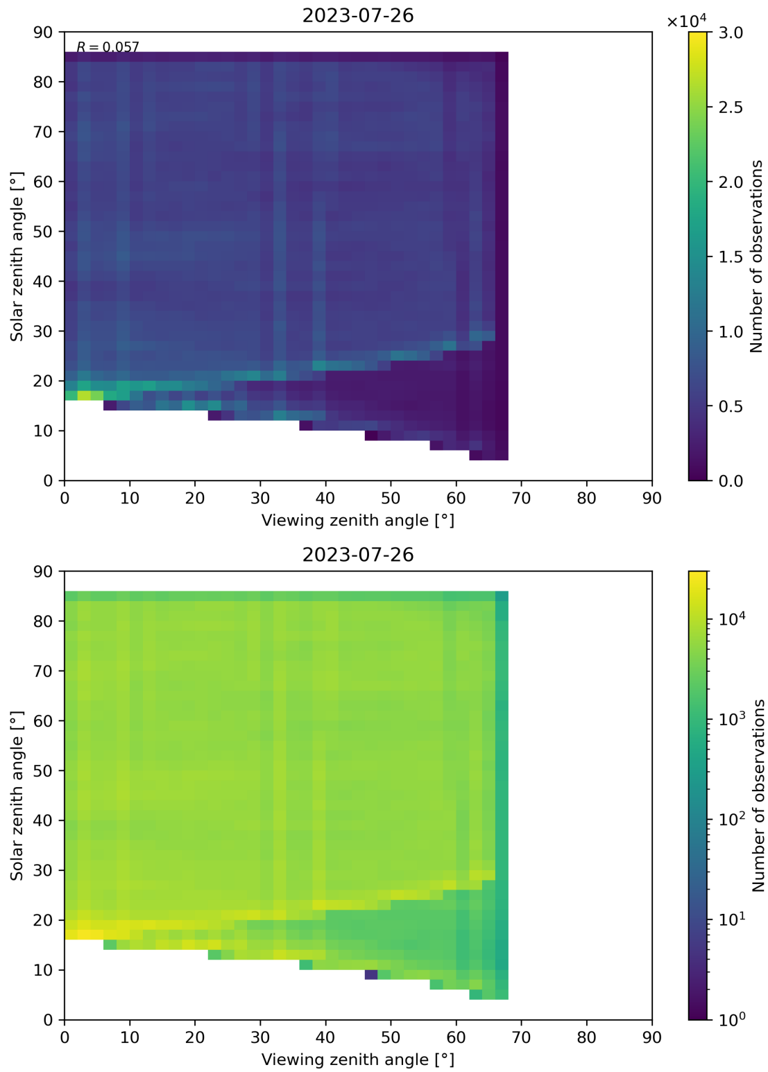
Figure 77: Scatter density plot of “Viewing zenith angle” against “Solar zenith angle” for 2023-07-25 to 2023-07-27.
