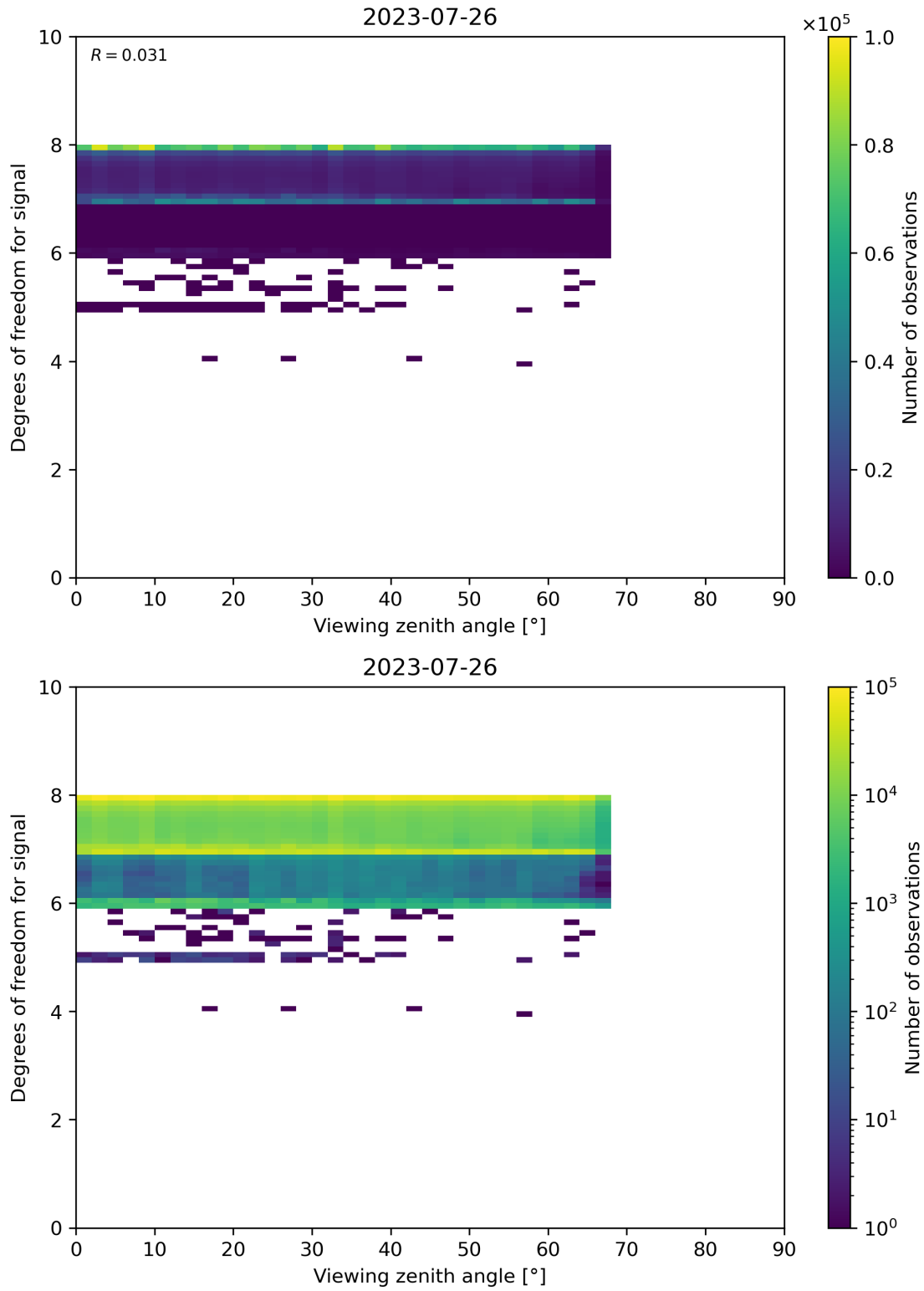
Figure 73: Scatter density plot of “Viewing zenith angle” against “Degrees of freedom for signal” for 2023-07-25 to 2023-07-27.
