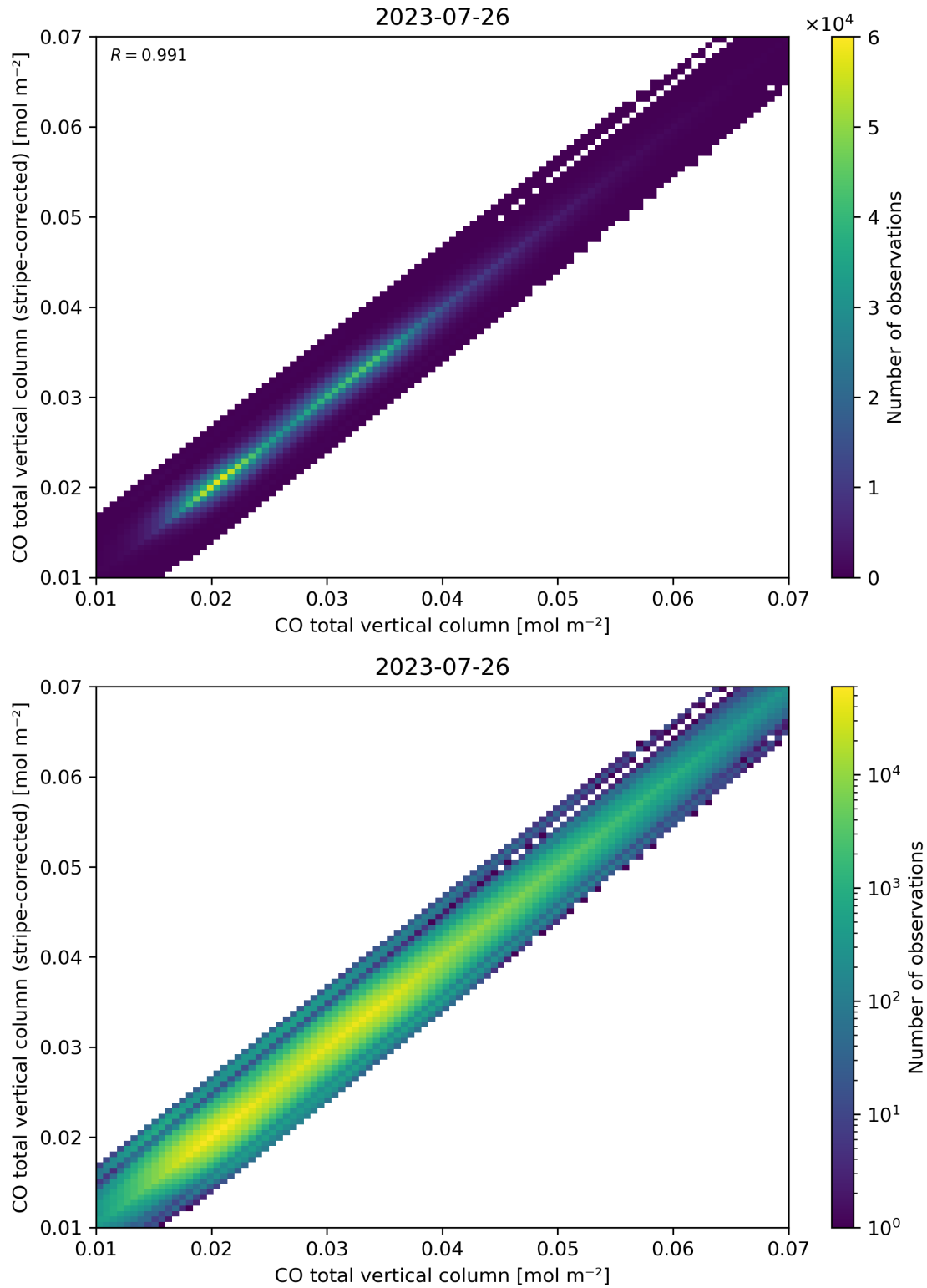
Figure 33: Scatter density plot of “CO total vertical column” against “CO total vertical column (stripe-corrected)” for 2023-07-25 to 2023-07-27.
