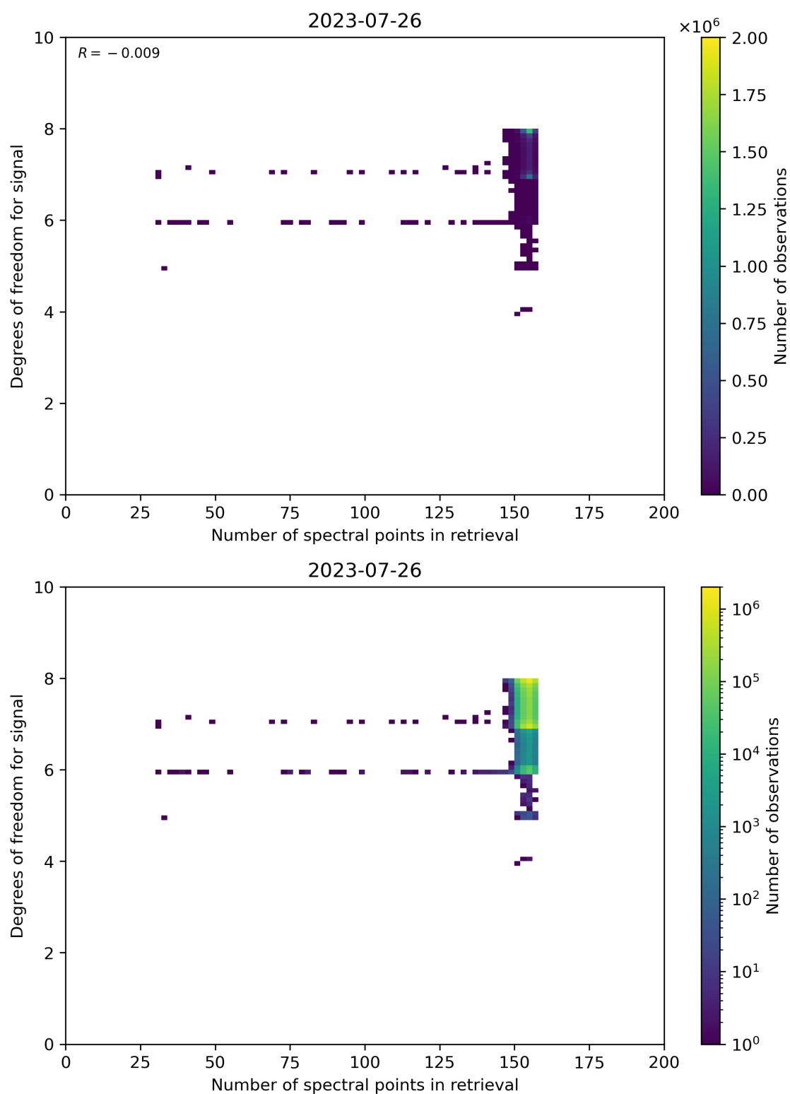
Figure 59: Scatter density plot of “Number of spectral points in retrieval” against “Degrees of freedom for signal” for 2023-07-25 to 2023-07-27.
