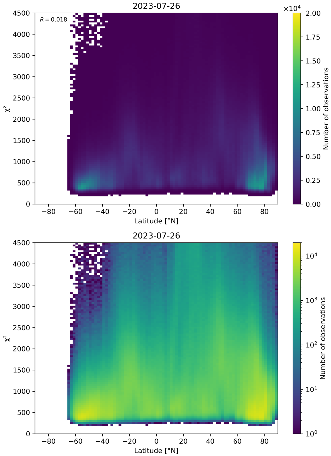
Figure 54: Scatter density plot of “Latitude” against “ \chi^2 ” for 2023-07-25 to 2023-07-27.
