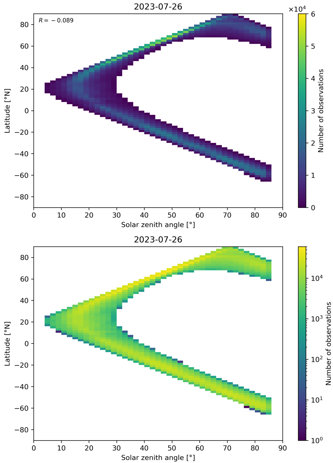
Figure 66: Scatter density plot of “Solar zenith angle” against “Latitude” for 2023-07-25 to 2023-07-27.
