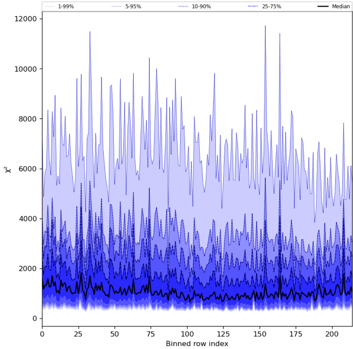
Figure 30: Along track statistics of “ \chi^2 ” for 2023-07-25 to 2023-07-27
