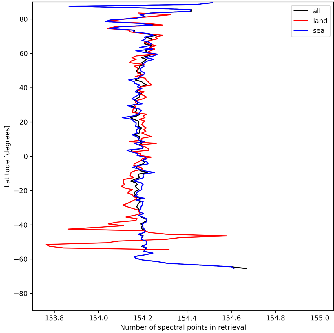
Figure 13: Zonal average of “Number of spectral points in retrieval” for 2023-07-25 to 2023-07-27.
