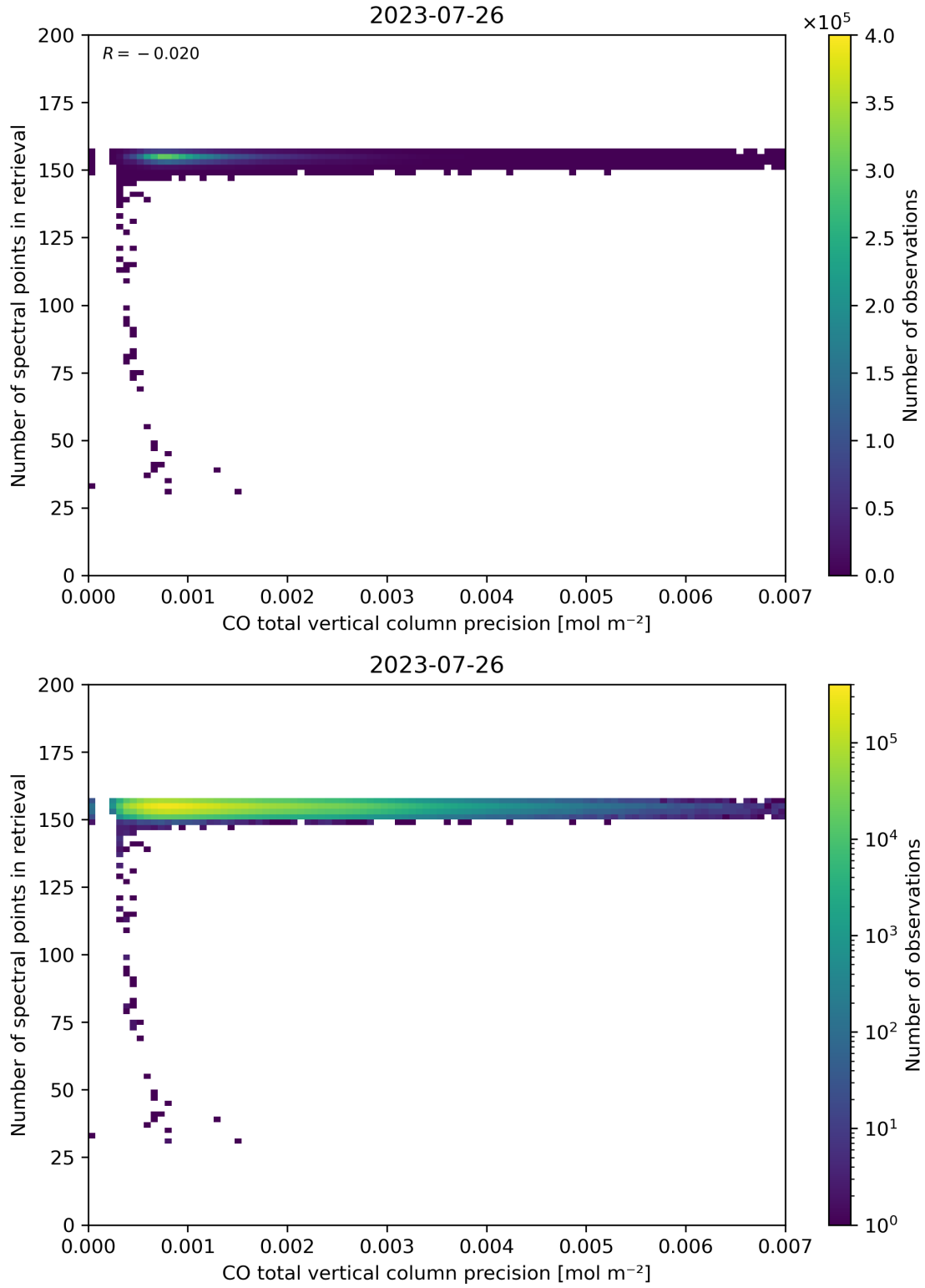
Figure 47: Scatter density plot of “CO total vertical column precision” against “Number of spectral points in retrieval” for 2023-07-25 to 2023-07-27.
