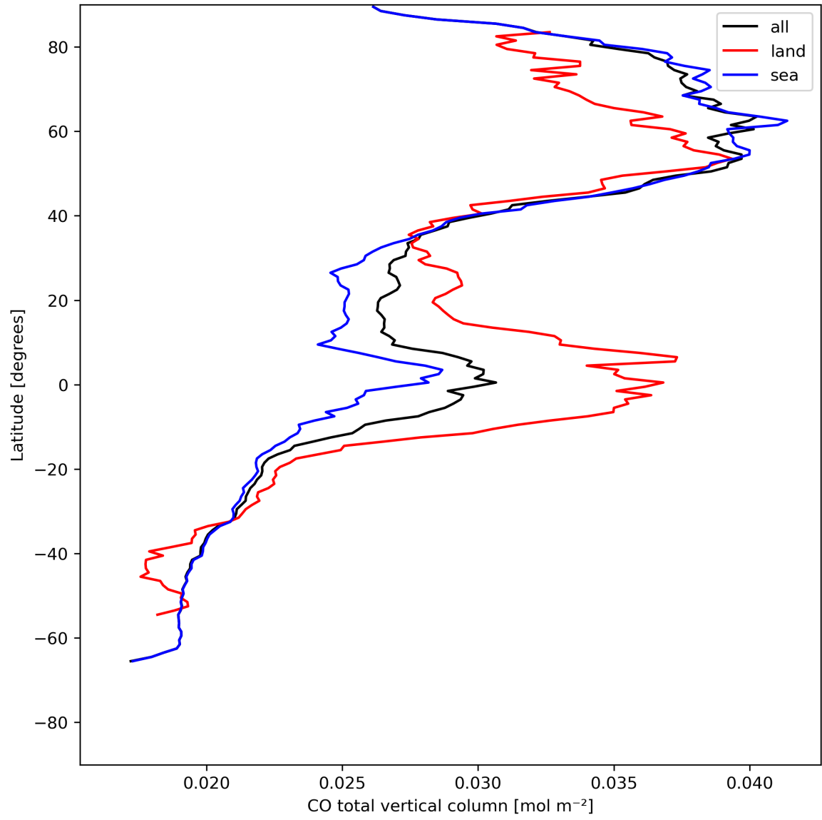
Figure 10: Zonal average of “CO total vertical column” for 2023-07-25 to 2023-07-27.
