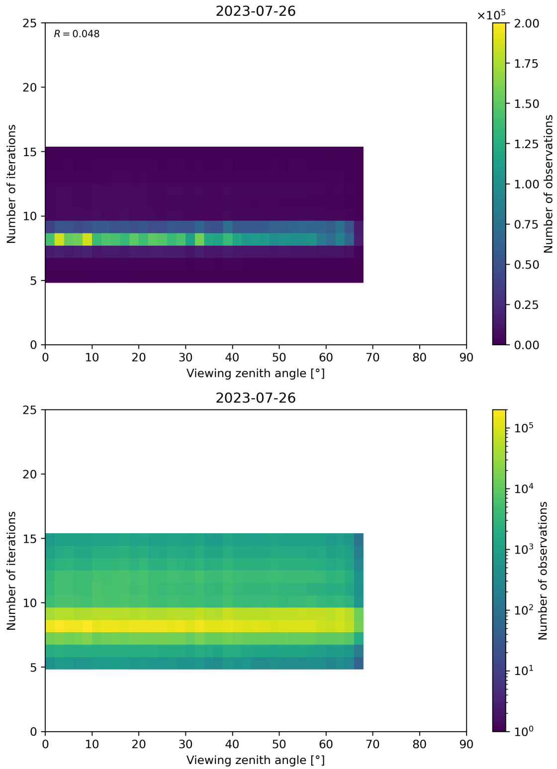
Figure 75: Scatter density plot of “Viewing zenith angle” against “Number of iterations” for 2023-07-25 to 2023-07-27.
