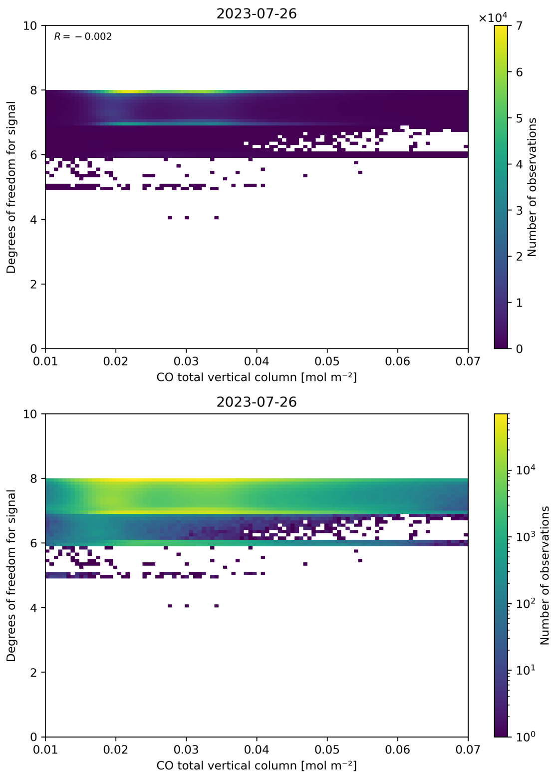
Figure 41: Scatter density plot of “CO total vertical column” against “Degrees of freedom for signal” for 2023-07-25 to 2023-07-27.
