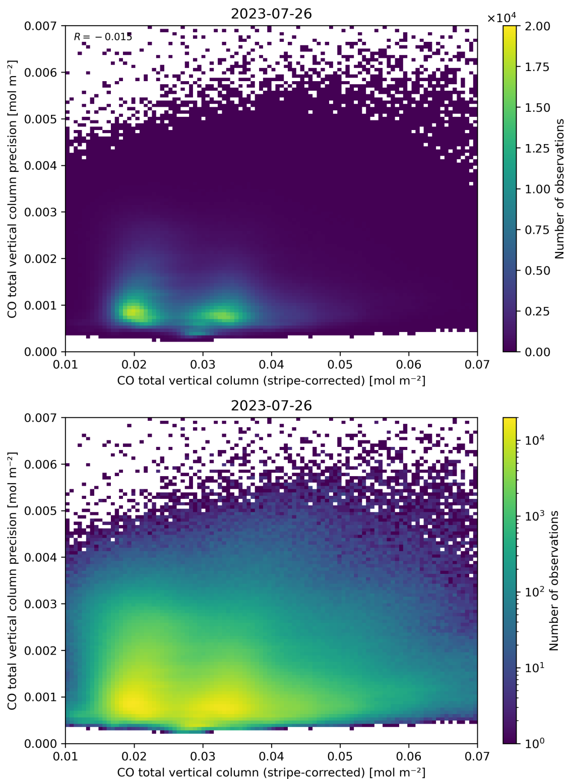
Figure 36: Scatter density plot of “CO total vertical column (stripe-corrected)” against “CO total vertical column precision” for 2023-07-25 to 2023-07-27.
