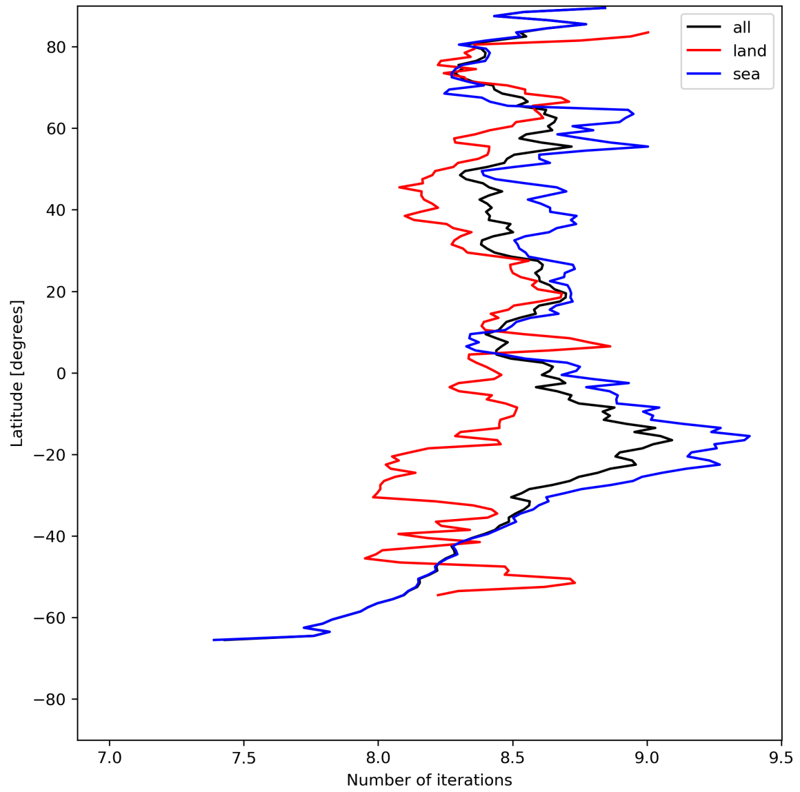
Figure 16: Zonal average of “Number of iterations” for 2023-07-25 to 2023-07-27.
