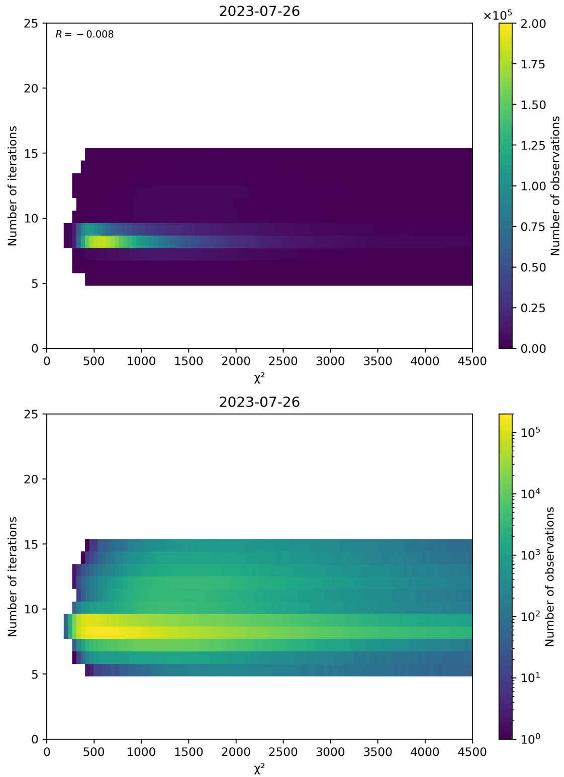
Figure 49: Scatter density plot of “ \chi^2 ” against “Number of iterations” for 2023-07-25 to 2023-07-27.
