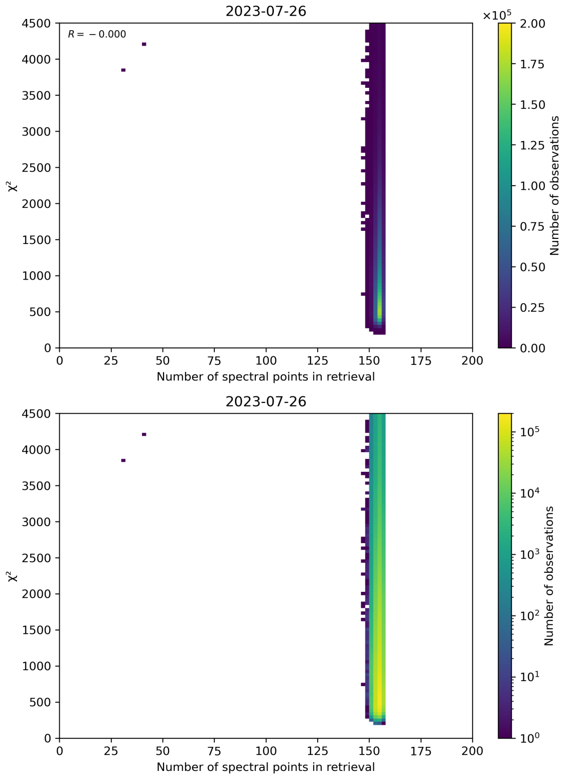
Figure 58: Scatter density plot of “Number of spectral points in retrieval” against “ \chi^2 ” for 2023-07-25 to 2023-07-27.
