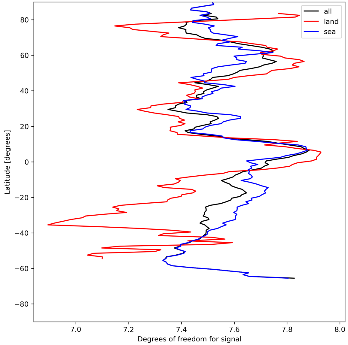
Figure 15: Zonal average of “Degrees of freedom for signal” for 2023-07-25 to 2023-07-27.
