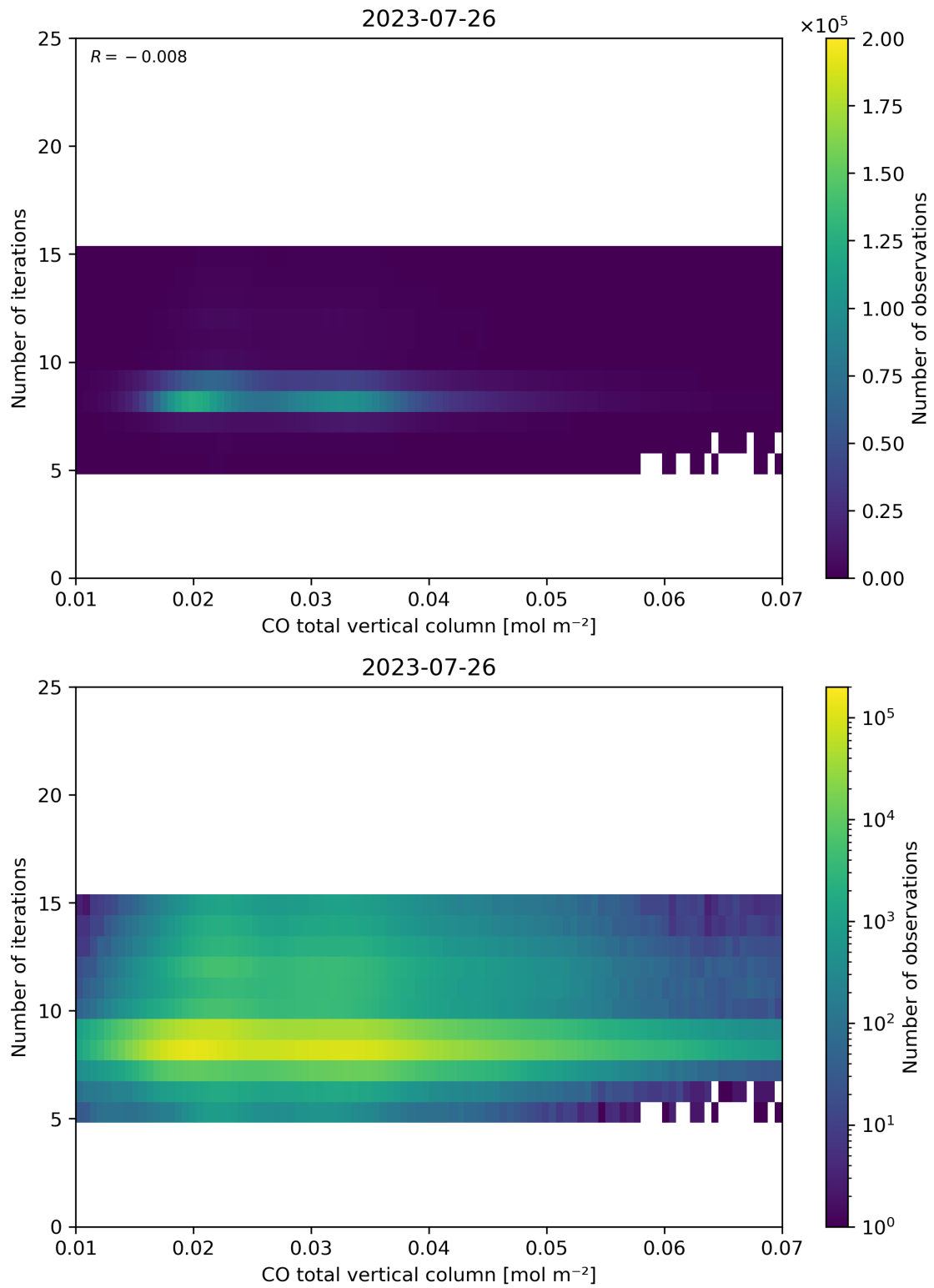
Figure 42: Scatter density plot of “CO total vertical column” against “Number of iterations” for 2023-07-25 to 2023-07-27.
