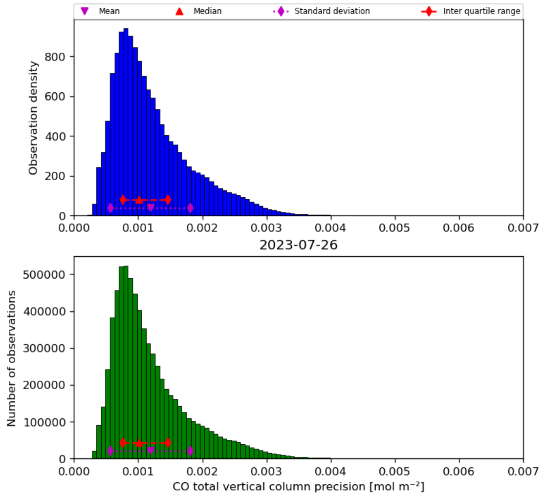
Figure 20: Histogram of “CO total vertical column precision” for 2023-07-25 to 2023-07-27
