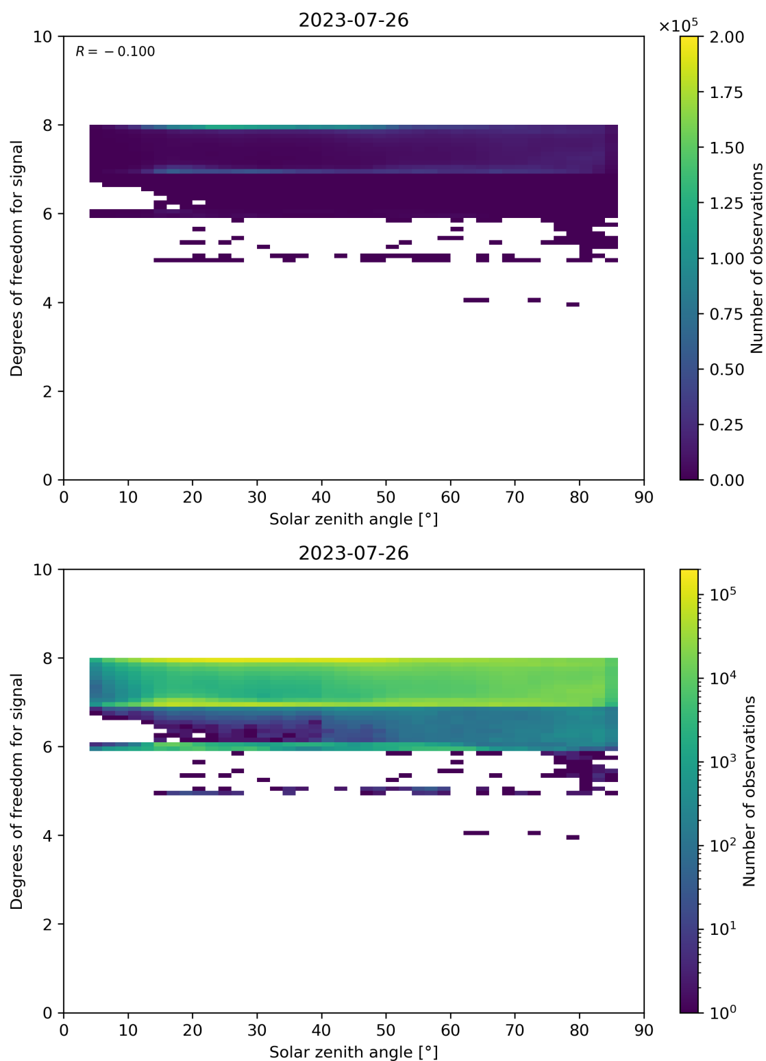
Figure 65: Scatter density plot of “Solar zenith angle” against “Degrees of freedom for signal” for 2023-07-25 to 2023-07-27.
