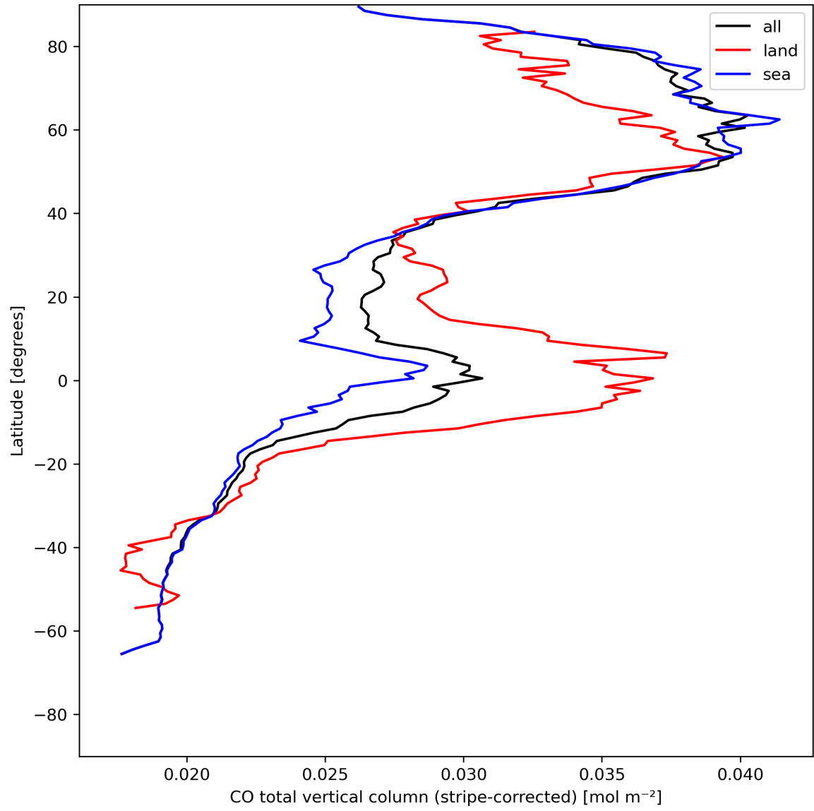
Figure 11: Zonal average of “CO total vertical column (stripe-corrected)” for 2023-07-25 to 2023-07-27.
