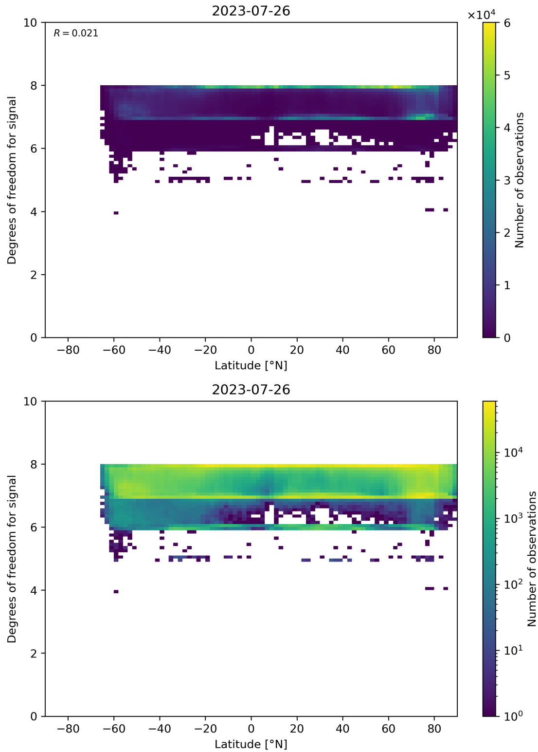
Figure 55: Scatter density plot of “Latitude” against “Degrees of freedom for signal” for 2023-07-25 to 2023-07-27.
