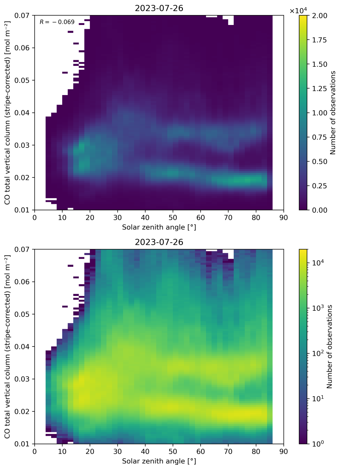
Figure 62: Scatter density plot of “Solar zenith angle” against “CO total vertical column (stripe-corrected)” for 2023-07-25 to 2023-07-27.
