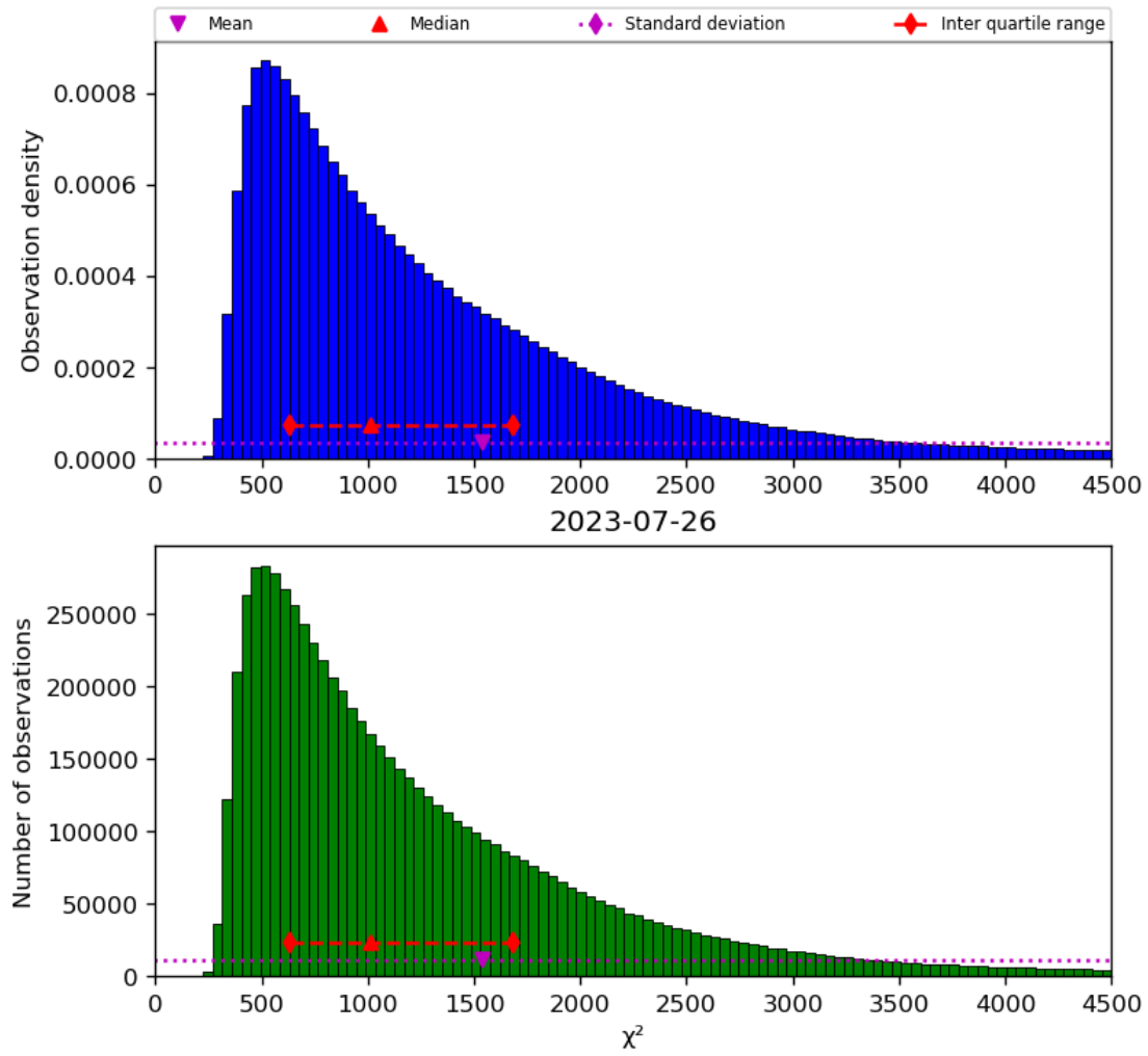
Figure 22: Histogram of “ \chi^2 ” for 2023-07-25 to 2023-07-27
