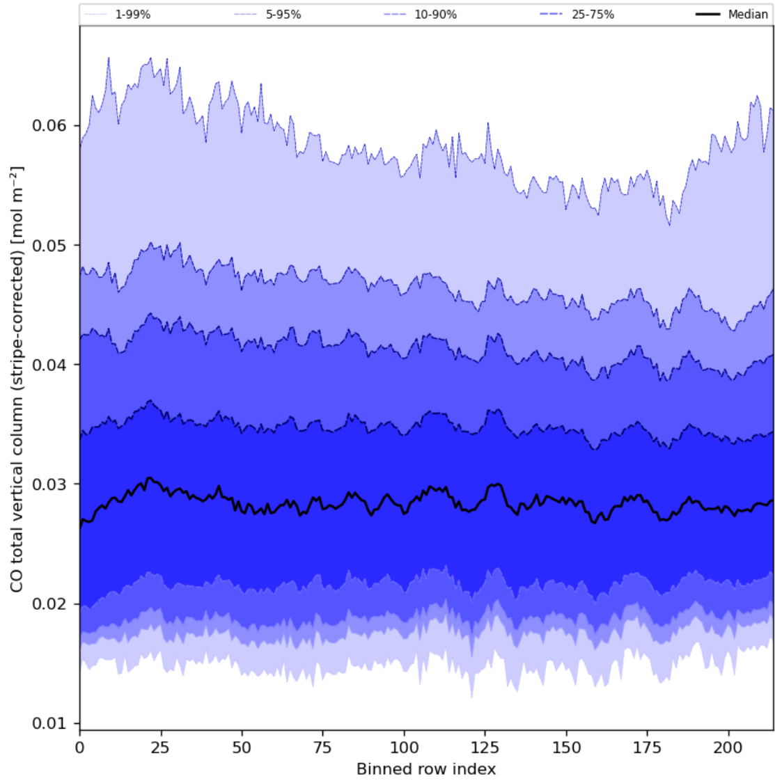
Figure 27: Along track statistics of “CO total vertical column (stripe-corrected)” for 2023-07-25 to 2023-07-27
