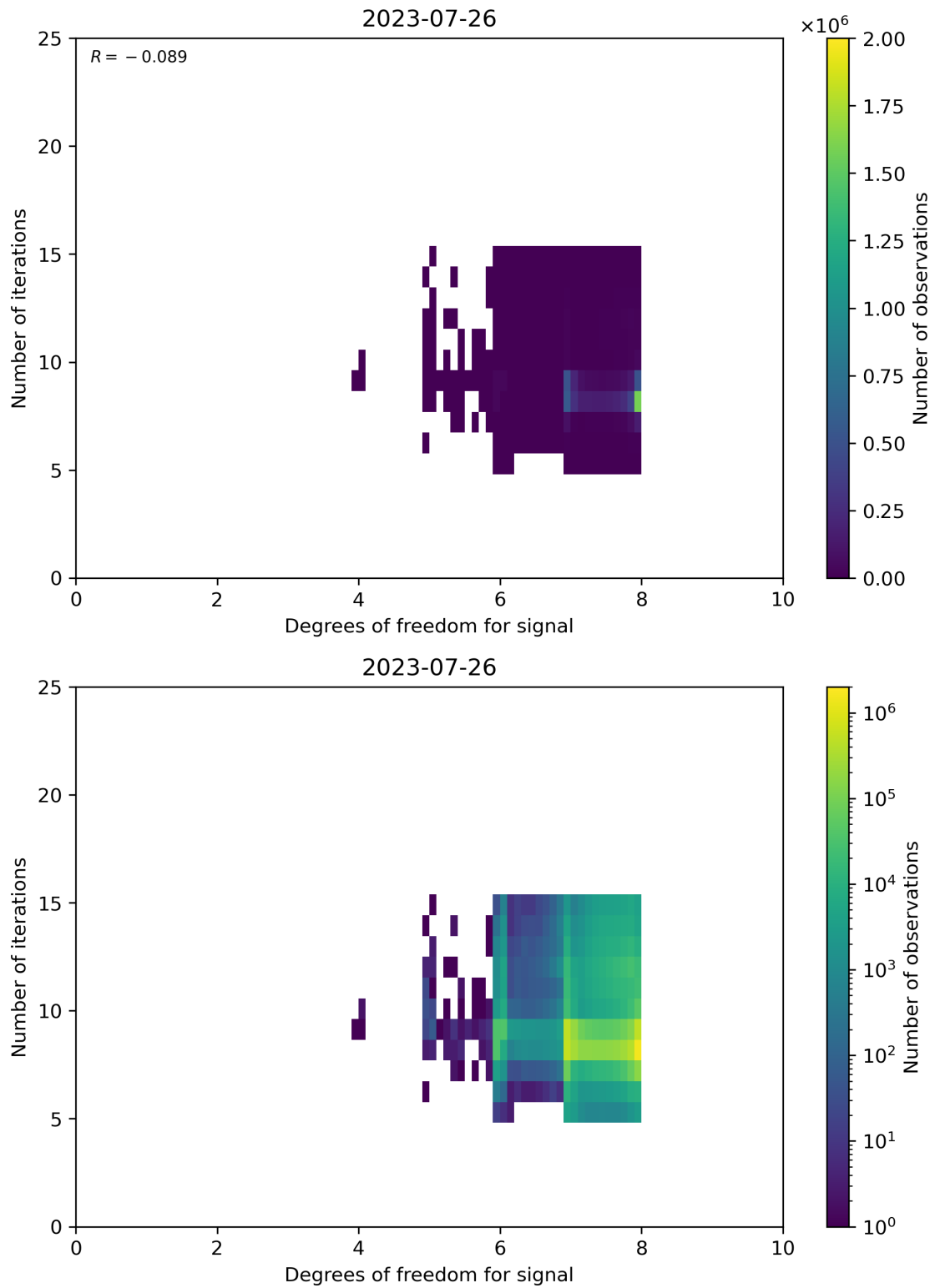
Figure 50: Scatter density plot of “Degrees of freedom for signal” against “Number of iterations” for 2023-07-25 to 2023-07-27.
