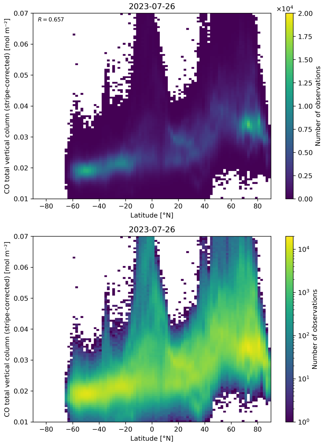
Figure 52: Scatter density plot of “Latitude” against “CO total vertical column (stripe-corrected)” for 2023-07-25 to 2023-07-27.
