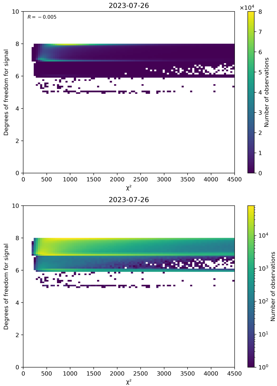
Figure 48: Scatter density plot of “ \chi^2 ” against “Degrees of freedom for signal” for 2023-07-25 to 2023-07-27.
