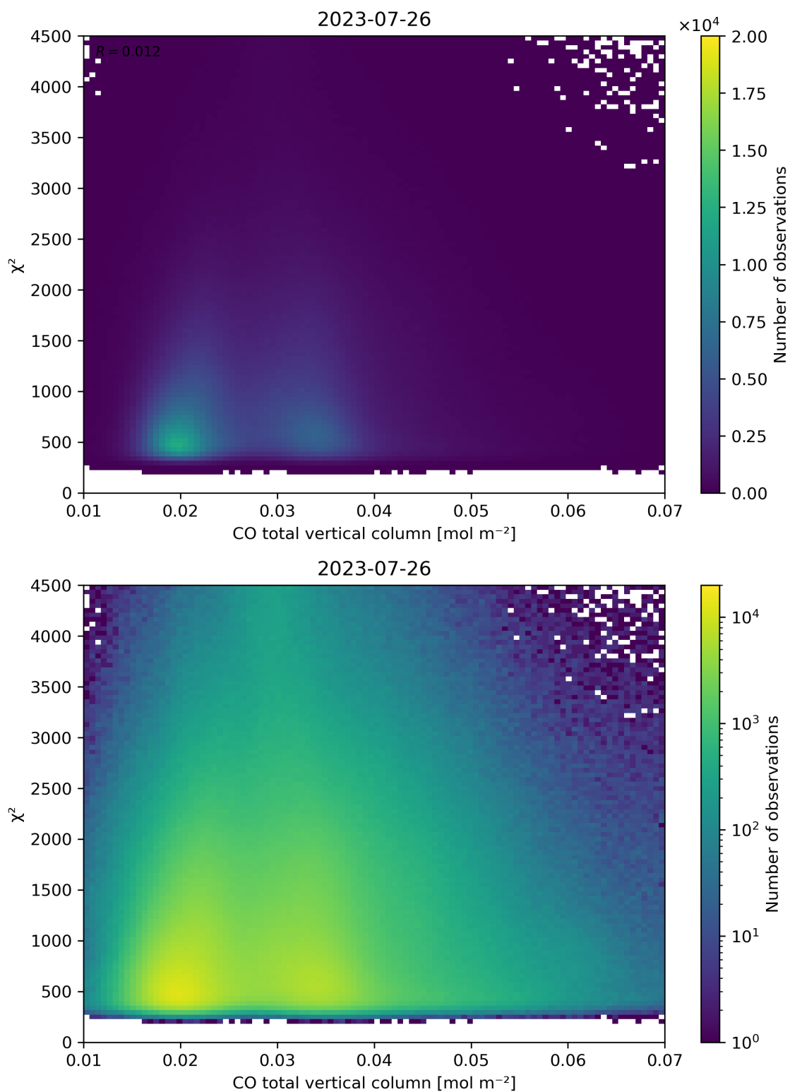
Figure 35: Scatter density plot of “CO total vertical column” against “ \chi^2 ” for 2023-07-25 to 2023-07-27.
