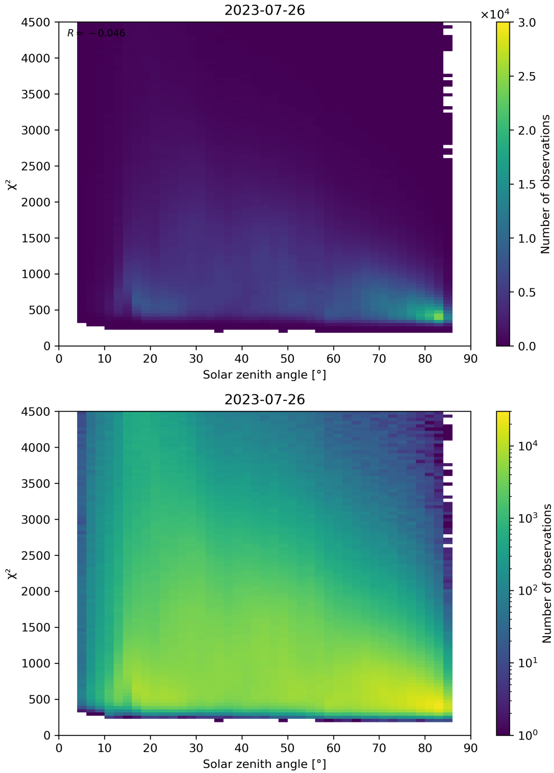
Figure 64: Scatter density plot of “Solar zenith angle” against “ \chi^2 ” for 2023-07-25 to 2023-07-27.
