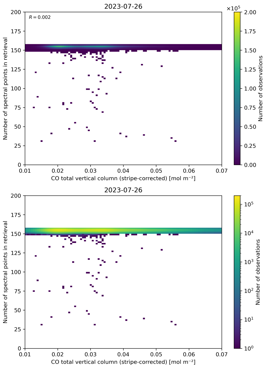
Figure 40: Scatter density plot of “CO total vertical column (stripe-corrected)” against “Number of spectral points in retrieval” for 2023-07-25 to 2023-07-27.
