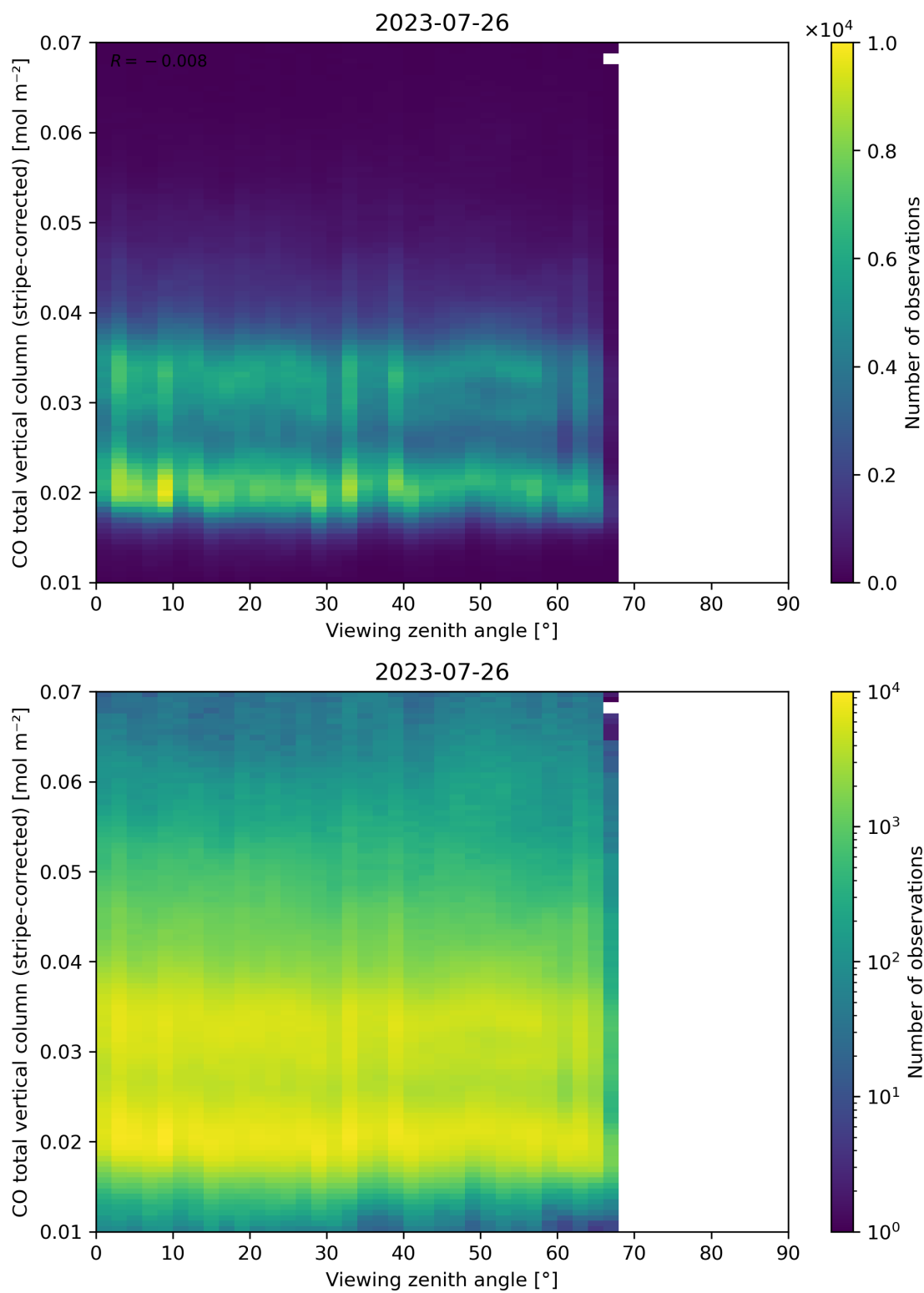
Figure 70: Scatter density plot of “Viewing zenith angle” against “CO total vertical column (stripe-corrected)” for 2023-07-25 to 2023-07-27.
