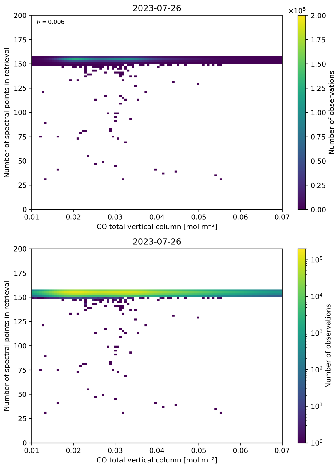
Figure 43: Scatter density plot of “CO total vertical column” against “Number of spectral points in retrieval” for 2023-07-25 to 2023-07-27.
