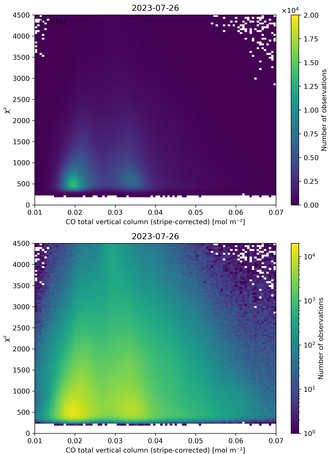
Figure 37: Scatter density plot of “CO total vertical column (stripe-corrected)” against “ \chi^2 ” for 2023-07-25 to 2023-07-27.
