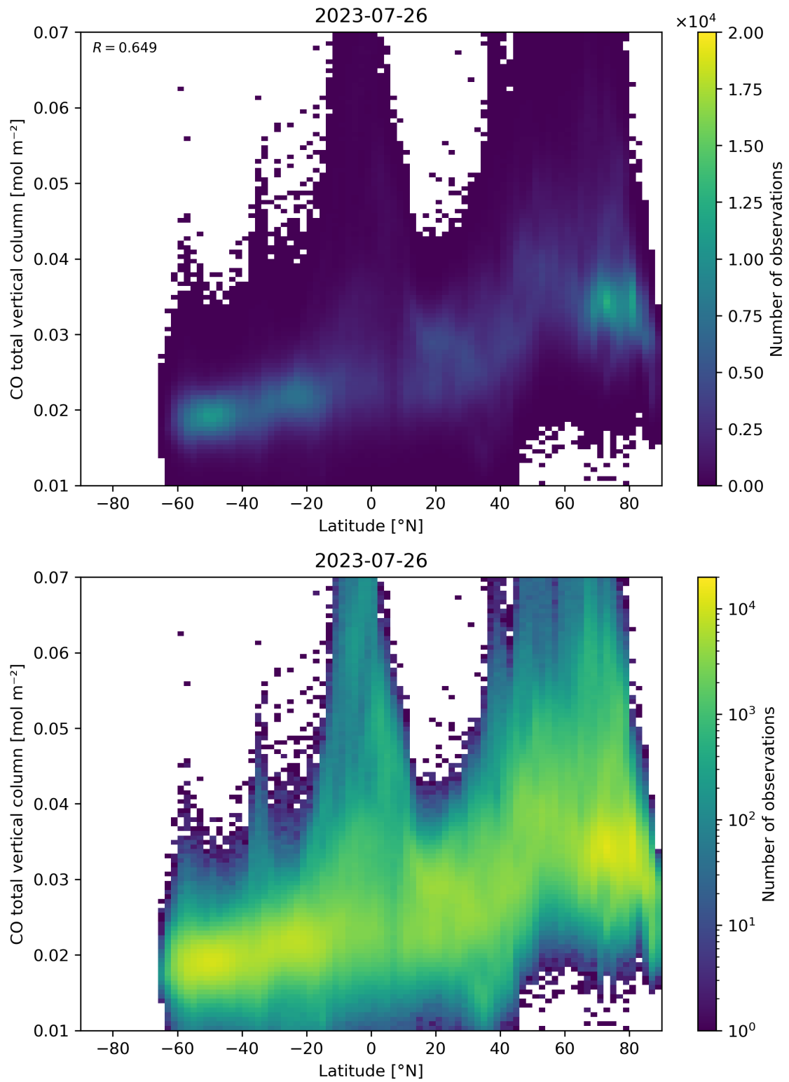
Figure 51: Scatter density plot of “Latitude” against “CO total vertical column” for 2023-07-25 to 2023-07-27.
