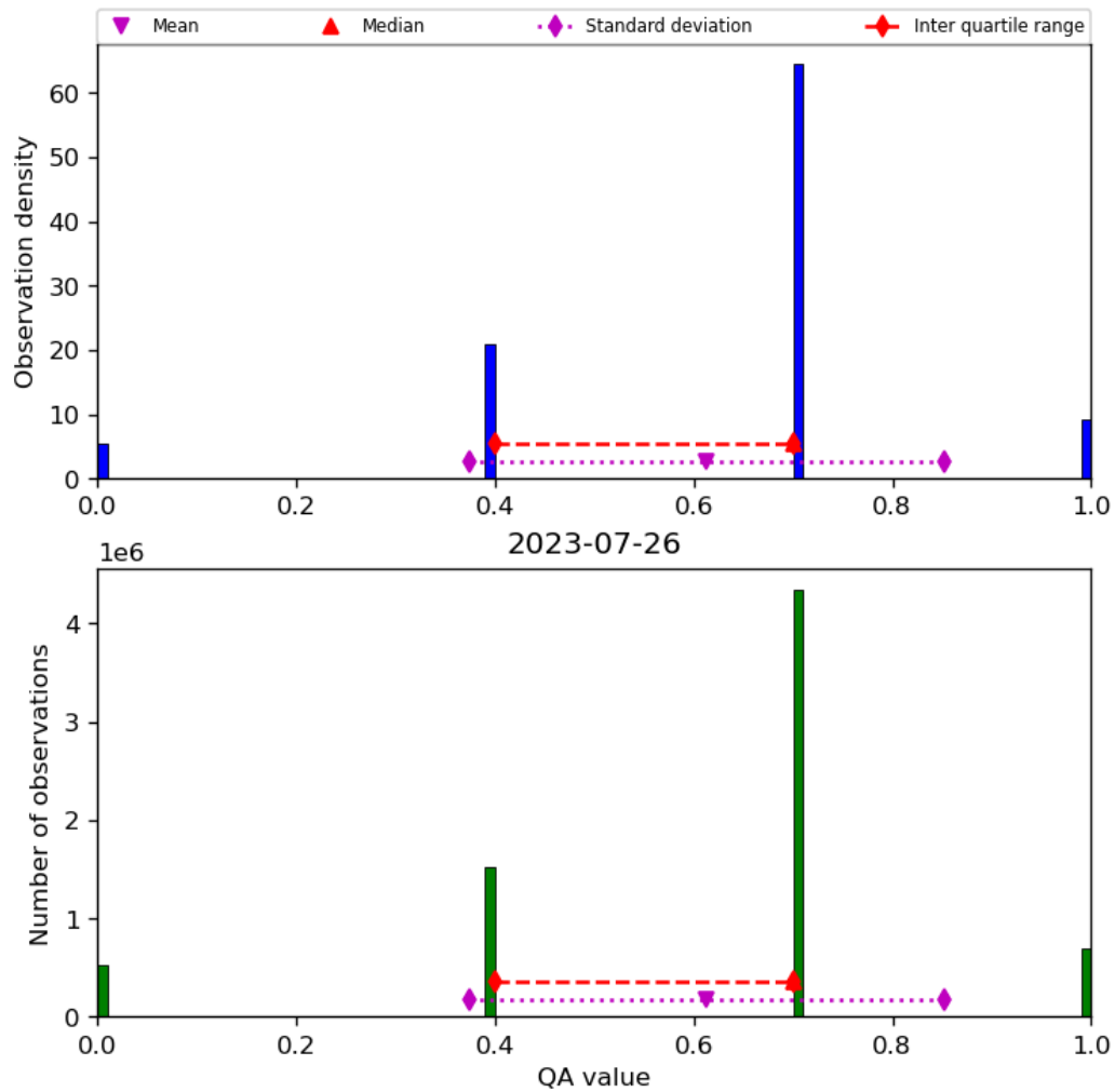
Figure 17: Histogram of “QA value” for 2023-07-25 to 2023-07-27
