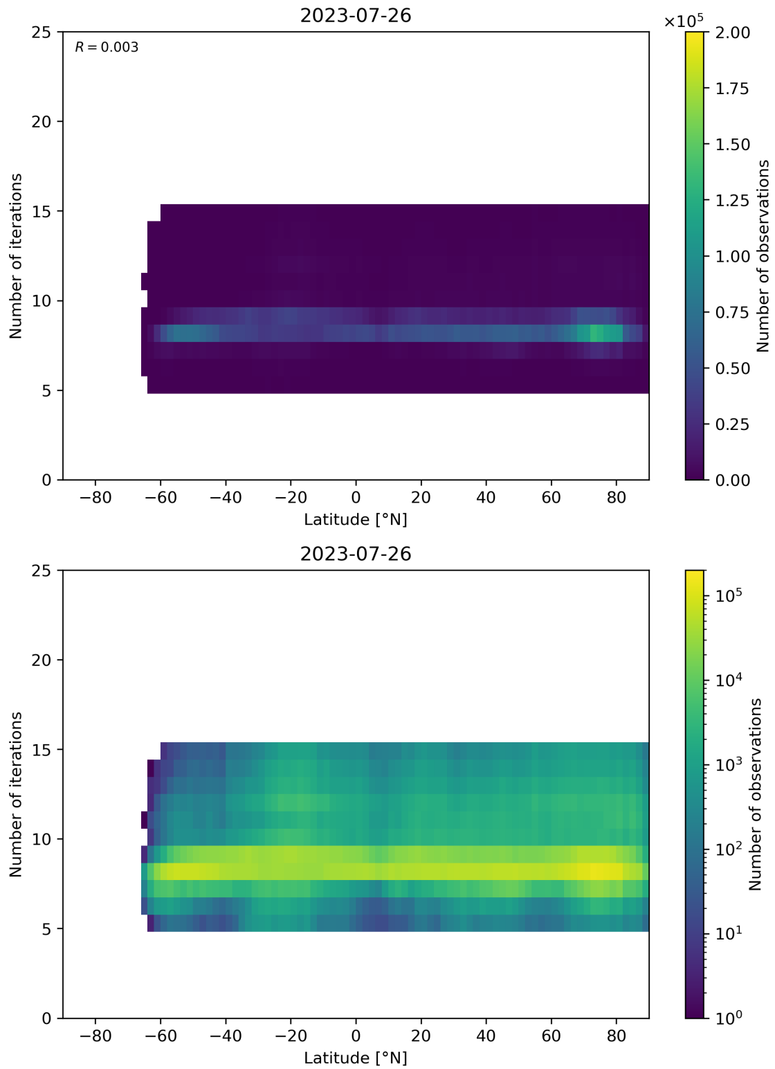
Figure 56: Scatter density plot of “Latitude” against “Number of iterations” for 2023-07-25 to 2023-07-27.
