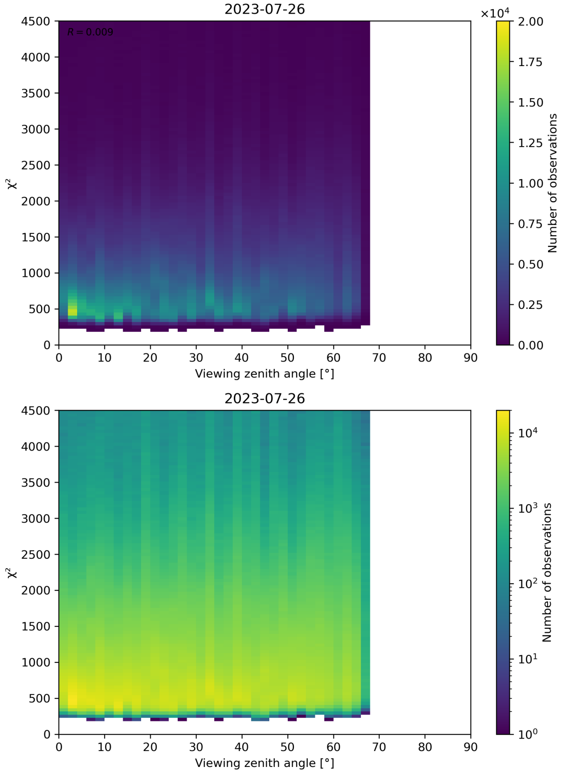
Figure 72: Scatter density plot of “Viewing zenith angle” against “ \chi^2 ” for 2023-07-25 to 2023-07-27.
