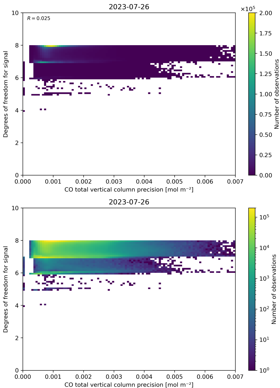
Figure 45: Scatter density plot of “CO total vertical column precision” against “Degrees of freedom for signal” for 2023-07-25 to 2023-07-27.
