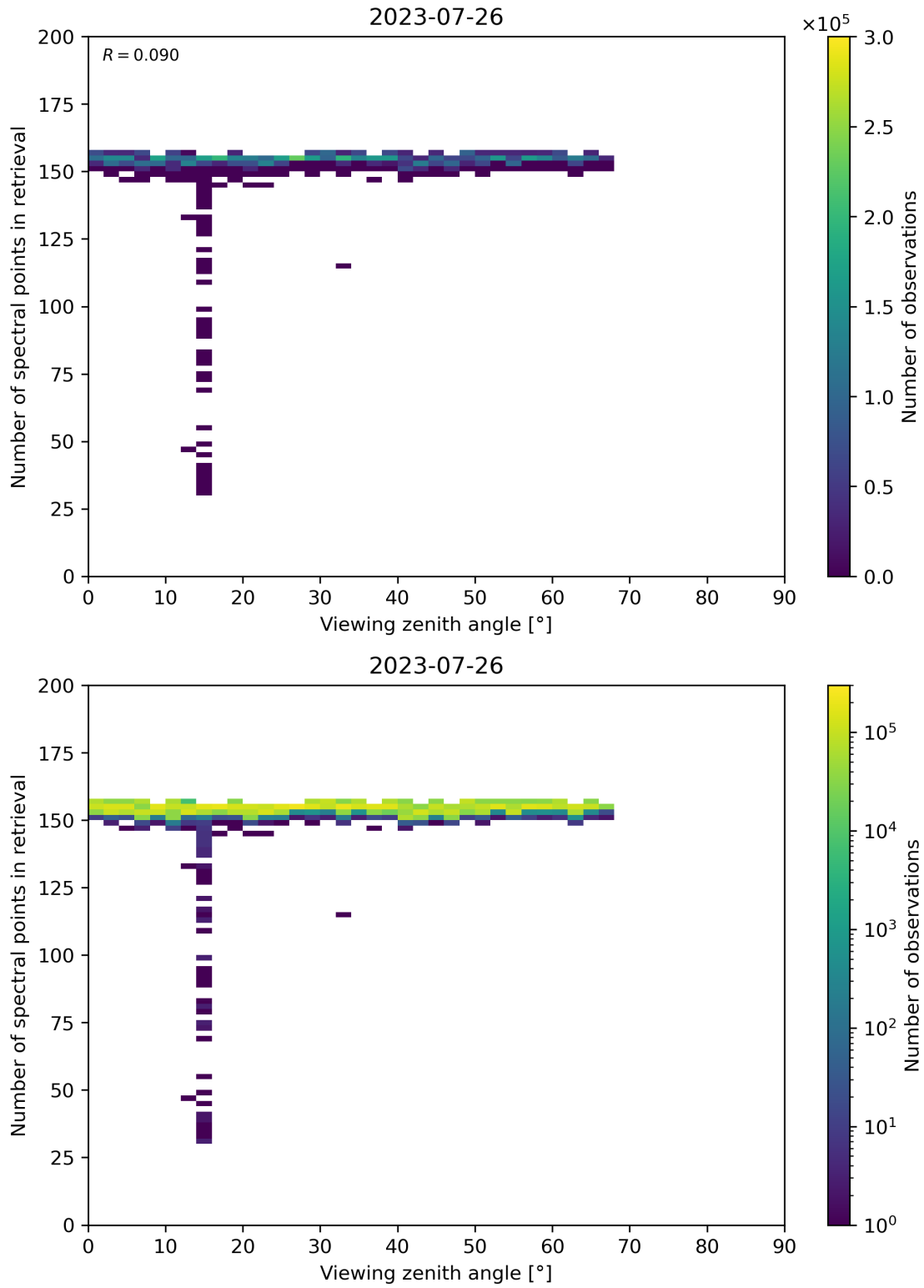
Figure 76: Scatter density plot of “Viewing zenith angle” against “Number of spectral points in retrieval” for 2023-07-25 to 2023-07-27.
