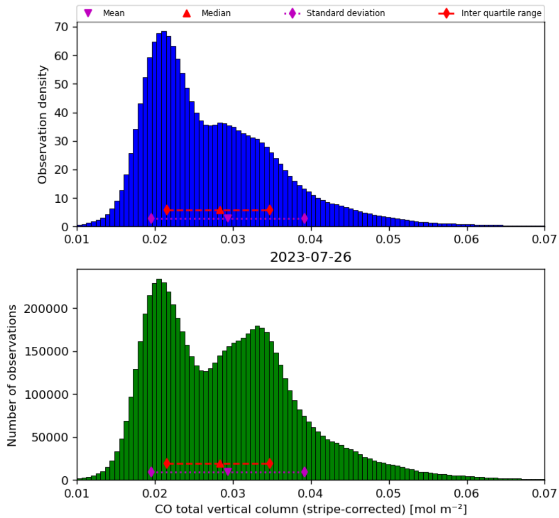
Figure 19: Histogram of “CO total vertical column (stripe-corrected)” for 2023-07-25 to 2023-07-27
