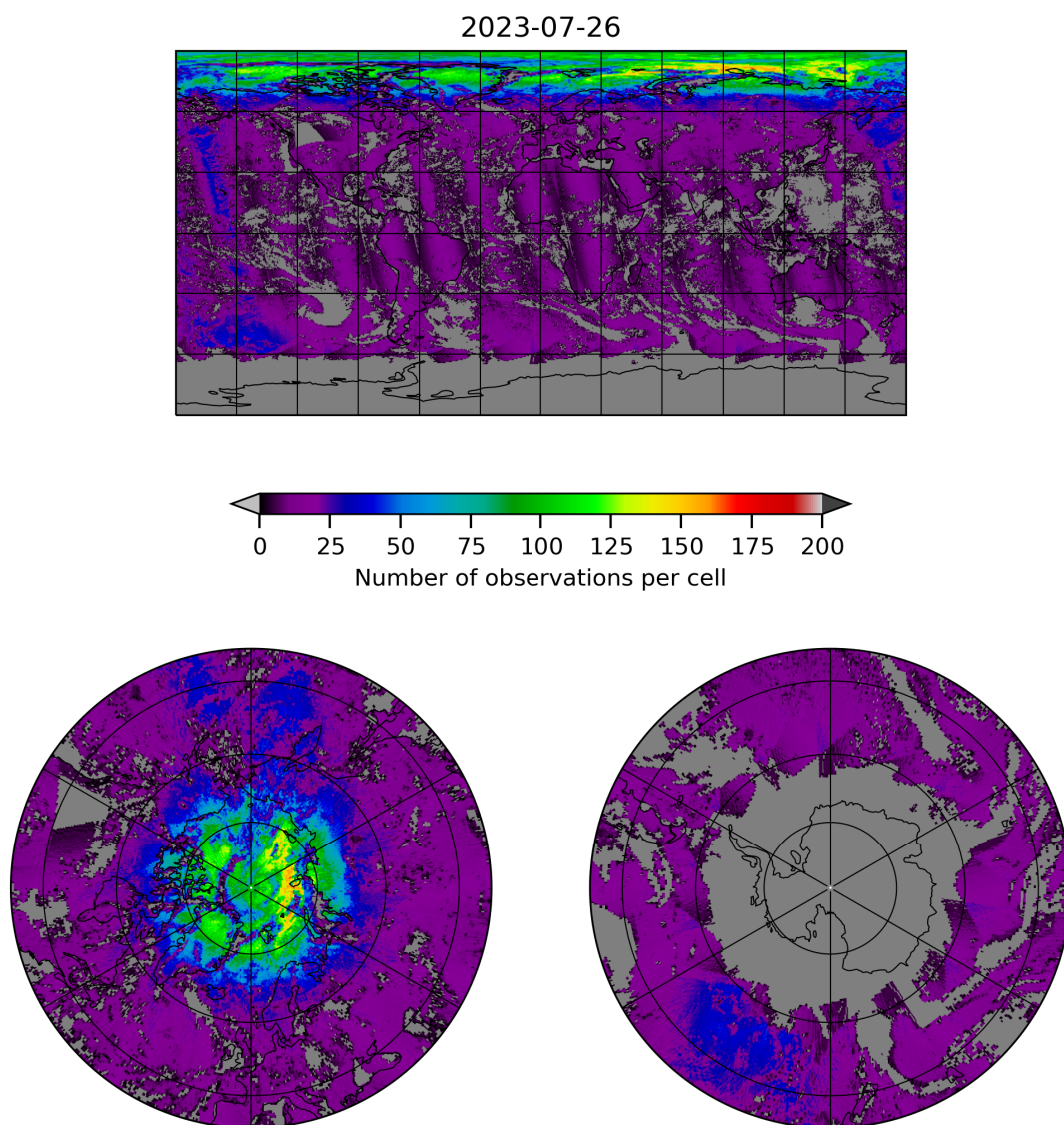
Figure 8: Map of the number of observations for 2023-07-25 to 2023-07-27
