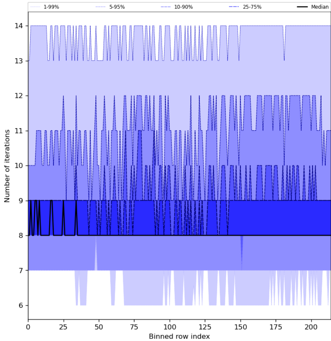
Figure 32: Along track statistics of “Number of iterations” for 2023-07-25 to 2023-07-27
