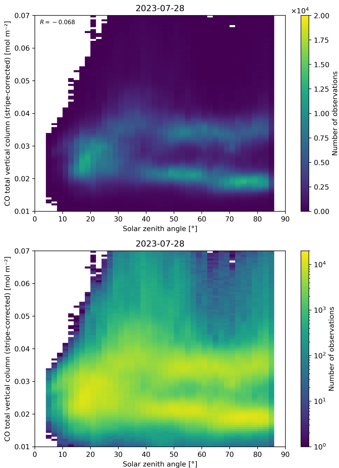
Figure 62: Scatter density plot of “Solar zenith angle” against “CO total vertical column (stripe-corrected)” for 2023-07-27 to 2023-07-29.
