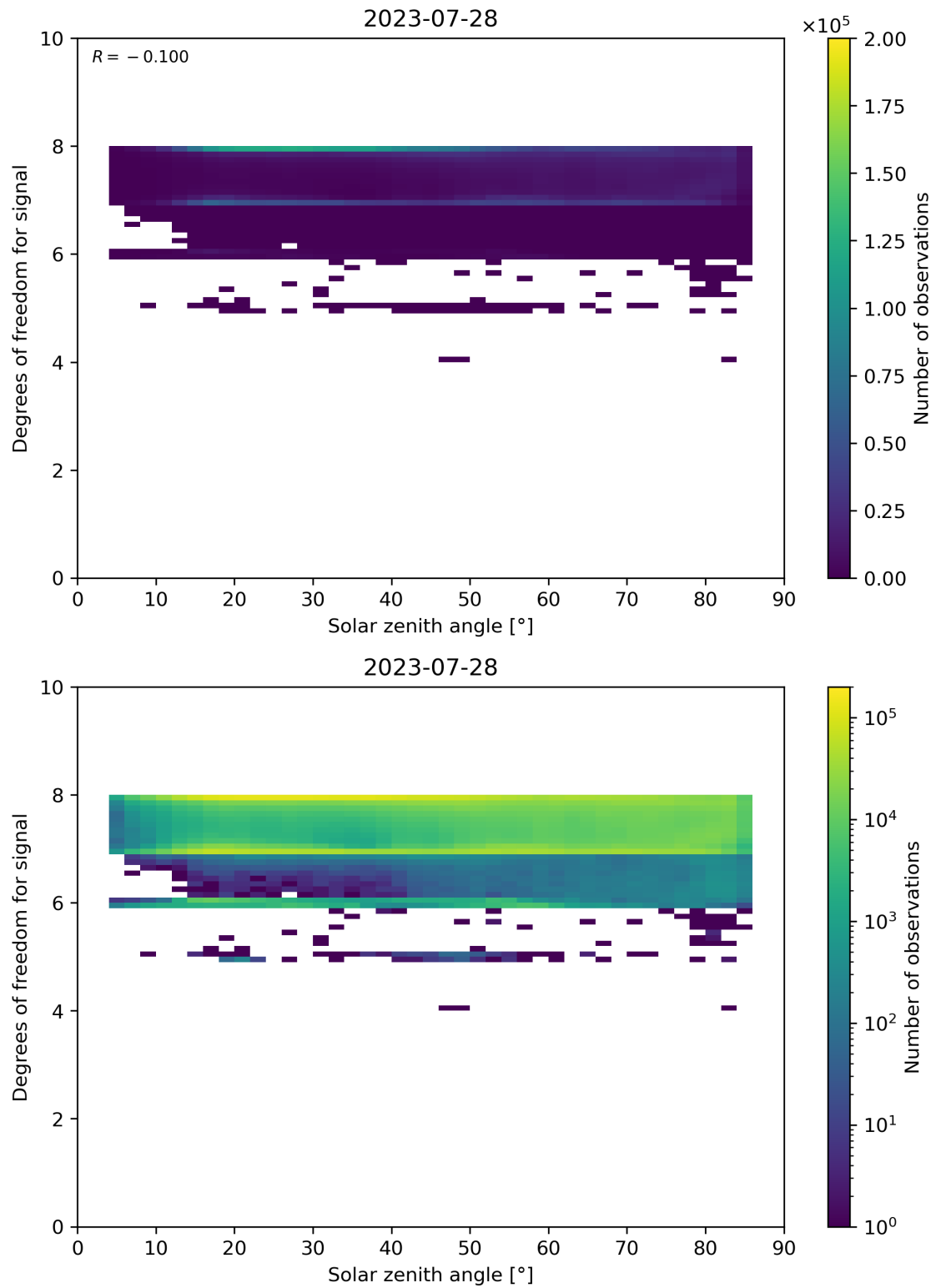
Figure 65: Scatter density plot of “Solar zenith angle” against “Degrees of freedom for signal” for 2023-07-27 to 2023-07-29.
