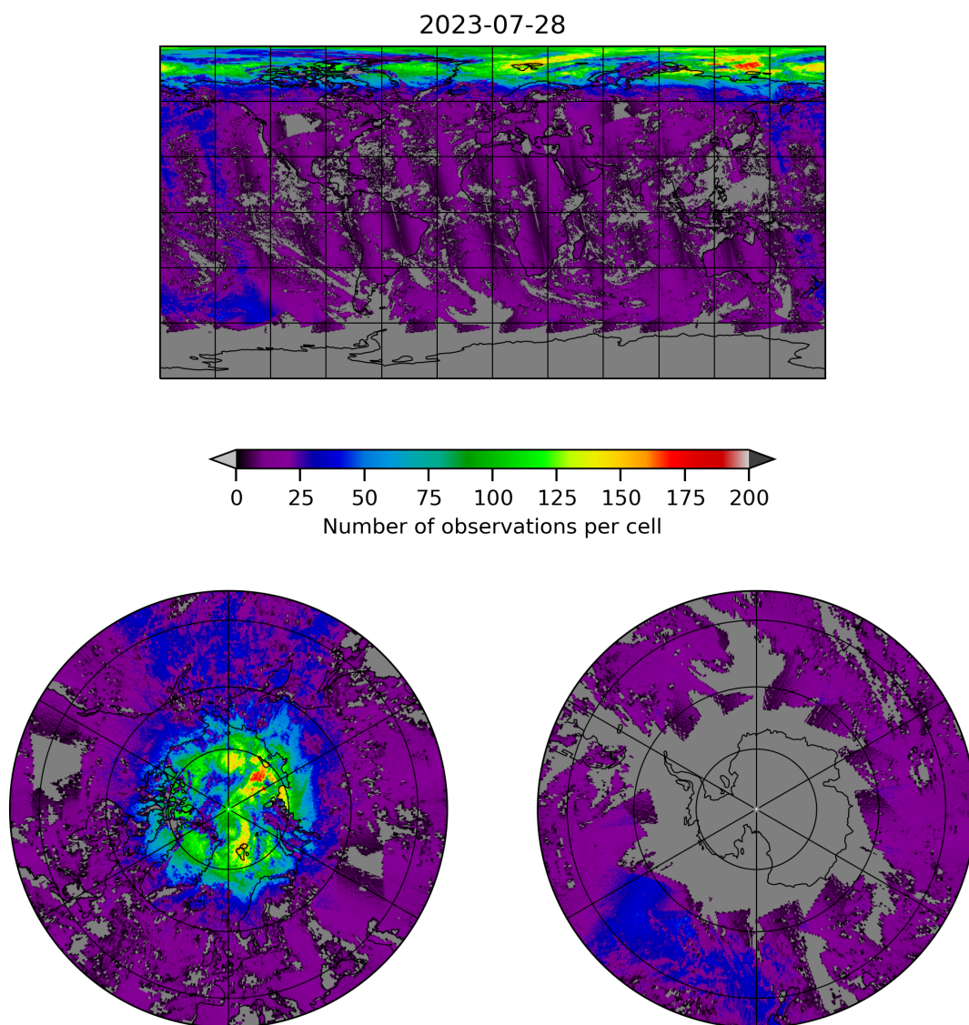
Figure 8: Map of the number of observations for 2023-07-27 to 2023-07-29
