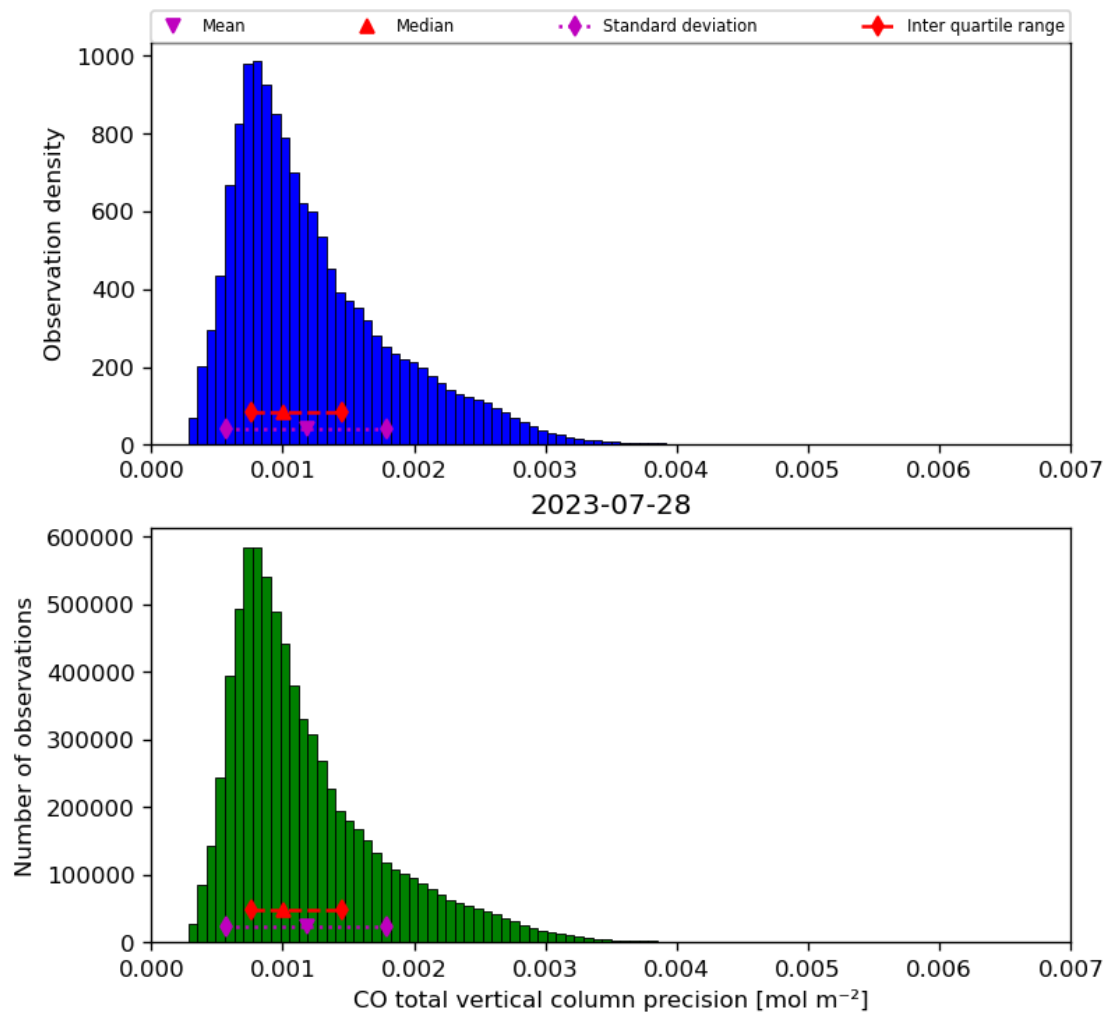
Figure 20: Histogram of “CO total vertical column precision” for 2023-07-27 to 2023-07-29
