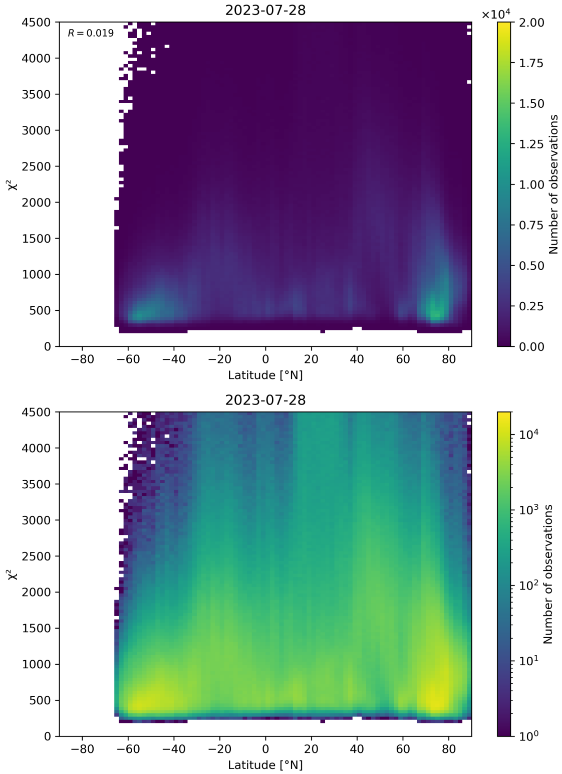
Figure 54: Scatter density plot of “Latitude” against “ \chi^2 ” for 2023-07-27 to 2023-07-29.
