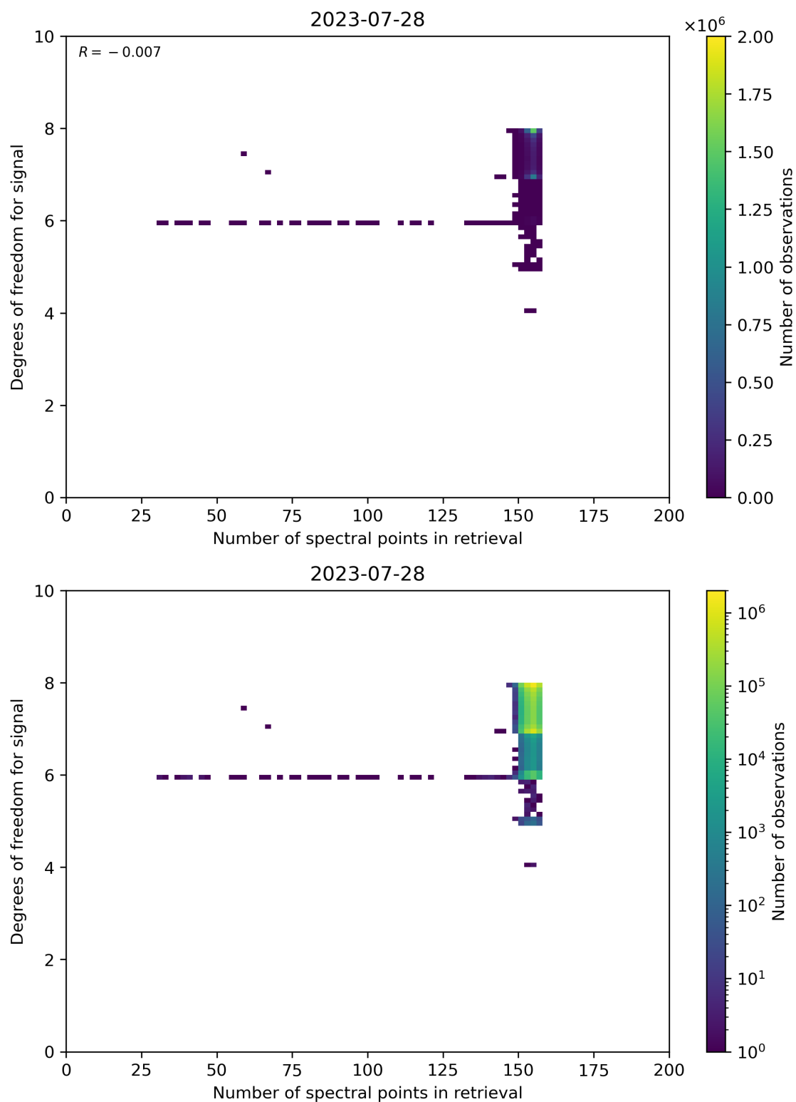
Figure 59: Scatter density plot of “Number of spectral points in retrieval” against “Degrees of freedom for signal” for 2023-07-27 to 2023-07-29.
