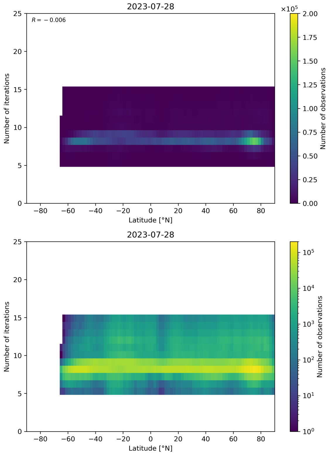
Figure 56: Scatter density plot of “Latitude” against “Number of iterations” for 2023-07-27 to 2023-07-29.
