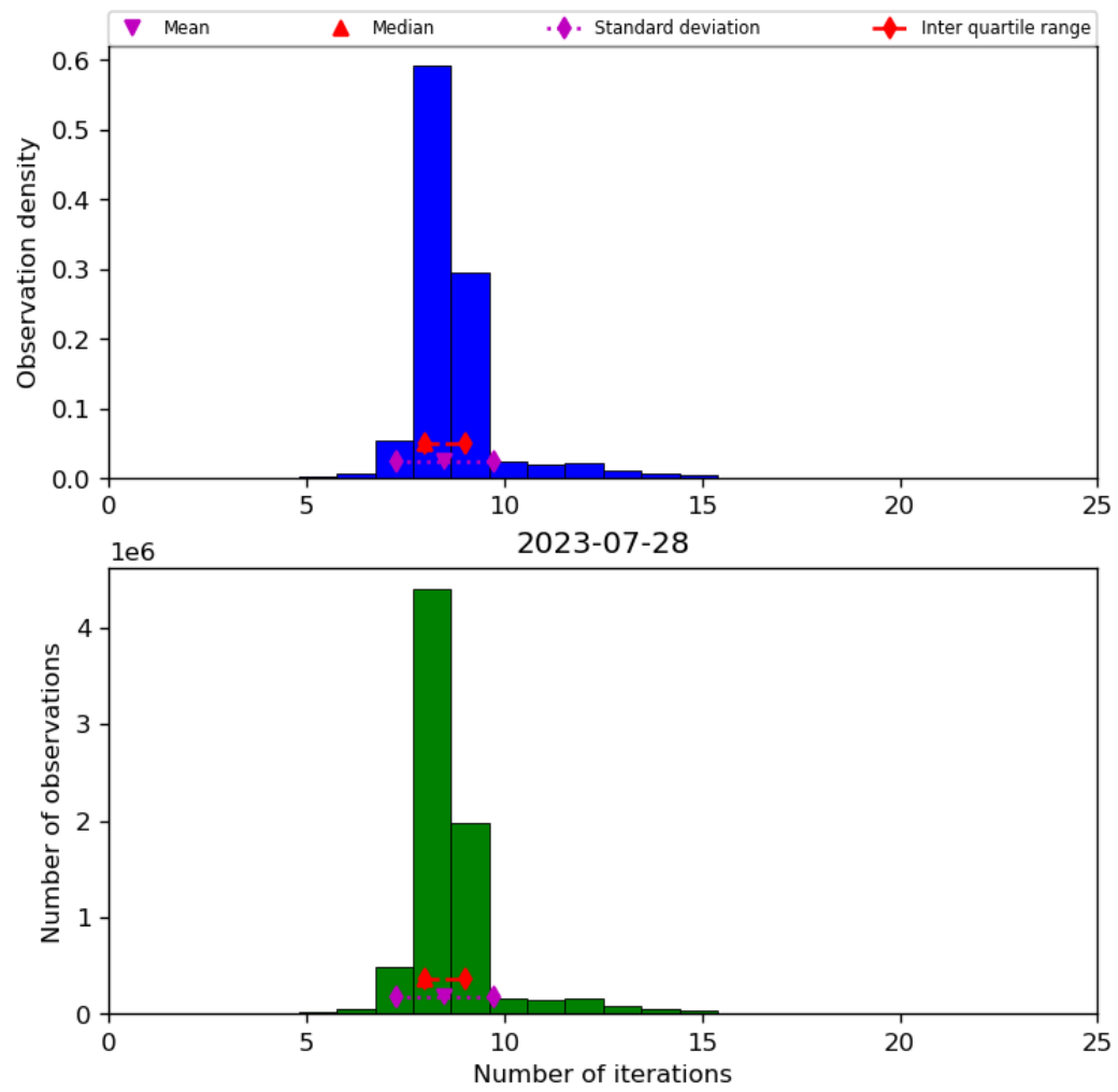
Figure 24: Histogram of “Number of iterations” for 2023-07-27 to 2023-07-29
