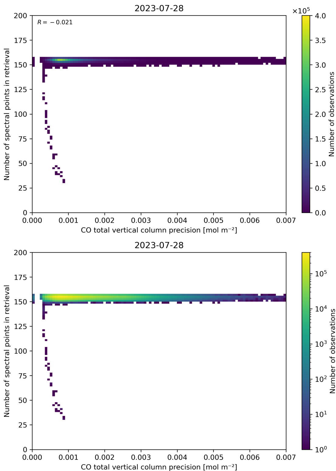
Figure 47: Scatter density plot of “CO total vertical column precision” against “Number of spectral points in retrieval” for 2023-07-27 to 2023-07-29.
