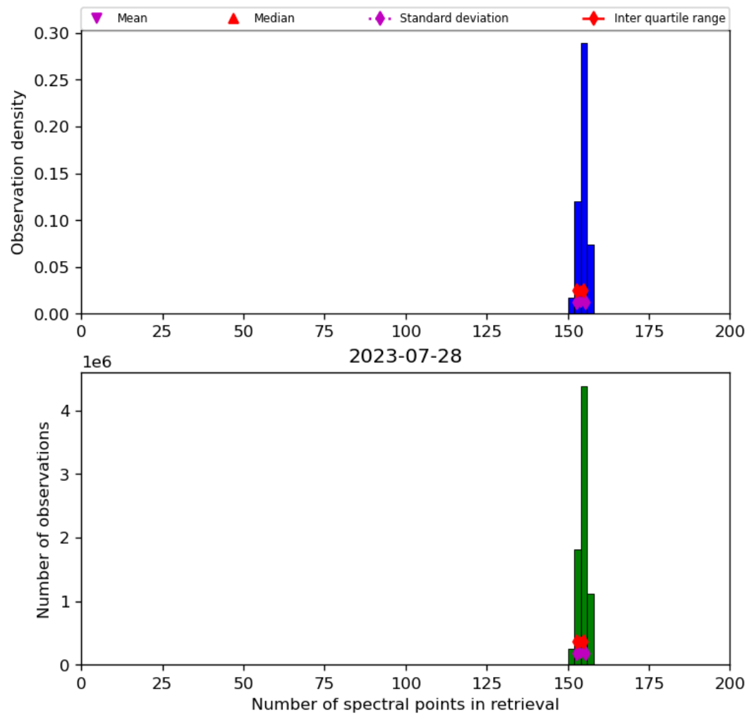
Figure 21: Histogram of “Number of spectral points in retrieval” for 2023-07-27 to 2023-07-29
