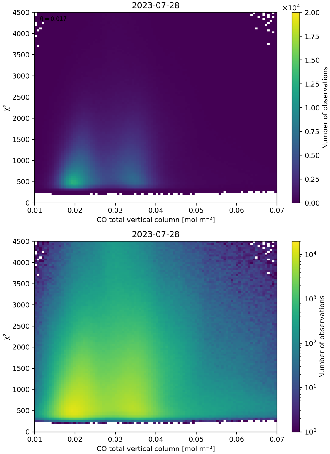
Figure 35: Scatter density plot of “CO total vertical column” against “ \chi^2 ” for 2023-07-27 to 2023-07-29.
