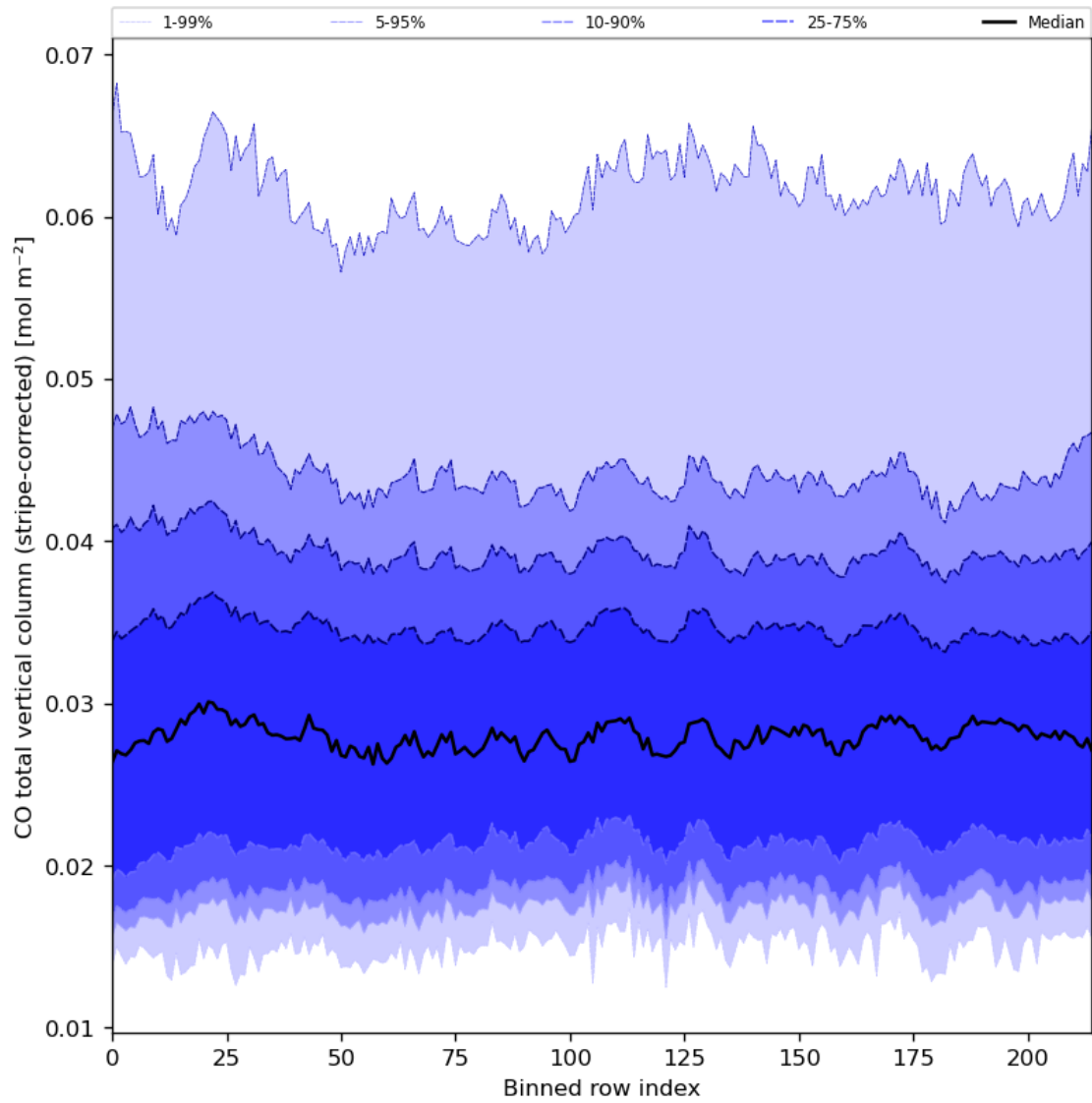
Figure 27: Along track statistics of “CO total vertical column (stripe-corrected)” for 2023-07-27 to 2023-07-29
