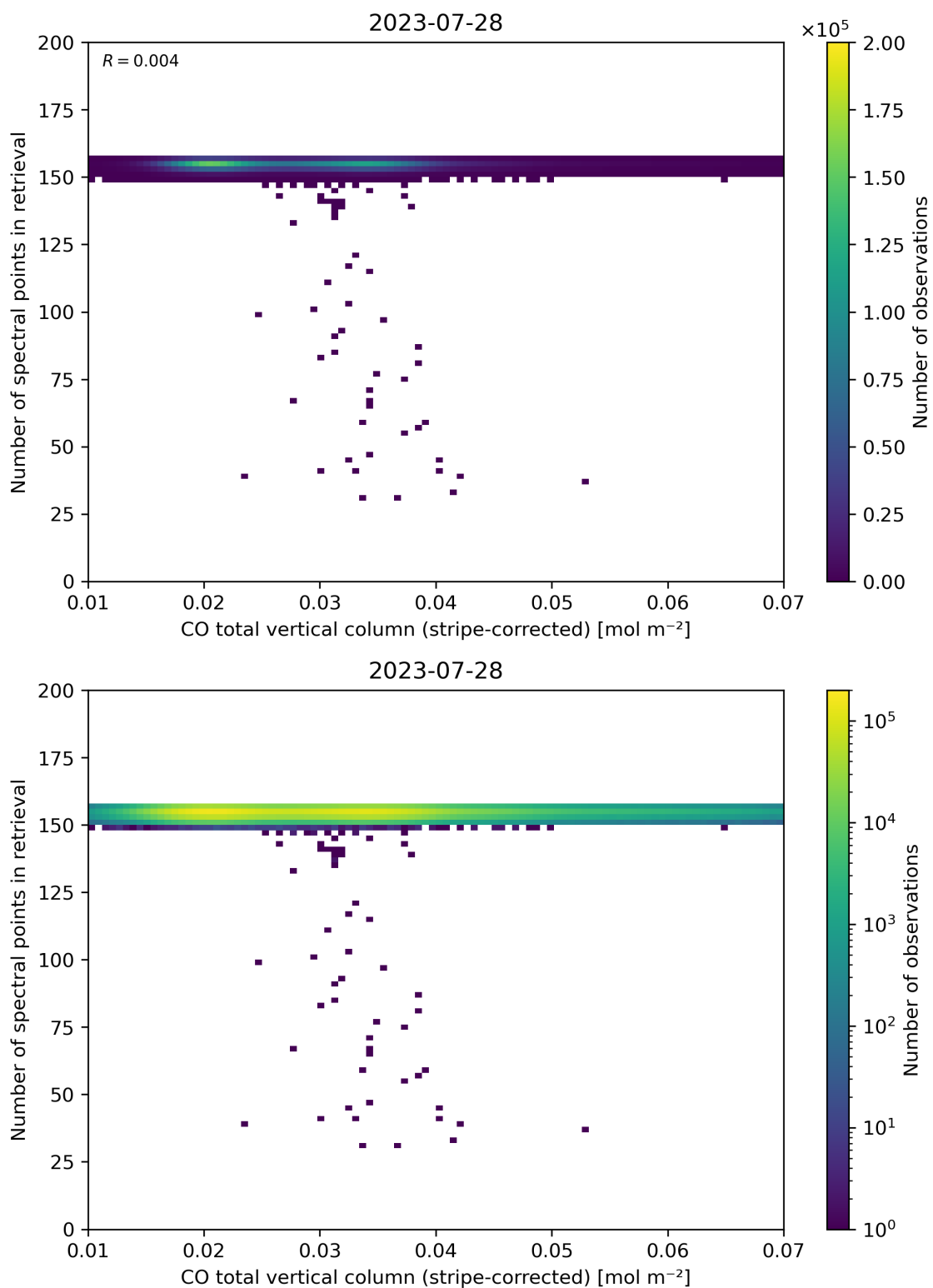
Figure 40: Scatter density plot of “CO total vertical column (stripe-corrected)” against “Number of spectral points in retrieval” for 2023-07-27 to 2023-07-29.
