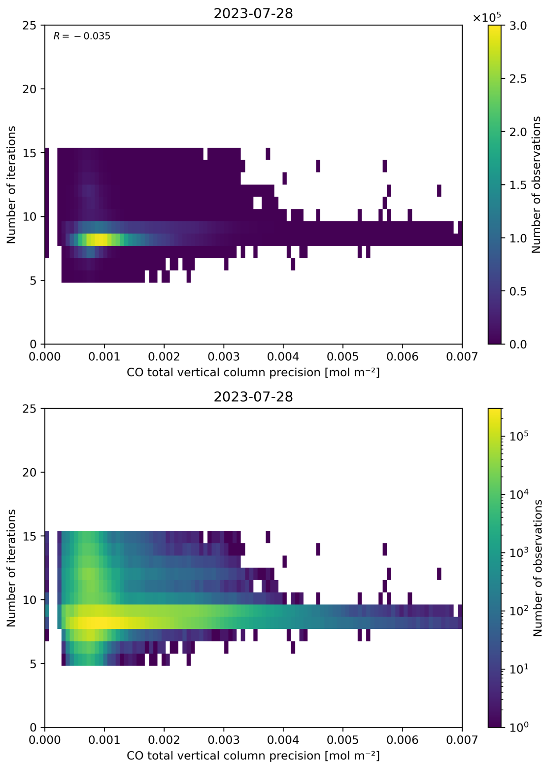
Figure 46: Scatter density plot of “CO total vertical column precision” against “Number of iterations” for 2023-07-27 to 2023-07-29.
