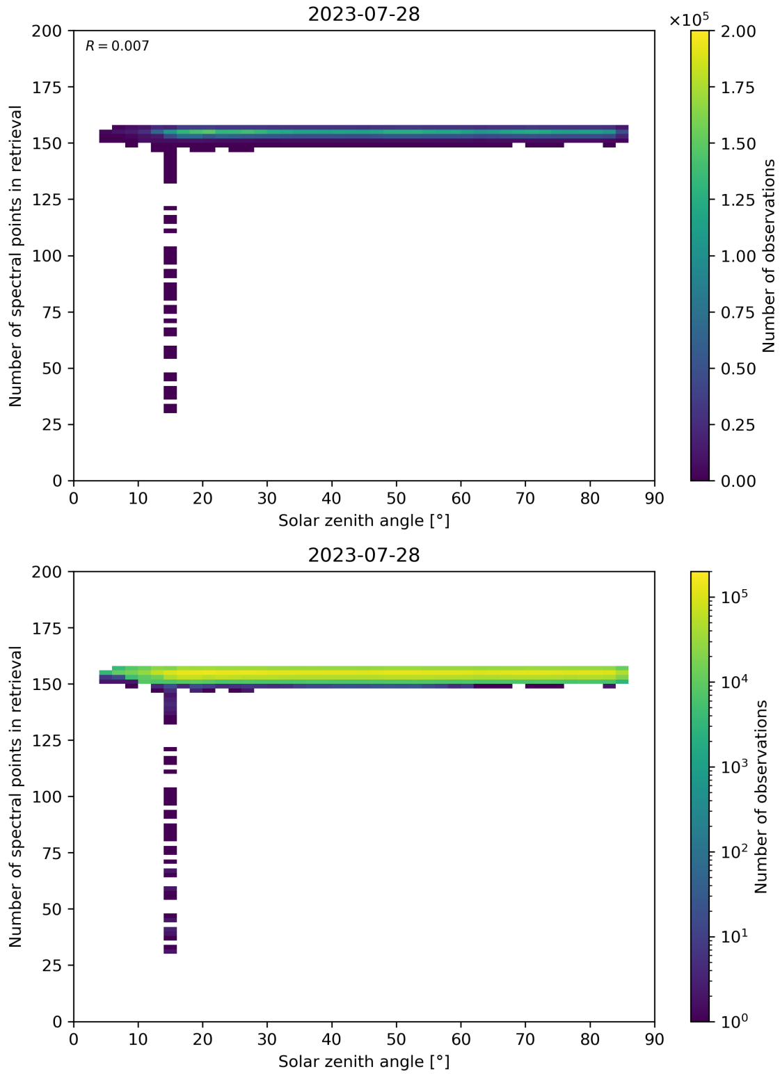
Figure 68: Scatter density plot of “Solar zenith angle” against “Number of spectral points in retrieval” for 2023-07-27 to 2023-07-29.
