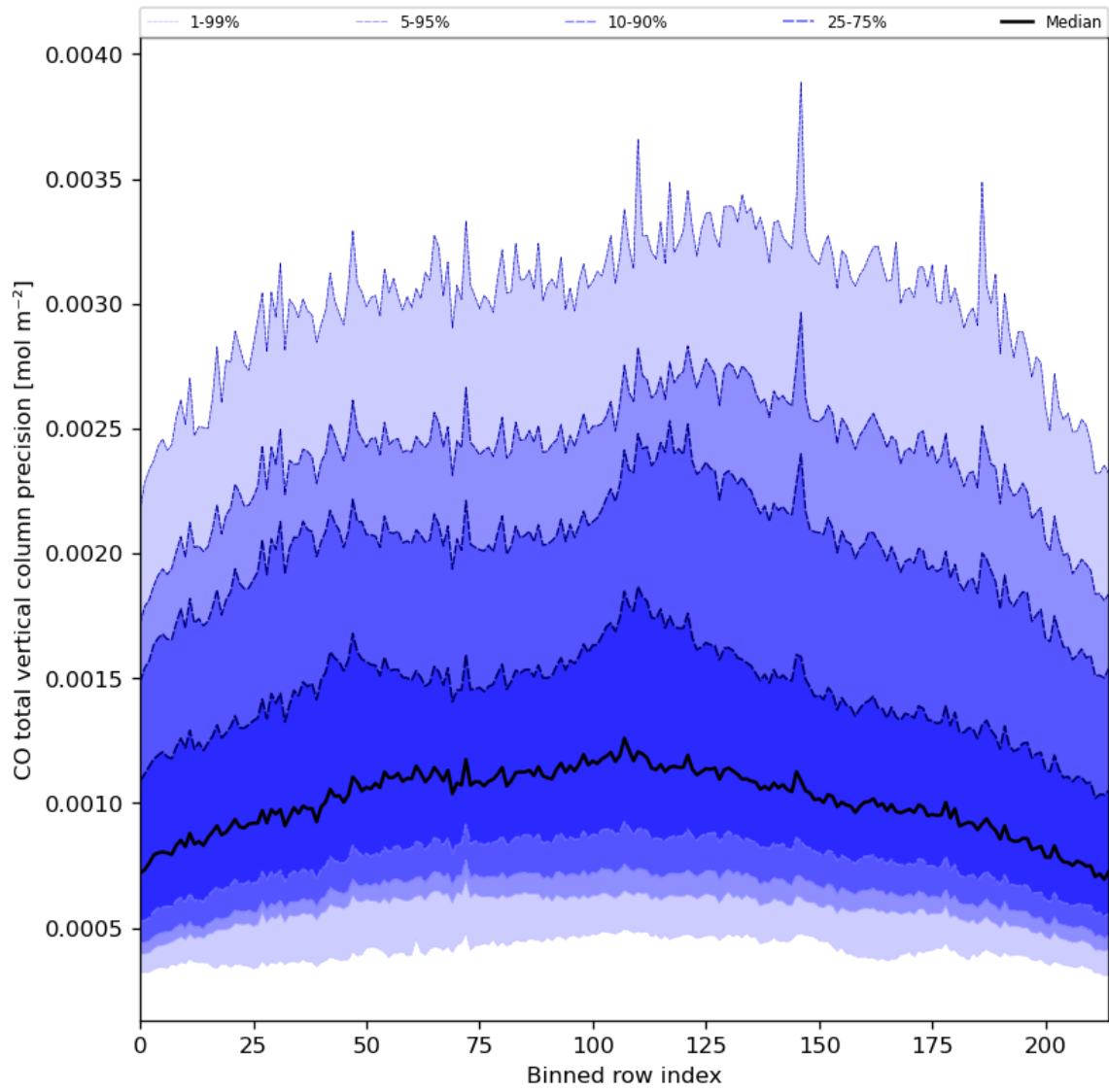
Figure 28: Along track statistics of “CO total vertical column precision” for 2023-07-27 to 2023-07-29
