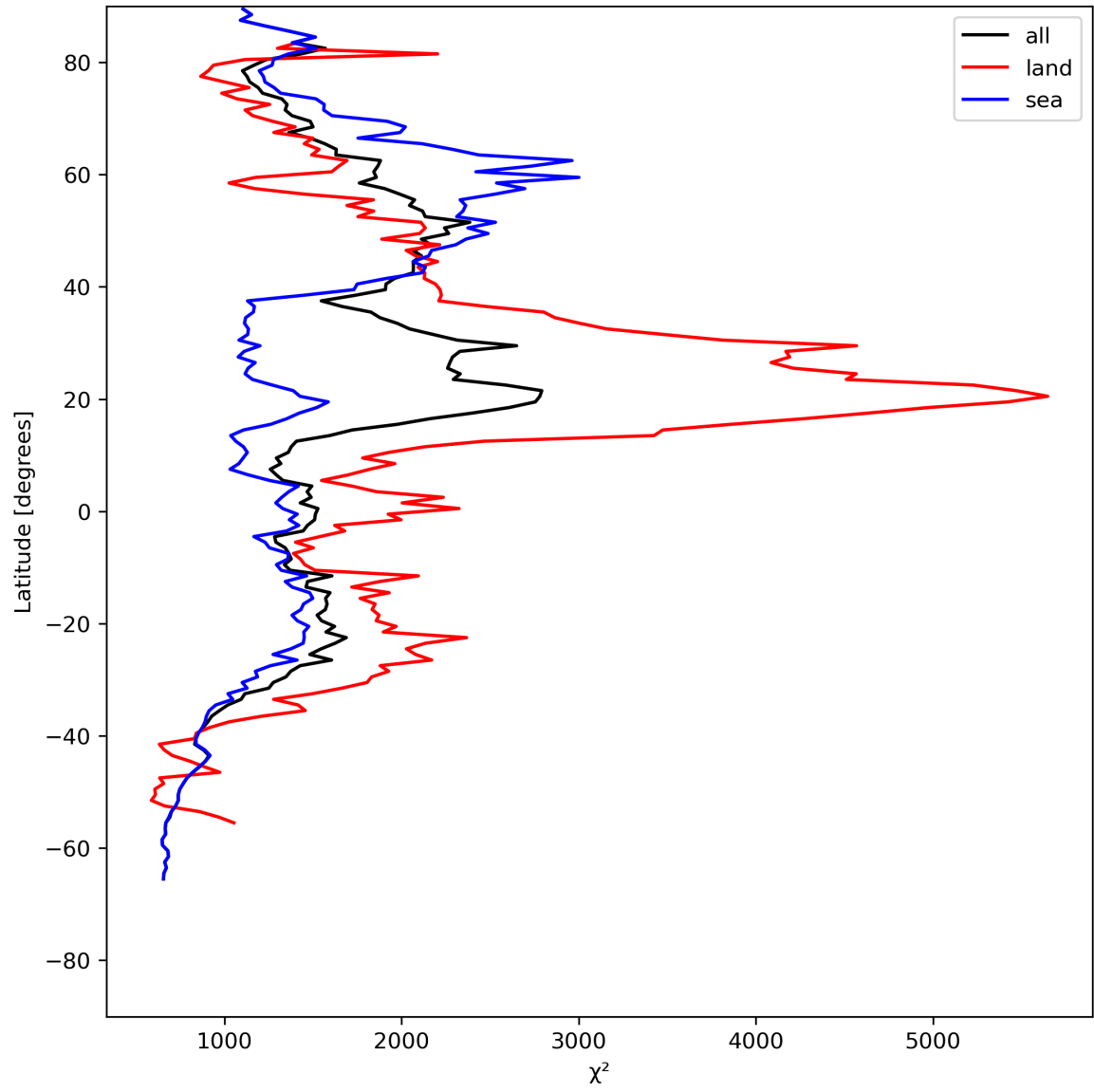
Figure 14: Zonal average of “ \chi^2 ” for 2023-07-27 to 2023-07-29.
