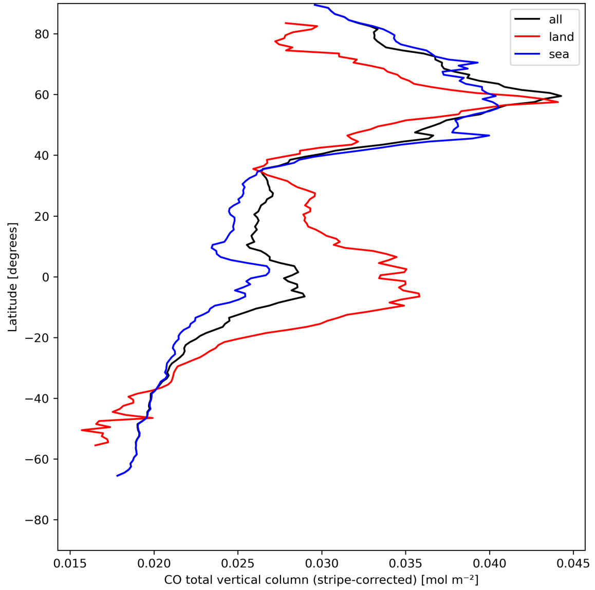
Figure 11: Zonal average of “CO total vertical column (stripe-corrected)” for 2023-07-27 to 2023-07-29.
