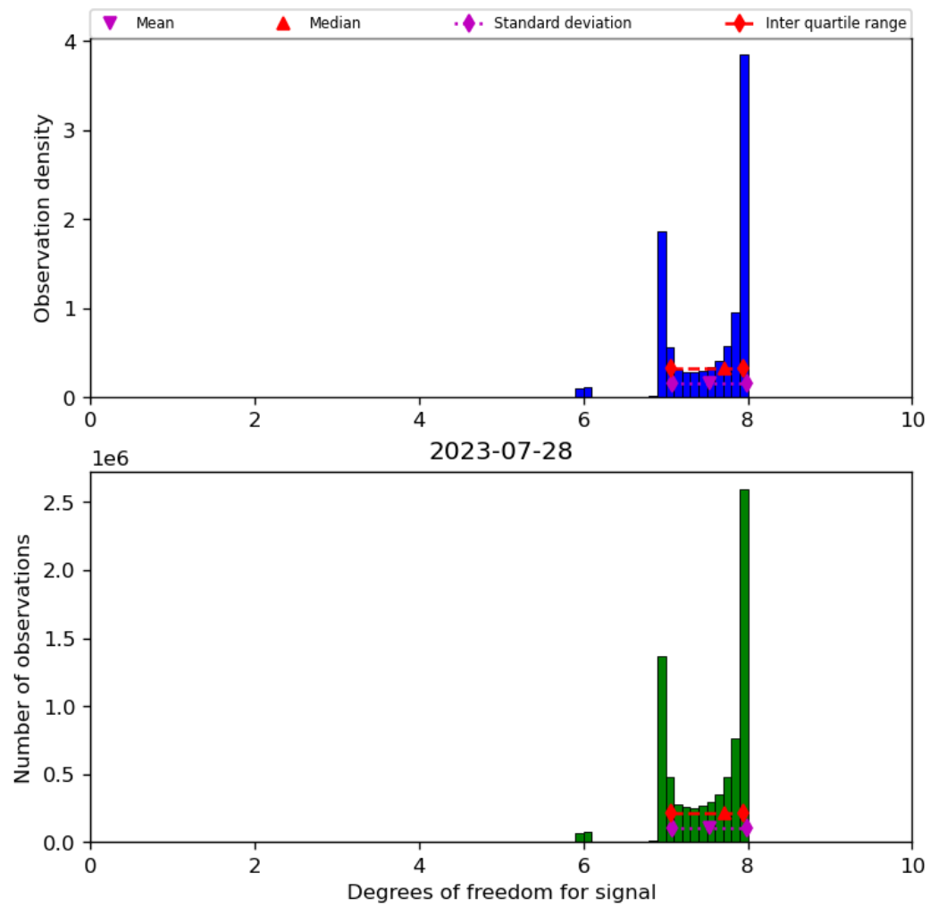
Figure 23: Histogram of “Degrees of freedom for signal” for 2023-07-27 to 2023-07-29
