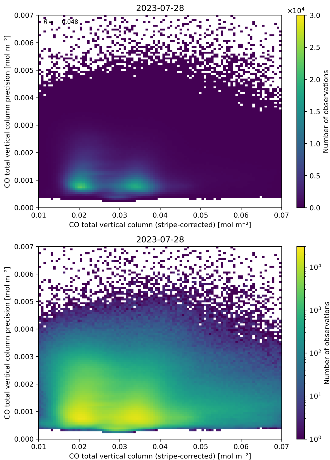
Figure 36: Scatter density plot of “CO total vertical column (stripe-corrected)” against “CO total vertical column precision” for 2023-07-27 to 2023-07-29.
