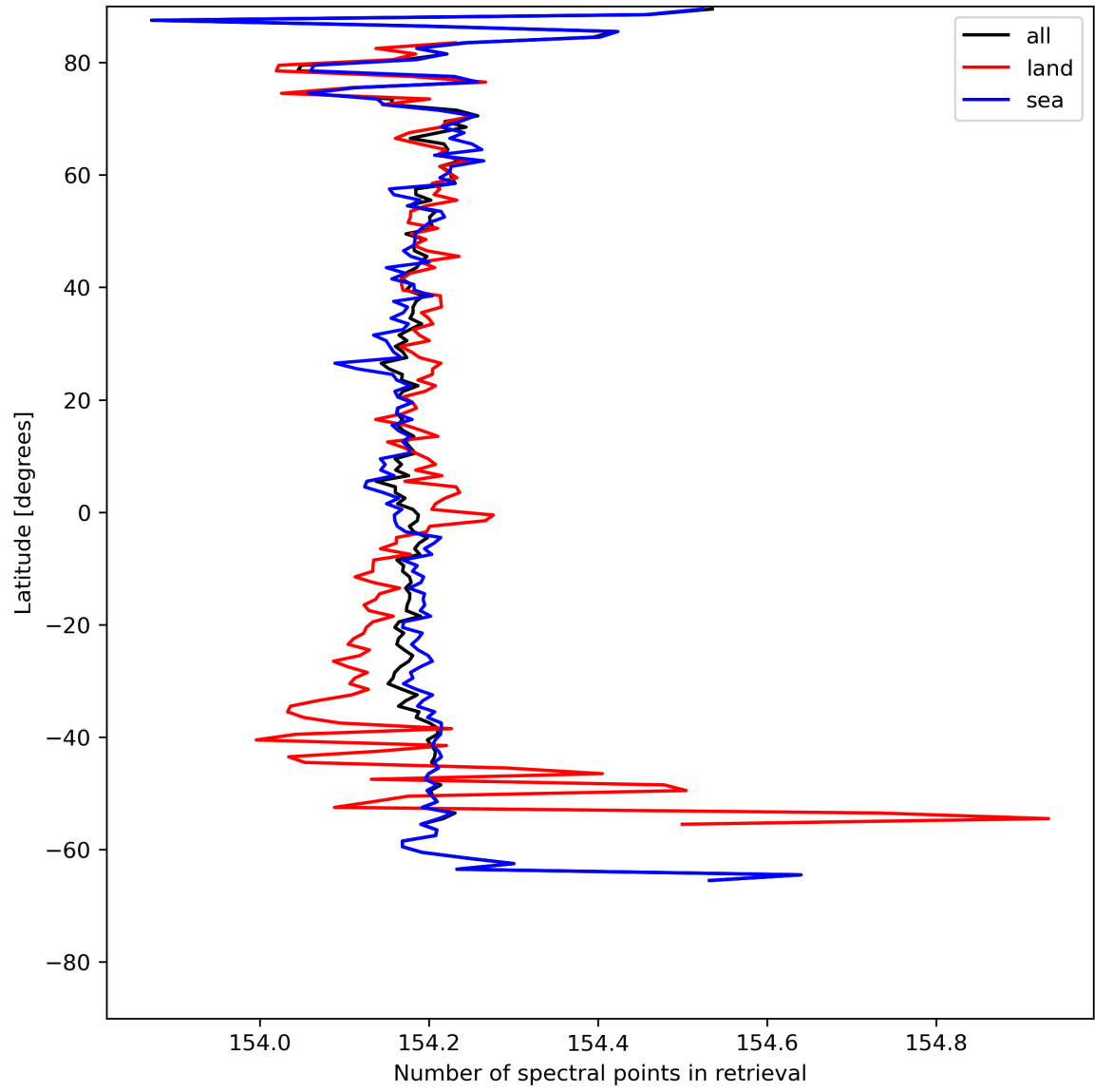
Figure 13: Zonal average of “Number of spectral points in retrieval” for 2023-07-27 to 2023-07-29.
