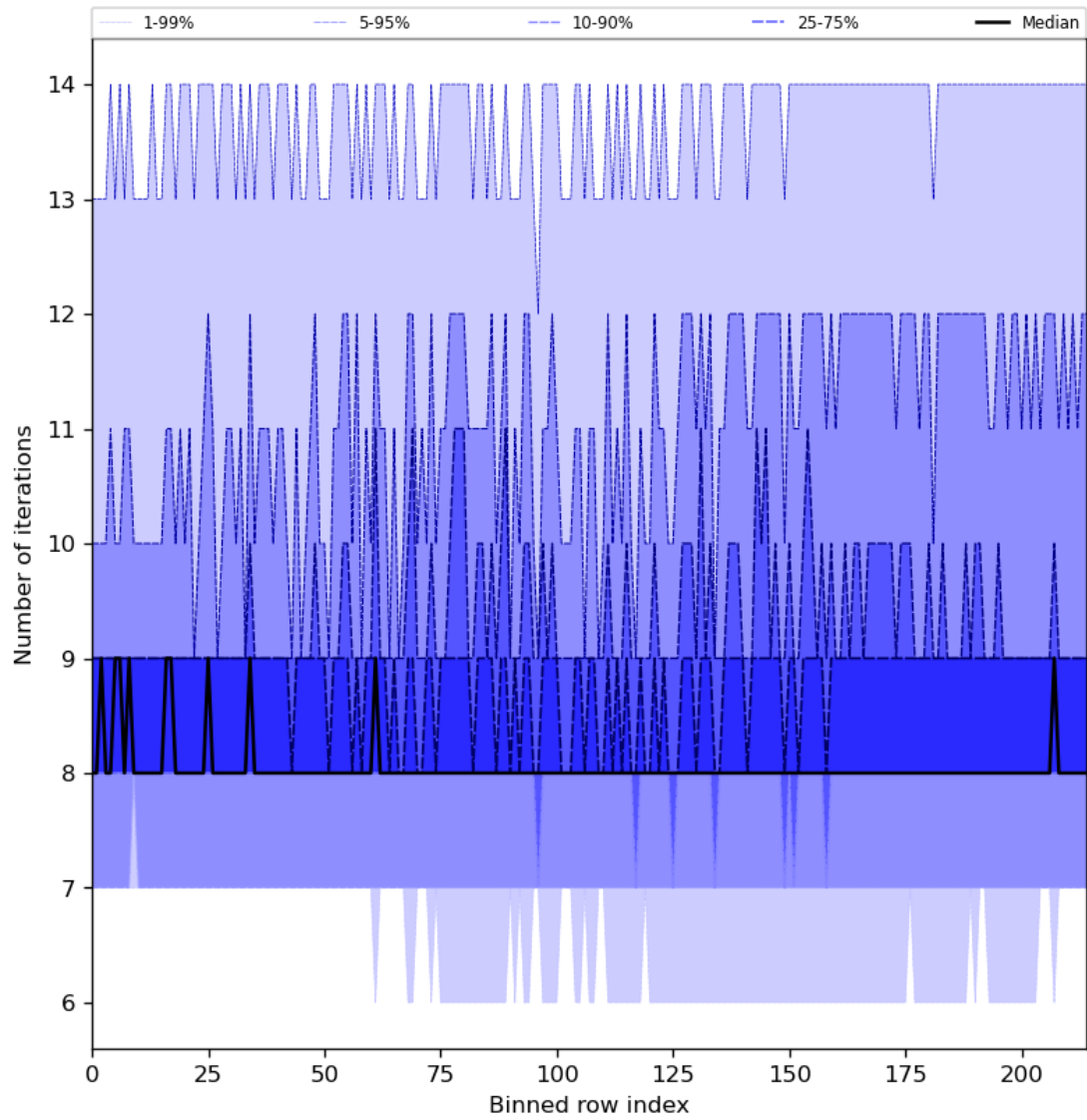
Figure 32: Along track statistics of “Number of iterations” for 2023-07-27 to 2023-07-29
