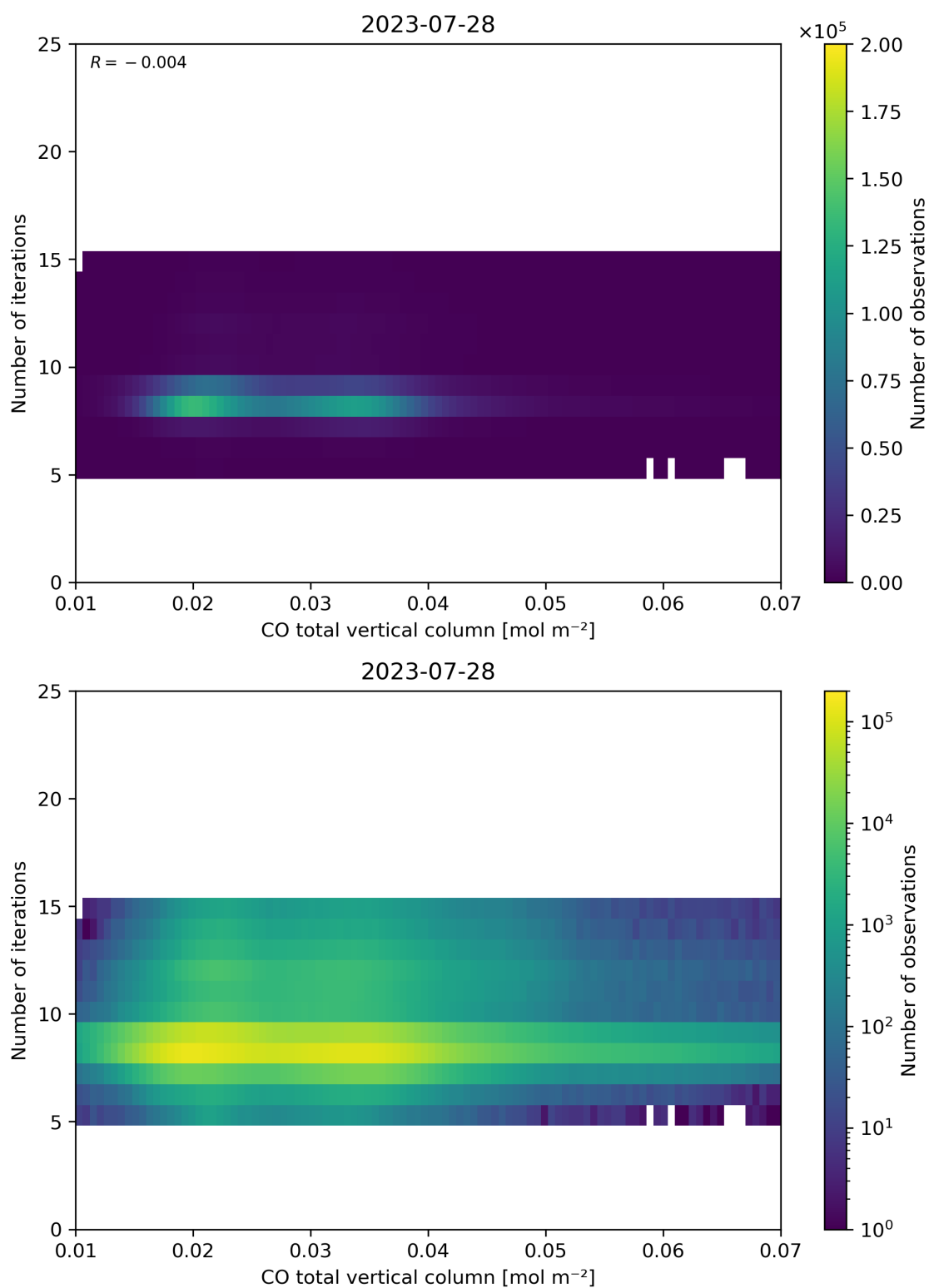
Figure 42: Scatter density plot of “CO total vertical column” against “Number of iterations” for 2023-07-27 to 2023-07-29.
