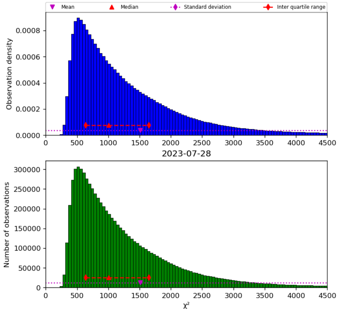
Figure 22: Histogram of “ \chi^2 ” for 2023-07-27 to 2023-07-29
