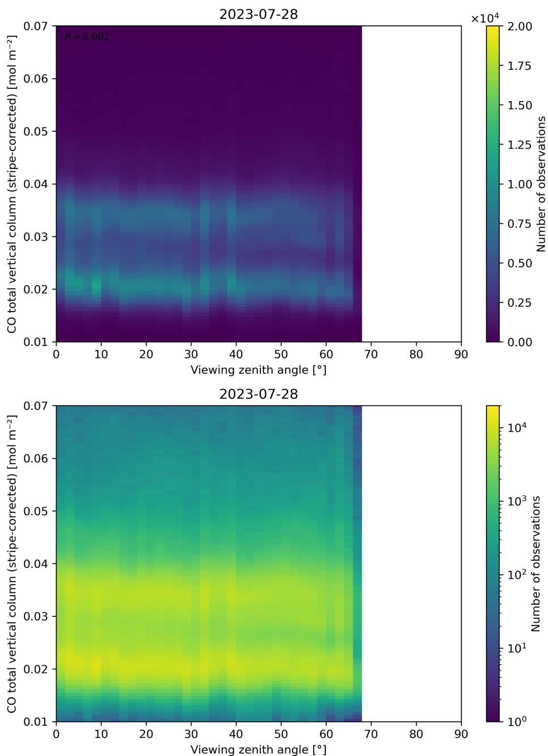
Figure 70: Scatter density plot of “Viewing zenith angle” against “CO total vertical column (stripe-corrected)” for 2023-07-27 to 2023-07-29.
