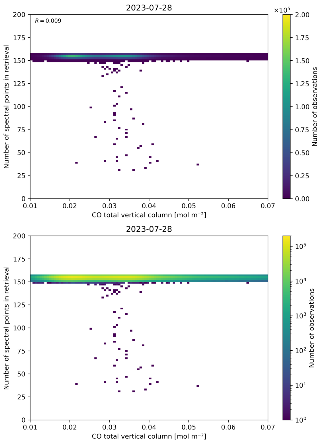
Figure 43: Scatter density plot of “CO total vertical column” against “Number of spectral points in retrieval” for 2023-07-27 to 2023-07-29.
