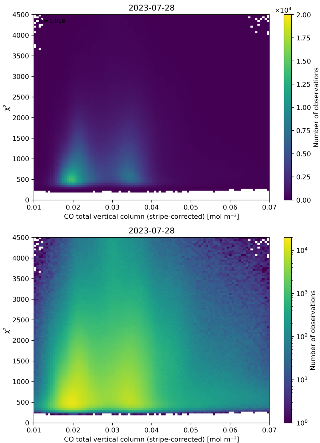
Figure 37: Scatter density plot of “CO total vertical column (stripe-corrected)” against “ \chi^2 ” for 2023-07-27 to 2023-07-29.
