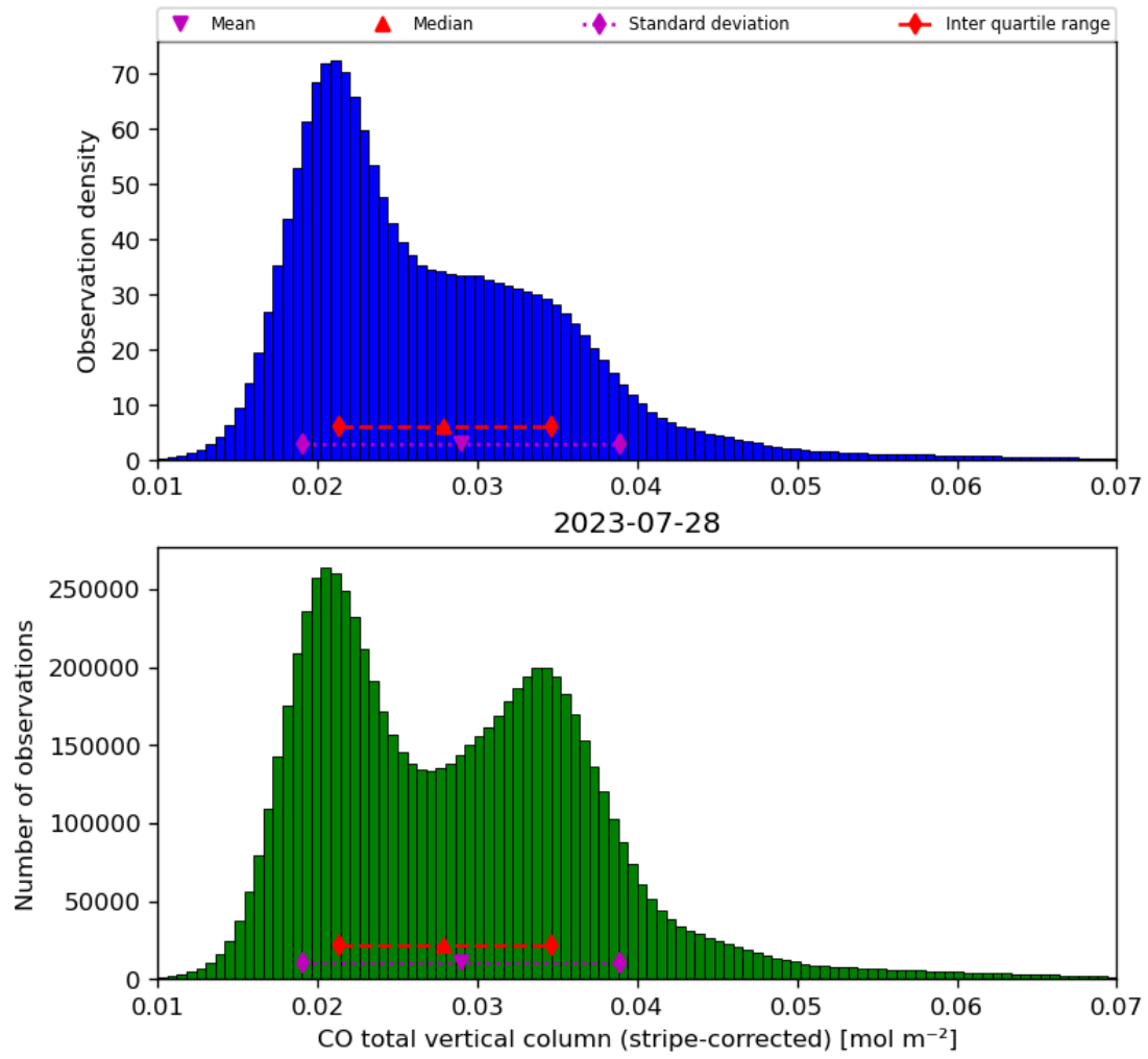
Figure 19: Histogram of “CO total vertical column (stripe-corrected)” for 2023-07-27 to 2023-07-29
