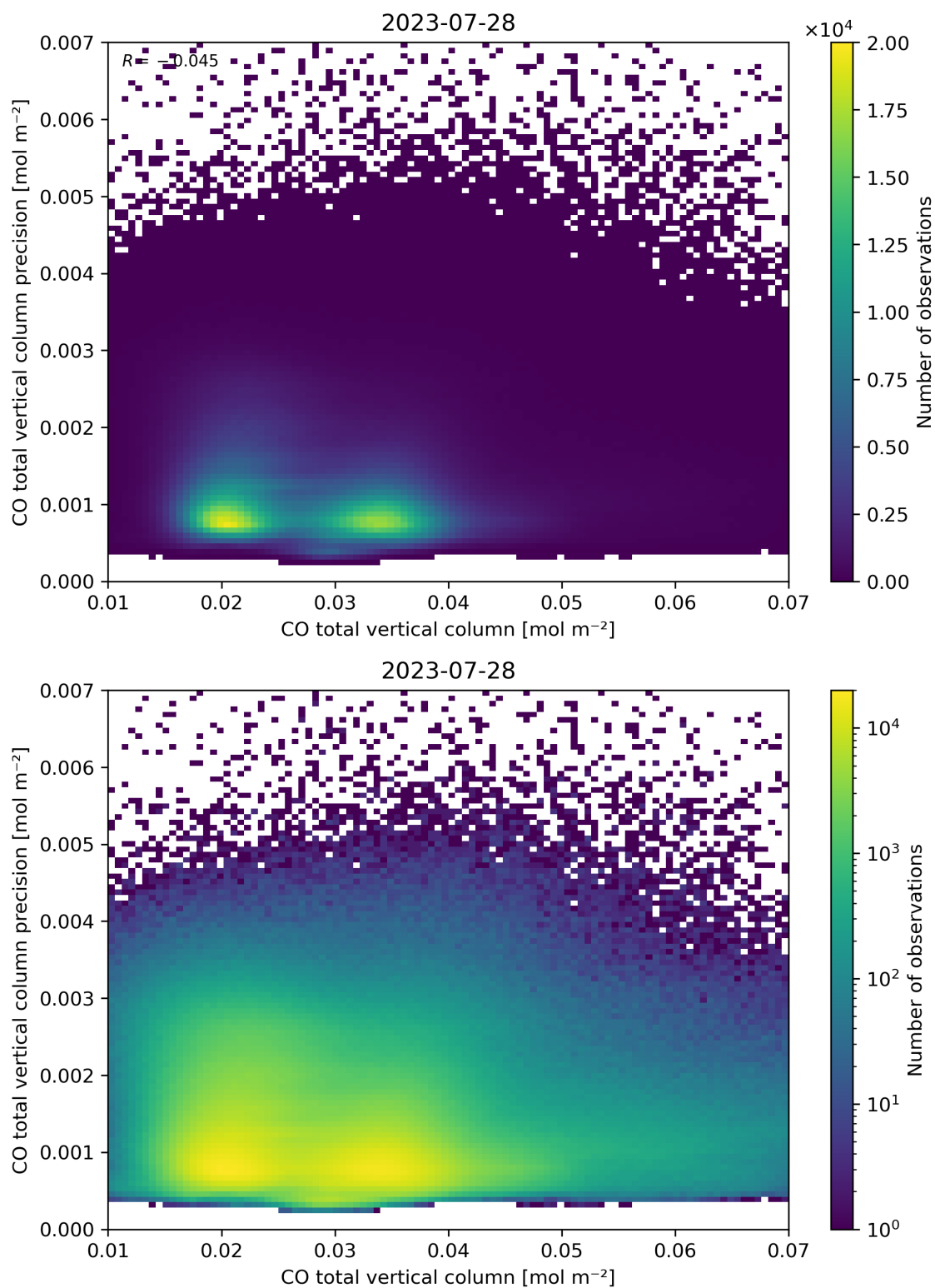
Figure 34: Scatter density plot of “CO total vertical column” against “CO total vertical column precision” for 2023-07-27 to 2023-07-29.
