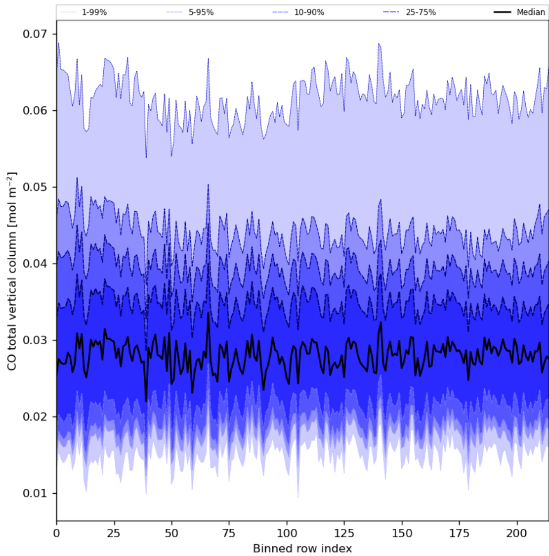
Figure 26: Along track statistics of “CO total vertical column” for 2023-07-27 to 2023-07-29
