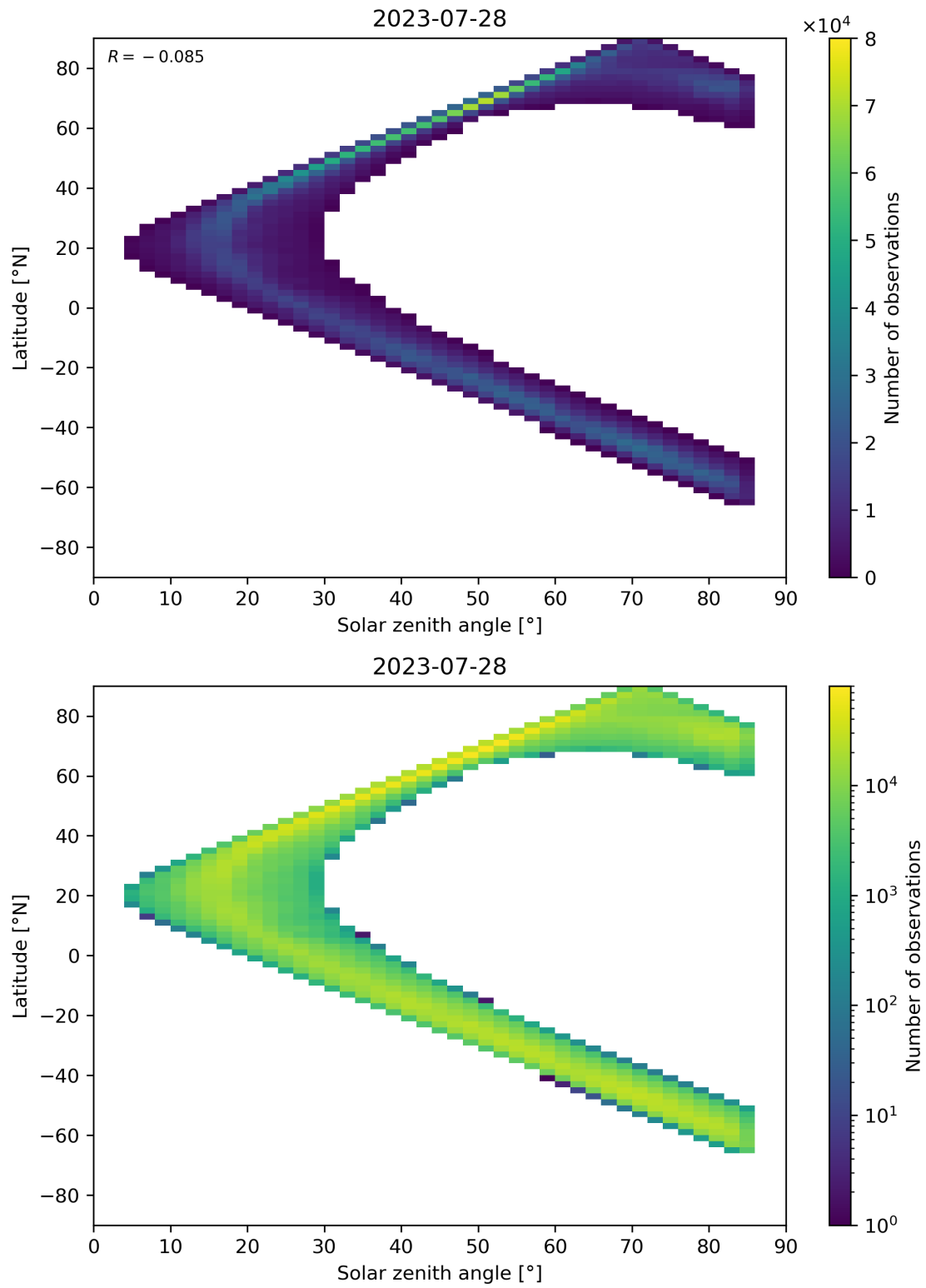
Figure 66: Scatter density plot of “Solar zenith angle” against “Latitude” for 2023-07-27 to 2023-07-29.
