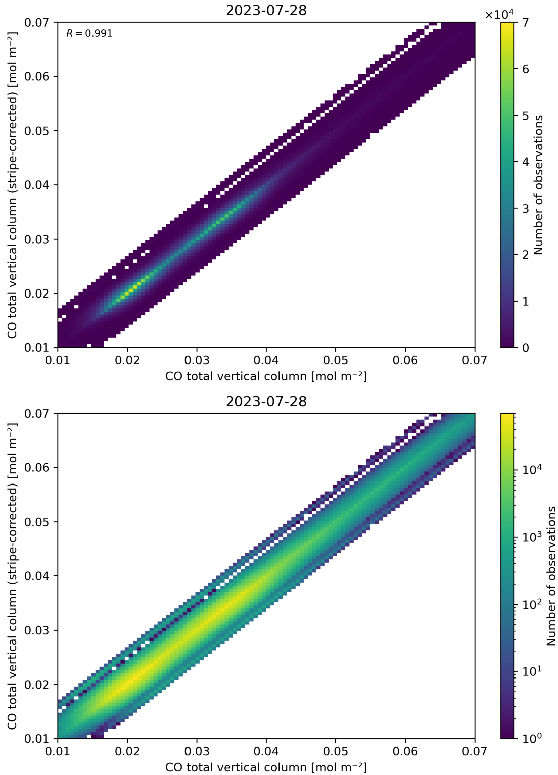
Figure 33: Scatter density plot of “CO total vertical column” against “CO total vertical column (stripe-corrected)” for 2023-07-27 to 2023-07-29.
