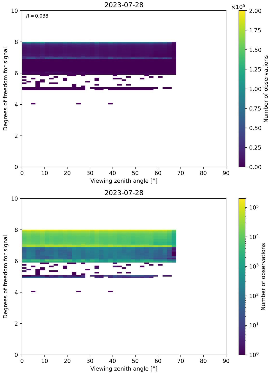
Figure 73: Scatter density plot of “Viewing zenith angle” against “Degrees of freedom for signal” for 2023-07-27 to 2023-07-29.
