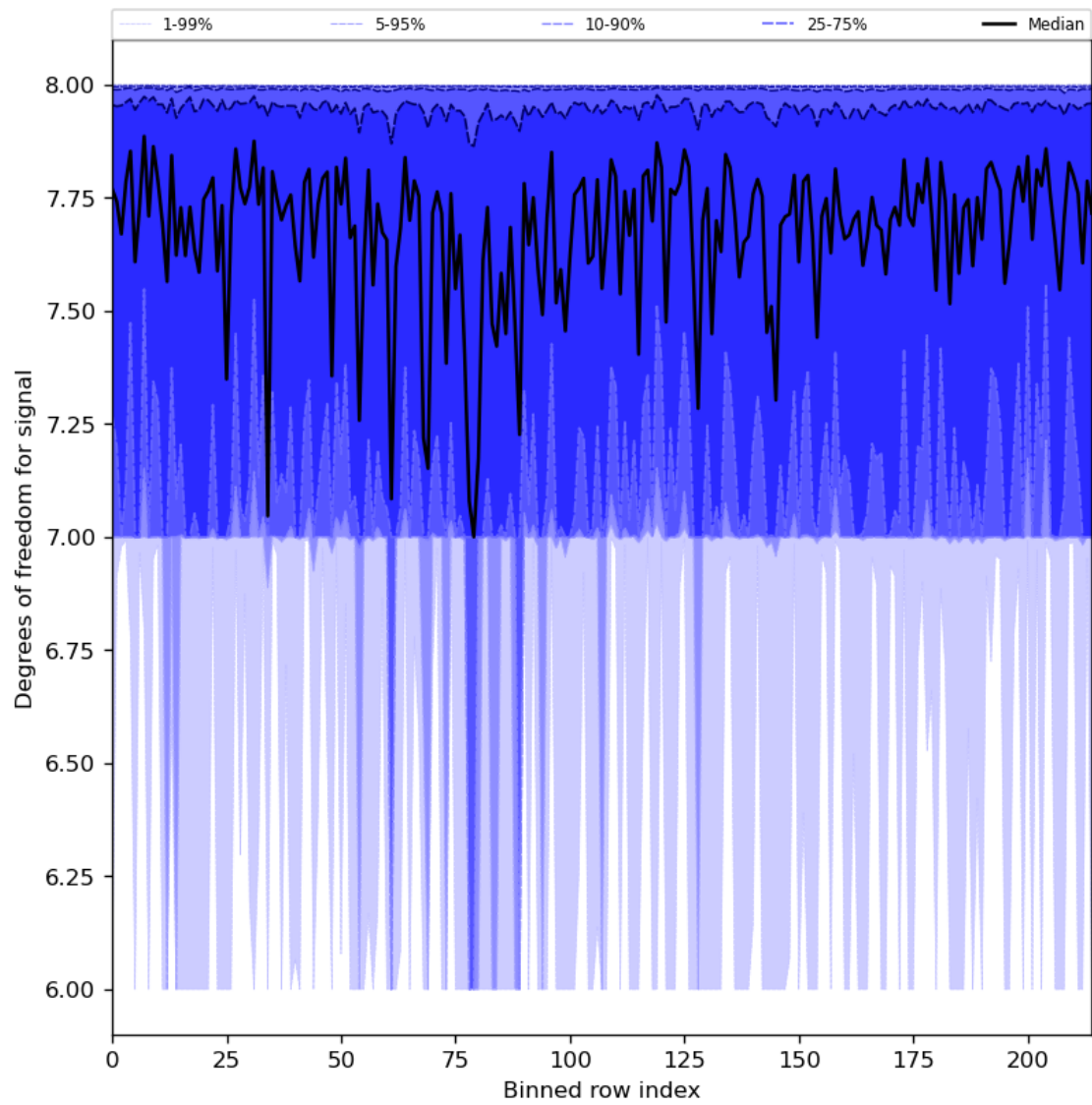
Figure 31: Along track statistics of “Degrees of freedom for signal” for 2023-07-27 to 2023-07-29
