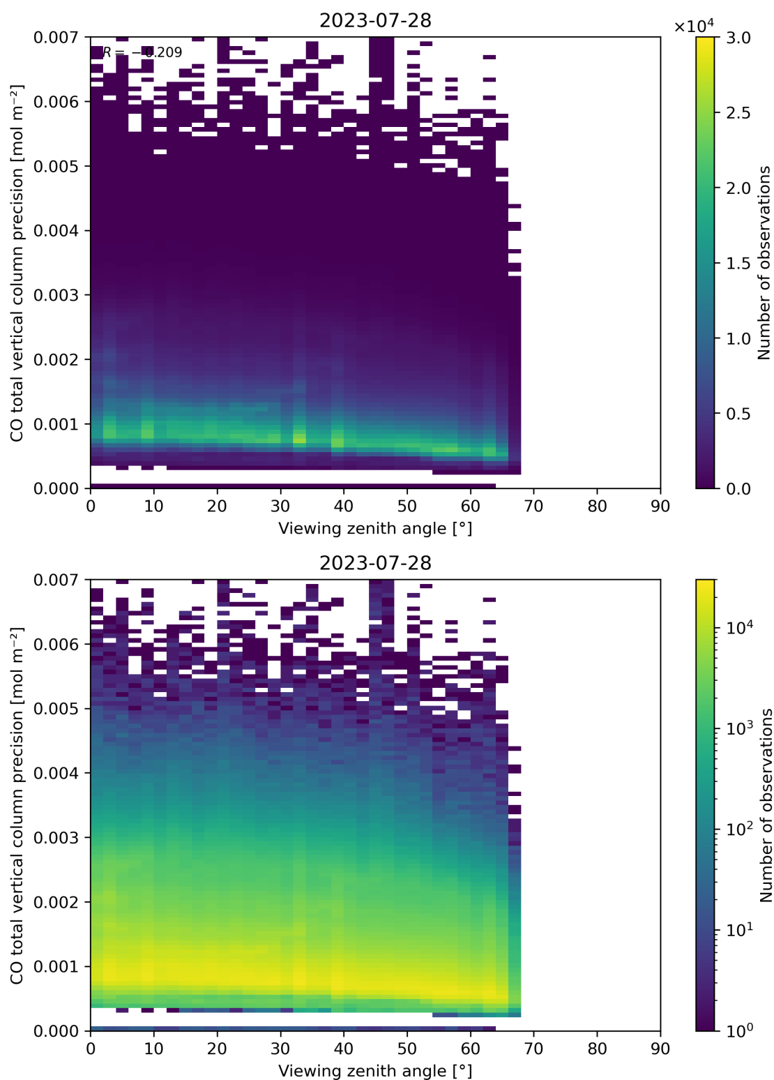
Figure 71: Scatter density plot of “Viewing zenith angle” against “CO total vertical column precision” for 2023-07-27 to 2023-07-29.
