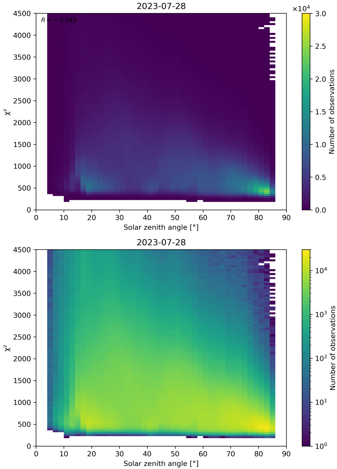
Figure 64: Scatter density plot of “Solar zenith angle” against “ \chi^2 ” for 2023-07-27 to 2023-07-29.
