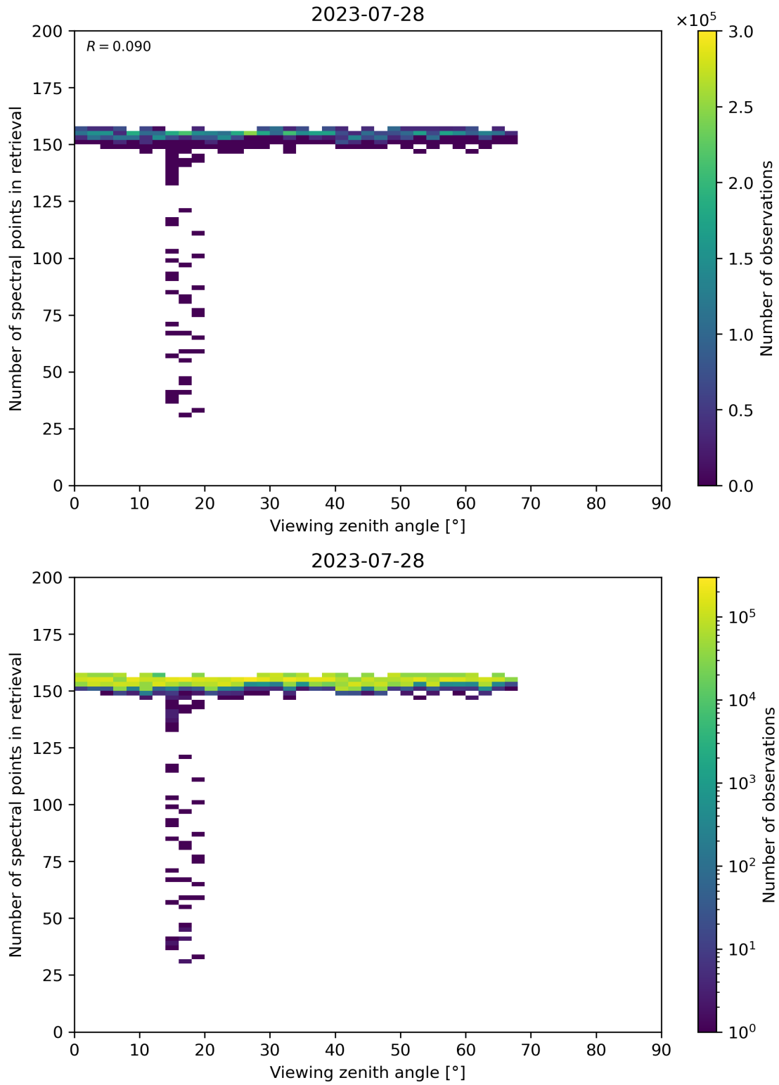
Figure 76: Scatter density plot of “Viewing zenith angle” against “Number of spectral points in retrieval” for 2023-07-27 to 2023-07-29.
