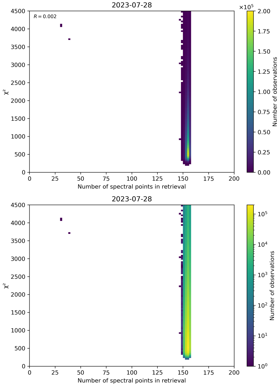
Figure 58: Scatter density plot of “Number of spectral points in retrieval” against “ \chi^2 ” for 2023-07-27 to 2023-07-29.
