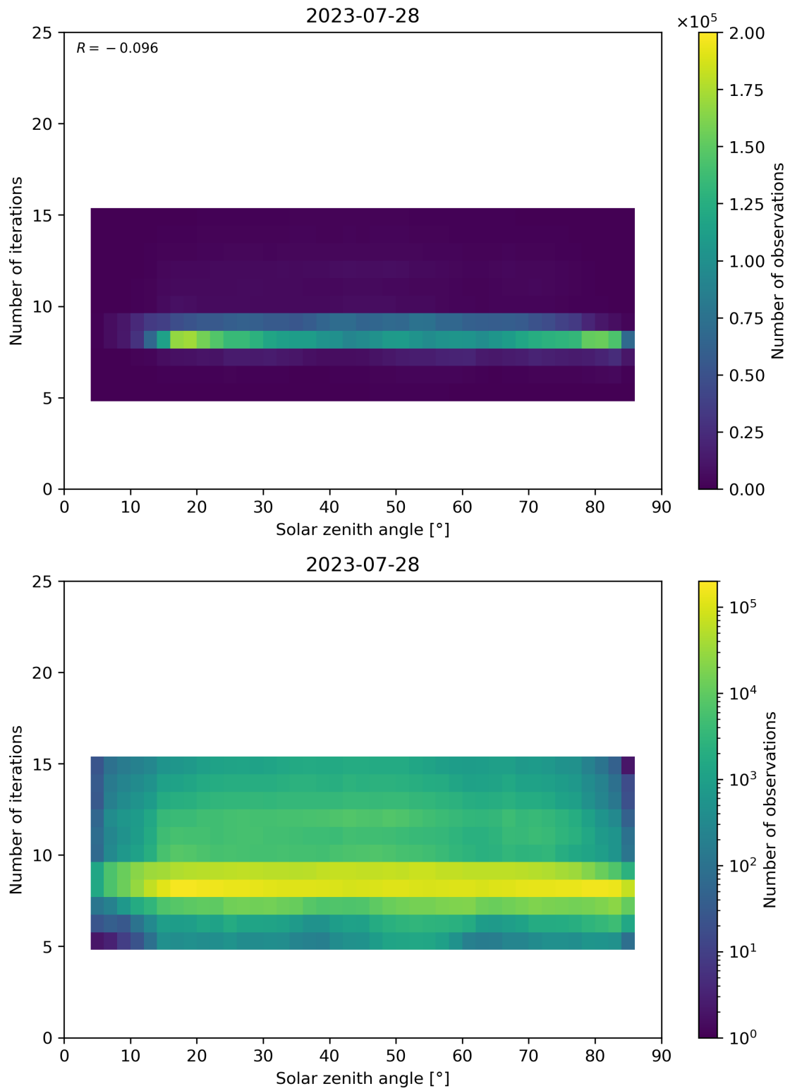
Figure 67: Scatter density plot of “Solar zenith angle” against “Number of iterations” for 2023-07-27 to 2023-07-29.
