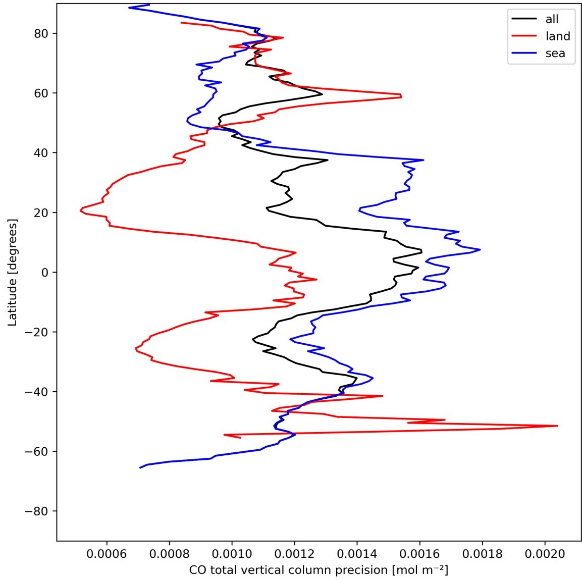
Figure 12: Zonal average of “CO total vertical column precision” for 2023-07-27 to 2023-07-29.
