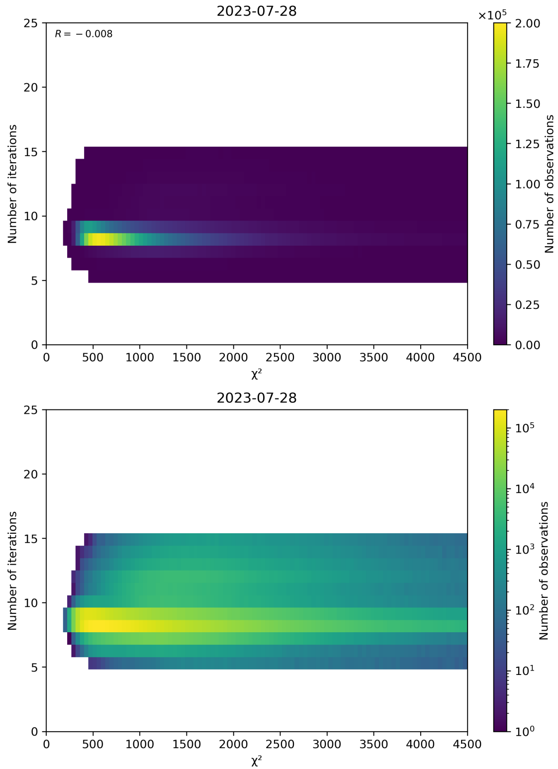
Figure 49: Scatter density plot of “ \chi^2 ” against “Number of iterations” for 2023-07-27 to 2023-07-29.
