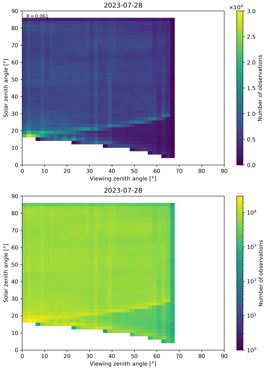
Figure 77: Scatter density plot of “Viewing zenith angle” against “Solar zenith angle” for 2023-07-27 to 2023-07-29.
