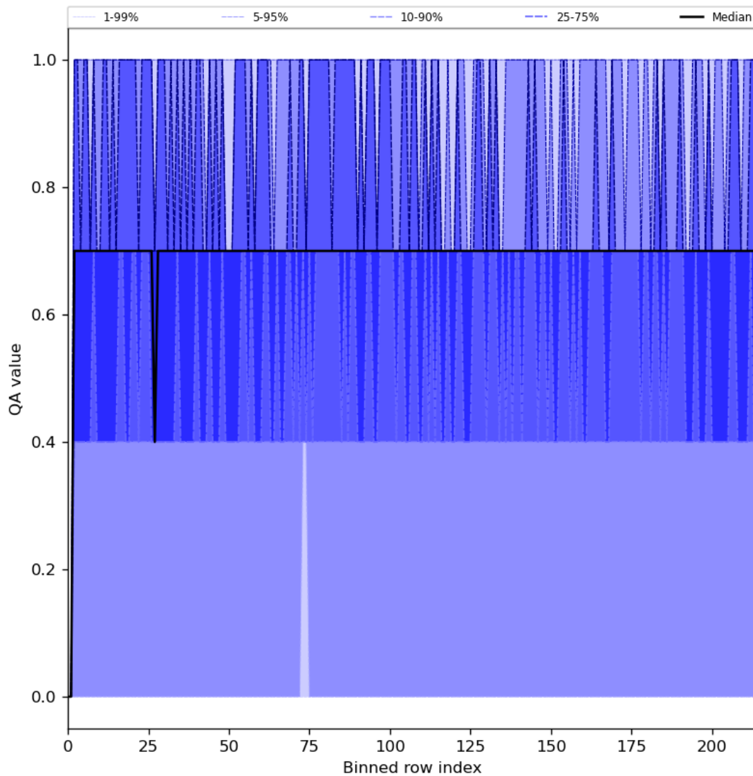
Figure 25: Along track statistics of “QA value” for 2023-07-27 to 2023-07-29
