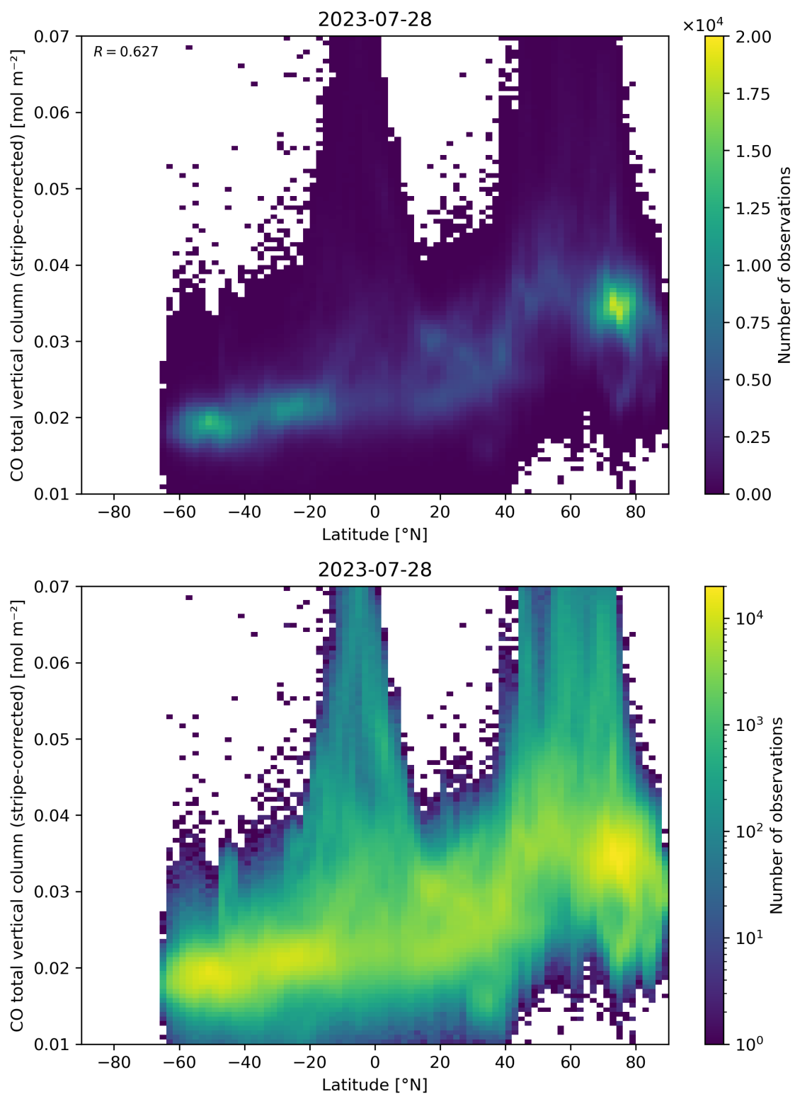
Figure 52: Scatter density plot of “Latitude” against “CO total vertical column (stripe-corrected)” for 2023-07-27 to 2023-07-29.
