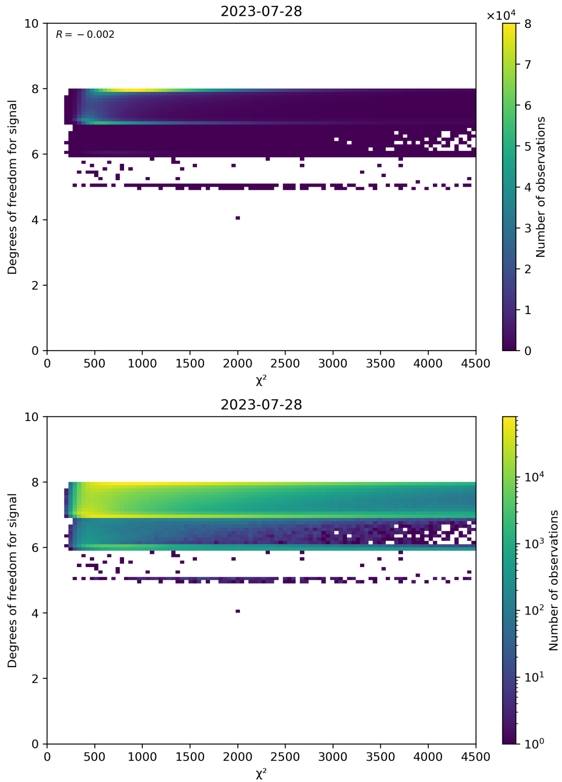
Figure 48: Scatter density plot of “ \chi^2 ” against “Degrees of freedom for signal” for 2023-07-27 to 2023-07-29.
