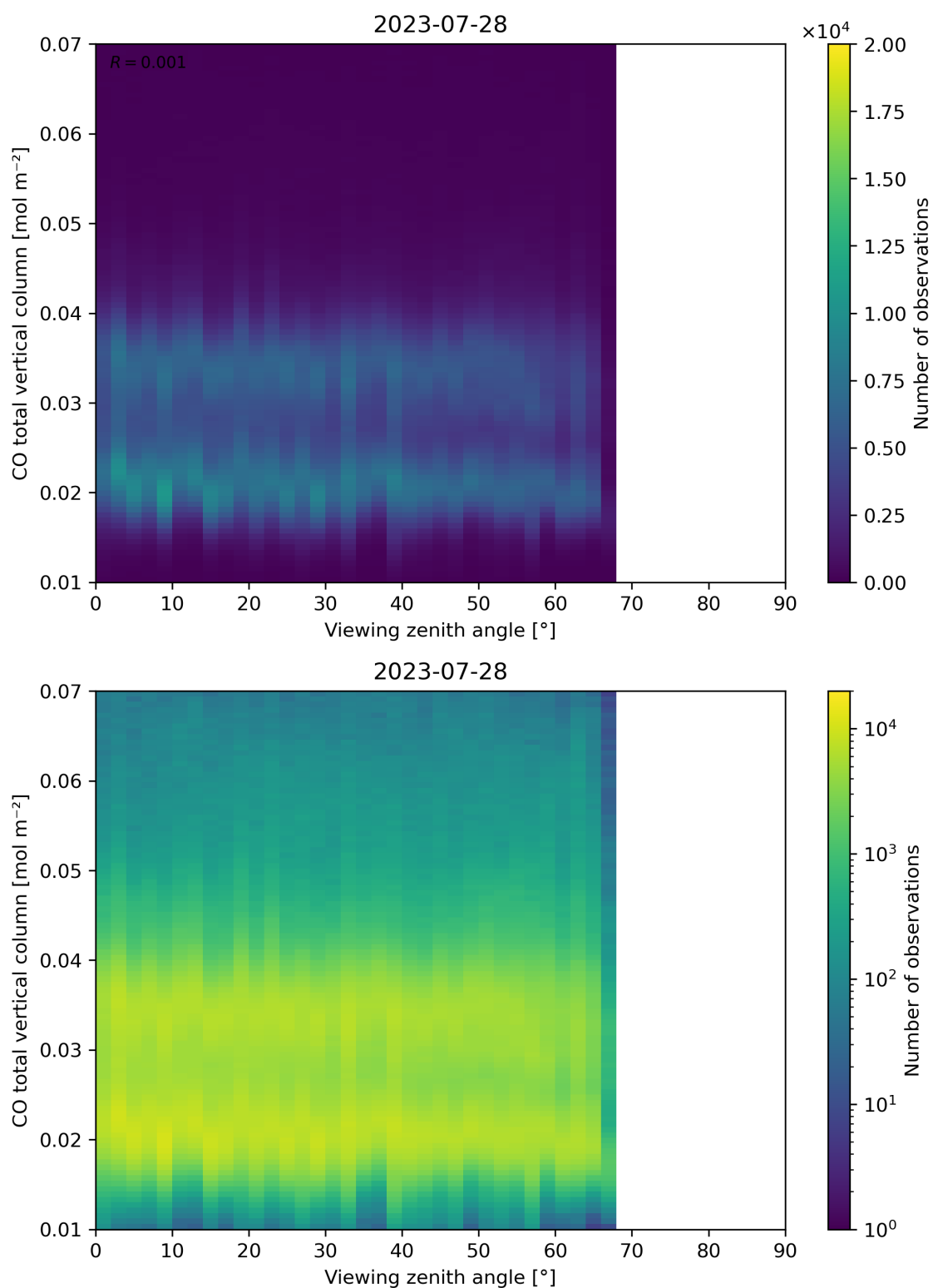
Figure 69: Scatter density plot of “Viewing zenith angle” against “CO total vertical column” for 2023-07-27 to 2023-07-29.
