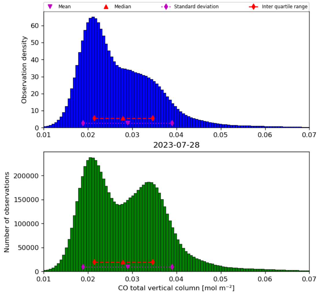
Figure 18: Histogram of “CO total vertical column” for 2023-07-27 to 2023-07-29
