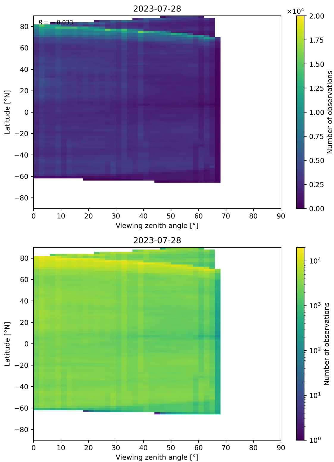
Figure 74: Scatter density plot of “Viewing zenith angle” against “Latitude” for 2023-07-27 to 2023-07-29.
