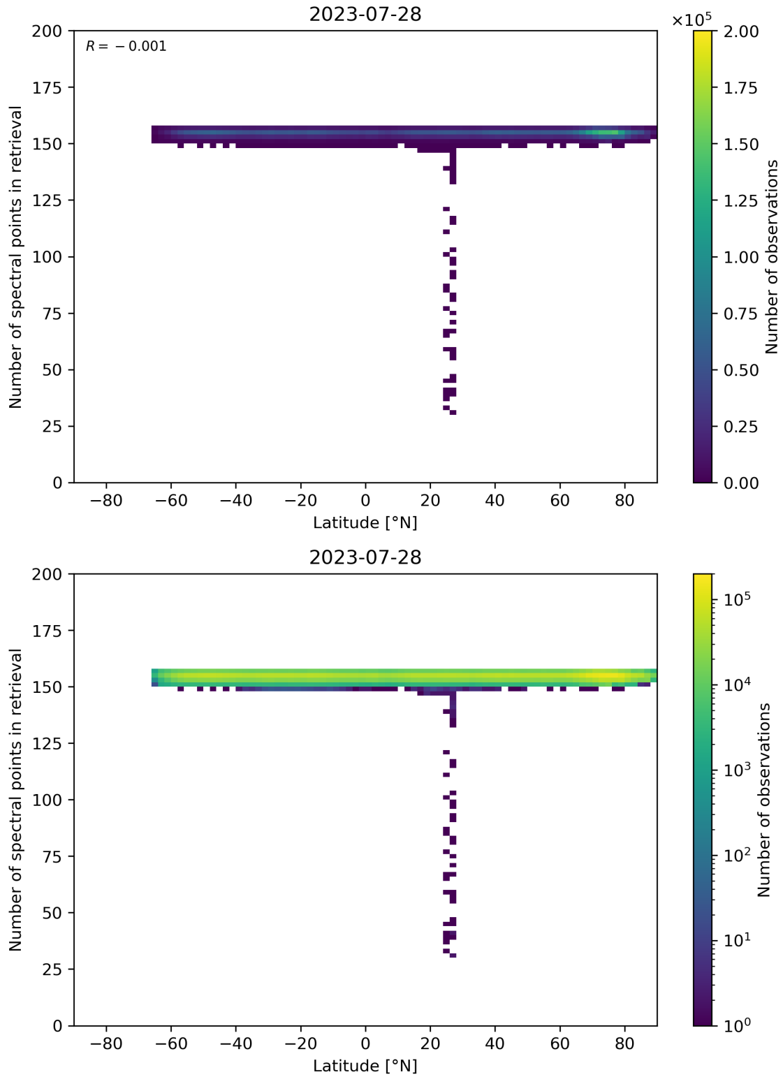
Figure 57: Scatter density plot of “Latitude” against “Number of spectral points in retrieval” for 2023-07-27 to 2023-07-29.
