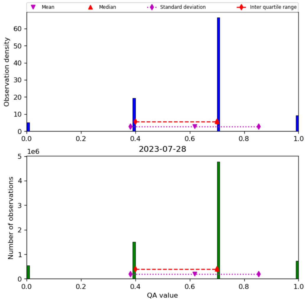
Figure 17: Histogram of “QA value” for 2023-07-27 to 2023-07-29
