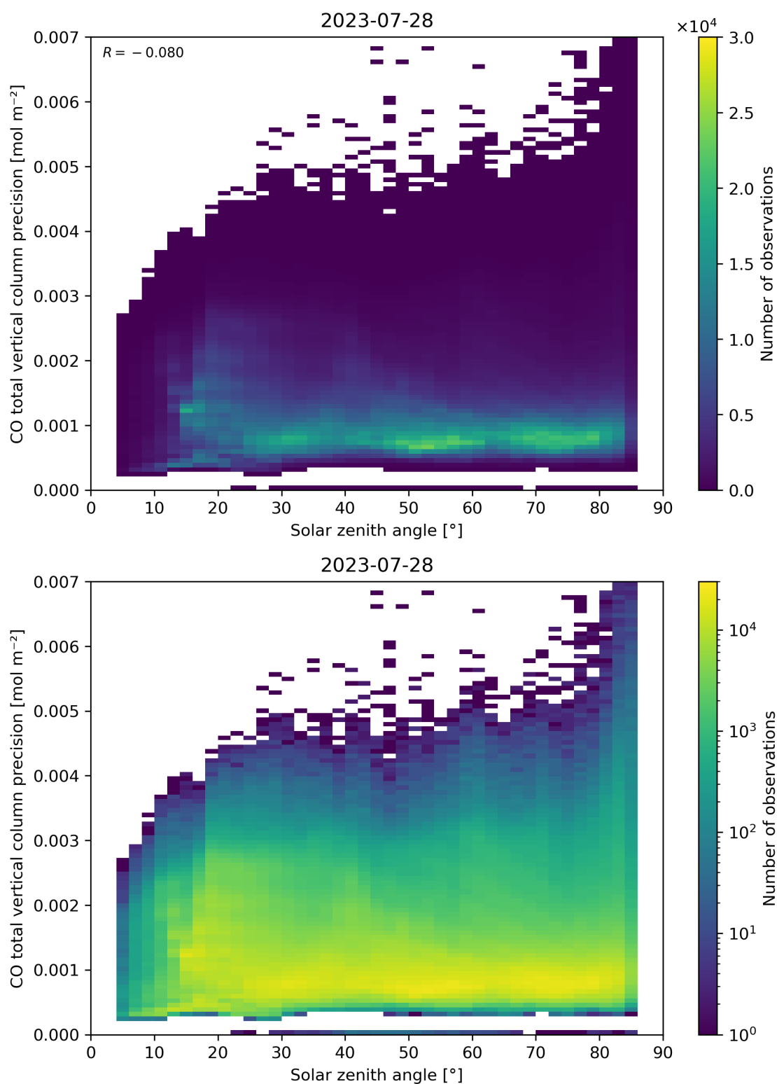
Figure 63: Scatter density plot of “Solar zenith angle” against “CO total vertical column precision” for 2023-07-27 to 2023-07-29.
