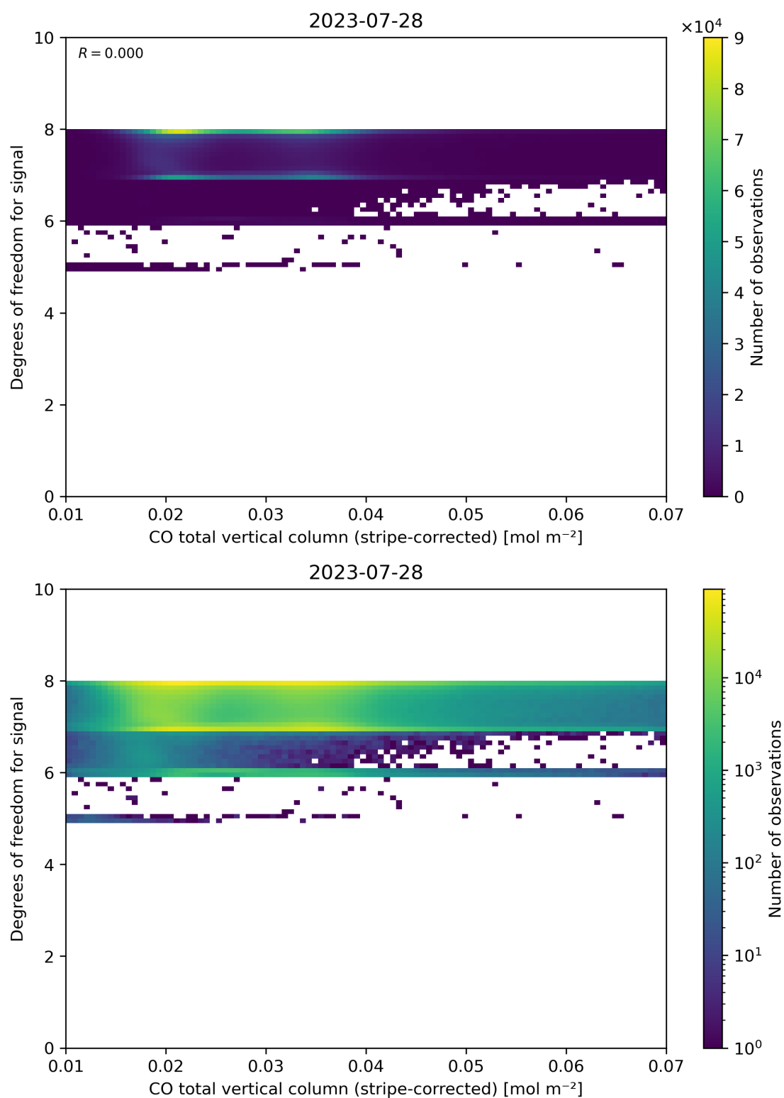
Figure 38: Scatter density plot of “CO total vertical column (stripe-corrected)” against “Degrees of freedom for signal” for 2023-07-27 to 2023-07-29.
