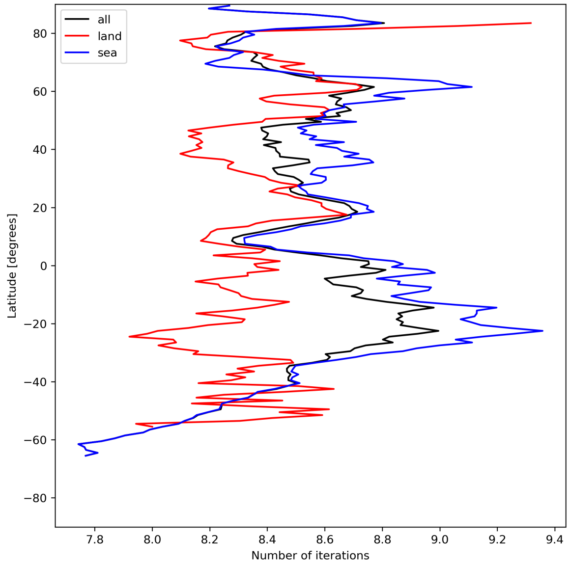
Figure 16: Zonal average of “Number of iterations” for 2023-07-27 to 2023-07-29.
