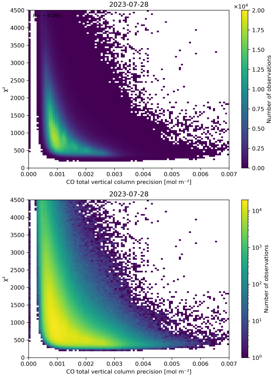
Figure 44: Scatter density plot of “CO total vertical column precision” against “ \chi^2 ” for 2023-07-27 to 2023-07-29.
