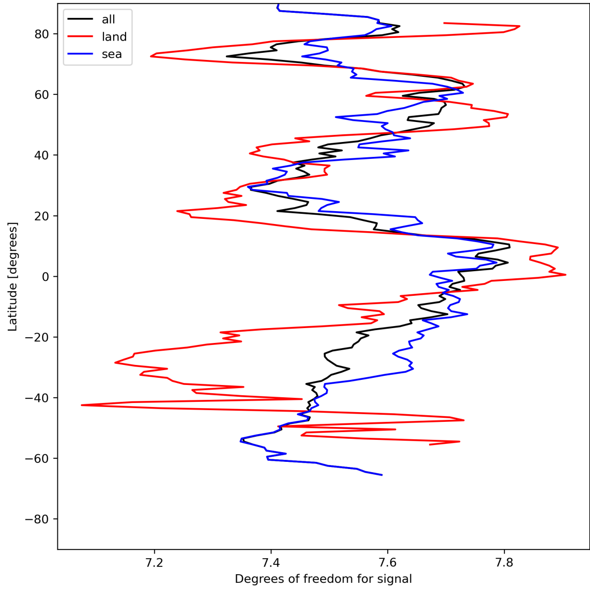
Figure 15: Zonal average of “Degrees of freedom for signal” for 2023-07-27 to 2023-07-29.
