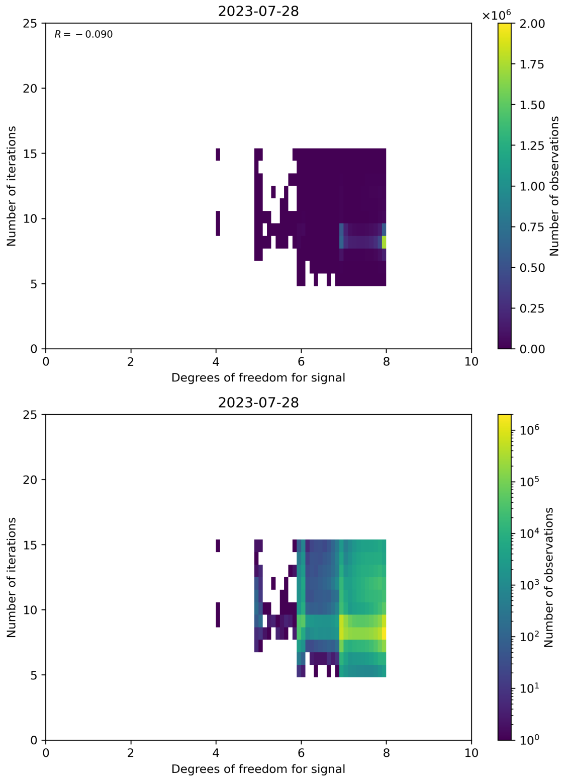
Figure 50: Scatter density plot of “Degrees of freedom for signal” against “Number of iterations” for 2023-07-27 to 2023-07-29.
