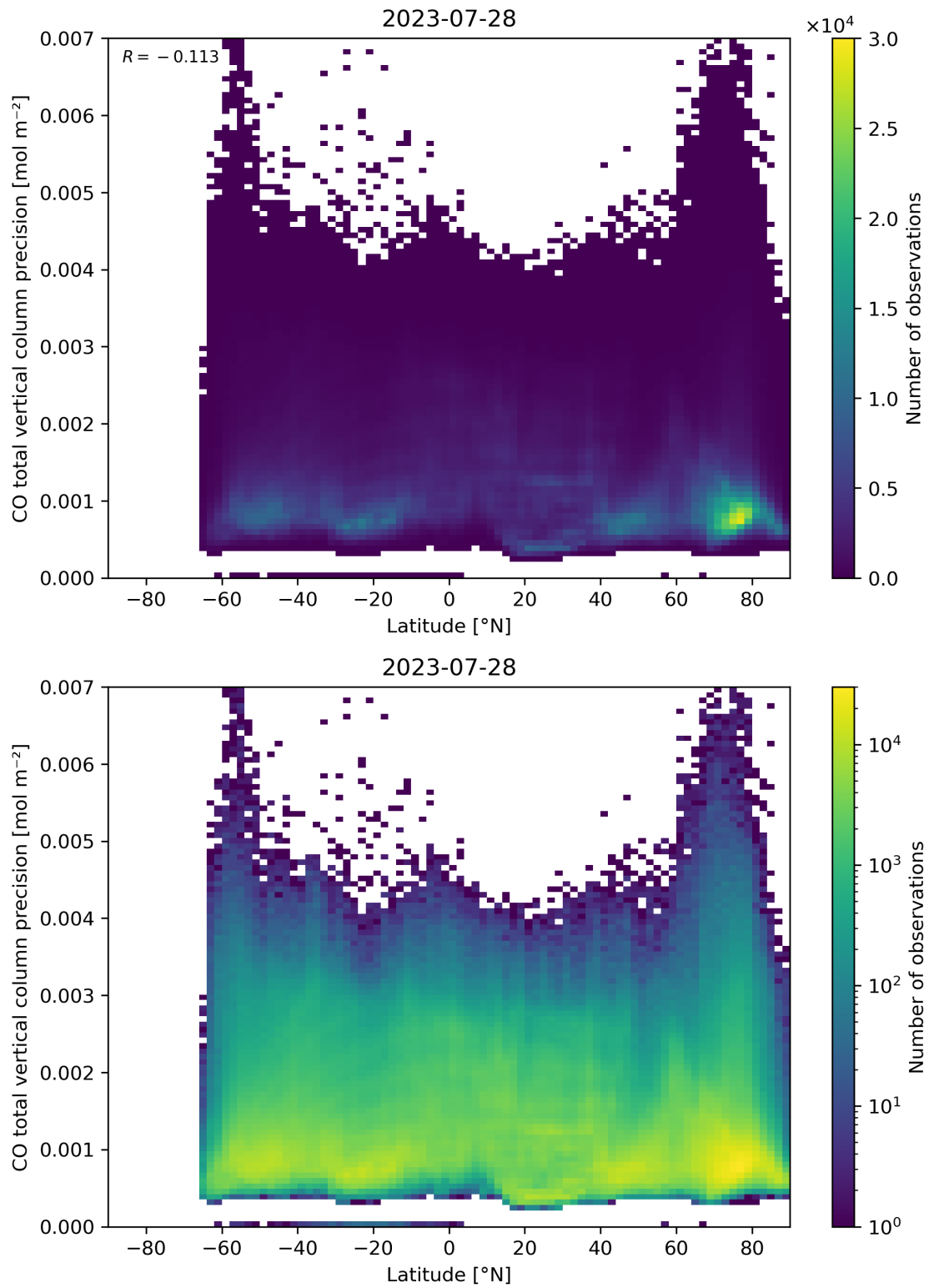
Figure 53: Scatter density plot of “Latitude” against “CO total vertical column precision” for 2023-07-27 to 2023-07-29.
