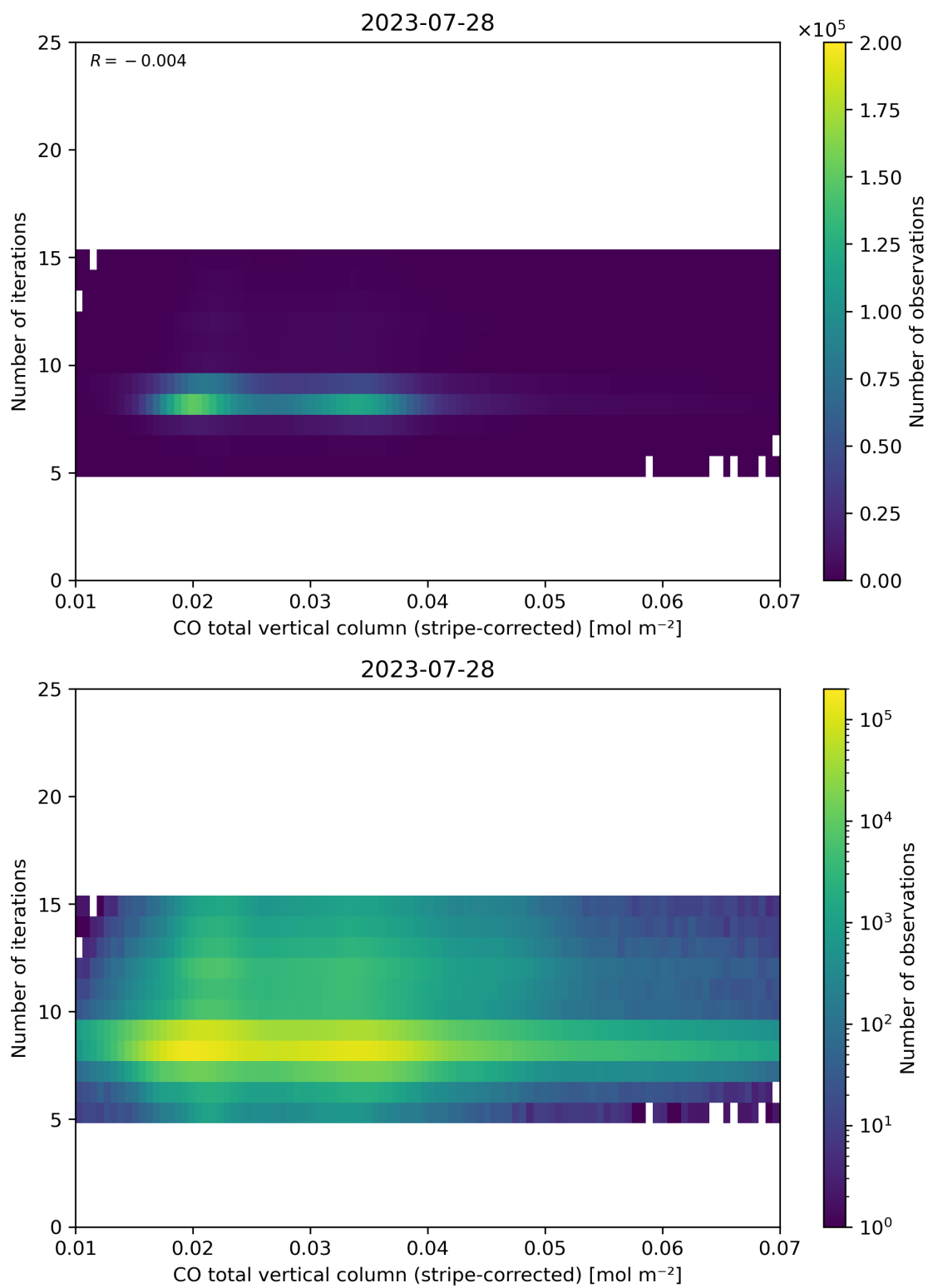
Figure 39: Scatter density plot of “CO total vertical column (stripe-corrected)” against “Number of iterations” for 2023-07-27 to 2023-07-29.
