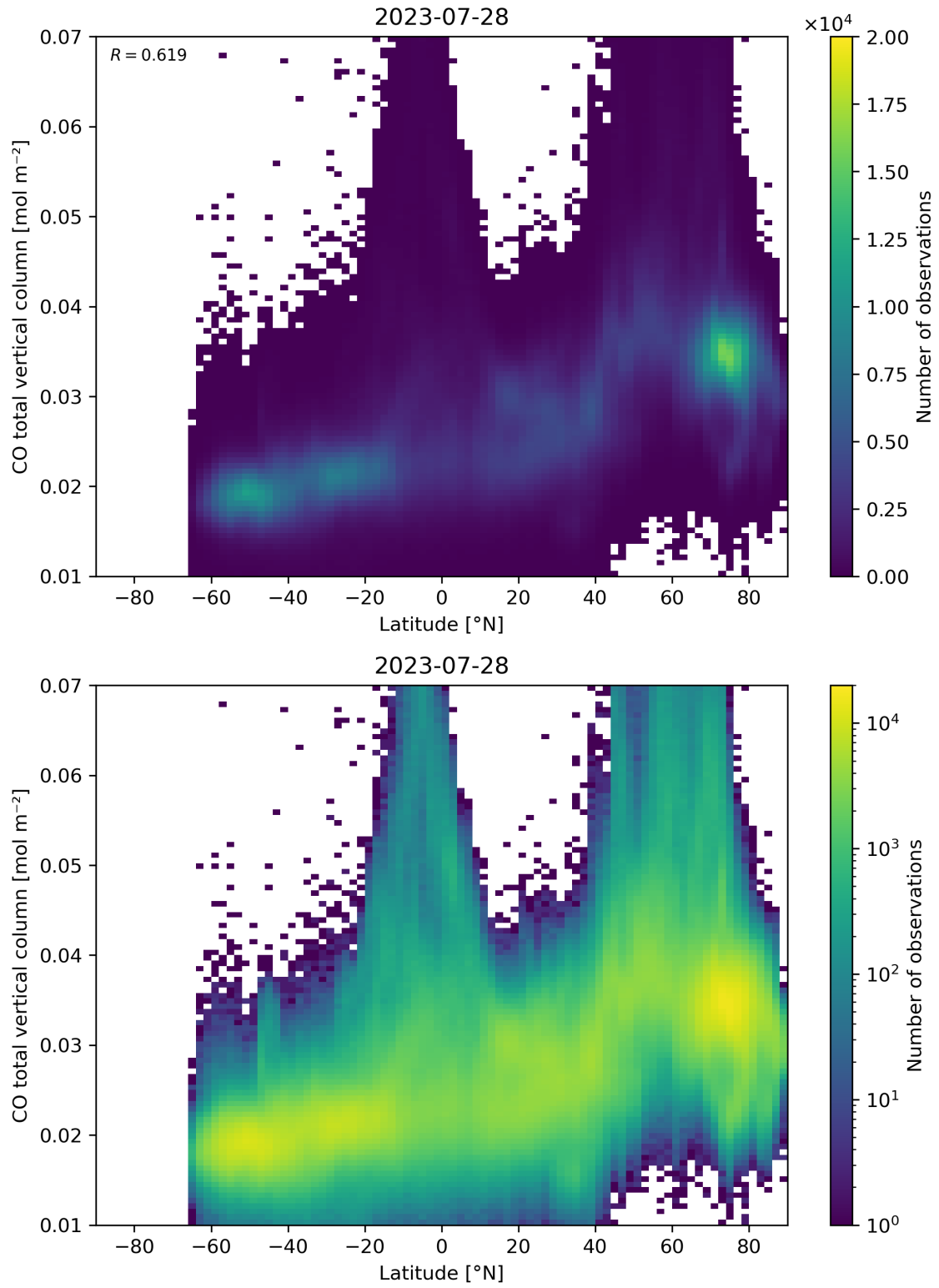
Figure 51: Scatter density plot of “Latitude” against “CO total vertical column” for 2023-07-27 to 2023-07-29.
