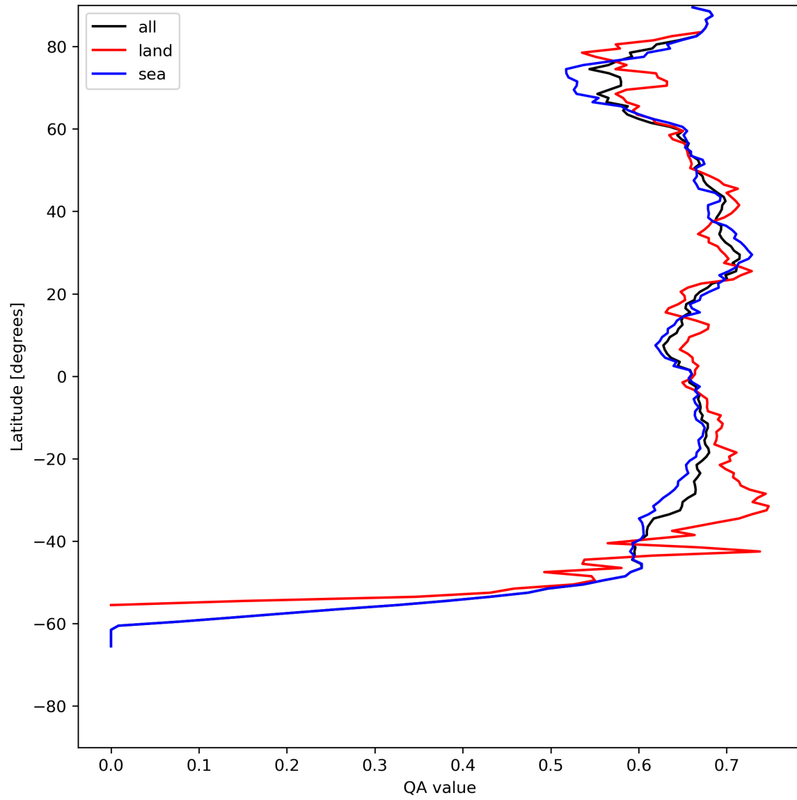
Figure 9: Zonal average of “QA value” for 2023-07-27 to 2023-07-29.
