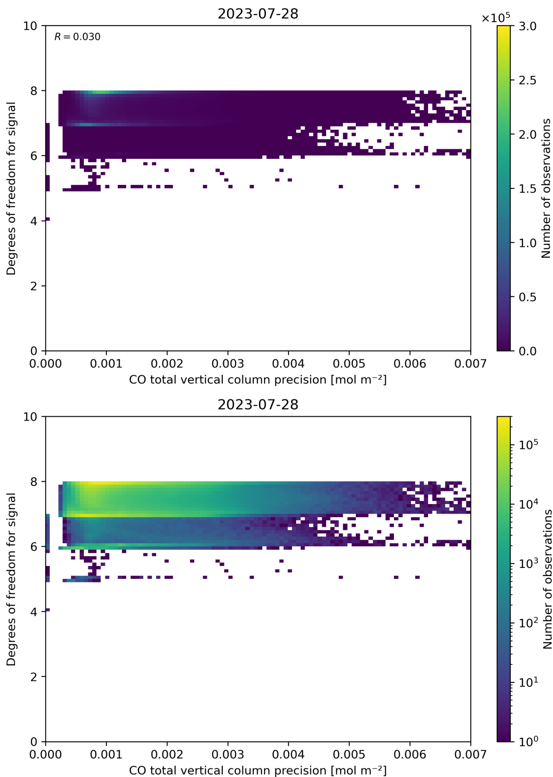
Figure 45: Scatter density plot of “CO total vertical column precision” against “Degrees of freedom for signal” for 2023-07-27 to 2023-07-29.
