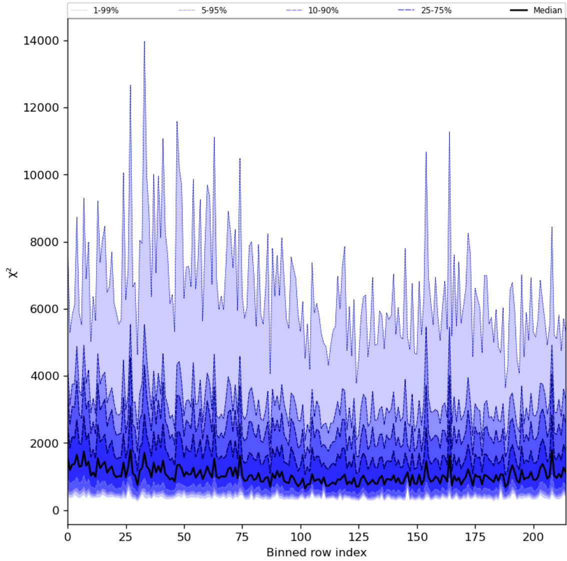
Figure 30: Along track statistics of “ \chi^2 ” for 2023-07-27 to 2023-07-29
