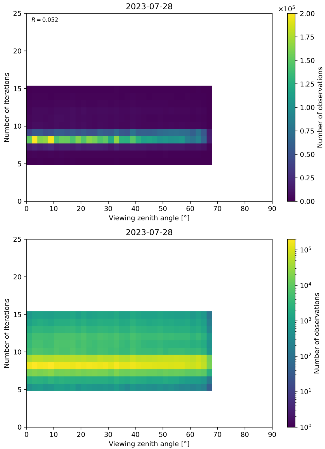
Figure 75: Scatter density plot of “Viewing zenith angle” against “Number of iterations” for 2023-07-27 to 2023-07-29.
