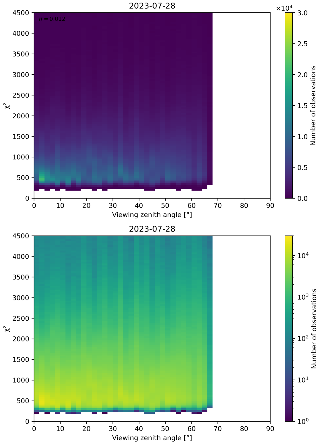
Figure 72: Scatter density plot of “Viewing zenith angle” against “ \chi^2 ” for 2023-07-27 to 2023-07-29.
