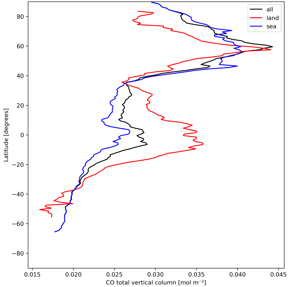
Figure 10: Zonal average of “CO total vertical column” for 2023-07-27 to 2023-07-29.
