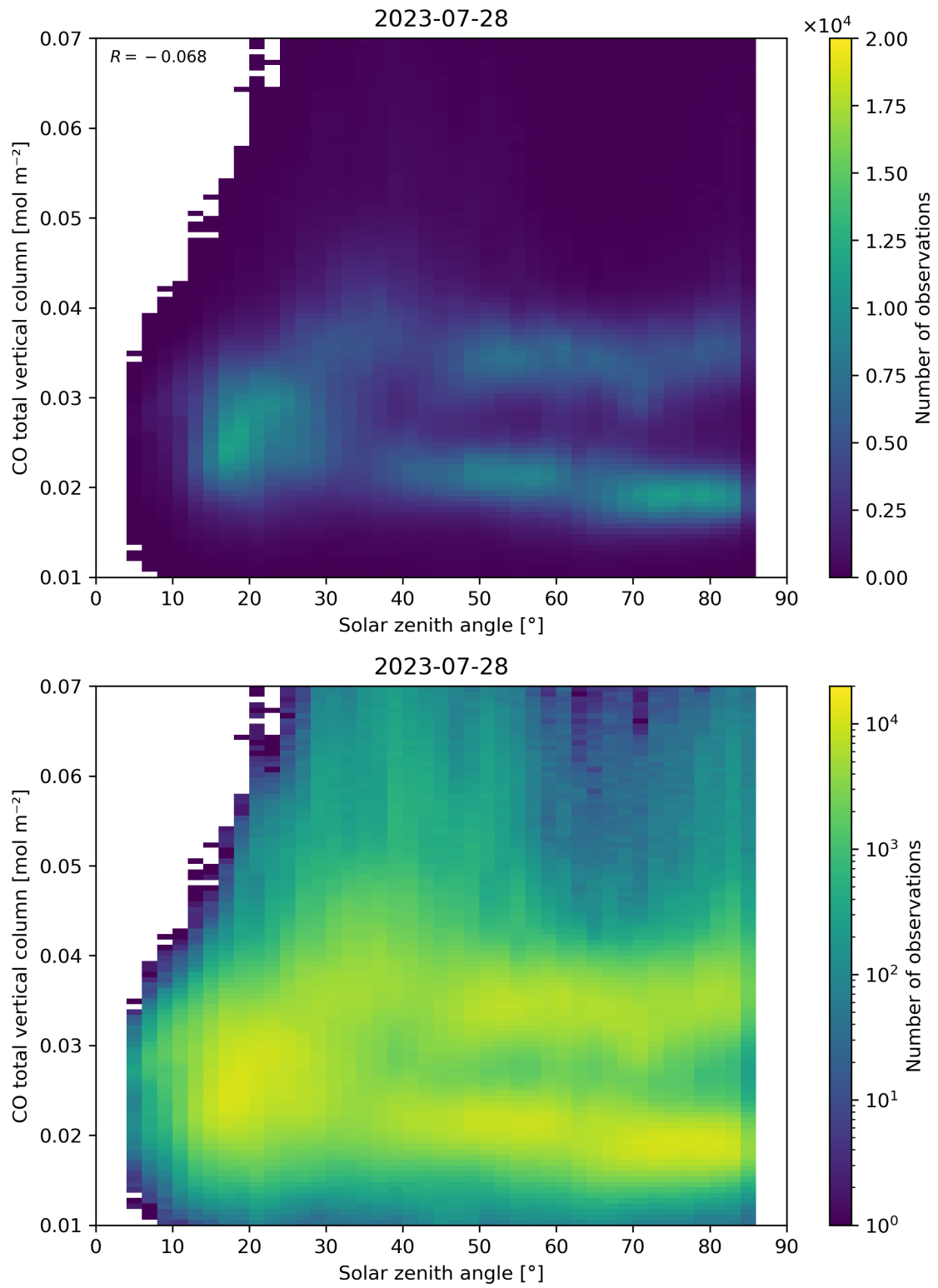
Figure 61: Scatter density plot of “Solar zenith angle” against “CO total vertical column” for 2023-07-27 to 2023-07-29.
