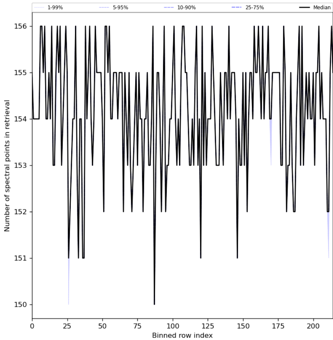
Figure 29: Along track statistics of “Number of spectral points in retrieval” for 2023-07-27 to 2023-07-29
