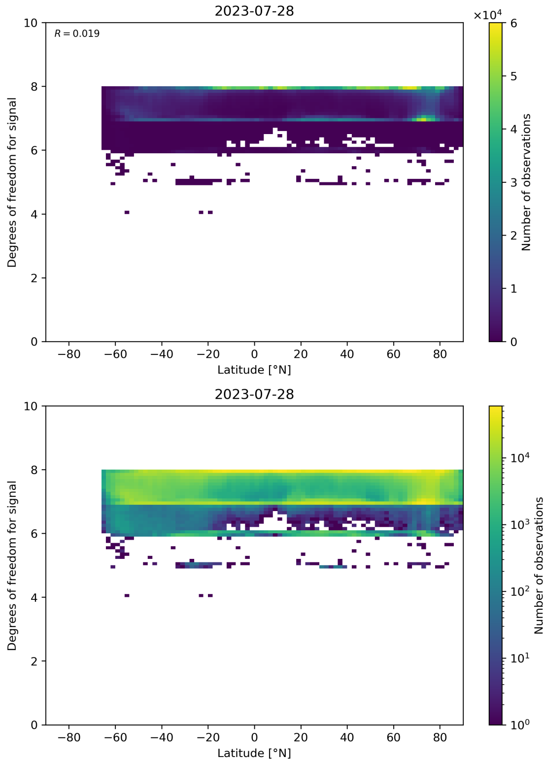
Figure 55: Scatter density plot of “Latitude” against “Degrees of freedom for signal” for 2023-07-27 to 2023-07-29.
