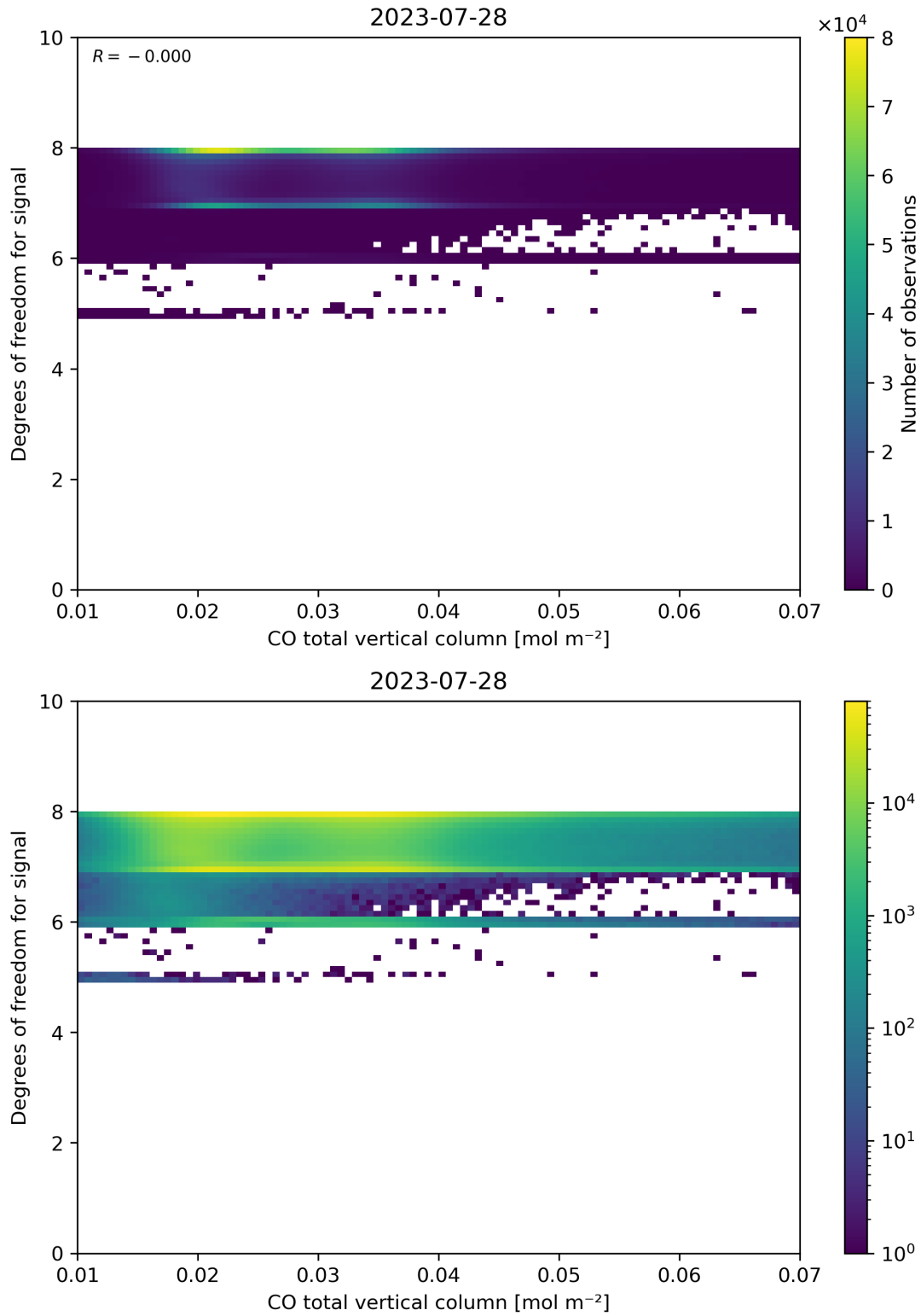
Figure 41: Scatter density plot of “CO total vertical column” against “Degrees of freedom for signal” for 2023-07-27 to 2023-07-29.
