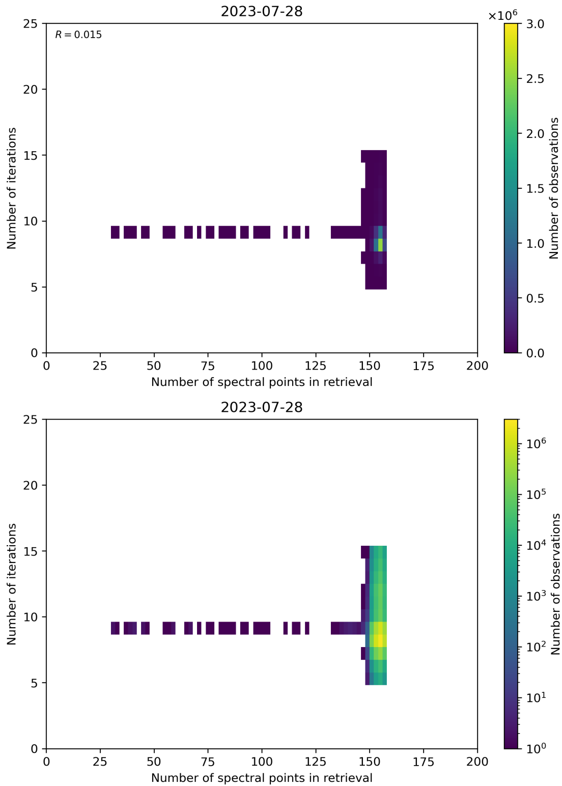
Figure 60: Scatter density plot of “Number of spectral points in retrieval” against “Number of iterations” for 2023-07-27 to 2023-07-29.
