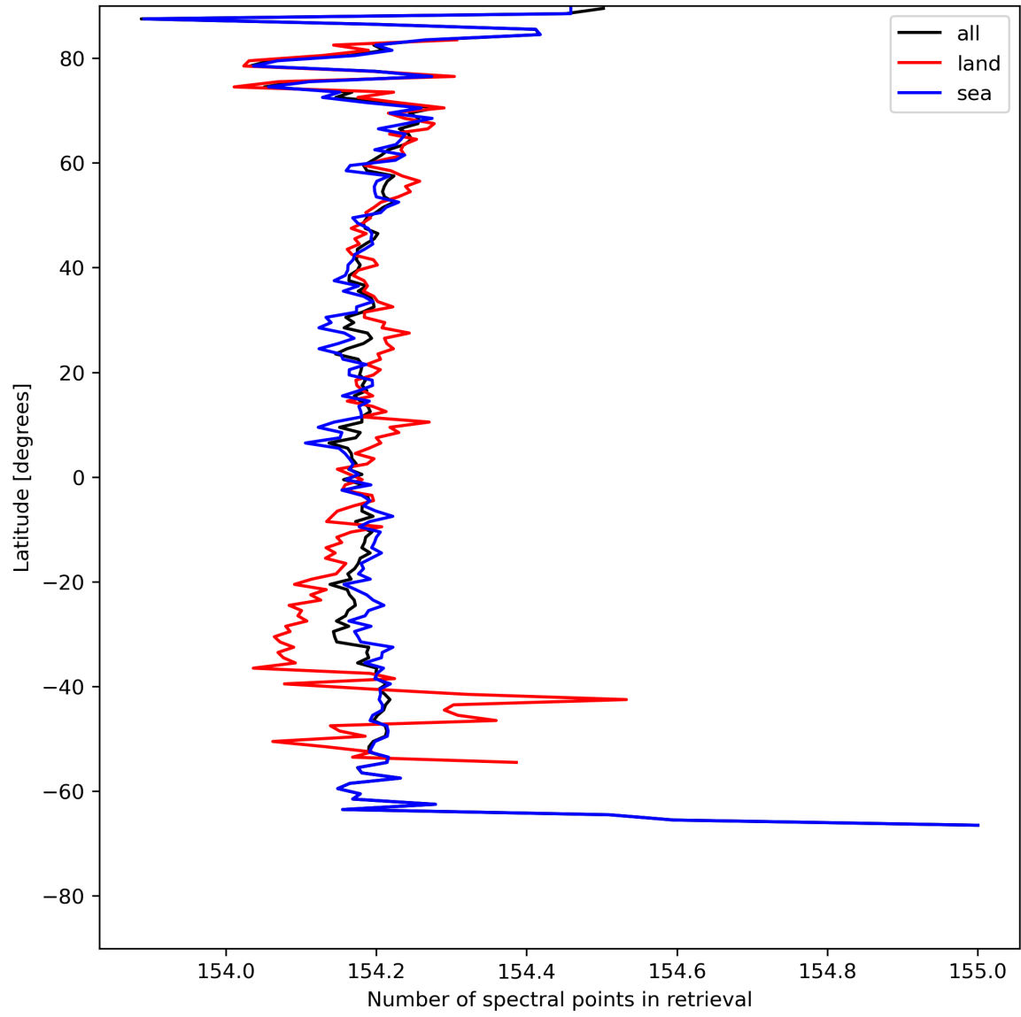
Figure 13: Zonal average of “Number of spectral points in retrieval” for 2023-07-29 to 2023-07-30.
