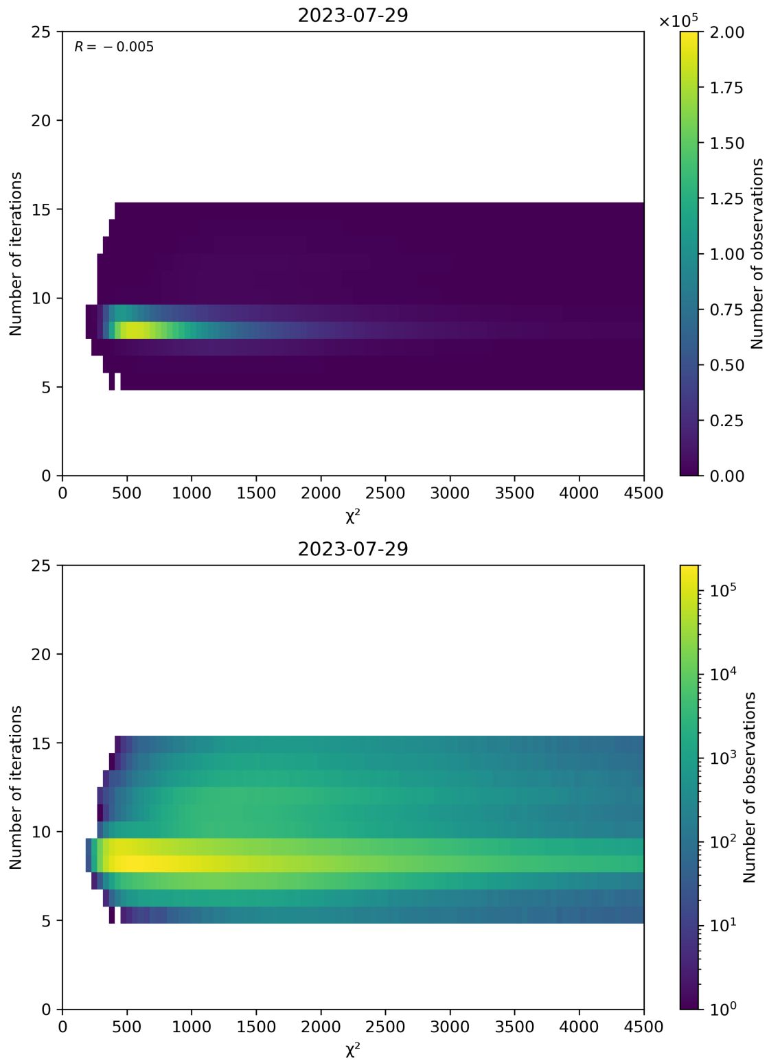
Figure 49: Scatter density plot of “ \chi^2 ” against “Number of iterations” for 2023-07-29 to 2023-07-30.
