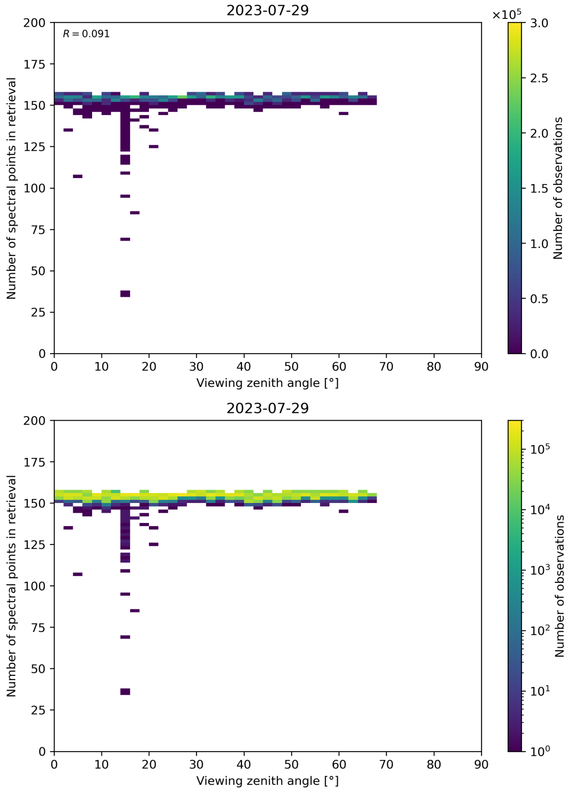
Figure 76: Scatter density plot of “Viewing zenith angle” against “Number of spectral points in retrieval” for 2023-07-29 to 2023-07-30.
