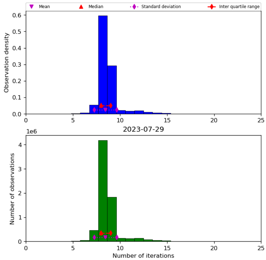
Figure 24: Histogram of “Number of iterations” for 2023-07-29 to 2023-07-30
