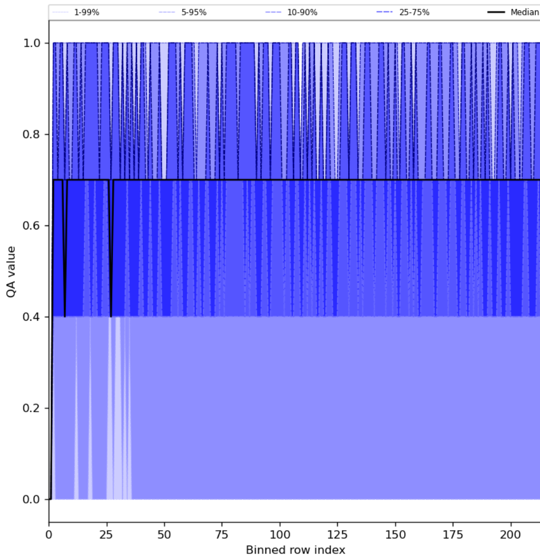
Figure 25: Along track statistics of “QA value” for 2023-07-29 to 2023-07-30
