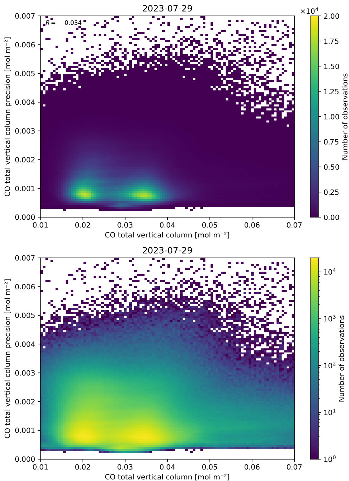
Figure 34: Scatter density plot of “CO total vertical column” against “CO total vertical column precision” for 2023-07-29 to 2023-07-30.
