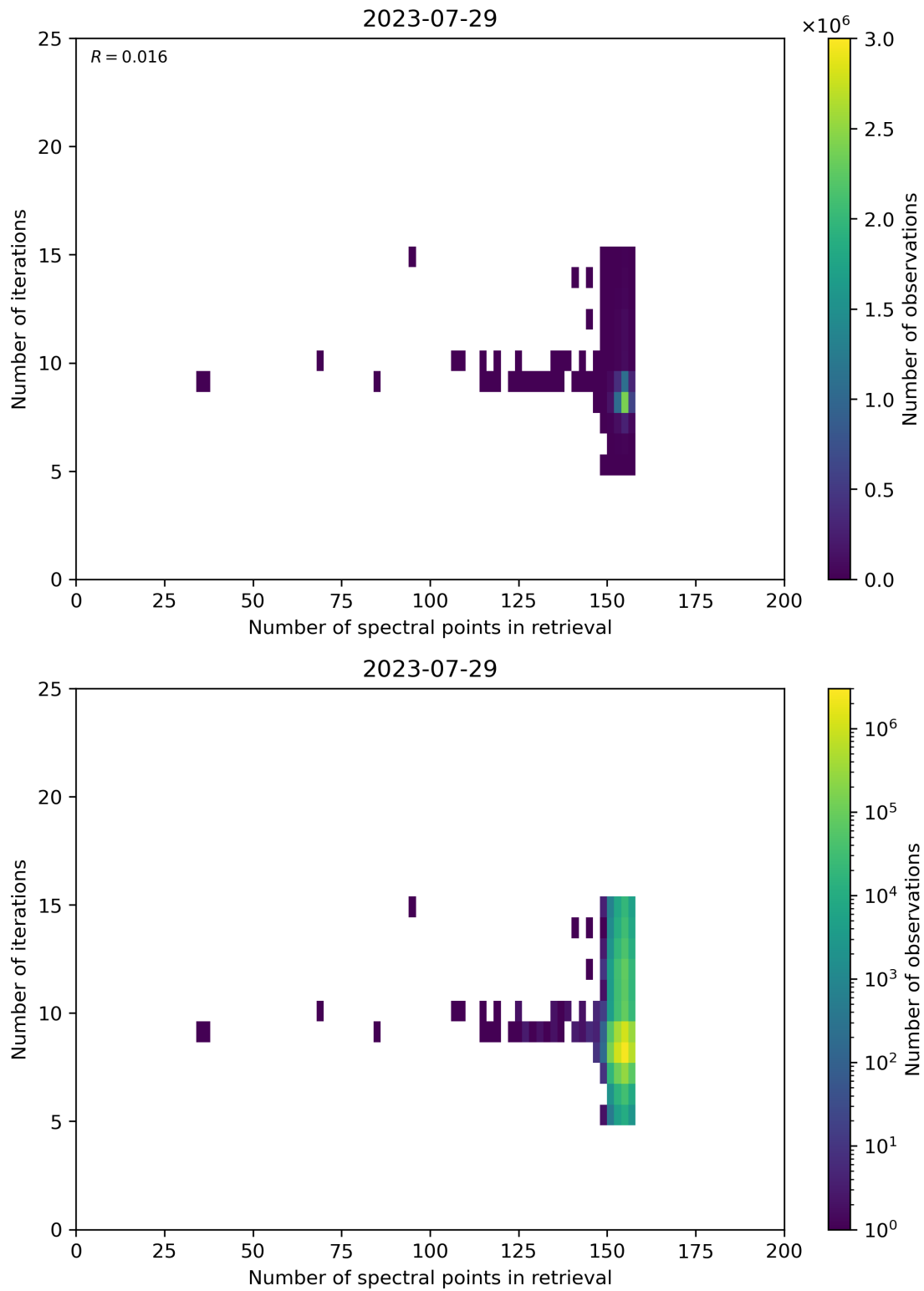
Figure 60: Scatter density plot of “Number of spectral points in retrieval” against “Number of iterations” for 2023-07-29 to 2023-07-30.
