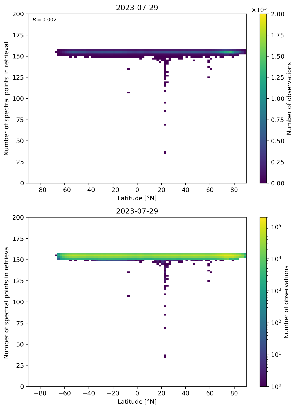
Figure 57: Scatter density plot of “Latitude” against “Number of spectral points in retrieval” for 2023-07-29 to 2023-07-30.
