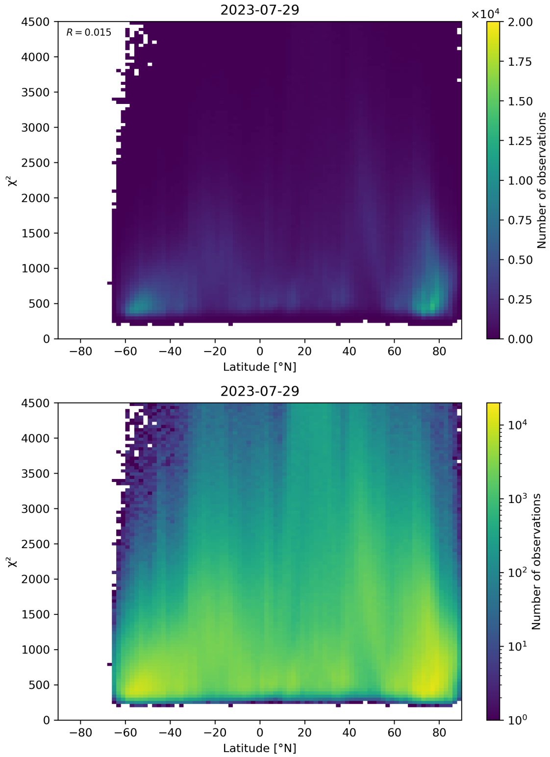
Figure 54: Scatter density plot of “Latitude” against “ \chi^2 ” for 2023-07-29 to 2023-07-30.
