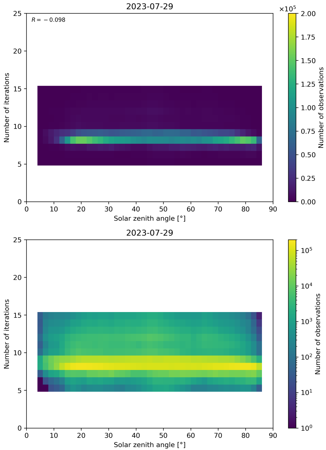
Figure 67: Scatter density plot of “Solar zenith angle” against “Number of iterations” for 2023-07-29 to 2023-07-30.
