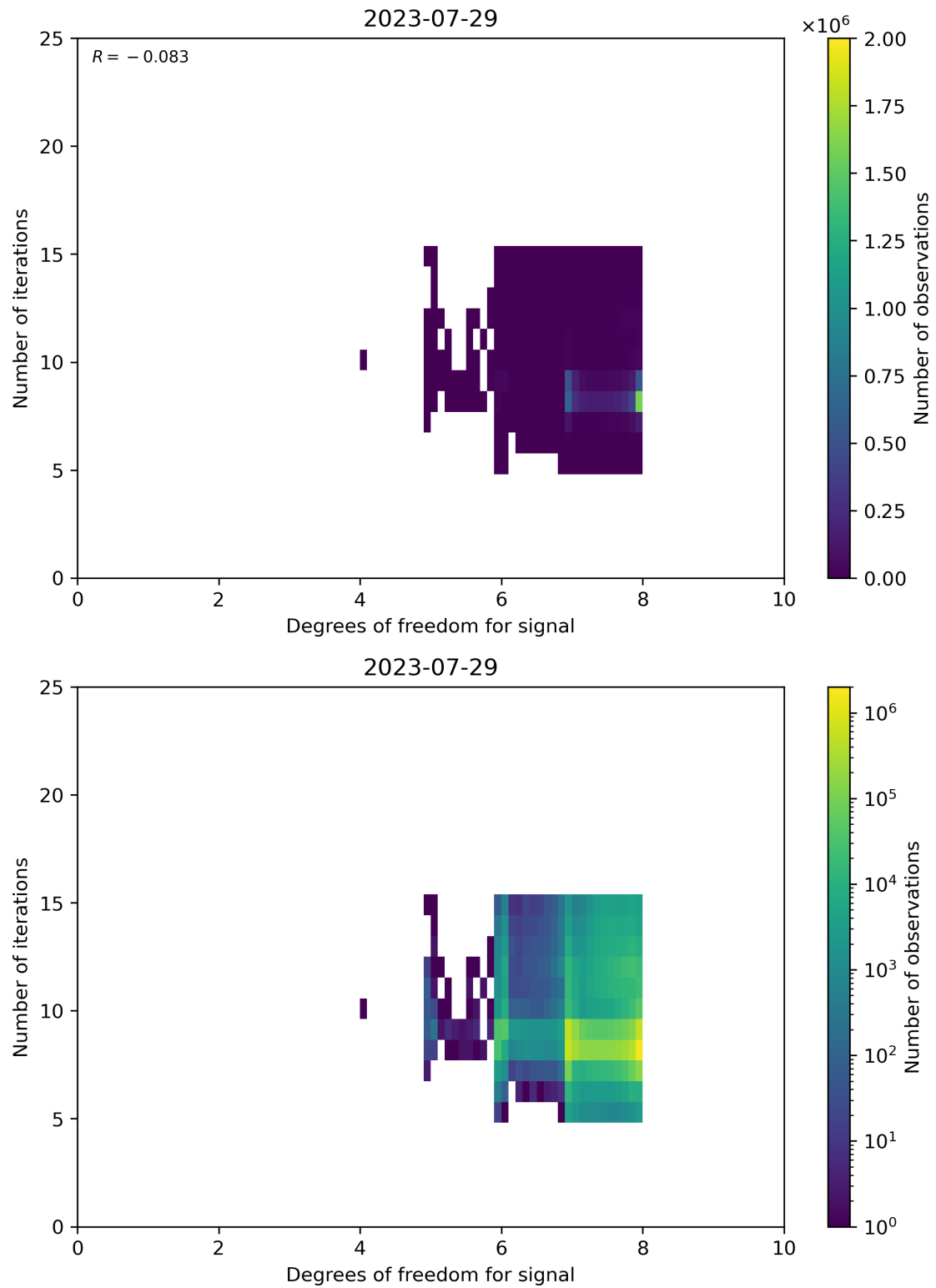
Figure 50: Scatter density plot of “Degrees of freedom for signal” against “Number of iterations” for 2023-07-29 to 2023-07-30.
