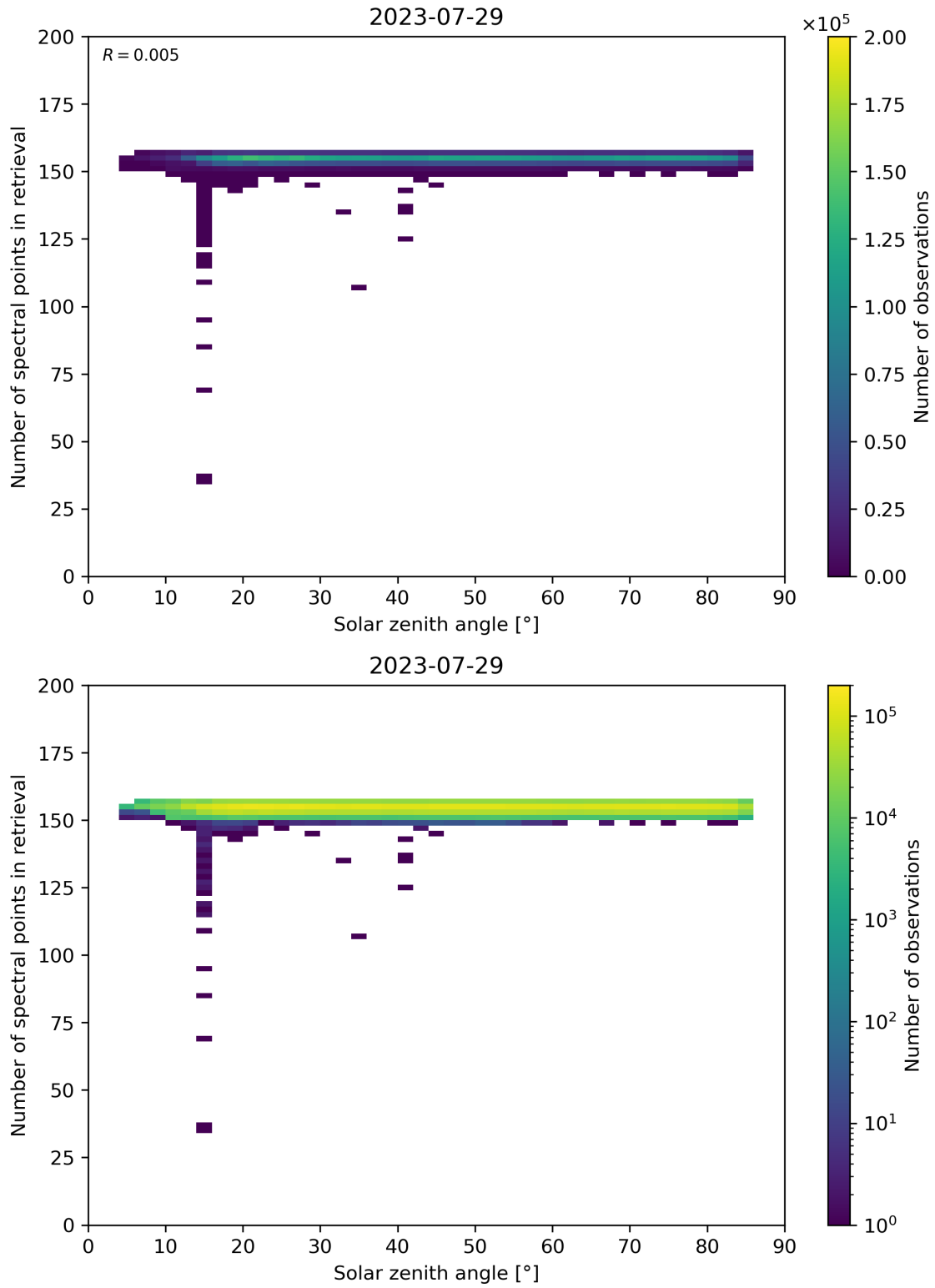
Figure 68: Scatter density plot of “Solar zenith angle” against “Number of spectral points in retrieval” for 2023-07-29 to 2023-07-30.
