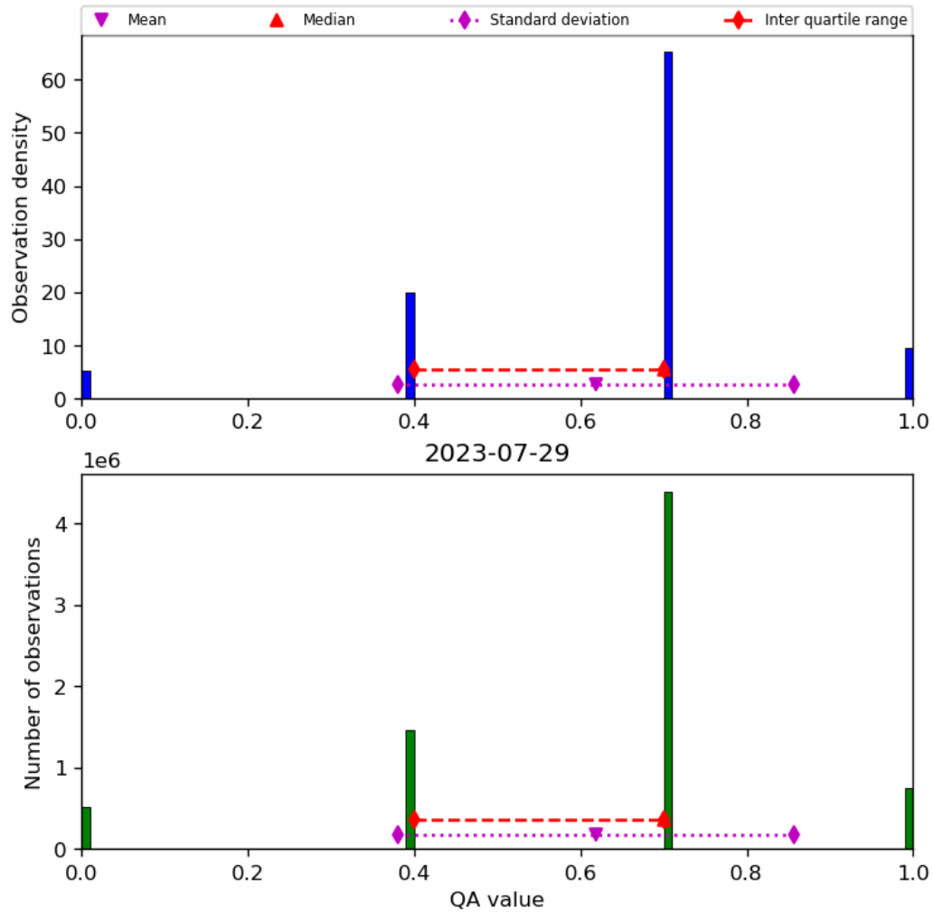
Figure 17: Histogram of “QA value” for 2023-07-29 to 2023-07-30
