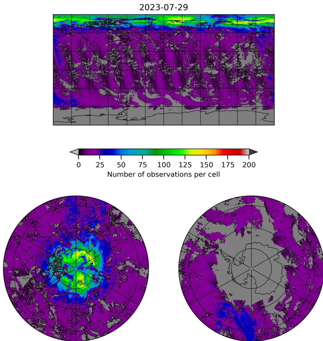
Figure 8: Map of the number of observations for 2023-07-29 to 2023-07-30
