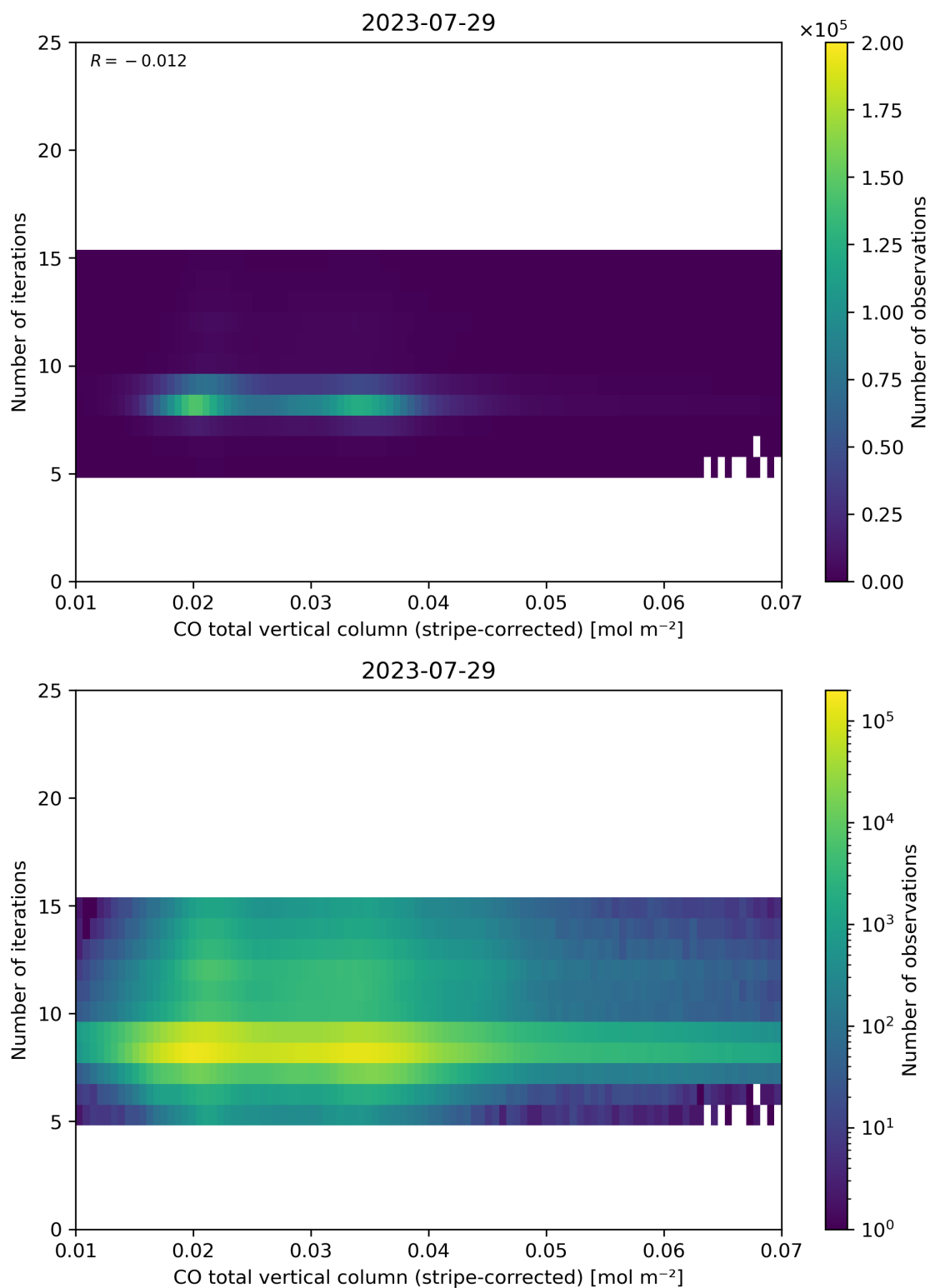
Figure 39: Scatter density plot of “CO total vertical column (stripe-corrected)” against “Number of iterations” for 2023-07-29 to 2023-07-30.
