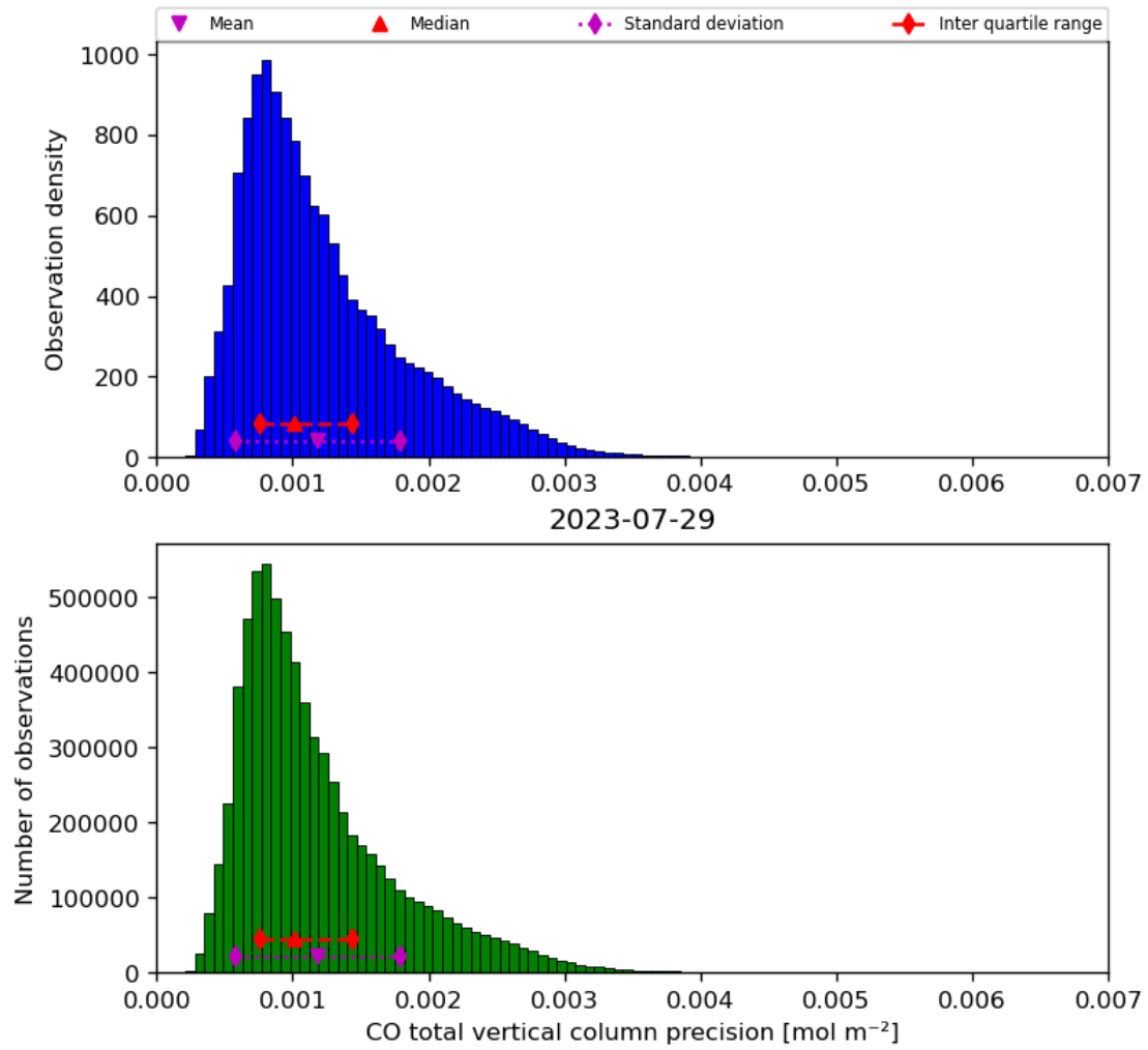
Figure 20: Histogram of “CO total vertical column precision” for 2023-07-29 to 2023-07-30
