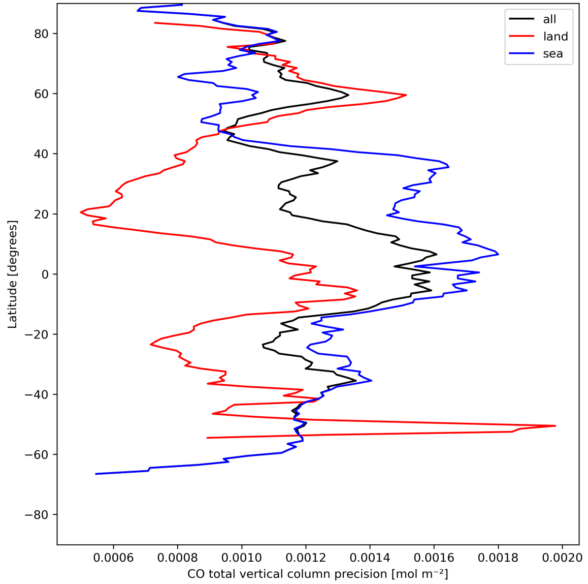
Figure 12: Zonal average of “CO total vertical column precision” for 2023-07-29 to 2023-07-30.
