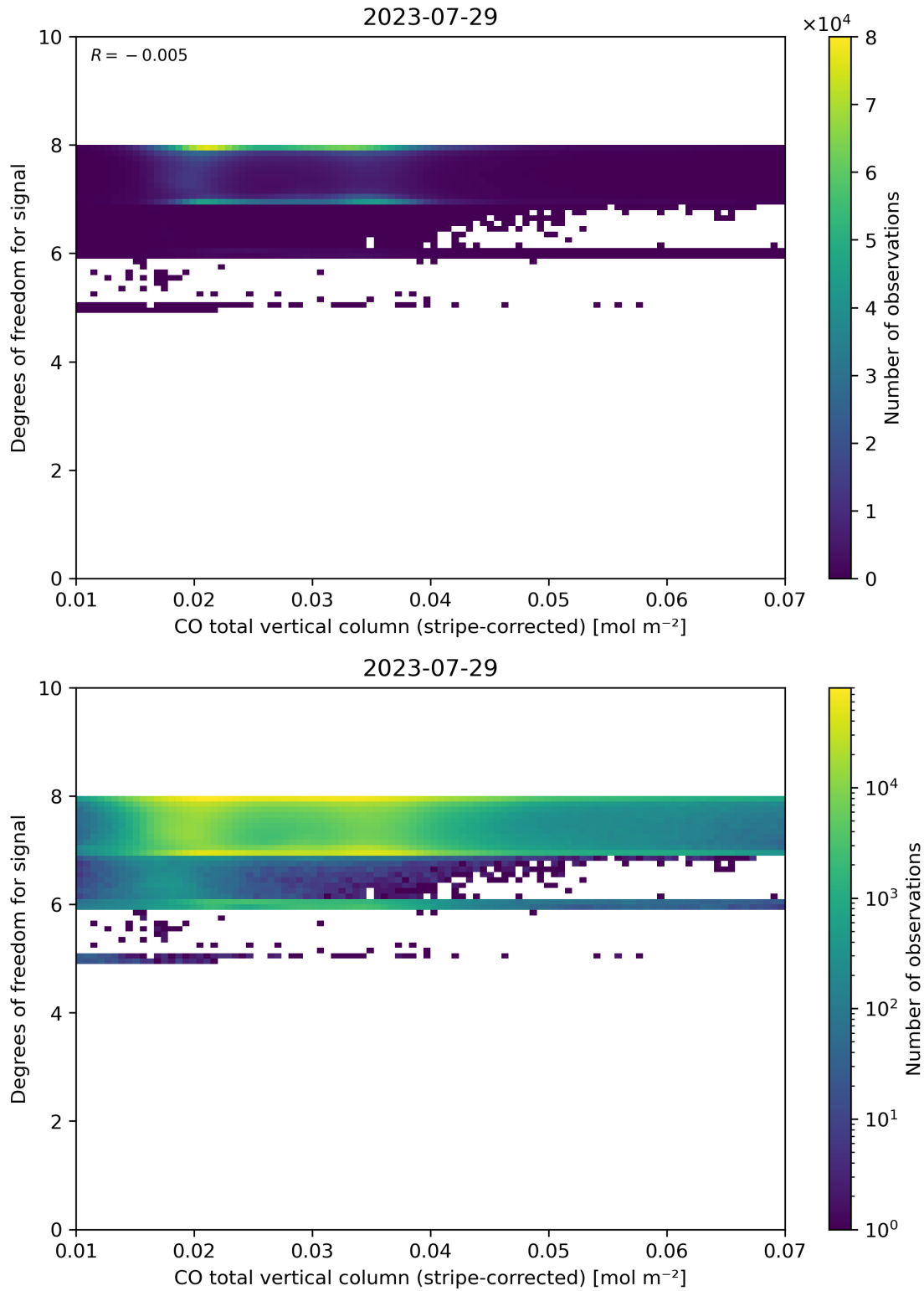
Figure 38: Scatter density plot of “CO total vertical column (stripe-corrected)” against “Degrees of freedom for signal” for 2023-07-29 to 2023-07-30.
