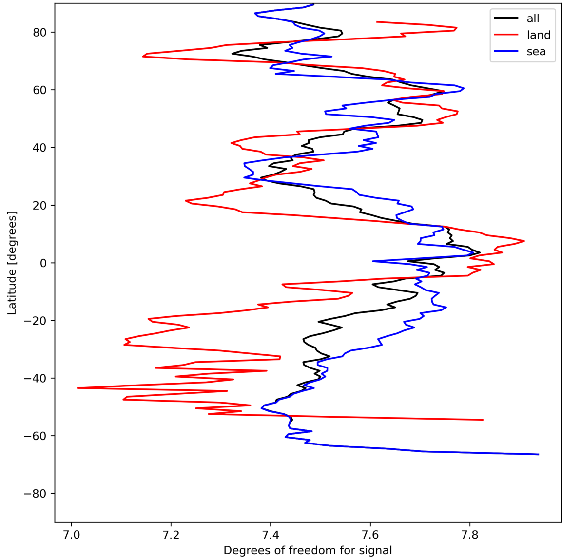
Figure 15: Zonal average of “Degrees of freedom for signal” for 2023-07-29 to 2023-07-30.
