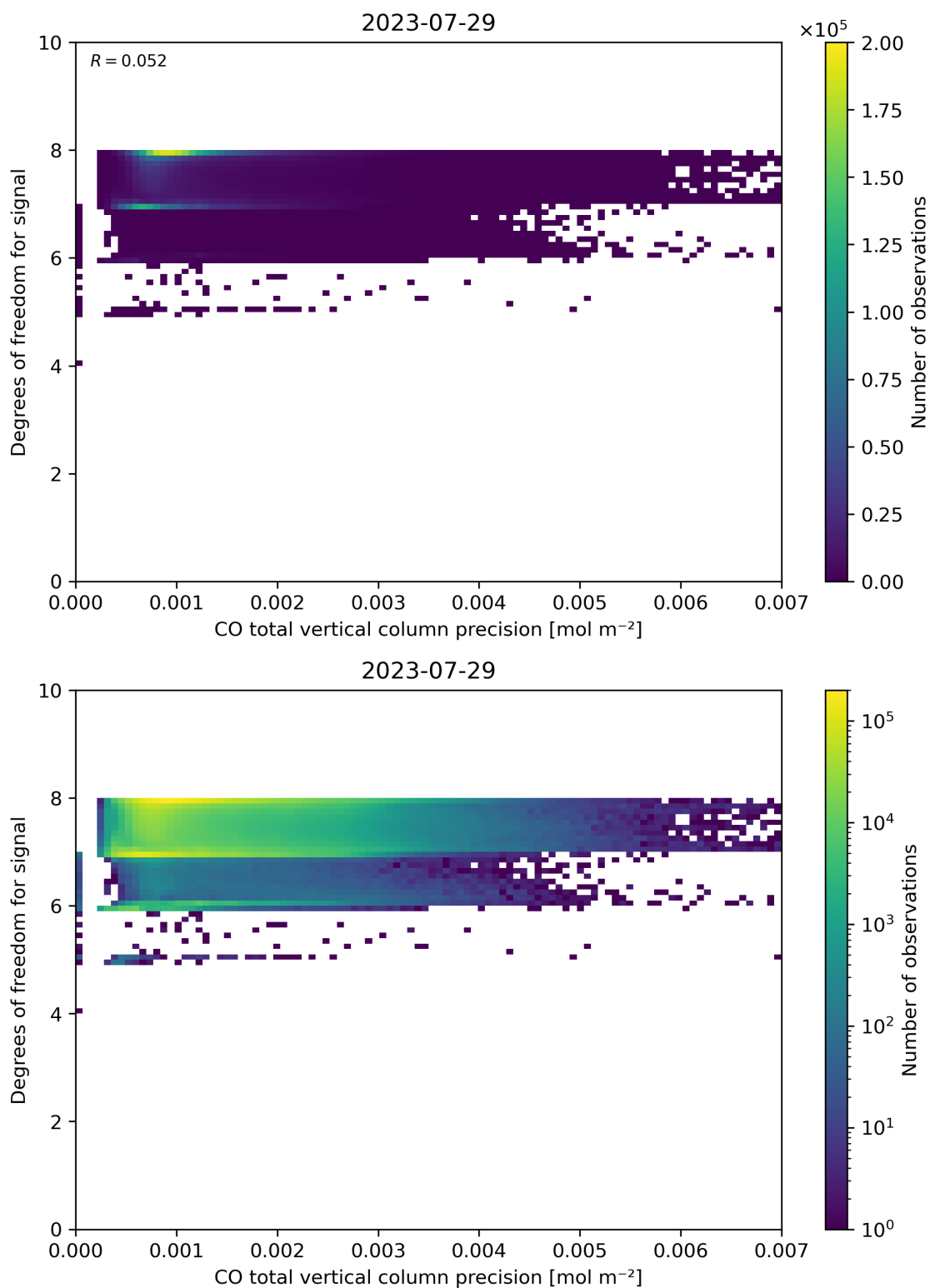
Figure 45: Scatter density plot of “CO total vertical column precision” against “Degrees of freedom for signal” for 2023-07-29 to 2023-07-30.
