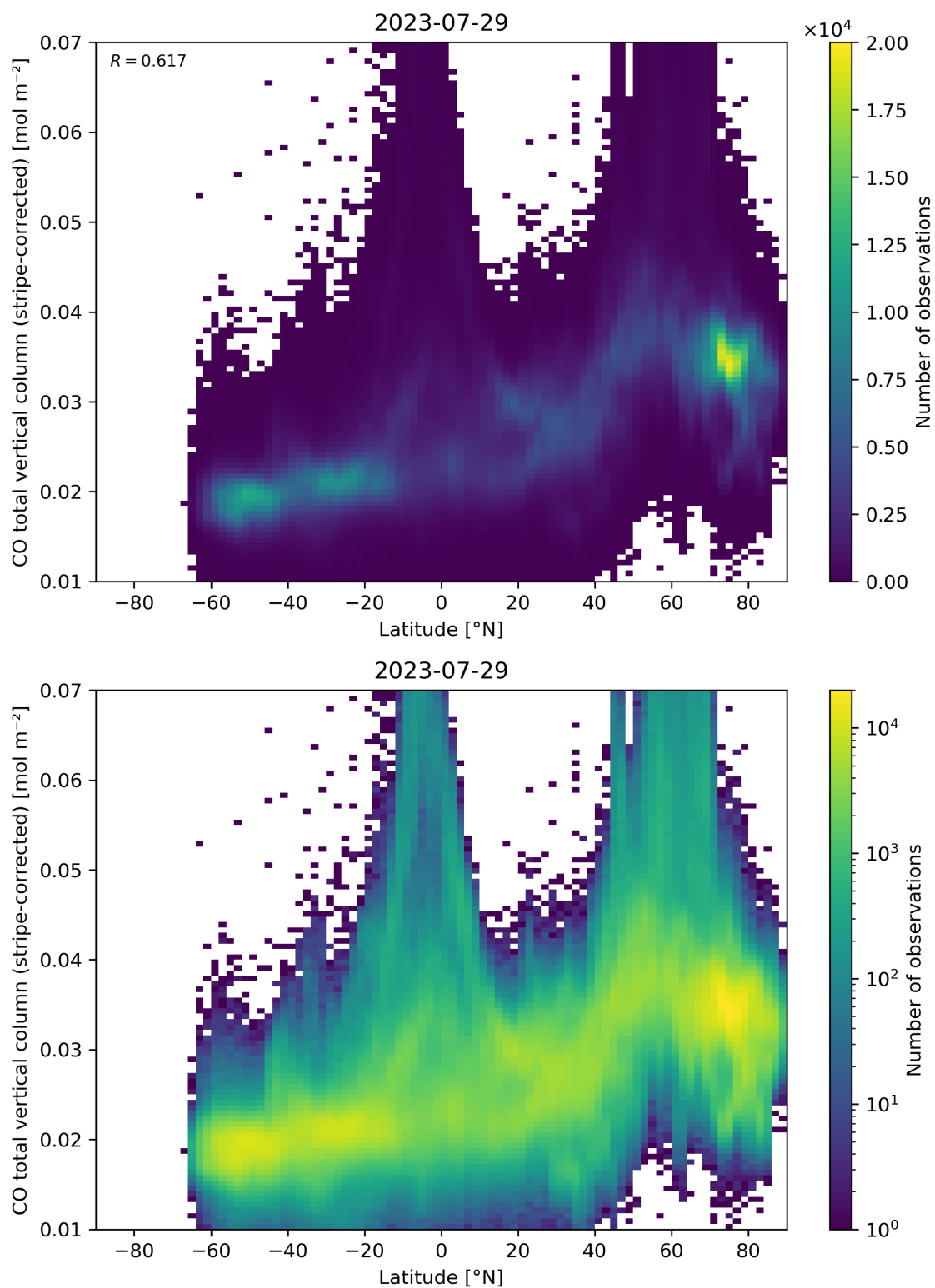
Figure 52: Scatter density plot of “Latitude” against “CO total vertical column (stripe-corrected)” for 2023-07-29 to 2023-07-30.
