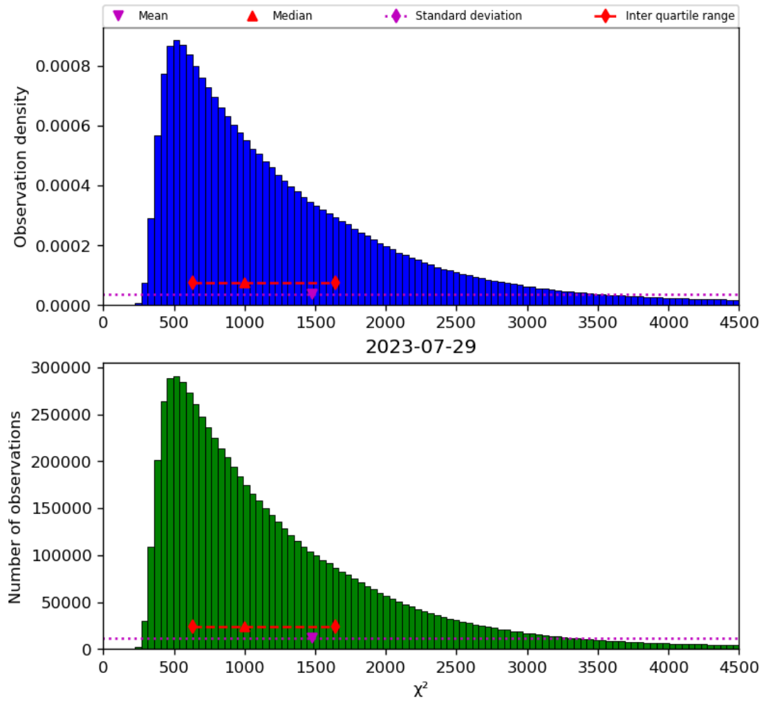
Figure 22: Histogram of “ \chi^2 ” for 2023-07-29 to 2023-07-30
