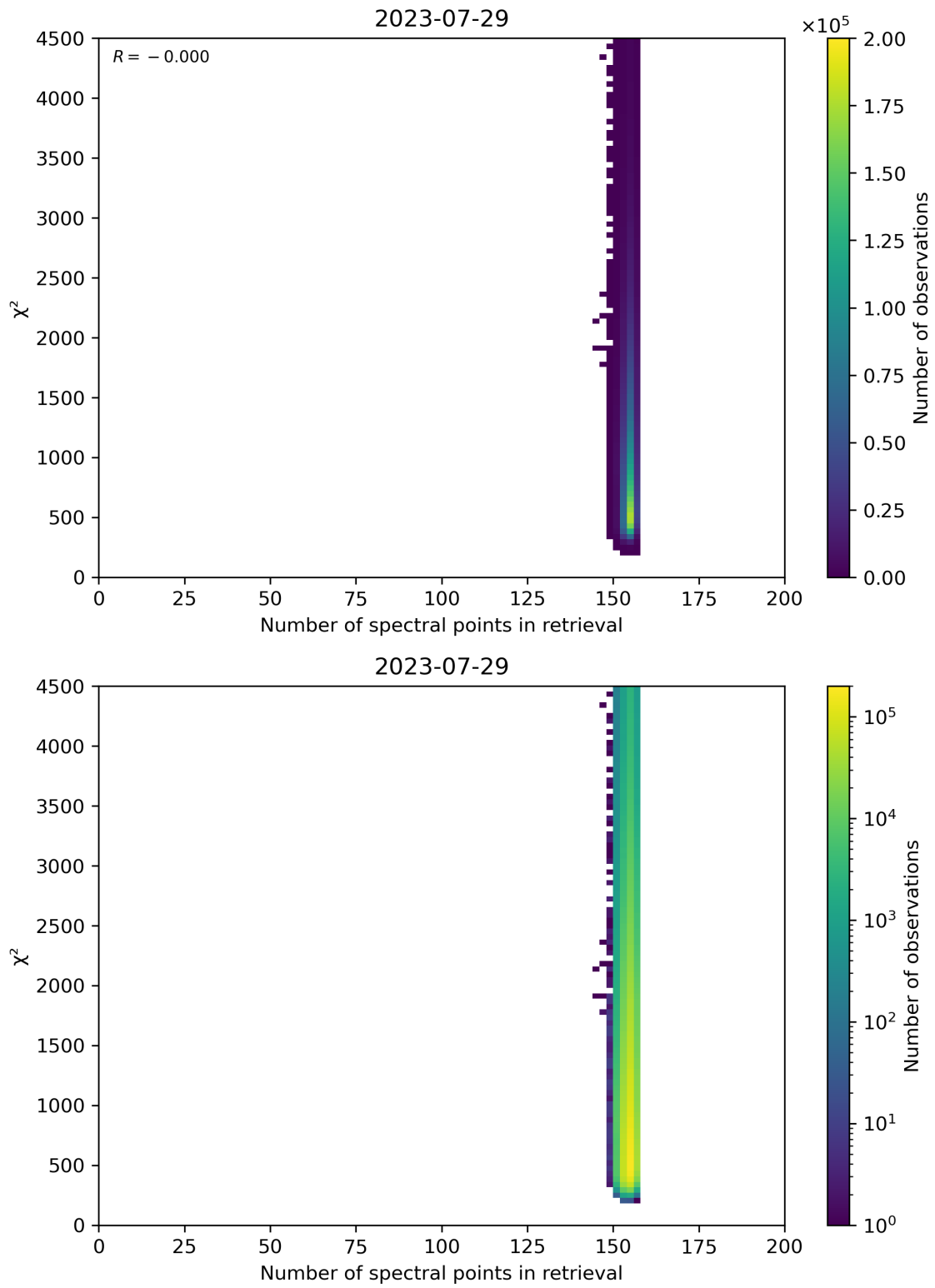
Figure 58: Scatter density plot of “Number of spectral points in retrieval” against “ \chi^2 ” for 2023-07-29 to 2023-07-30.
