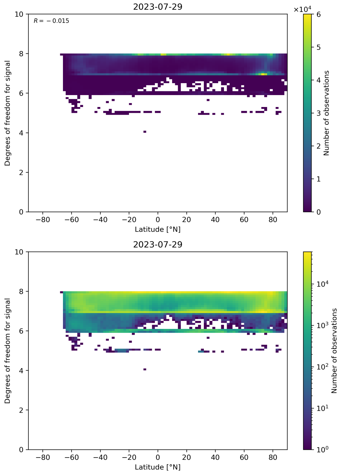
Figure 55: Scatter density plot of “Latitude” against “Degrees of freedom for signal” for 2023-07-29 to 2023-07-30.
