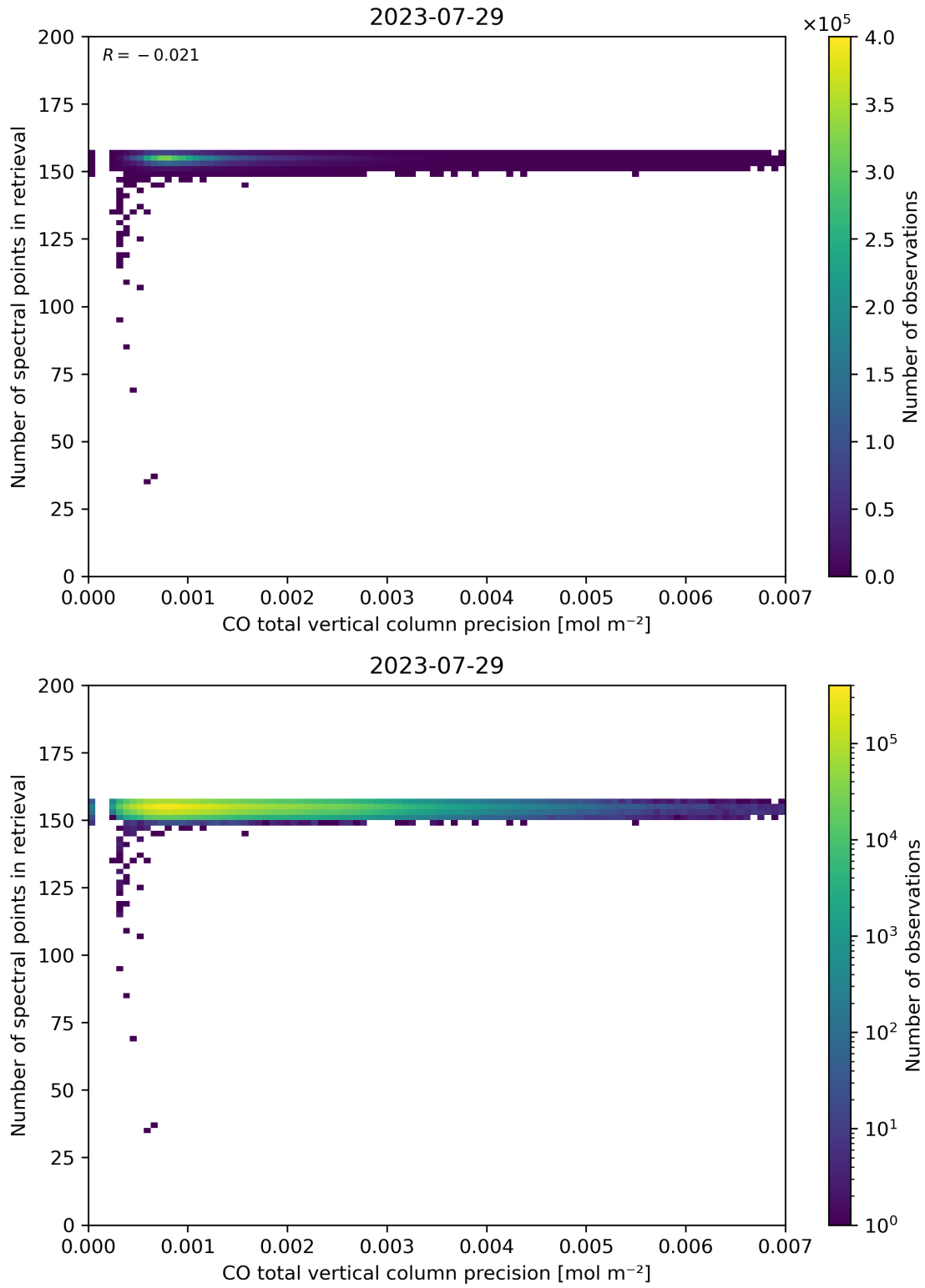
Figure 47: Scatter density plot of “CO total vertical column precision” against “Number of spectral points in retrieval” for 2023-07-29 to 2023-07-30.
