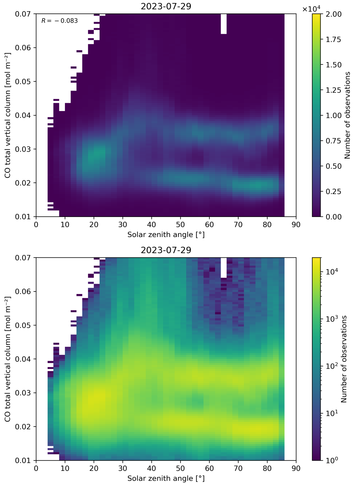
Figure 61: Scatter density plot of “Solar zenith angle” against “CO total vertical column” for 2023-07-29 to 2023-07-30.
