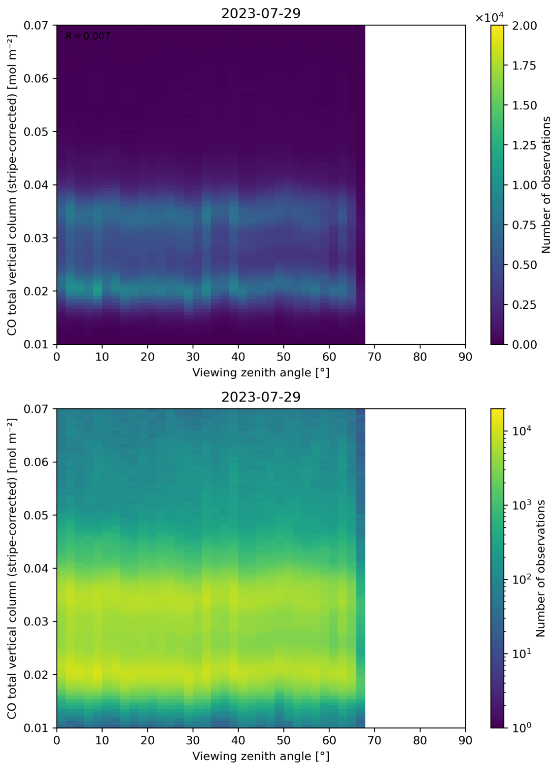
Figure 70: Scatter density plot of “Viewing zenith angle” against “CO total vertical column (stripe-corrected)” for 2023-07-29 to 2023-07-30.
