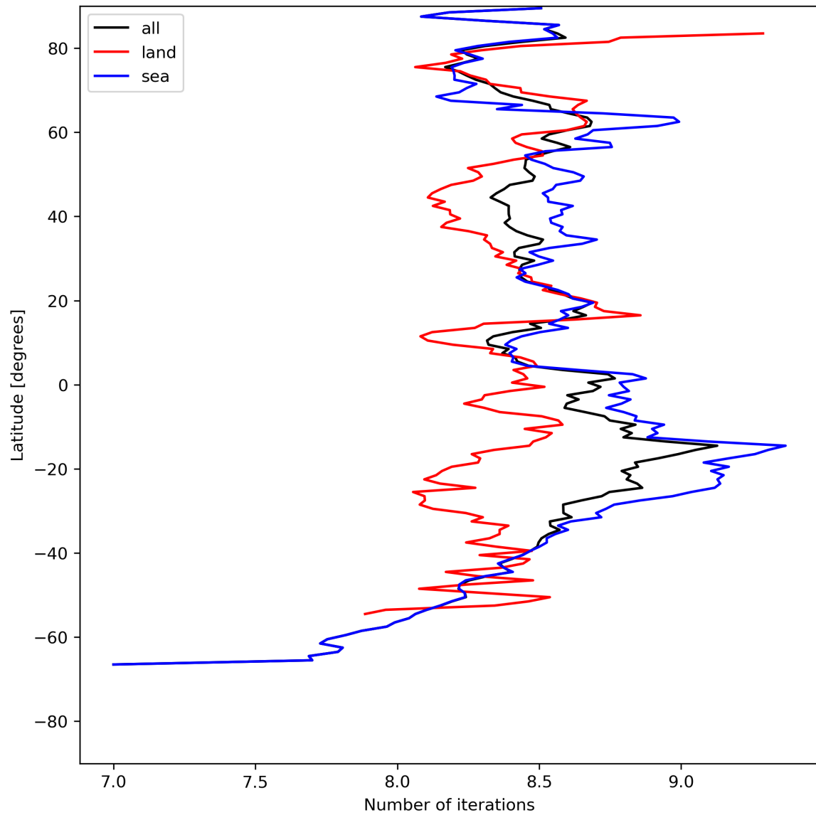
Figure 16: Zonal average of “Number of iterations” for 2023-07-29 to 2023-07-30.
