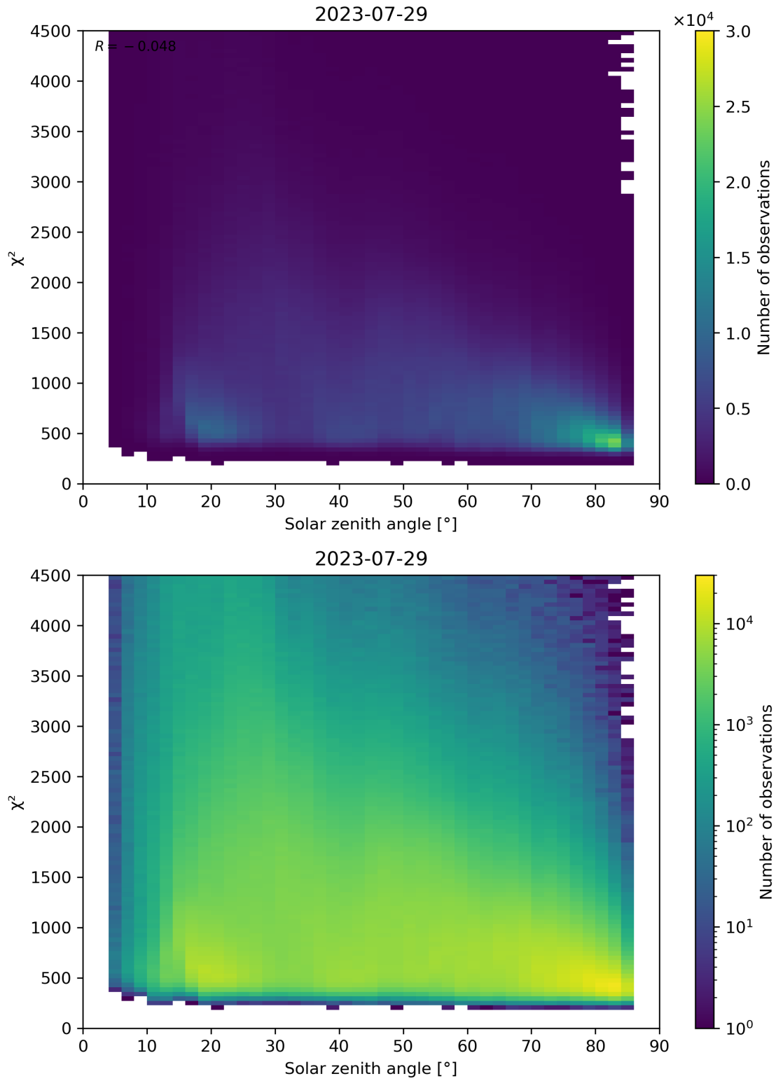
Figure 64: Scatter density plot of “Solar zenith angle” against “ \chi^2 ” for 2023-07-29 to 2023-07-30.
