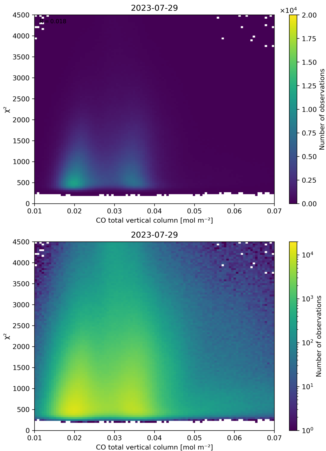
Figure 35: Scatter density plot of “CO total vertical column” against “ \chi^2 ” for 2023-07-29 to 2023-07-30.
