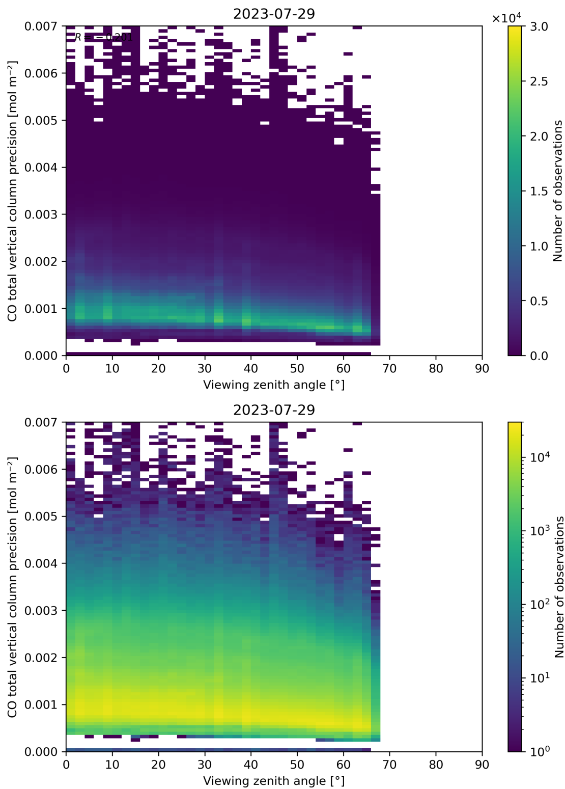
Figure 71: Scatter density plot of “Viewing zenith angle” against “CO total vertical column precision” for 2023-07-29 to 2023-07-30.
