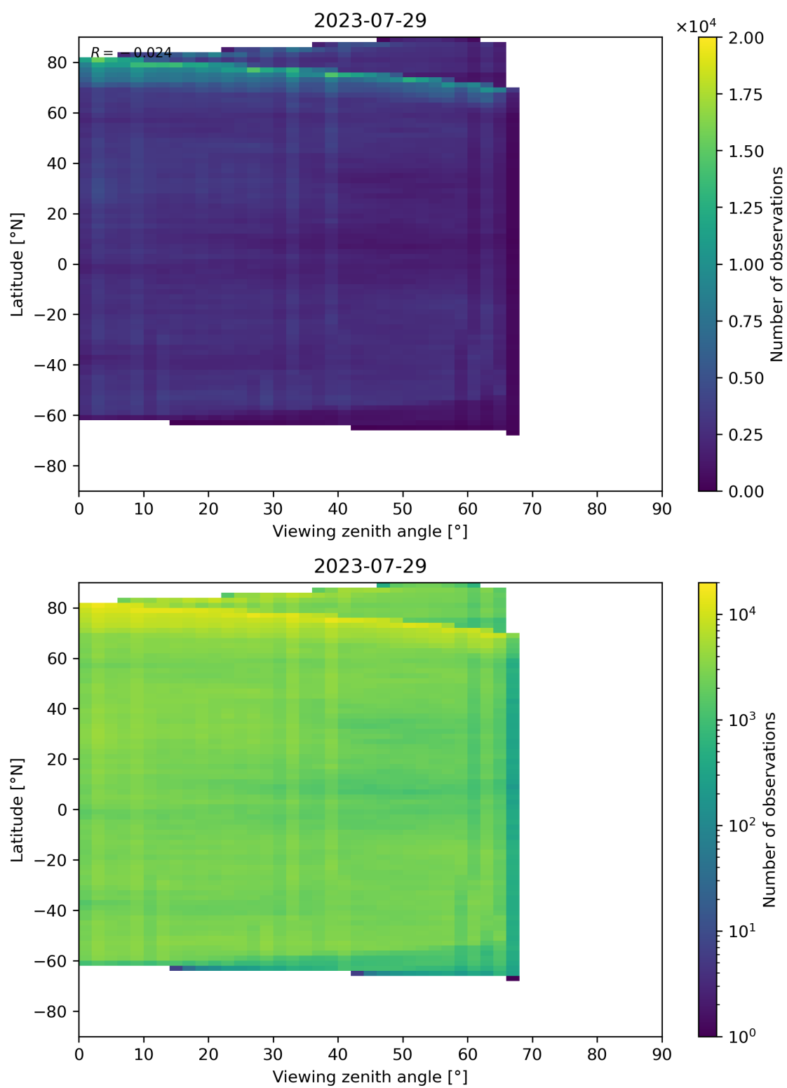
Figure 74: Scatter density plot of “Viewing zenith angle” against “Latitude” for 2023-07-29 to 2023-07-30.
