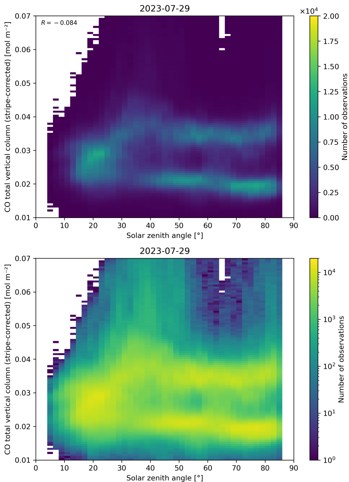
Figure 62: Scatter density plot of “Solar zenith angle” against “CO total vertical column (stripe-corrected)” for 2023-07-29 to 2023-07-30.
