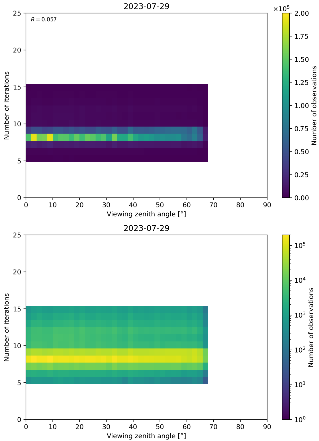
Figure 75: Scatter density plot of “Viewing zenith angle” against “Number of iterations” for 2023-07-29 to 2023-07-30.
