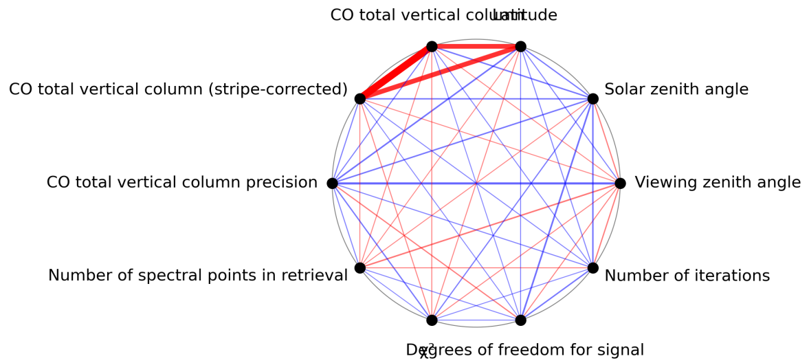
Figure 1: Map of correlation graph for 2023-07-29 to 2023-07-30.
