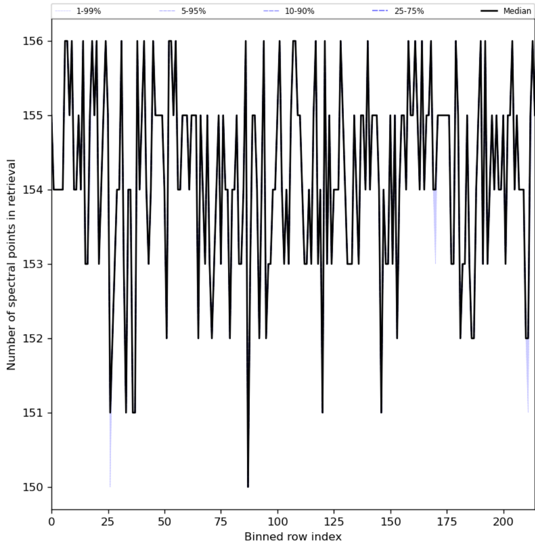
Figure 29: Along track statistics of “Number of spectral points in retrieval” for 2023-07-29 to 2023-07-30
