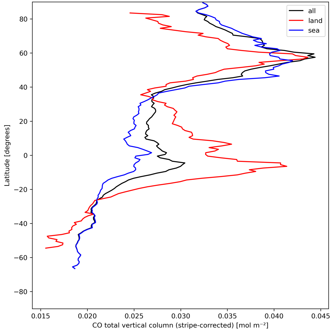
Figure 11: Zonal average of “CO total vertical column (stripe-corrected)” for 2023-07-29 to 2023-07-30.
