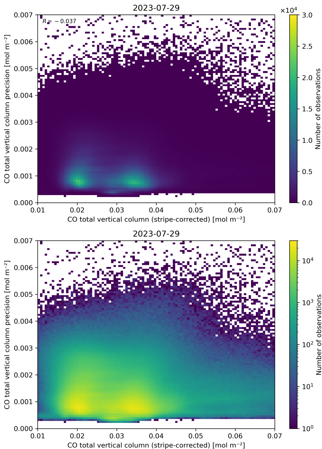
Figure 36: Scatter density plot of “CO total vertical column (stripe-corrected)” against “CO total vertical column precision” for 2023-07-29 to 2023-07-30.
