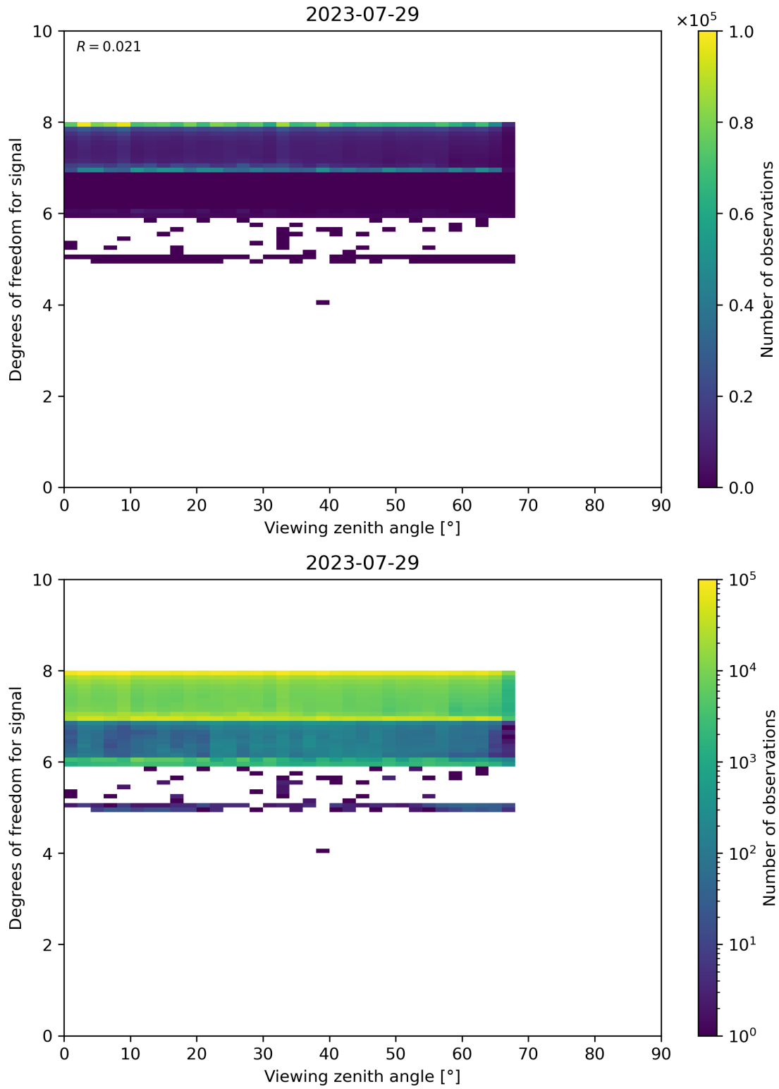
Figure 73: Scatter density plot of “Viewing zenith angle” against “Degrees of freedom for signal” for 2023-07-29 to 2023-07-30.
