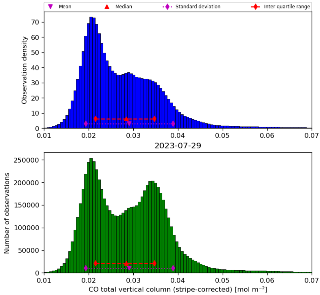
Figure 19: Histogram of “CO total vertical column (stripe-corrected)” for 2023-07-29 to 2023-07-30
