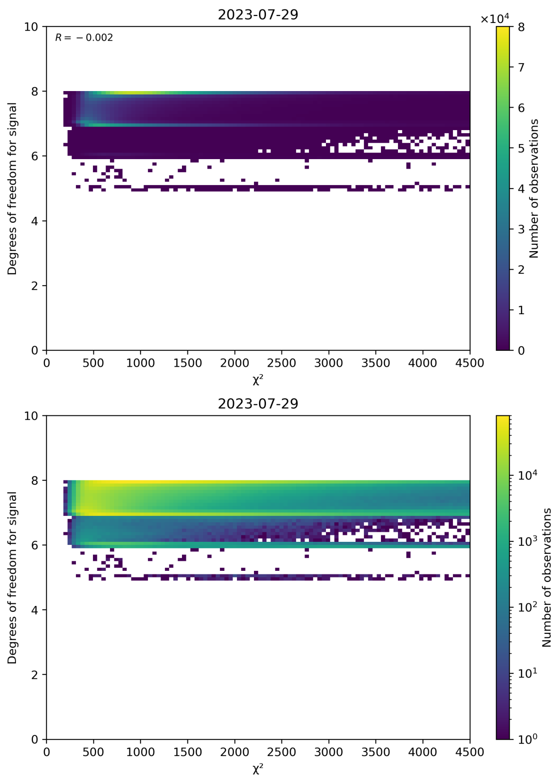
Figure 48: Scatter density plot of “ \chi^2 ” against “Degrees of freedom for signal” for 2023-07-29 to 2023-07-30.
