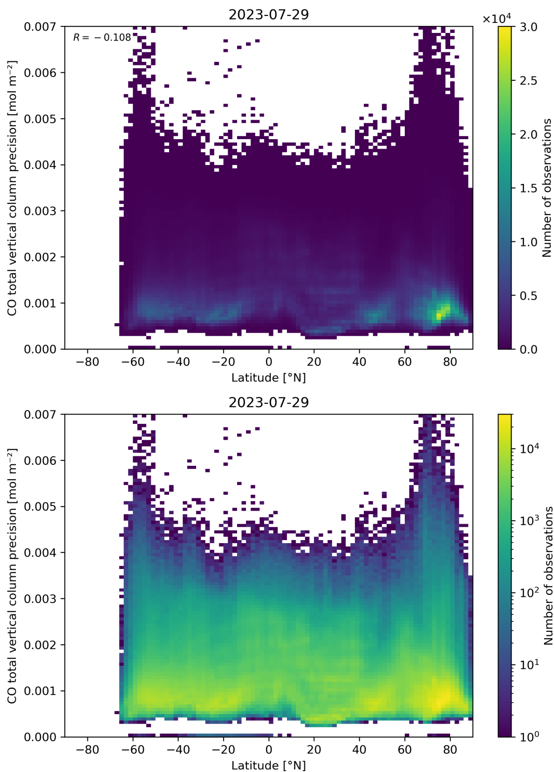
Figure 53: Scatter density plot of “Latitude” against “CO total vertical column precision” for 2023-07-29 to 2023-07-30.
