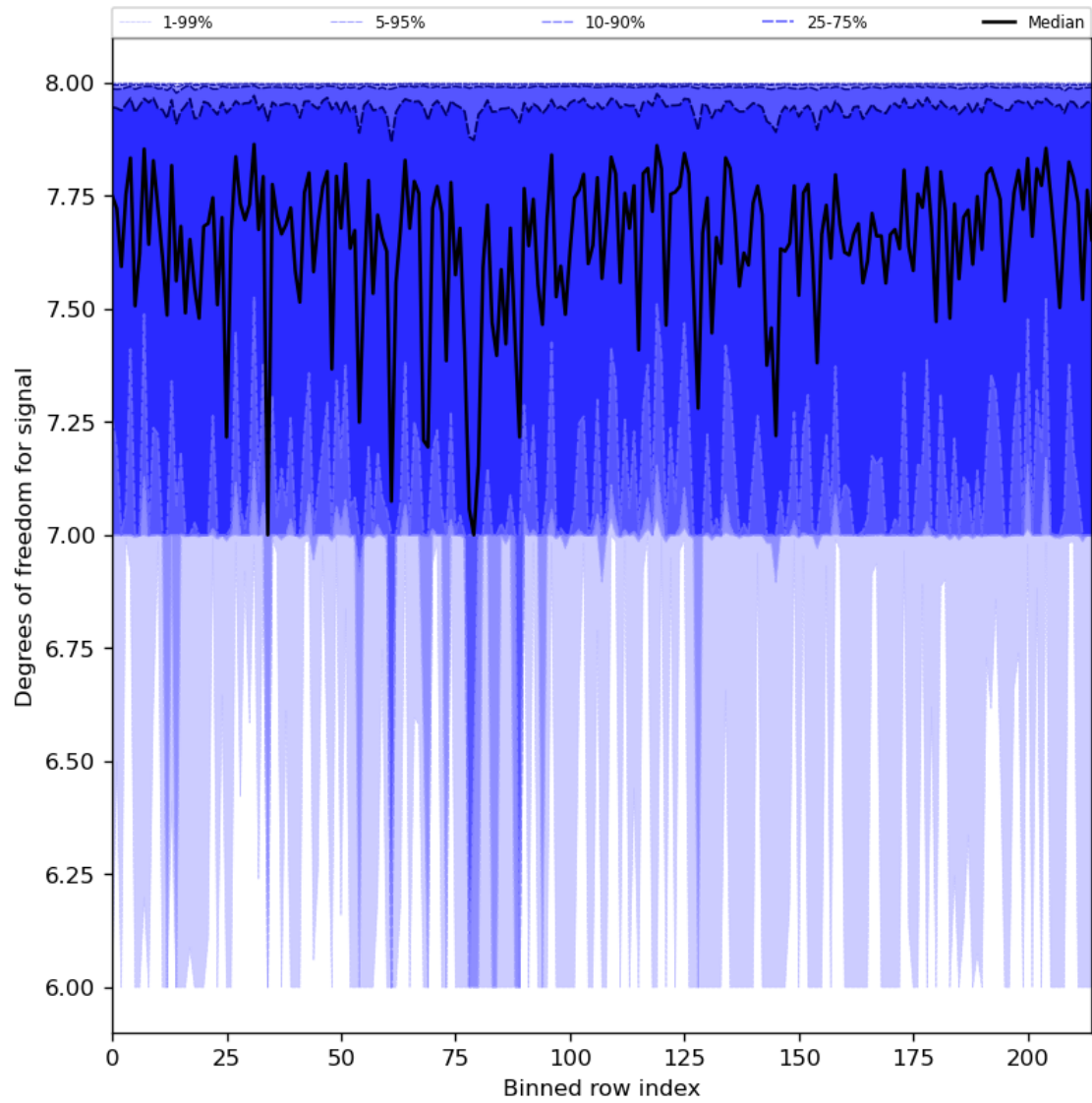
Figure 31: Along track statistics of “Degrees of freedom for signal” for 2023-07-29 to 2023-07-30
