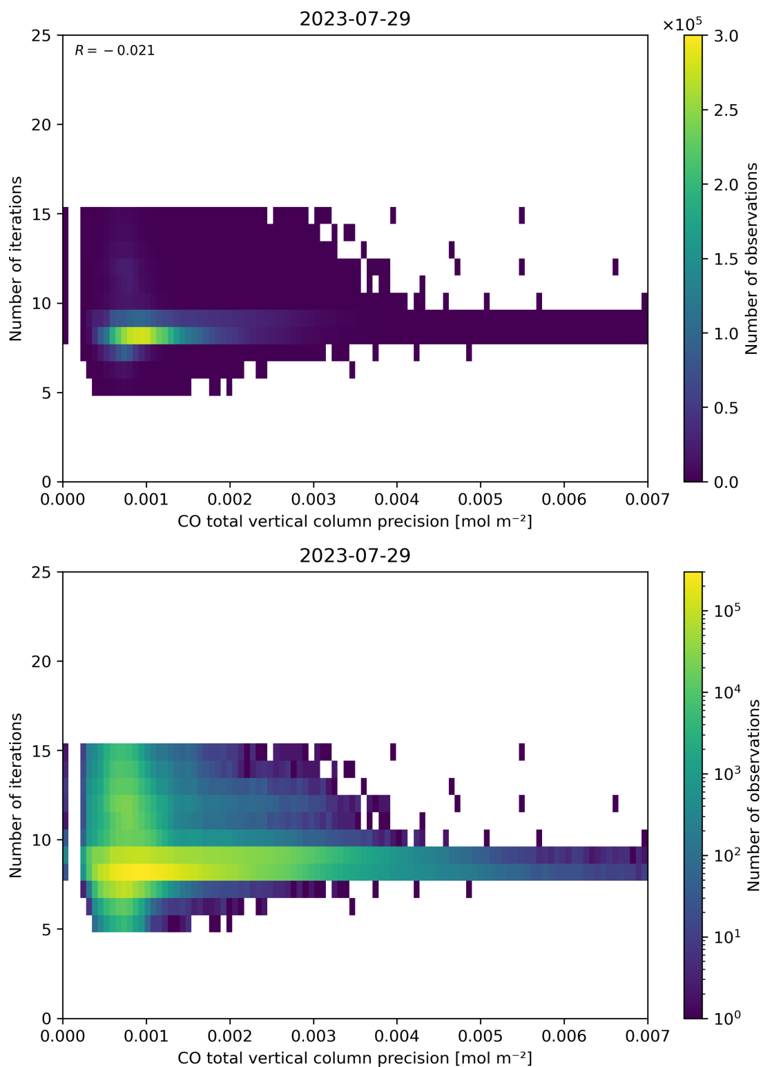
Figure 46: Scatter density plot of “CO total vertical column precision” against “Number of iterations” for 2023-07-29 to 2023-07-30.
