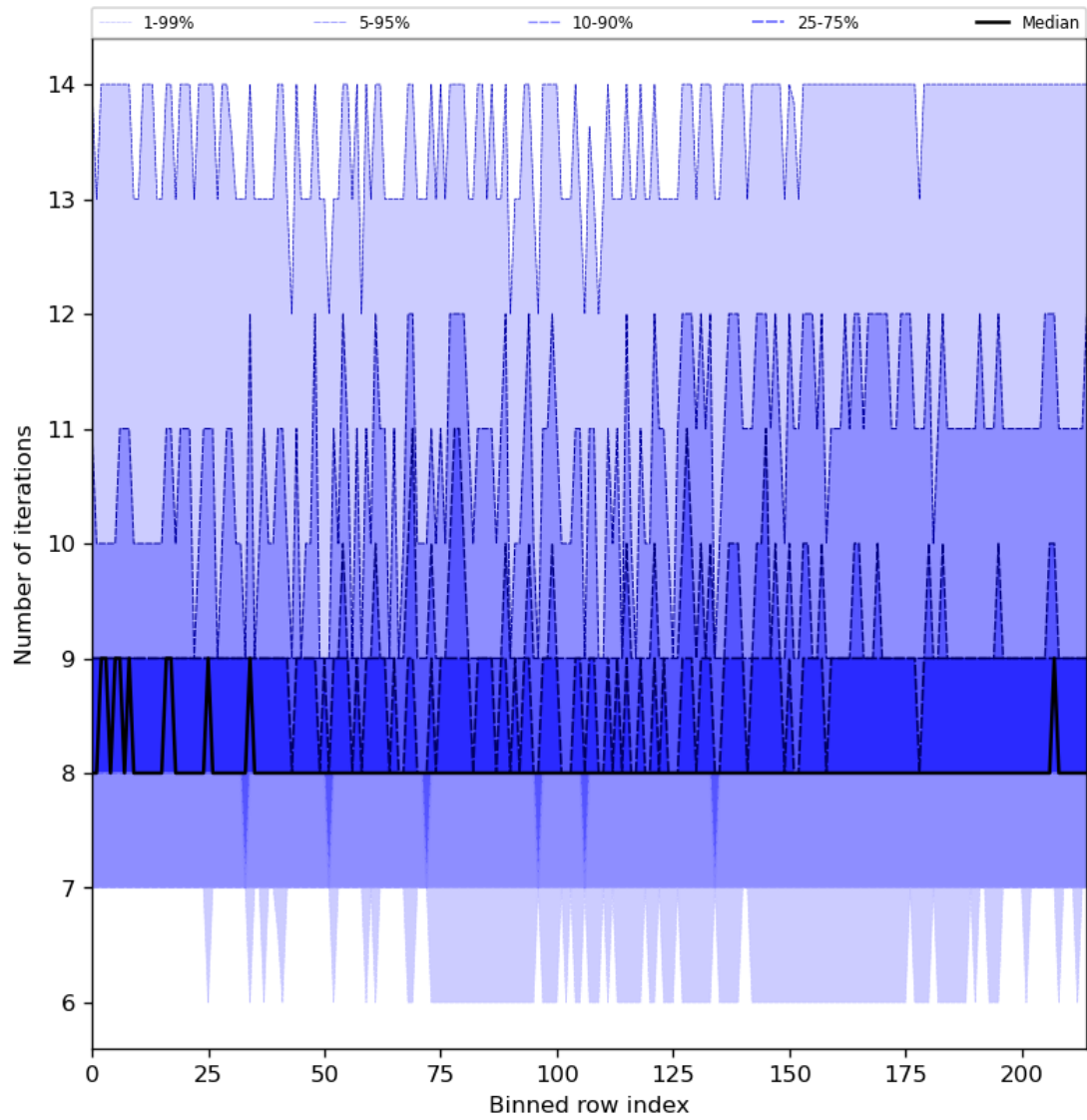
Figure 32: Along track statistics of “Number of iterations” for 2023-07-29 to 2023-07-30
