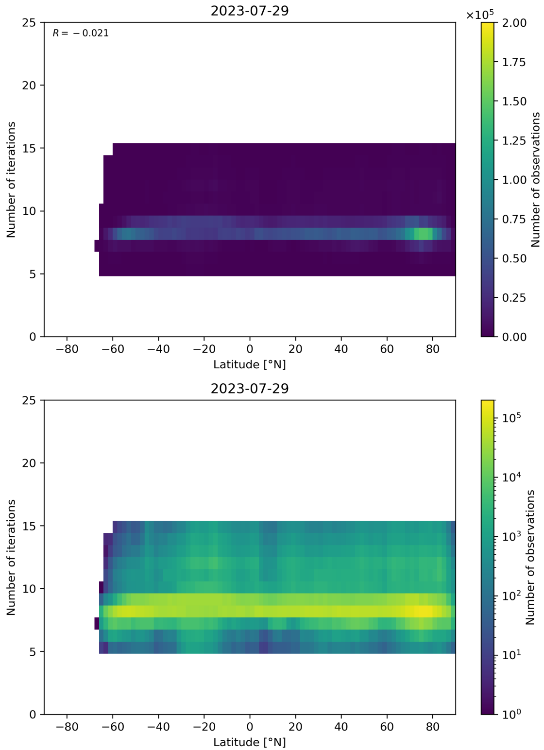
Figure 56: Scatter density plot of “Latitude” against “Number of iterations” for 2023-07-29 to 2023-07-30.
