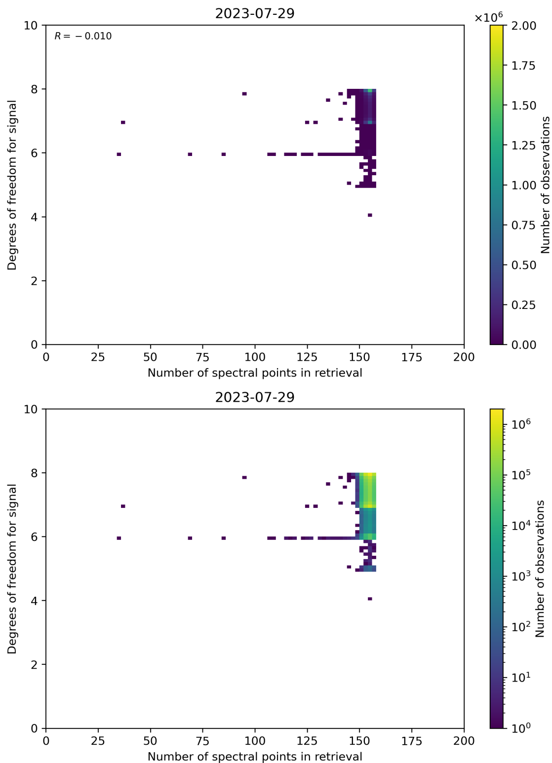
Figure 59: Scatter density plot of “Number of spectral points in retrieval” against “Degrees of freedom for signal” for 2023-07-29 to 2023-07-30.
