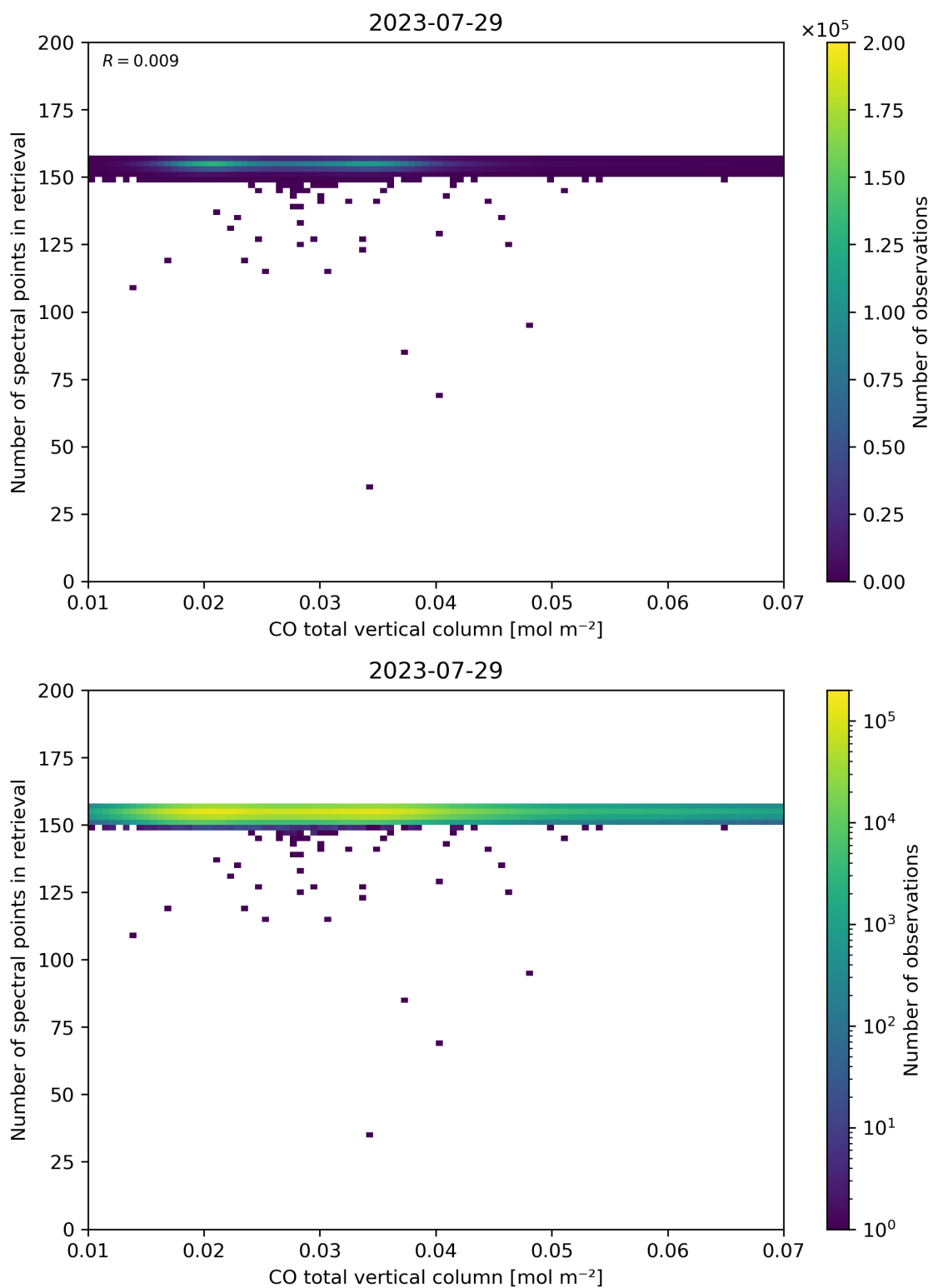
Figure 43: Scatter density plot of “CO total vertical column” against “Number of spectral points in retrieval” for 2023-07-29 to 2023-07-30.
