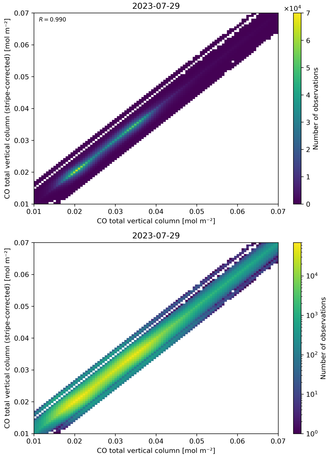
Figure 33: Scatter density plot of “CO total vertical column” against “CO total vertical column (stripe-corrected)” for 2023-07-29 to 2023-07-30.
