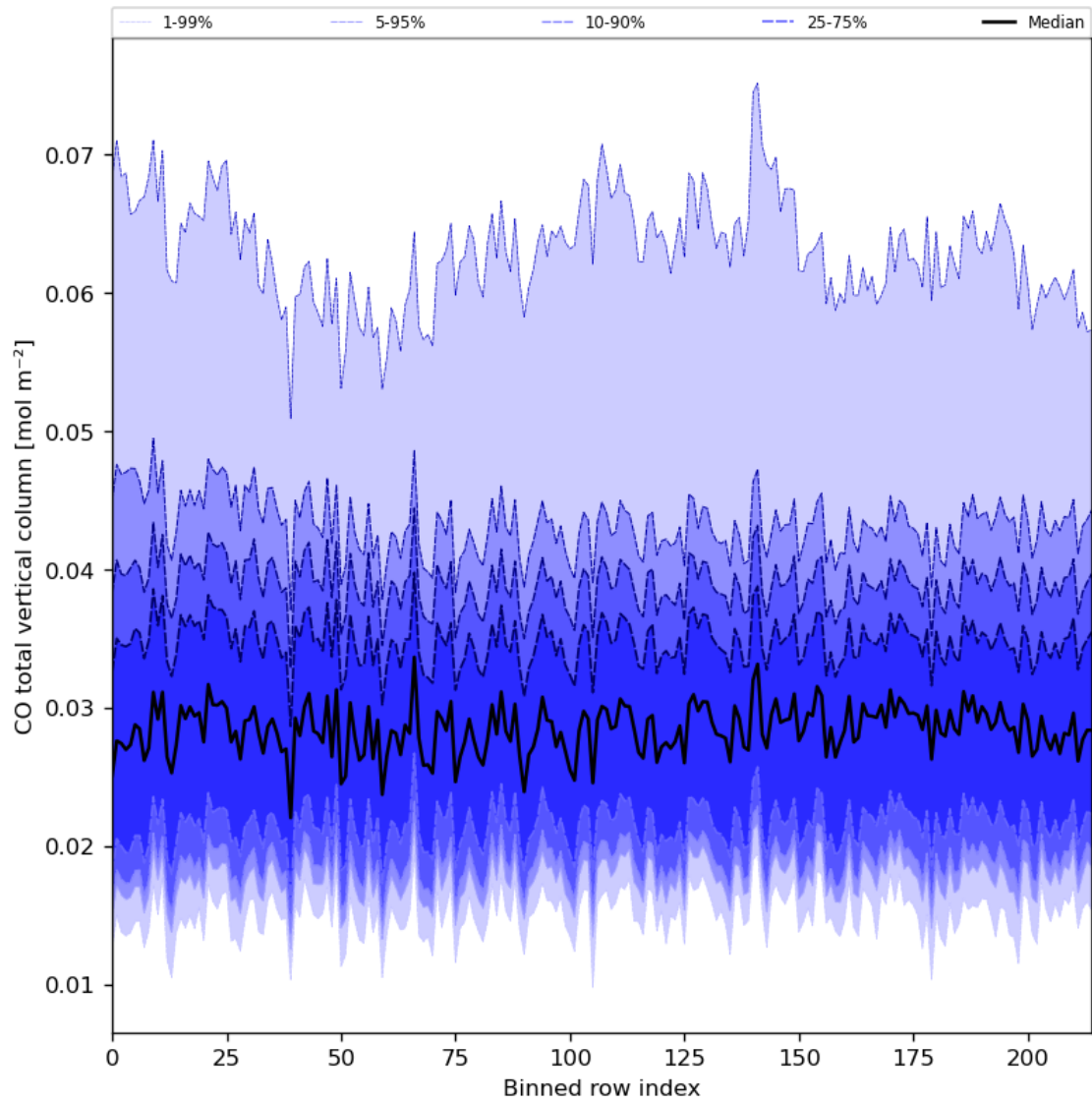
Figure 26: Along track statistics of “CO total vertical column” for 2023-07-29 to 2023-07-30
