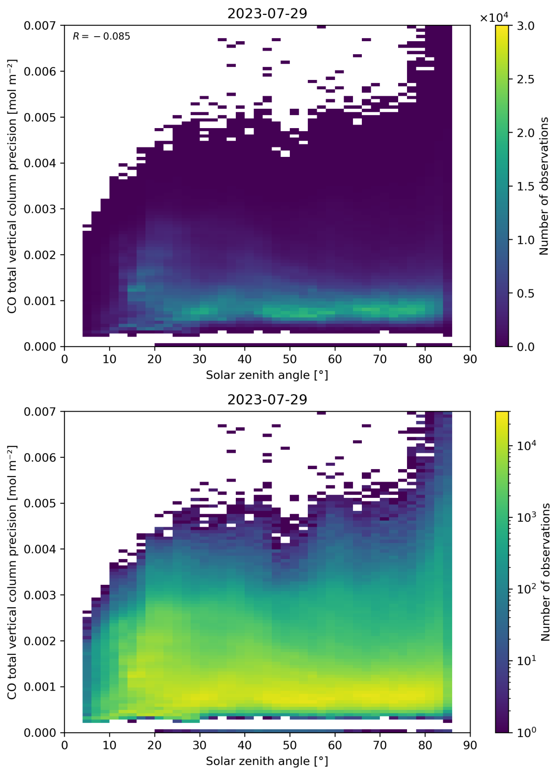
Figure 63: Scatter density plot of “Solar zenith angle” against “CO total vertical column precision” for 2023-07-29 to 2023-07-30.
