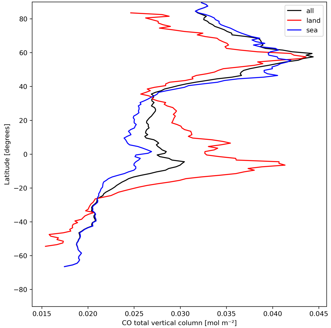
Figure 10: Zonal average of “CO total vertical column” for 2023-07-29 to 2023-07-30.
