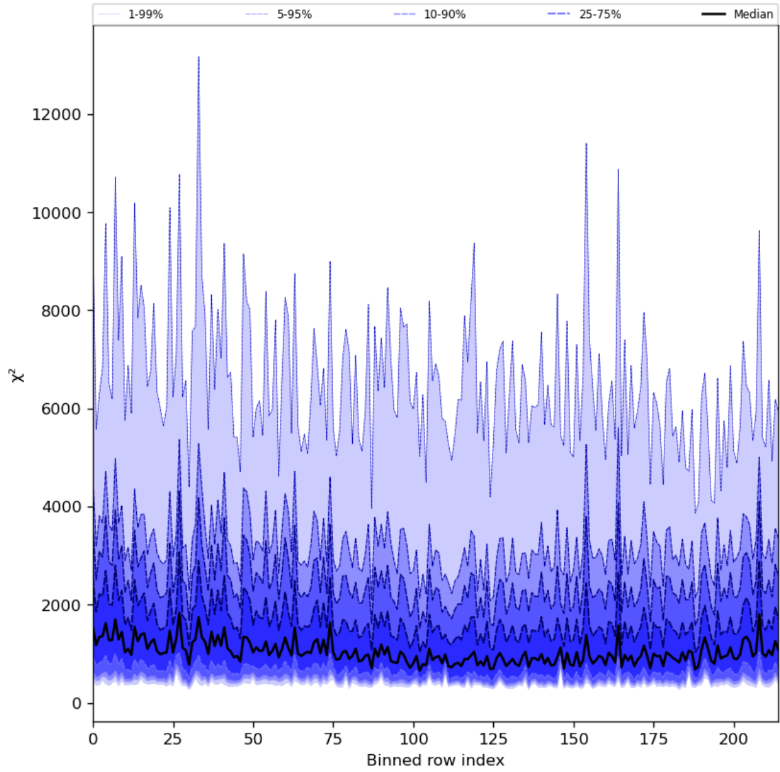
Figure 30: Along track statistics of “ \chi^2 ” for 2023-07-29 to 2023-07-30
