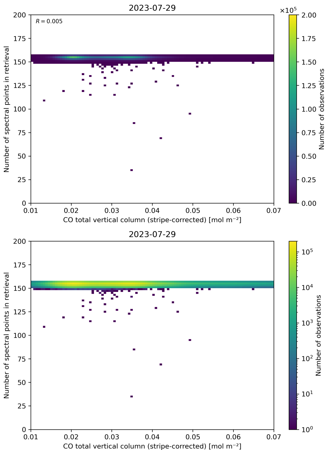
Figure 40: Scatter density plot of “CO total vertical column (stripe-corrected)” against “Number of spectral points in retrieval” for 2023-07-29 to 2023-07-30.
