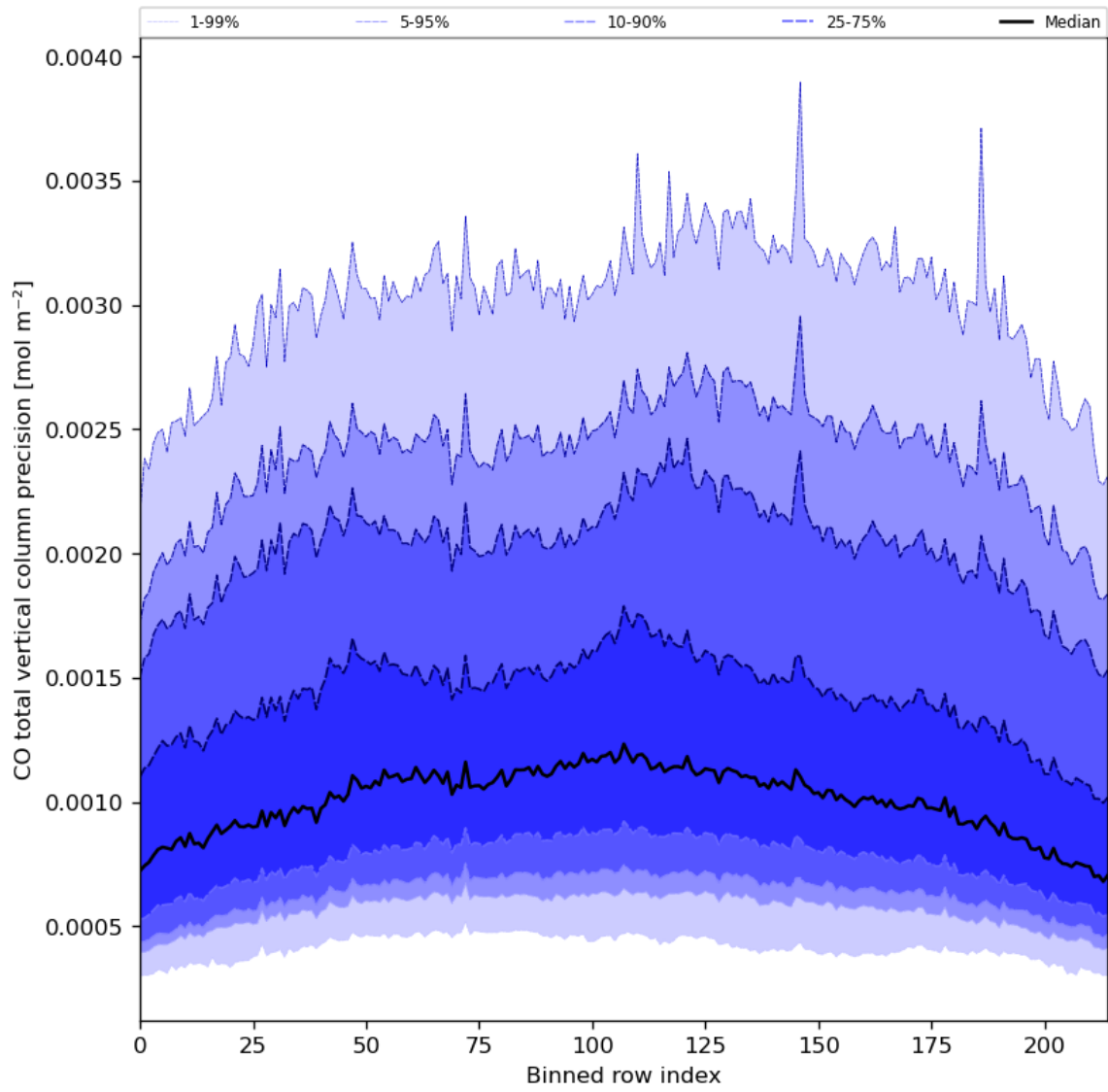
Figure 28: Along track statistics of “CO total vertical column precision” for 2023-07-29 to 2023-07-30
