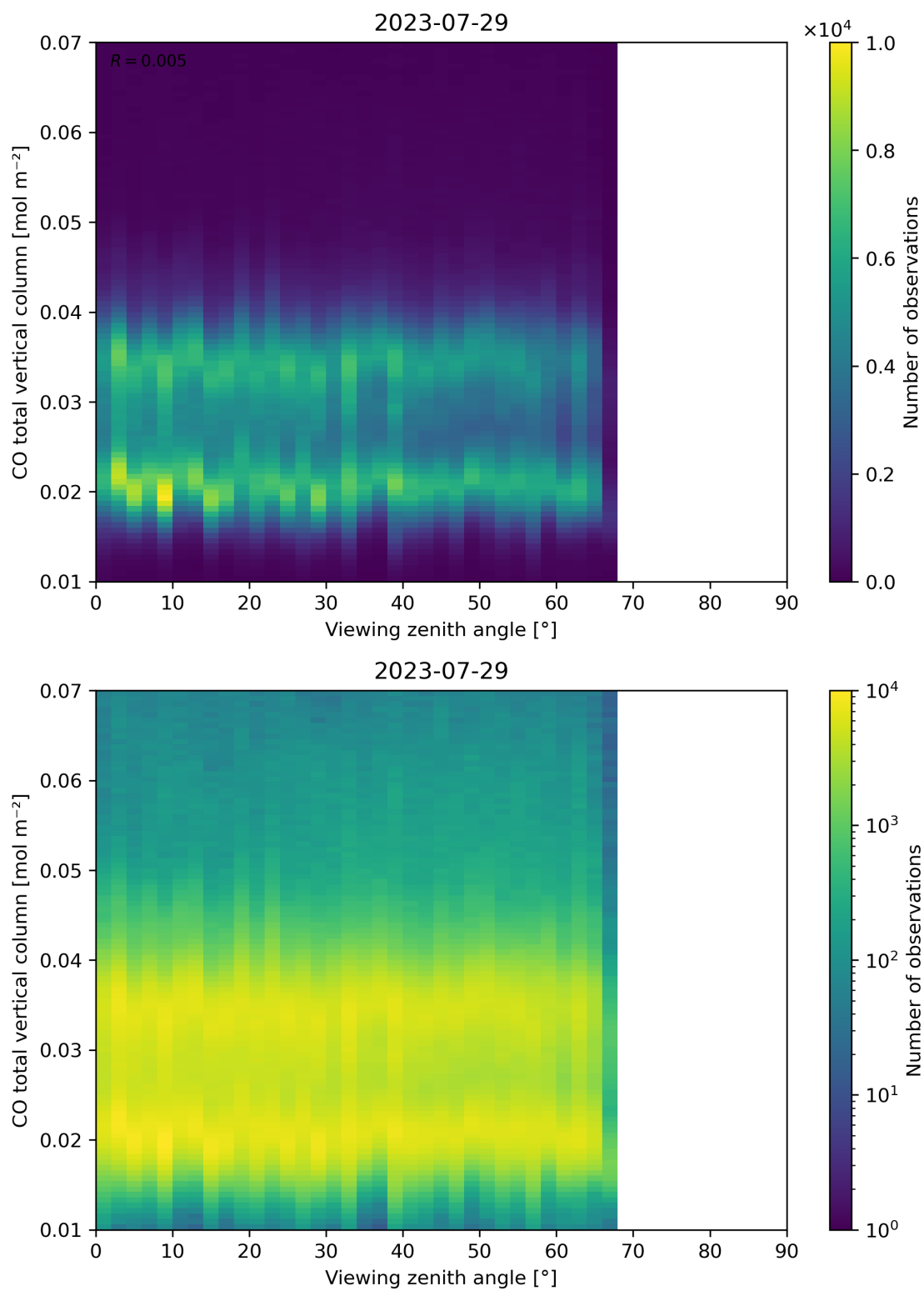
Figure 69: Scatter density plot of “Viewing zenith angle” against “CO total vertical column” for 2023-07-29 to 2023-07-30.
