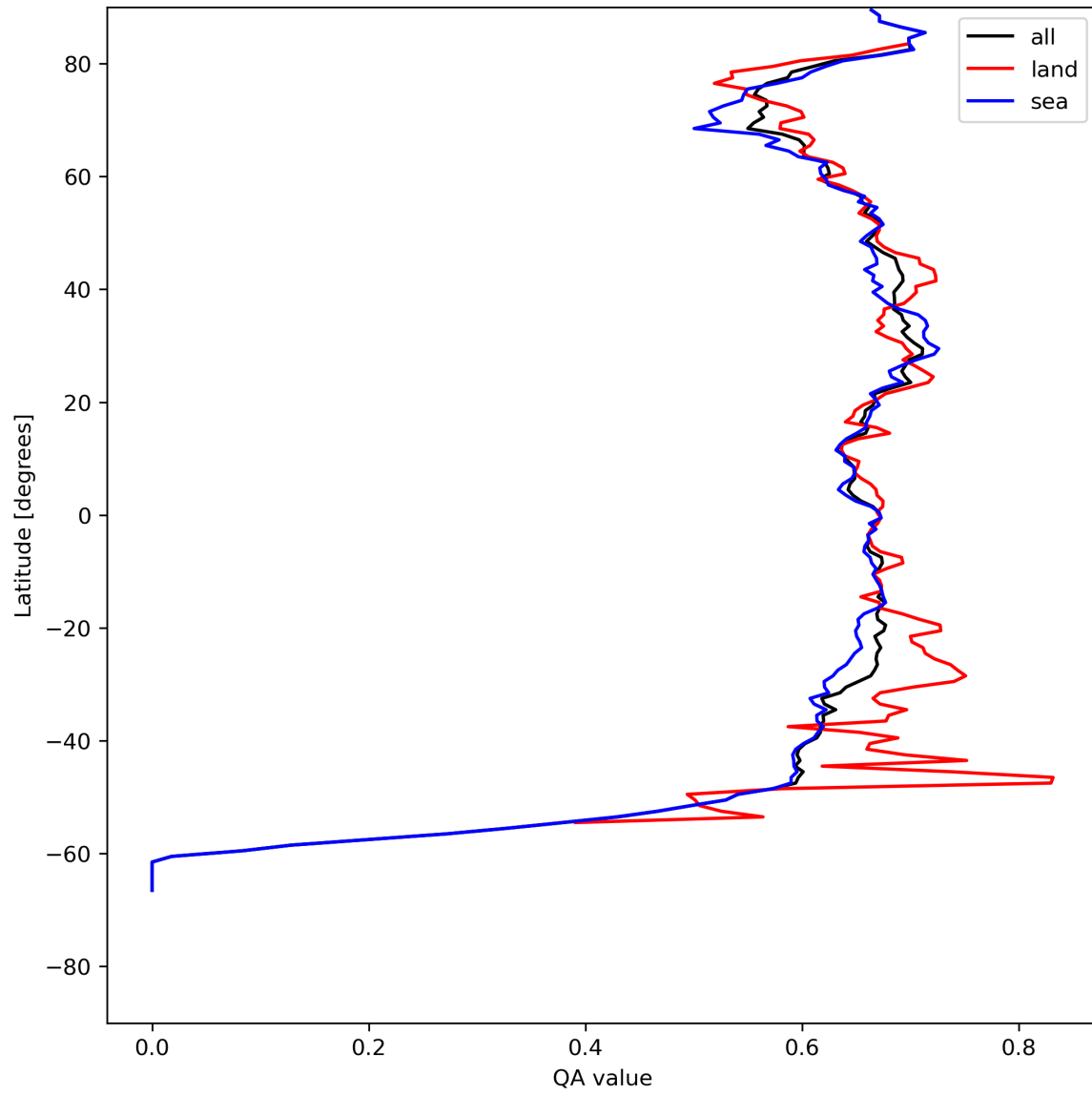
Figure 9: Zonal average of “QA value” for 2023-07-29 to 2023-07-30.
