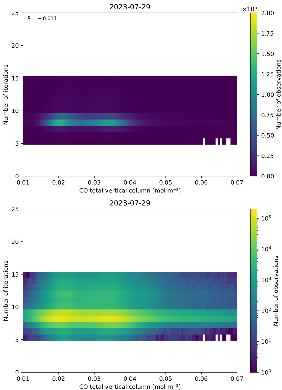
Figure 42: Scatter density plot of “CO total vertical column” against “Number of iterations” for 2023-07-29 to 2023-07-30.
