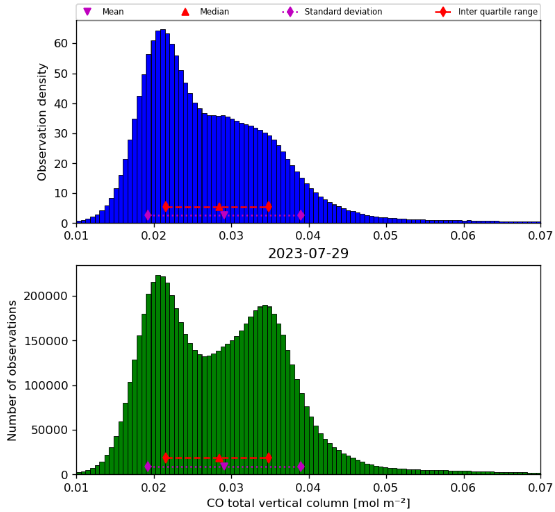
Figure 18: Histogram of “CO total vertical column” for 2023-07-29 to 2023-07-30
