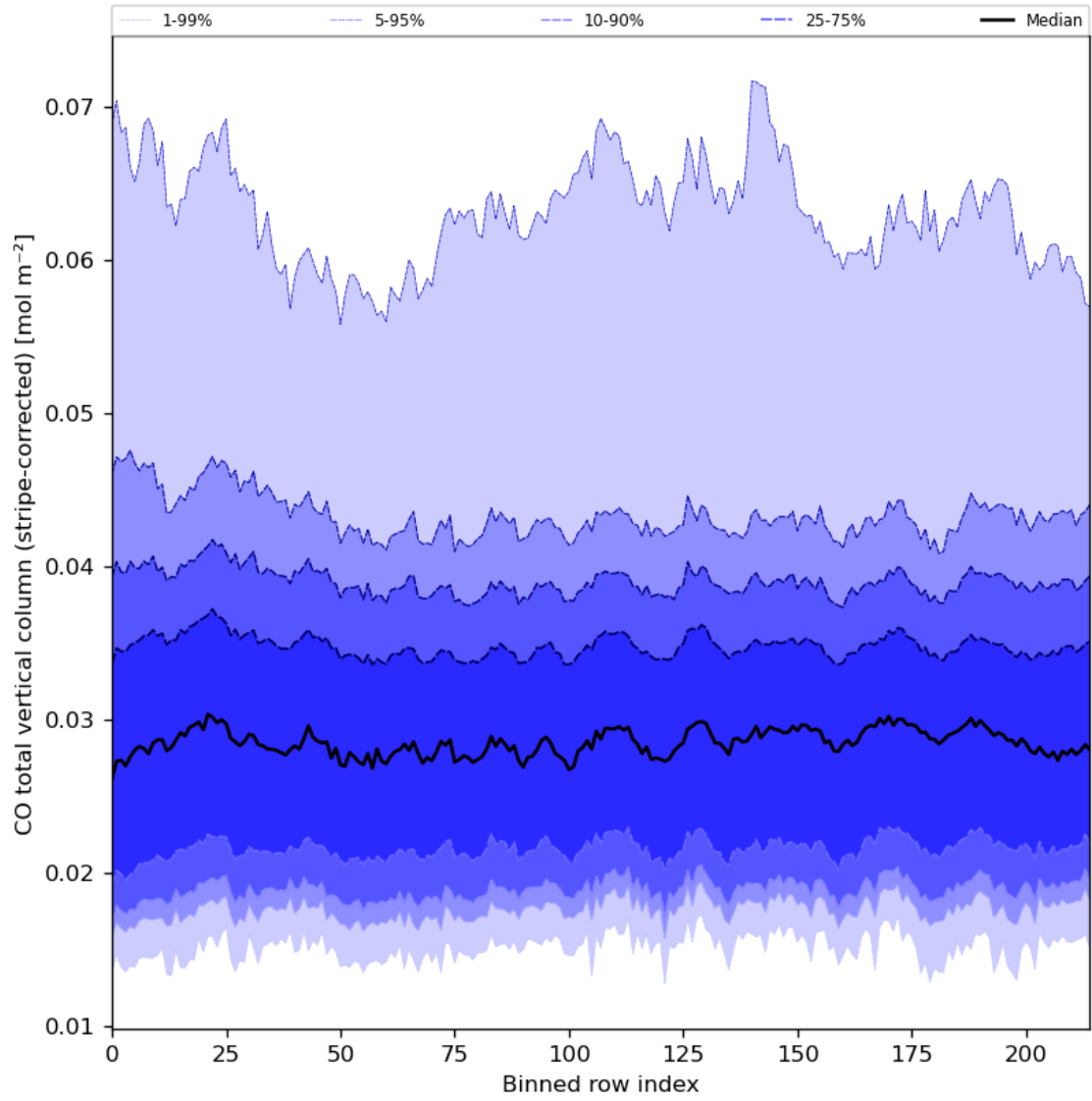
Figure 27: Along track statistics of “CO total vertical column (stripe-corrected)” for 2023-07-29 to 2023-07-30
