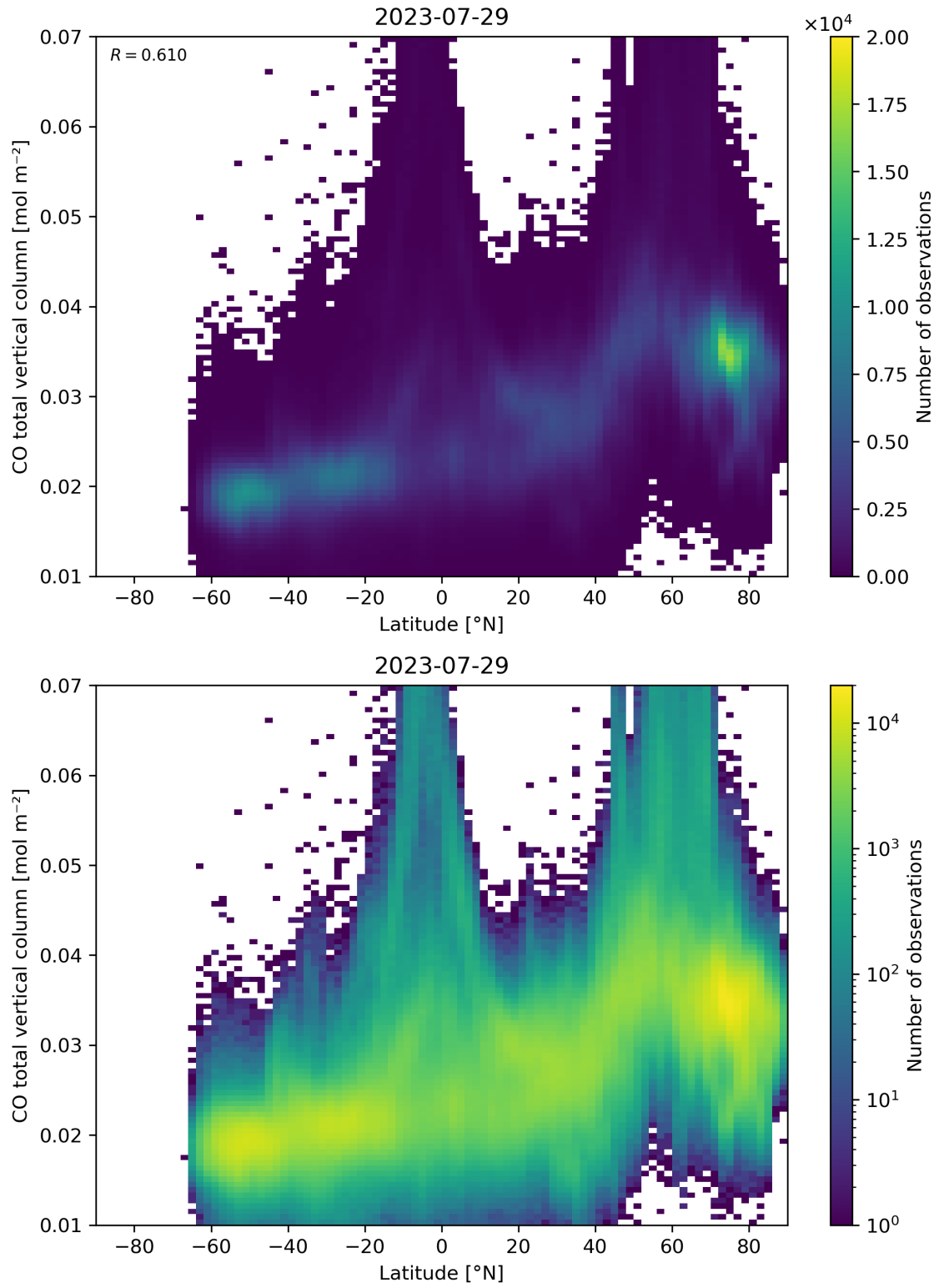
Figure 51: Scatter density plot of “Latitude” against “CO total vertical column” for 2023-07-29 to 2023-07-30.
