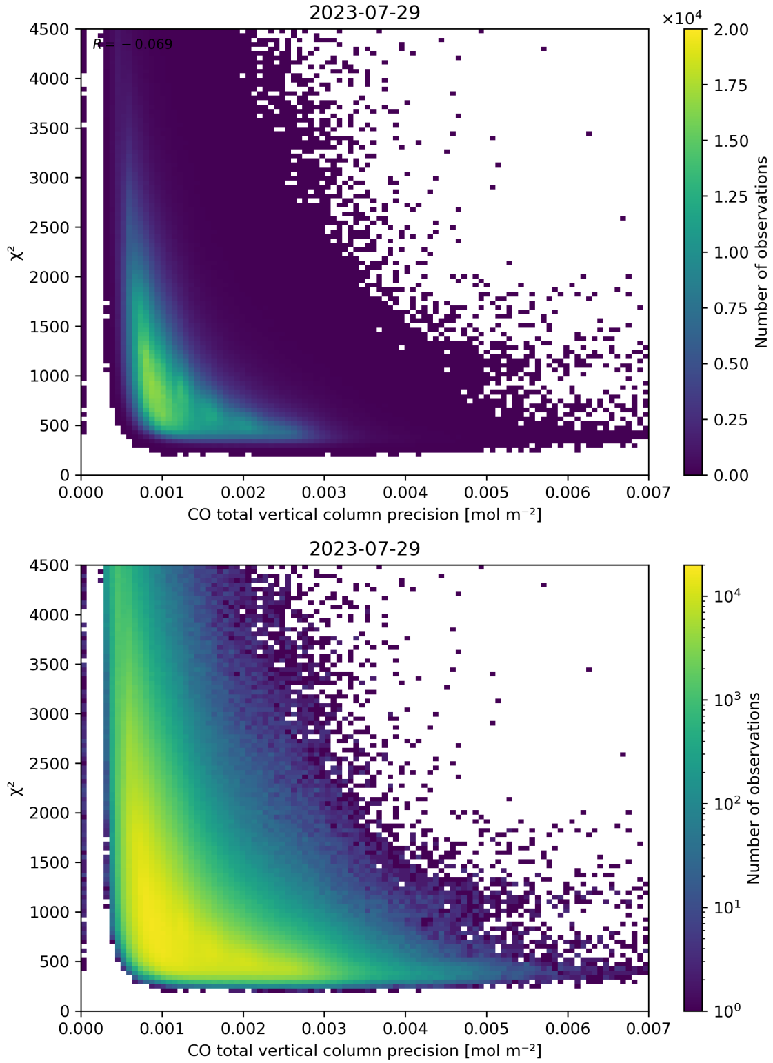
Figure 44: Scatter density plot of “CO total vertical column precision” against “ \chi^2 ” for 2023-07-29 to 2023-07-30.
