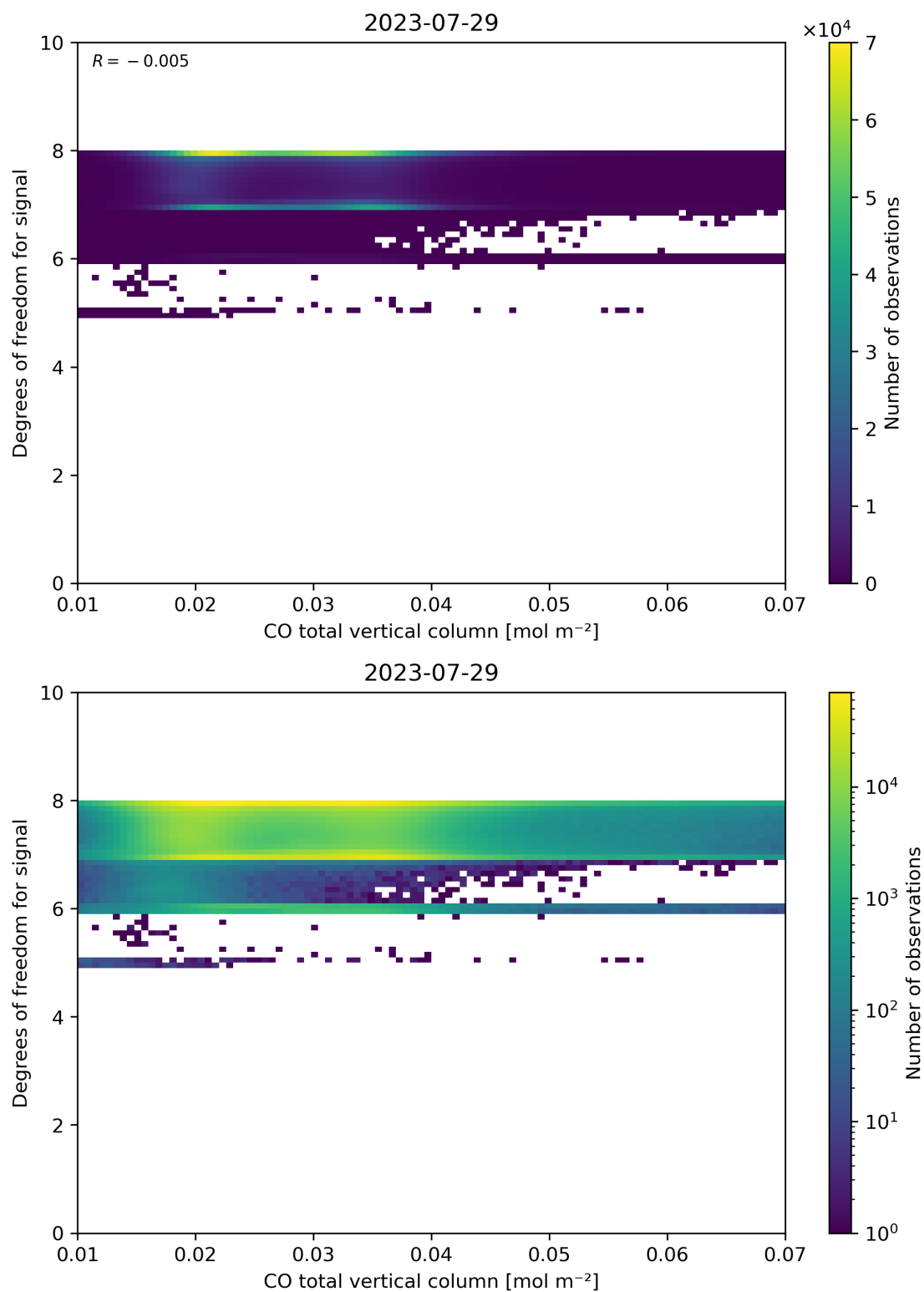
Figure 41: Scatter density plot of “CO total vertical column” against “Degrees of freedom for signal” for 2023-07-29 to 2023-07-30.
