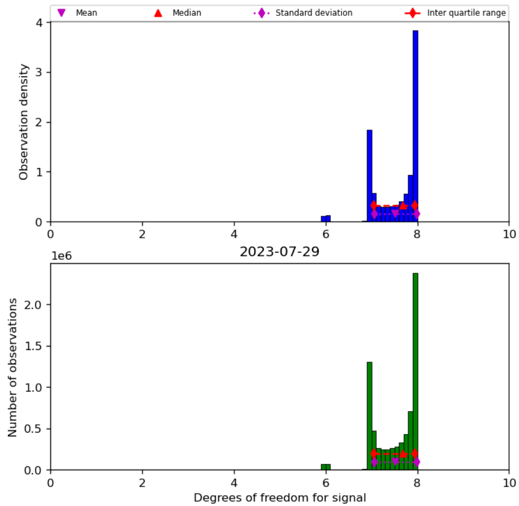
Figure 23: Histogram of “Degrees of freedom for signal” for 2023-07-29 to 2023-07-30
