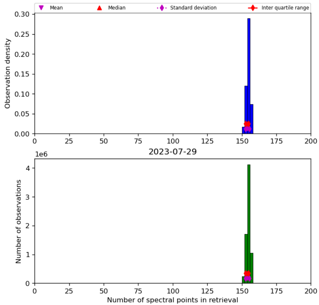
Figure 21: Histogram of “Number of spectral points in retrieval” for 2023-07-29 to 2023-07-30
