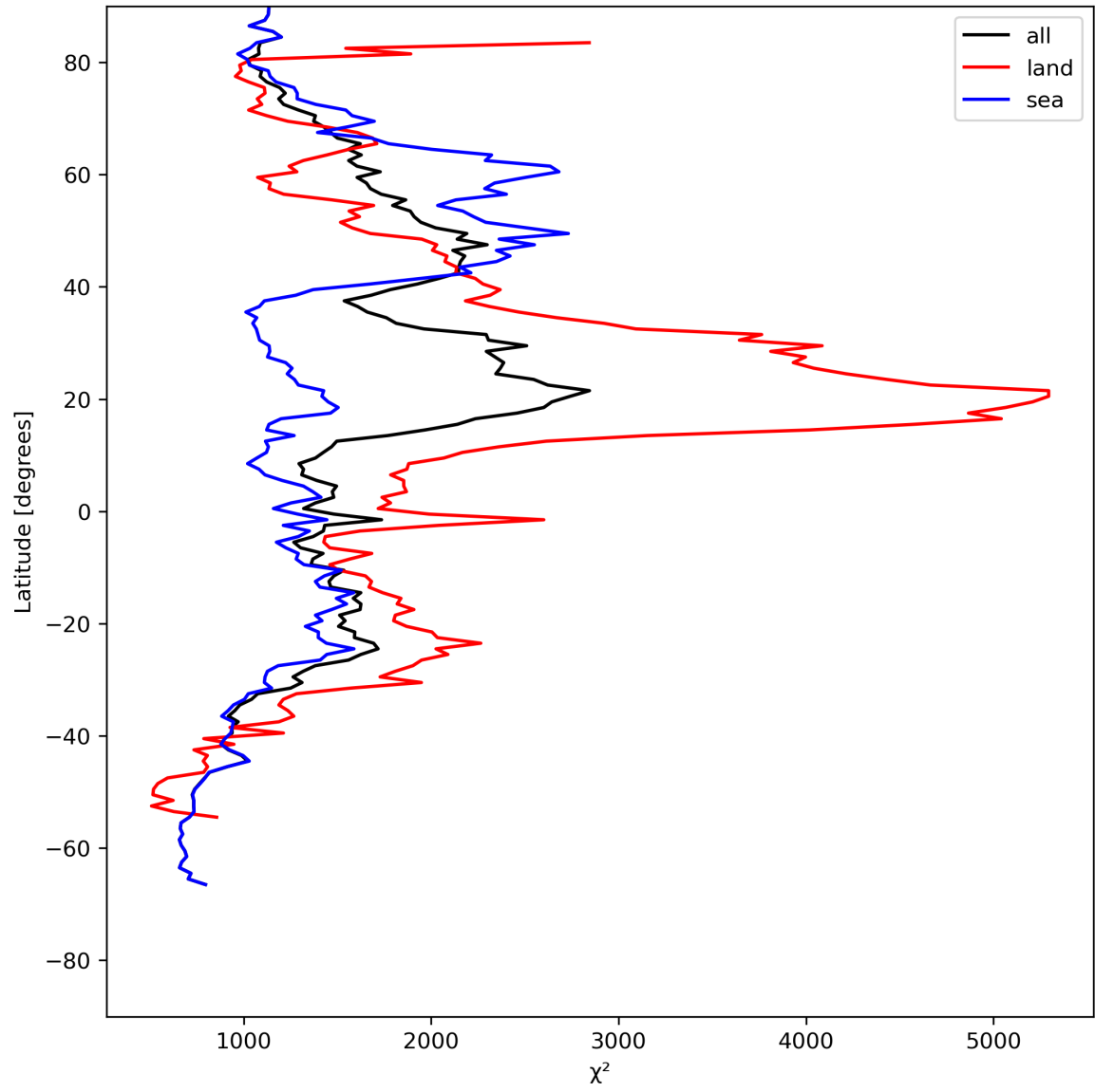
Figure 14: Zonal average of “ \chi^2 ” for 2023-07-29 to 2023-07-30.
