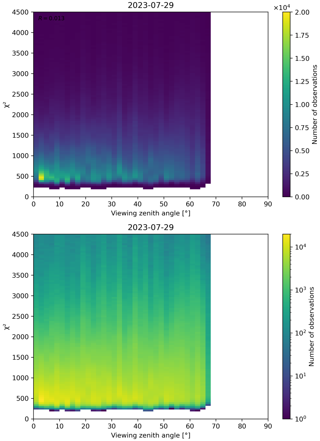
Figure 72: Scatter density plot of “Viewing zenith angle” against “ \chi^2 ” for 2023-07-29 to 2023-07-30.
