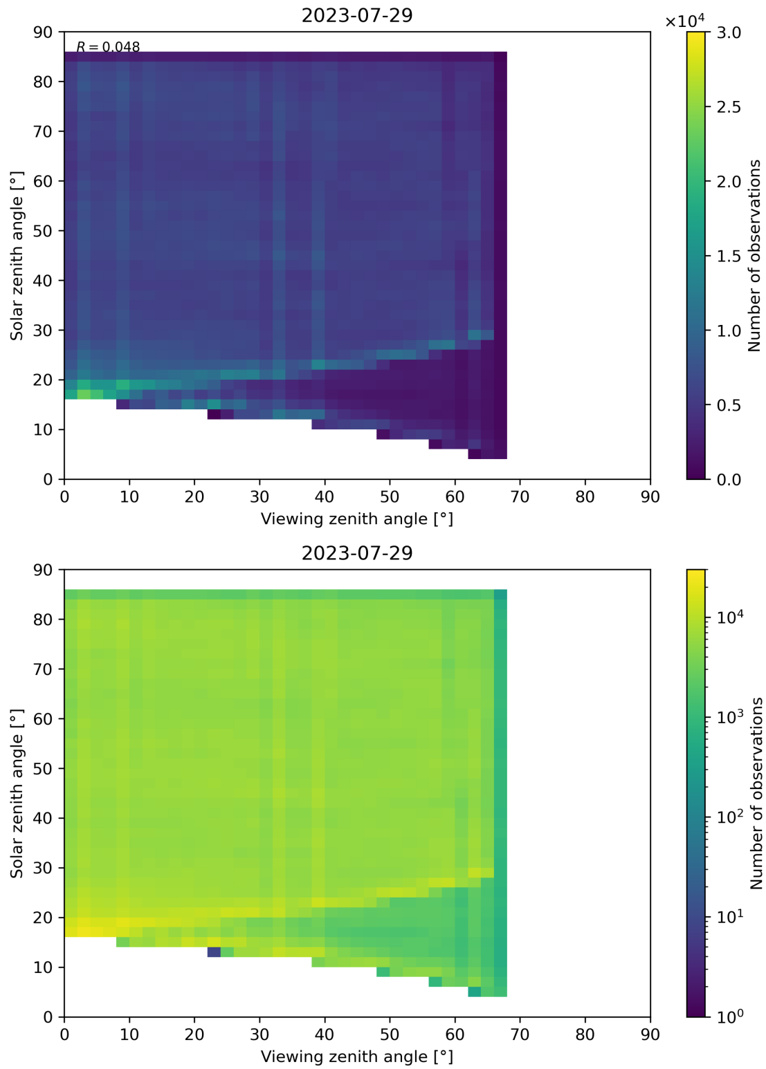
Figure 77: Scatter density plot of “Viewing zenith angle” against “Solar zenith angle” for 2023-07-29 to 2023-07-30.
