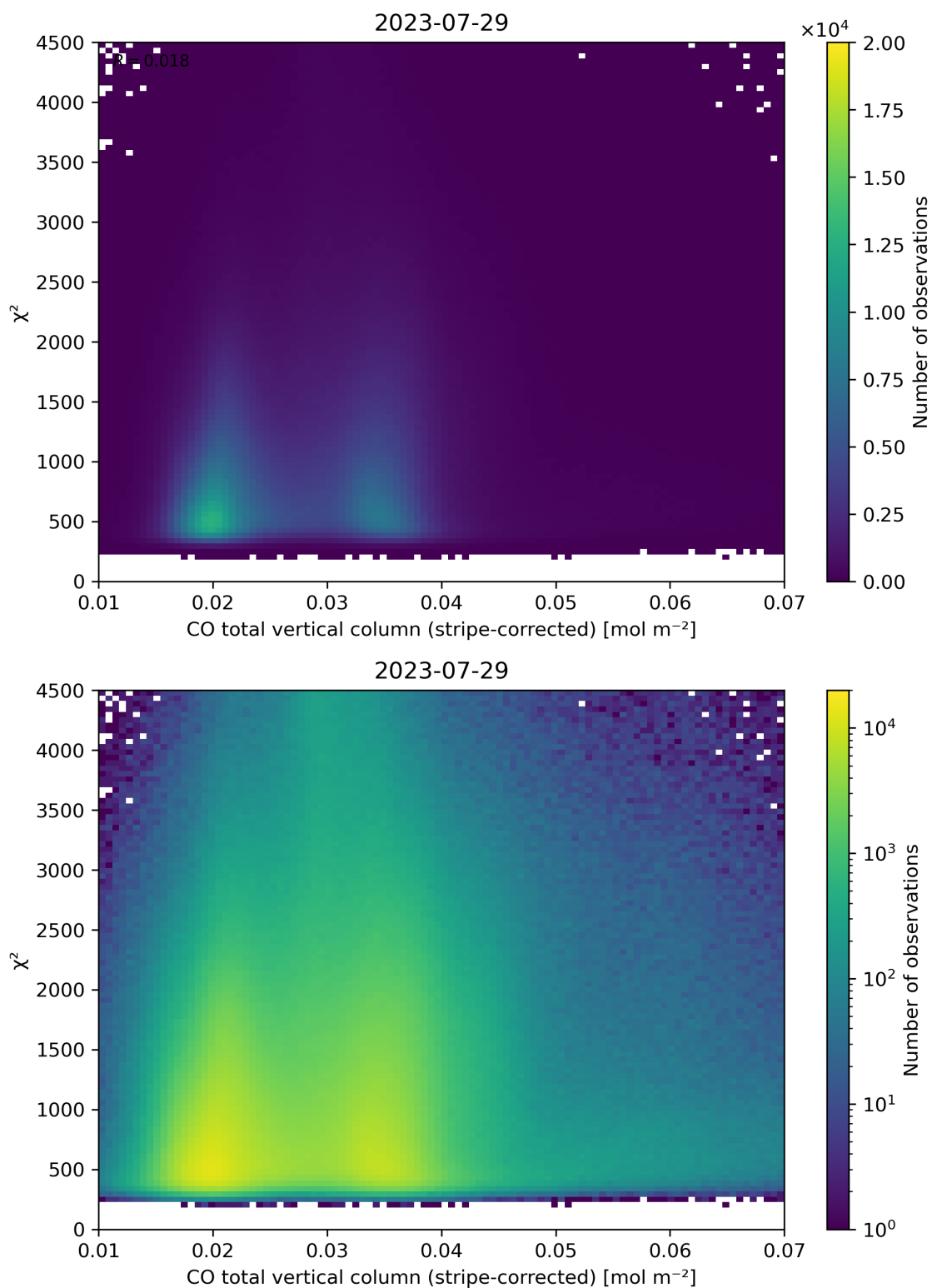
Figure 37: Scatter density plot of “CO total vertical column (stripe-corrected)” against “ \chi^2 ” for 2023-07-29 to 2023-07-30.
