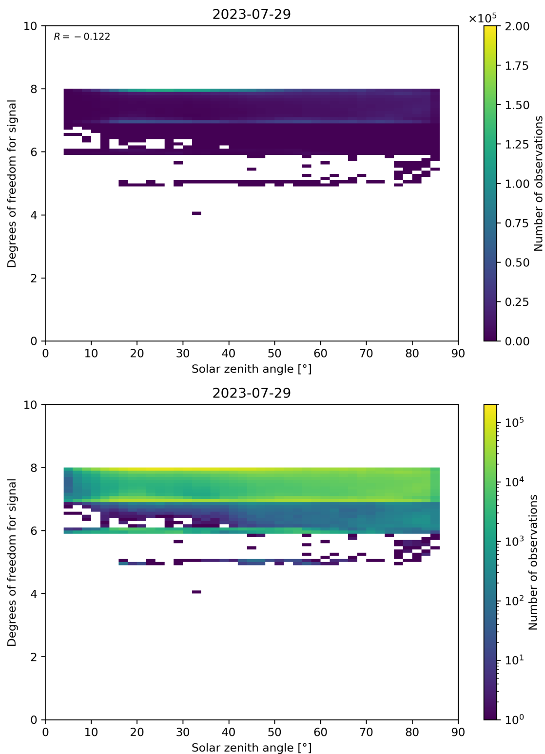
Figure 65: Scatter density plot of “Solar zenith angle” against “Degrees of freedom for signal” for 2023-07-29 to 2023-07-30.
