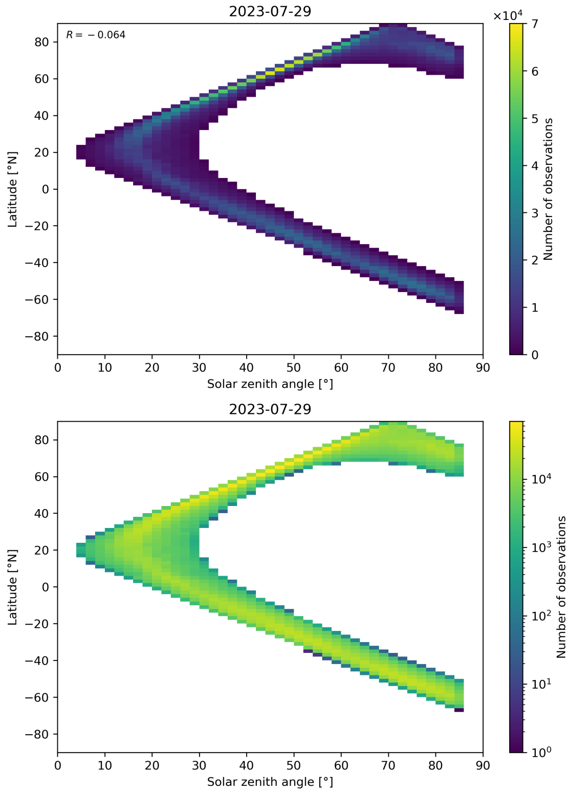
Figure 66: Scatter density plot of “Solar zenith angle” against “Latitude” for 2023-07-29 to 2023-07-30.
