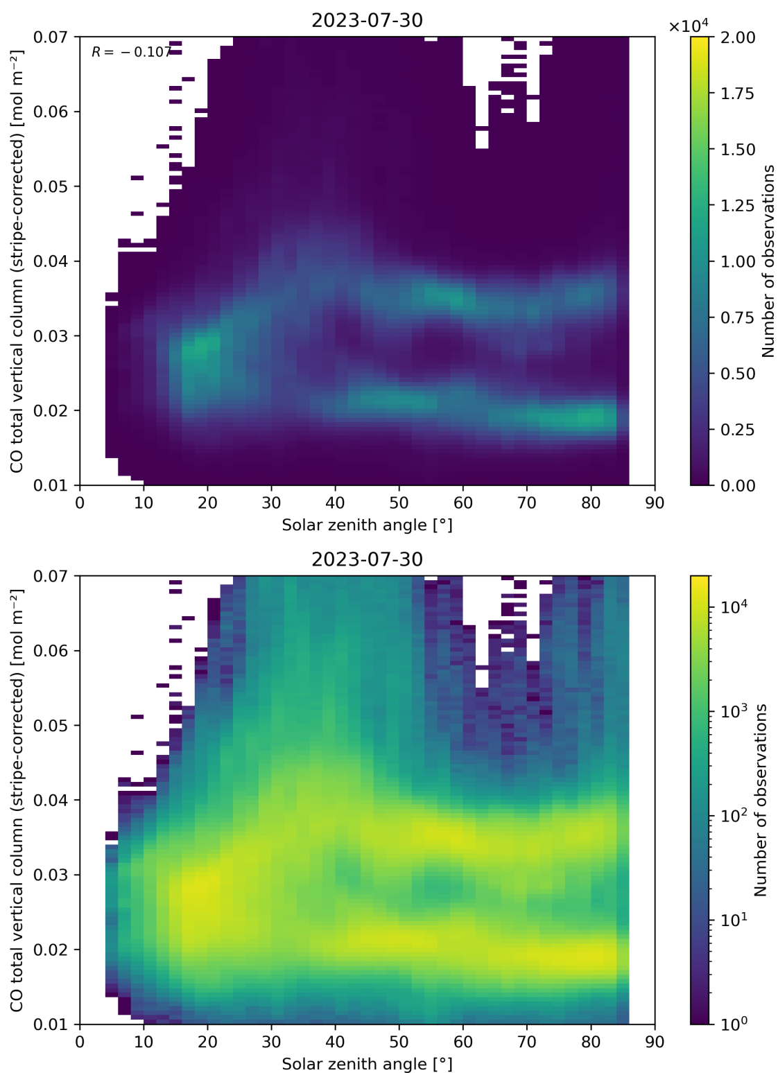
Figure 62: Scatter density plot of “Solar zenith angle” against “CO total vertical column (stripe-corrected)” for 2023-07-29 to 2023-07-31.
