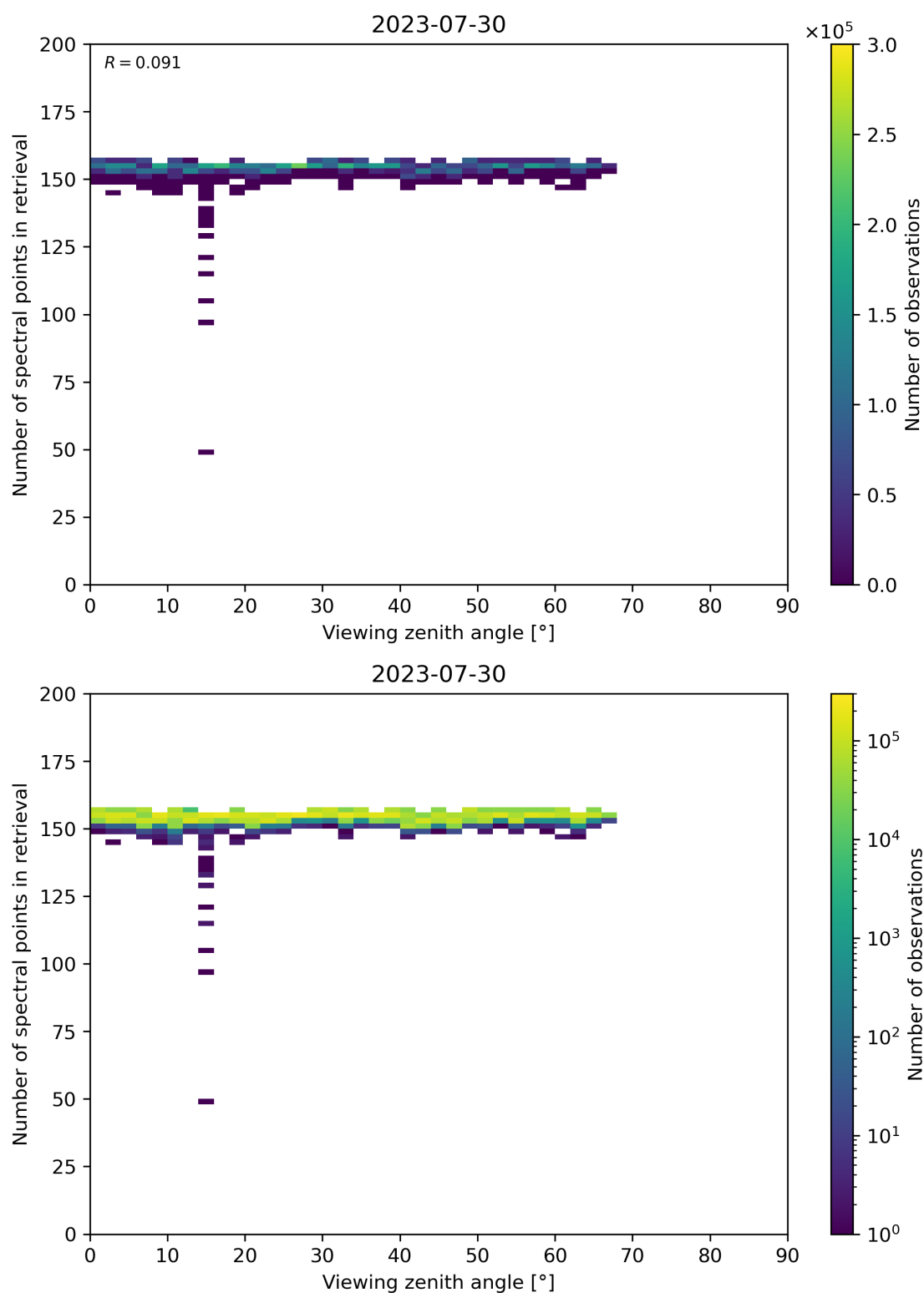
Figure 76: Scatter density plot of “Viewing zenith angle” against “Number of spectral points in retrieval” for 2023-07-29 to 2023-07-31.
