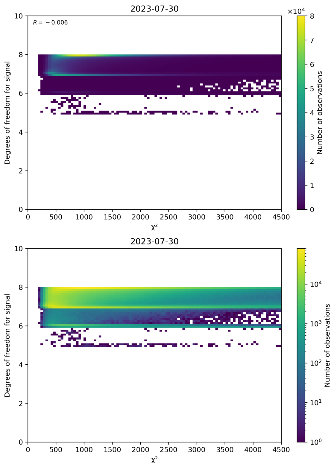
Figure 48: Scatter density plot of “ \chi^2 ” against “Degrees of freedom for signal” for 2023-07-29 to 2023-07-31.
