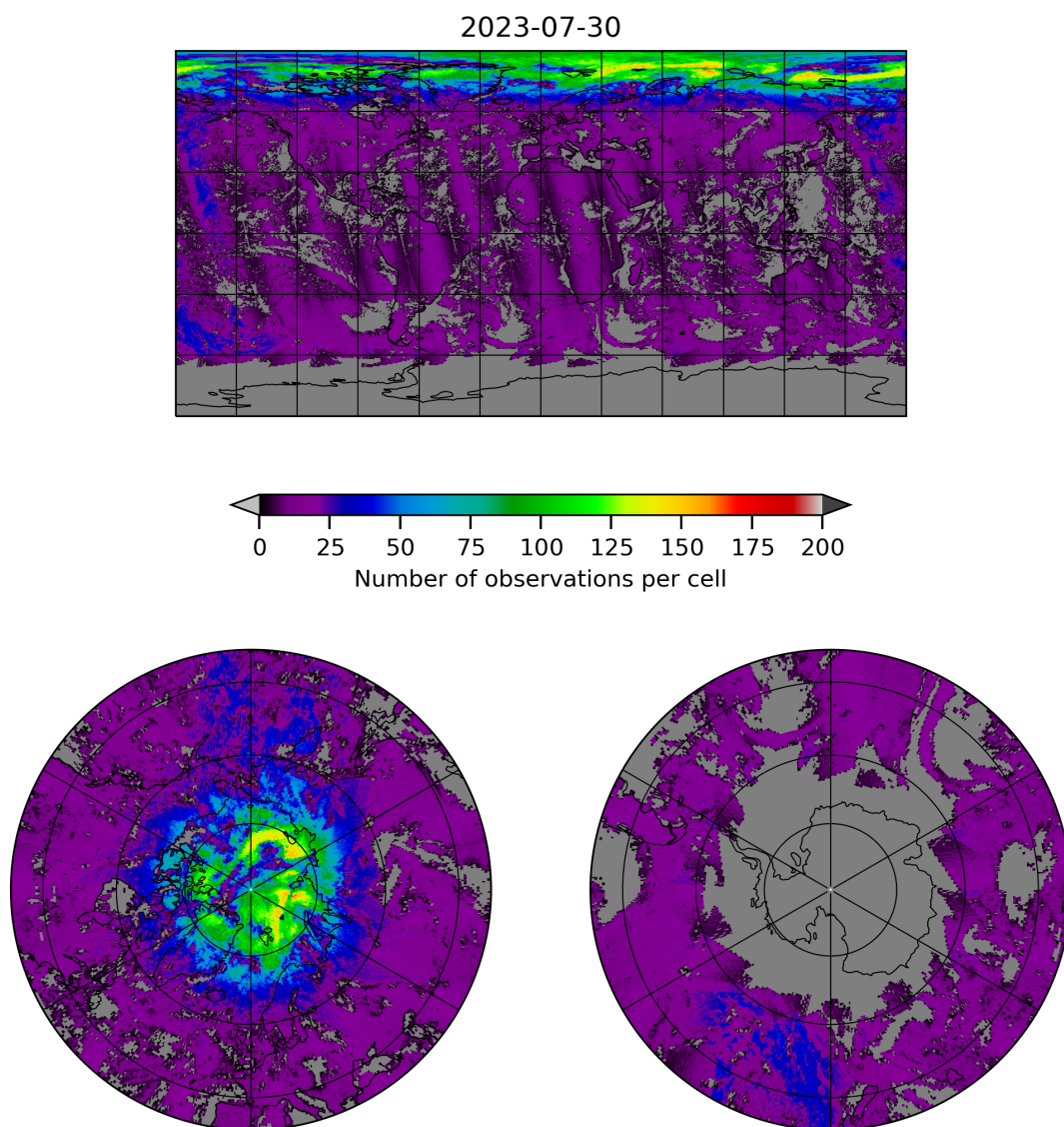
Figure 8: Map of the number of observations for 2023-07-29 to 2023-07-31
