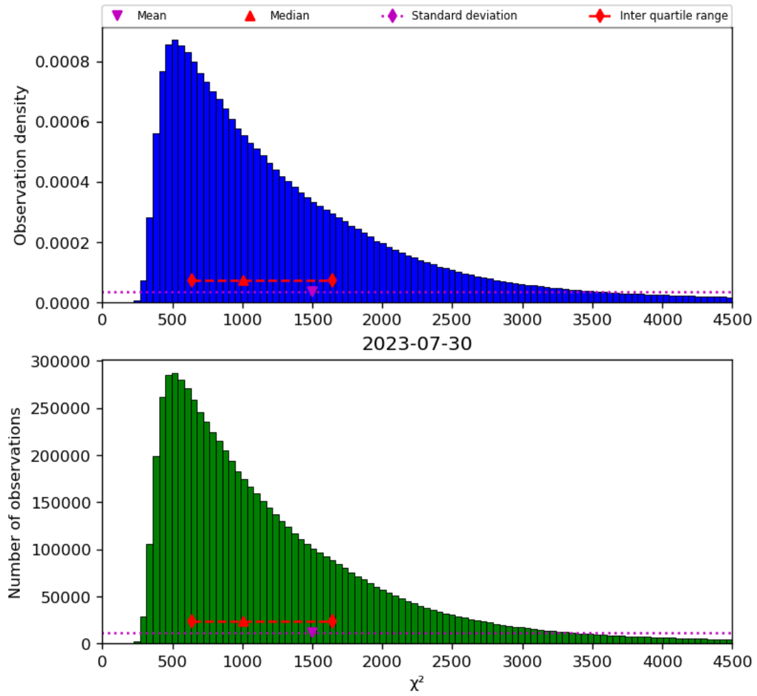
Figure 22: Histogram of " \chi^2 " for 2023-07-29 to 2023-07-31
