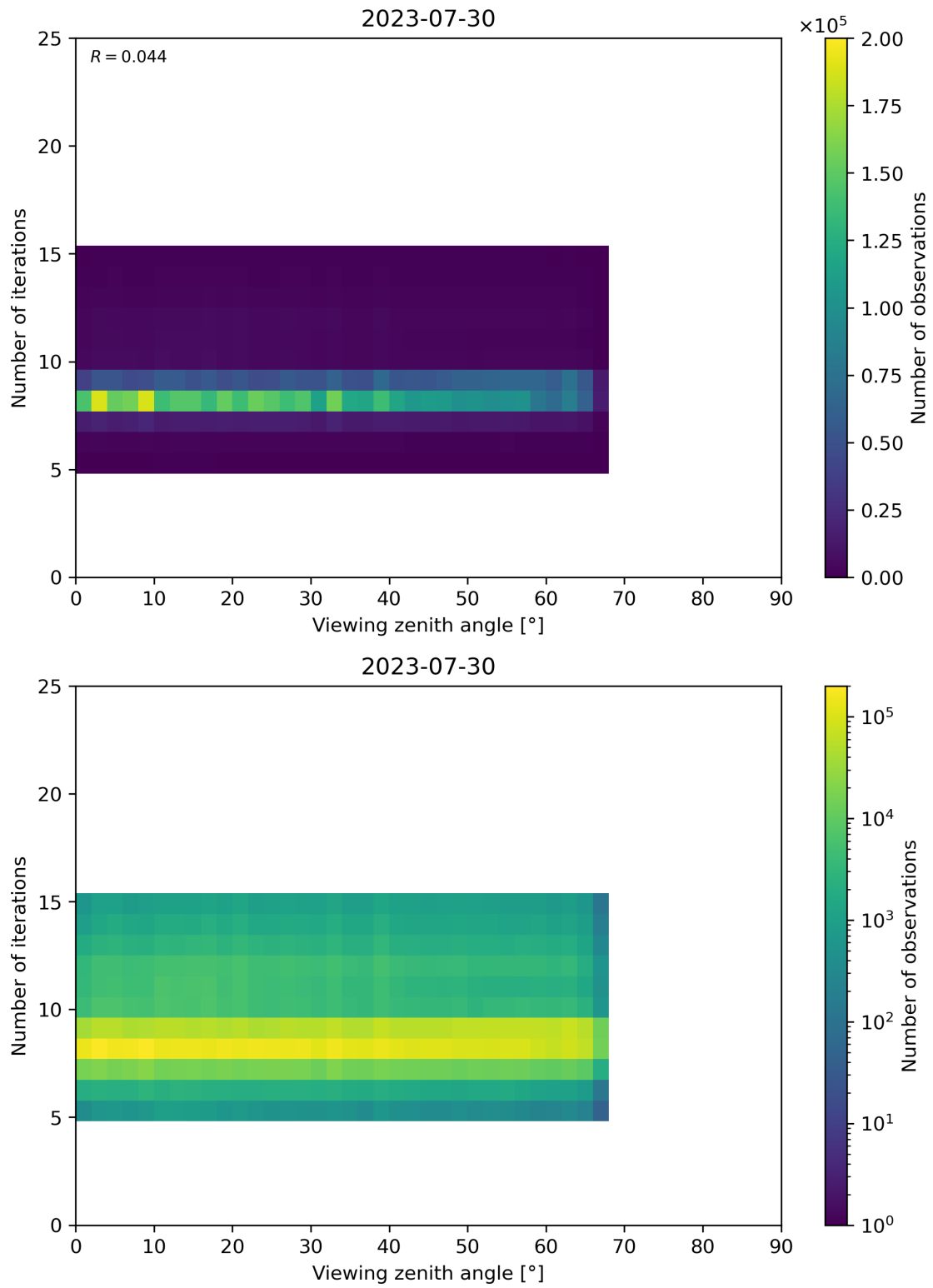
Figure 75: Scatter density plot of “Viewing zenith angle” against “Number of iterations” for 2023-07-29 to 2023-07-31.
