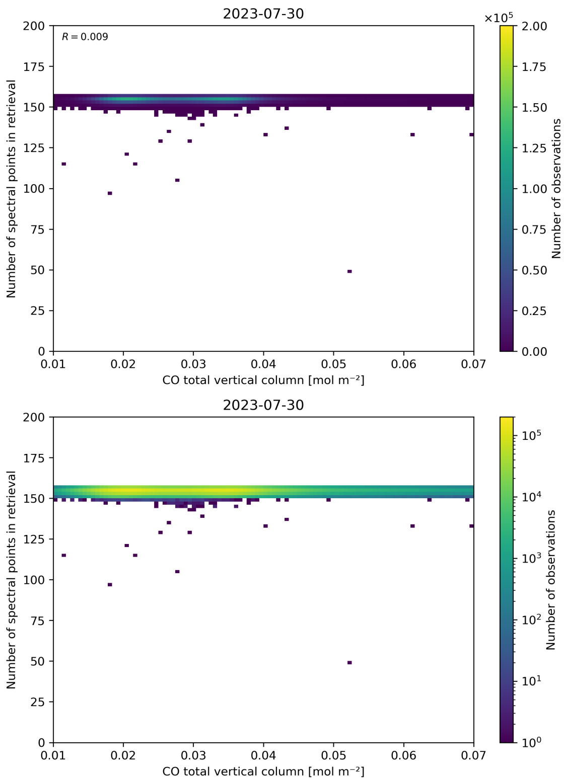
Figure 43: Scatter density plot of “CO total vertical column” against “Number of spectral points in retrieval” for 2023-07-29 to 2023-07-31.
