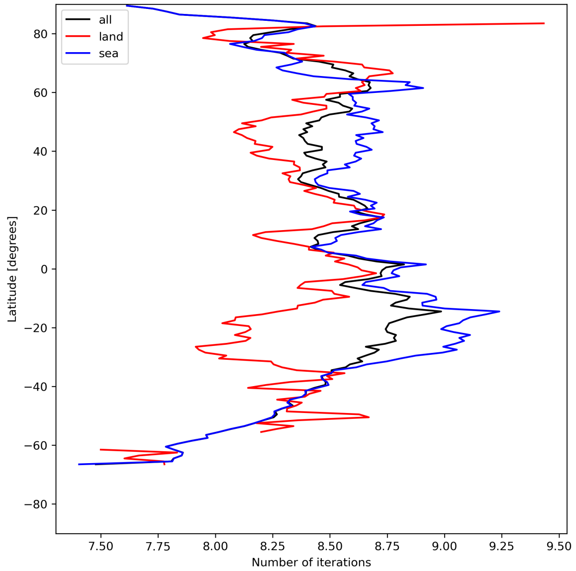
Figure 16: Zonal average of “Number of iterations” for 2023-07-29 to 2023-07-31.
