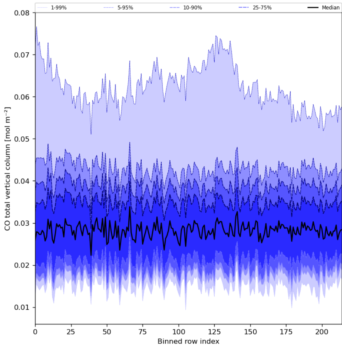
Figure 26: Along track statistics of “CO total vertical column” for 2023-07-29 to 2023-07-31
