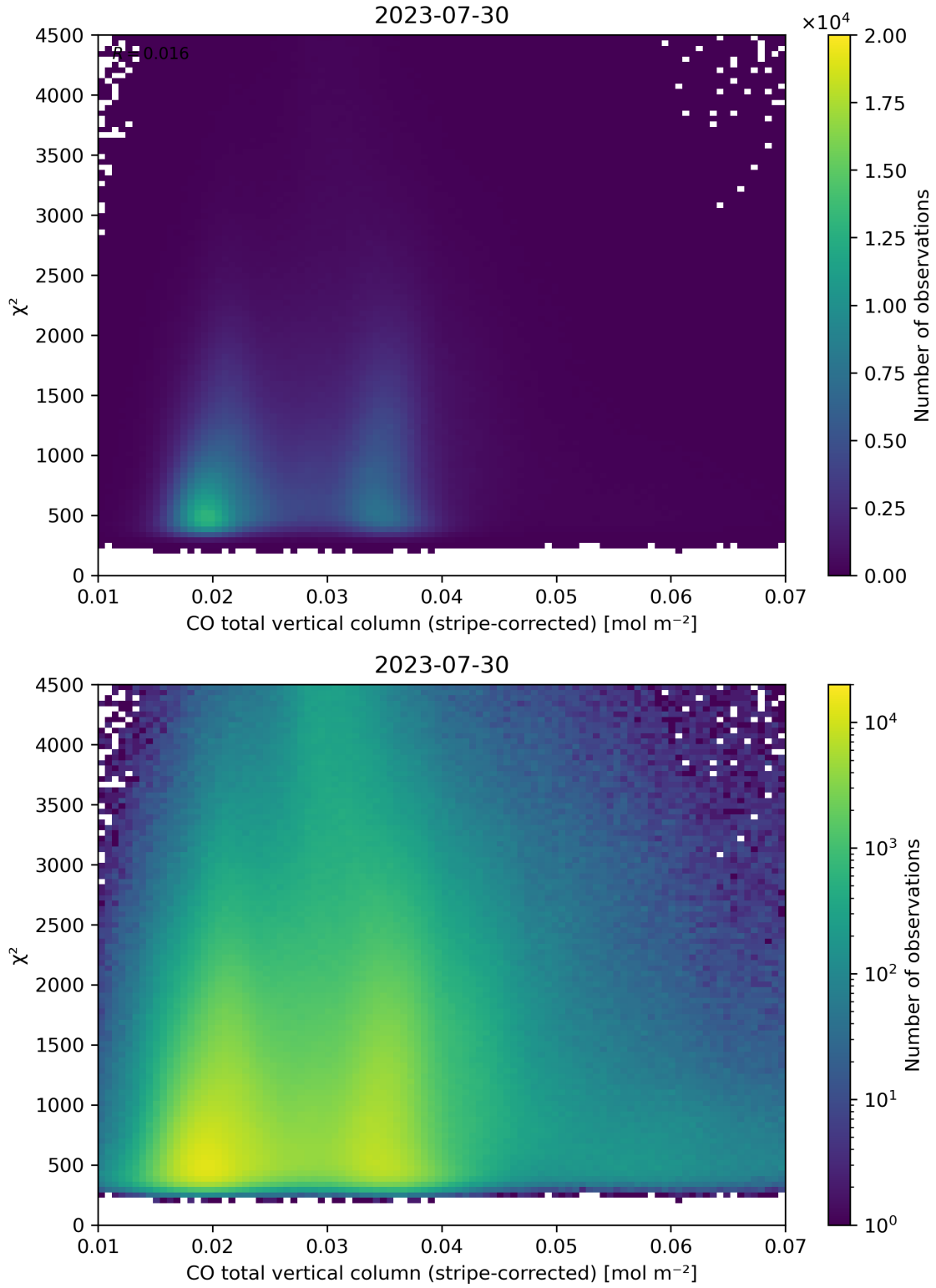
Figure 37: Scatter density plot of “CO total vertical column (stripe-corrected)” against “ \chi^2 ” for 2023-07-29 to 2023-07-31.
