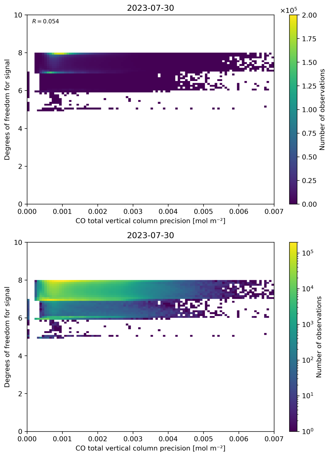
Figure 45: Scatter density plot of “CO total vertical column precision” against “Degrees of freedom for signal” for 2023-07-29 to 2023-07-31.
