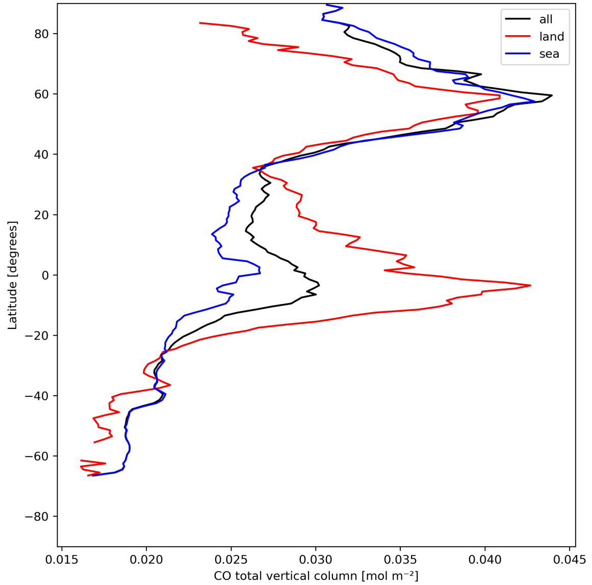
Figure 10: Zonal average of “CO total vertical column” for 2023-07-29 to 2023-07-31.
