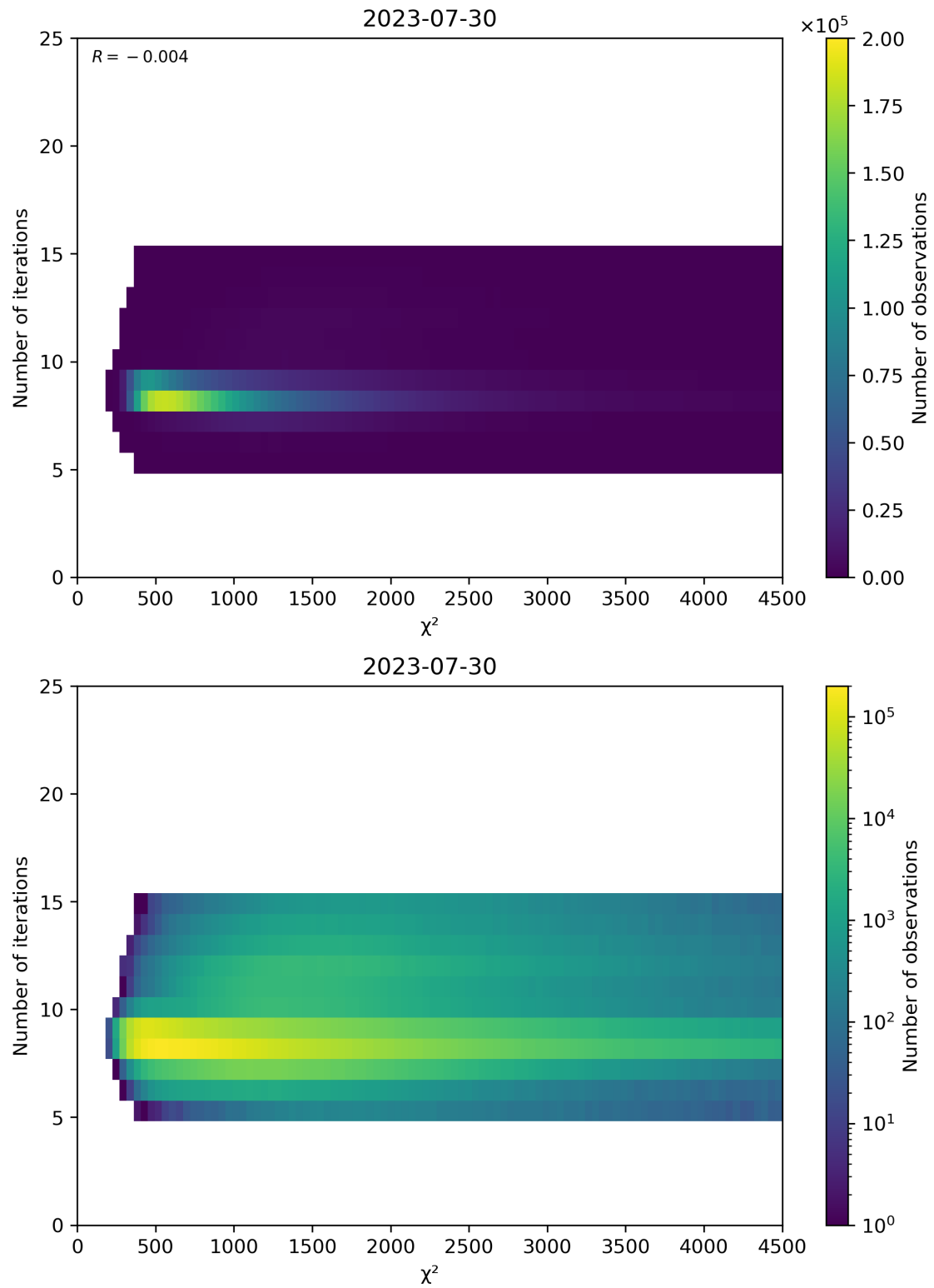
Figure 49: Scatter density plot of “ \chi^2 ” against “Number of iterations” for 2023-07-29 to 2023-07-31.
