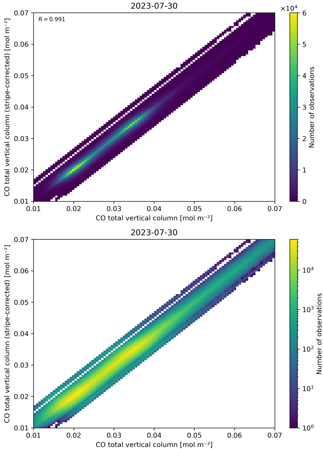
Figure 33: Scatter density plot of “CO total vertical column” against “CO total vertical column (stripe-corrected)” for 2023-07-29 to 2023-07-31.
