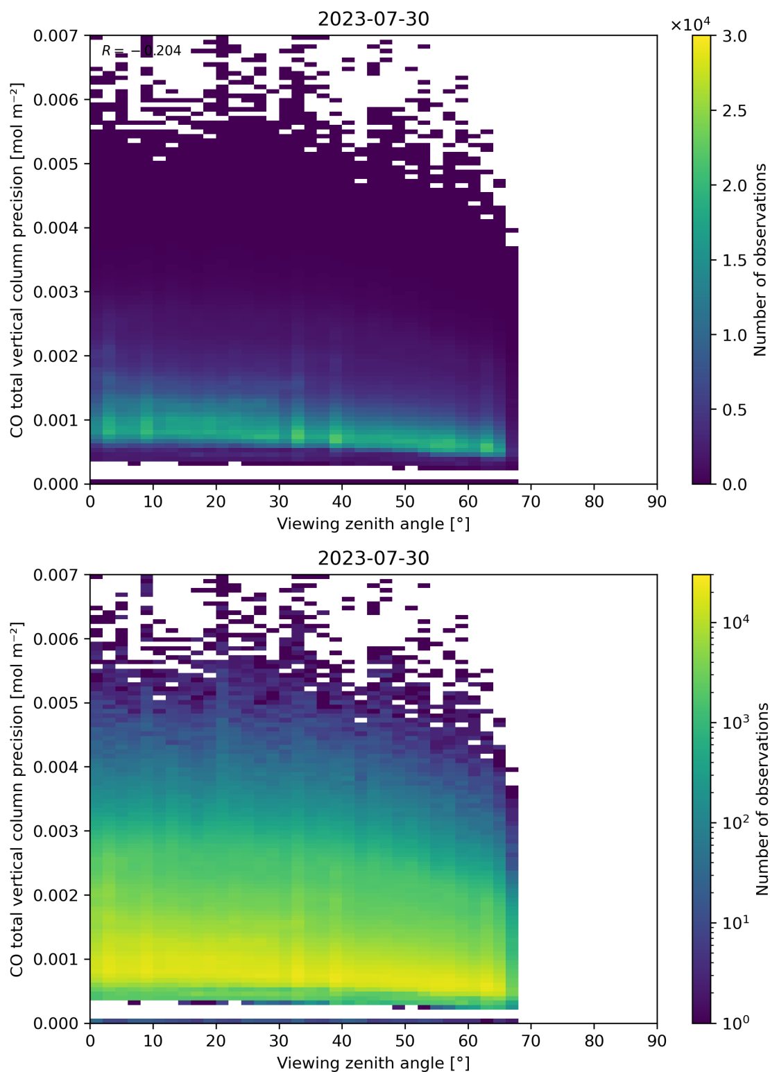
Figure 71: Scatter density plot of “Viewing zenith angle” against “CO total vertical column precision” for 2023-07-29 to 2023-07-31.
