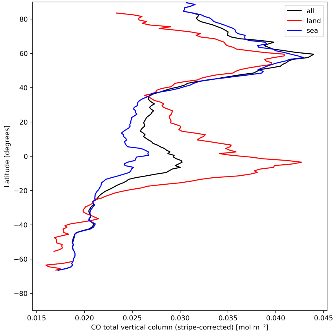
Figure 11: Zonal average of “CO total vertical column (stripe-corrected)” for 2023-07-29 to 2023-07-31.
