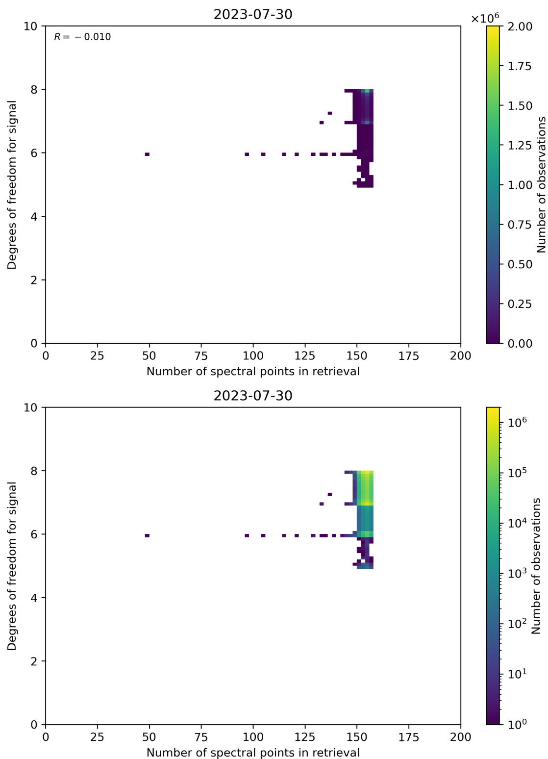
Figure 59: Scatter density plot of “Number of spectral points in retrieval” against “Degrees of freedom for signal” for 2023-07-29 to 2023-07-31.
