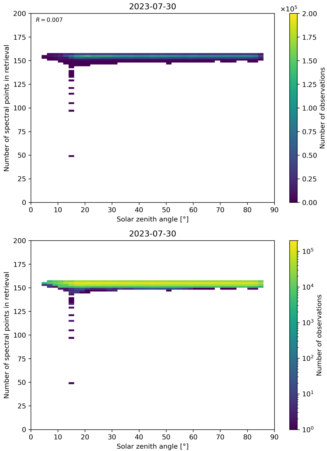
Figure 68: Scatter density plot of “Solar zenith angle” against “Number of spectral points in retrieval” for 2023-07-29 to 2023-07-31.
