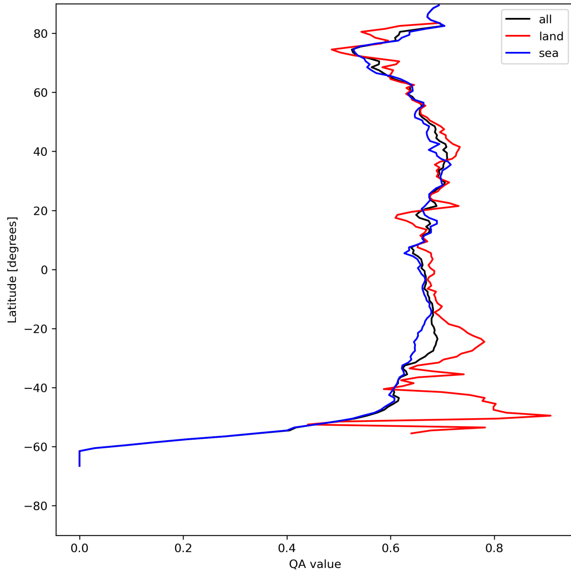
Figure 9: Zonal average of “QA value” for 2023-07-29 to 2023-07-31.
