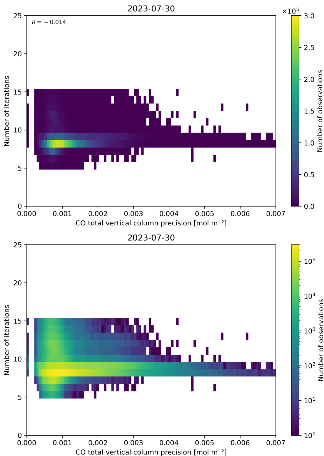
Figure 46: Scatter density plot of “CO total vertical column precision” against “Number of iterations” for 2023-07-29 to 2023-07-31.
