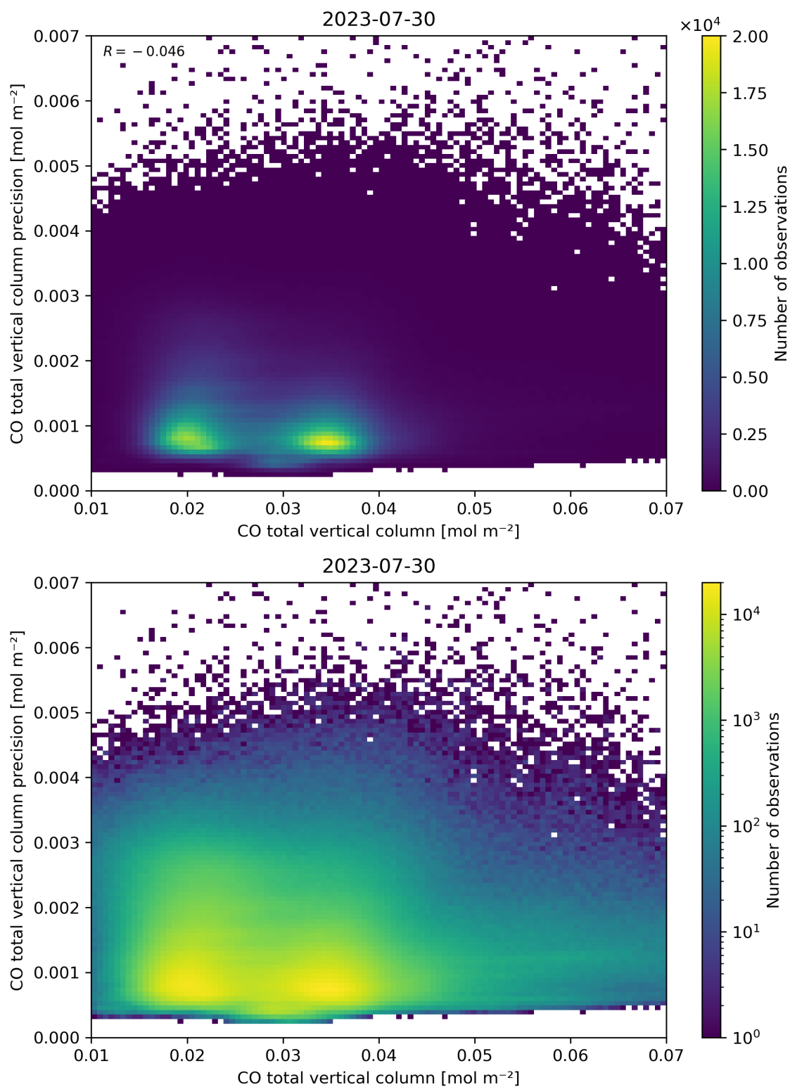
Figure 34: Scatter density plot of “CO total vertical column” against “CO total vertical column precision” for 2023-07-29 to 2023-07-31.
