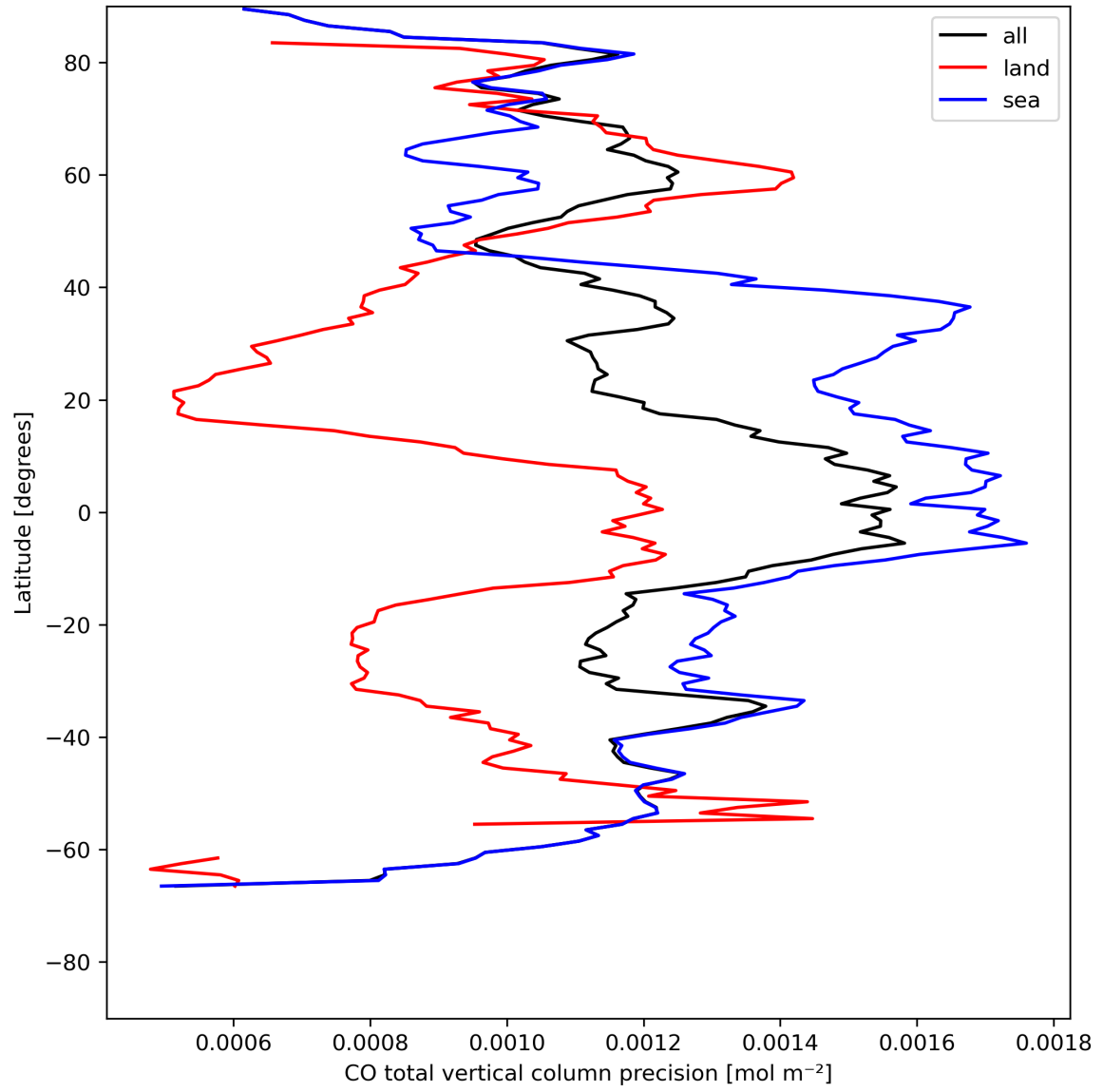
Figure 12: Zonal average of “CO total vertical column precision” for 2023-07-29 to 2023-07-31.
