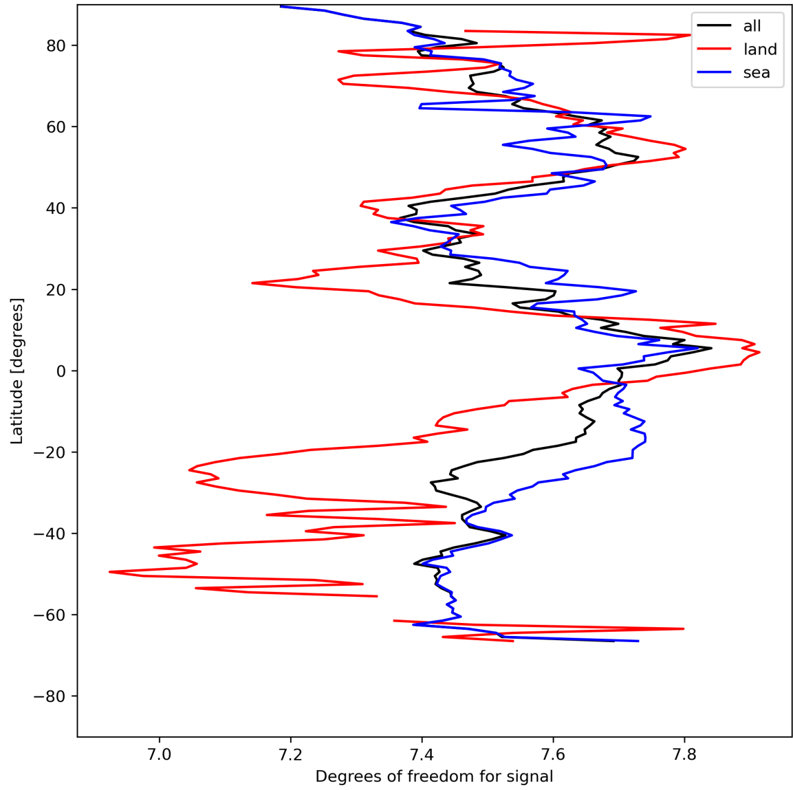
Figure 15: Zonal average of “Degrees of freedom for signal” for 2023-07-29 to 2023-07-31.
