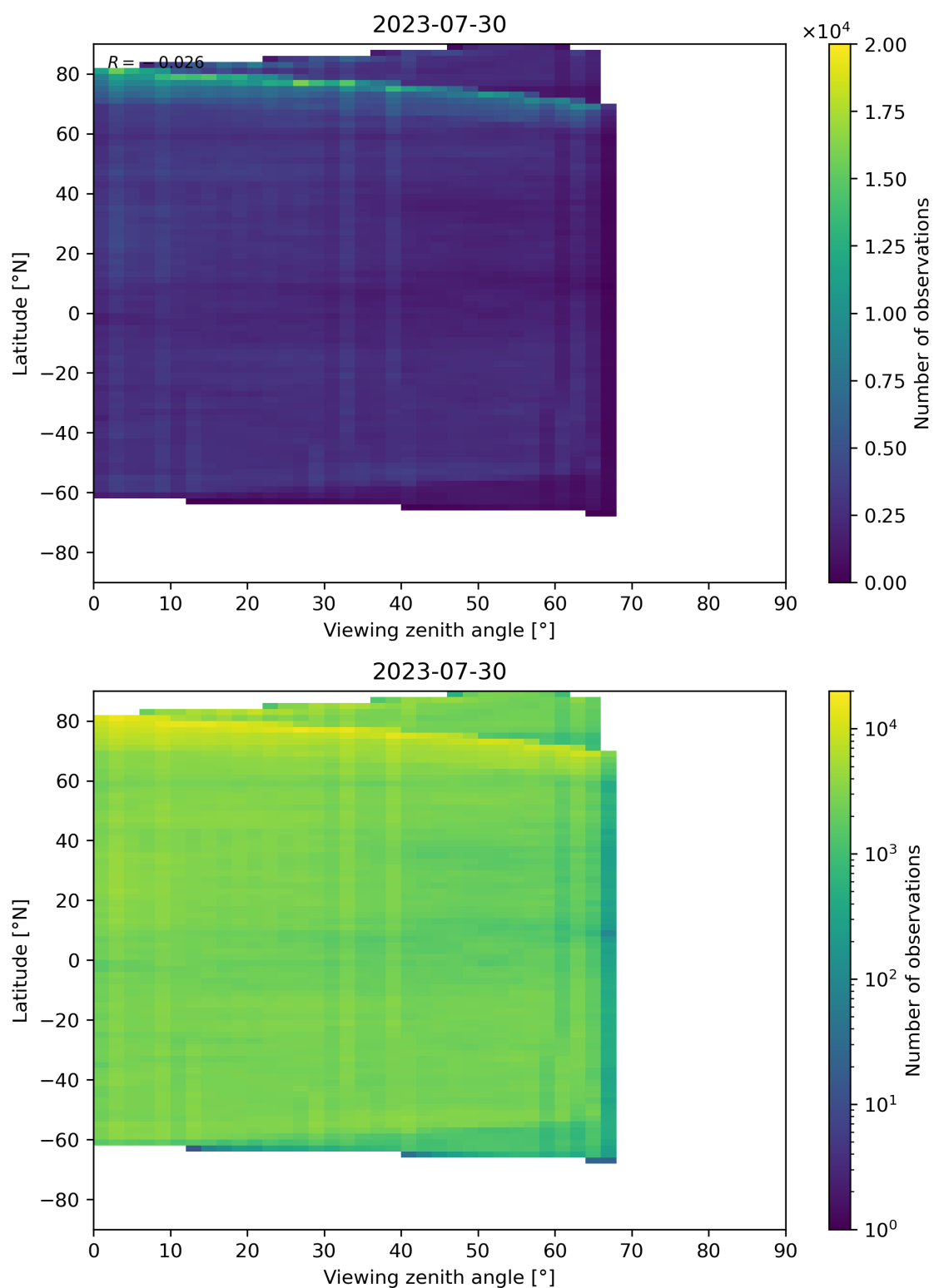
Figure 74: Scatter density plot of “Viewing zenith angle” against “Latitude” for 2023-07-29 to 2023-07-31.
