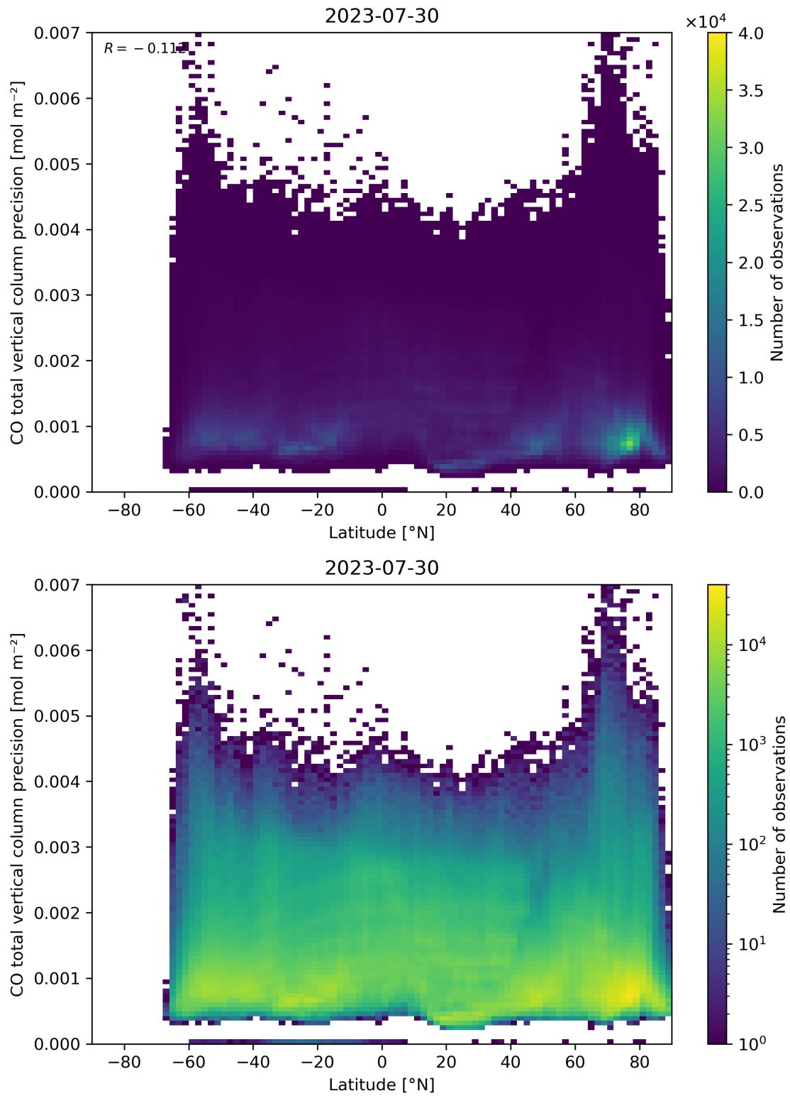
Figure 53: Scatter density plot of “Latitude” against “CO total vertical column precision” for 2023-07-29 to 2023-07-31.
