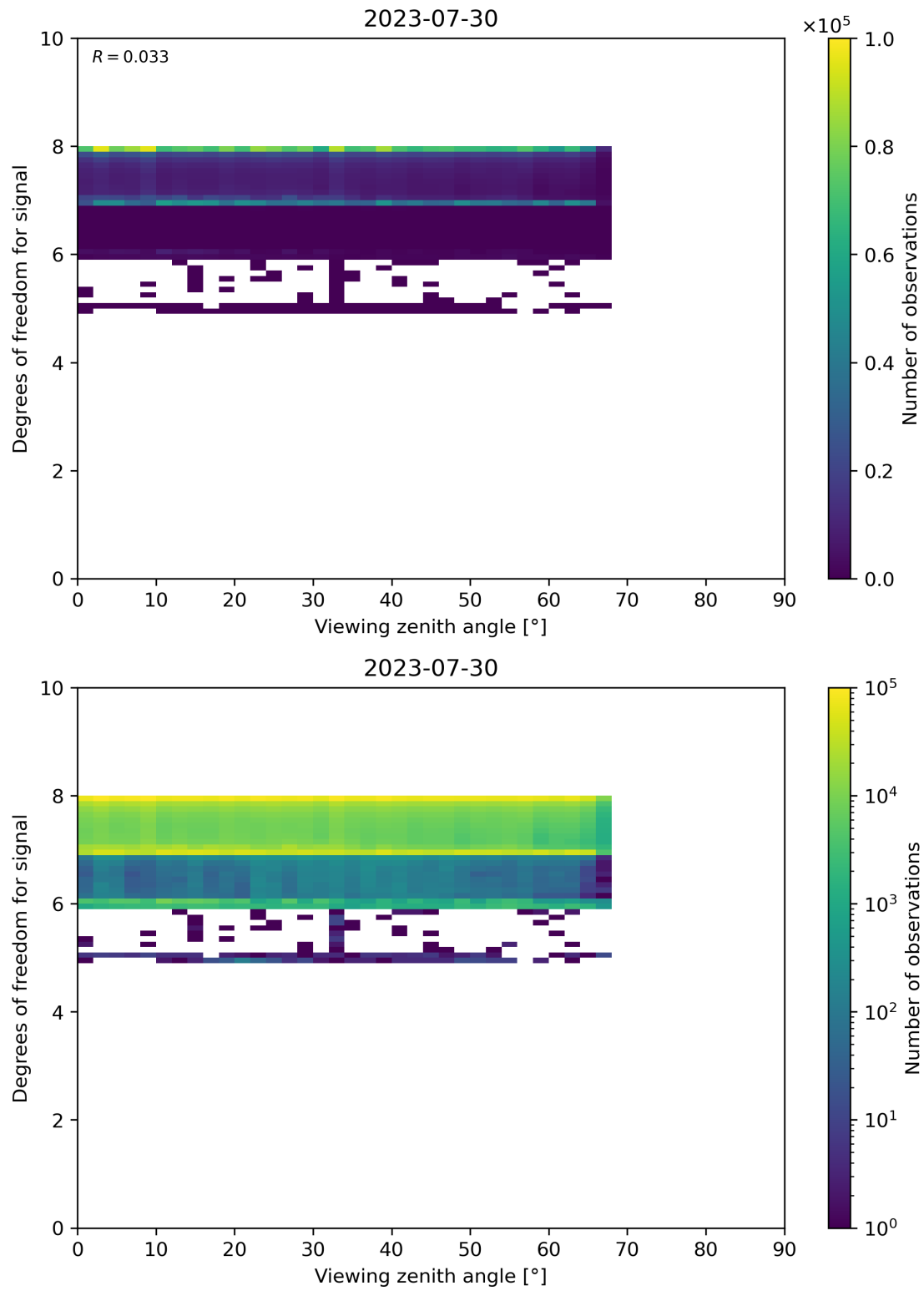
Figure 73: Scatter density plot of “Viewing zenith angle” against “Degrees of freedom for signal” for 2023-07-29 to 2023-07-31.
