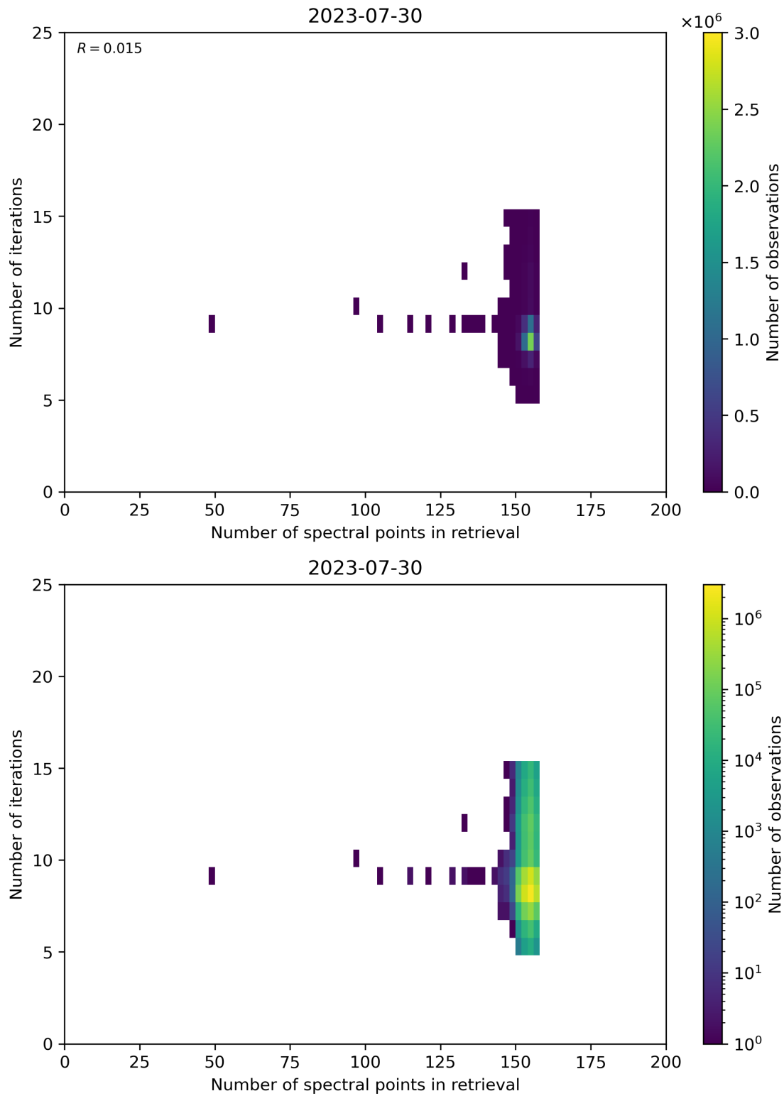
Figure 60: Scatter density plot of “Number of spectral points in retrieval” against “Number of iterations” for 2023-07-29 to 2023-07-31.
