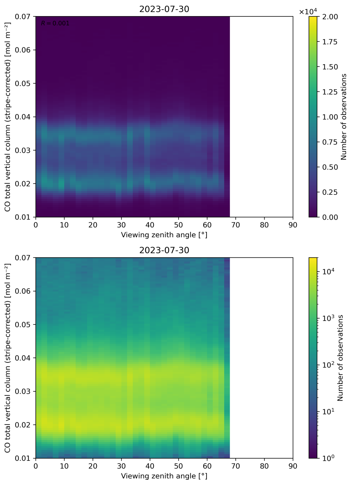
Figure 70: Scatter density plot of “Viewing zenith angle” against “CO total vertical column (stripe-corrected)” for 2023-07-29 to 2023-07-31.
