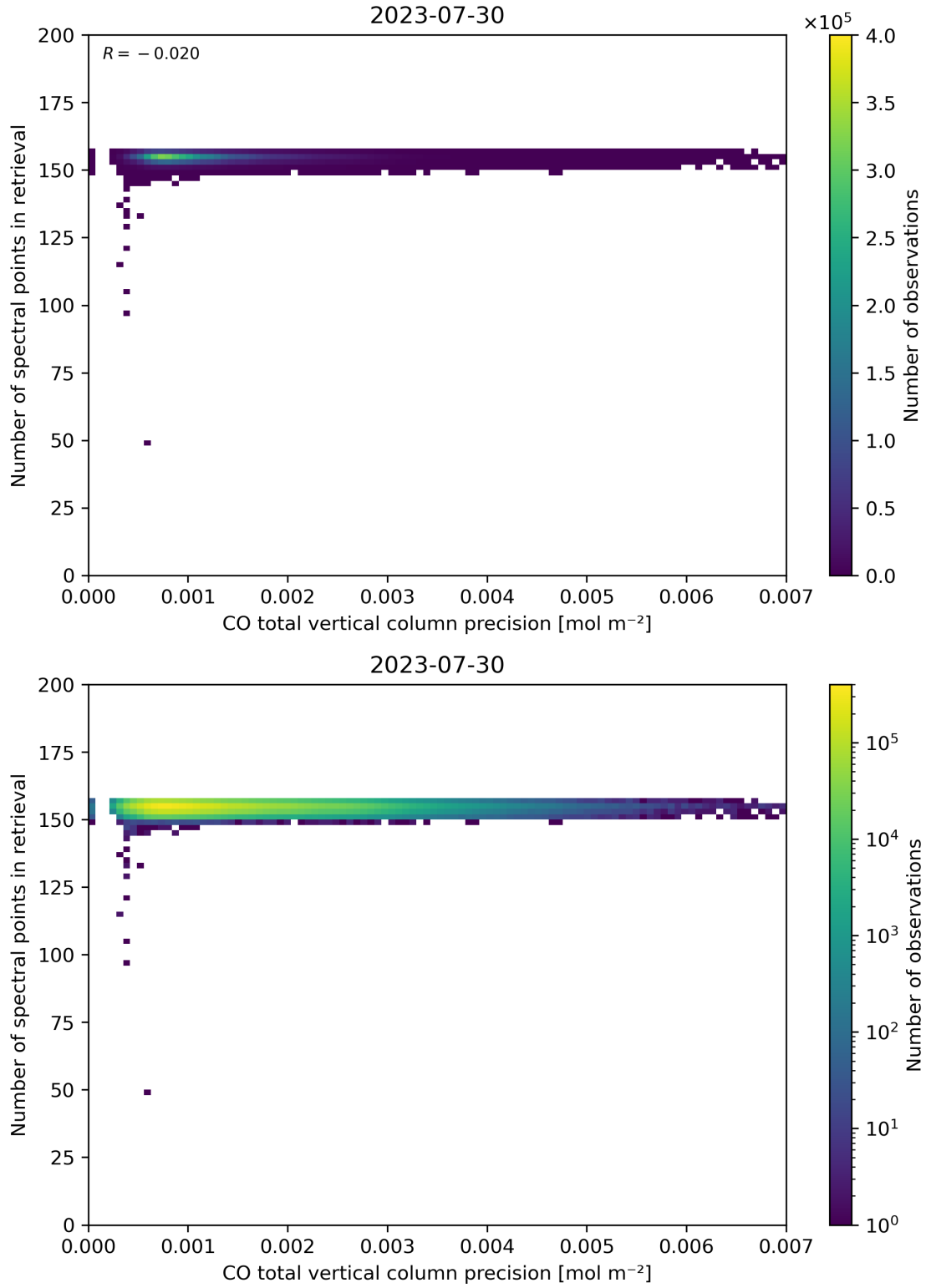
Figure 47: Scatter density plot of “CO total vertical column precision” against “Number of spectral points in retrieval” for 2023-07-29 to 2023-07-31.
