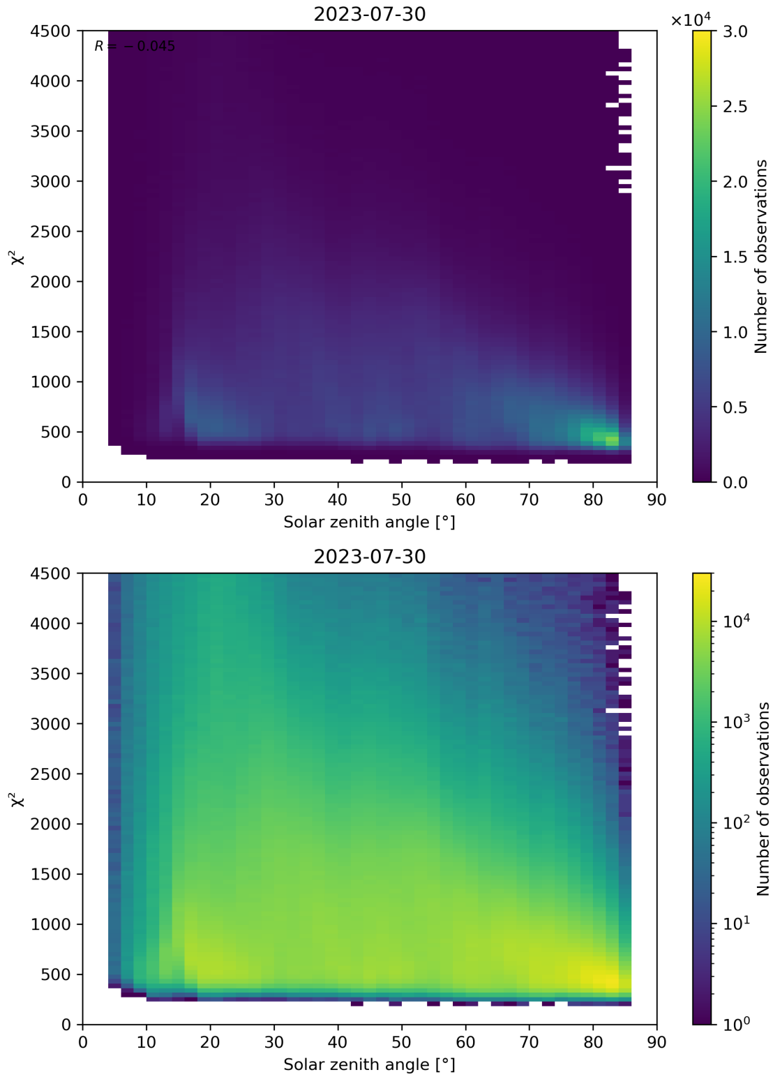
Figure 64: Scatter density plot of “Solar zenith angle” against “ \chi^2 ” for 2023-07-29 to 2023-07-31.
