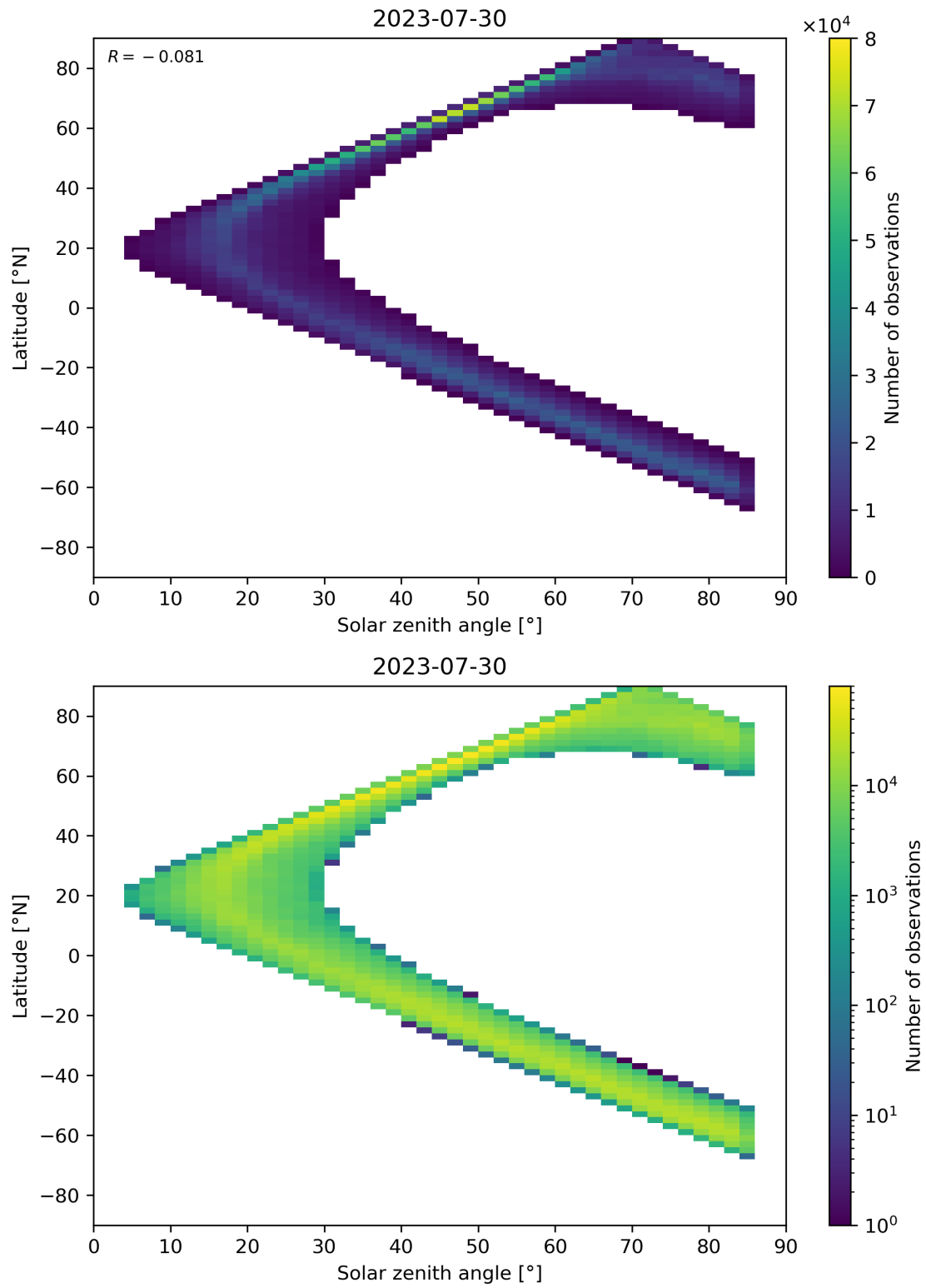
Figure 66: Scatter density plot of “Solar zenith angle” against “Latitude” for 2023-07-29 to 2023-07-31.
