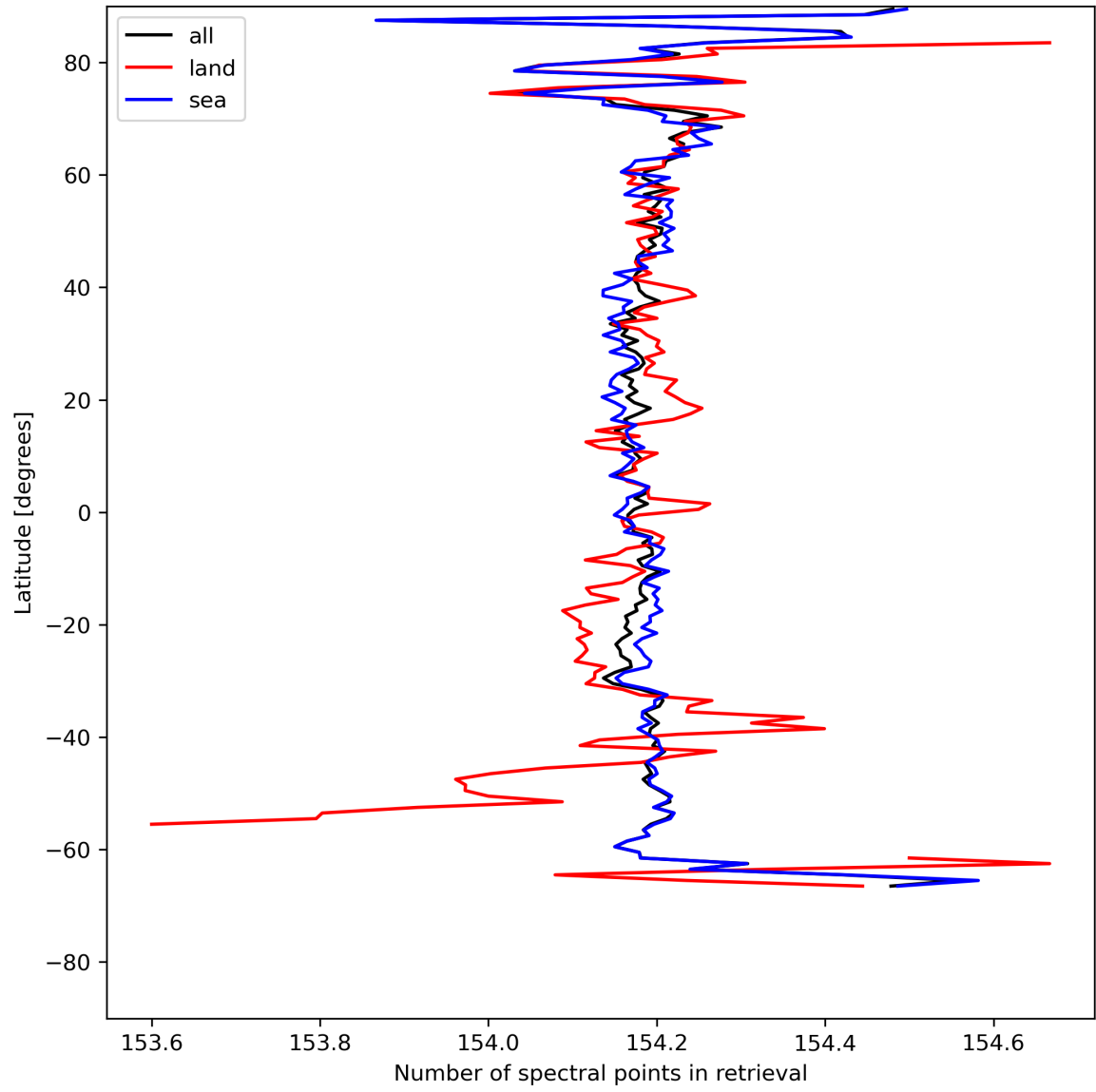
Figure 13: Zonal average of “Number of spectral points in retrieval” for 2023-07-29 to 2023-07-31.
