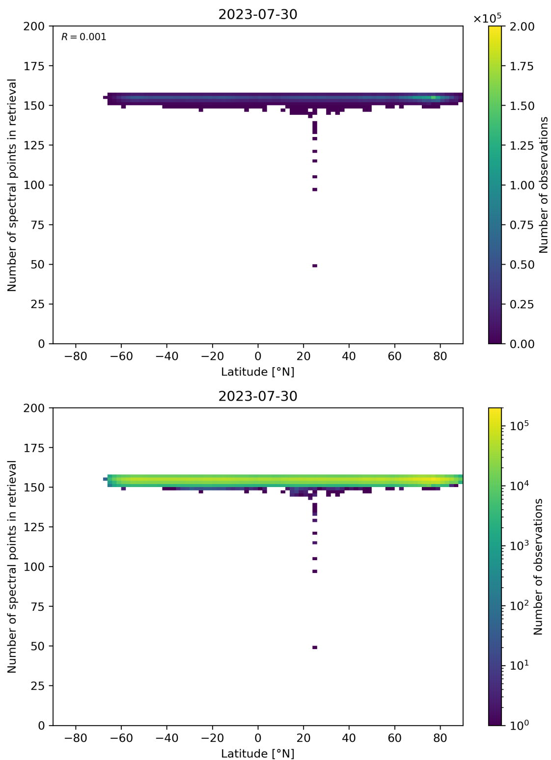
Figure 57: Scatter density plot of “Latitude” against “Number of spectral points in retrieval” for 2023-07-29 to 2023-07-31.
