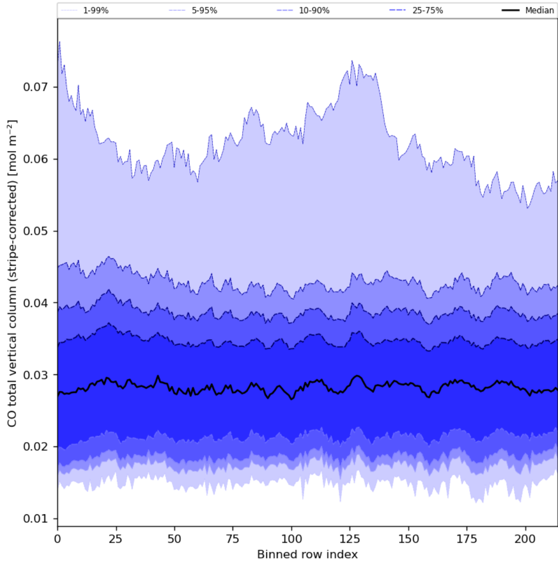
Figure 27: Along track statistics of “CO total vertical column (stripe-corrected)” for 2023-07-29 to 2023-07-31
