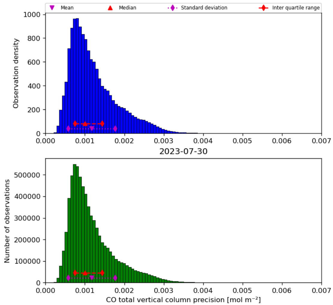
Figure 20: Histogram of “CO total vertical column precision” for 2023-07-29 to 2023-07-31
