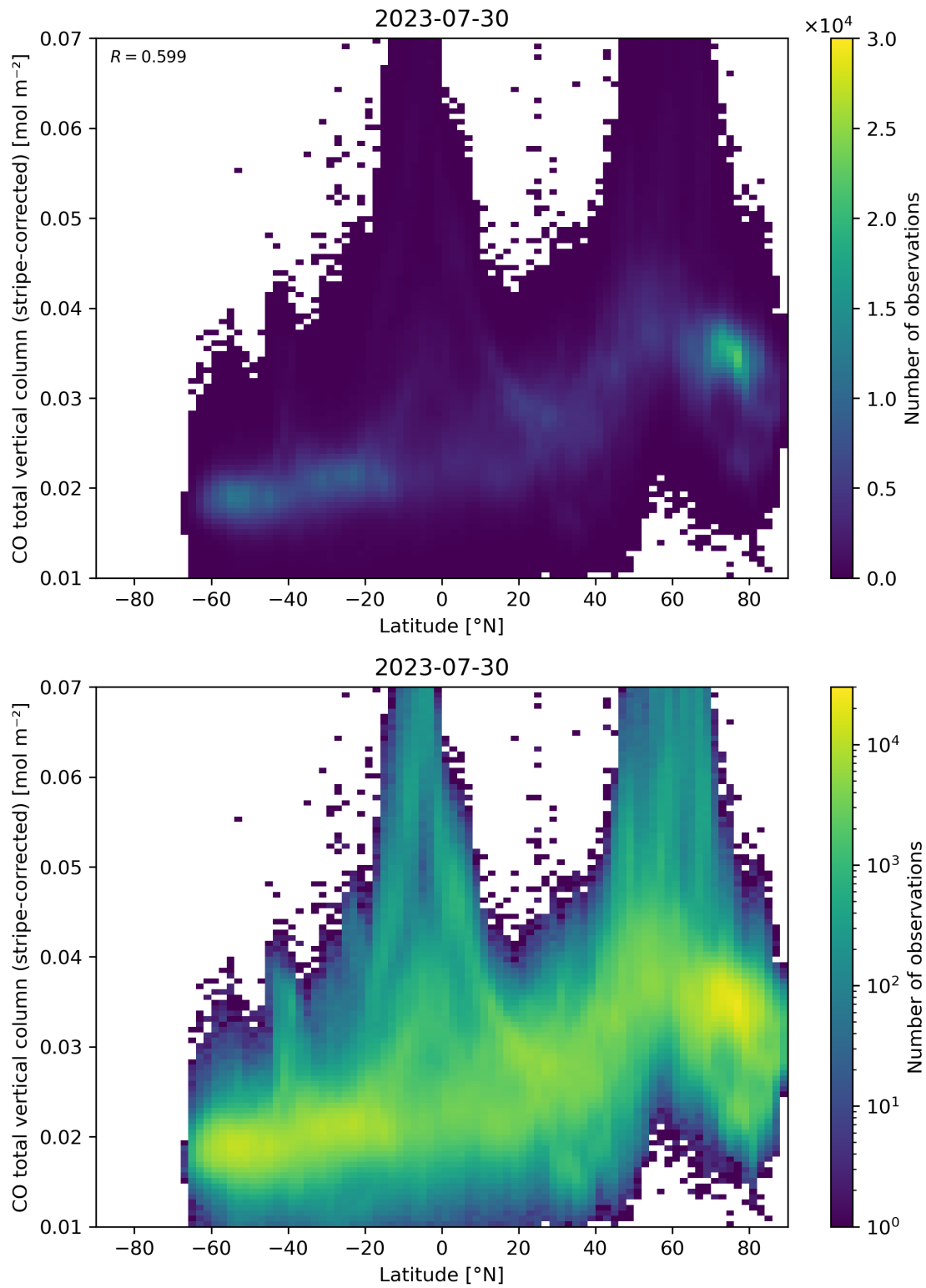
Figure 52: Scatter density plot of “Latitude” against “CO total vertical column (stripe-corrected)” for 2023-07-29 to 2023-07-31.
