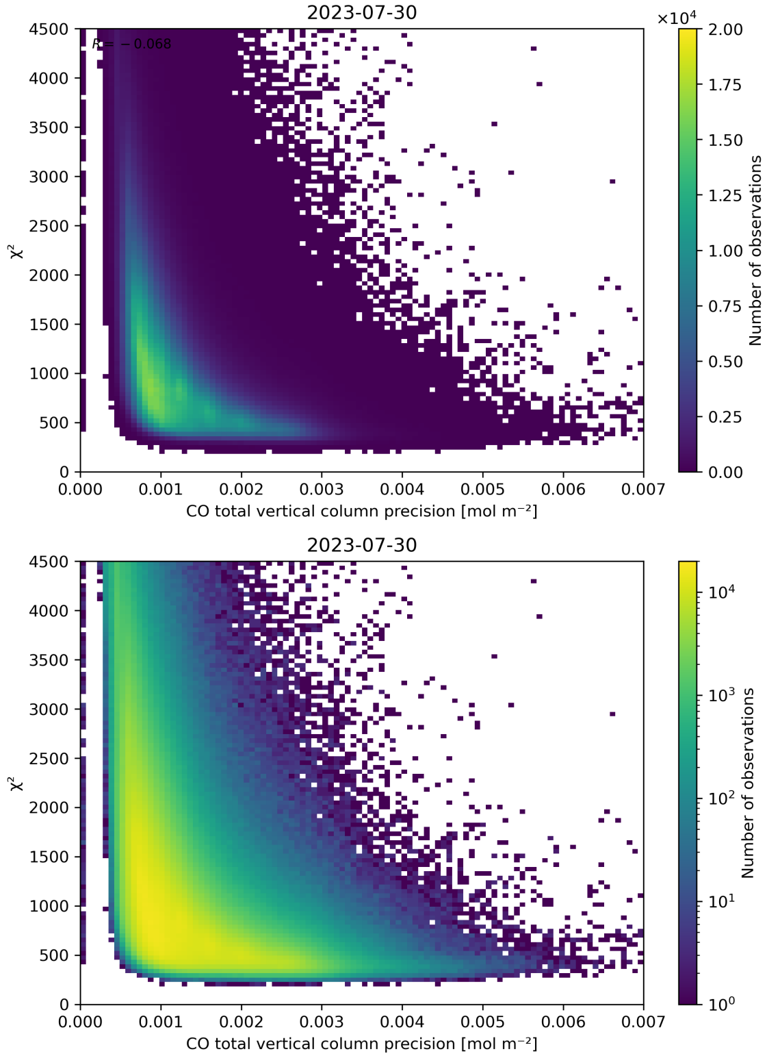
Figure 44: Scatter density plot of “CO total vertical column precision” against “ \chi^2 ” for 2023-07-29 to 2023-07-31.
