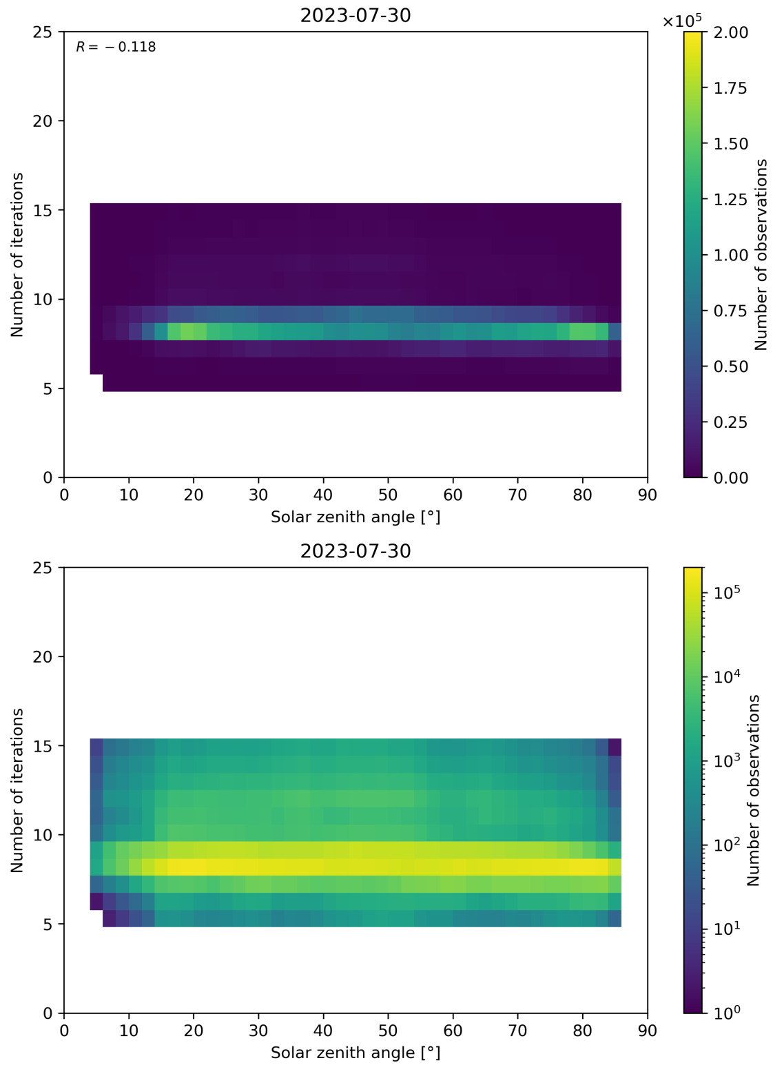
Figure 67: Scatter density plot of “Solar zenith angle” against “Number of iterations” for 2023-07-29 to 2023-07-31.
