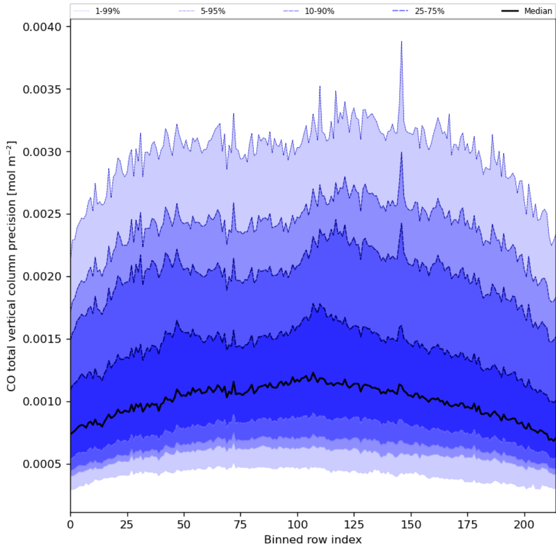
Figure 28: Along track statistics of “CO total vertical column precision” for 2023-07-29 to 2023-07-31
