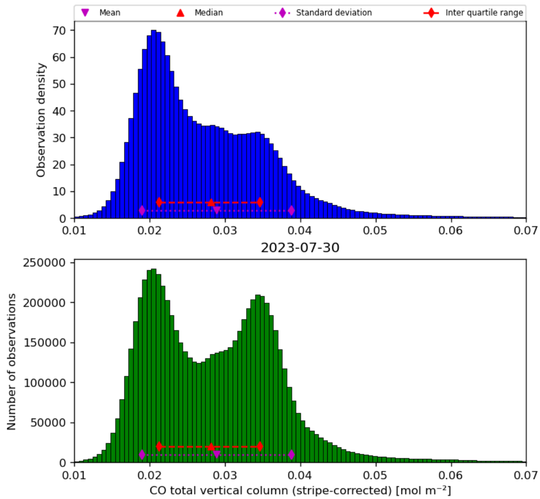
Figure 19: Histogram of “CO total vertical column (stripe-corrected)” for 2023-07-29 to 2023-07-31
