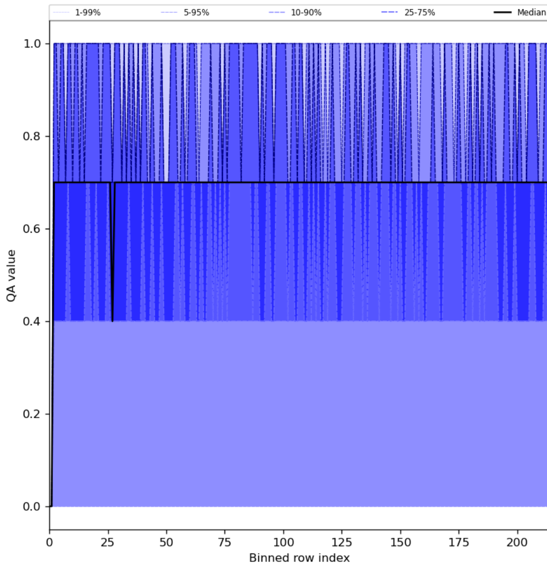
Figure 25: Along track statistics of “QA value” for 2023-07-29 to 2023-07-31
