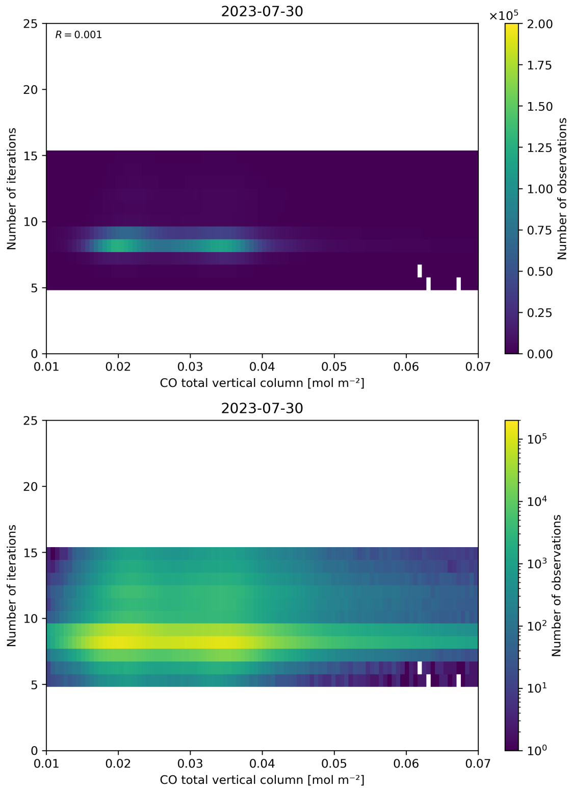
Figure 42: Scatter density plot of “CO total vertical column” against “Number of iterations” for 2023-07-29 to 2023-07-31.
