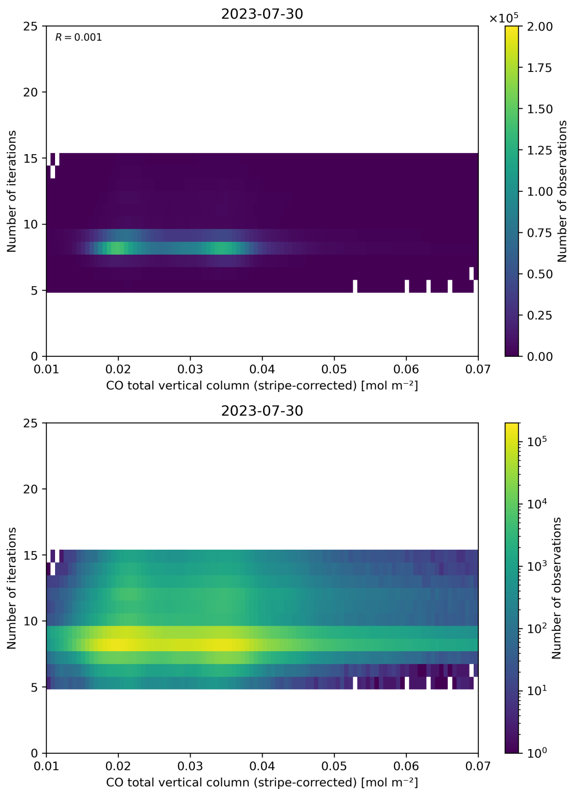
Figure 39: Scatter density plot of “CO total vertical column (stripe-corrected)” against “Number of iterations” for 2023-07-29 to 2023-07-31.
