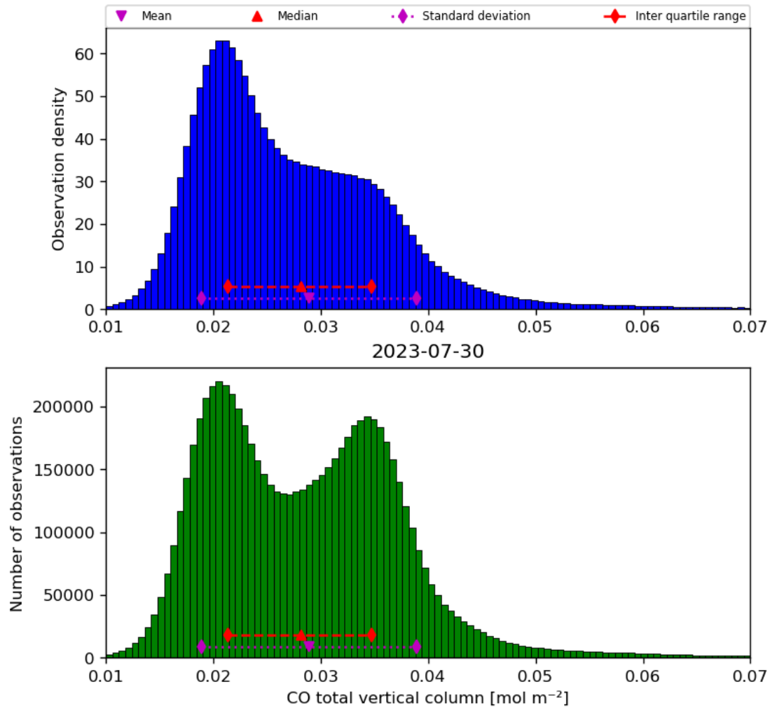
Figure 18: Histogram of “CO total vertical column” for 2023-07-29 to 2023-07-31
