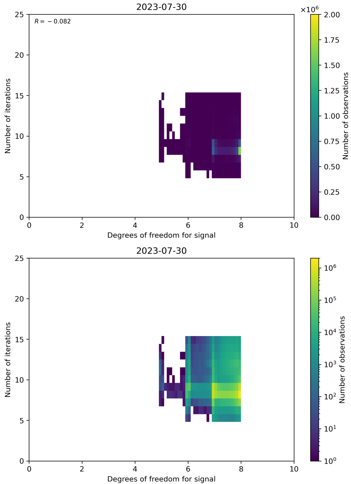
Figure 50: Scatter density plot of “Degrees of freedom for signal” against “Number of iterations” for 2023-07-29 to 2023-07-31.
