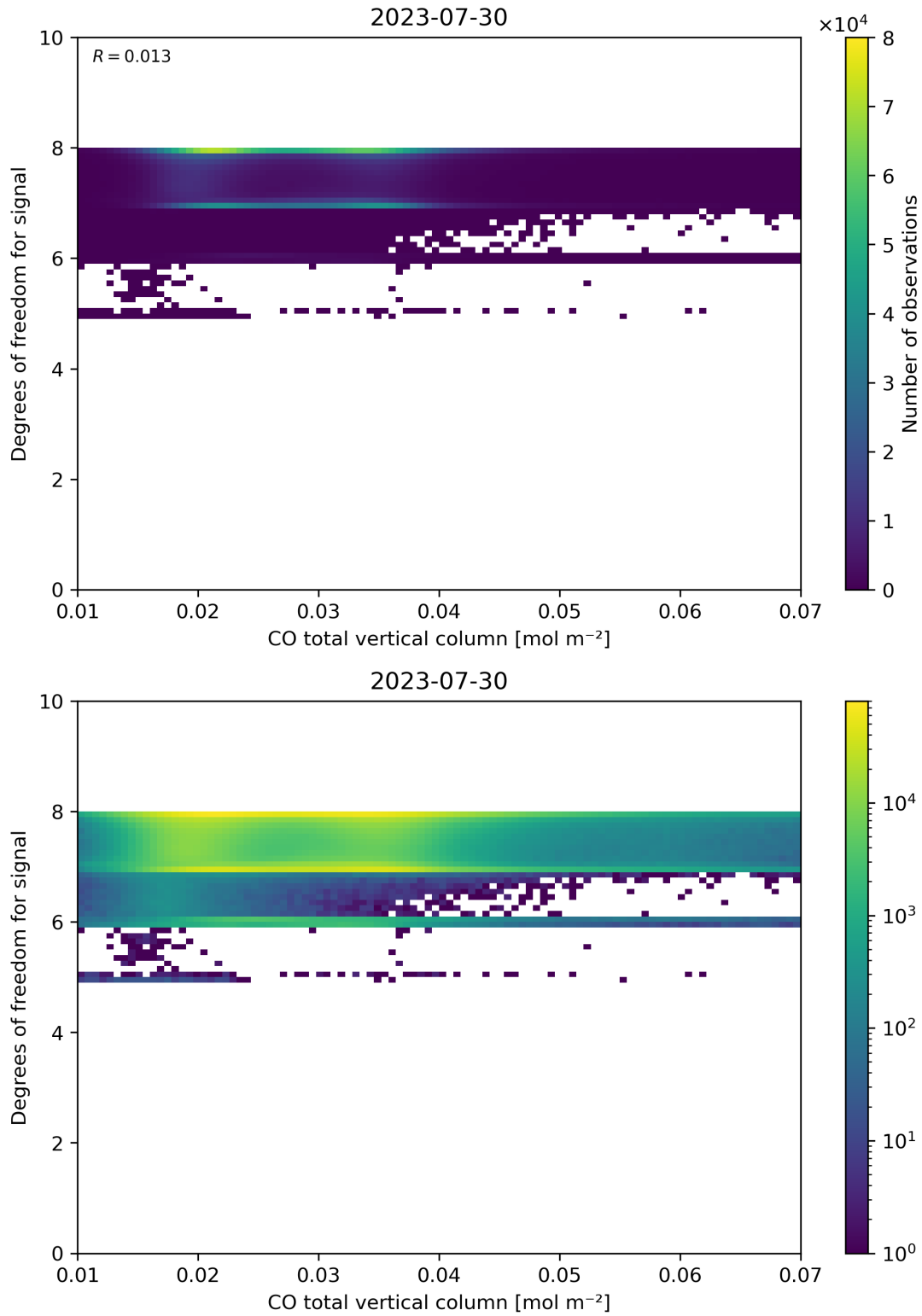
Figure 41: Scatter density plot of “CO total vertical column” against “Degrees of freedom for signal” for 2023-07-29 to 2023-07-31.
