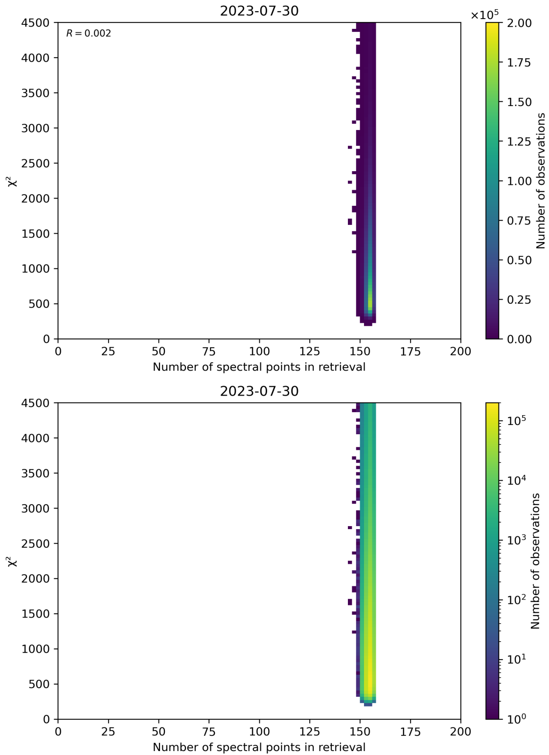
Figure 58: Scatter density plot of “Number of spectral points in retrieval” against “ \chi^2 ” for 2023-07-29 to 2023-07-31.
