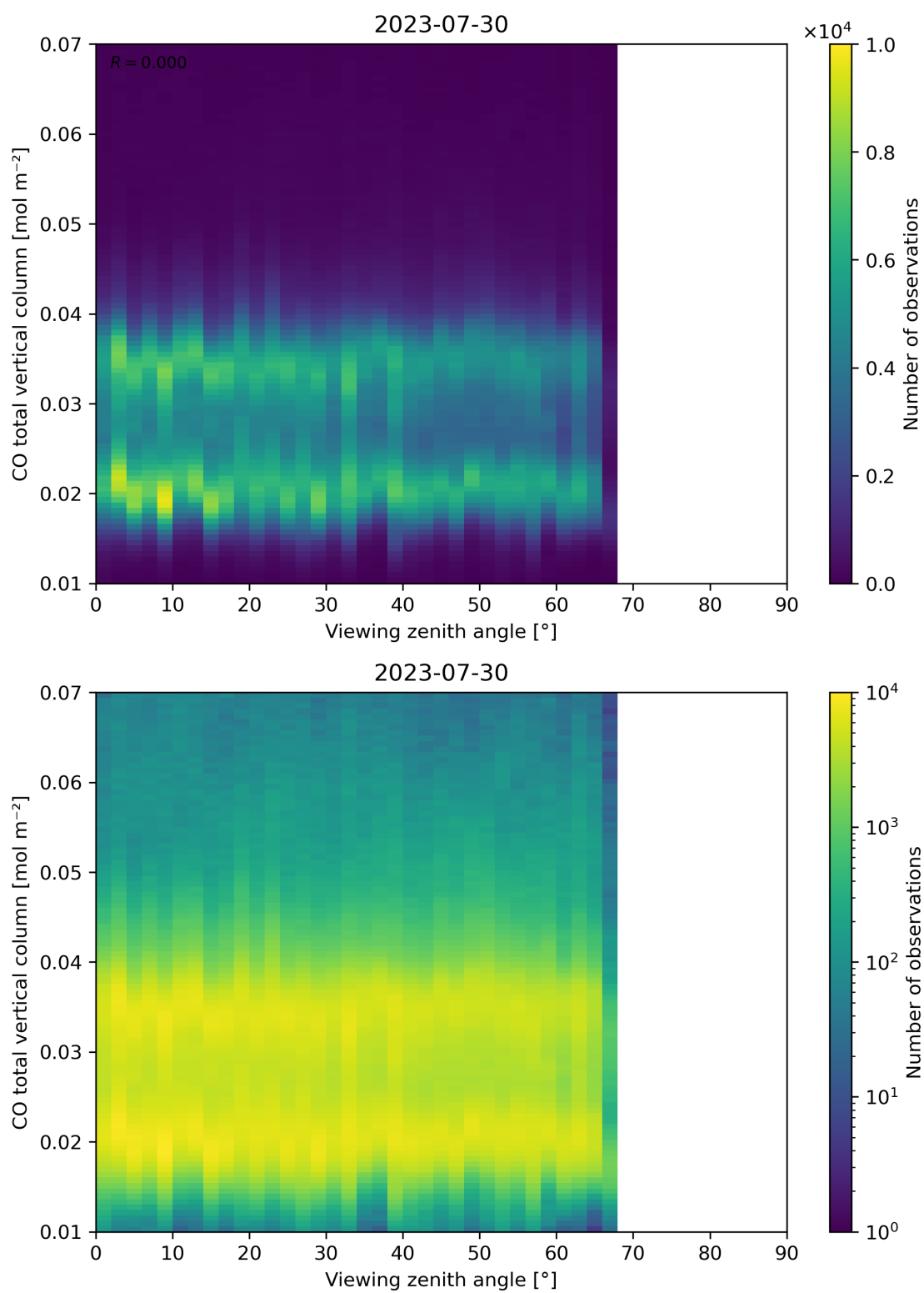
Figure 69: Scatter density plot of “Viewing zenith angle” against “CO total vertical column” for 2023-07-29 to 2023-07-31.
