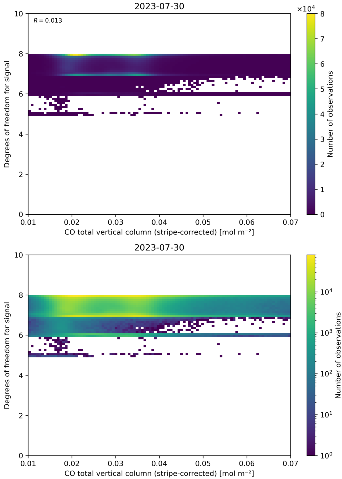
Figure 38: Scatter density plot of “CO total vertical column (stripe-corrected)” against “Degrees of freedom for signal” for 2023-07-29 to 2023-07-31.
