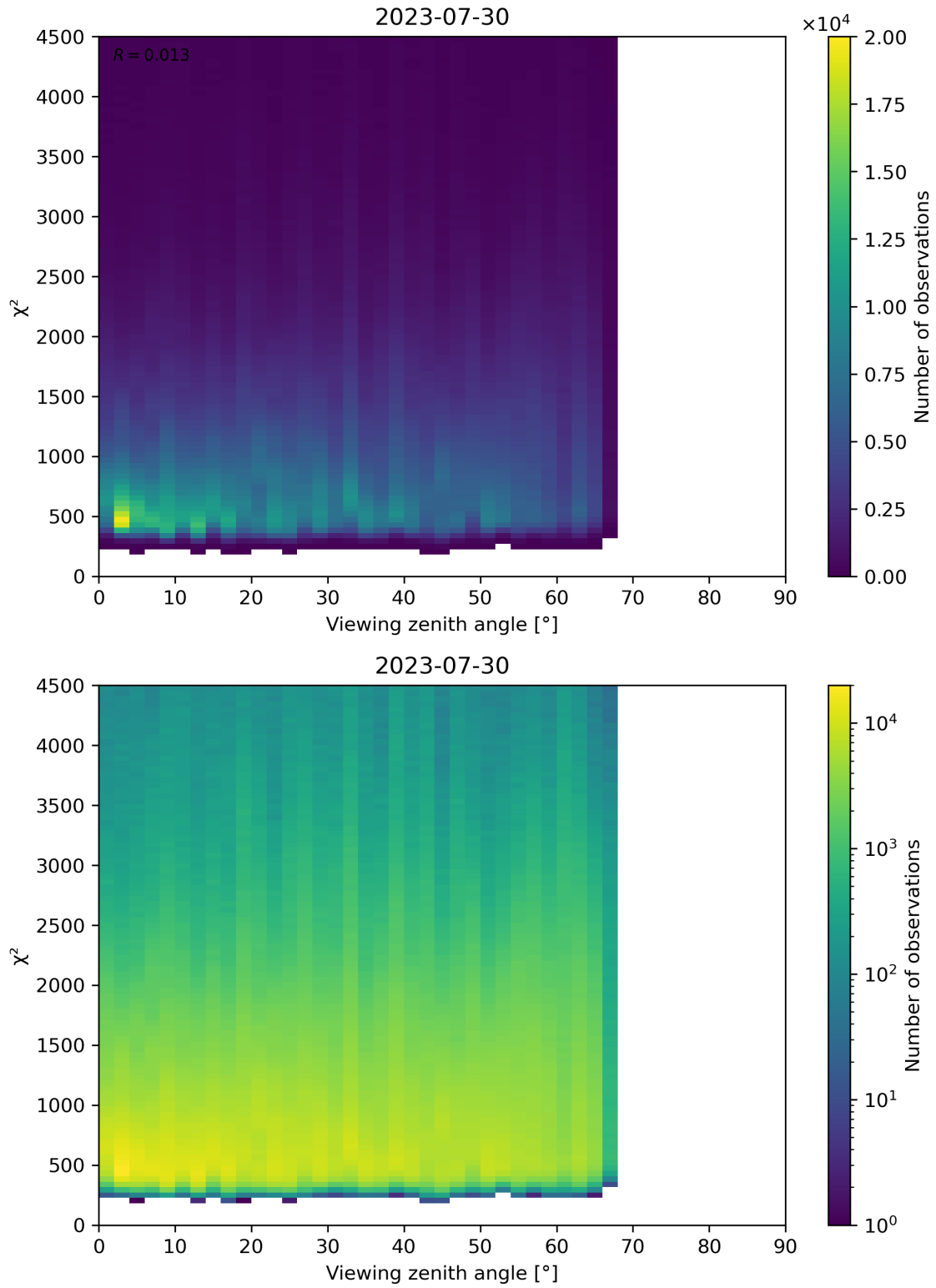
Figure 72: Scatter density plot of “Viewing zenith angle” against “ \chi^2 ” for 2023-07-29 to 2023-07-31.
