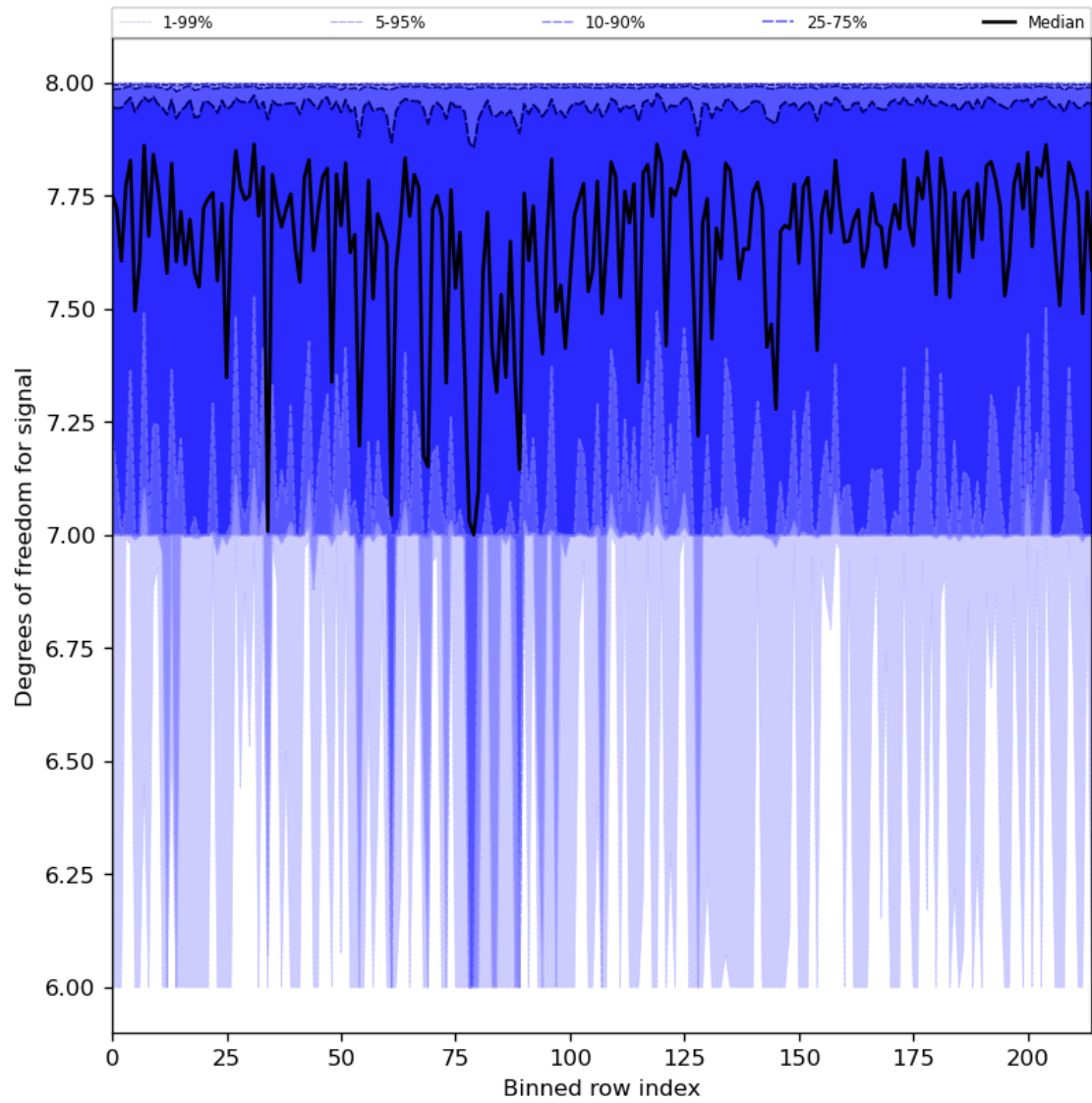
Figure 31: Along track statistics of “Degrees of freedom for signal” for 2023-07-29 to 2023-07-31
