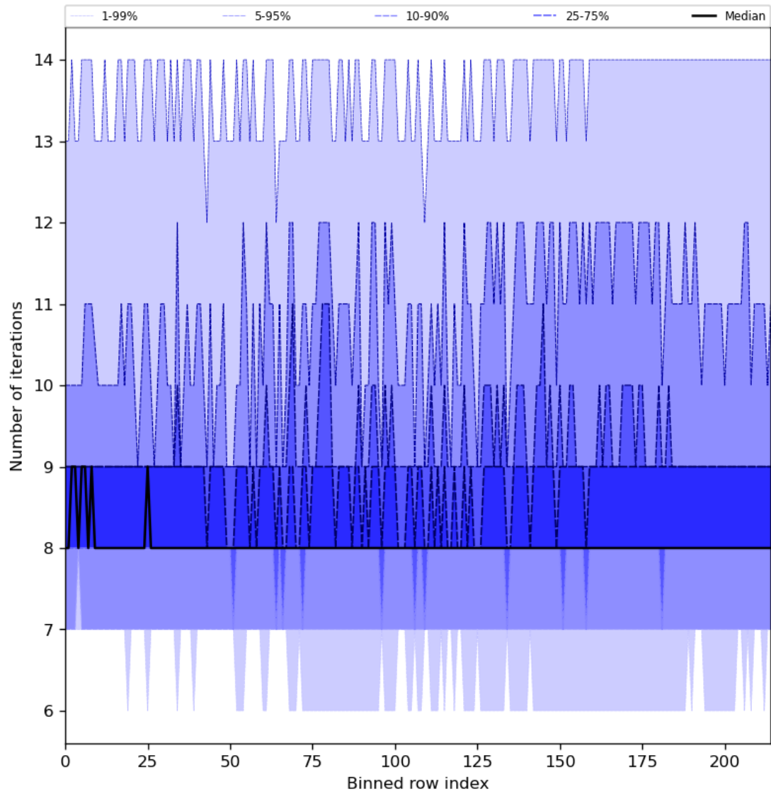
Figure 32: Along track statistics of “Number of iterations” for 2023-07-29 to 2023-07-31
