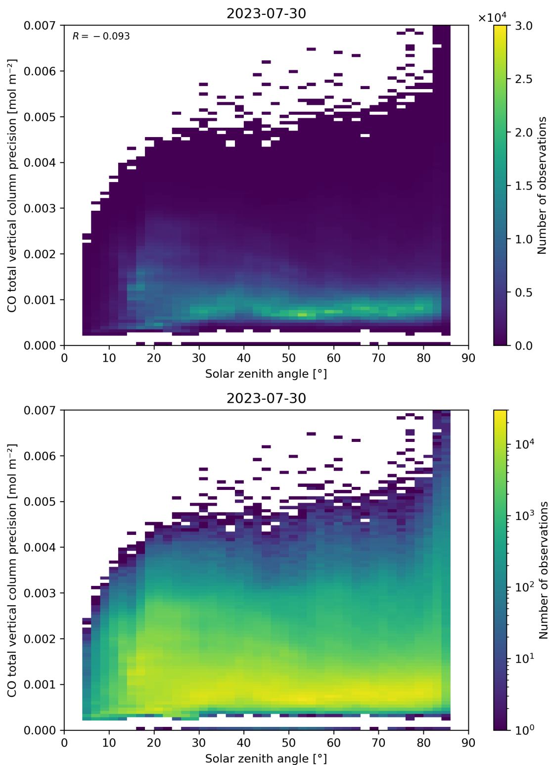
Figure 63: Scatter density plot of “Solar zenith angle” against “CO total vertical column precision” for 2023-07-29 to 2023-07-31.
