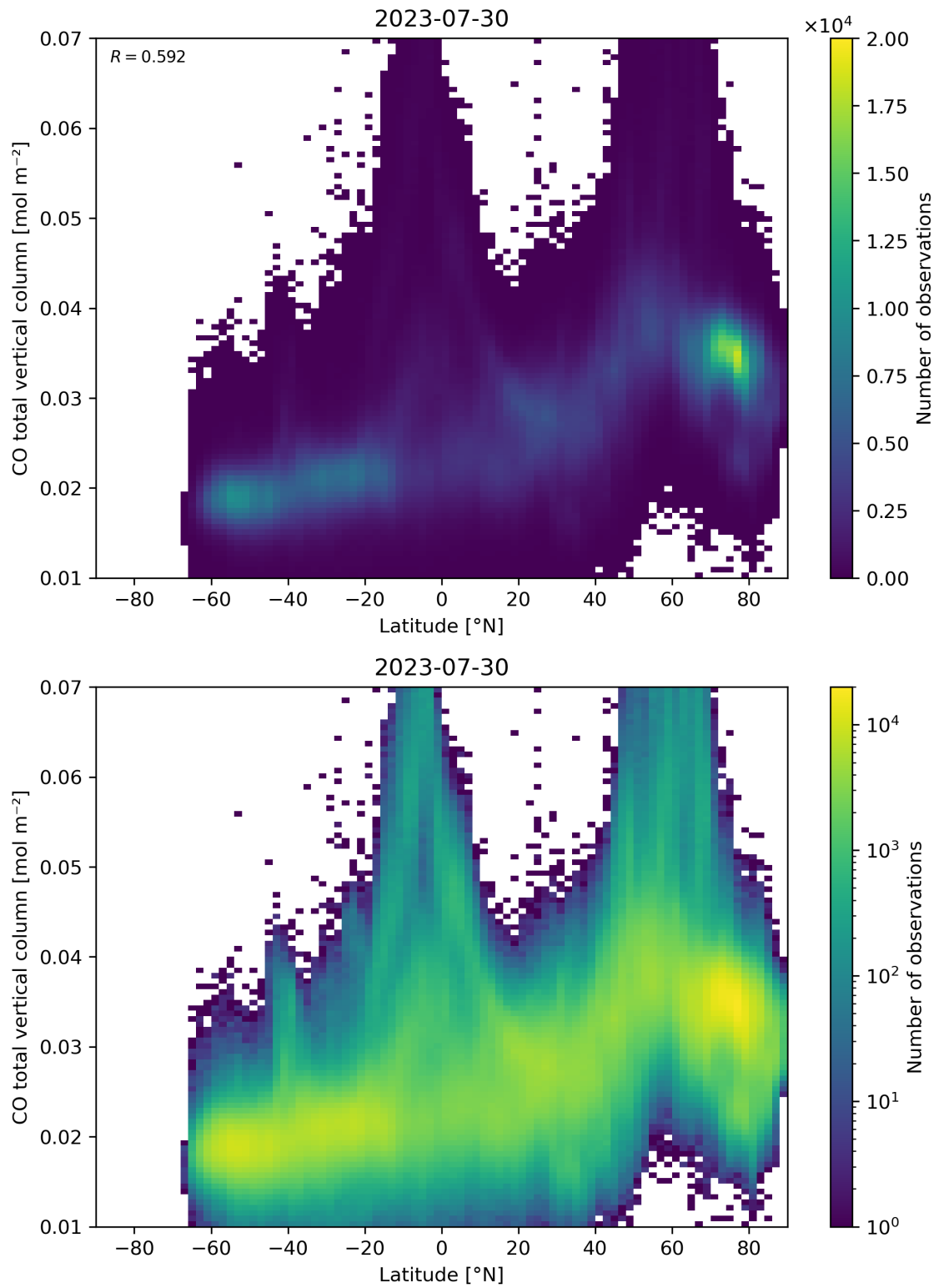
Figure 51: Scatter density plot of “Latitude” against “CO total vertical column” for 2023-07-29 to 2023-07-31.
