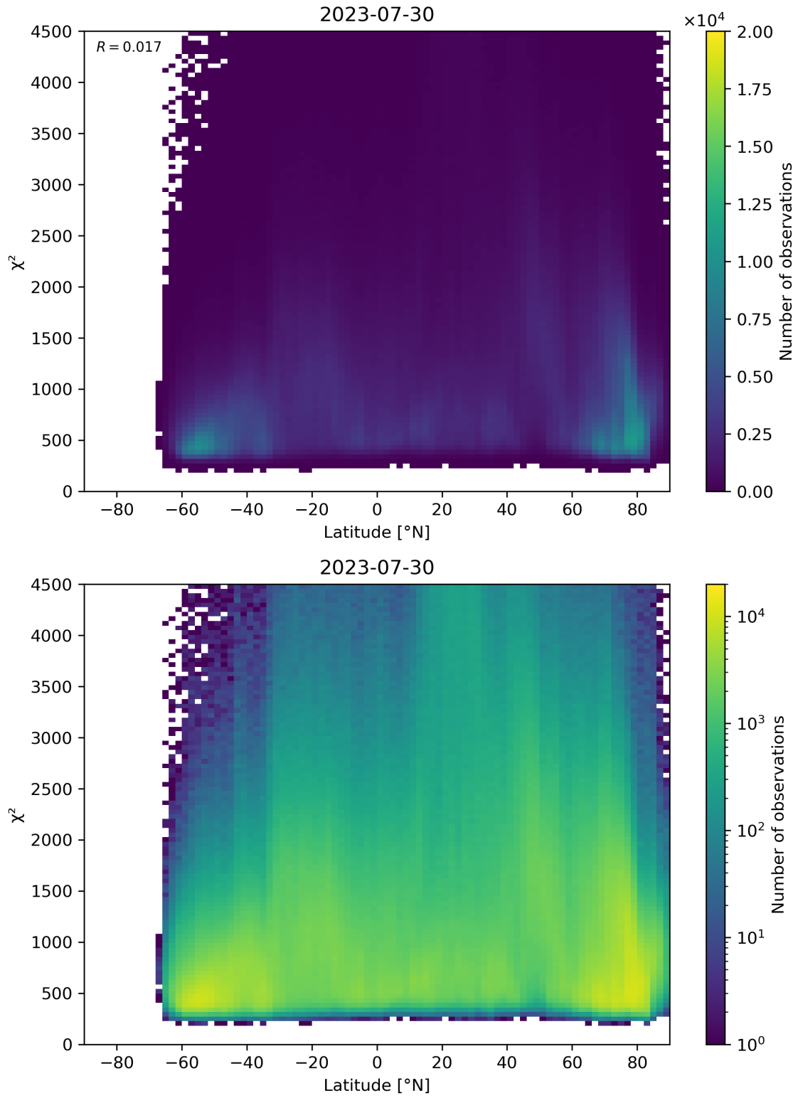
Figure 54: Scatter density plot of “Latitude” against “ \chi^2 ” for 2023-07-29 to 2023-07-31.
