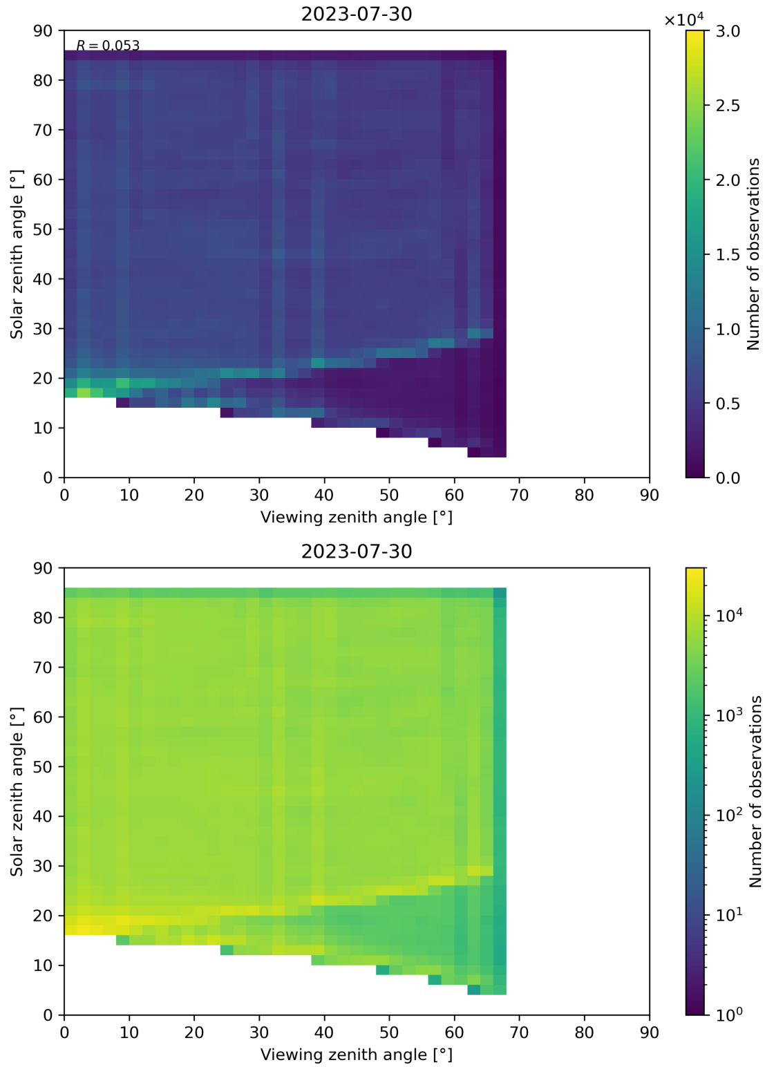
Figure 77: Scatter density plot of “Viewing zenith angle” against “Solar zenith angle” for 2023-07-29 to 2023-07-31.
