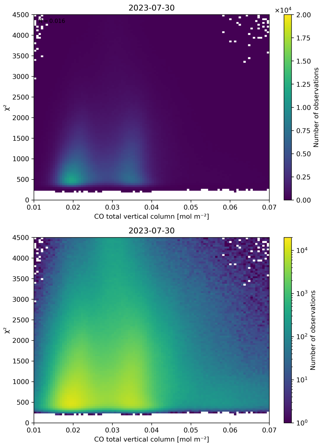
Figure 35: Scatter density plot of “CO total vertical column” against “ \chi^2 ” for 2023-07-29 to 2023-07-31.
