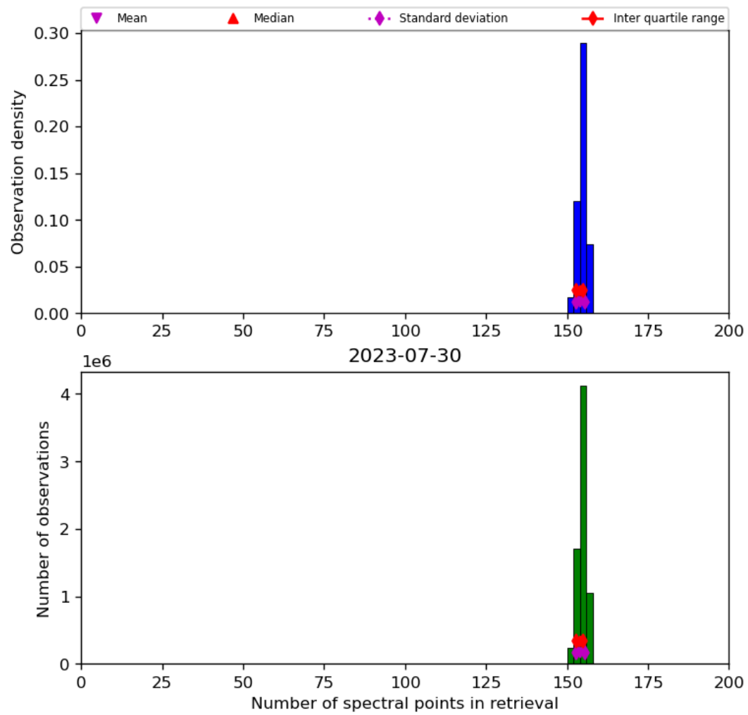
Figure 21: Histogram of “Number of spectral points in retrieval” for 2023-07-29 to 2023-07-31
