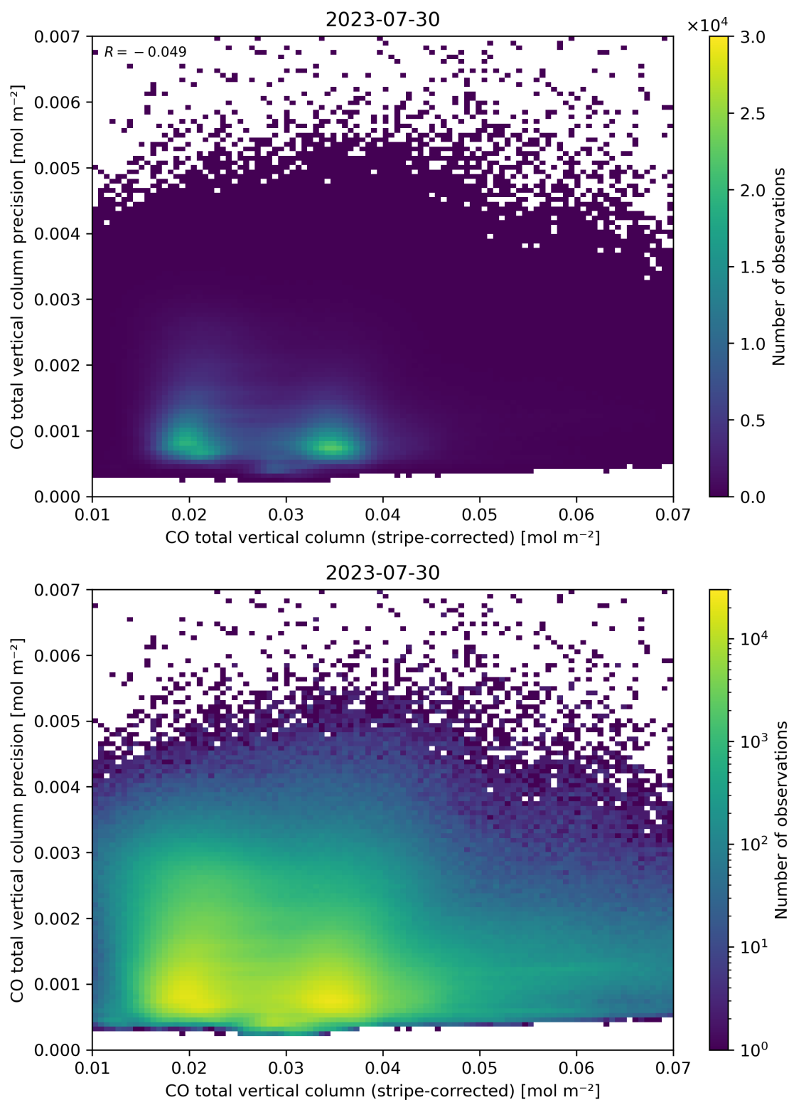
Figure 36: Scatter density plot of “CO total vertical column (stripe-corrected)” against “CO total vertical column precision” for 2023-07-29 to 2023-07-31.
