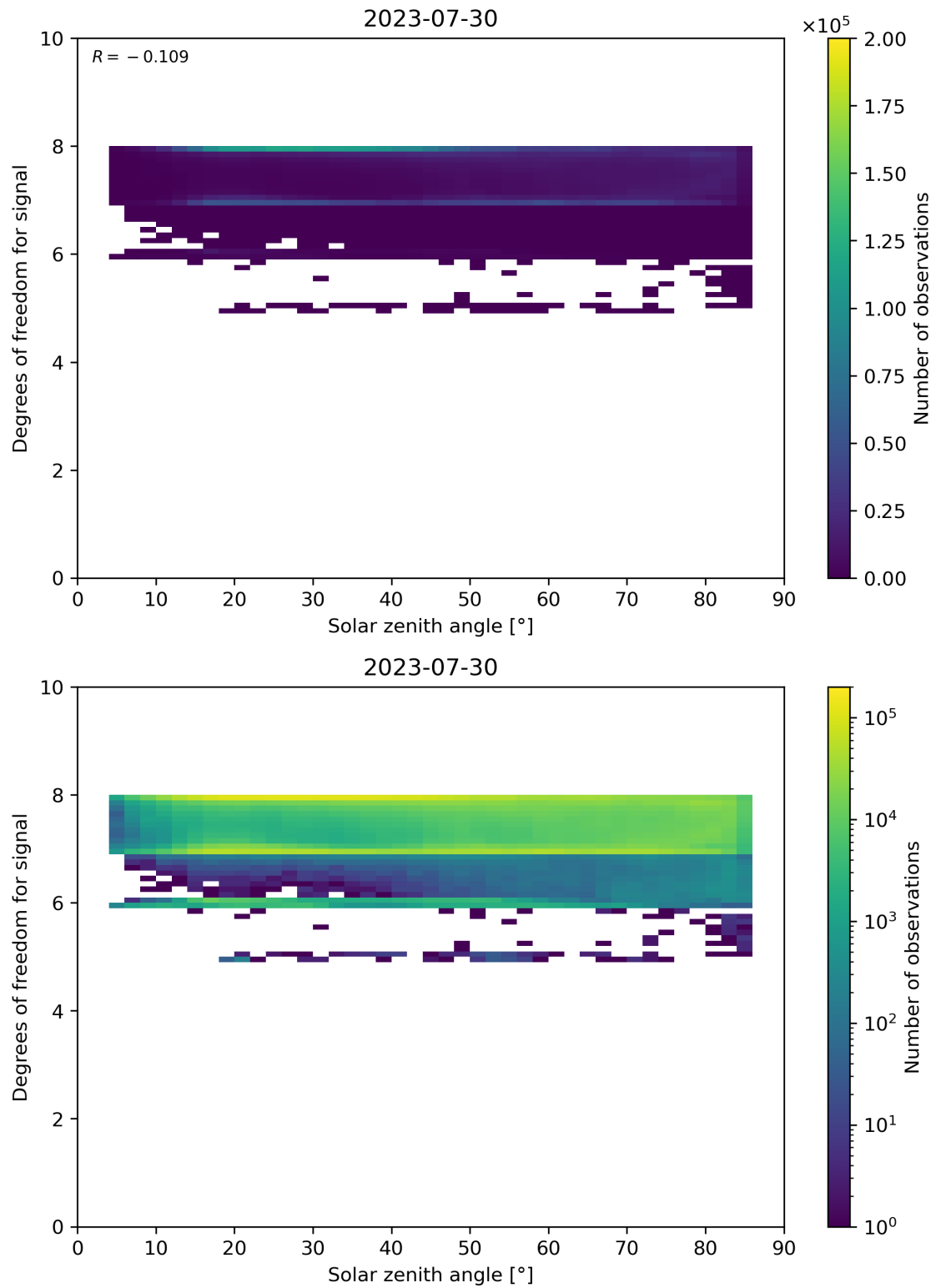
Figure 65: Scatter density plot of “Solar zenith angle” against “Degrees of freedom for signal” for 2023-07-29 to 2023-07-31.
