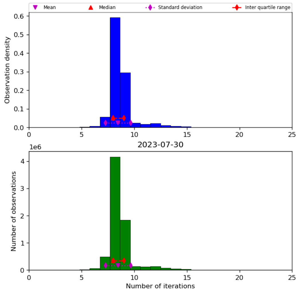
Figure 24: Histogram of “Number of iterations” for 2023-07-29 to 2023-07-31
