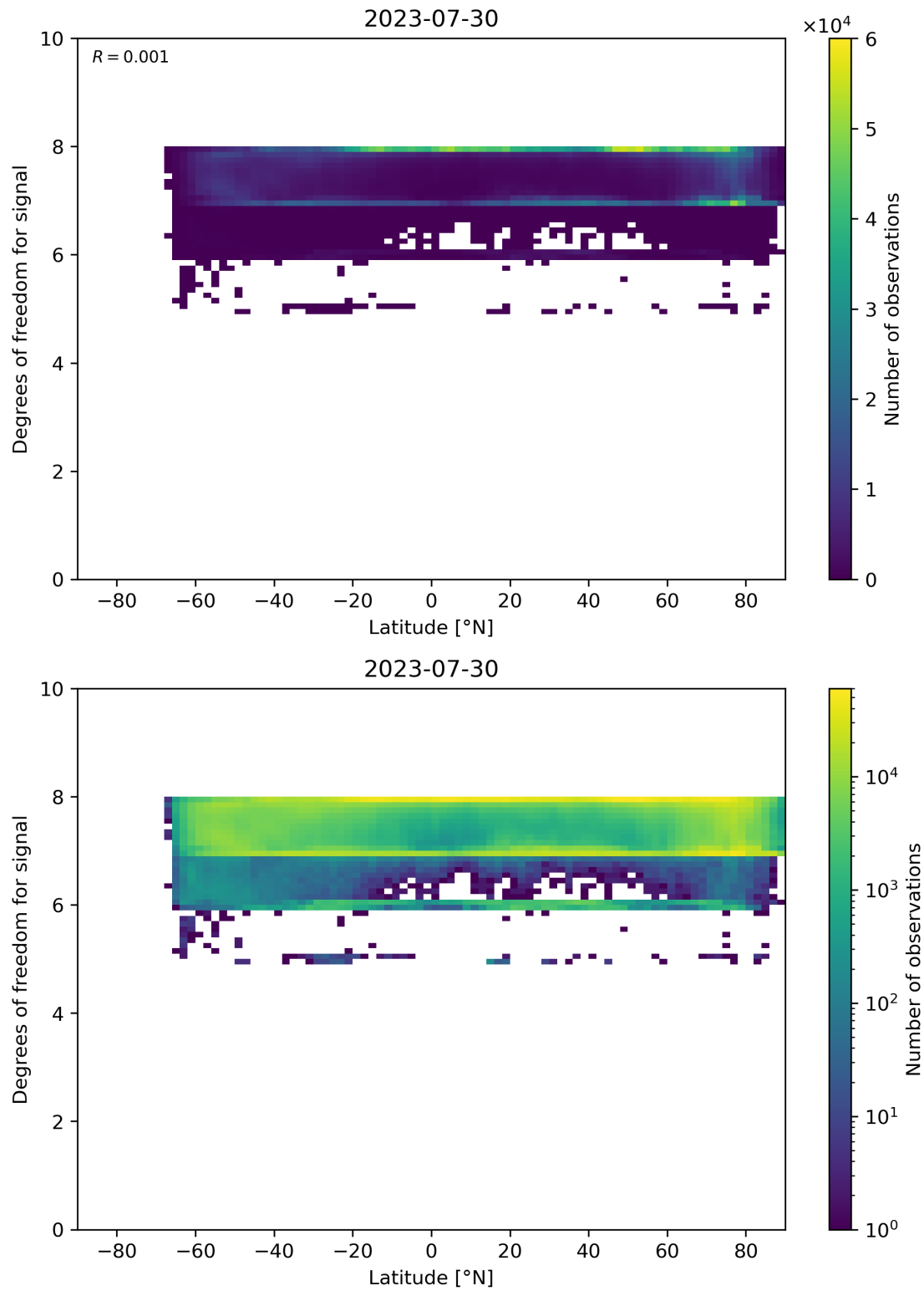
Figure 55: Scatter density plot of “Latitude” against “Degrees of freedom for signal” for 2023-07-29 to 2023-07-31.
