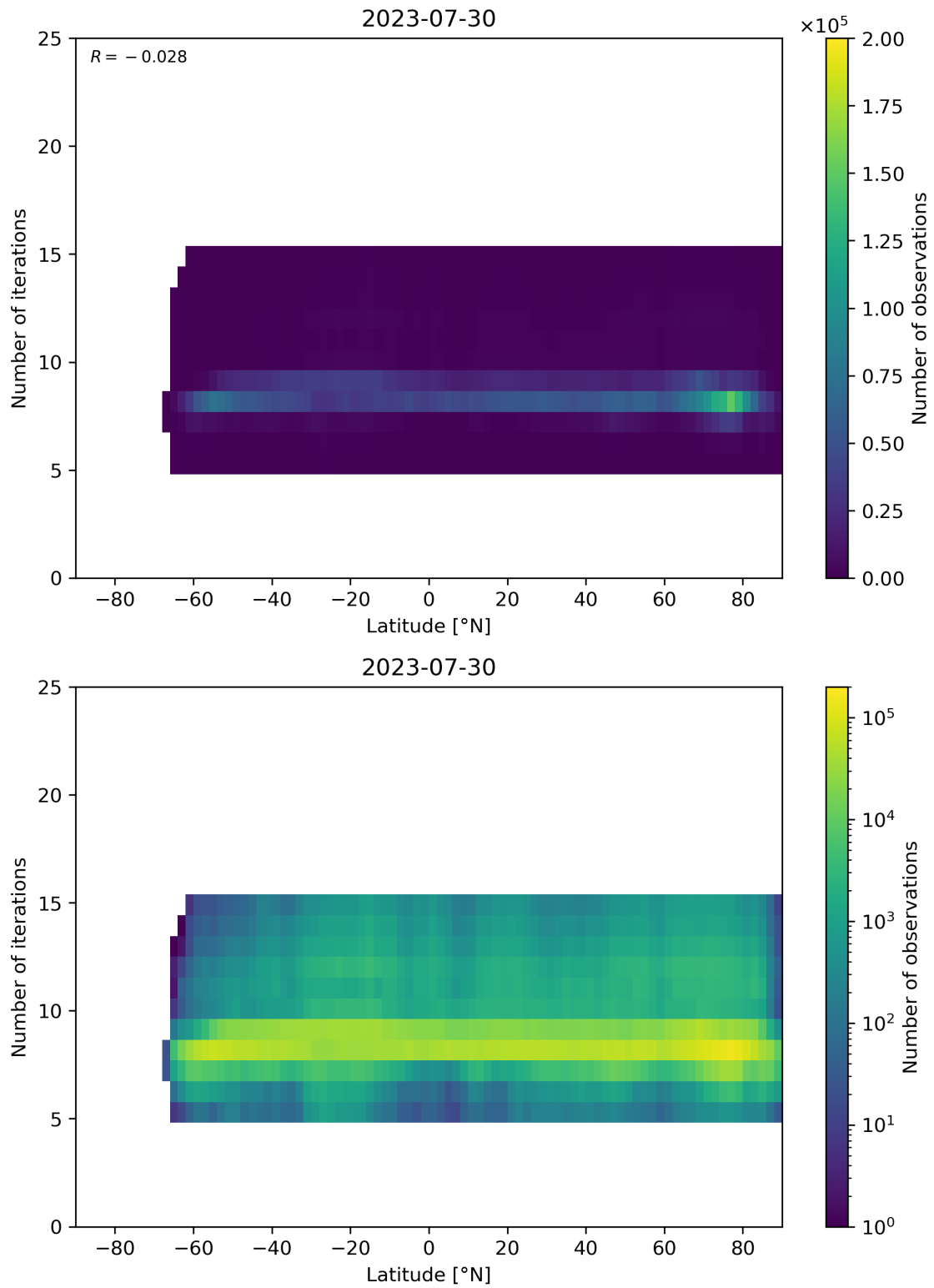
Figure 56: Scatter density plot of “Latitude” against “Number of iterations” for 2023-07-29 to 2023-07-31.
