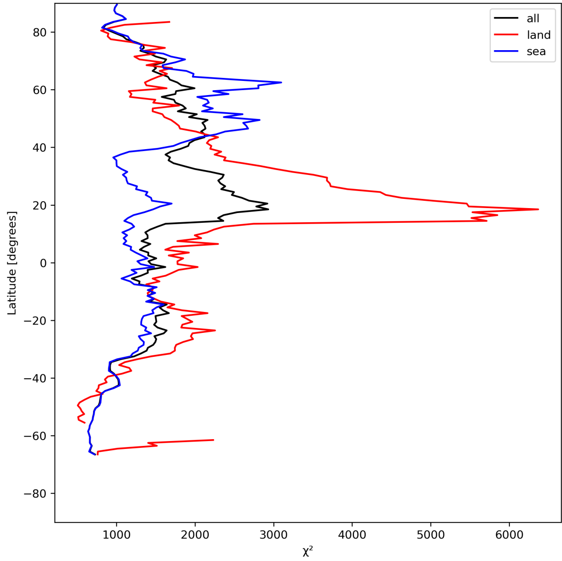
Figure 14: Zonal average of “ \chi^2 ” for 2023-07-29 to 2023-07-31.
