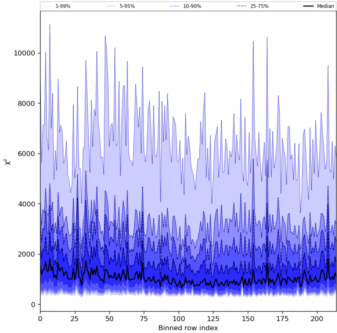
Figure 30: Along track statistics of “ \chi^2 ” for 2023-07-29 to 2023-07-31
