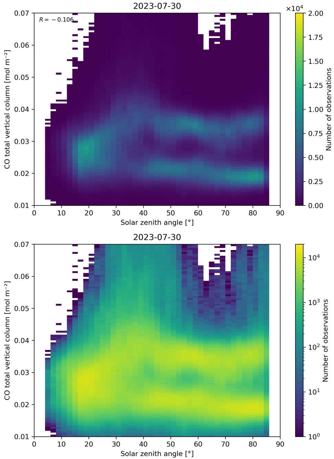
Figure 61: Scatter density plot of “Solar zenith angle” against “CO total vertical column” for 2023-07-29 to 2023-07-31.
