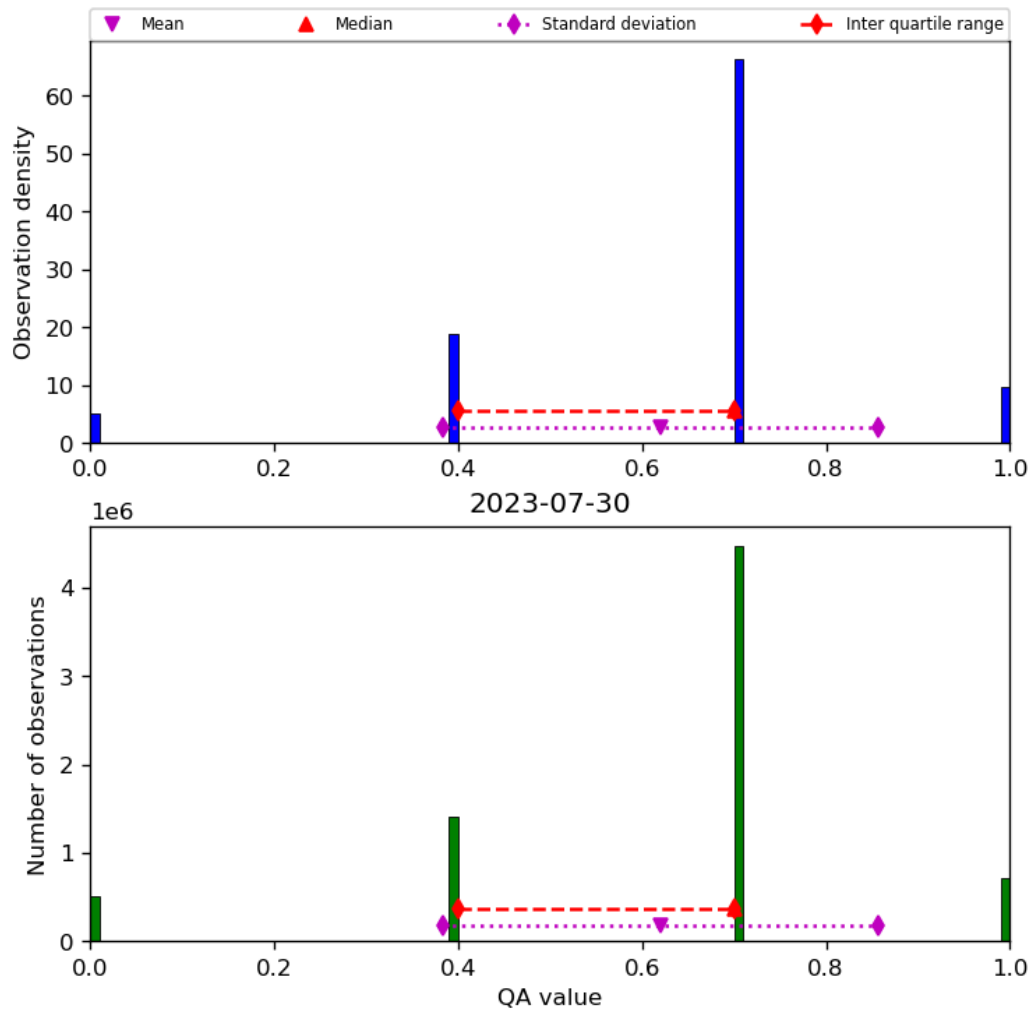
Figure 17: Histogram of “QA value” for 2023-07-29 to 2023-07-31
