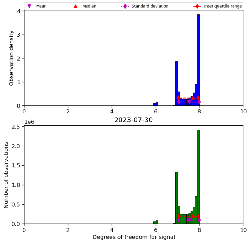
Figure 23: Histogram of “Degrees of freedom for signal” for 2023-07-29 to 2023-07-31
