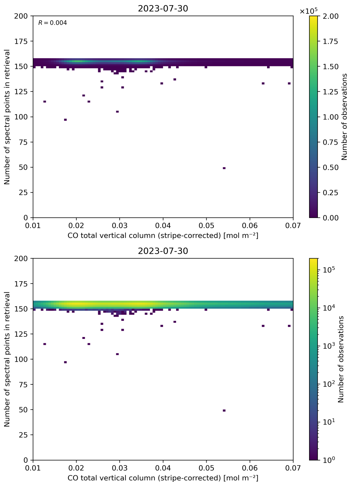
Figure 40: Scatter density plot of “CO total vertical column (stripe-corrected)” against “Number of spectral points in retrieval” for 2023-07-29 to 2023-07-31.
